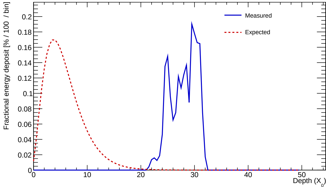
Cluster 430 E=3.409 GeV profileStart=23.50 X_0 \chi=0.5793
