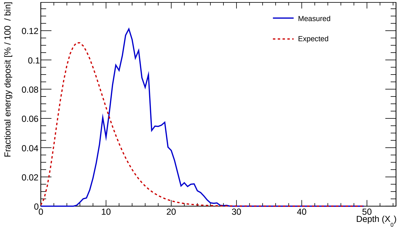
Cluster 568 E=25.008 GeV profileStart=7.00 X_0 \chi=0.1356
