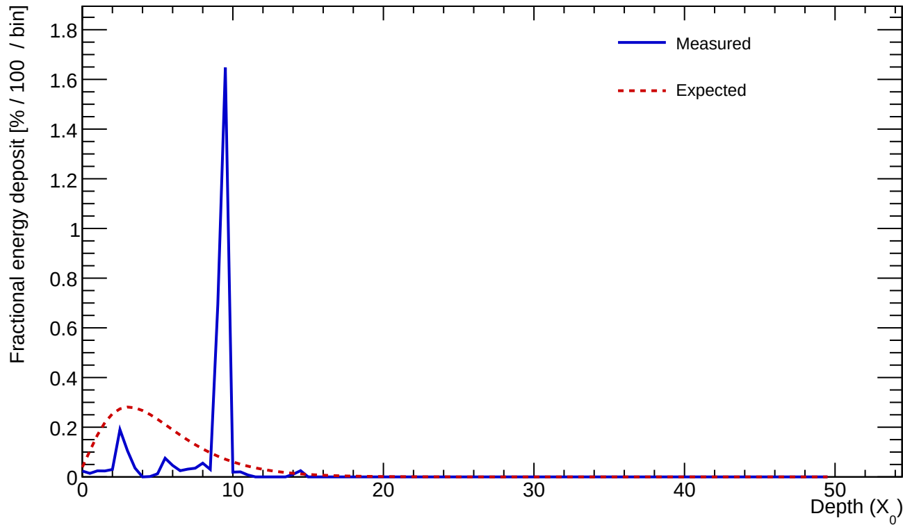
Cluster 618 E=1.730 GeV profileStart=1.00 X_0 \chi=1.3797
