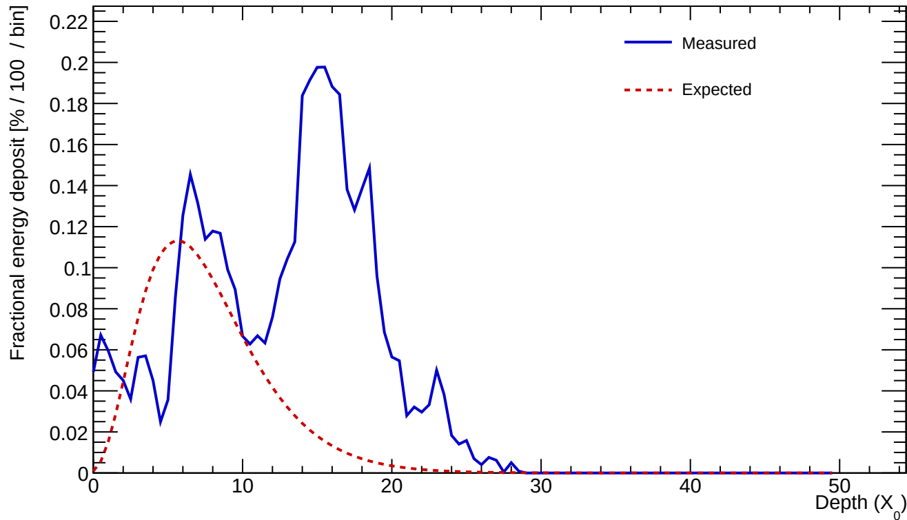
Cluster 134 E=22.439 GeV profileStart=7.00 X_0 \chi=0.6244
