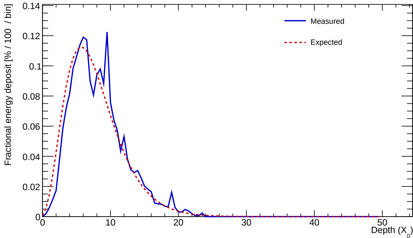
Cluster 294 E=23.998 GeV \text{profileStart}=0.50 X_0 \chi=0.1077
