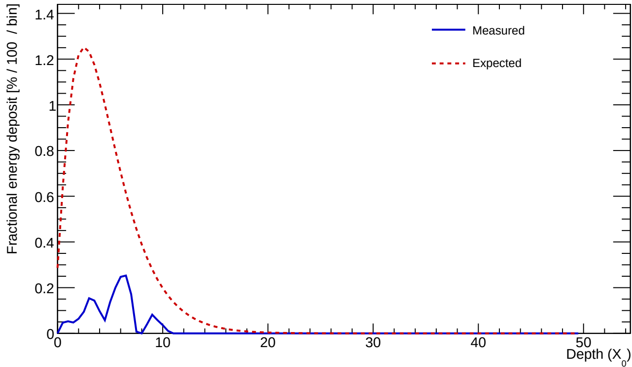
Cluster 651 E=1.015 GeV profileStart=1.50 X_0 \chi=0.4753
