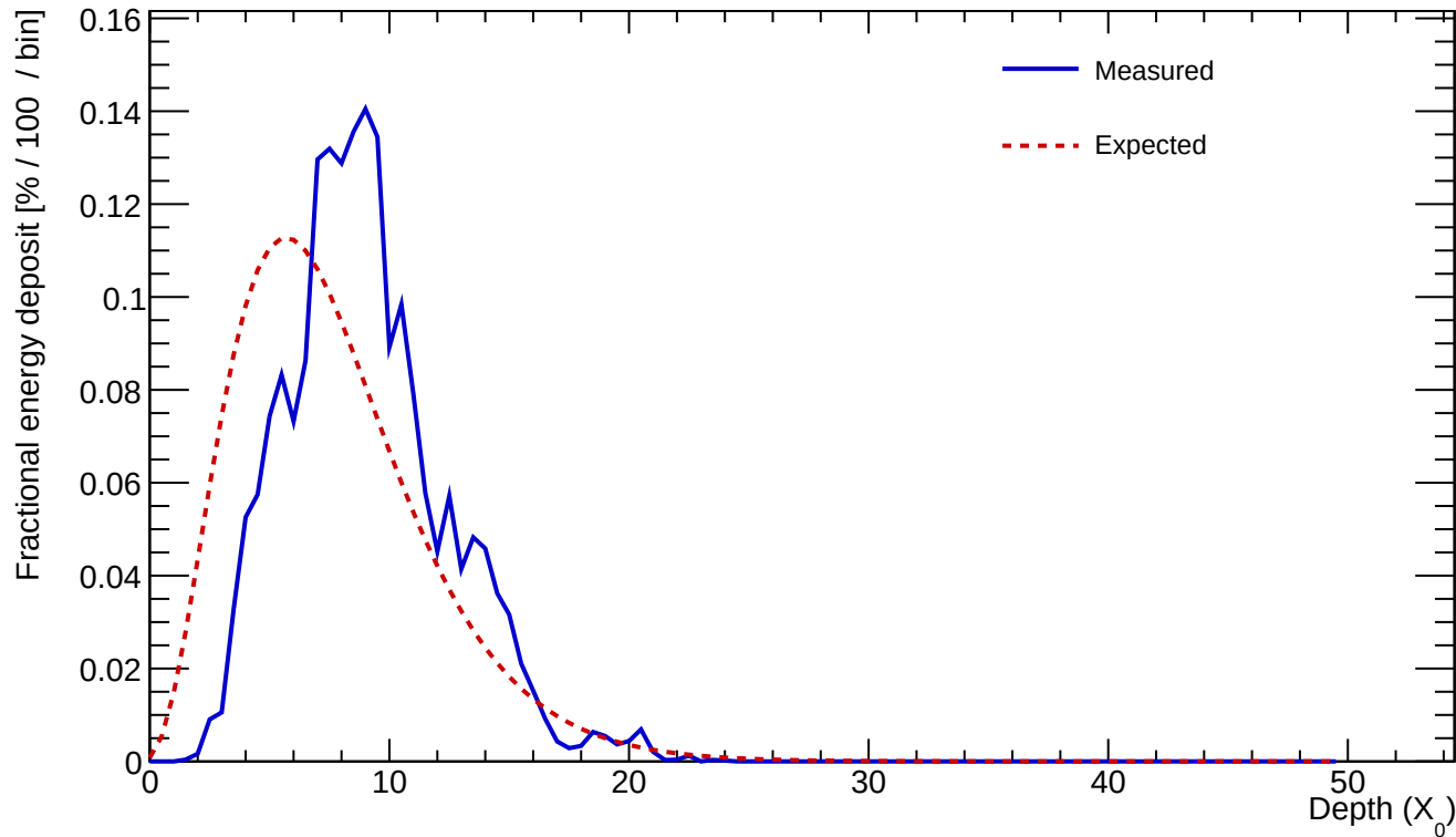
Cluster 479 E=23.279 GeV profileStart=2.00 X_0 \chi=0.1981
