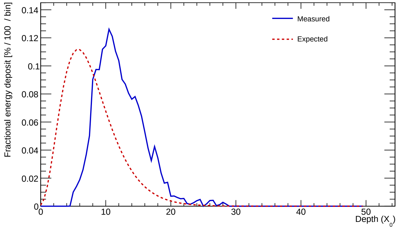
Cluster 91 E=25.344 GeV profileStart=4.50 X_0 \chi=0.1308
