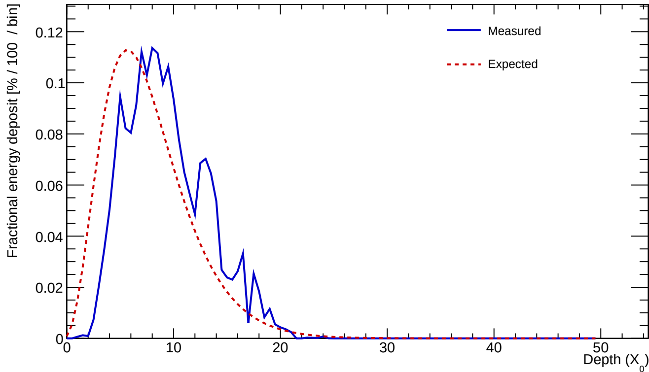
Cluster 404 E=23.140 GeV profileStart=2.00 X_0 \chi=0.1643
