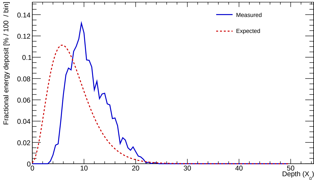
Cluster 654 E=25.919 GeV profileStart=3.50 X_0 \chi=0.1092
