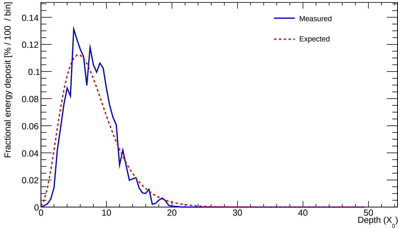
Cluster 528 E=24.228 GeV profileStart=0.50 X_0 \chi=0.1591
