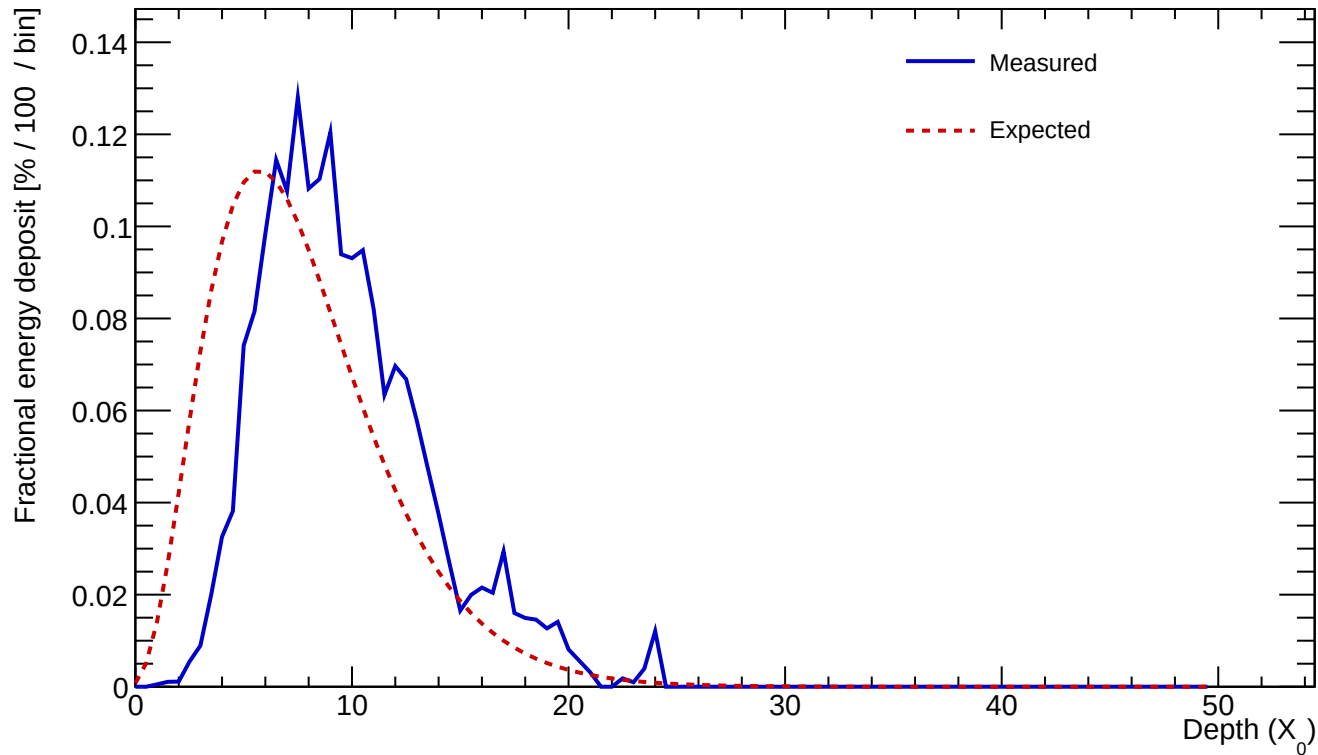
Cluster 155 E=24.618 GeV profileStart=2.00 X_0 \chi=0.1119
