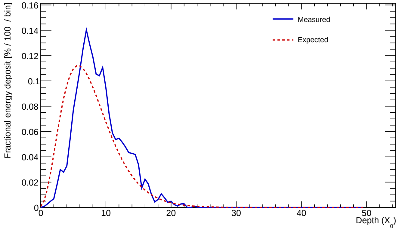
Cluster 473 E=24.683 GeV profileStart=1.50 X_0 \chi=0.1549
