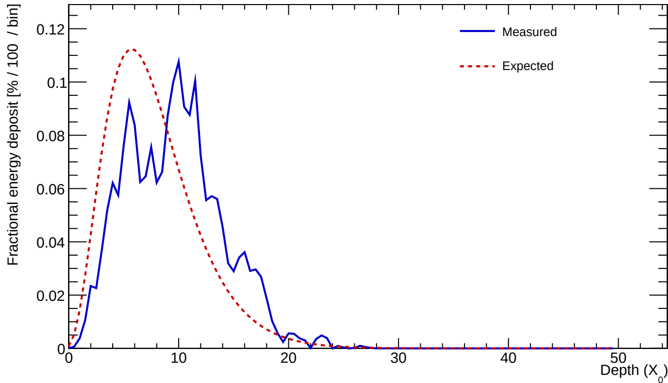
Cluster 237 E=24.021 GeV profileStart=2.00 X_0 \chi=0.2718
