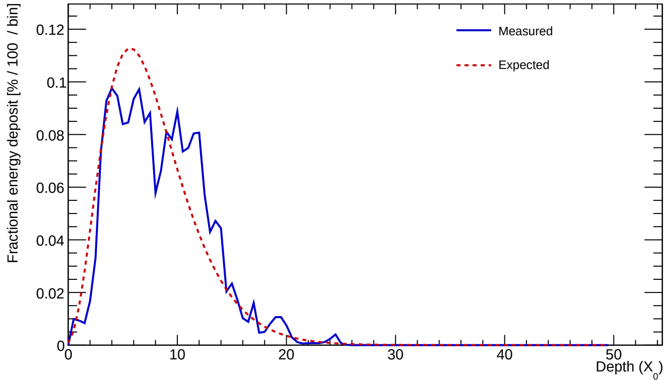
Cluster 195 E=23.247 GeV profileStart=0.50 X_0 \chi=0.2433
