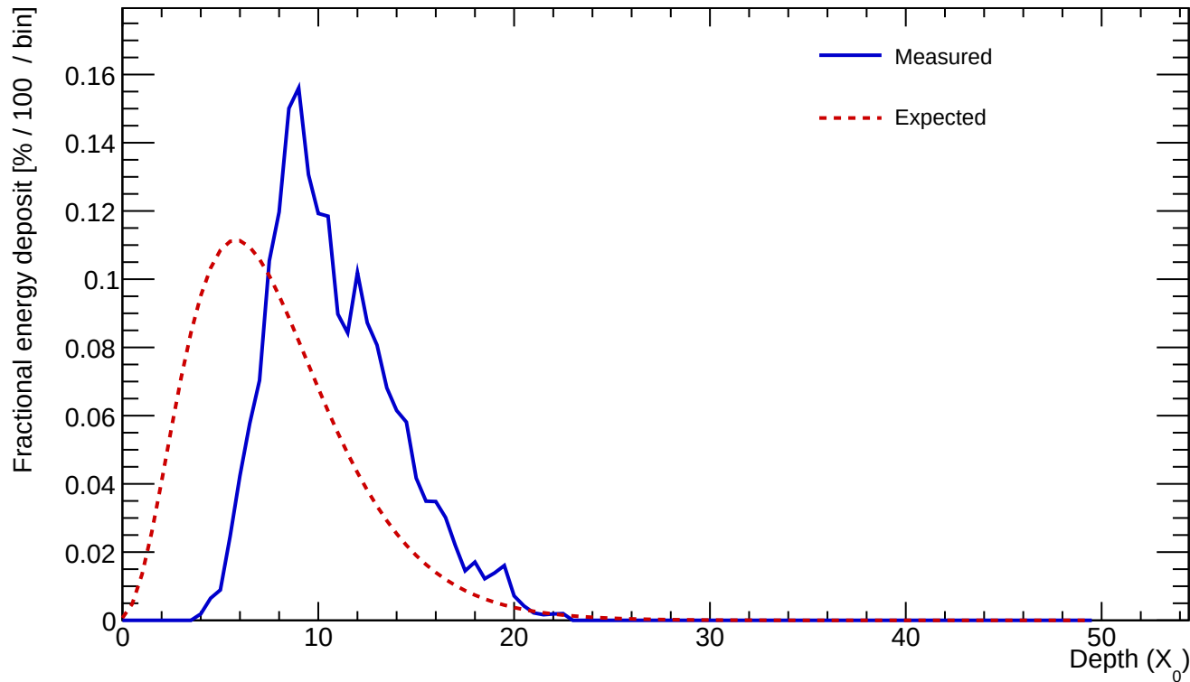
Cluster 491 E=26.140 GeV profileStart=4.00 X_0 \chi=0.1898
