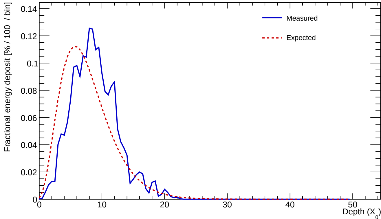
Cluster 662 E=24.360 GeV profileStart=1.50 X_0 \chi=0.1669
