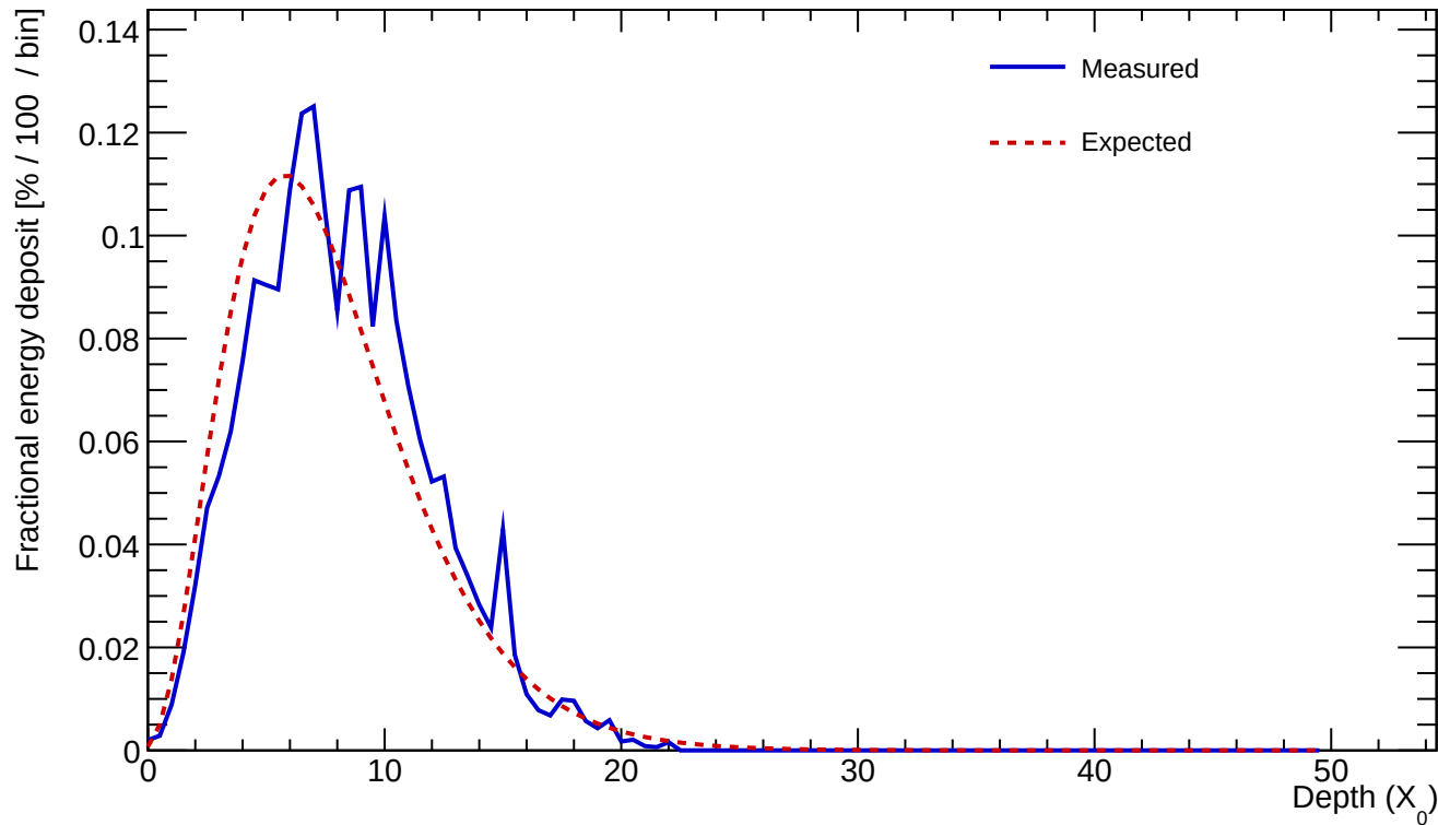
Cluster 501 E=25.345 GeV profileStart=0.50 X_0 \chi=0.1436
