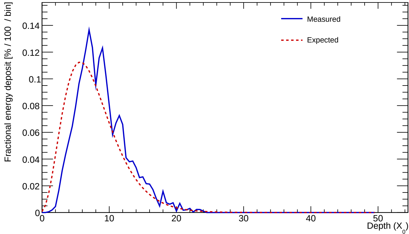
Cluster 44 E=23.738 GeV profileStart=1.50 X_0 \chi=0.1323
