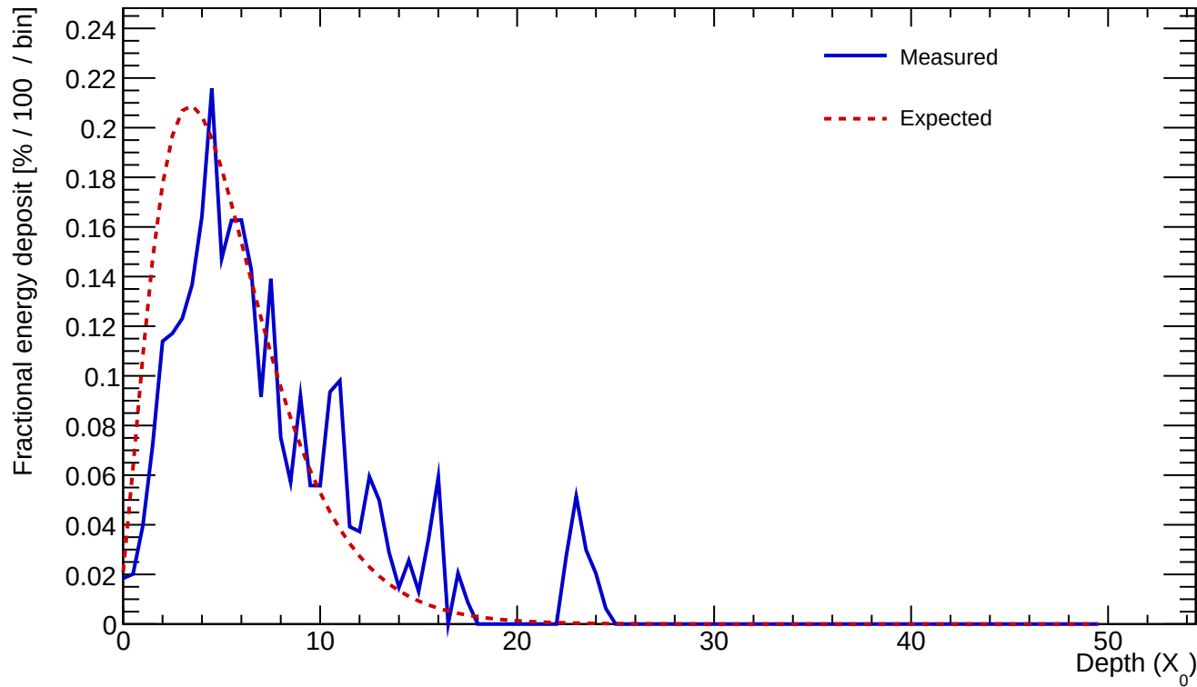
Cluster 504 E=2.378 GeV profileStart=1.00 X_0 \chi=0.3260
