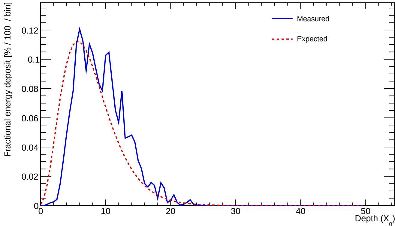
Cluster 641 E=24.281 GeV profileStart=1.50 X_0 \chi=0.1613
