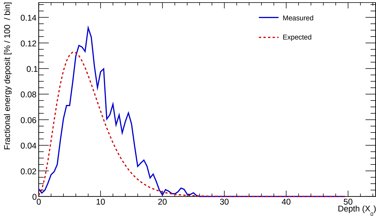
Cluster 621 E=23.091 GeV profileStart=2.00 X_0 \chi=0.1673
