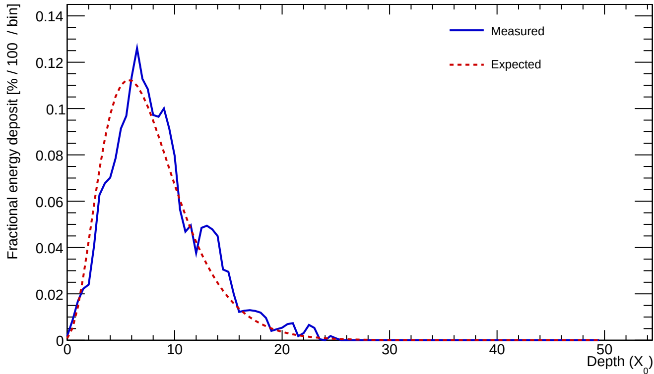
Cluster 169 E=23.973 GeV profileStart=0.50 X_0 \chi=0.1452
