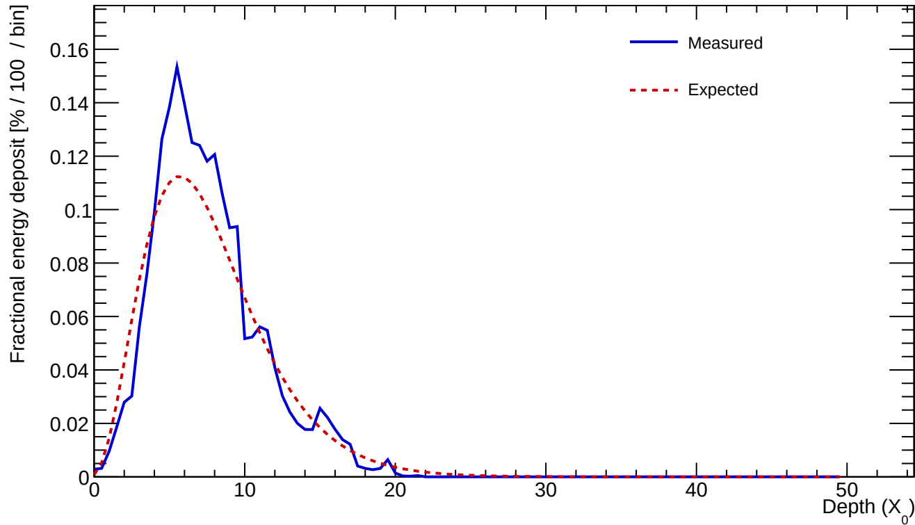
Cluster 555 E=23.855 GeV profileStart=0.50 X_0 \chi=0.1741
