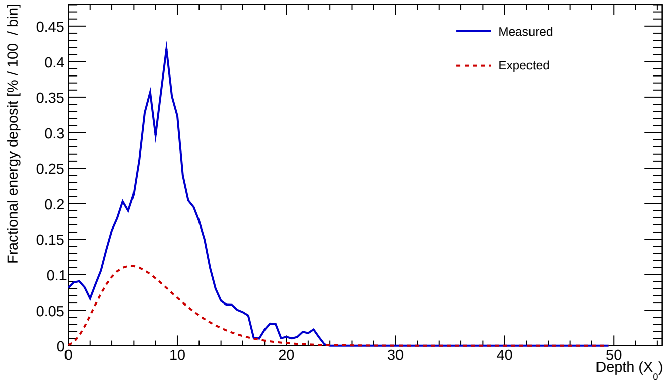
Cluster 182 E=24.354 GeV profileStart=1.50 X_0 \chi=0.2672
