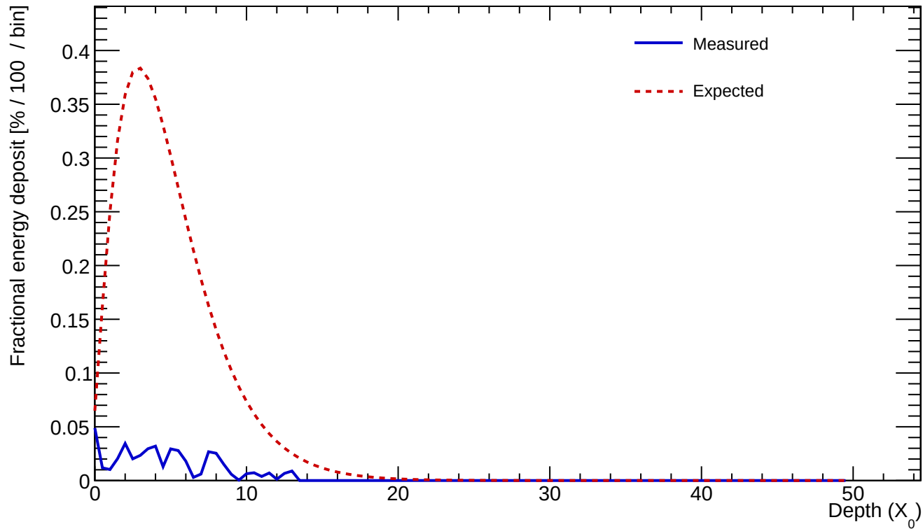
Cluster 284 E=1.407 GeV profileStart=0.50 X_0 \chi=0.4414
