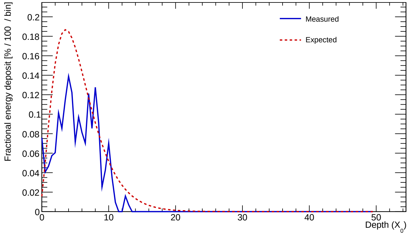
Cluster 338 E=2.837 GeV profileStart=0.50 X_0 \chi=0.3117
