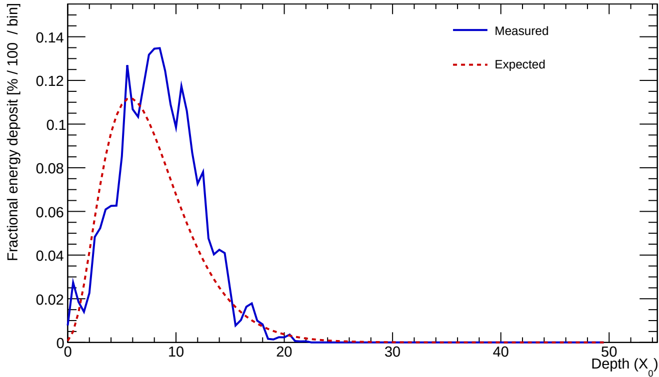
Cluster 48 E=25.350 GeV profileStart=1.50 X_0 \chi=0.2016
