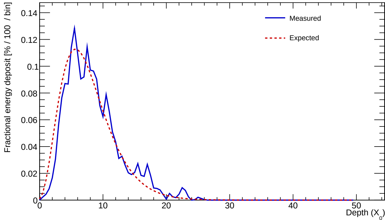
Cluster 239 E=23.217 GeV profileStart=0.50 X_0 \chi=0.1413
