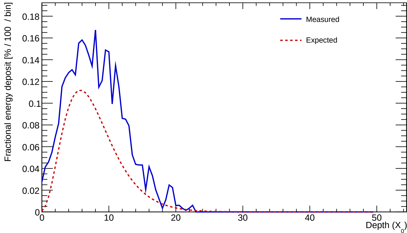
Cluster 276 E=24.984 GeV profileStart=0.50 X_0 \chi=0.2275
