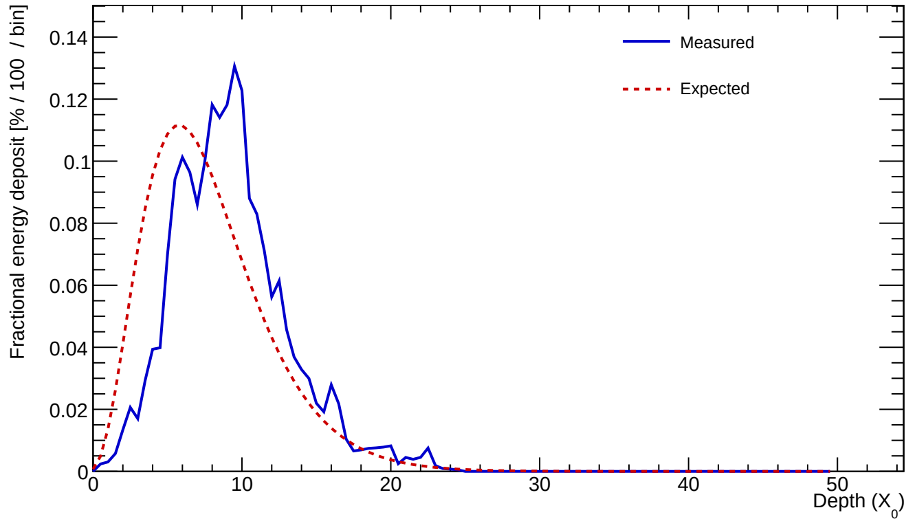
Cluster 235 E=25.754 GeV profileStart=2.00 X_0 \chi=0.1658
