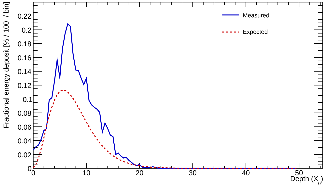
Cluster 4 E=22.907 GeV profileStart=0.50 X_0 \chi=0.1476
