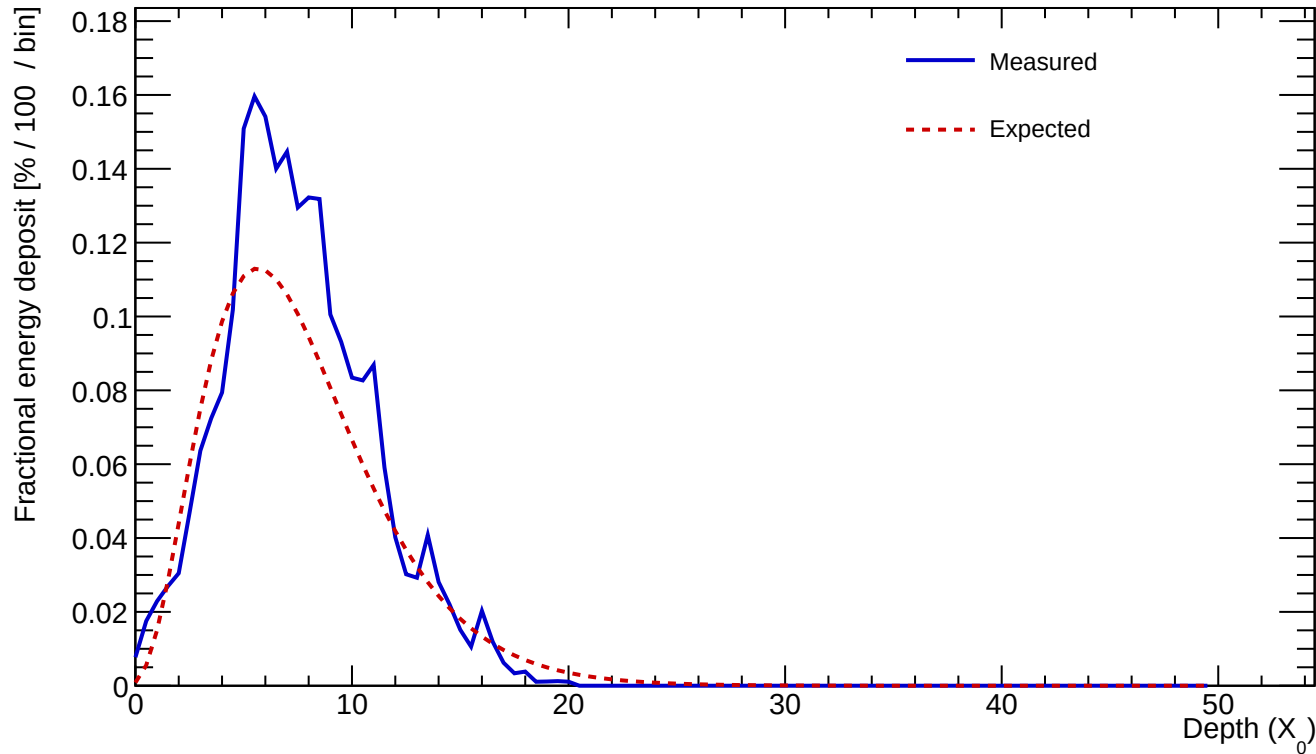
Cluster 678 E=22.818 GeV profileStart=0.50 X_0 \chi=0.1752
