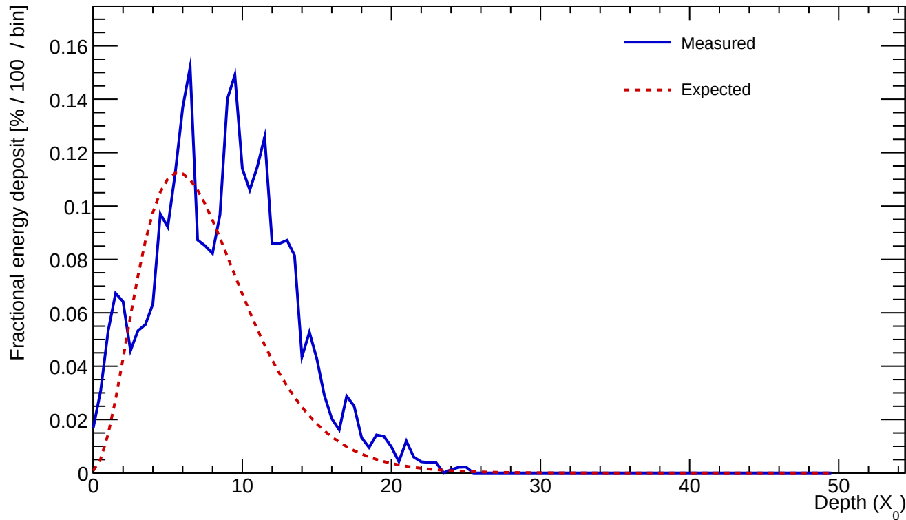
Cluster 328 E=23.831 GeV profileStart=2.00 X_0 \chi=0.2942
