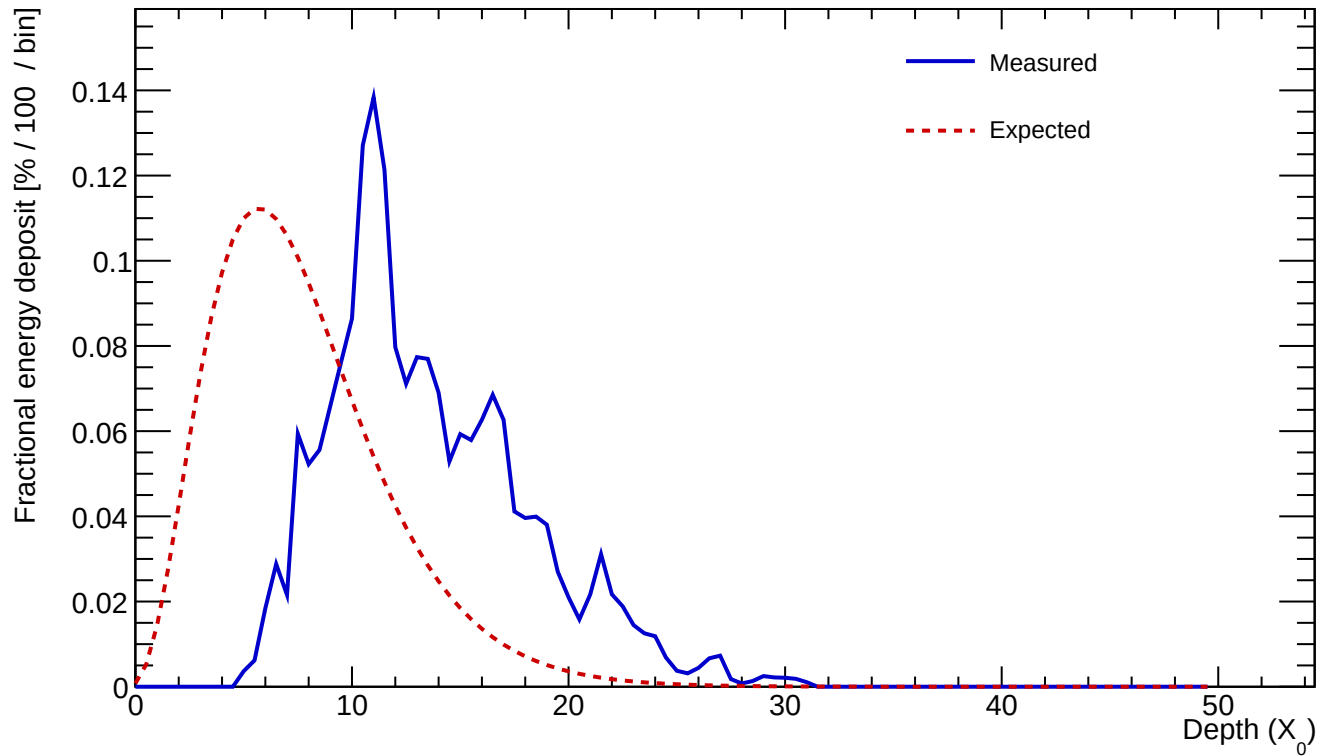
Cluster 478 E=24.089 GeV profileStart=5.50 X_0 \chi=0.2507
