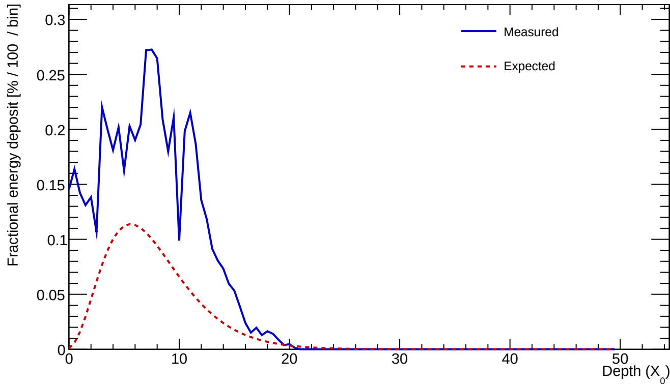
Cluster 505 E=21.484 GeV profileStart=0.50 X_0 \chi=0.3058
