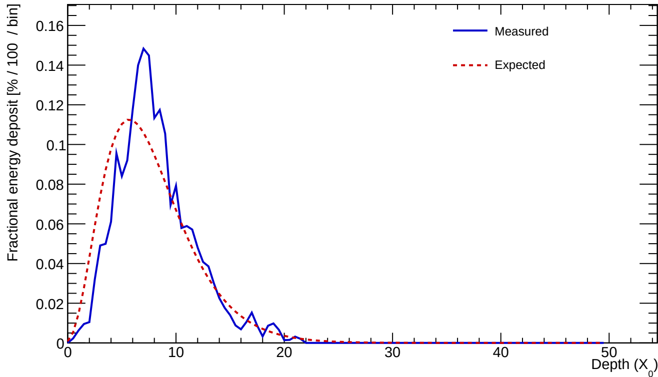
Cluster 497 E=23.630 GeV profileStart=1.00 X_0 \chi=0.1875
