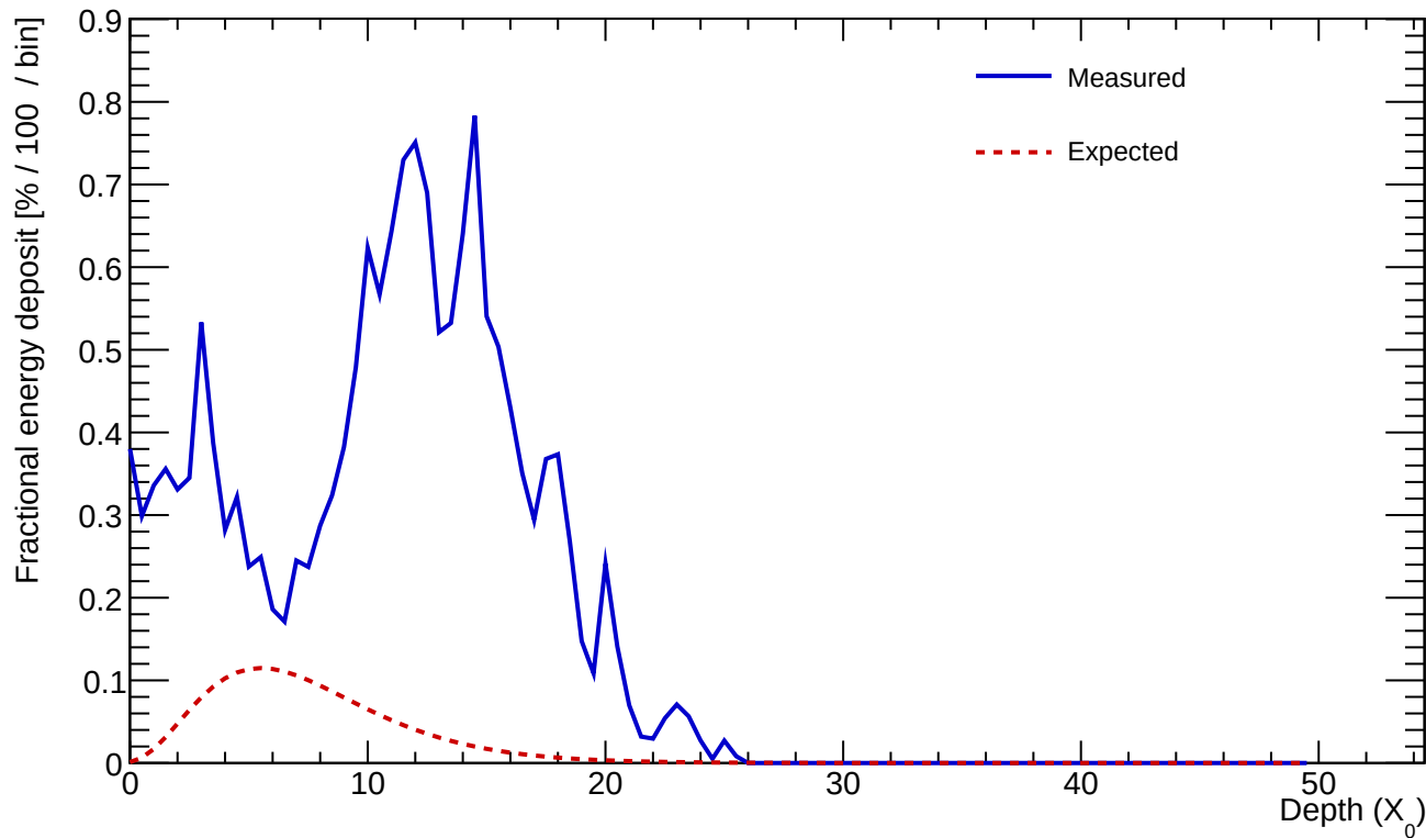
Cluster 125 E=19.683 GeV profileStart=5.50 X_0 \chi=0.5264
