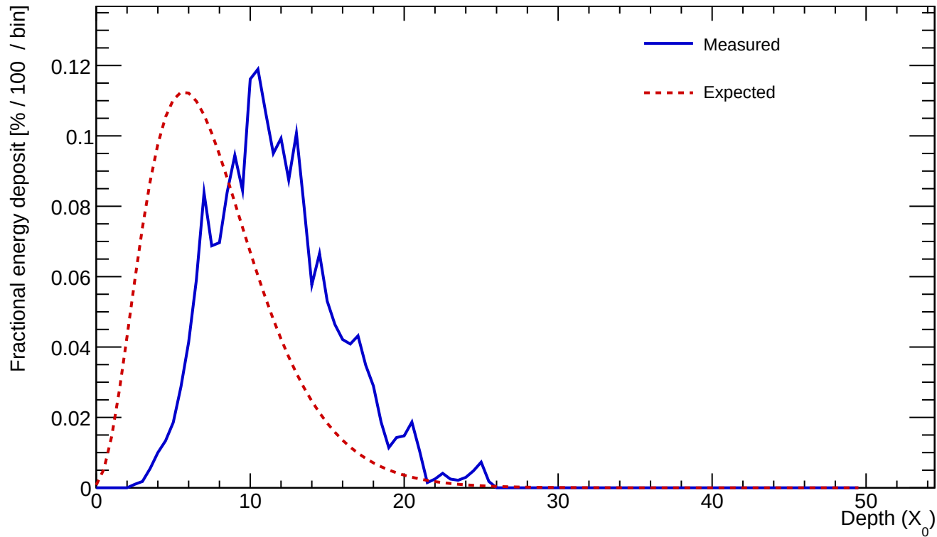
Cluster 266 E=23.720 GeV profileStart=4.00 X_0 \chi=0.1476
