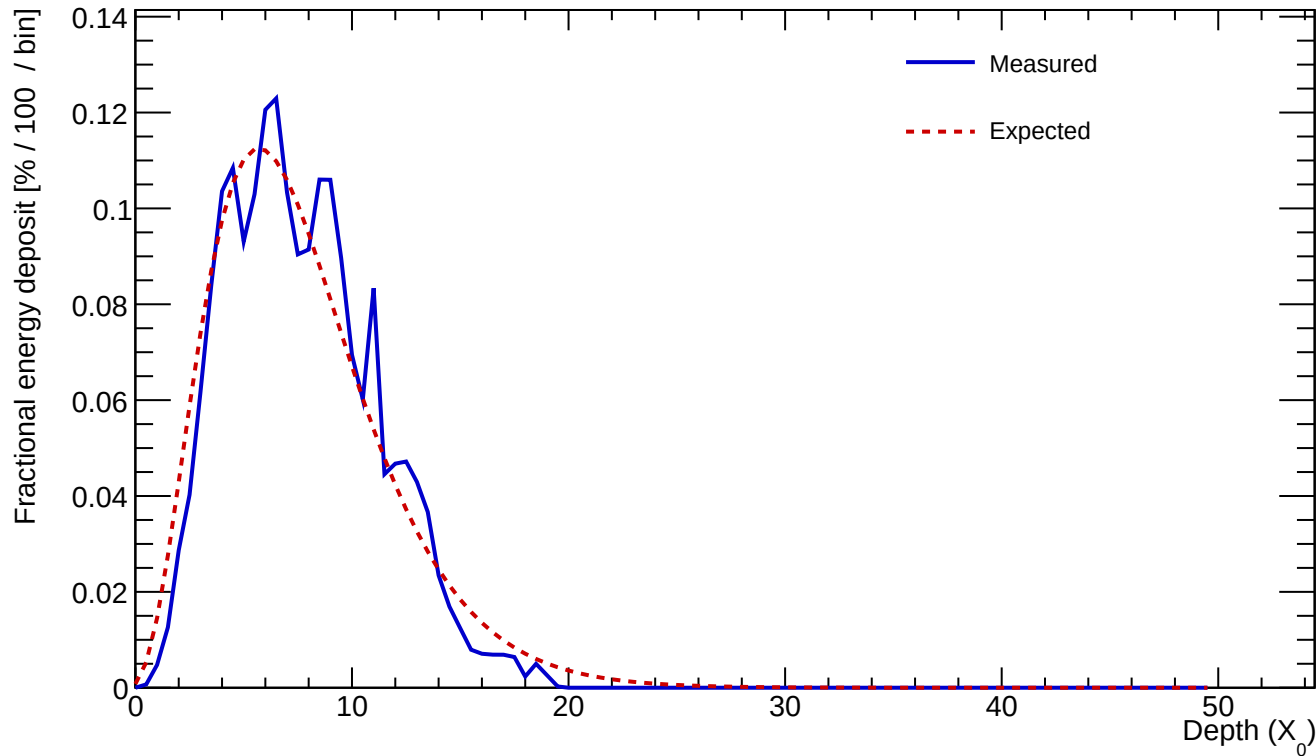
Cluster 287 E=23.825 GeV profileStart=0.50 X_0 \chi=0.1406
