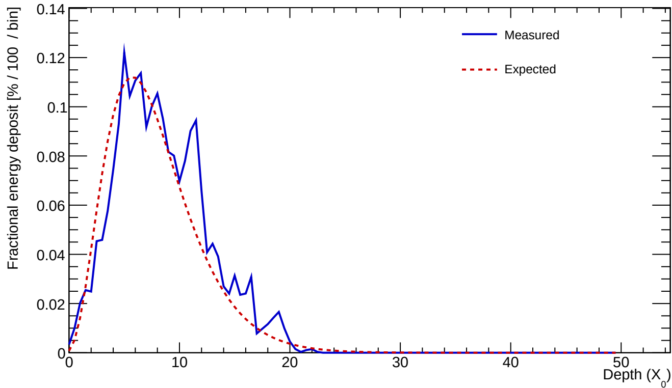
Cluster 193 E=24.650 GeV profileStart=1.00 X_0 \chi=0.1779
