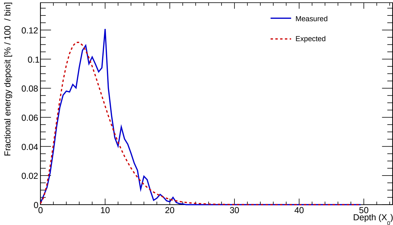
Cluster 622 E=25.441 GeV profileStart=0.50 X_0 \chi=0.1636
