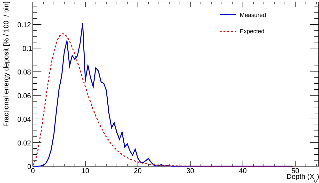
Cluster 222 E=24.286 GeV profileStart=2.50 X_0 \chi=0.1580
