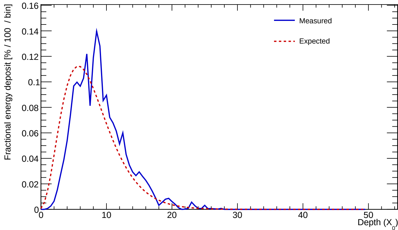
Cluster 210 E=24.203 GeV profileStart=1.50 X_0 \chi=0.1360
