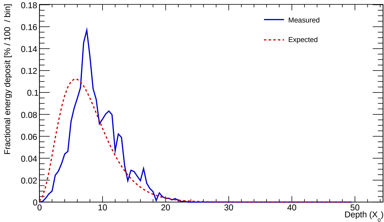
Cluster 283 E=24.171 GeV profileStart=1.50 X_0 \chi=0.1894
