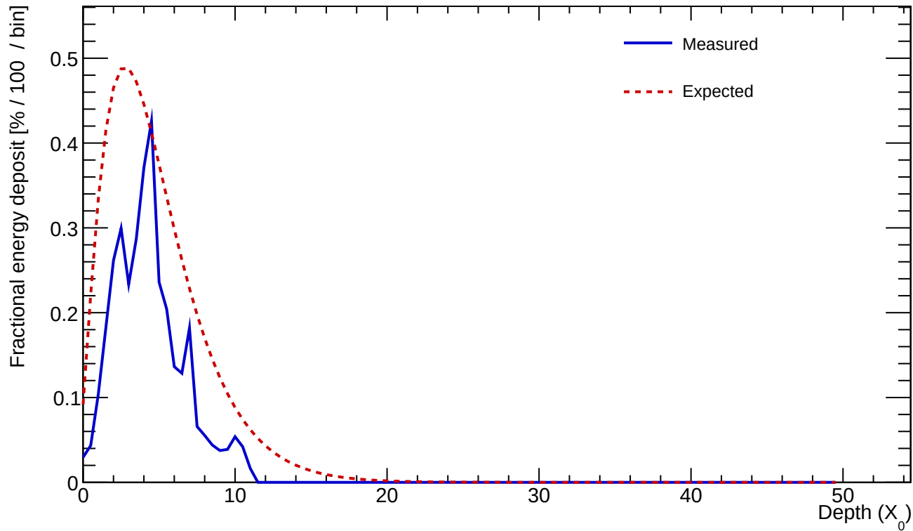
Cluster 390 E=1.261 GeV profileStart=0.50 X_0 \chi=0.2519
