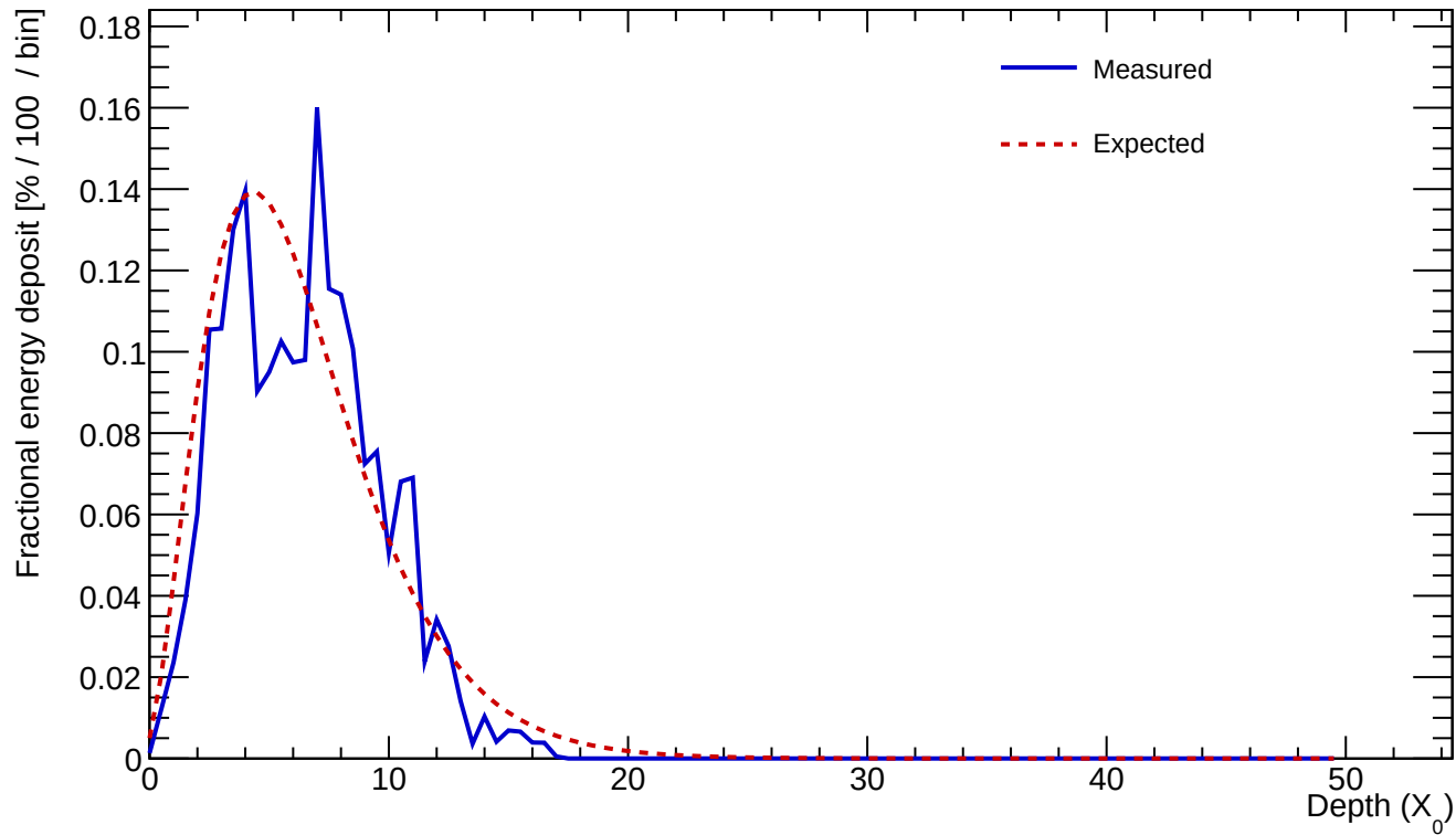
Cluster 20 E=6.160 GeV profileStart=0.50 X_0 \chi=0.2246
