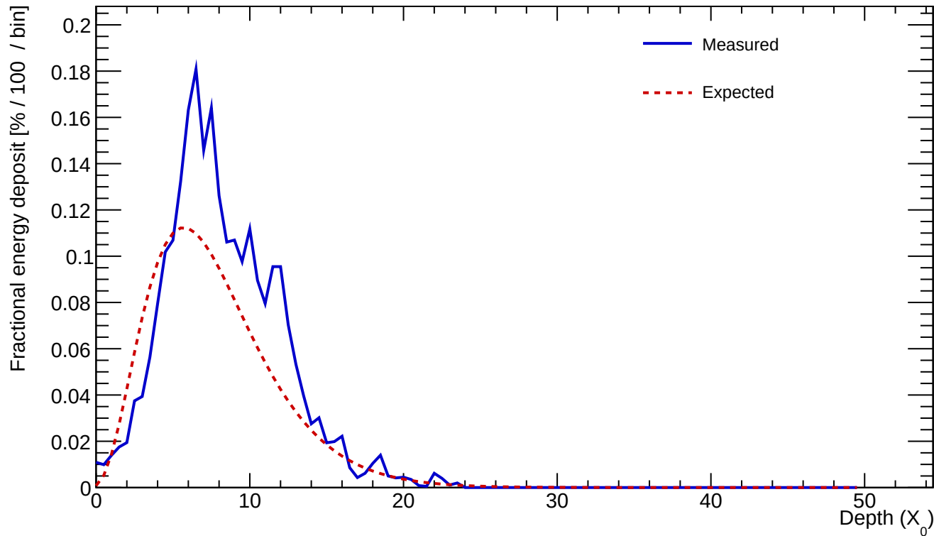
Cluster 278 E=24.094 GeV profileStart=1.00 X_0 \chi=0.1753
