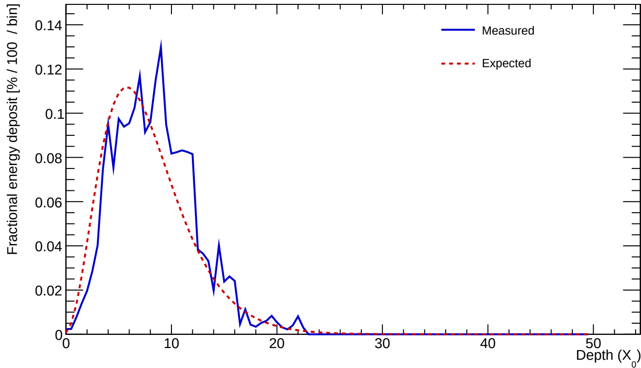
Cluster 526 E=25.339 GeV profileStart=1.00 X_0 \chi=0.1798
