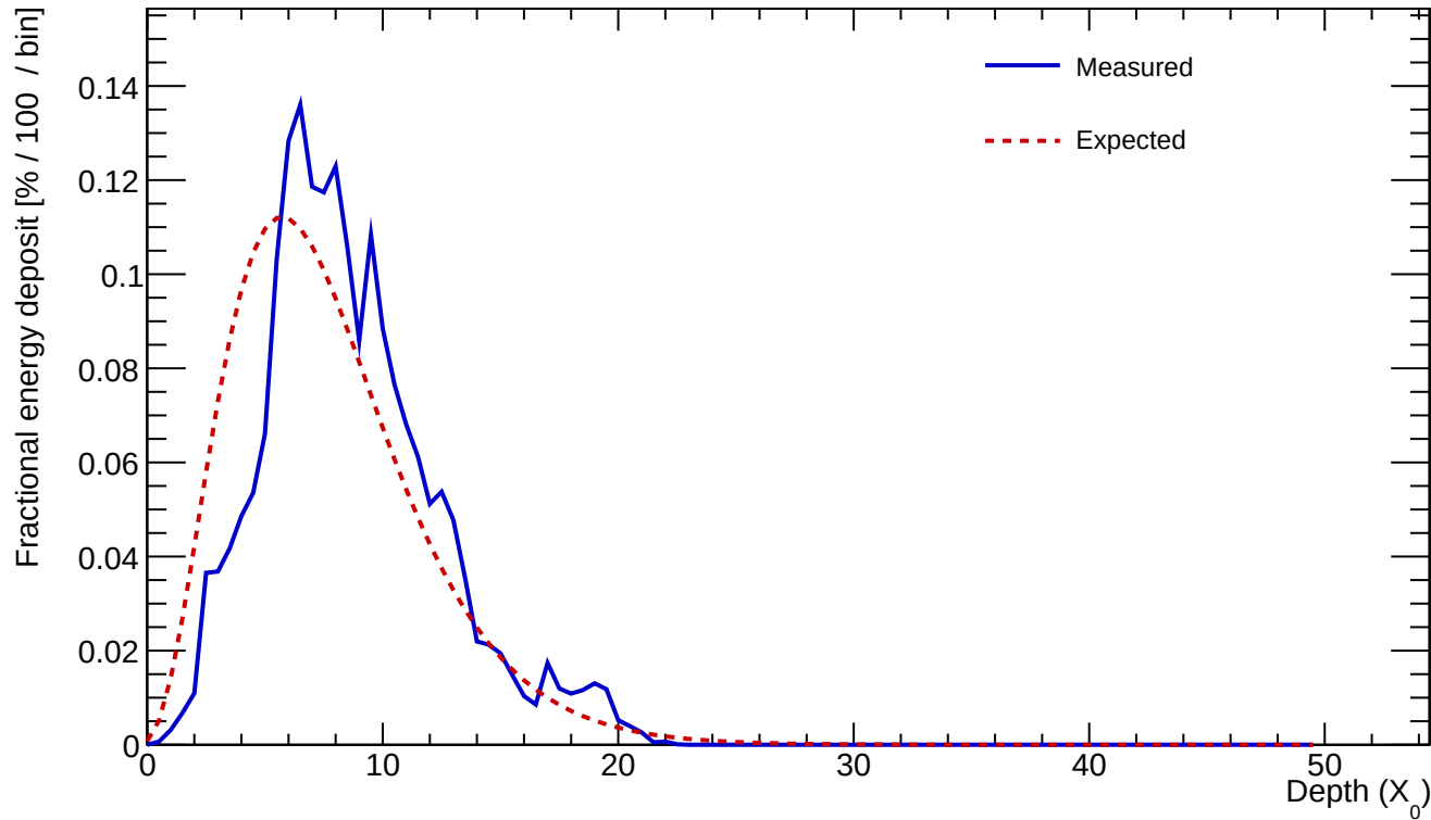
Cluster 384 E=24.547 GeV profileStart=1.50 X_0 \chi=0.1686
