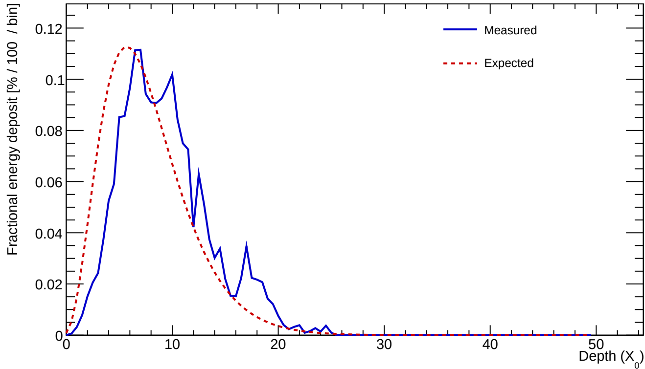
Cluster 14 E=23.453 GeV profileStart=1.50 X_0 \chi=0.1516
