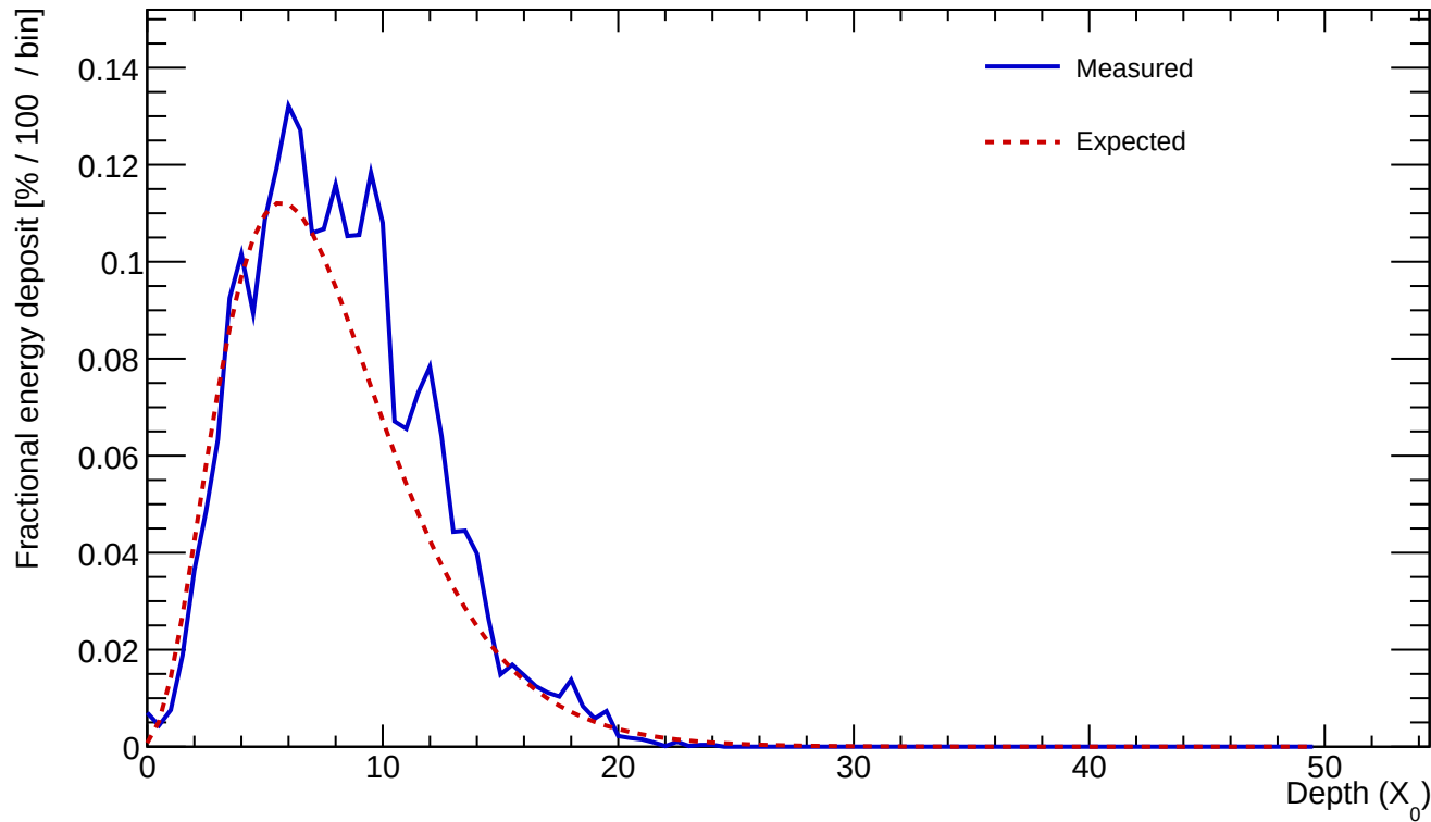
Cluster 39 E=24.350 GeV profileStart=0.50 X_0 \chi=0.1268
