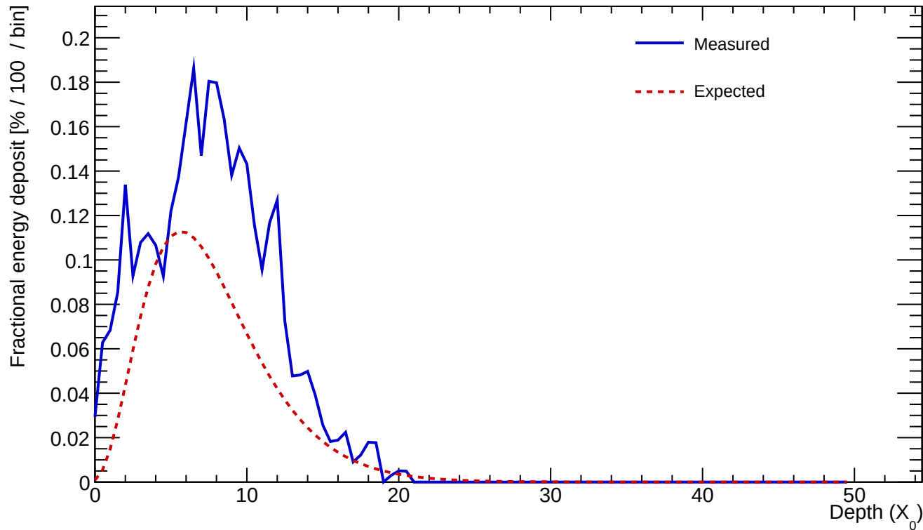
Cluster 487 E=23.232 GeV profileStart=0.50 X_0 \chi=0.2510
