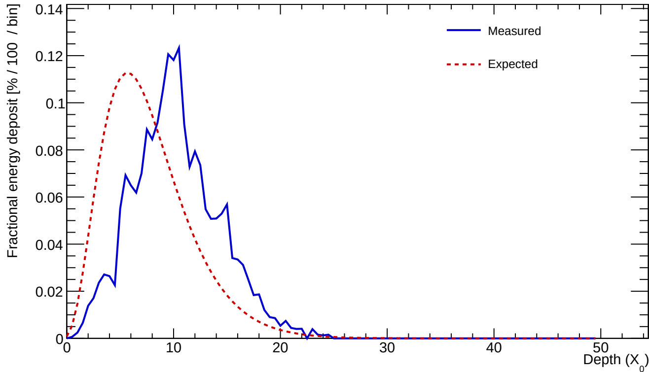
Cluster 240 E=23.379 GeV profileStart=3.00 X_0 \chi=0.1974
