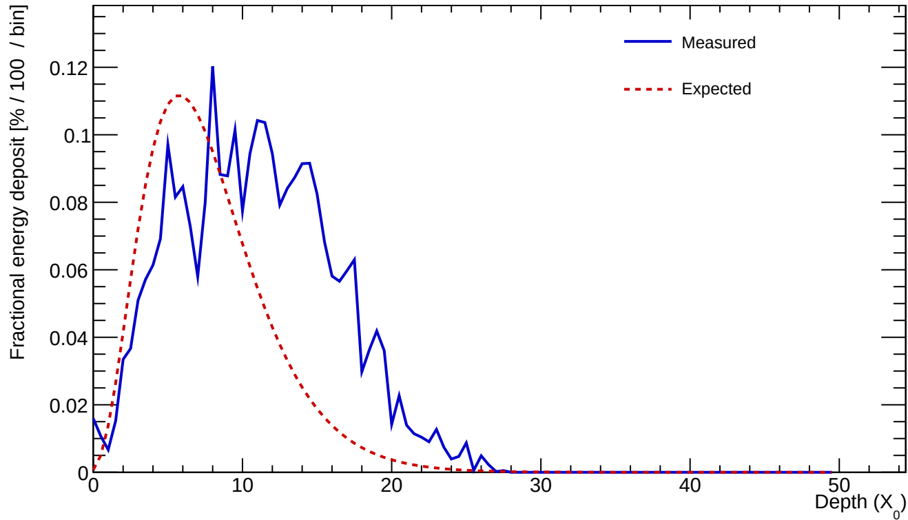
Cluster 689 E=25.375 GeV profileStart=4.00 X_0 \chi=0.4390
