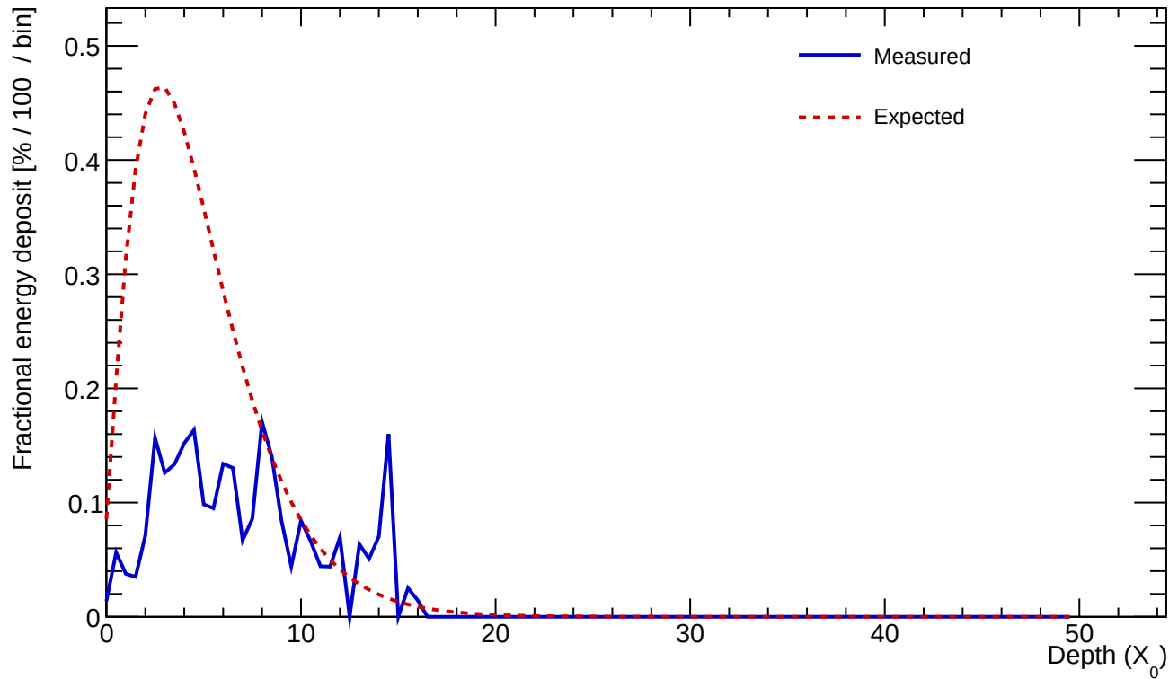
Cluster 215 E=1.287 GeV profileStart=1.50 X_0 \chi=0.4567
