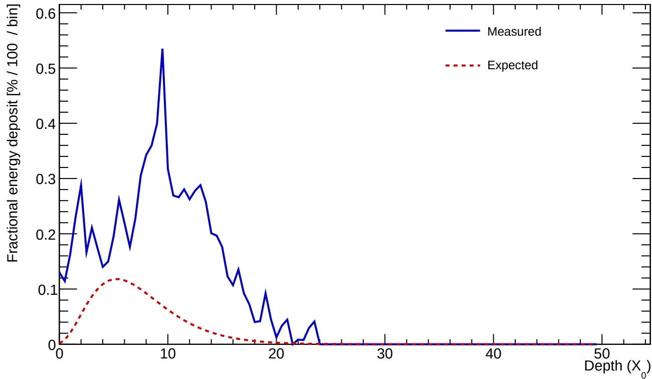
Cluster 95 E=15.558 GeV profileStart=3.00 X_0 \chi=0.4212
