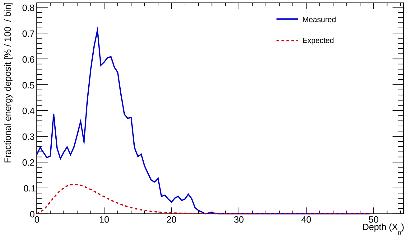
Cluster 111 E=21.223 GeV profileStart=3.00 X_0 \chi=0.3529
