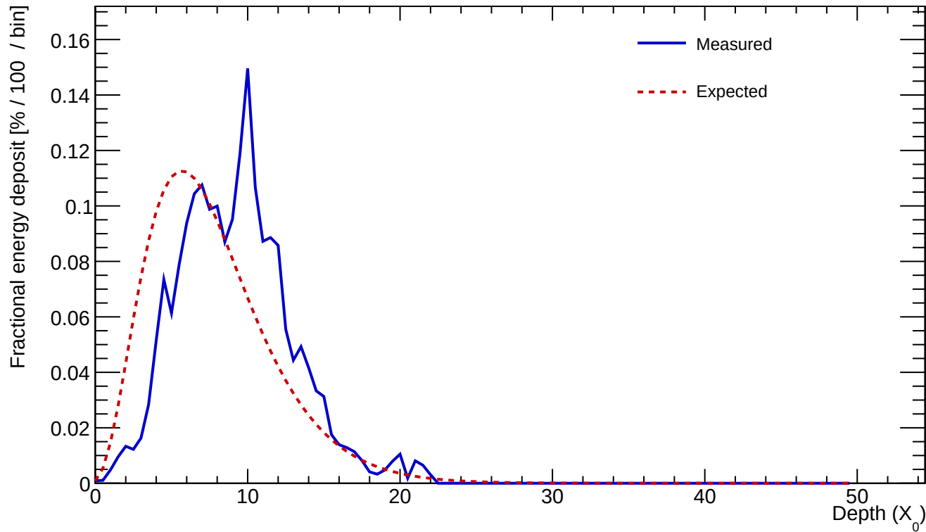
Cluster 11 E=23.395 GeV profileStart=2.00 X_0 \chi=0.1878
