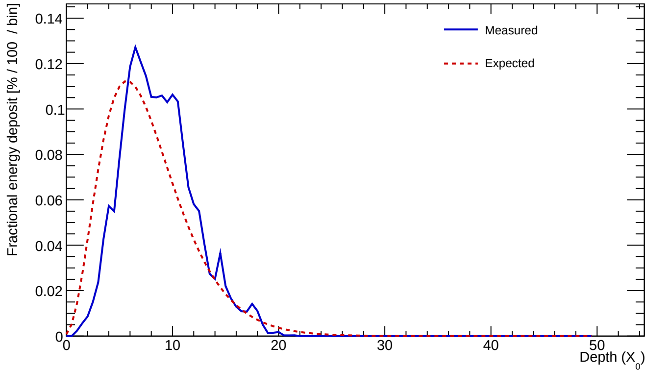
Cluster 70 E=24.222 GeV profileStart=1.50 X_0 \chi=0.1379
