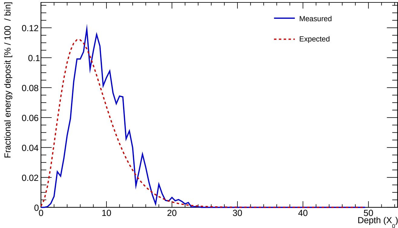
Cluster 332 E=24.425 GeV profileStart=1.50 X_0 \chi=0.1340
