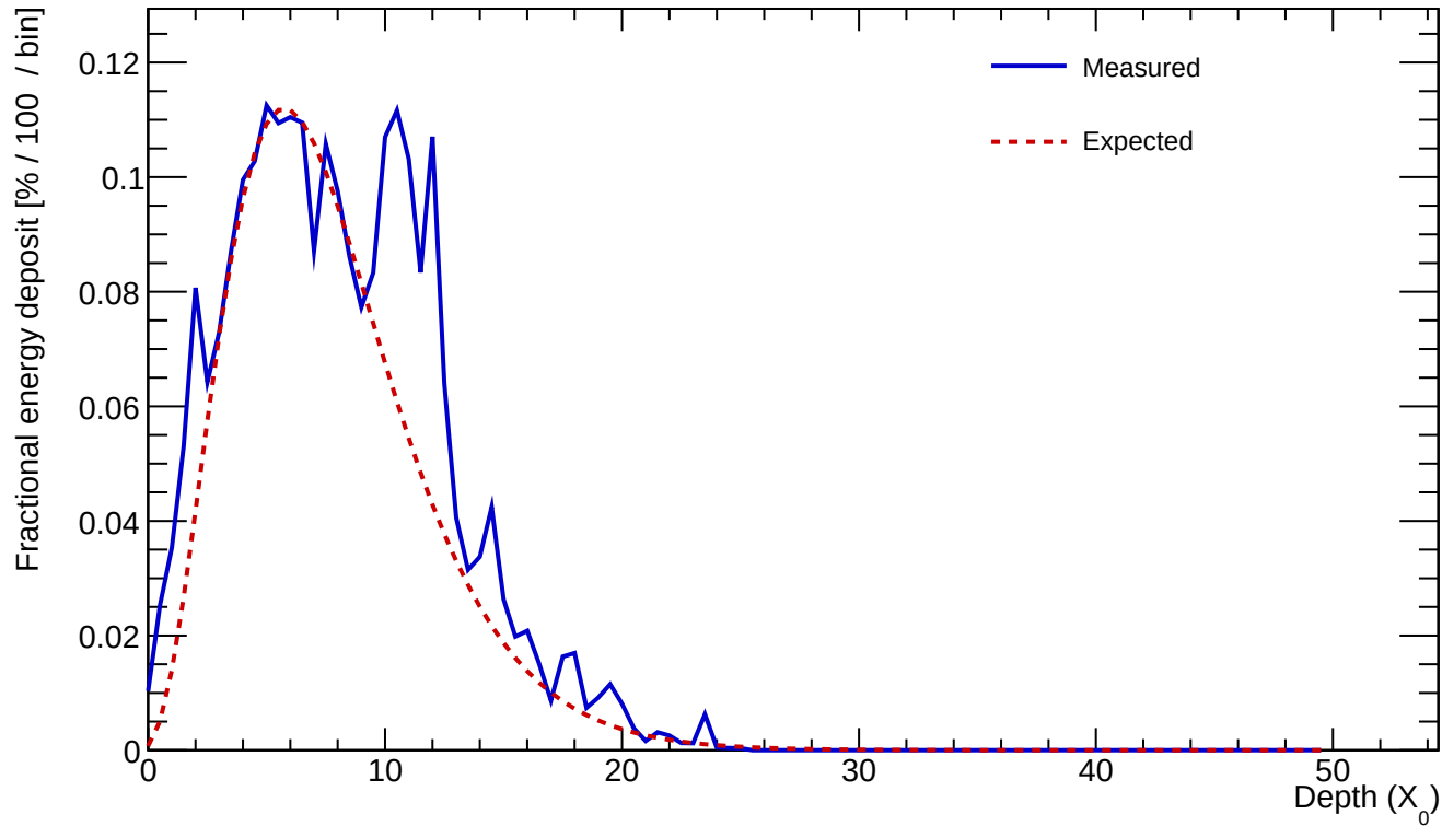
Cluster 22 E=24.998 GeV profileStart=0.50 X_0 \chi=0.2719
