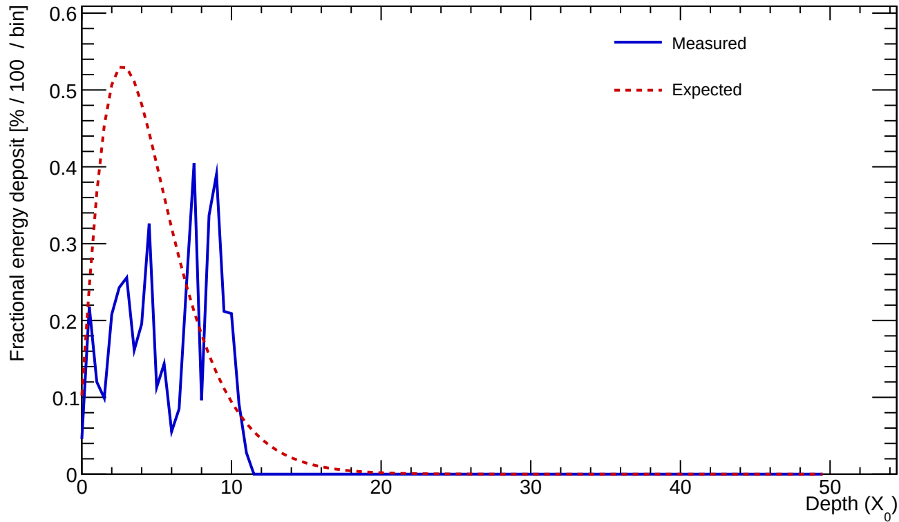
Cluster 113 E=1.224 GeV profileStart=1.00 X_0 \chi=0.5798
