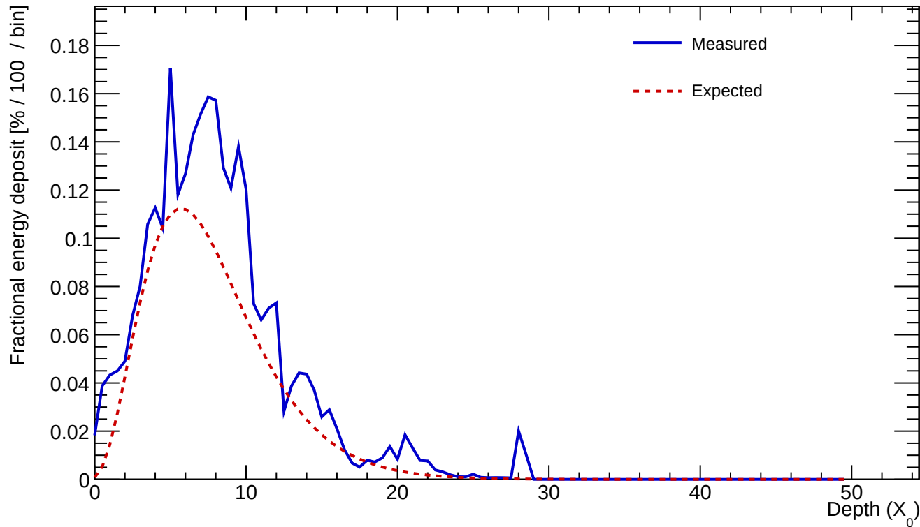
Cluster 110 E=24.185 GeV profileStart=0.50 X_0 \chi=0.1995
