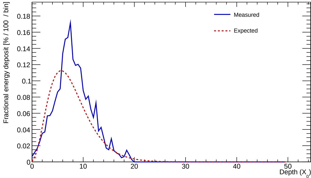
Cluster 453 E=23.600 GeV profileStart=1.00 X_0 \chi=0.2002
