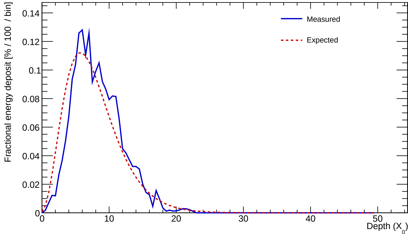
Cluster 511 E=24.544 GeV profileStart=1.00 X_0 \chi=0.1291
