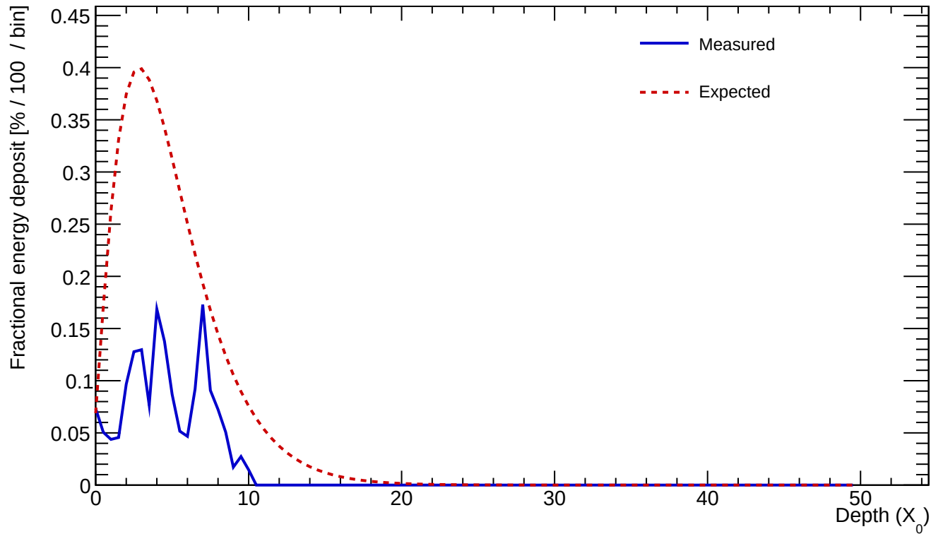
Cluster 244 E=1.379 GeV profileStart=0.50 X_0 \chi=0.3580
