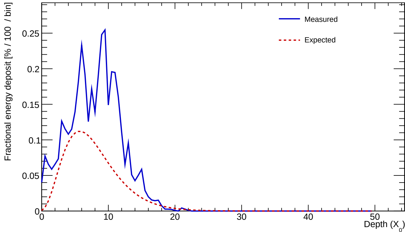
Cluster 643 E=24.687 GeV profileStart=0.50 X_0 \chi=0.3236
