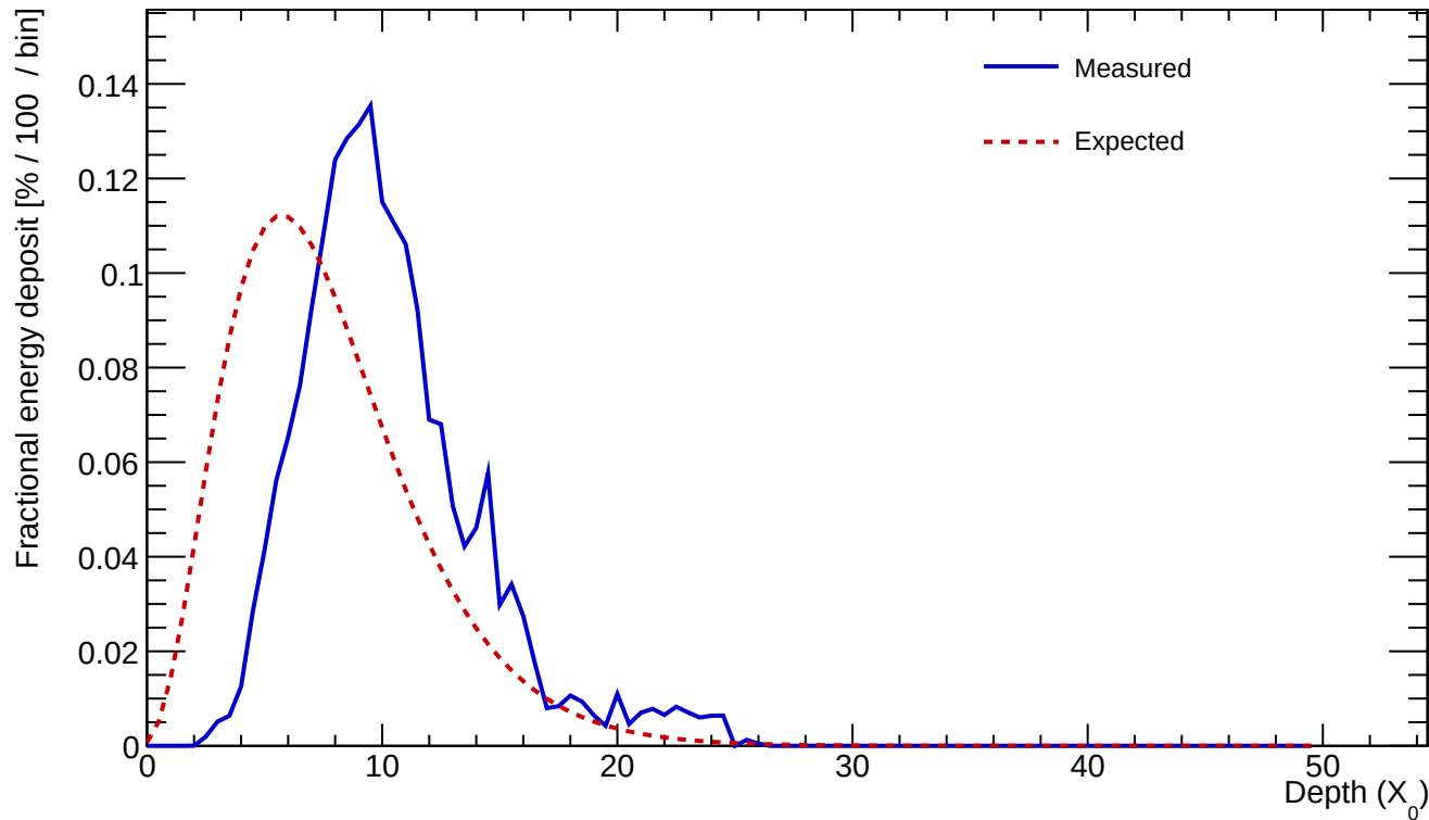
Cluster 330 E=24.458 GeV \text{profileStart}=3.00 X_0 \chi=0.1709
