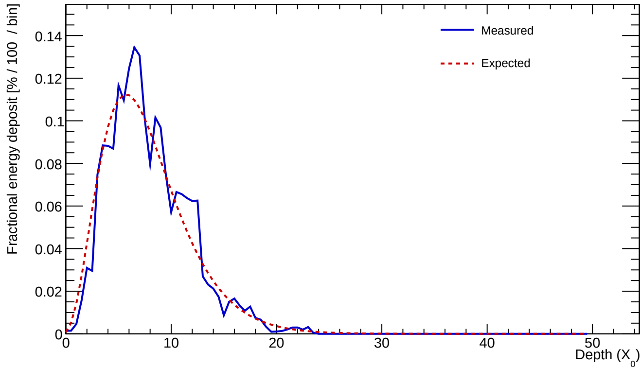
Cluster 166 E=24.185 GeV profileStart=0.50 X_0 \chi=0.1536
