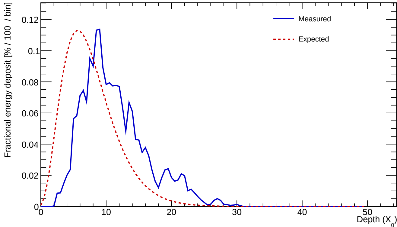
Cluster 389 E=22.847 GeV profileStart=3.00 X_0 \chi=0.2073
