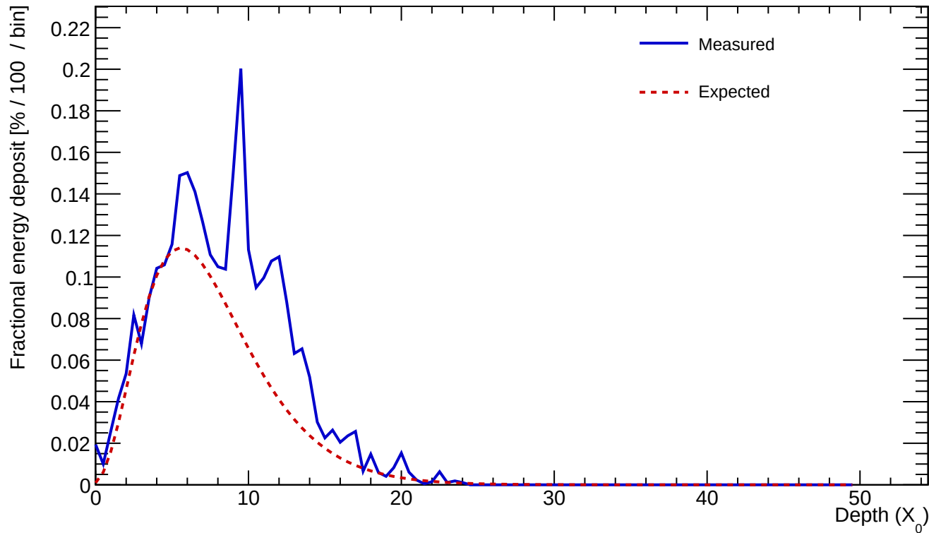
Cluster 253 E=21.033 GeV profileStart=1.00 X_0 \chi=0.2459
