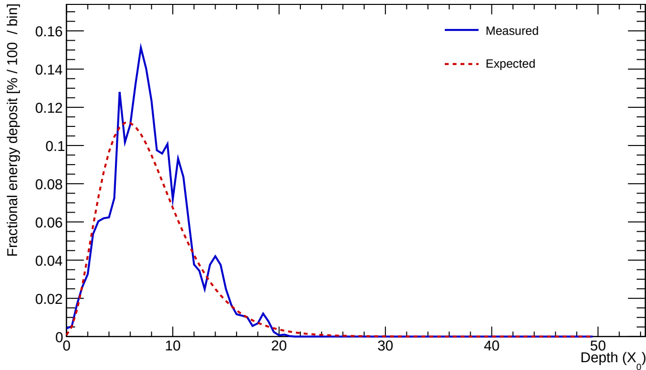
Cluster 575 E=24.614 GeV profileStart=0.50 X_0 \chi=0.1907
