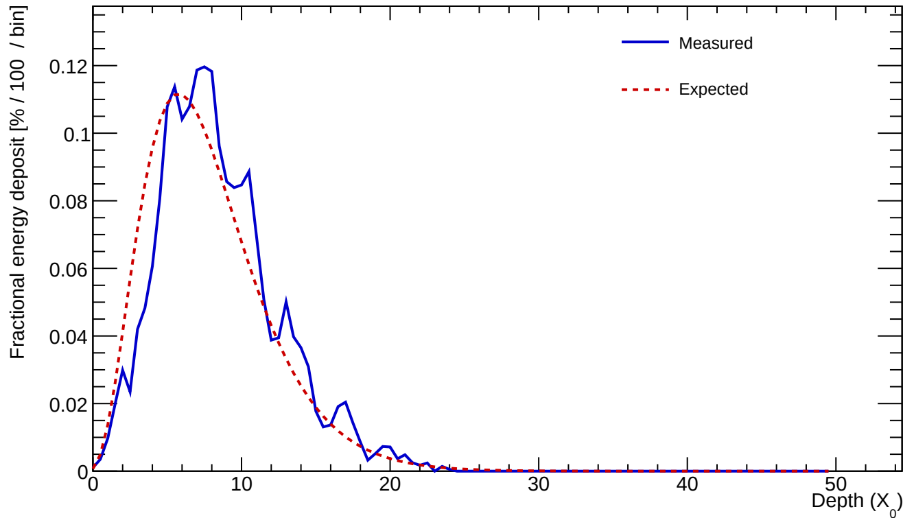
Cluster 414 E=25.666 GeV profileStart=1.00 X_0 \chi=0.1318
