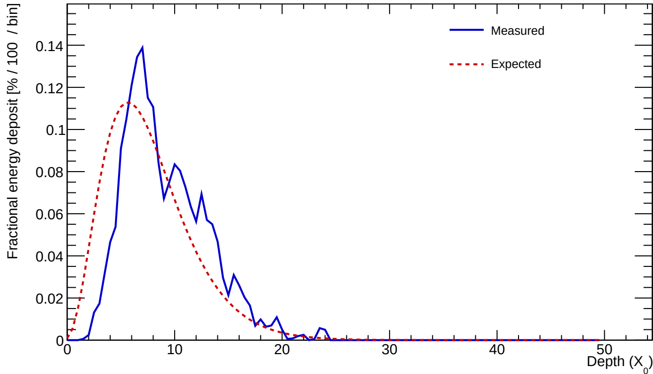
Cluster 137 E=22.989 GeV profileStart=1.50 X_0 \chi=0.1687
