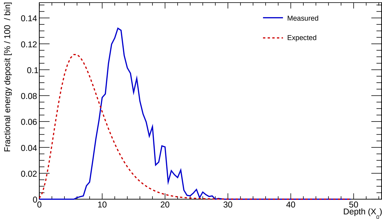
Cluster 426 E=24.985 GeV profileStart=6.50 X_0 \chi=0.1459
