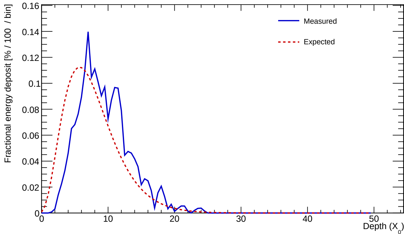
Cluster 617 E=23.973 GeV profileStart=2.00 X_0 \chi=0.1428
