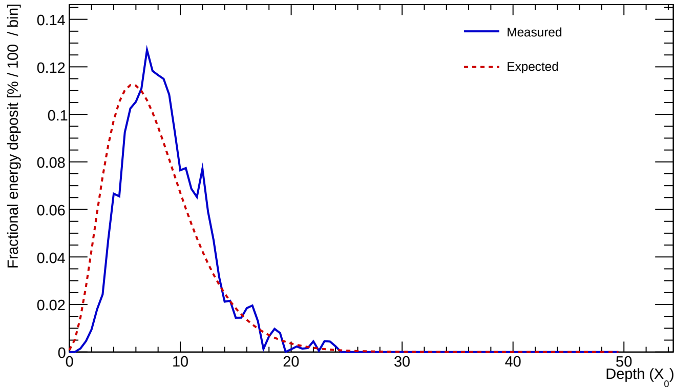
Cluster 503 E=23.863 GeV profileStart=1.50 X_0 \chi=0.1308
