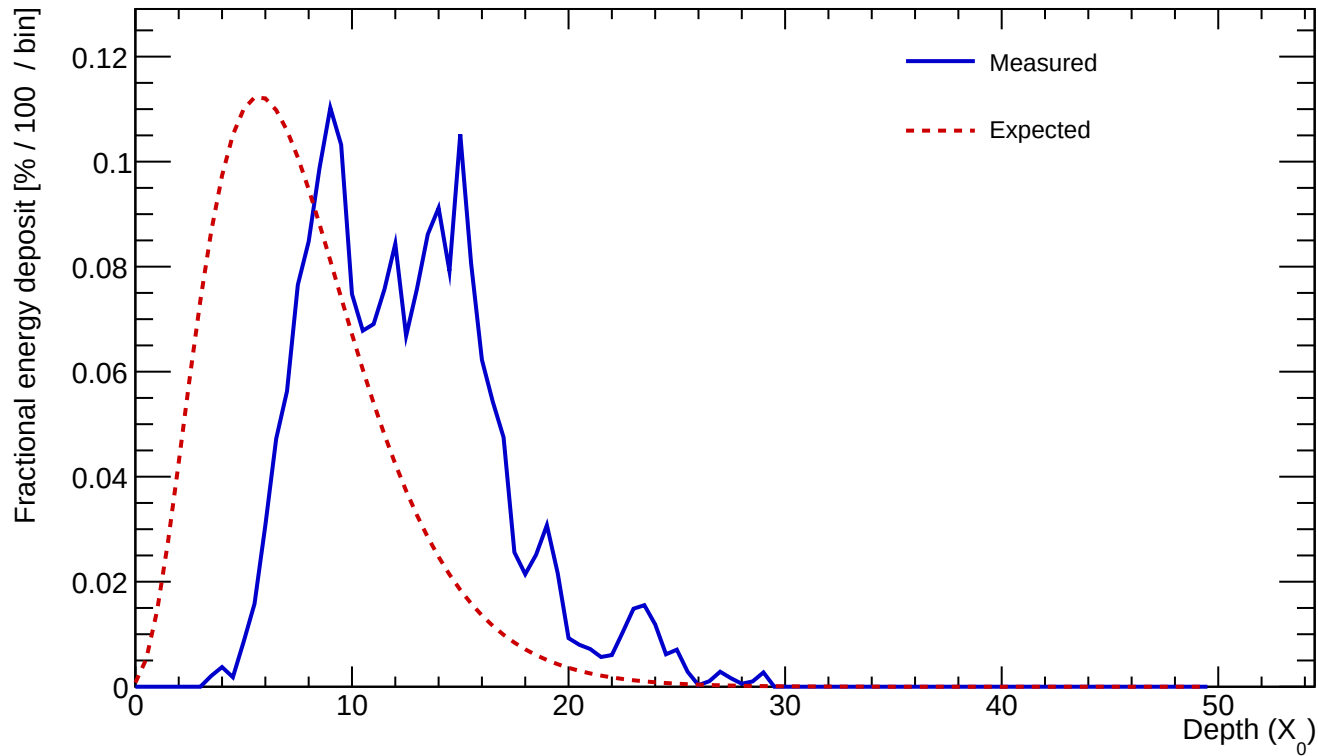
Cluster 636 E=24.021 GeV profileStart=4.50 X_0 \chi=0.2400
