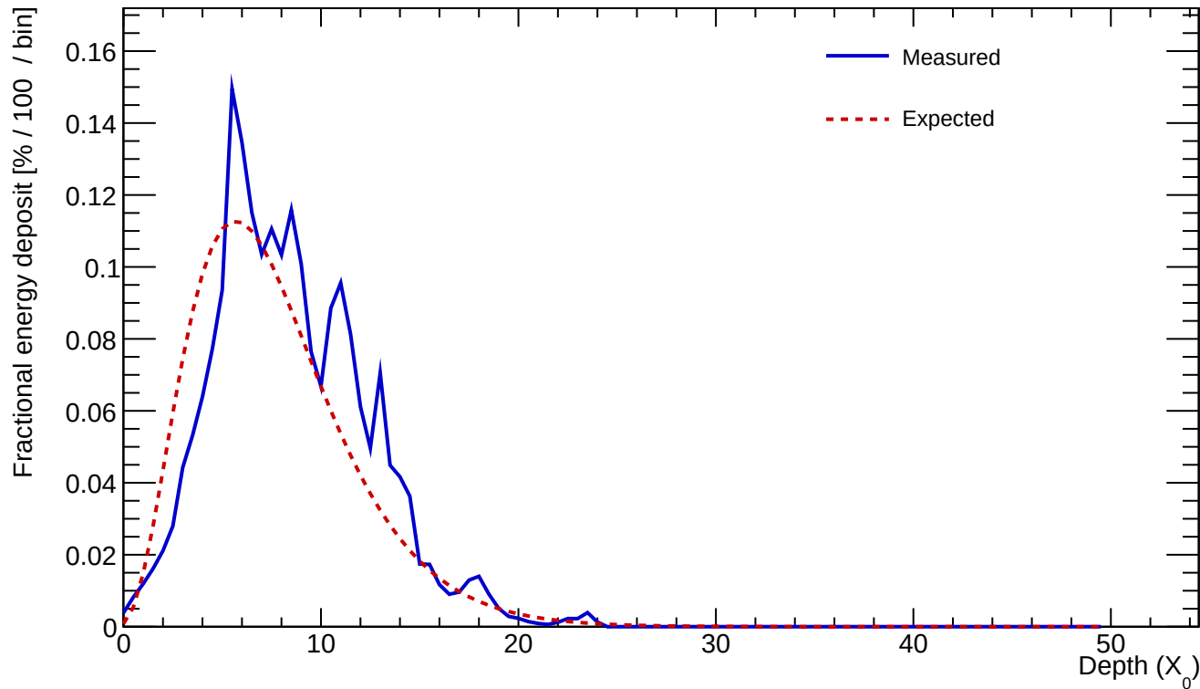
Cluster 221 E=23.302 GeV profileStart=1.00 X_0 \chi=0.1810
