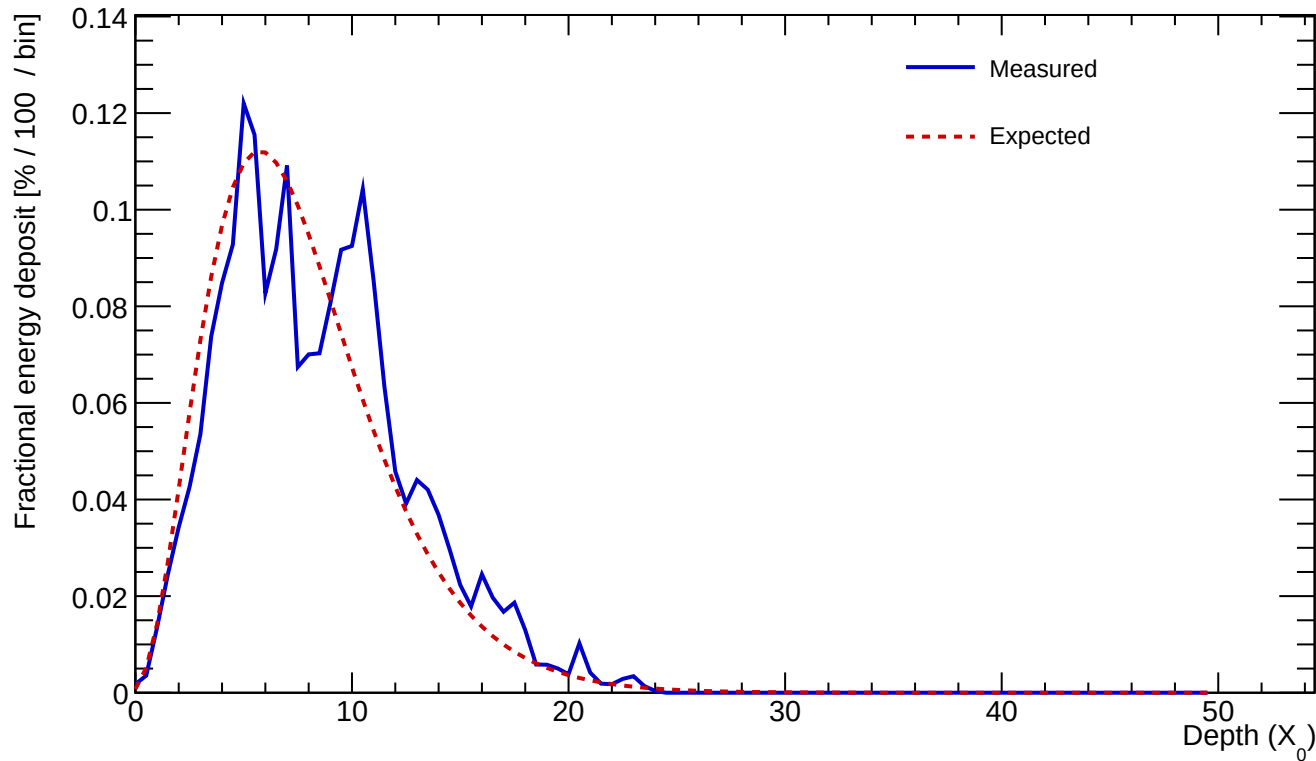
Cluster 524 E=24.541 GeV profileStart=0.50 X_0 \chi=0.1942
