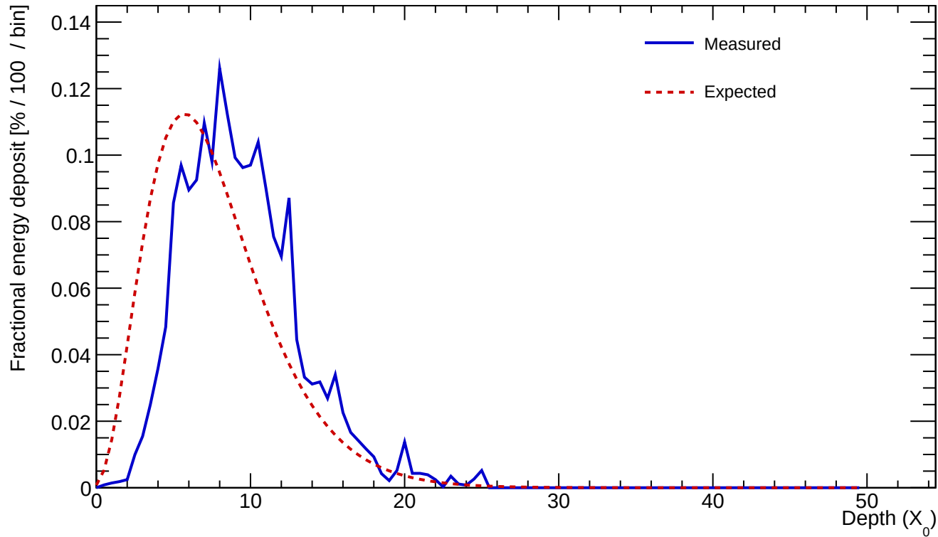
Cluster 139 E=23.917 GeV profileStart=2.00 X_0 \chi=0.1401
