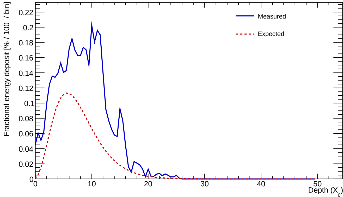
Cluster 383 E=22.392 GeV profileStart=0.50 X_0 \chi=0.3160
