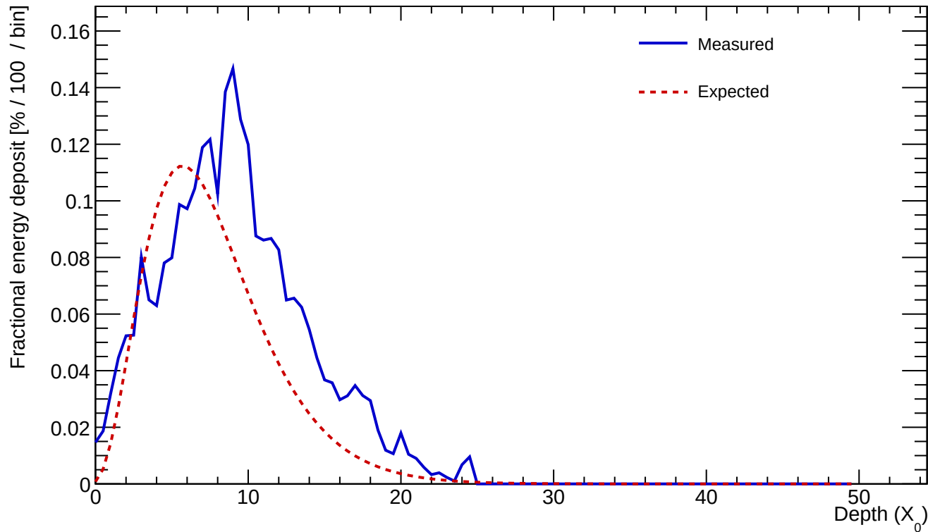
Cluster 608 E=24.103 GeV profileStart=1.50 X_0 \chi=0.2546
