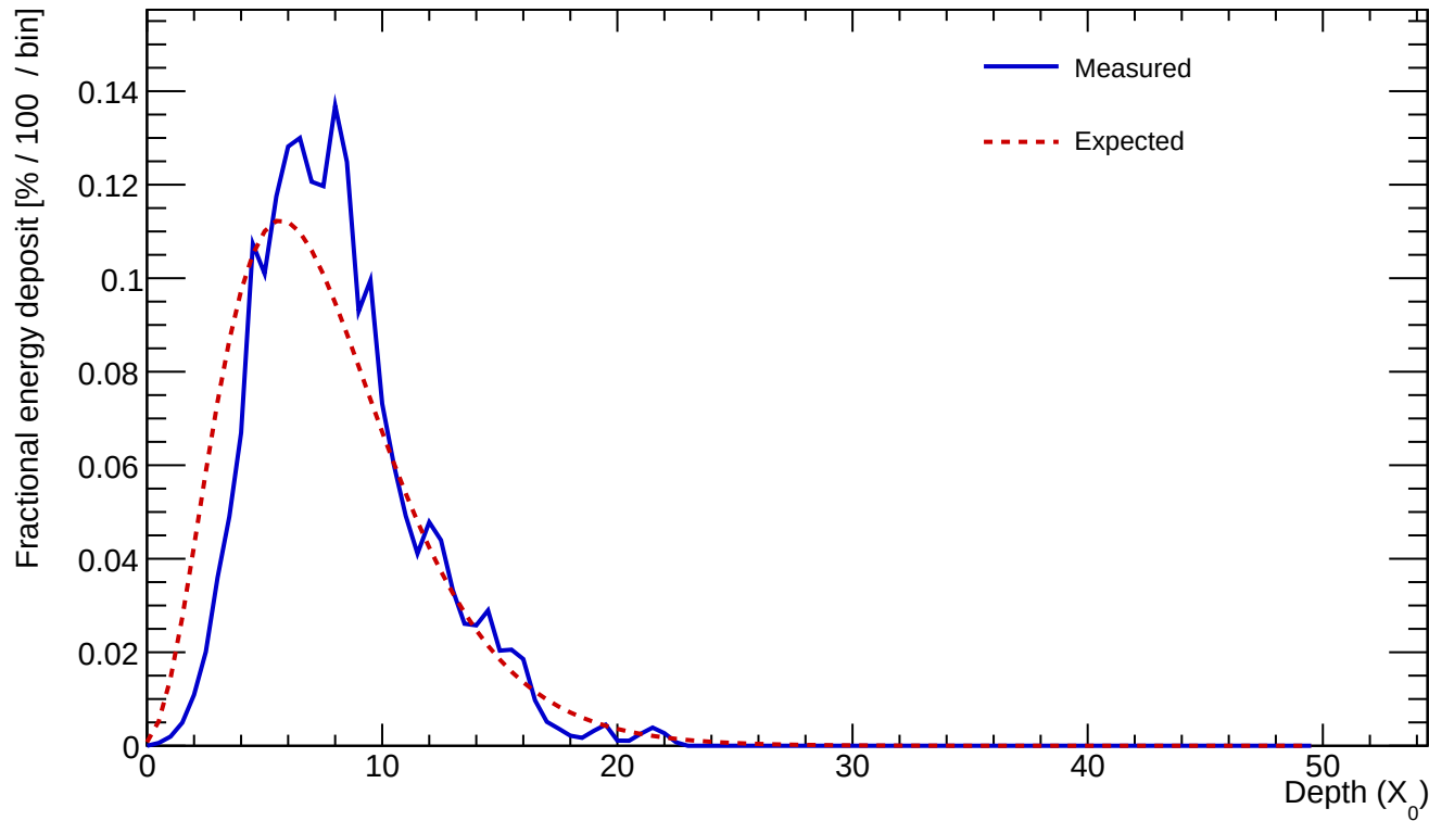
Cluster 289 E=23.999 GeV profileStart=1.00 X_0 \chi=0.1760
