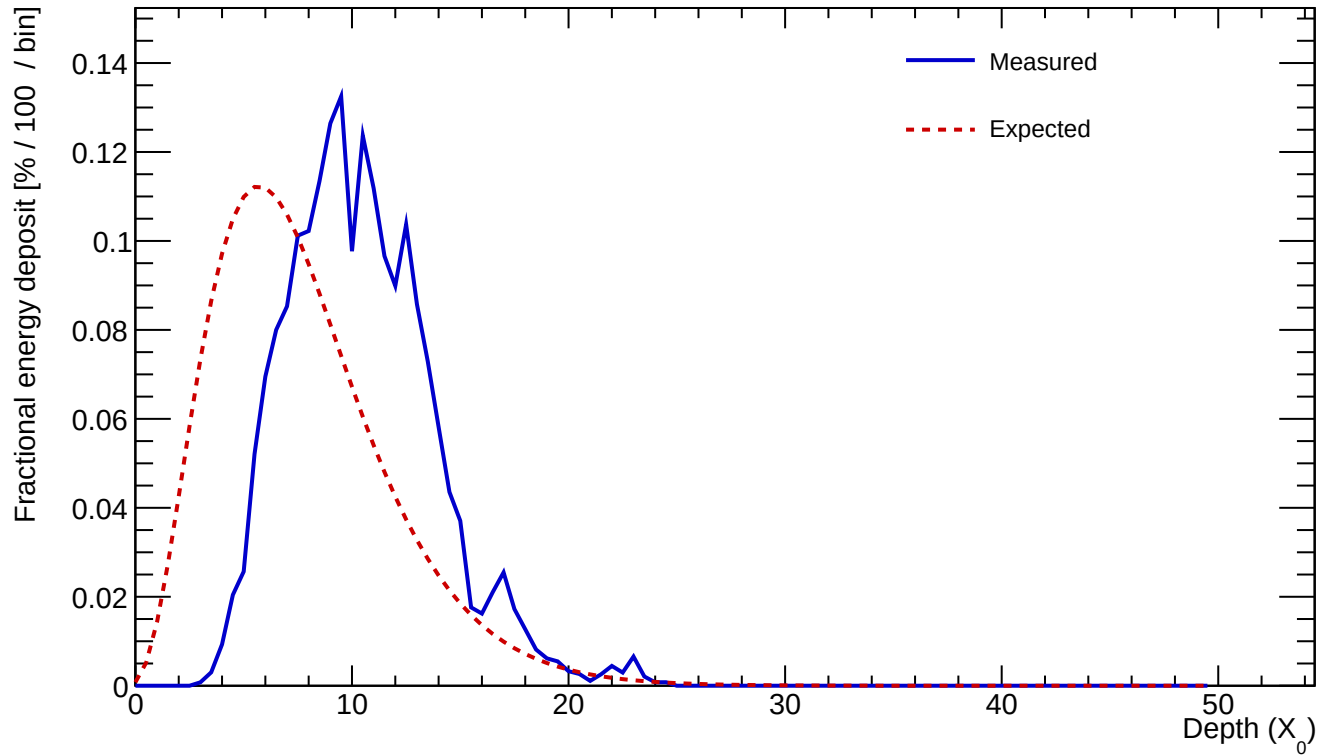
Cluster 63 E=24.189 GeV profileStart=3.50 X_0 \chi=0.1744
