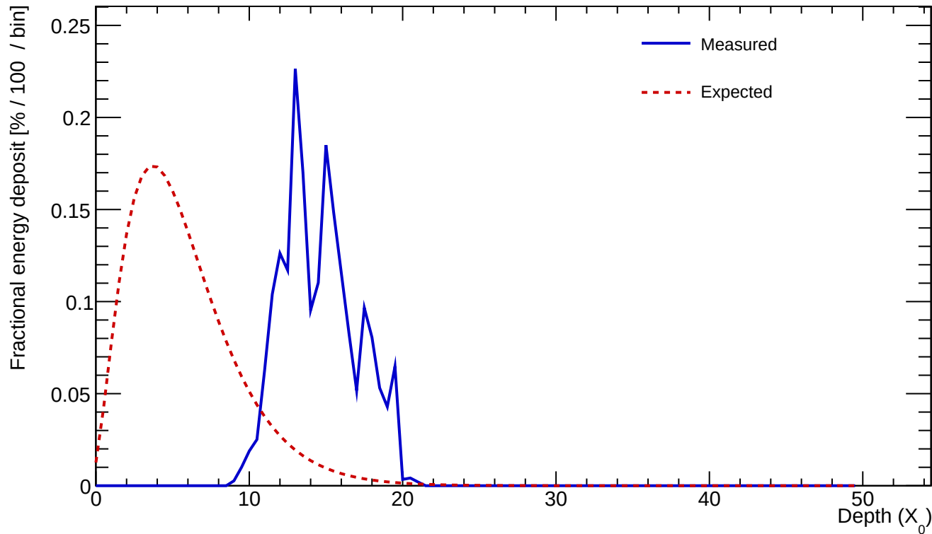
Cluster 243 E=3.250 GeV profileStart=10.00 X_0 \chi=0.2782
