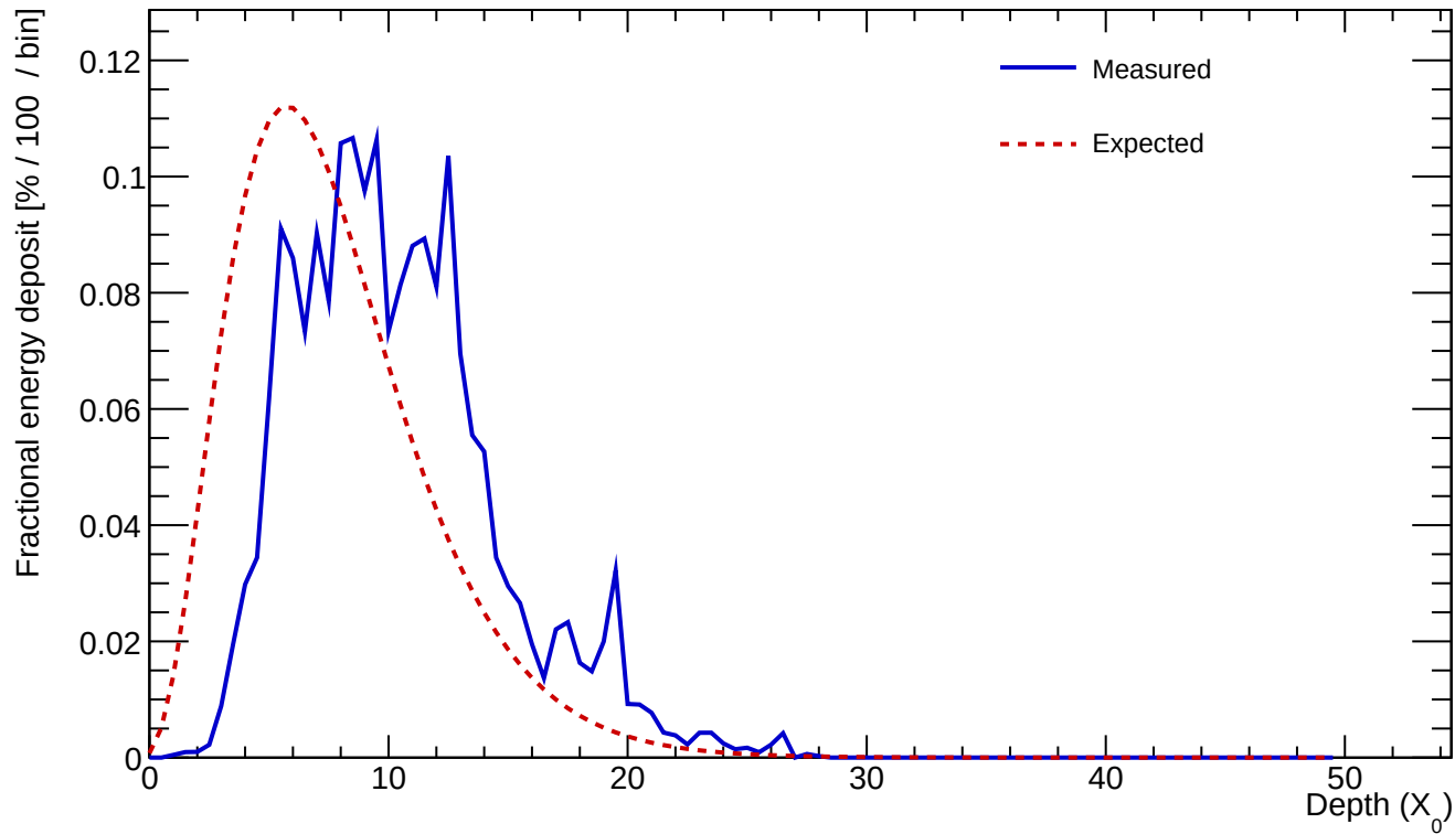
Cluster 89 E=24.633 GeV profileStart=2.50 X_0 \chi=0.1693
