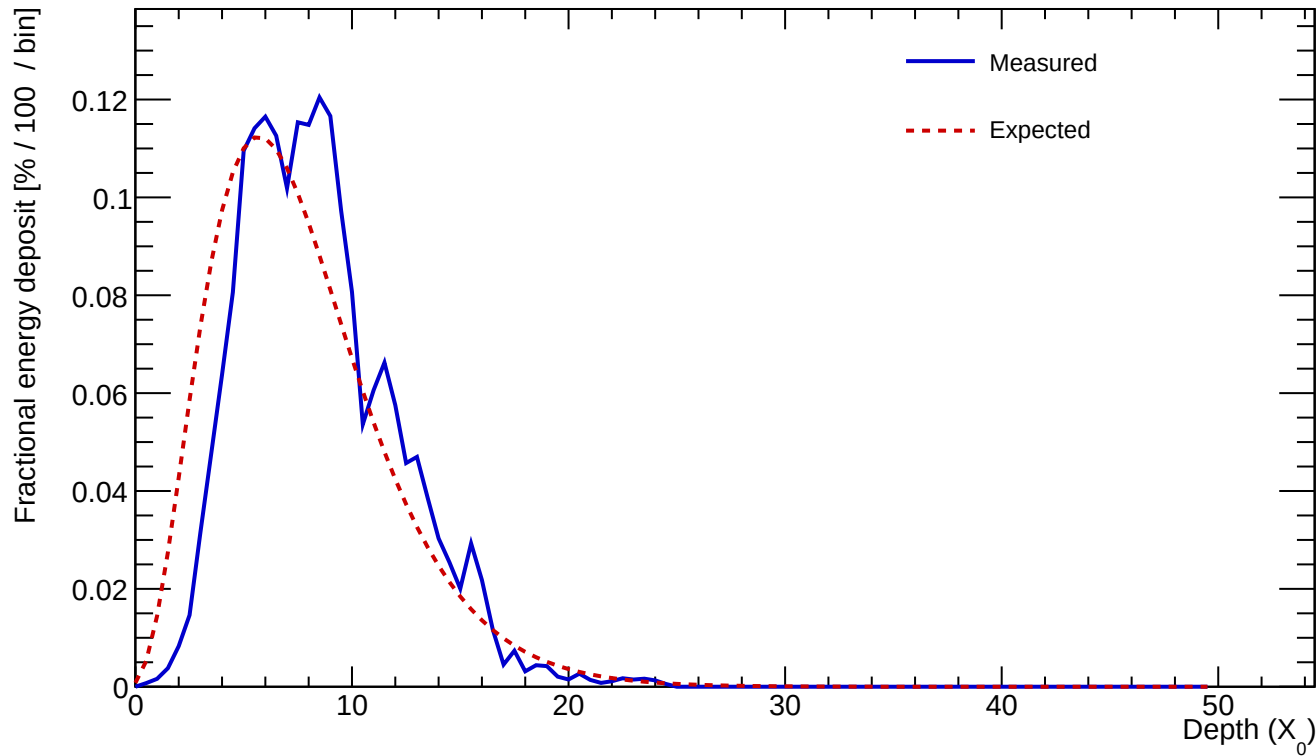
Cluster 359 E=23.998 GeV profileStart=1.00 X_0 \chi=0.1423
