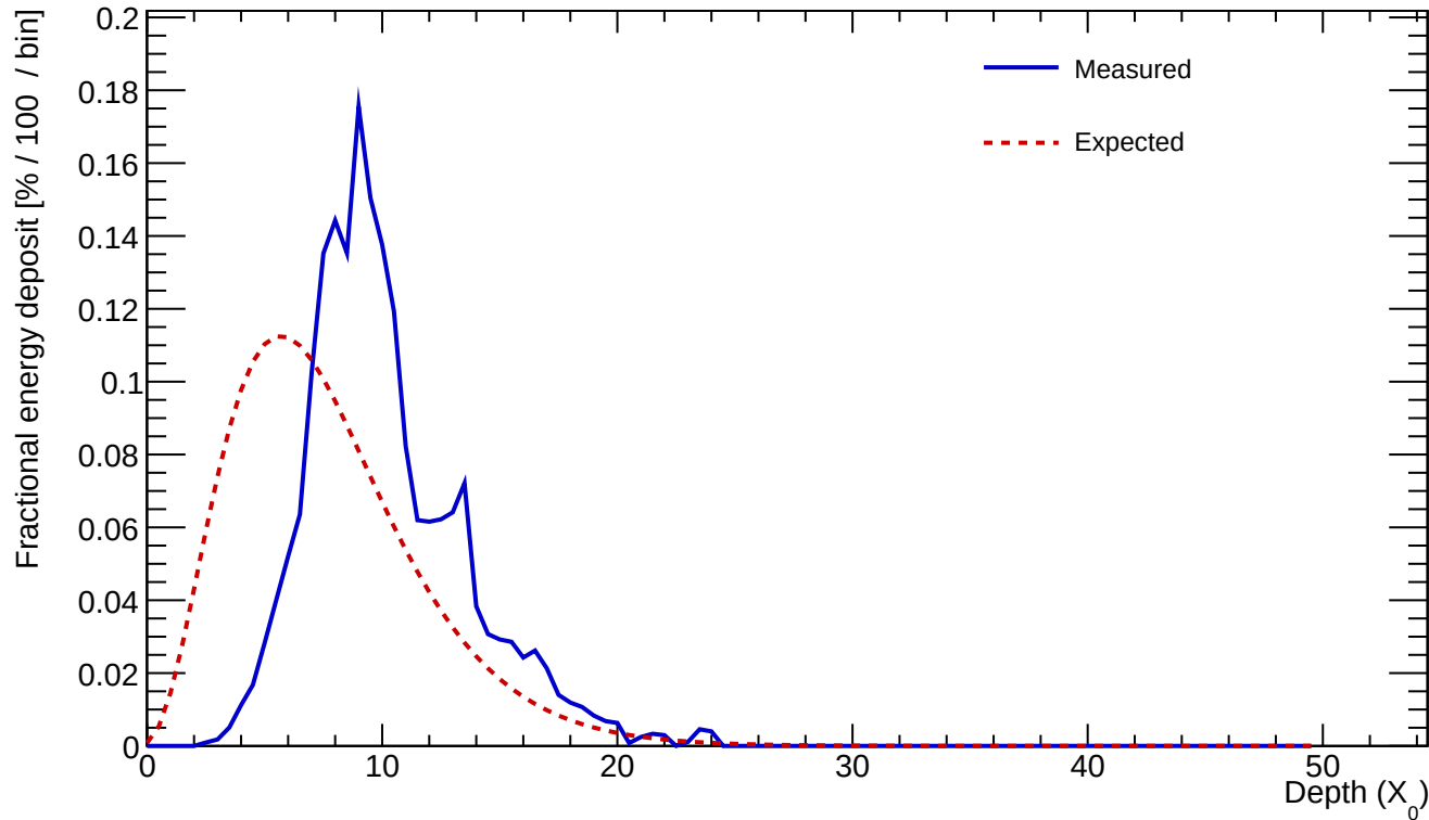
Cluster 219 E=23.649 GeV profileStart=3.00 X_0 \chi=0.2735
