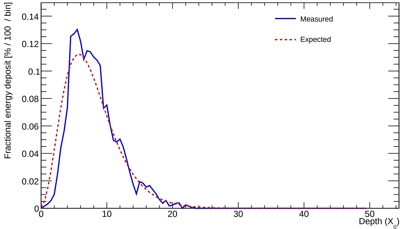
Cluster 159 E=24.299 GeV profileStart=1.00 X_0 \chi=0.1565
