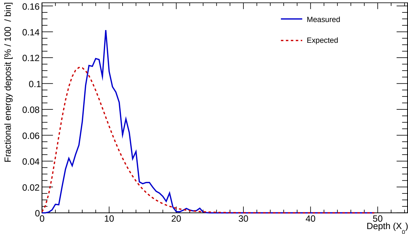
Cluster 694 E=23.708 GeV profileStart=2.50 X_0 \chi=0.1773
