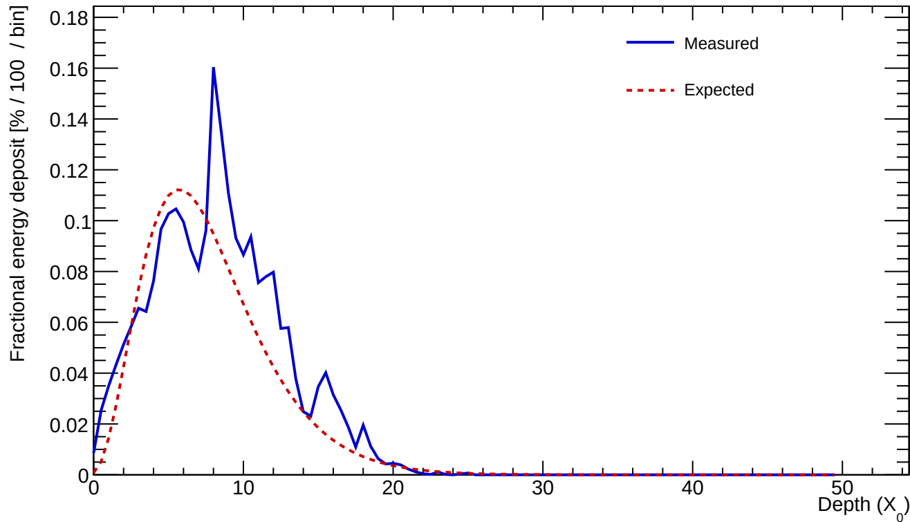
Cluster 124 E=24.184 GeV profileStart=1.00 X_0 \chi=0.2540
