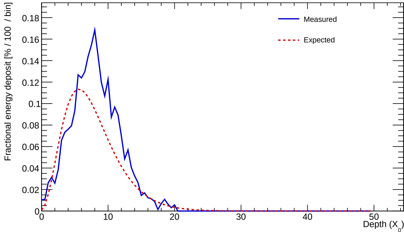
Cluster 341 E=22.195 GeV profileStart=1.00 X_0 \chi=0.1798
