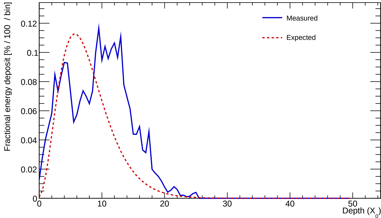
Cluster 233 E=23.407 GeV profileStart=2.50 X_0 \chi=0.4667
