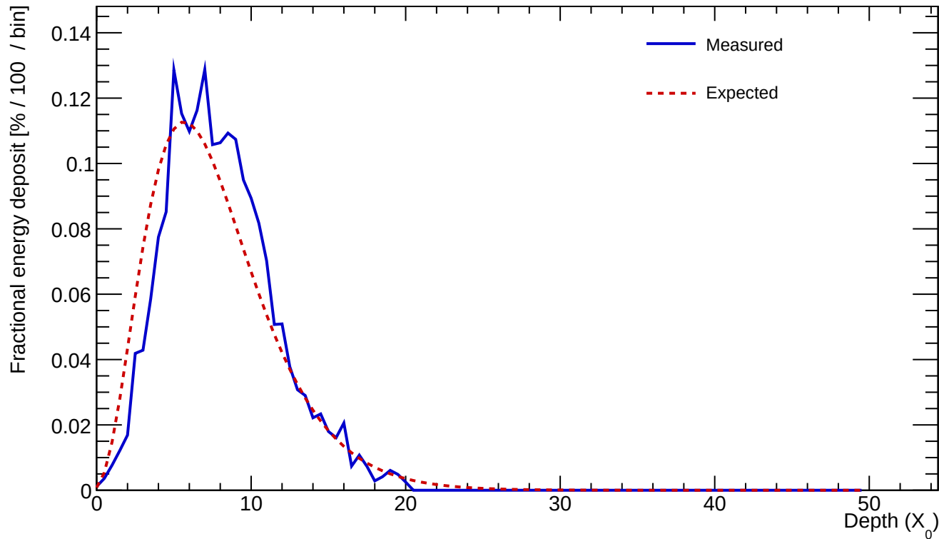
Cluster 163 E=23.340 GeV profileStart=1.00 X_0 \chi=0.1224
