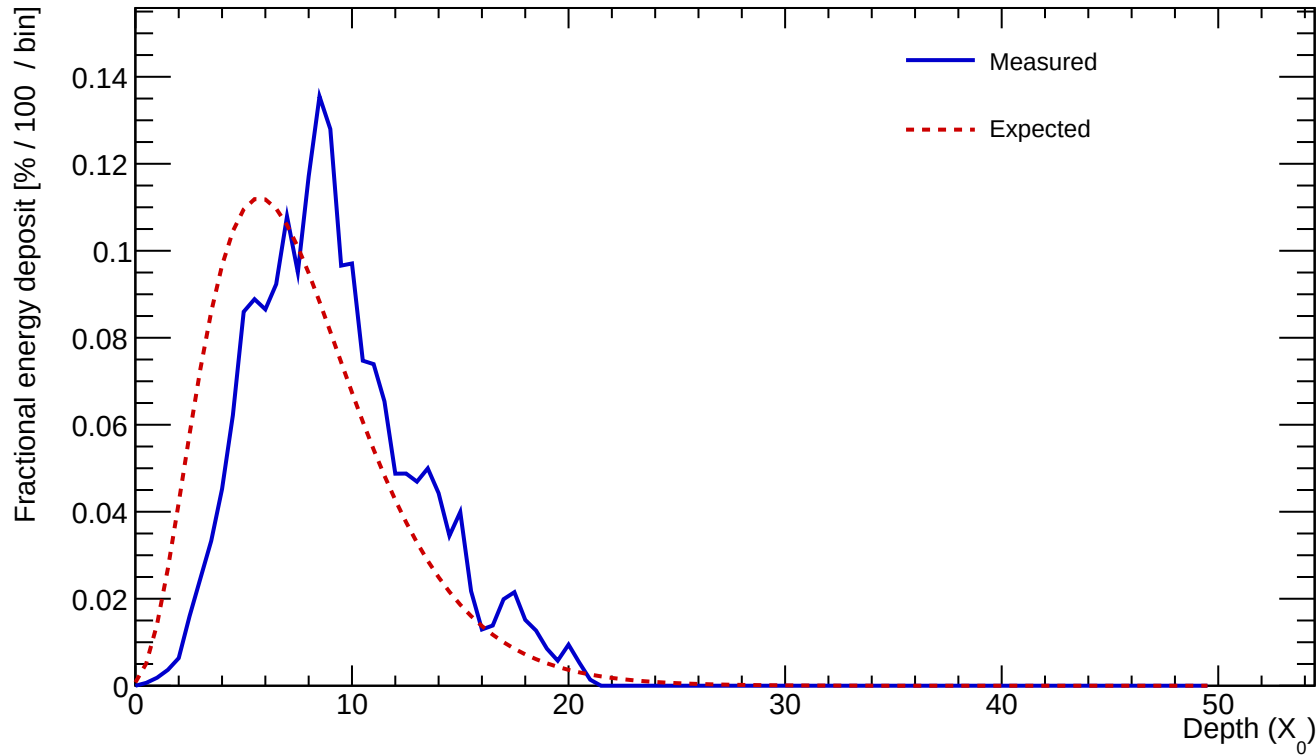
Cluster 147 E=24.678 GeV profileStart=1.50 X_0 \chi=0.1351
