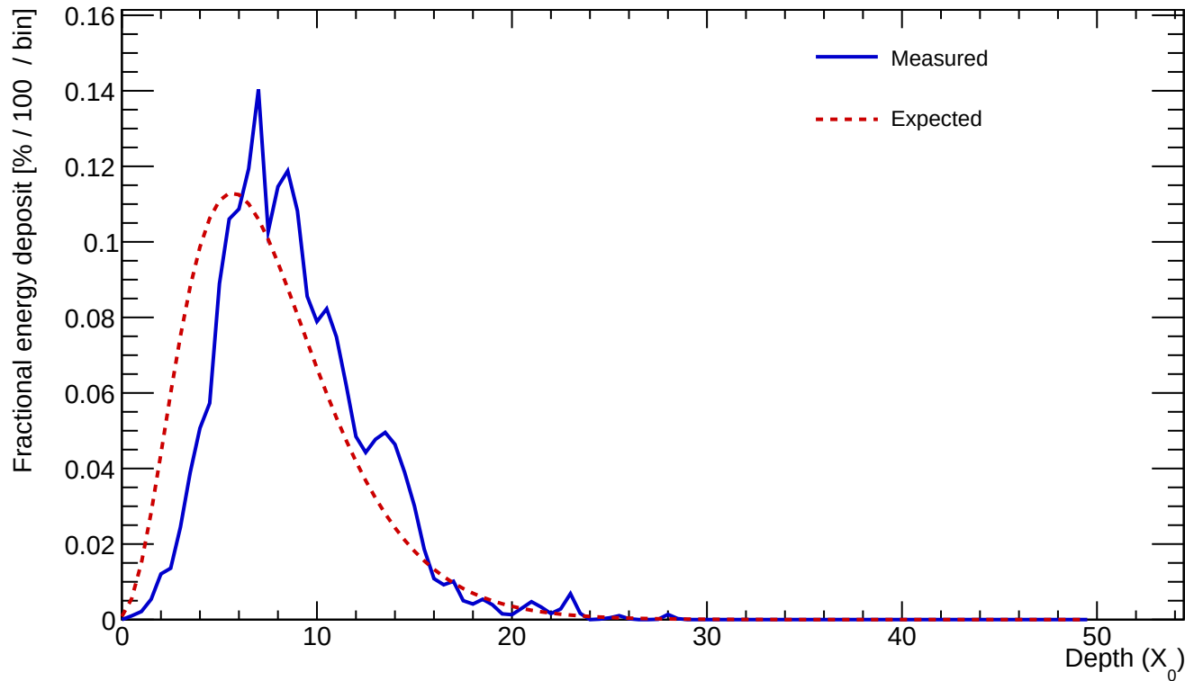
Cluster 472 E=22.828 GeV profileStart=1.50 X_0 \chi=0.1458
