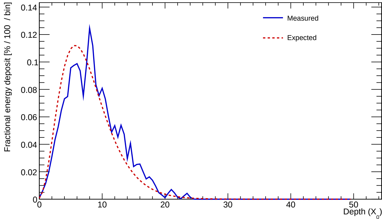
Cluster 262 E=24.593 GeV profileStart=1.00 X_0 \chi=0.1692
