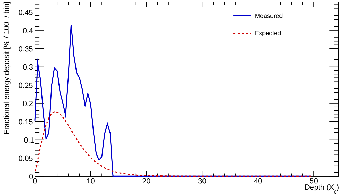
Cluster 415 E=3.143 GeV profileStart=1.50 X_0 \chi=0.3689
