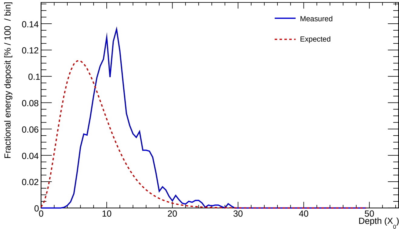
Cluster 354 E=24.916 GeV profileStart=4.00 X_0 \chi=0.1520
