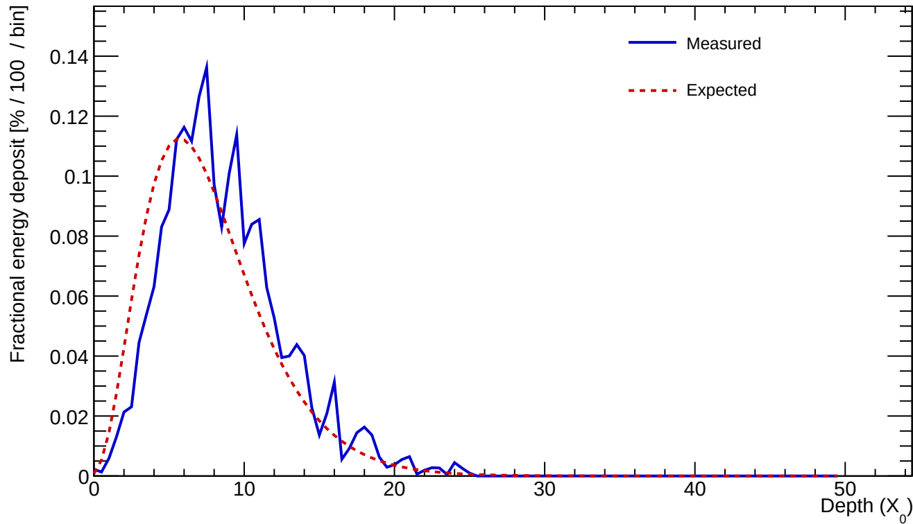
Cluster 380 E=23.923 GeV profileStart=1.00 X_0 \chi=0.1466
