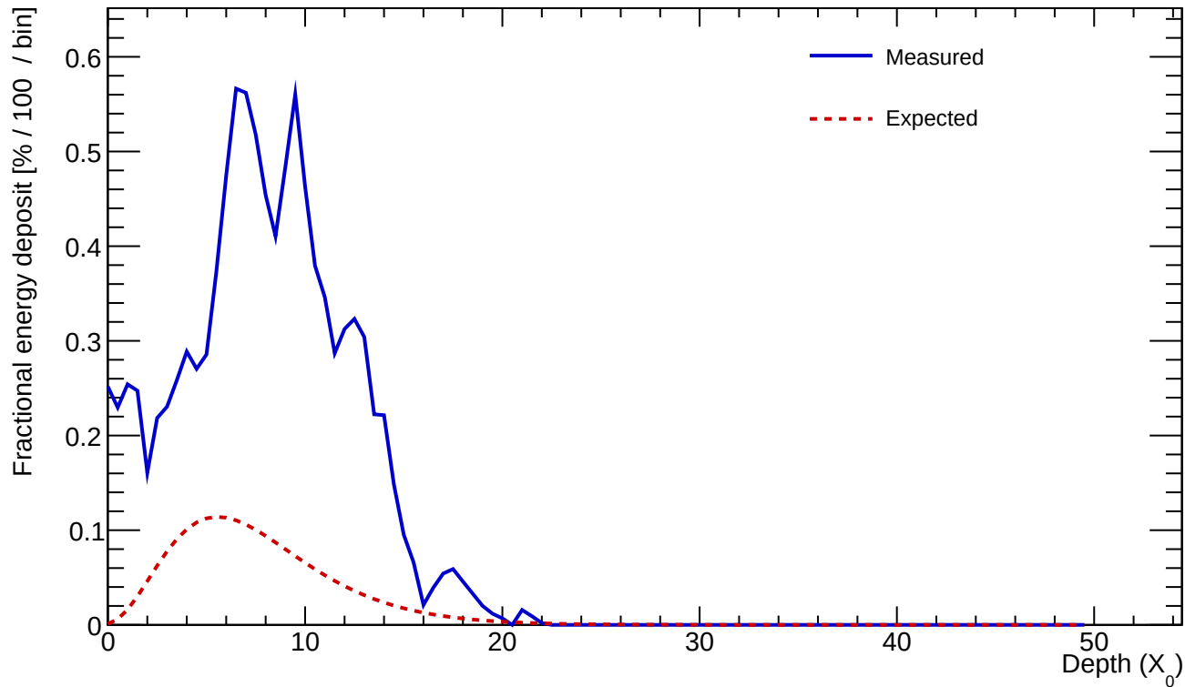
Cluster 396 E=20.893 GeV profileStart=1.00 X_0 \chi=0.2919
