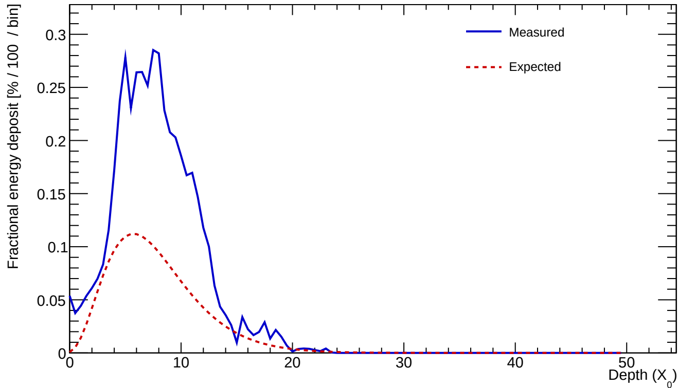
Cluster 548 E=24.552 GeV profileStart=1.00 X_0 \chi=0.1775
