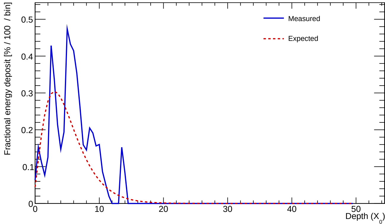
Cluster 572 E=1.628 GeV profileStart=1.50 X_0 \chi=0.4064
