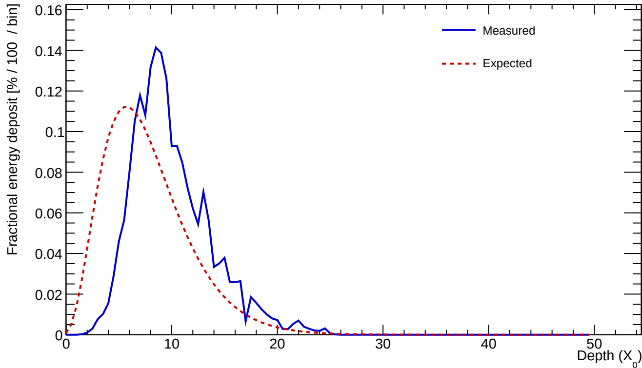
Cluster 456 E=24.238 GeV profileStart=2.50 X_0 \chi=0.1570
