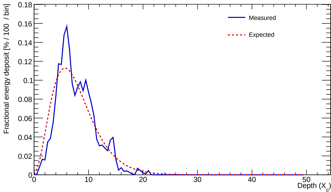
Cluster 303 E=23.055 GeV profileStart=0.50 X_0 \chi=0.2260
