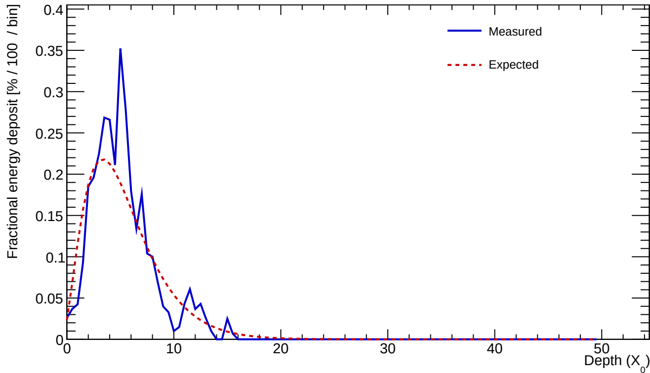
Cluster 19 E=2.247 GeV profileStart=0.50 X_0 \chi=0.2630
