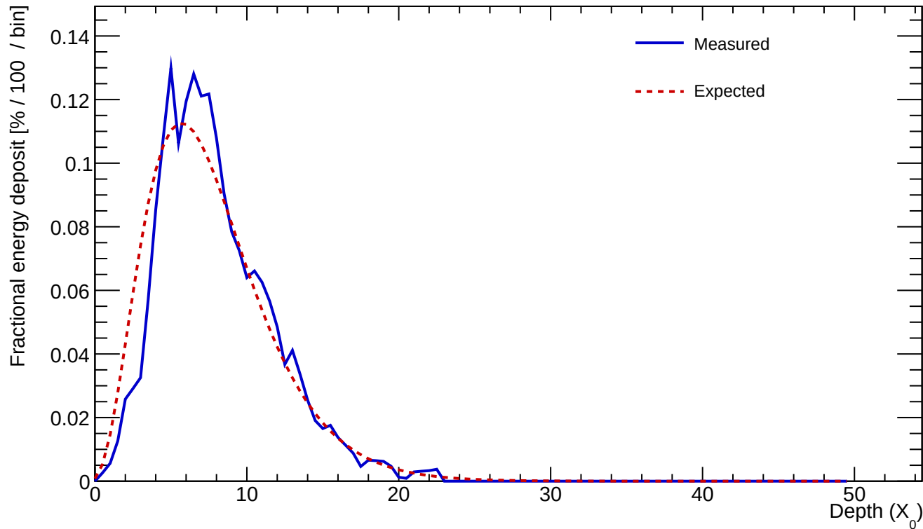
Cluster 291 E=23.574 GeV profileStart=0.50 X_0 \chi=0.1238
