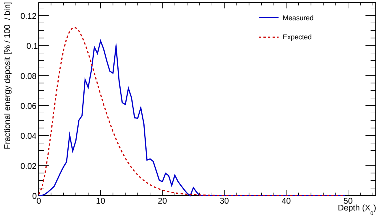
Cluster 391 E=24.735 GeV profileStart=4.00 X_0 \chi=0.2096
