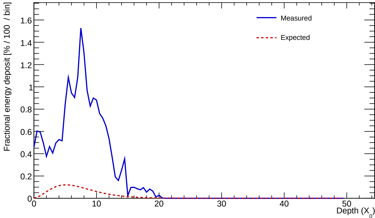
Cluster 230 E=13.411 GeV profileStart=1.50 X_0 \chi=0.3136
