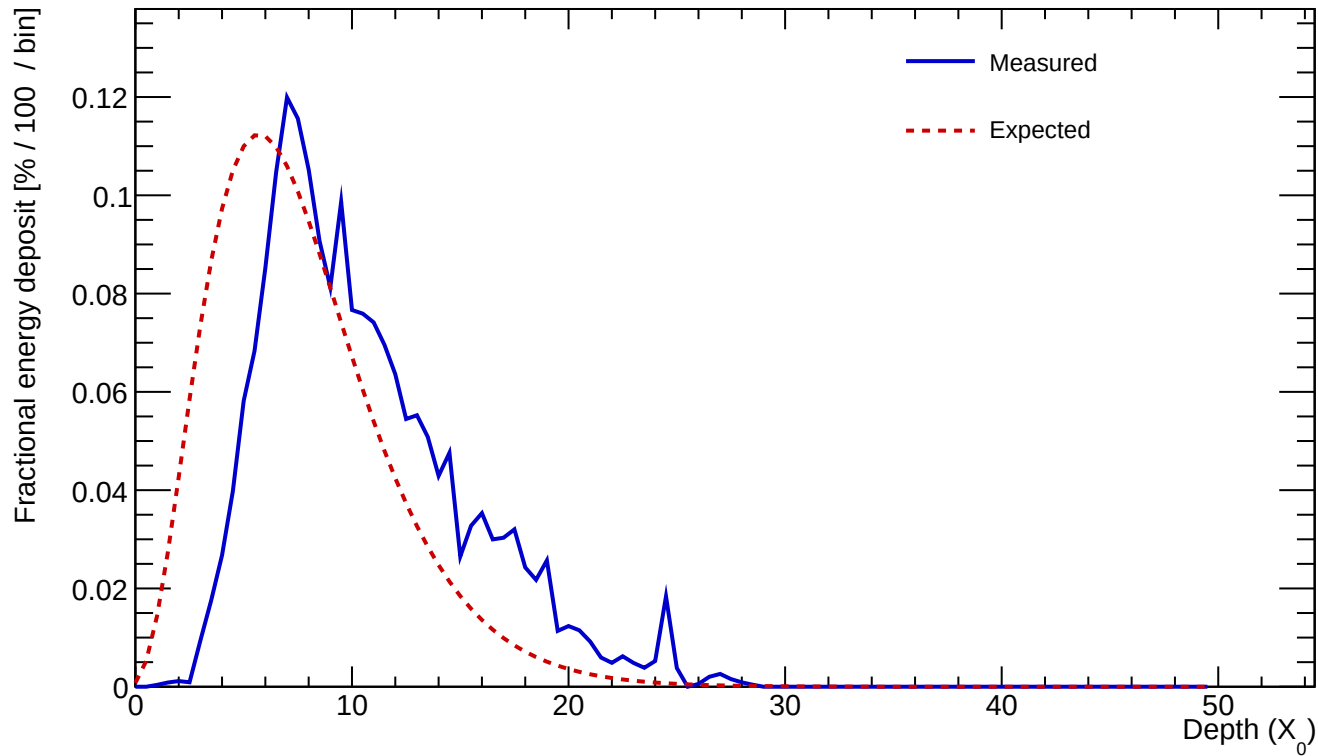
Cluster 310 E=24.068 GeV profileStart=2.50 X_0 \chi=0.1665
