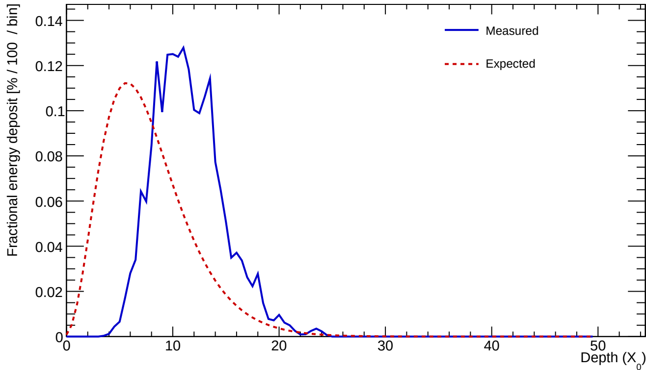
Cluster 671 E=24.106 GeV profileStart=4.50 X_0 \chi=0.1805
