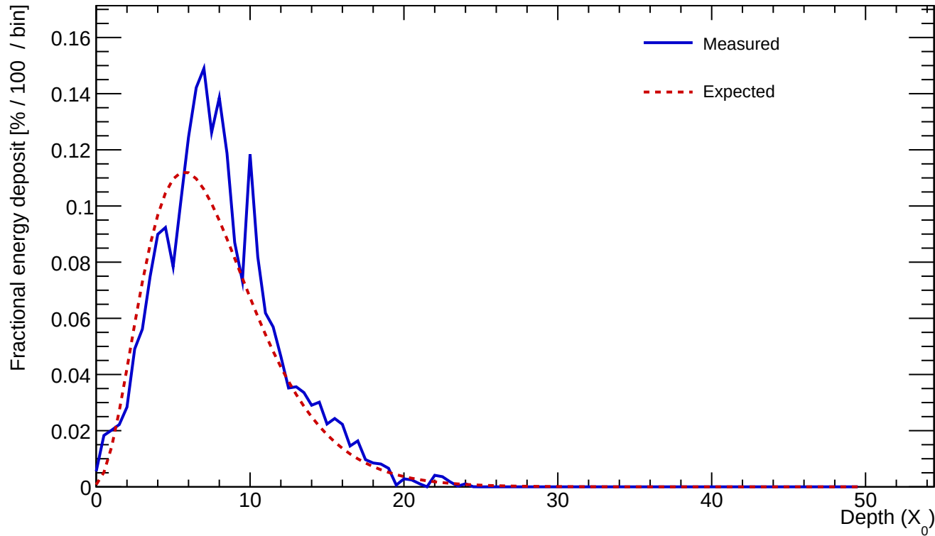
Cluster 637 E=24.556 GeV profileStart=0.50 X_0 \chi=0.1691
