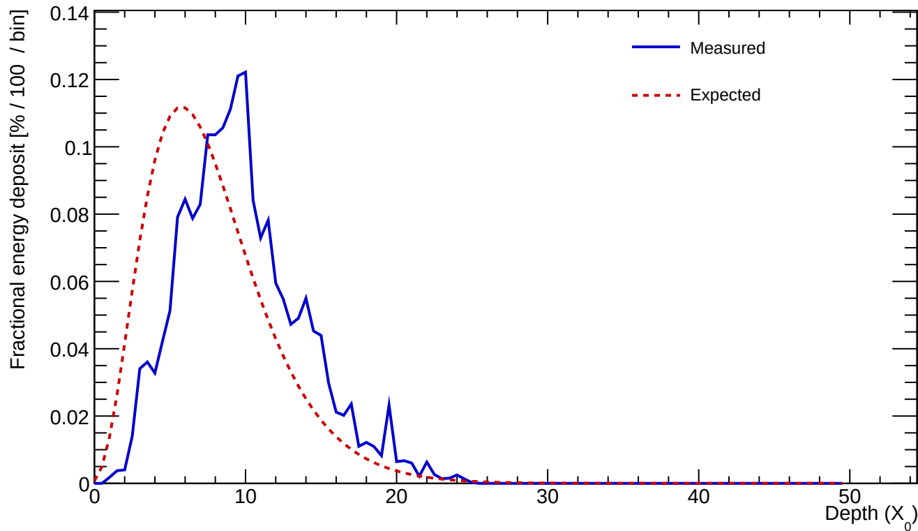
Cluster 187 E=25.273 GeV profileStart=2.50 X_0 \chi=0.1662
