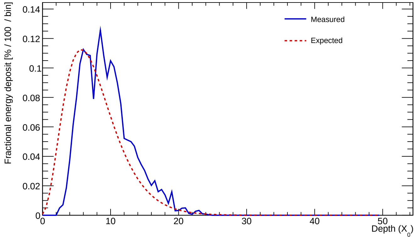
Cluster 192 E=23.905 GeV profileStart=2.00 X_0 \chi=0.1232
