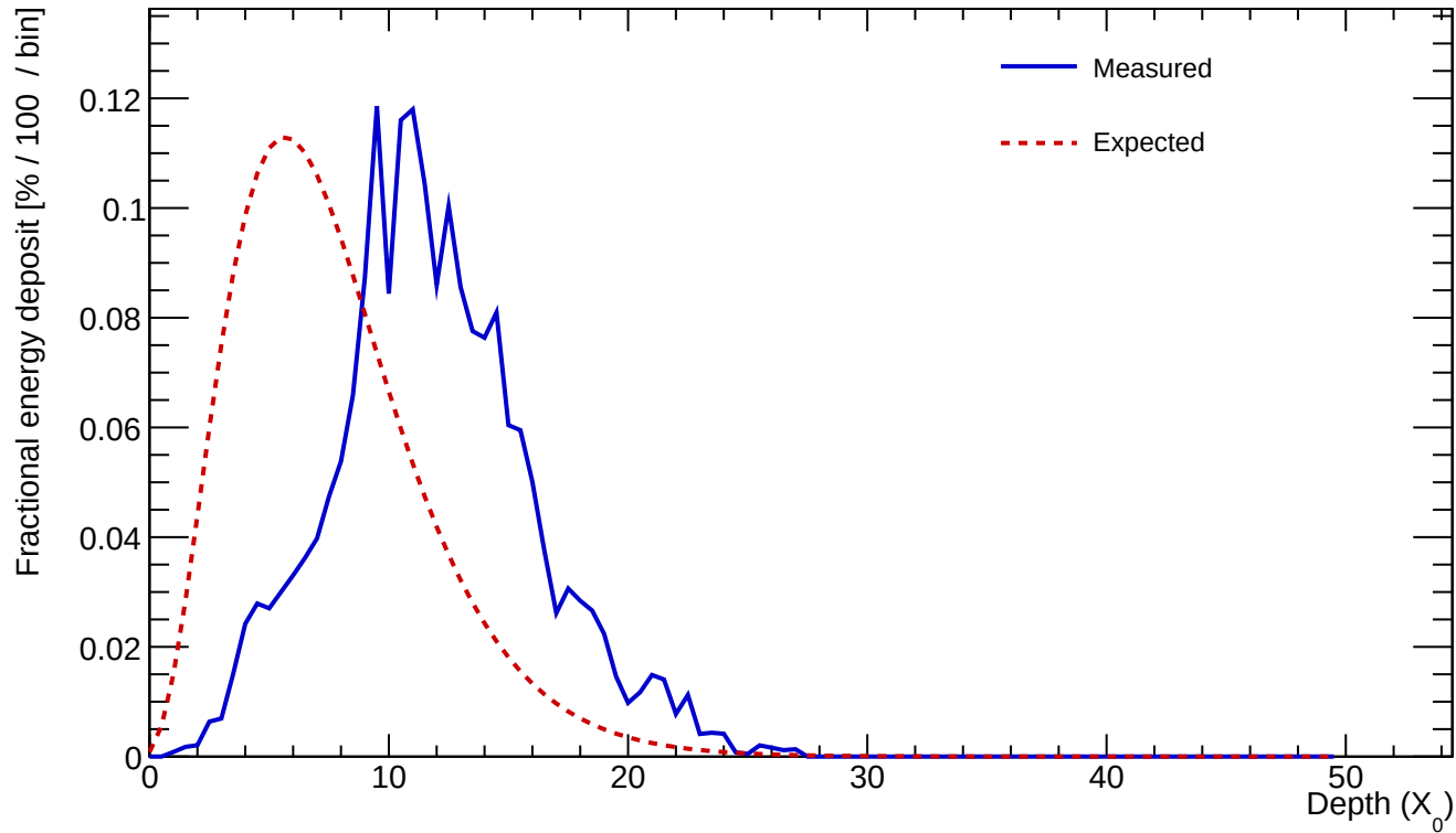
Cluster 93 E=22.795 GeV profileStart=5.00 X_0 \chi=0.2058
