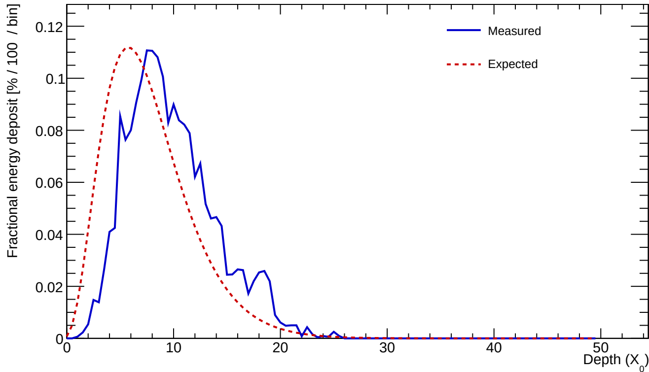
Cluster 534 E=25.142 GeV profileStart=2.00 X_0 \chi=0.1133
