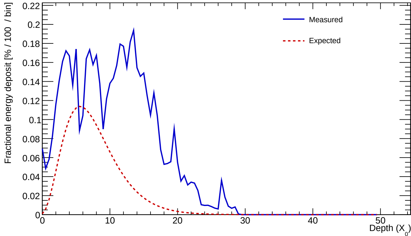
Cluster 514 E=21.378 GeV profileStart=4.00 X_0 \chi=0.5696
