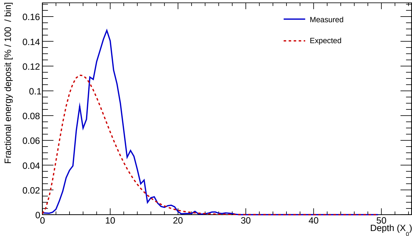
Cluster 401 E=23.330 GeV profileStart=2.00 X_0 \chi=0.2370
