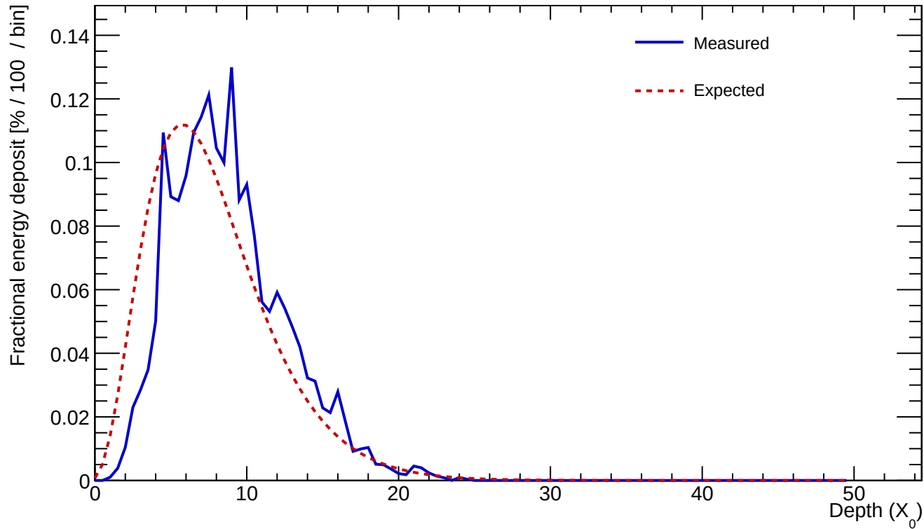
Cluster 496 E=24.879 GeV profileStart=1.50 X_0 \chi=0.1251
