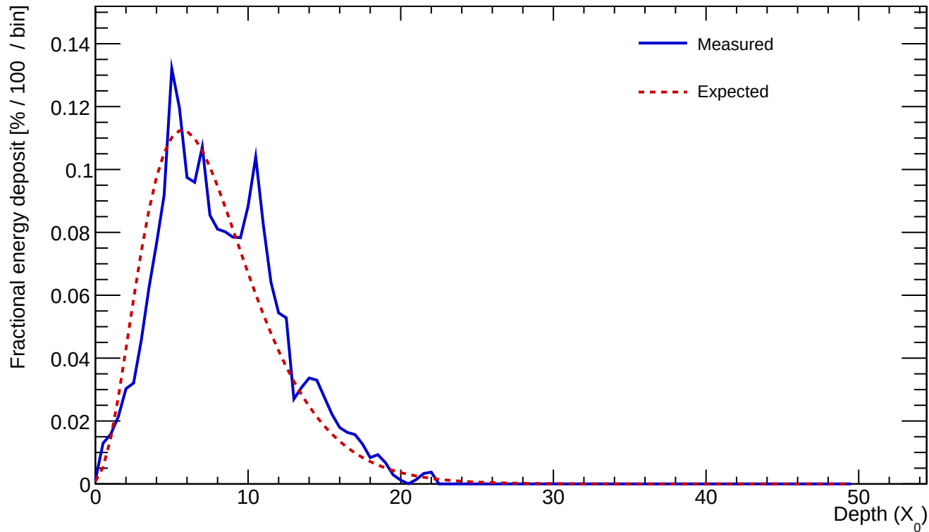
Cluster 140 E=23.807 GeV profileStart=1.00 X_0 \chi=0.1796
