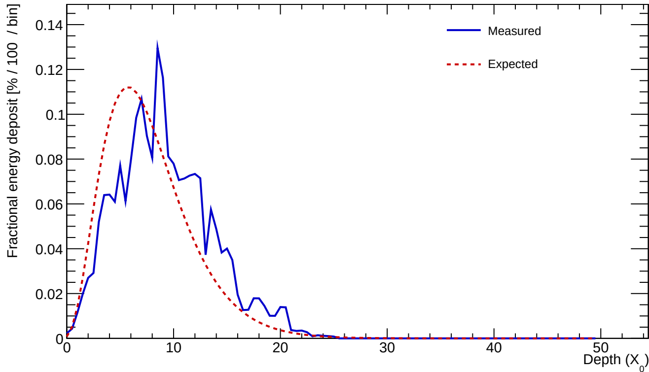
Cluster 170 E=24.462 GeV profileStart=1.50 X_0 \chi=0.2465
