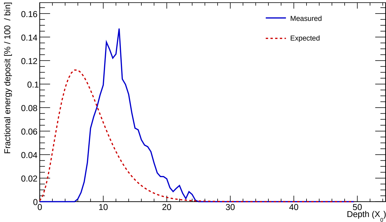
Cluster 318 E=24.526 GeV profileStart=5.50 X_0 \chi=0.1339
