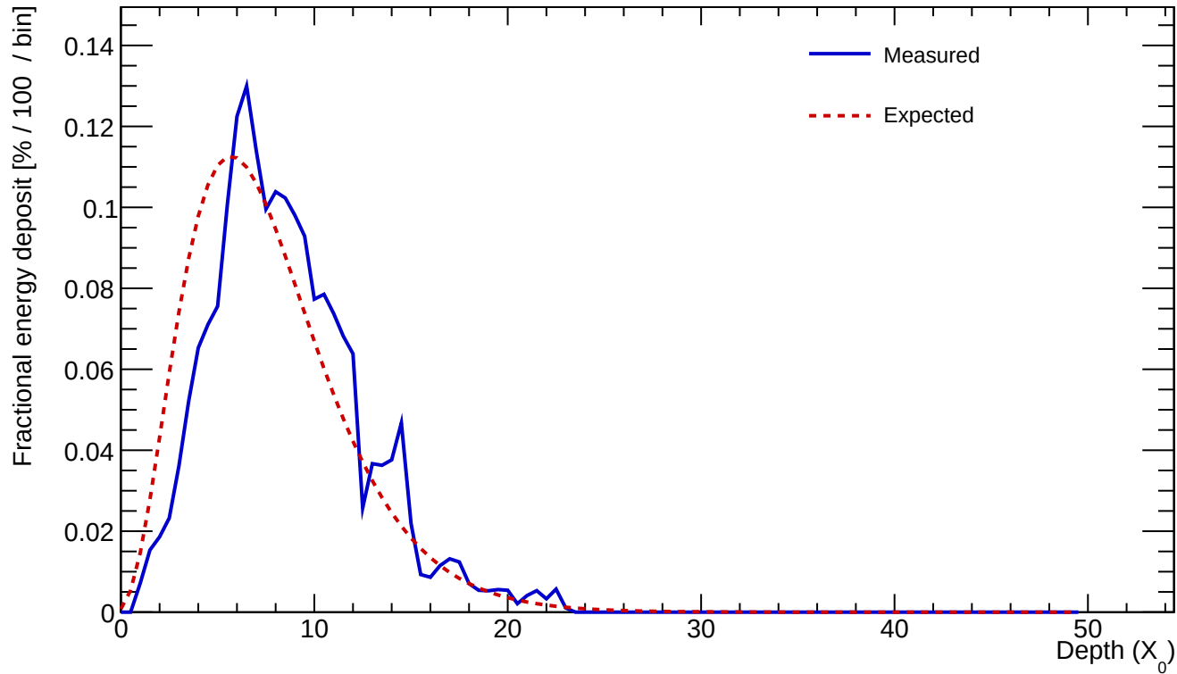
Cluster 58 E=23.538 GeV profileStart=1.00 X_0 \chi=0.1380
