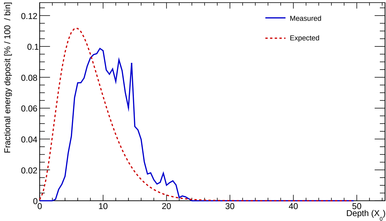
Cluster 114 E=25.130 GeV profileStart=3.00 X_0 \chi=0.1654
