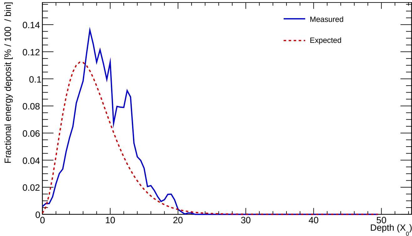
Cluster 127 E=23.953 GeV profileStart=1.50 X_0 \chi=0.1614
