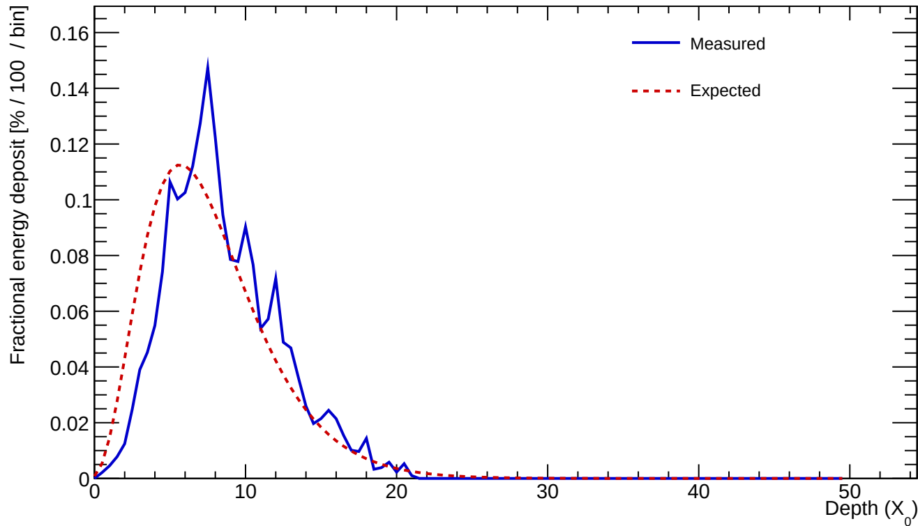
Cluster 277 E=23.676 GeV profileStart=1.00 X_0 \chi=0.1407
