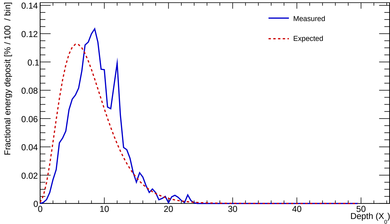
Cluster 630 E=23.502 GeV profileStart=1.50 X_0 \chi=0.1846
