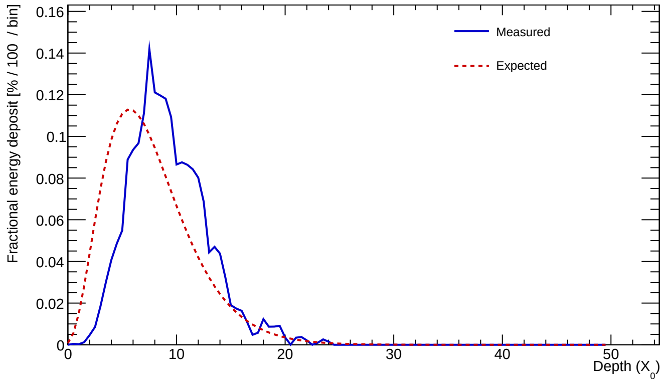
Cluster 84 E=22.970 GeV profileStart=2.00 X_0 \chi=0.1460
