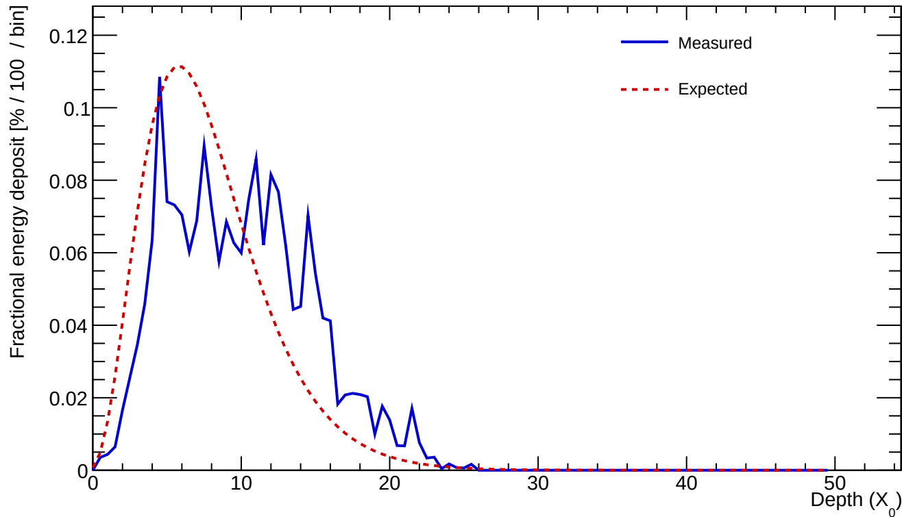
Cluster 664 E=26.021 GeV profileStart=1.50 X_0 \chi=0.3523
