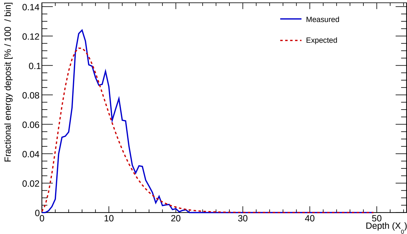
Cluster 408 E=24.971 GeV profileStart=1.00 X_0 \chi=0.1483
