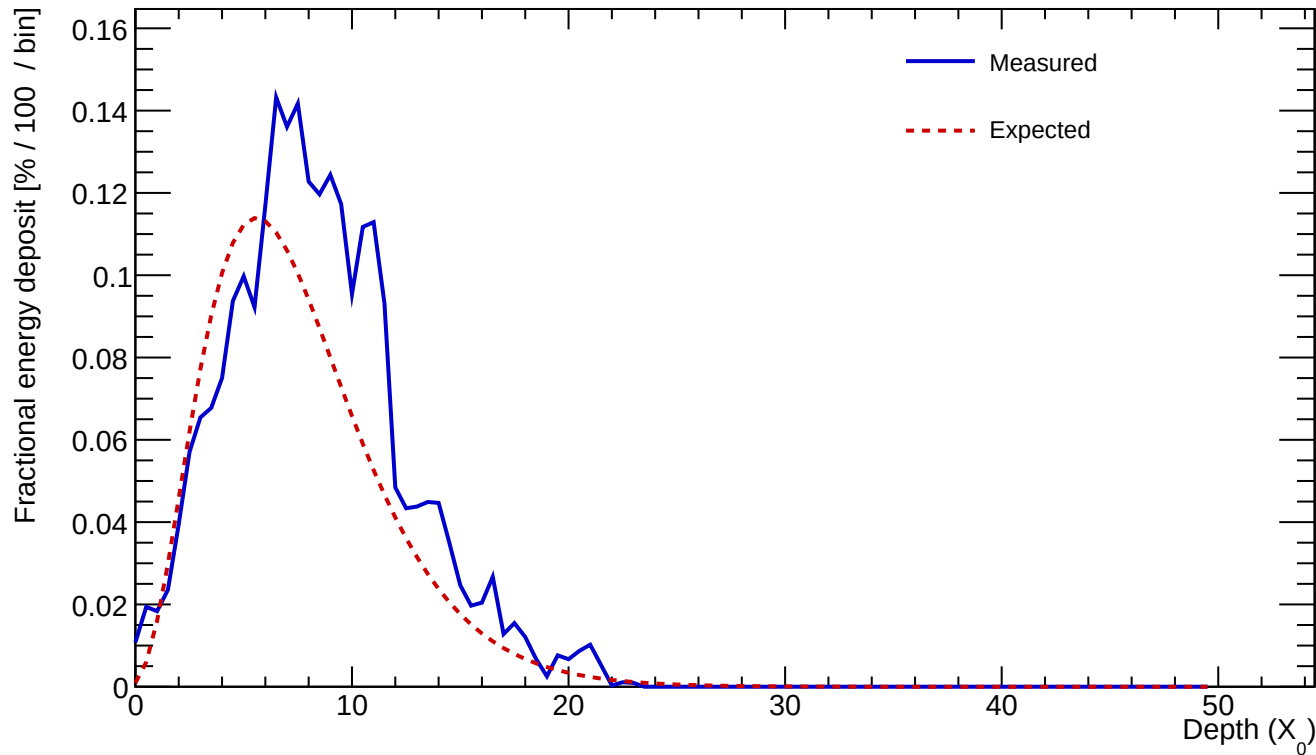
Cluster 357 E=21.217 GeV profileStart=1.00 X_0 \chi=0.1825
