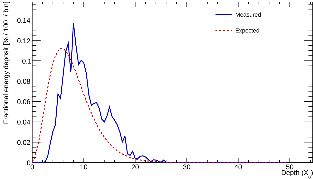
Cluster 274 E=24.555 GeV profileStart=2.50 X_0 \chi=0.1668
