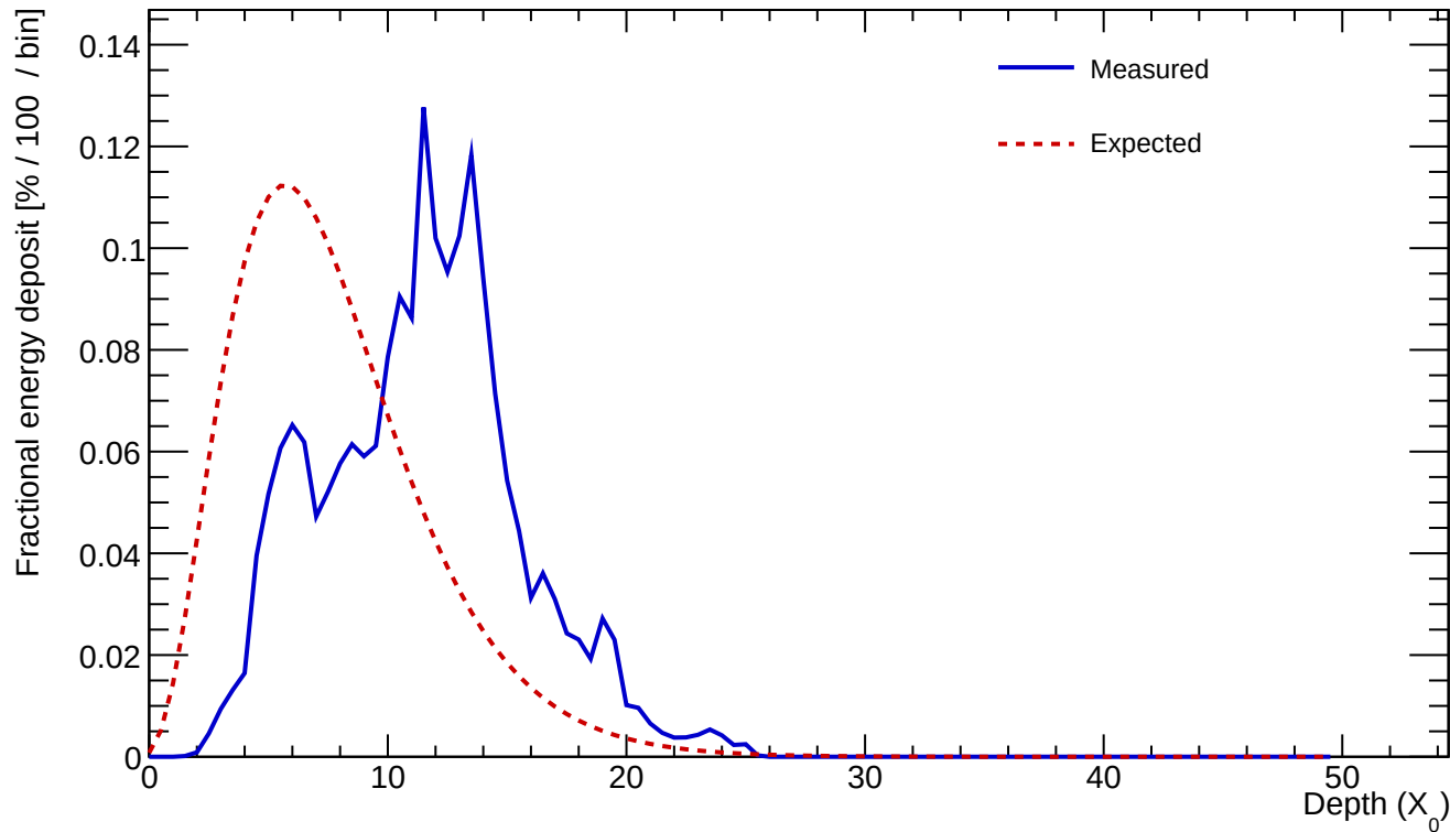
Cluster 377 E=23.976 GeV profileStart=4.00 X_0 \chi=0.3467
