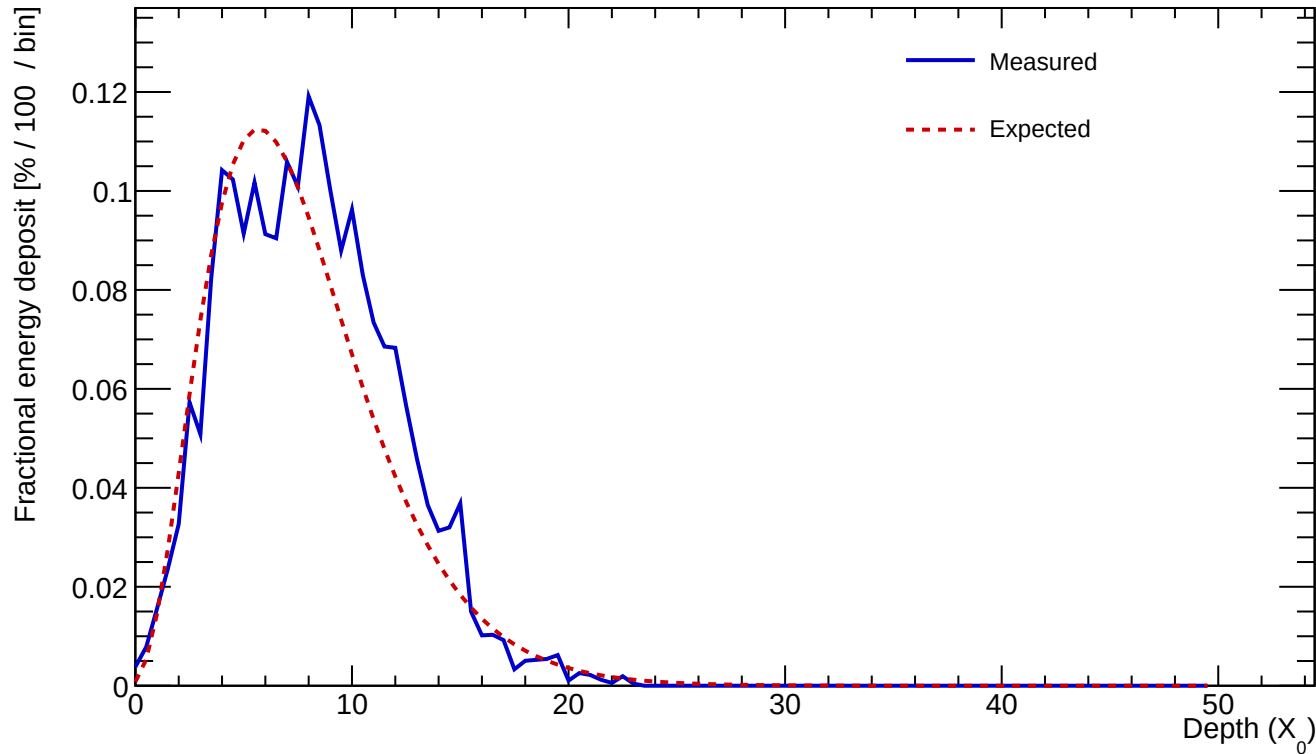
Cluster 657 E=23.730 GeV profileStart=0.50 X_0 \chi=0.1688
