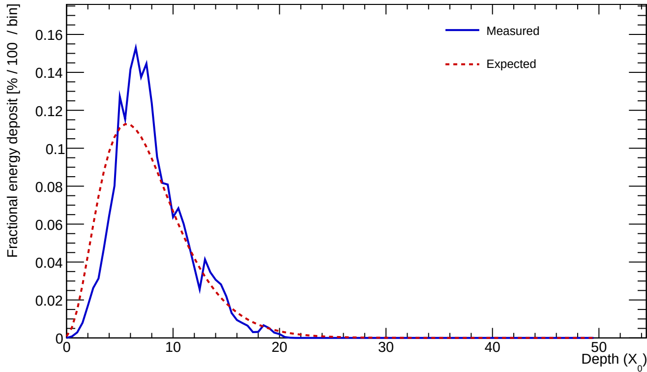
Cluster 8 E=23.171 GeV profileStart=1.00 X_0 \chi=0.2008
