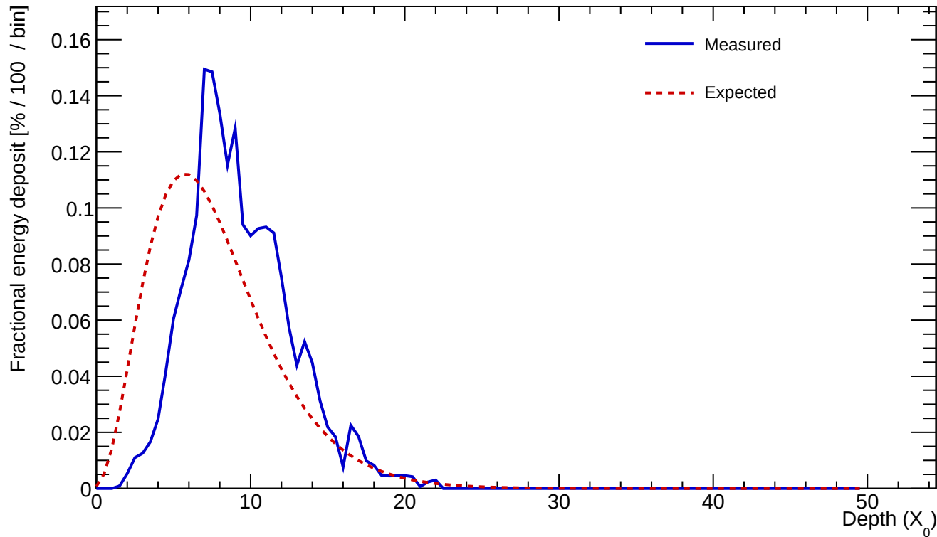
Cluster 121 E=24.414 GeV profileStart=2.50 X_0 \chi=0.1791
