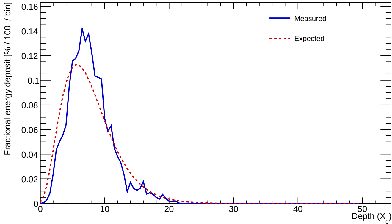
Cluster 315 E=23.563 GeV profileStart=0.50 X_0 \chi=0.1987
