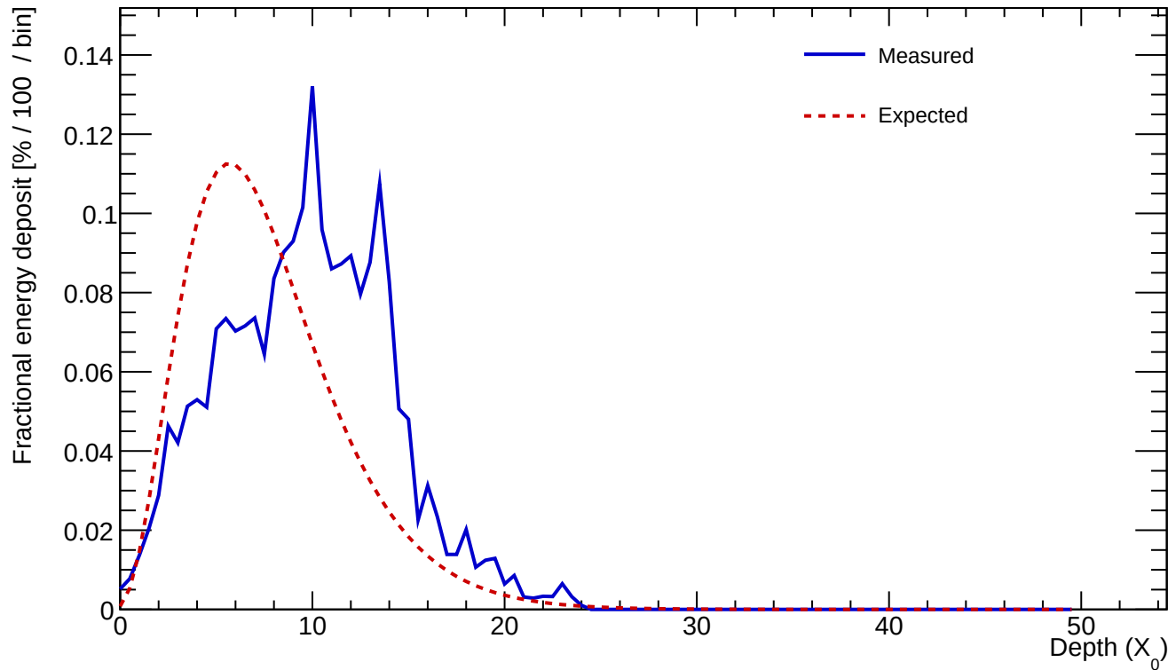
Cluster 672 E=23.613 GeV profileStart=2.50 X_0 \chi=0.3273
