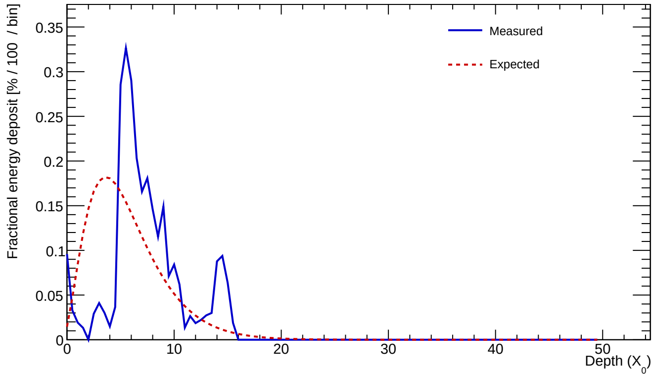
Cluster 300 E=2.968 GeV profileStart=2.50 X_0 \chi=0.4997
