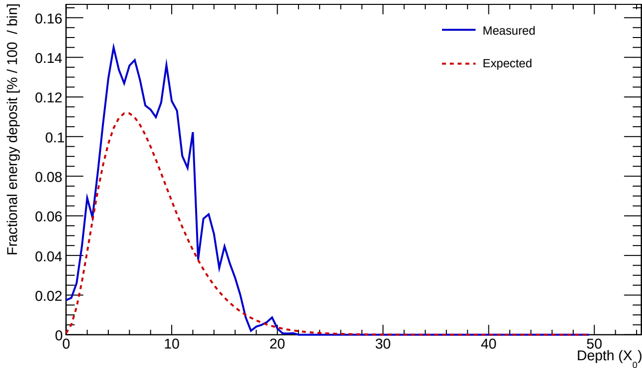
Cluster 594 E=24.913 GeV profileStart=0.50 X_0 \chi=0.1964
