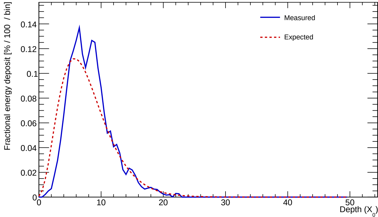
Cluster 119 E=24.929 GeV profileStart=1.00 X_0 \chi=0.1819
