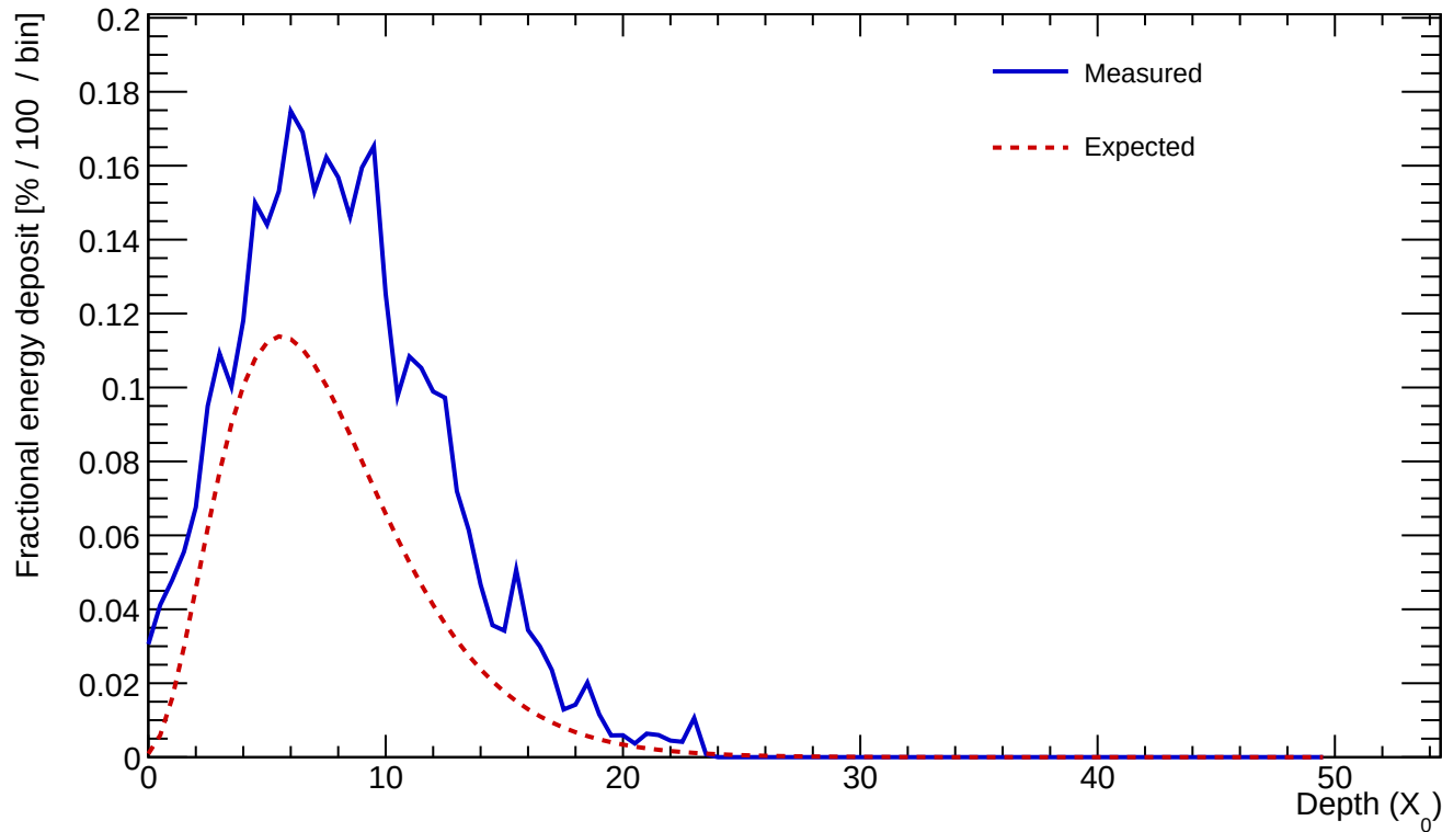
Cluster 506 E=21.310 GeV profileStart=0.50 X_0 \chi=0.1983
