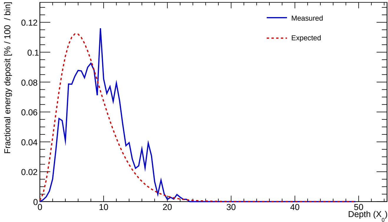
Cluster 13 E=23.990 GeV profileStart=1.50 X_0 \chi=0.2232
