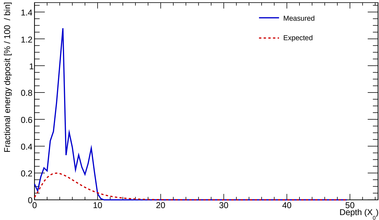
Cluster 539 E=2.553 GeV profileStart=0.50 X_0 \chi=0.3439
