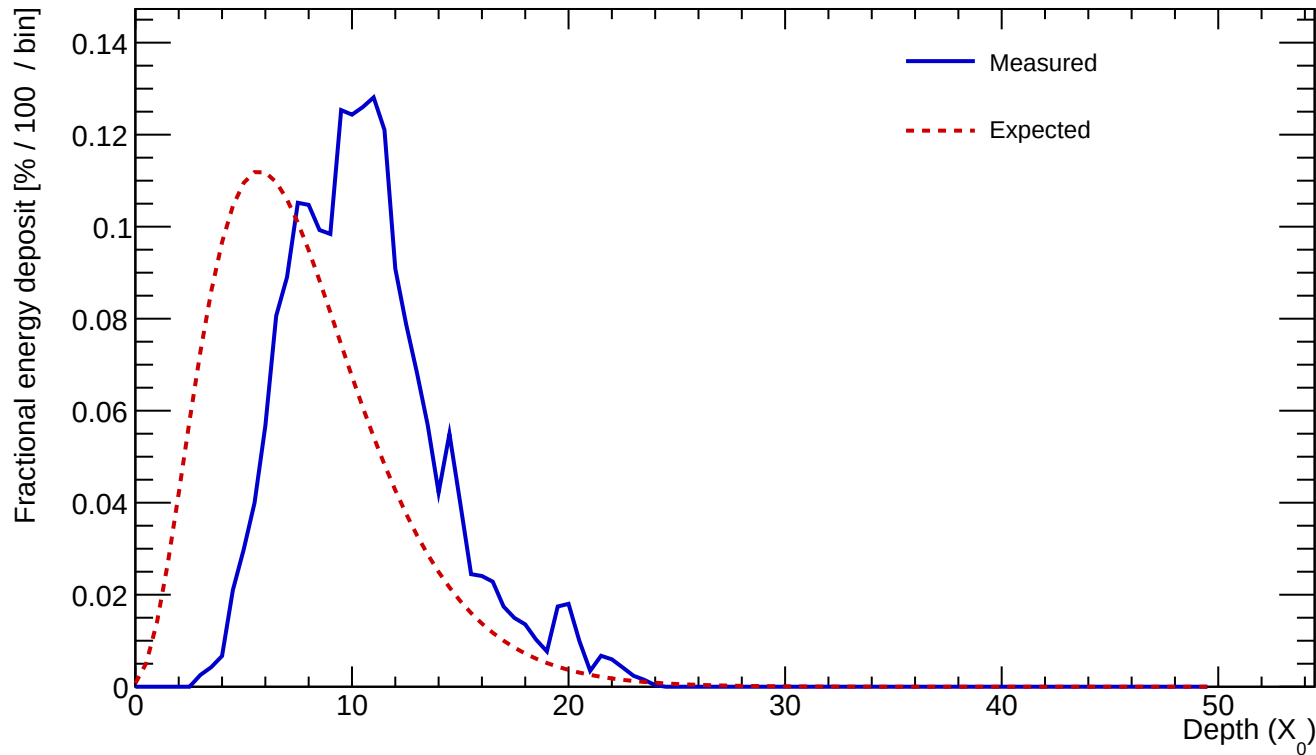
Cluster 647 E=24.703 GeV profileStart=3.50 X_0 \chi=0.1638
