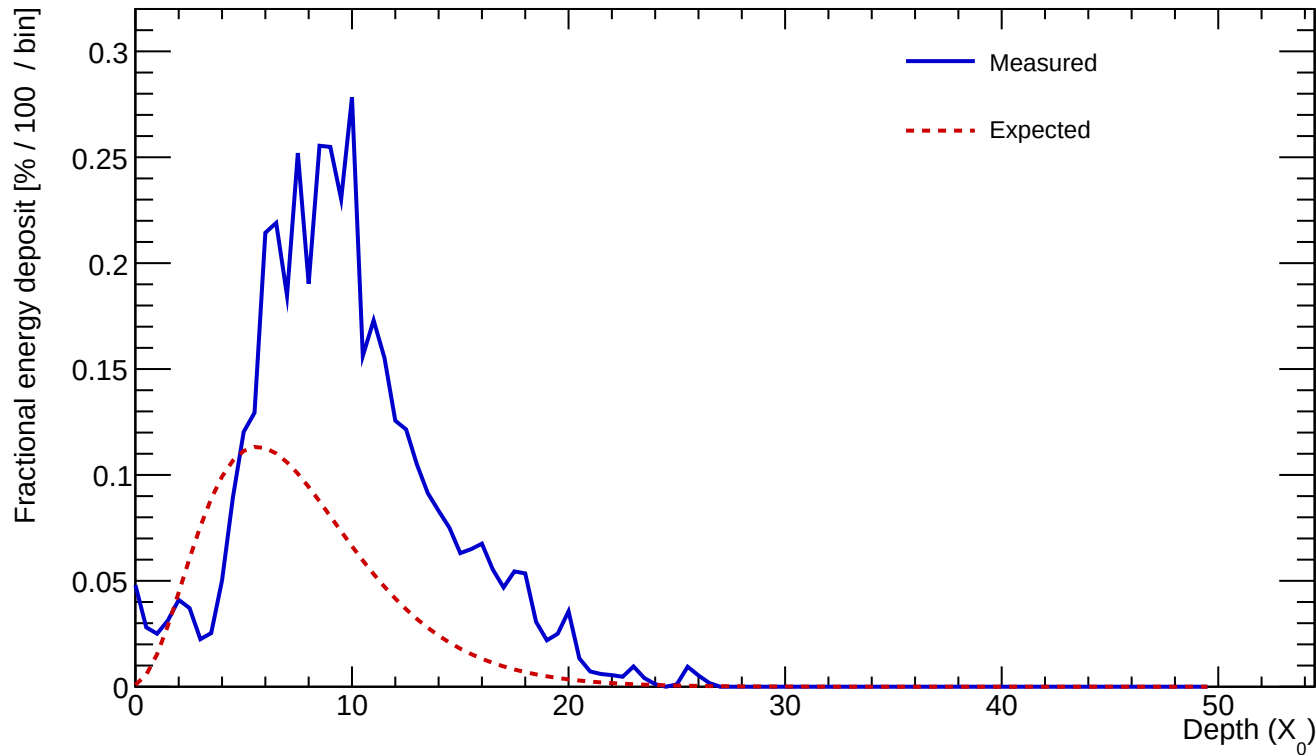
Cluster 603 E=22.323 GeV profileStart=2.50 X_0 \chi=0.1983
