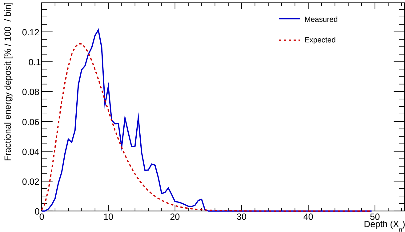
Cluster 595 E=24.397 GeV profileStart=2.00 X_0 \chi=0.1723
