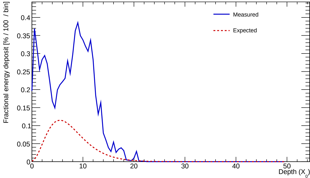
Cluster 463 E=19.530 GeV profileStart=0.50 X_0 \chi=0.5121
