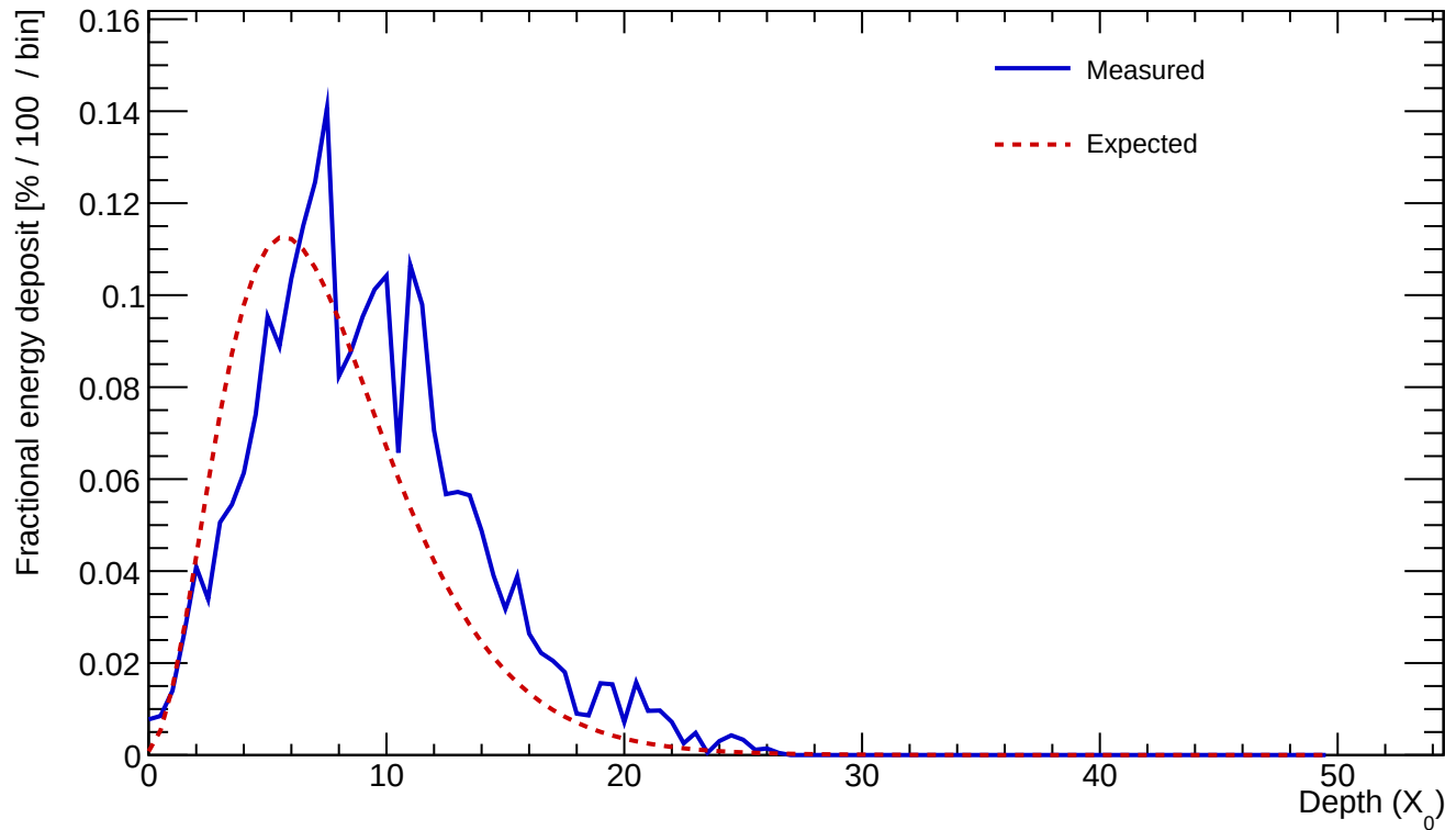
Cluster 691 E=23.523 GeV profileStart=1.50 X_0 \chi=0.2145
