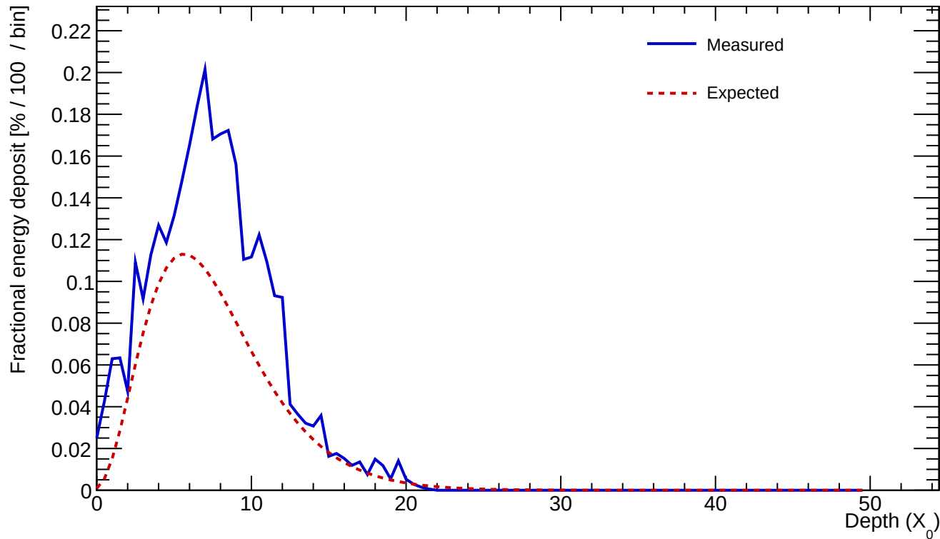
Cluster 261 E=22.646 GeV profileStart=0.50 X_0 \chi=0.2054
