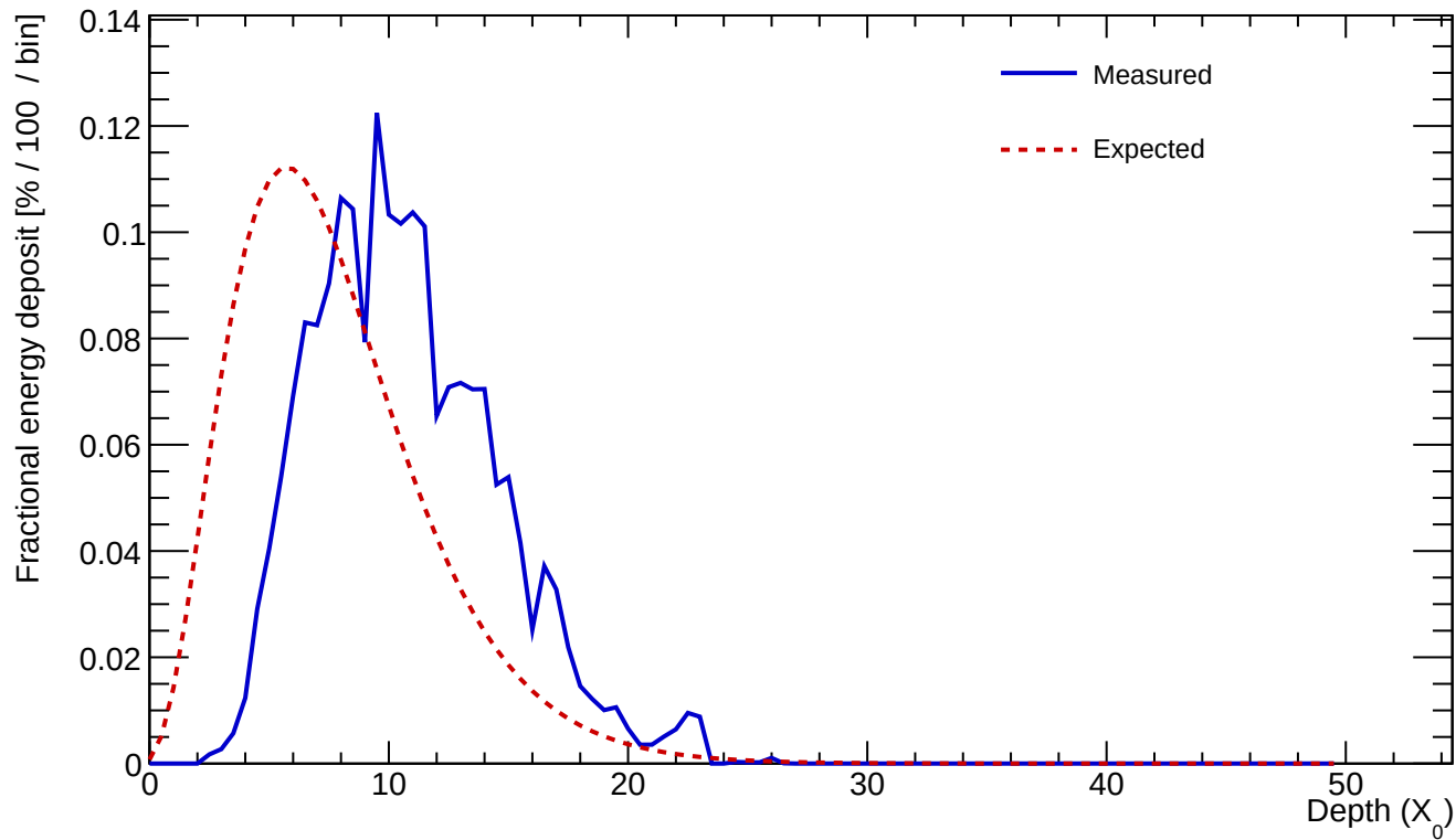
Cluster 12 E=24.385 GeV profileStart=3.00 X_0 \chi=0.1329
