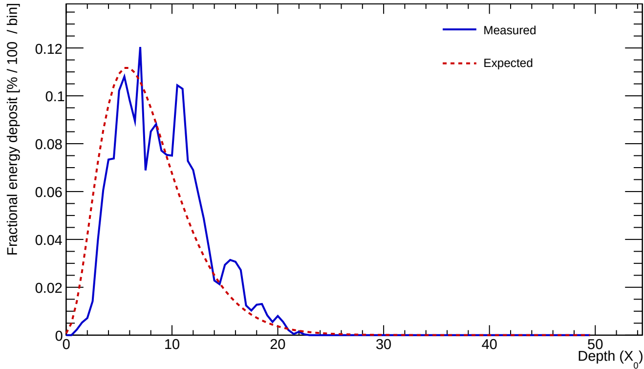
Cluster 458 E=25.086 GeV profileStart=1.00 X_0 \chi=0.1921
