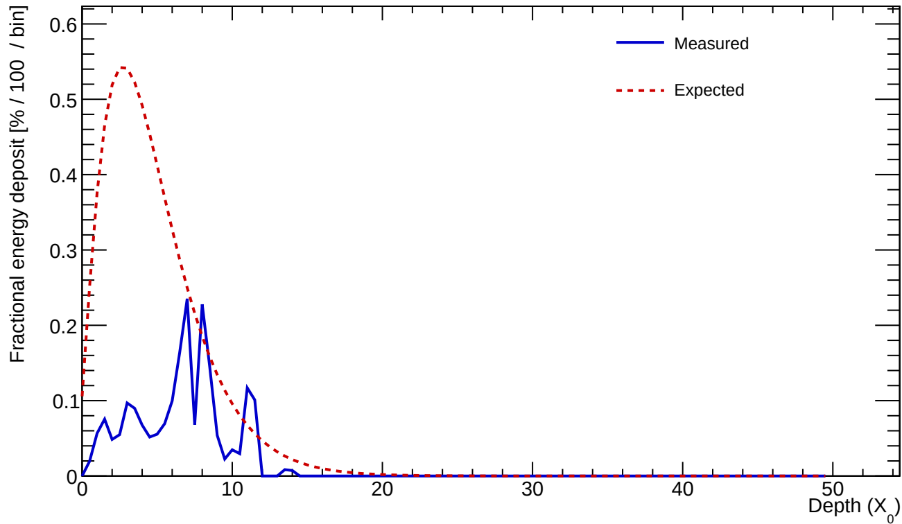
Cluster 29 E=1.215 GeV profileStart=2.00 X_0 \chi=0.6539
