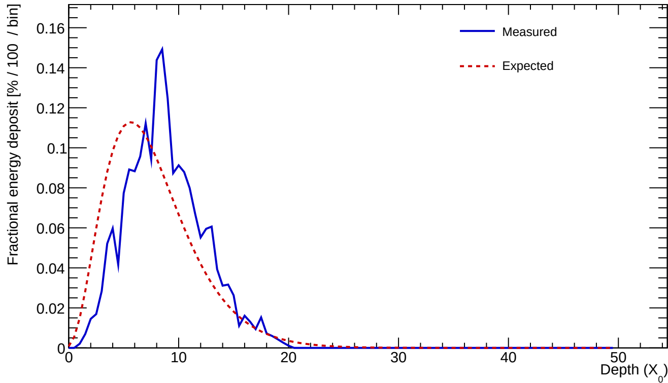
Cluster 688 E=22.972 GeV profileStart=1.50 X_0 \chi=0.1694
