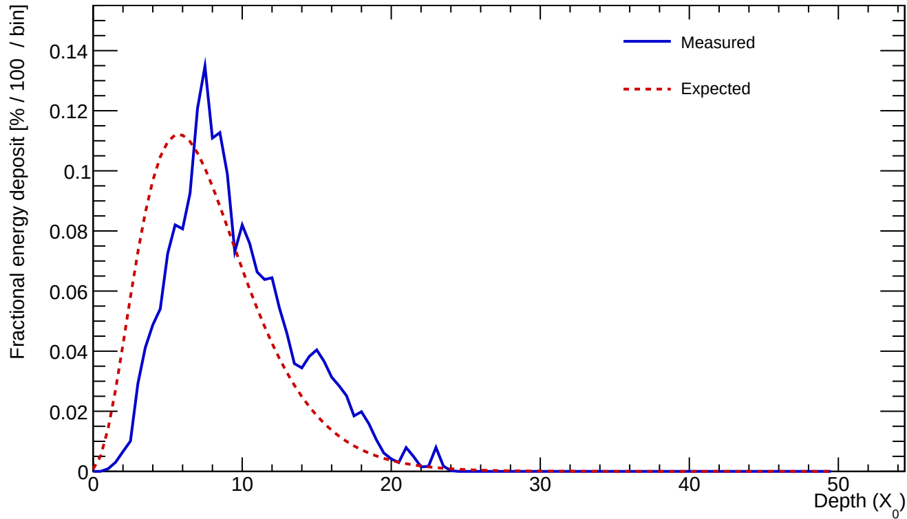
Cluster 37 E=24.508 GeV profileStart=1.50 X_0 \chi=0.1502
