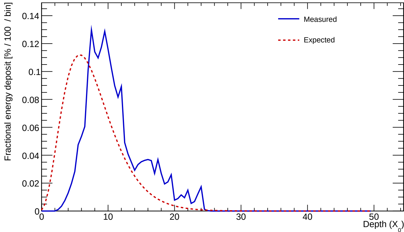
Cluster 258 E=24.980 GeV profileStart=3.00 X_0 \chi=0.2067
