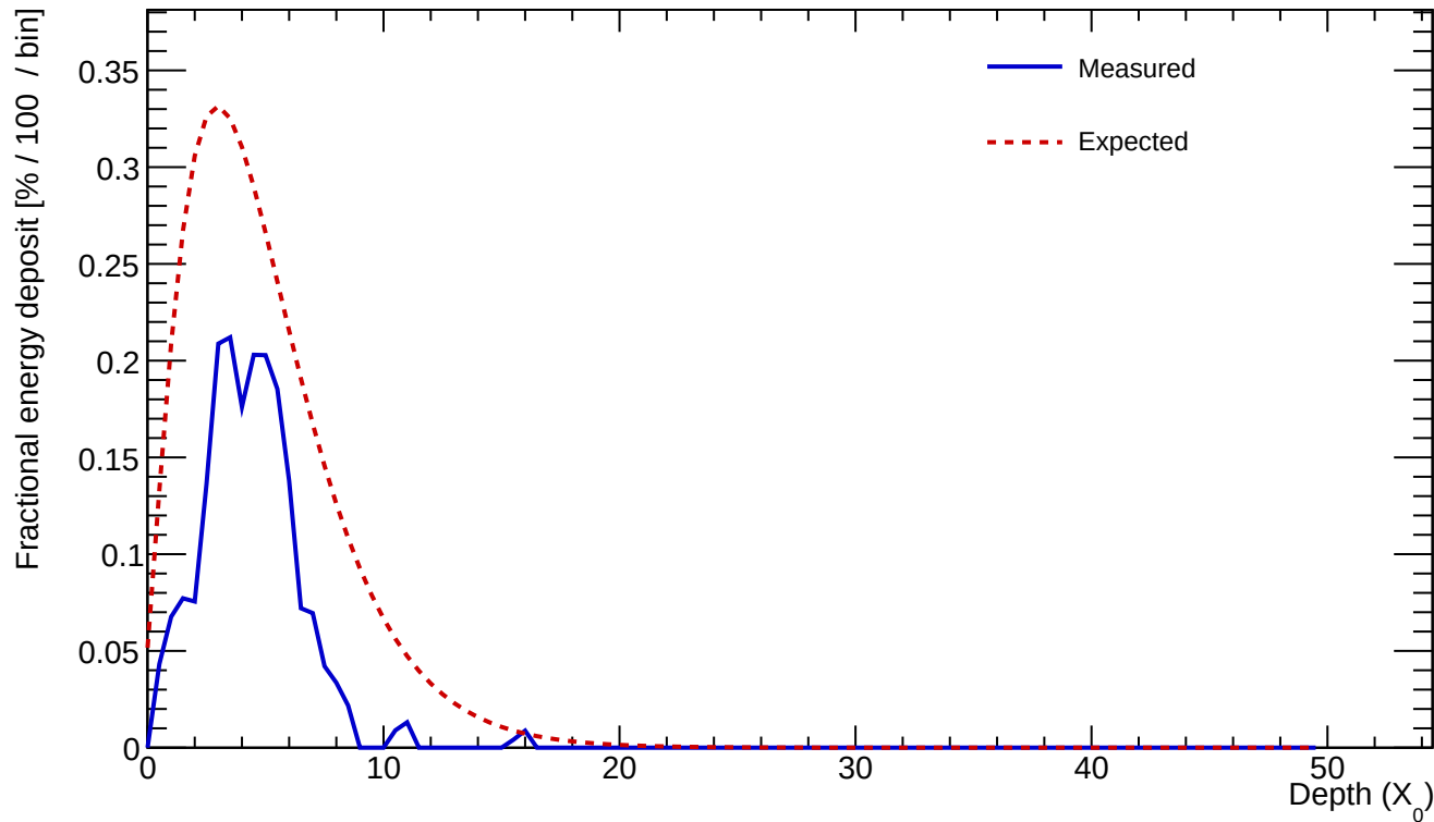
Cluster 566 E=1.533 GeV profileStart=0.50 X_0 \chi=0.4407
