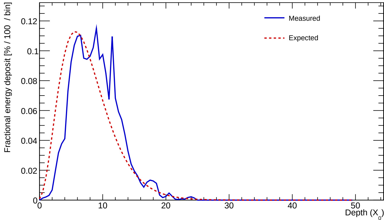
Cluster 305 E=23.068 GeV profileStart=1.50 X_0 \chi=0.1456
