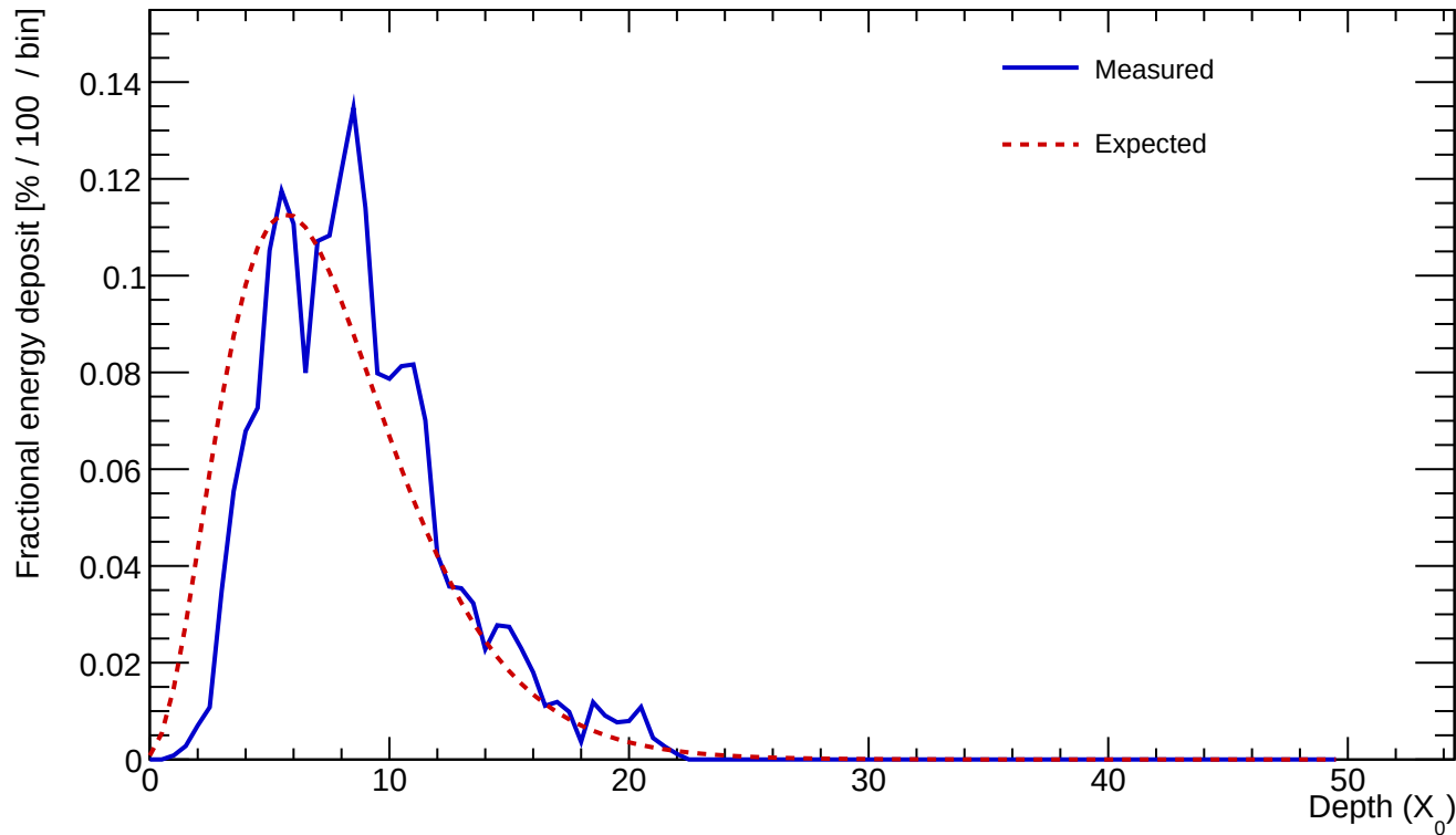
Cluster 663 E=23.313 GeV profileStart=1.00 X_0 \chi=0.1552
