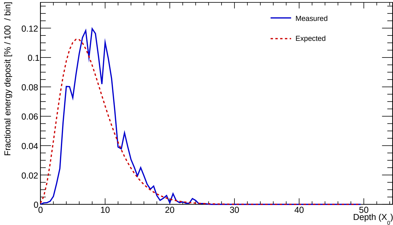
Cluster 208 E=23.748 GeV profileStart=1.50 X_0 \chi=0.1499
