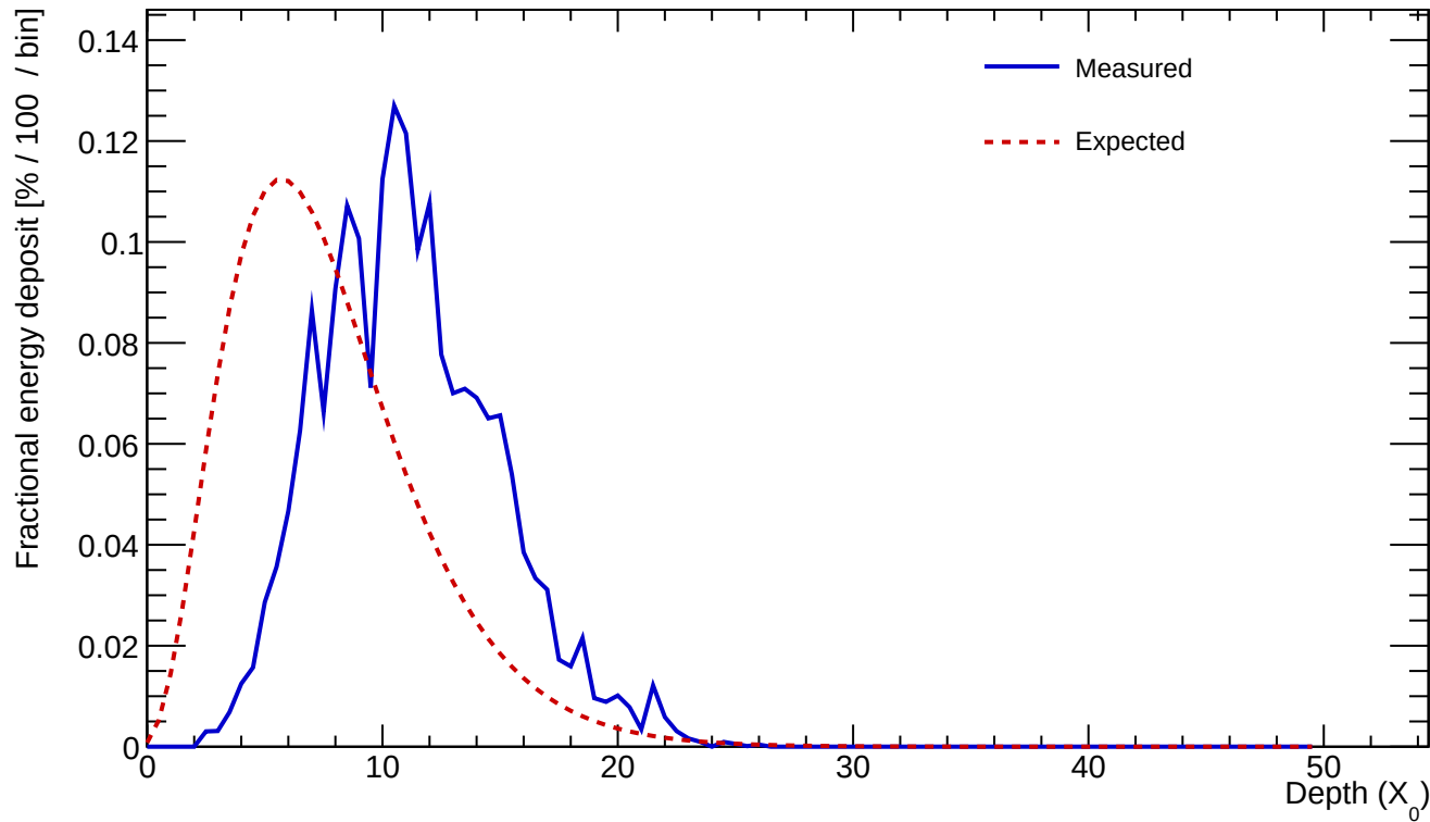
Cluster 387 E=23.920 GeV profileStart=4.00 X_0 \chi=0.1690
