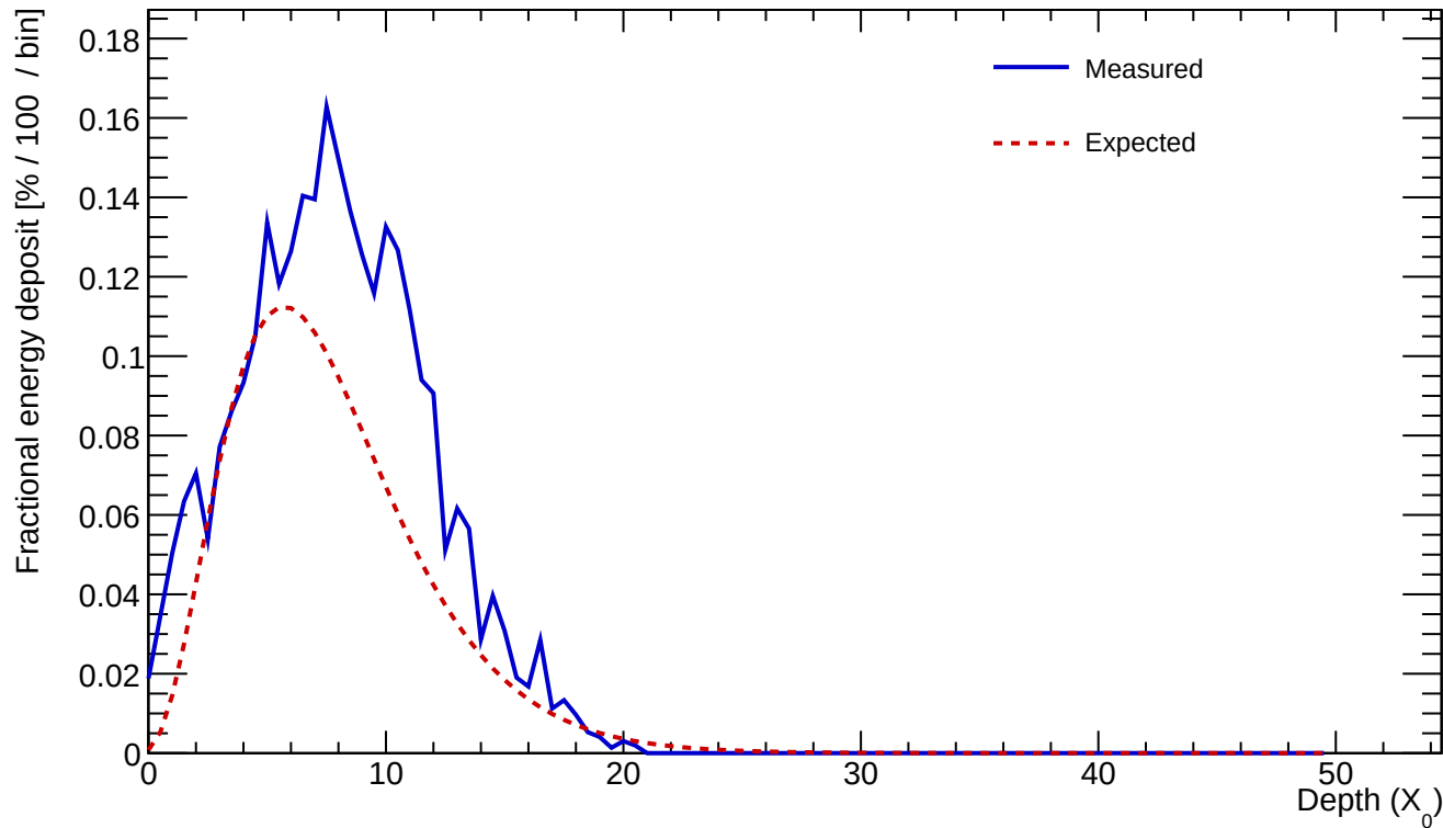
Cluster 402 E=23.881 GeV profileStart=1.00 X_0 \chi=0.2079
