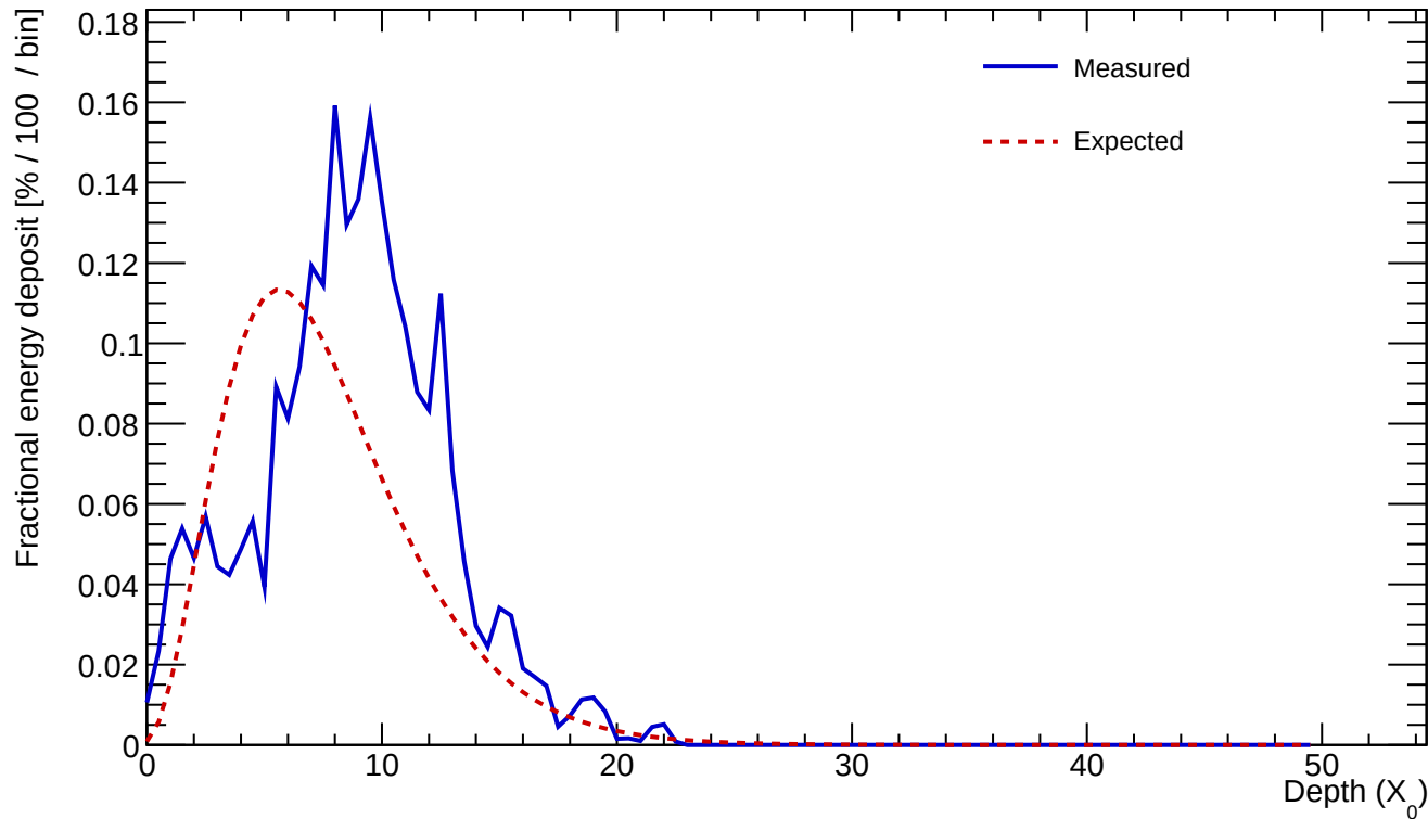
Cluster 650 E=22.113 GeV profileStart=2.00 X_0 \chi=0.3016
