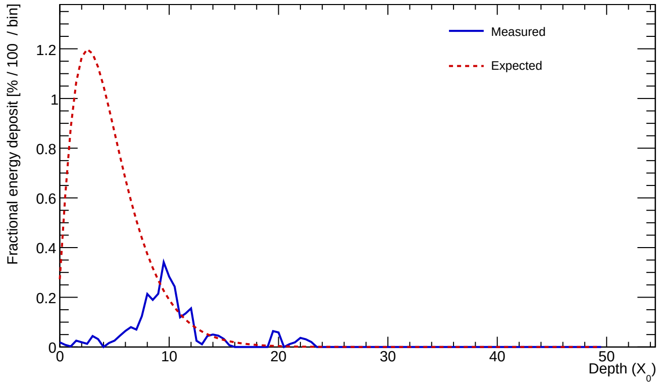
Cluster 348 E=1.021 GeV profileStart=6.00 X_0 \chi=0.5174
