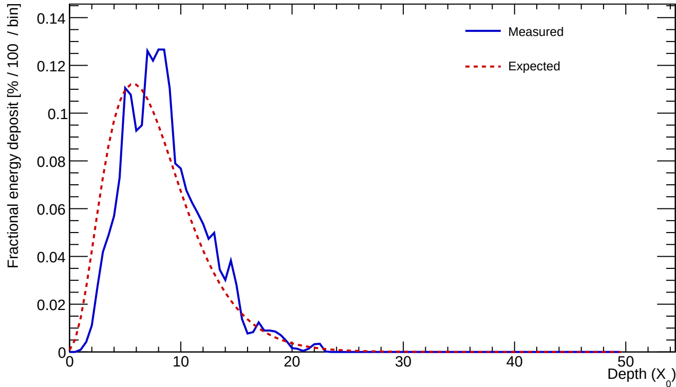
Cluster 680 E=24.372 GeV profileStart=1.00 X_0 \chi=0.1399
