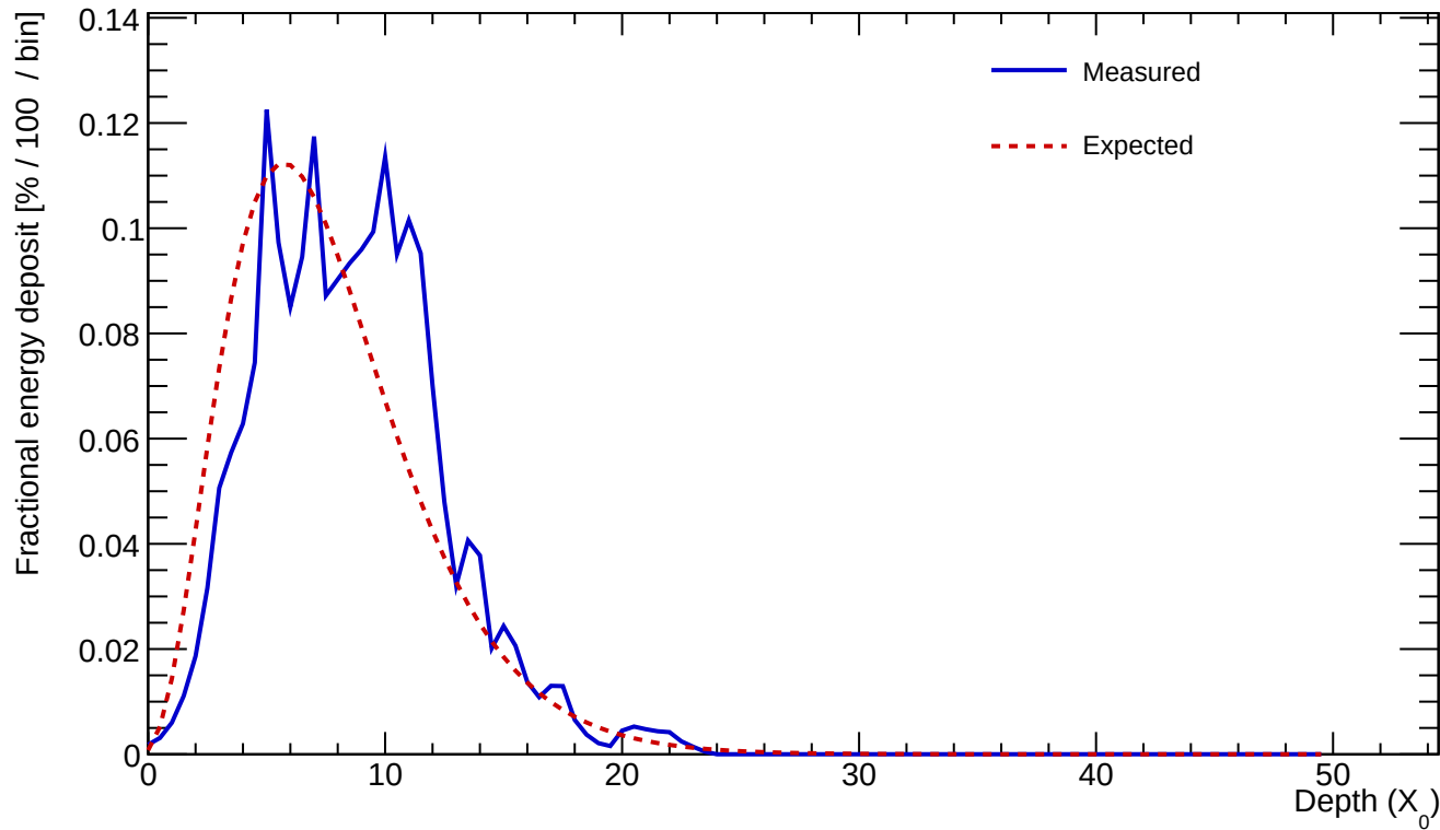
Cluster 194 E=24.143 GeV profileStart=1.00 X_0 \chi=0.1939
