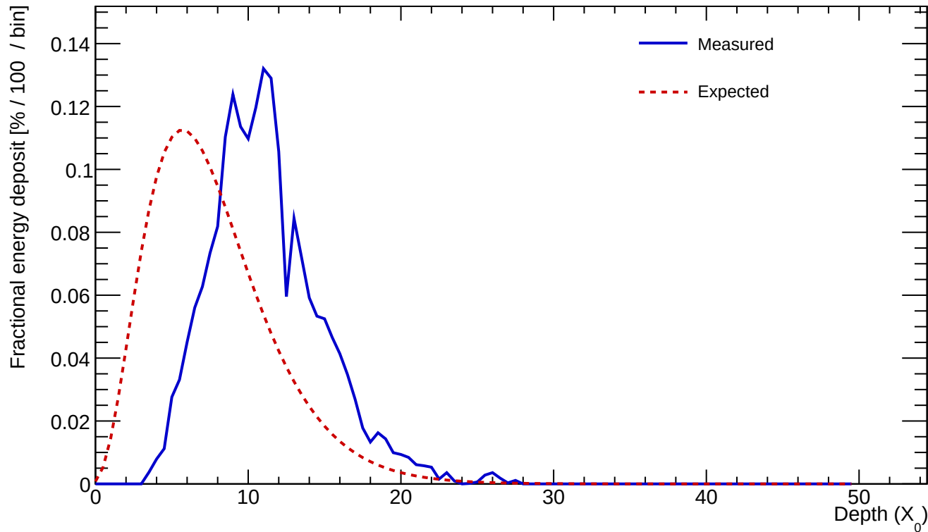
Cluster 397 E=23.723 GeV profileStart=4.00 X_0 \chi=0.1540
