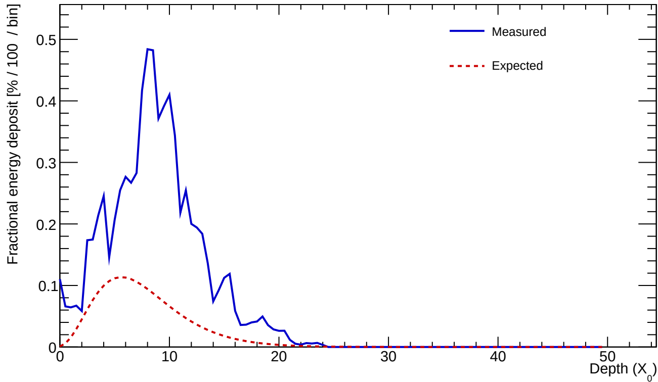
Cluster 557 E=21.902 GeV profileStart=1.50 X_0 \chi=0.2774
