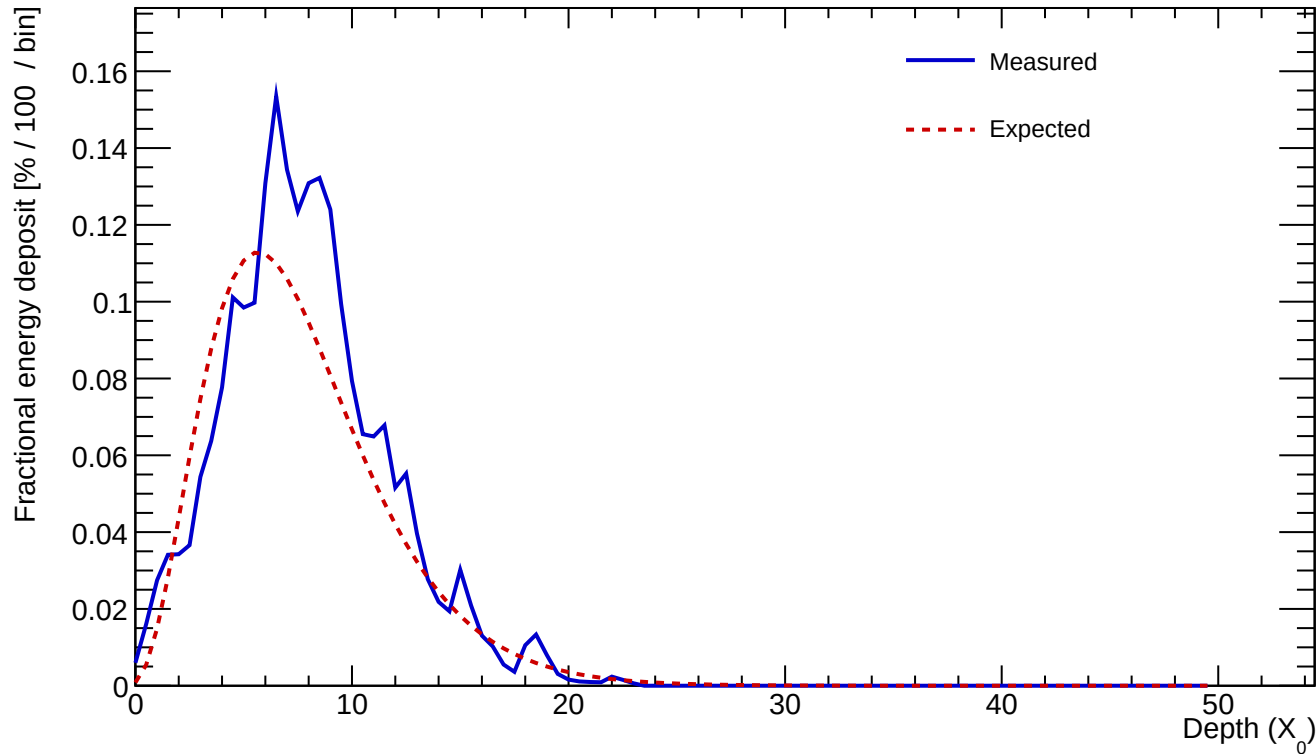
Cluster 104 E=23.134 GeV profileStart=1.00 X_0 \chi=0.1728
