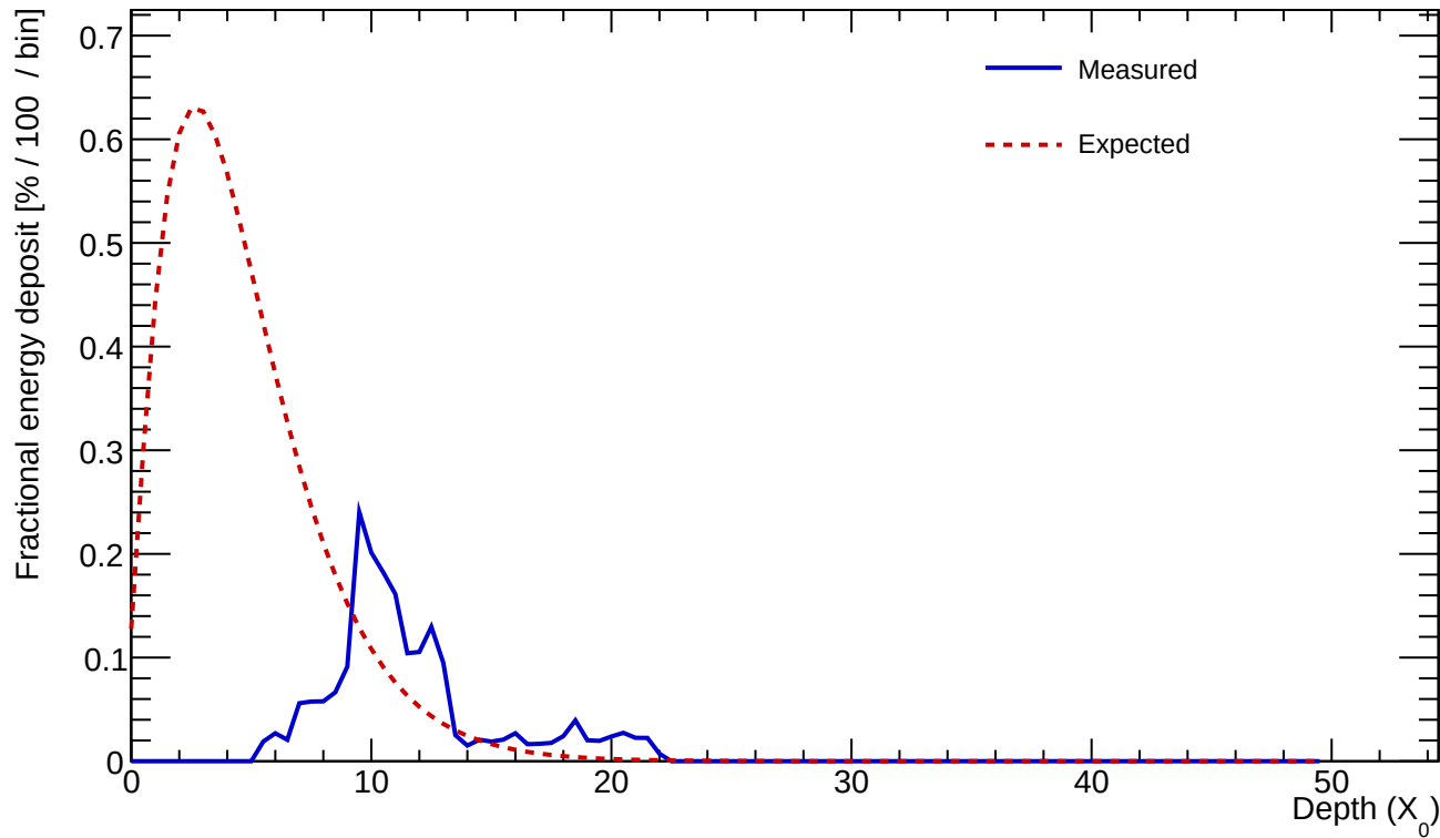
Cluster 66 E=1.160 GeV profileStart=7.00 X_0 \chi=0.4445
