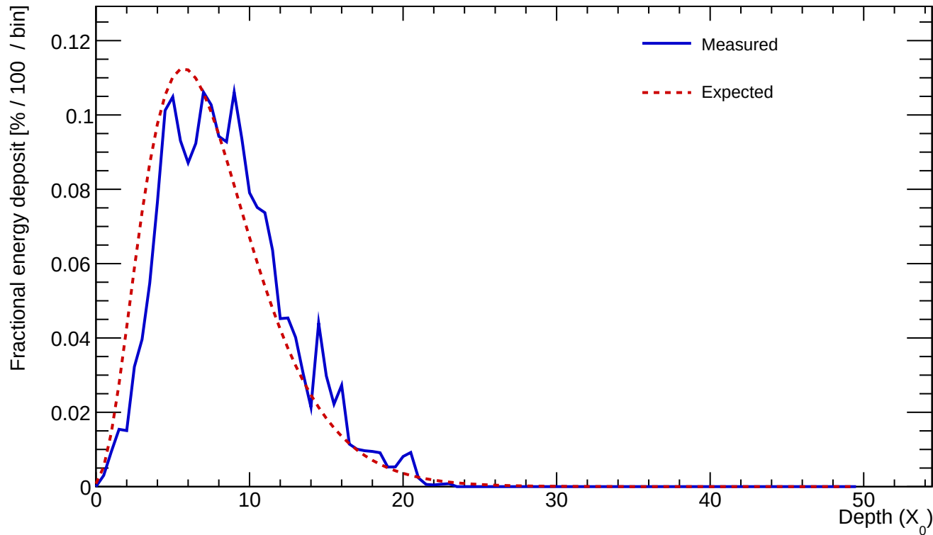
Cluster 254 E=23.796 GeV profileStart=1.00 X_0 \chi=0.1295
