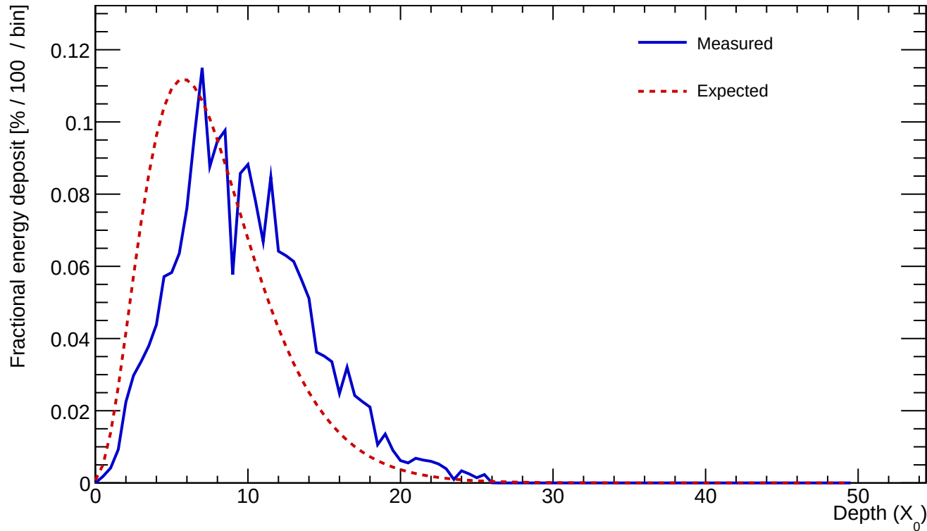
Cluster 427 E=25.125 GeV profileStart=2.00 X_0 \chi=0.1997
