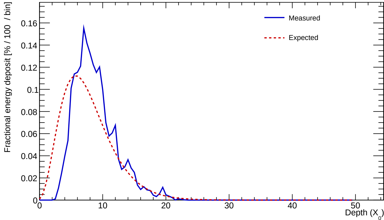
Cluster 306 E=24.242 GeV profileStart=1.50 X_0 \chi=0.2445
