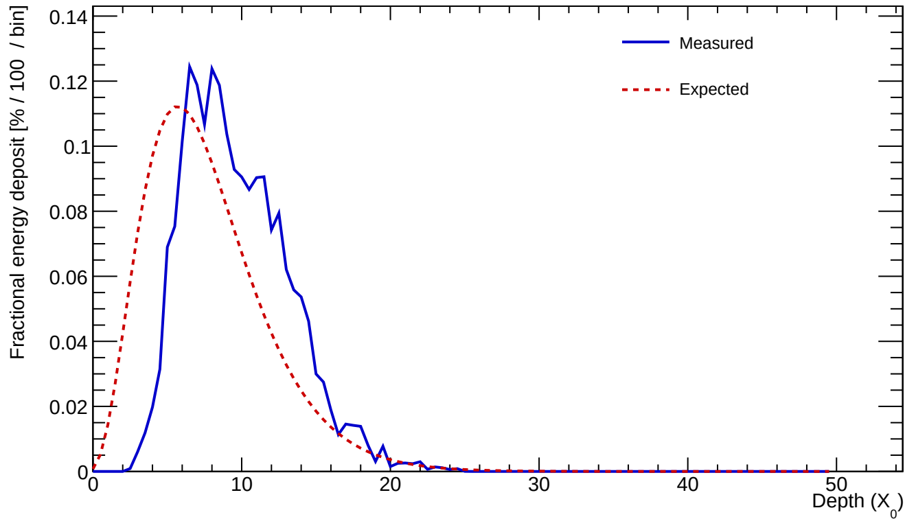
Cluster 409 E=24.285 GeV profileStart=2.50 X_0 \chi=0.1427
