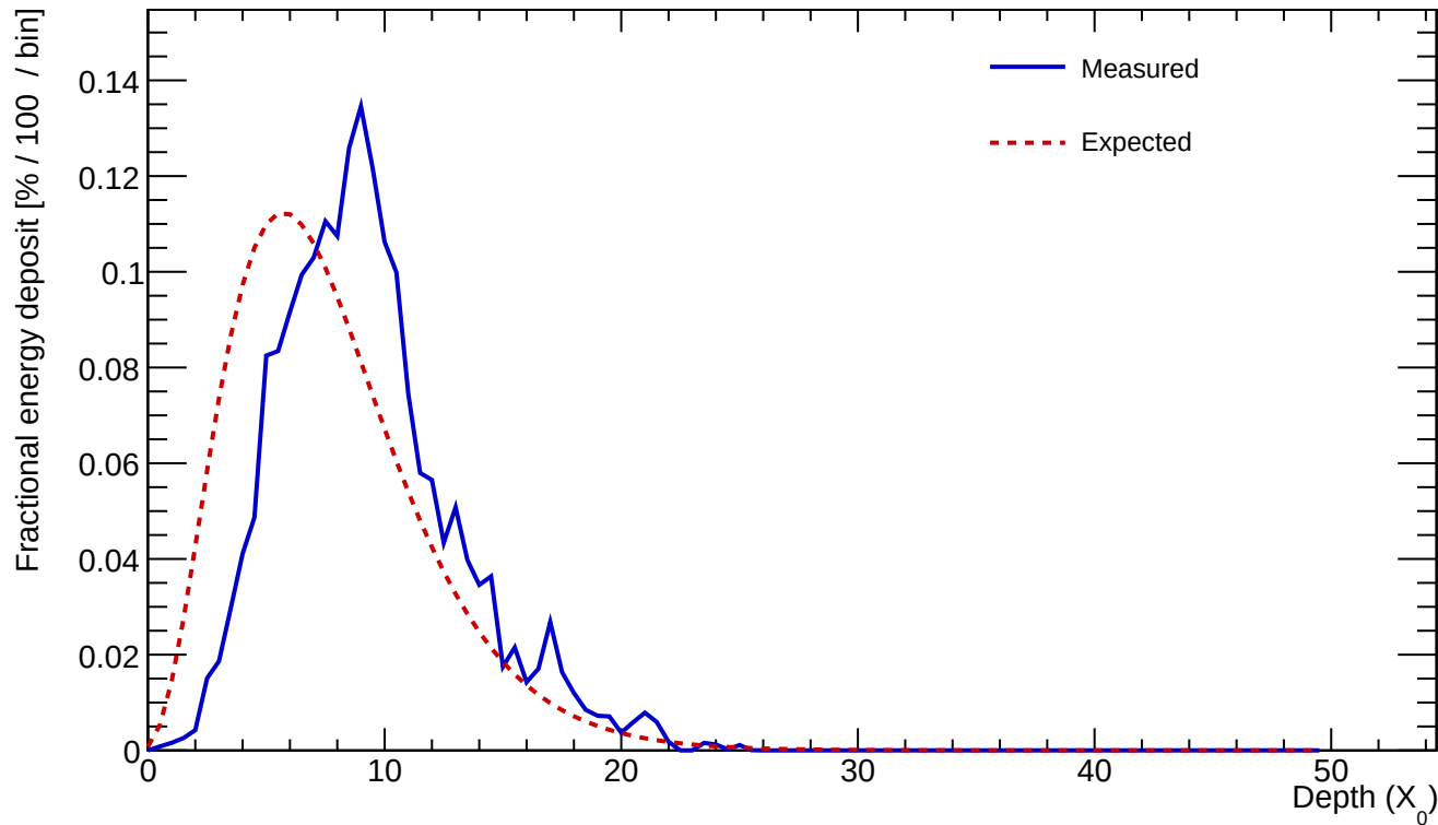
Cluster 581 E=24.091 GeV profileStart=2.00 X_0 \chi=0.1461
