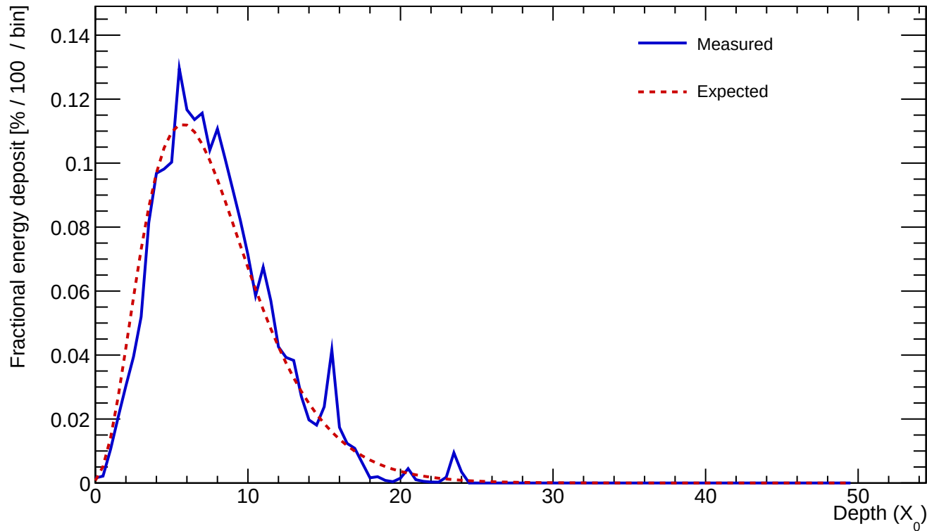
Cluster 349 E=24.468 GeV profileStart=0.50 X_0 \chi=0.1083
