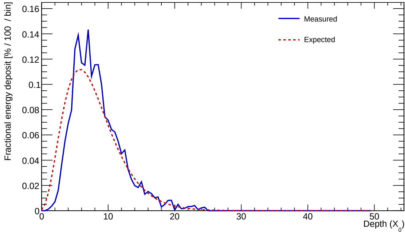
Cluster 693 E=25.167 GeV profileStart=1.00 X_0 \chi=0.1629
