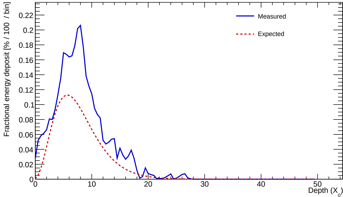
Cluster 220 E=23.146 GeV profileStart=0.50 X_0 \chi=0.2115
