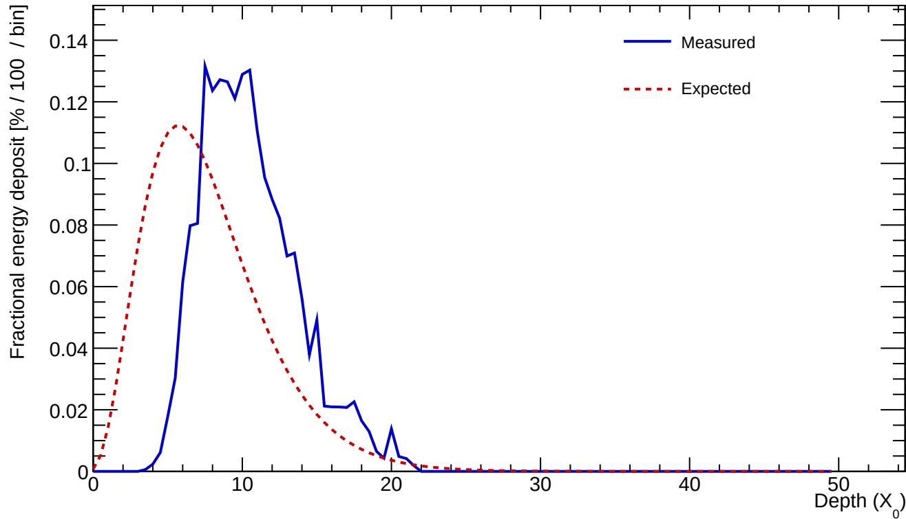
Cluster 633 E=24.188 GeV profileStart=3.50 X_0 \chi=0.1708
