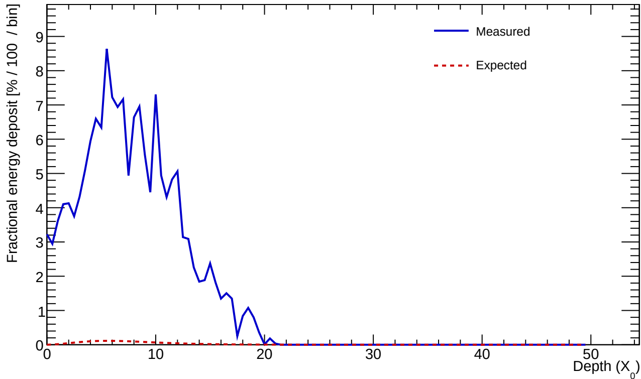
Cluster 116 E=21.382 GeV profileStart=0.50 X_0 \chi=0.2649
