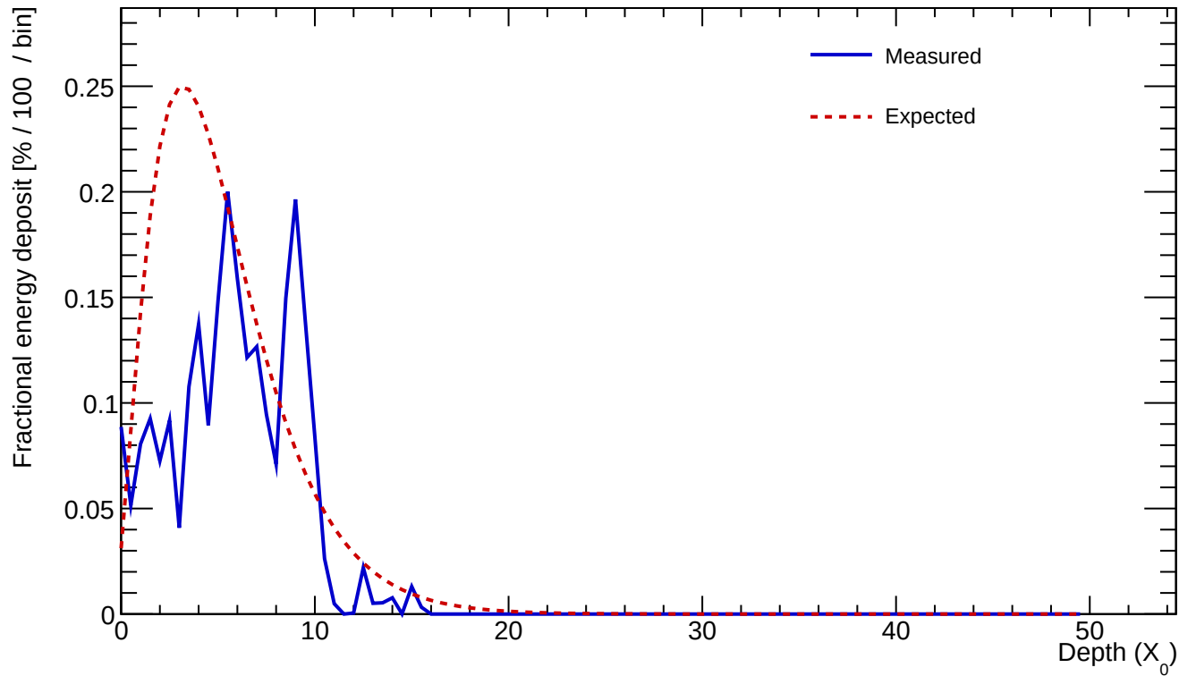
Cluster 437 E=1.924 GeV profileStart=0.50 X_0 \chi=0.4728
