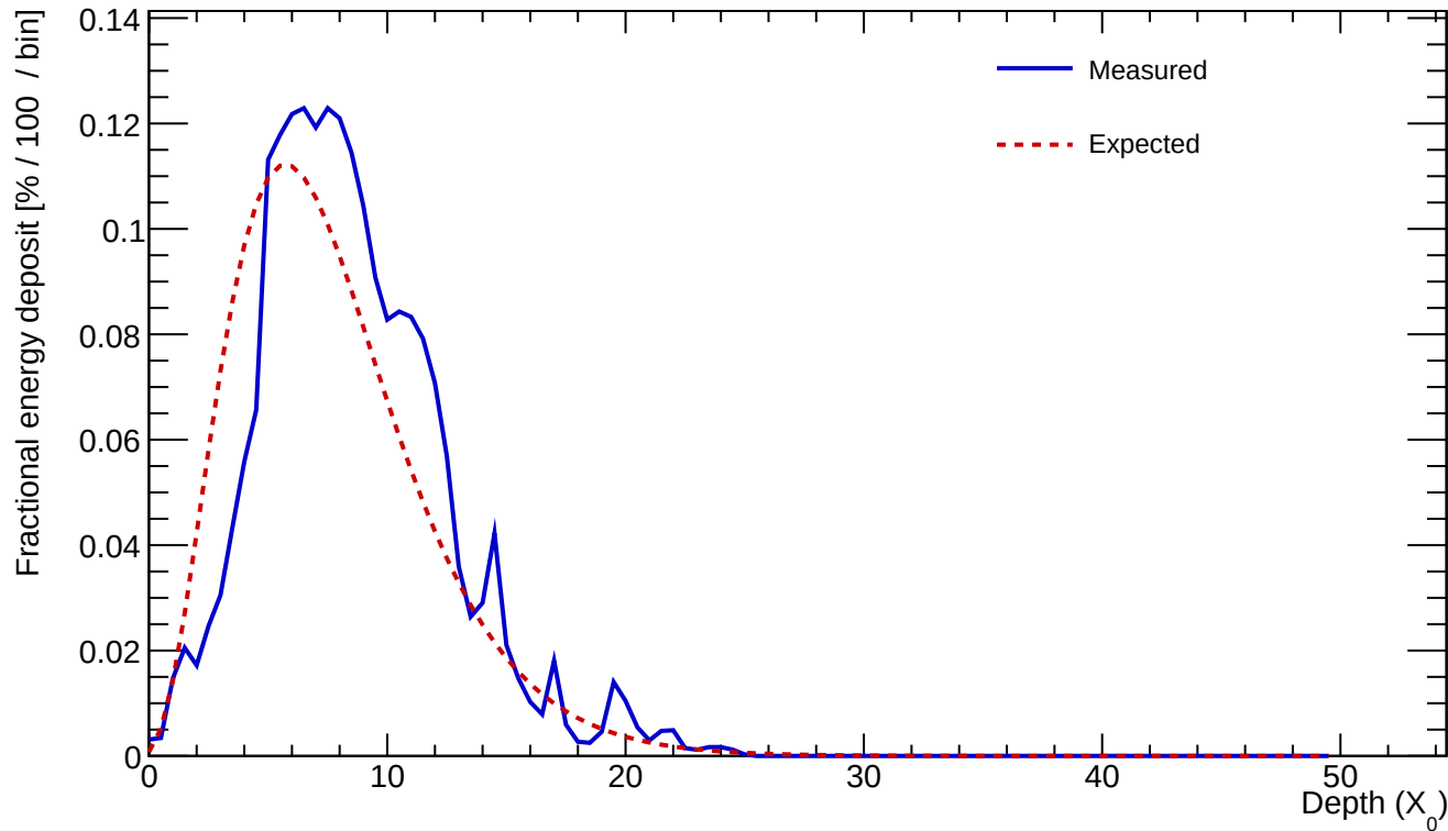
Cluster 83 E=24.475 GeV profileStart=1.50 X_0 \chi=0.1581
