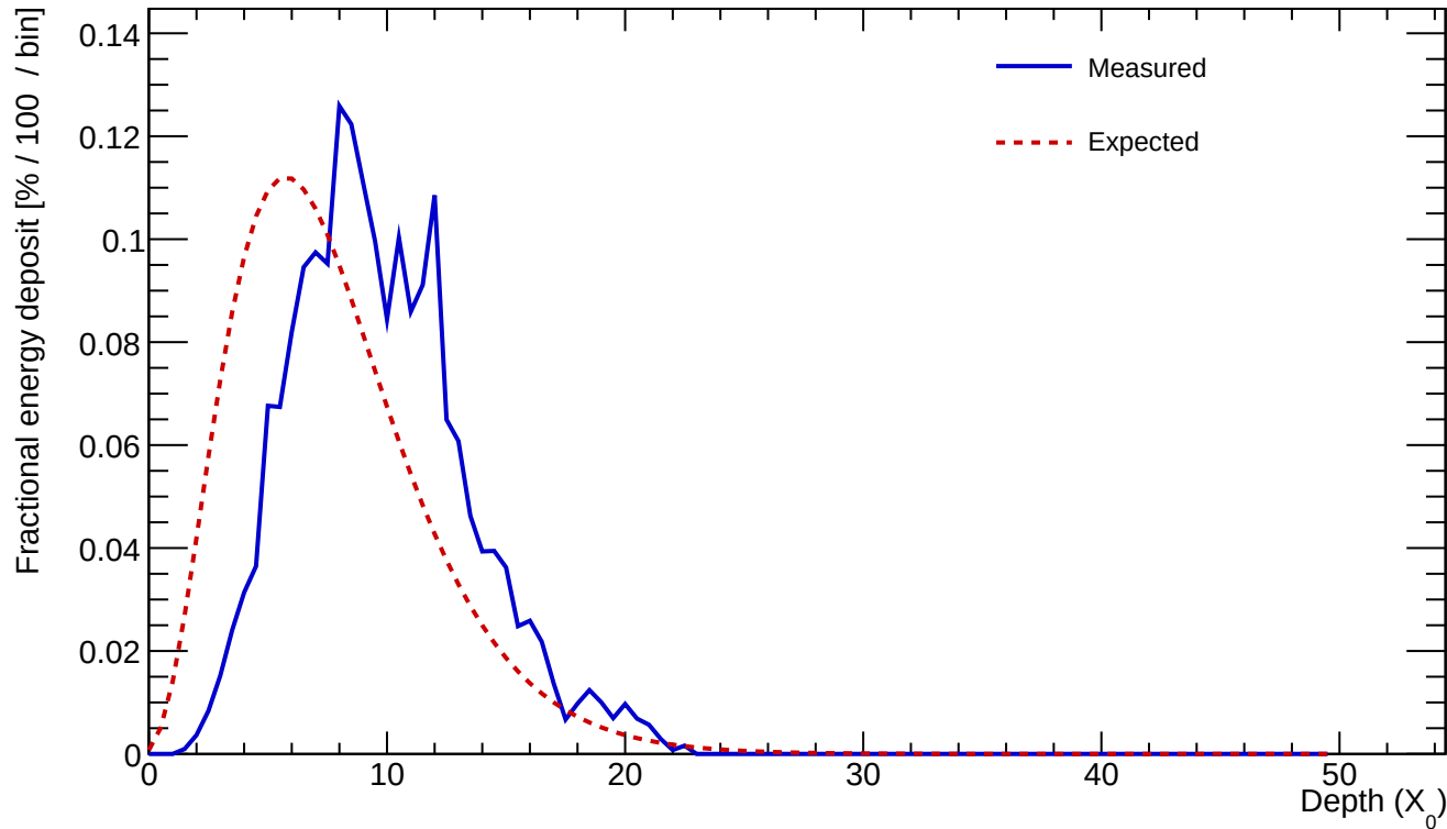
Cluster 592 E=24.761 GeV profileStart=2.50 X_0 \chi=0.1271
