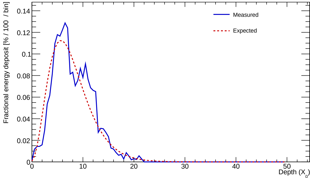
Cluster 241 E=23.903 GeV profileStart=0.50 X_0 \chi=0.1837
