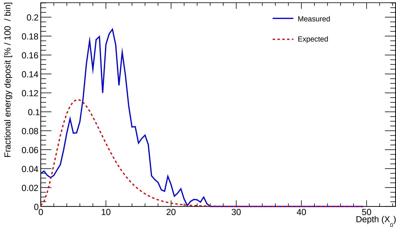
Cluster 550 E=23.087 GeV profileStart=3.50 X_0 \chi=0.2765
