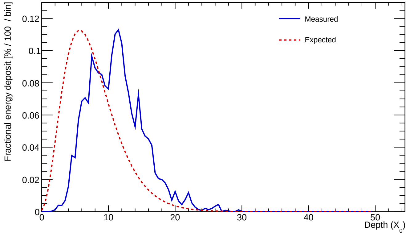
Cluster 350 E=23.576 GeV profileStart=3.50 X_0 \chi=0.1957
