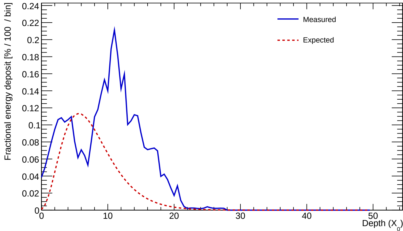
Cluster 325 E=22.361 GeV profileStart=4.00 X_0 \chi=0.4839
