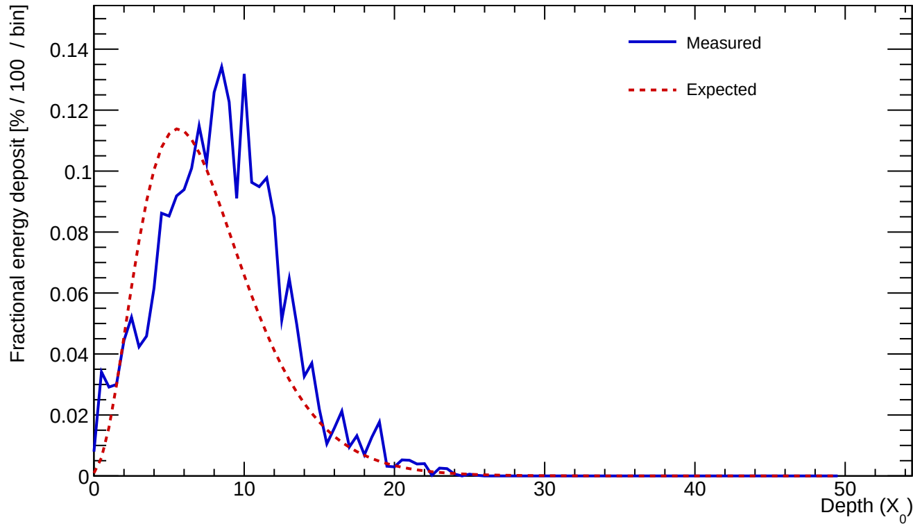
Cluster 656 E=21.299 GeV profileStart=1.50 X_0 \chi=0.2438
