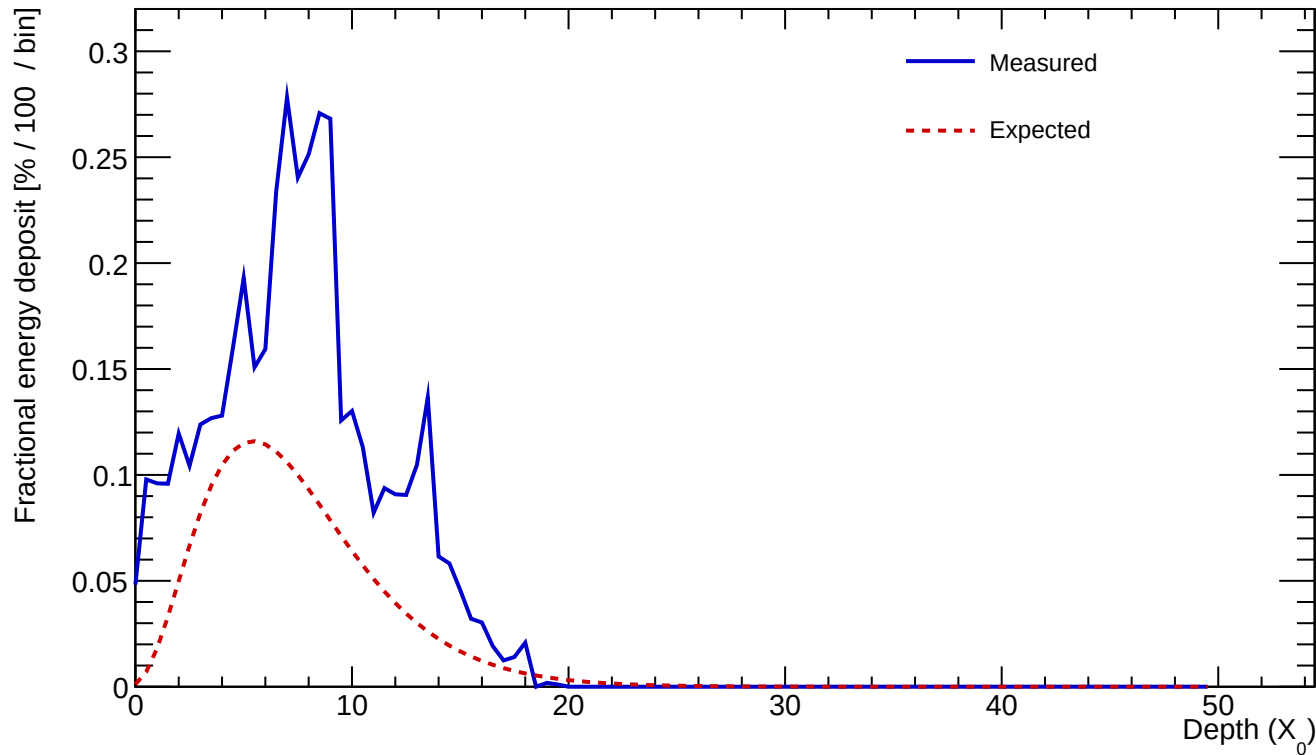
Cluster 165 E=18.130 GeV profileStart=0.50 X_0 \chi=0.3085
