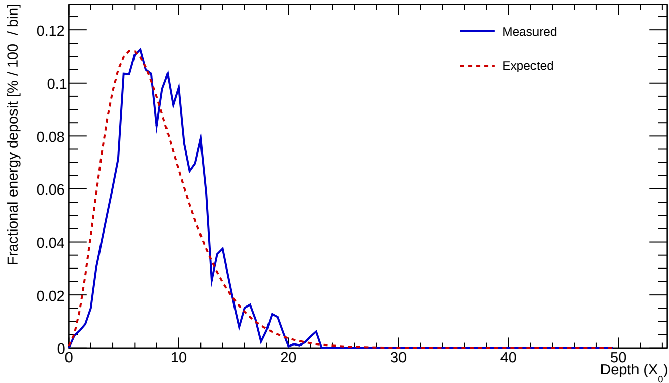
Cluster 536 E=24.266 GeV profileStart=1.00 X_0 \chi=0.1353
