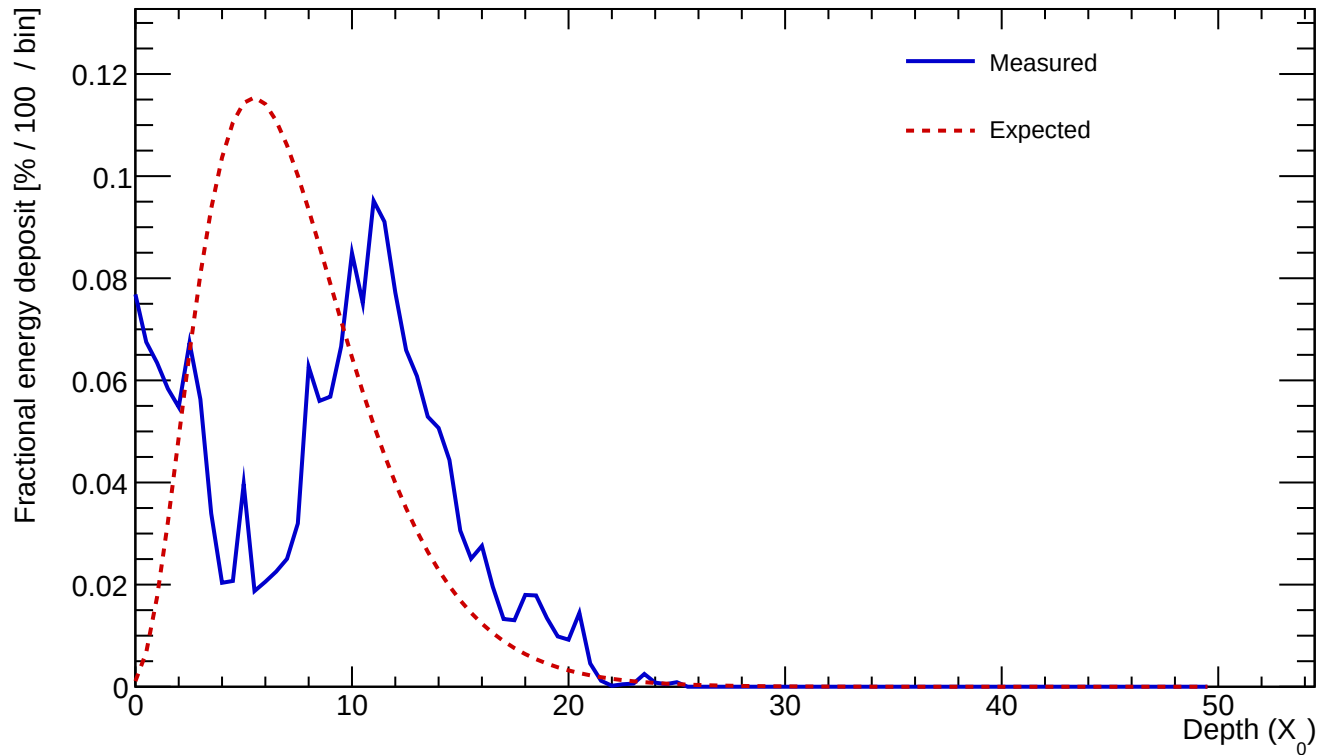
Cluster 445 E=18.852 GeV profileStart=3.50 X_0 \chi=0.5709
