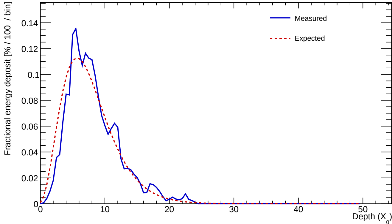
Cluster 447 E=23.484 GeV profileStart=0.50 X_0 \chi=0.1485
