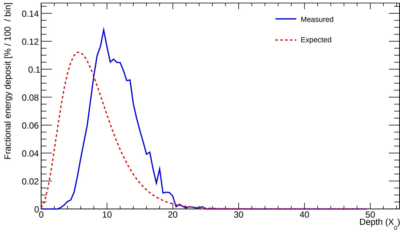
Cluster 5 E=24.314 GeV profileStart=4.00 X_0 \chi=0.1333
