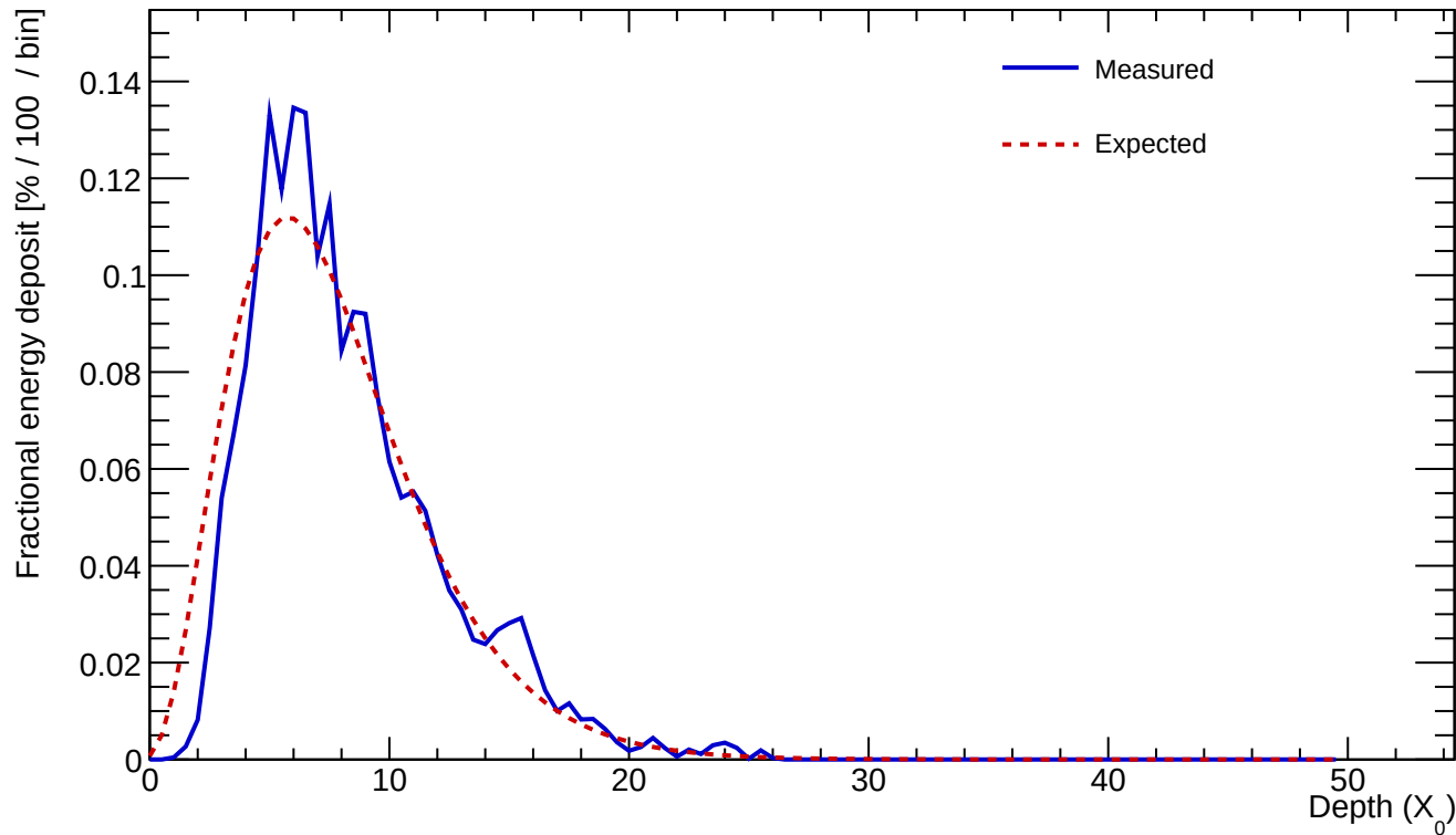
Cluster 606 E=24.976 GeV profileStart=0.50 X_0 \chi=0.1527
