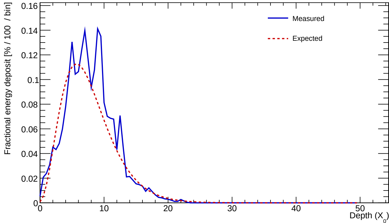
Cluster 211 E=23.773 GeV profileStart=0.50 X_0 \chi=0.1996
