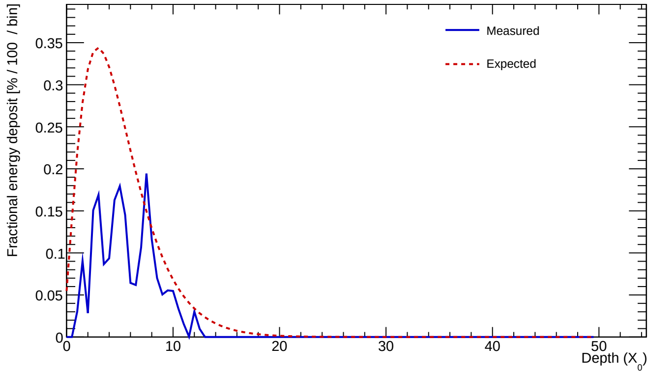
Cluster 527 E=1.498 GeV profileStart=1.00 X_0 \chi=0.3528
