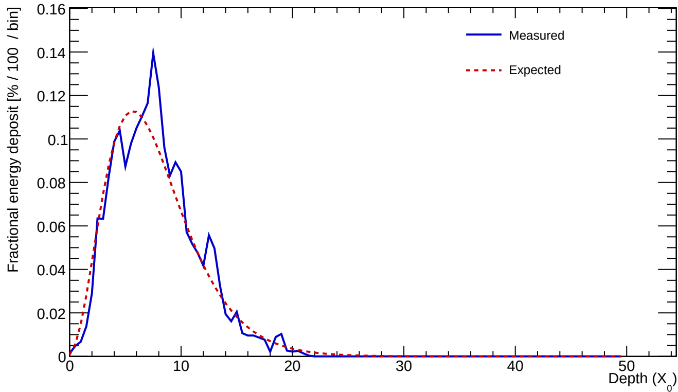
Cluster 106 E=23.082 GeV profileStart=0.50 X_0 \chi=0.1451
