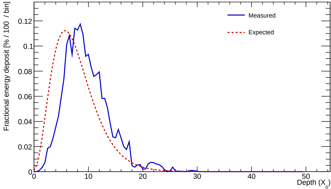
Cluster 577 E=24.018 GeV profileStart=2.00 X_0 \chi=0.1279
