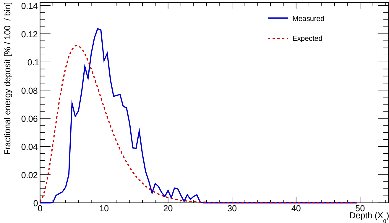
Cluster 142 E=25.411 GeV profileStart=3.00 X_0 \chi=0.1374
