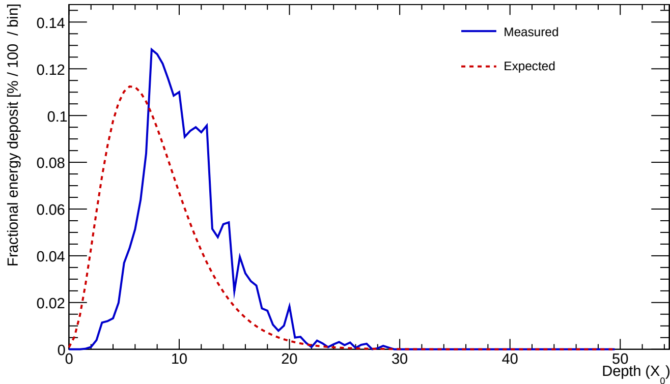
Cluster 461 E=23.671 GeV profileStart=3.00 X_0 \chi=0.1666
