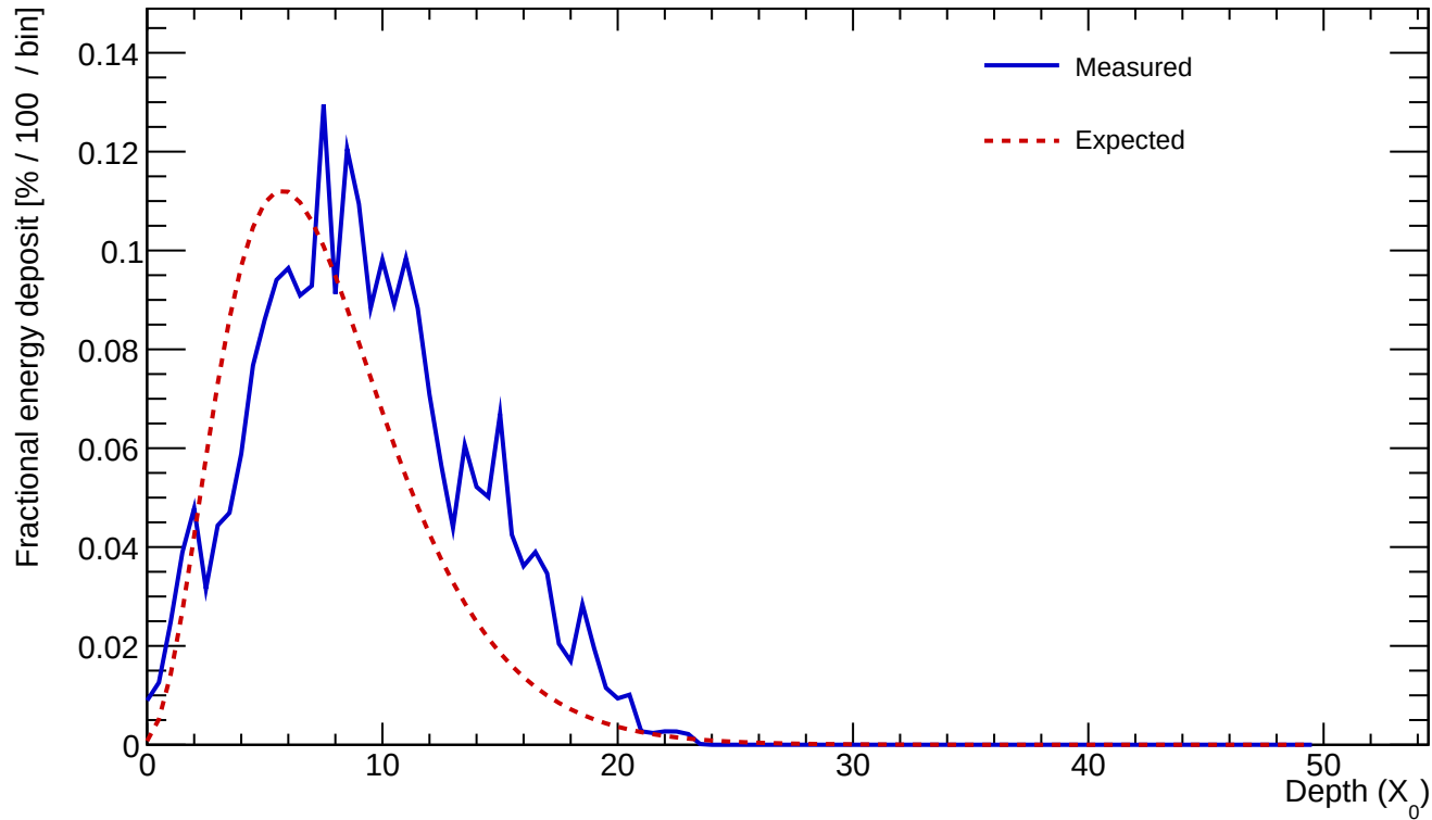
Cluster 57 E=24.478 GeV profileStart=2.00 X_0 \chi=0.2554
