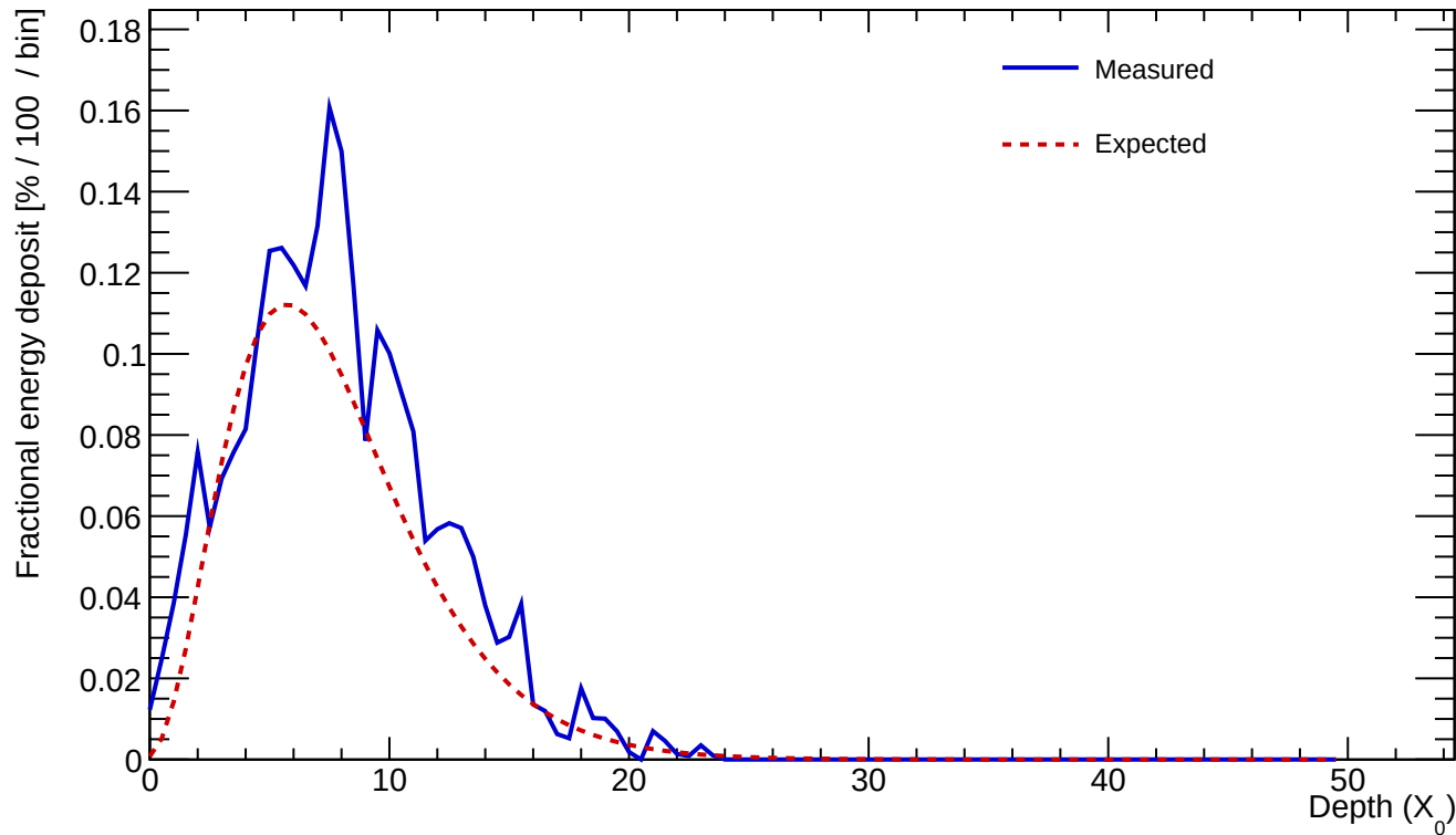
Cluster 161 E=24.282 GeV profileStart=0.50 X_0 \chi=0.1993
