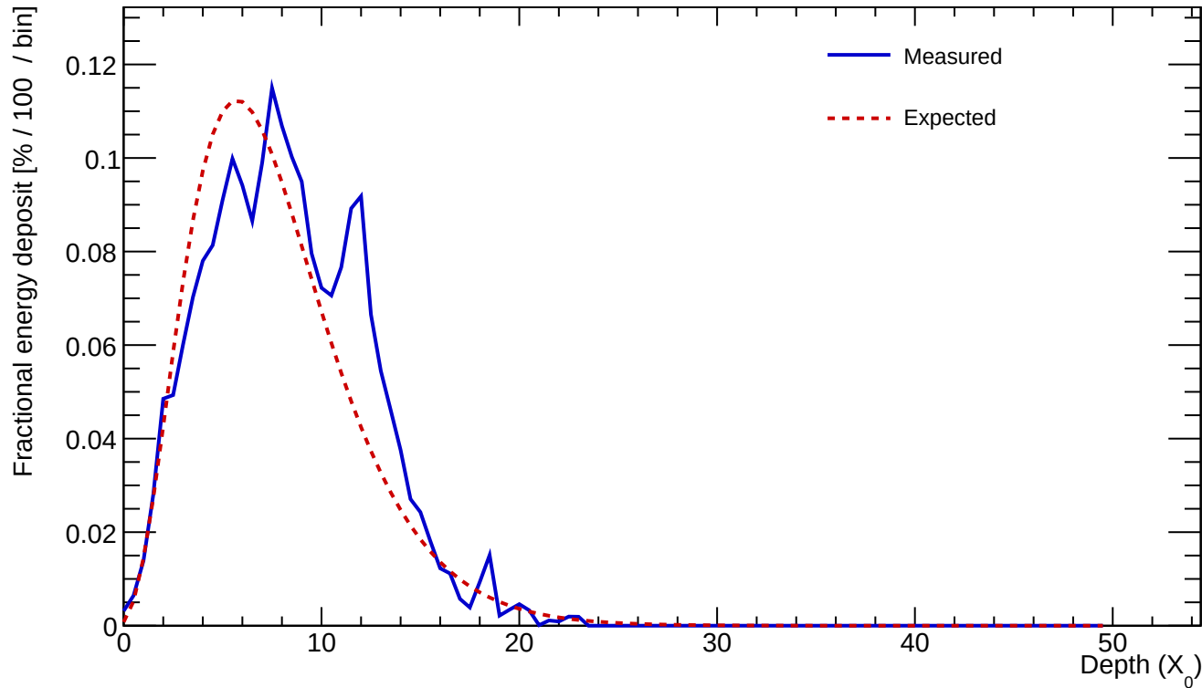
Cluster 132 E=24.090 GeV profileStart=0.50 X_0 \chi=0.1916
