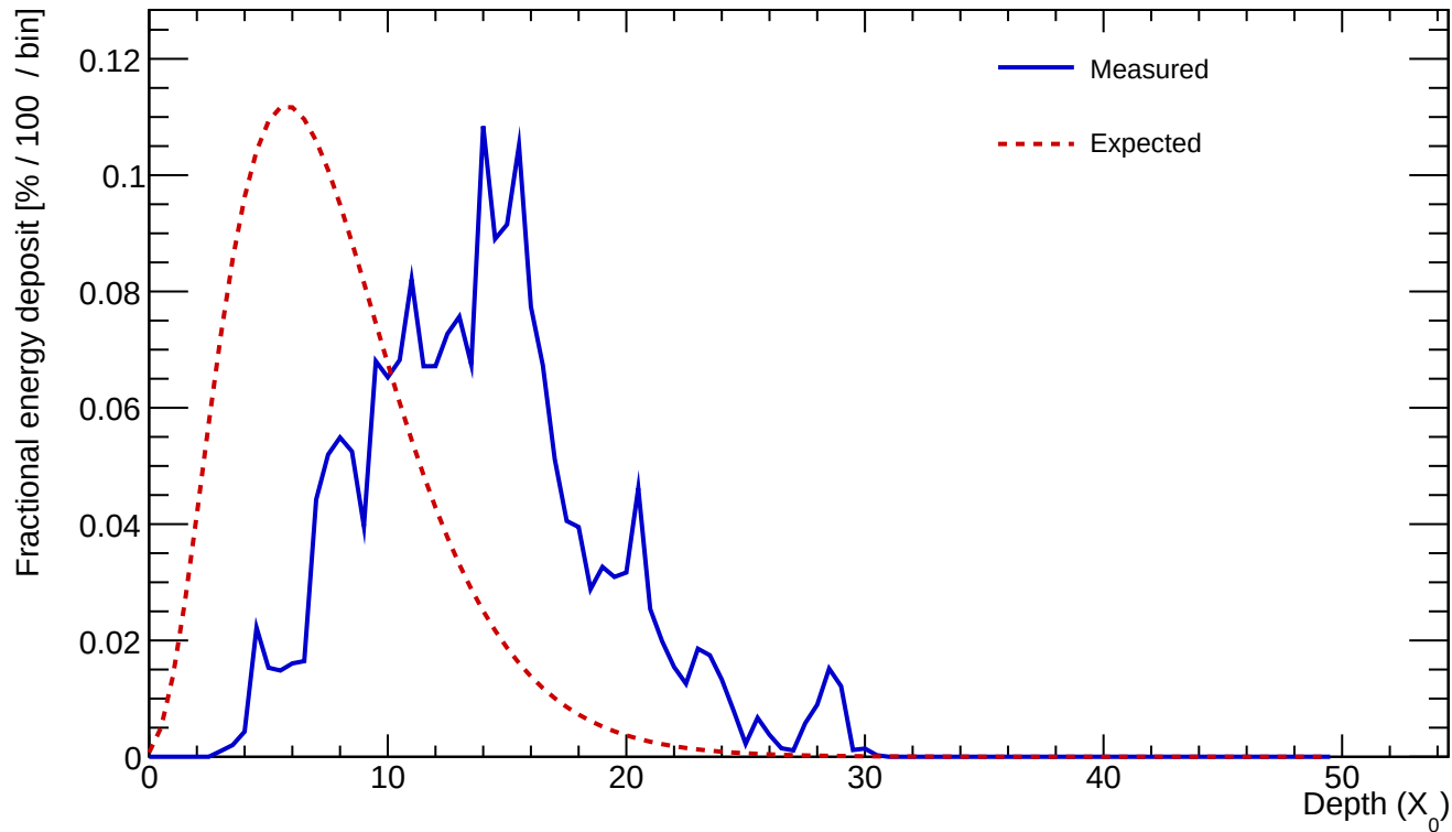
Cluster 205 E=25.065 GeV profileStart=6.50 X_0 \chi=0.3380
