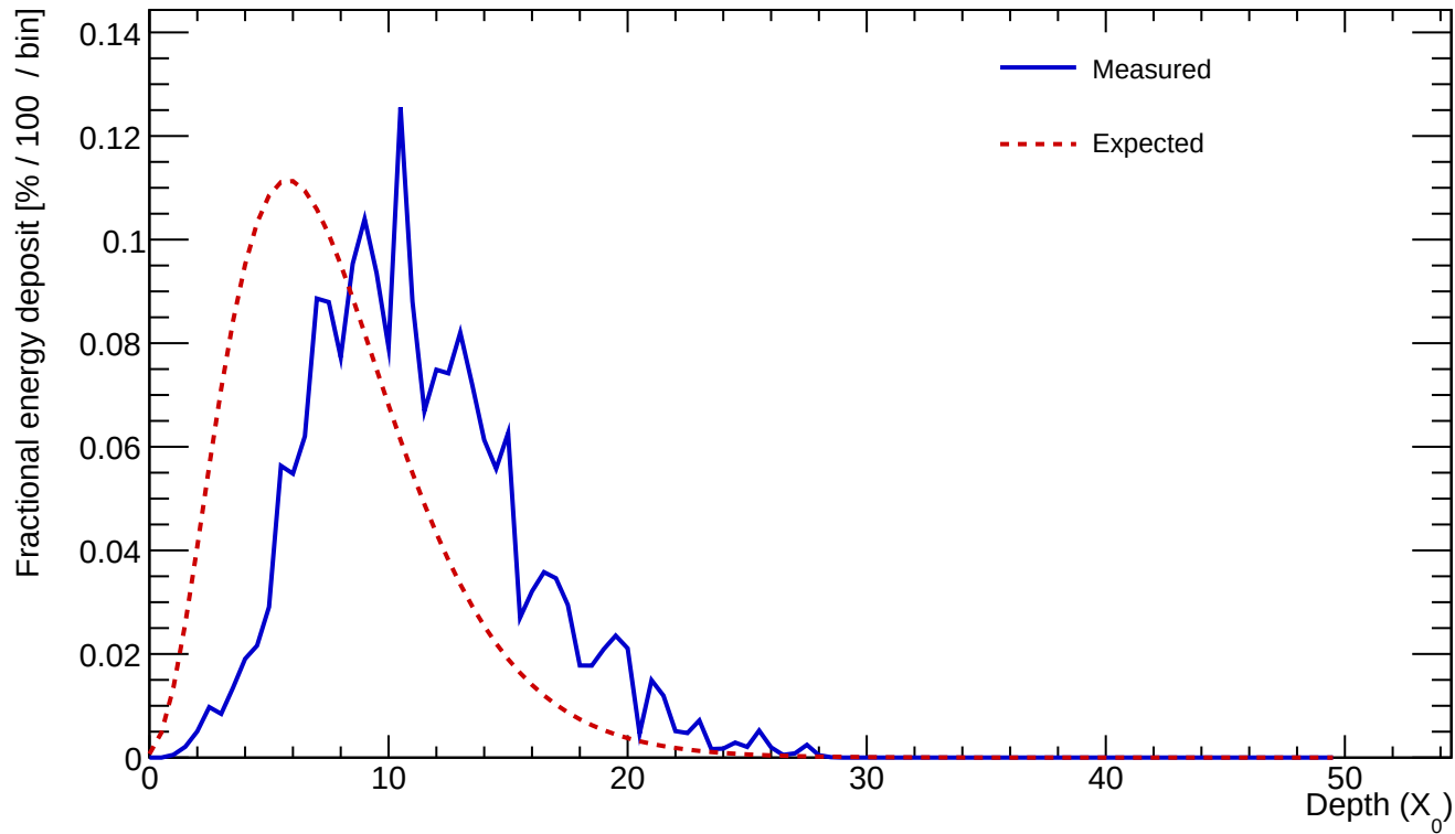
Cluster 214 E=26.132 GeV profileStart=3.50 X_0 \chi=0.1945
