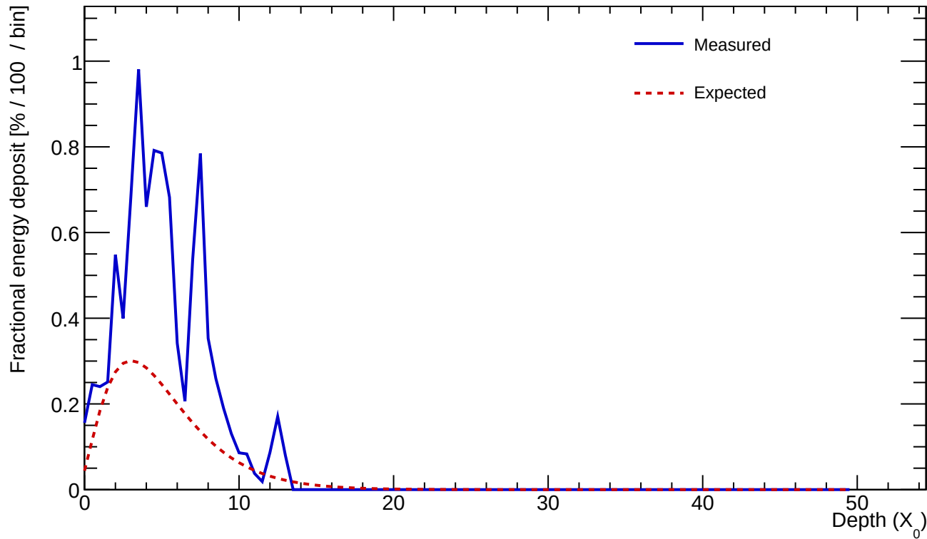
Cluster 587 E=1.639 GeV profileStart=0.50 X_0 \chi=0.3111
