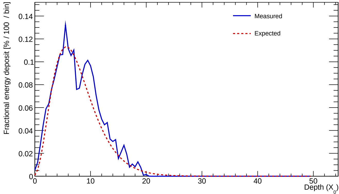
Cluster 418 E=22.626 GeV profileStart=0.50 X_0 \chi=0.1723
