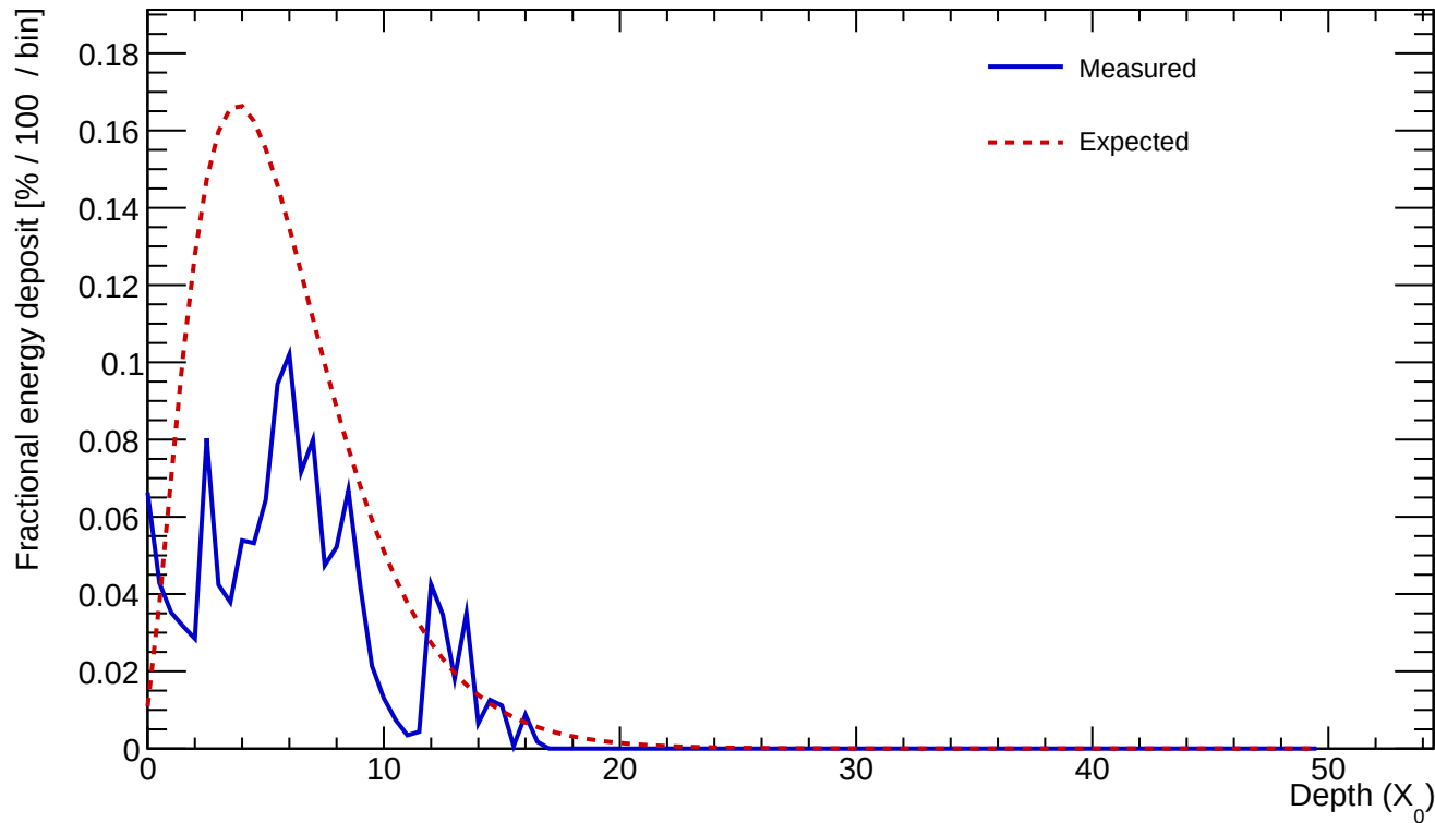
Cluster 659 E=3.571 GeV profileStart=0.50 X_0 \chi=0.4573
