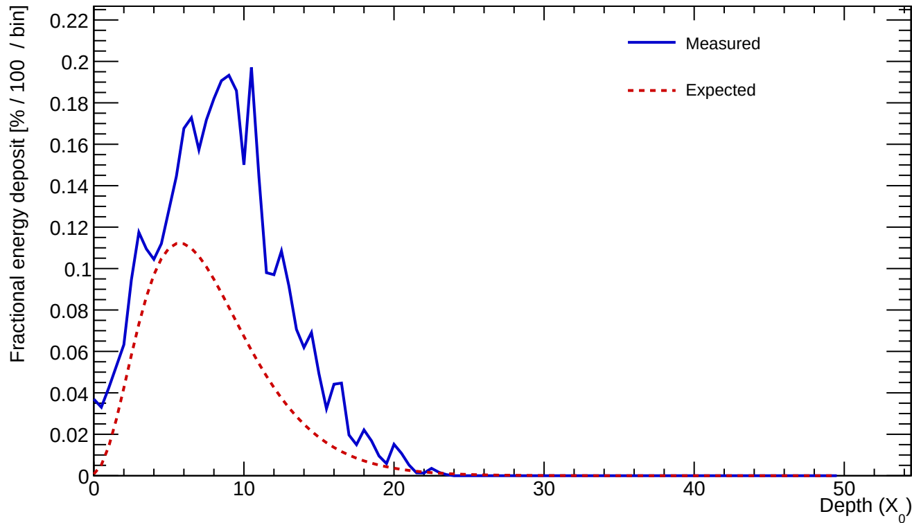
Cluster 538 E=24.341 GeV profileStart=1.00 X_0 \chi=0.2360
