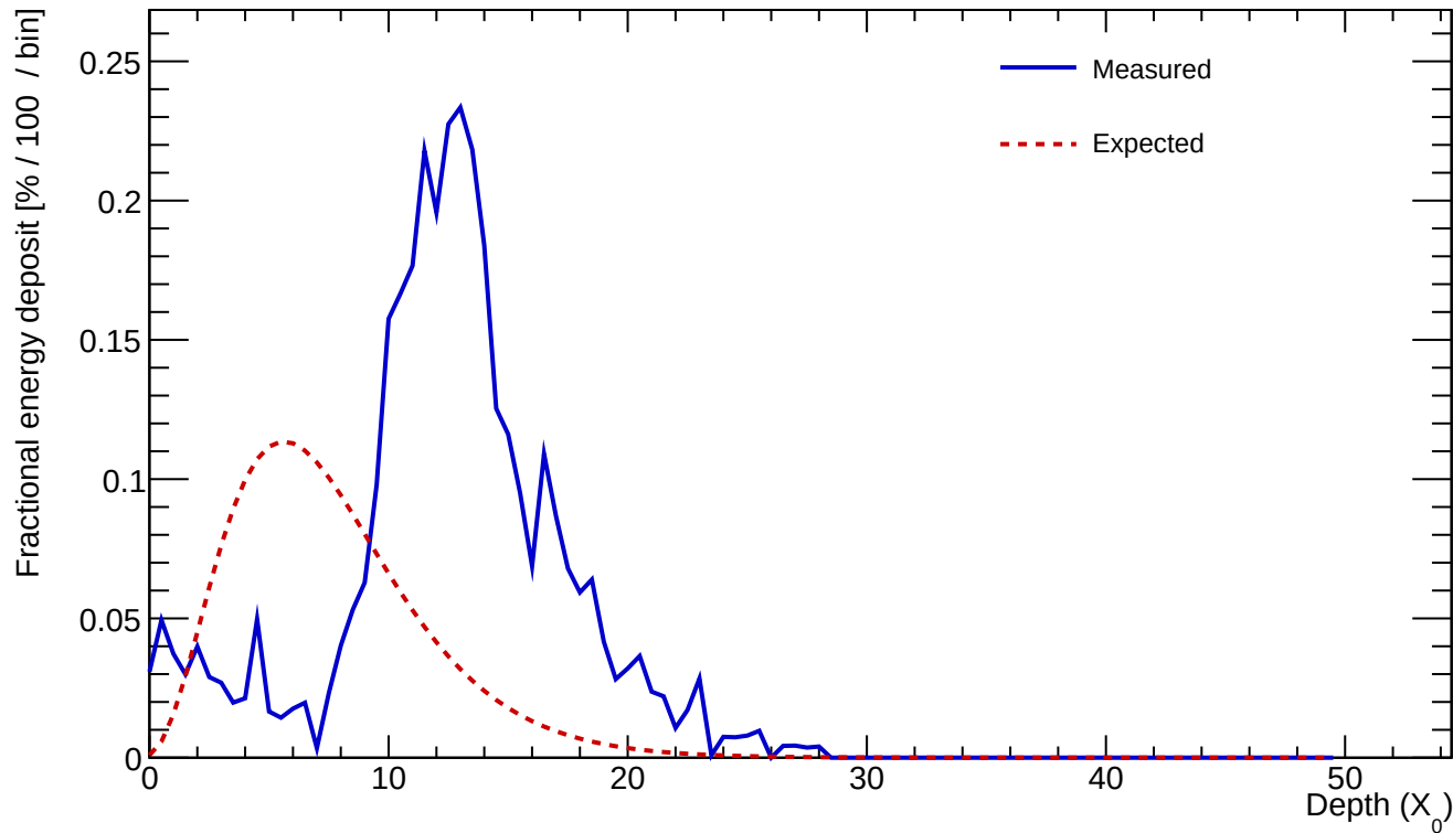
Cluster 645 E=21.875 GeV profileStart=6.50 X_0 \chi=0.3098
