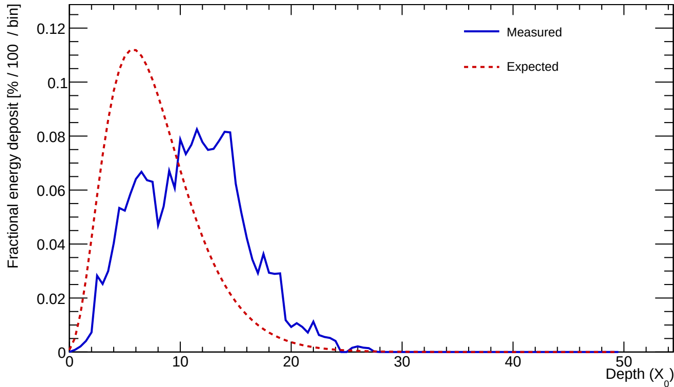
Cluster 207 E=24.601 GeV profileStart=3.50 X_0 \chi=0.3756
