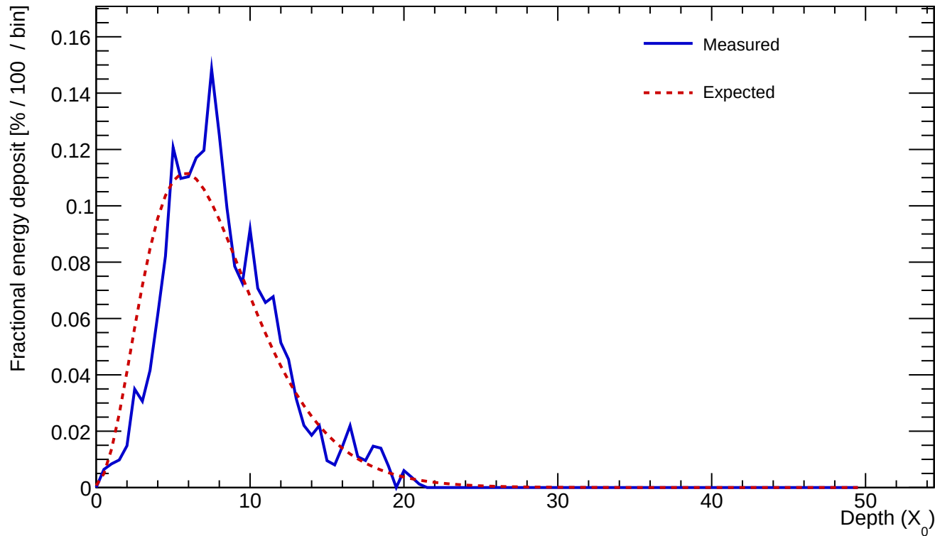
Cluster 443 E=25.676 GeV profileStart=1.00 X_0 \chi=0.1737
