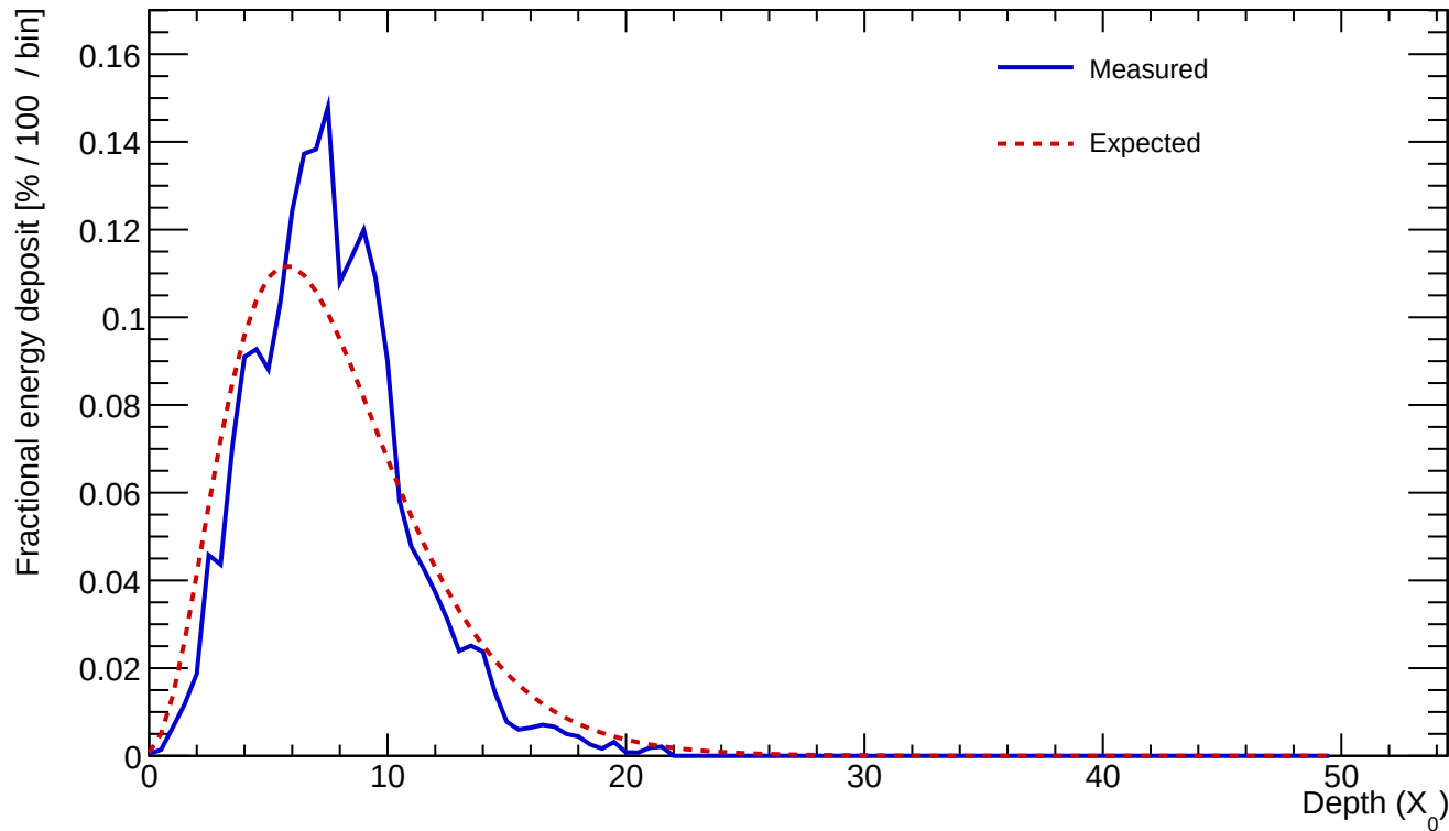
Cluster 495 E=25.362 GeV profileStart=0.50 X_0 \chi=0.2191
