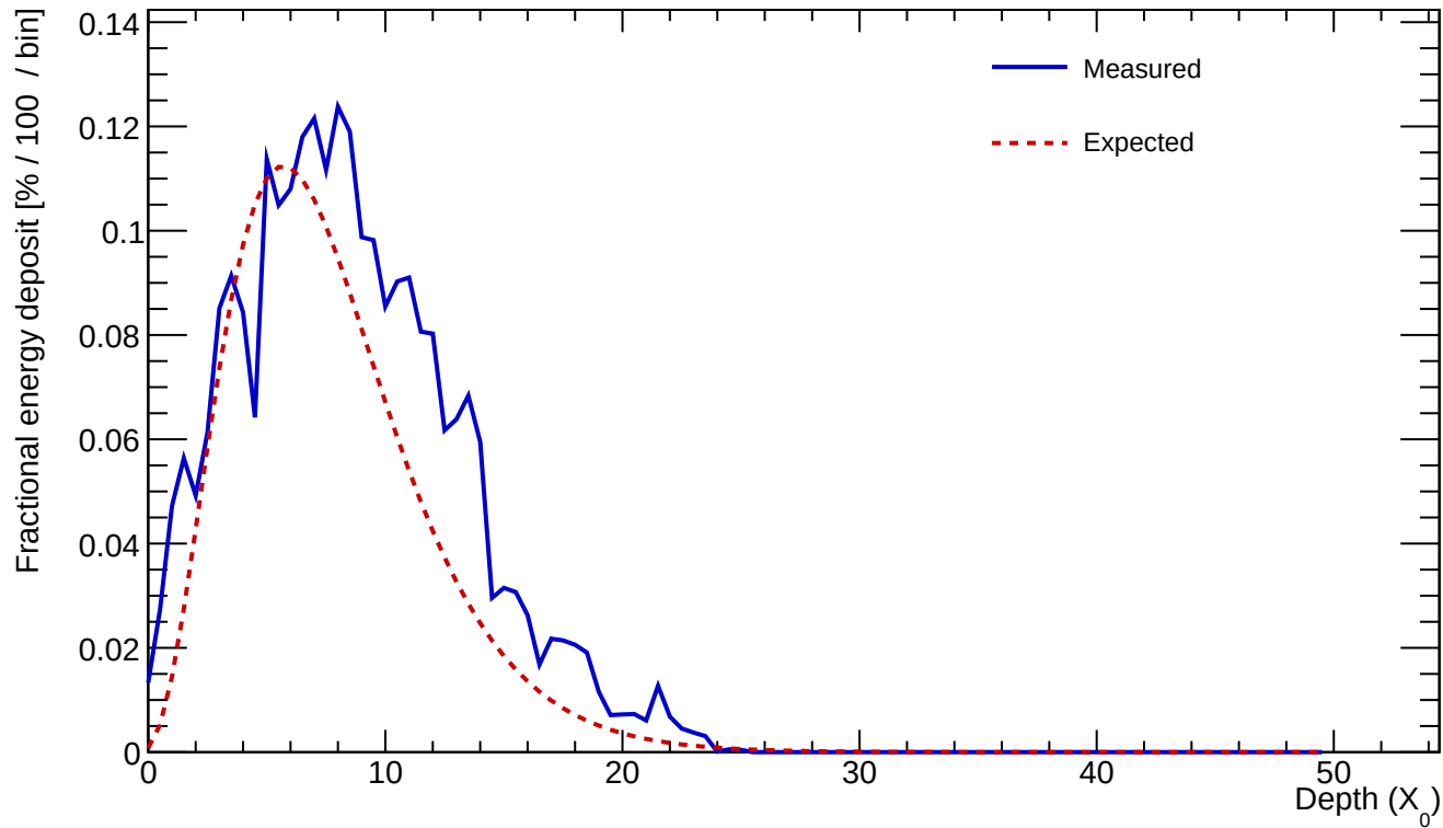
Cluster 542 E=24.009 GeV profileStart=0.50 X_0 \chi=0.2497
