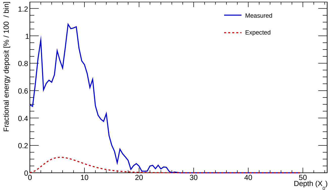
Cluster 616 E=21.962 GeV profileStart=0.50 X_0 \chi=0.3050
