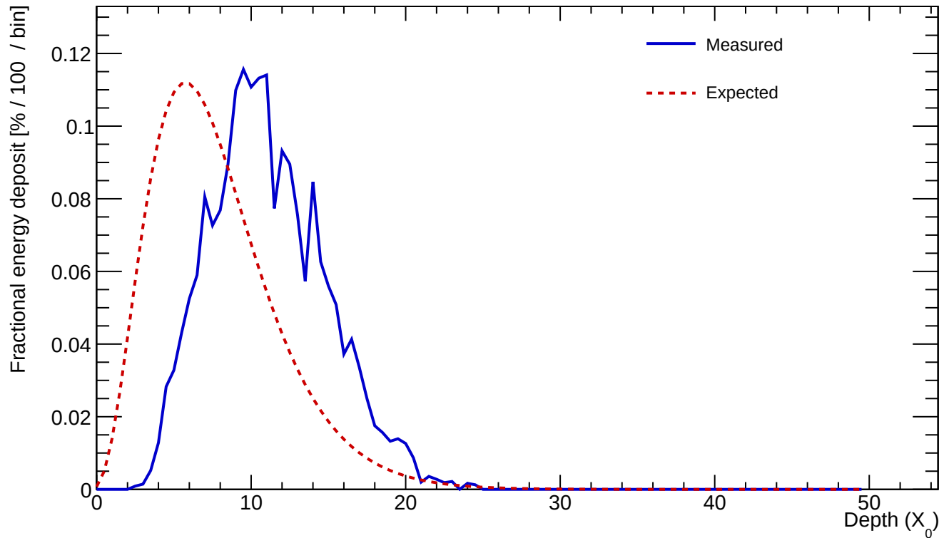
Cluster 565 E=24.997 GeV profileStart=3.50 X_0 \chi=0.1504
