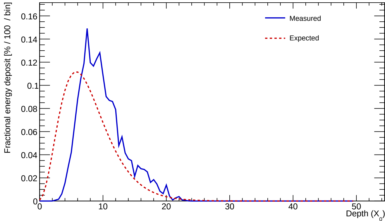
Cluster 167 E=25.603 GeV profileStart=2.50 X_0 \chi=0.1606
