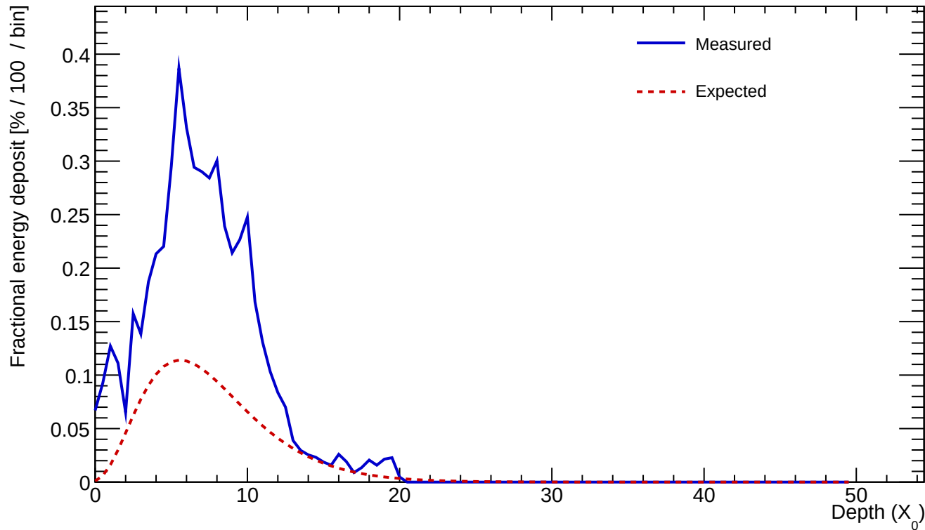
Cluster 625 E=21.057 GeV profileStart=0.50 X_0 \chi=0.2332
