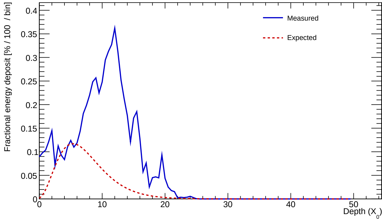
Cluster 327 E=16.587 GeV profileStart=4.50 X_0 \chi=0.4024
