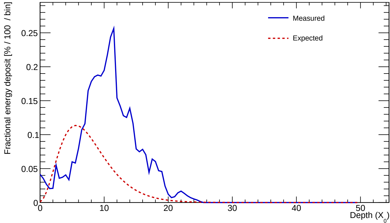
Cluster 42 E=21.789 GeV profileStart=4.00 X_0 \chi=0.2393
