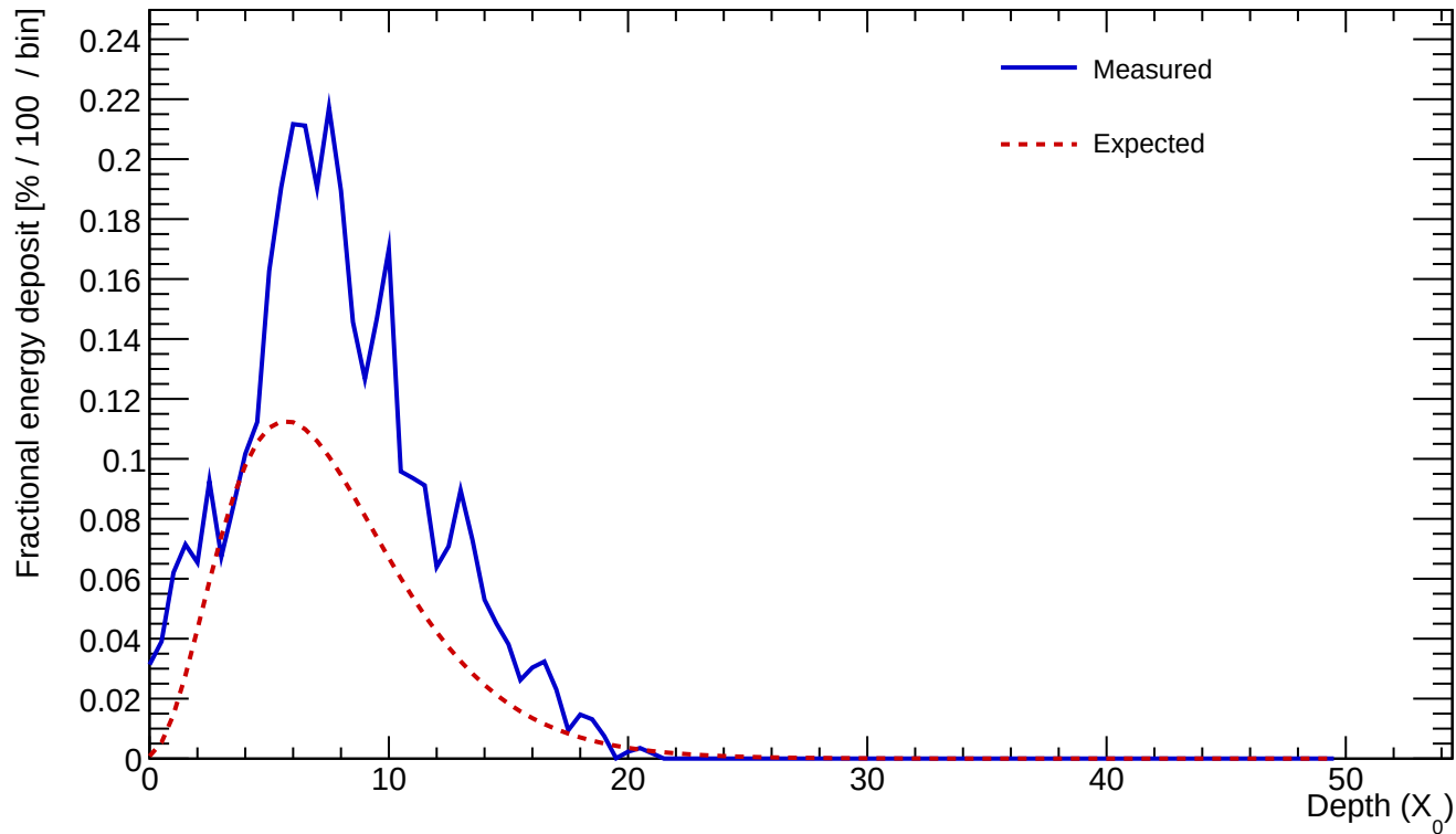
Cluster 47 E=23.550 GeV profileStart=0.50 X_0 \chi=0.2076
