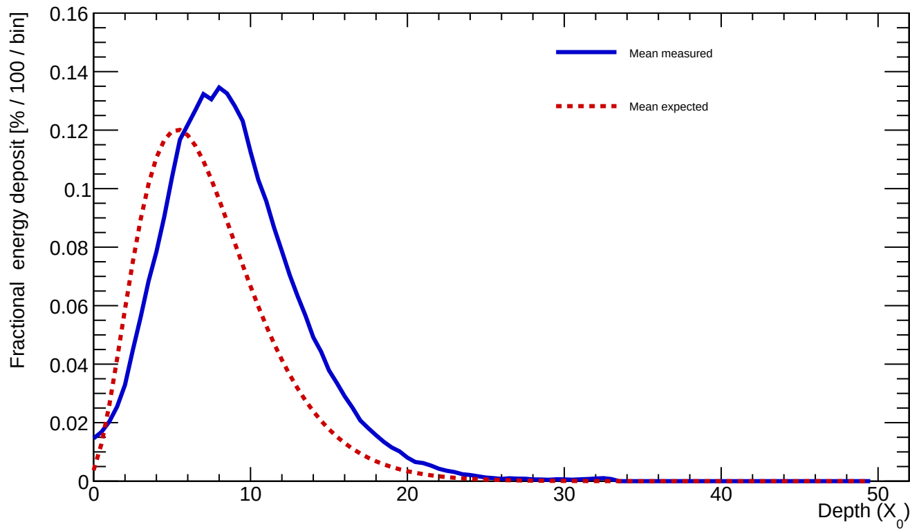
Average longitudinal profile (700 clusters): measured vs expected
