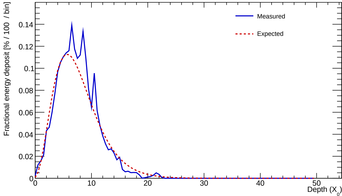
Cluster 521 E=23.291 GeV profileStart=0.50 X_0 \chi=0.1533
