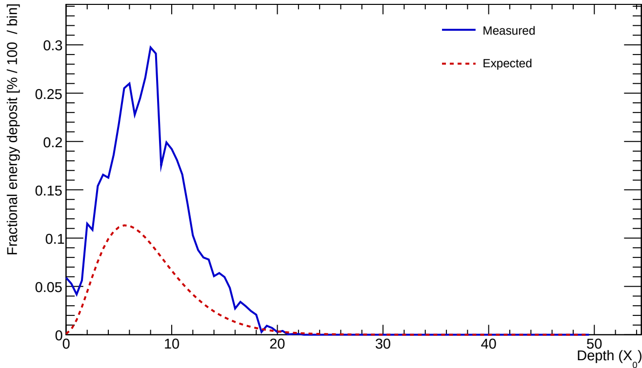
Cluster 674 E=22.324 GeV profileStart=0.50 X_0 \chi=0.1664
