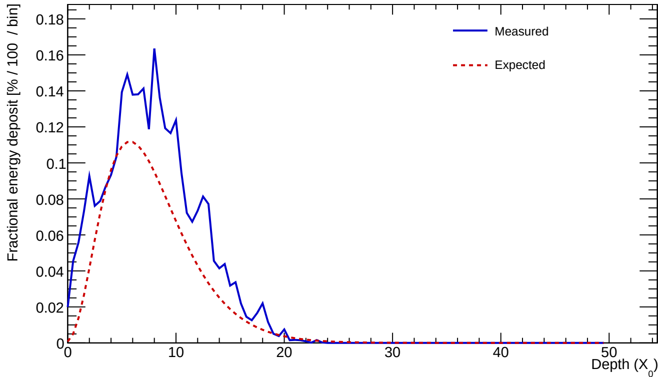
Cluster 183 E=25.252 GeV profileStart=0.50 X_0 \chi=0.2176
