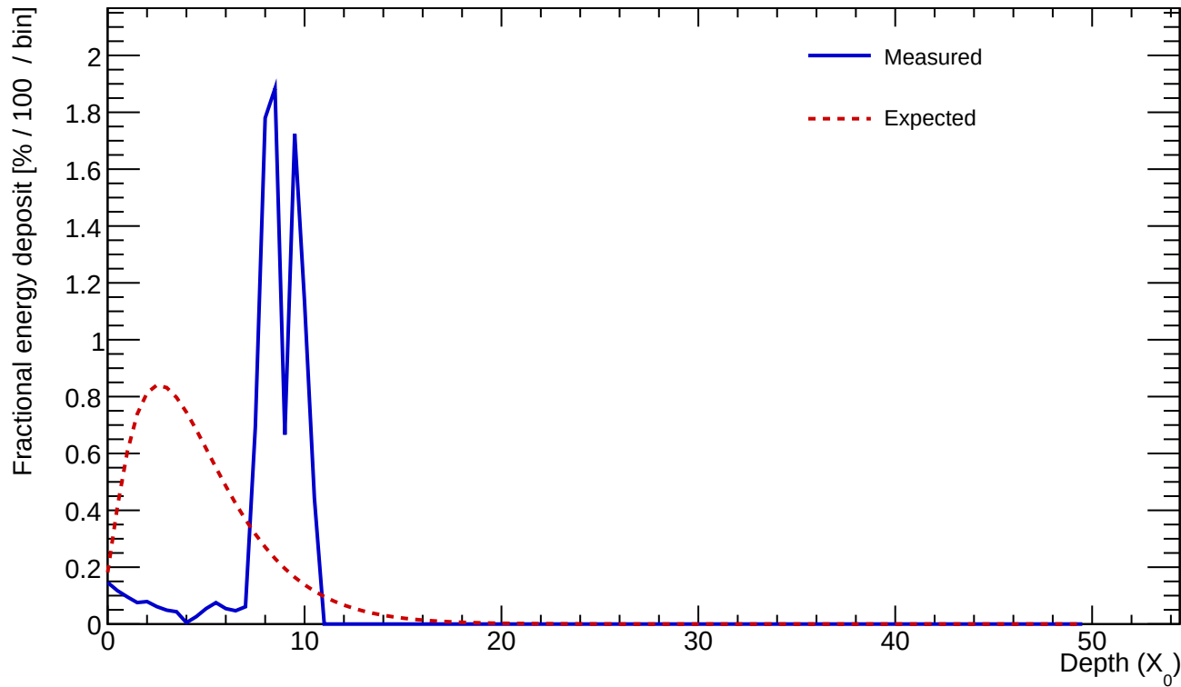
Cluster 356 E=1.083 GeV profileStart=6.50 X_0 \chi=0.5742
