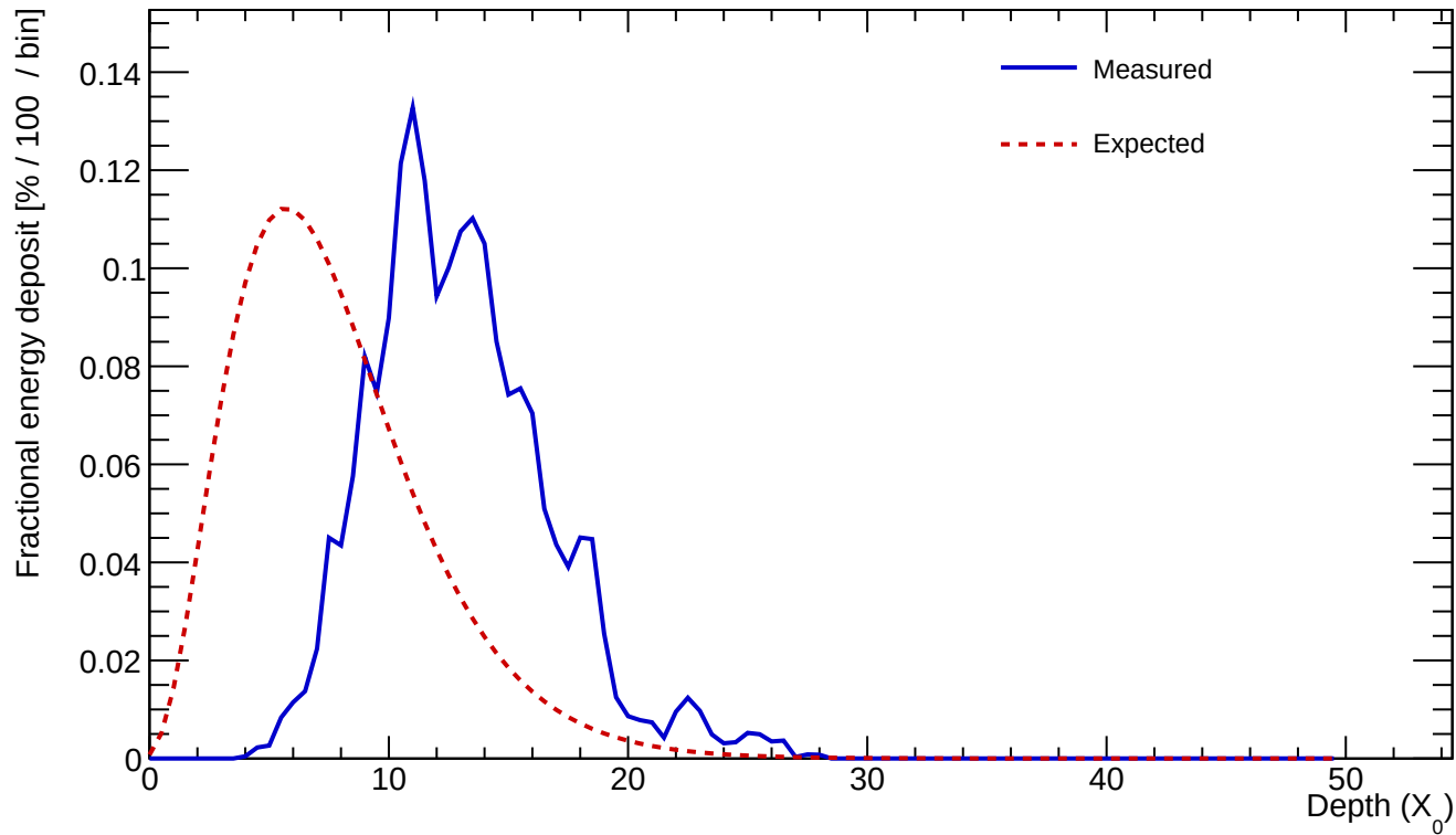
Cluster 554 E=24.278 GeV profileStart=5.50 X_0 \chi=0.1641
