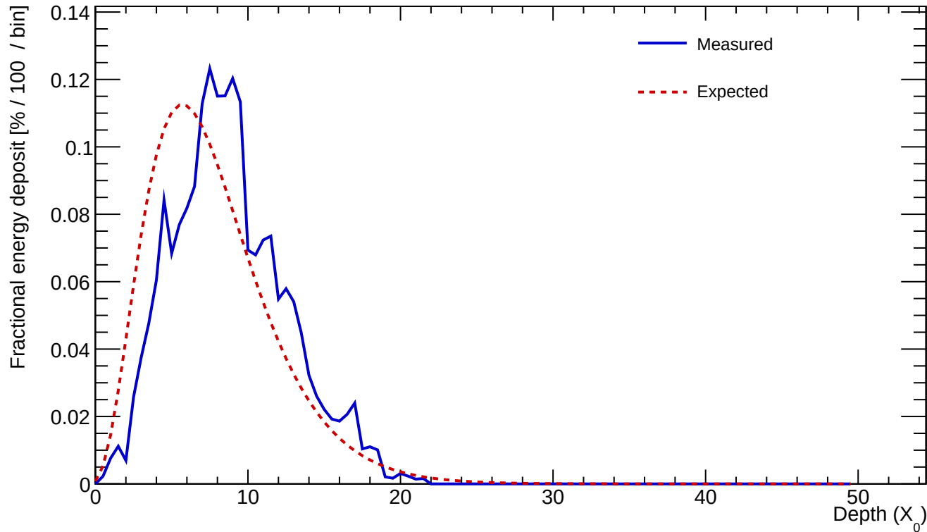
Cluster 411 E=23.760 GeV profileStart=1.50 X_0 \chi=0.1654
