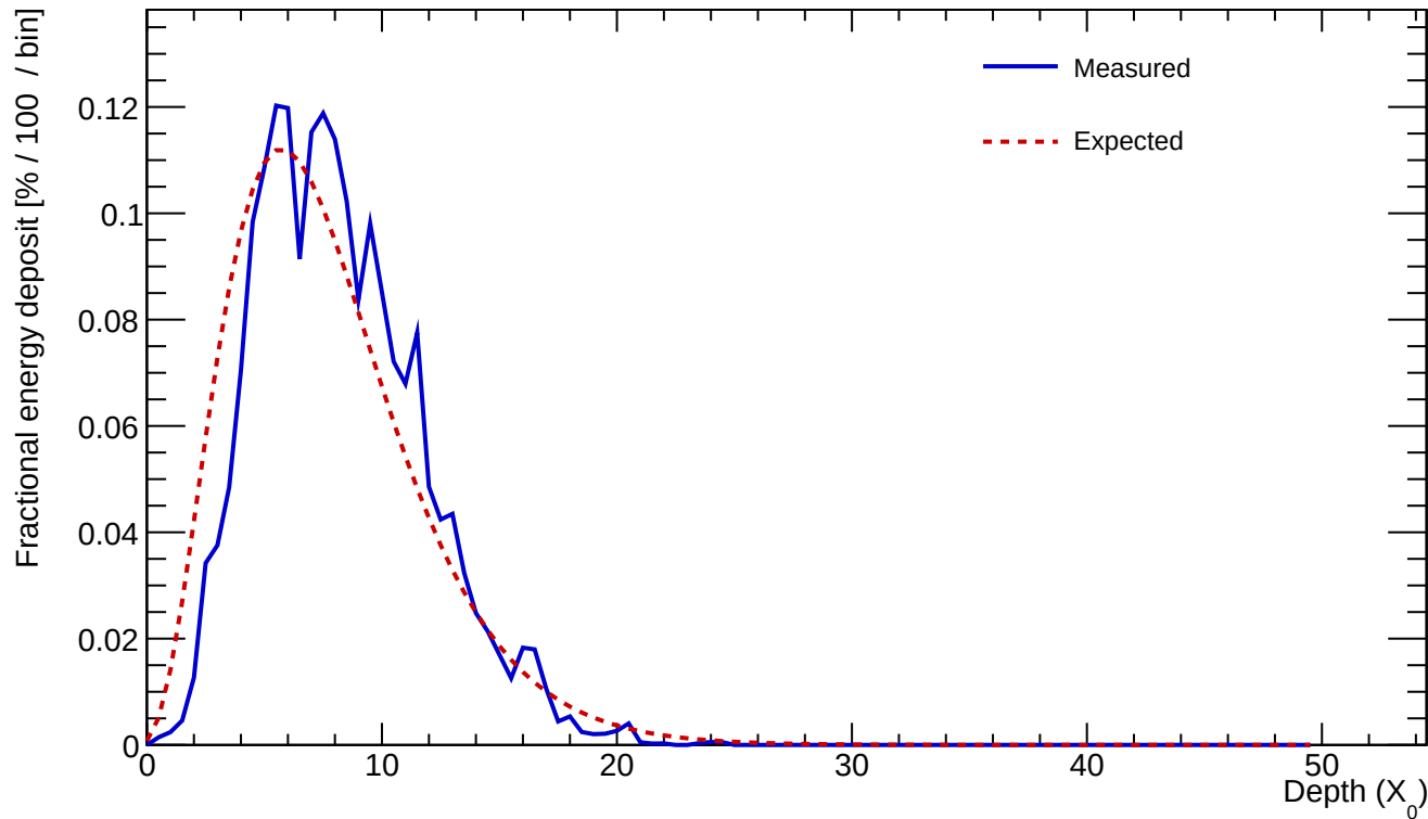
Cluster 344 E=24.669 GeV profileStart=1.00 X_0 \chi=0.1363
