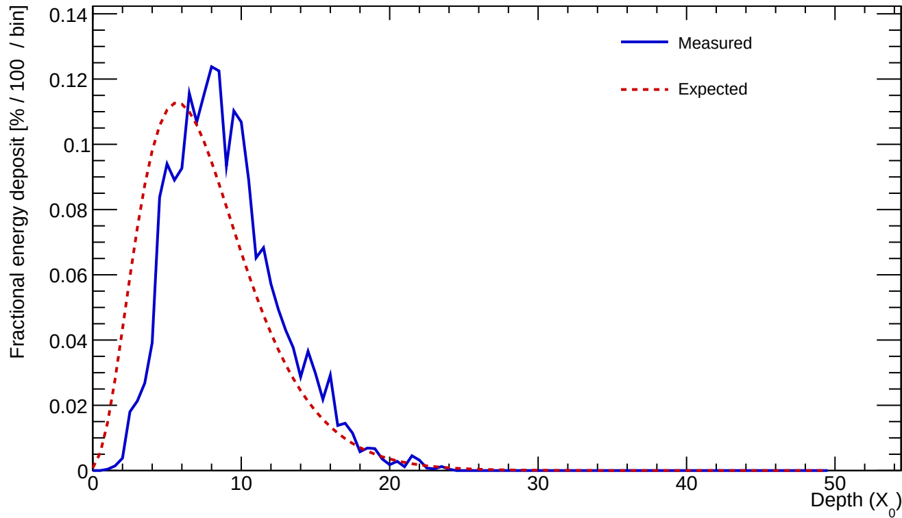
Cluster 206 E=23.342 GeV profileStart=1.50 X_0 \chi=0.1348
