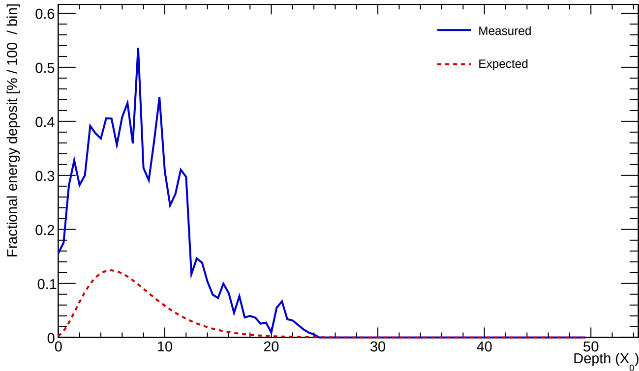
Cluster 190 E=10.909 GeV profileStart=0.50 X_0 \chi=0.3205
