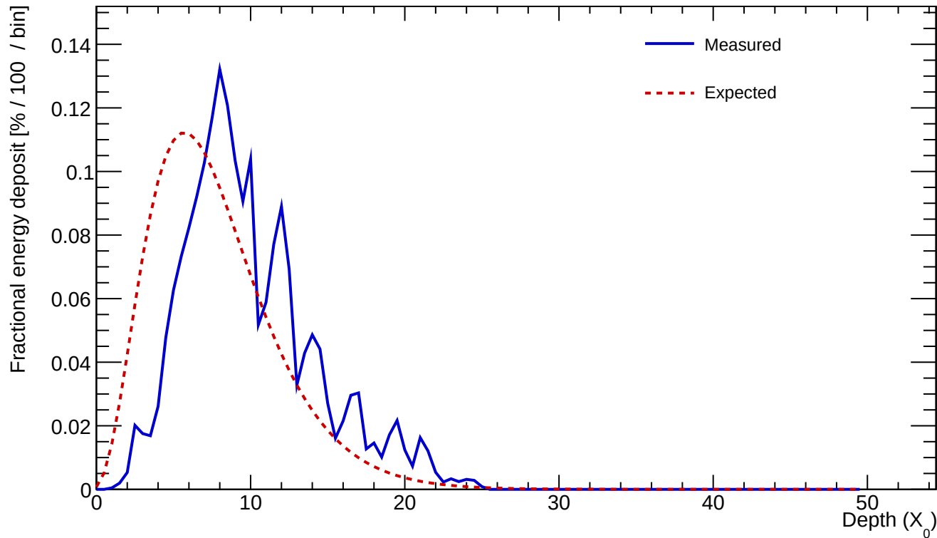
Cluster 45 E=24.352 GeV profileStart=2.50 X_0 \chi=0.1797
