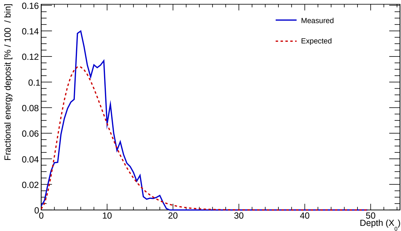
Cluster 73 E=24.872 GeV profileStart=0.50 X_0 \chi=0.1553
