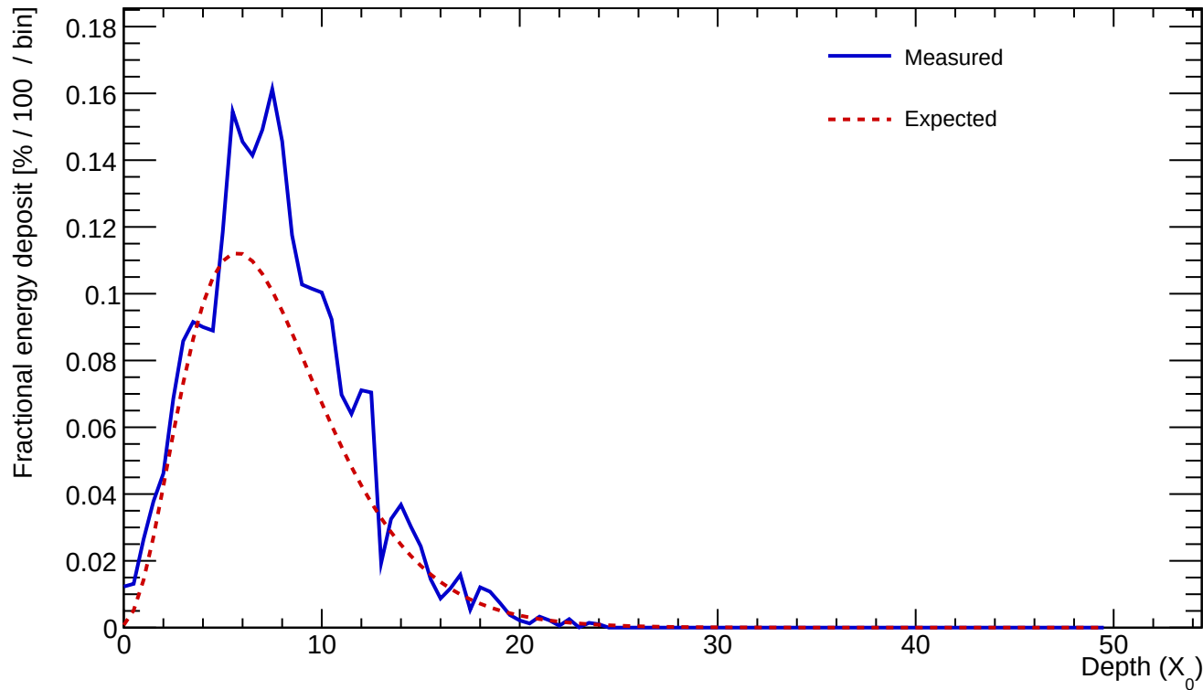
Cluster 547 E=24.356 GeV profileStart=0.50 X_0 \chi=0.1555
