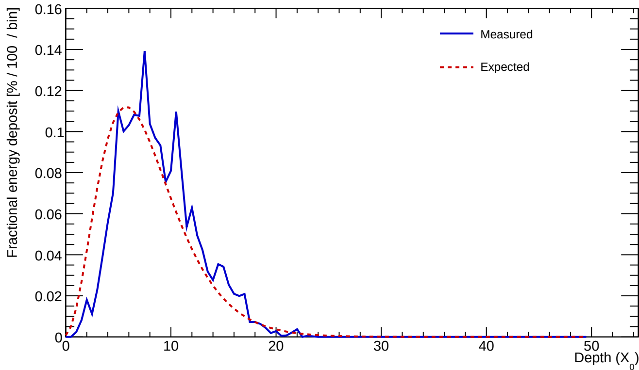
Cluster 162 E=24.792 GeV profileStart=1.50 X_0 \chi=0.1385
