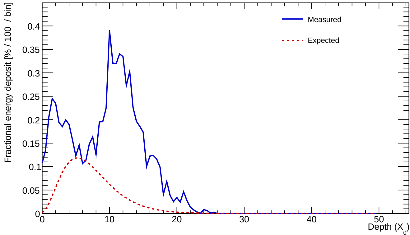
Cluster 78 E=15.113 GeV profileStart=4.00 X_0 \chi=0.5323
