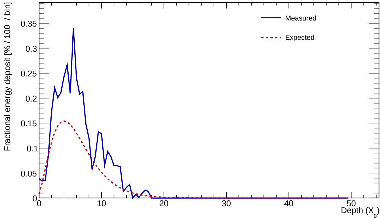
Cluster 117 E=4.366 GeV profileStart=0.50 X_0 \chi=0.2104
