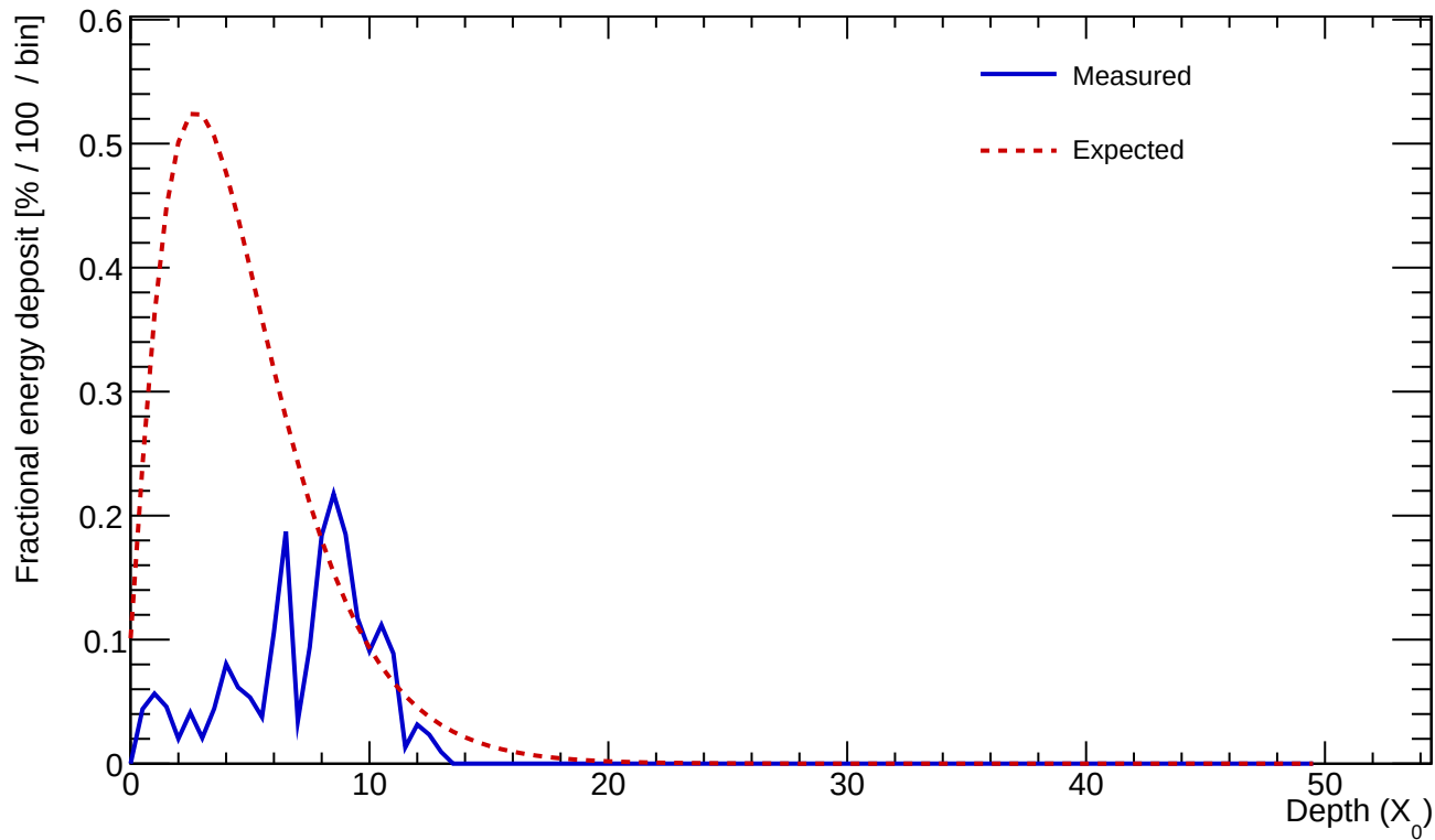
Cluster 661 E=1.229 GeV profileStart=5.00 X_0 \chi=0.5179
