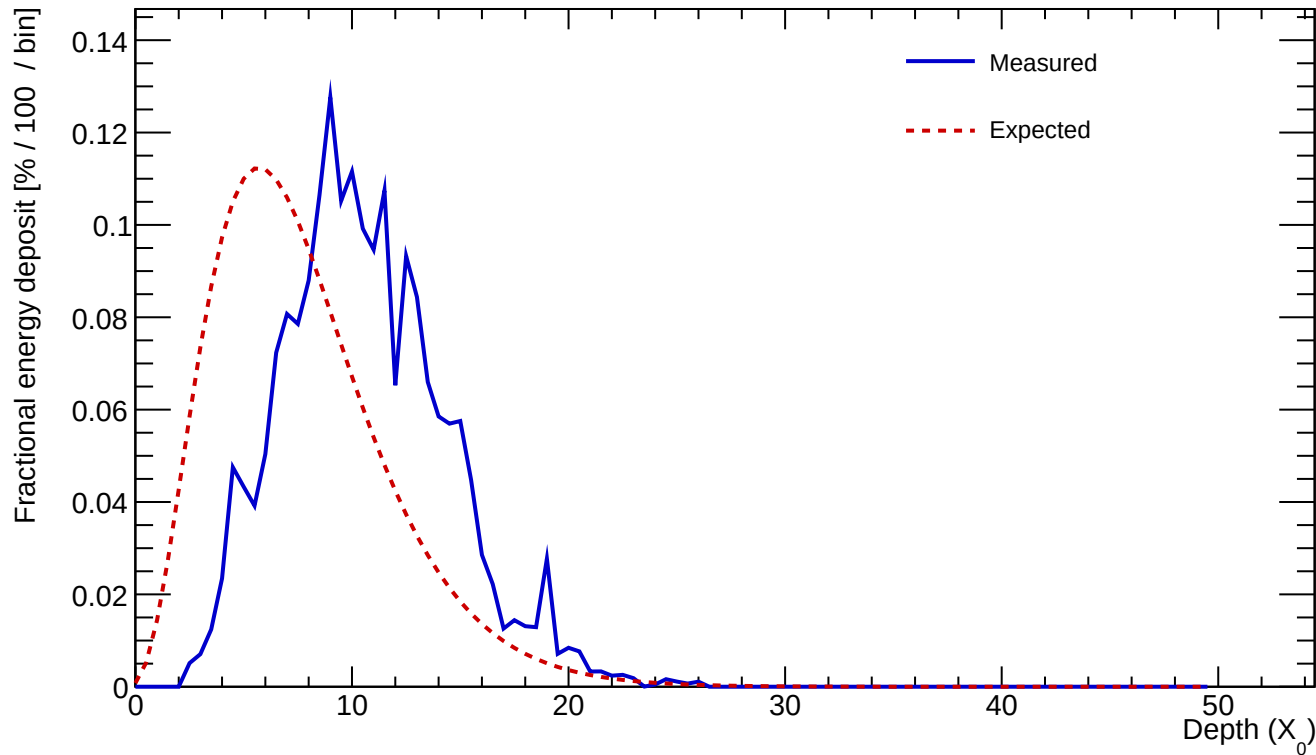
Cluster 313 E=24.058 GeV profileStart=3.50 X_0 \chi=0.1796
