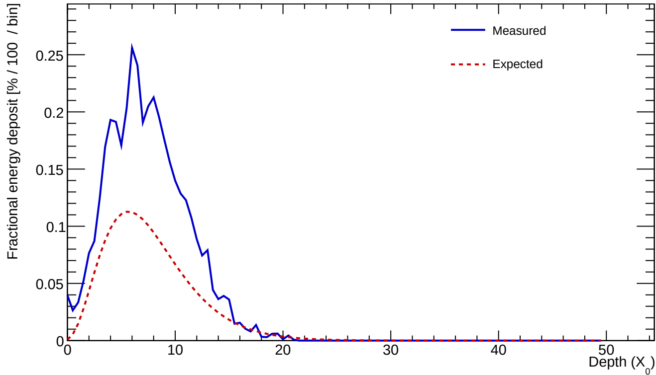
Cluster 18 E=23.236 GeV profileStart=0.50 X_0 \chi=0.1385
