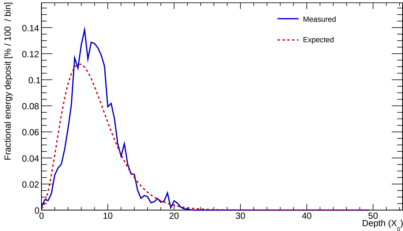
Cluster 586 E=24.534 GeV profileStart=1.00 X_0 \chi=0.1866
