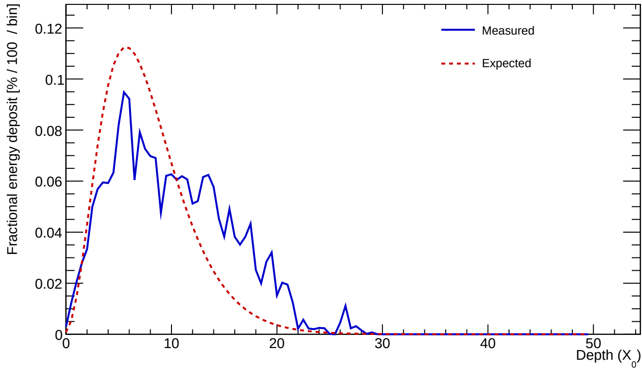
Cluster 335 E=23.768 GeV profileStart=0.50 X_0 \chi=0.4358
