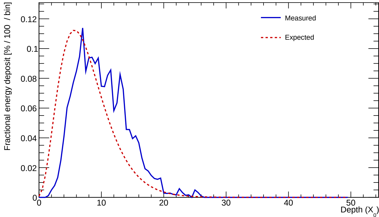
Cluster 419 E=24.107 GeV profileStart=2.00 X_0 \chi=0.1642
