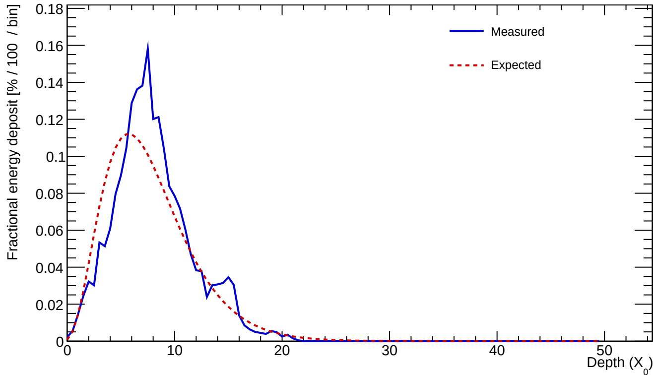
Cluster 352 E=24.615 GeV profileStart=0.50 X_0 \chi=0.2004
