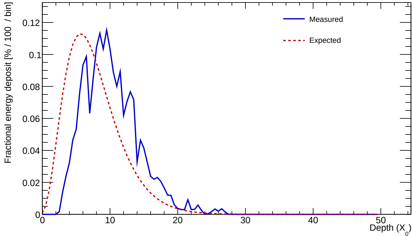
Cluster 256 E=22.940 GeV profileStart=2.50 X_0 \chi=0.1411
