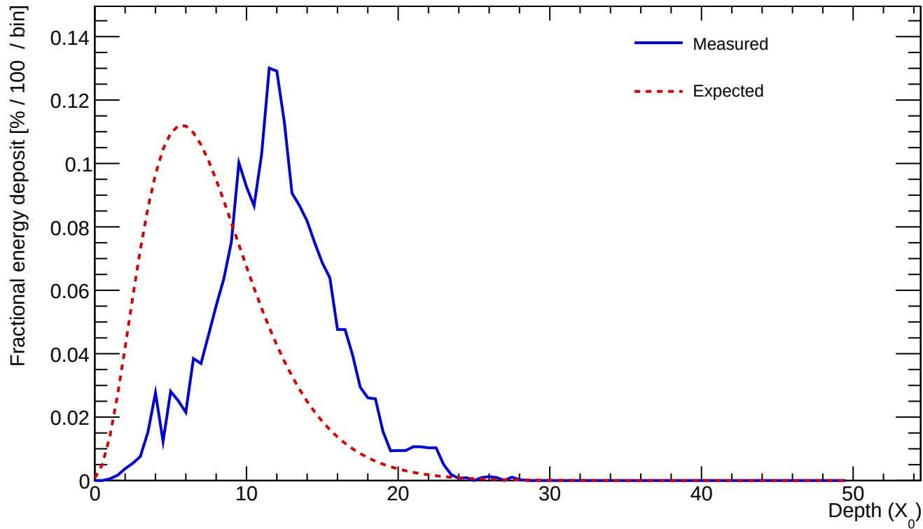
Cluster 35 E=24.696 GeV profileStart=5.00 X_0 \chi=0.2129
