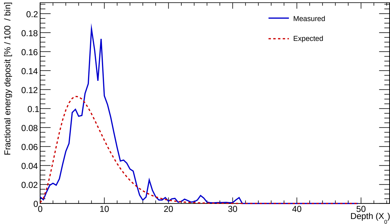
Cluster 619 E=23.033 GeV profileStart=1.50 X_0 \chi=0.2556
