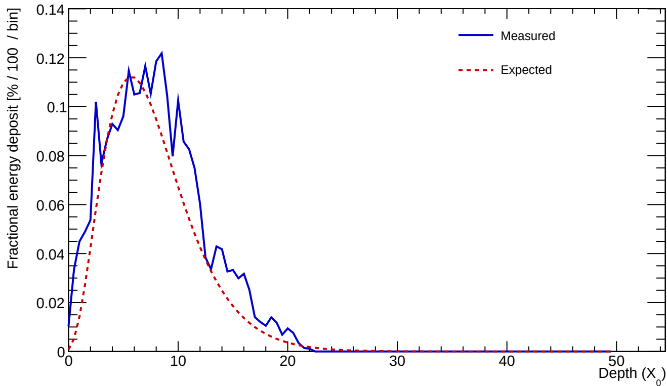
Cluster 646 E=24.395 GeV profileStart=0.50 X_0 \chi=0.2209
