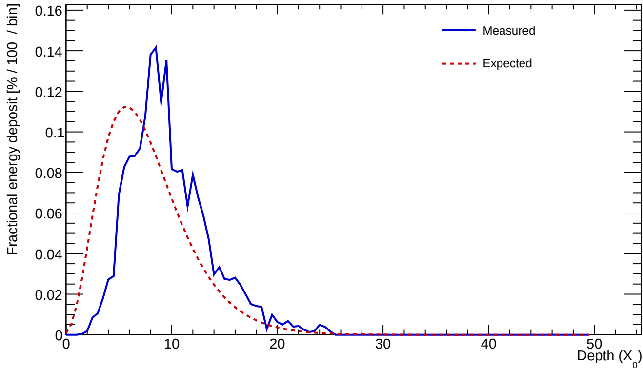
Cluster 683 E=23.954 GeV profileStart=2.50 X_0 \chi=0.1543
