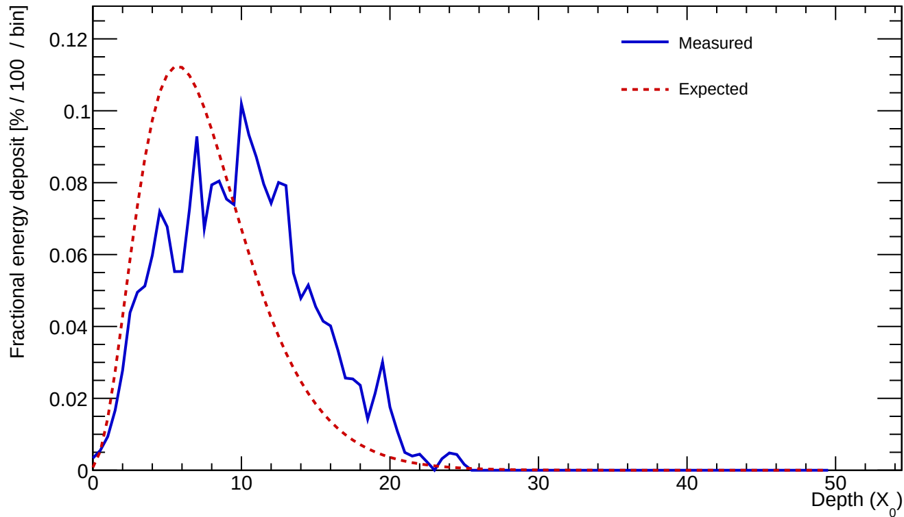
Cluster 280 E=23.979 GeV profileStart=2.00 X_0 \chi=0.3372
