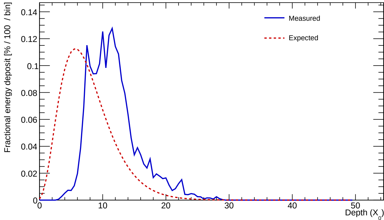
Cluster 361 E=23.841 GeV profileStart=4.50 X_0 \chi=0.1879
