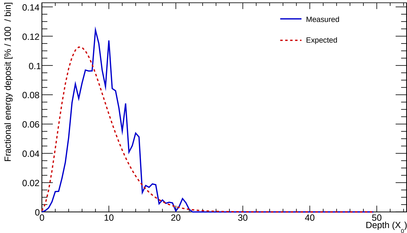
Cluster 435 E=23.452 GeV profileStart=1.50 X_0 \chi=0.1677
