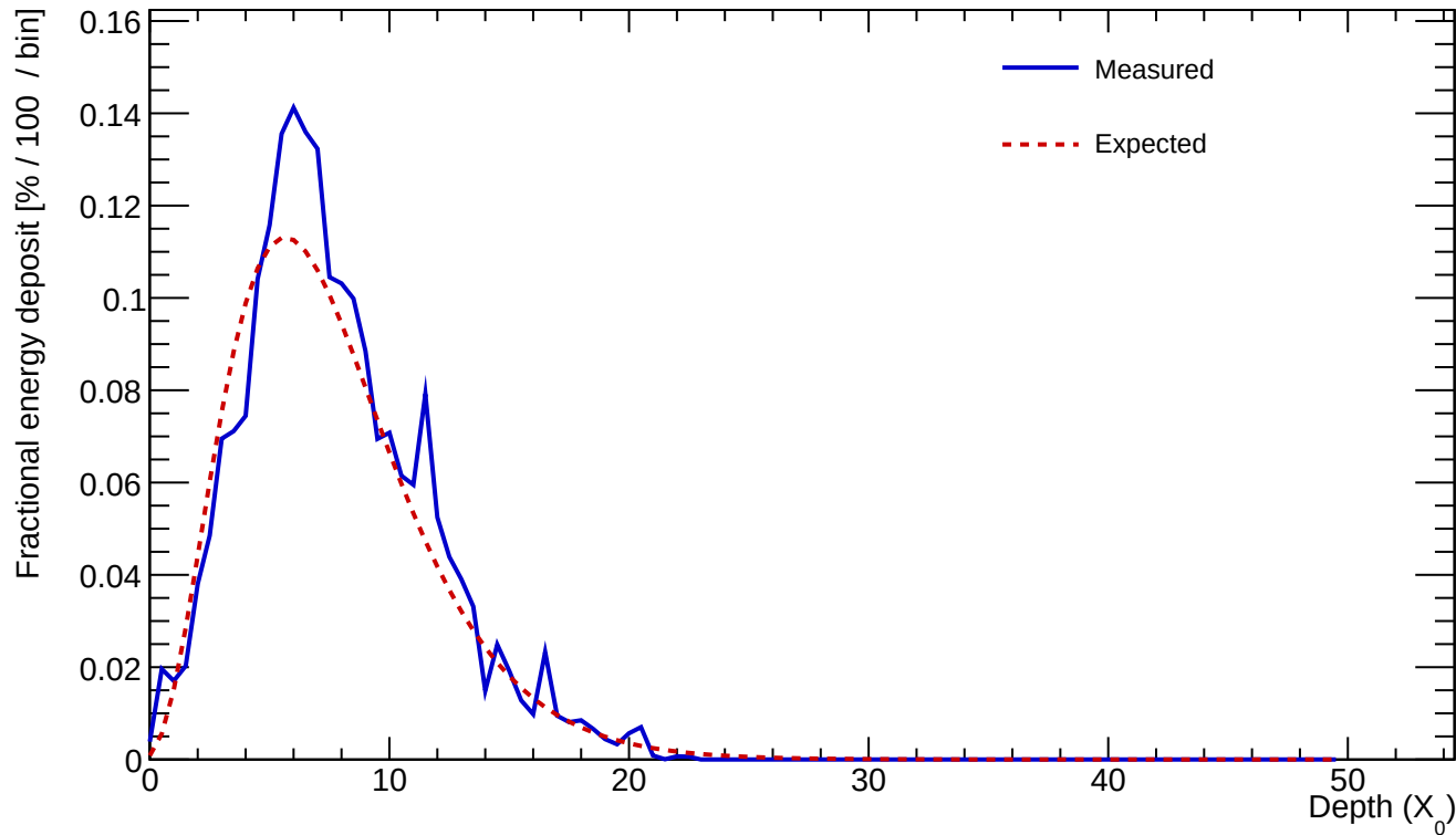
Cluster 610 E=22.643 GeV profileStart=0.50 X_0 \chi=0.1368
