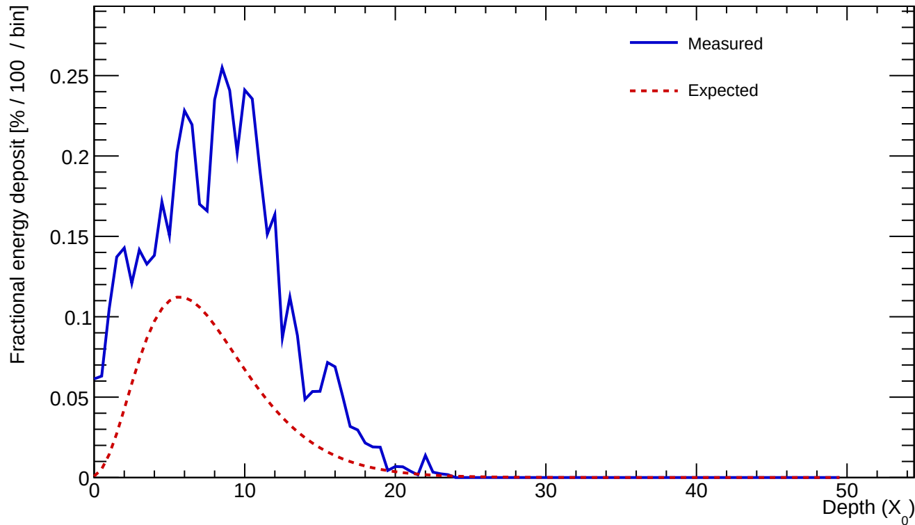
Cluster 263 E=24.124 GeV profileStart=1.00 X_0 \chi=0.3007
