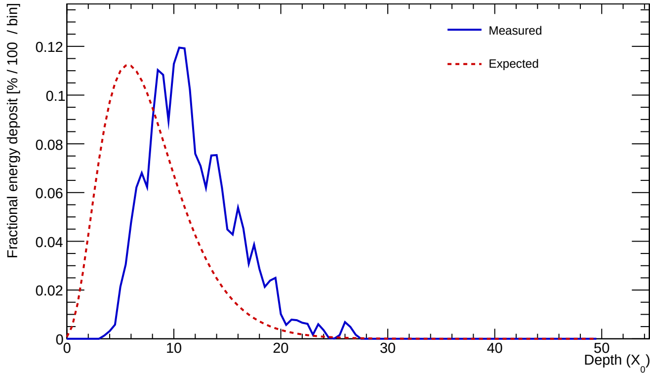
Cluster 545 E=24.201 GeV profileStart=4.00 X_0 \chi=0.1409
