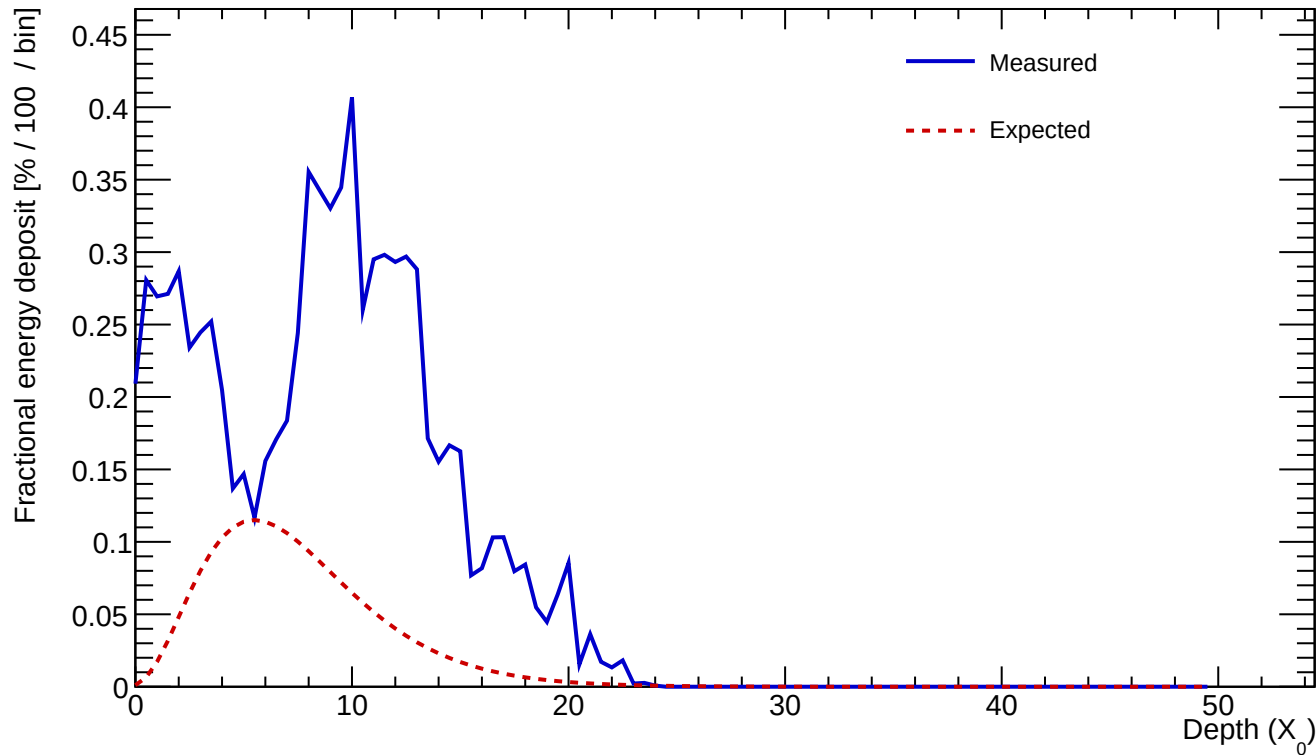
Cluster 460 E=19.344 GeV profileStart=3.00 X_0 \chi=0.5329
