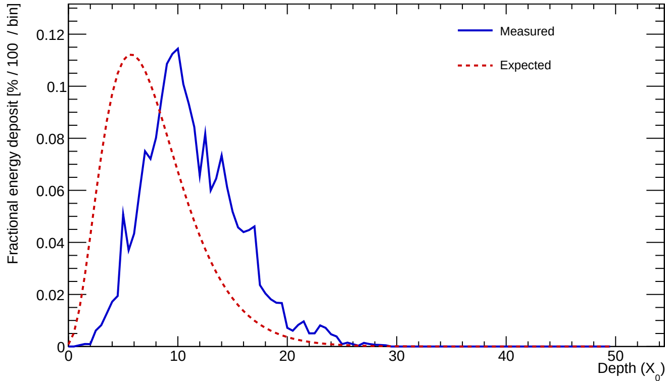
Cluster 407 E=24.230 GeV profileStart=4.00 X_0 \chi=0.1650
