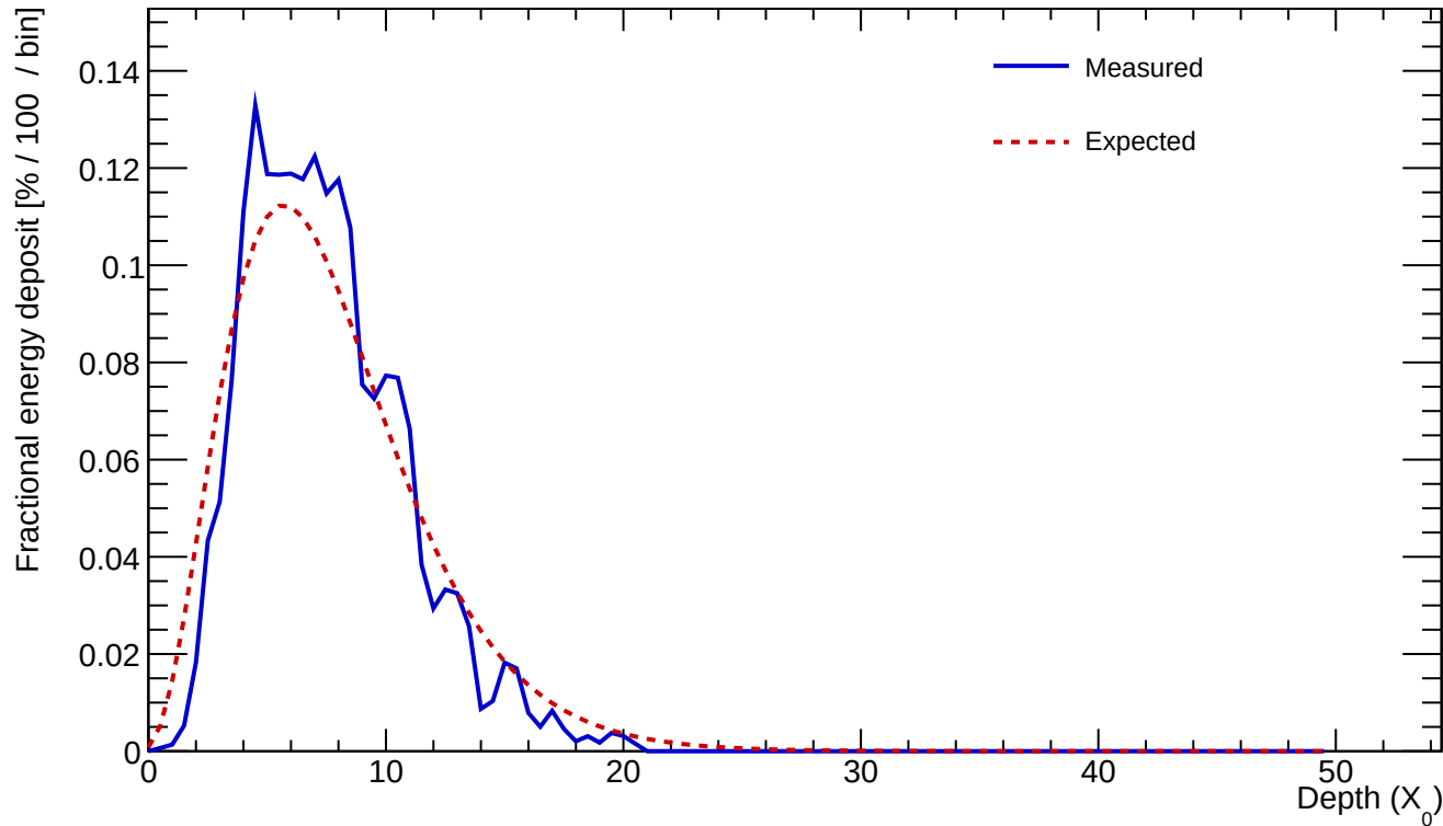
Cluster 112 E=24.050 GeV profileStart=0.50 X_0 \chi=0.1841
