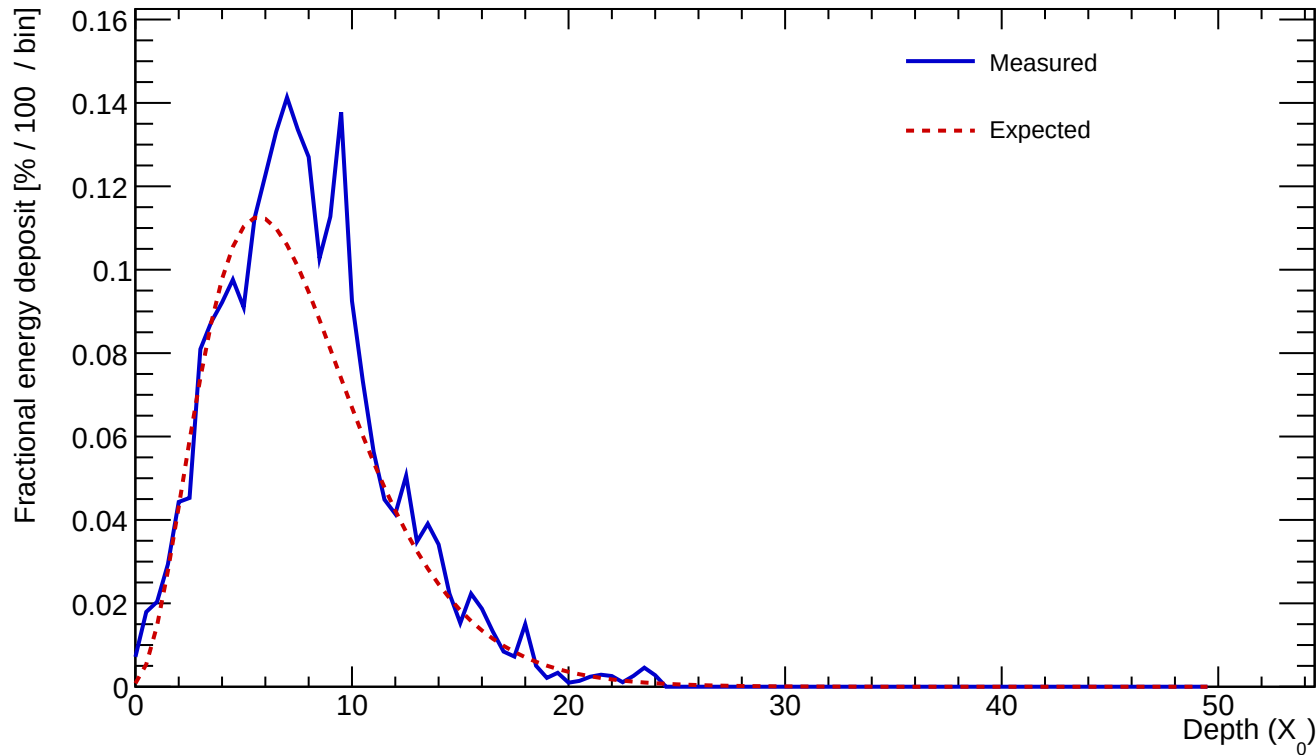
Cluster 388 E=23.597 GeV profileStart=0.50 X_0 \chi=0.1638
