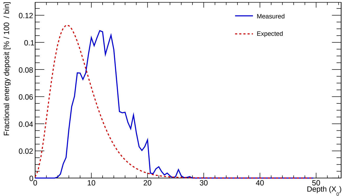
Cluster 635 E=23.325 GeV profileStart=4.50 X_0 \chi=0.1564
