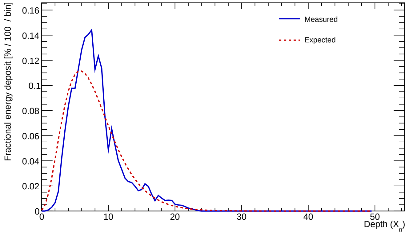
Cluster 549 E=25.816 GeV profileStart=0.50 X_0 \chi=0.2206
