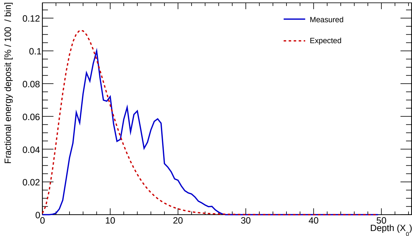
Cluster 154 E=23.600 GeV profileStart=2.50 X_0 \chi=0.3482
