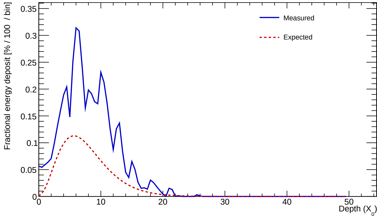
Cluster 441 E=22.762 GeV profileStart=0.50 X_0 \chi=0.2364
