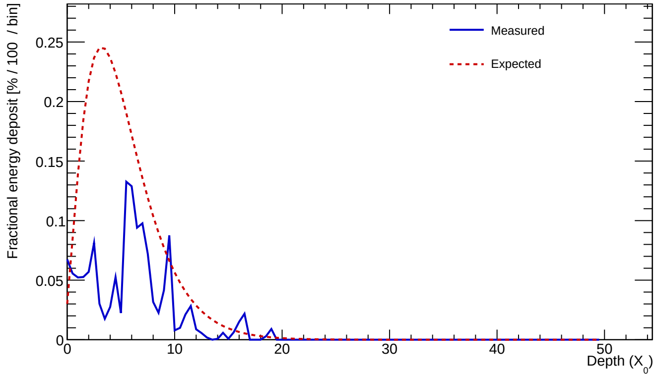
Cluster 508 E=1.958 GeV profileStart=0.50 X_0 \chi=0.6362
