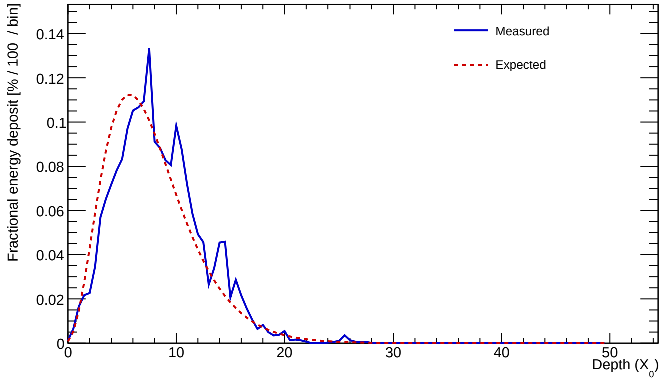
Cluster 32 E=23.842 GeV profileStart=1.00 X_0 \chi=0.1687
