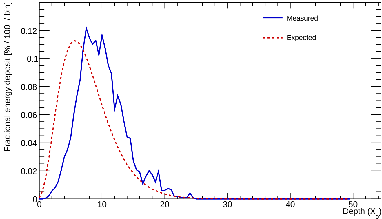
Cluster 578 E=23.243 GeV profileStart=3.00 X_0 \chi=0.1393
