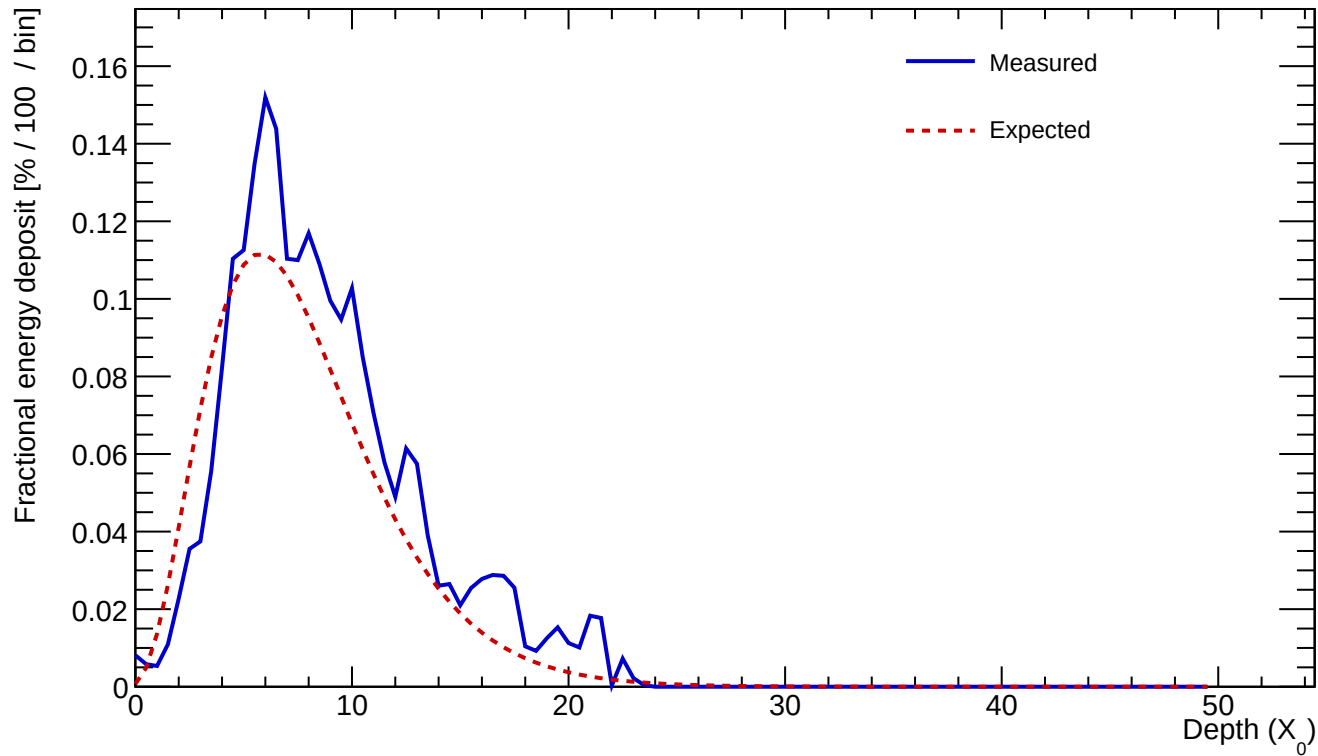
Cluster 570 E=25.704 GeV profileStart=1.00 X_0 \chi=0.1641
