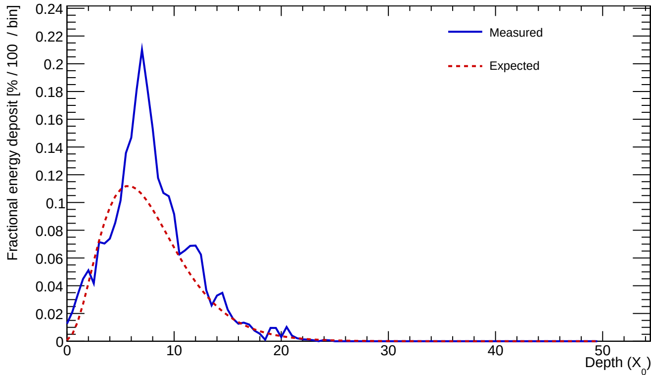
Cluster 312 E=24.861 GeV profileStart=0.50 X_0 \chi=0.2306
