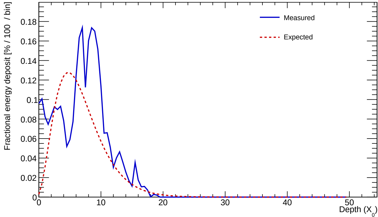
Cluster 171 E=9.272 GeV profileStart=0.50 X_0 \chi=0.4305
