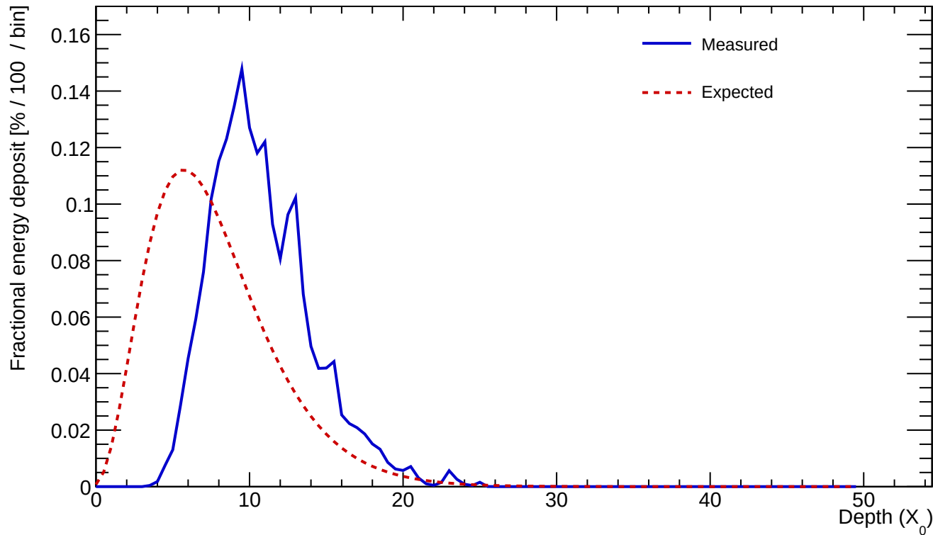
Cluster 238 E=24.480 GeV profileStart=3.50 X_0 \chi=0.2007
