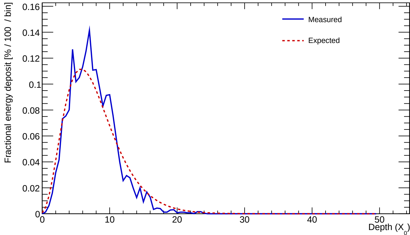
Cluster 246 E=25.758 GeV profileStart=0.50 X_0 \chi=0.1798
