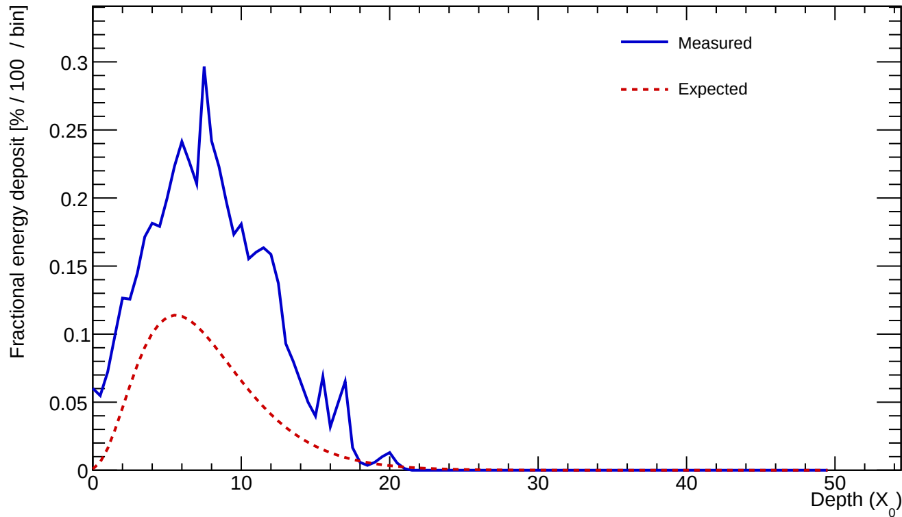
Cluster 685 E=21.149 GeV profileStart=0.50 X_0 \chi=0.2160
