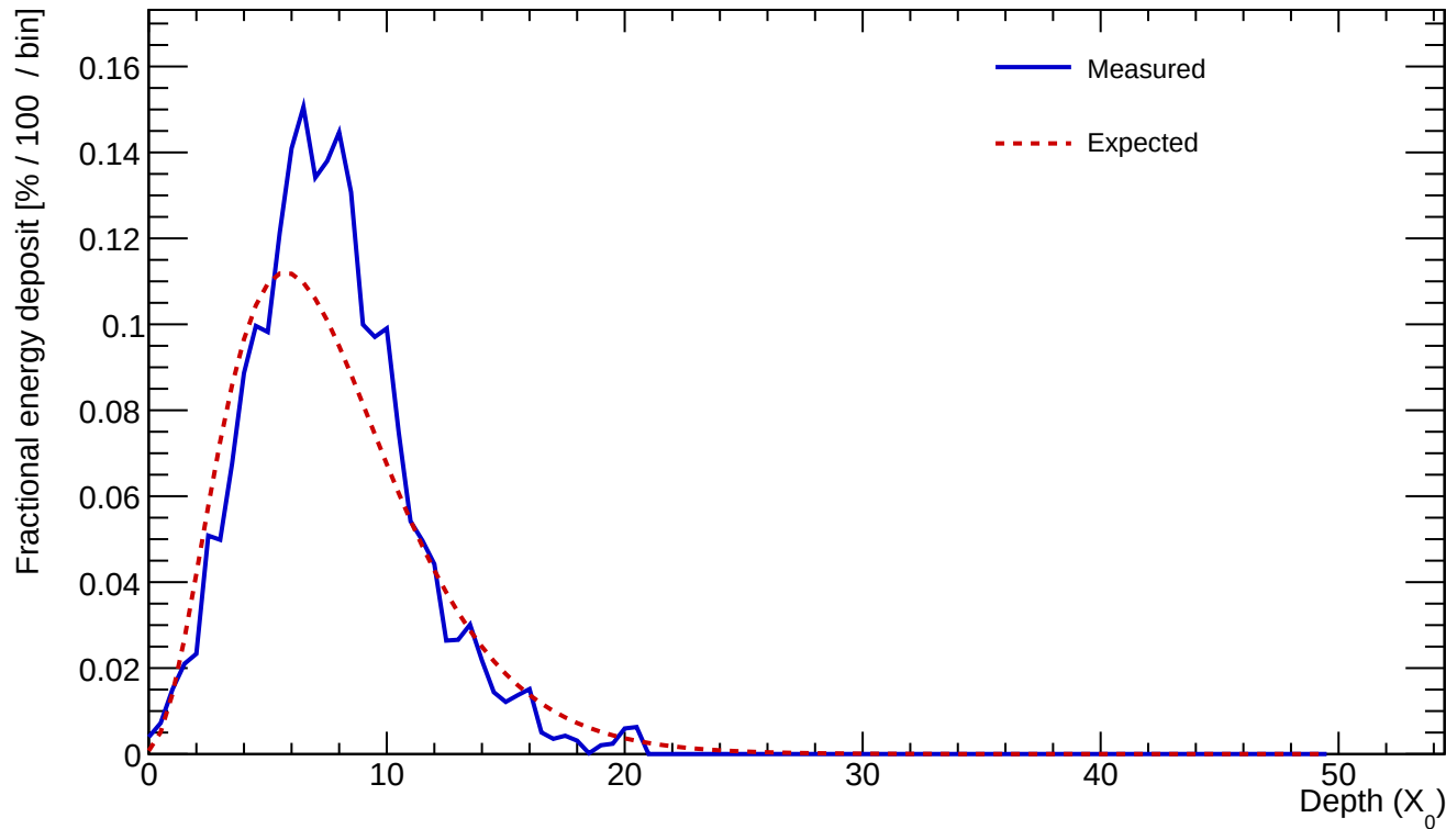
Cluster 339 E=24.786 GeV profileStart=0.50 X_0 \chi=0.1968
