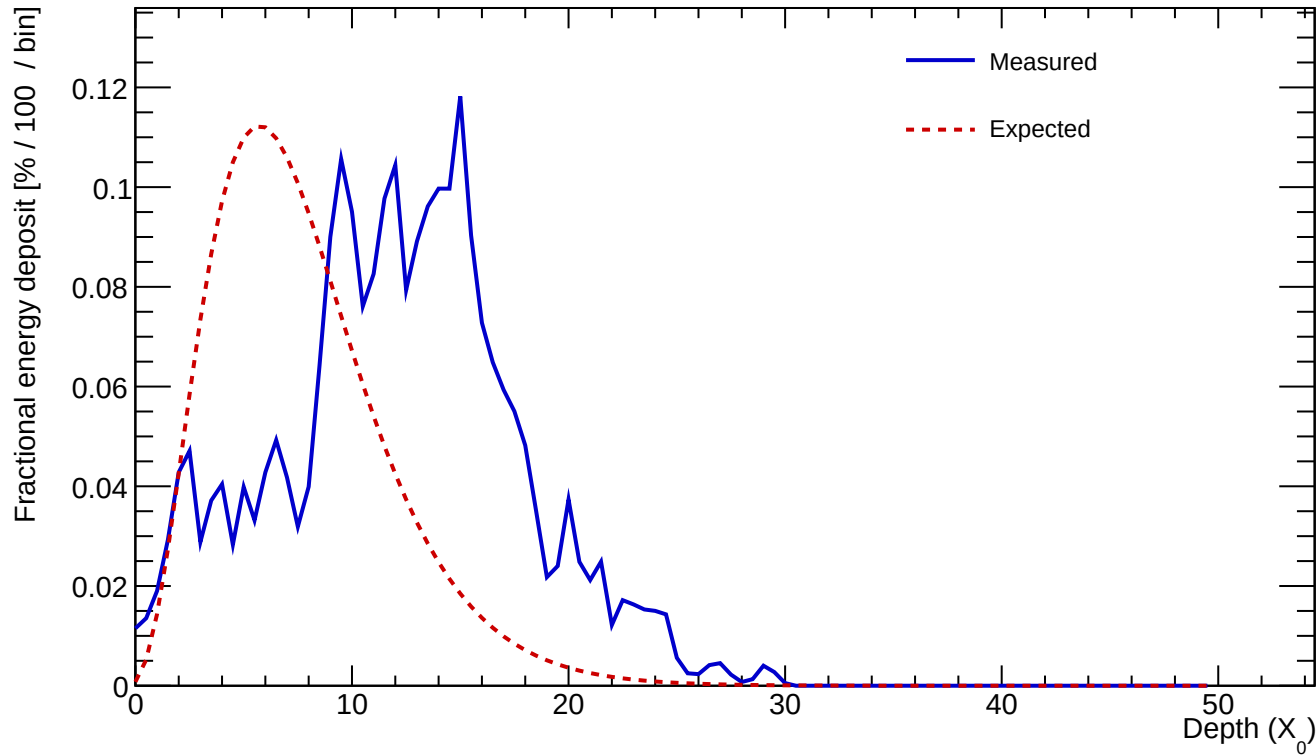
Cluster 164 E=24.145 GeV profileStart=6.00 X_0 \chi=0.4131
