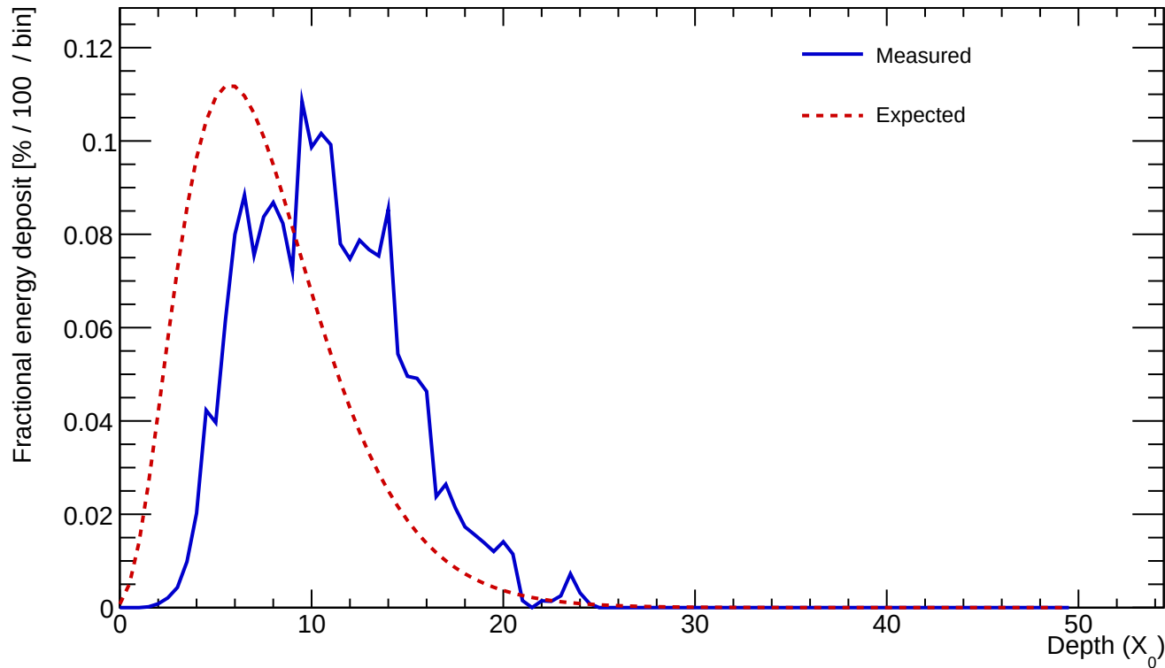
Cluster 347 E=24.916 GeV profileStart=3.00 X_0 \chi=0.1746
