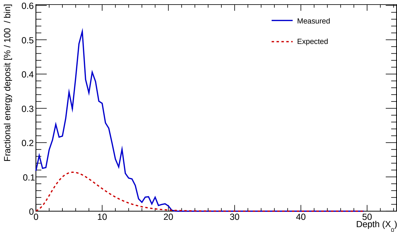
Cluster 517 E=21.446 GeV profileStart=0.50 X_0 \chi=0.2224
