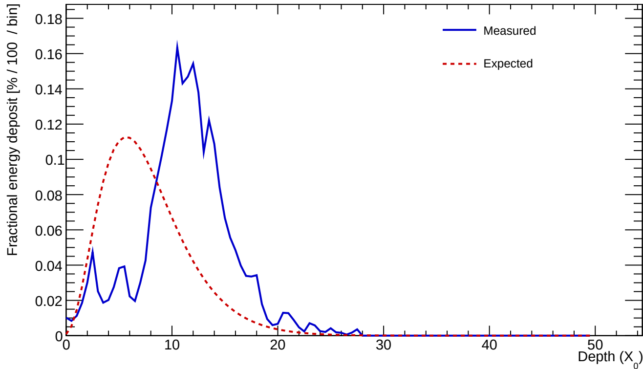
Cluster 247 E=23.448 GeV profileStart=5.50 X_0 \chi=0.3062
