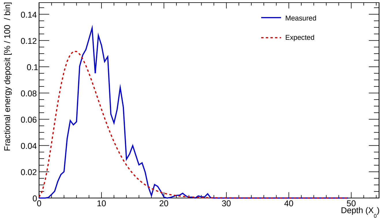
Cluster 677 E=25.080 GeV profileStart=2.50 X_0 \chi=0.1927
