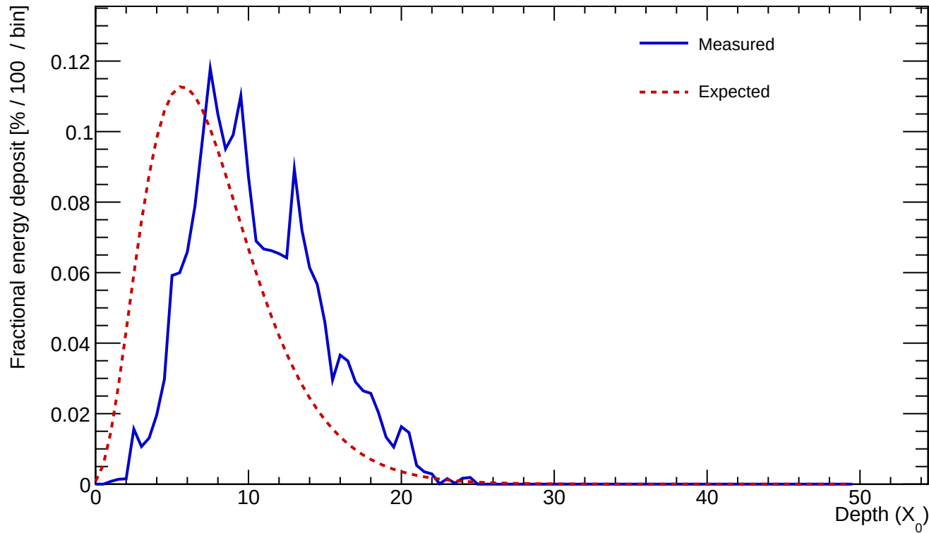
Cluster 553 E=23.220 GeV profileStart=3.00 X_0 \chi=0.1857
