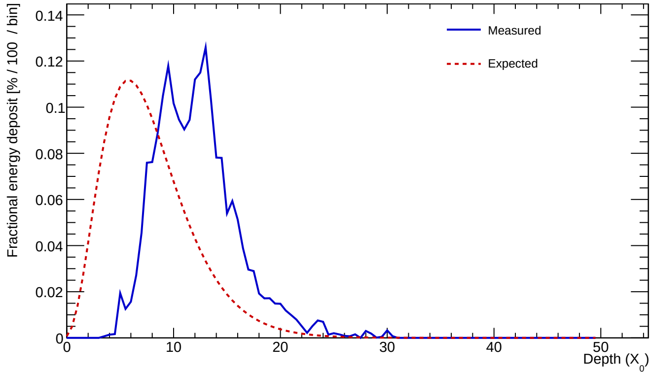
Cluster 88 E=25.577 GeV profileStart=4.50 X_0 \chi=0.1684
