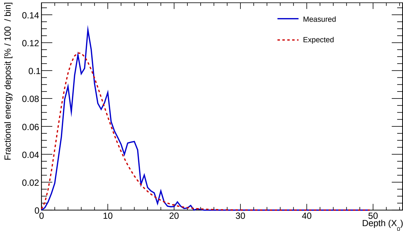
Cluster 189 E=23.334 GeV \text{profileStart}=0.50 X_0 \chi=0.1450
