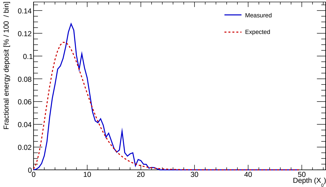
Cluster 41 E=24.330 GeV profileStart=1.00 X_0 \chi=0.1138
