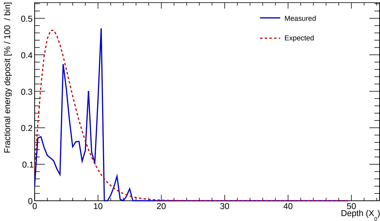
Cluster 301 E=1.283 GeV profileStart=0.50 X_0 \chi=0.6243
