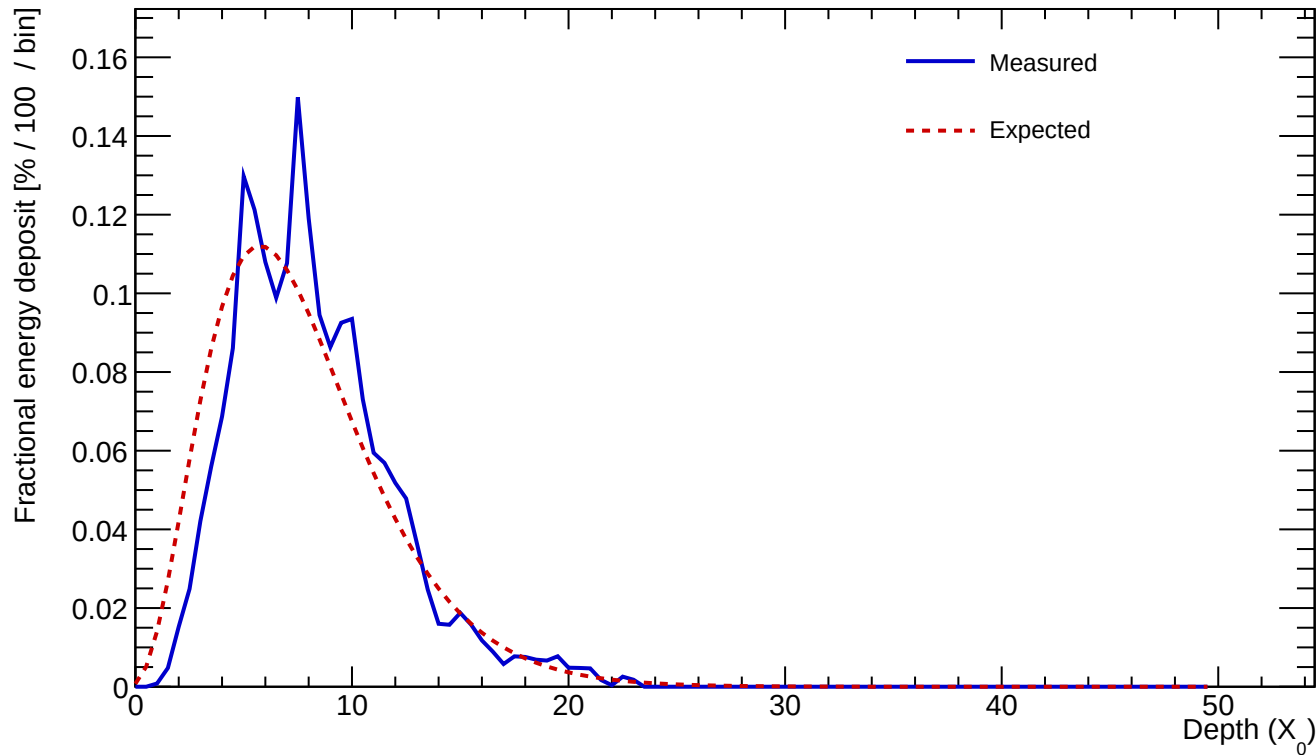
Cluster 298 E=24.691 GeV profileStart=1.00 X_0 \chi=0.1349
