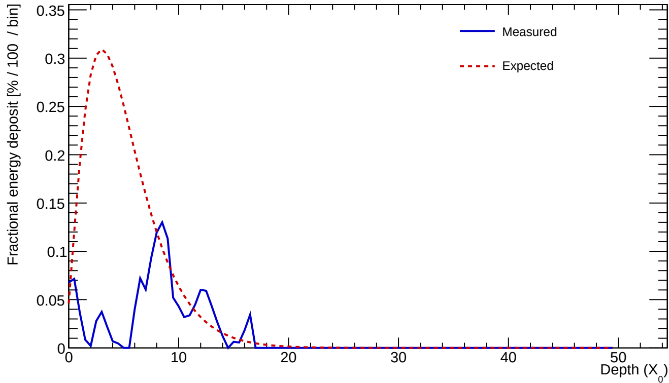
Cluster 483 E=1.608 GeV profileStart=5.50 X_0 \chi=0.5065
