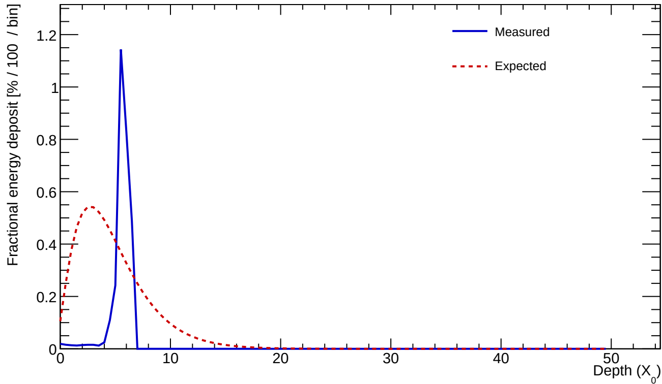
Cluster 658 E=1.215 GeV profileStart=4.00 X_0 \chi=0.6115
