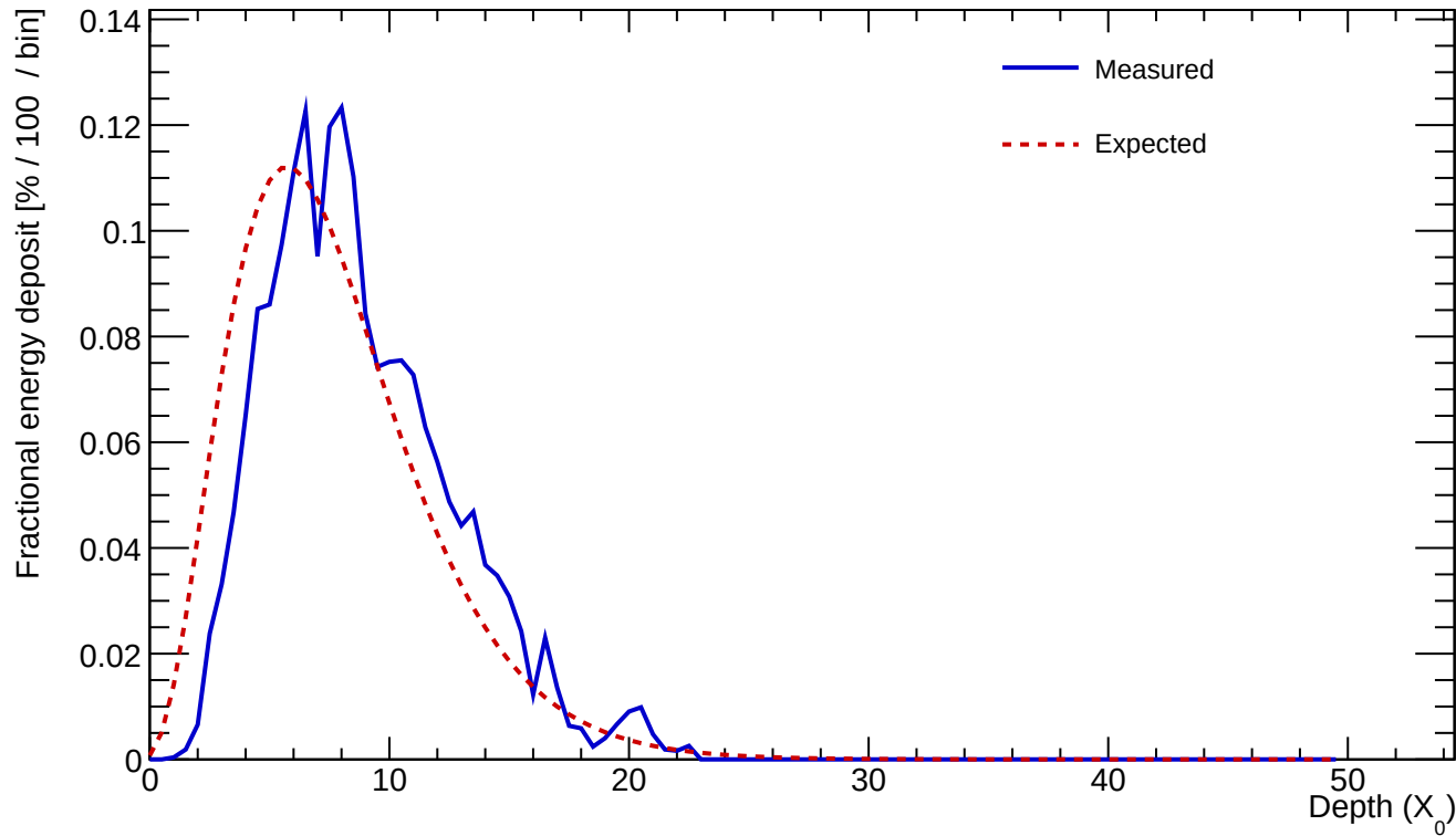
Cluster 252 E=24.652 GeV profileStart=1.00 X_0 \chi=0.1234
