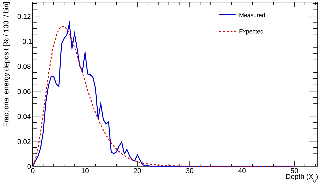
Cluster 316 E=24.737 GeV \text{profileStart}=0.50 X_0 \chi=0.1610
