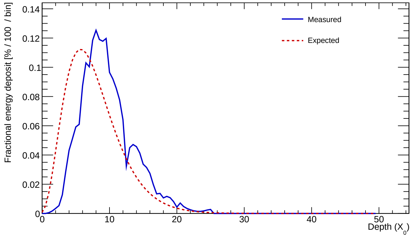
Cluster 120 E=24.183 GeV profileStart=2.00 X_0 \chi=0.1168
