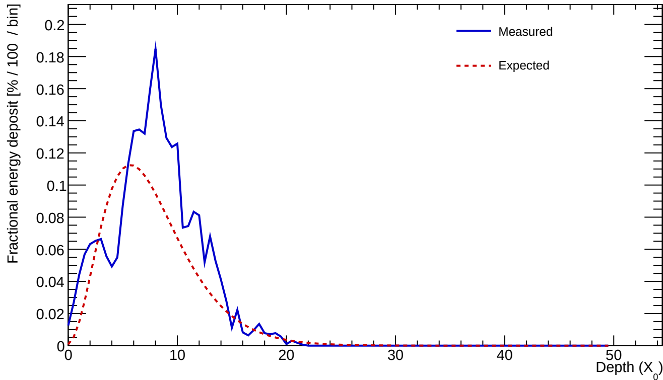
Cluster 46 E=23.742 GeV profileStart=1.50 X_0 \chi=0.2699
