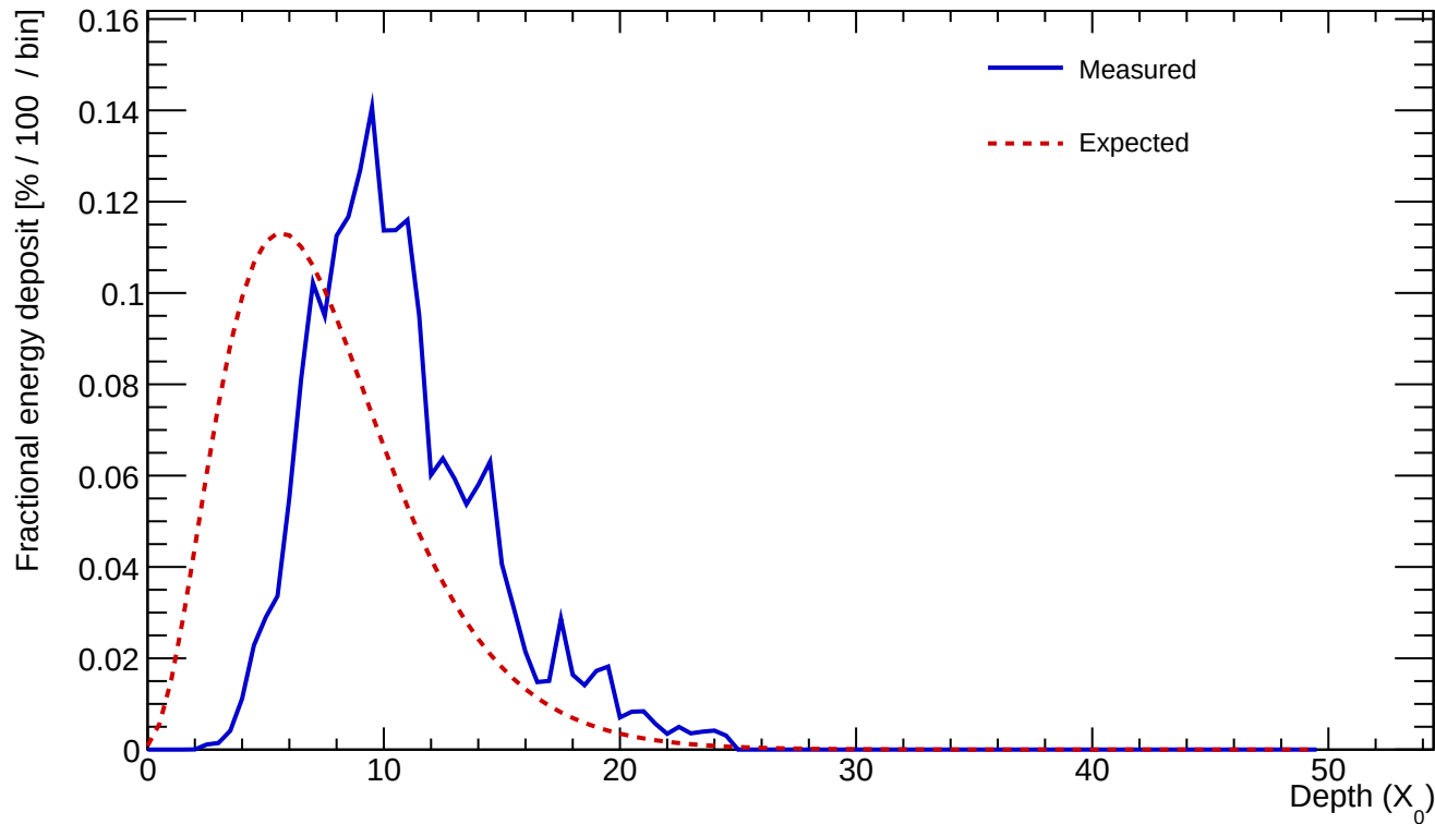
Cluster 293 E=22.469 GeV profileStart=3.50 X_0 \chi=0.1617
