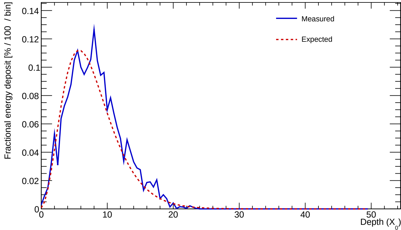
Cluster 695 E=25.051 GeV profileStart=0.50 X_0 \chi=0.1476
