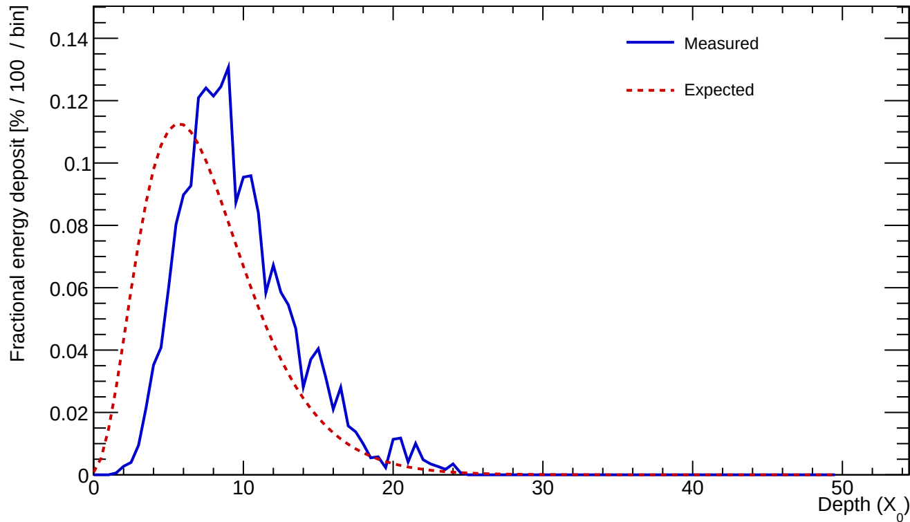
Cluster 260 E=23.444 GeV profileStart=2.00 X_0 \chi=0.1413
