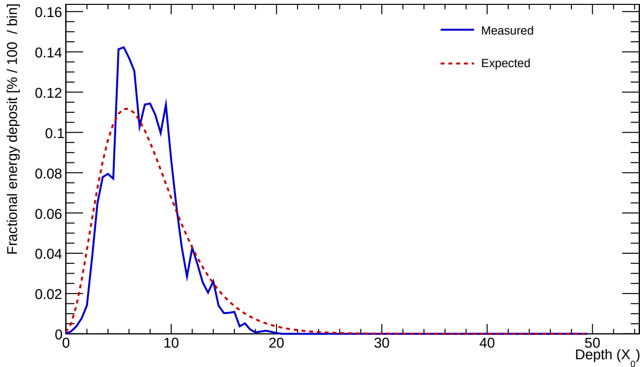
Cluster 529 E=25.019 GeV profileStart=0.50 X_0 \chi=0.2255
