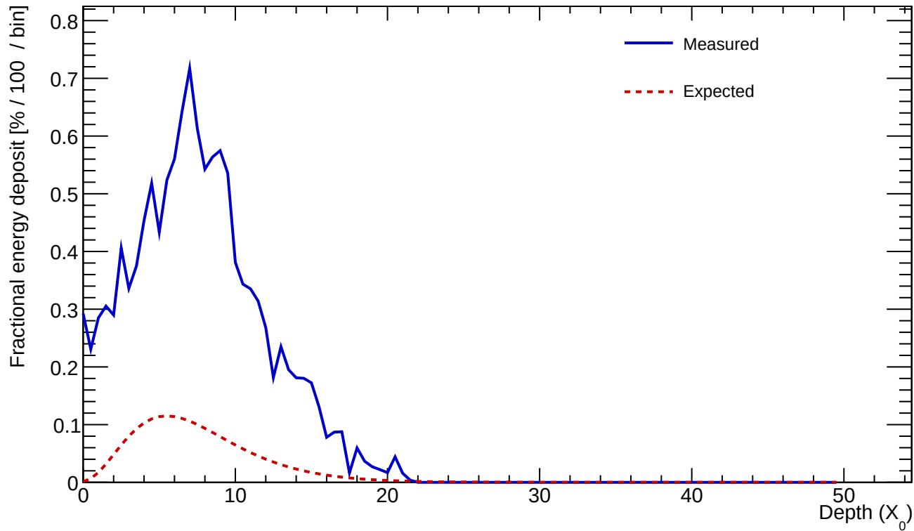
Cluster 440 E=19.362 GeV profileStart=0.50 X_0 \chi=0.2354
