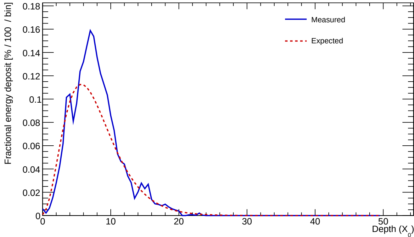
Cluster 141 E=23.562 GeV profileStart=0.50 X_0 \chi=0.1752
