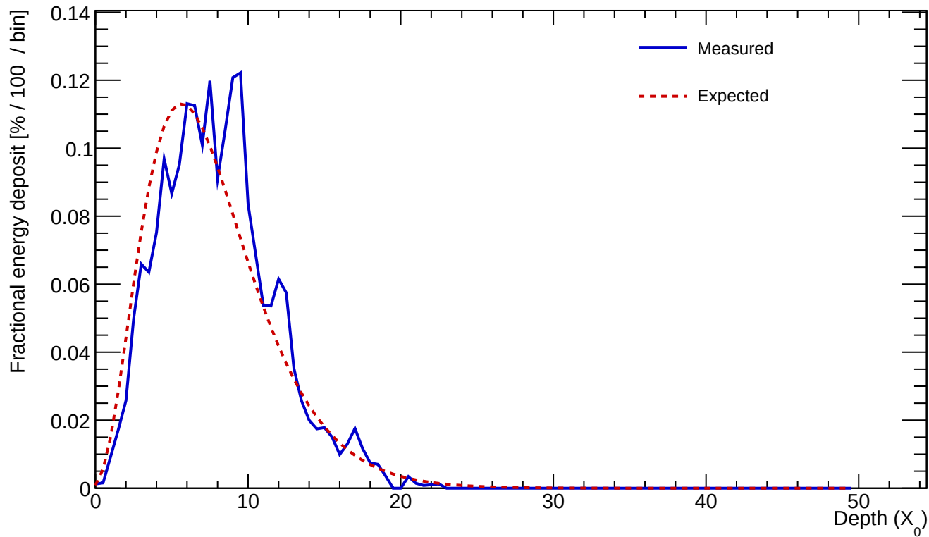
Cluster 290 E=22.578 GeV profileStart=0.50 X_0 \chi=0.1531
