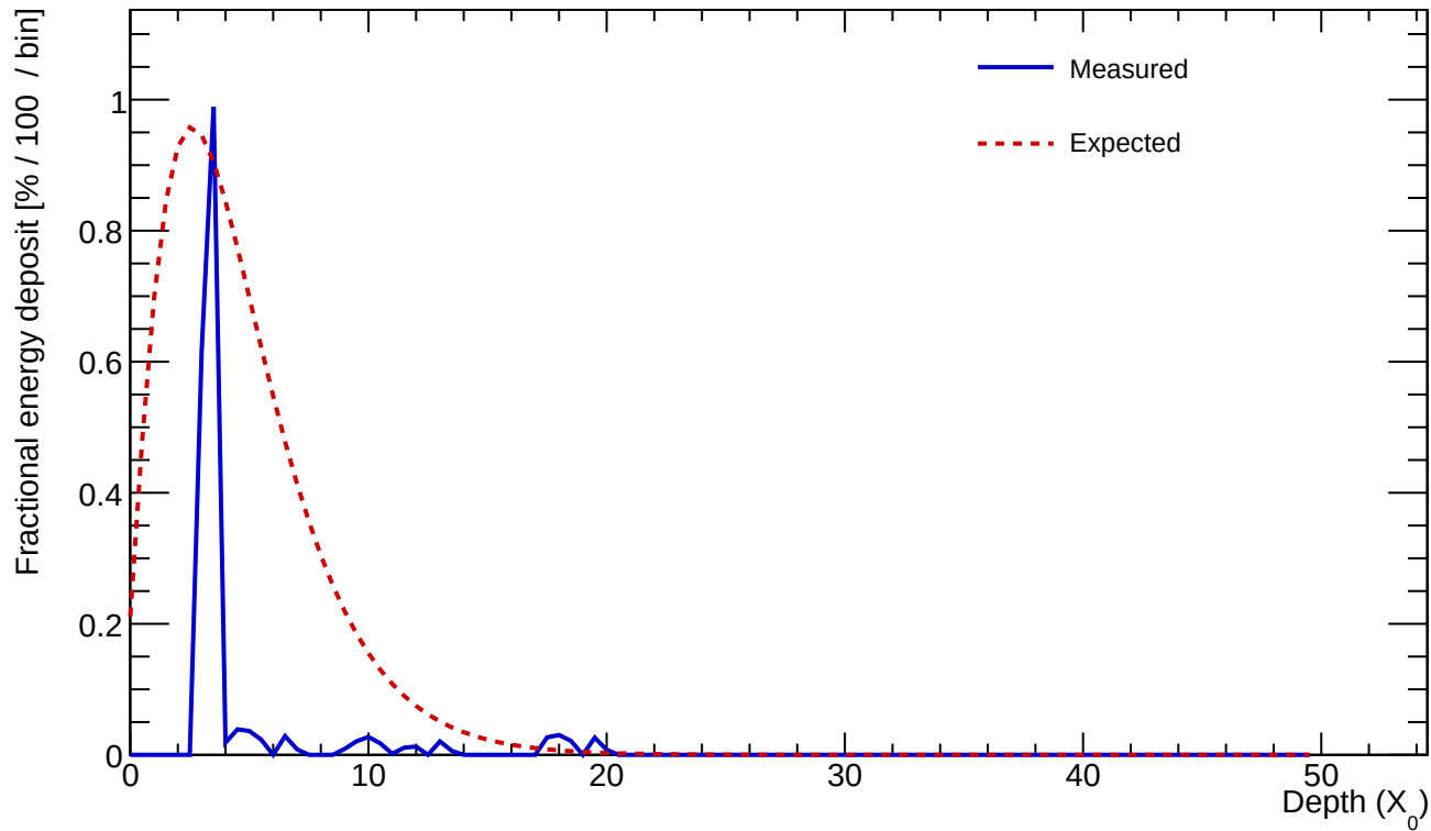
Cluster 429 E=1.057 GeV profileStart=1.00 X_0 \chi=1.4154
