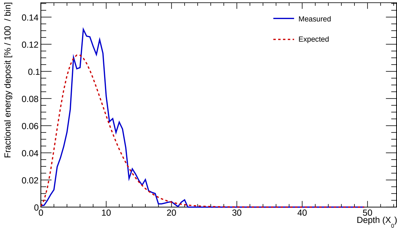
Cluster 424 E=24.446 GeV profileStart=1.00 X_0 \chi=0.1594
