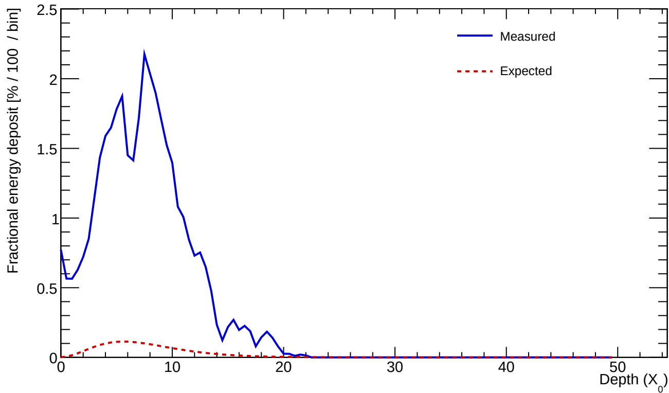
Cluster 296 E=22.202 GeV profileStart=0.50 X_0 \chi=0.1941
