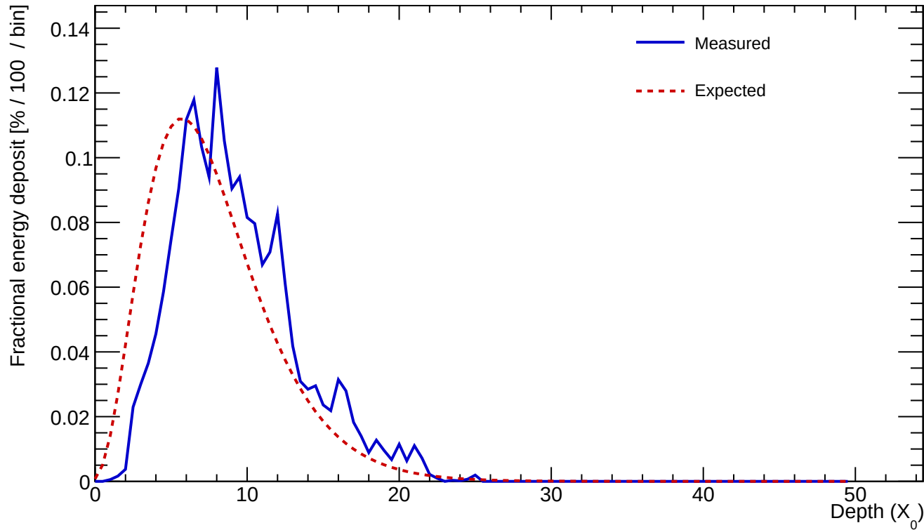
Cluster 59 E=24.551 GeV profileStart=1.50 X_0 \chi=0.1340
