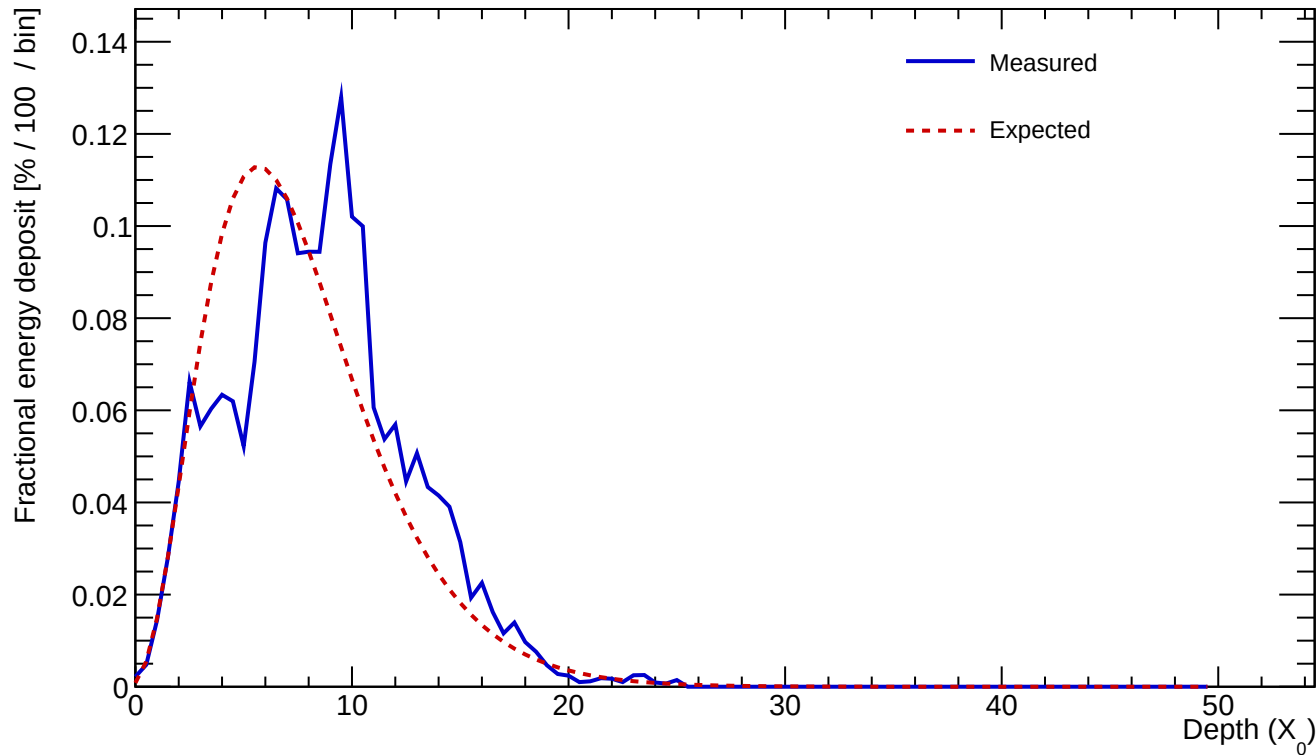
Cluster 272 E=23.102 GeV profileStart=1.00 X_0 \chi=0.2468
