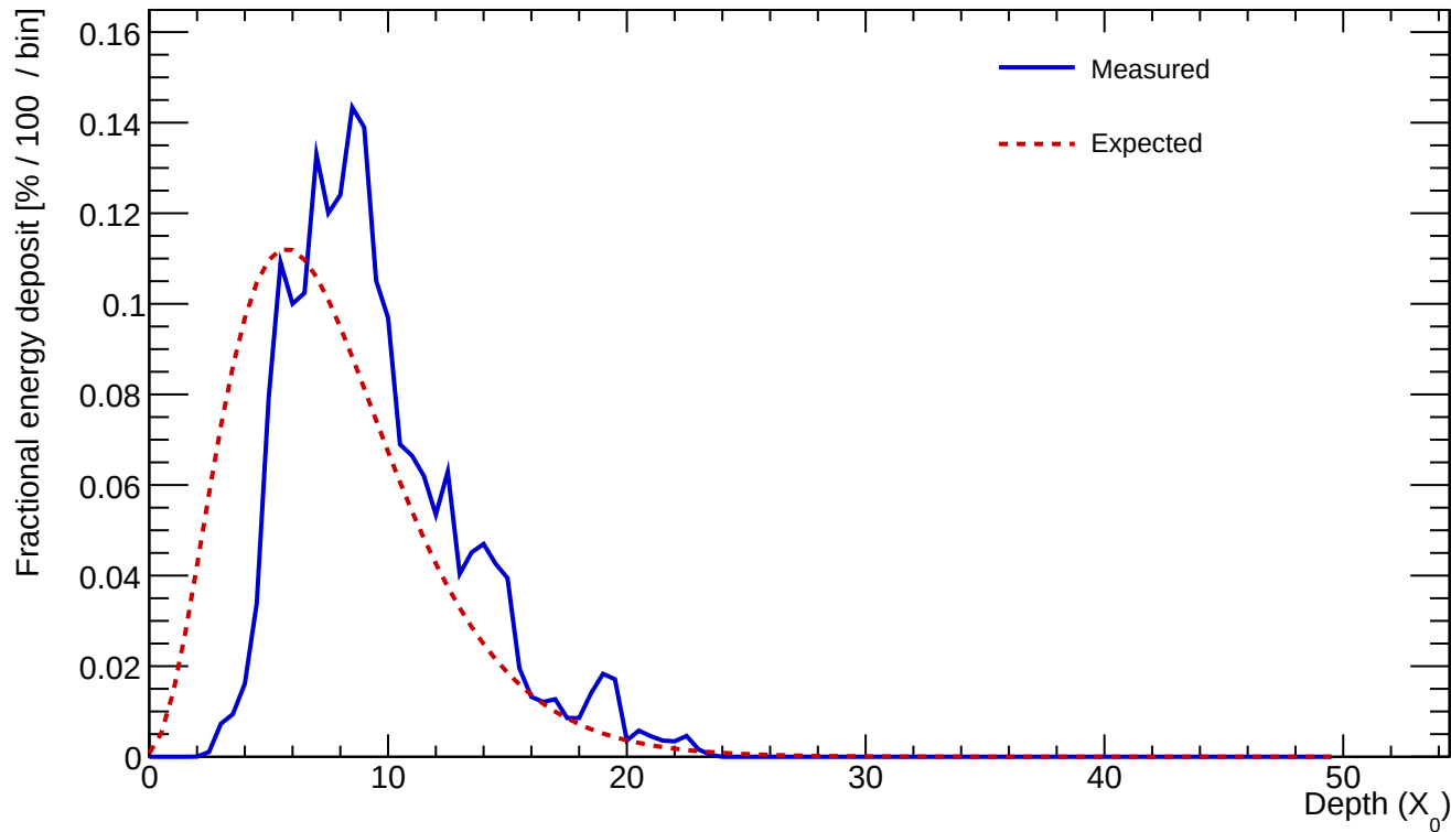
Cluster 451 E=24.502 GeV profileStart=2.00 X_0 \chi=0.2048
