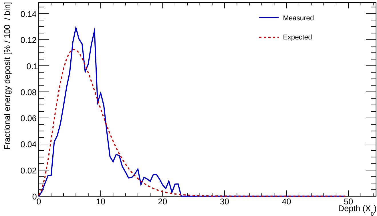
Cluster 628 E=23.612 GeV profileStart=1.00 X_0 \chi=0.1996
