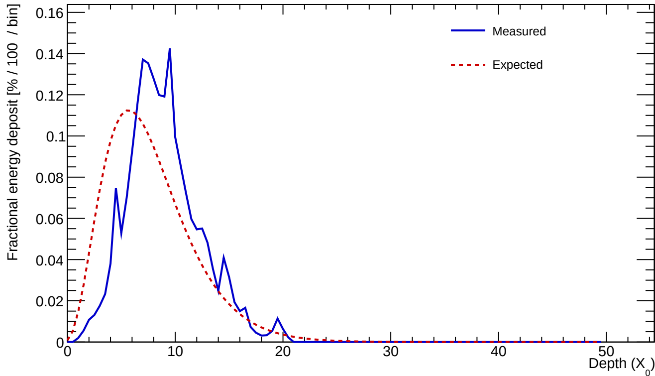
Cluster 366 E=23.763 GeV profileStart=2.00 X_0 \chi=0.1984
