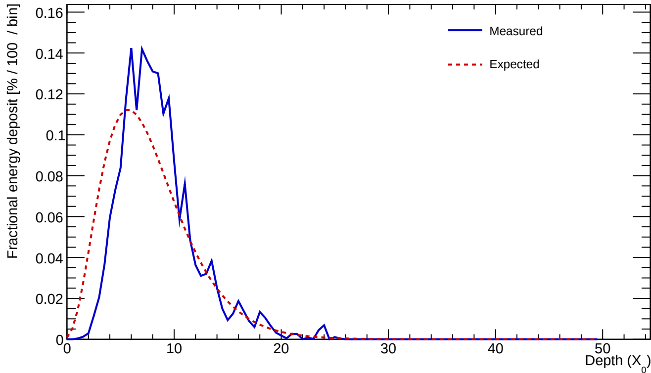
Cluster 406 E=24.241 GeV profileStart=1.50 X_0 \chi=0.2262
