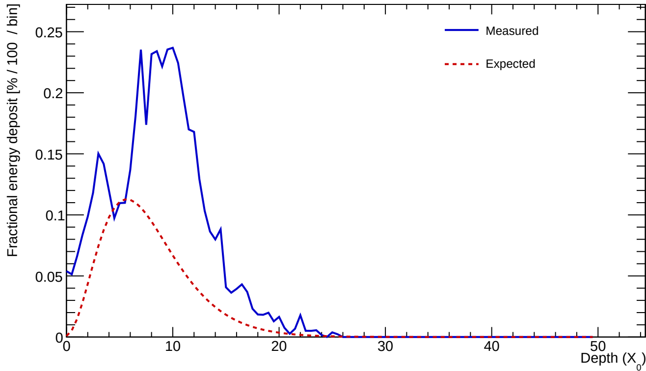
Cluster 257 E=23.314 GeV profileStart=1.50 X_0 \chi=0.3190
