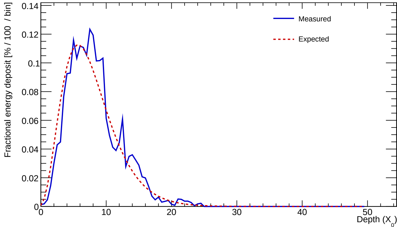
Cluster 675 E=23.840 GeV profileStart=0.50 X_0 \chi=0.1444
