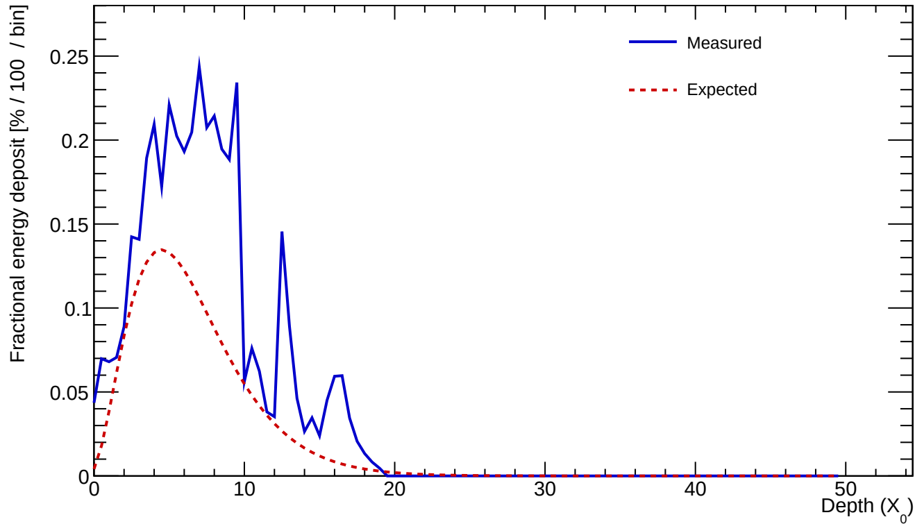
Cluster 362 E=7.114 GeV profileStart=1.00 X_0 \chi=0.2897
