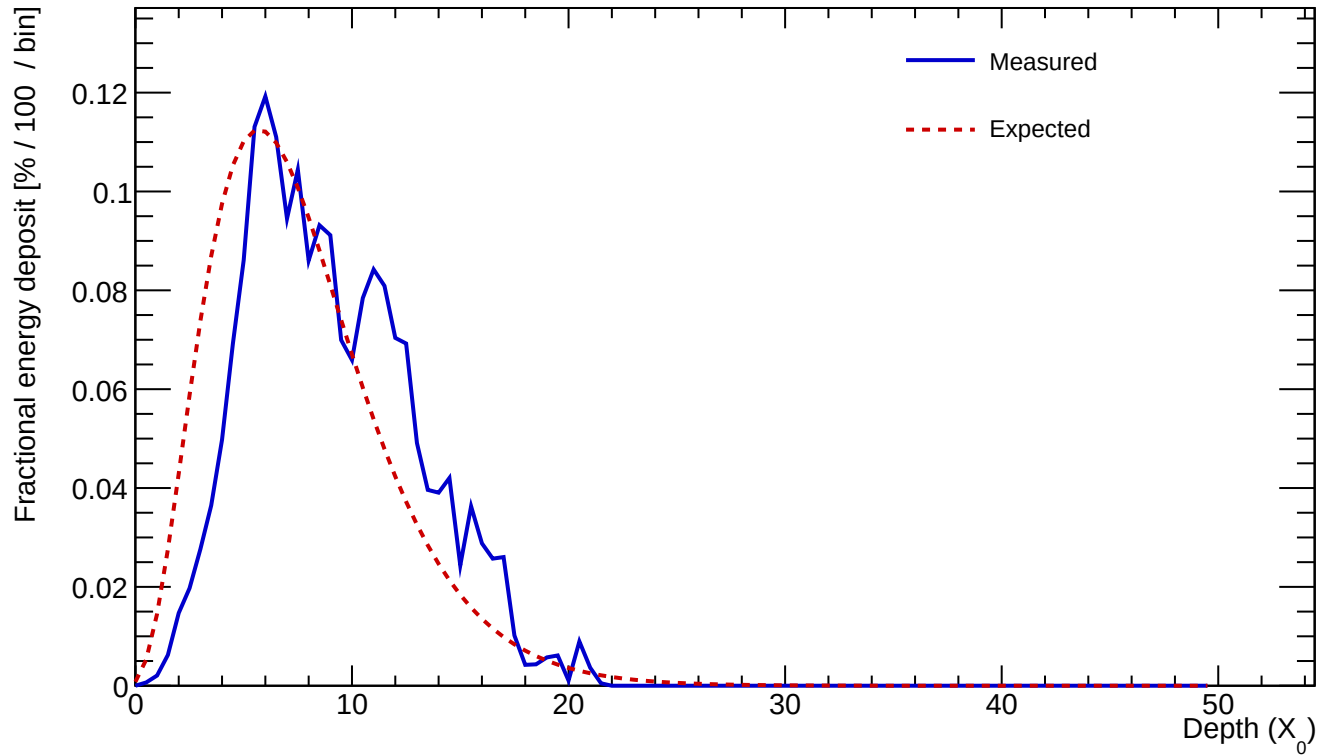
Cluster 61 E=23.833 GeV profileStart=1.50 X_0 \chi=0.1622
