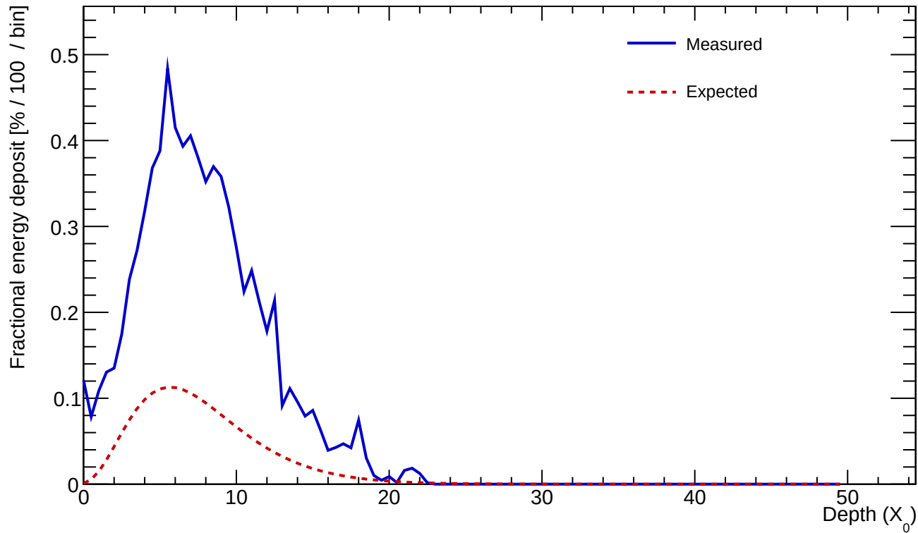
Cluster 591 E=23.008 GeV profileStart=0.50 X_0 \chi=0.1399
