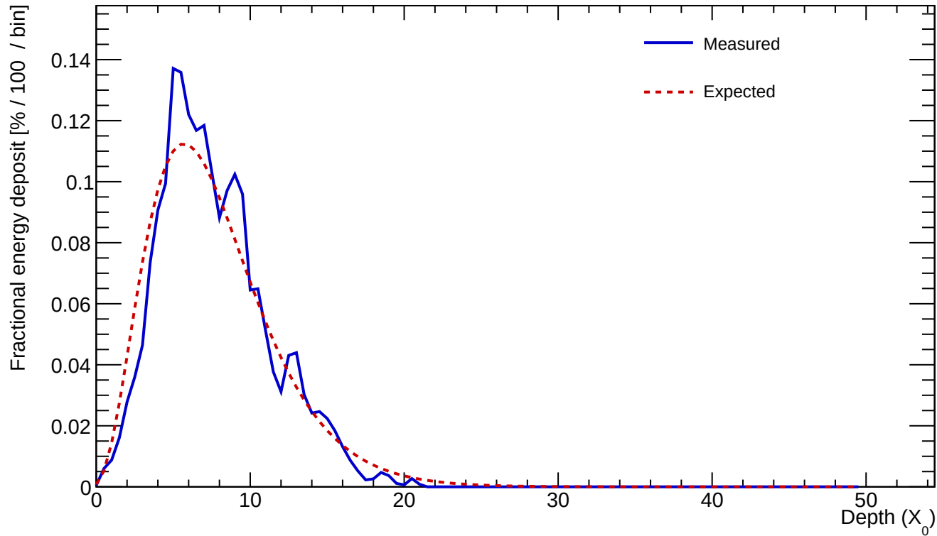
Cluster 53 E=23.987 GeV profileStart=0.50 X_0 \chi=0.1370
