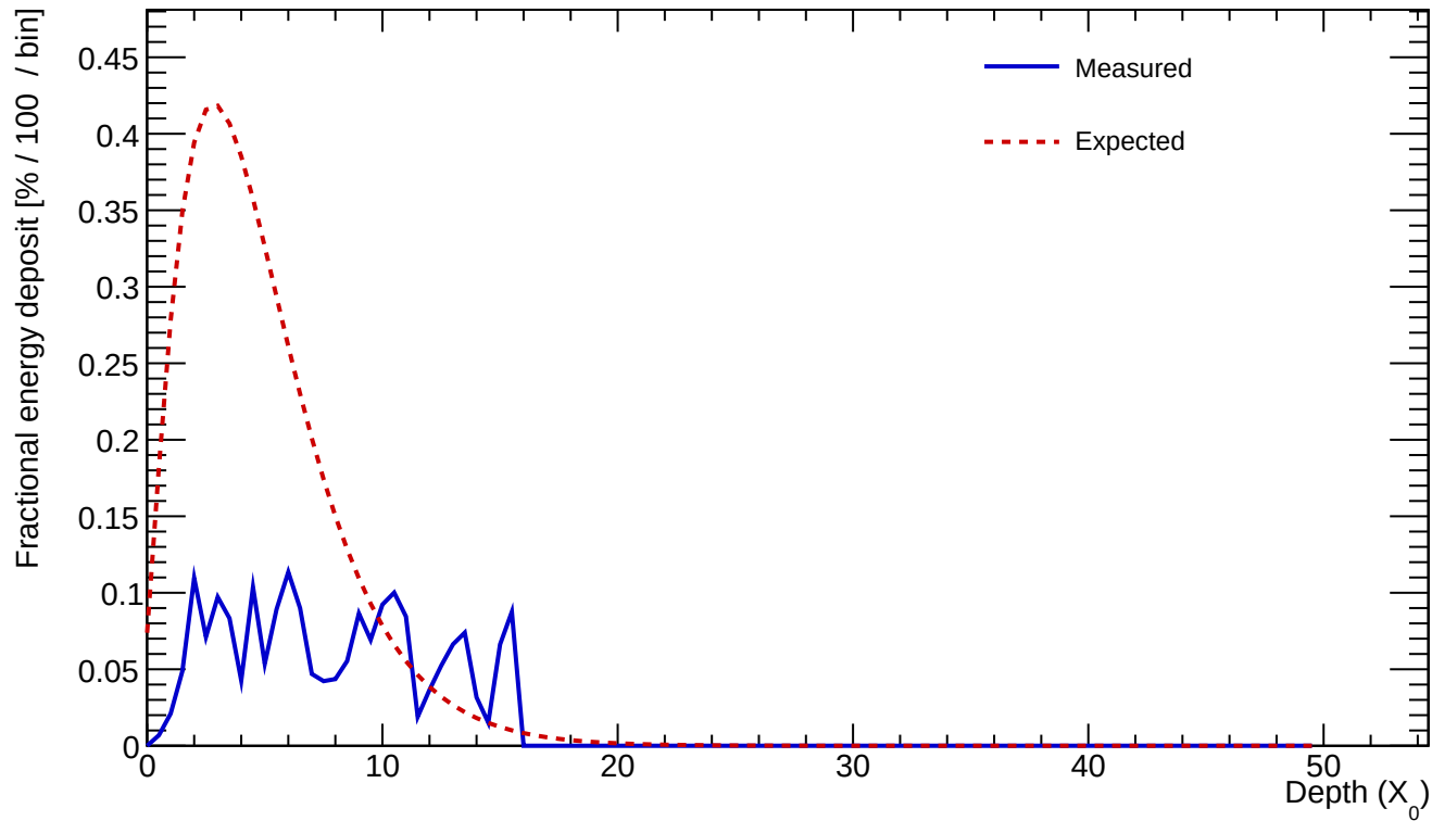
Cluster 612 E=1.347 GeV profileStart=1.00 X_0 \chi=0.5423
