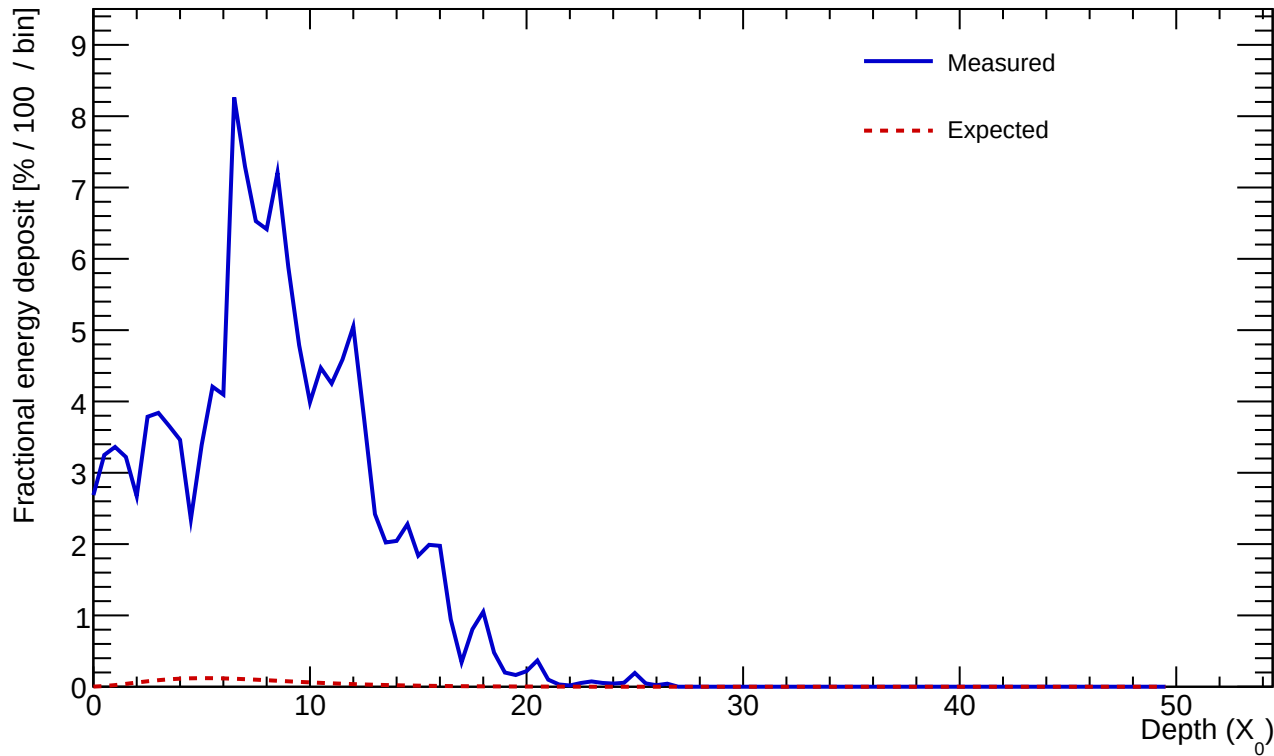
Cluster 178 E=13.436 GeV profileStart=1.00 X_0 \chi=0.3543
