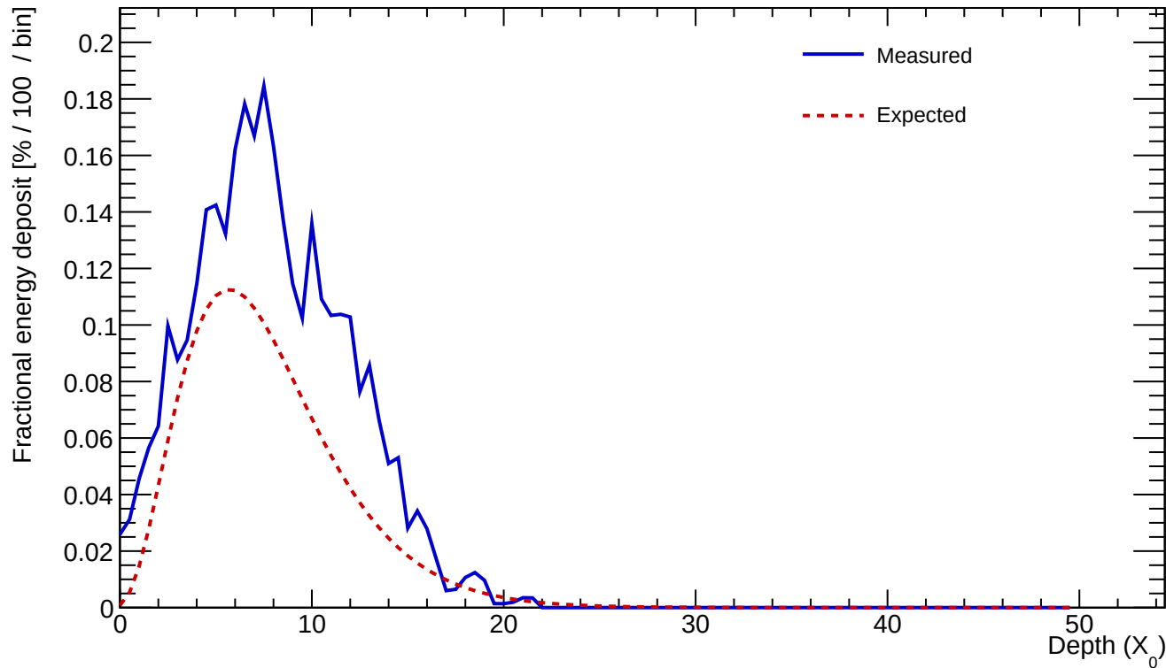
Cluster 131 E=23.540 GeV profileStart=1.00 X_0 \chi=0.1915
