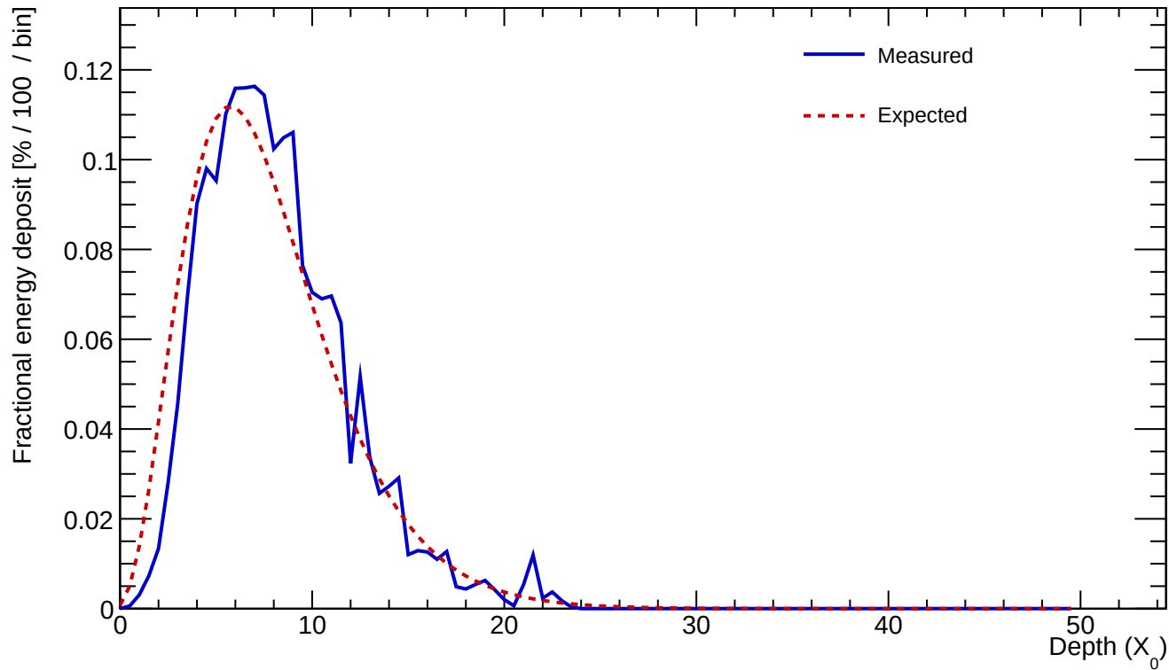
Cluster 175 E=25.173 GeV profileStart=0.50 X_0 \chi=0.1273
