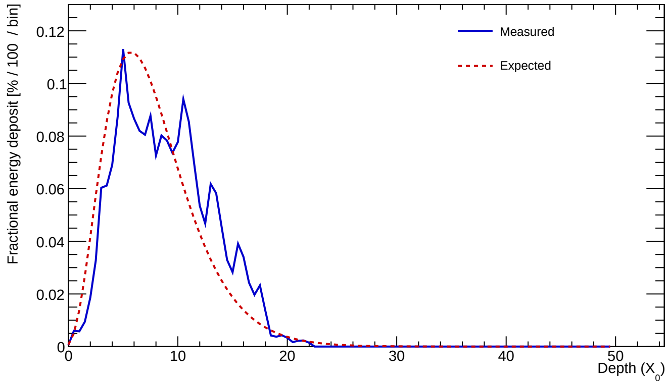
Cluster 597 E=25.059 GeV profileStart=1.00 X_0 \chi=0.2272
