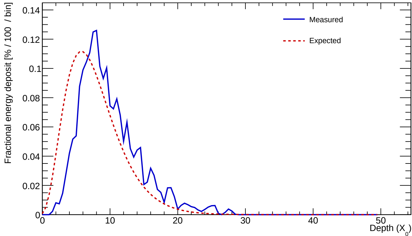
Cluster 123 E=25.692 GeV profileStart=2.00 X_0 \chi=0.1420
