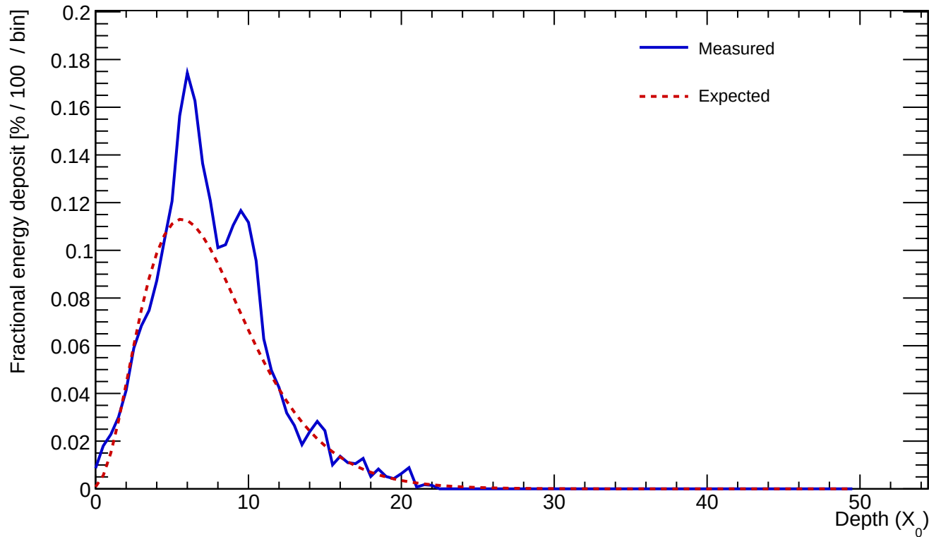
Cluster 329 E=22.692 GeV profileStart=0.50 X_0 \chi=0.1924
