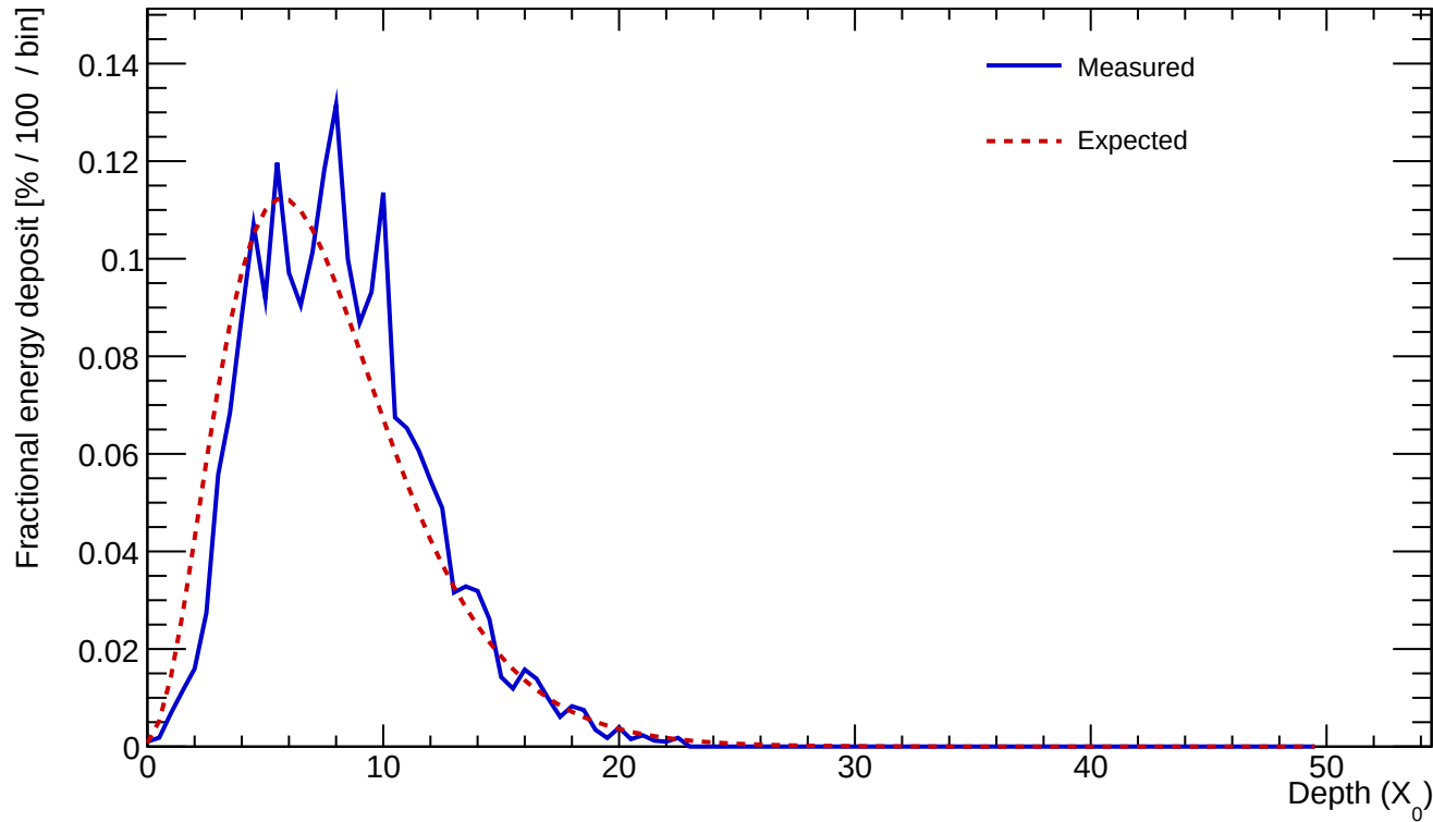
Cluster 381 E=24.075 GeV profileStart=0.50 X_0 \chi=0.1402
