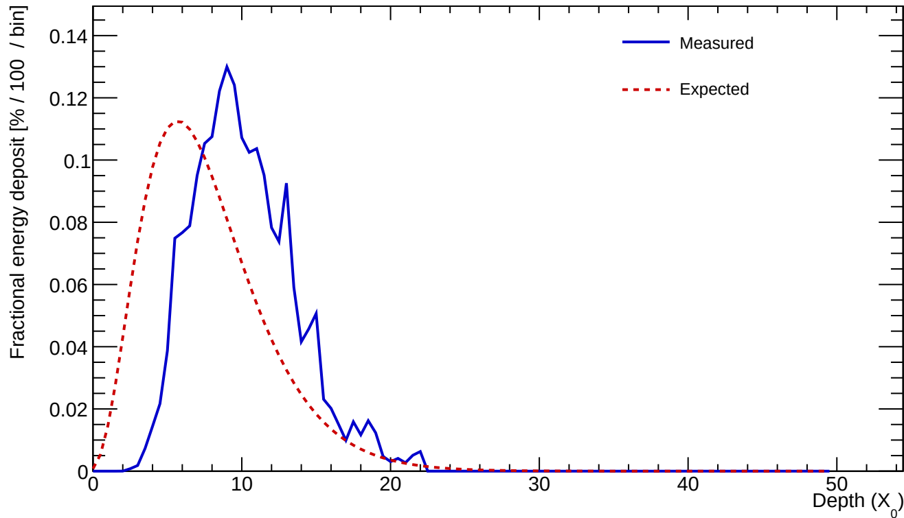
Cluster 173 E=23.693 GeV profileStart=3.00 X_0 \chi=0.1287
