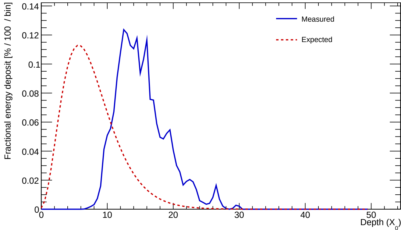
Cluster 203 E=22.966 GeV profileStart=8.00 X_0 \chi=0.1399
