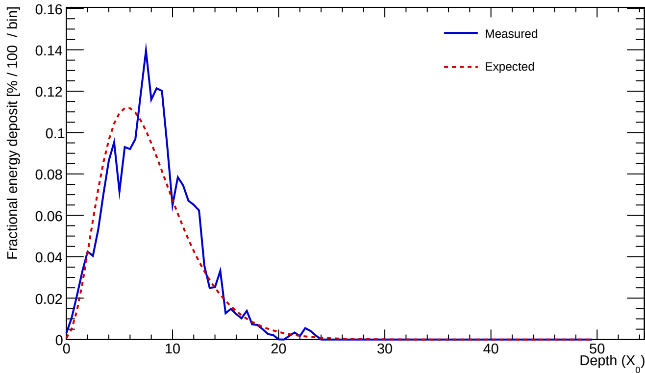
Cluster 36 E=24.846 GeV profileStart=0.50 X_0 \chi=0.2083
