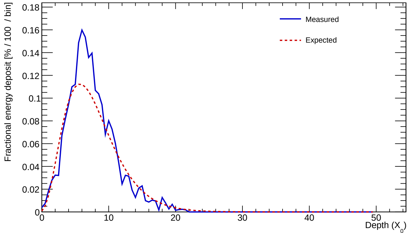
Cluster 324 E=24.193 GeV profileStart=0.50 X_0 \chi=0.1799
