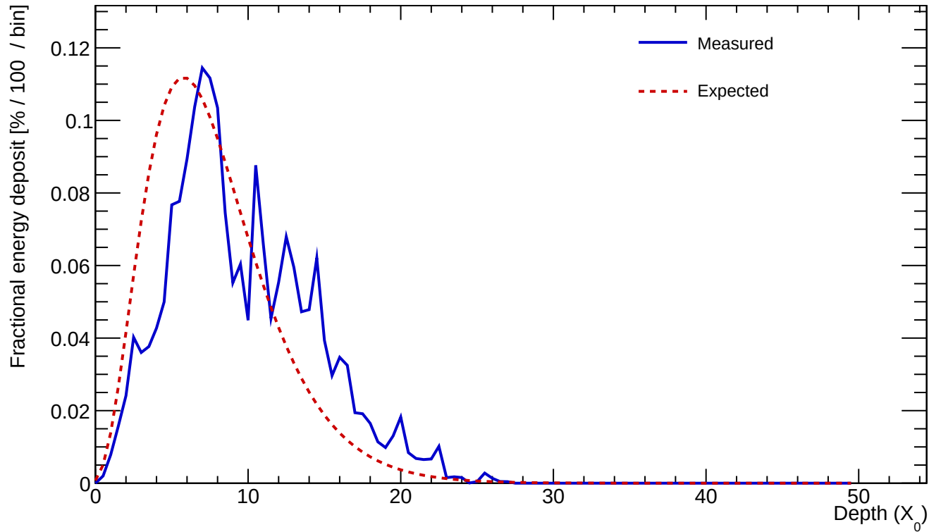
Cluster 62 E=25.162 GeV profileStart=2.00 X_0 \chi=0.2518
