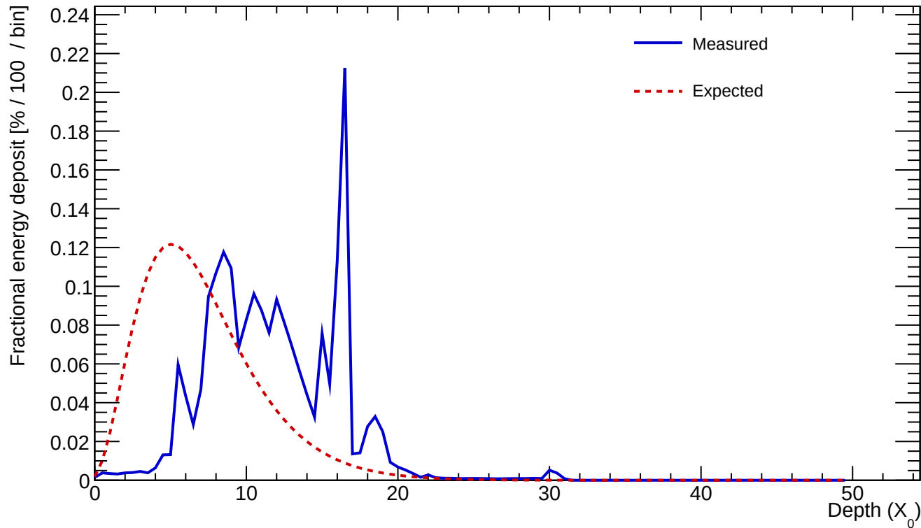
Cluster 136 E=12.530 GeV profileStart=4.00 X_0 \chi=0.3899
