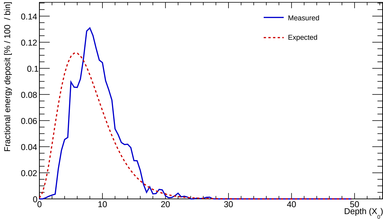
Cluster 682 E=25.157 GeV profileStart=2.00 X_0 \chi=0.1521
