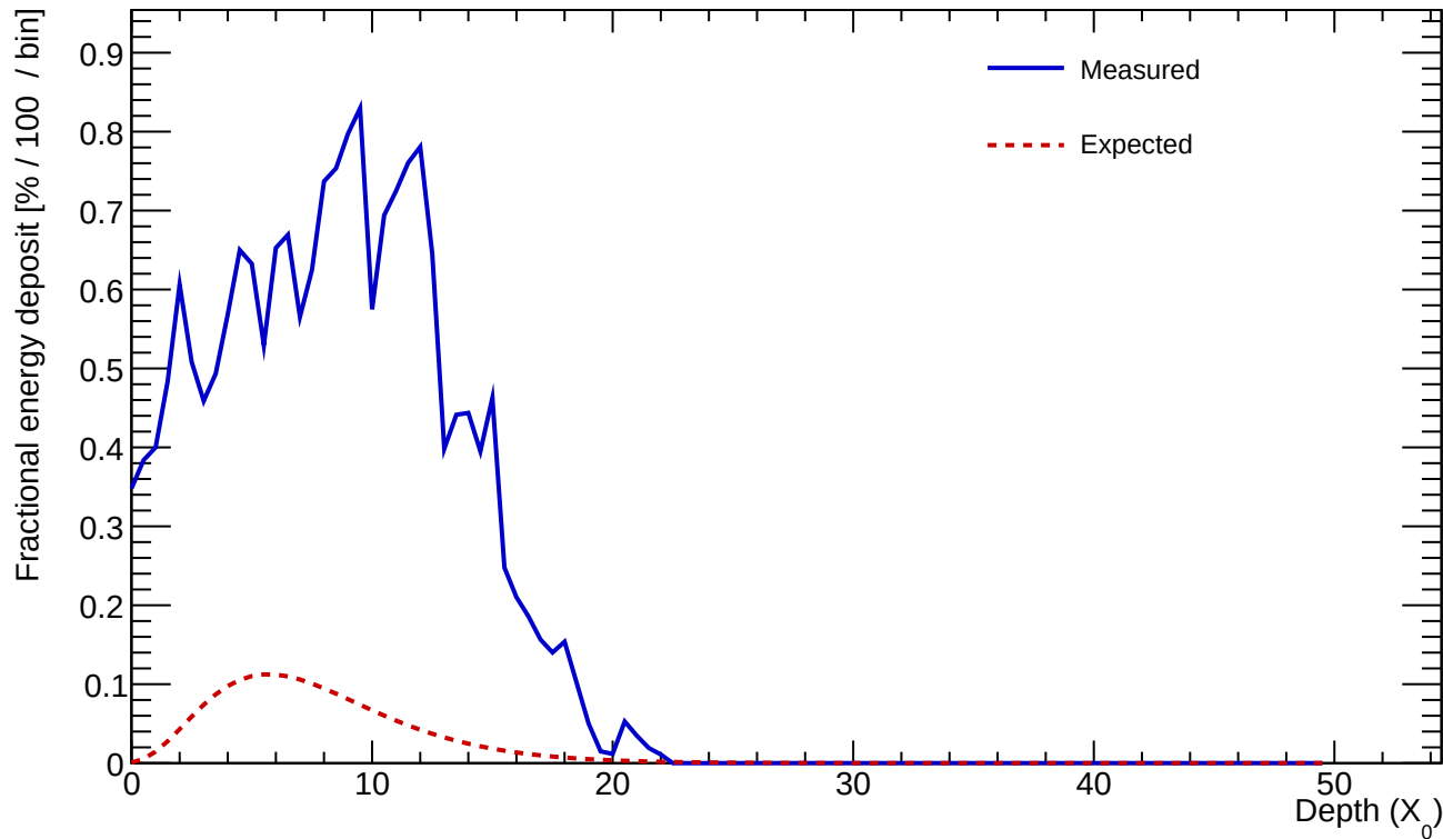
Cluster 157 E=23.698 GeV profileStart=1.50 X_0 \chi=0.3856
