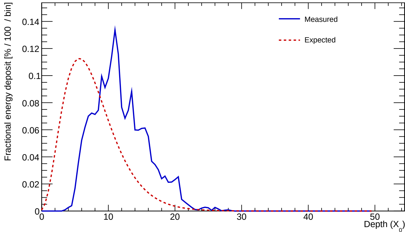
Cluster 626 E=23.463 GeV profileStart=4.00 X_0 \chi=0.1769
