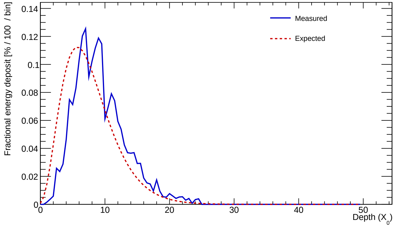
Cluster 43 E=24.158 GeV profileStart=1.50 X_0 \chi=0.1394
