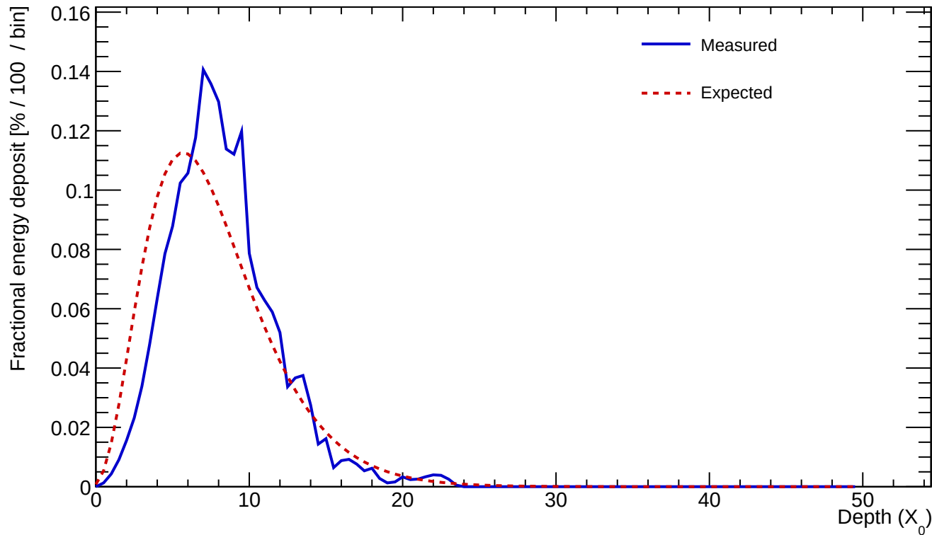
Cluster 197 E=23.636 GeV profileStart=1.00 X_0 \chi=0.1716
