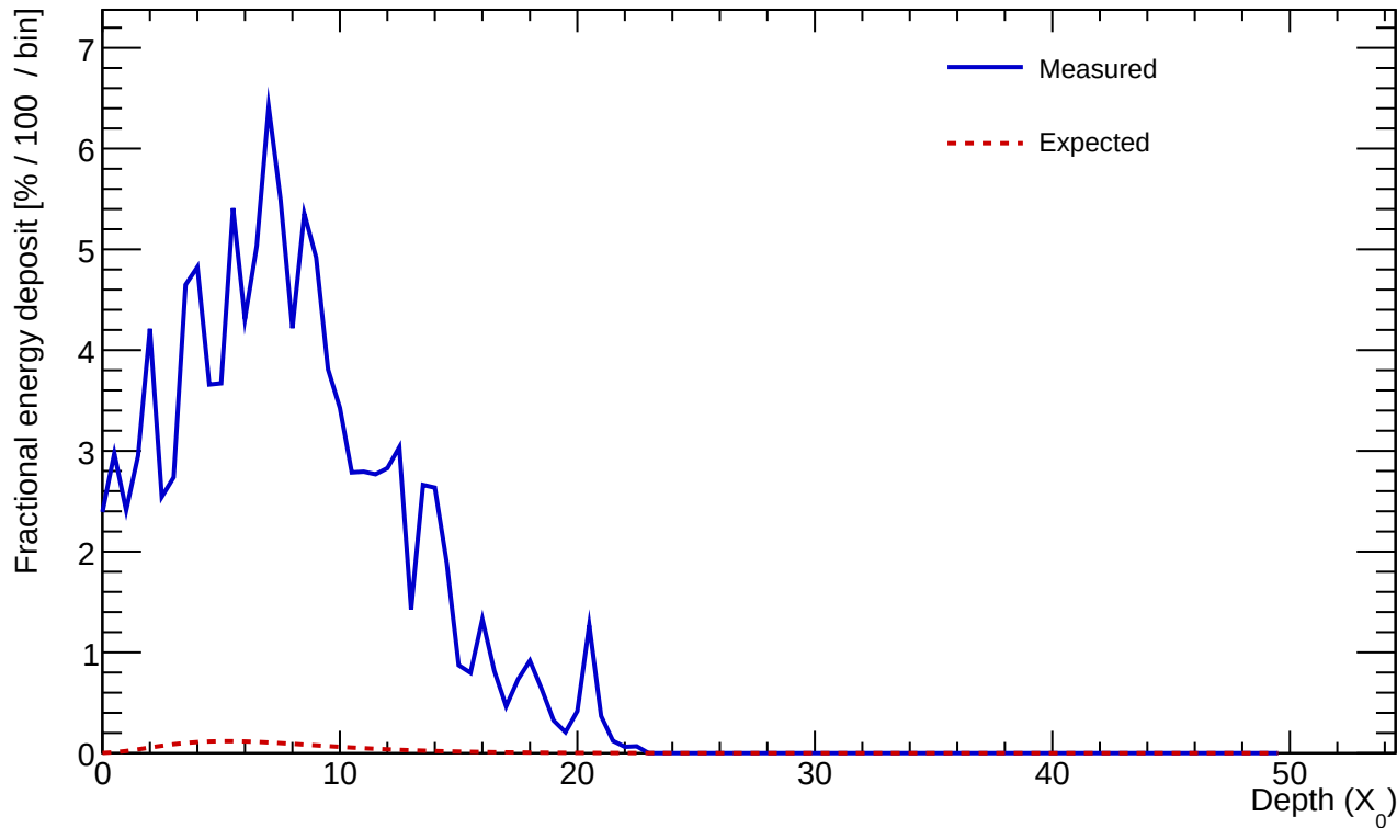
Cluster 604 E=14.981 GeV profileStart=0.50 X_0 \chi=0.3225
