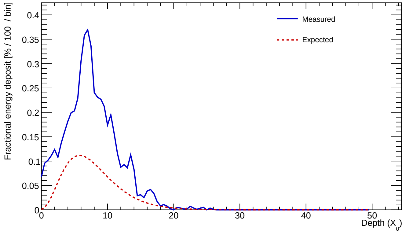
Cluster 442 E=25.550 GeV profileStart=0.50 X_0 \chi=0.2409
