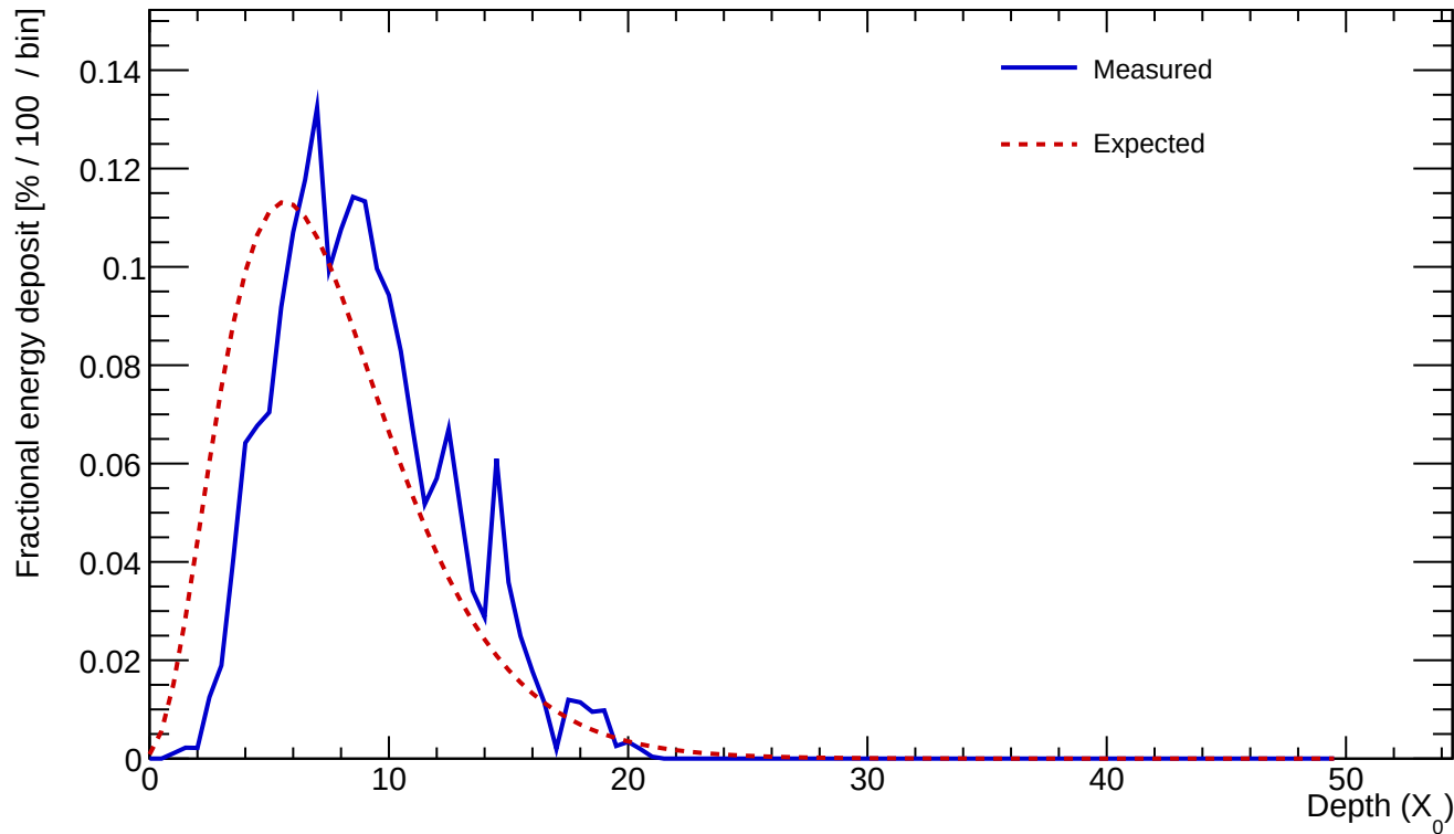
Cluster 367 E=22.533 GeV profileStart=1.50 X_0 \chi=0.1344
