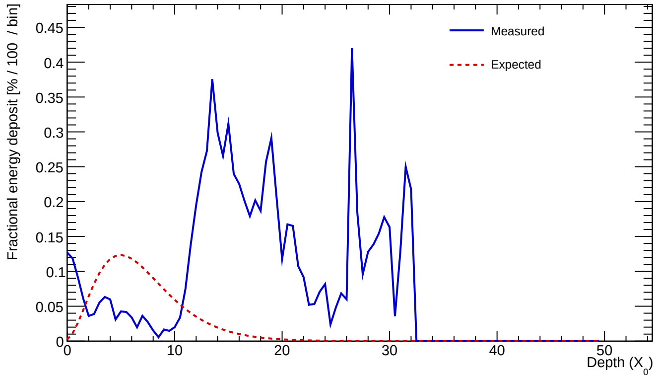
Cluster 80 E=11.415 GeV profileStart=10.50 X_0 \chi=0.9995
