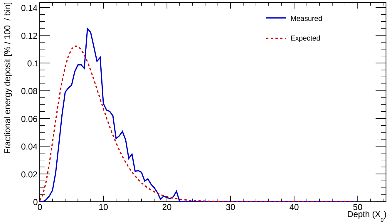
Cluster 436 E=24.062 GeV profileStart=1.00 X_0 \chi=0.1174
