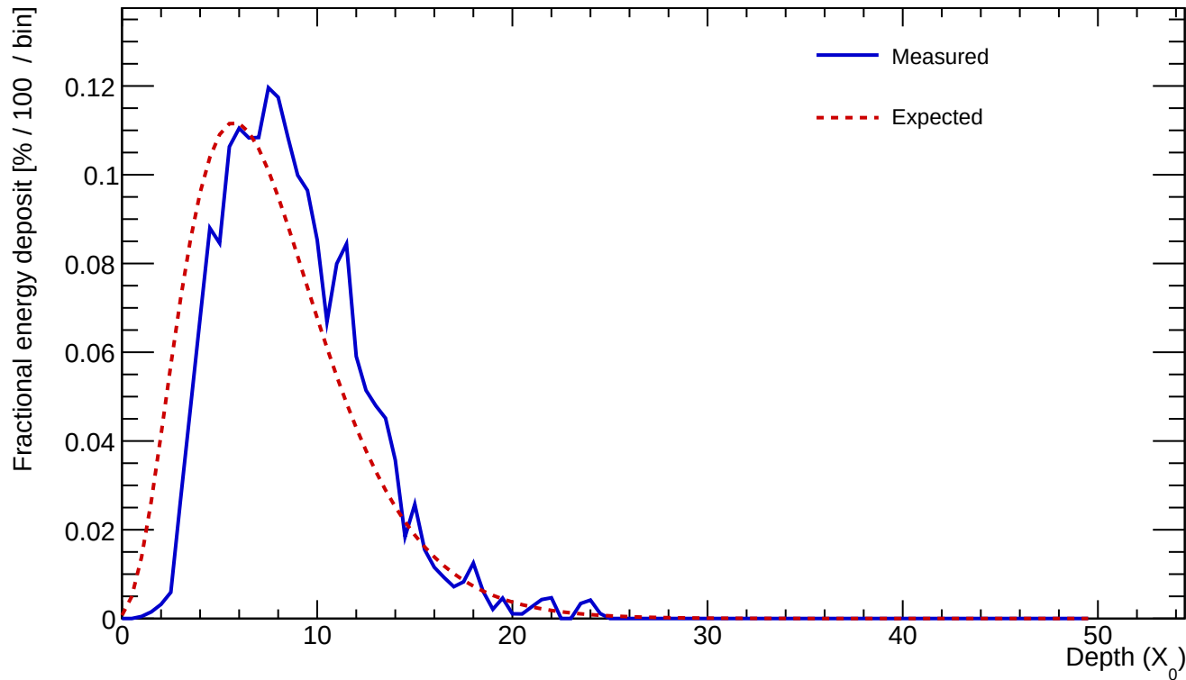
Cluster 425 E=25.339 GeV profileStart=1.50 X_0 \chi=0.1203
