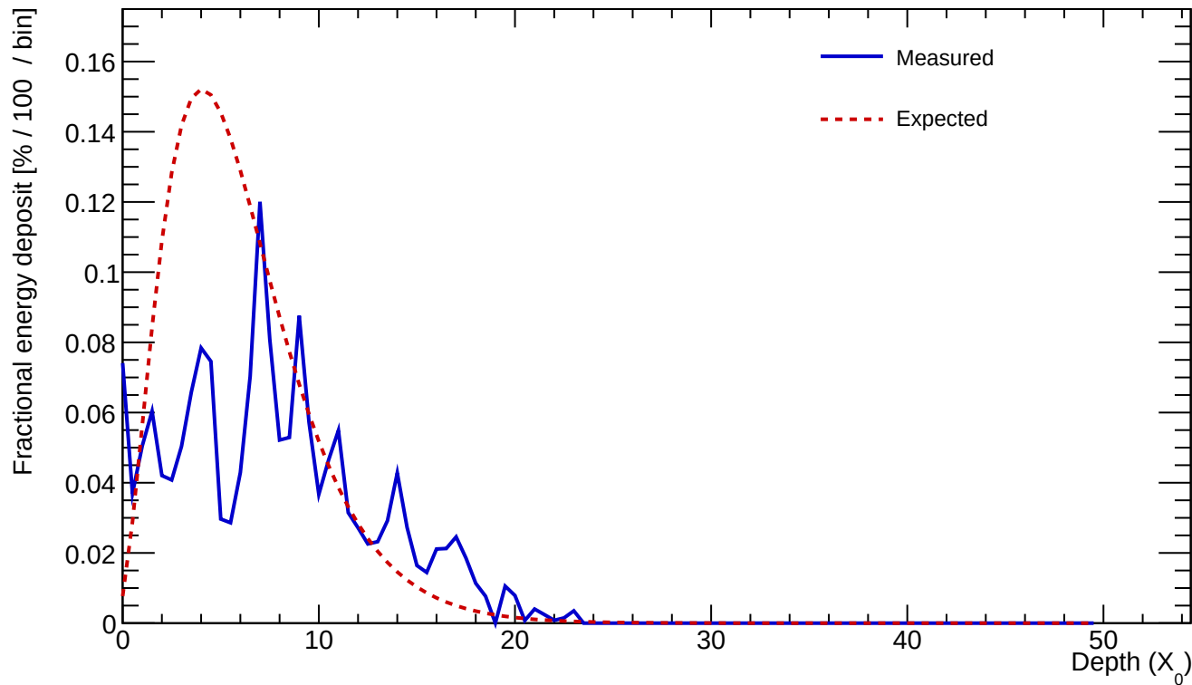
Cluster 98 E=4.543 GeV profileStart=1.50 X_0 \chi=0.5077
