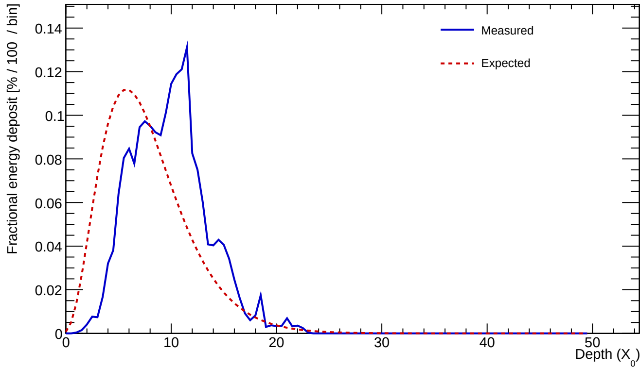
Cluster 470 E=25.151 GeV profileStart=2.50 X_0 \chi=0.1886
