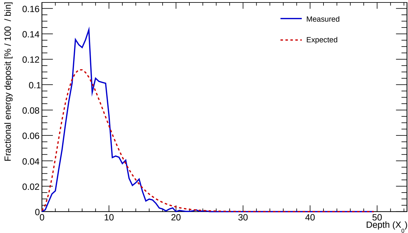
Cluster 639 E=25.114 GeV profileStart=0.50 X_0 \chi=0.2044
