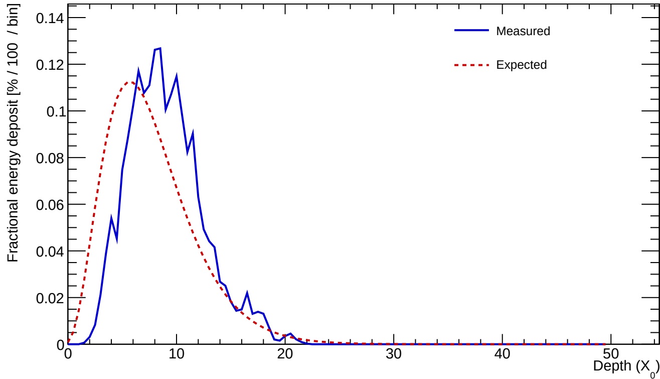
Cluster 493 E=23.847 GeV profileStart=1.50 X_0 \chi=0.1509
