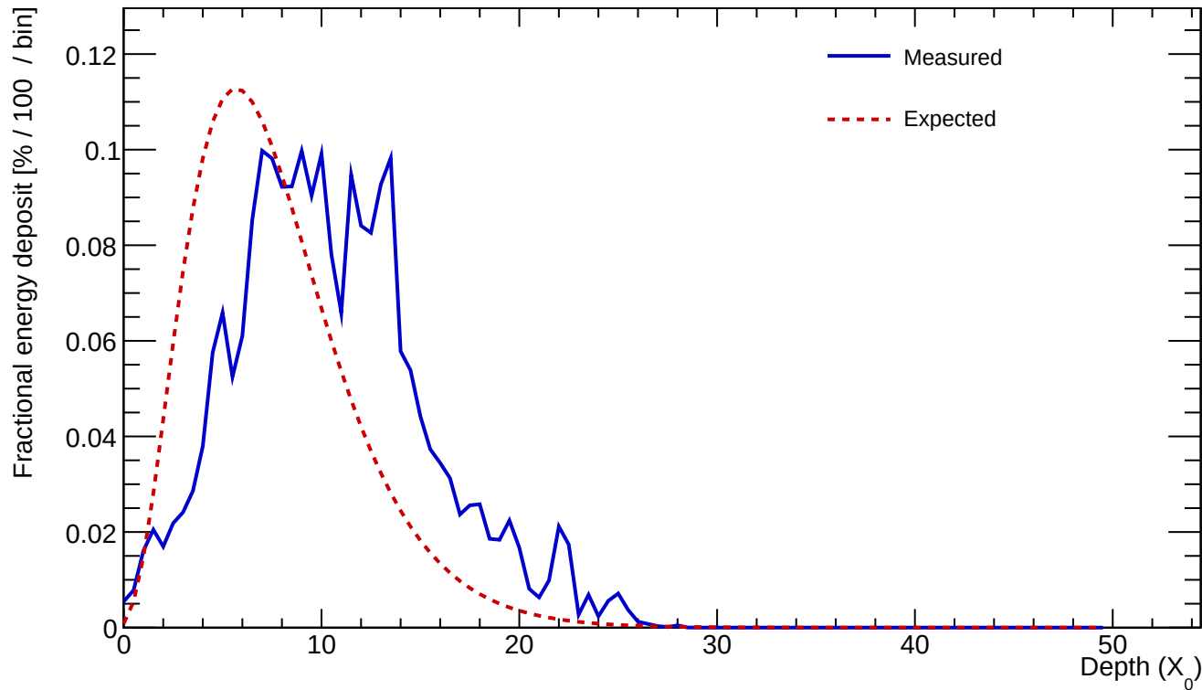
Cluster 270 E=23.218 GeV profileStart=3.00 X_0 \chi=0.2835
