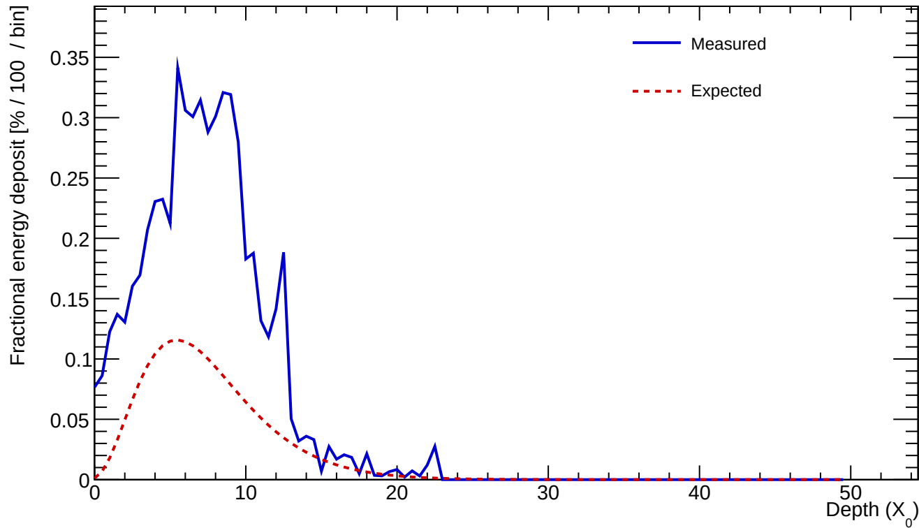
Cluster 394 E=18.402 GeV profileStart=0.50 X_0 \chi=0.2511
