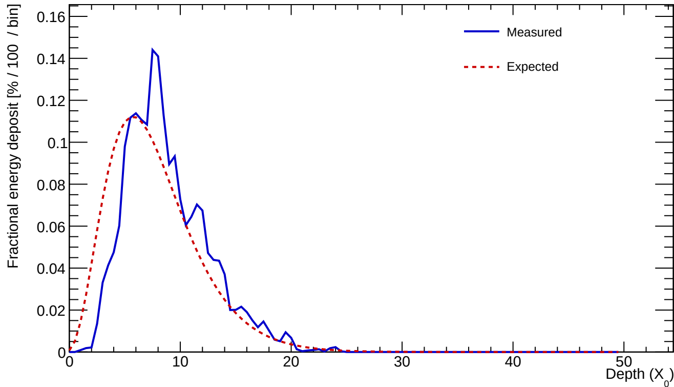
Cluster 386 E=24.510 GeV profileStart=1.50 X_0 \chi=0.1455
