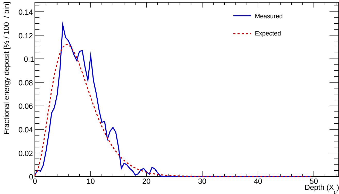
Cluster 249 E=24.276 GeV profileStart=1.00 X_0 \chi=0.1379
