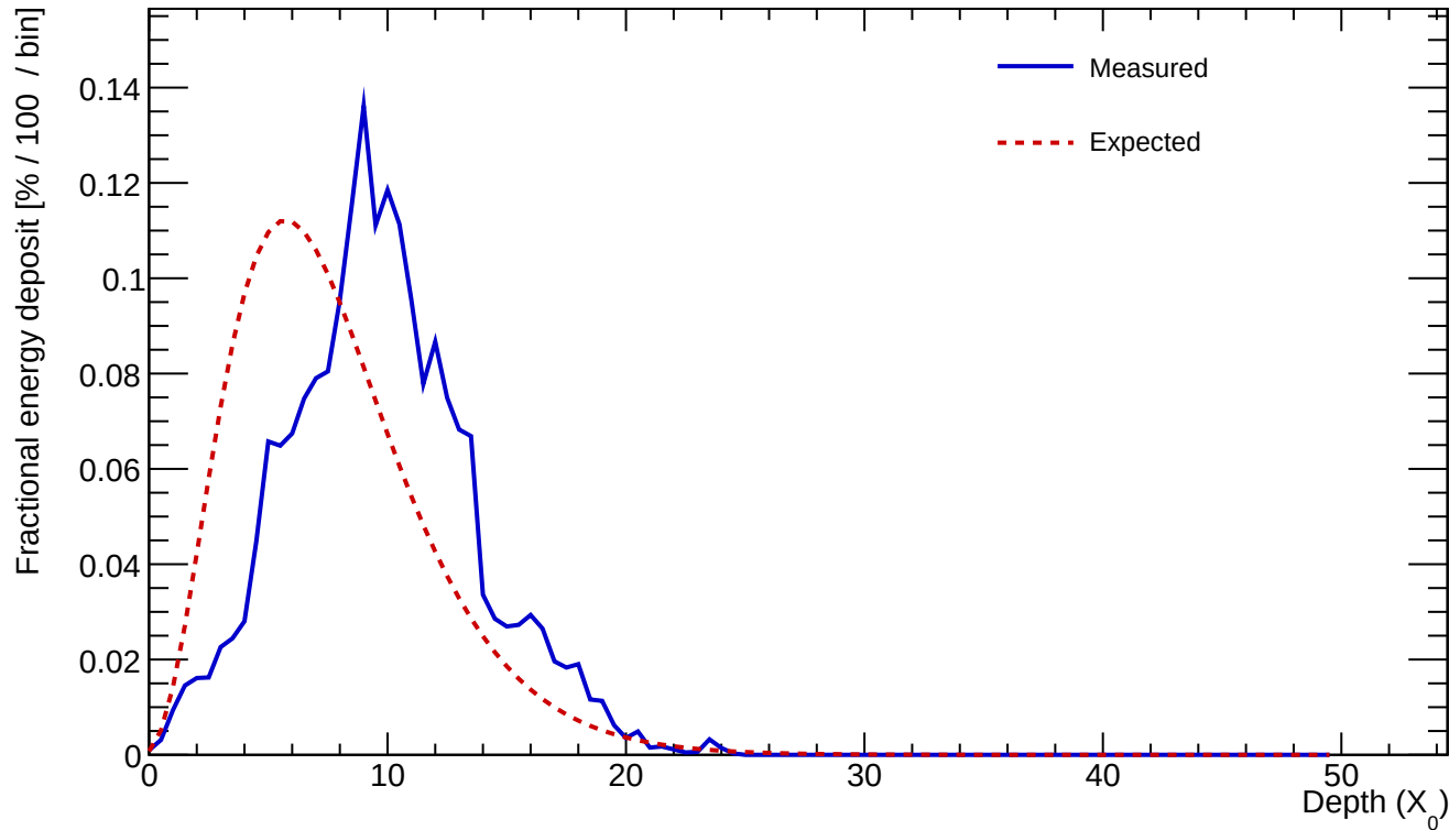
Cluster 681 E=24.510 GeV profileStart=2.50 X_0 \chi=0.2062
