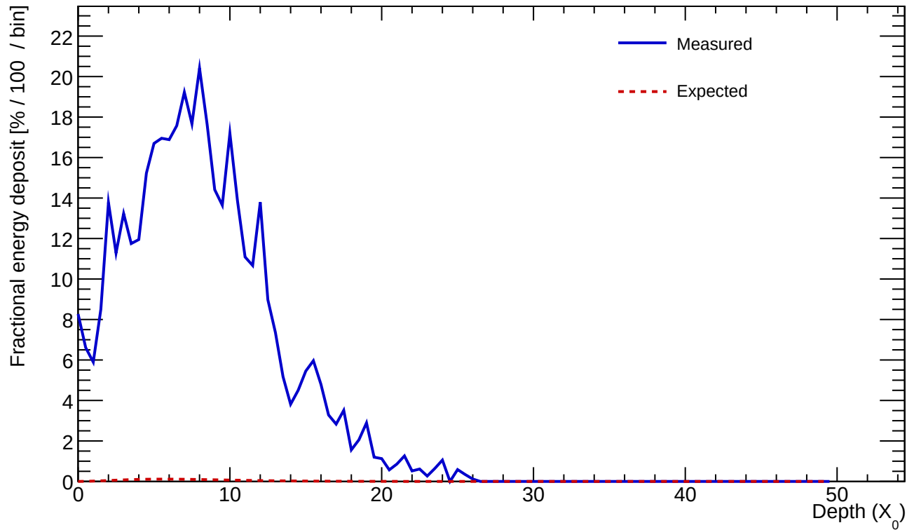
Cluster 68 E=22.137 GeV profileStart=0.50 X_0 \chi=0.2750
