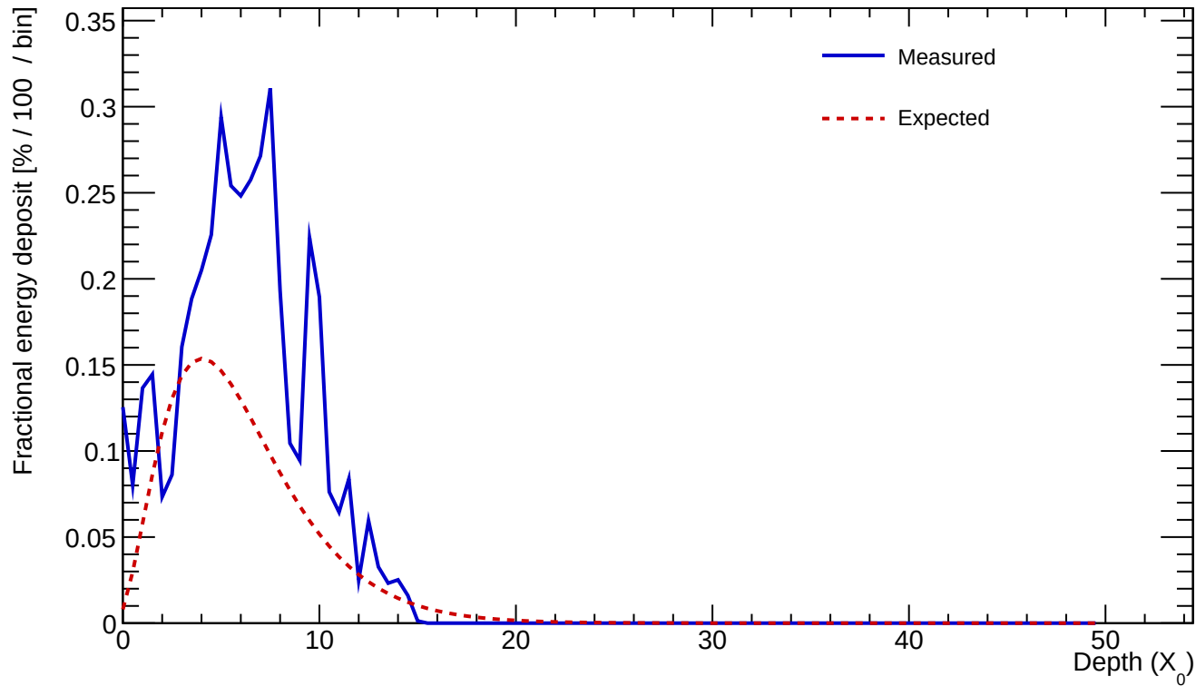
Cluster 151 E=4.409 GeV profileStart=1.50 X_0 \chi=0.3072
