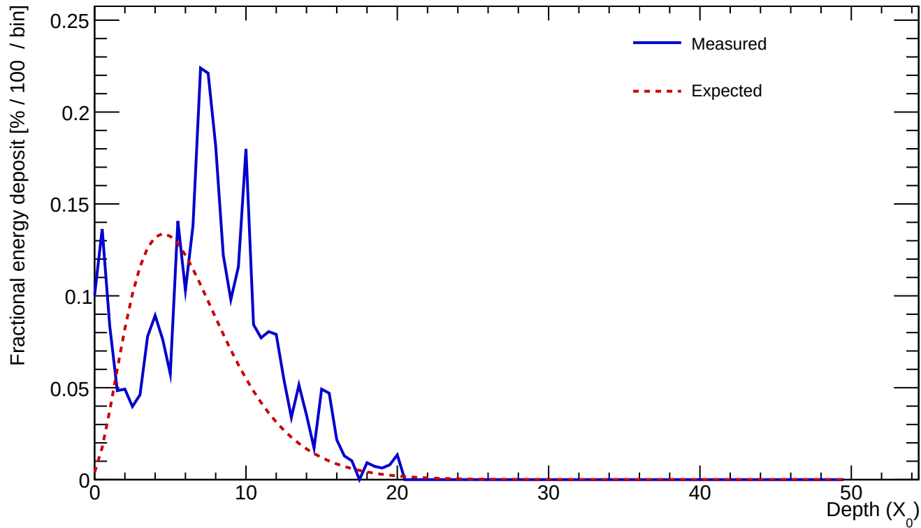
Cluster 382 E=7.316 GeV profileStart=2.00 X_0 \chi=0.4090
