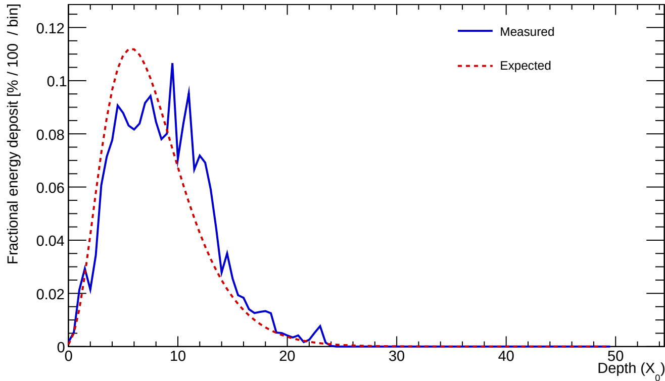
Cluster 223 E=24.710 GeV profileStart=1.00 X_0 \chi=0.2265
