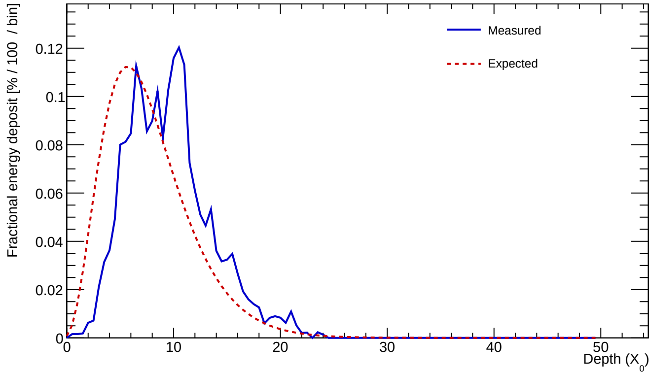
Cluster 438 E=24.060 GeV profileStart=2.00 X_0 \chi=0.1565
