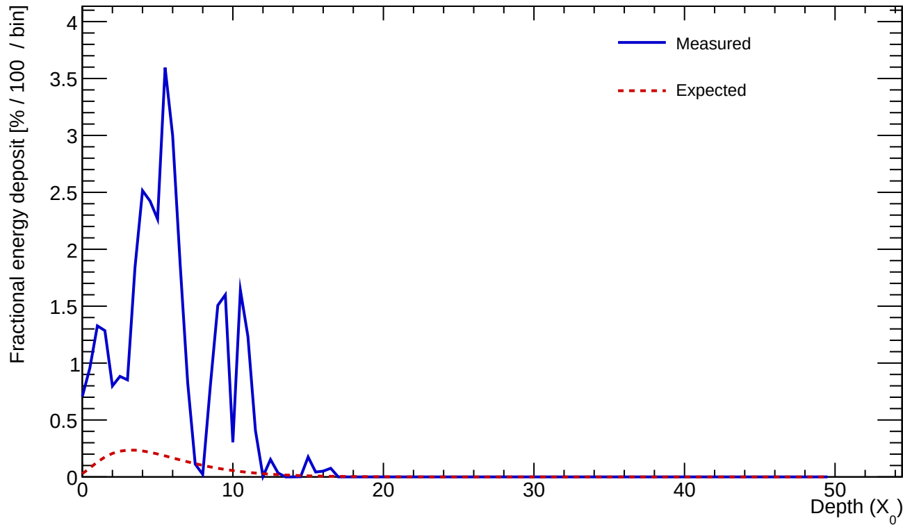
Cluster 202 E=2.048 GeV profileStart=0.50 X_0 \chi=0.5269
