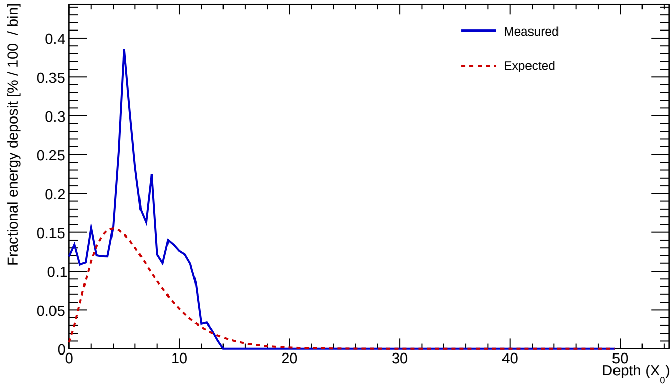
Cluster 474 E=4.310 GeV profileStart=0.50 X_0 \chi=0.3304
