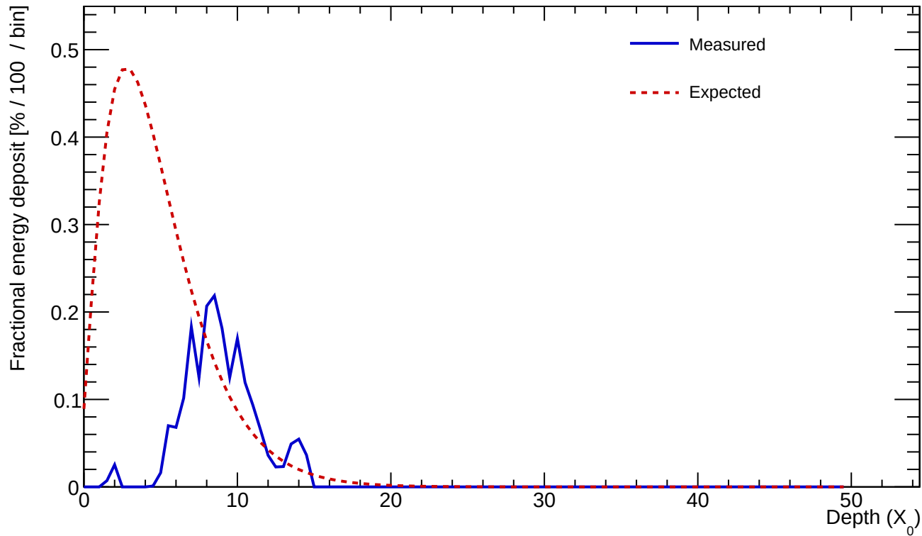
Cluster 224 E=1.272 GeV profileStart=5.00 X_0 \chi=0.2808
