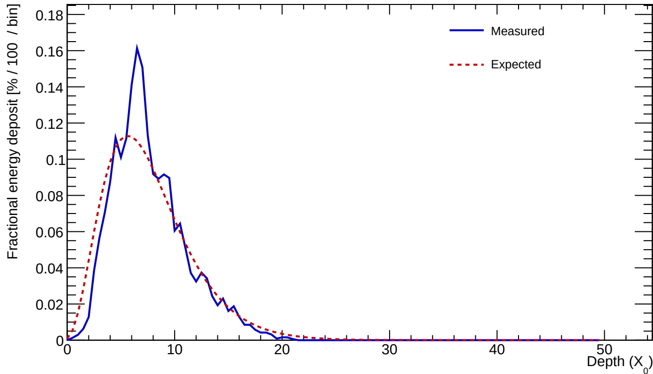
Cluster 515 E=22.848 GeV profileStart=0.50 X_0 \chi=0.1632
