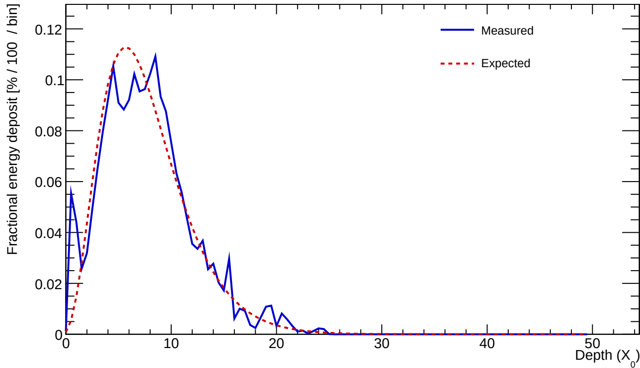
Cluster 268 E=23.156 GeV profileStart=0.50 X_0 \chi=0.1827
