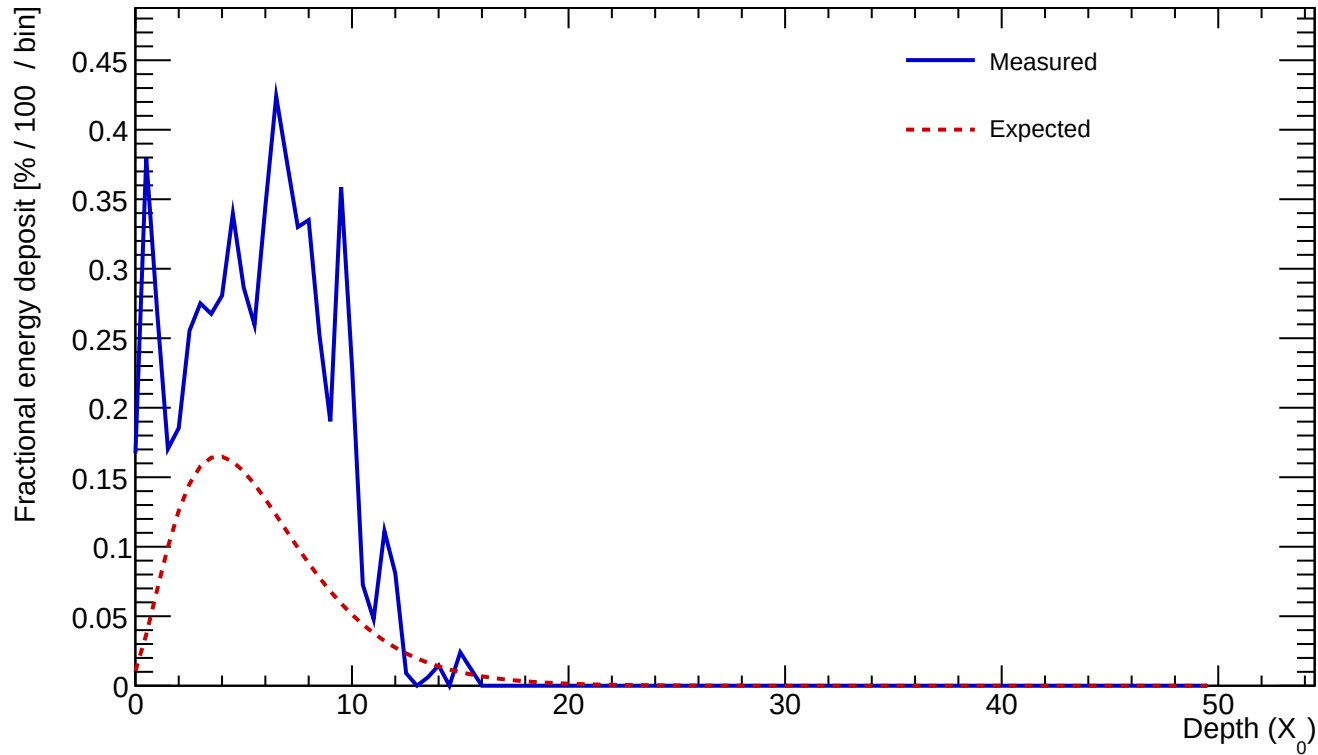
Cluster 556 E=3.652 GeV profileStart=1.00 X_0 \chi=0.3800
