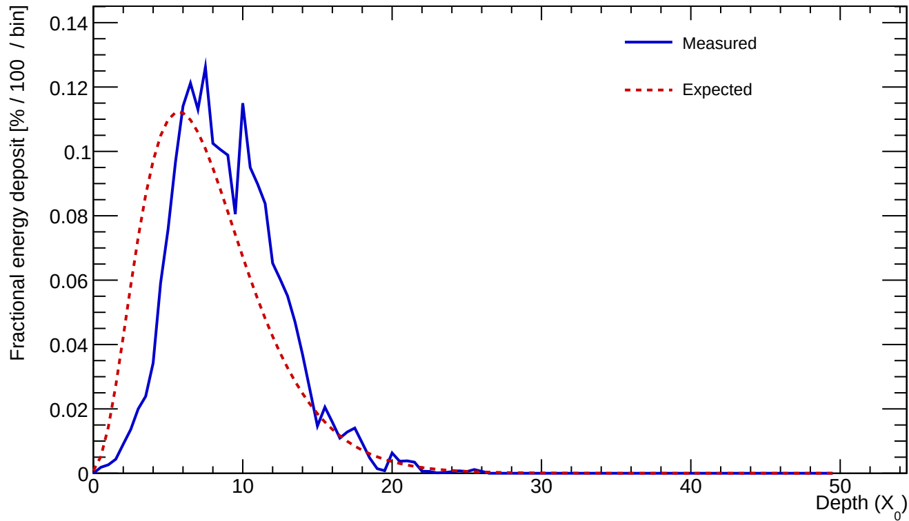
Cluster 149 E=24.265 GeV profileStart=2.00 X_0 \chi=0.1607
