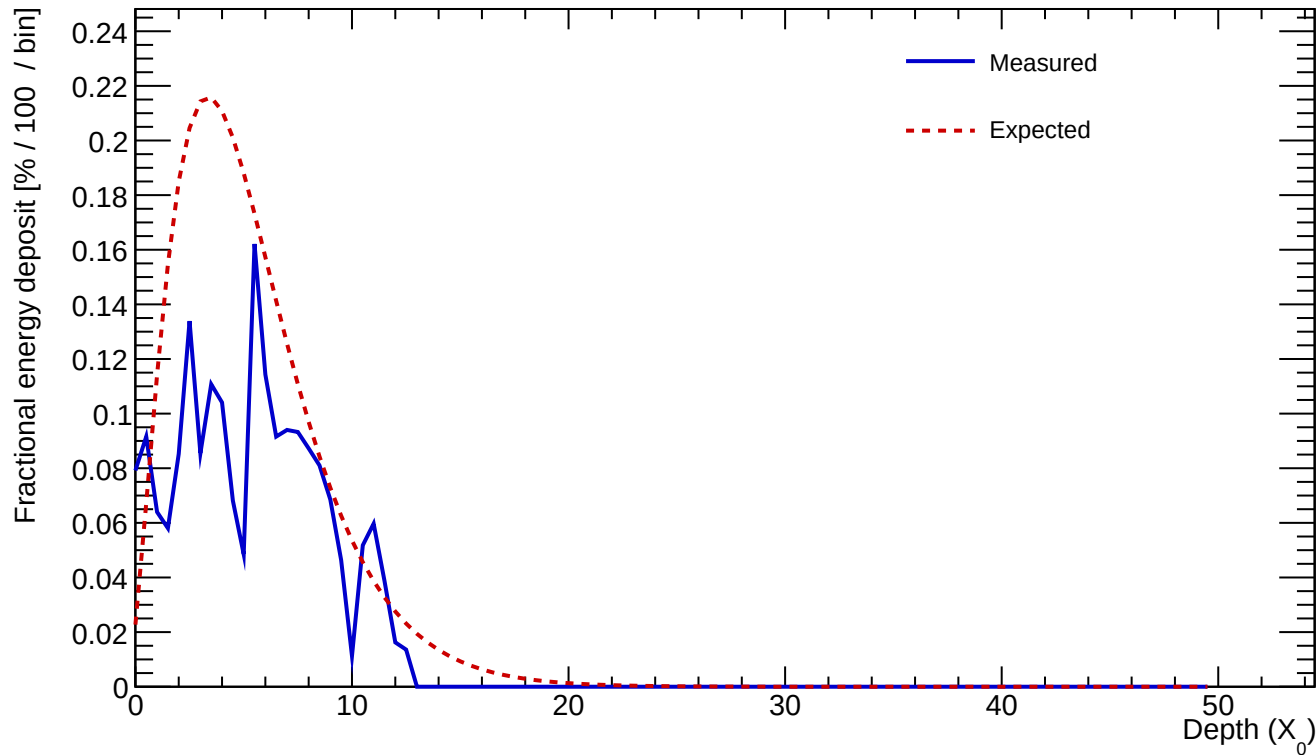
Cluster 439 E=2.274 GeV profileStart=0.50 X_0 \chi=0.3511
