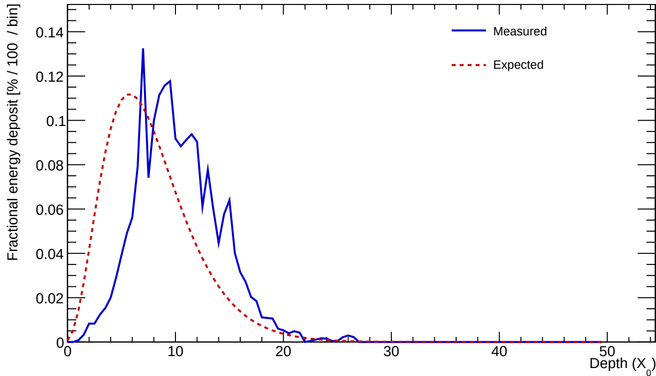
Cluster 471 E=25.098 GeV profileStart=3.00 X_0 \chi=0.1722
