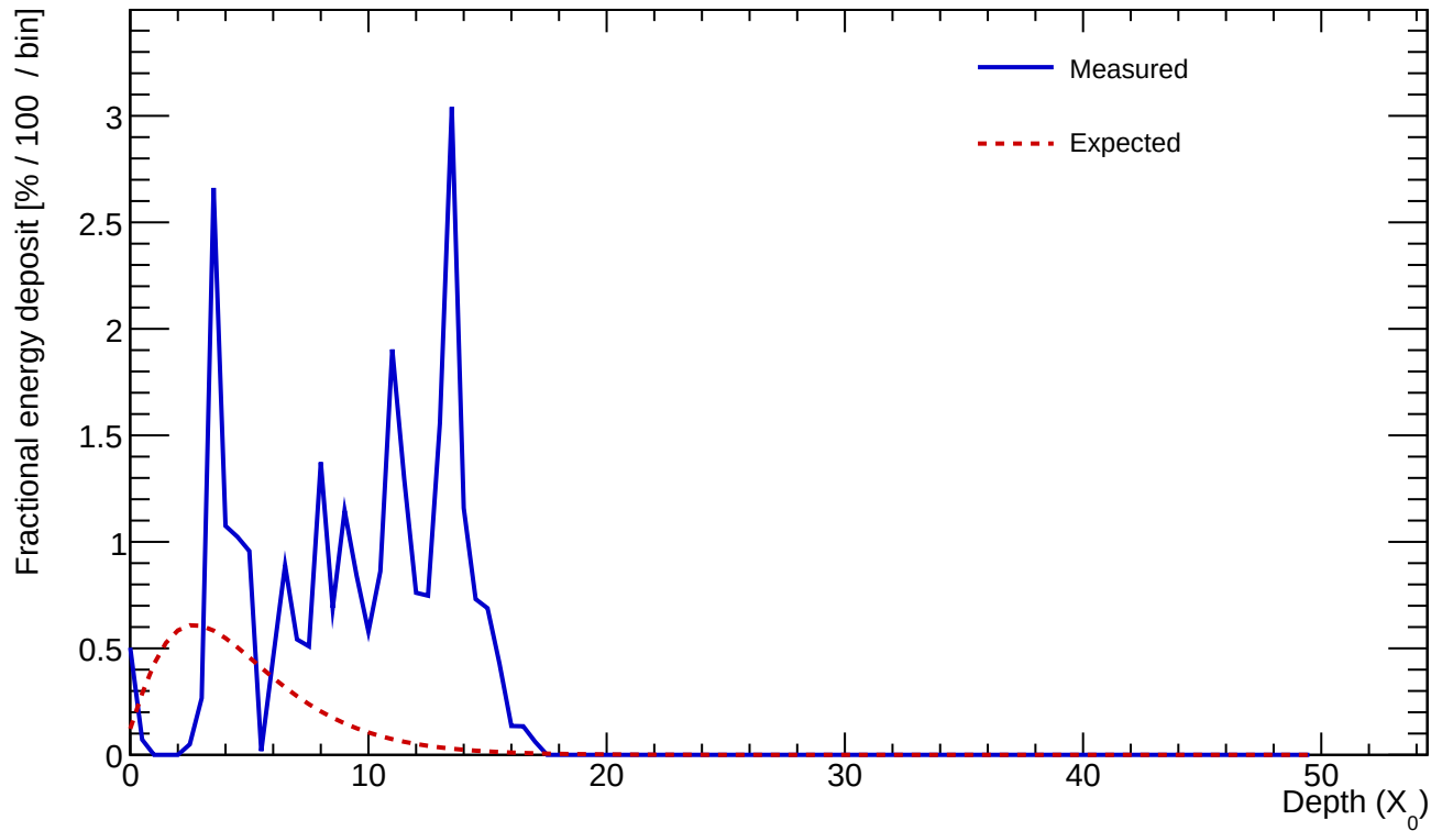
Cluster 150 E=1.172 GeV profileStart=7.00 X_0 \chi=0.7174
