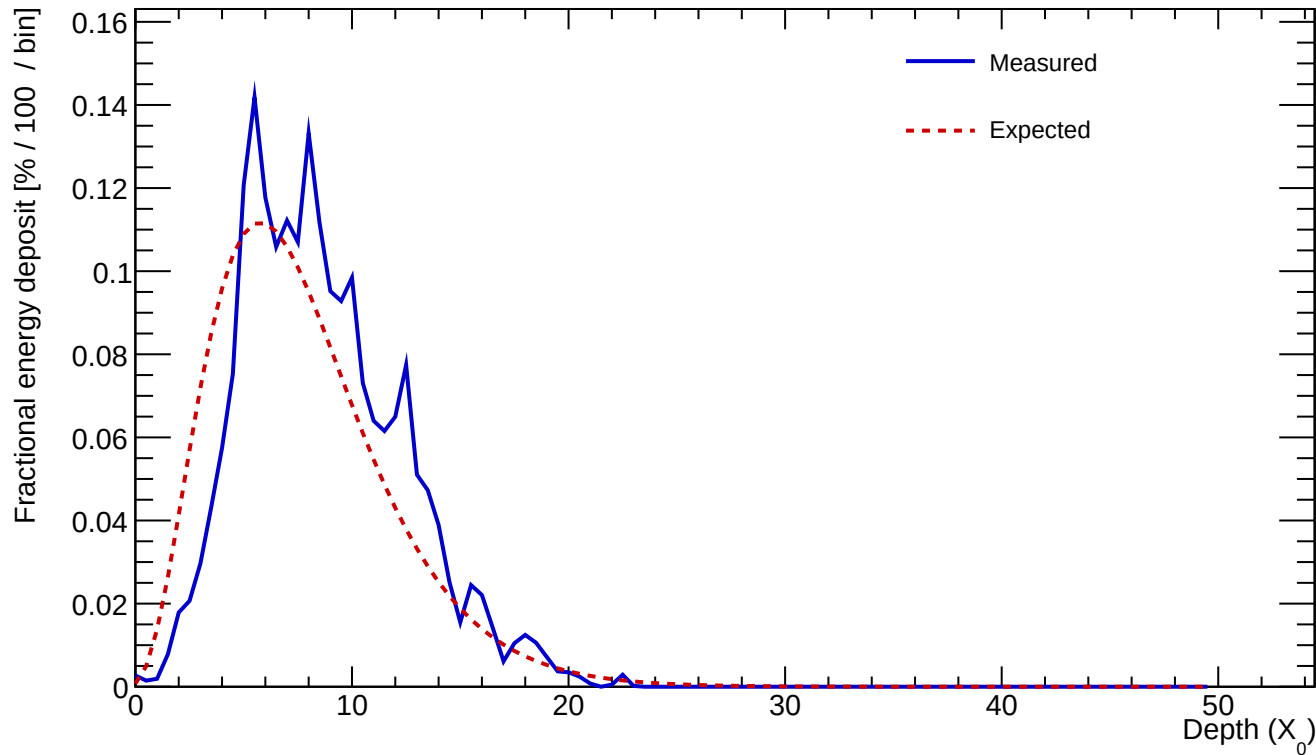
Cluster 273 E=25.475 GeV profileStart=1.50 X_0 \chi=0.1472
