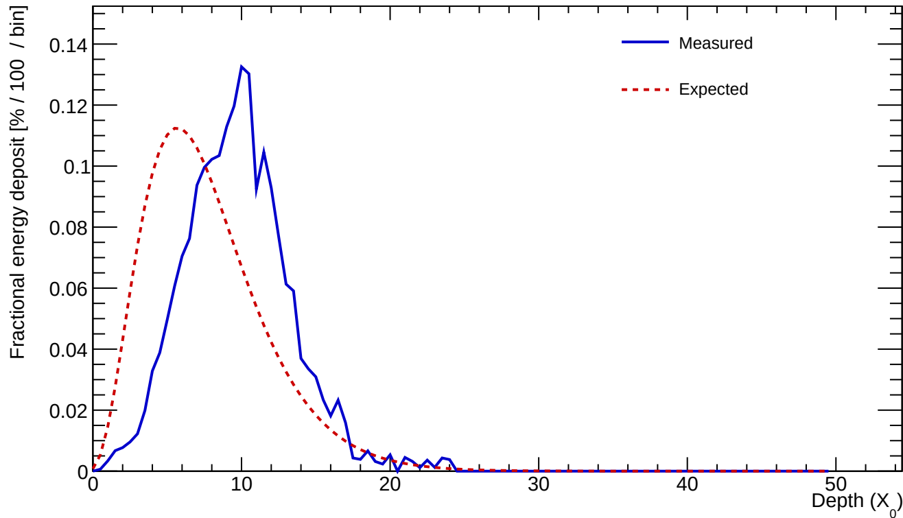
Cluster 535 E=23.743 GeV profileStart=3.00 X_0 \chi=0.2019
