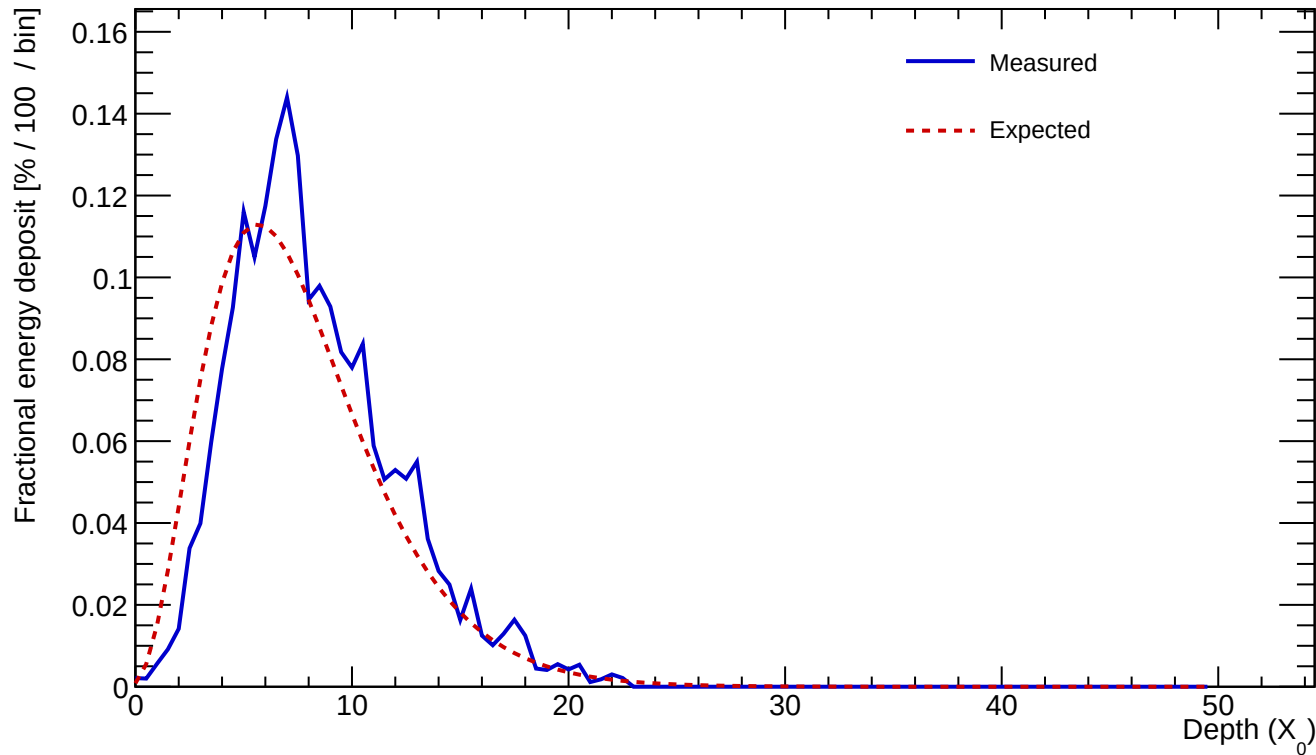
Cluster 269 E=22.819 GeV profileStart=1.00 X_0 \chi=0.1189
