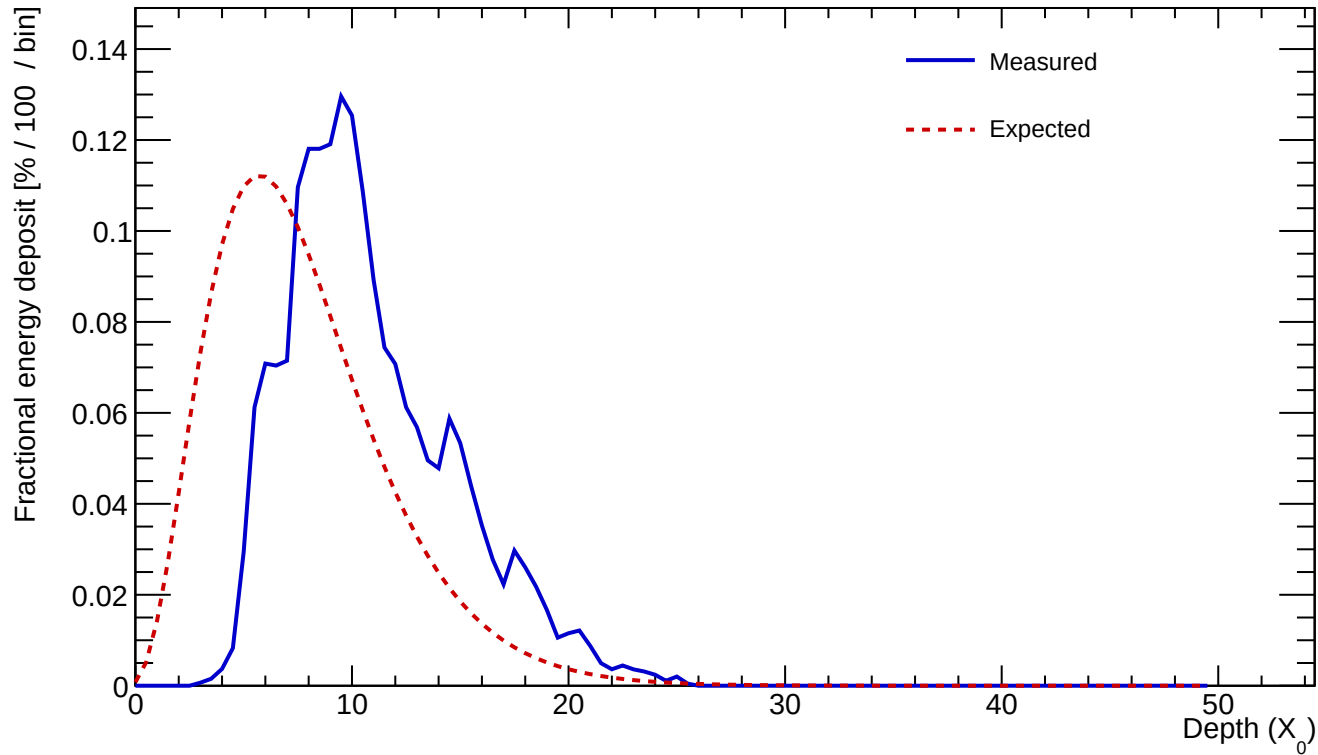
Cluster 126 E=24.313 GeV profileStart=3.00 X_0 \chi=0.1551
