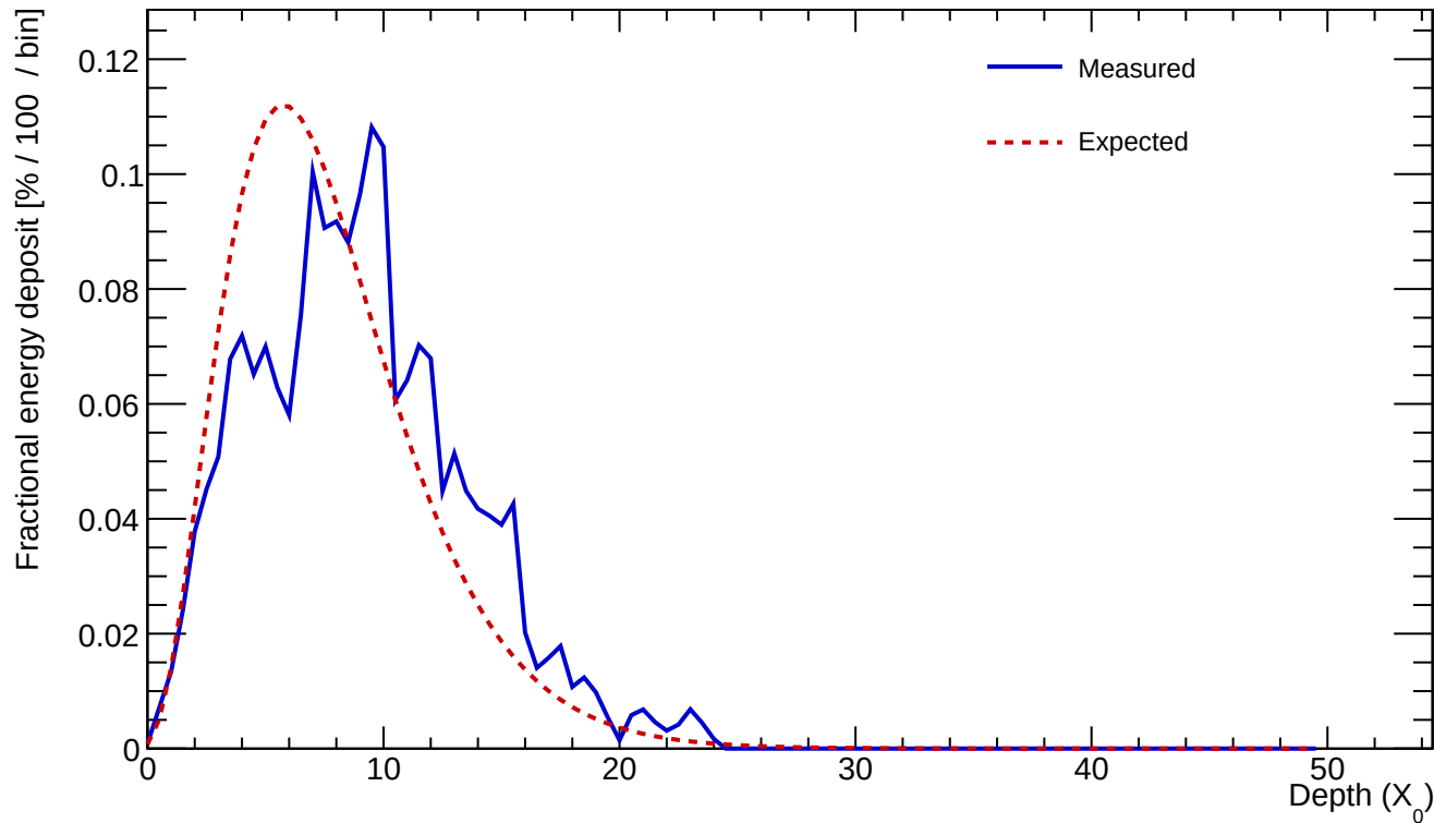
Cluster 94 E=24.761 GeV profileStart=1.00 X_0 \chi=0.2624
