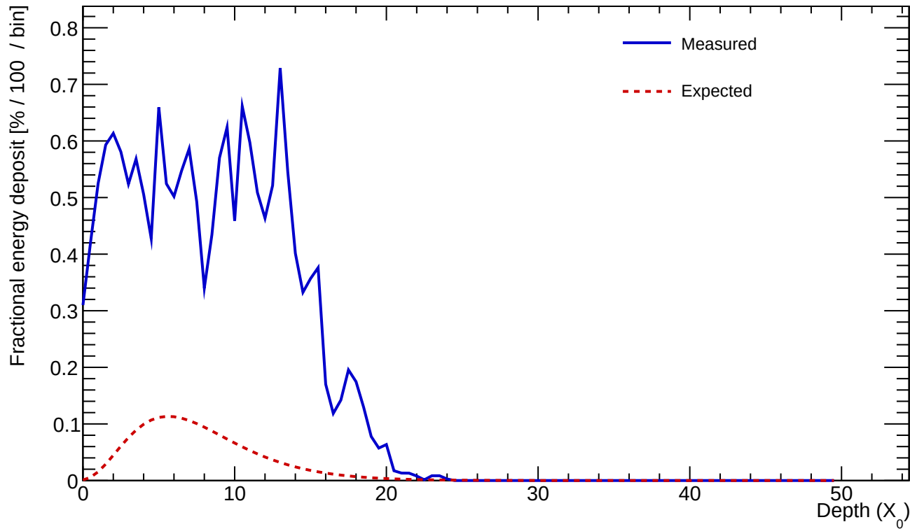
Cluster 86 E=22.162 GeV profileStart=1.00 X_0 \chi=0.5120
