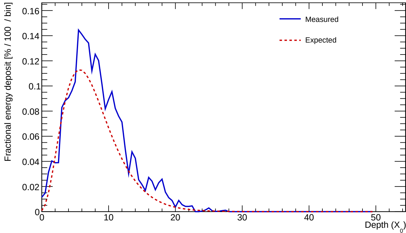
Cluster 560 E=23.033 GeV profileStart=0.50 X_0 \chi=0.1634
