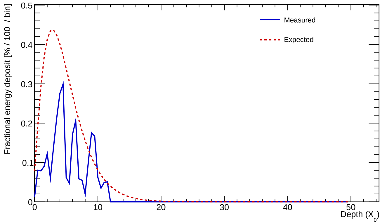
Cluster 585 E=1.321 GeV profileStart=1.00 X_0 \chi=0.4895
