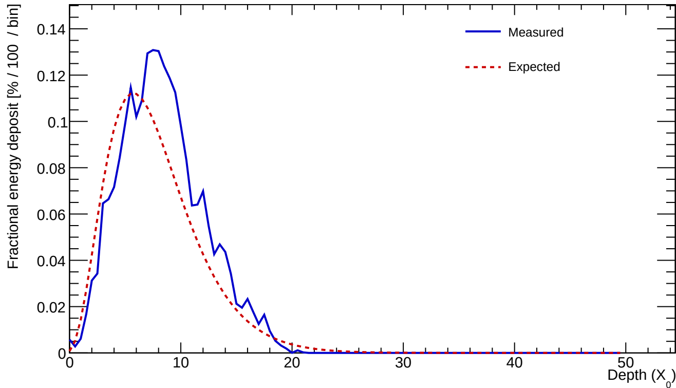
Cluster 692 E=24.468 GeV profileStart=1.00 X_0 \chi=0.1275
