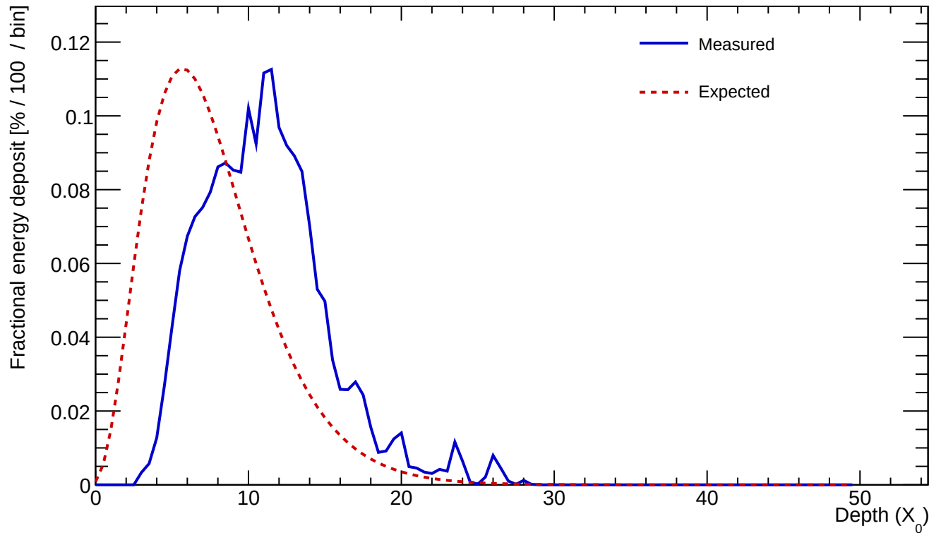
Cluster 516 E=23.079 GeV profileStart=3.50 X_0 \chi=0.2005
