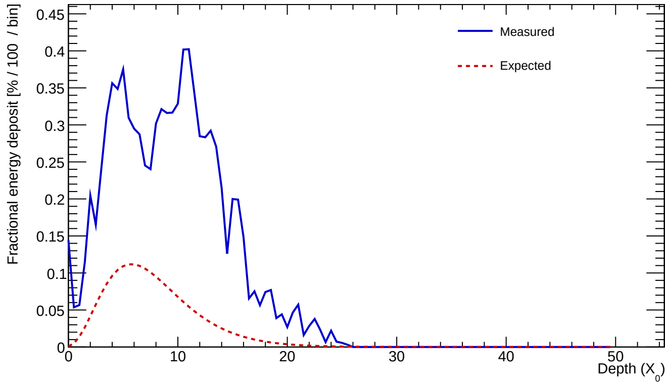
Cluster 228 E=25.162 GeV profileStart=1.00 X_0 \chi=0.3820
