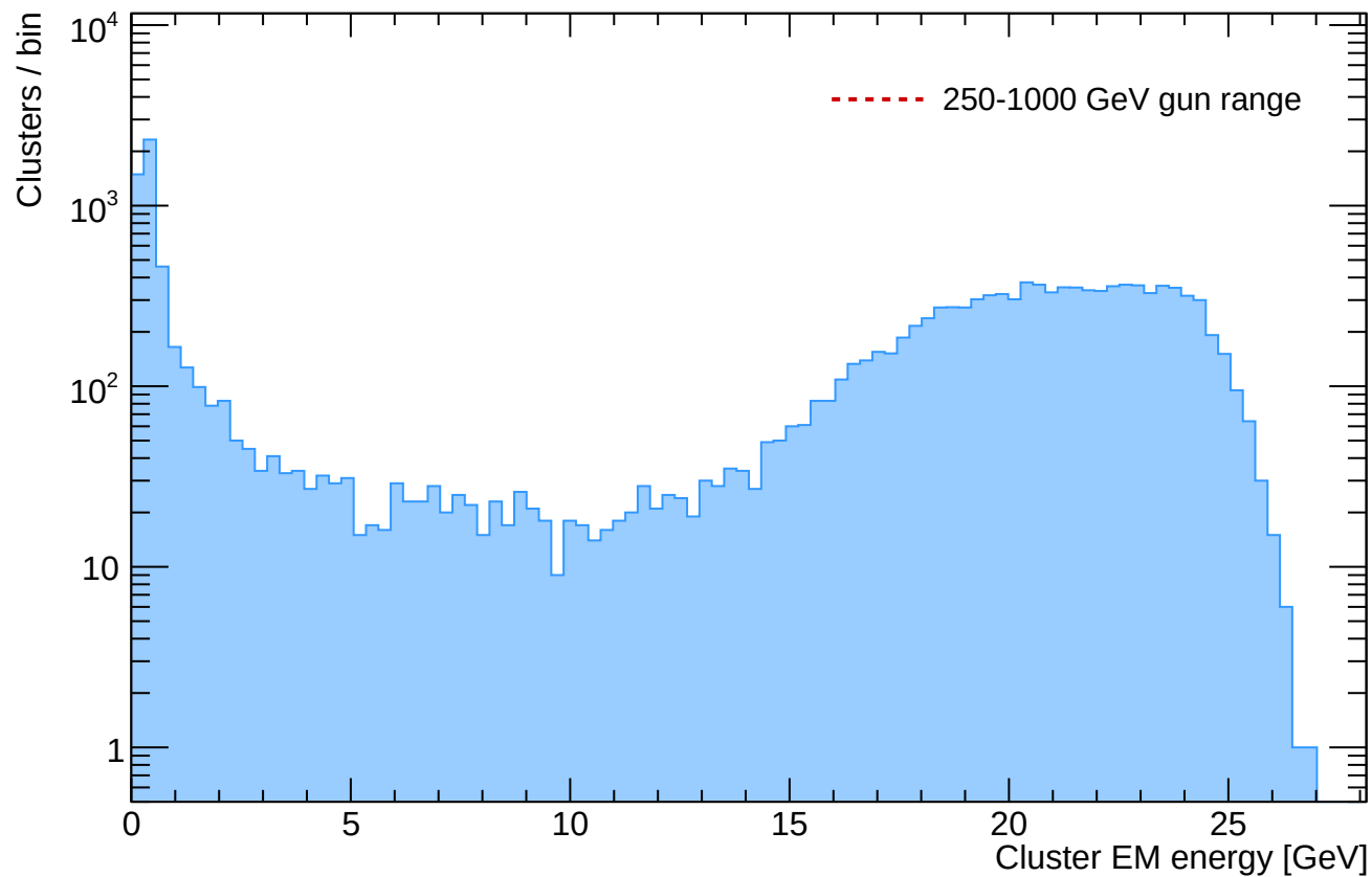
Cluster energy distribution (all clusters)
