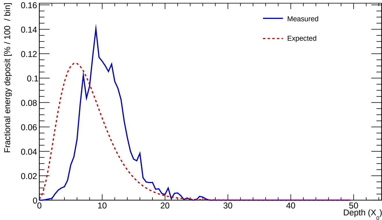
Cluster 176 E=24.271 GeV profileStart=3.50 X_0 \chi=0.1785
