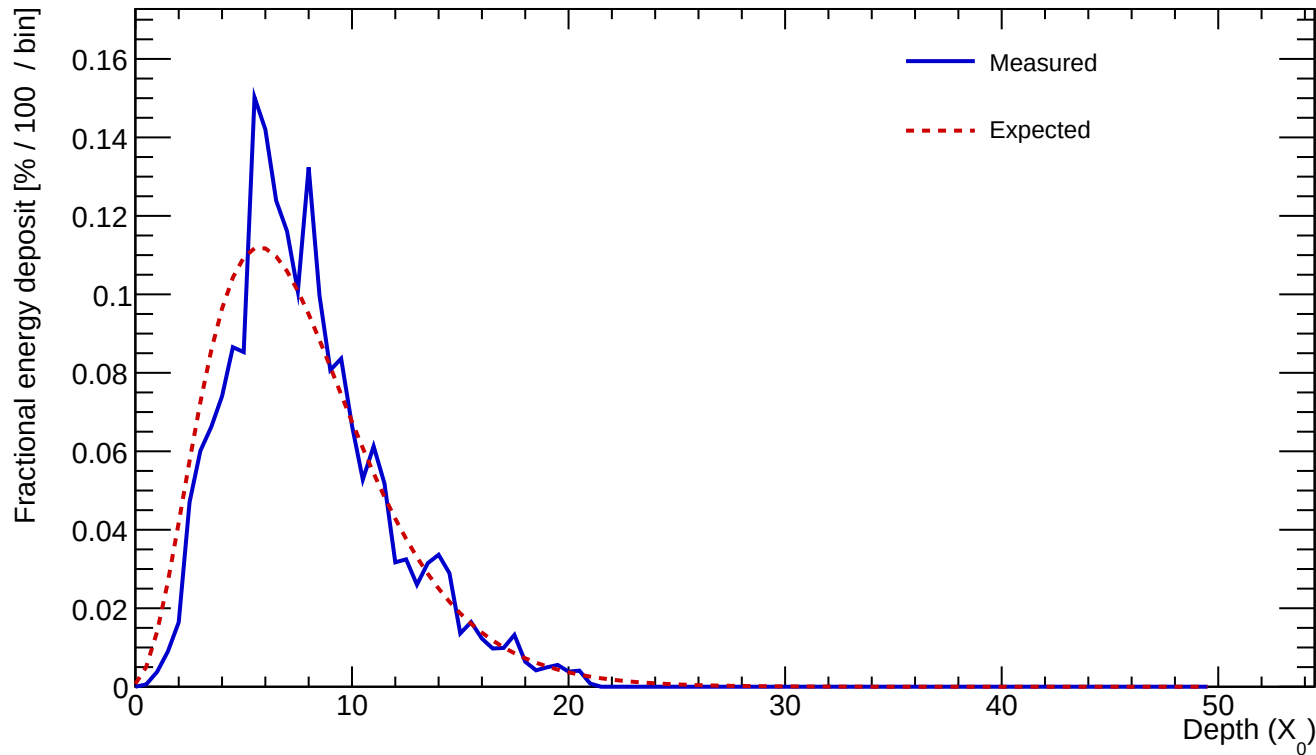
Cluster 699 E=24.934 GeV profileStart=0.50 X_0 \chi=0.1579
