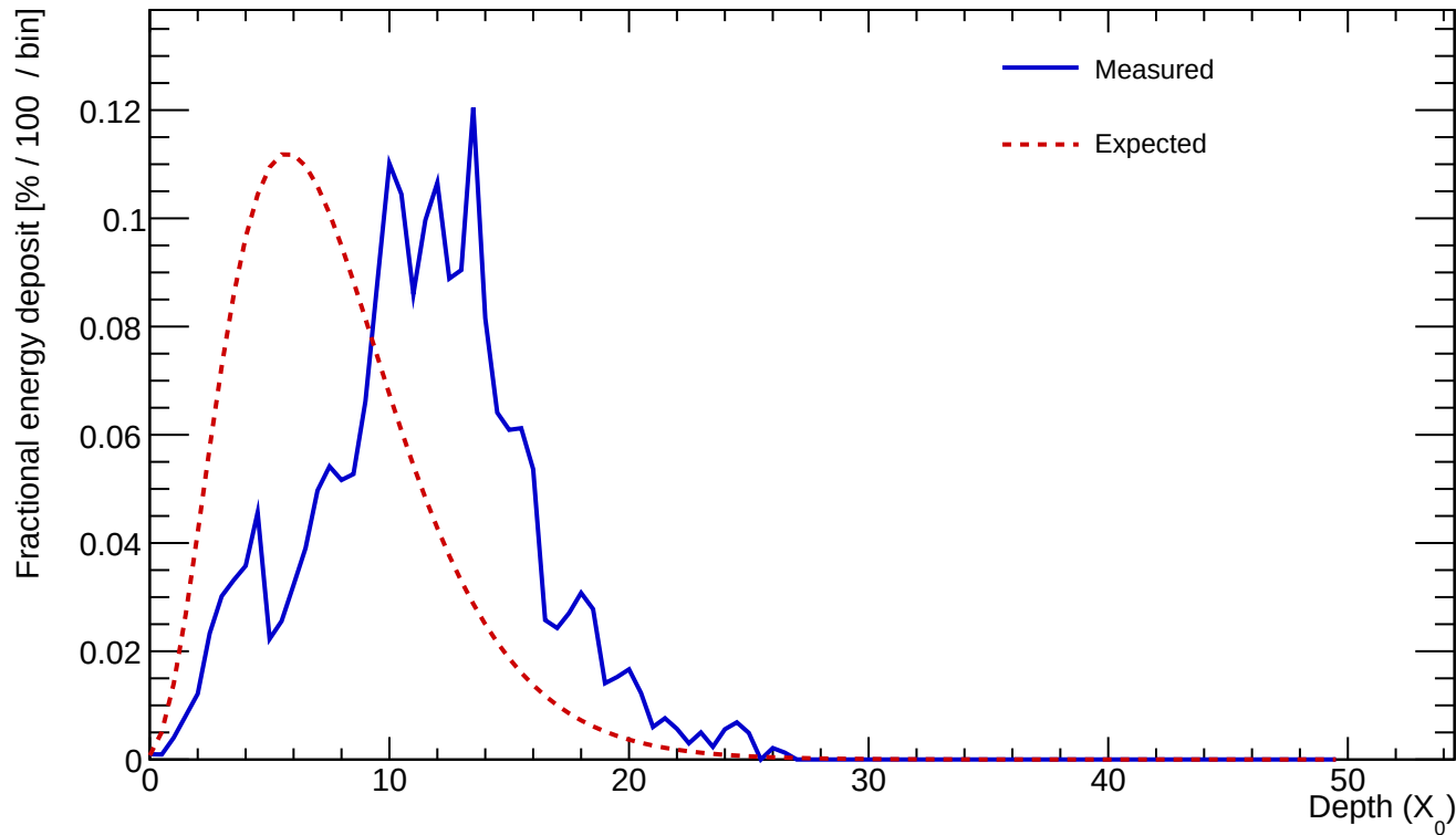
Cluster 345 E=24.818 GeV profileStart=4.50 X_0 \chi=0.2906
