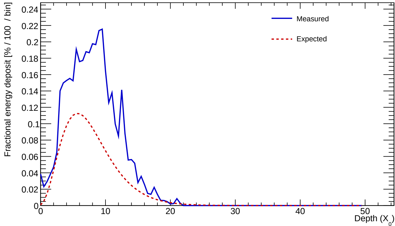
Cluster 476 E=23.669 GeV profileStart=0.50 X_0 \chi=0.1861
