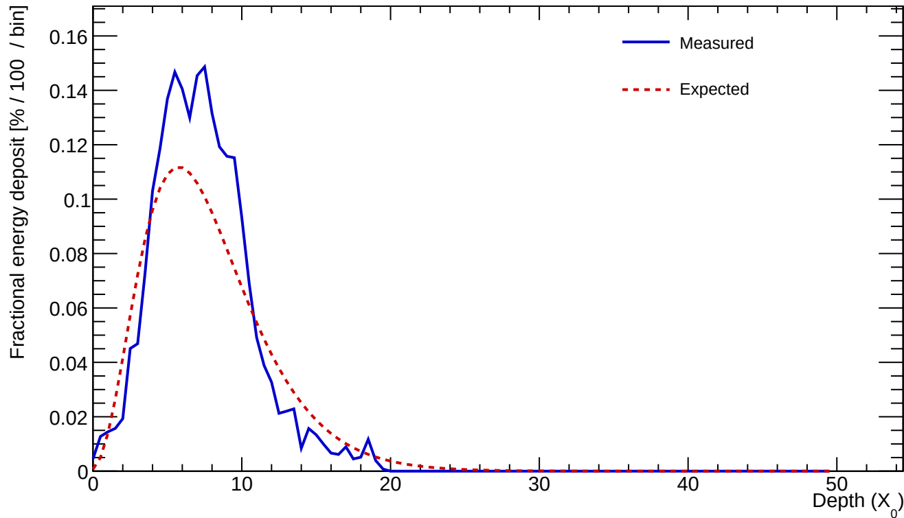
Cluster 558 E=25.267 GeV profileStart=0.50 X_0 \chi=0.2377
