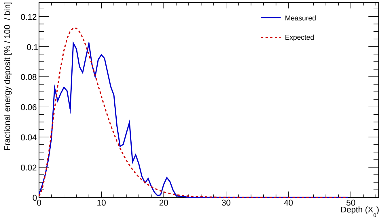
Cluster 541 E=23.839 GeV profileStart=0.50 X_0 \chi=0.2457
