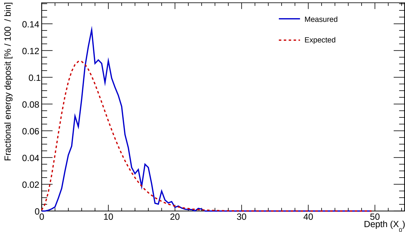
Cluster 245 E=24.695 GeV profileStart=2.00 X_0 \chi=0.1570
