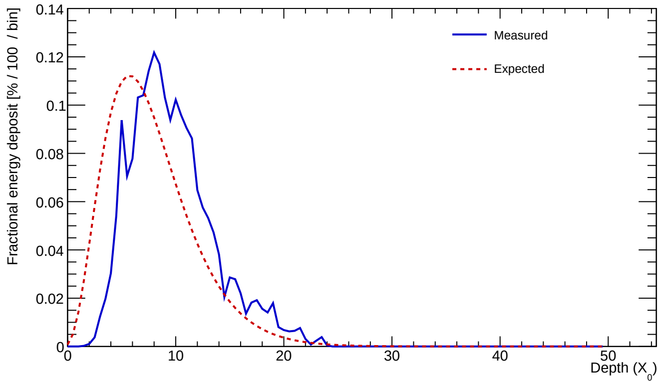
Cluster 218 E=24.408 GeV profileStart=2.00 X_0 \chi=0.1104
