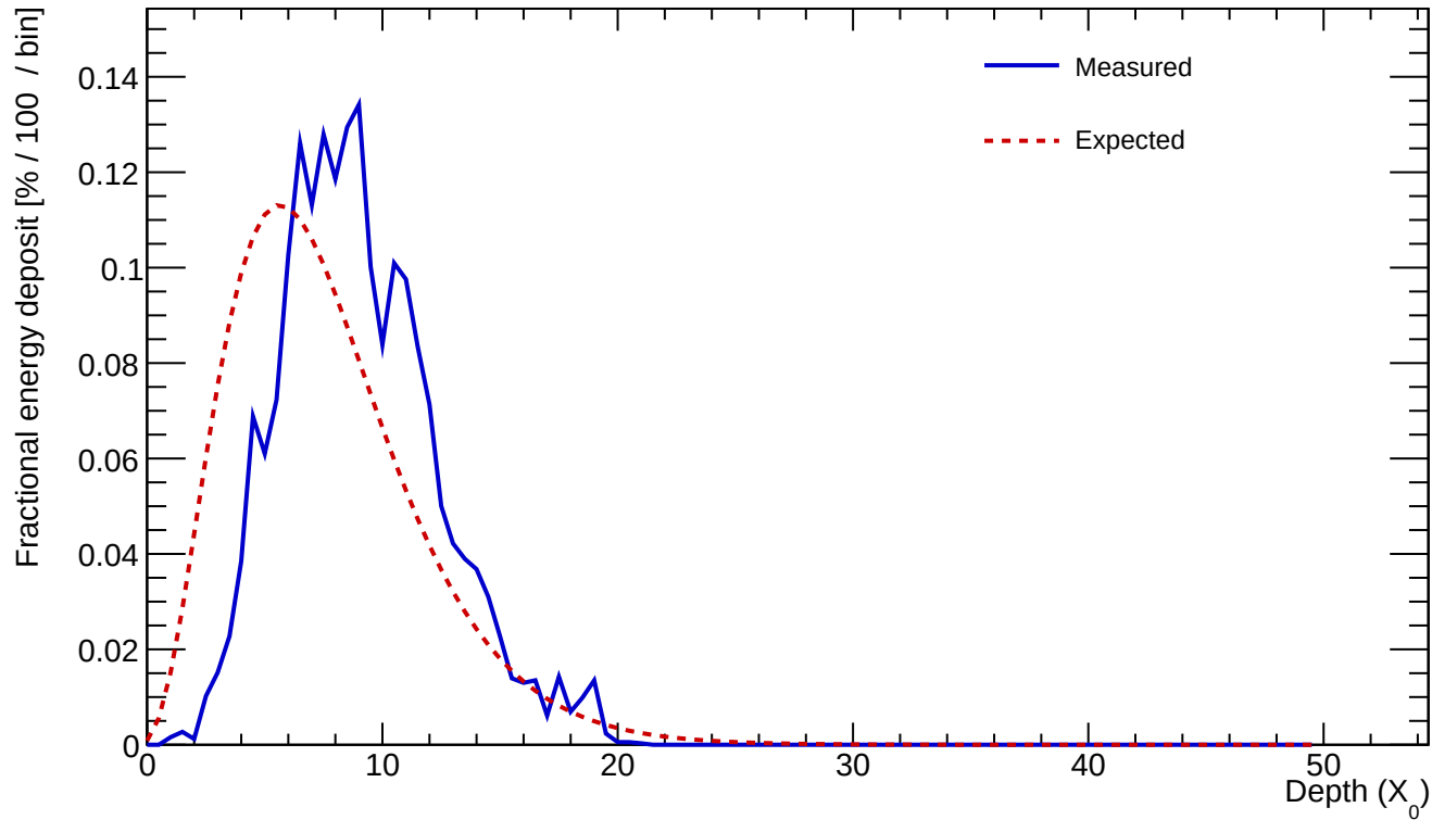
Cluster 23 E=22.573 GeV profileStart=2.00 X_0 \chi=0.1717
