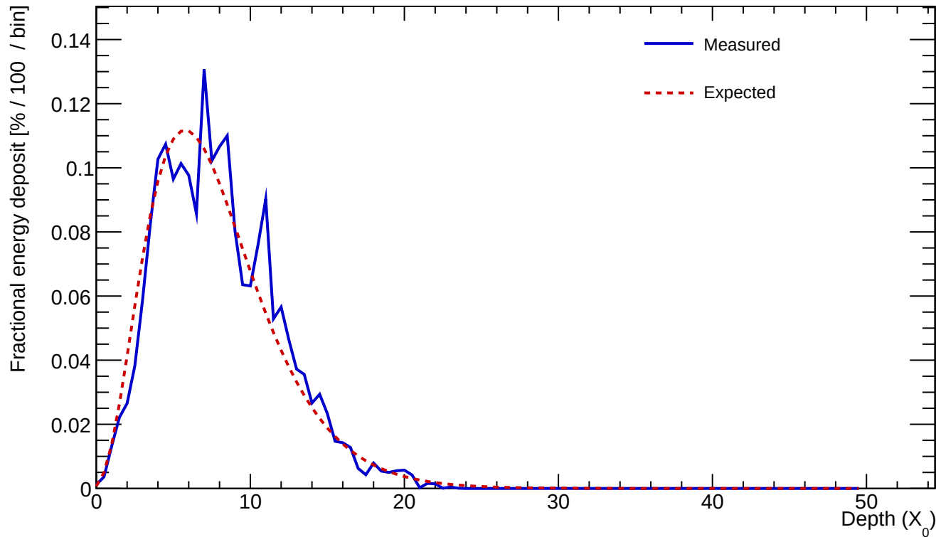
Cluster 475 E=25.500 GeV profileStart=0.50 X_0 \chi=0.1446
