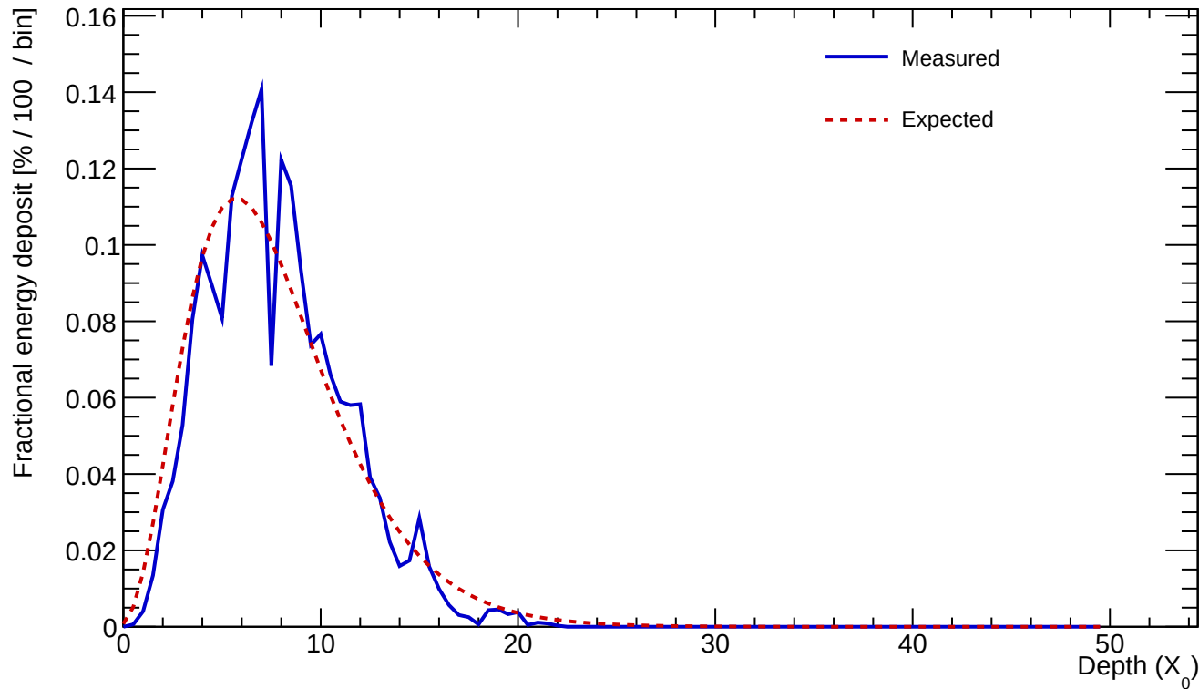
Cluster 428 E=24.465 GeV profileStart=0.50 X_0 \chi=0.1723
