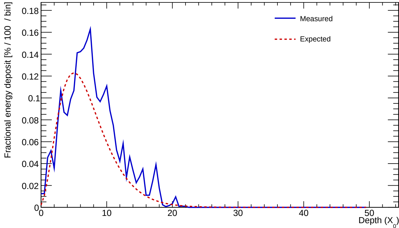
Cluster 423 E=11.694 GeV profileStart=1.00 X_0 \chi=0.2213
