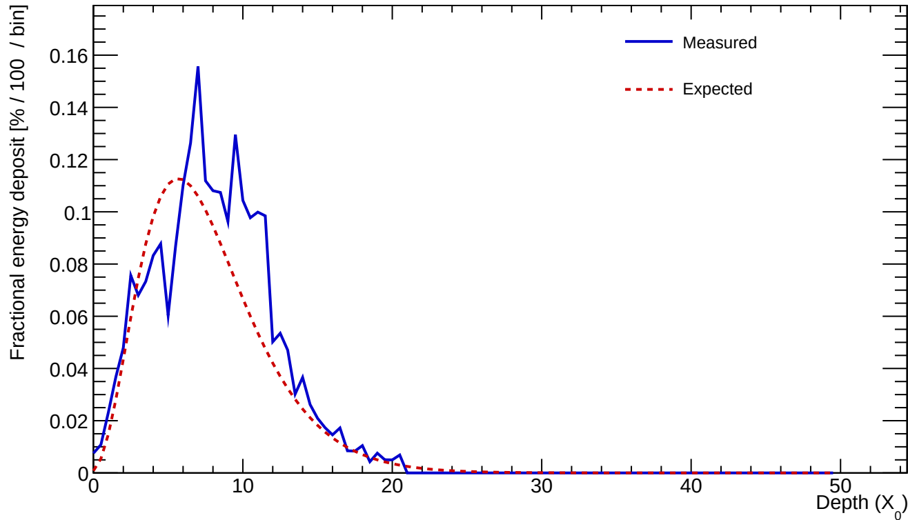
Cluster 103 E=23.221 GeV profileStart=0.50 X_0 \chi=0.2253
