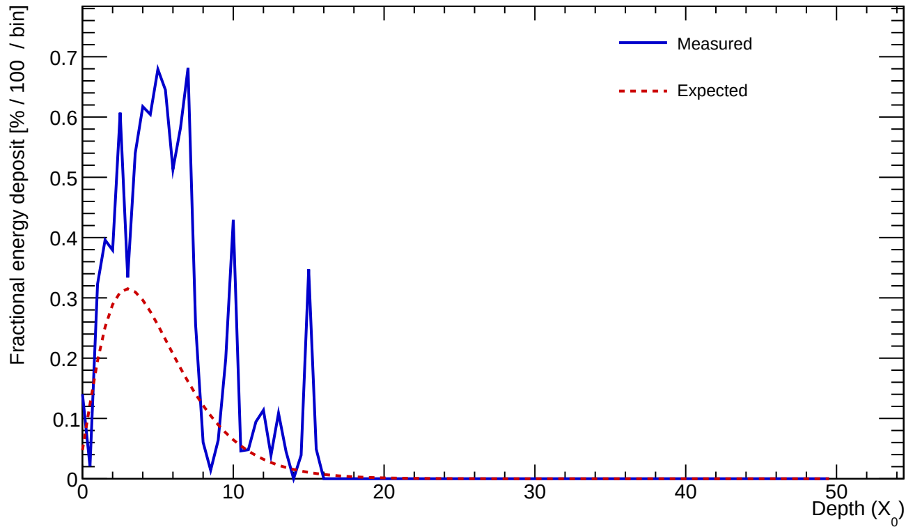
Cluster 105 E=1.586 GeV profileStart=0.50 X_0 \chi=0.3573
