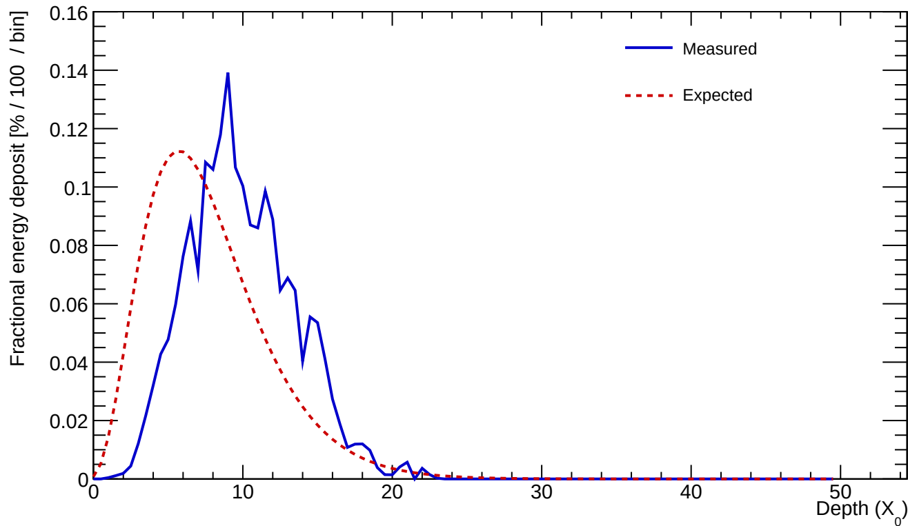
Cluster 482 E=24.016 GeV profileStart=2.50 X_0 \chi=0.1595
