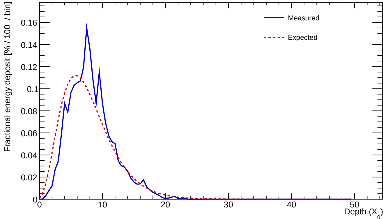
Cluster 108 E=25.136 GeV profileStart=1.00 X_0 \chi=0.1578
