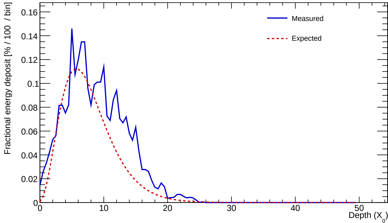
Cluster 77 E=24.200 GeV profileStart=0.50 X_0 \chi=0.2852
