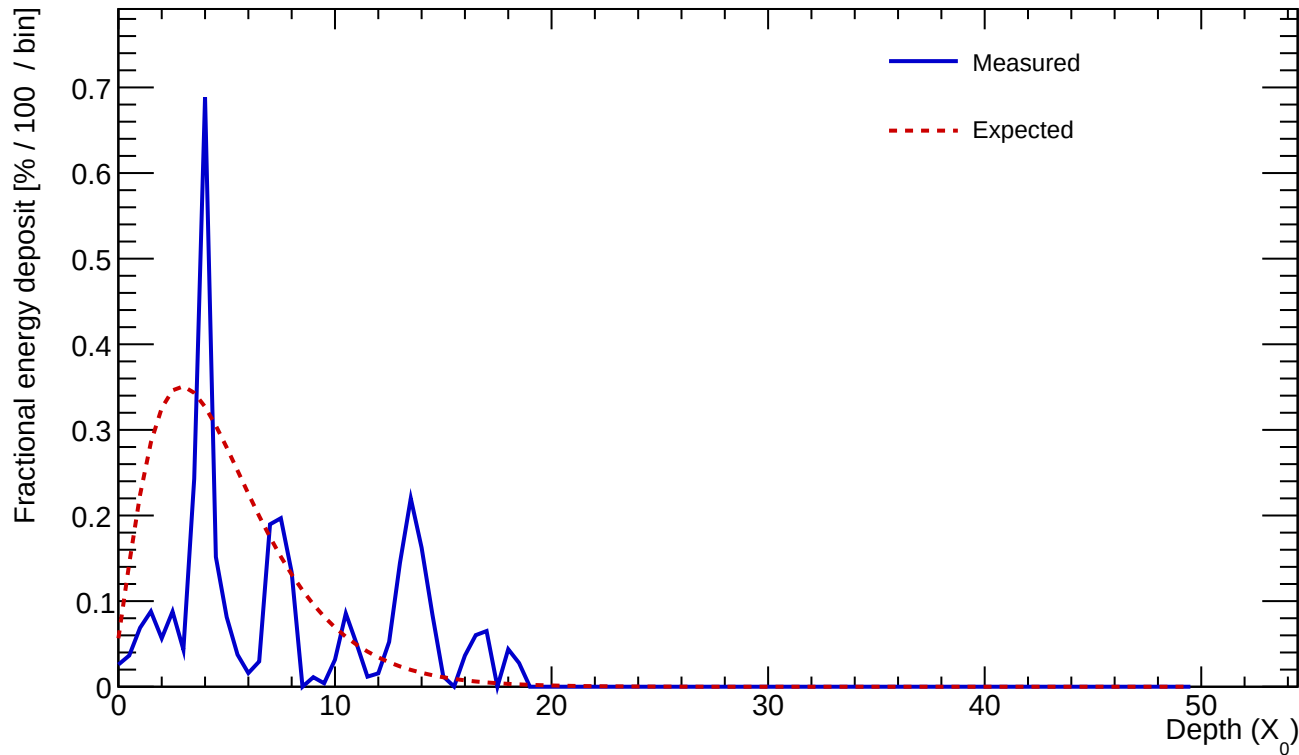
Cluster 448 E=1.480 GeV profileStart=1.00 X_0 \chi=0.8781
