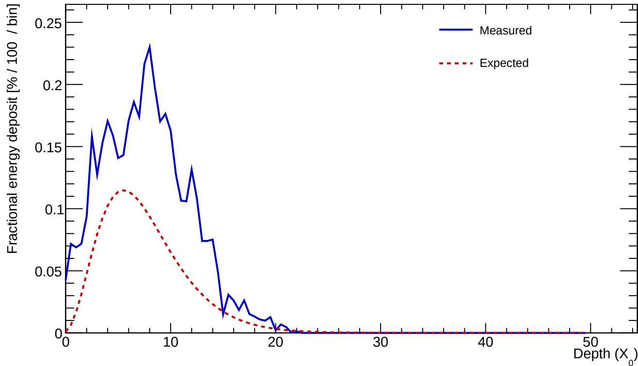
Cluster 494 E=19.751 GeV profileStart=0.50 X_0 \chi=0.2314
