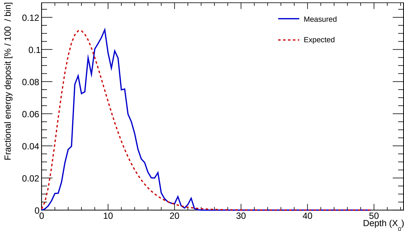
Cluster 638 E=25.234 GeV profileStart=2.50 X_0 \chi=0.1536
