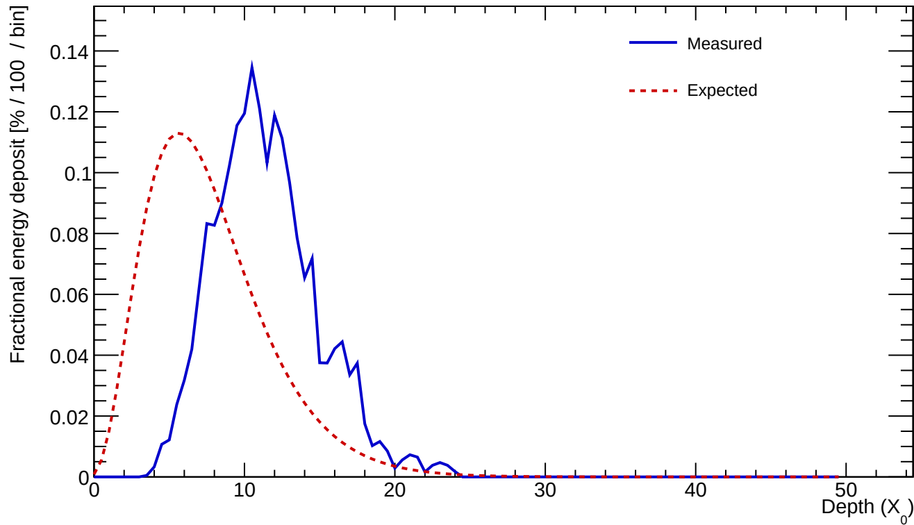
Cluster 25 E=22.659 GeV profileStart=4.50 X_0 \chi=0.1545
