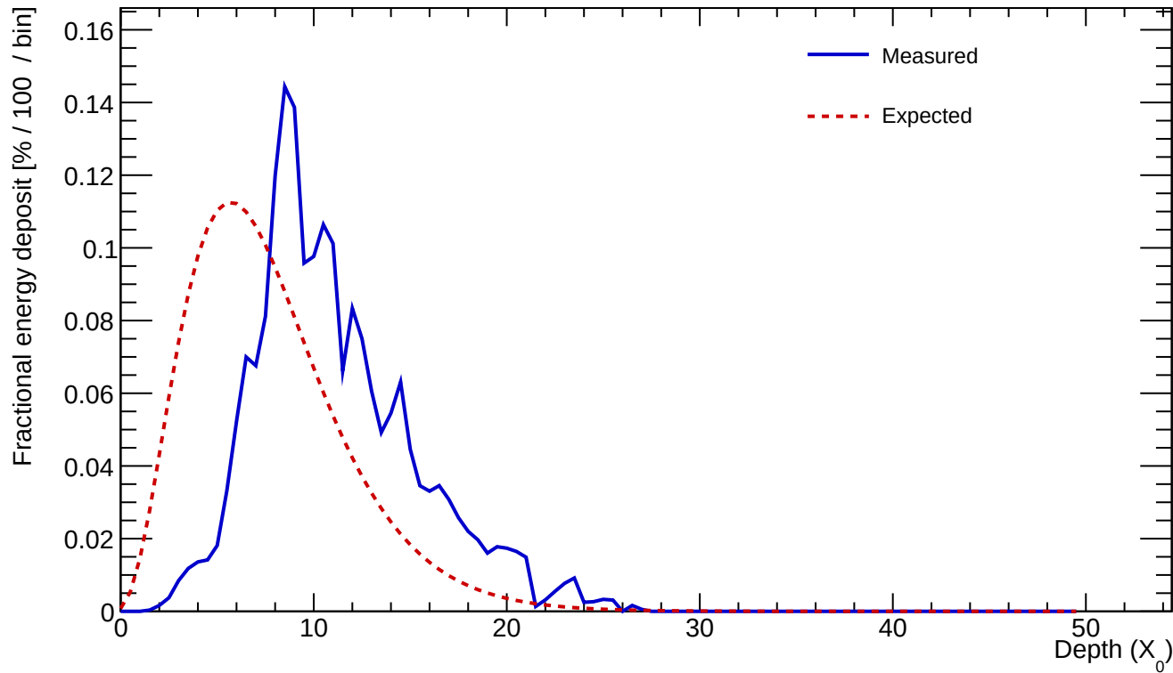
Cluster 467 E=23.601 GeV profileStart=3.50 X_0 \chi=0.1753
