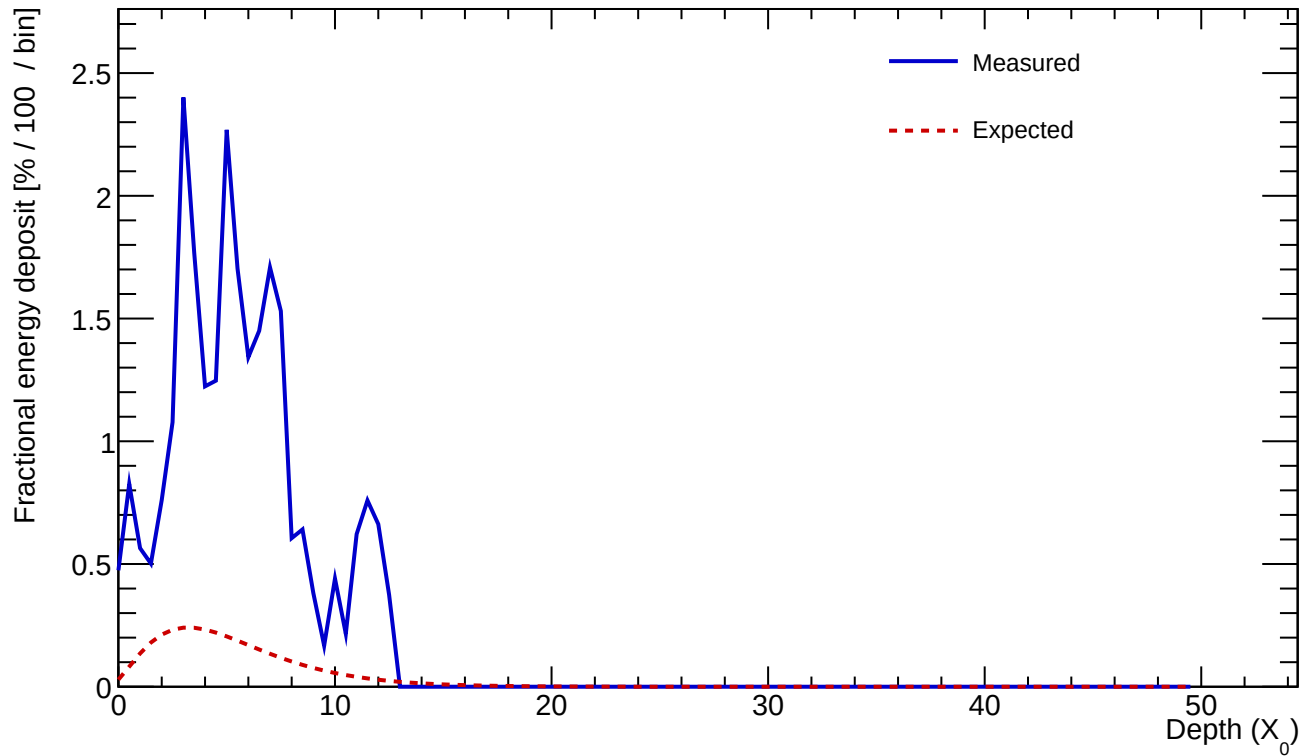
Cluster 477 E=1.996 GeV profileStart=1.00 X_0 \chi=0.3424
