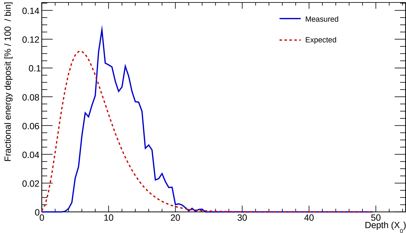
Cluster 593 E=25.538 GeV profileStart=4.00 X_0 \chi=0.1570
