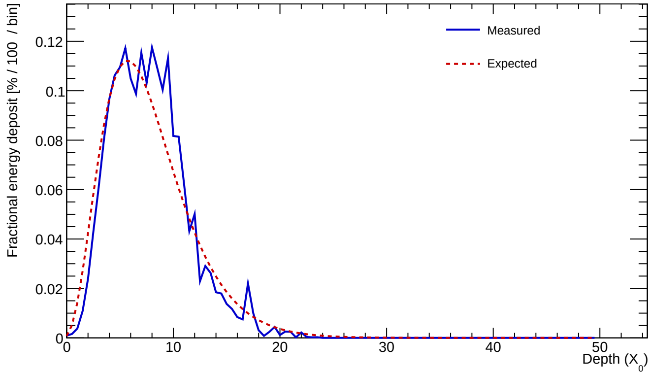
Cluster 531 E=24.376 GeV profileStart=0.50 X_0 \chi=0.1501
