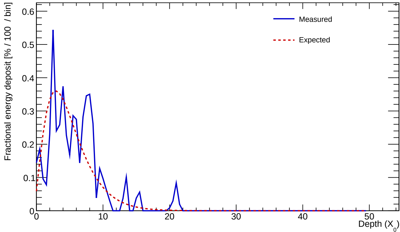
Cluster 177 E=1.458 GeV profileStart=1.00 X_0 \chi=0.4933
