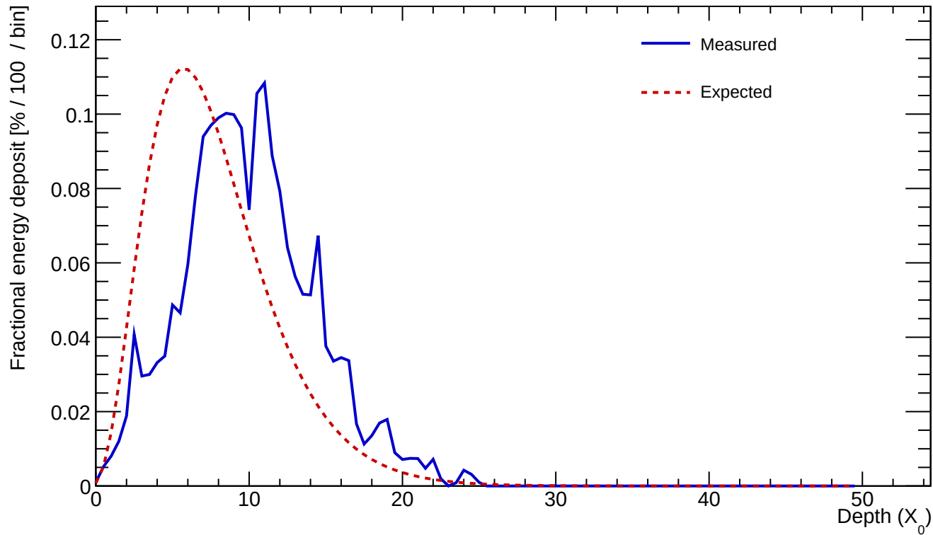
Cluster 421 E=24.171 GeV profileStart=3.00 X_0 \chi=0.2147
