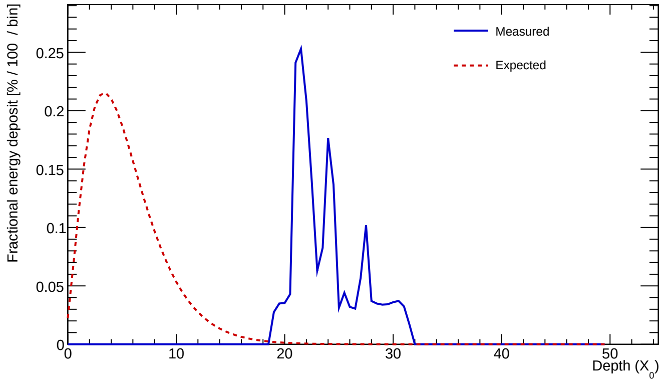
Cluster 168 E=2.284 GeV profileStart=31.00 X_0 \chi=1.0114
