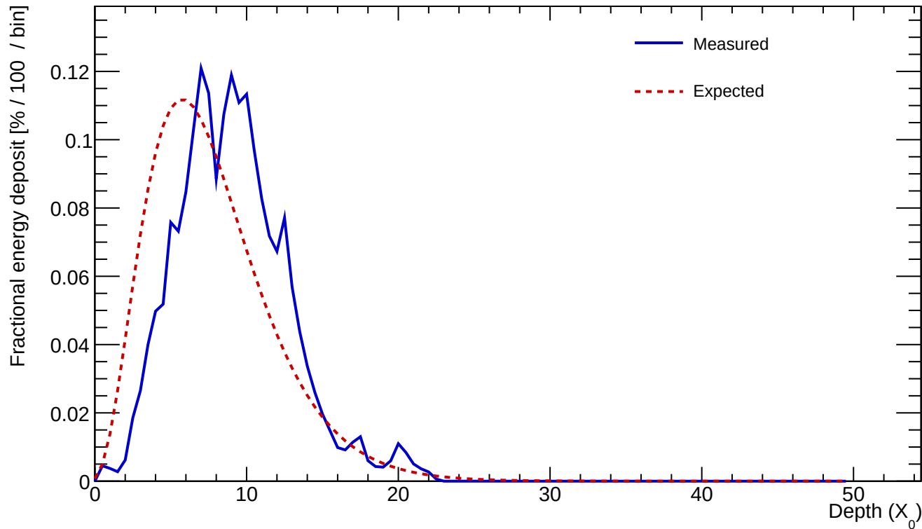
Cluster 107 E=25.183 GeV profileStart=2.00 X_0 \chi=0.1676
