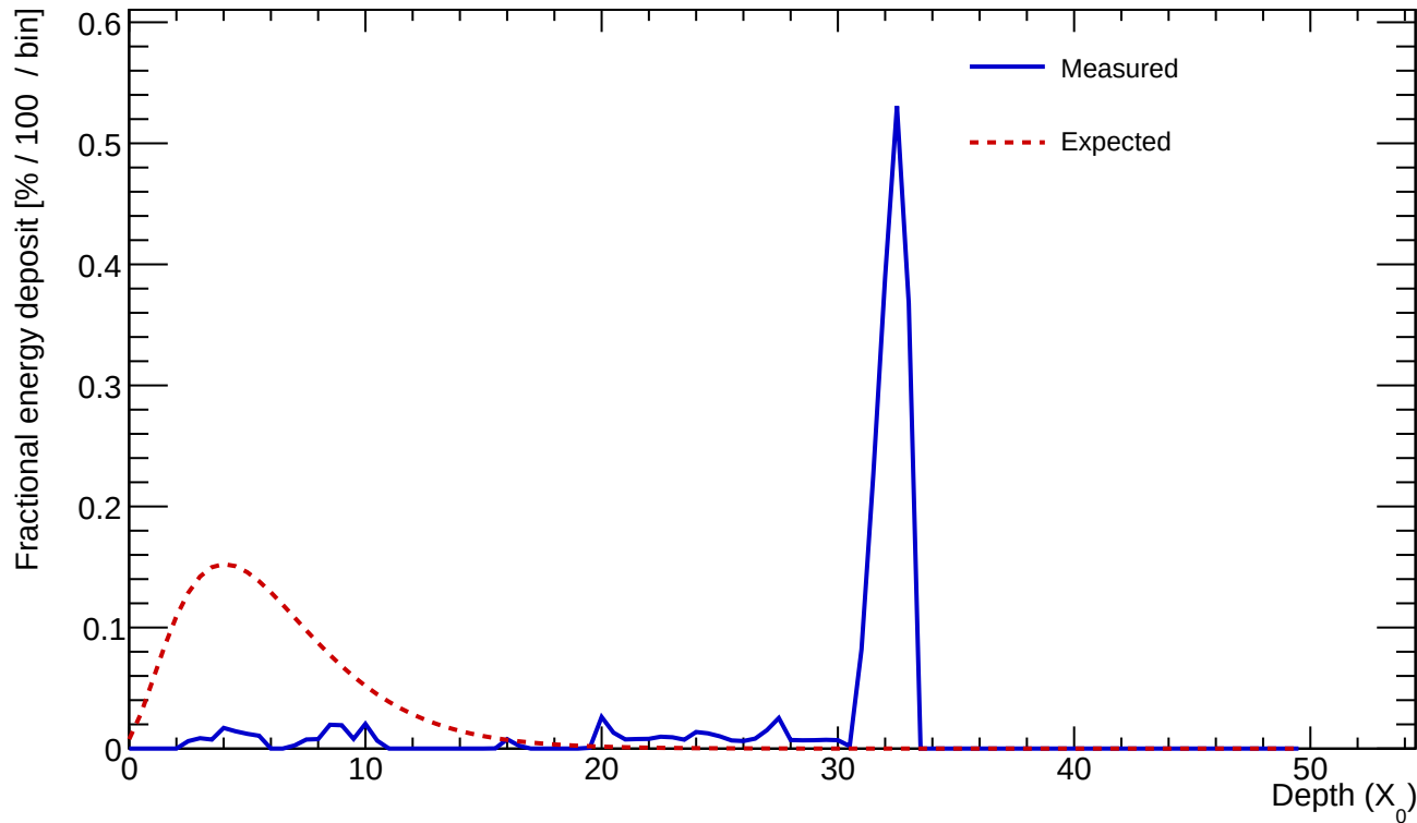
Cluster 422 E=4.520 GeV profileStart=30.00 X_0 \chi=0.4170
