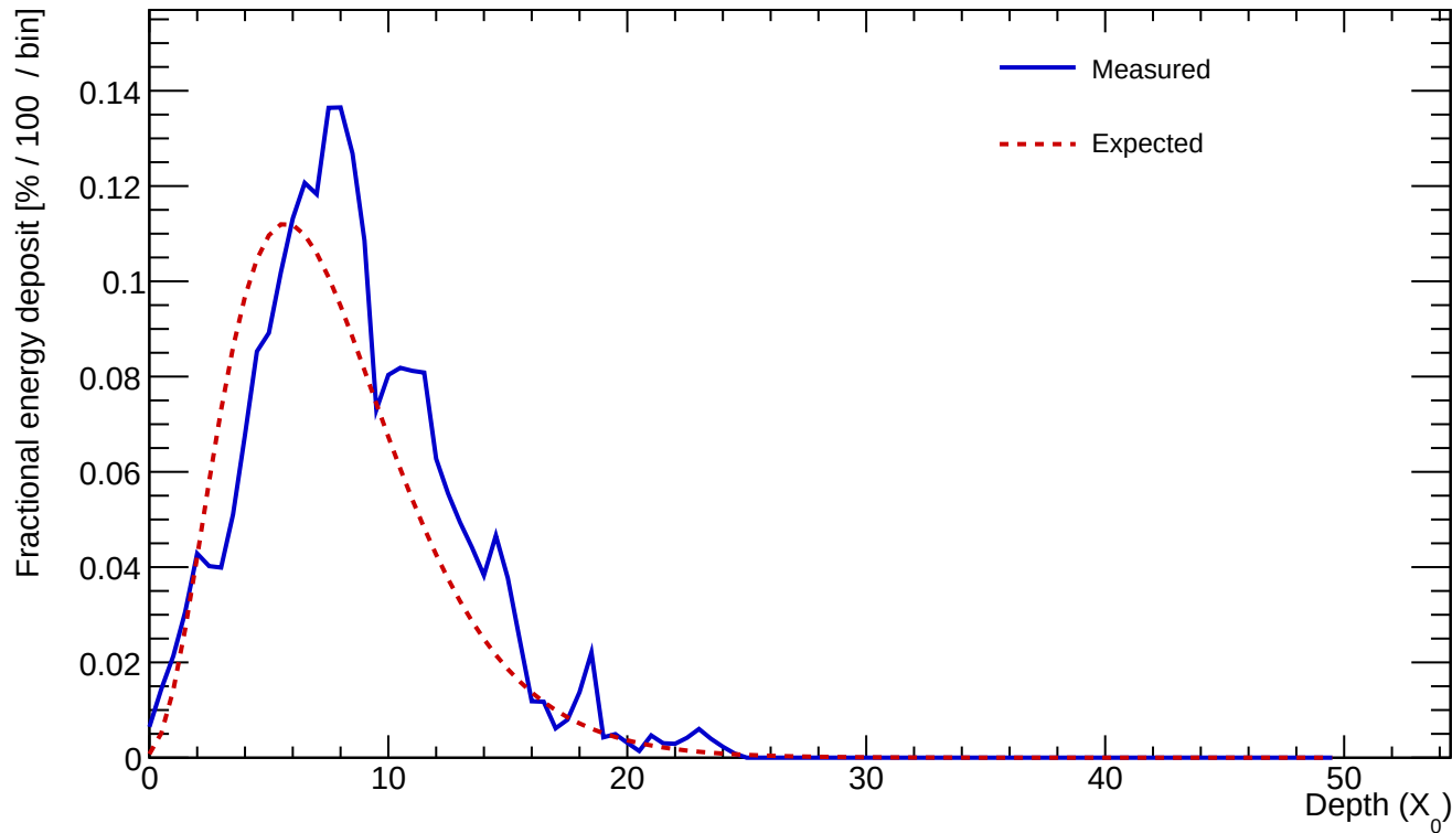
Cluster 331 E=24.528 GeV profileStart=1.00 X_0 \chi=0.1782
