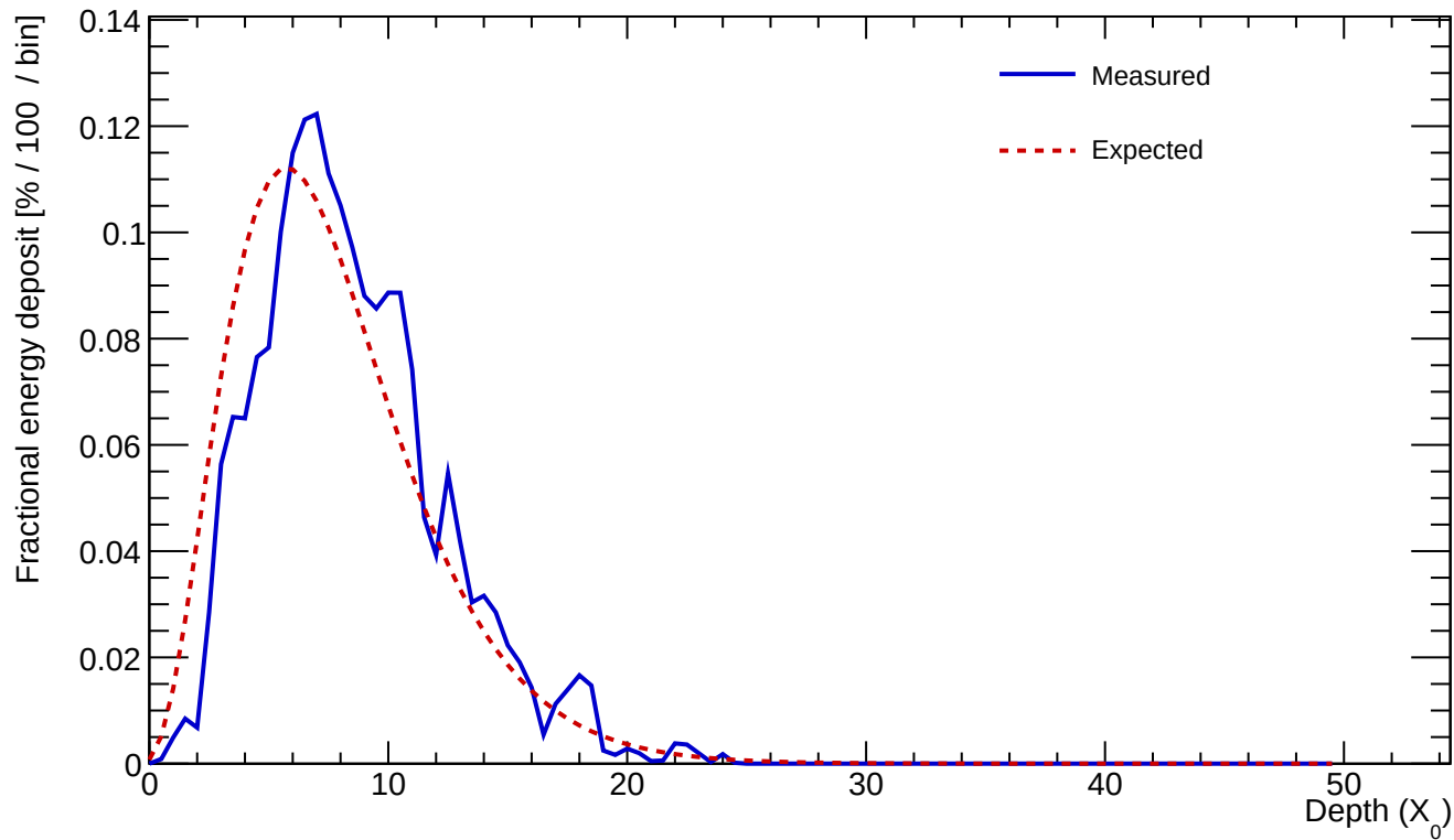
Cluster 96 E=24.565 GeV profileStart=1.00 X_0 \chi=0.1264
