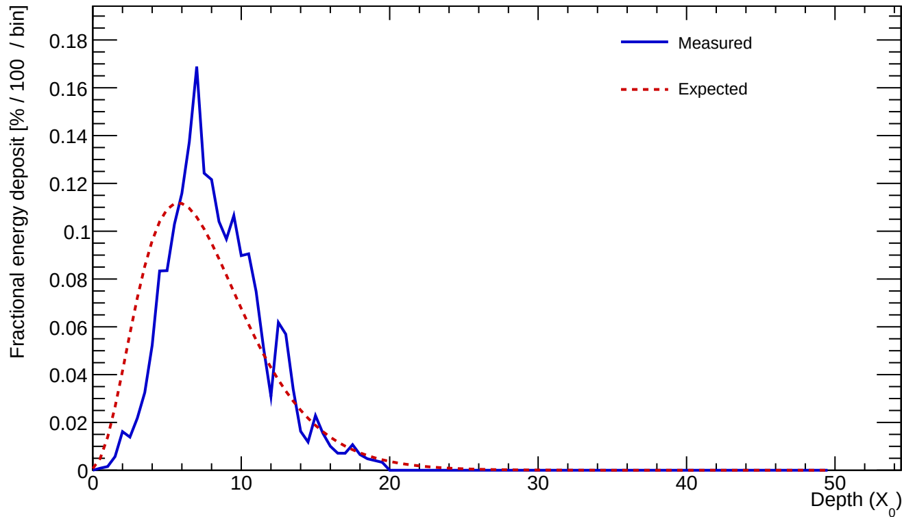
Cluster 143 E=25.264 GeV profileStart=1.50 X_0 \chi=0.1971
