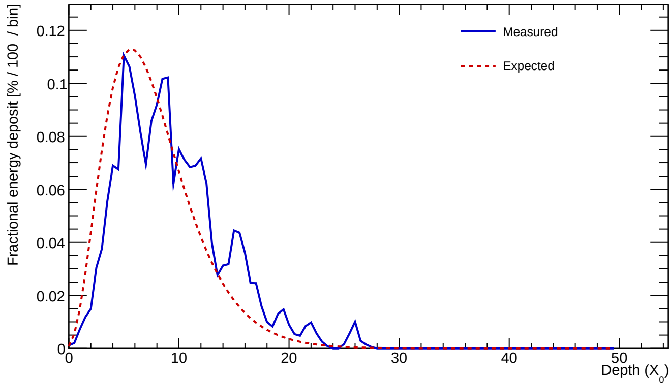
Cluster 679 E=23.013 GeV profileStart=1.00 X_0 \chi=0.2167
