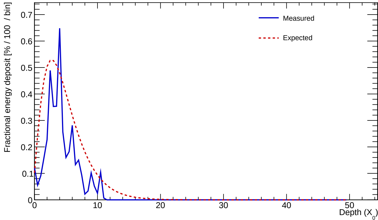
Cluster 271 E=1.226 GeV profileStart=0.50 X_0 \chi=0.3796
