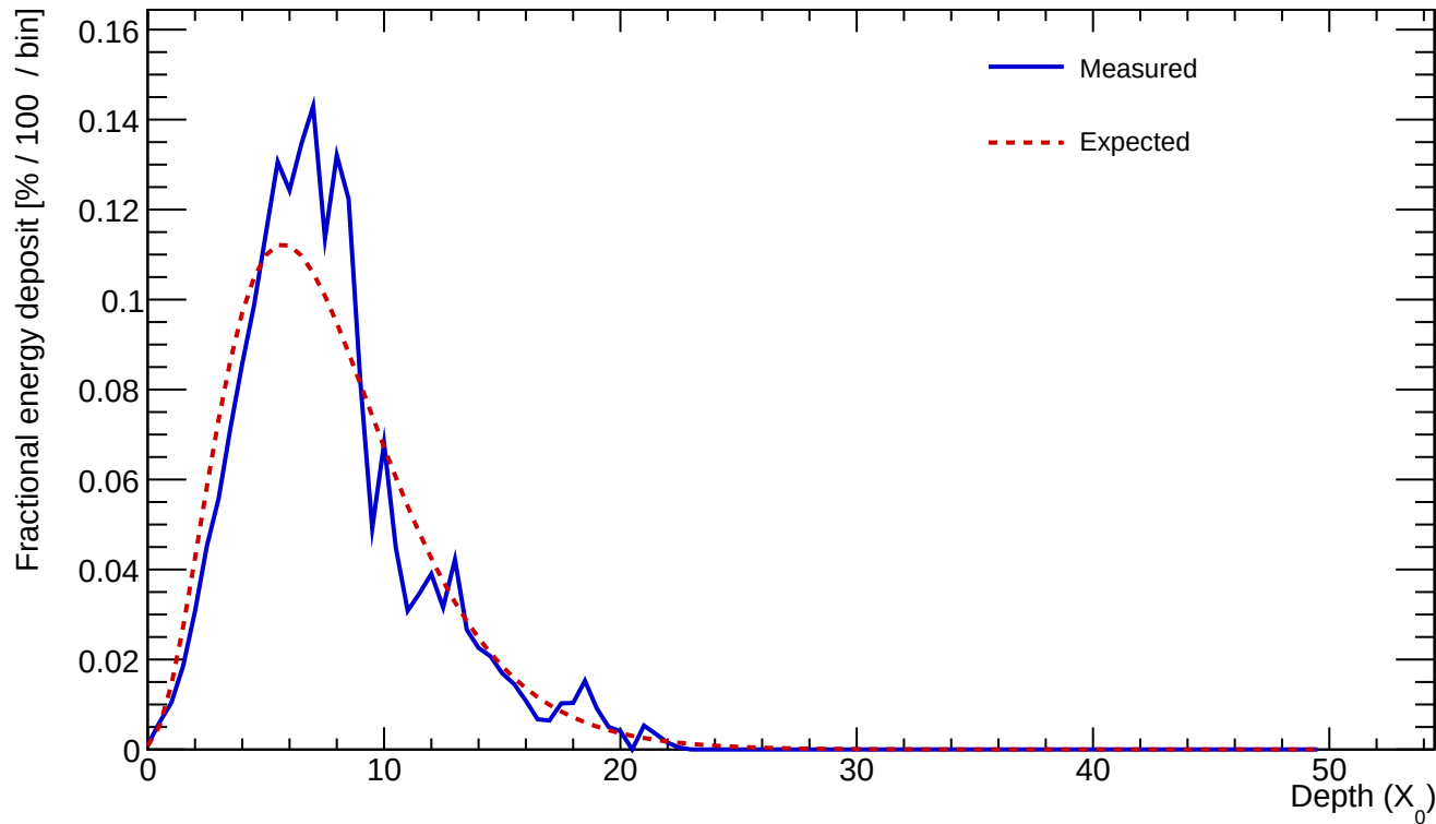
Cluster 135 E=24.199 GeV profileStart=0.50 X_0 \chi=0.1933
