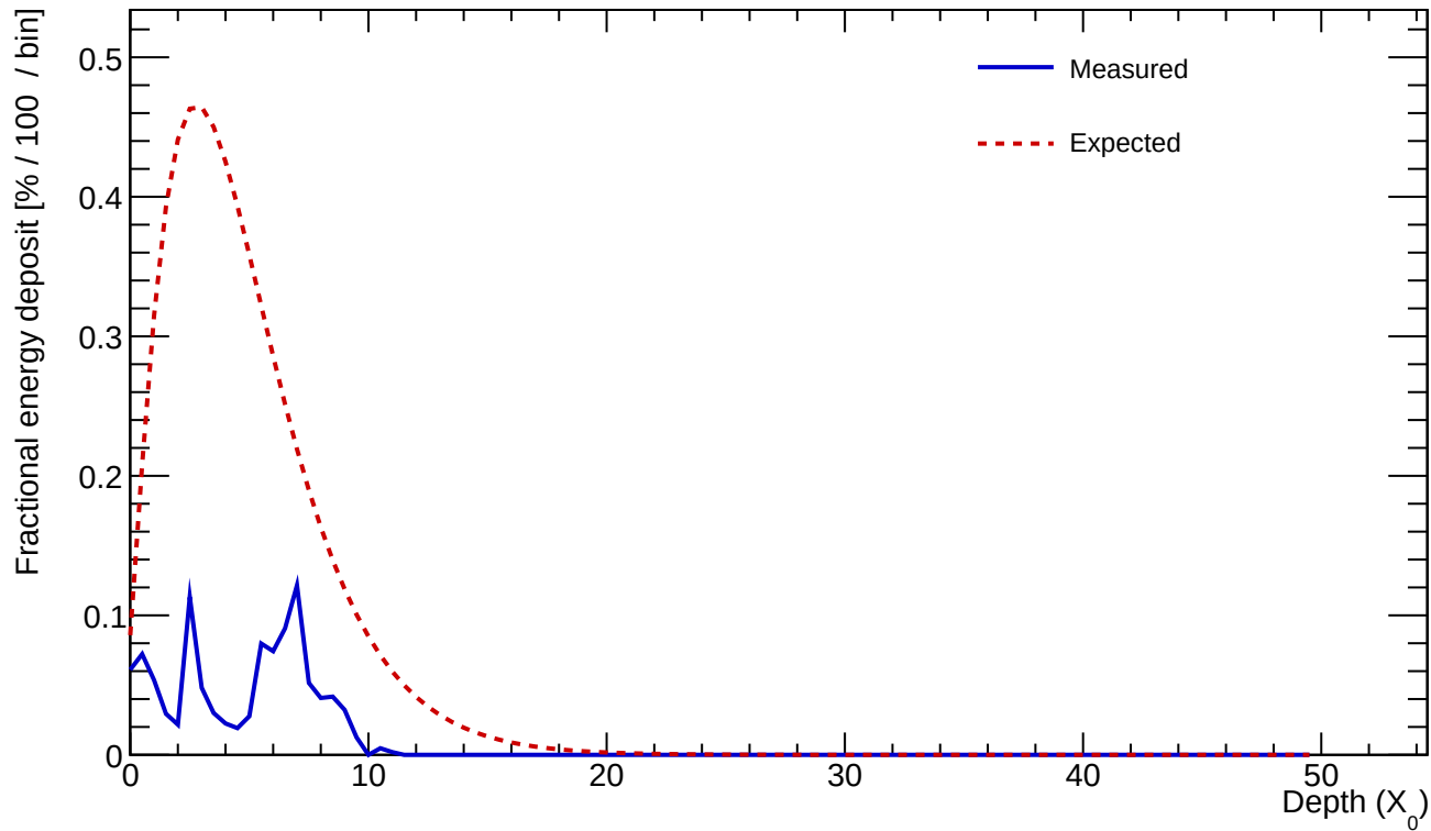
Cluster 288 E=1.287 GeV profileStart=2.00 X_0 \chi=0.6420
