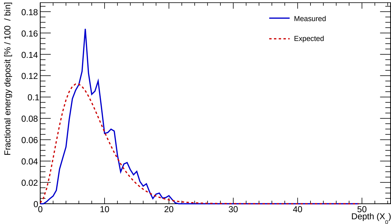
Cluster 322 E=24.126 GeV profileStart=1.00 X_0 \chi=0.1452
