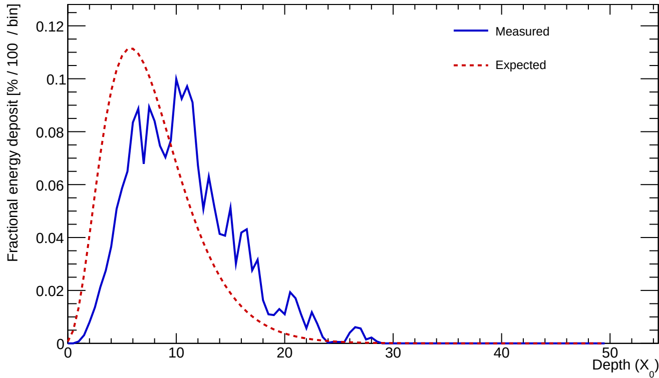
Cluster 667 E=25.929 GeV profileStart=2.50 X_0 \chi=0.2322
