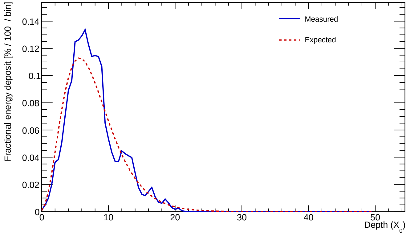
Cluster 255 E=23.008 GeV profileStart=0.50 X_0 \chi=0.1669
