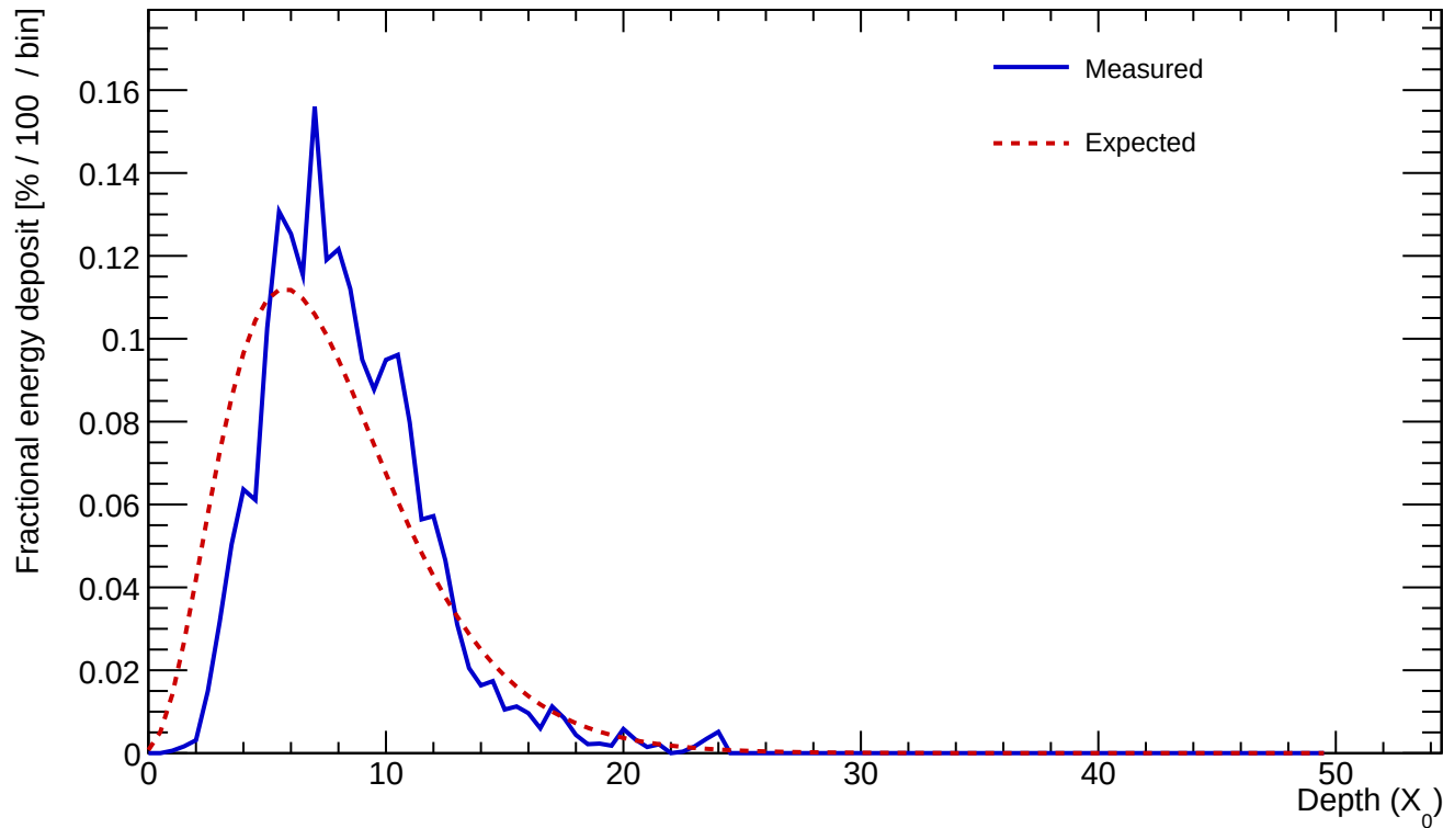
Cluster 148 E=24.797 GeV profileStart=1.00 X_0 \chi=0.2082
