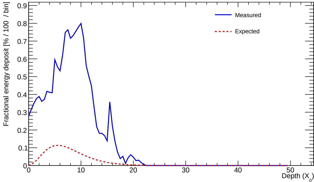
Cluster 444 E=21.455 GeV profileStart=1.50 X_0 \chi=0.3223
