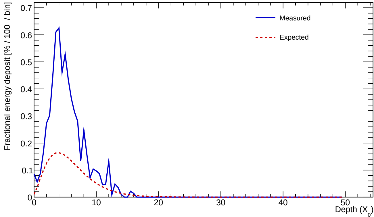
Cluster 412 E=3.695 GeV profileStart=0.50 X_0 \chi=0.2844
