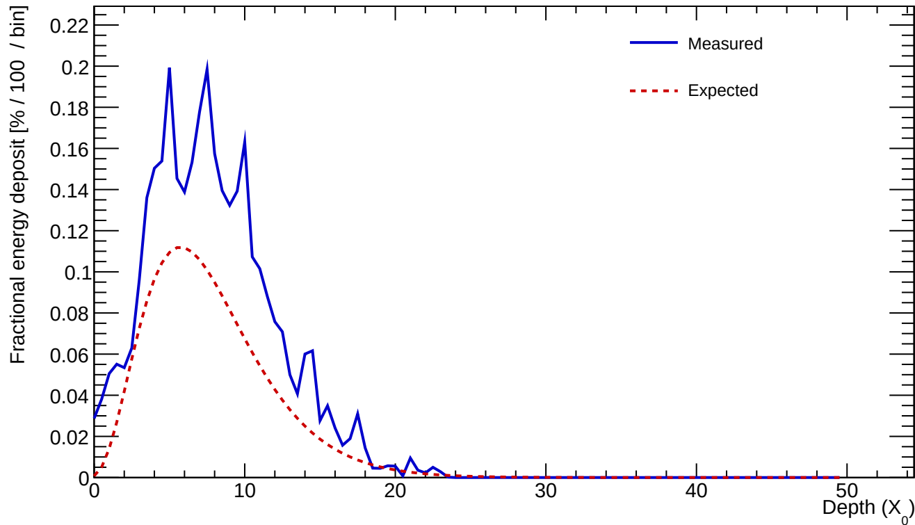
Cluster 343 E=24.843 GeV profileStart=0.50 X_0 \chi=0.1732
