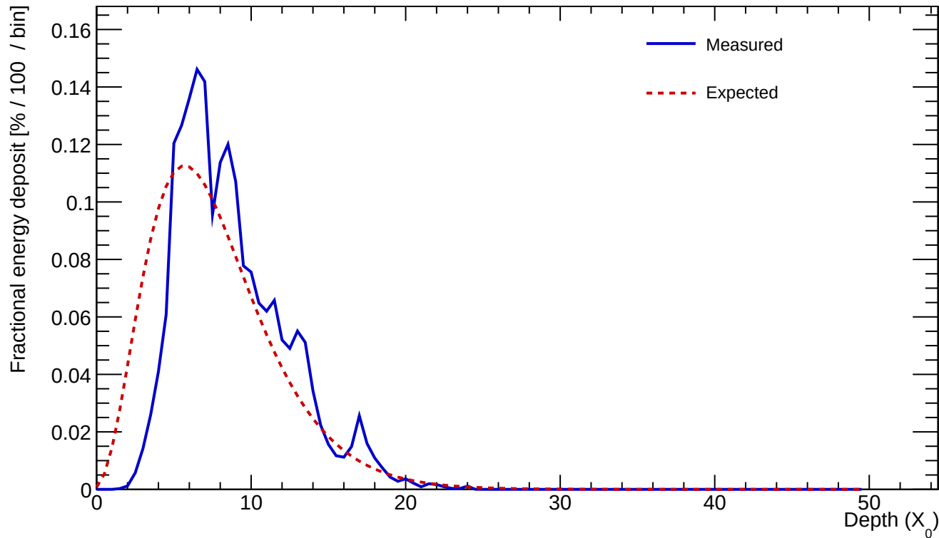
Cluster 231 E=23.657 GeV profileStart=1.50 X_0 \chi=0.2262
