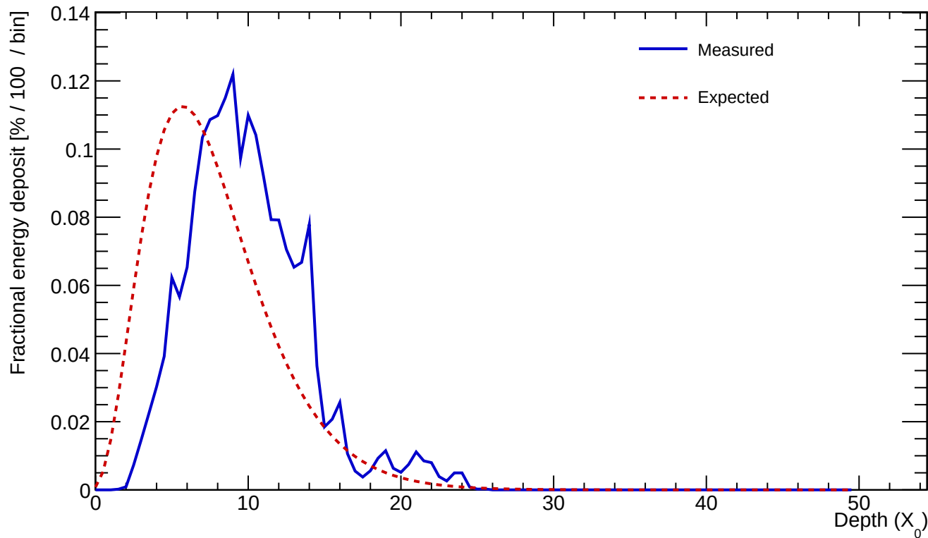
Cluster 583 E=23.512 GeV profileStart=2.50 X_0 \chi=0.1598
