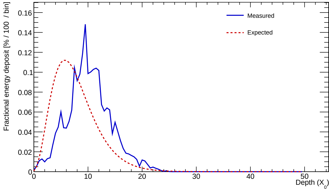
Cluster 71 E=24.472 GeV profileStart=3.00 X_0 \chi=0.2346
