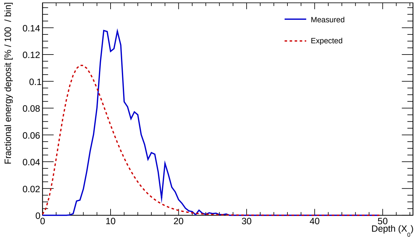
Cluster 532 E=24.602 GeV profileStart=4.50 X_0 \chi=0.1893
