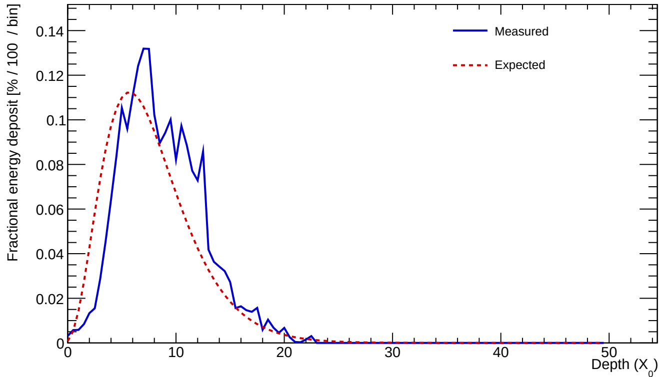
Cluster 185 E=24.087 GeV profileStart=1.50 X_0 \chi=0.1383
