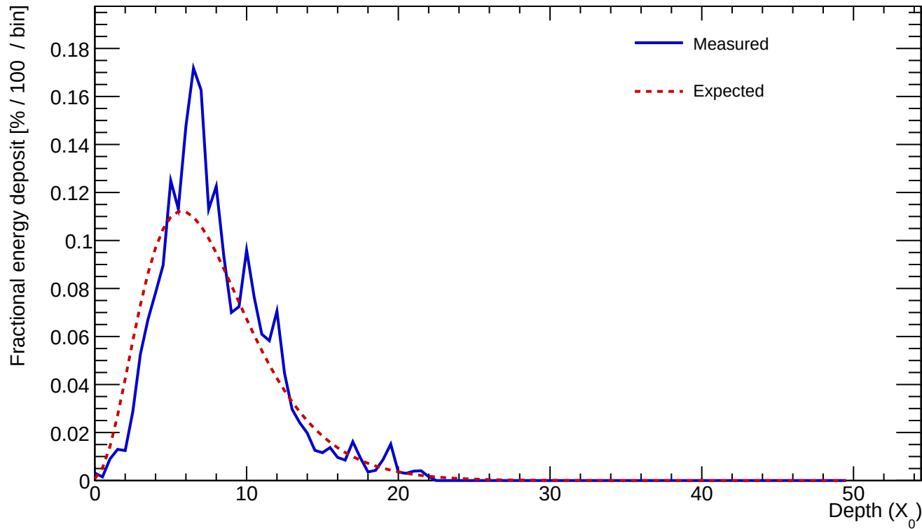
Cluster 543 E=24.385 GeV profileStart=0.50 X_0 \chi=0.2064
