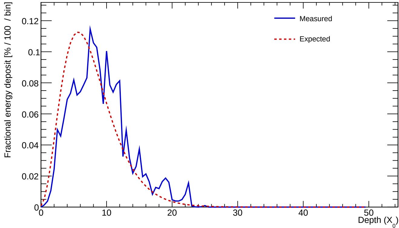
Cluster 79 E=23.377 GeV profileStart=1.00 X_0 \chi=0.2225
