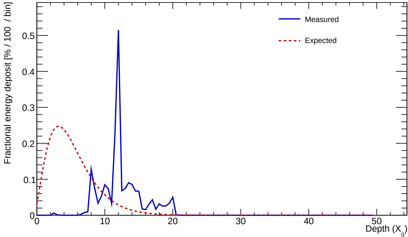
Cluster 152 E=1.943 GeV profileStart=7.50 X_0 \chi=0.6201
