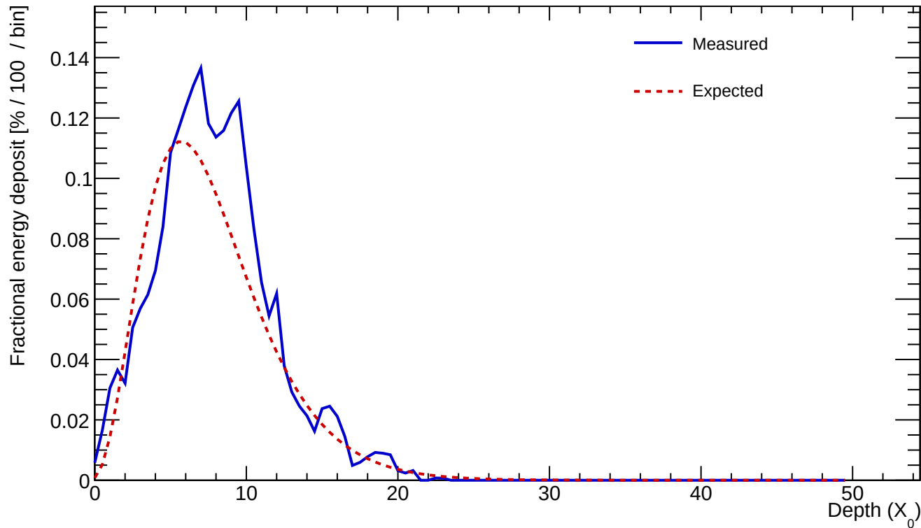
Cluster 605 E=24.203 GeV profileStart=1.00 X_0 \chi=0.1733
