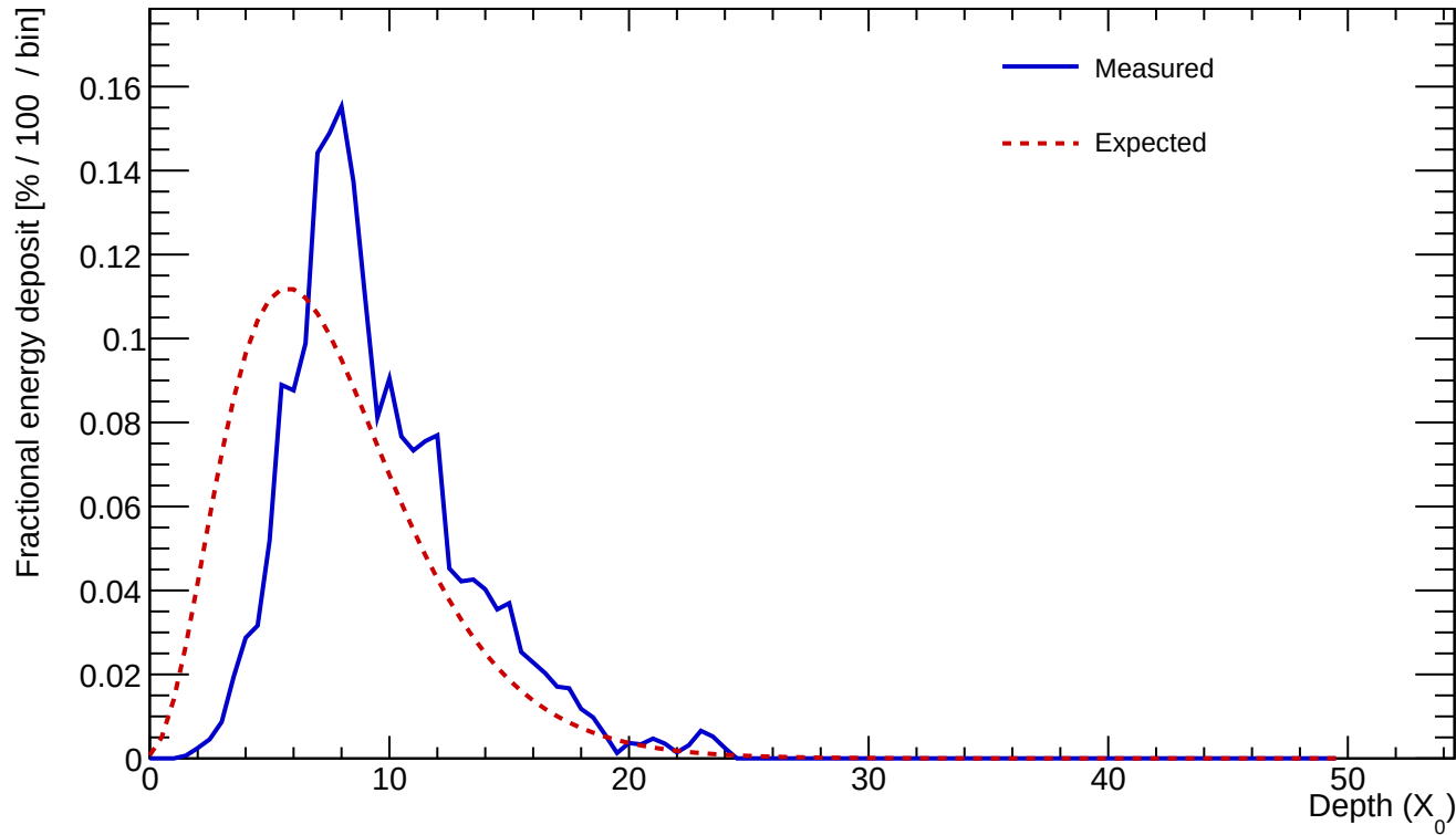
Cluster 342 E=24.908 GeV profileStart=2.00 X_0 \chi=0.1855
