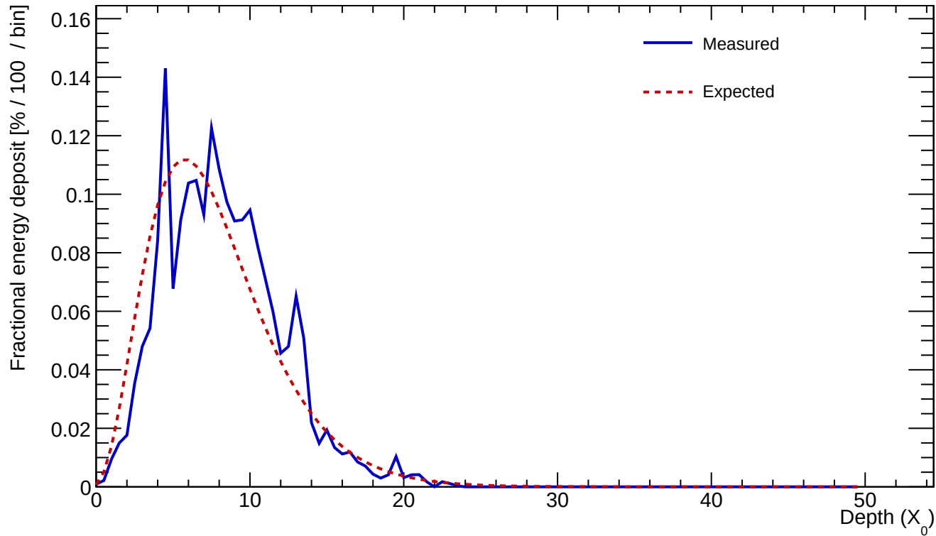
Cluster 28 E=24.977 GeV profileStart=1.00 X_0 \chi=0.1808
