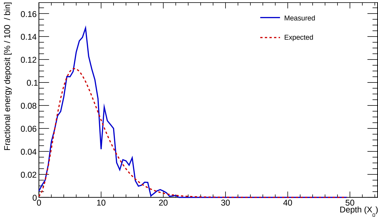
Cluster 563 E=24.369 GeV profileStart=0.50 X_0 \chi=0.1515
