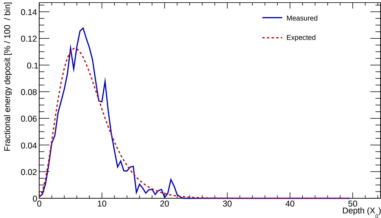
Cluster 669 E=23.639 GeV profileStart=0.50 X_0 \chi=0.1514
