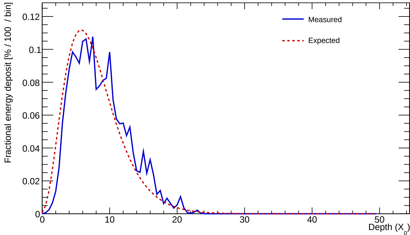
Cluster 615 E=25.294 GeV profileStart=0.50 X_0 \chi=0.1422
