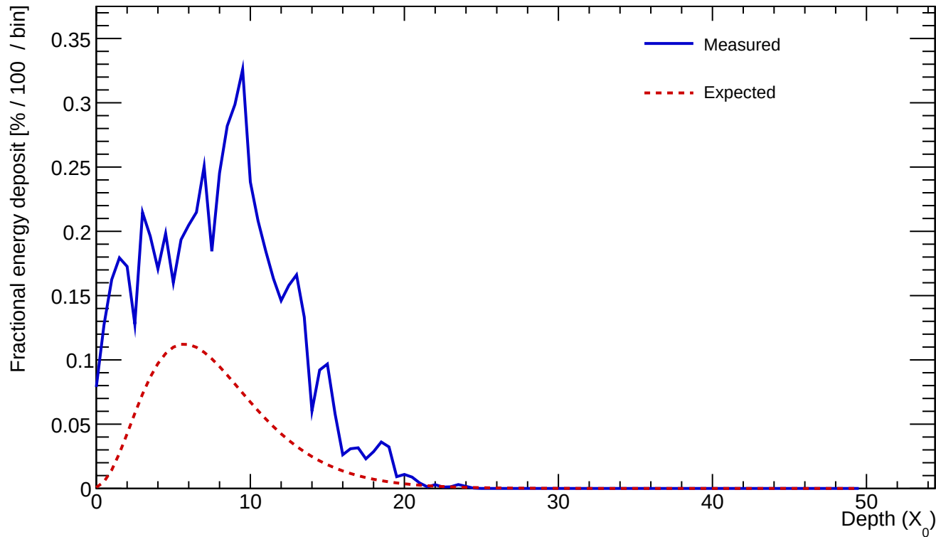
Cluster 454 E=24.188 GeV profileStart=0.50 X_0 \chi=0.3477
