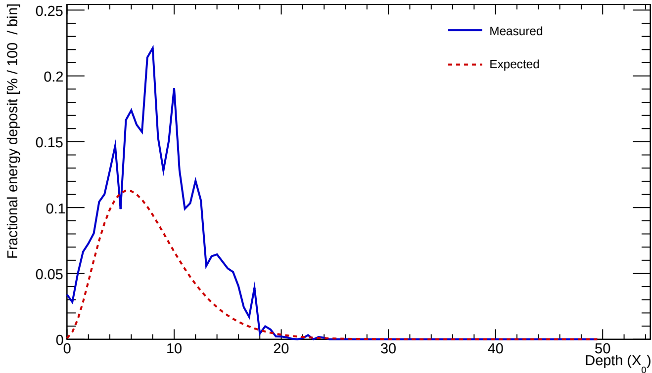
Cluster 468 E=22.828 GeV profileStart=1.00 X_0 \chi=0.2473
