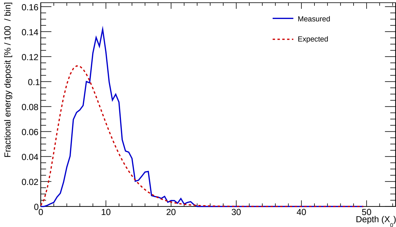
Cluster 573 E=23.451 GeV profileStart=2.50 X_0 \chi=0.1914
