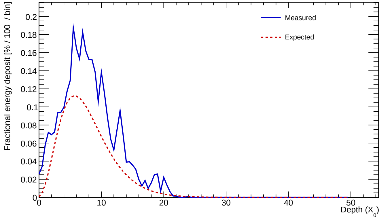
Cluster 372 E=24.410 GeV profileStart=0.50 X_0 \chi=0.2062
