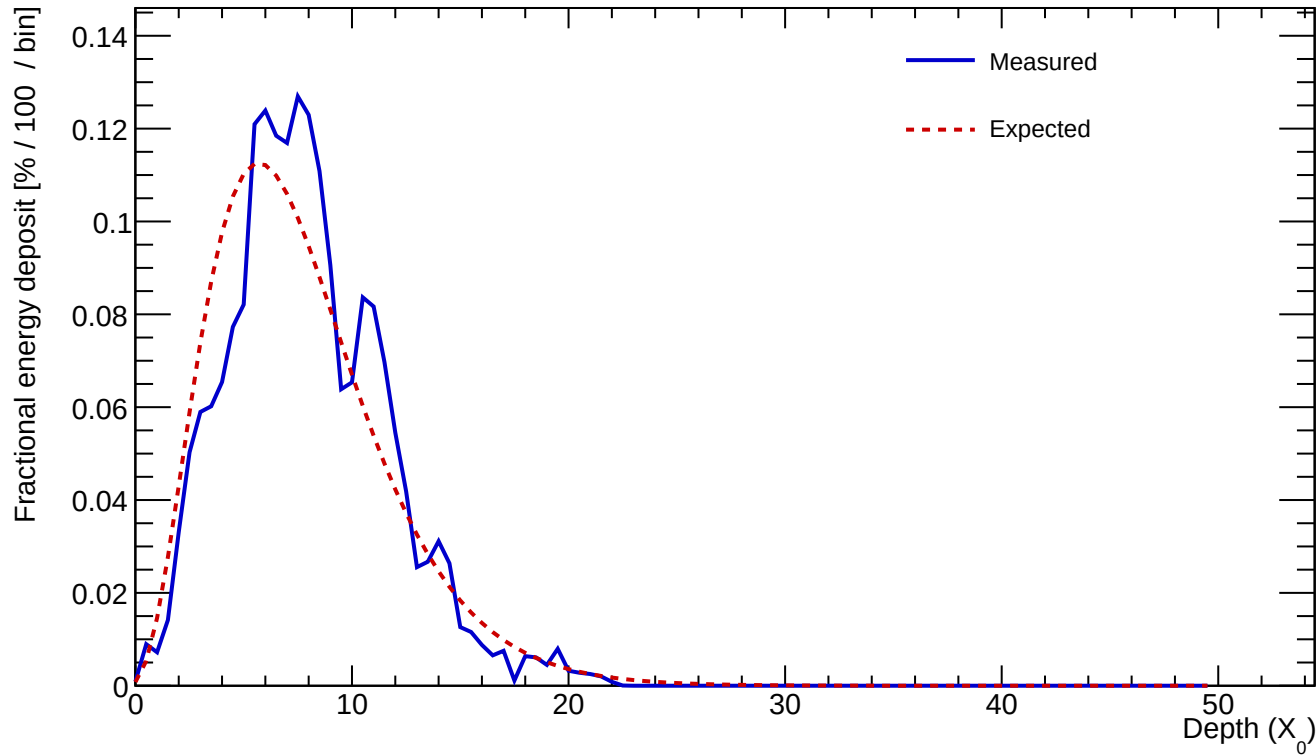
Cluster 67 E=23.720 GeV profileStart=0.50 X_0 \chi=0.1770
