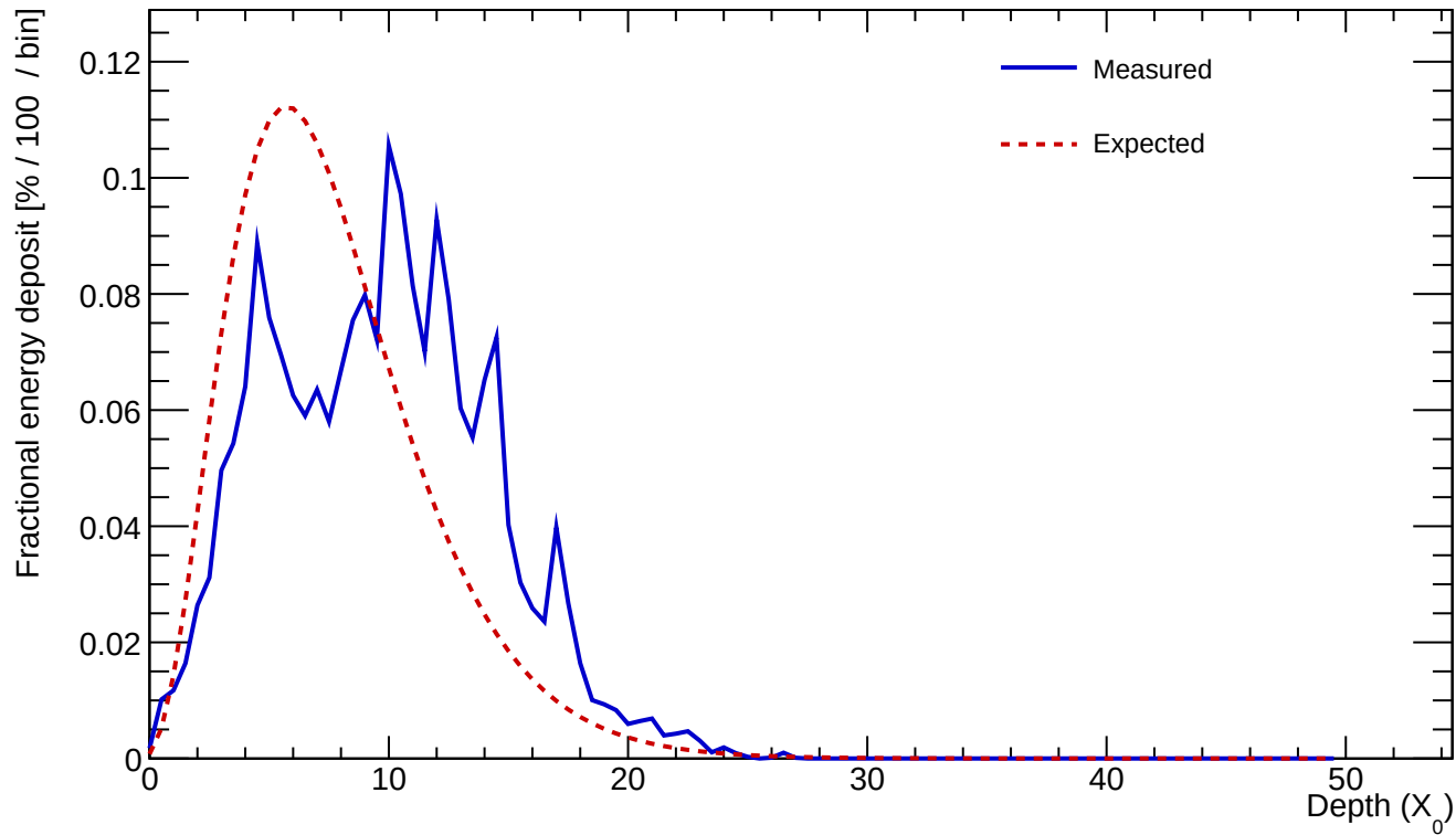
Cluster 7 E=24.263 GeV profileStart=2.00 X_0 \chi=0.3575
