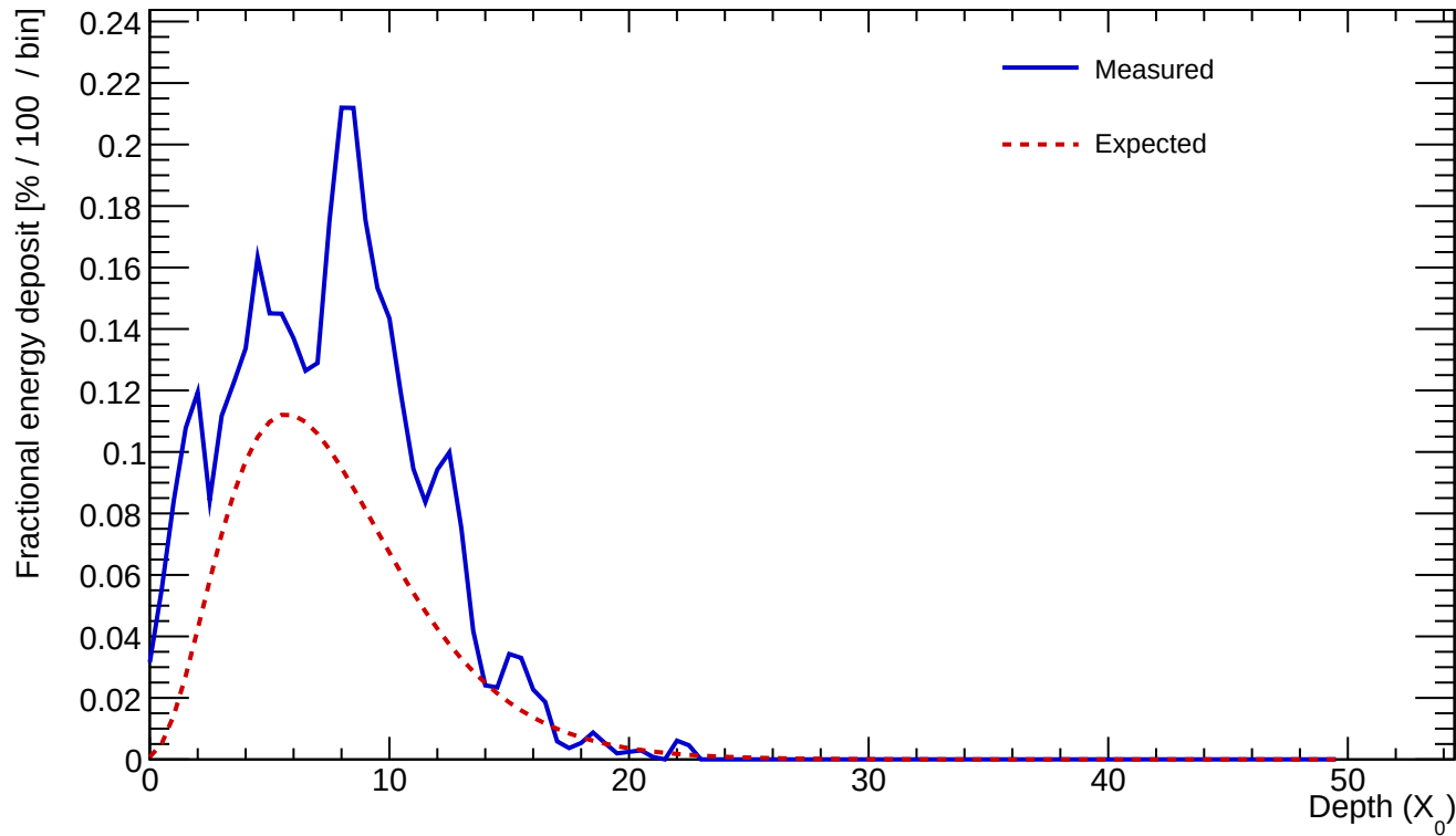
Cluster 146 E=24.325 GeV \text{profileStart}=0.50 X_0 \chi=0.2794
