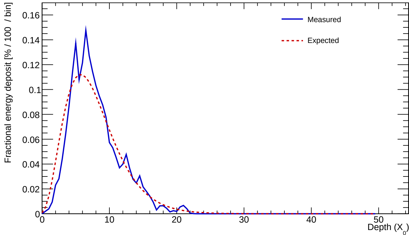
Cluster 297 E=24.682 GeV profileStart=0.50 X_0 \chi=0.1573
