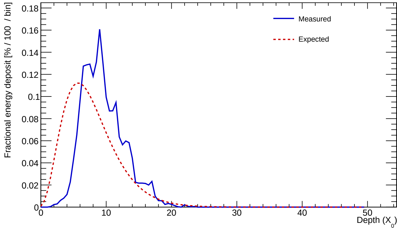
Cluster 85 E=24.265 GeV profileStart=2.50 X_0 \chi=0.2230
