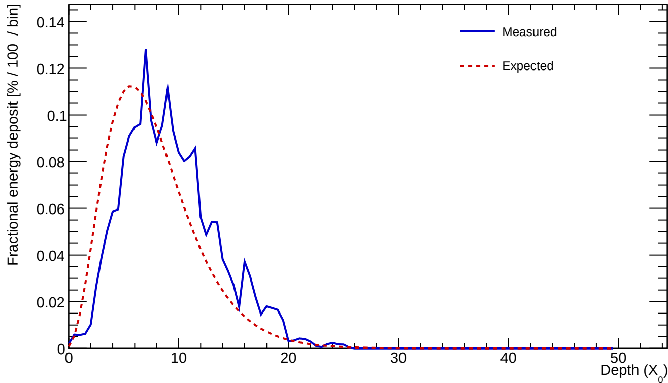
Cluster 576 E=24.014 GeV profileStart=1.50 X_0 \chi=0.1615
