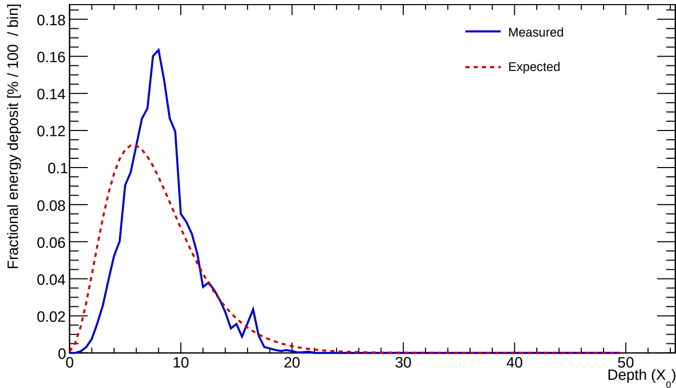
Cluster 574 E=24.545 GeV profileStart=1.50 X_0 \chi=0.2648
