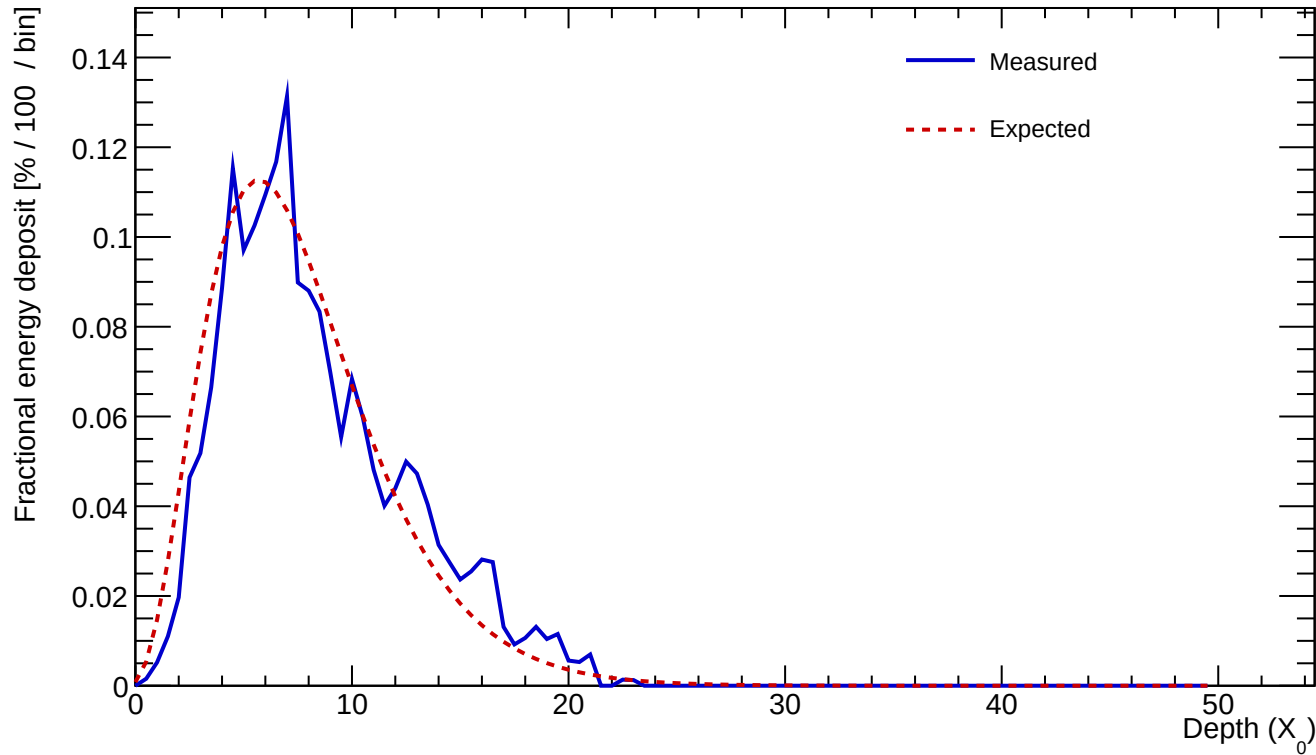
Cluster 624 E=23.517 GeV profileStart=0.50 X_0 \chi=0.1556
