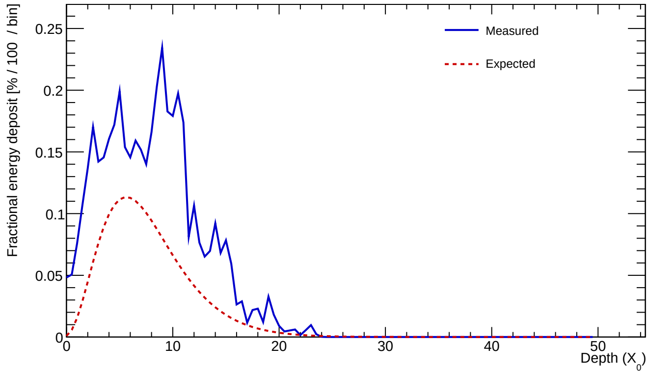
Cluster 502 E=22.110 GeV profileStart=0.50 X_0 \chi=0.3244
