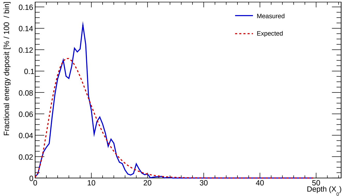
Cluster 75 E=24.954 GeV profileStart=0.50 X_0 \chi=0.1806
