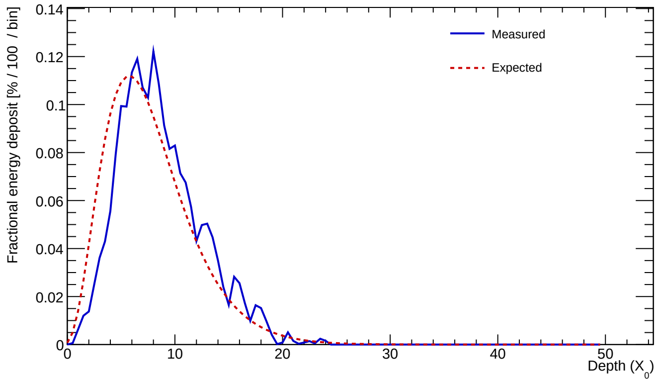
Cluster 40 E=25.142 GeV profileStart=1.00 X_0 \chi=0.1120
