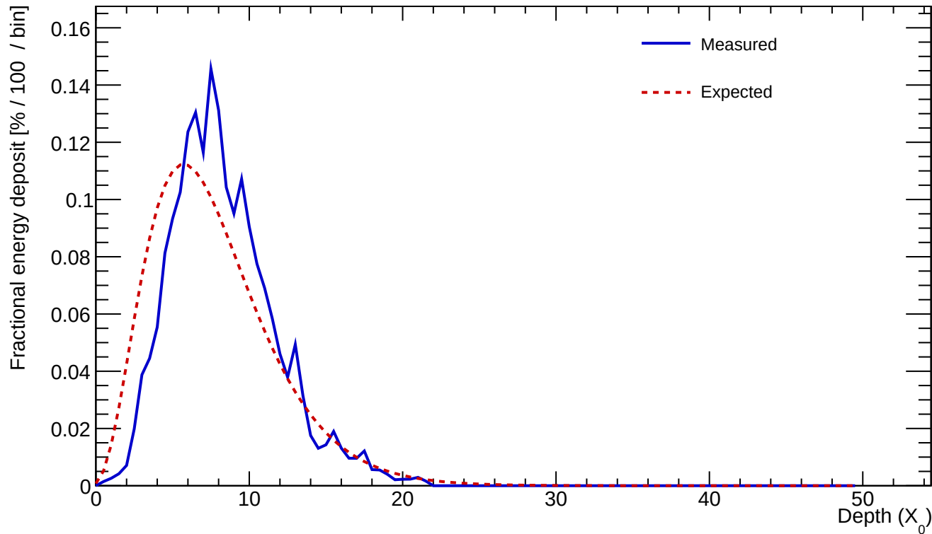
Cluster 376 E=24.260 GeV profileStart=1.00 X_0 \chi=0.1587
