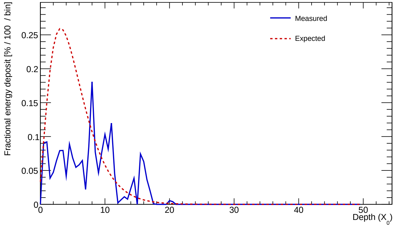
Cluster 320 E=1.857 GeV profileStart=1.50 X_0 \chi=0.7136
