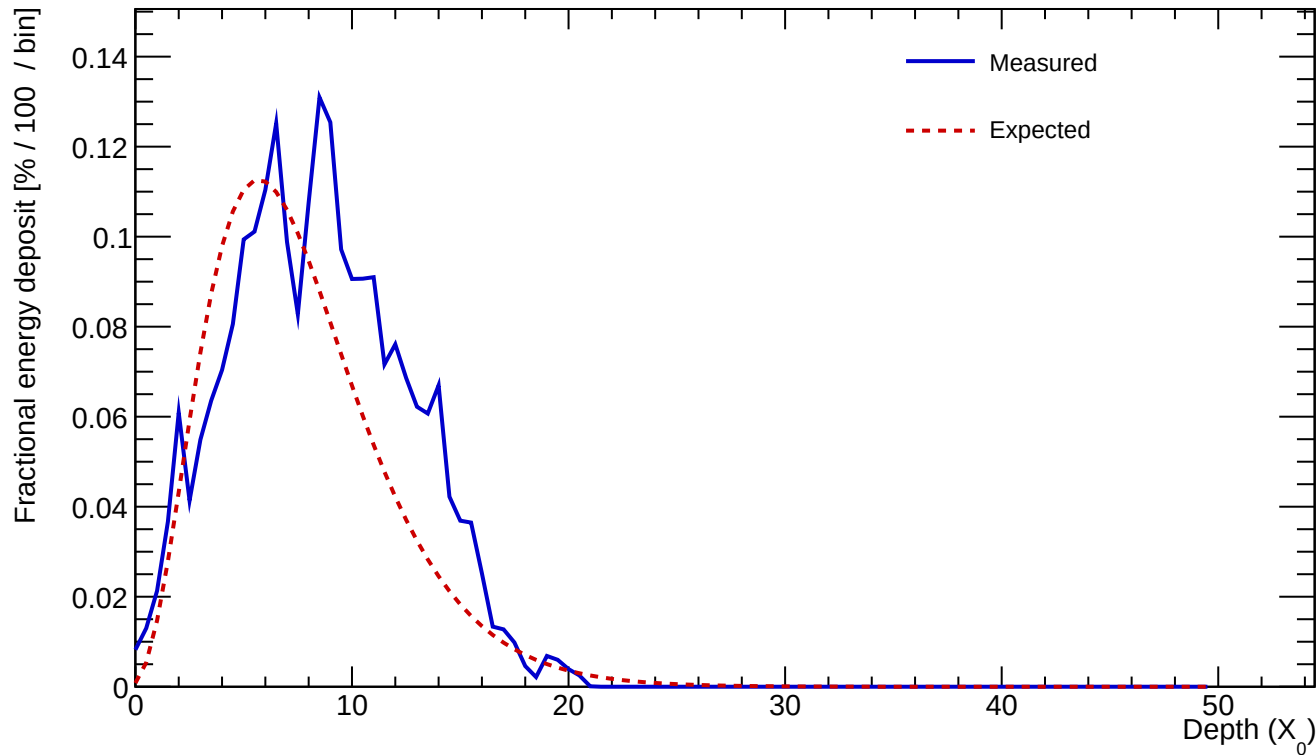
Cluster 128 E=23.490 GeV profileStart=1.50 X_0 \chi=0.2134
