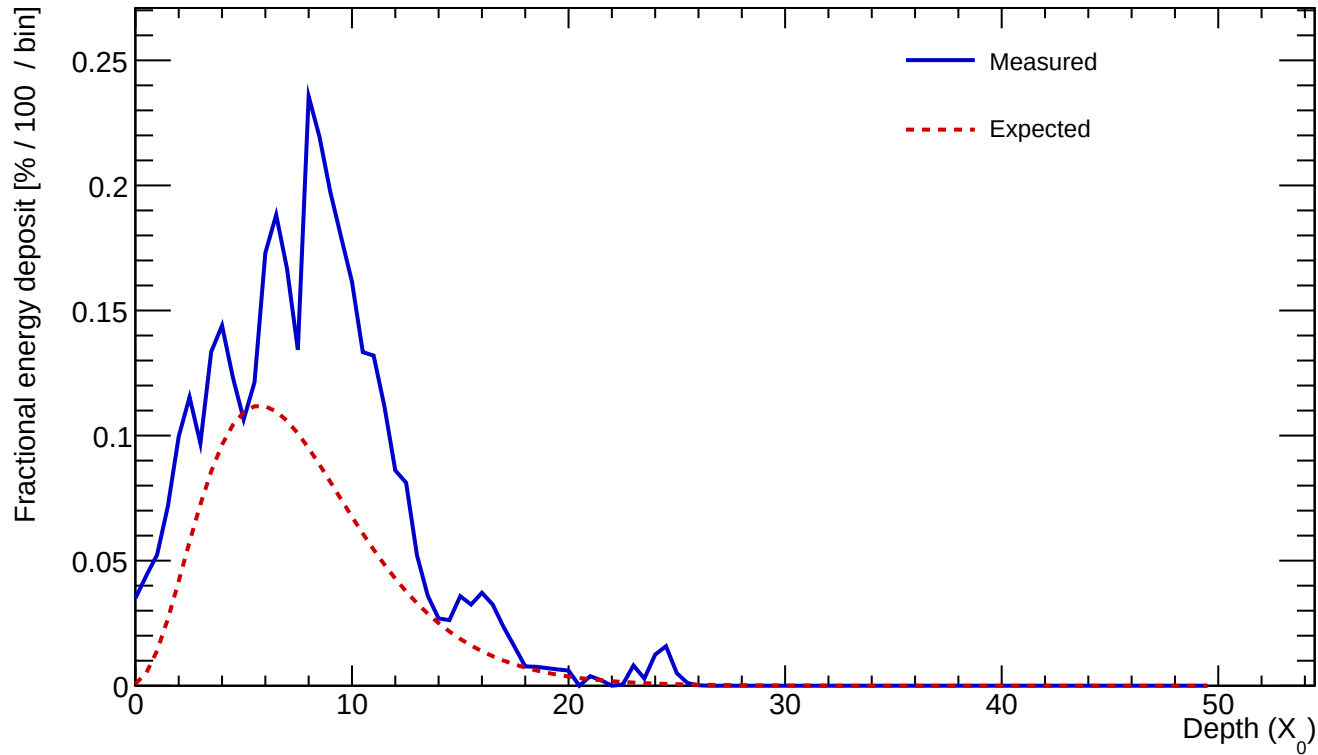
Cluster 60 E=24.960 GeV profileStart=0.50 X_0 \chi=0.2829
