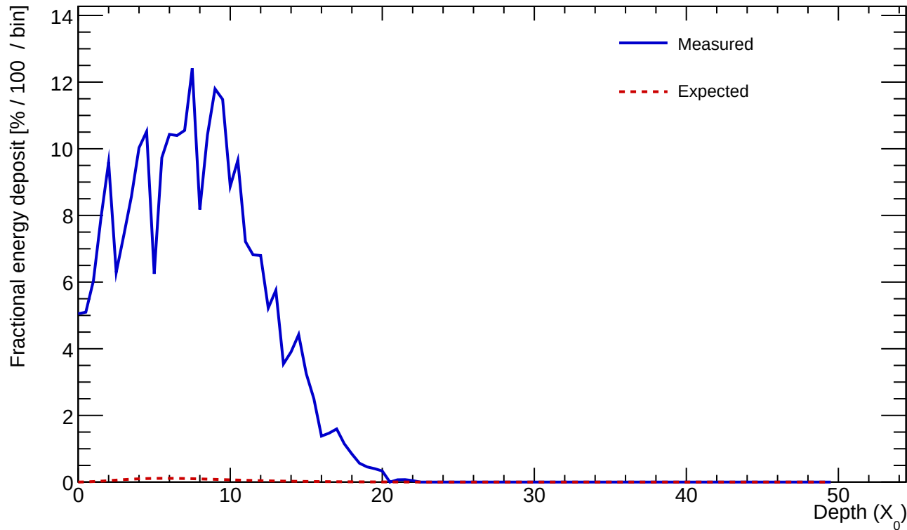
Cluster 446 E=23.921 GeV profileStart=0.50 X_0 \chi=0.2836
