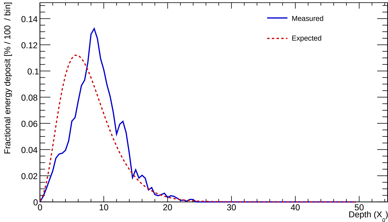
Cluster 302 E=24.444 GeV profileStart=2.00 X_0 \chi=0.2111
