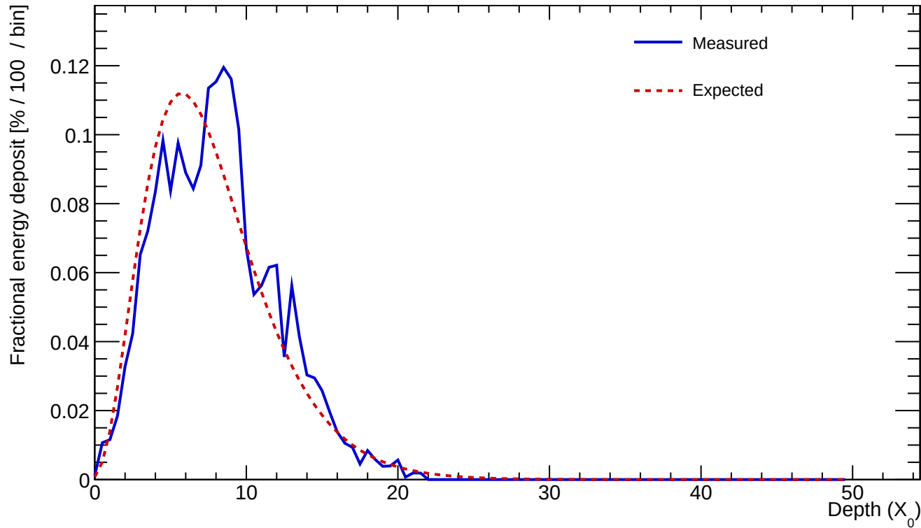
Cluster 24 E=24.810 GeV profileStart=0.50 X_0 \chi=0.1716
