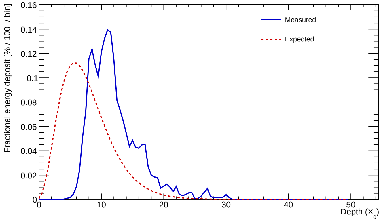
Cluster 567 E=24.119 GeV profileStart=4.50 X_0 \chi=0.2193
