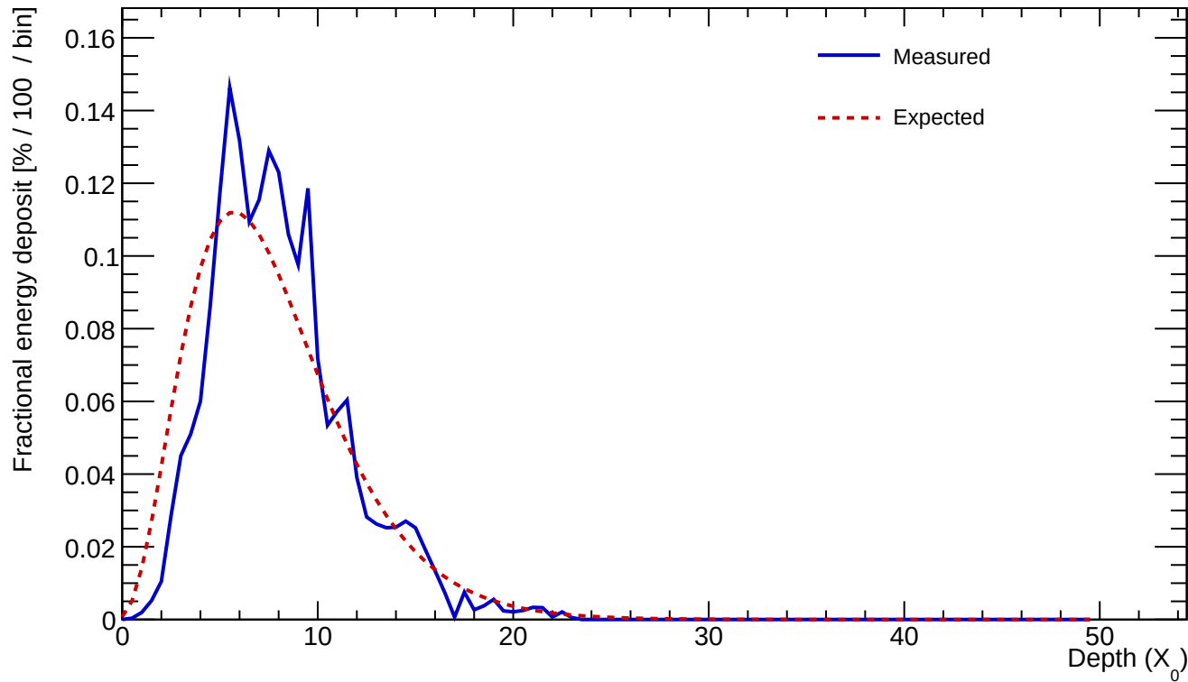
Cluster 432 E=24.624 GeV profileStart=1.00 X_0 \chi=0.1865
