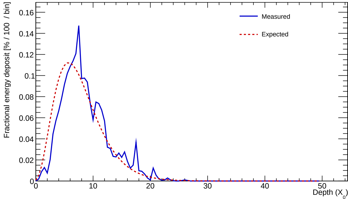
Cluster 627 E=24.513 GeV profileStart=1.00 X_0 \chi=0.1433
