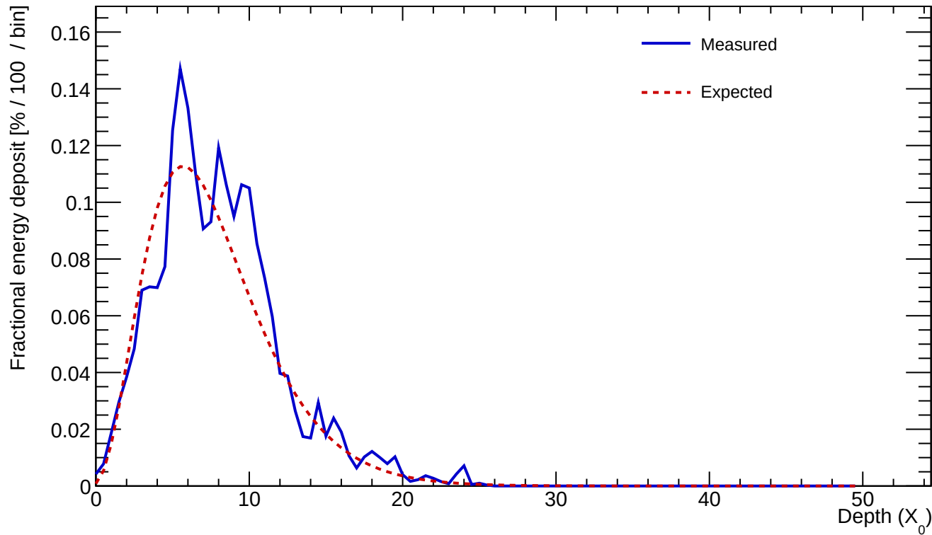
Cluster 449 E=23.401 GeV profileStart=0.50 X_0 \chi=0.1919
