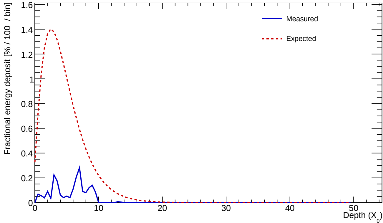
Cluster 279 E=1.001 GeV profileStart=1.50 X_0 \chi=0.6838
