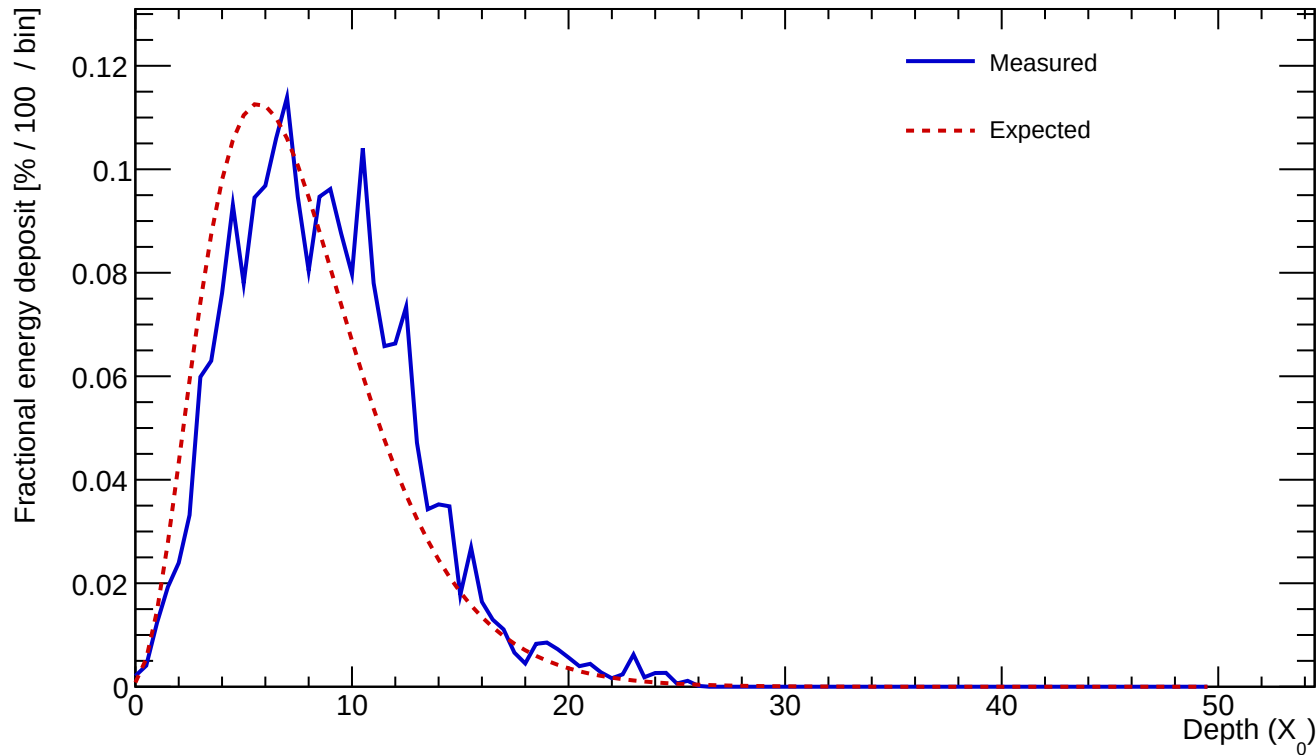
Cluster 351 E=23.445 GeV profileStart=1.00 X_0 \chi=0.1586
