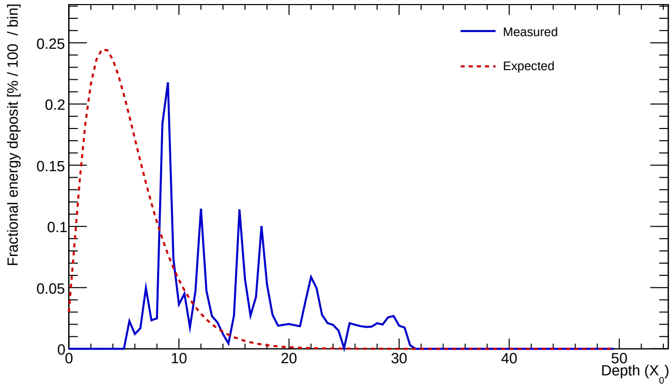
Cluster 353 E=1.963 GeV profileStart=7.00 X_0 \chi=3.0381
