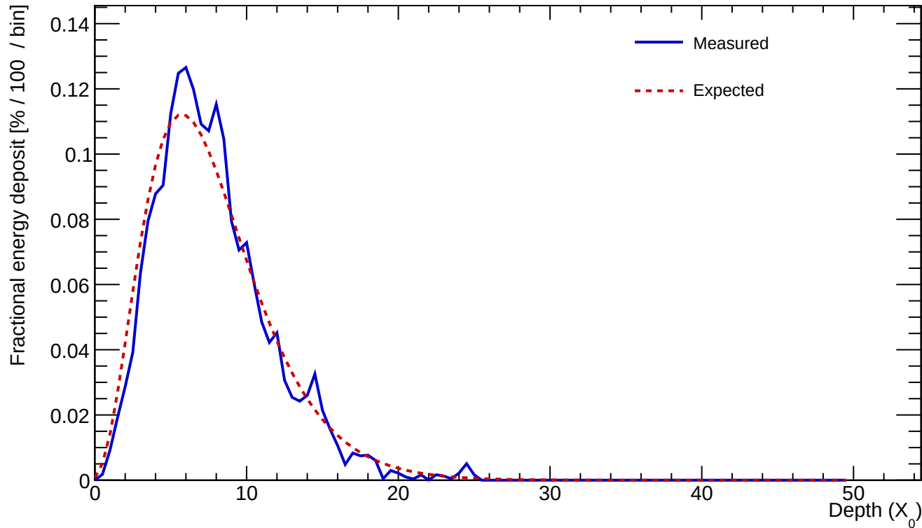
Cluster 282 E=24.622 GeV profileStart=0.50 X_0 \chi=0.1298
