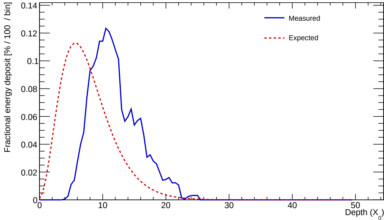
Cluster 584 E=23.060 GeV profileStart=4.50 X_0 \chi=0.1087
