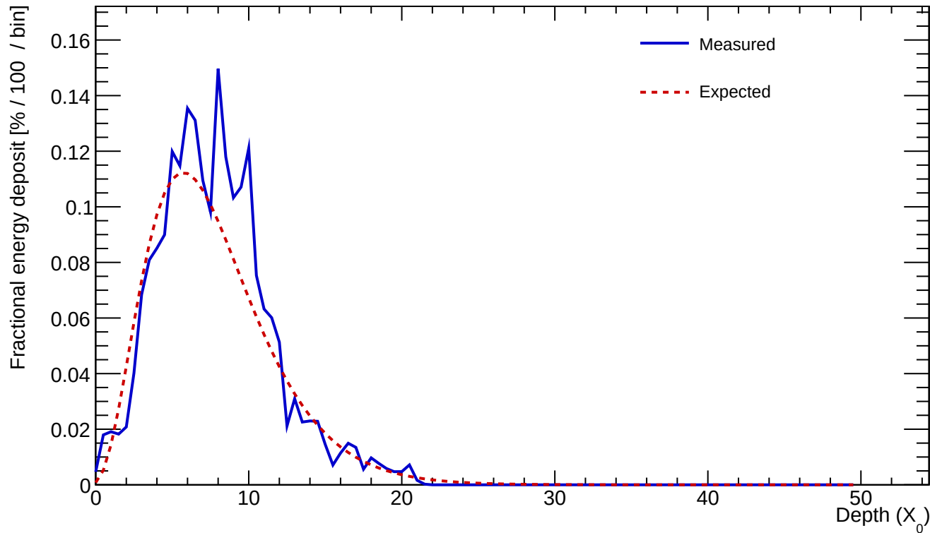
Cluster 144 E=24.165 GeV profileStart=0.50 X_0 \chi=0.1666
