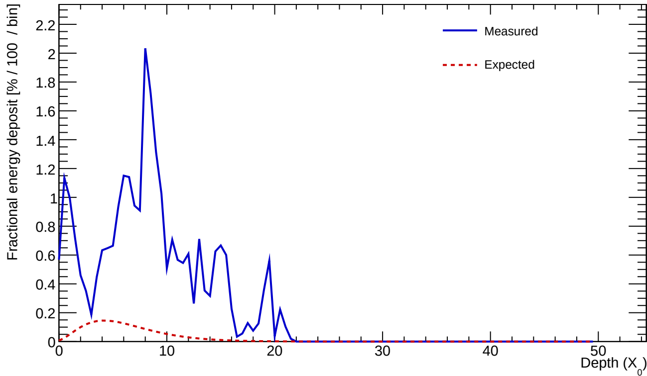
Cluster 379 E=5.227 GeV profileStart=3.00 X_0 \chi=0.5388
