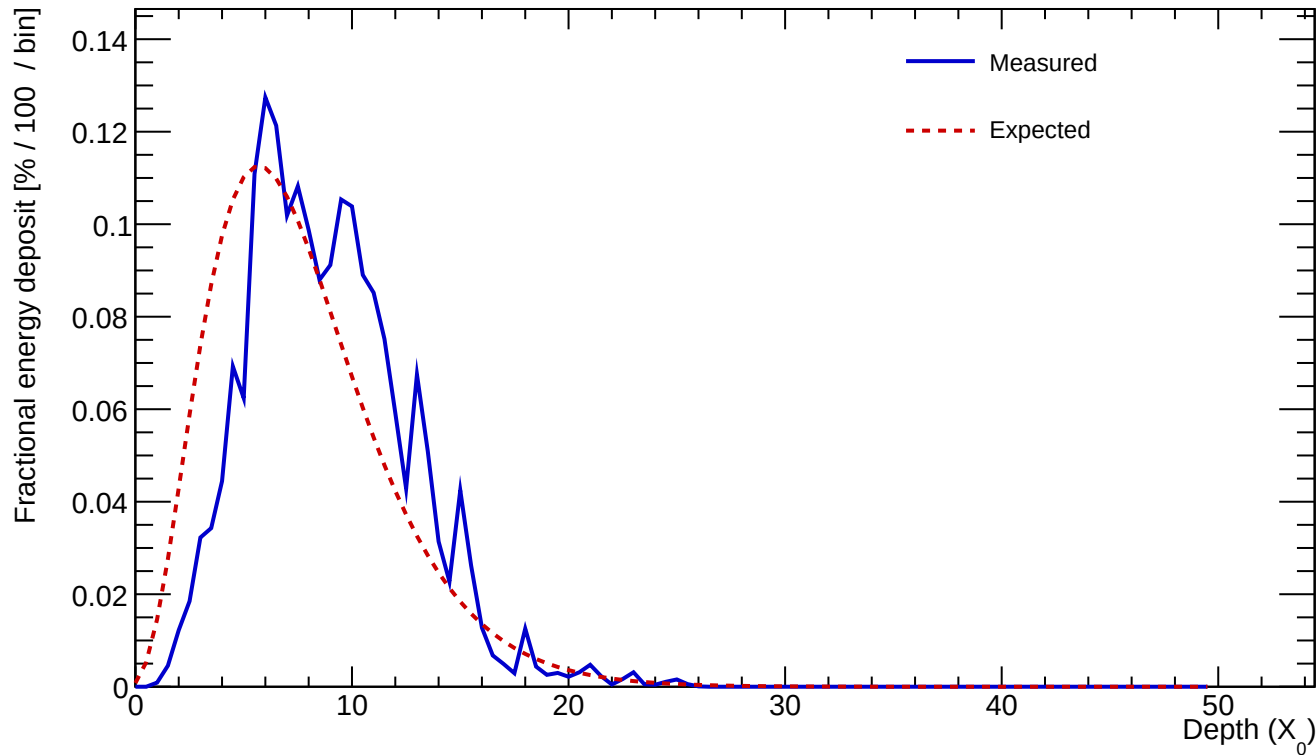
Cluster 201 E=23.802 GeV profileStart=1.50 X_0 \chi=0.1837
