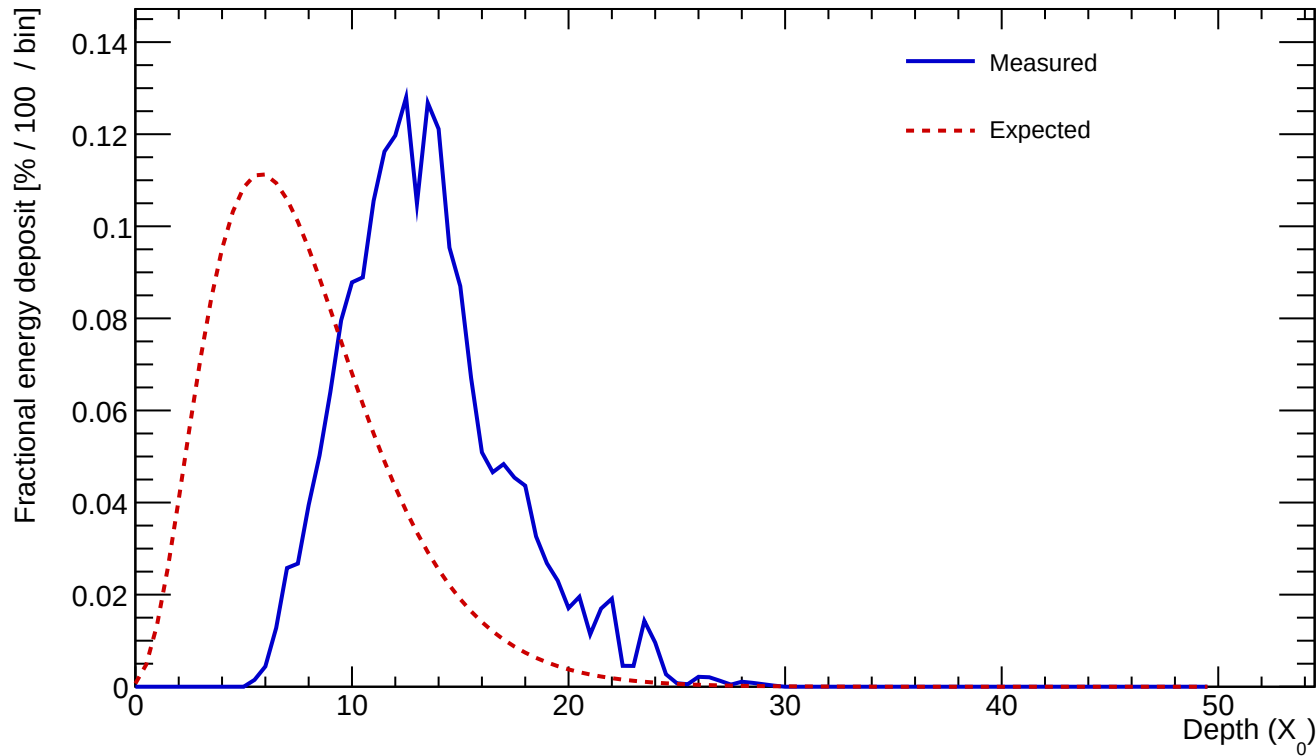
Cluster 250 E=26.218 GeV profileStart=6.00 X_0 \chi=0.1499
