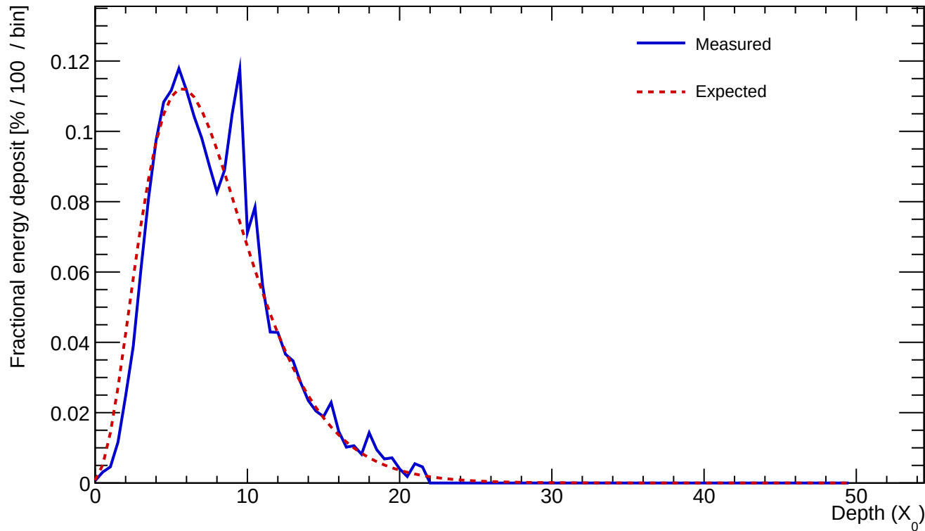
Cluster 360 E=24.324 GeV profileStart=0.50 X_0 \chi=0.1270
