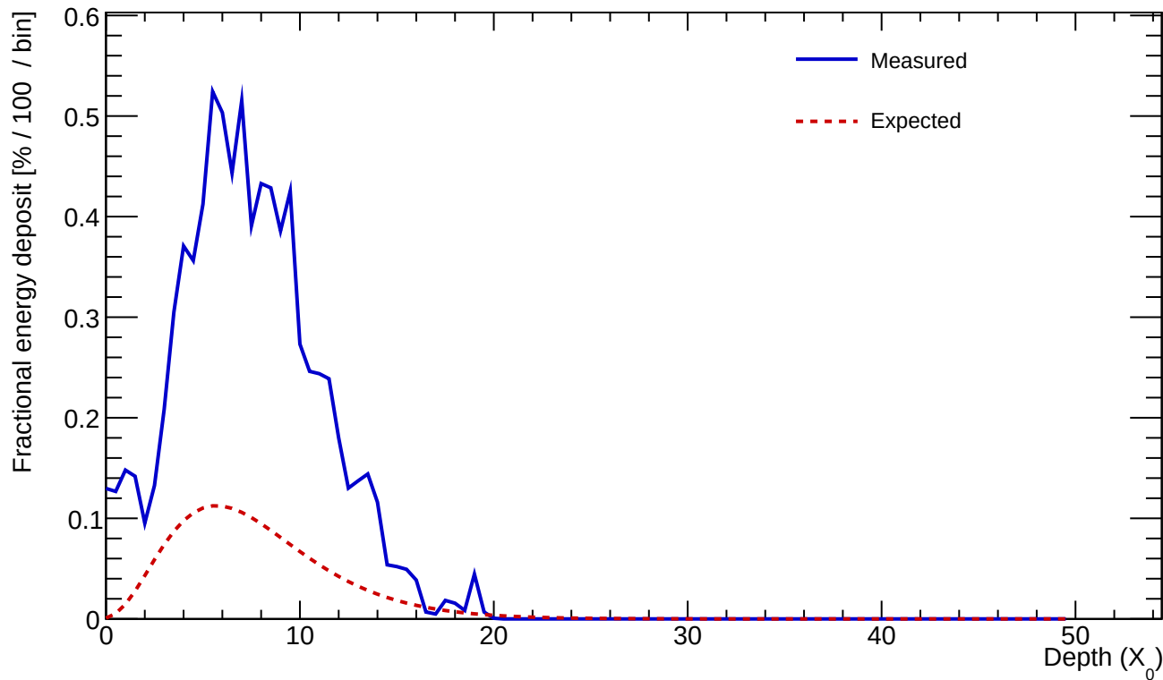
Cluster 486 E=23.685 GeV profileStart=0.50 X_0 \chi=0.1825
