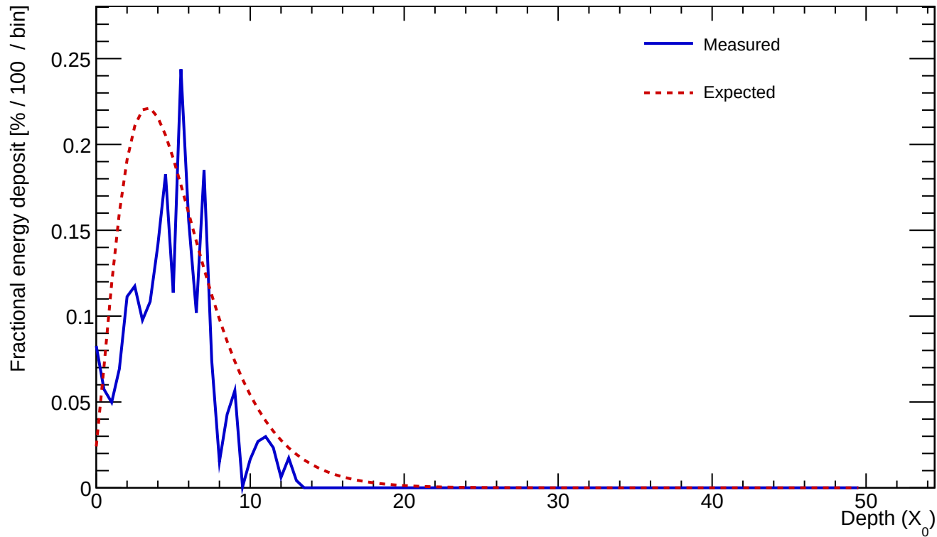
Cluster 199 E=2.201 GeV profileStart=0.50 X_0 \chi=0.3491
