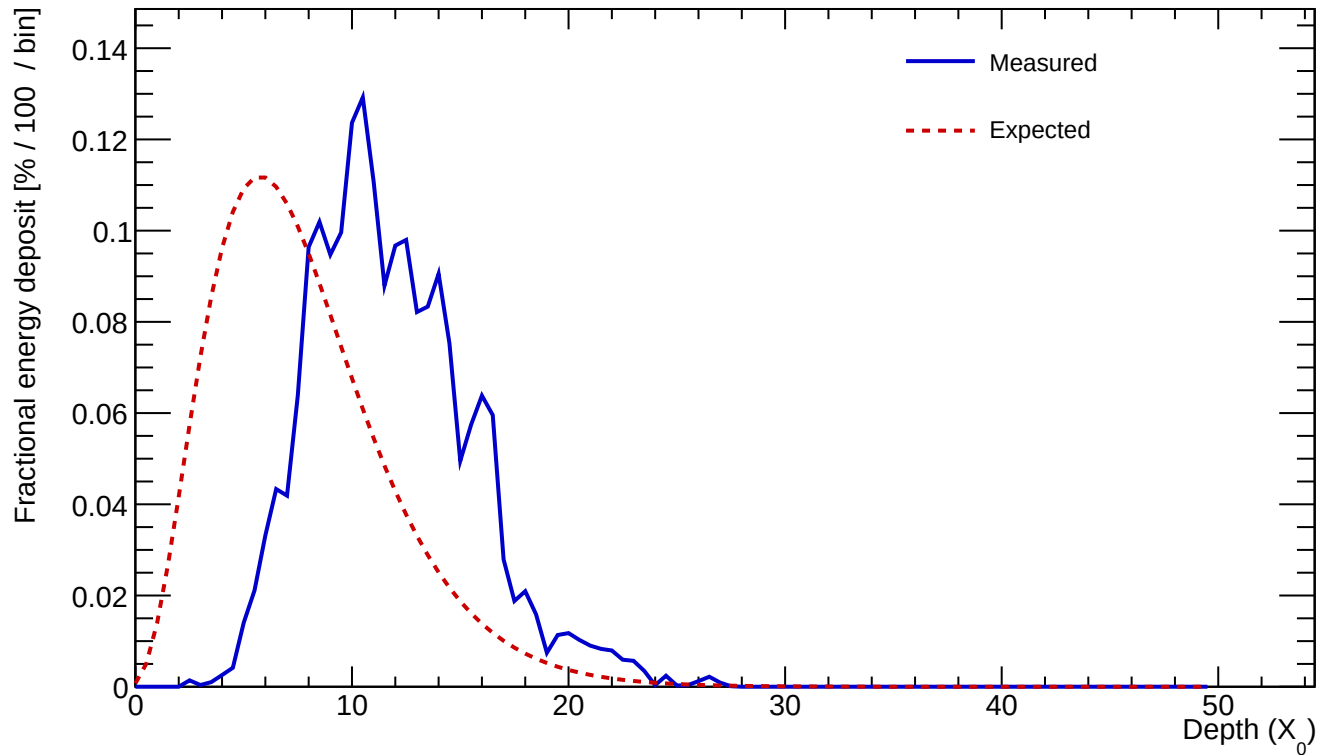
Cluster 122 E=25.118 GeV profileStart=4.50 X_0 \chi=0.1603
