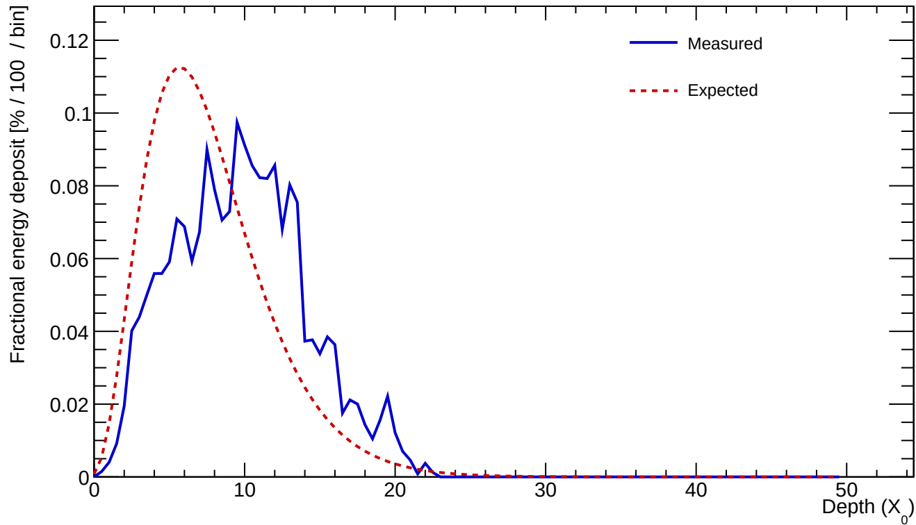
Cluster 102 E=23.594 GeV profileStart=2.50 X_0 \chi=0.2820
