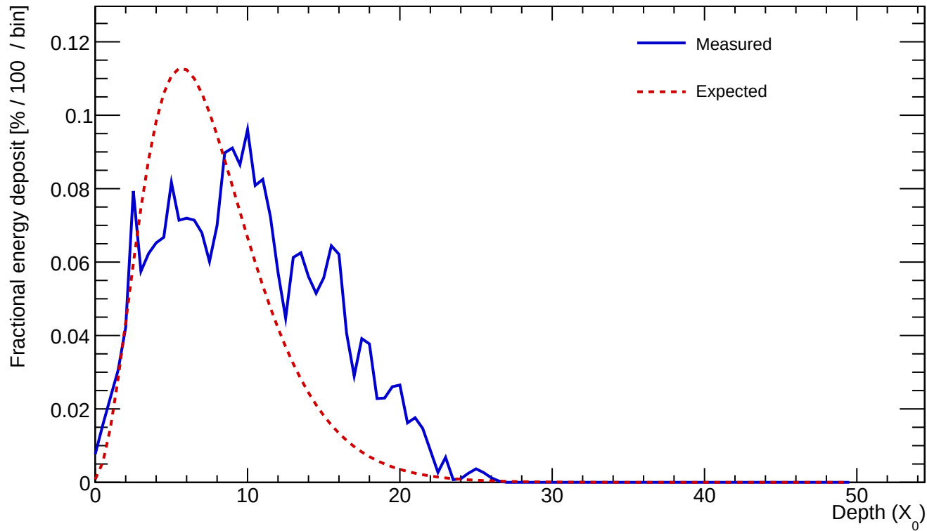
Cluster 304 E=23.103 GeV \text{profileStart}=1.50 X_0 \chi=0.4527
