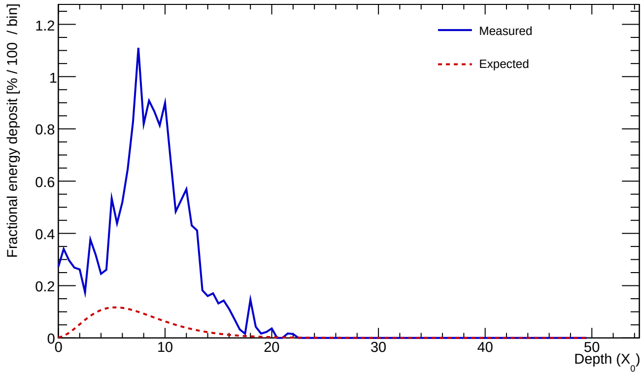
Cluster 15 E=16.750 GeV profileStart=2.50 X_0 \chi=0.3272
