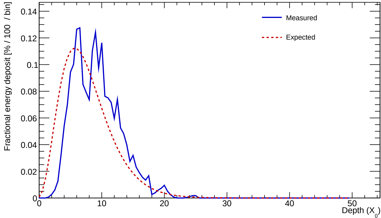
Cluster 52 E=24.266 GeV profileStart=1.50 X_0 \chi=0.1782
