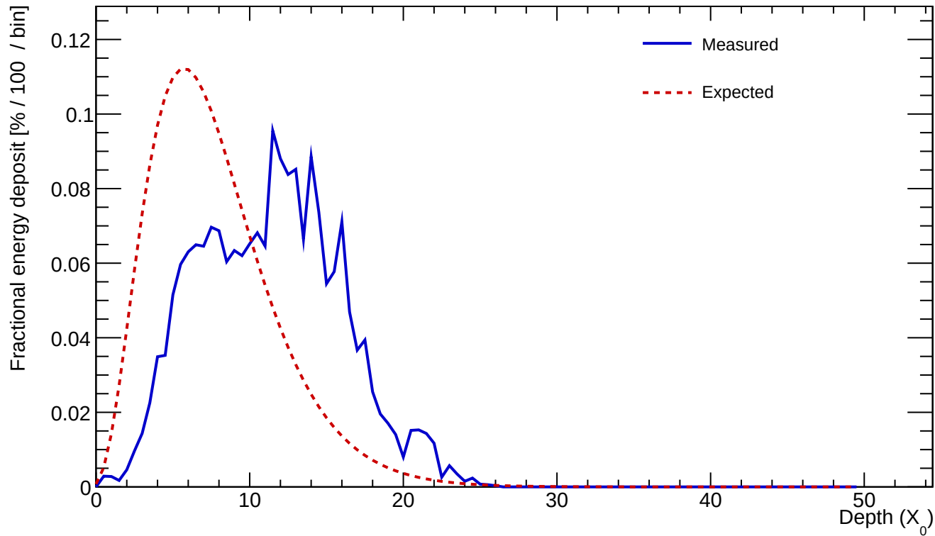
Cluster 56 E=24.331 GeV profileStart=4.00 X_0 \chi=0.3490
