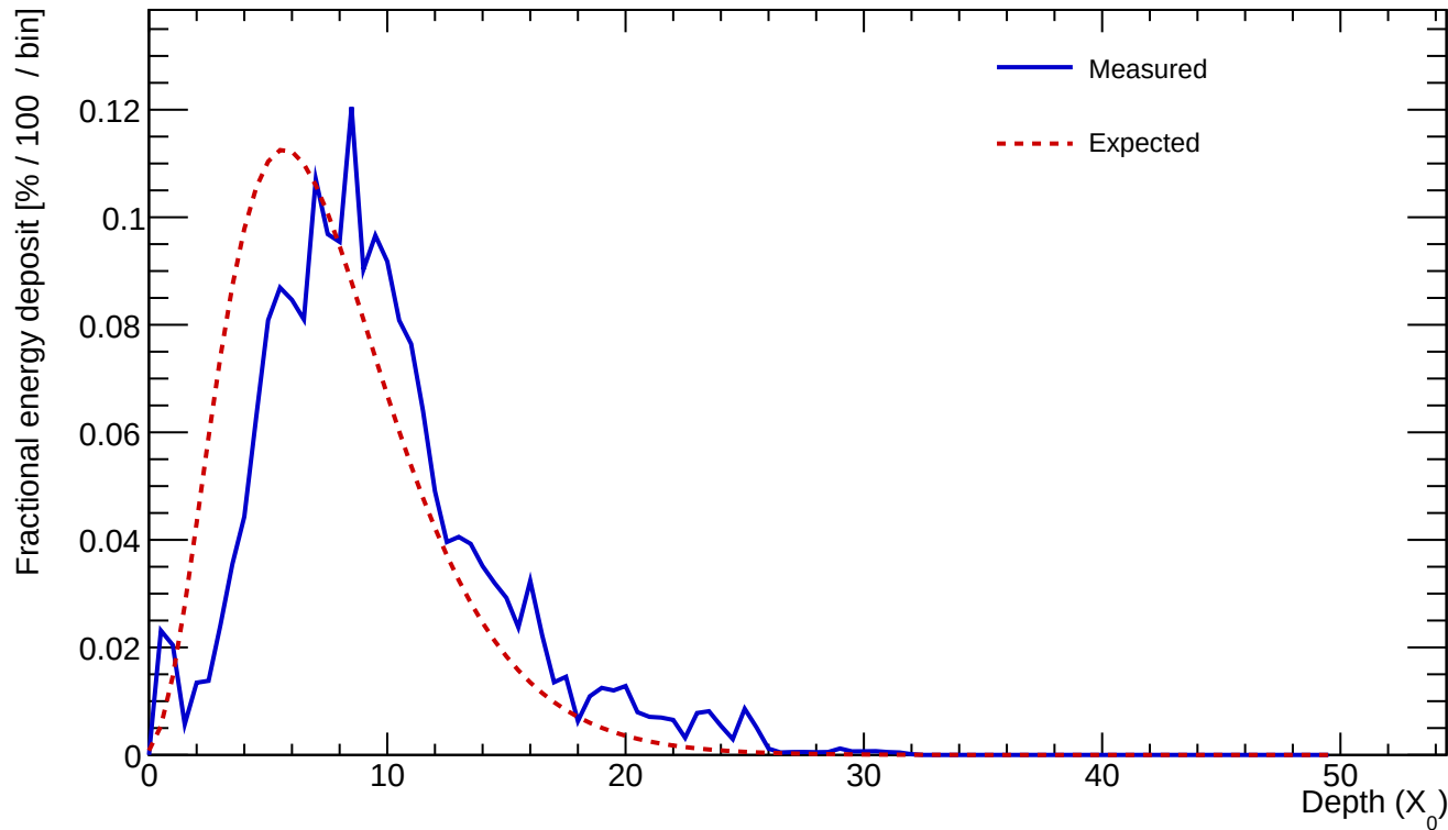
Cluster 500 E=23.566 GeV \text{profileStart}=1.50 X_0 \chi=0.1757
