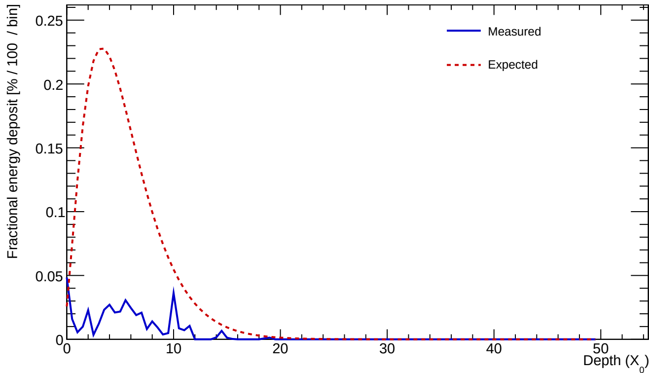
Cluster 27 E=2.123 GeV profileStart=0.50 X_0 \chi=0.5375
