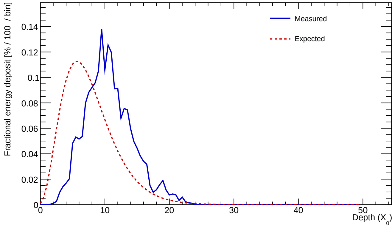
Cluster 174 E=23.408 GeV profileStart=3.50 X_0 \chi=0.1583
