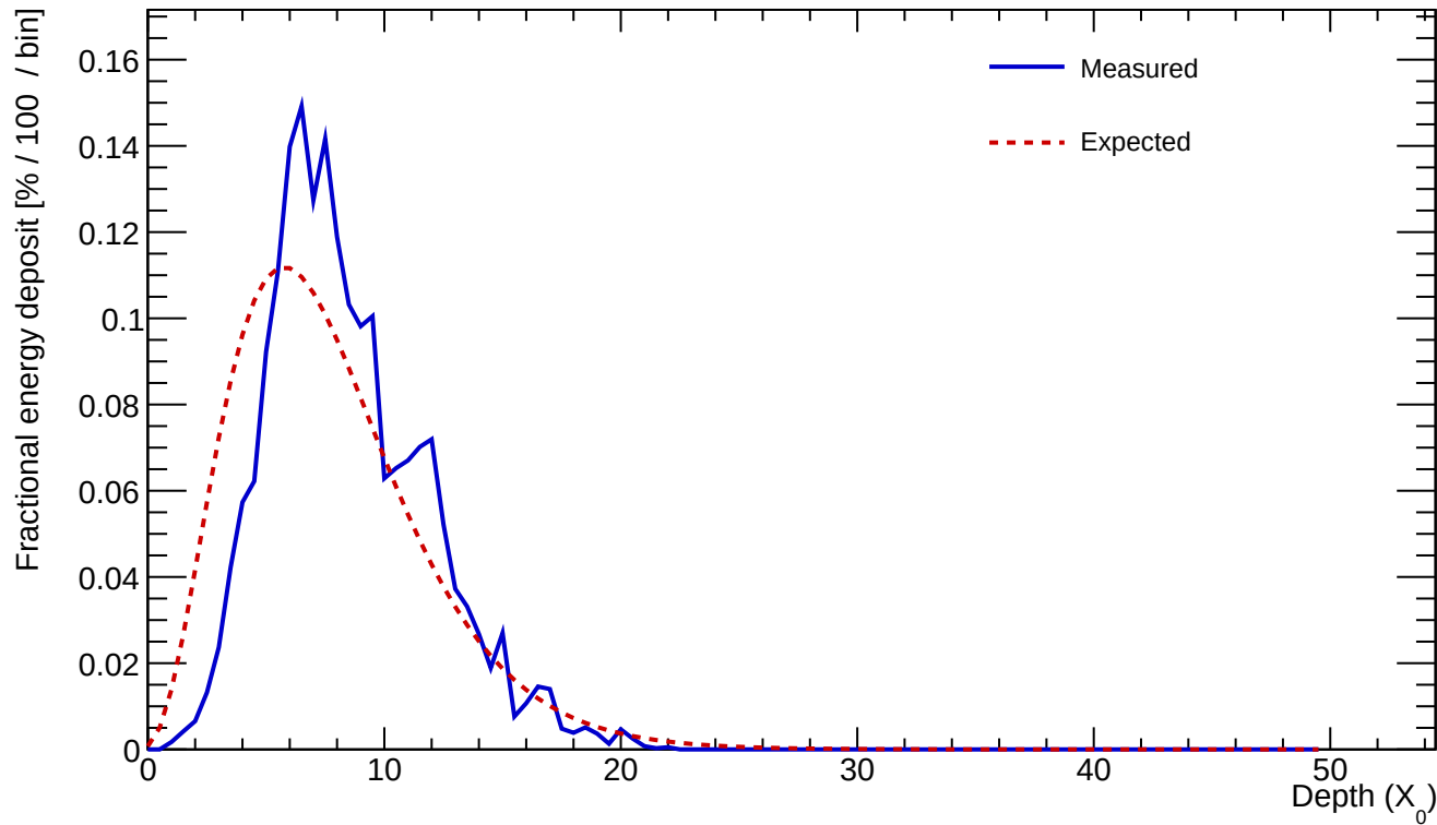
Cluster 65 E=25.119 GeV profileStart=1.50 X_0 \chi=0.1889
