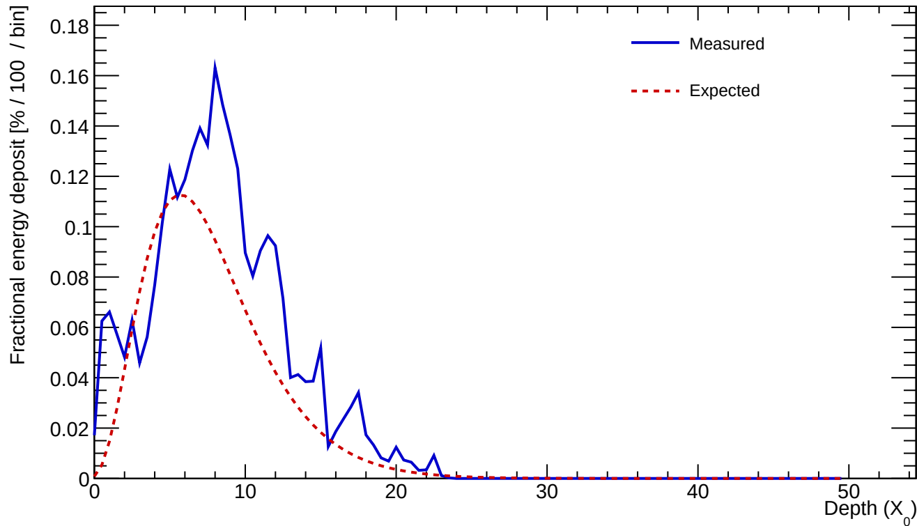
Cluster 369 E=23.460 GeV profileStart=1.50 X_0 \chi=0.2454
