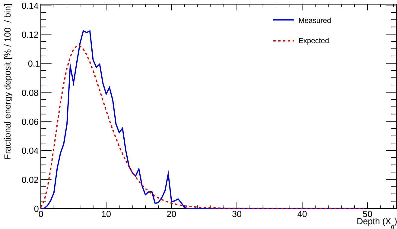
Cluster 363 E=24.738 GeV profileStart=1.00 X_0 \chi=0.1180
