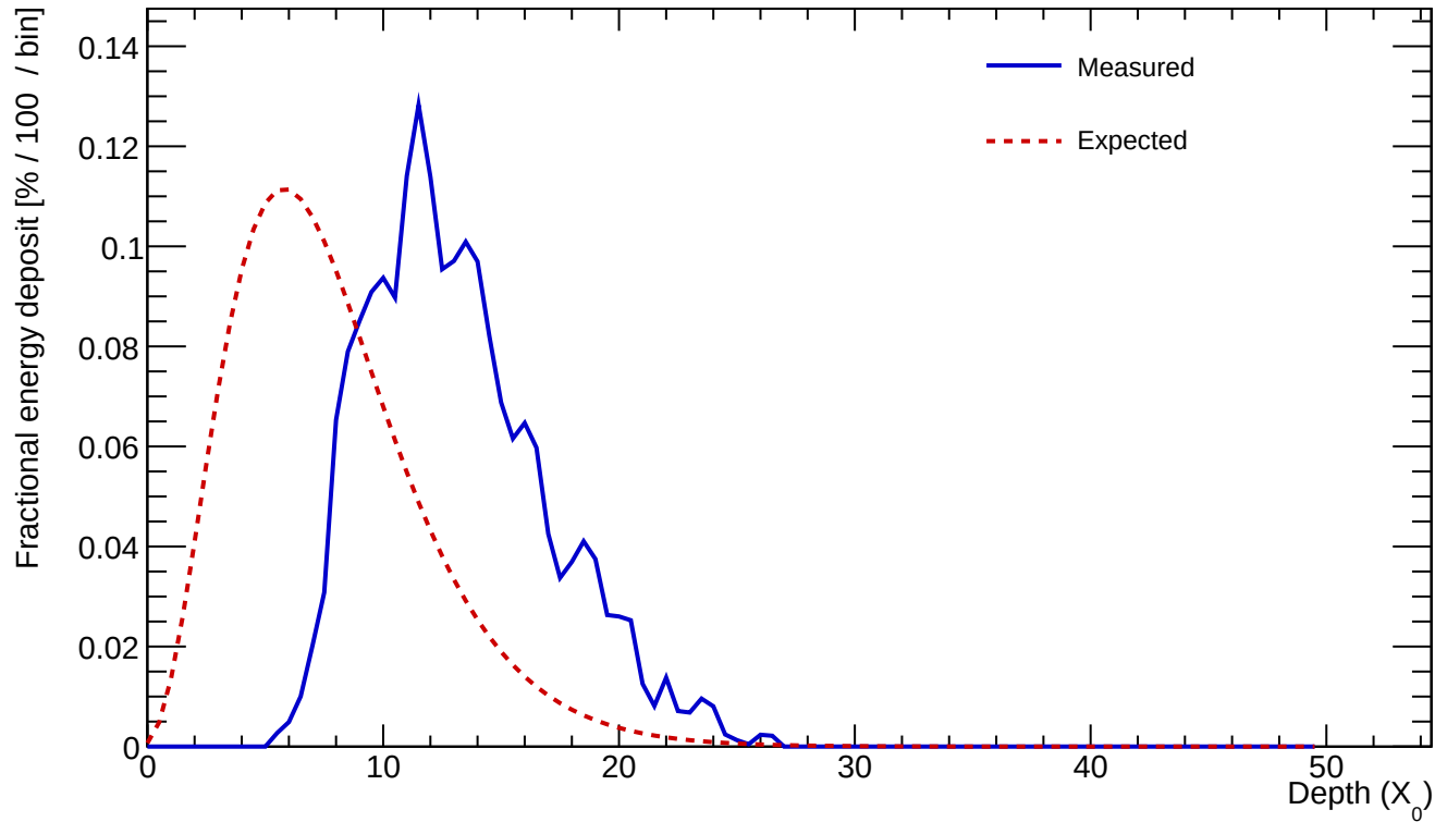
Cluster 99 E=25.932 GeV profileStart=5.50 X_0 \chi=0.1113
