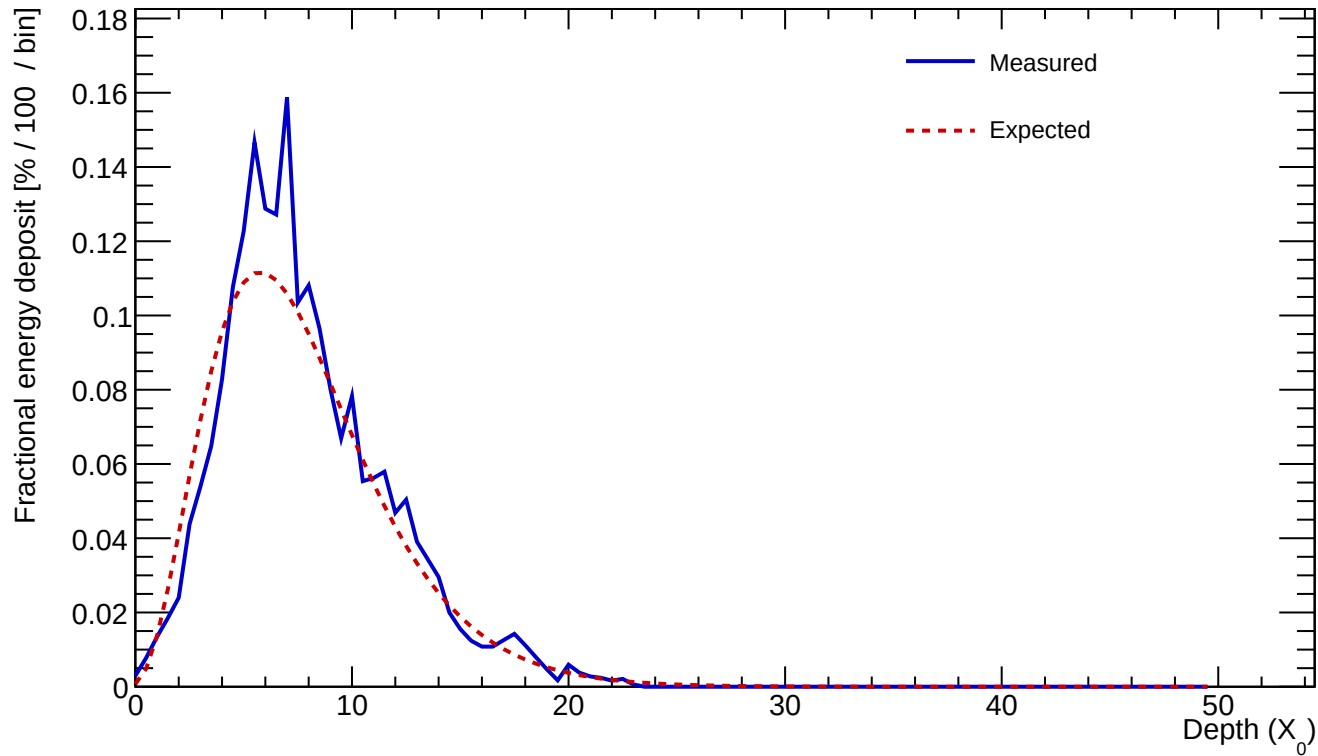
Cluster 518 E=25.586 GeV profileStart=0.50 X_0 \chi=0.1377
