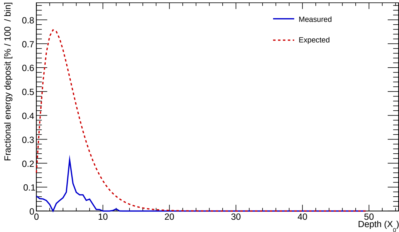
Cluster 420 E=1.108 GeV profileStart=2.00 X_0 \chi=0.6207
