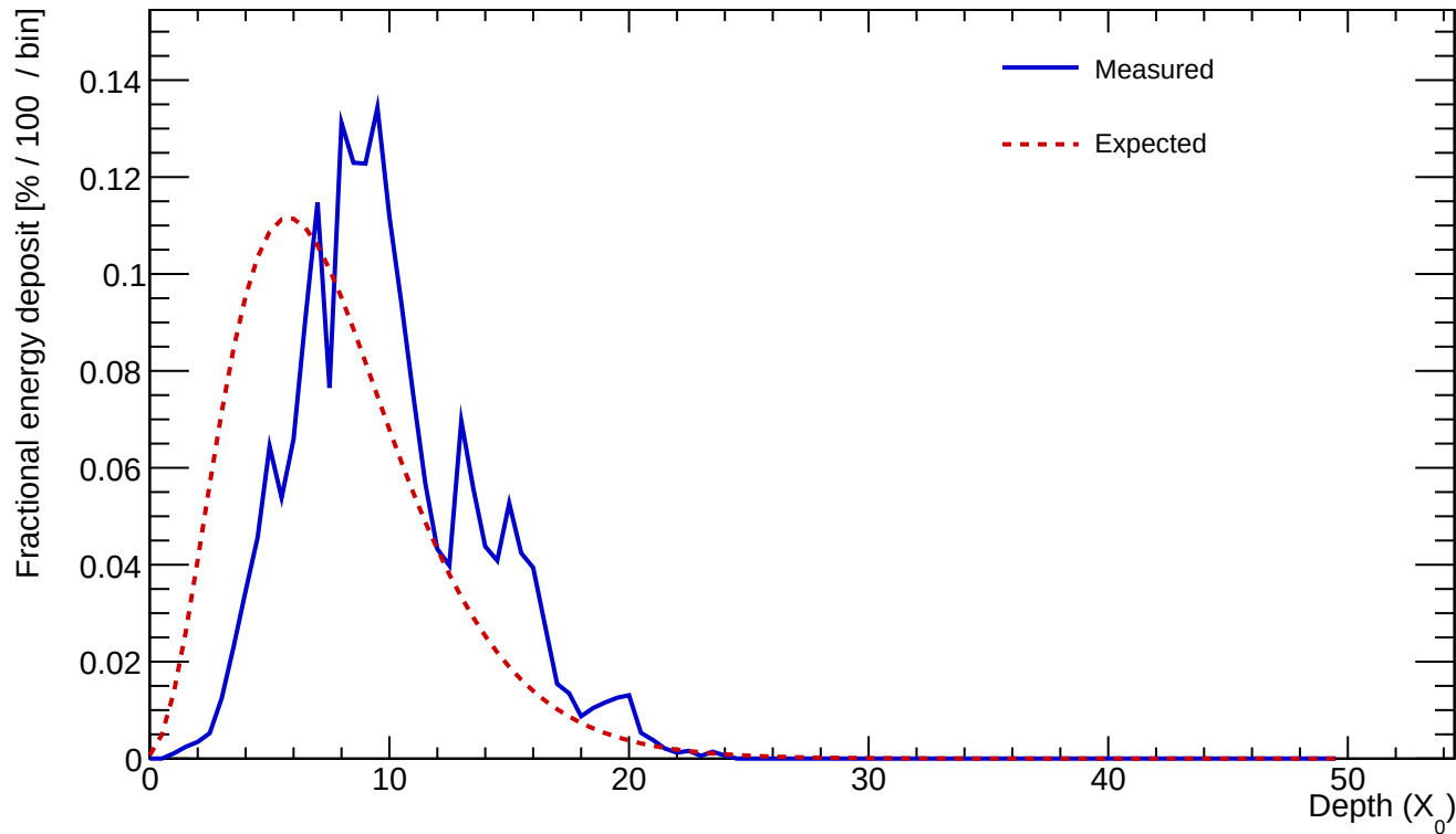
Cluster 457 E=25.830 GeV profileStart=2.50 X_0 \chi=0.2098
