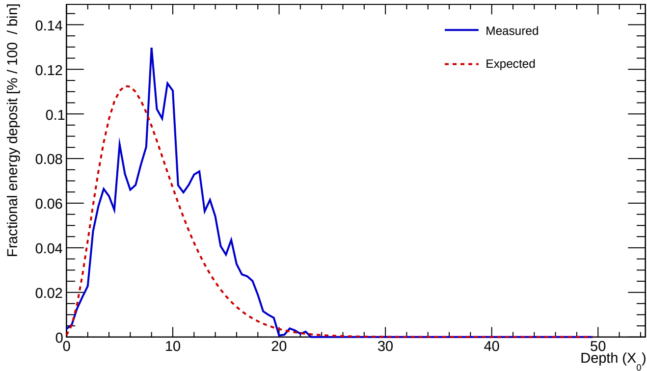
Cluster 333 E=23.581 GeV profileStart=2.00 X_0 \chi=0.2781
