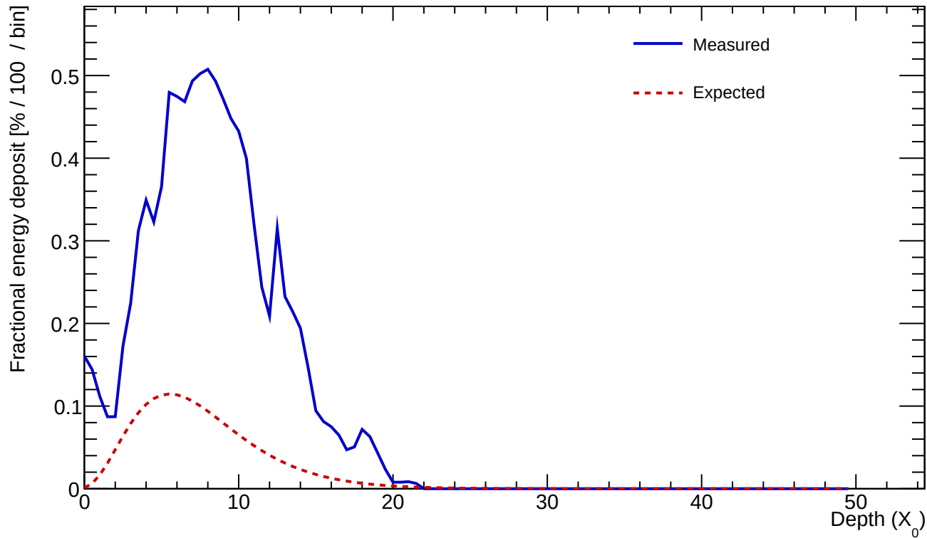
Cluster 569 E=20.053 GeV profileStart=1.00 X_0 \chi=0.1741
