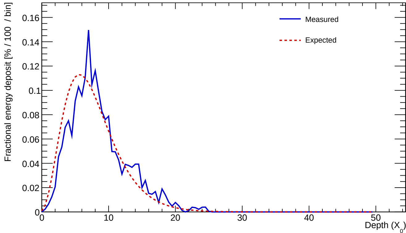
Cluster 537 E=22.780 GeV profileStart=0.50 X_0 \chi=0.1644
