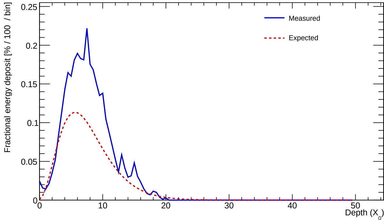
Cluster 398 E=22.053 GeV profileStart=0.50 X_0 \chi=0.1346
