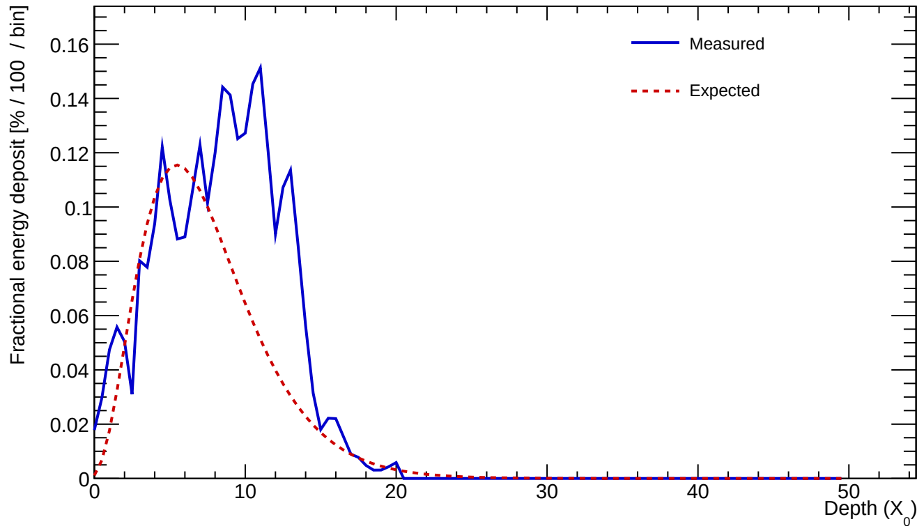
Cluster 216 E=18.783 GeV profileStart=1.50 X_0 \chi=0.3334
