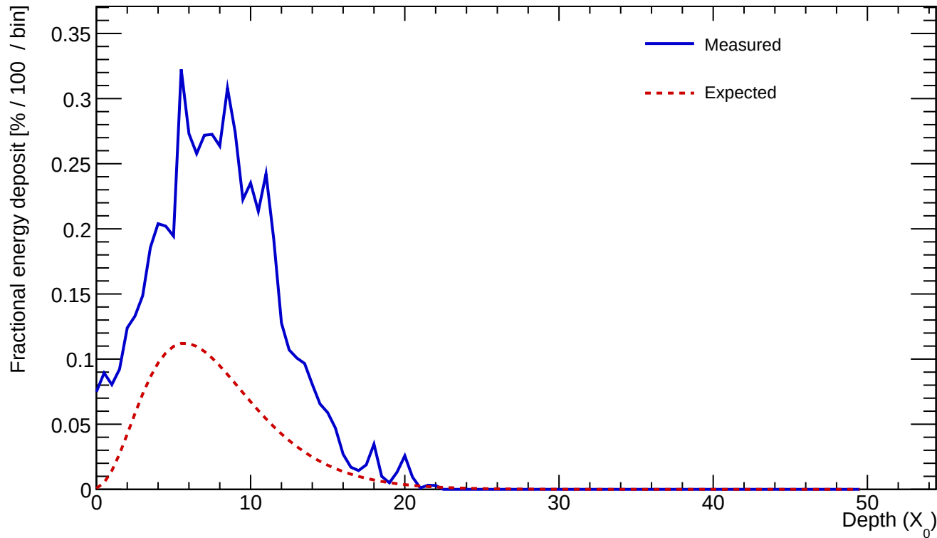
Cluster 465 E=24.352 GeV profileStart=0.50 X_0 \chi=0.2068
