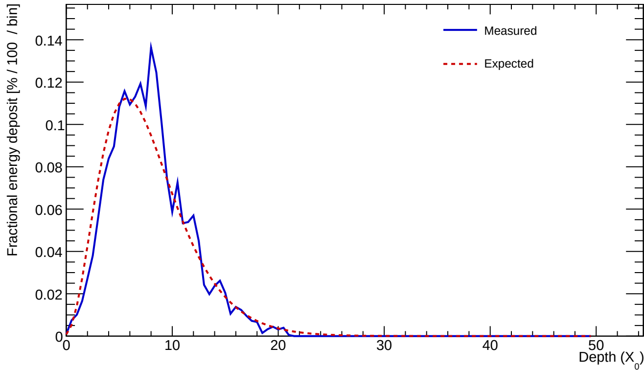
Cluster 459 E=24.208 GeV profileStart=0.50 X_0 \chi=0.1187
