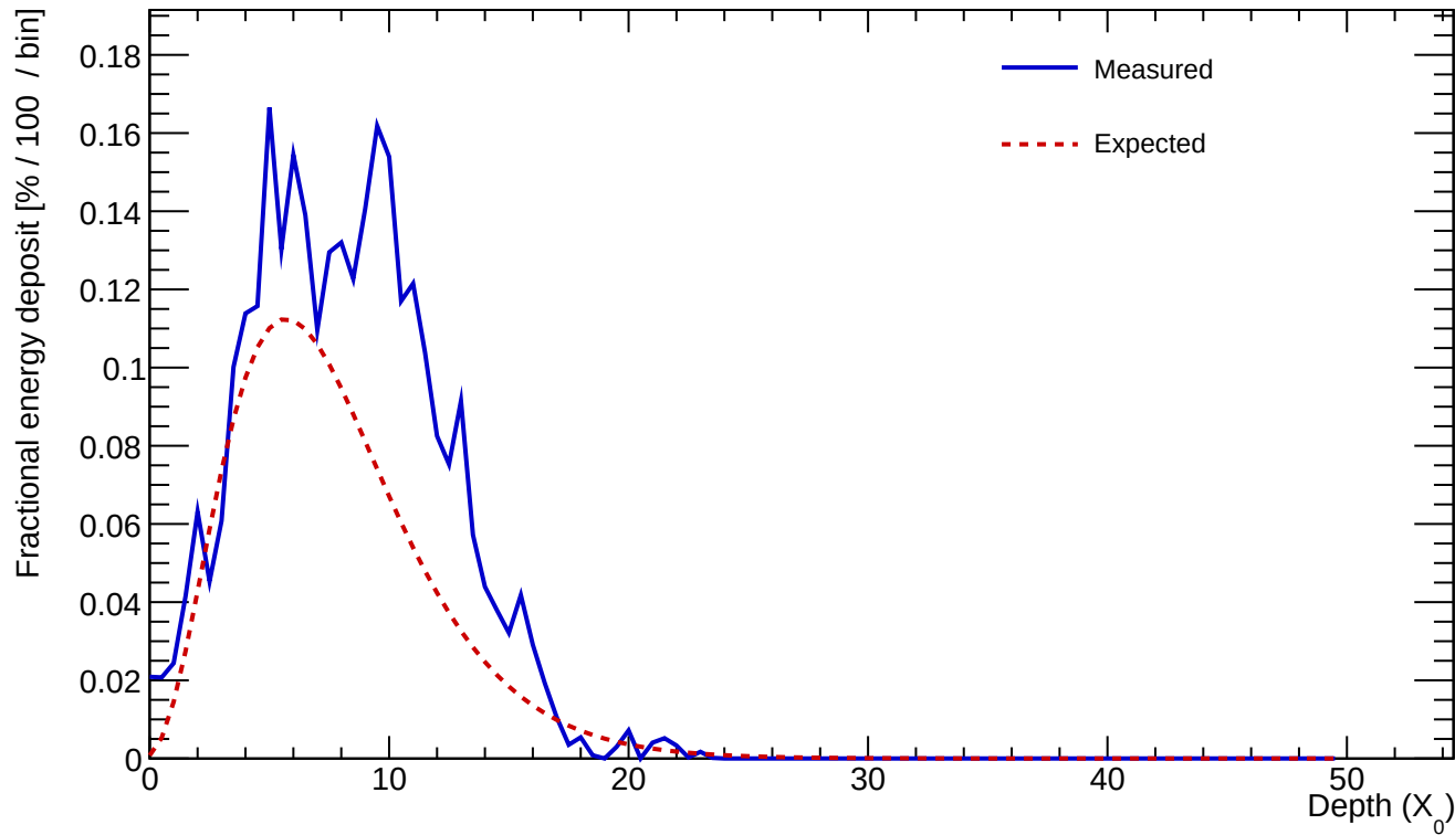
Cluster 6 E=23.925 GeV profileStart=1.00 X_0 \chi=0.2152
