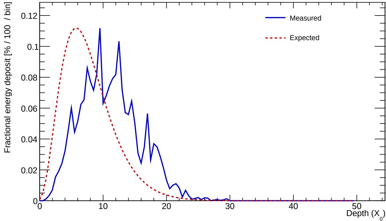
Cluster 179 E=24.999 GeV profileStart=3.50 X_0 \chi=0.3031
