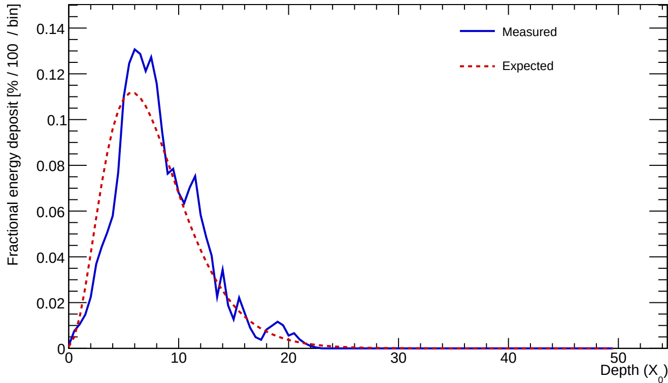
Cluster 196 E=25.337 GeV profileStart=1.00 X_0 \chi=0.1729
