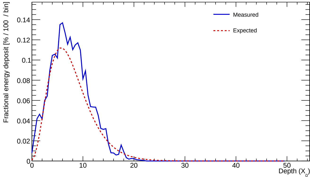
Cluster 642 E=24.719 GeV profileStart=0.50 X_0 \chi=0.1499
