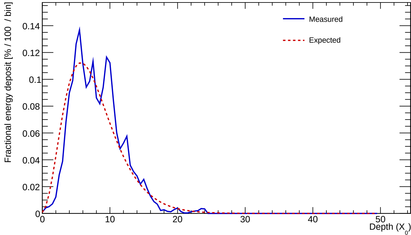
Cluster 50 E=24.182 GeV profileStart=0.50 X_0 \chi=0.1794
