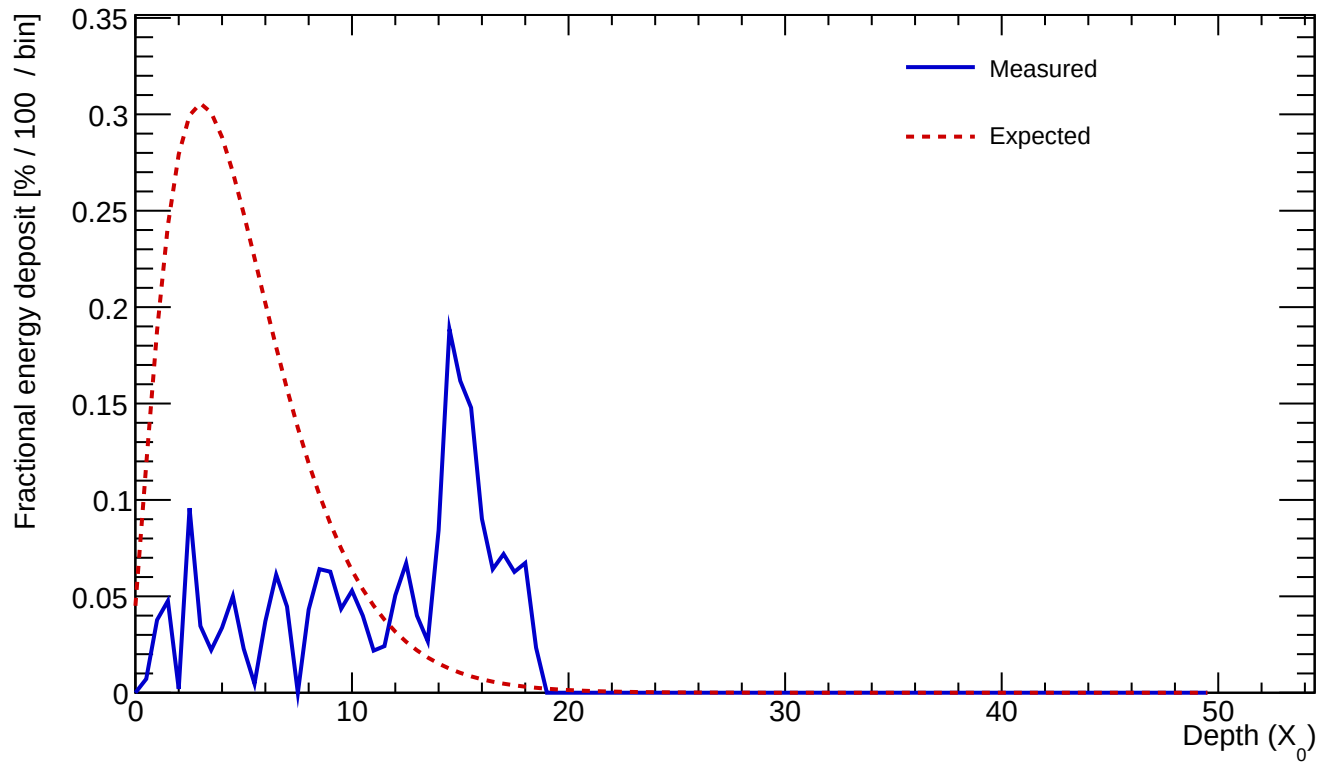
Cluster 38 E=1.621 GeV profileStart=11.50 X_0 \chi=0.6721
