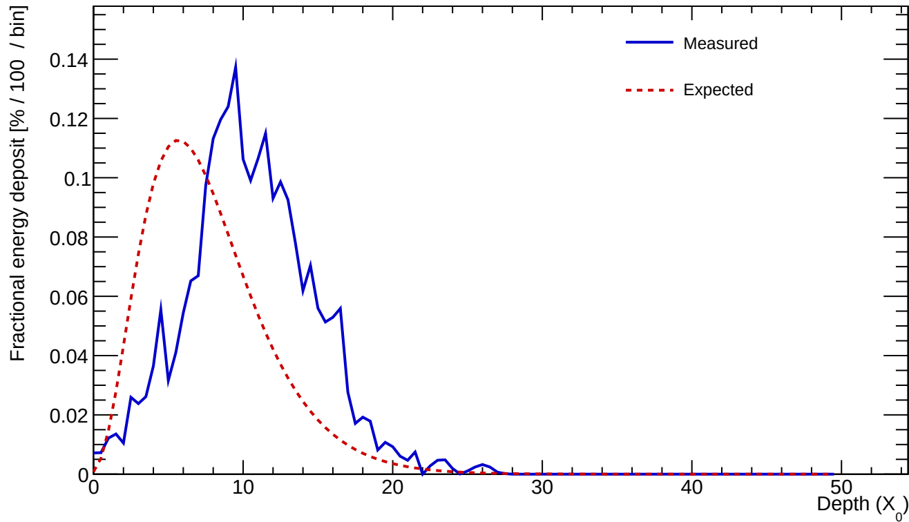
Cluster 217 E=23.445 GeV profileStart=3.50 X_0 \chi=0.2216
