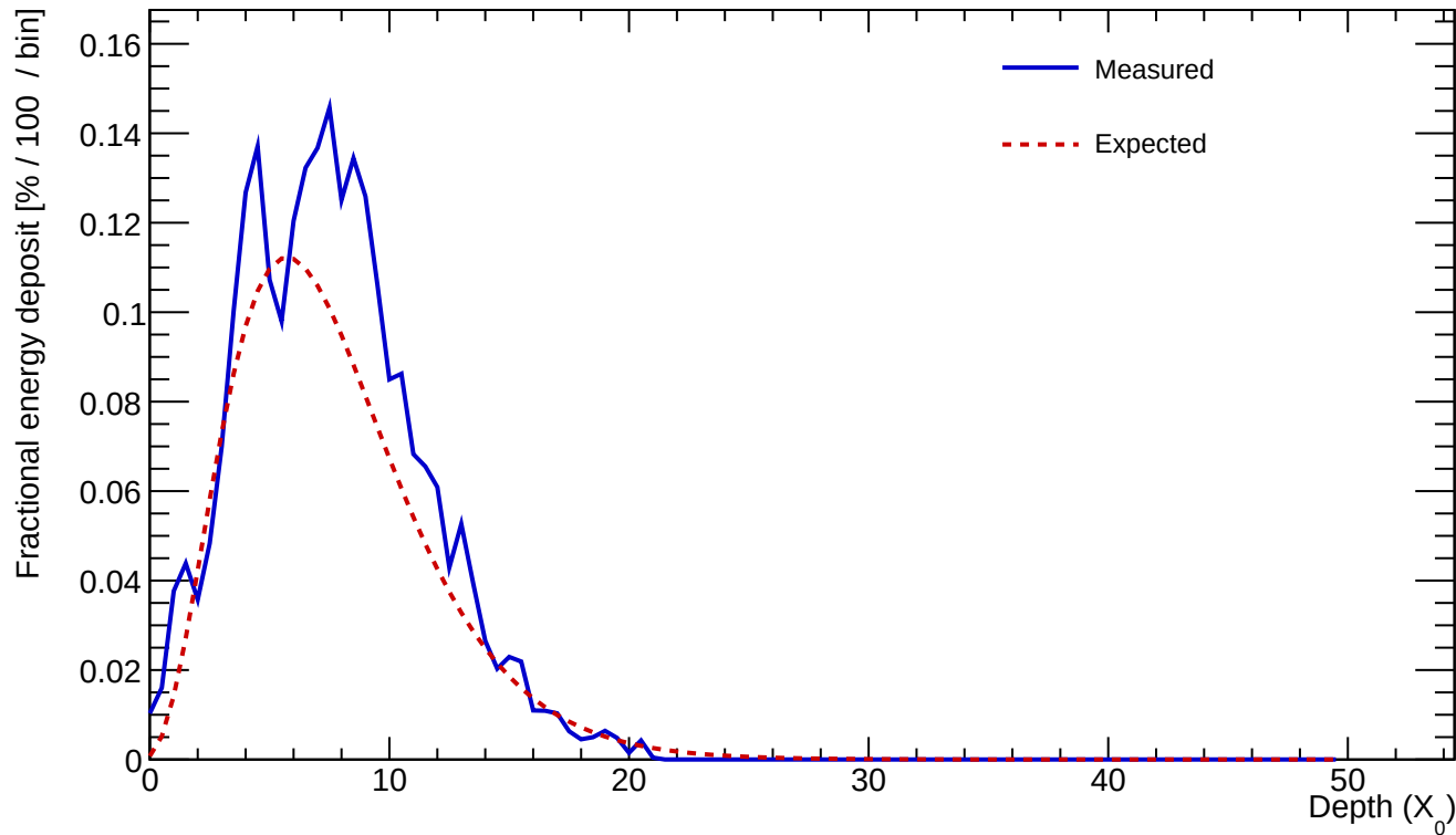
Cluster 561 E=24.430 GeV profileStart=0.50 X_0 \chi=0.1512
