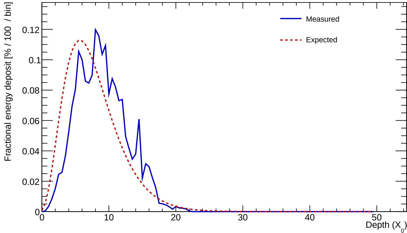
Cluster 579 E=23.129 GeV profileStart=1.50 X_0 \chi=0.1705
