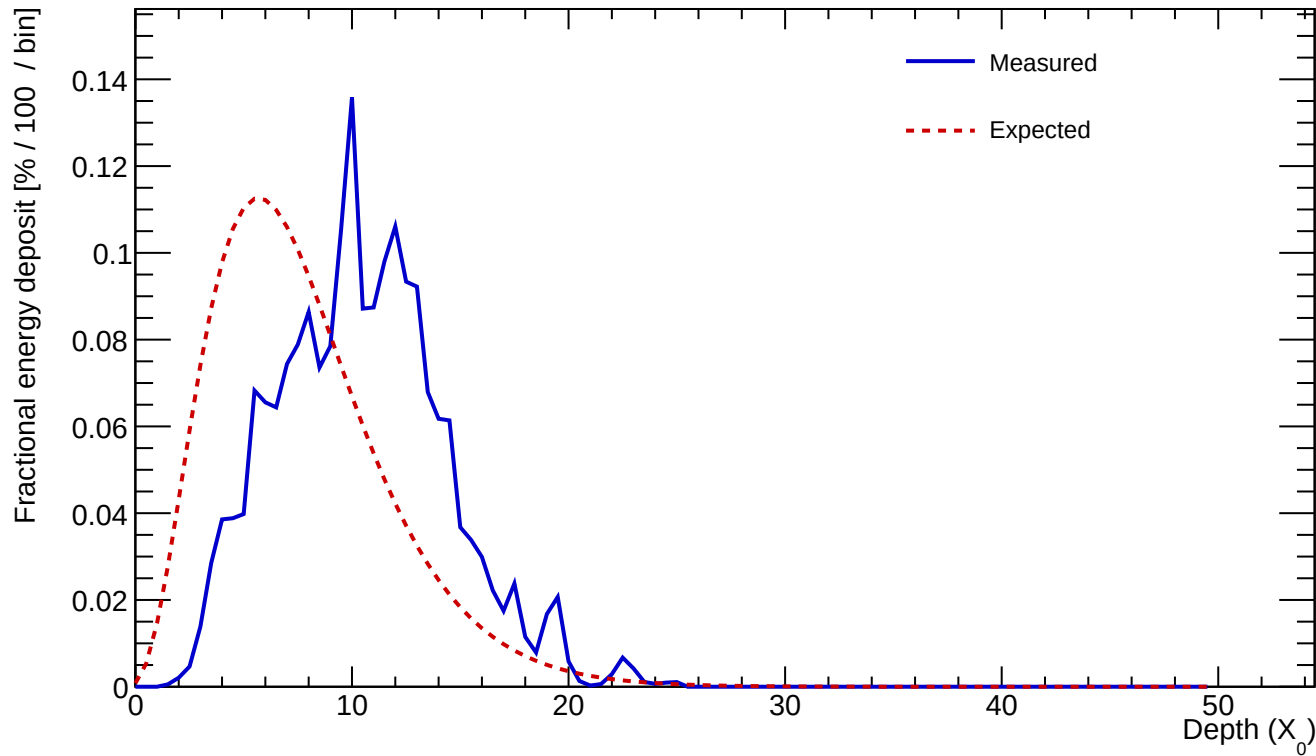
Cluster 480 E=23.576 GeV profileStart=3.00 X_0 \chi=0.2549
