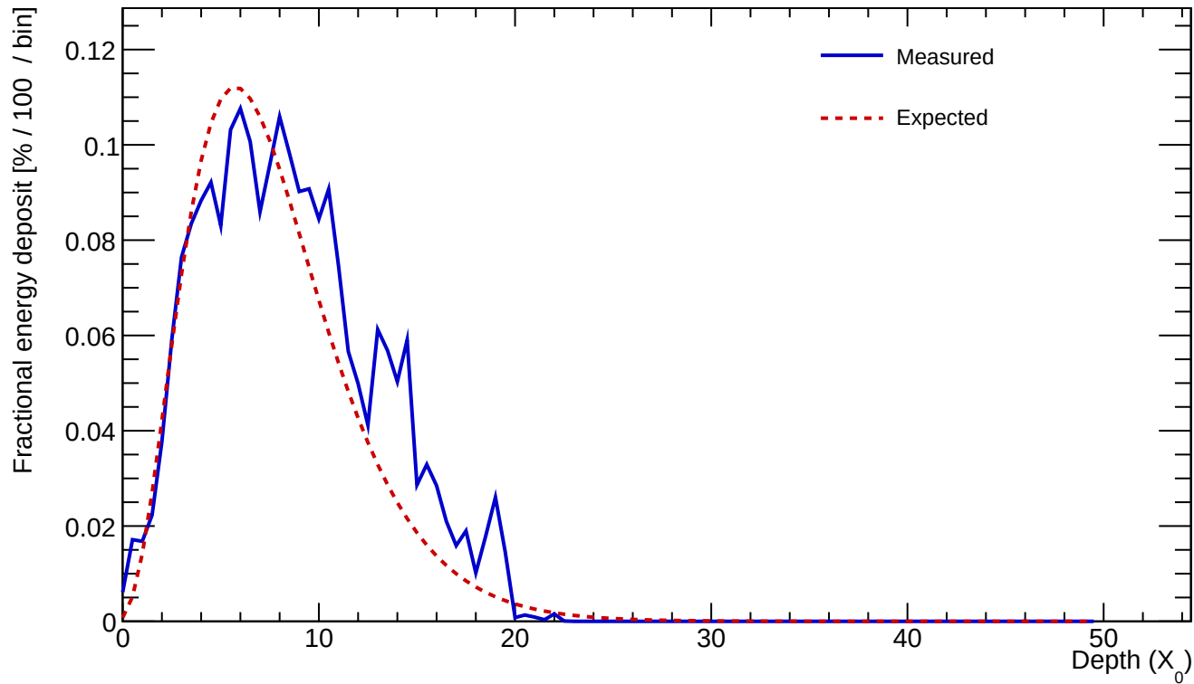
Cluster 513 E=24.610 GeV profileStart=0.50 X_0 \chi=0.2191
