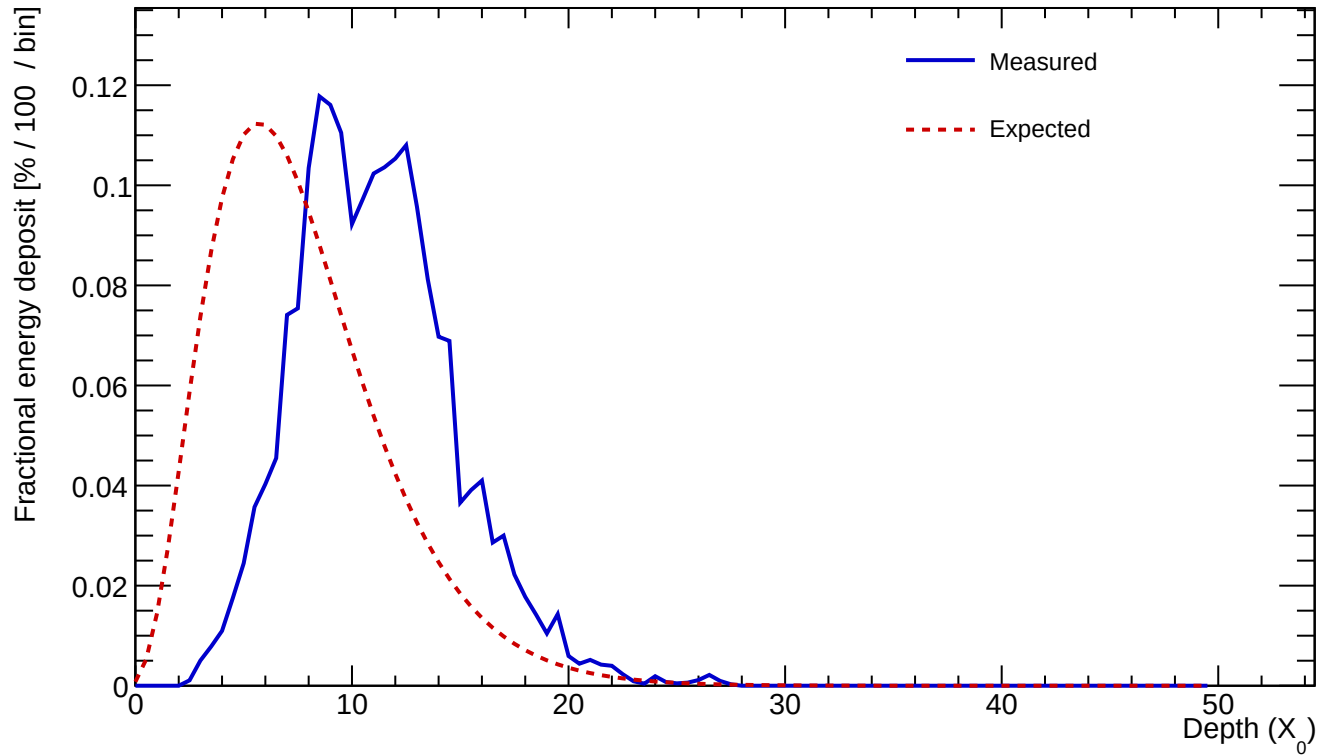
Cluster 72 E=23.887 GeV profileStart=4.00 X_0 \chi=0.1636
