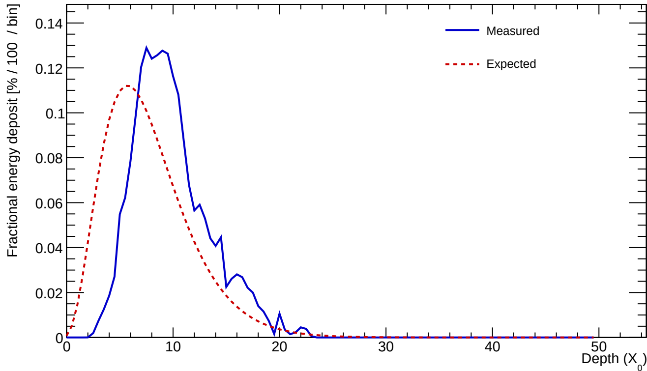
Cluster 498 E=24.413 GeV profileStart=2.50 X_0 \chi=0.1548
