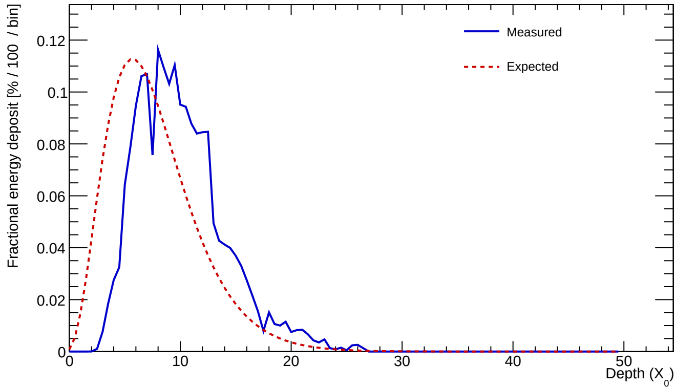
Cluster 405 E=23.431 GeV profileStart=2.50 X_0 \chi=0.1056
