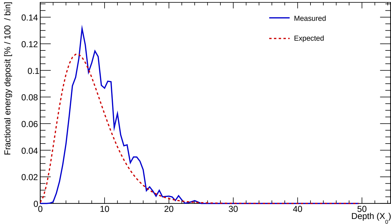
Cluster 464 E=24.293 GeV profileStart=1.50 X_0 \chi=0.1274
