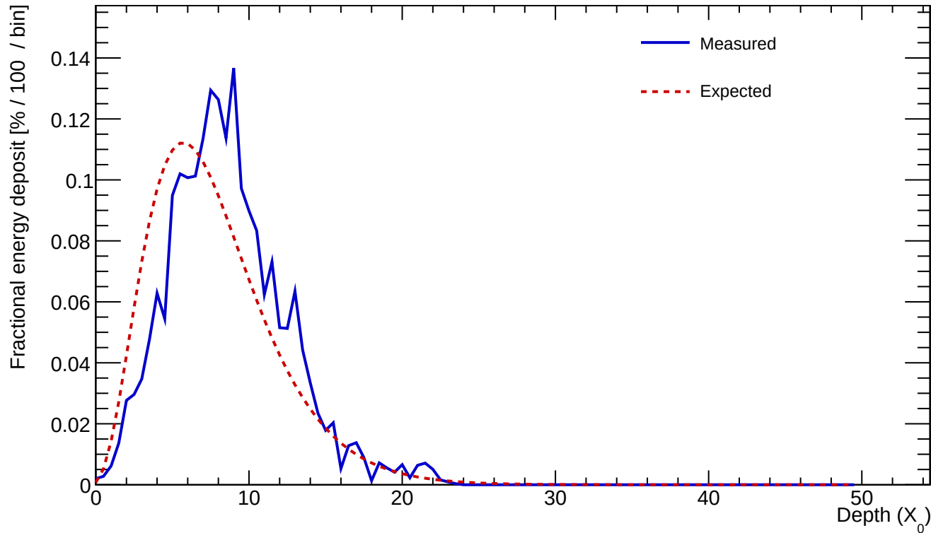
Cluster 364 E=24.347 GeV profileStart=1.50 X_0 \chi=0.1595
