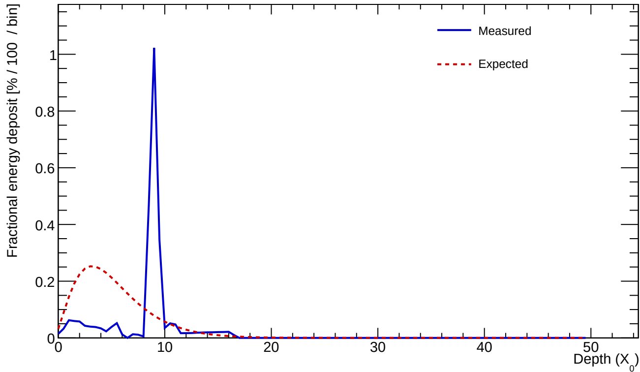
Cluster 562 E=1.903 GeV profileStart=5.00 X_0 \chi=1.2100
