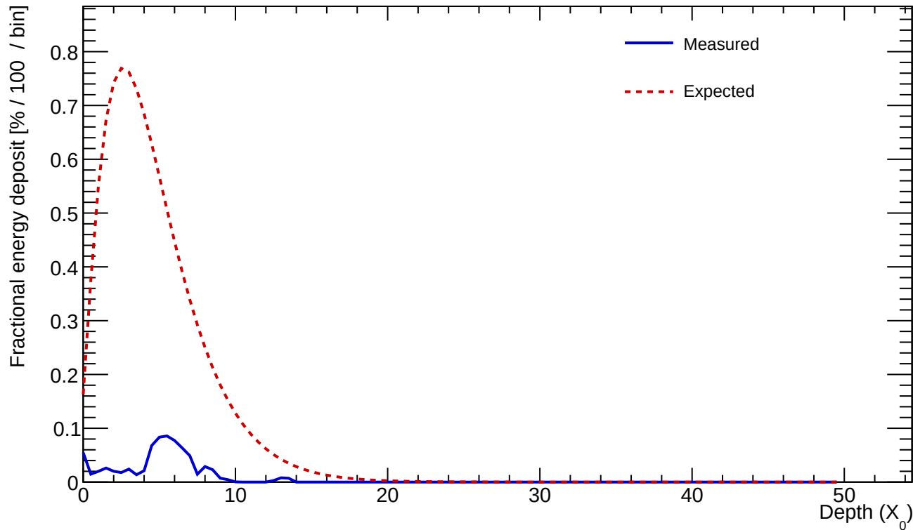
Cluster 466 E=1.104 GeV profileStart=2.00 X_0 \chi=0.6549
