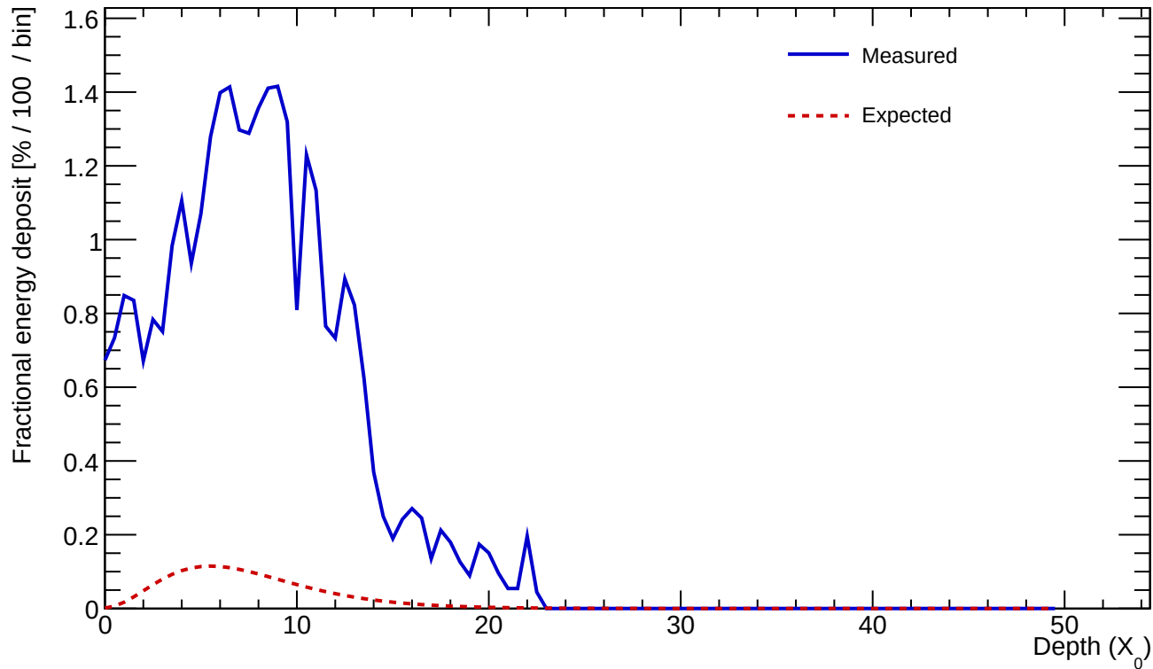
Cluster 138 E=19.514 GeV profileStart=1.00 X_0 \chi=0.3065
