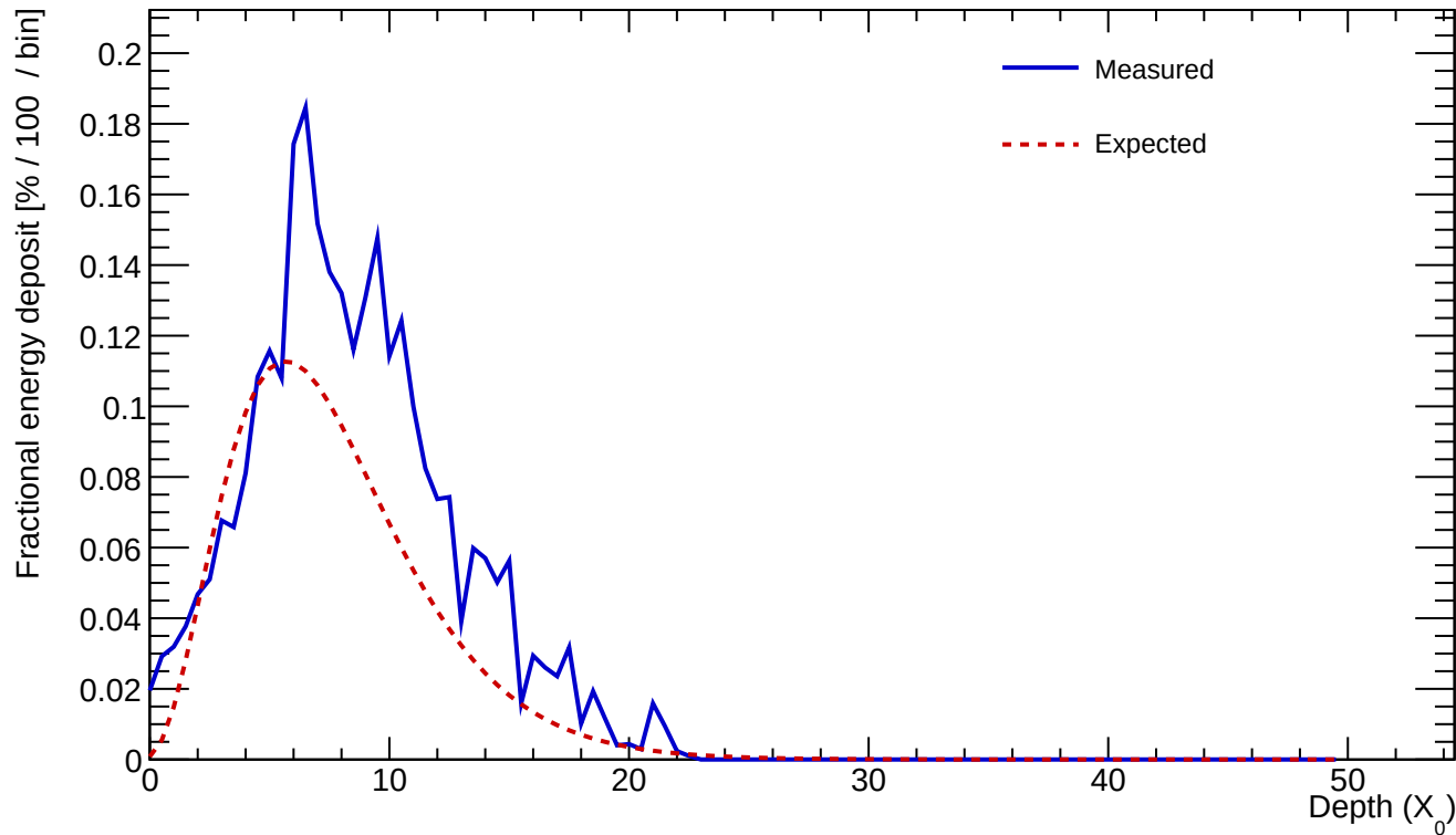
Cluster 673 E=23.123 GeV profileStart=1.00 X_0 \chi=0.2096
