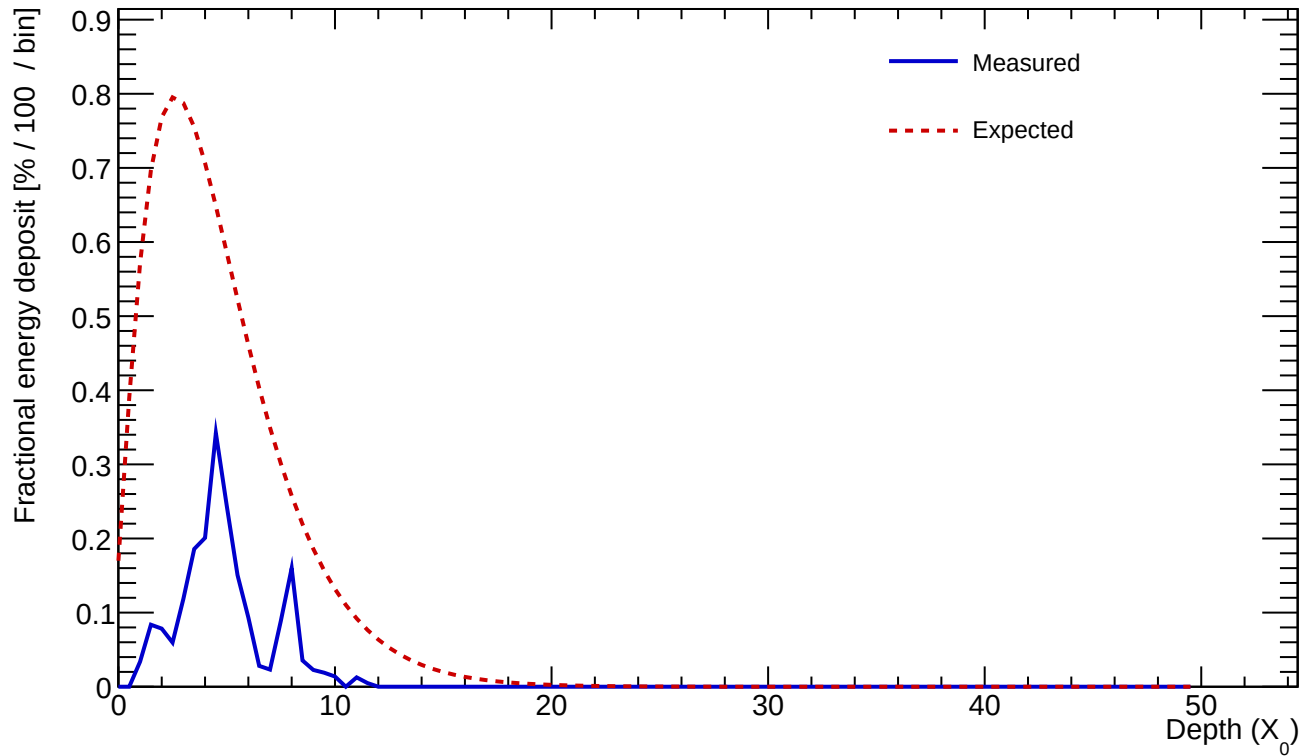
Cluster 184 E=1.096 GeV profileStart=1.00 X_0 \chi=0.4790
