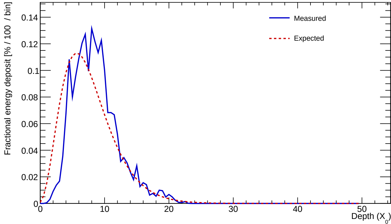
Cluster 492 E=23.005 GeV profileStart=1.50 X_0 \chi=0.1839
