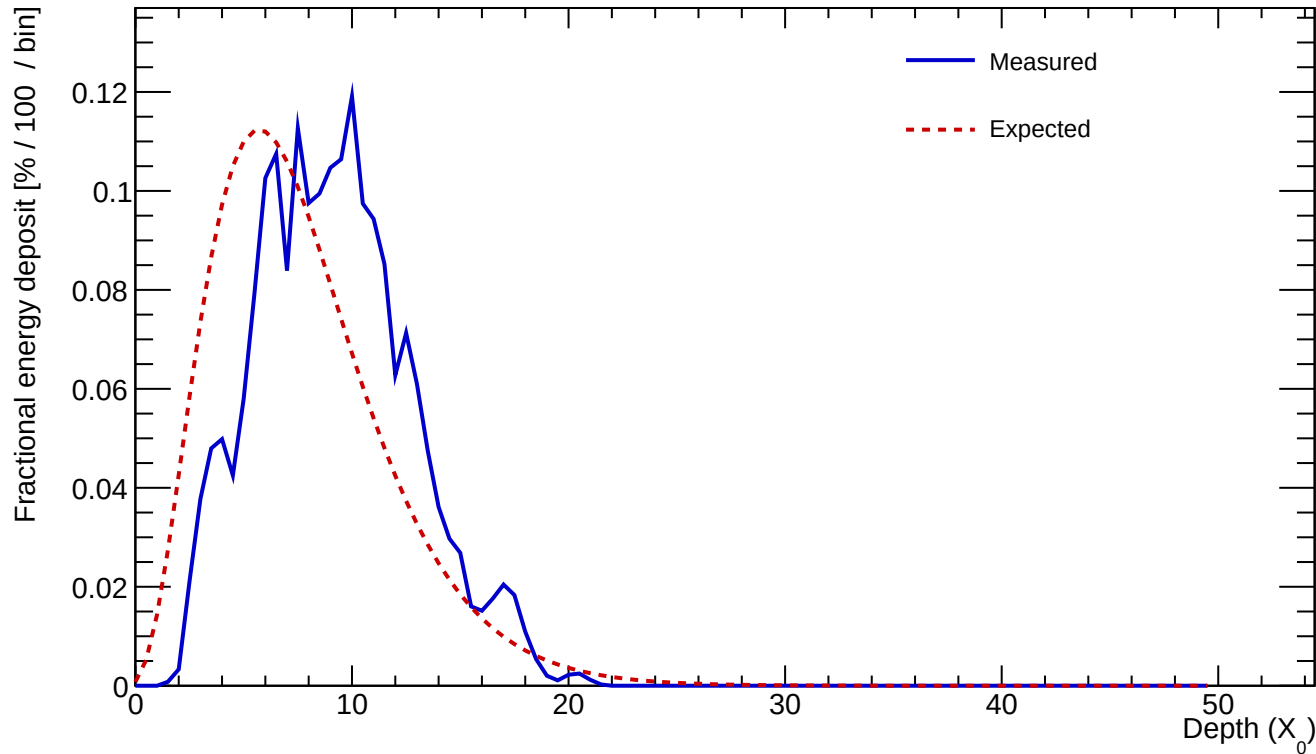
Cluster 655 E=24.110 GeV profileStart=2.00 X_0 \chi=0.1720
