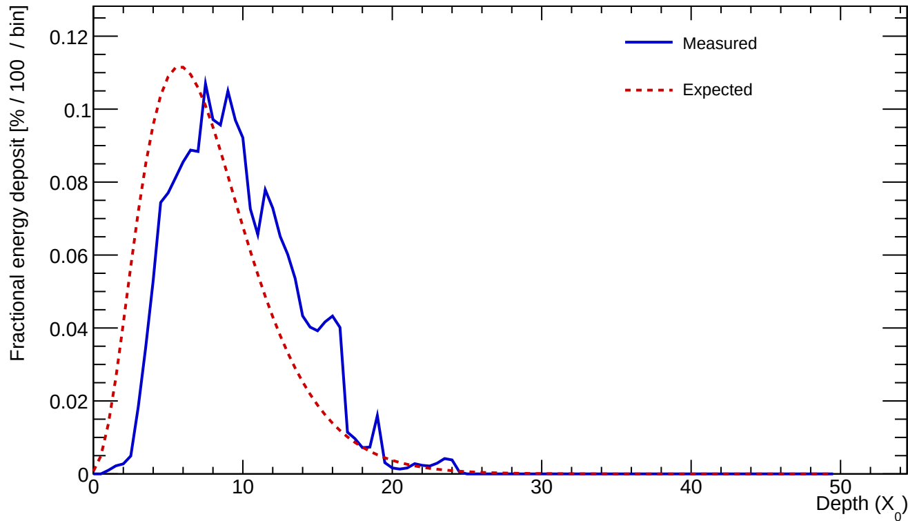
Cluster 571 E=25.547 GeV profileStart=2.00 X_0 \chi=0.1529
