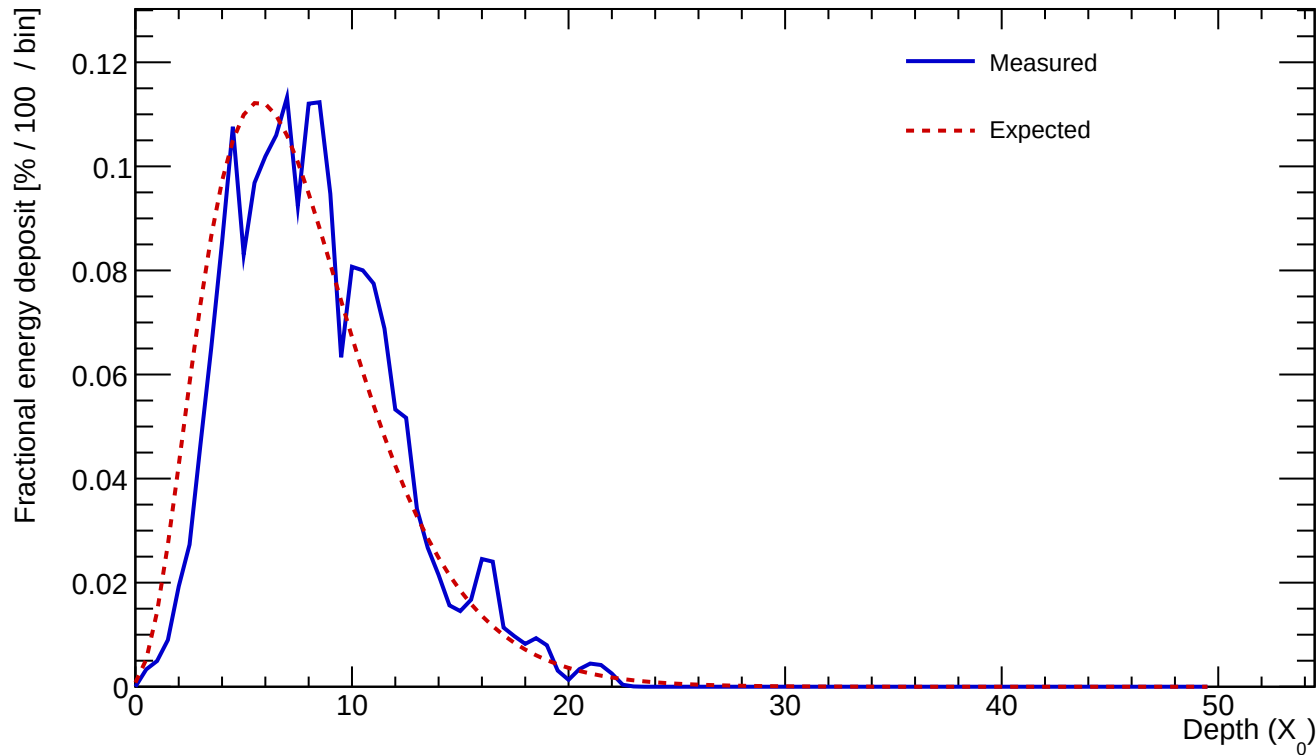
Cluster 191 E=24.160 GeV profileStart=1.00 X_0 \chi=0.1405
