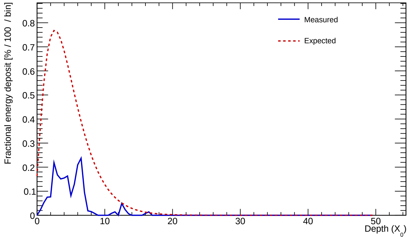
Cluster 292 E=1.104 GeV profileStart=1.00 X_0 \chi=0.4733
