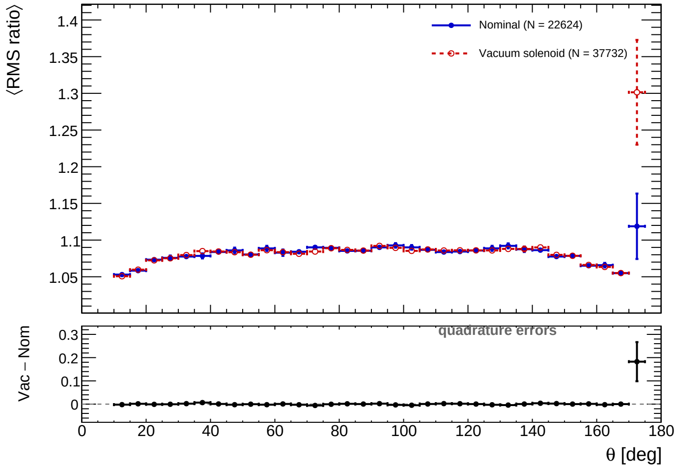
RMS ratio vs \theta (profile-selected clusters)
