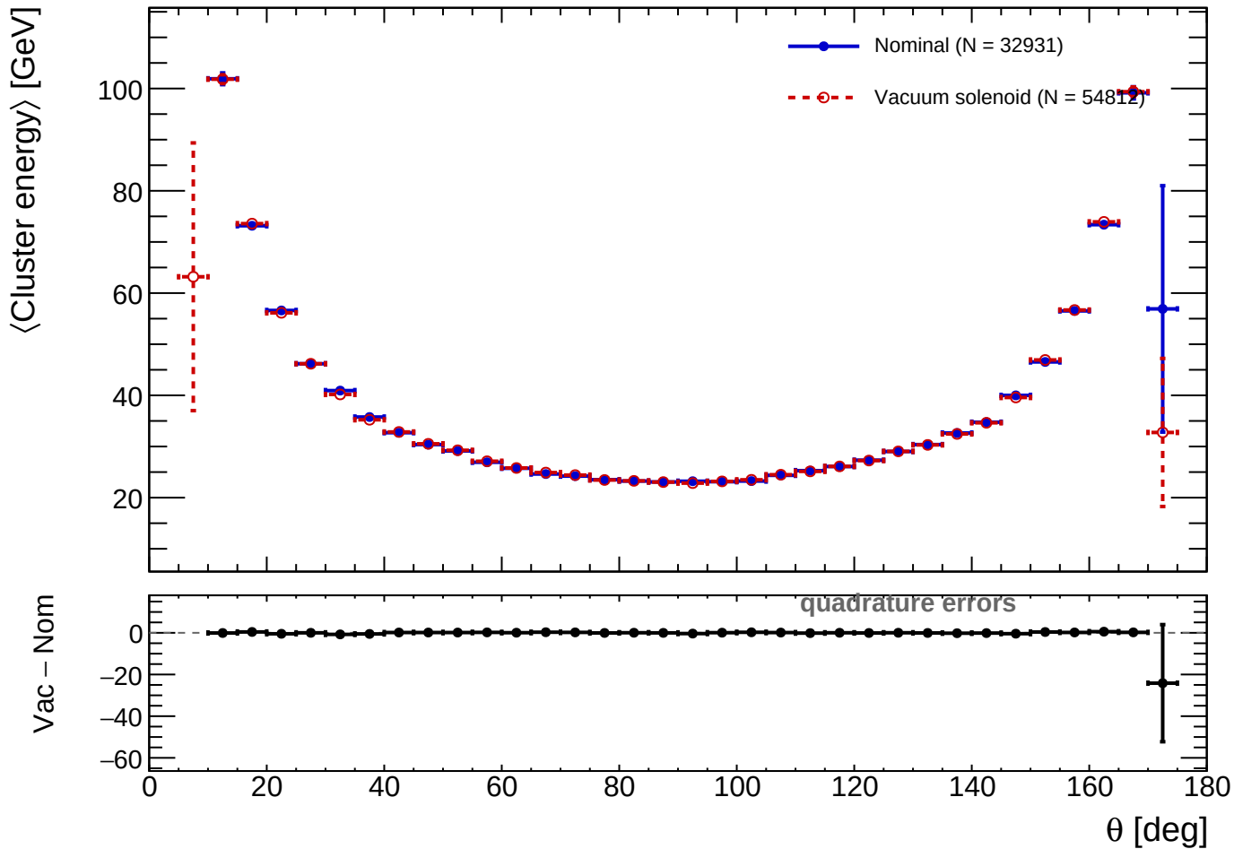
Cluster energy vs \theta (all clusters)
