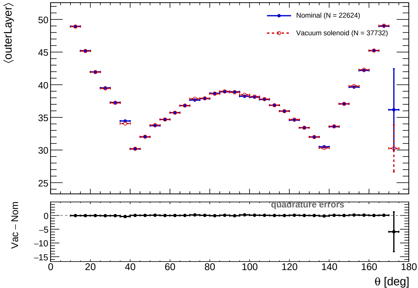
outerLayer vs \theta (profile-selected clusters)
