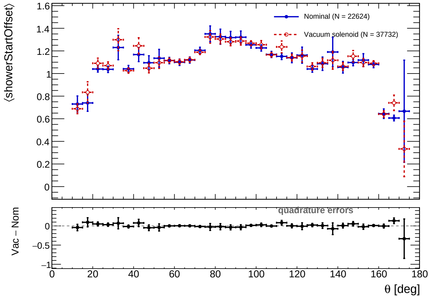
showerStartOffset vs \theta (profile-selected clusters)
