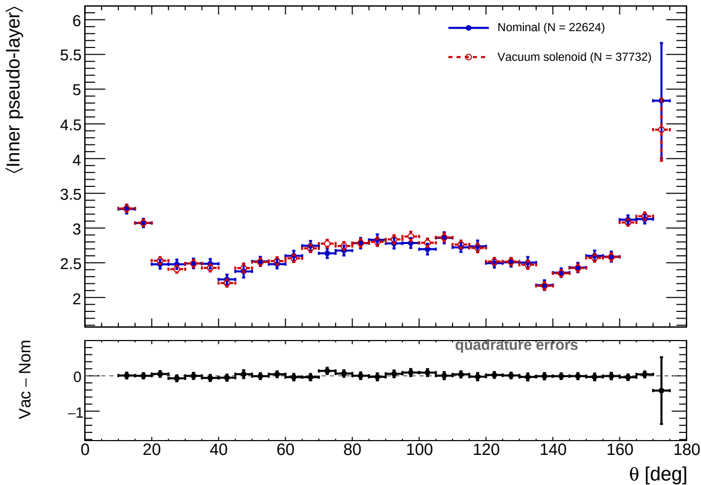
Inner pseudo-layer vs \theta (profile-selected clusters)
