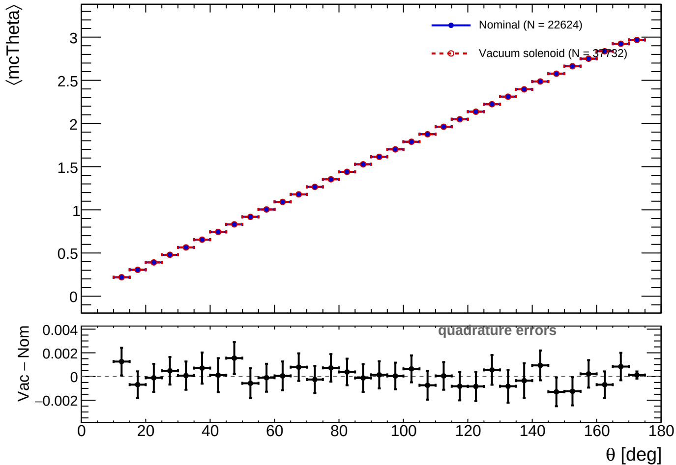
mcTheta vs \theta (profile-selected clusters)
