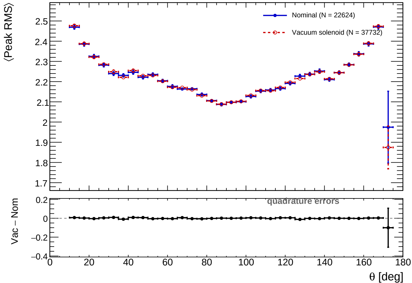
Peak RMS vs \theta (profile-selected clusters)
