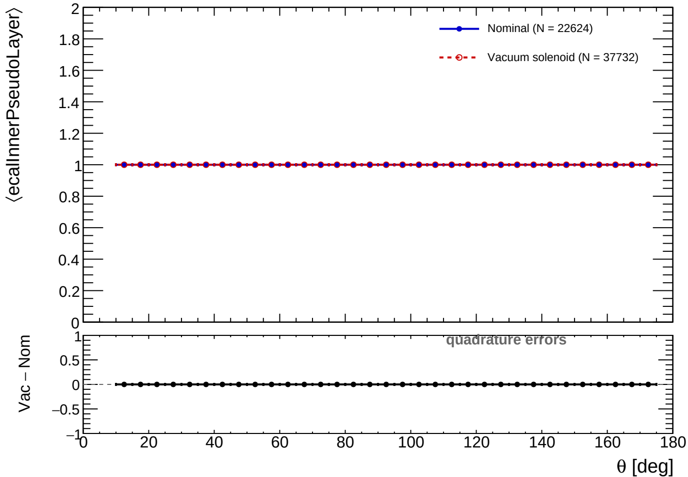
ecallInnerPseudoLayer vs \theta (profile-selected clusters)
