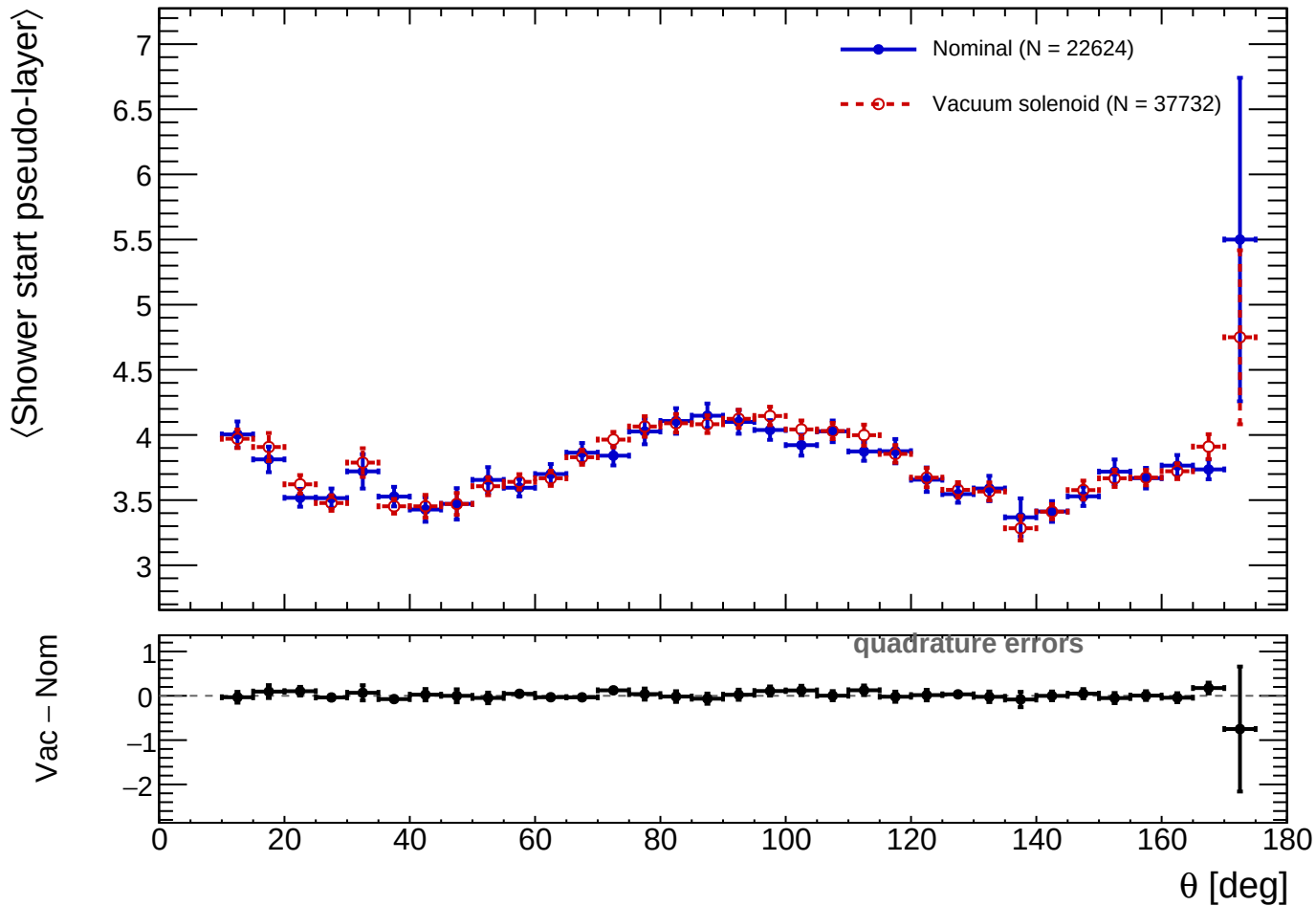
Shower start pseudo-layer vs \theta (profile-selected clusters)
