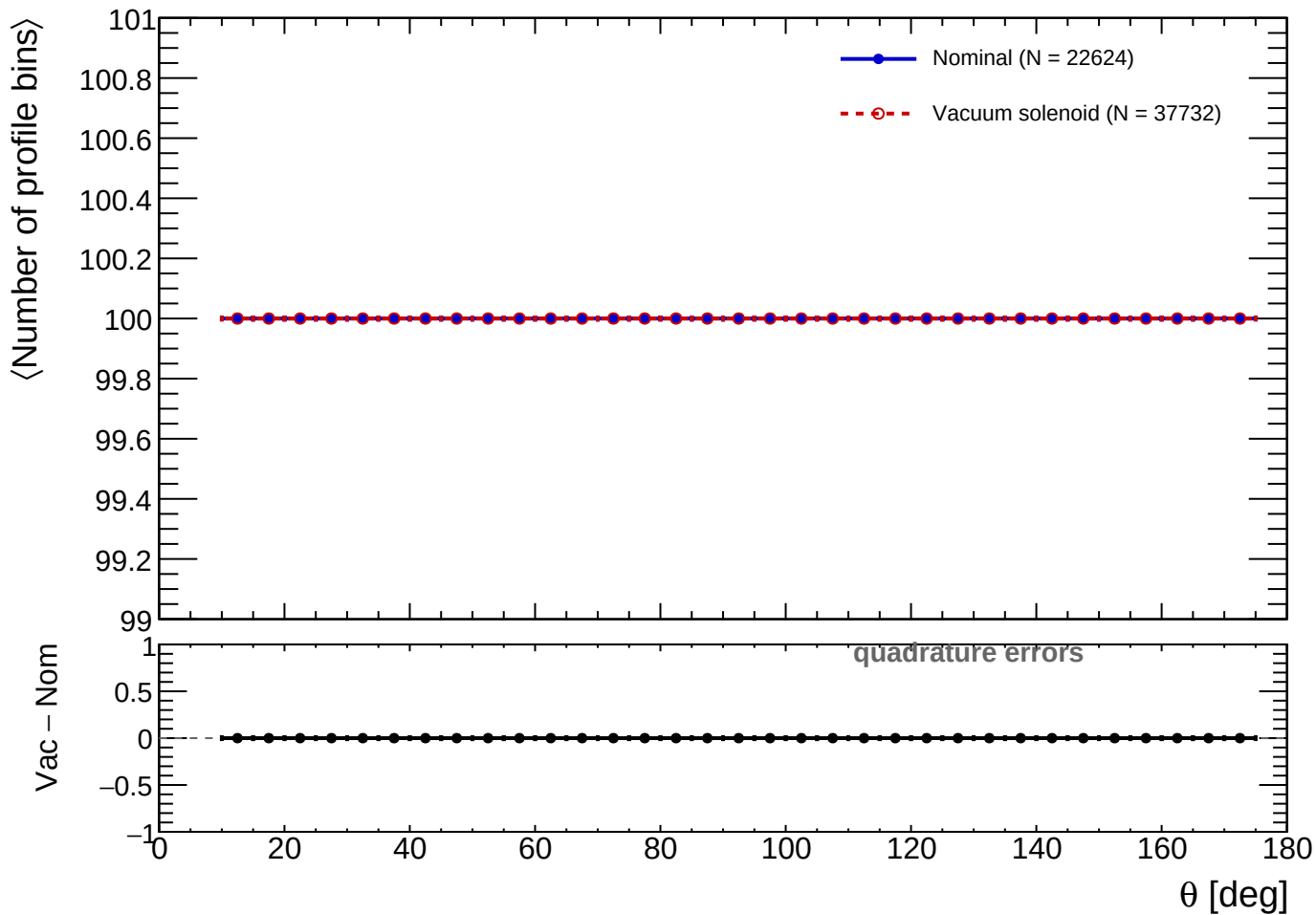
Number of profile bins vs \theta (profile-selected clusters)
