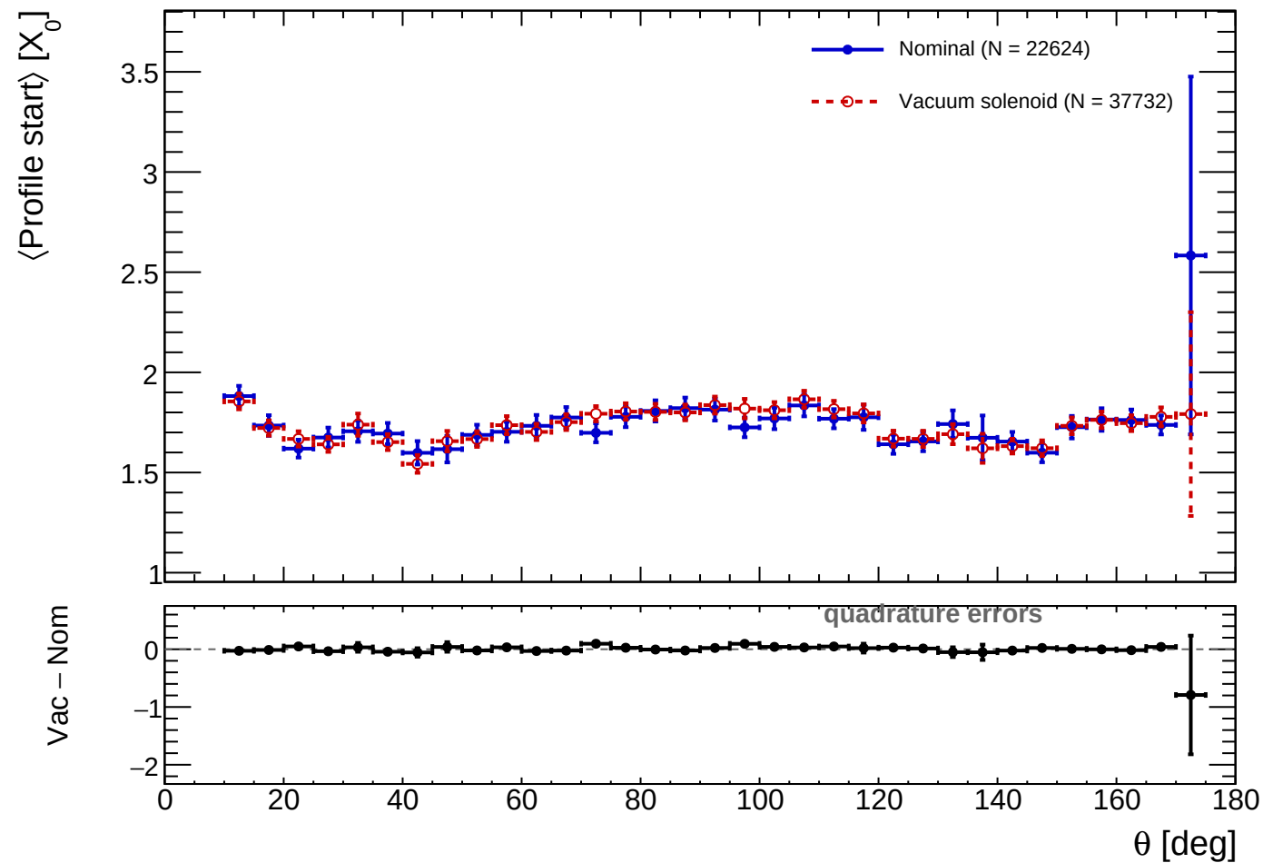
Profile start vs \theta (profile-selected clusters)
