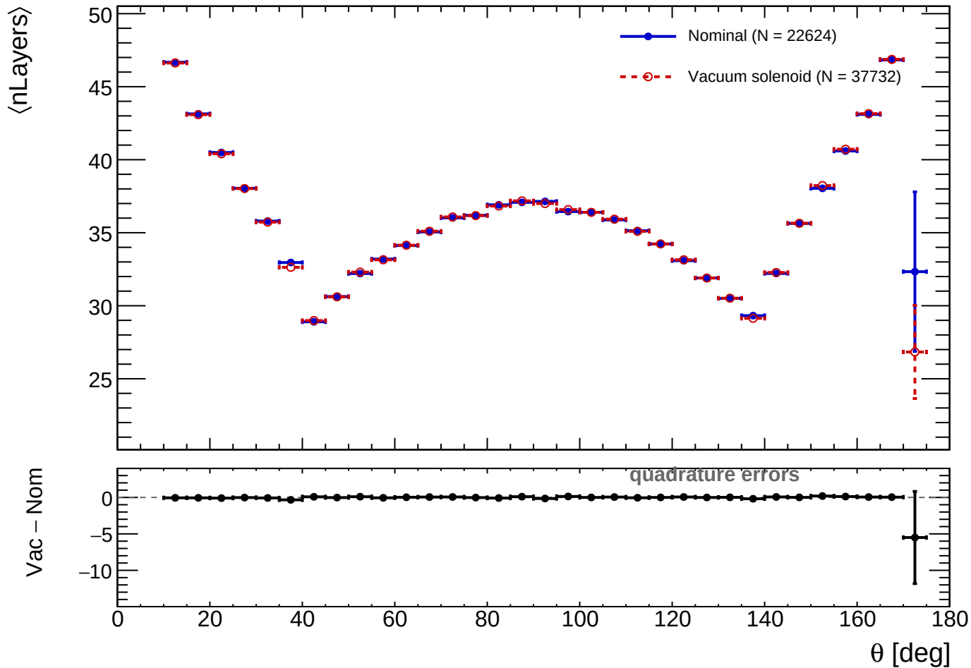
nLayers vs \theta (profile-selected clusters)
