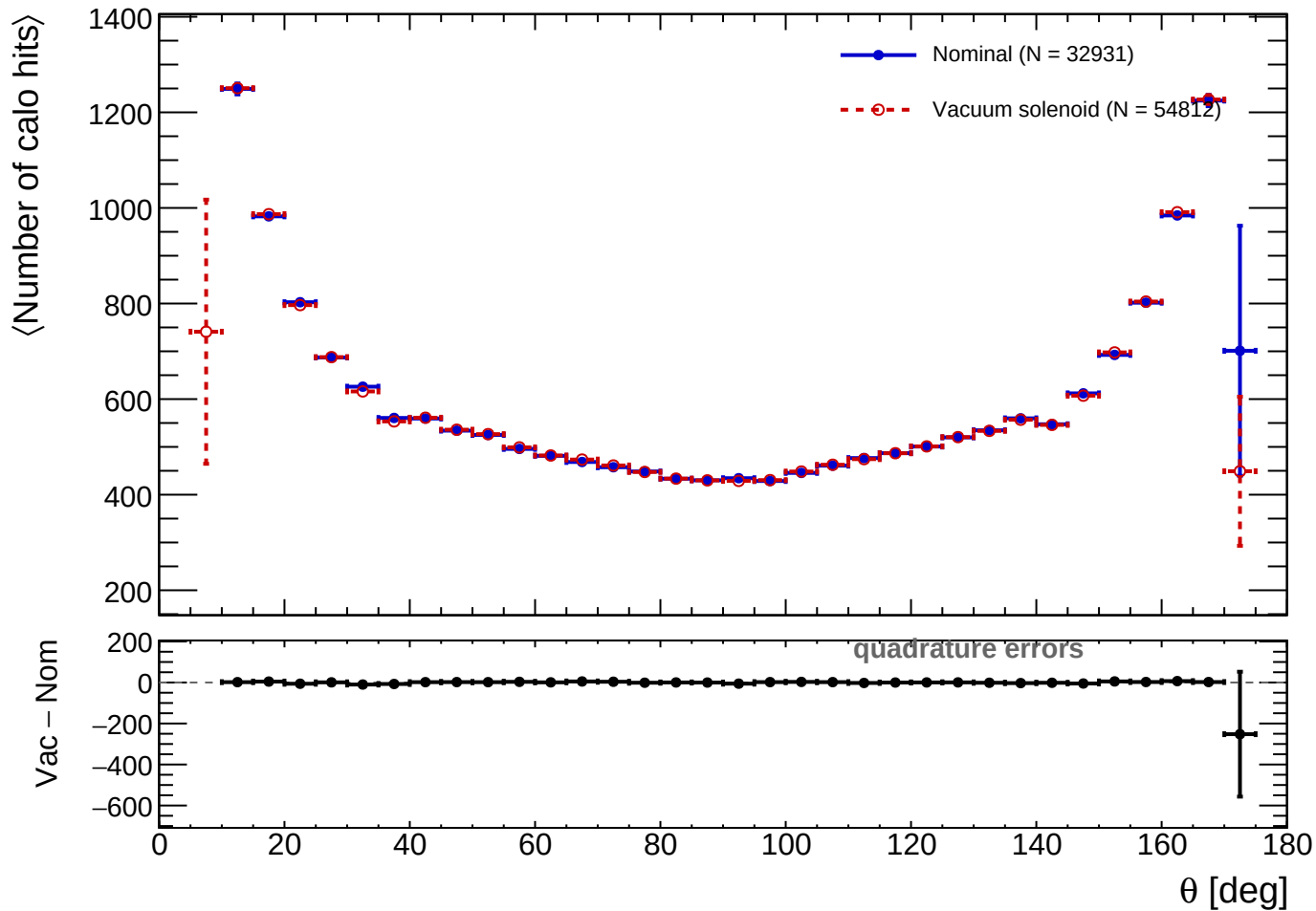
Number of calo hits vs \theta (all clusters)
