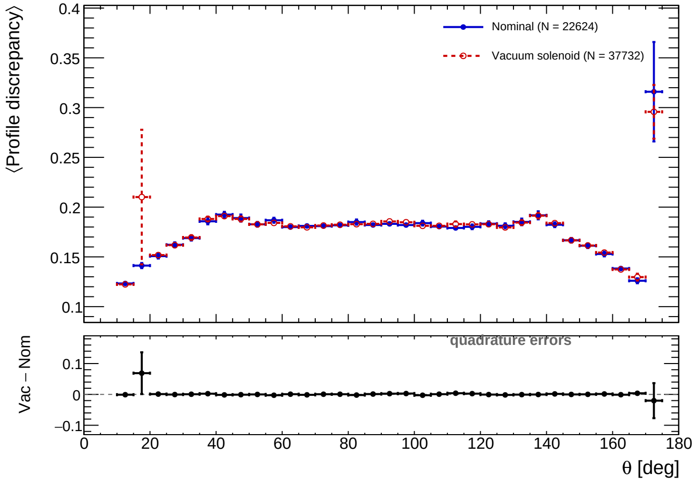
Profile discrepancy vs \theta (profile-selected clusters)
