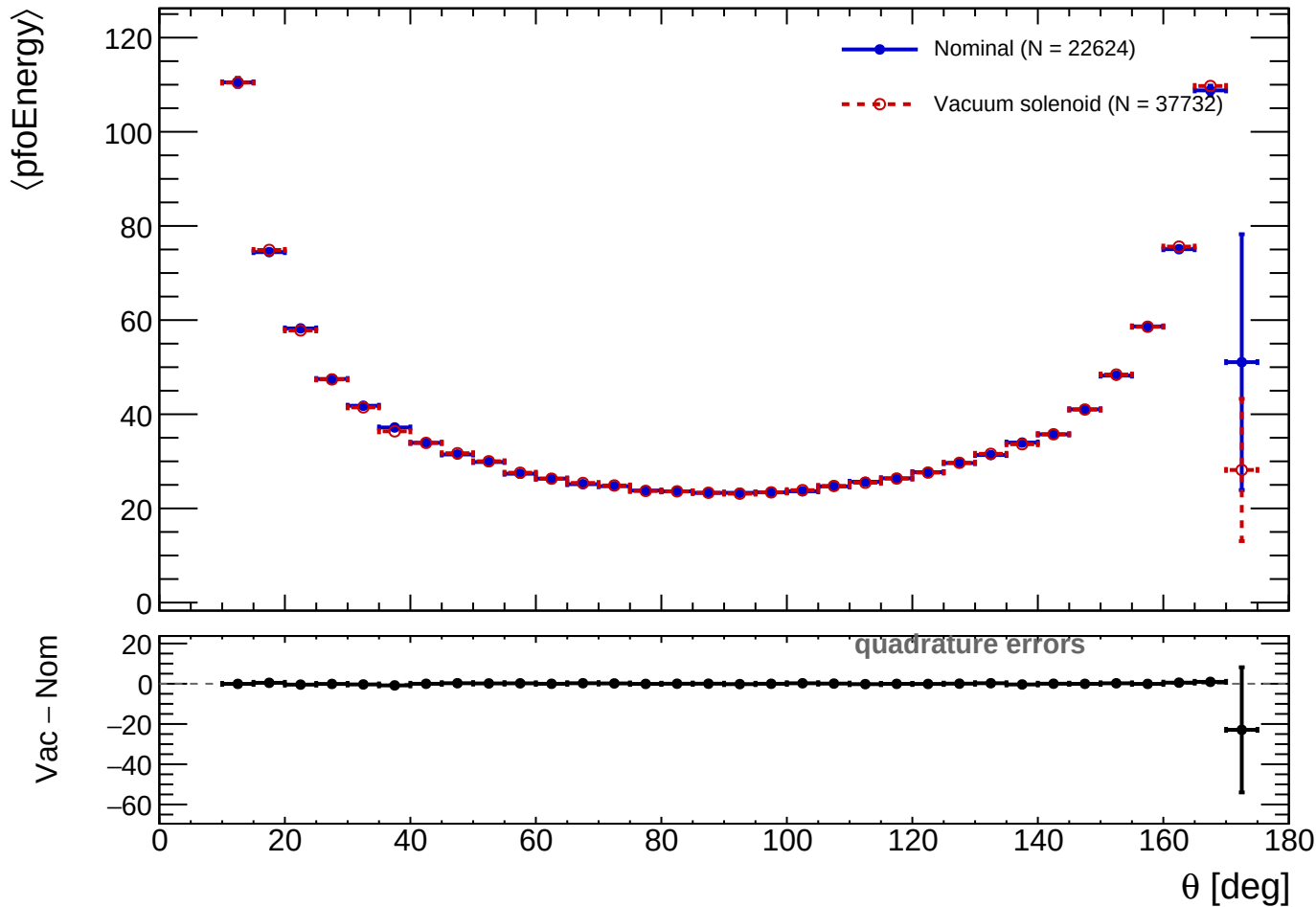
pfoEnergy vs \theta (profile-selected clusters)
