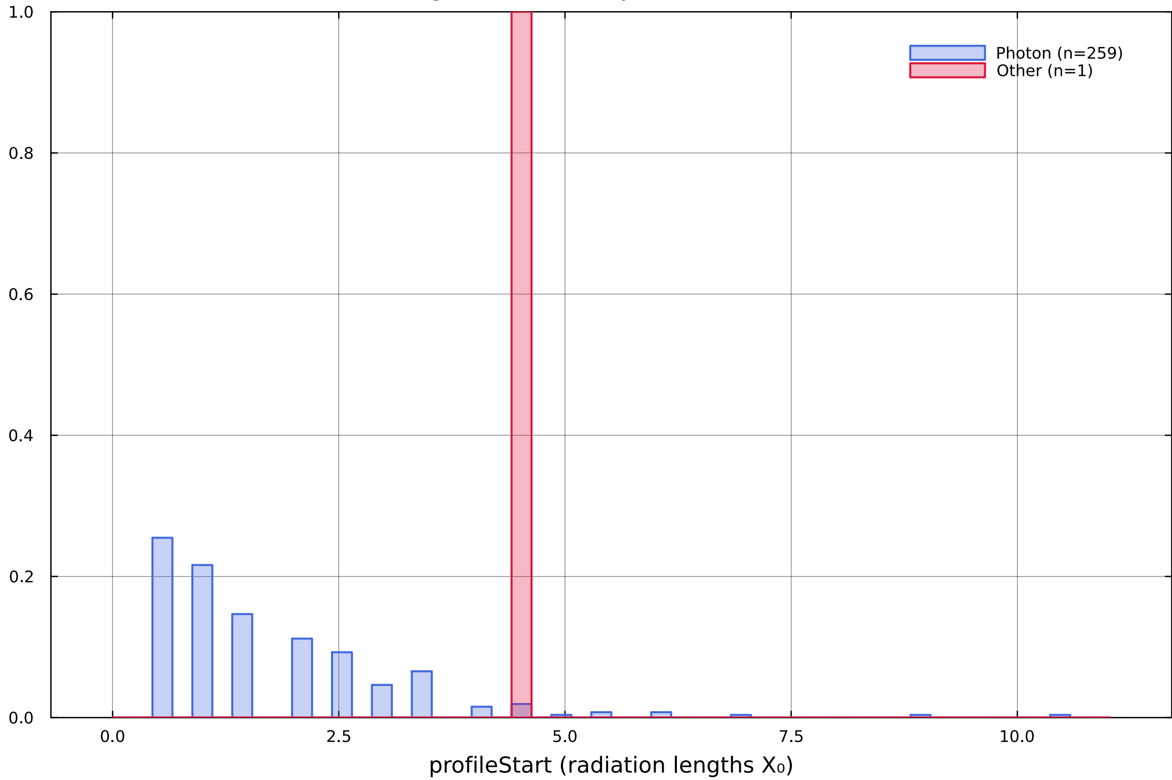
LongProfileStart: photon vs other
