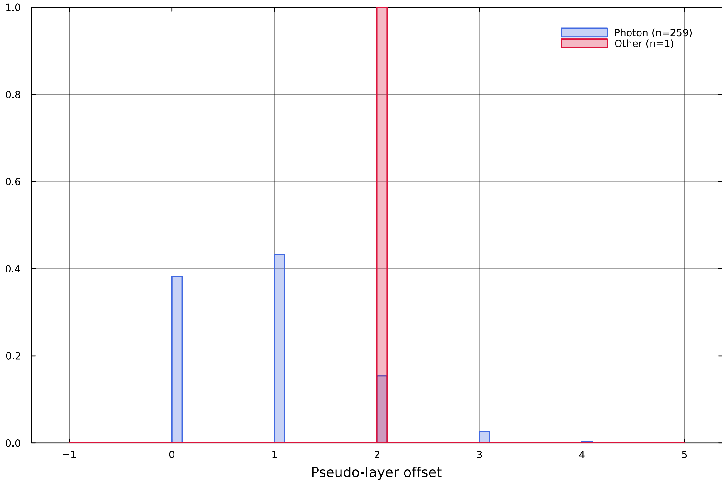
Shower start offset: photon vs other (showerStartLayer – innerLayer)
