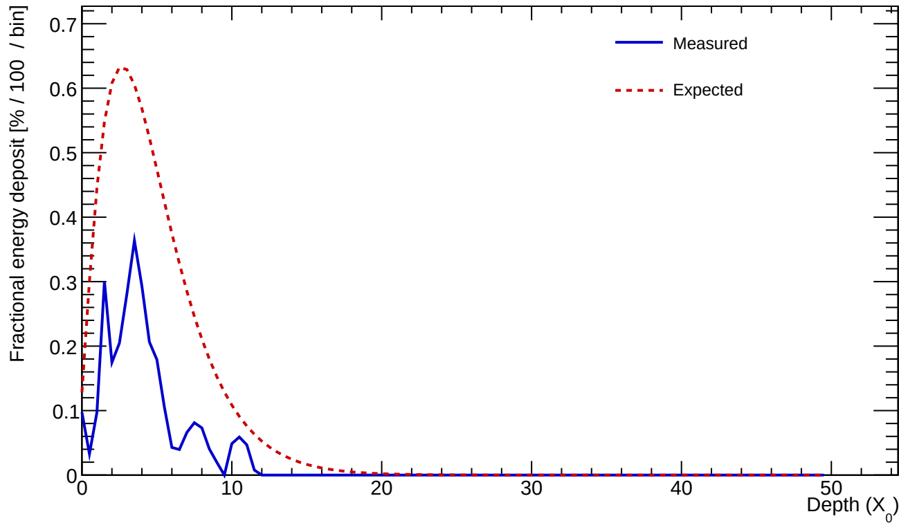
Cluster 3 E=1.159 GeV profileStart=0.50 X_0 \chi=0.3762
