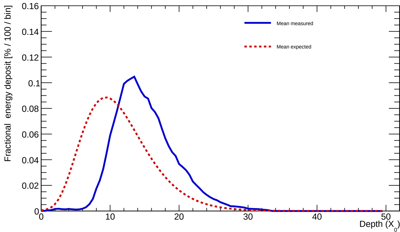
Average longitudinal profile (12 clusters): measured vs expected
