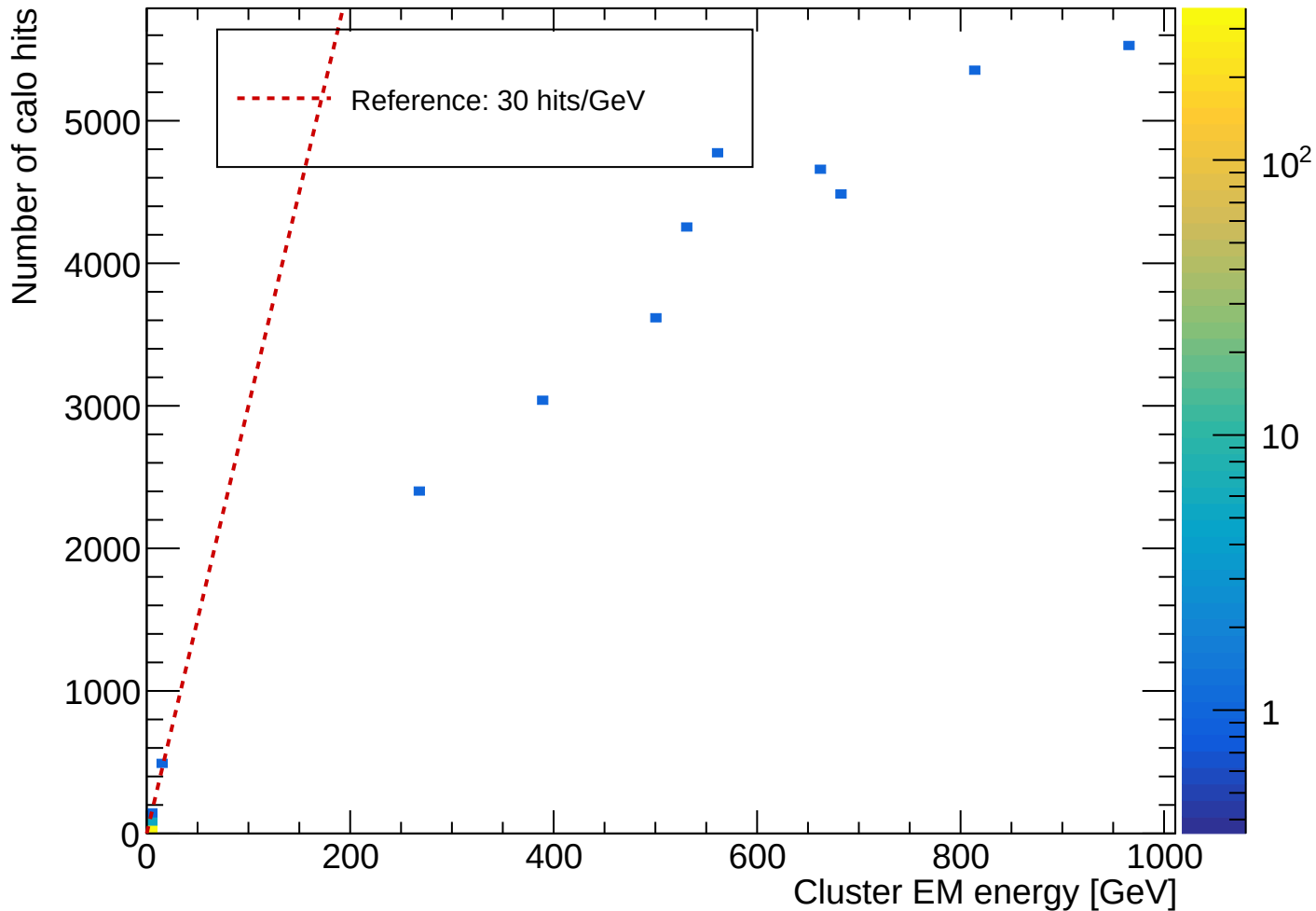
Cluster energy vs number of calo hits
