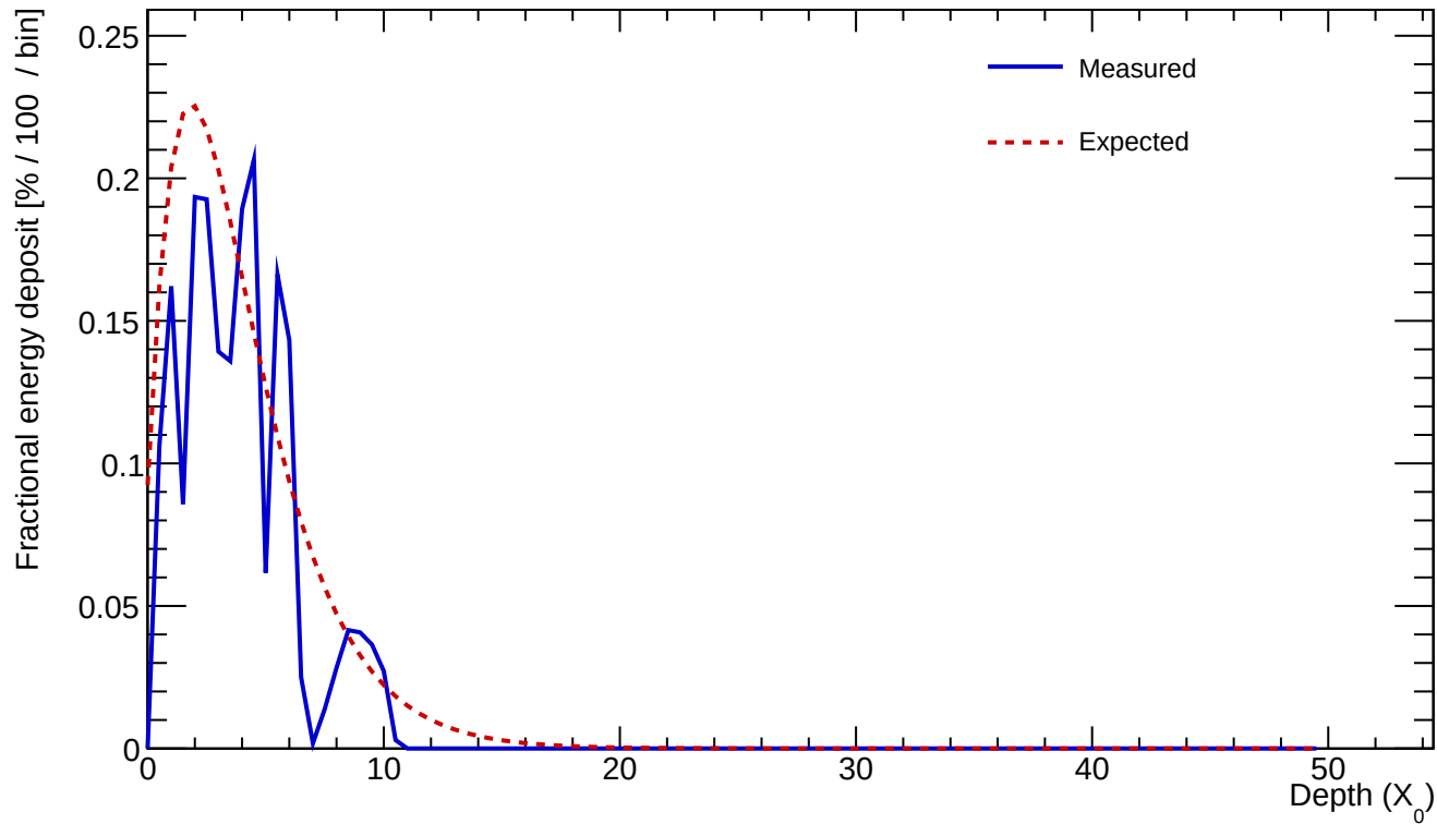
Cluster 4 E=0.508 GeV profileStart=0.50 X_0 \chi=0.3668
