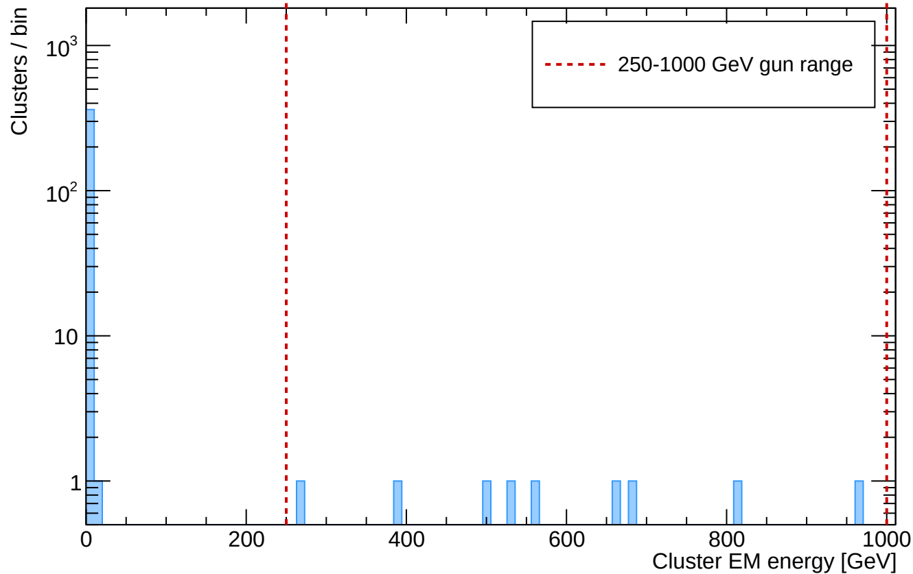
Cluster energy distribution (all clusters)
