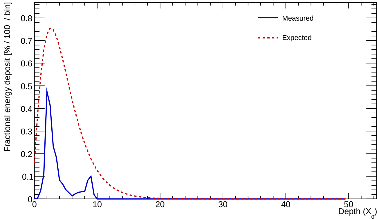
Cluster 9 E=1.109 GeV profileStart=0.50 X_0 \chi=0.7207
