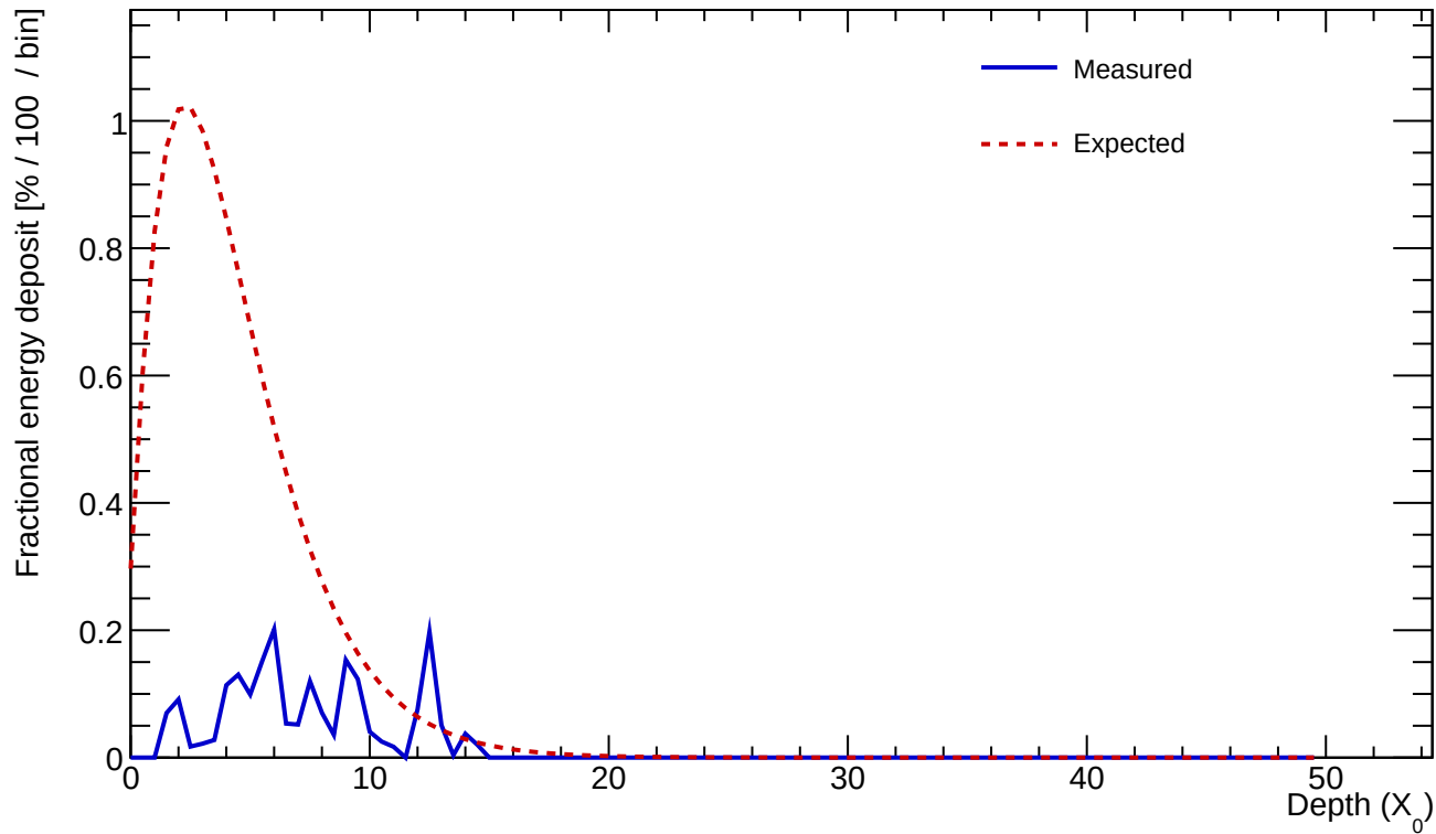
Cluster 8 E=0.778 GeV profileStart=3.50 X_0 \chi=0.5871
