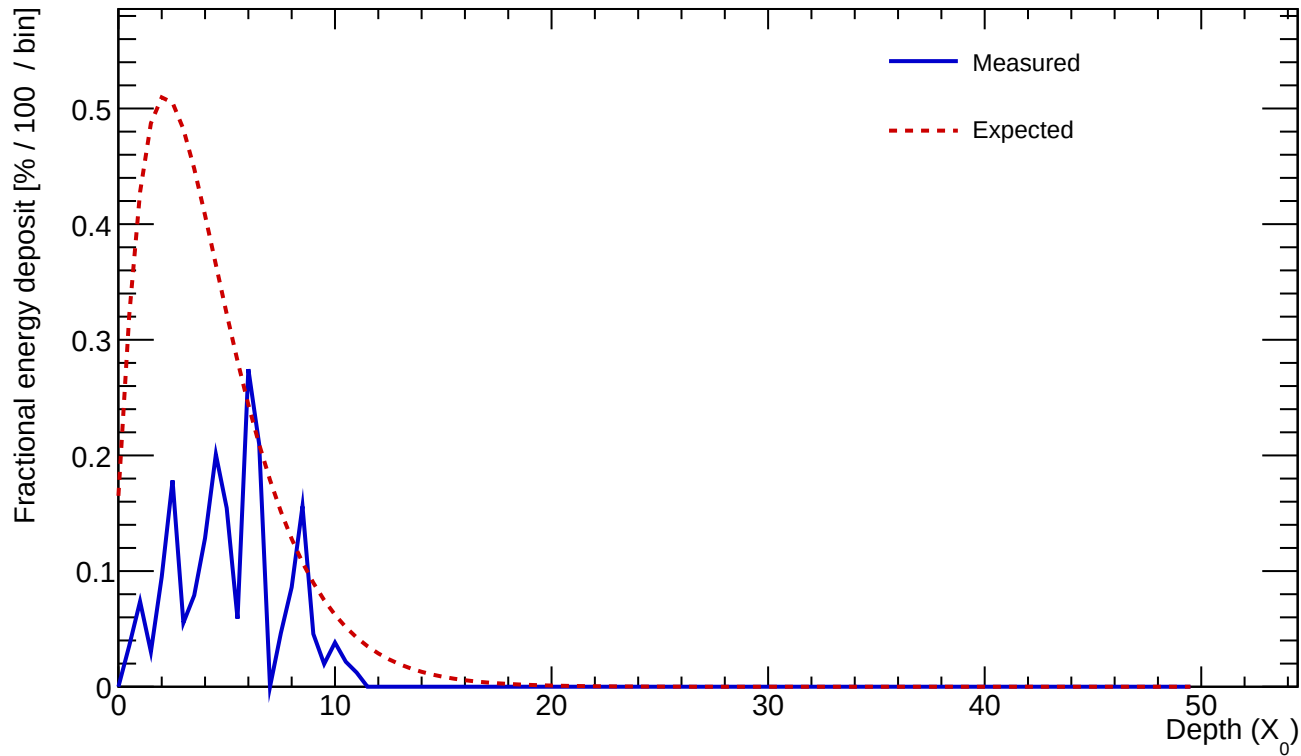
Cluster 6 E=0.682 GeV profileStart=1.50 X_0 \chi=0.5335
