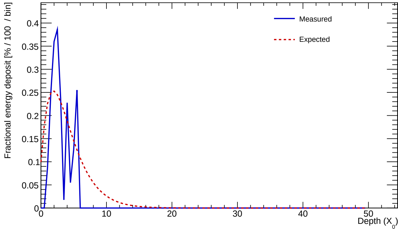
Cluster 5 E=0.536 GeV profileStart=1.00 X_0 \chi=0.4748
