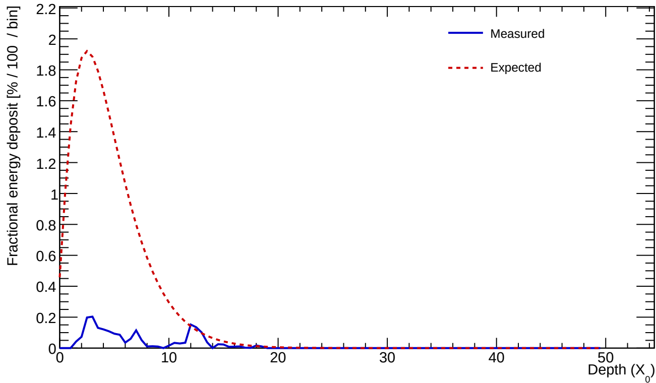
Cluster 10 E=0.971 GeV profileStart=1.50 X_0 \chi=0.6129
