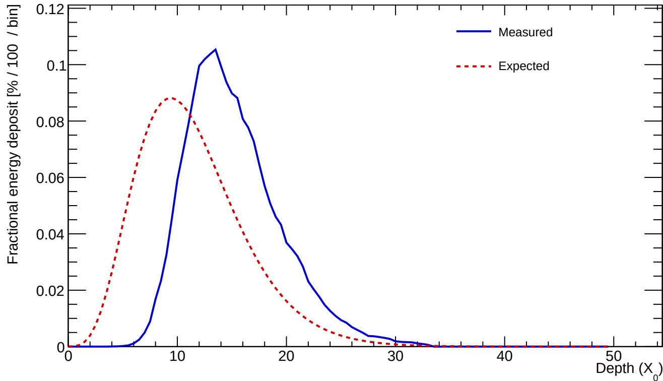
Cluster 11 E=962.911 GeV profileStart=4.00 X_0 \chi=0.1287
