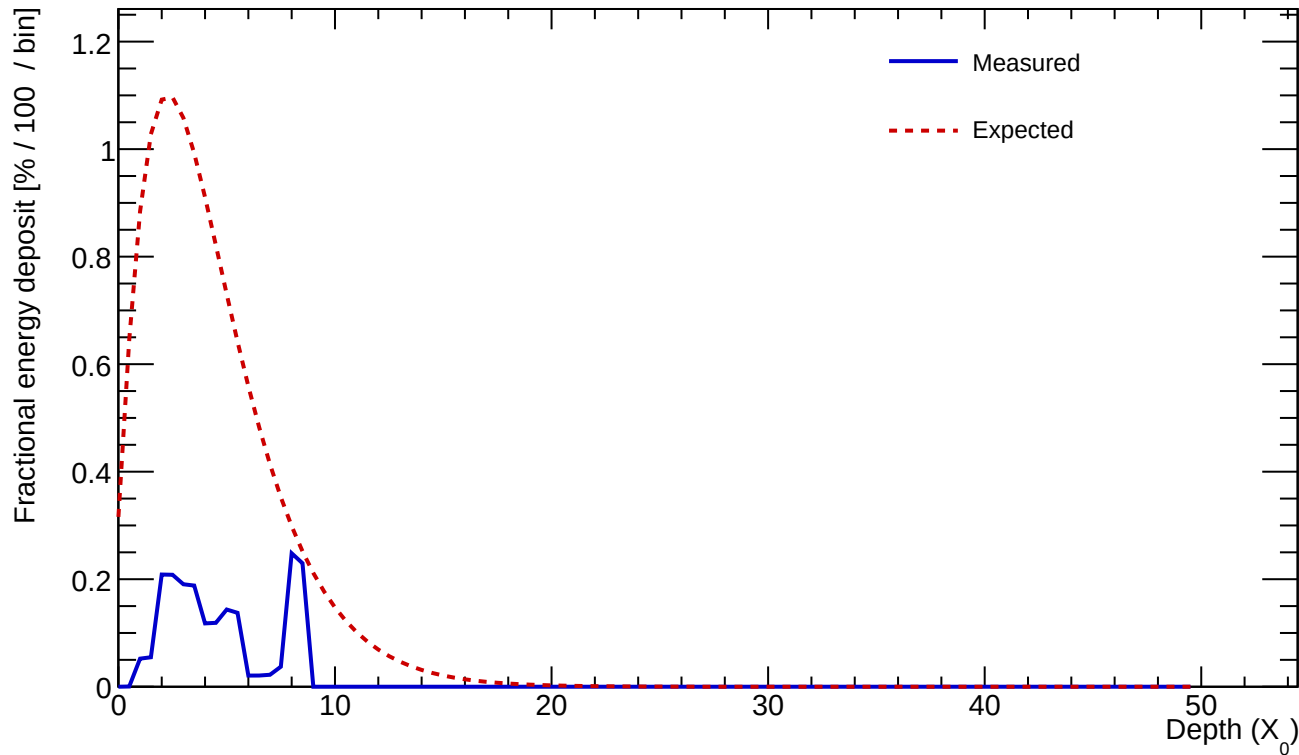
Cluster 7 E=0.785 GeV profileStart=1.00 X_0 \chi=0.3874
