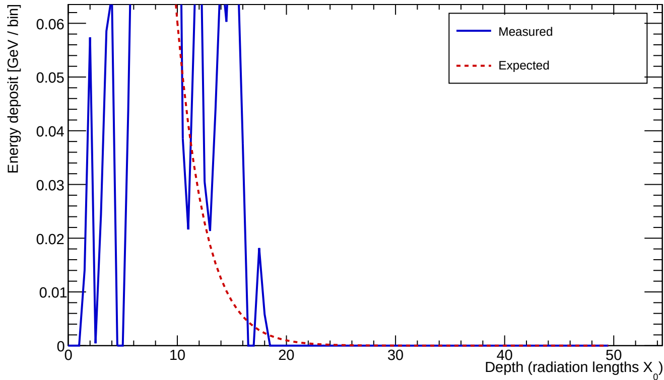
Cluster 6 E=0.678 GeV \text{profileStart}=5.50 X_0 \chi=0.4876
