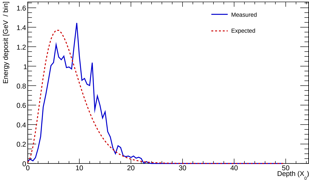
Cluster 128 E=24.960 GeV profileStart=1.00 X_0 \chi=0.1905
