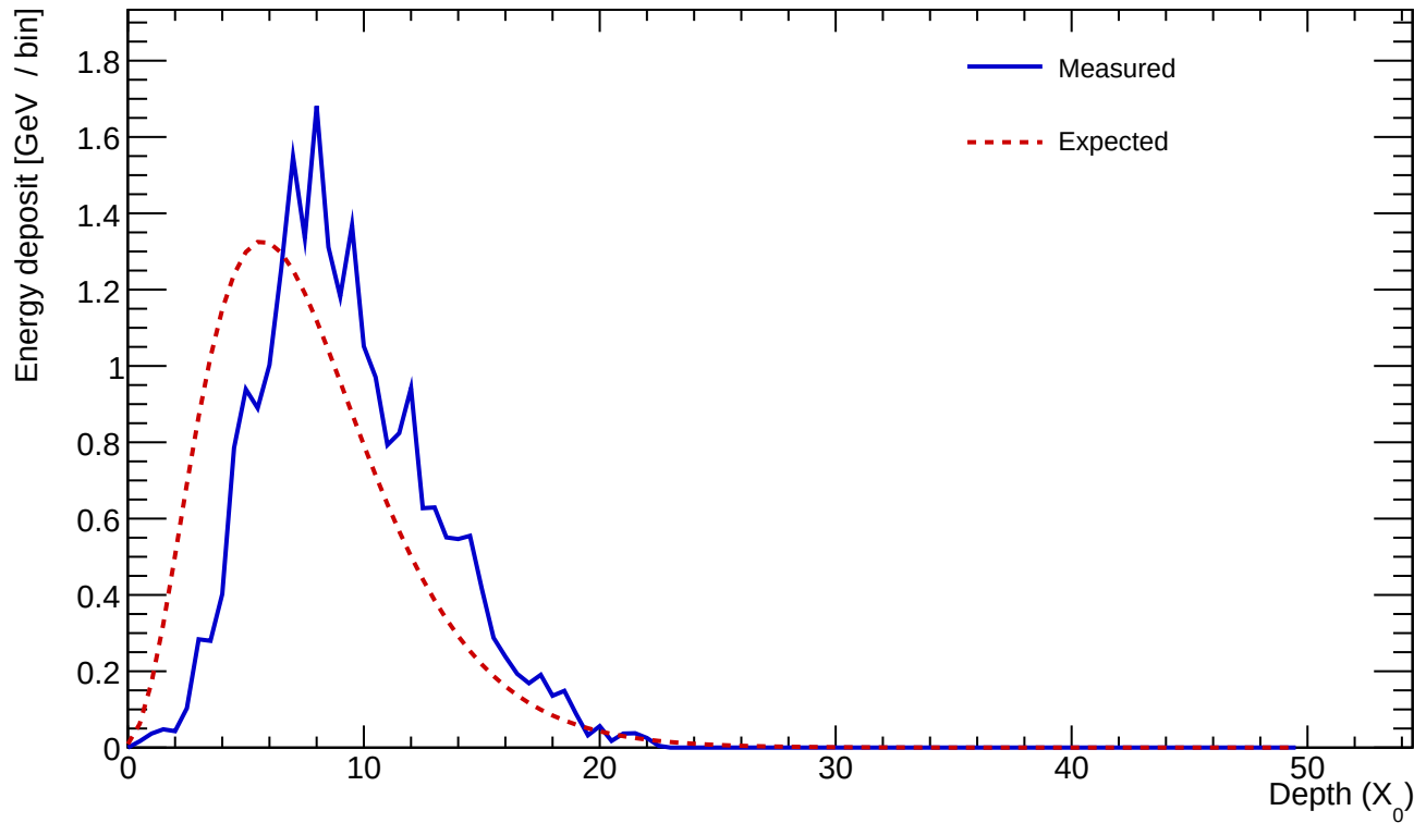
Cluster 179 E=24.078 GeV profileStart=2.00 X_0 \chi=0.1271
