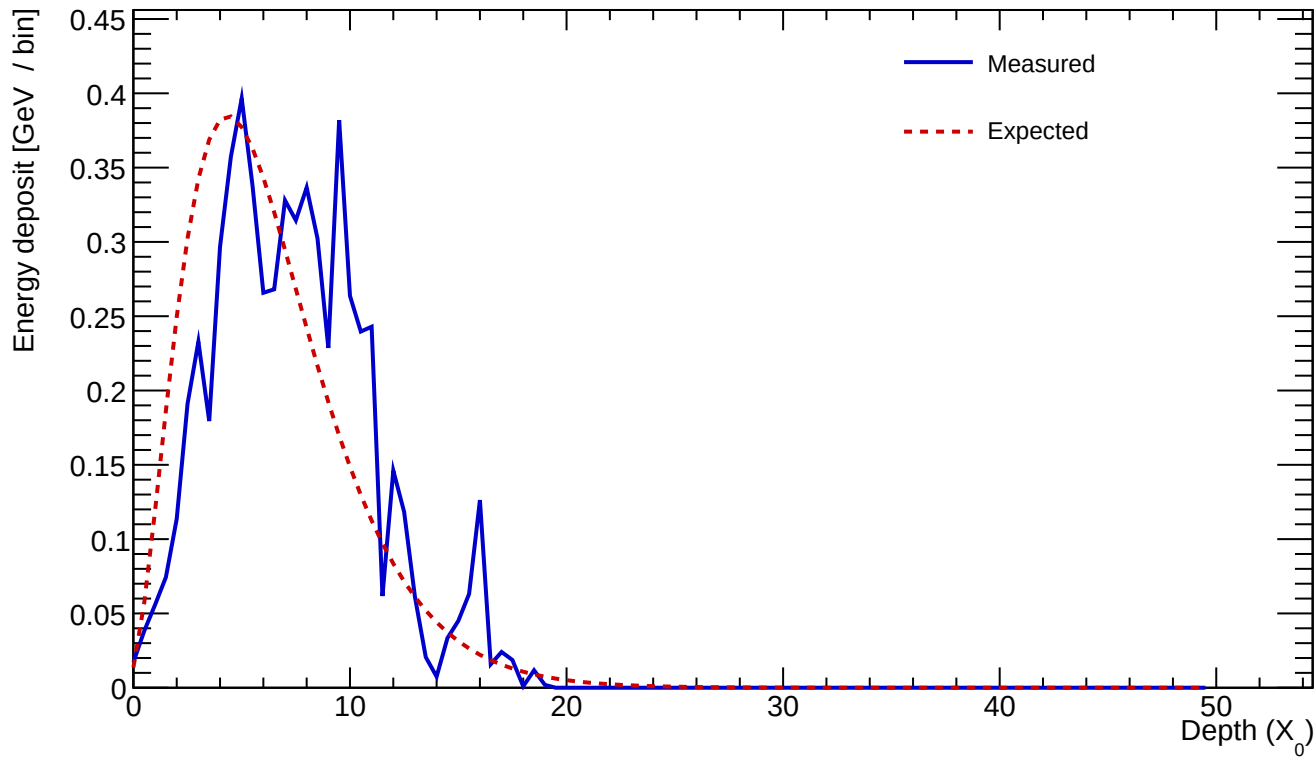
Cluster 323 E=6.220 GeV profileStart=1.00 X_0 \chi=0.2441
