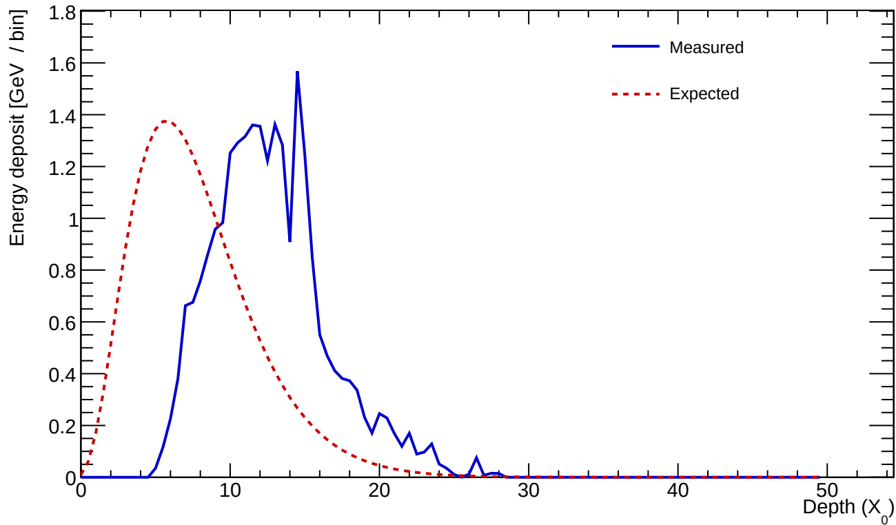
Cluster 552 E=25.066 GeV profileStart=5.00 X_0 \chi=0.1689
