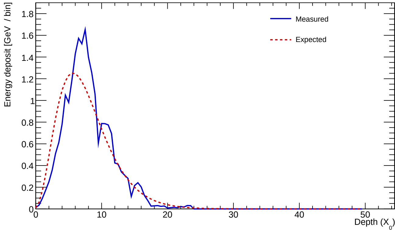
Cluster 798 E=22.610 GeV profileStart=1.00 X_0 \chi=0.1900
