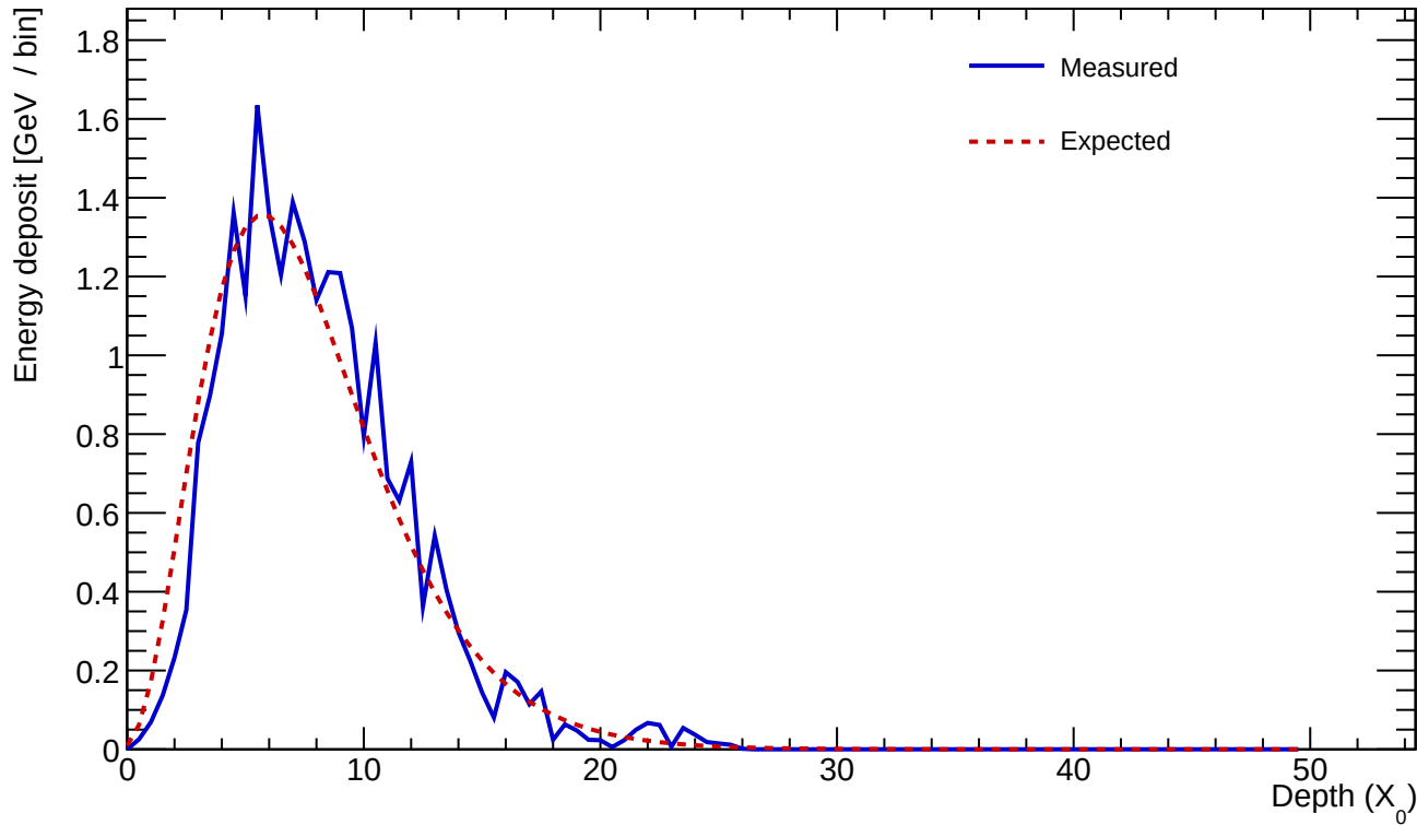
Cluster 762 E=24.656 GeV profileStart=0.50 X_0 \chi=0.1337
