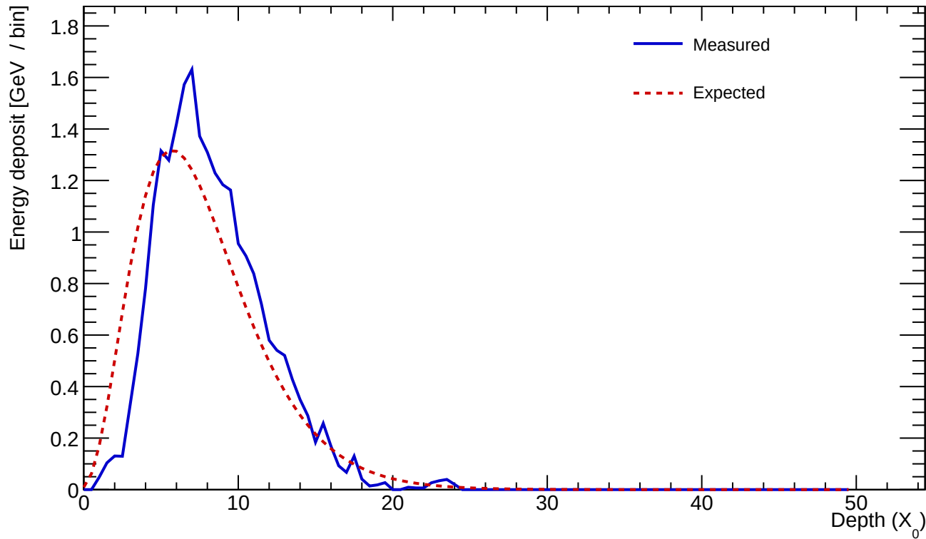
Cluster 748 E=23.899 GeV profileStart=1.00 X_0 \chi=0.1377
