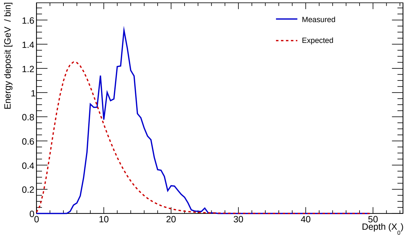
Cluster 297 E=22.642 GeV profileStart=5.50 X_0 \chi=0.1677
