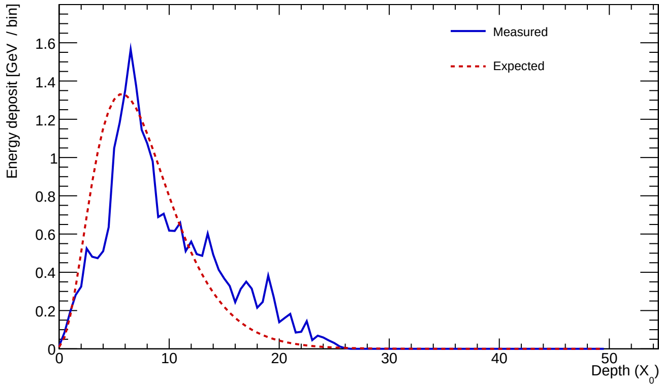
Cluster 305 E=24.189 GeV profileStart=0.50 X_0 \chi=0.2990
