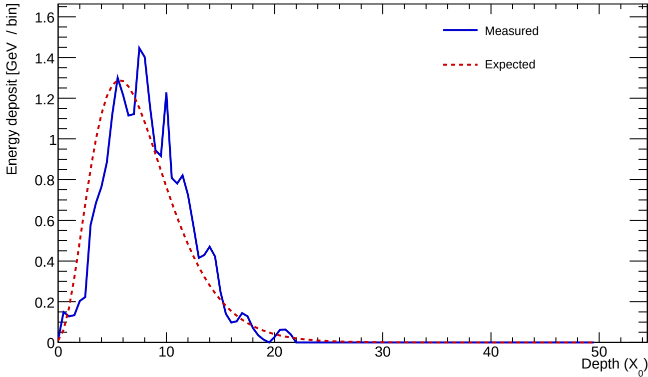
Cluster 825 E=23.344 GeV profileStart=1.00 X_0 \chi=0.1455
