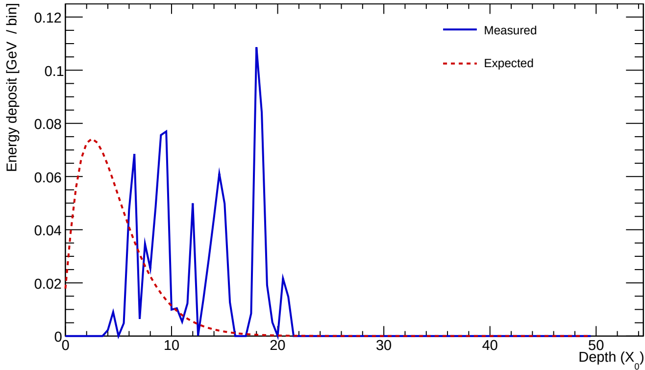
Cluster 105 E=0.961 GeV profileStart=5.50 X_0 \chi=0.8540
