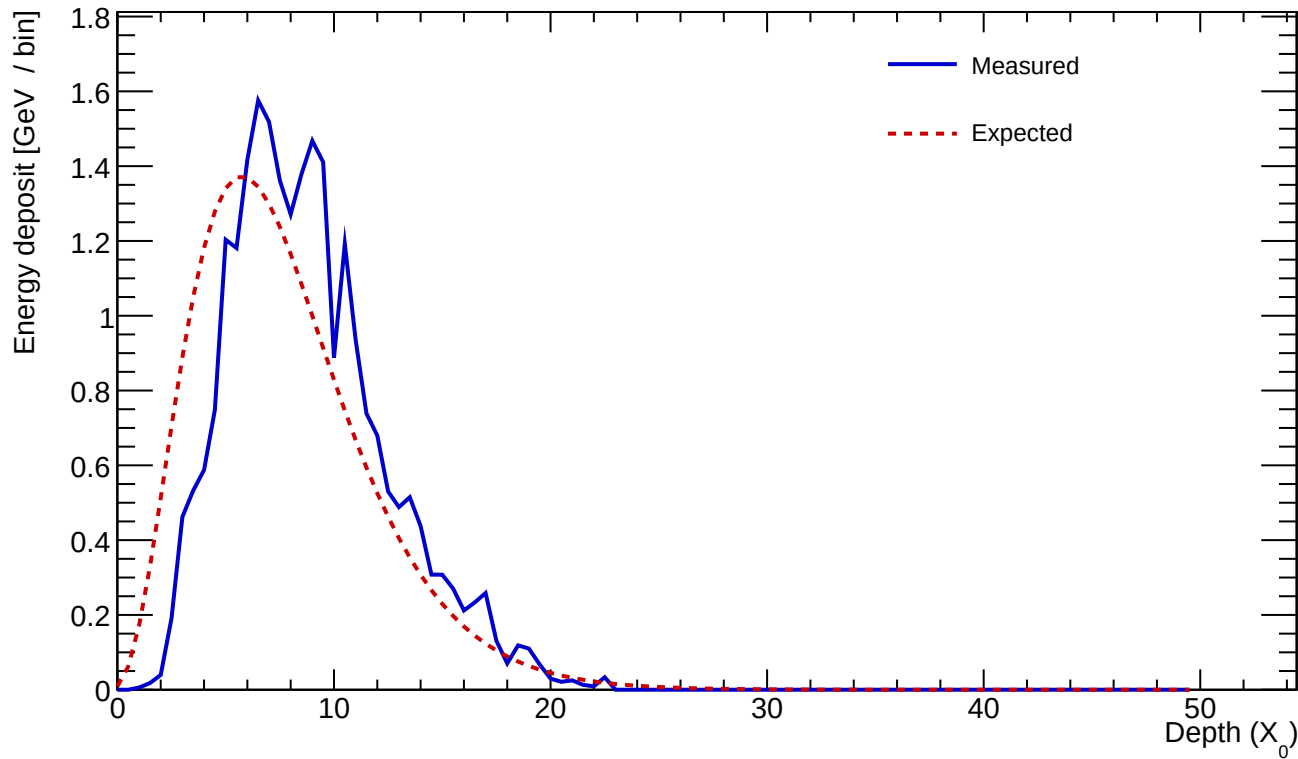
Cluster 367 E=24.993 GeV profileStart=1.50 X_0 \chi=0.1301
