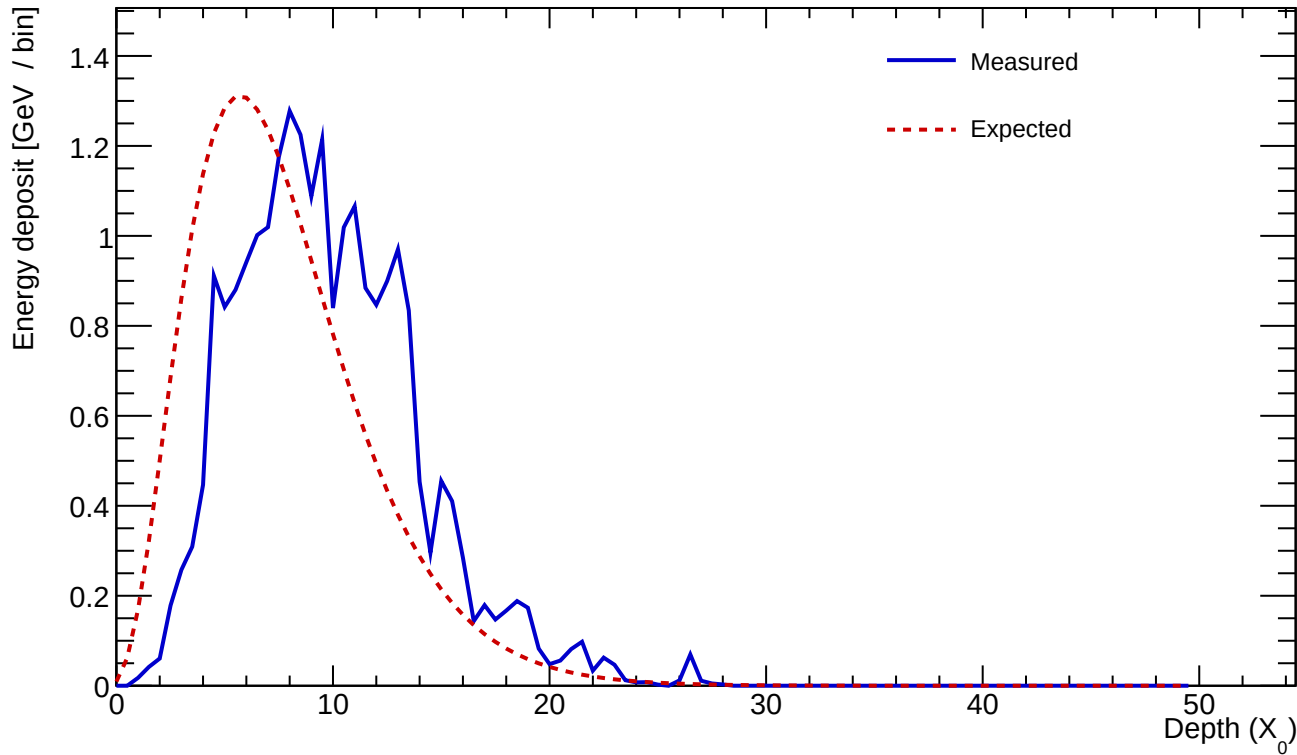
Cluster 532 E=23.783 GeV profileStart=2.00 X_0 \chi=0.1722
