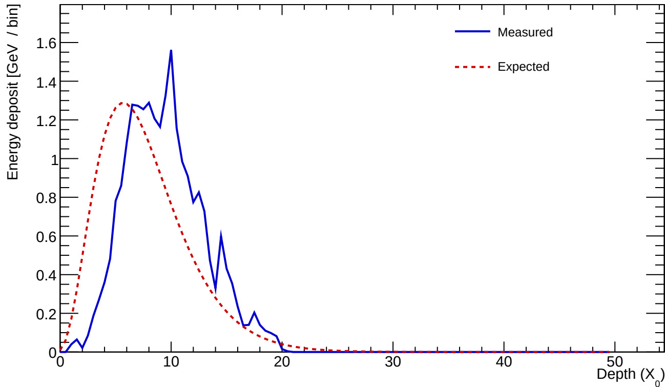
Cluster 332 E=23.317 GeV profileStart=2.50 X_0 \chi=0.1262
