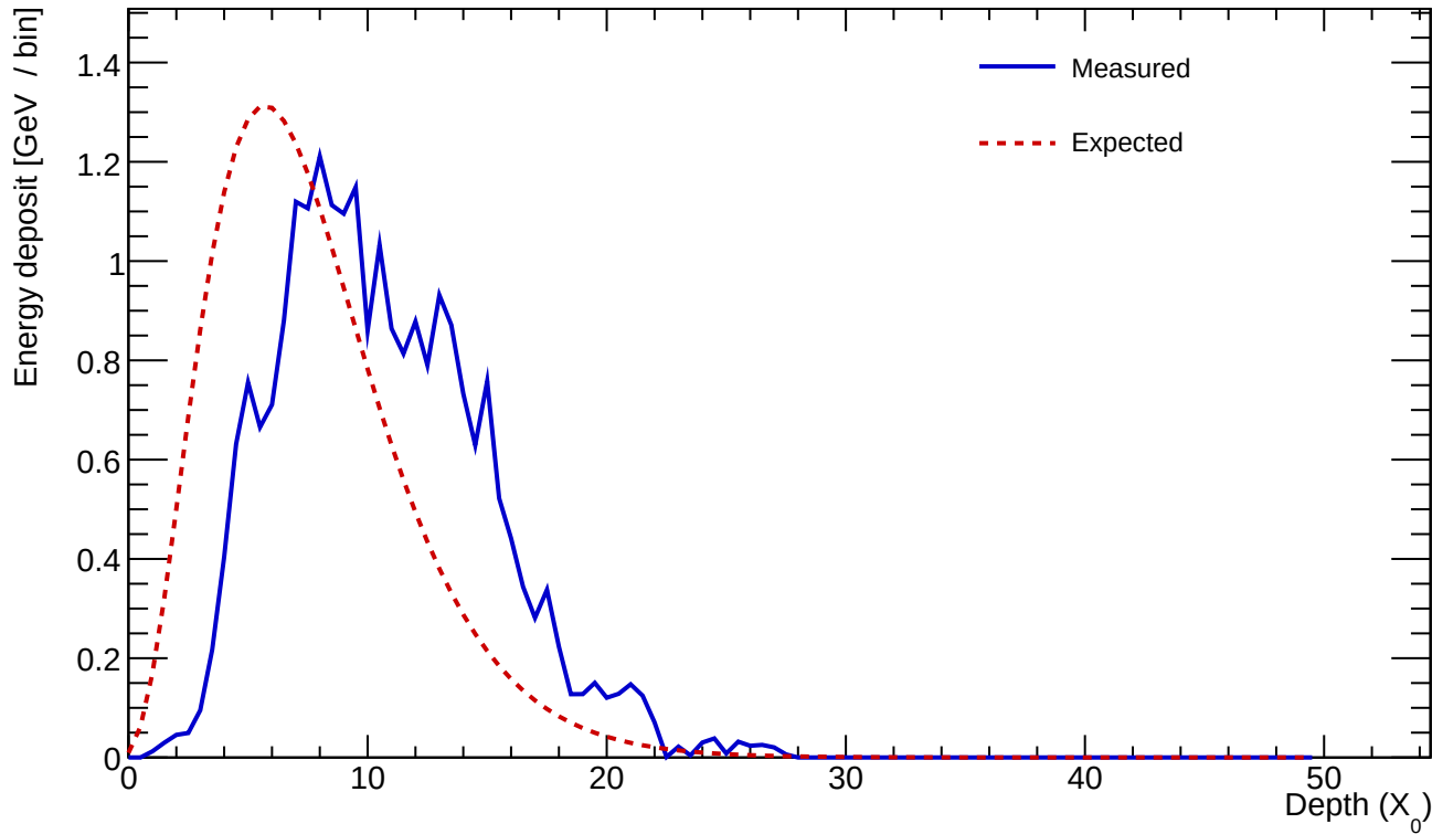
Cluster 841 E=23.811 GeV profileStart=3.00 X_0 \chi=0.2026
