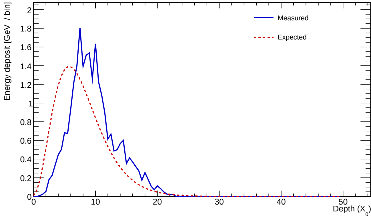
Cluster 740 E=25.315 GeV profileStart=2.50 X_0 \chi=0.1629
