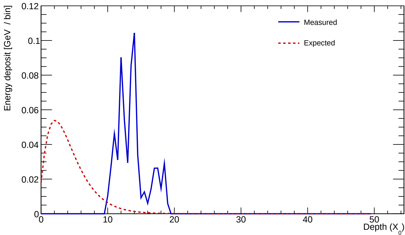
Cluster 240 E=0.657 GeV profileStart=10.00 X_0 \chi=0.4631
