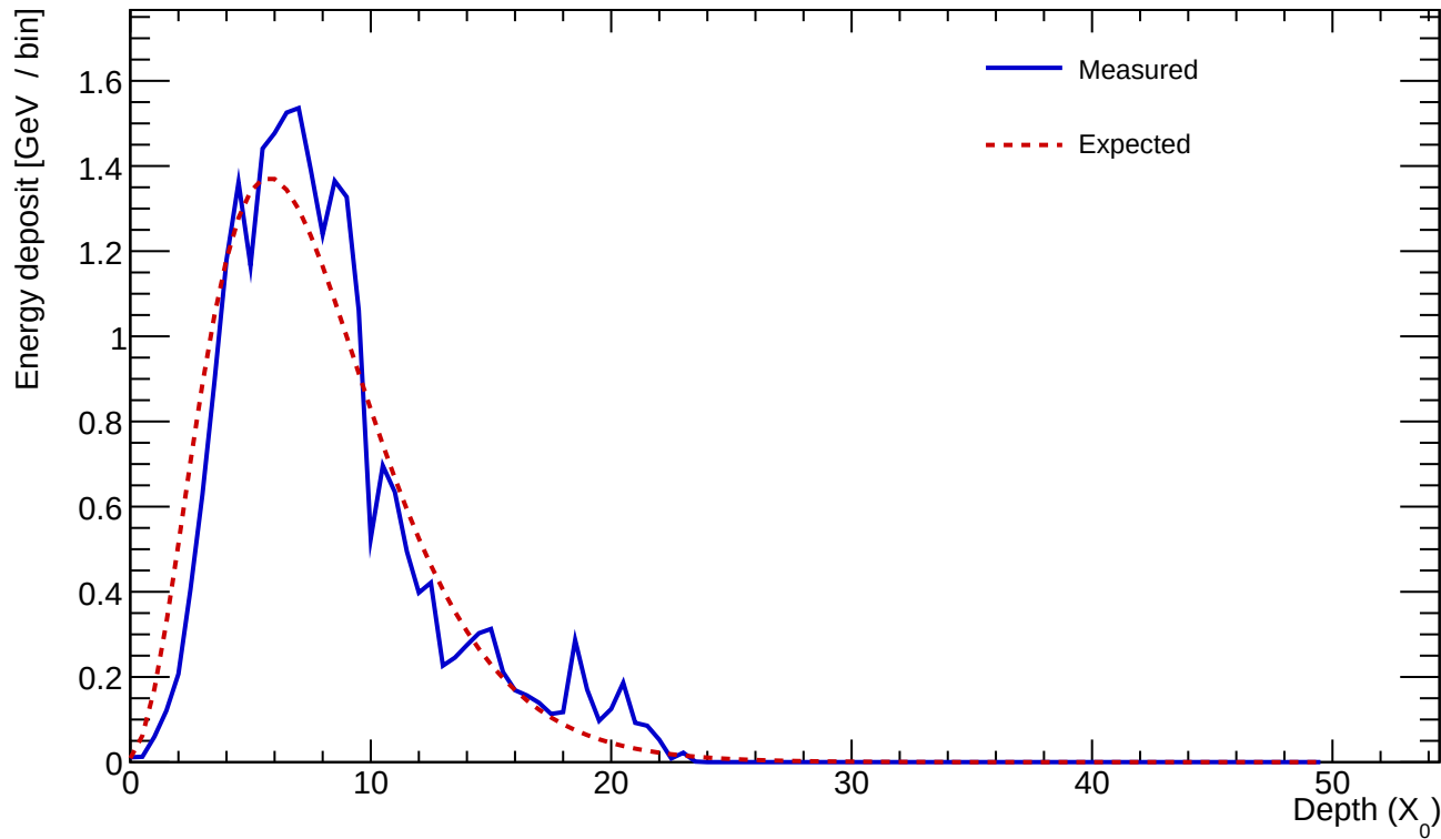
Cluster 490 E=24.979 GeV profileStart=0.50 X_0 \chi=0.1747
