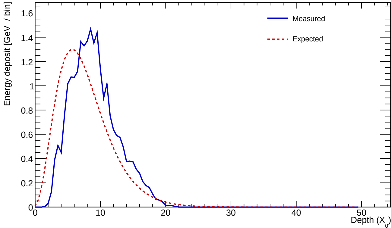
Cluster 342 E=23.550 GeV profileStart=1.50 X_0 \chi=0.1173
