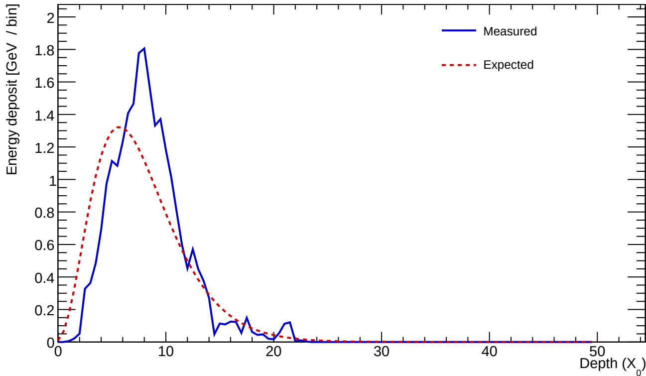
Cluster 589 E=24.009 GeV profileStart=1.50 X_0 \chi=0.2199
