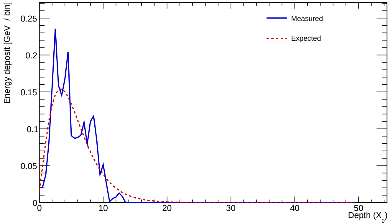
Cluster 231 E=2.234 GeV profileStart=0.50 X_0 \chi=0.2939
