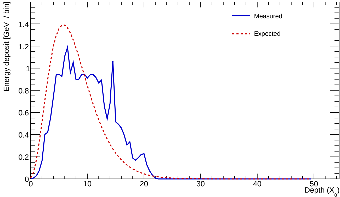
Cluster 19 E=25.346 GeV profileStart=1.50 X_0 \chi=0.2627
