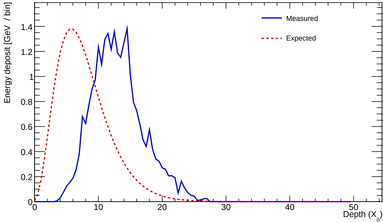
Cluster 59 E=25.138 GeV profileStart=5.50 X_0 \chi=0.1399
