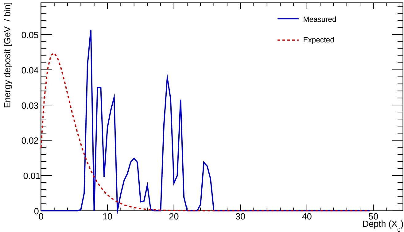
Cluster 225 E=0.526 GeV profileStart=6.00 X_0 \chi=0.7729
