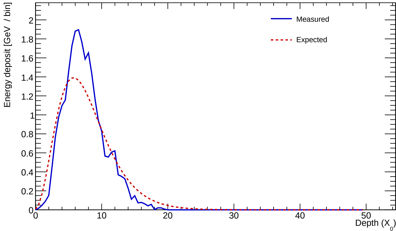
Cluster 388 E=25.351 GeV profileStart=0.50 X_0 \chi=0.2302
