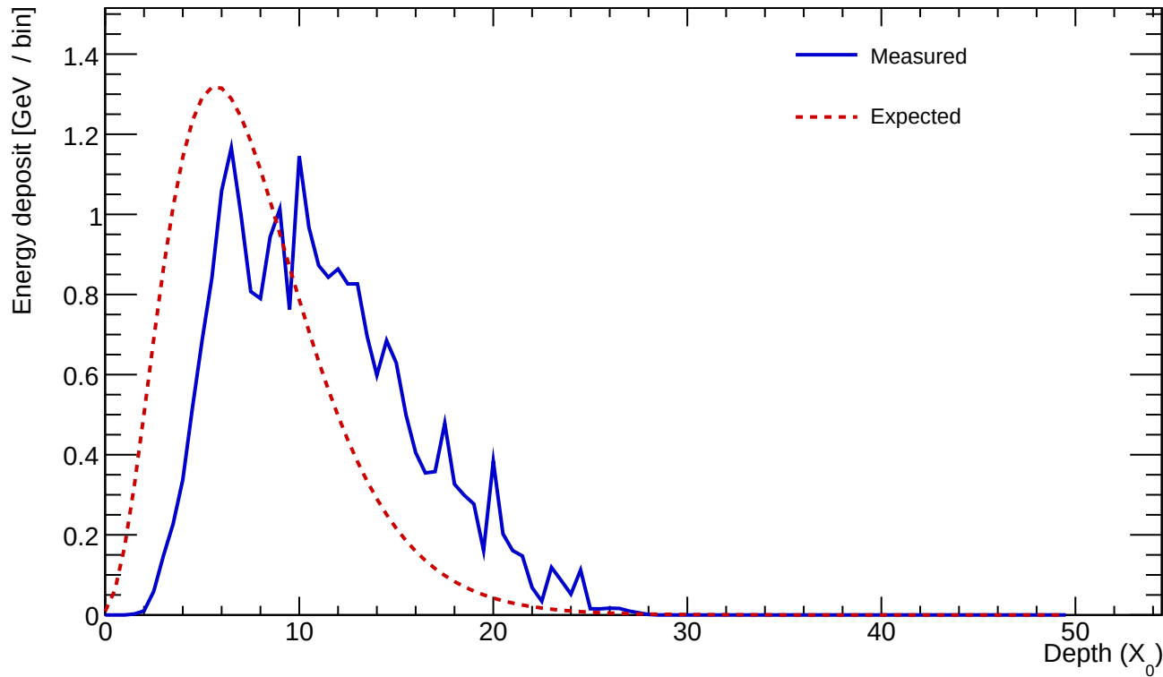
Cluster 248 E=23.929 GeV profileStart=2.50 X_0 \chi=0.2408
