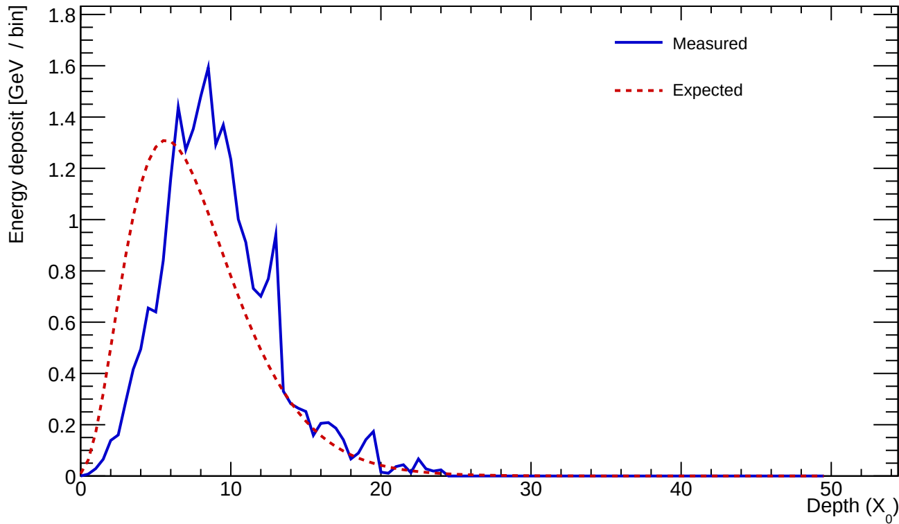
Cluster 292 E=23.741 GeV profileStart=2.00 X_0 \chi=0.1831
