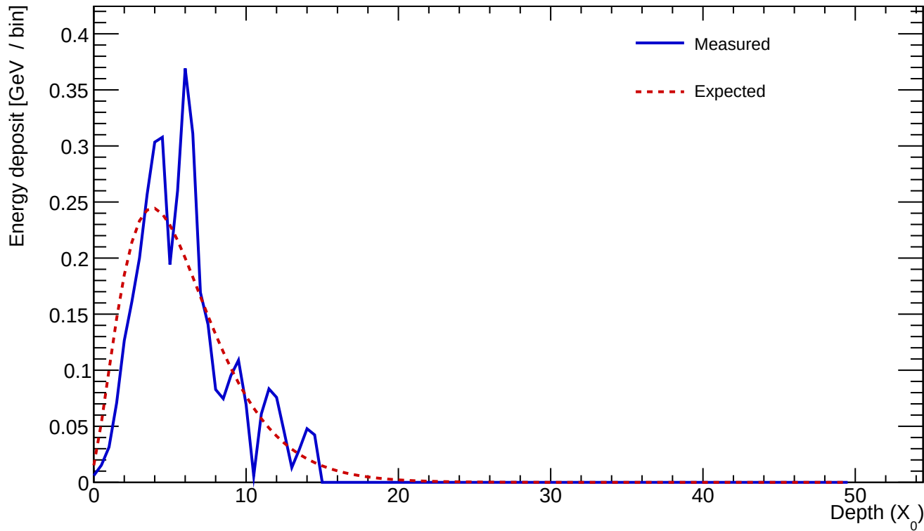
Cluster 800 E=3.759 GeV profileStart=0.50 X_0 \chi=0.2635
