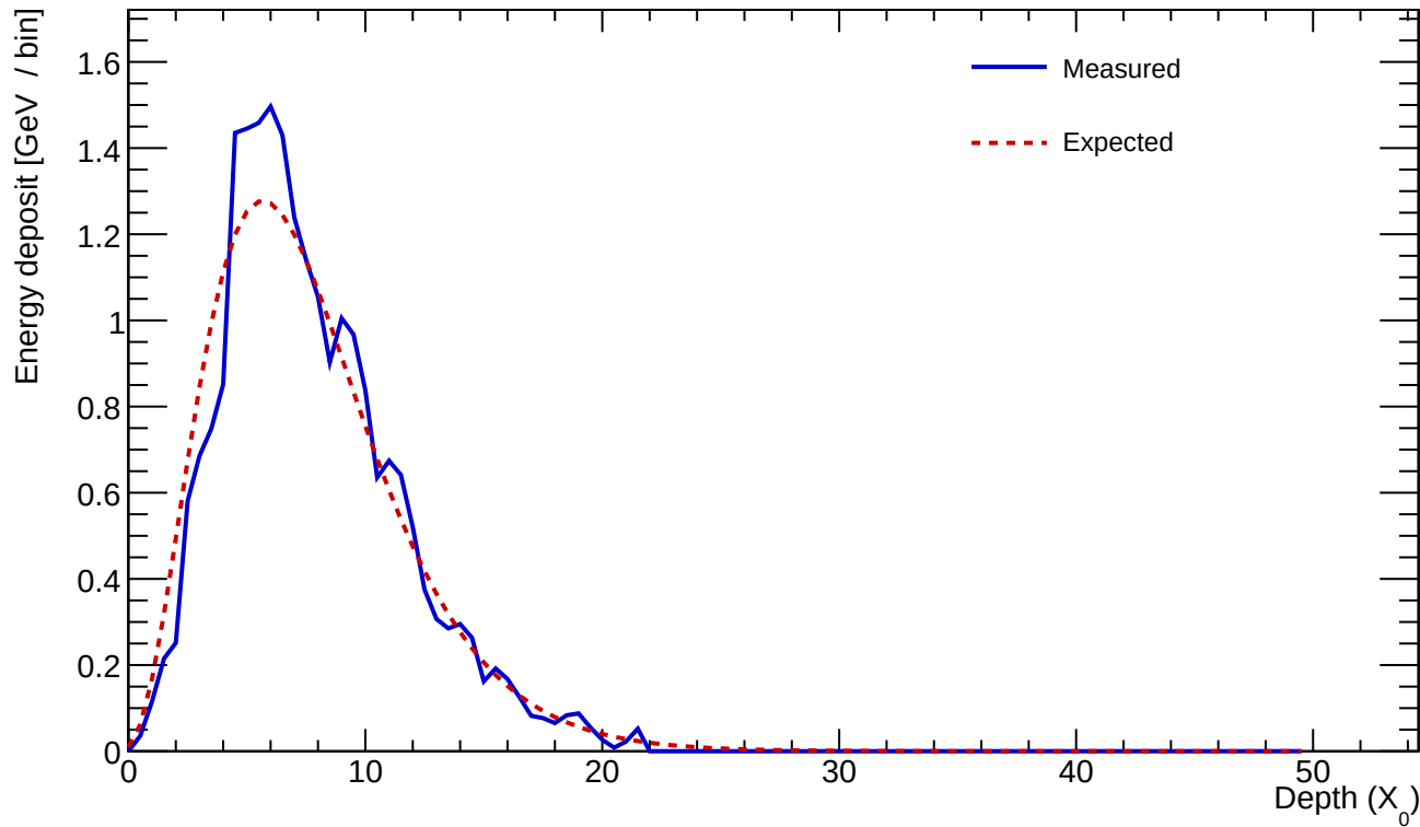
Cluster 160 E=23.103 GeV profileStart=0.50 X_0 \chi=0.1254
