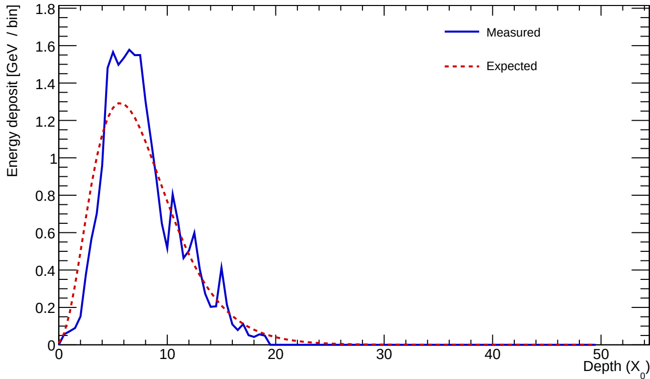
Cluster 616 E=23.420 GeV profileStart=0.50 X_0 \chi=0.2090
