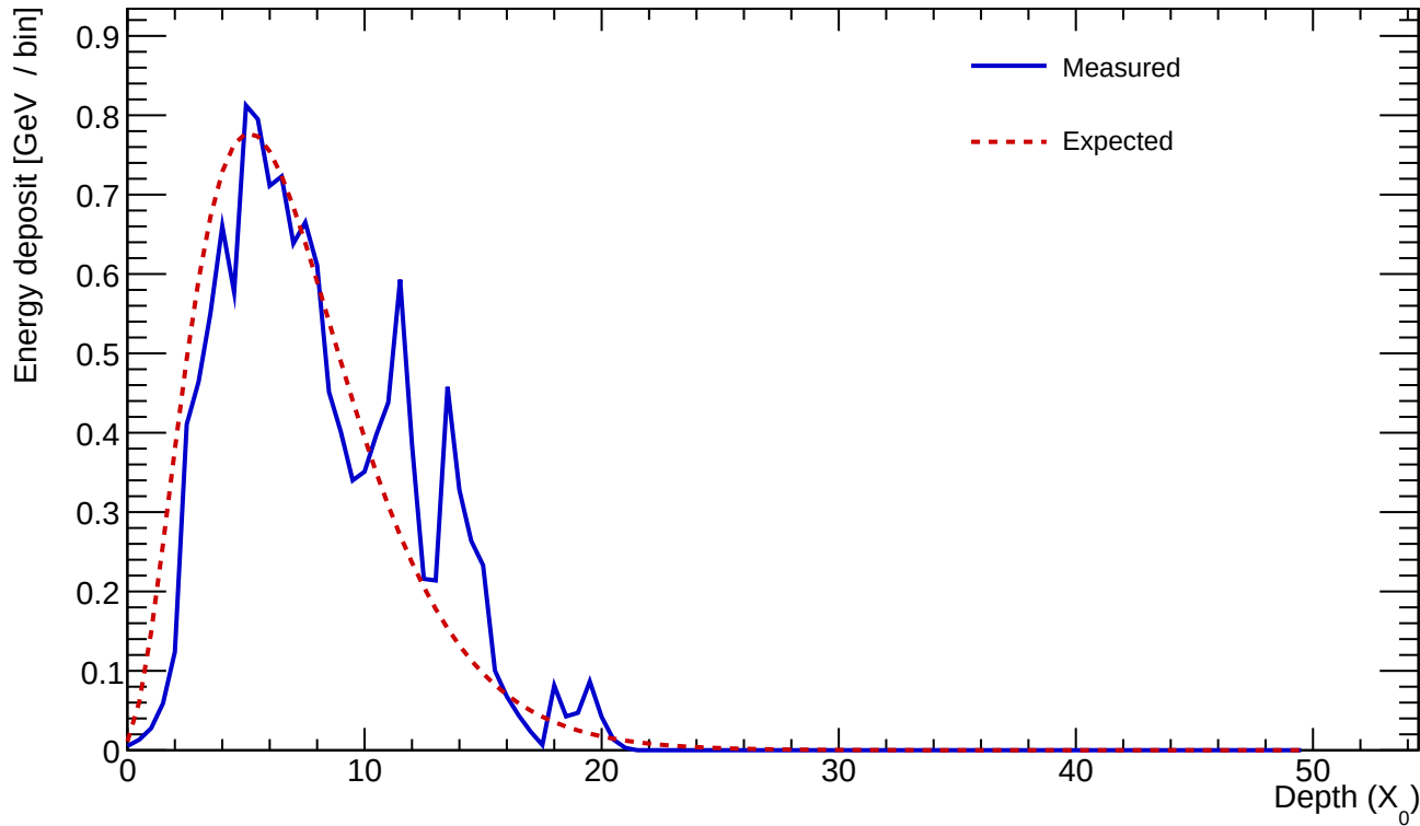
Cluster 382 E=13.476 GeV profileStart=0.50 X_0 \chi=0.2110
