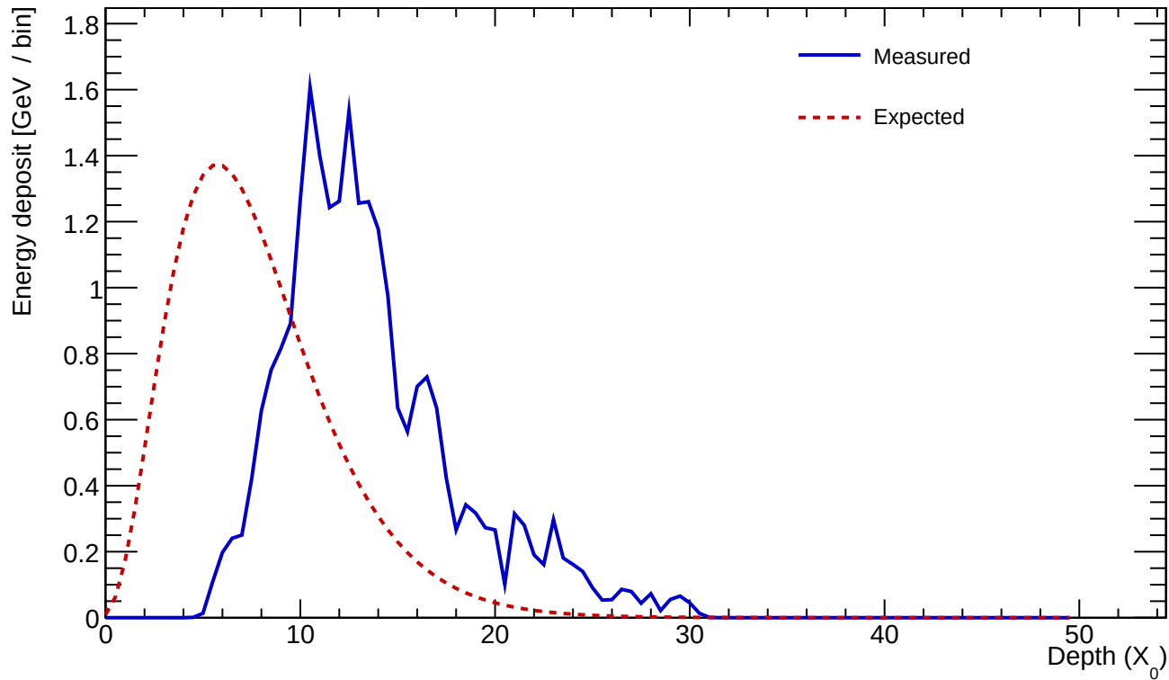
Cluster 392 E=24.986 GeV profileStart=5.50 X_0 \chi=0.1850
