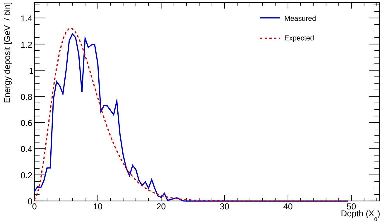
Cluster 804 E=23.967 GeV profileStart=1.00 X_0 \chi=0.1595
