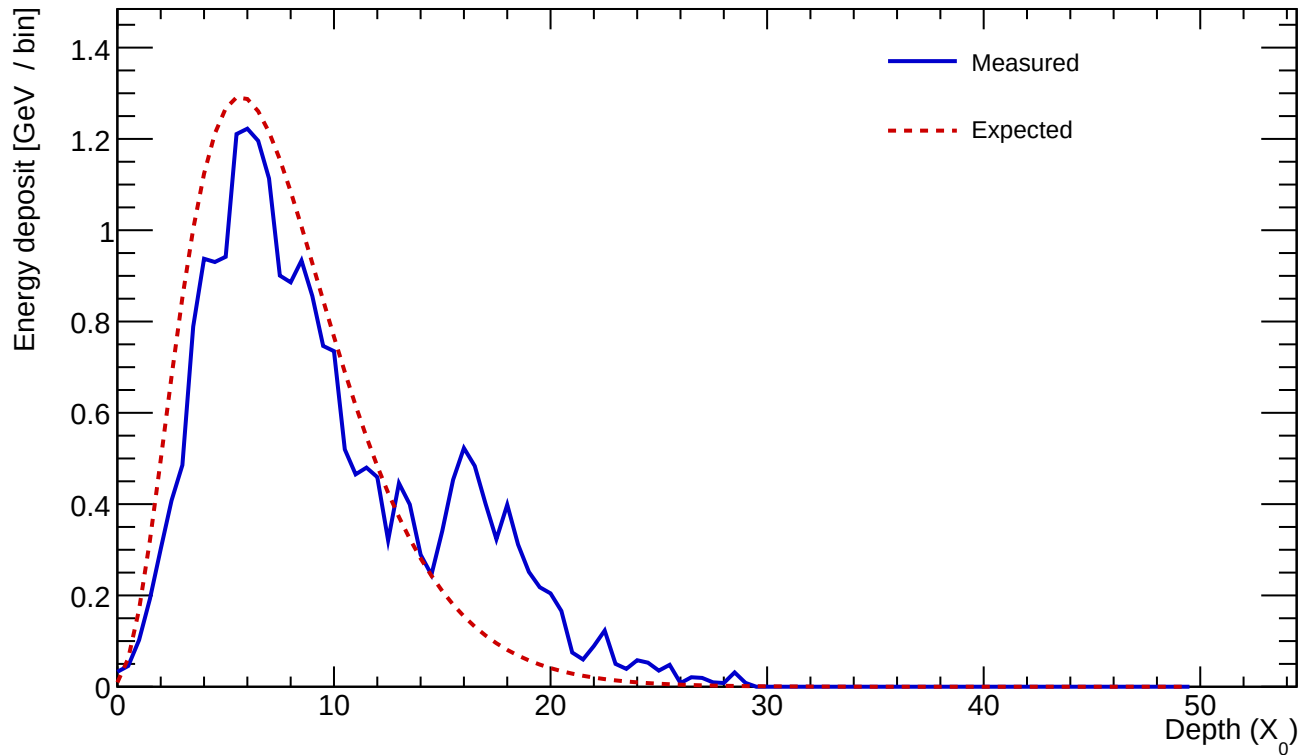
Cluster 732 E=23.401 GeV profileStart=0.50 X_0 \chi=0.2876
