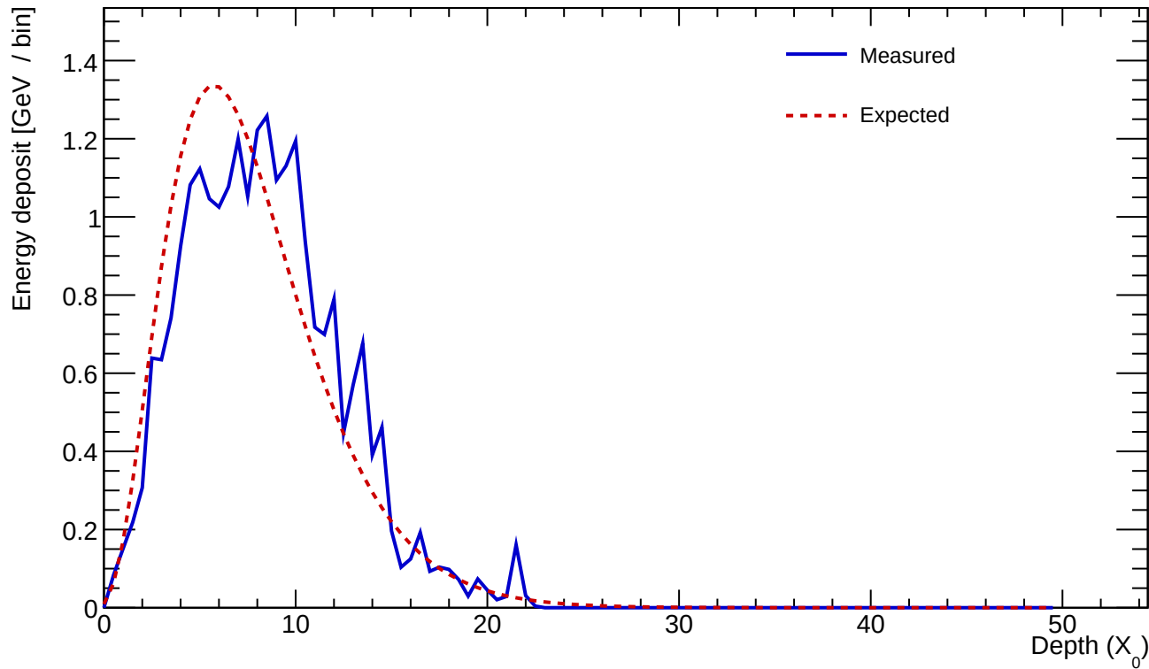
Cluster 629 E=24.272 GeV profileStart=1.00 X_0 \chi=0.1774
