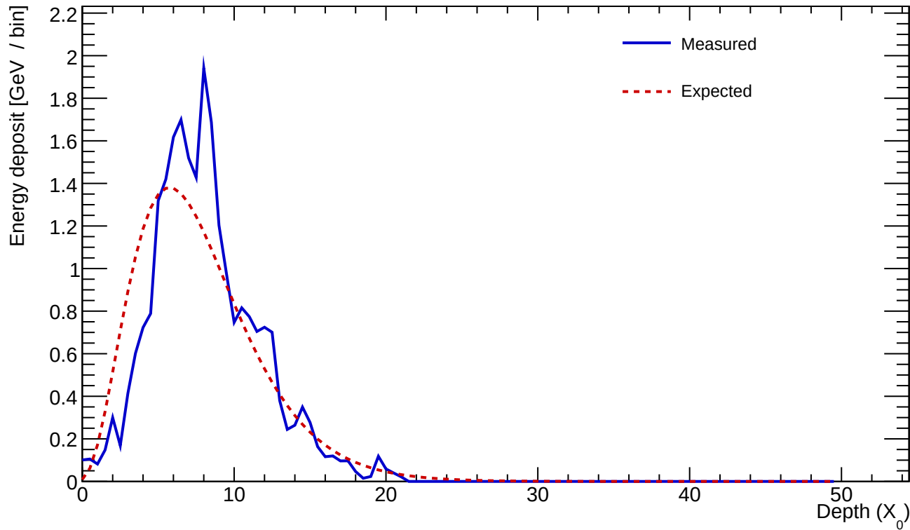
Cluster 60 E=25.134 GeV profileStart=1.00 X_0 \chi=0.2186
