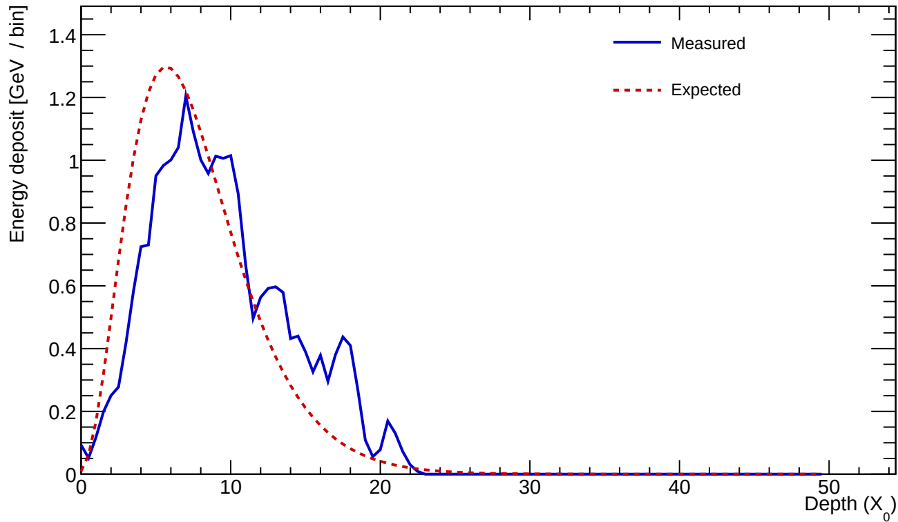
Cluster 90 E=23.507 GeV profileStart=1.50 X_0 \chi=0.2204
