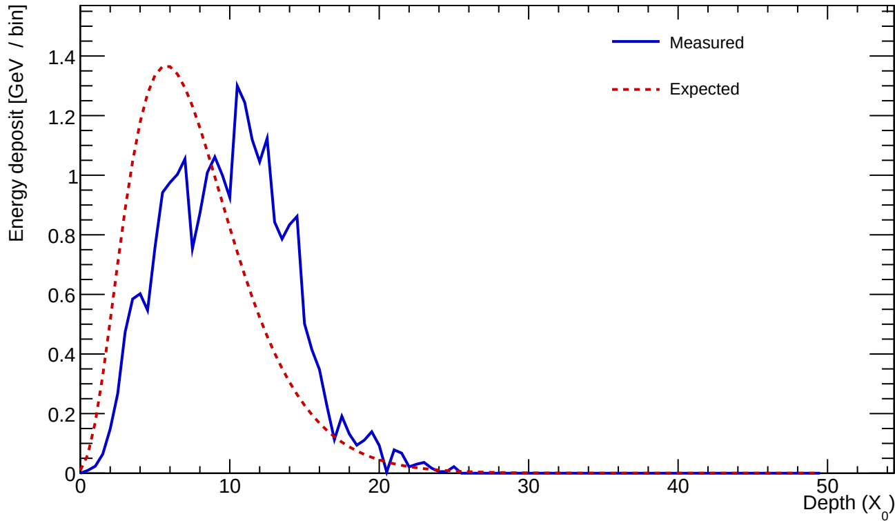
Cluster 524 E=24.880 GeV profileStart=2.50 X_0 \chi=0.2777
