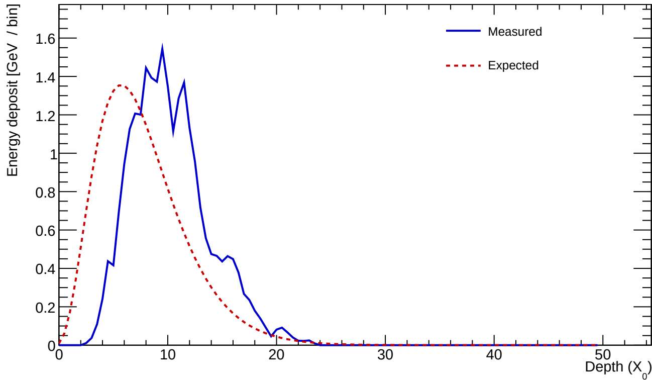
Cluster 620 E=24.646 GeV profileStart=3.00 X_0 \chi=0.1258
