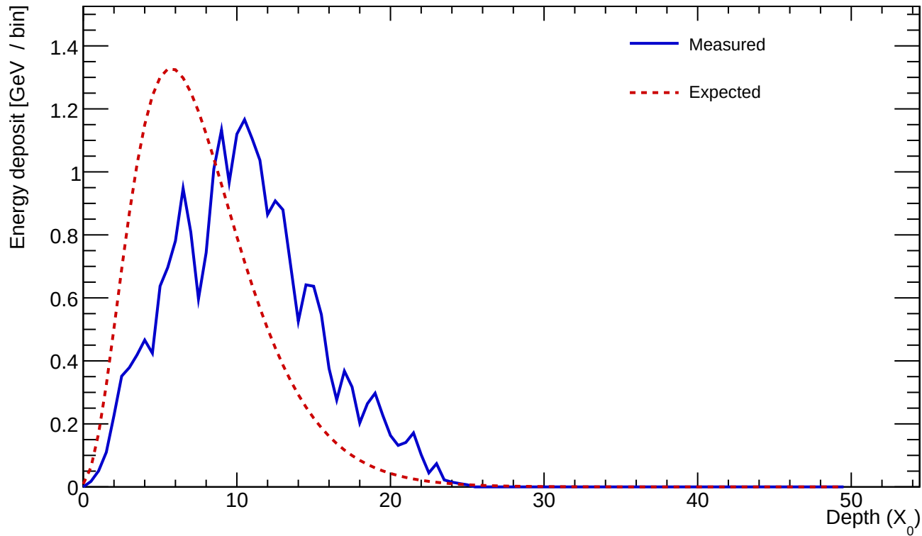
Cluster 477 E=24.111 GeV profileStart=3.00 X_0 \chi=0.2606
