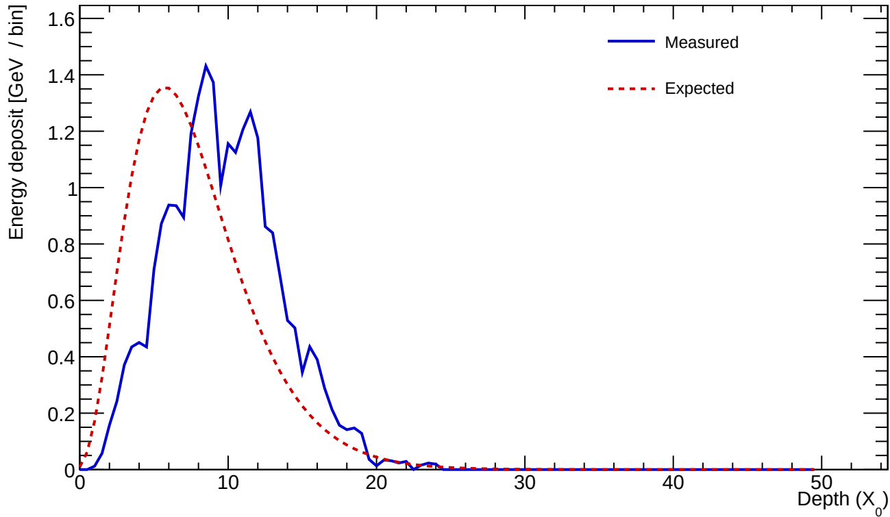
Cluster 405 E=24.658 GeV profileStart=2.50 X_0 \chi=0.1769
