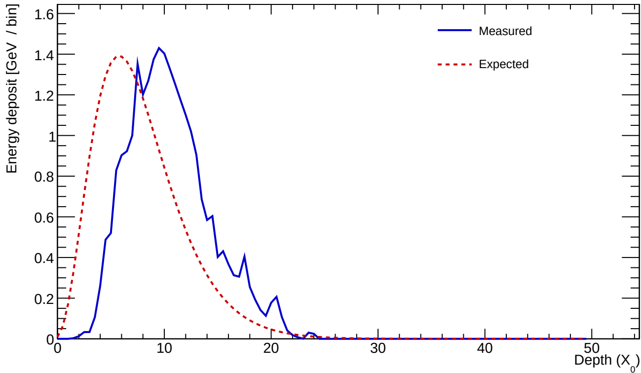
Cluster 813 E=25.345 GeV profileStart=3.00 X_0 \chi=0.1107
