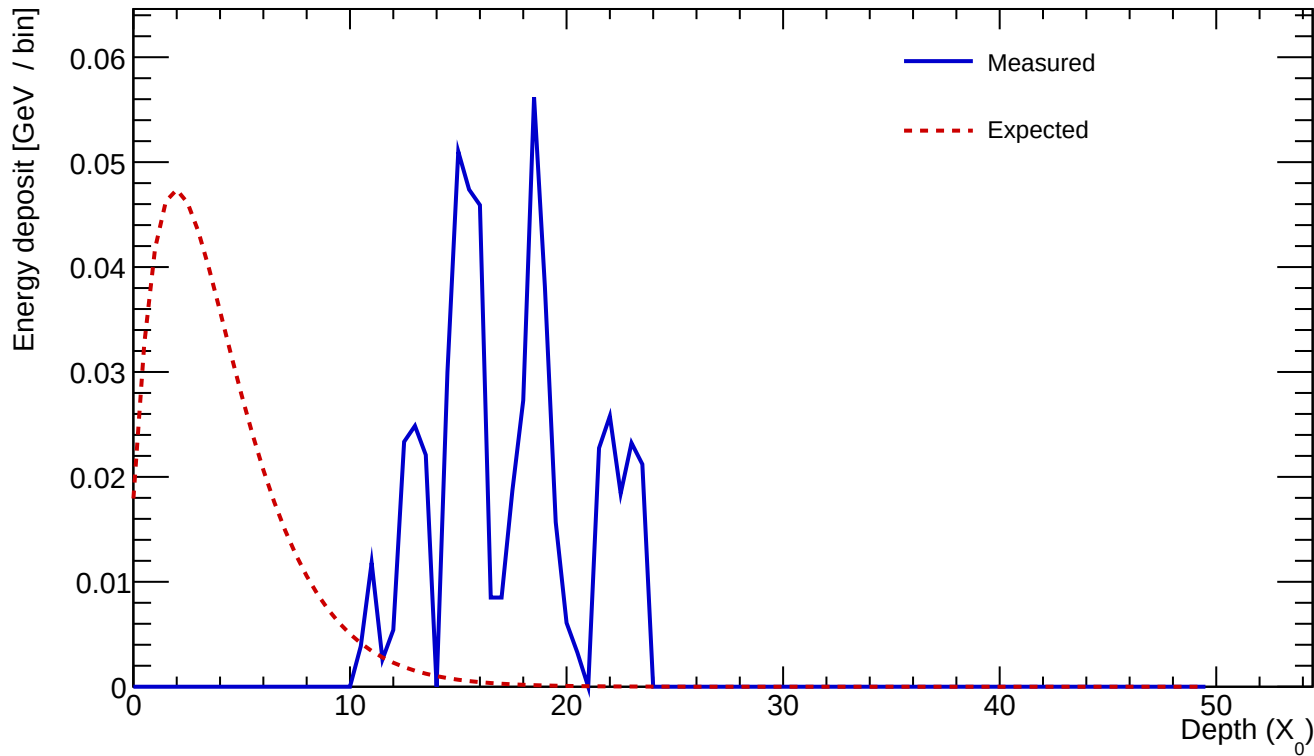
Cluster 582 E=0.562 GeV profileStart=12.50 X_0 \chi=0.6139
