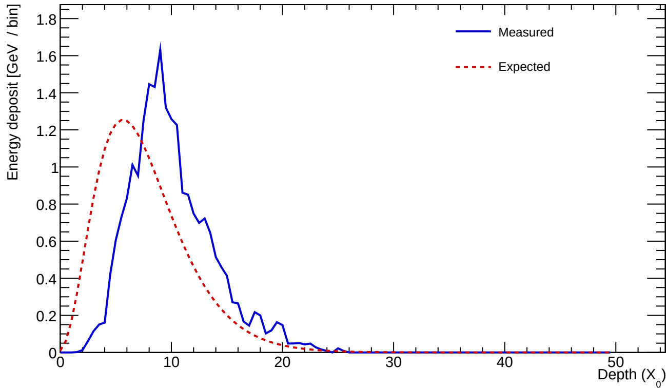
Cluster 882 E=22.651 GeV profileStart=2.50 X_0 \chi=0.1458
