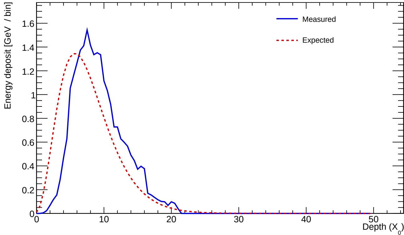
Cluster 434 E=24.458 GeV profileStart=2.00 X_0 \chi=0.1021
