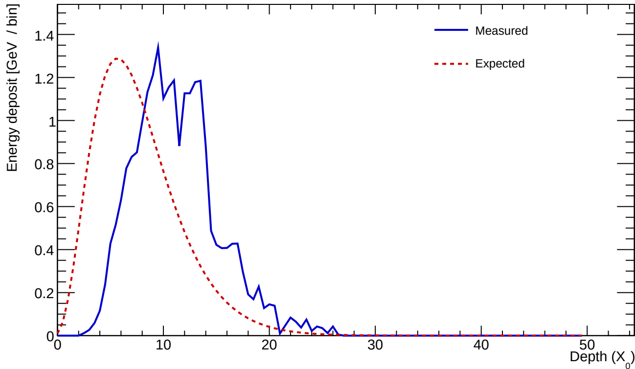
Cluster 543 E=23.334 GeV profileStart=3.50 X_0 \chi=0.1747
