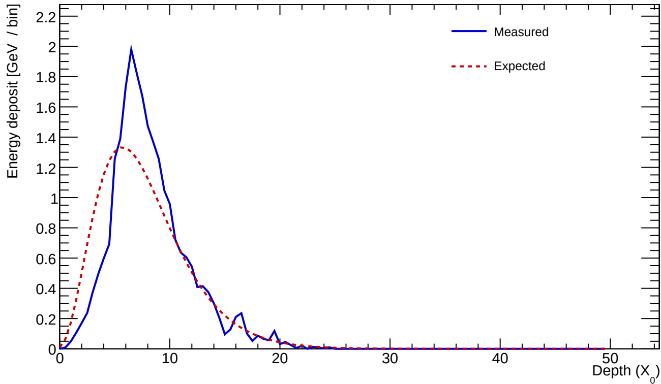
Cluster 75 E=24.204 GeV profileStart=1.00 X_0 \chi=0.2360
