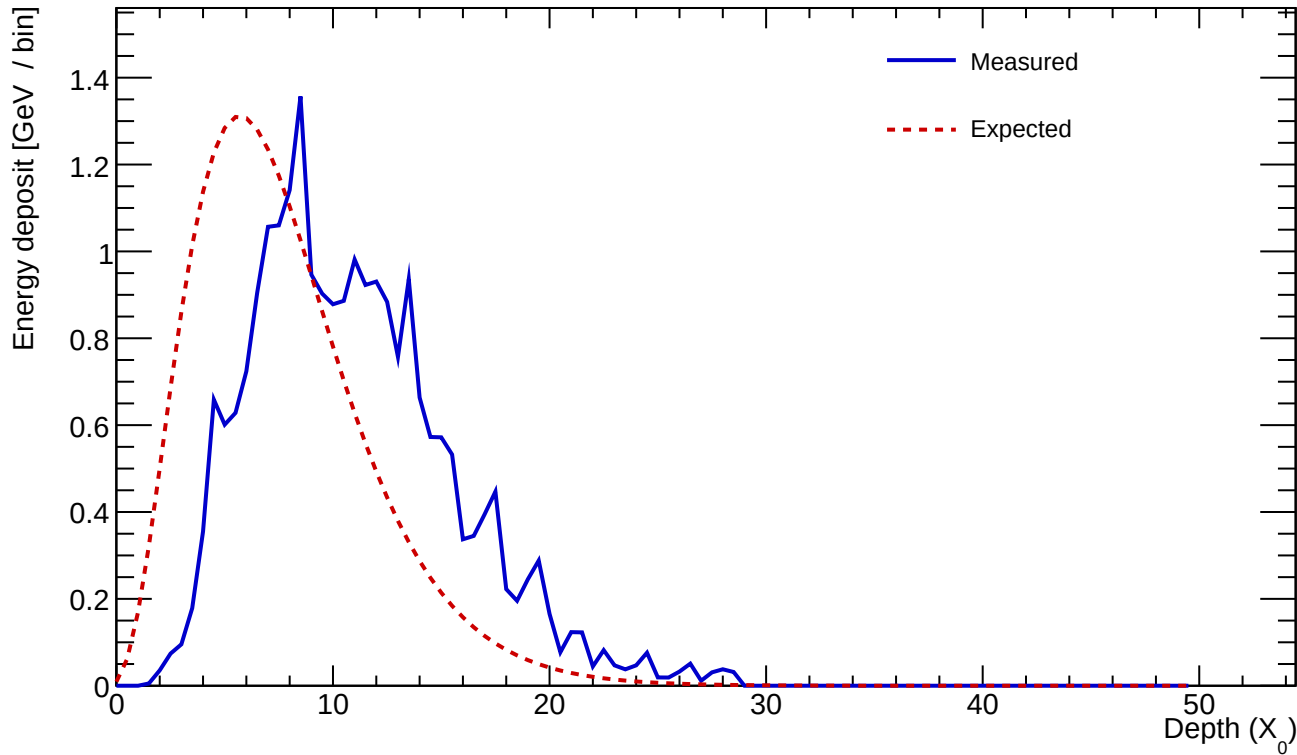
Cluster 331 E=23.772 GeV profileStart=3.00 X_0 \chi=0.2035
