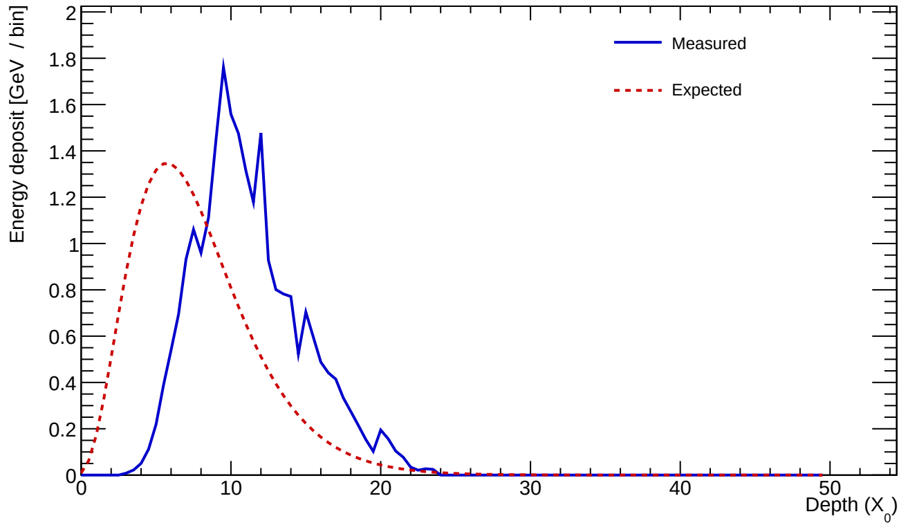
Cluster 64 E=24.479 GeV profileStart=4.00 X_0 \chi=0.1337
