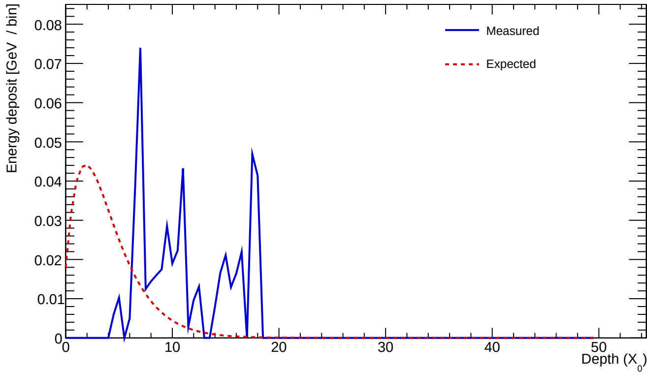
Cluster 839 E=0.517 GeV profileStart=6.00 X_0 \chi=0.7546
