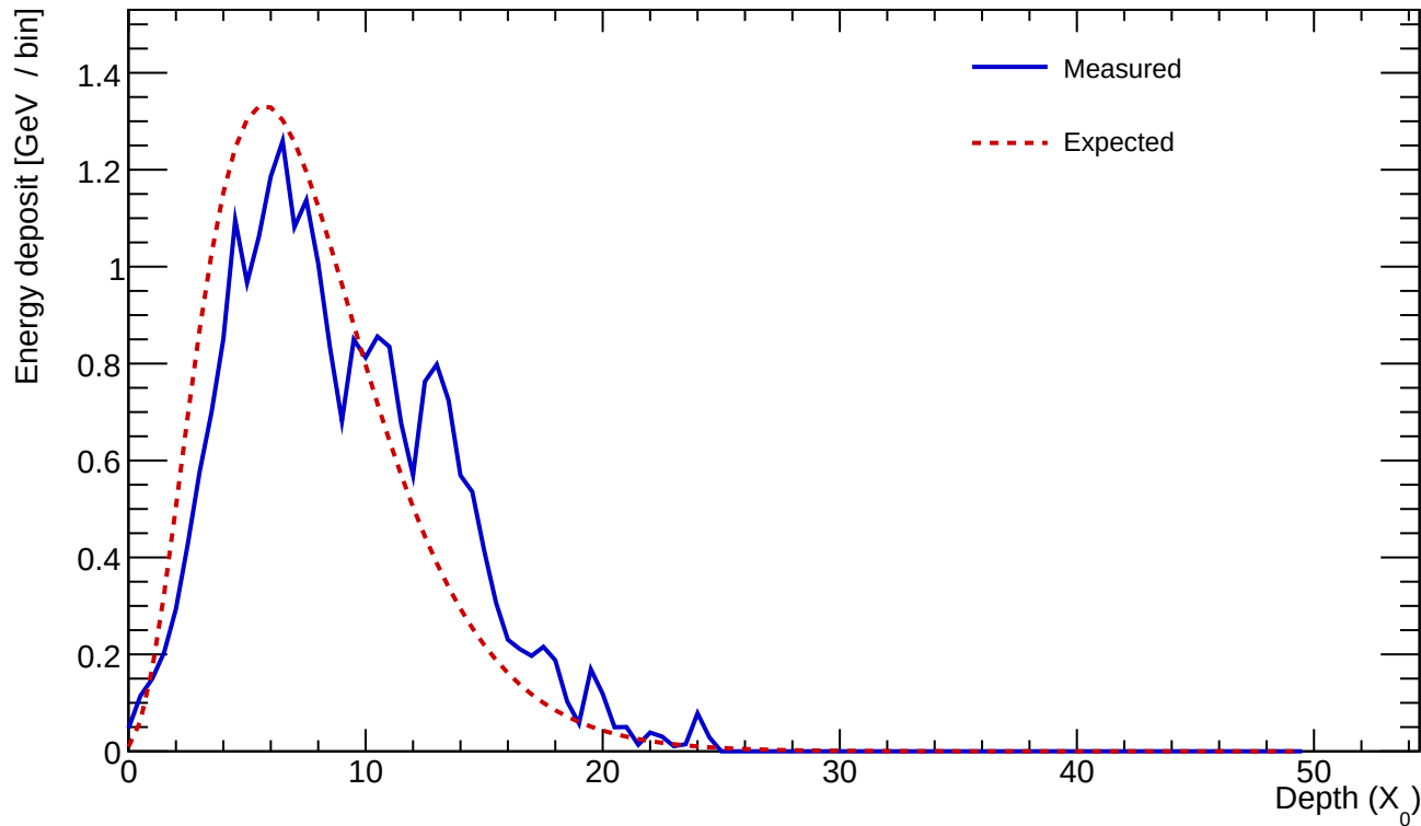
Cluster 686 E=24.190 GeV profileStart=1.00 X_0 \chi=0.2162
