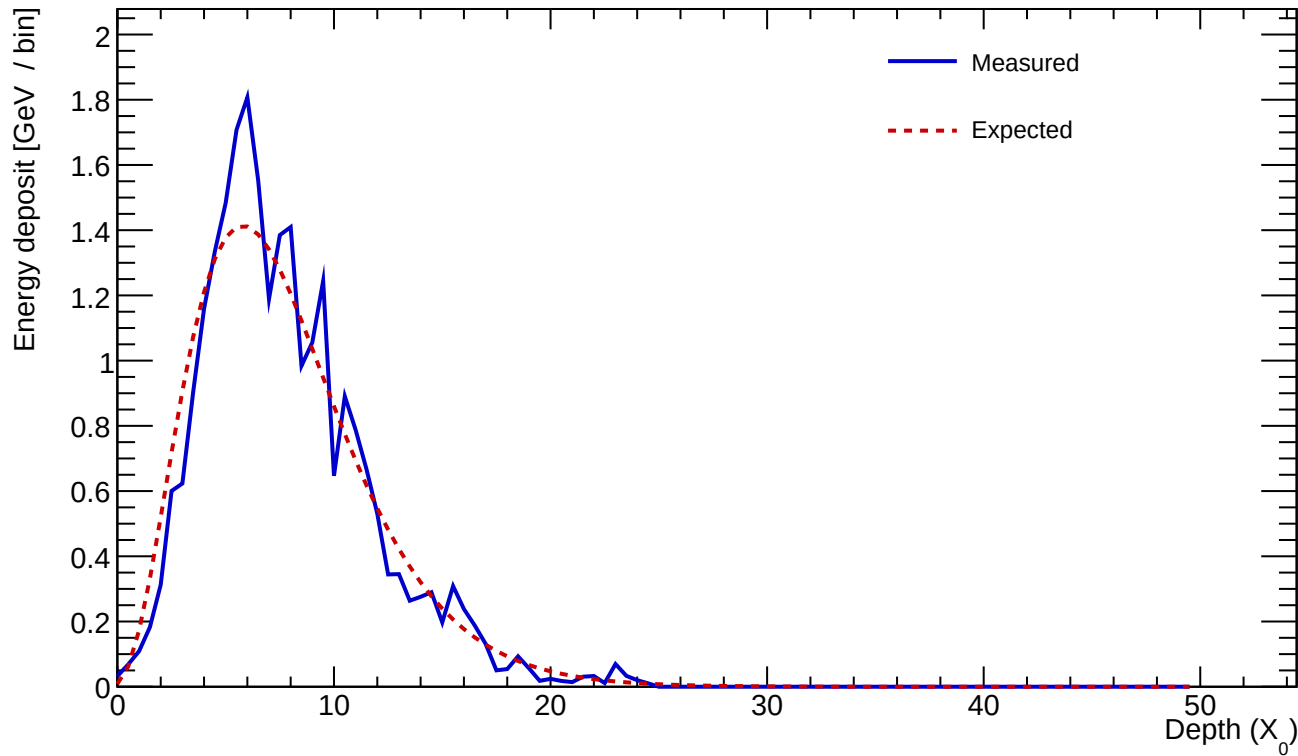
Cluster 773 E=25.789 GeV profileStart=0.50 X_0 \chi=0.1606
