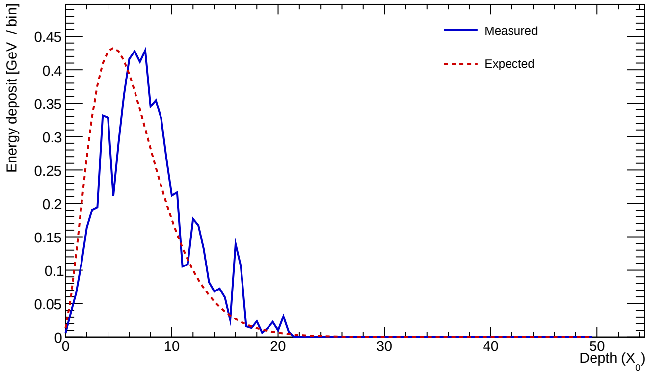
Cluster 38 E=7.083 GeV profileStart=1.00 X_0 \chi=0.2111
