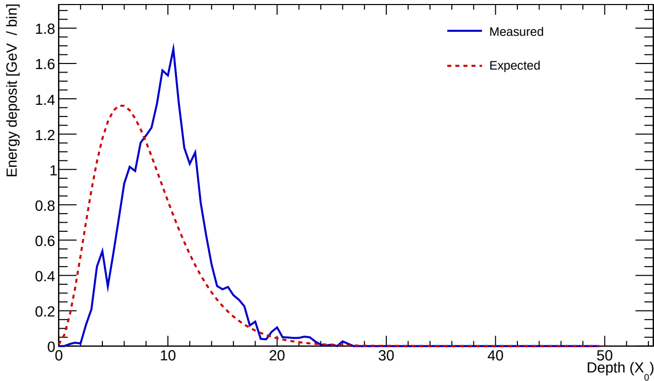
Cluster 647 E=24.803 GeV profileStart=3.00 X_0 \chi=0.2112
