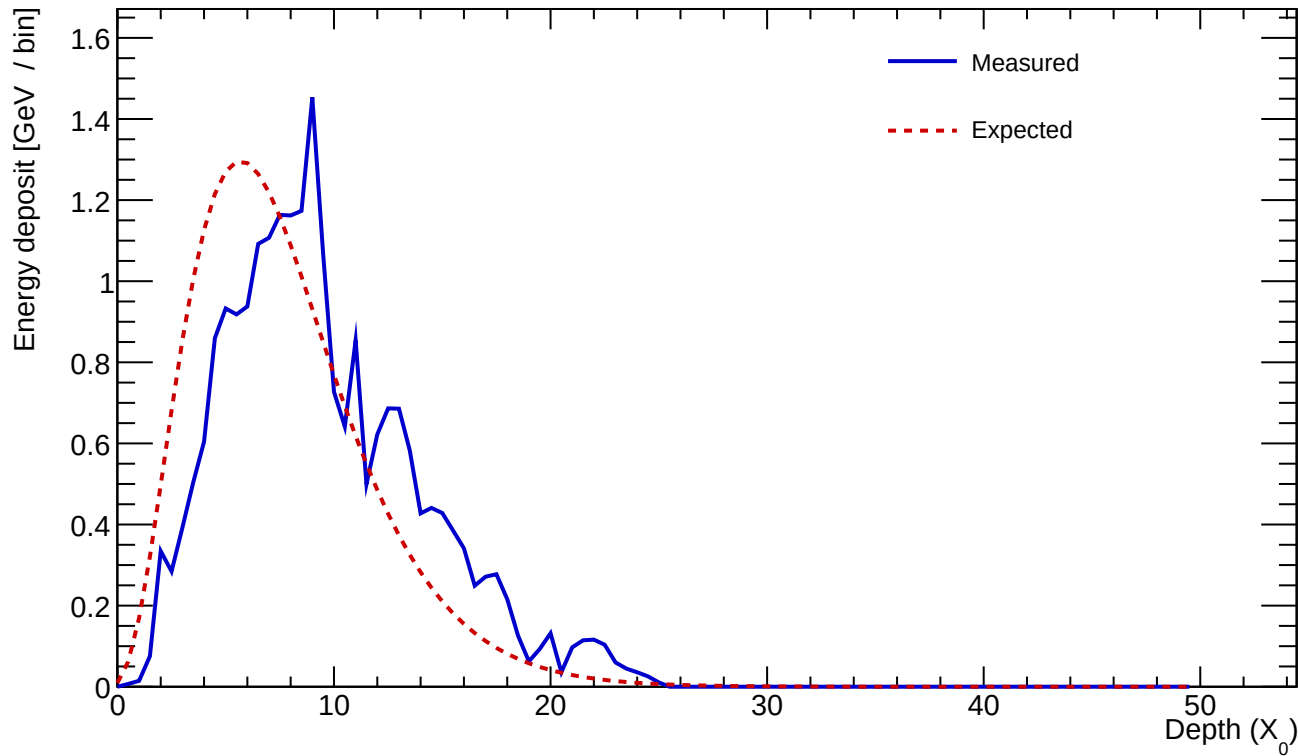
Cluster 915 E=23.475 GeV profileStart=1.50 X_0 \chi=0.1955
