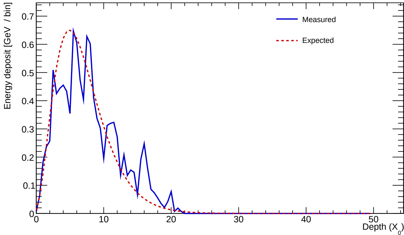
Cluster 404 E=11.071 GeV profileStart=0.50 X_0 \chi=0.2789
