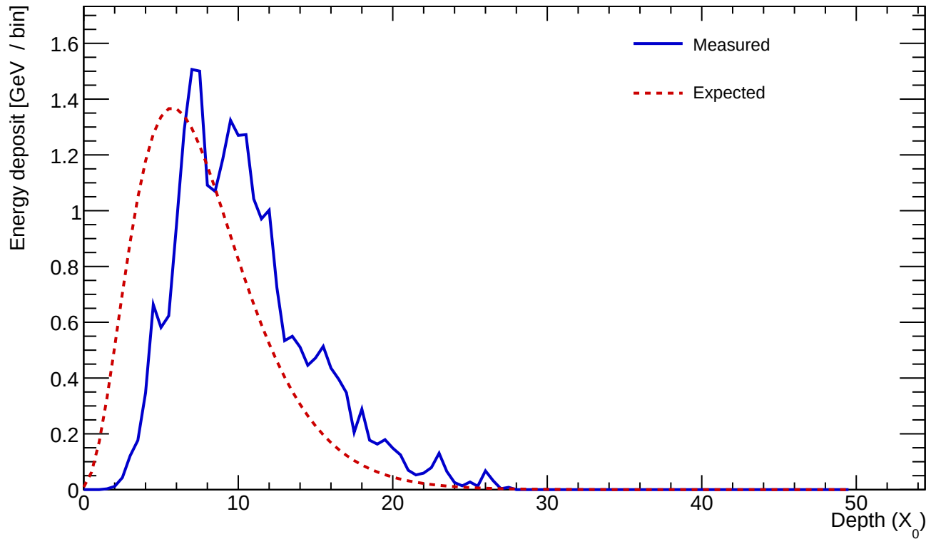
Cluster 614 E=24.903 GeV profileStart=2.50 X_0 \chi=0.1550
