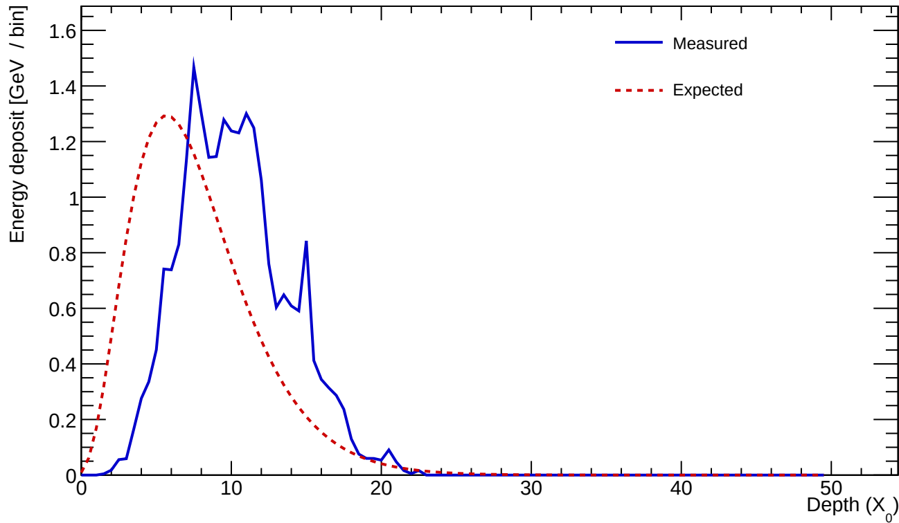
Cluster 916 E=23.422 GeV profileStart=3.00 X_0 \chi=0.1432
