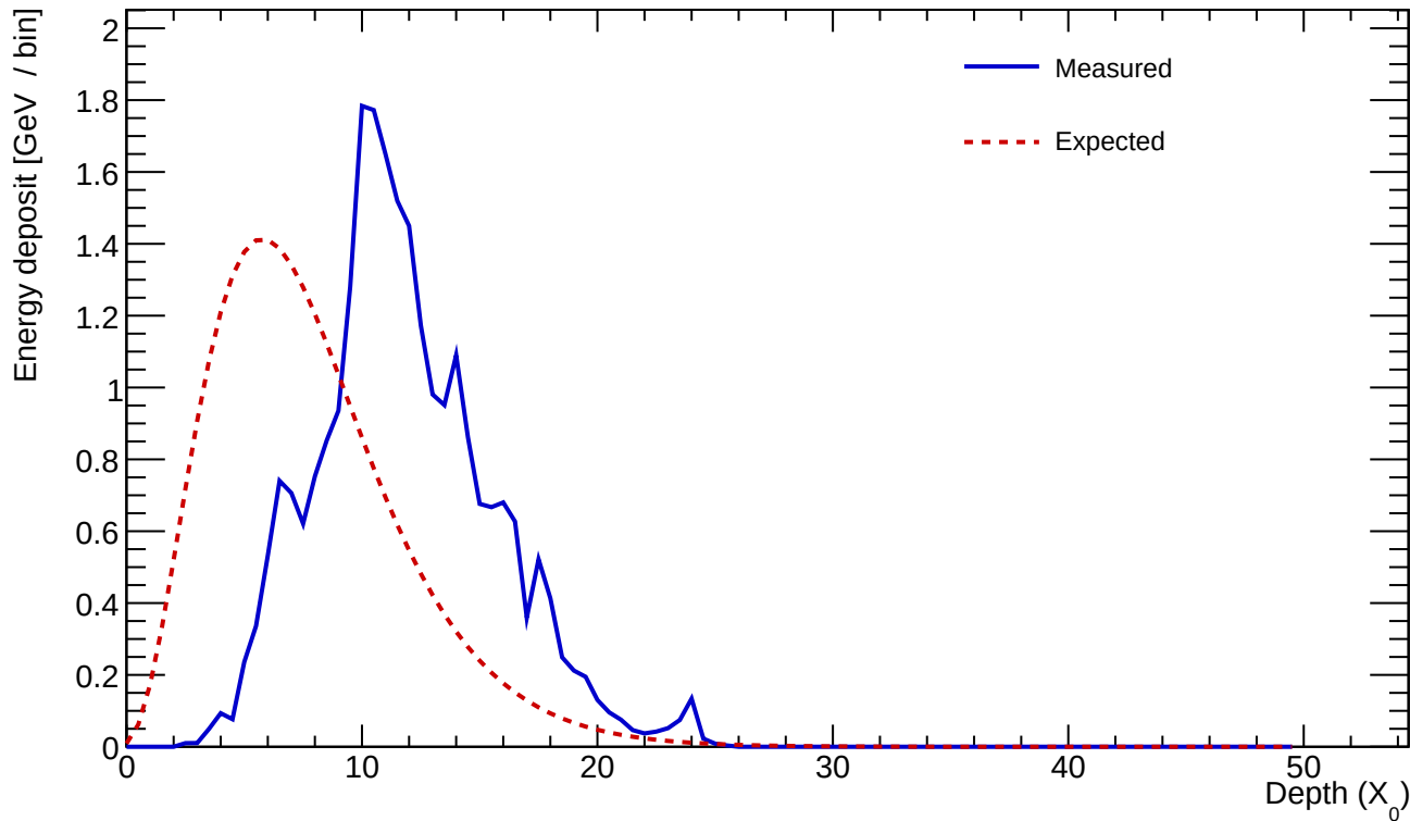
Cluster 679 E=25.788 GeV profileStart=4.50 X_0 \chi=0.2138
