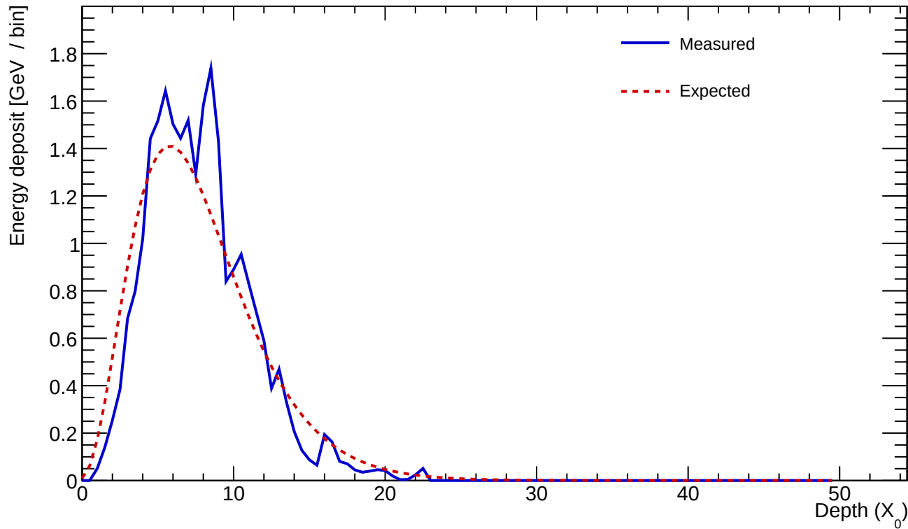
Cluster 894 E=25.743 GeV profileStart=0.50 X_0 \chi=0.1748
