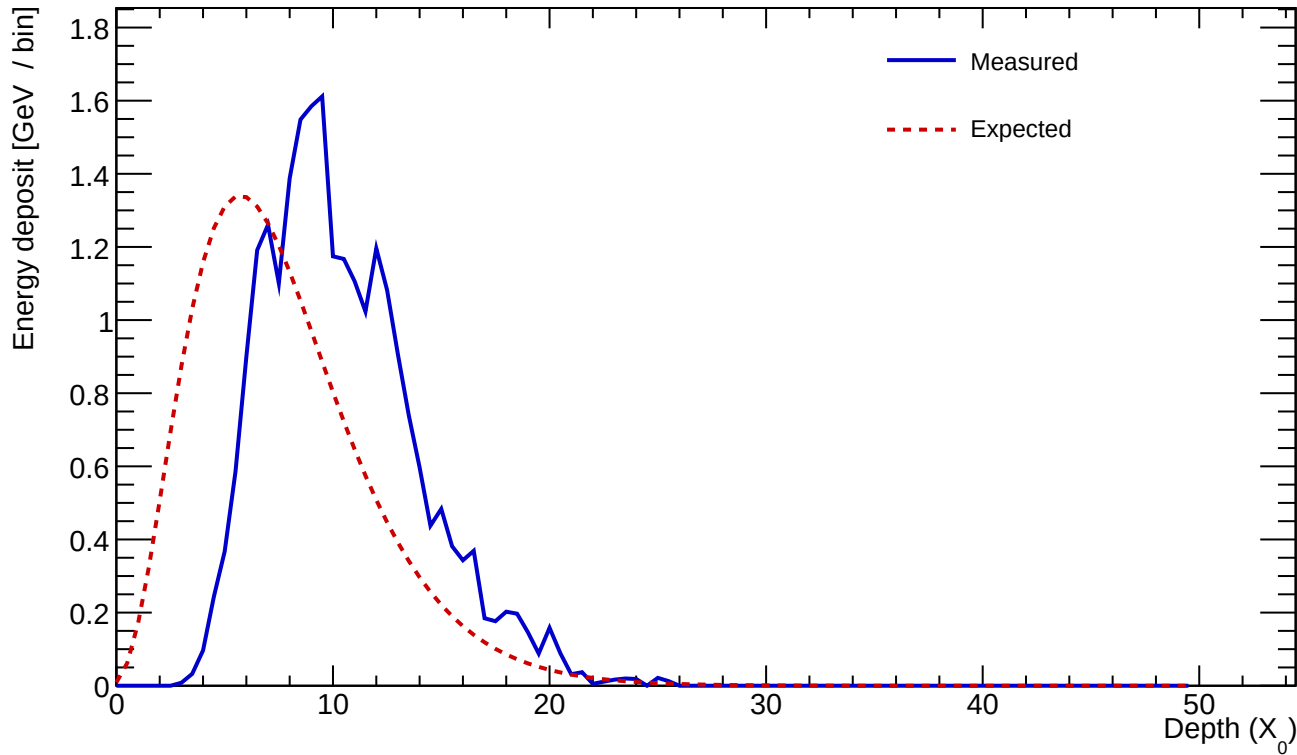
Cluster 276 E=24.340 GeV profileStart=3.00 X_0 \chi=0.1393
