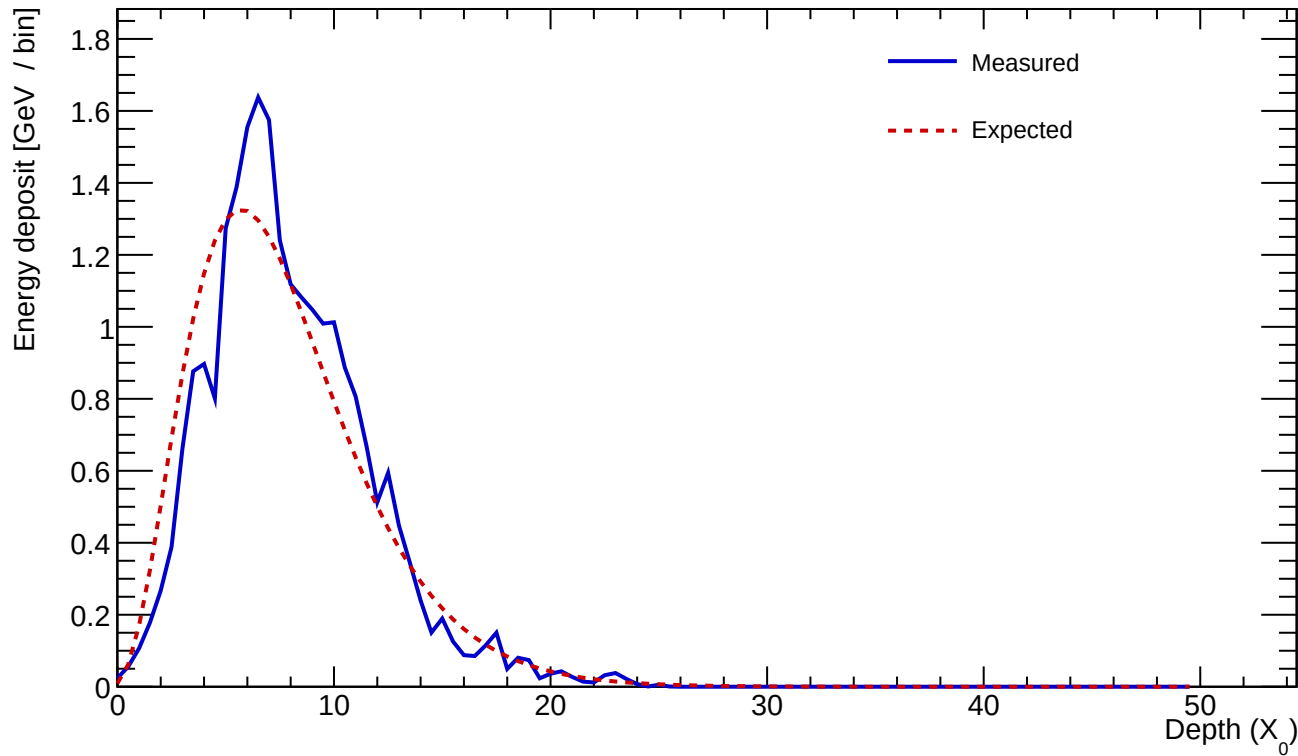
Cluster 681 E=24.065 GeV profileStart=0.50 X_0 \chi=0.1375
