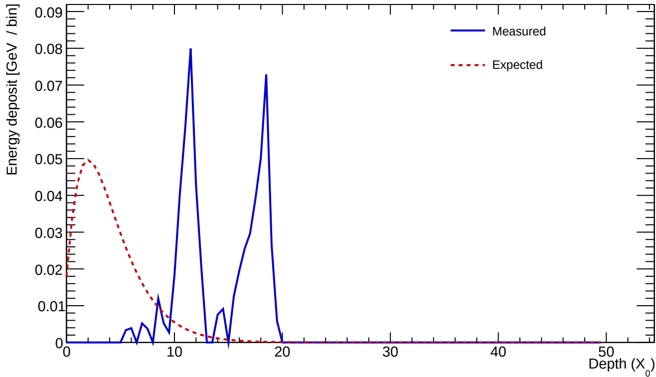
Cluster 65 E=0.594 GeV profileStart=9.50 X_0 \chi=0.8083
