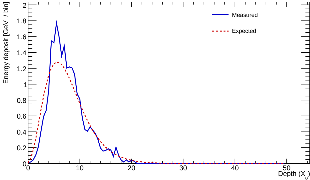
Cluster 466 E=23.154 GeV profileStart=0.50 X_0 \chi=0.1933
