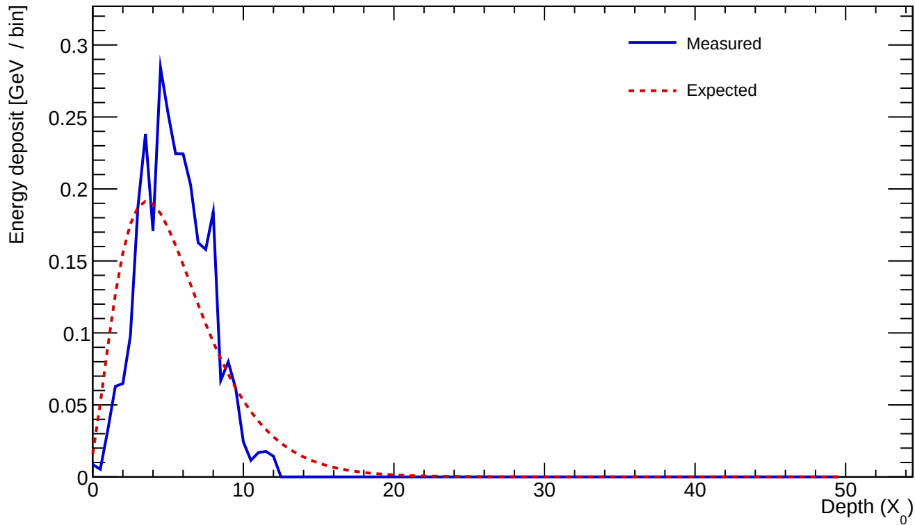
Cluster 547 E=2.854 GeV profileStart=1.00 X_0 \chi=0.2933
