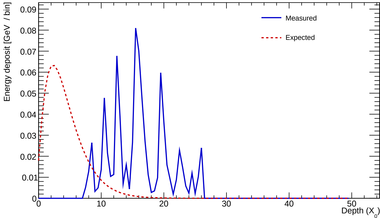
Cluster 351 E=0.797 GeV profileStart=12.00 X_0 \chi=0.8205
