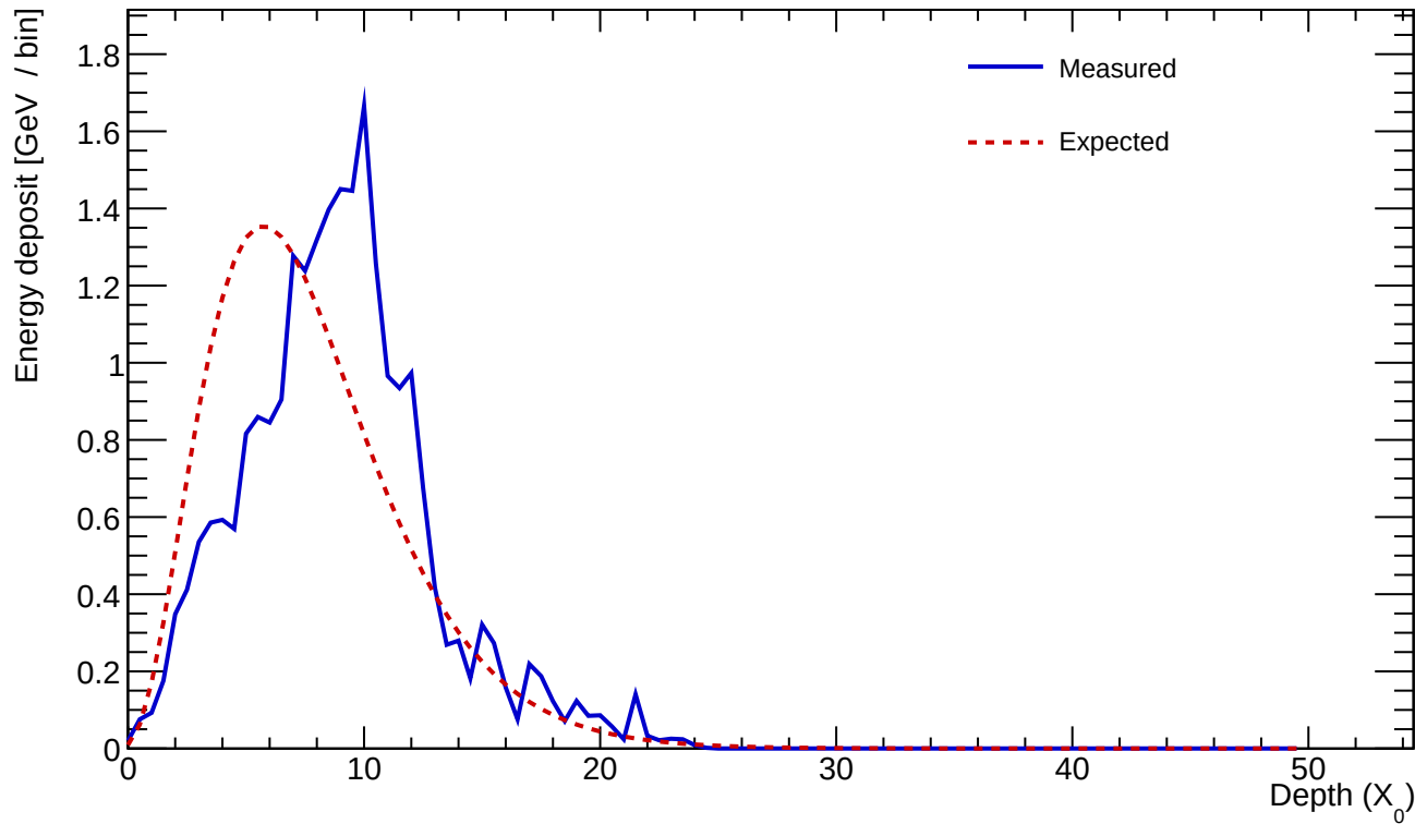
Cluster 887 E=24.637 GeV profileStart=2.00 X_0 \chi=0.2572
