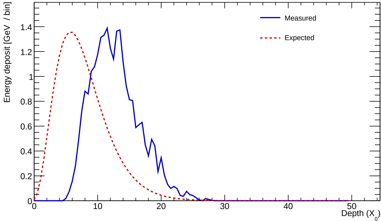
Cluster 157 E=24.685 GeV profileStart=5.00 X_0 \chi=0.1115
