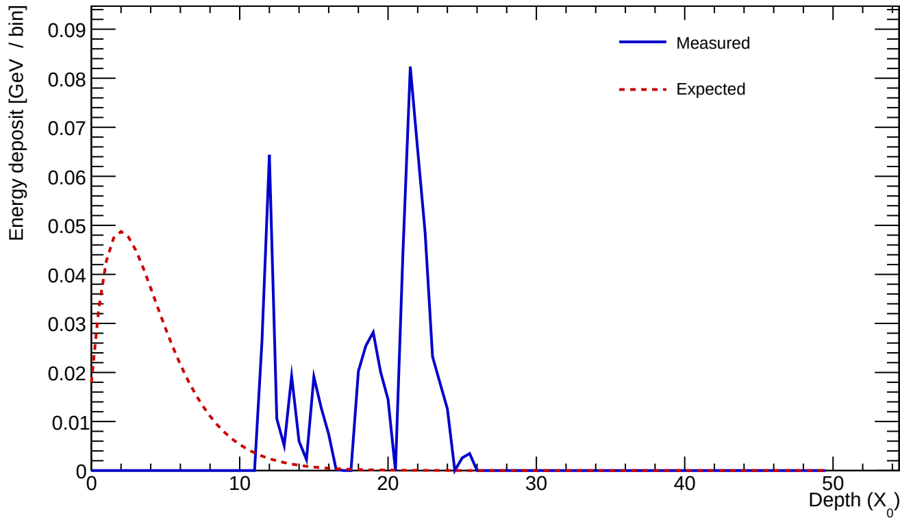
Cluster 567 E=0.582 GeV profileStart=18.00 X_0 \chi=0.7662
