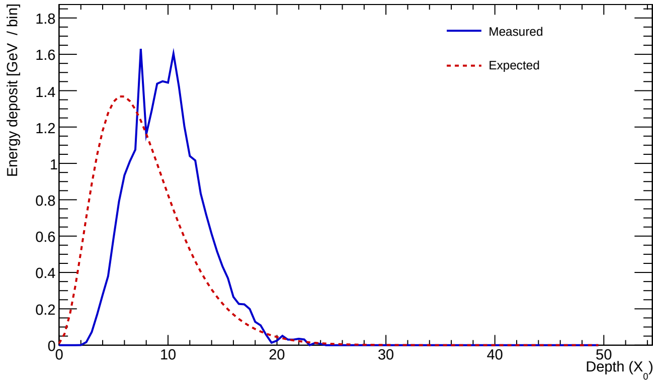
Cluster 636 E=24.950 GeV profileStart=3.00 X_0 \chi=0.1643
