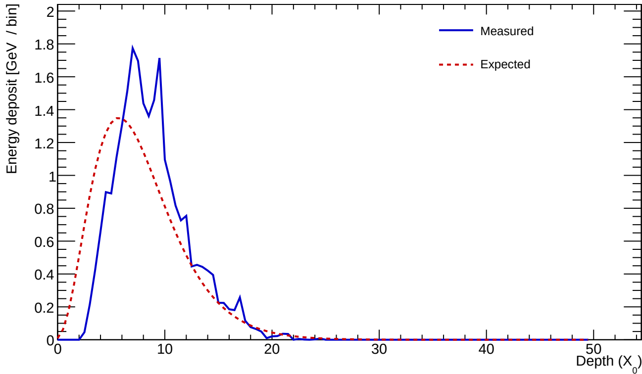
Cluster 199 E=24.541 GeV profileStart=1.50 X_0 \chi=0.1740
