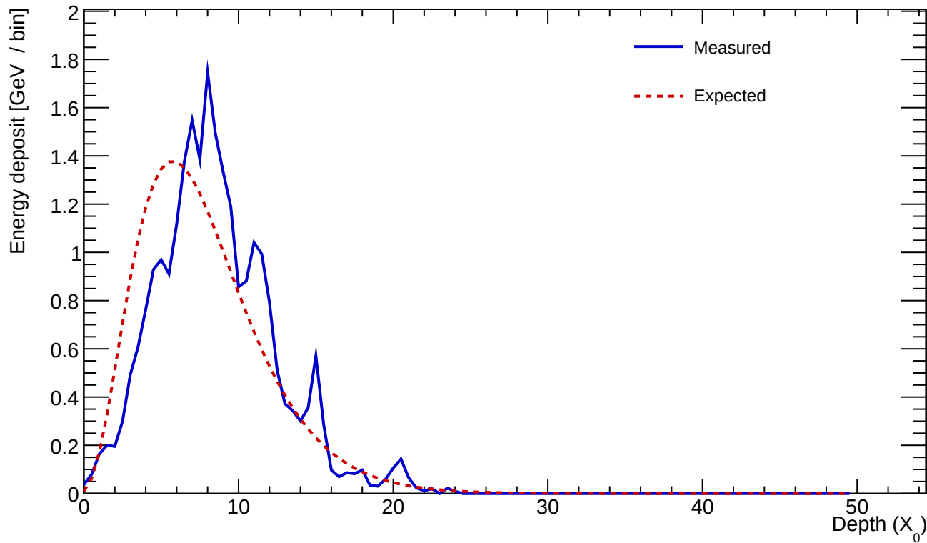
Cluster 134 E=25.097 GeV profileStart=1.00 X_0 \chi=0.2043
