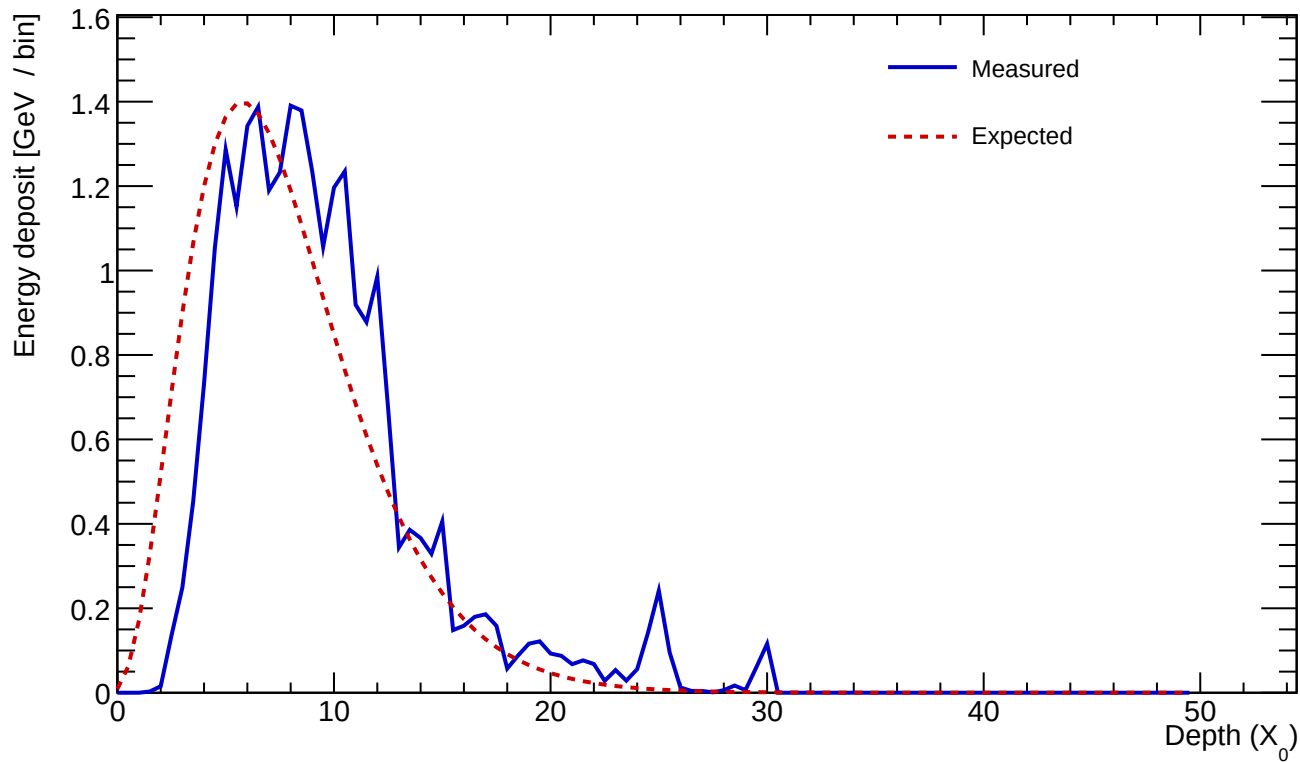
Cluster 4 E=25.490 GeV profileStart=1.50 X_0 \chi=0.1503
