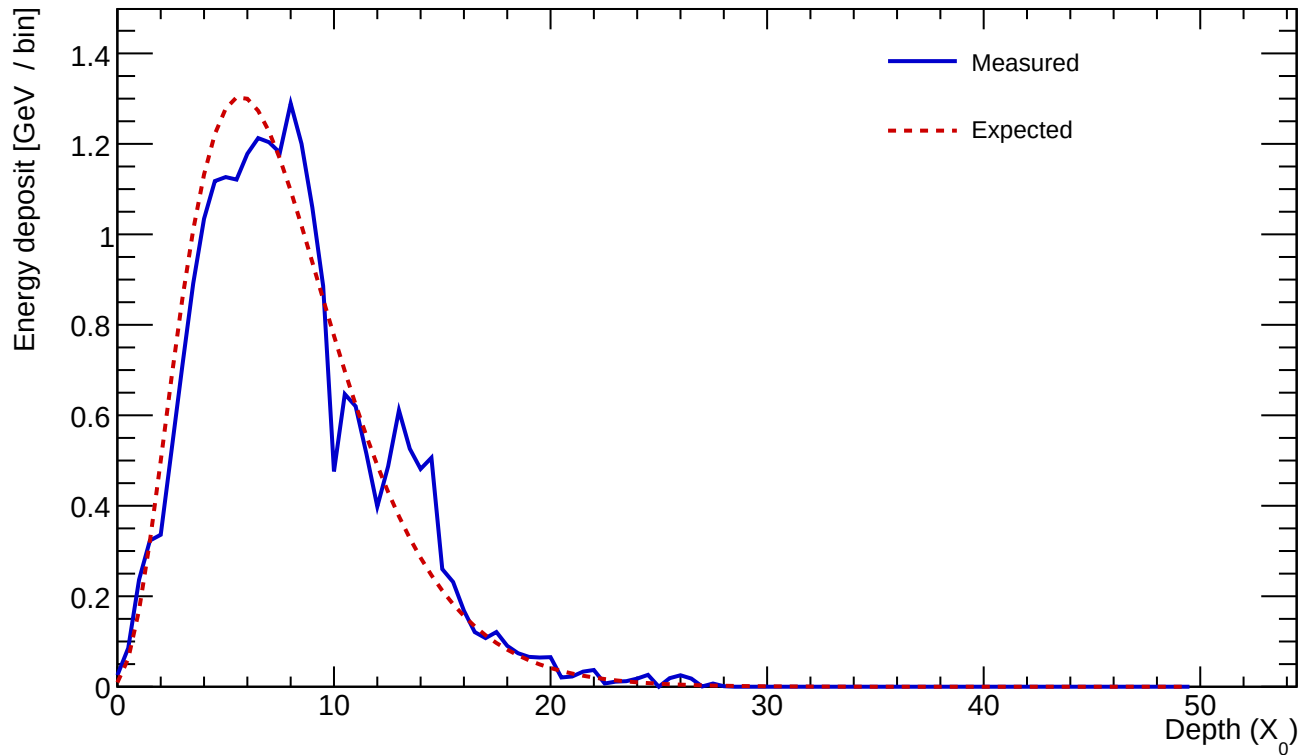
Cluster 737 E=23.637 GeV profileStart=0.50 X_0 \chi=0.1410
