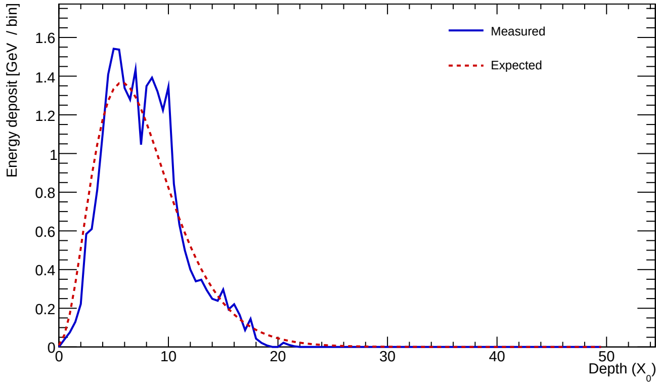
Cluster 792 E=24.851 GeV profileStart=0.50 X_0 \chi=0.1807
