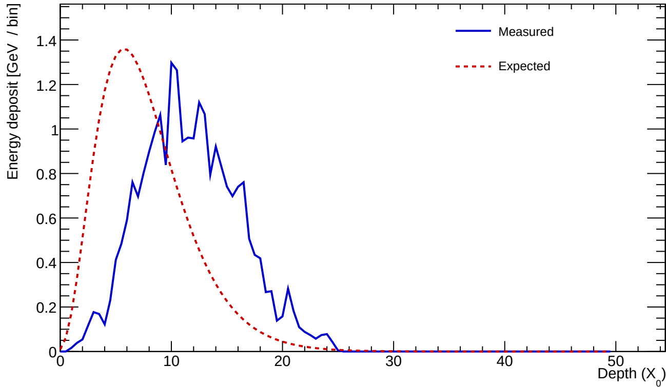
Cluster 584 E=24.739 GeV profileStart=4.50 X_0 \chi=0.2266
