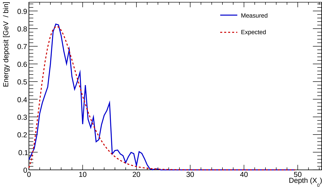
Cluster 322 E=14.136 GeV profileStart=0.50 X_0 \chi=0.2316
