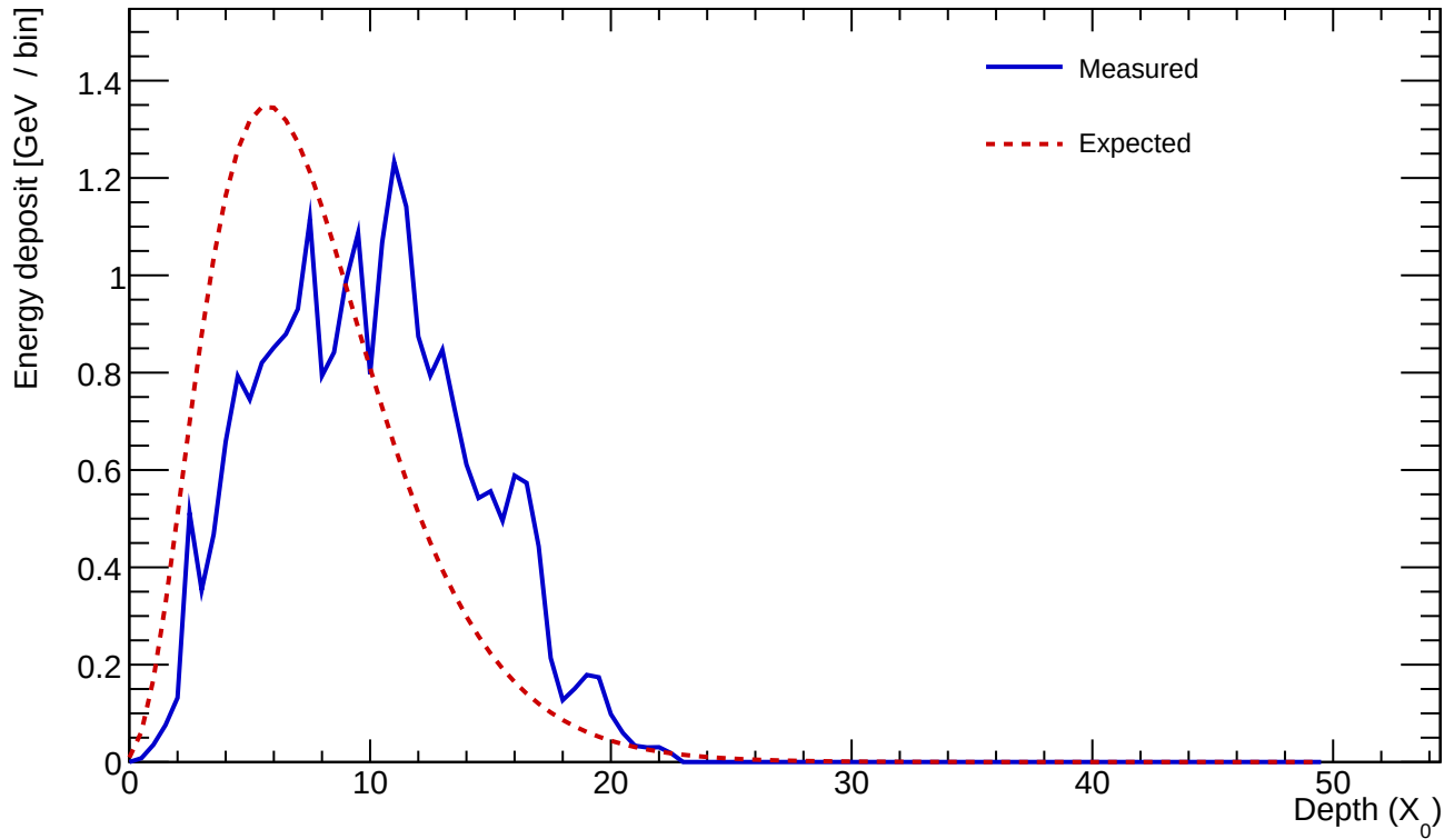
Cluster 27 E=24.495 GeV profileStart=2.50 X_0 \chi=0.2841
