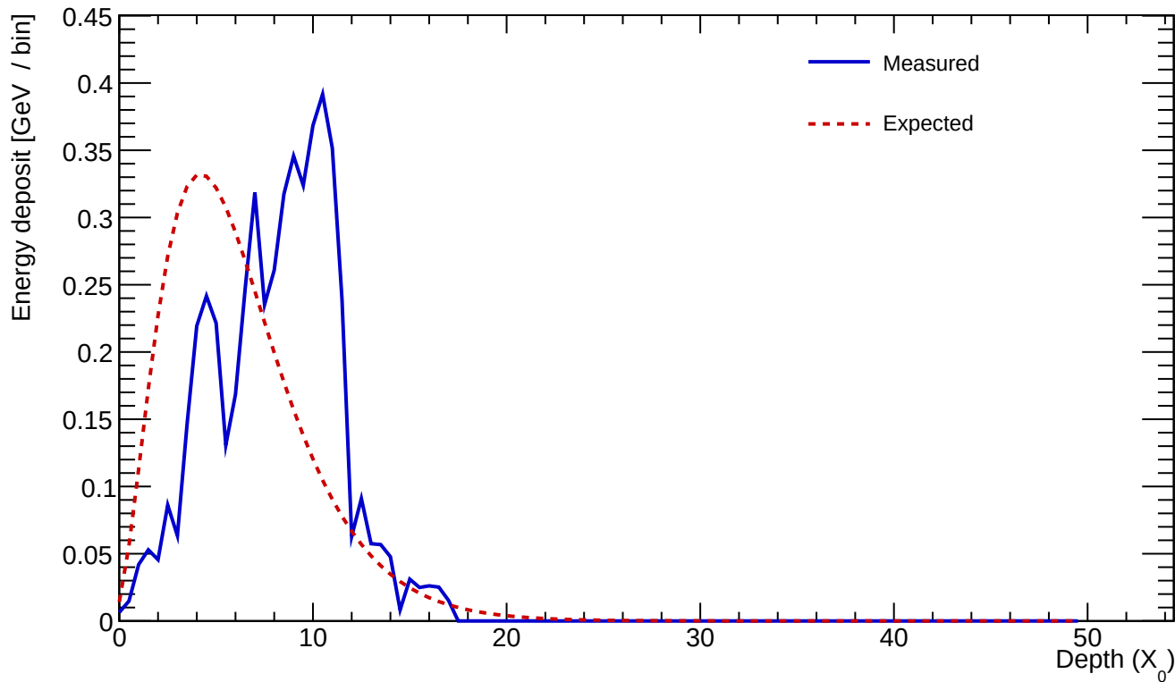
Cluster 815 E=5.286 GeV profileStart=2.50 X_0 \chi=0.3915
