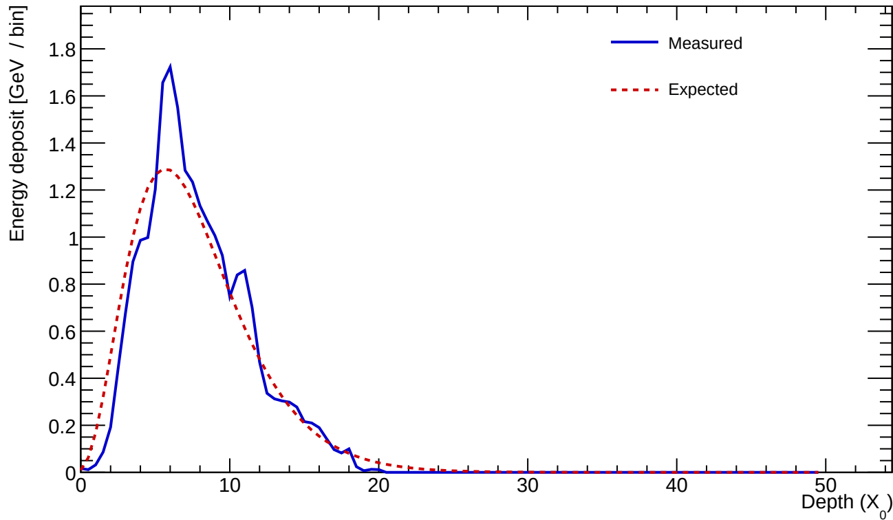
Cluster 247 E=23.349 GeV profileStart=0.50 X_0 \chi=0.1210
