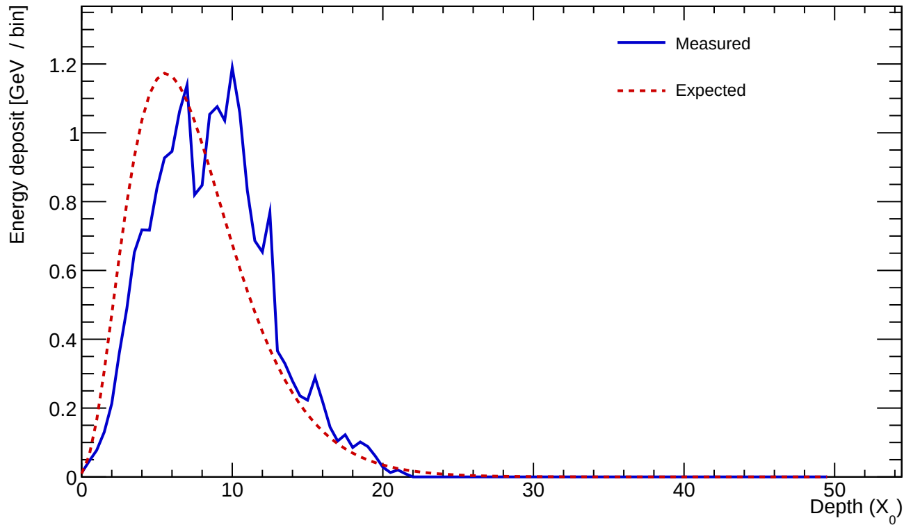
Cluster 548 E=21.065 GeV profileStart=1.00 X_0 \chi=0.1887
