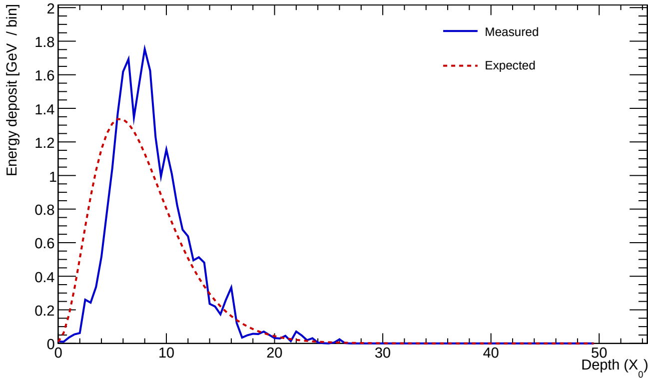
Cluster 918 E=24.306 GeV profileStart=1.50 X_0 \chi=0.2062
