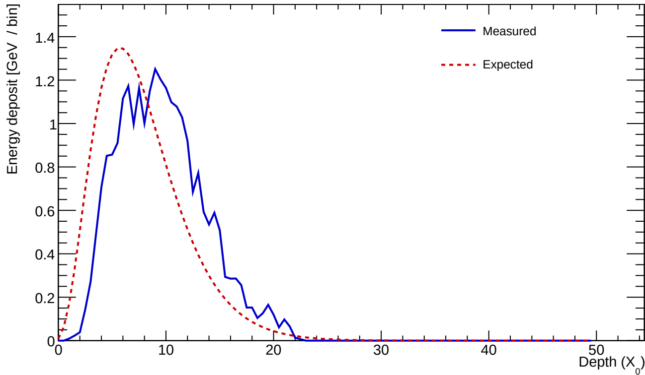
Cluster 501 E=24.512 GeV profileStart=2.00 X_0 \chi=0.1383
