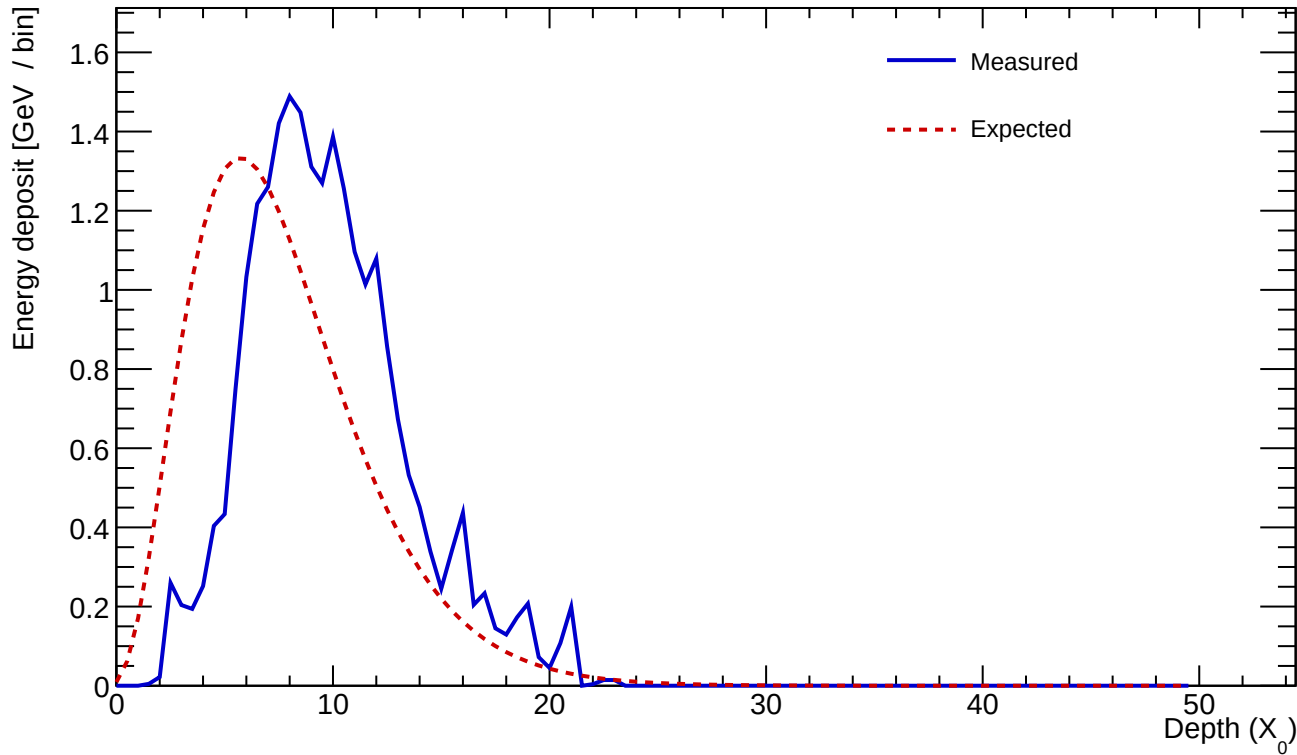
Cluster 287 E=24.231 GeV profileStart=2.50 X_0 \chi=0.1509
