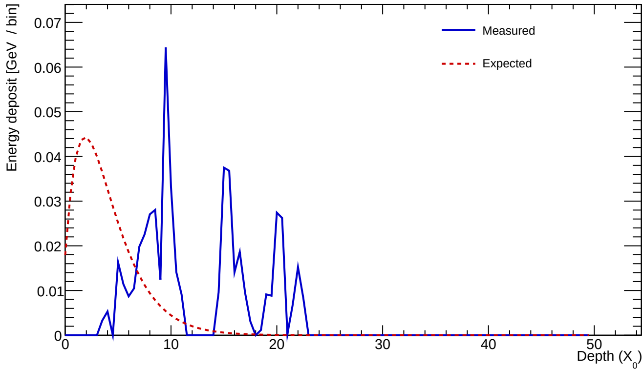
Cluster 10 E=0.519 GeV profileStart=6.50 X_0 \chi=0.9586
