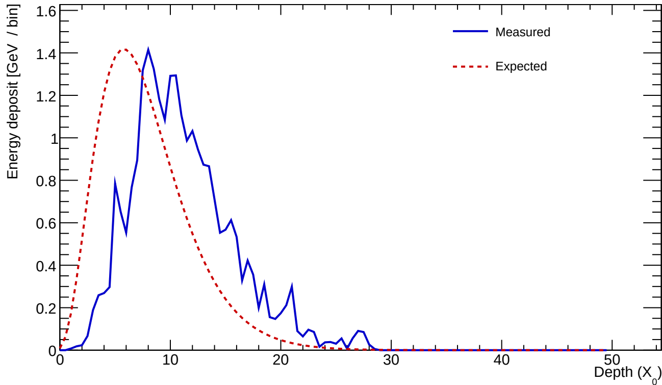
Cluster 419 E=25.863 GeV profileStart=3.00 X_0 \chi=0.1738
