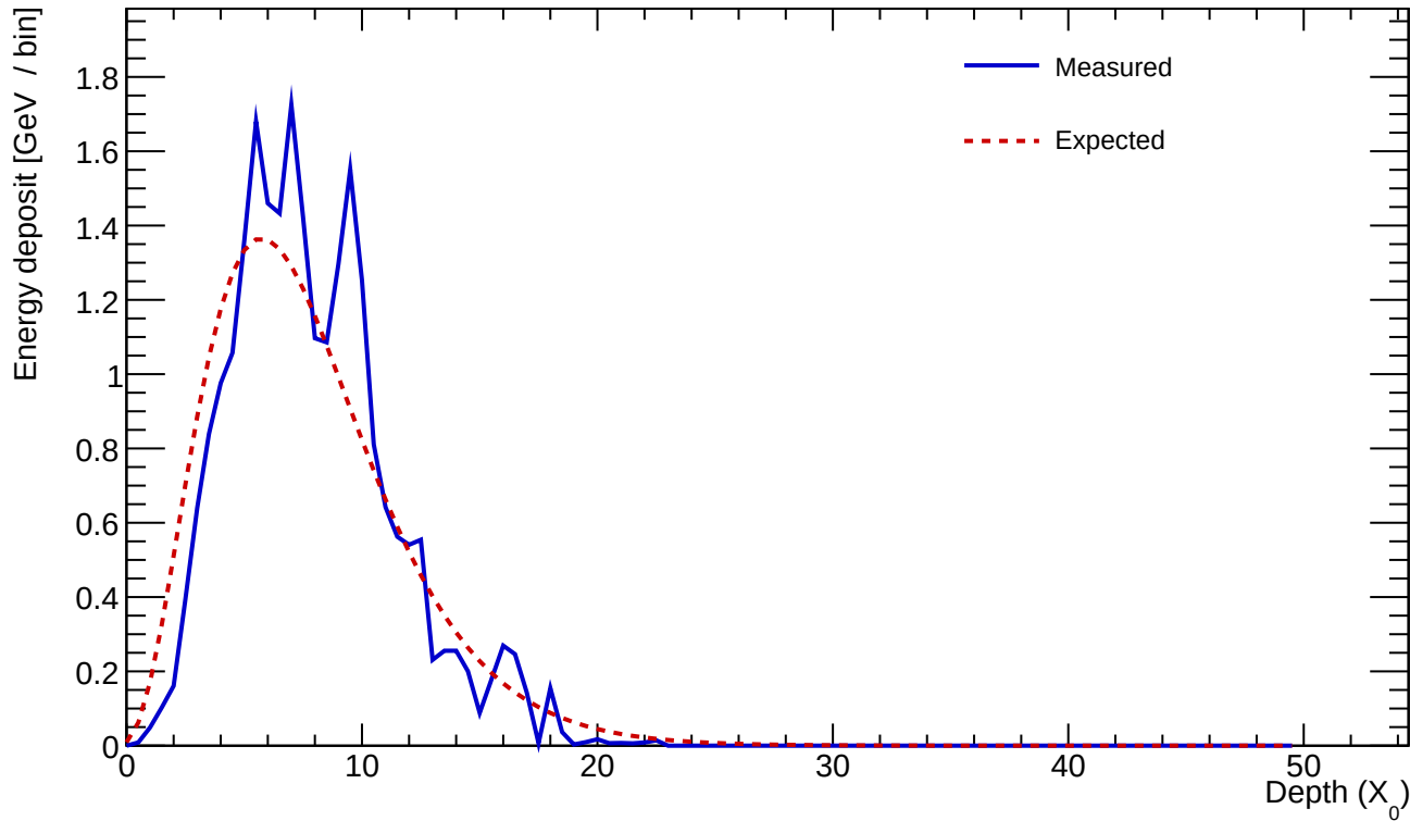
Cluster 390 E=24.836 GeV profileStart=0.50 X_0 \chi=0.1950
