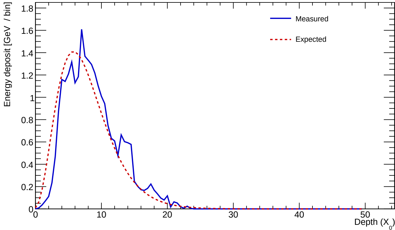
Cluster 721 E=25.705 GeV profileStart=1.00 X_0 \chi=0.1230
