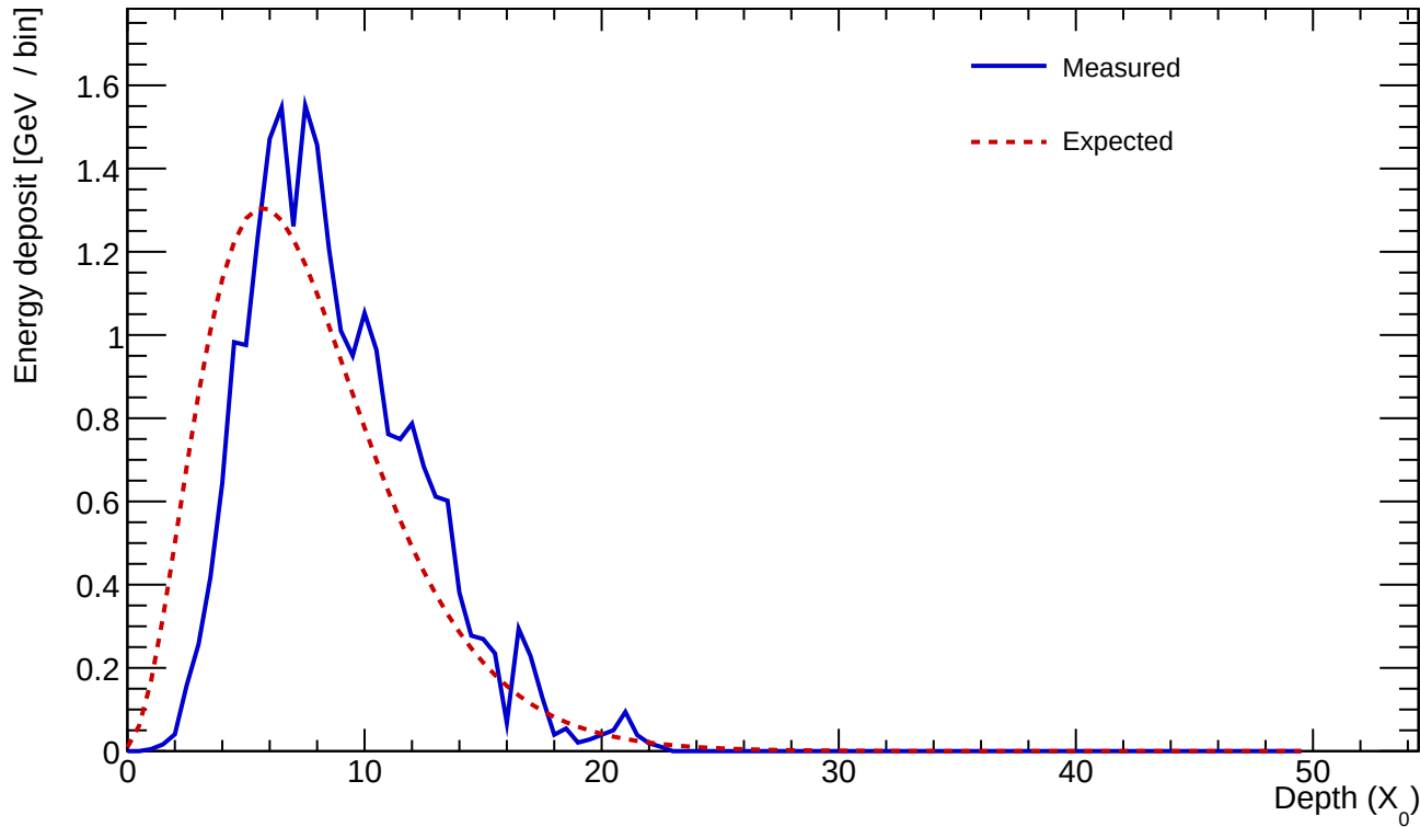
Cluster 502 E=23.678 GeV profileStart=1.50 X_0 \chi=0.1389
