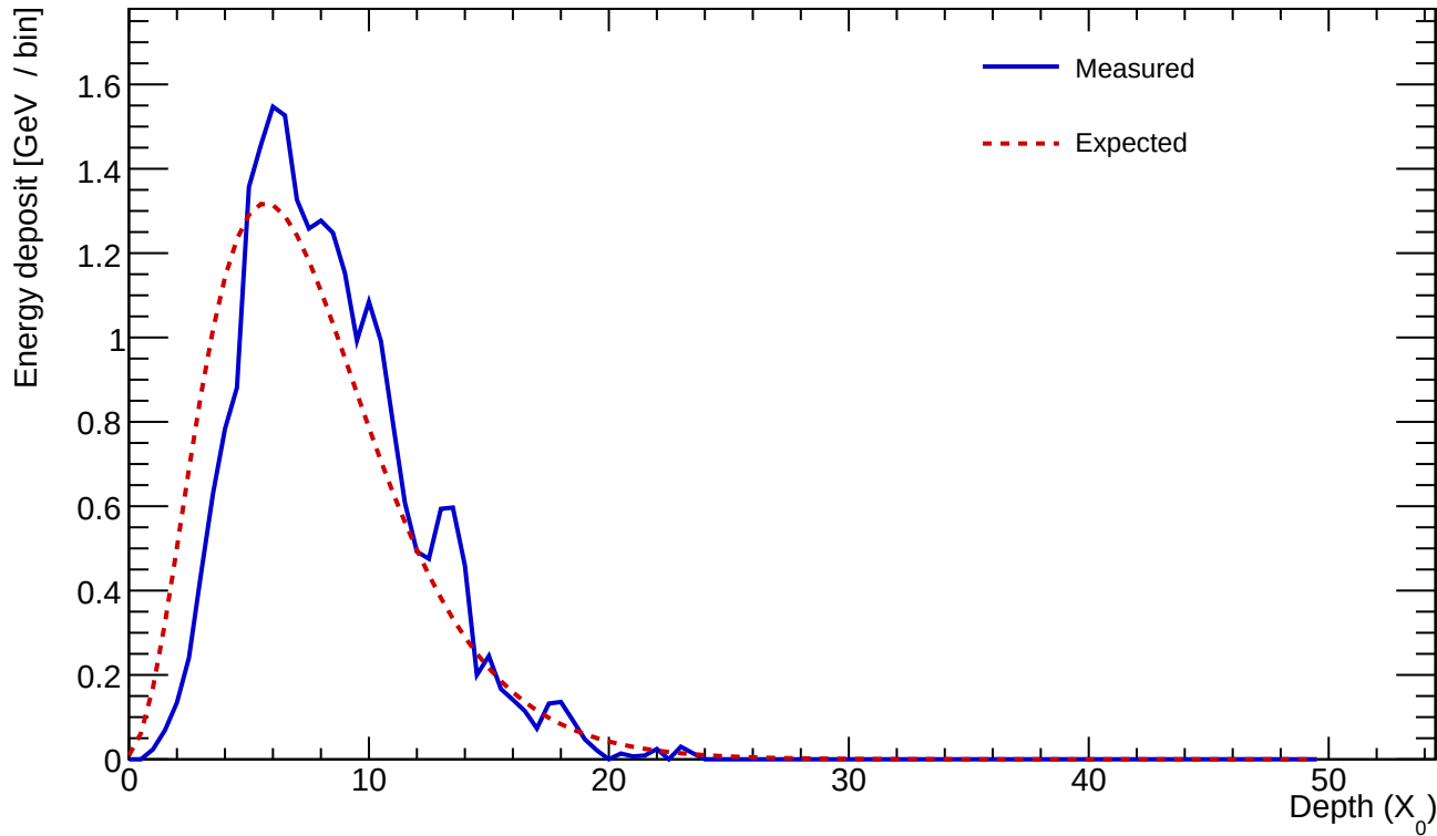
Cluster 215 E=23.912 GeV profileStart=1.00 X_0 \chi=0.1398
