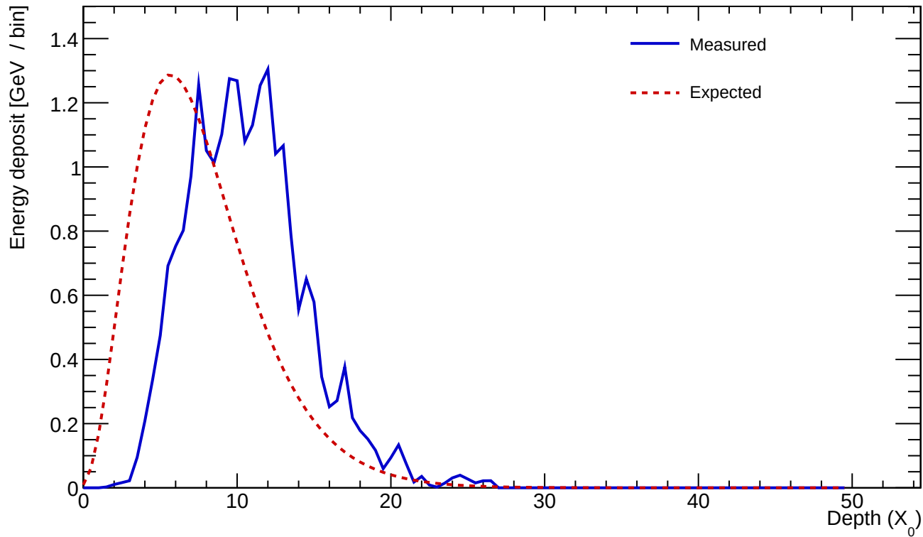
Cluster 274 E=23.306 GeV profileStart=3.00 X_0 \chi=0.1638
