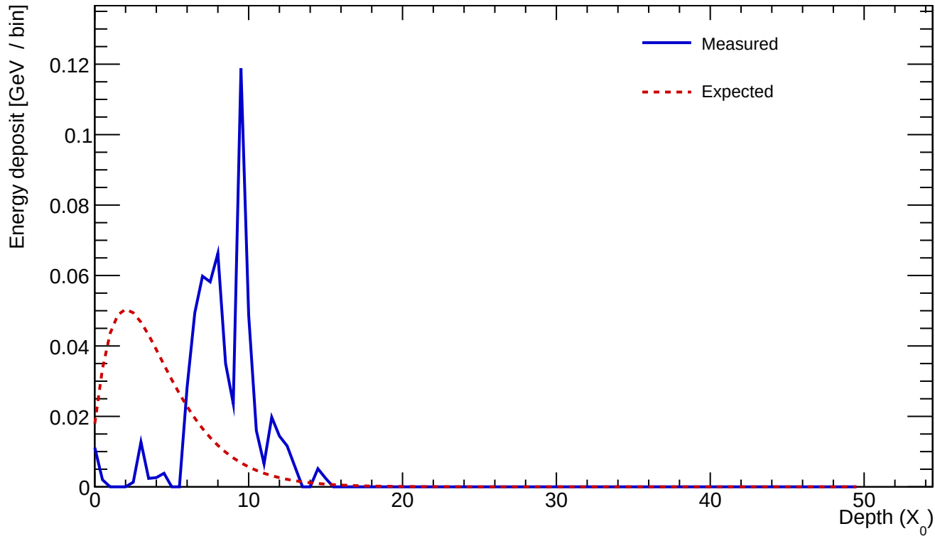
Cluster 651 E=0.606 GeV profileStart=5.50 X_0 \chi=0.5053
