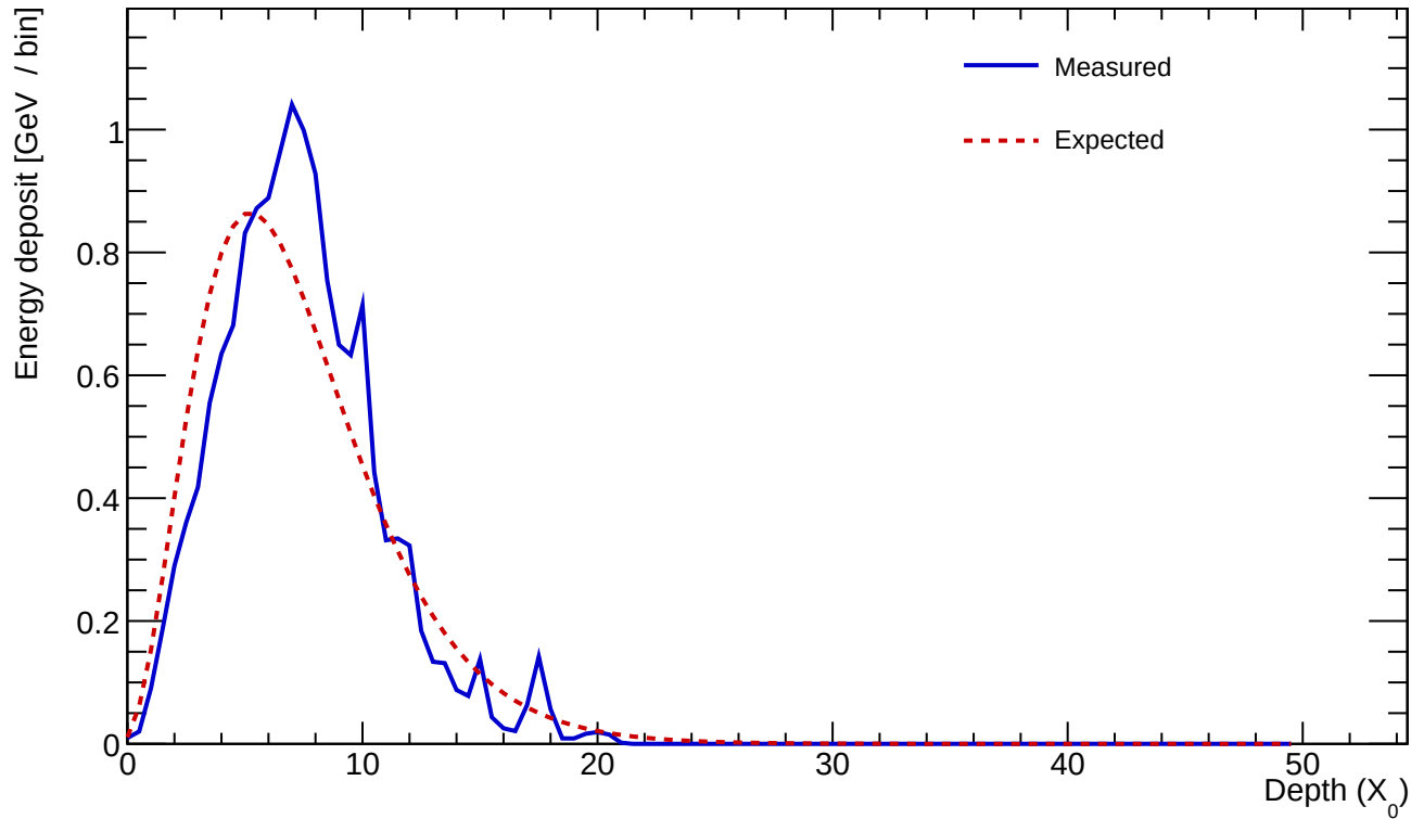
Cluster 385 E=15.127 GeV profileStart=0.50 X_0 \chi=0.1796
