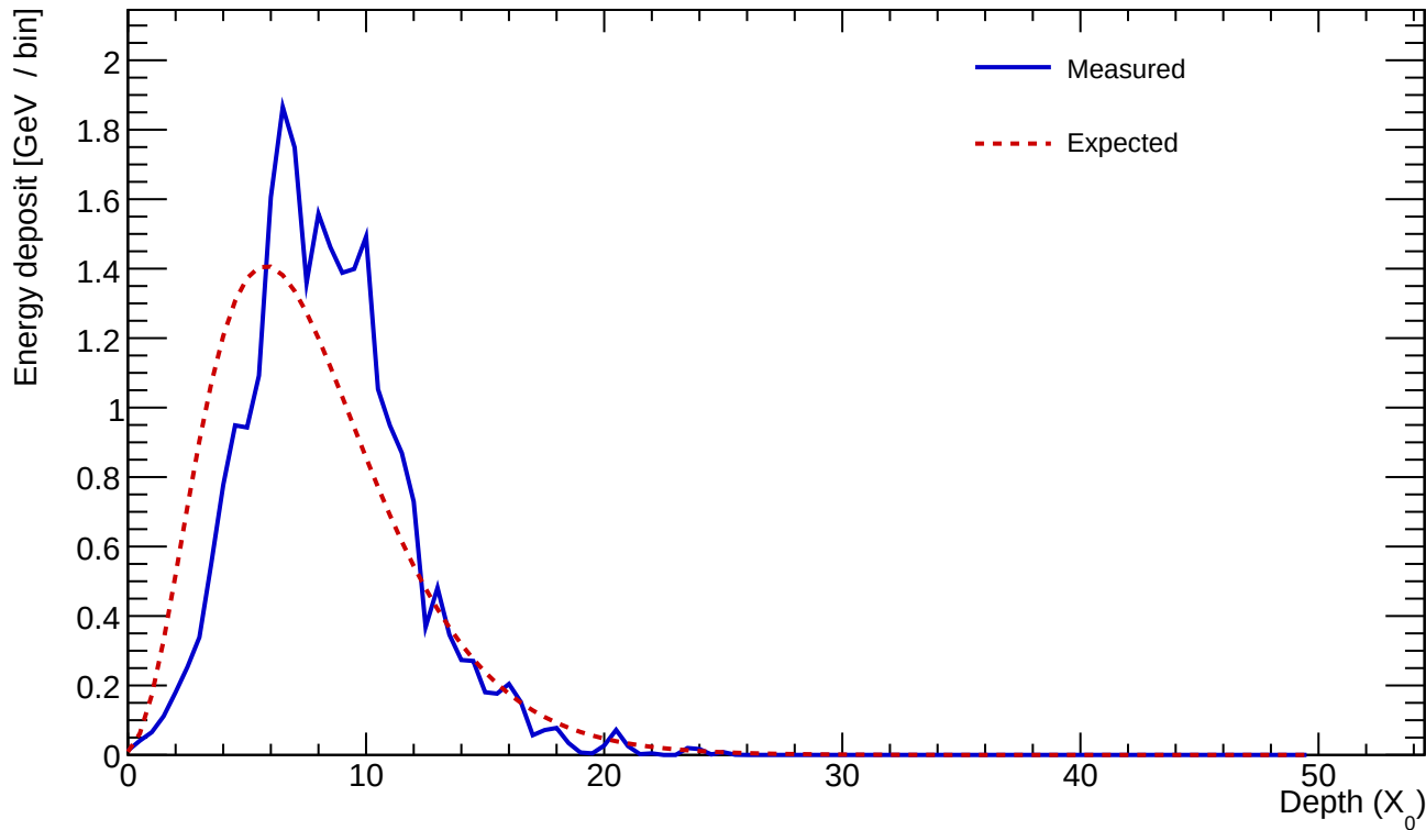
Cluster 430 E=25.680 GeV profileStart=1.50 X_0 \chi=0.2112
