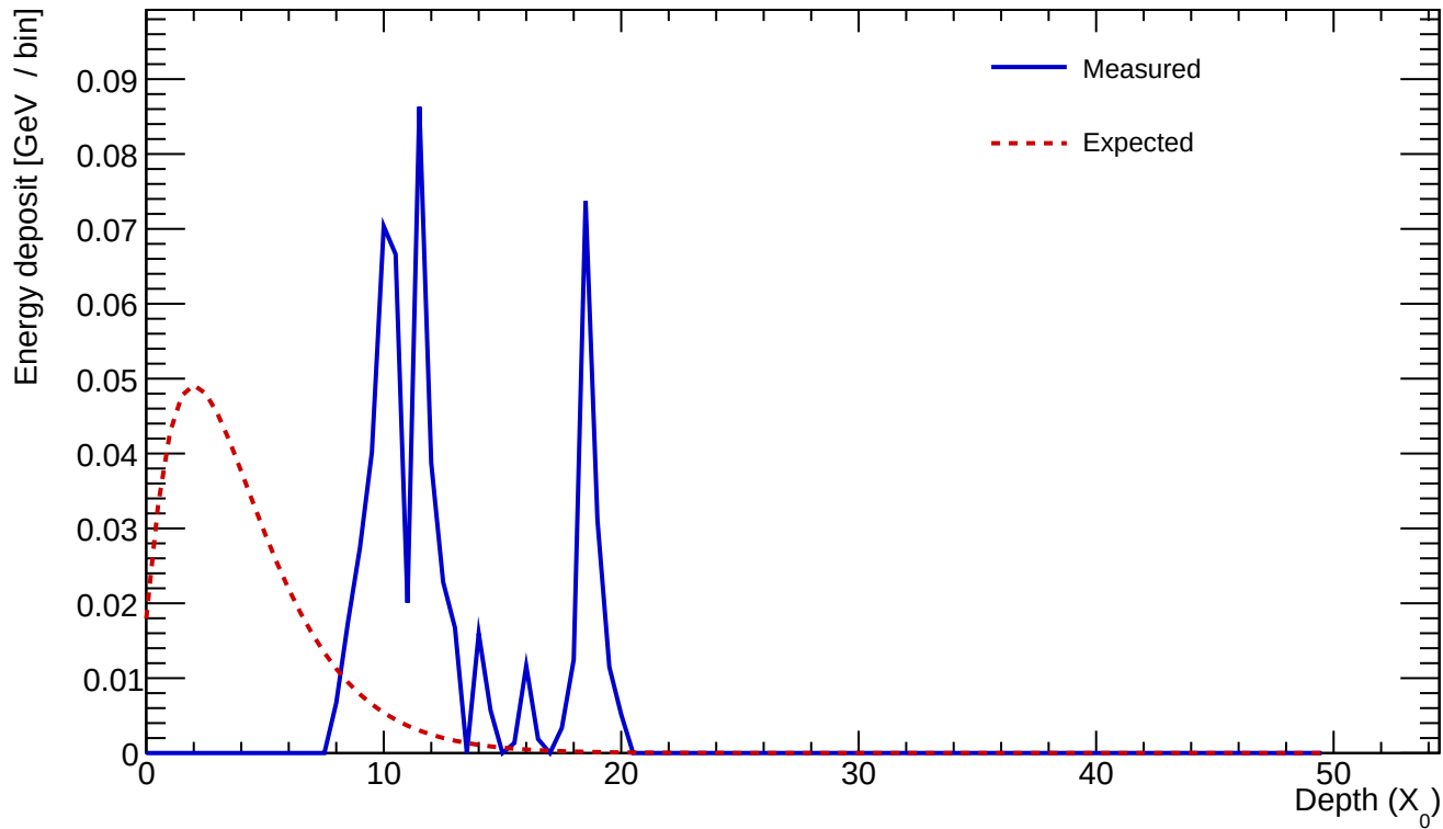
Cluster 685 E=0.587 GeV profileStart=8.50 X_0 \chi=0.6483
