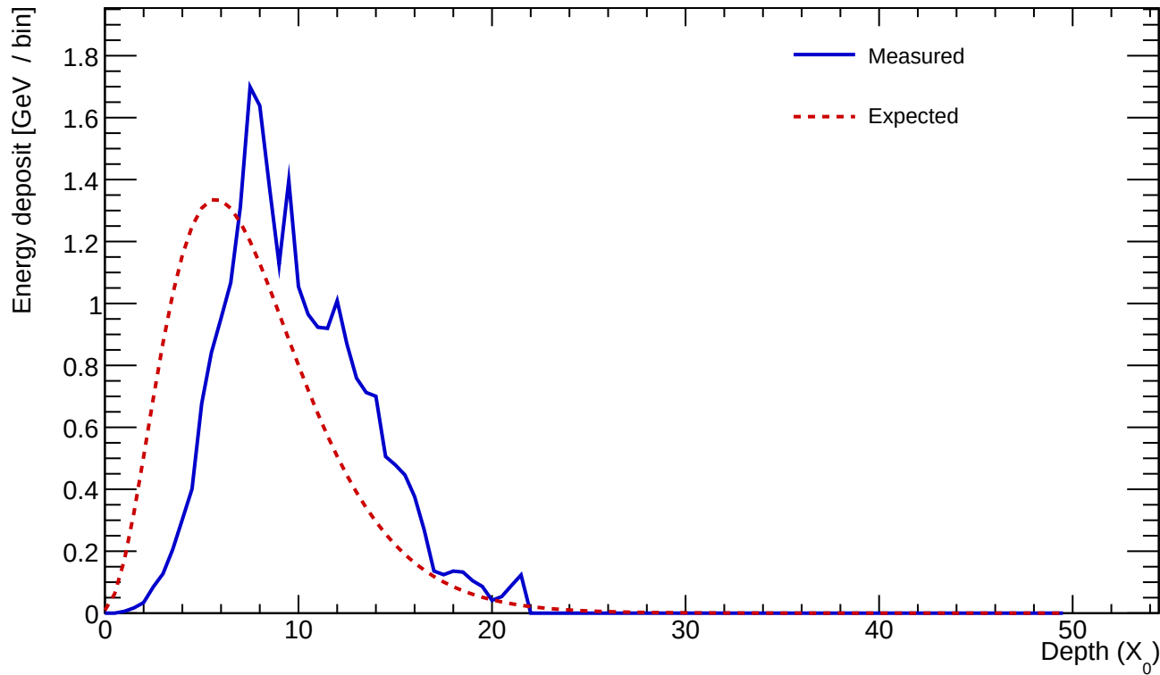
Cluster 459 E=24.278 GeV profileStart=2.50 X_0 \chi=0.1332
