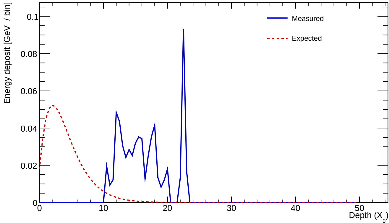
Cluster 243 E=0.633 GeV profileStart=11.00 X_0 \chi=0.5543
