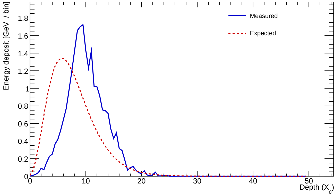
Cluster 327 E=24.368 GeV profileStart=3.00 X_0 \chi=0.2058
