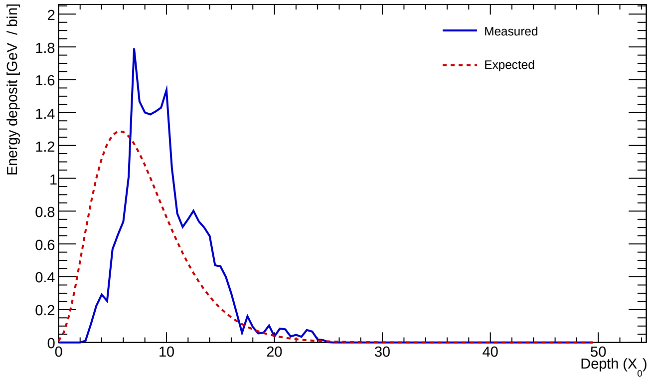
Cluster 49 E=23.310 GeV profileStart=2.50 X_0 \chi=0.1949
