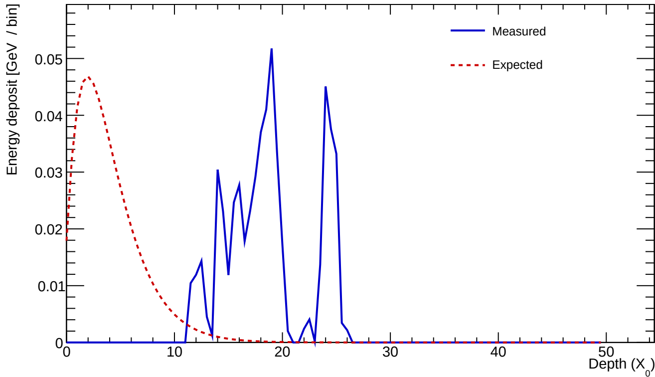
Cluster 408 E=0.555 GeV profileStart=14.00 X_0 \chi=0.7475
