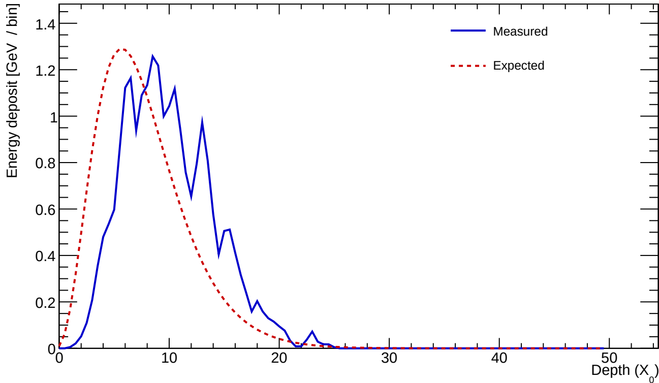
Cluster 341 E=23.369 GeV profileStart=2.50 X_0 \chi=0.1558
