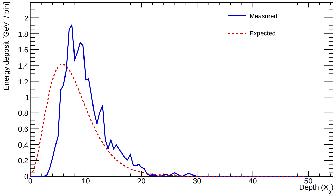
Cluster 8 E=25.856 GeV profileStart=2.50 X_0 \chi=0.2024
