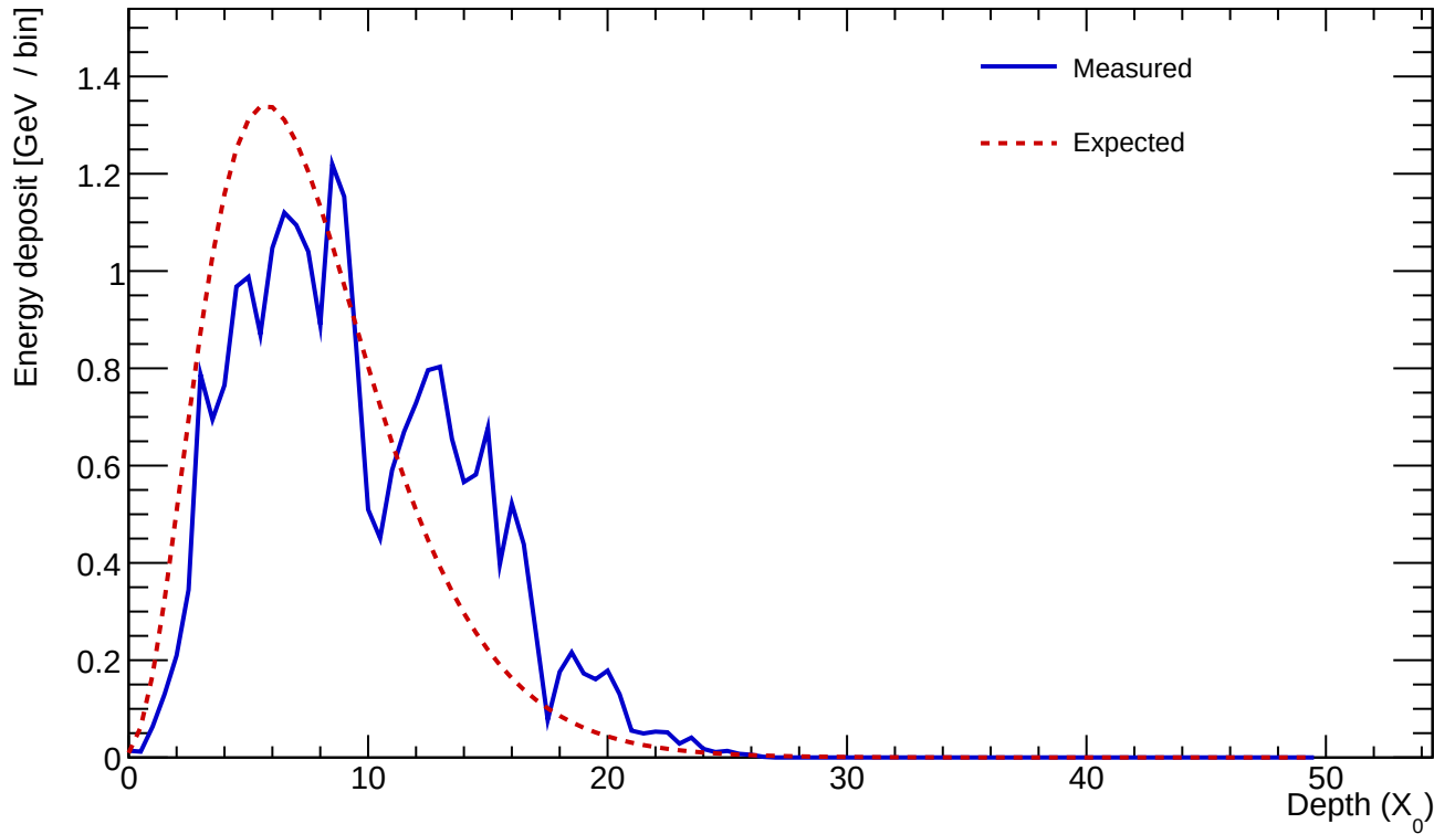
Cluster 826 E=24.349 GeV profileStart=1.00 X_0 \chi=0.2915
