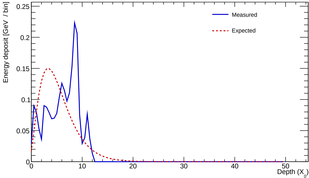
Cluster 194 E=2.166 GeV profileStart=1.50 X_0 \chi=0.4873
