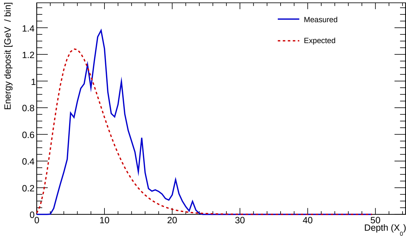
Cluster 472 E=22.402 GeV profileStart=2.50 X_0 \chi=0.1675
