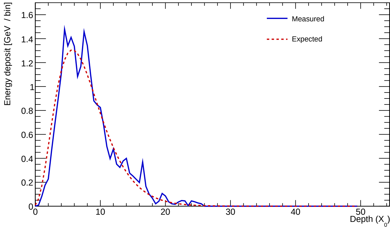
Cluster 122 E=23.656 GeV profileStart=0.50 X_0 \chi=0.1489
