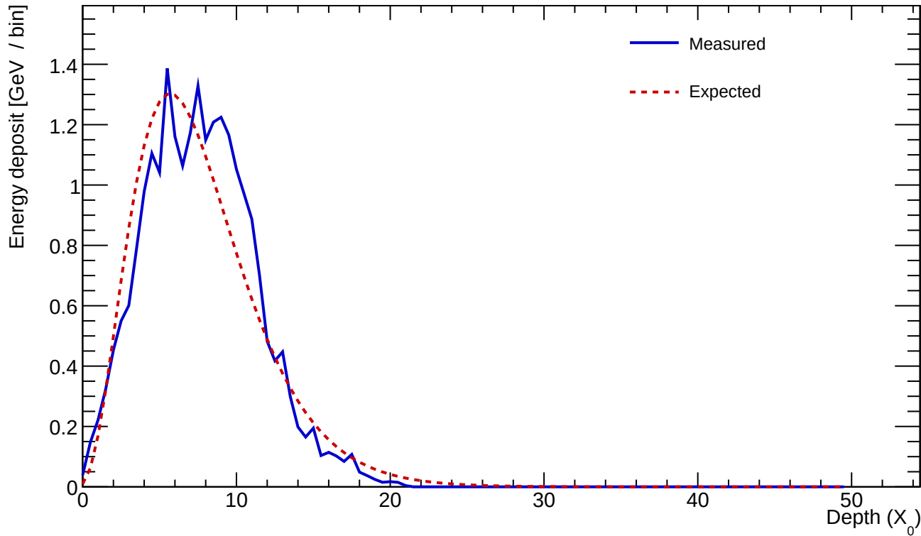
Cluster 346 E=23.596 GeV profileStart=0.50 X_0 \chi=0.1710
