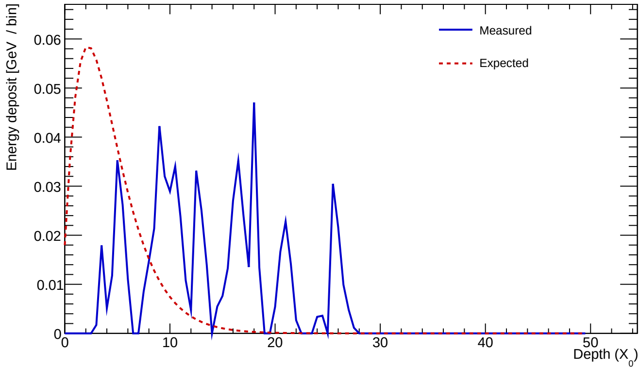
Cluster 127 E=0.725 GeV profileStart=8.00 X_0 \chi=0.9296
