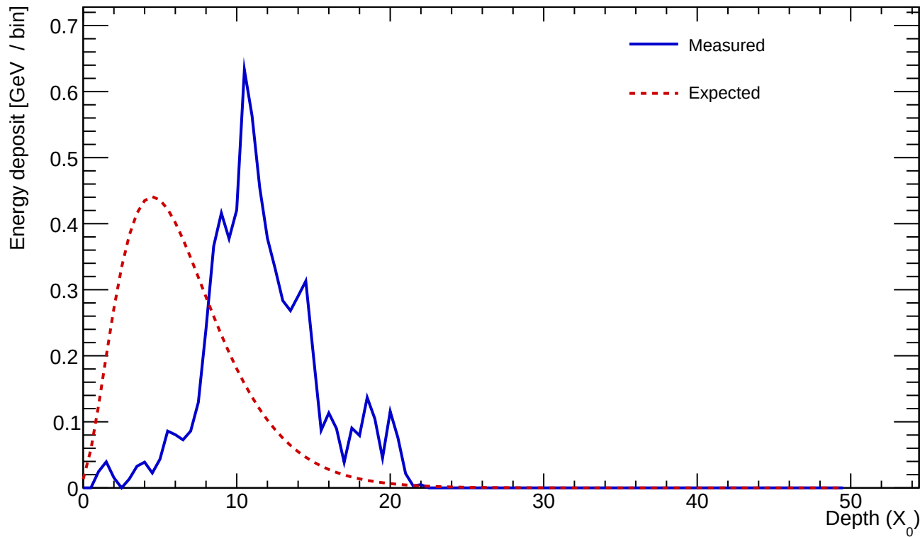
Cluster 13 E=7.228 GeV profileStart=6.00 X_0 \chi=0.2652
