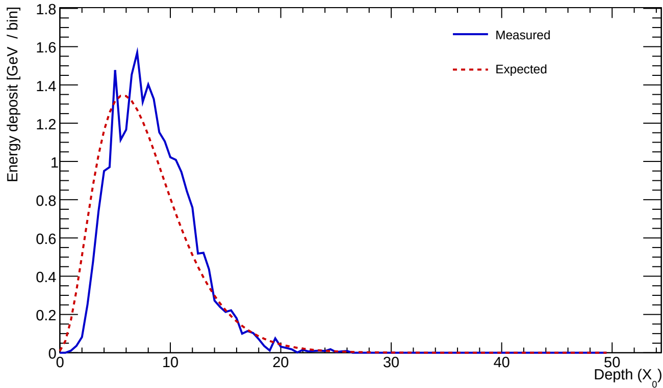
Cluster 68 E=24.446 GeV profileStart=1.00 X_0 \chi=0.1320
