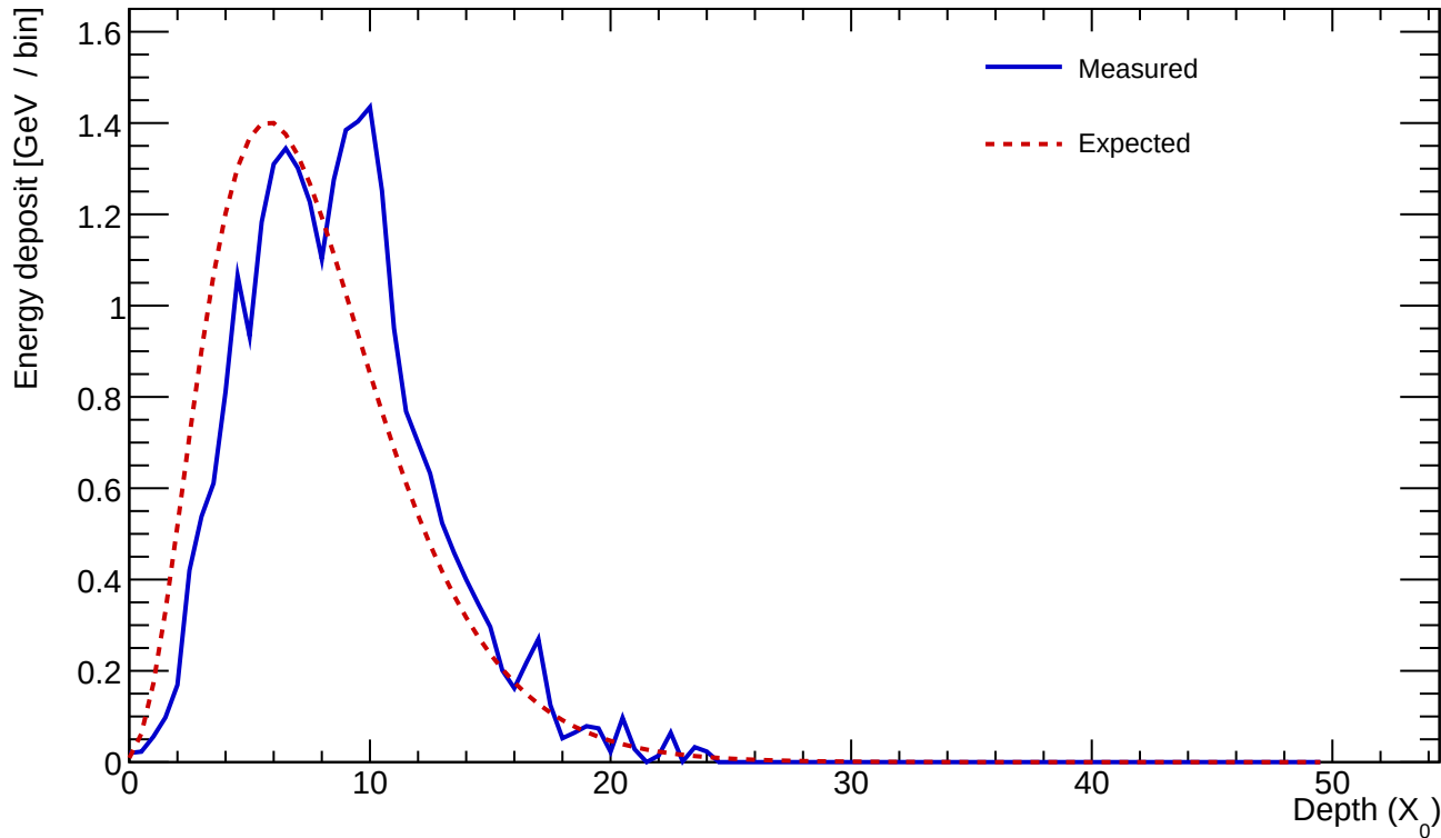
Cluster 269 E=25.570 GeV profileStart=1.00 X_0 \chi=0.1368
