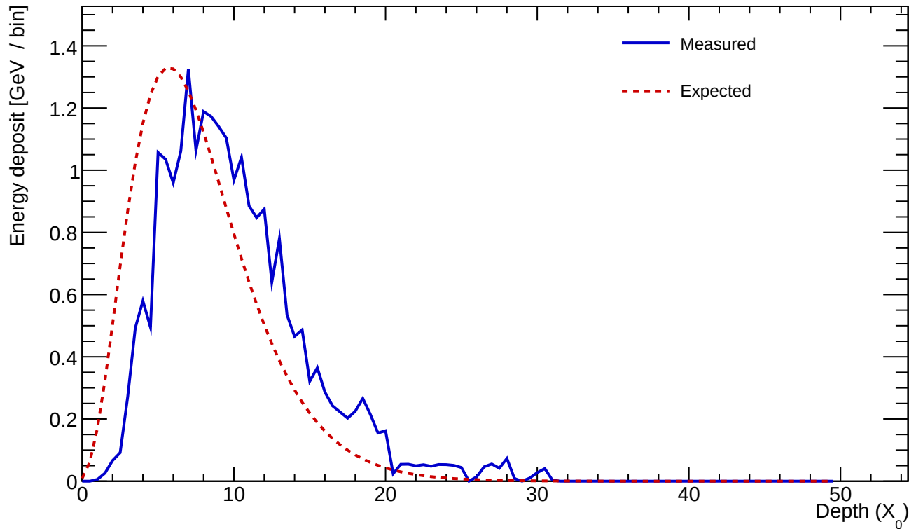
Cluster 214 E=24.139 GeV profileStart=2.00 X_0 \chi=0.1543
