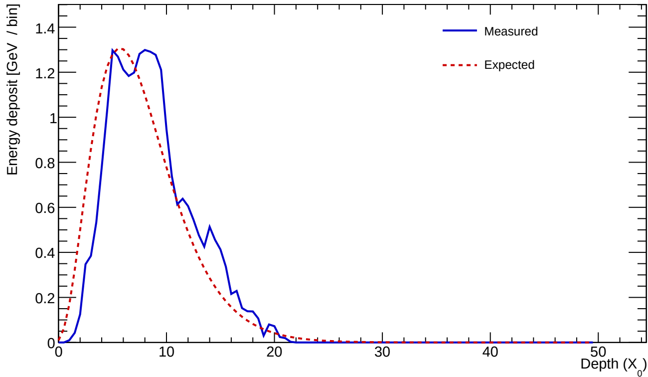
Cluster 139 E=23.682 GeV profileStart=1.00 X_0 \chi=0.1105
