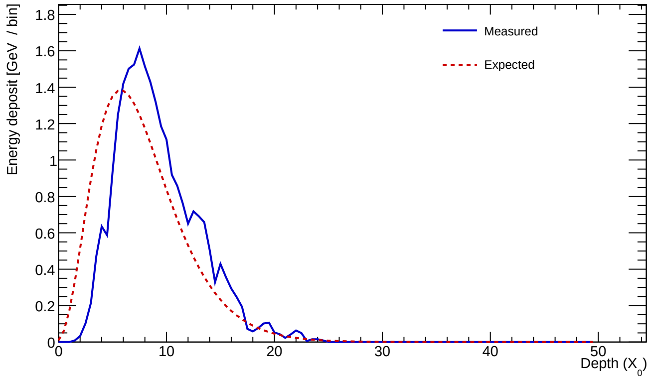
Cluster 831 E=25.193 GeV profileStart=1.50 X_0 \chi=0.1250
