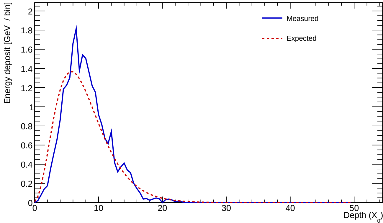
Cluster 899 E=24.890 GeV profileStart=1.00 X_0 \chi=0.1540
