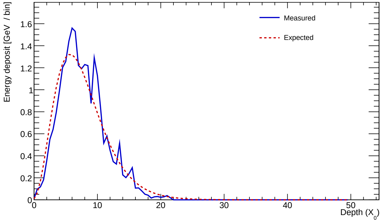
Cluster 659 E=23.971 GeV profileStart=0.50 X_0 \chi=0.1539
