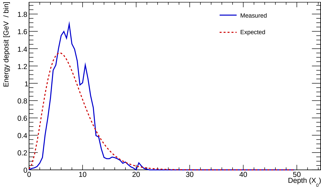
Cluster 449 E=24.561 GeV profileStart=1.00 X_0 \chi=0.2061
