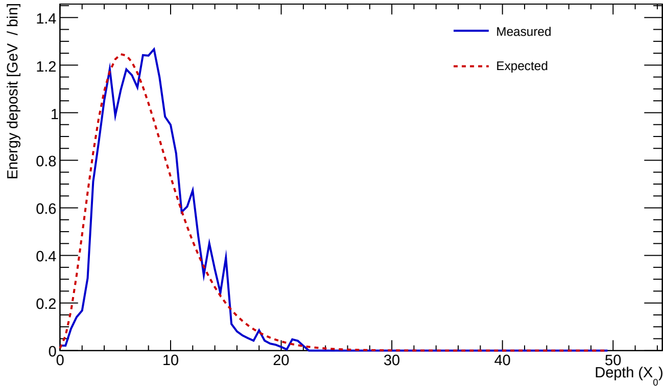
Cluster 780 E=22.502 GeV profileStart=0.50 X_0 \chi=0.1537
