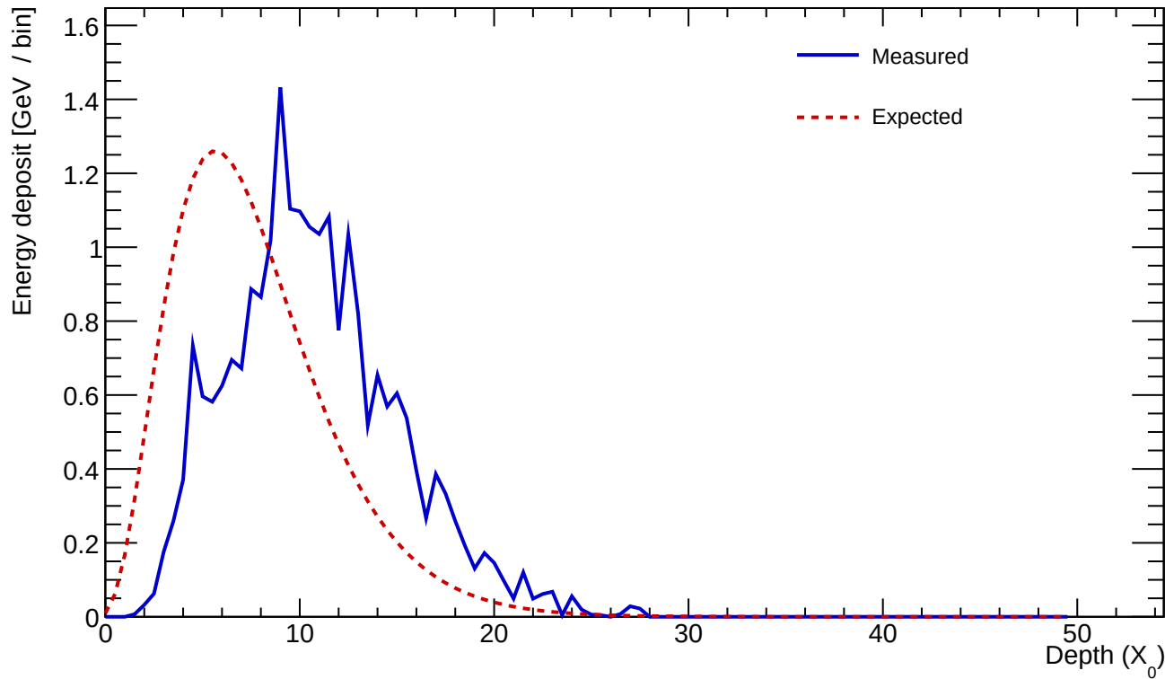
Cluster 583 E=22.778 GeV profileStart=3.50 X_0 \chi=0.2243
