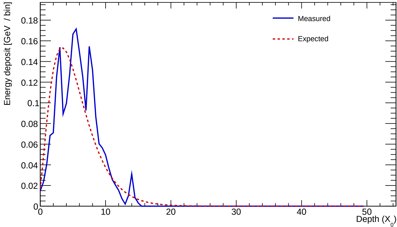
Cluster 290 E=2.219 GeV profileStart=0.50 X_0 \chi=0.2563
