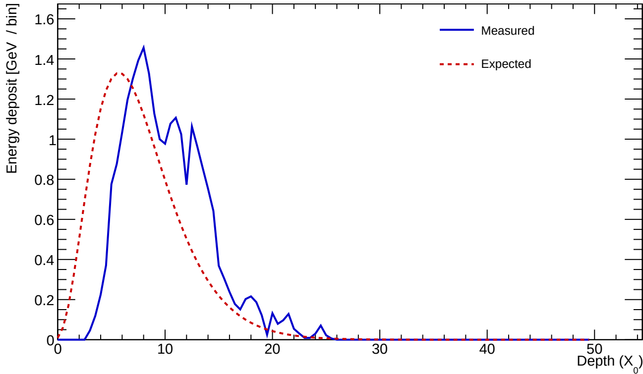
Cluster 900 E=24.144 GeV profileStart=2.50 X_0 \chi=0.1495
