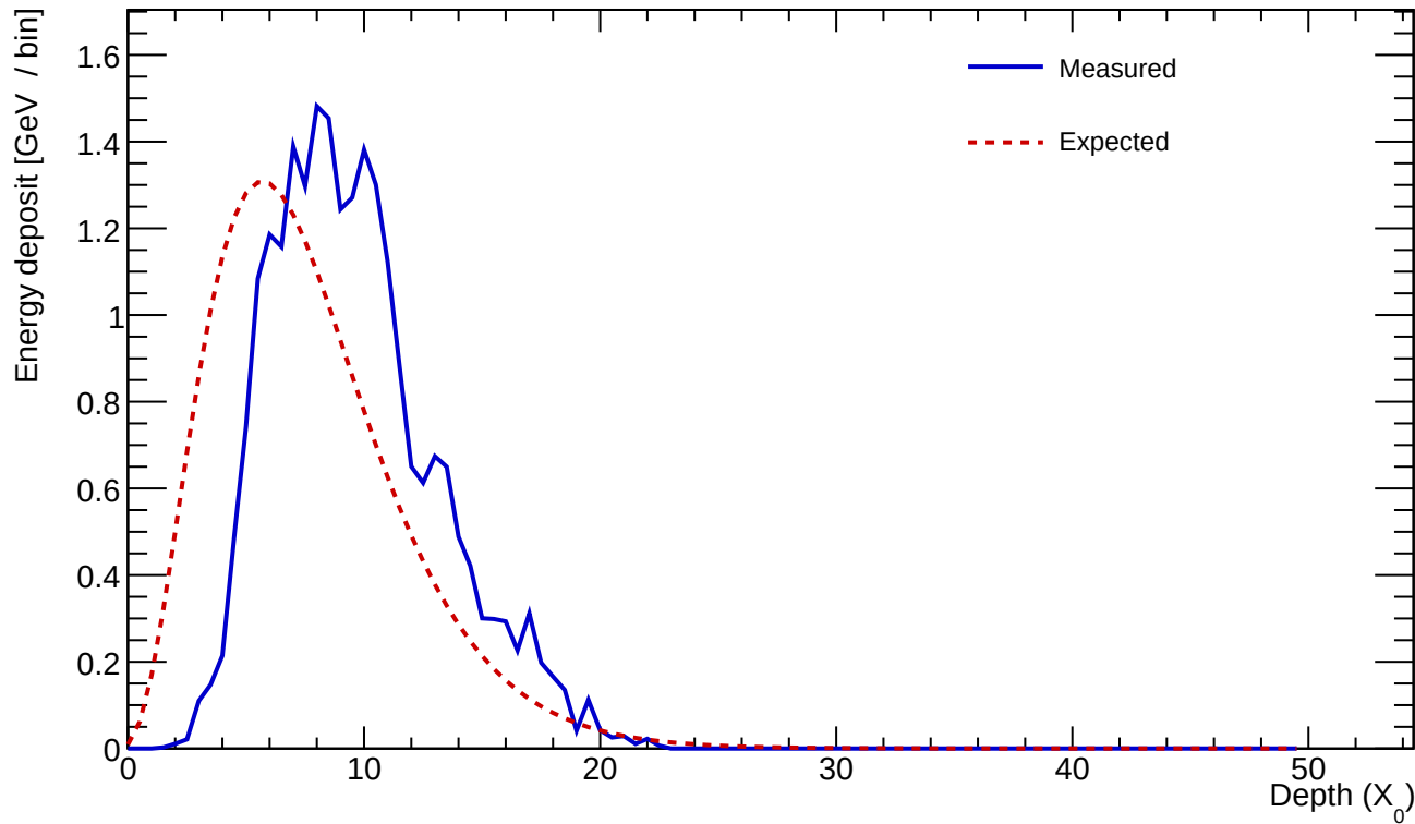
Cluster 375 E=23.706 GeV profileStart=2.50 X_0 \chi=0.1330
