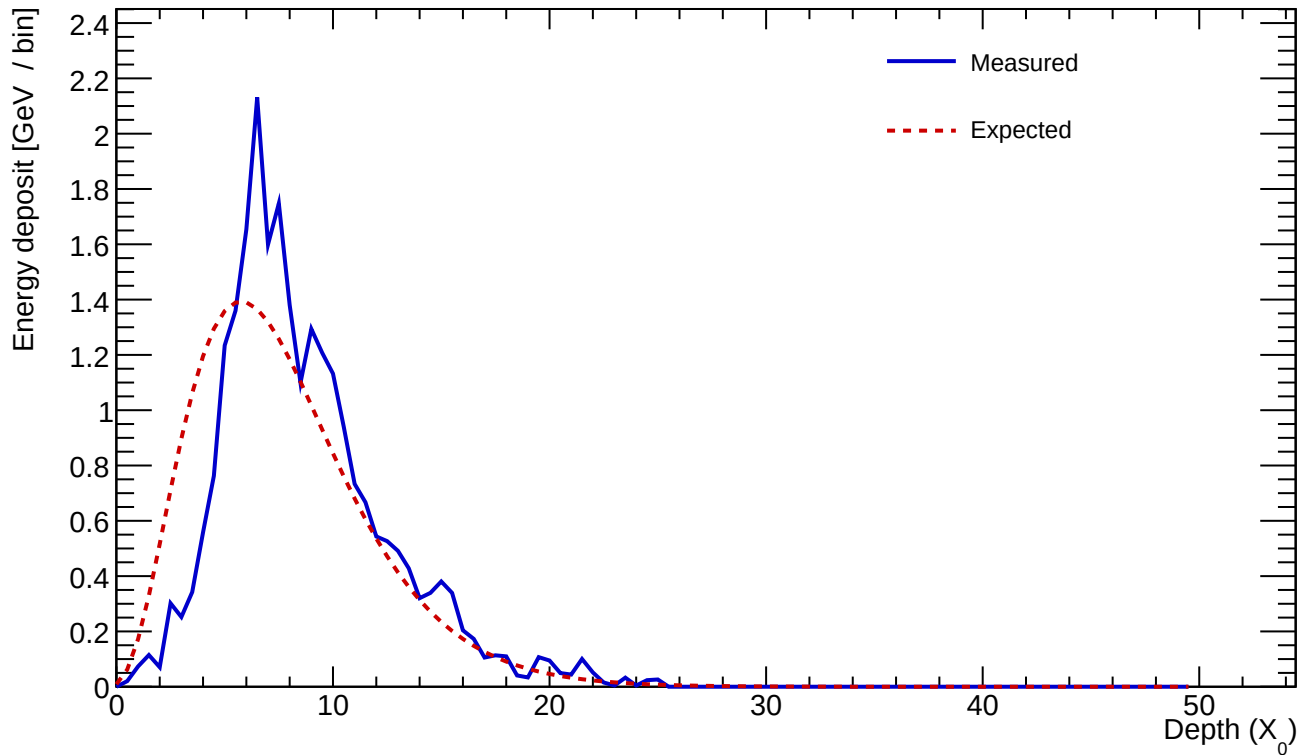
Cluster 493 E=25.378 GeV profileStart=1.00 X_0 \chi=0.2010
