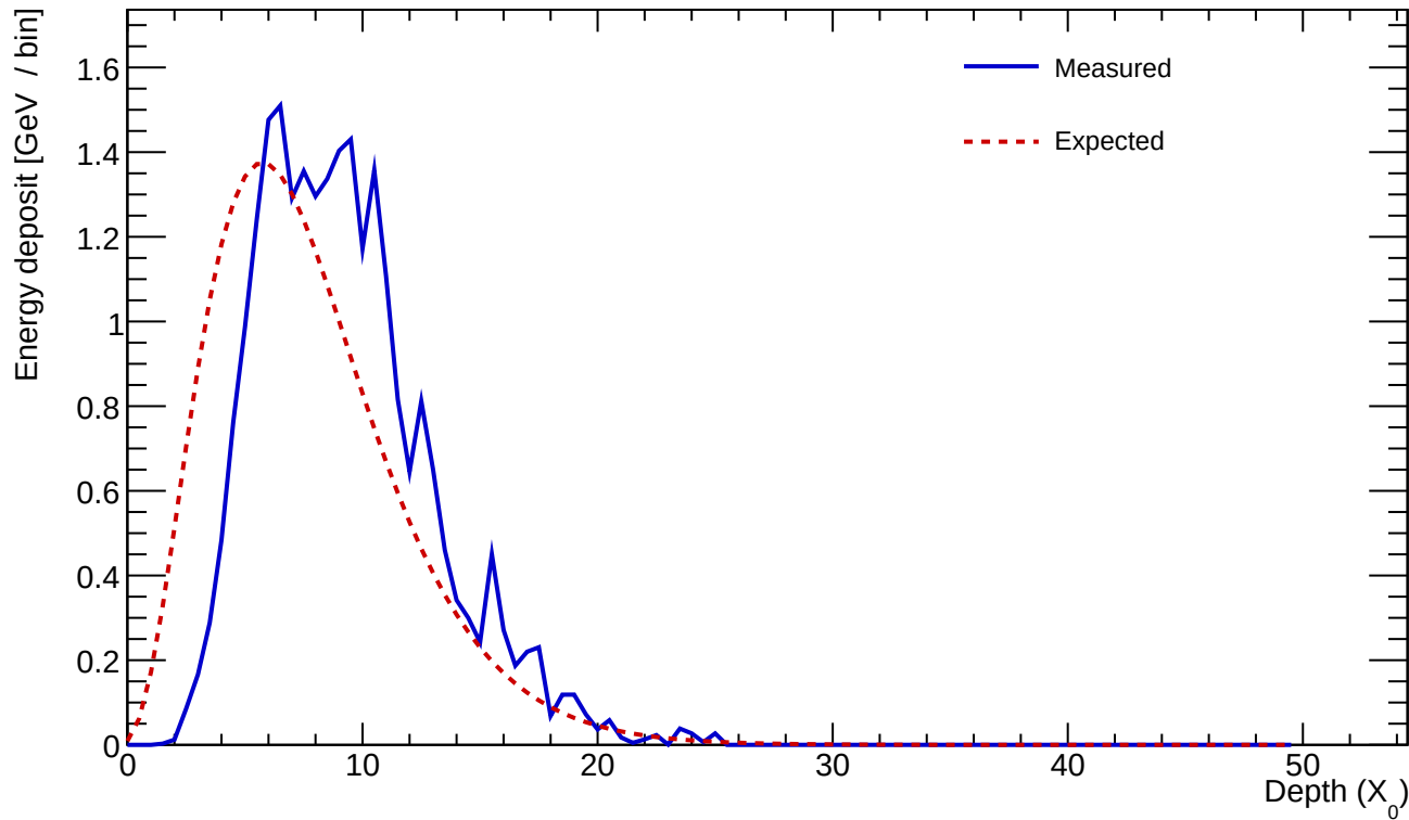
Cluster 745 E=25.023 GeV profileStart=2.00 X_0 \chi=0.1405
