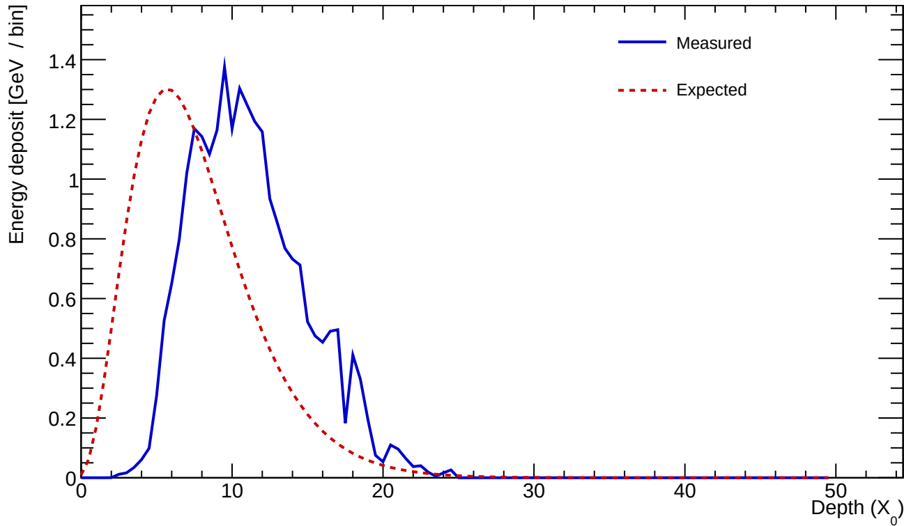
Cluster 617 E=23.593 GeV profileStart=3.50 X_0 \chi=0.1072
