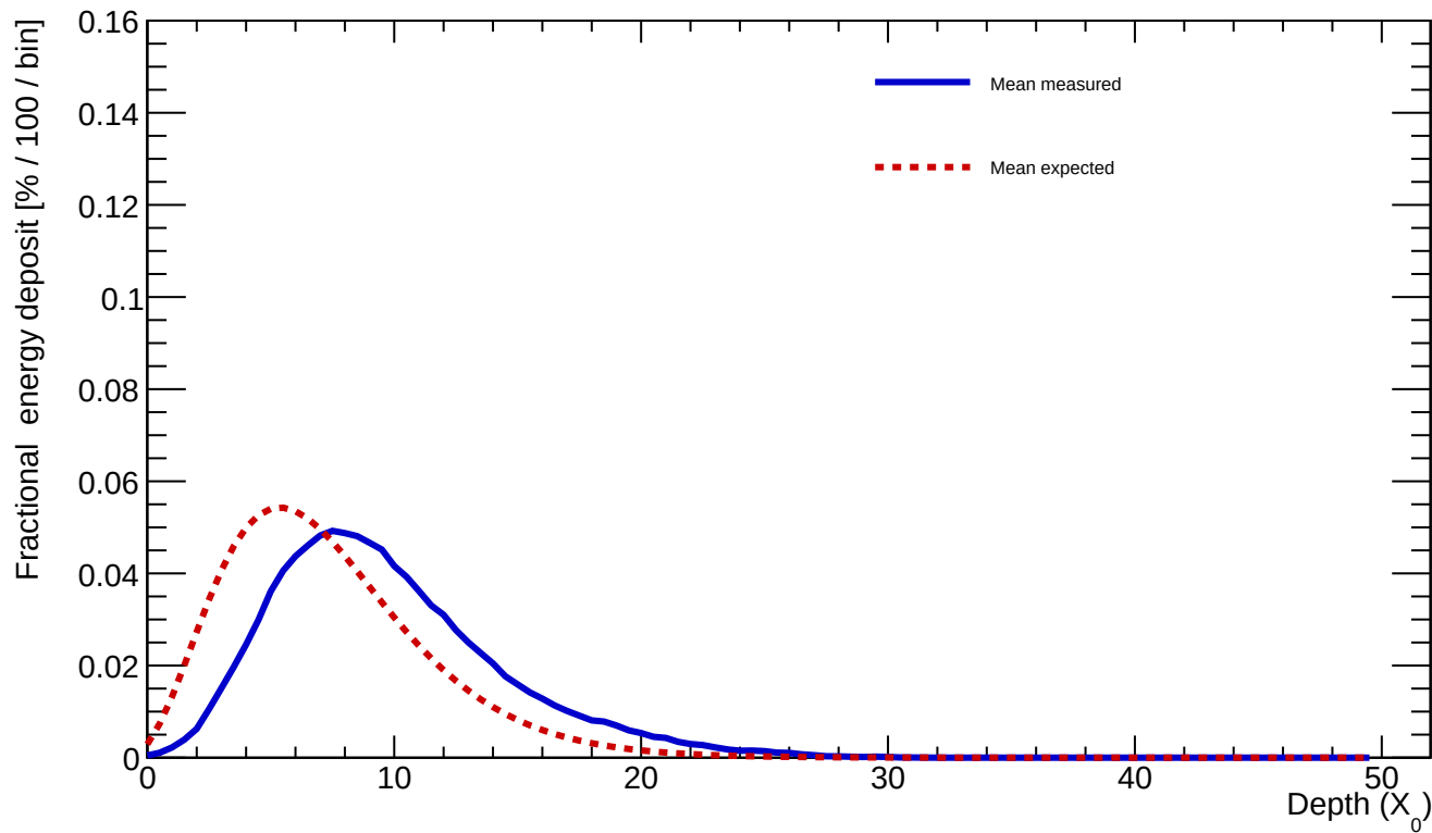
Average longitudinal profile (926 clusters): measured vs expected
