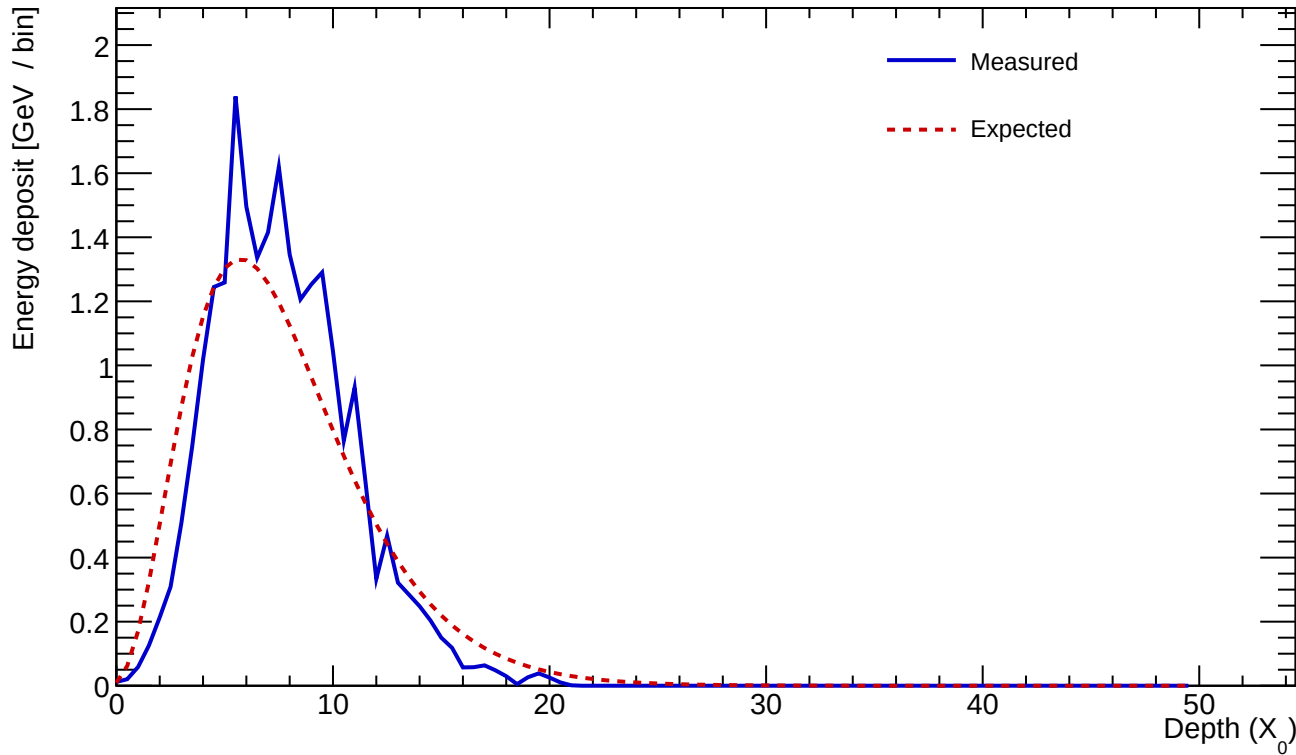
Cluster 146 E=24.186 GeV profileStart=0.50 X_0 \chi=0.1944
