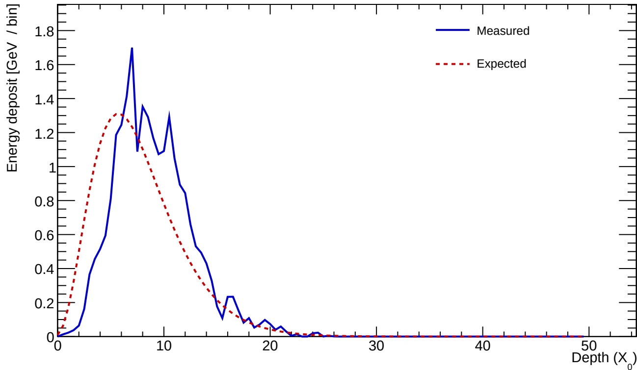
Cluster 821 E=23.752 GeV profileStart=1.50 X_0 \chi=0.1475
