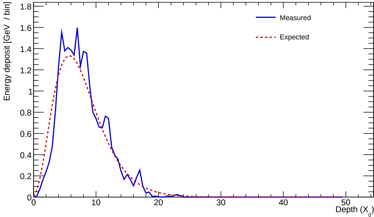
Cluster 566 E=24.212 GeV profileStart=0.50 X_0 \chi=0.1674
