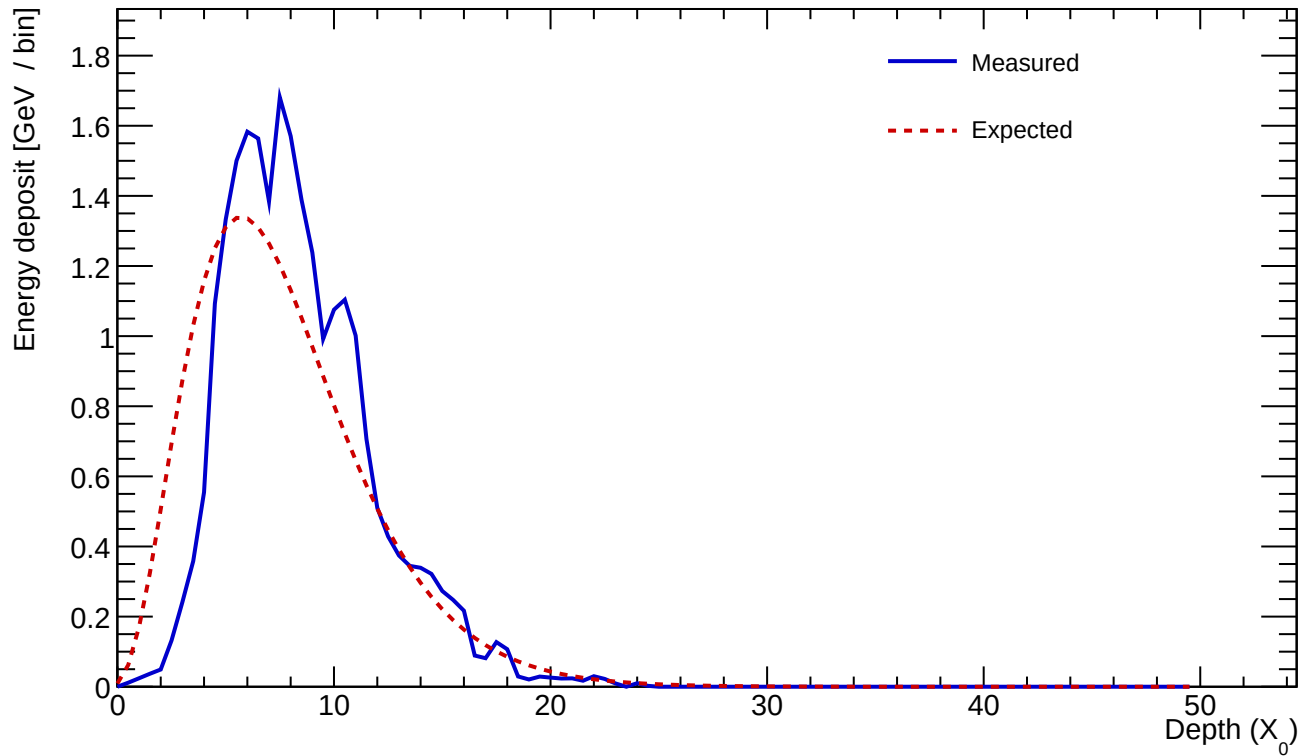
Cluster 710 E=24.328 GeV profileStart=1.00 X_0 \chi=0.2072
