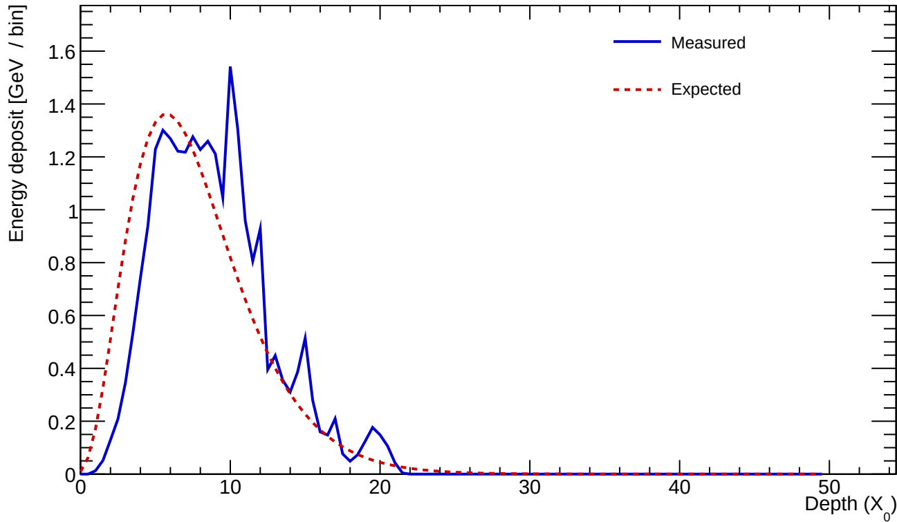
Cluster 156 E=24.766 GeV profileStart=1.50 X_0 \chi=0.1543
