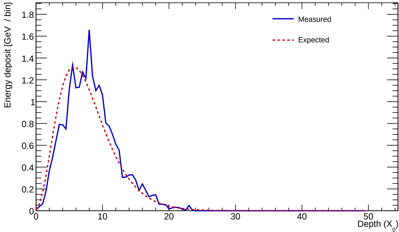
Cluster 86 E=23.904 GeV profileStart=1.00 X_0 \chi=0.1404
