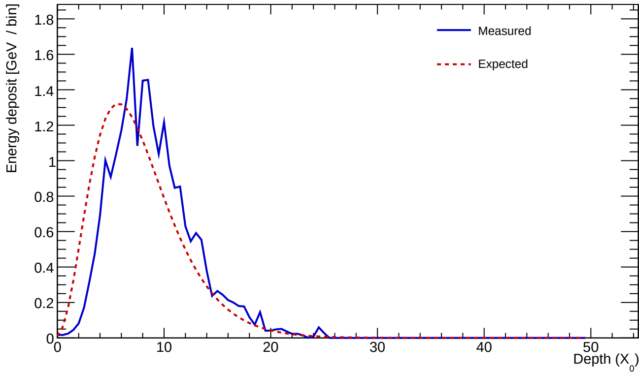
Cluster 830 E=23.980 GeV profileStart=1.50 X_0 \chi=0.1204
