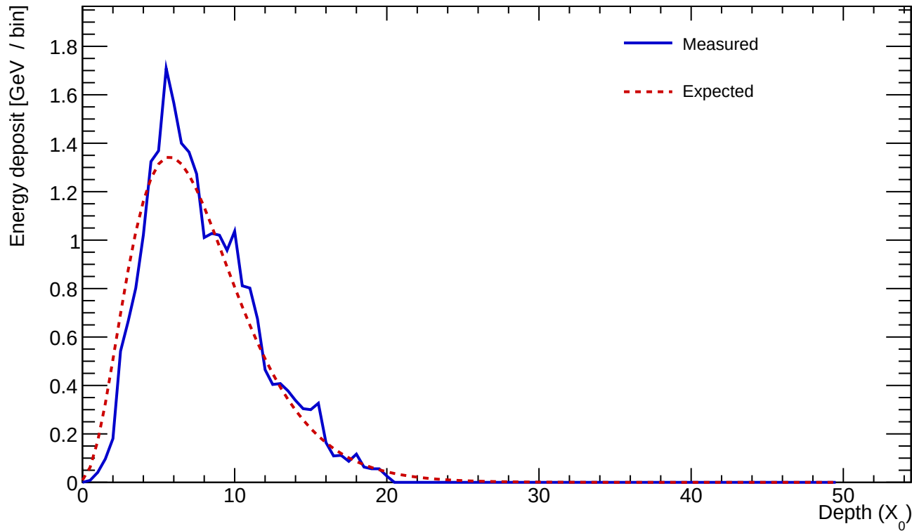
Cluster 413 E=24.415 GeV profileStart=0.50 X_0 \chi=0.1086
