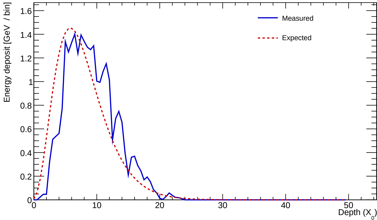
Cluster 579 E=26.544 GeV profileStart=1.50 X_0 \chi=0.1393
