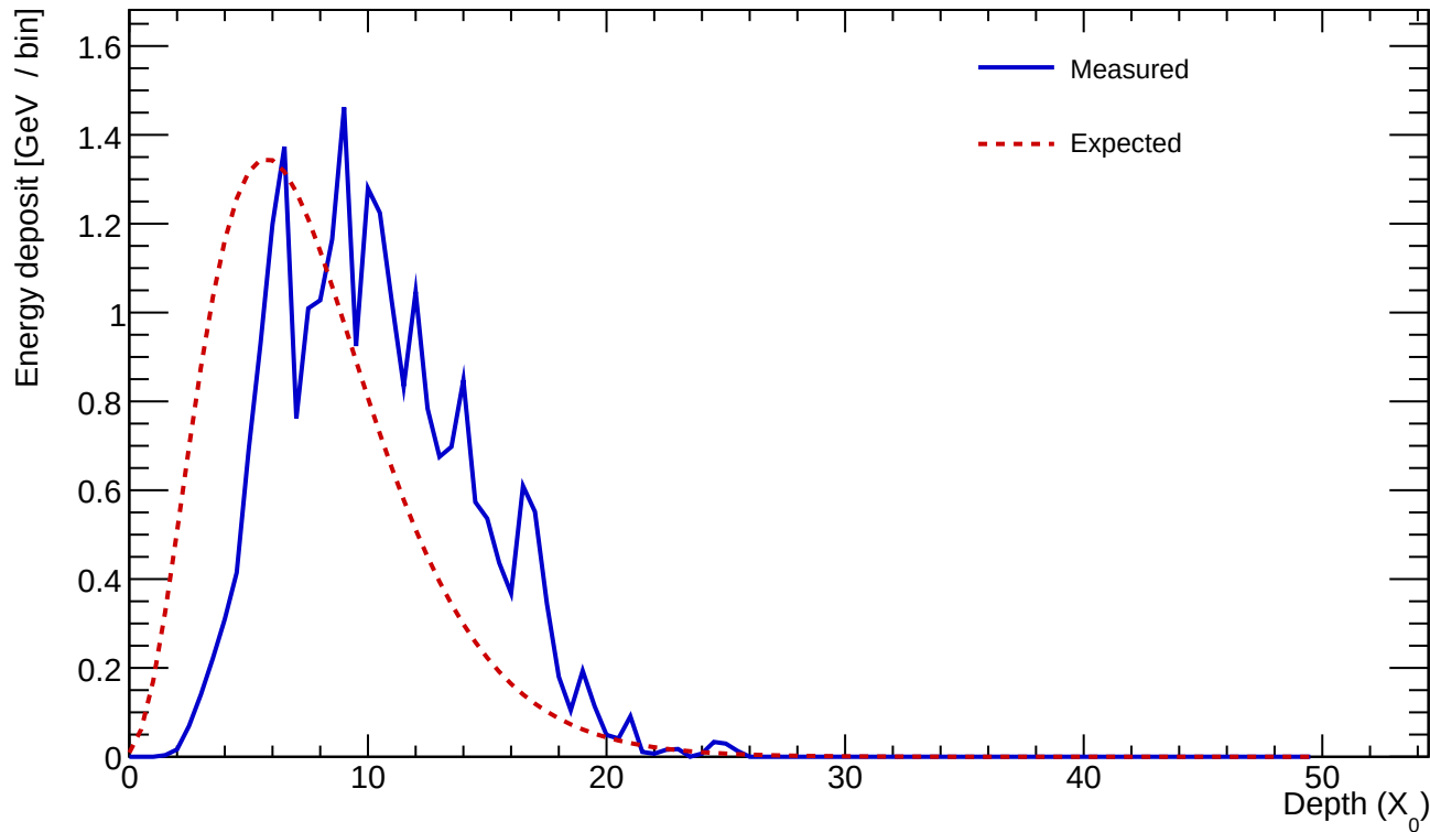
Cluster 690 E=24.463 GeV profileStart=2.50 X_0 \chi=0.1972
