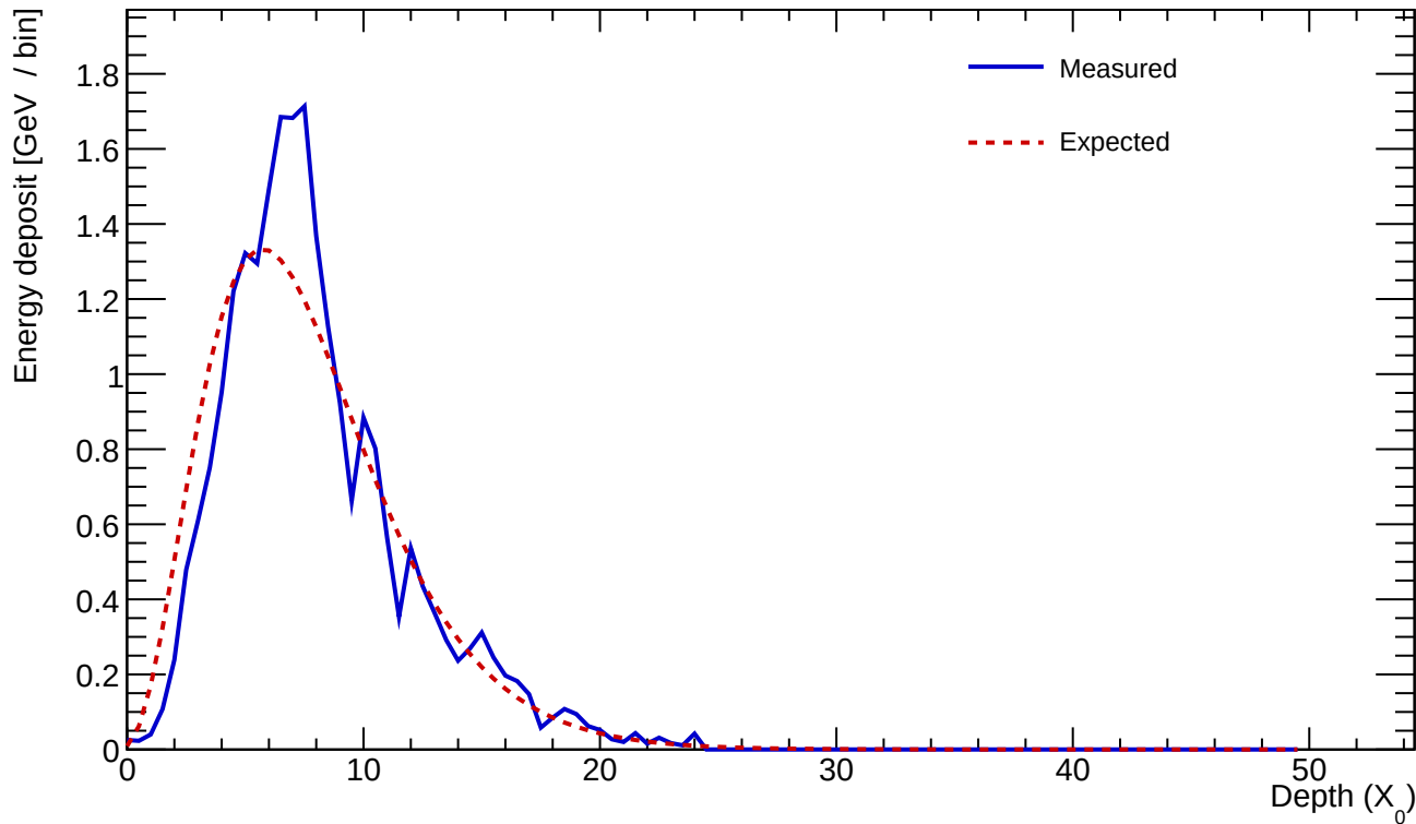
Cluster 448 E=24.207 GeV profileStart=0.50 X_0 \chi=0.1564
