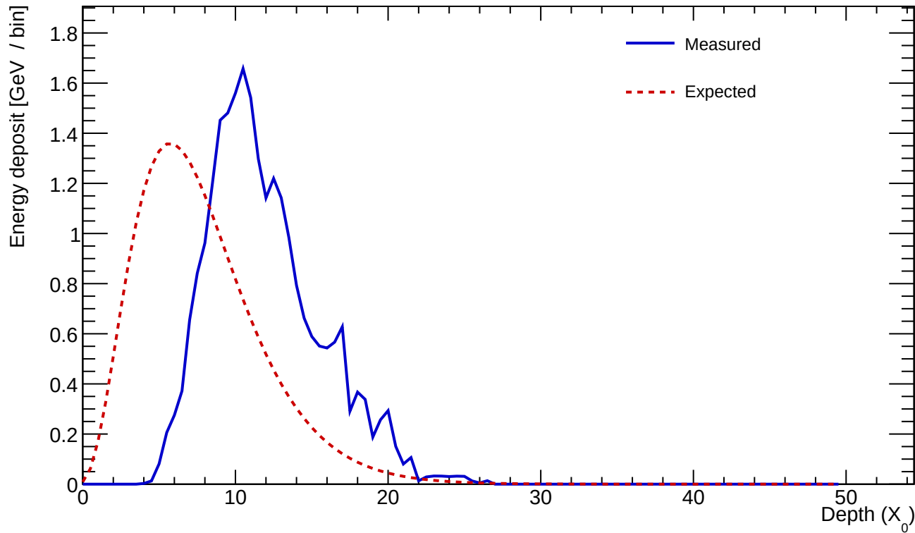
Cluster 220 E=24.728 GeV profileStart=4.50 X_0 \chi=0.1327
