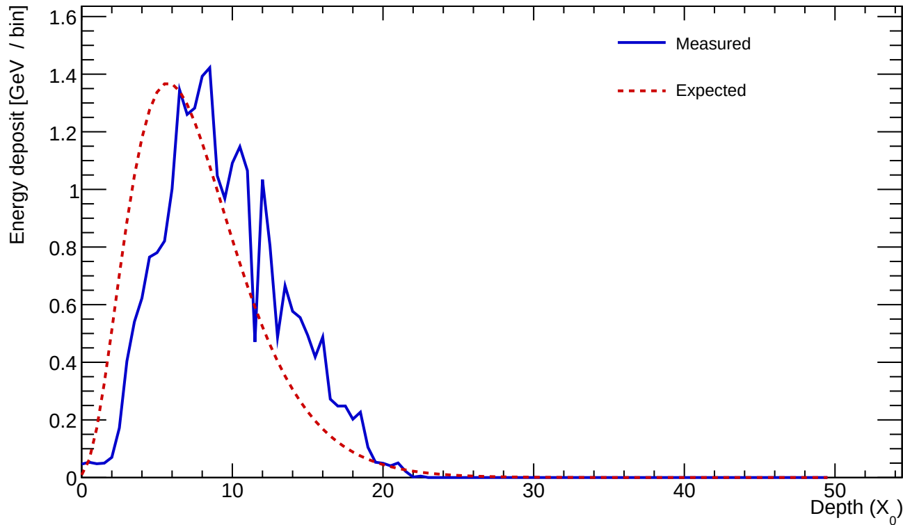
Cluster 338 E=24.915 GeV profileStart=2.00 X_0 \chi=0.1776
