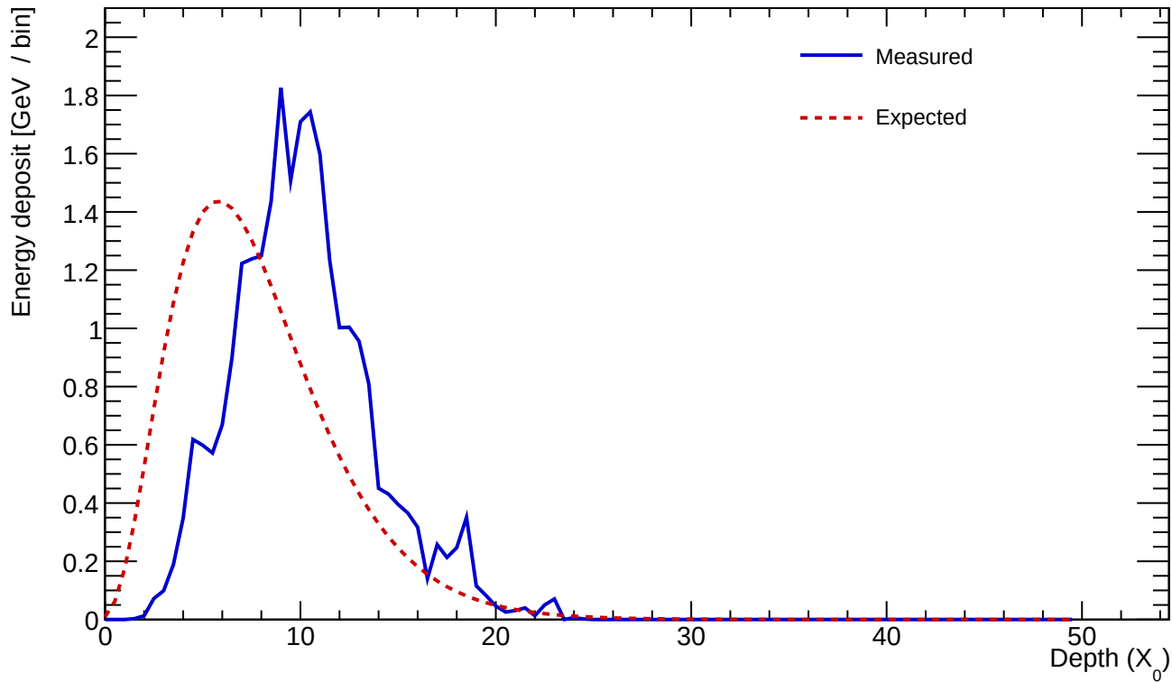
Cluster 717 E=26.268 GeV profileStart=3.00 X_0 \chi=0.2111
