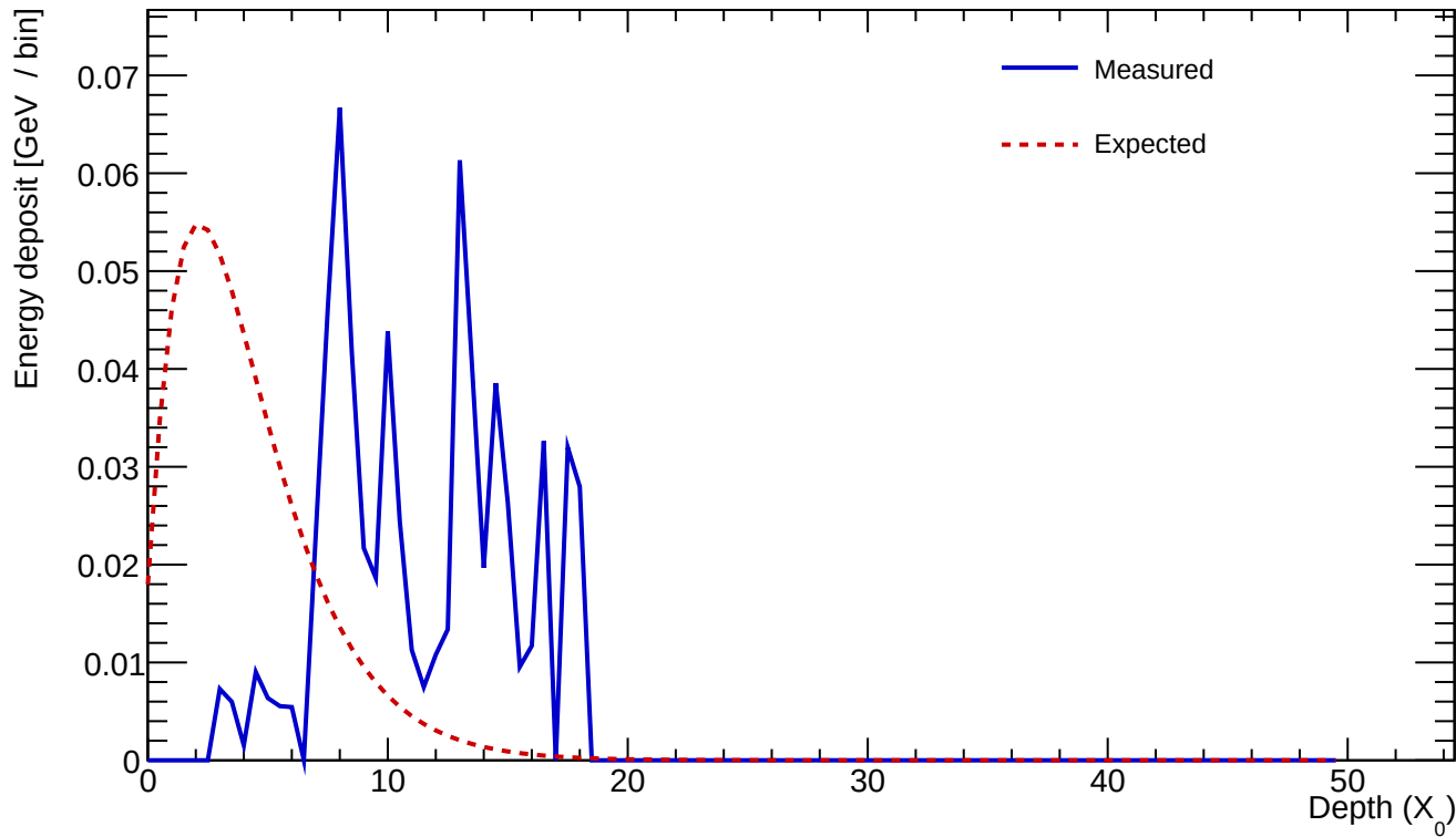
Cluster 347 E=0.671 GeV profileStart=6.50 X_0 \chi=0.6564
