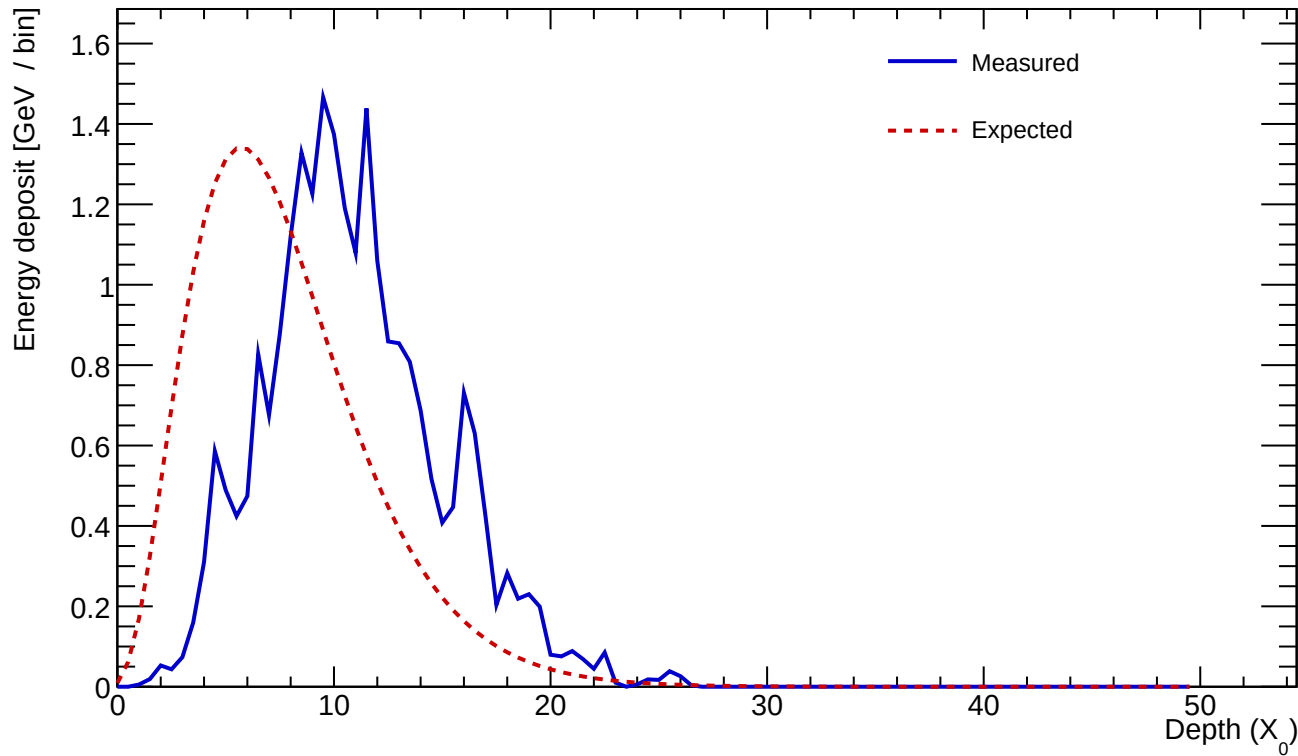
Cluster 141 E=24.364 GeV profileStart=3.50 X_0 \chi=0.1977
