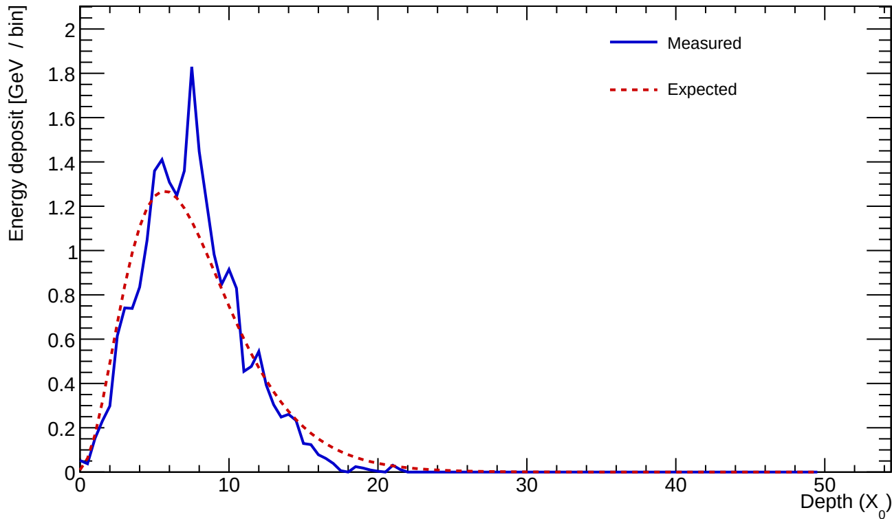
Cluster 409 E=22.948 GeV profileStart=0.50 X_0 \chi=0.1853
