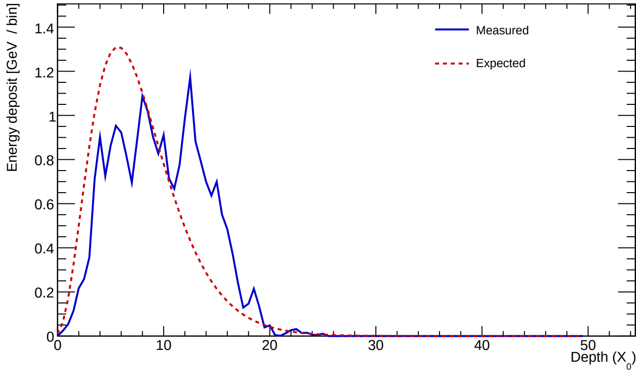
Cluster 80 E=23.760 GeV profileStart=1.50 X_0 \chi=0.3427
