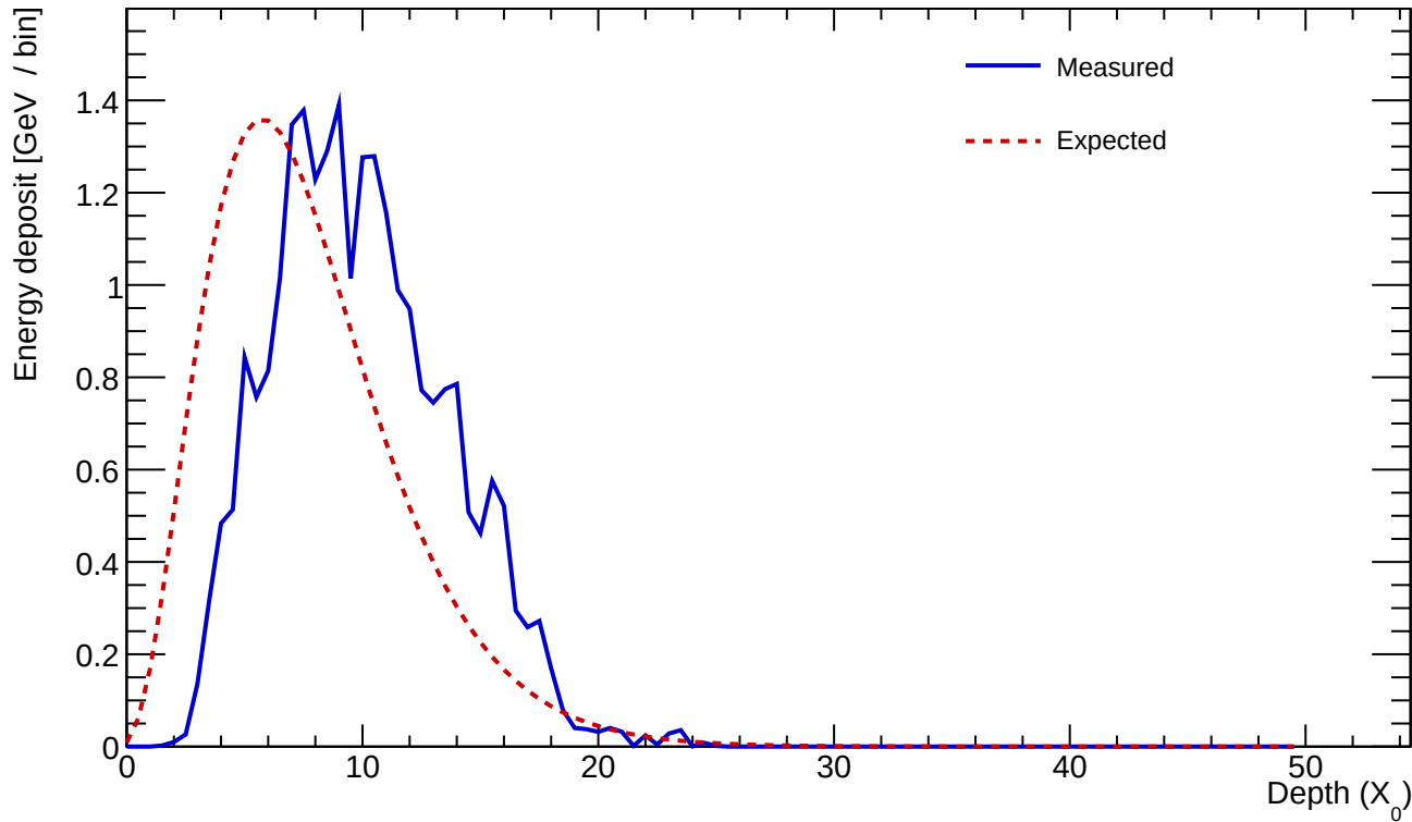
Cluster 358 E=24.722 GeV profileStart=2.50 X_0 \chi=0.1402
