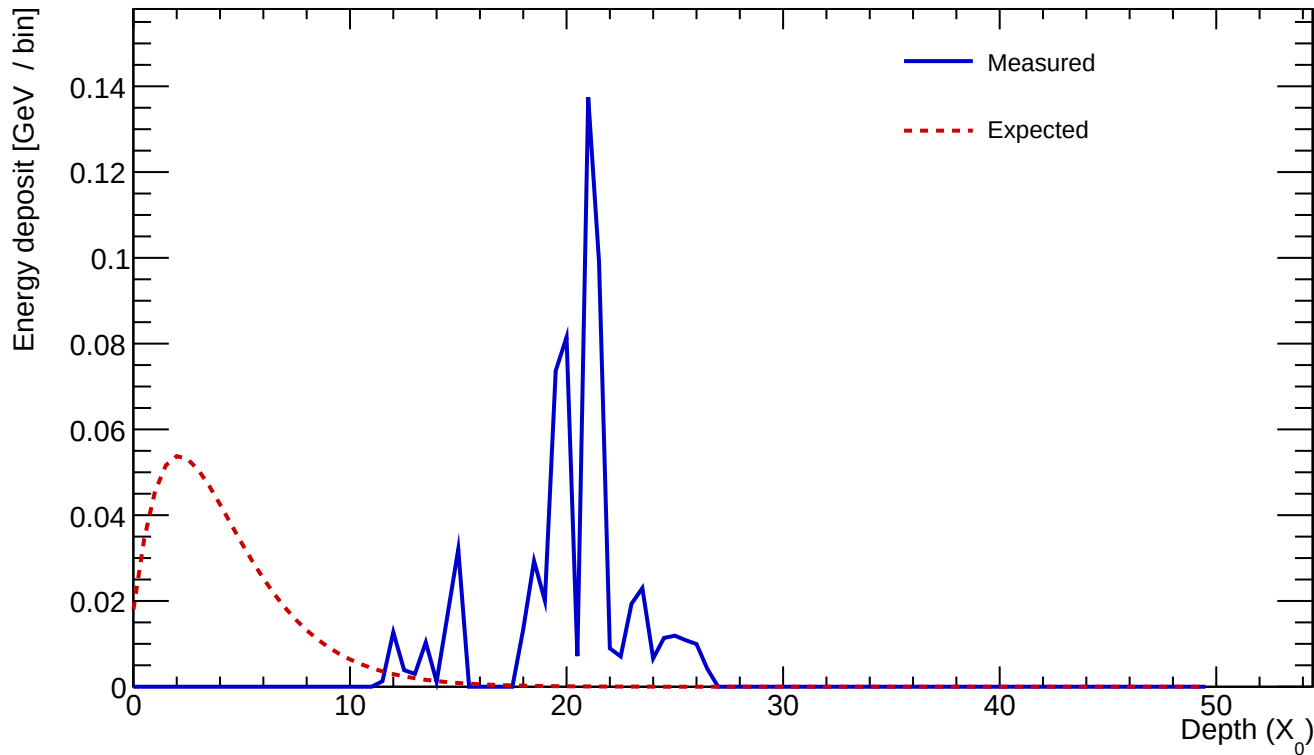
Cluster 754 E=0.656 GeV profileStart=18.00 X_0 \chi=0.7312
