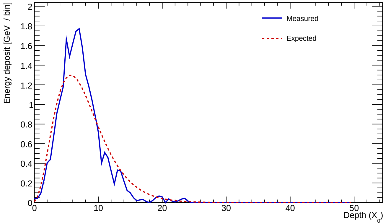
Cluster 235 E=23.529 GeV profileStart=0.50 X_0 \chi=0.2541
