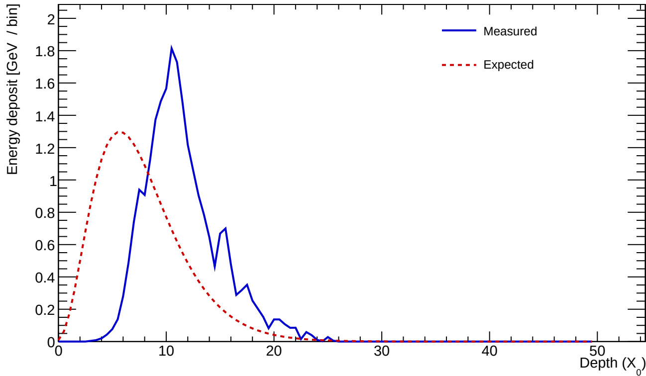
Cluster 491 E=23.503 GeV profileStart=4.50 X_0 \chi=0.1848
