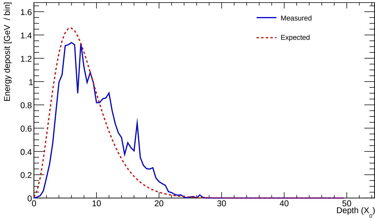
Cluster 345 E=26.719 GeV profileStart=1.00 X_0 \chi=0.1912
