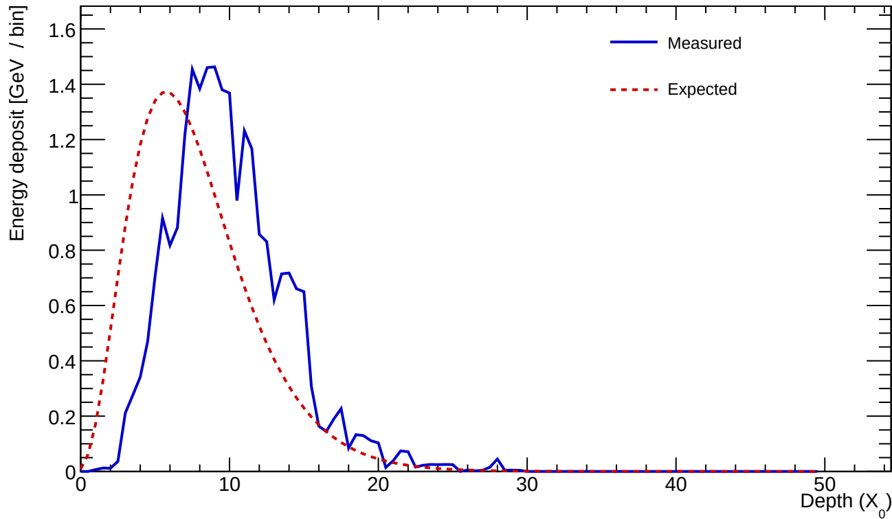
Cluster 763 E=24.986 GeV profileStart=2.50 X_0 \chi=0.1494
