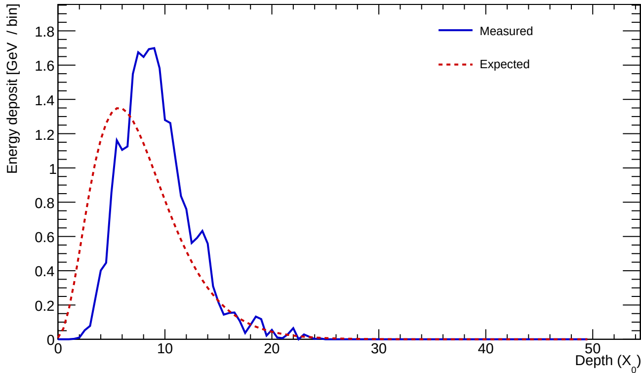
Cluster 190 E=24.547 GeV \text{profileStart}=2.00 X_0 \chi=0.2132
