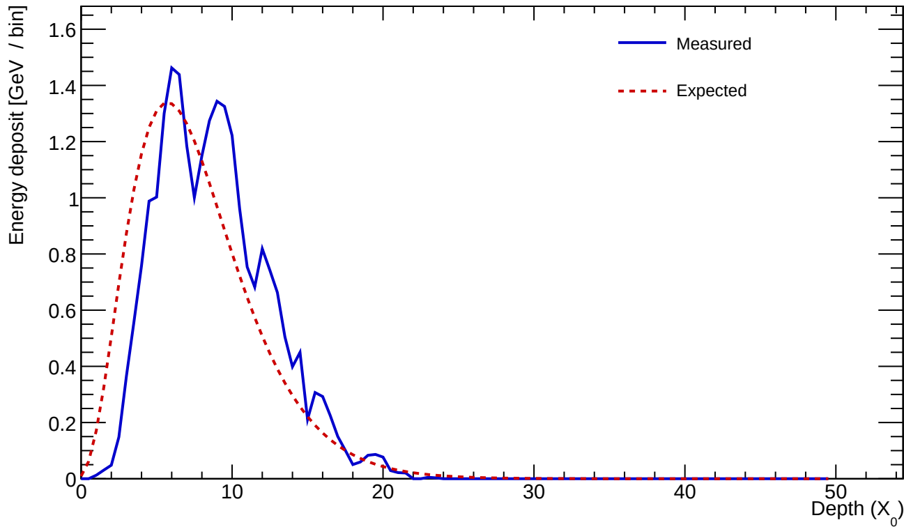
Cluster 593 E=24.312 GeV profileStart=1.50 X_0 \chi=0.1354
