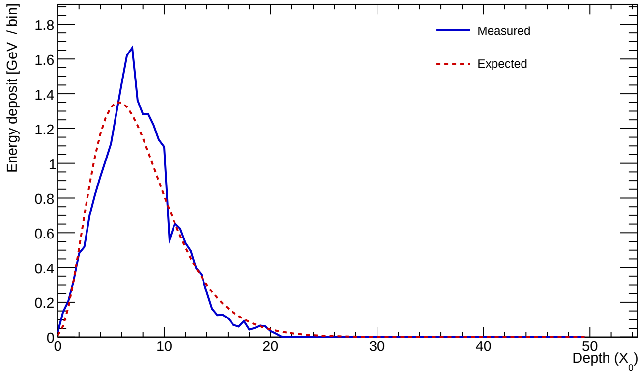
Cluster 273 E=24.591 GeV profileStart=0.50 X_0 \chi=0.1653
