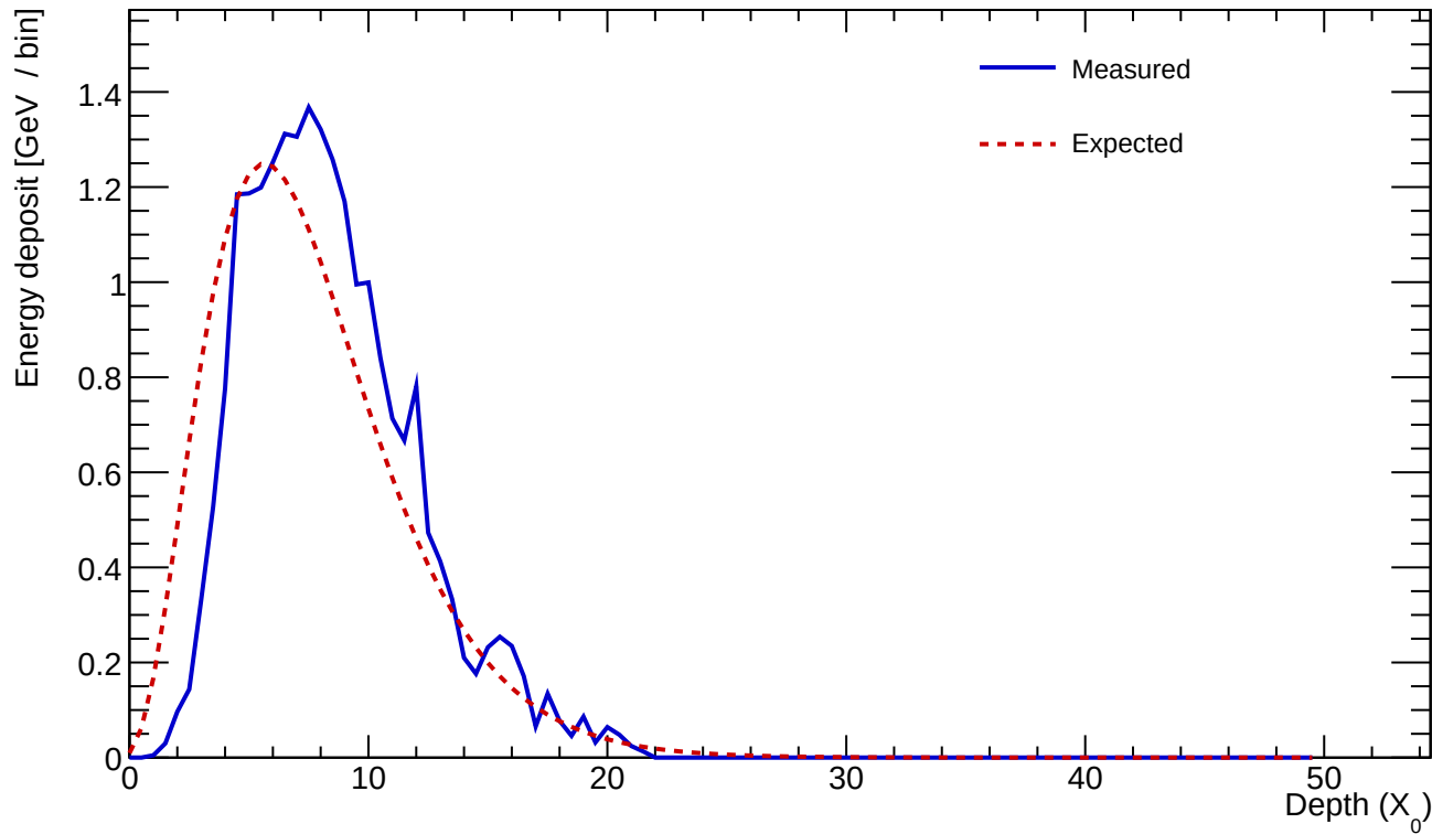
Cluster 438 E=22.554 GeV profileStart=1.00 X_0 \chi=0.1261
