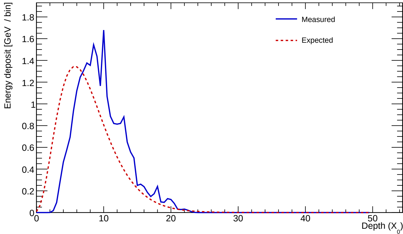
Cluster 556 E=24.428 GeV profileStart=2.00 X_0 \chi=0.1290
