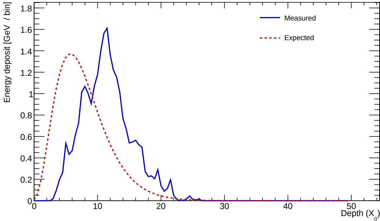
Cluster 633 E=24.949 GeV profileStart=4.00 X_0 \chi=0.2079
