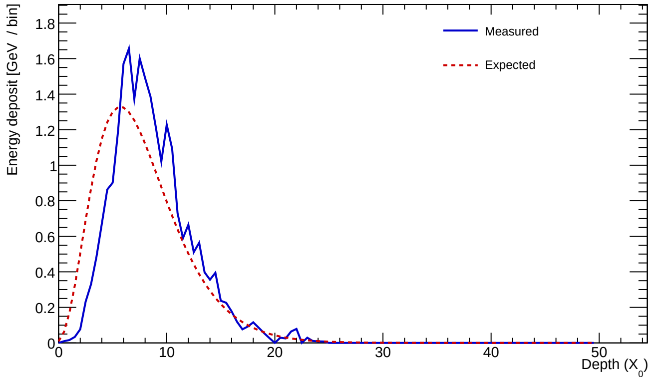
Cluster 176 E=24.117 GeV profileStart=1.50 X_0 \chi=0.1563
