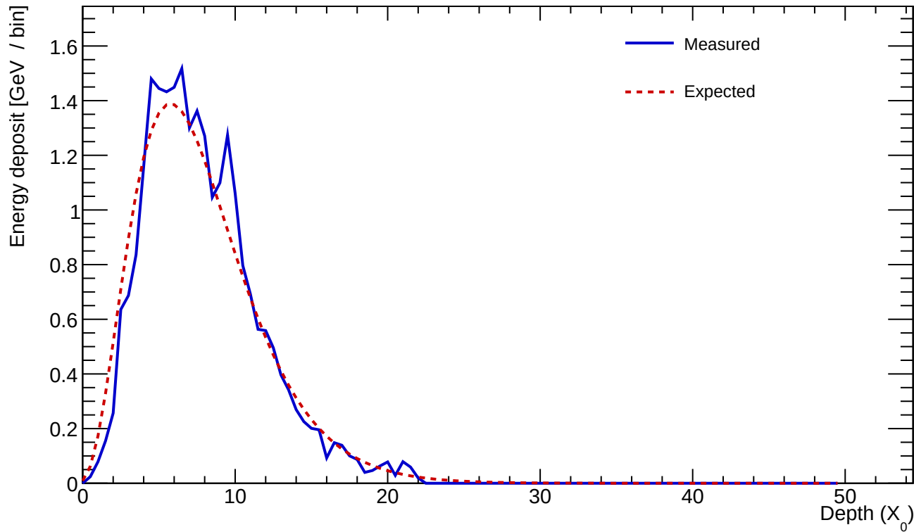
Cluster 661 E=25.287 GeV profileStart=0.50 X_0 \chi=0.1146
