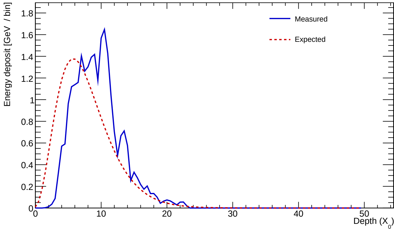
Cluster 203 E=25.070 GeV profileStart=2.00 X_0 \chi=0.1619
