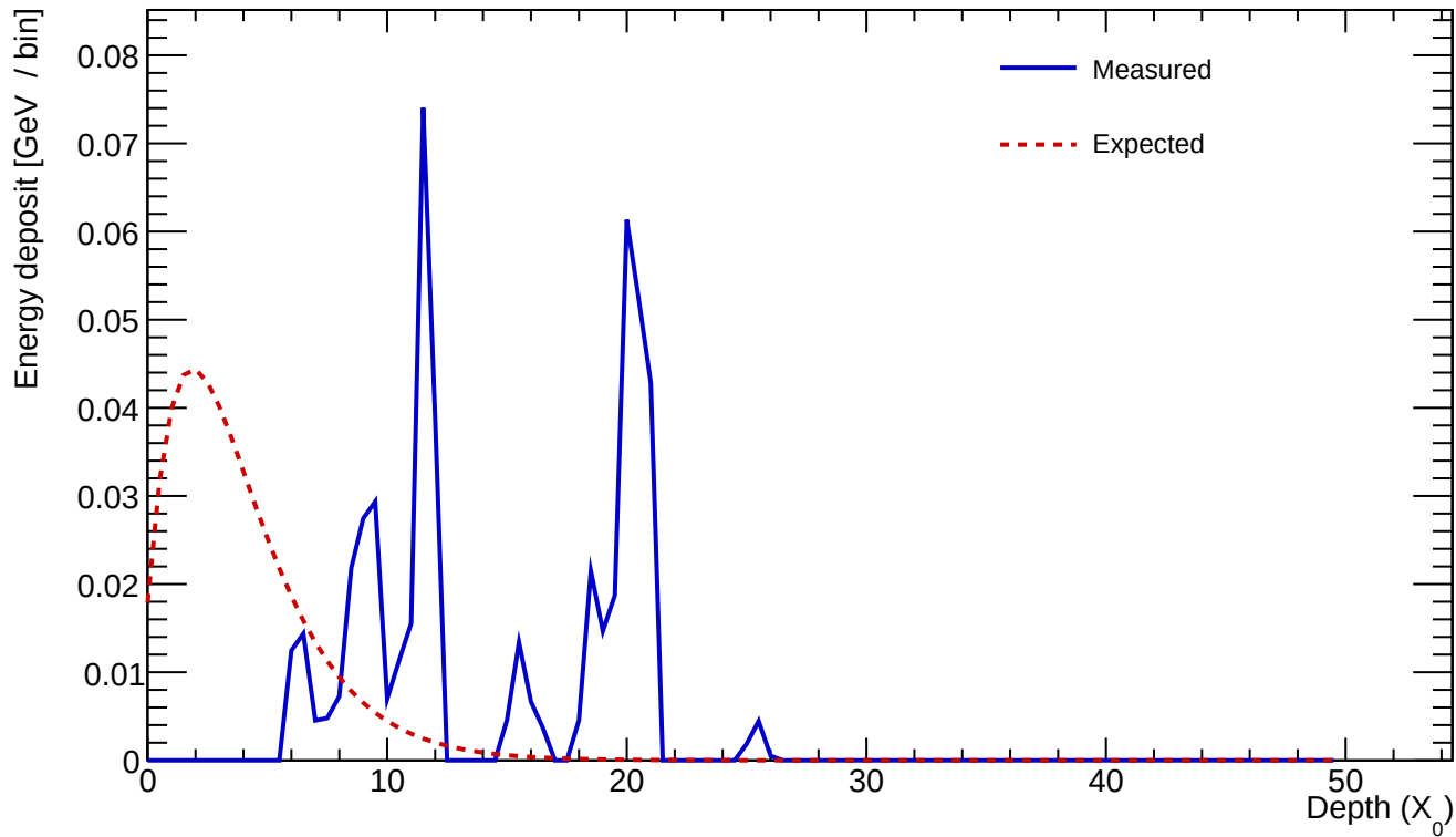
Cluster 98 E=0.520 GeV profileStart=8.50 X_0 \chi=1.0869
