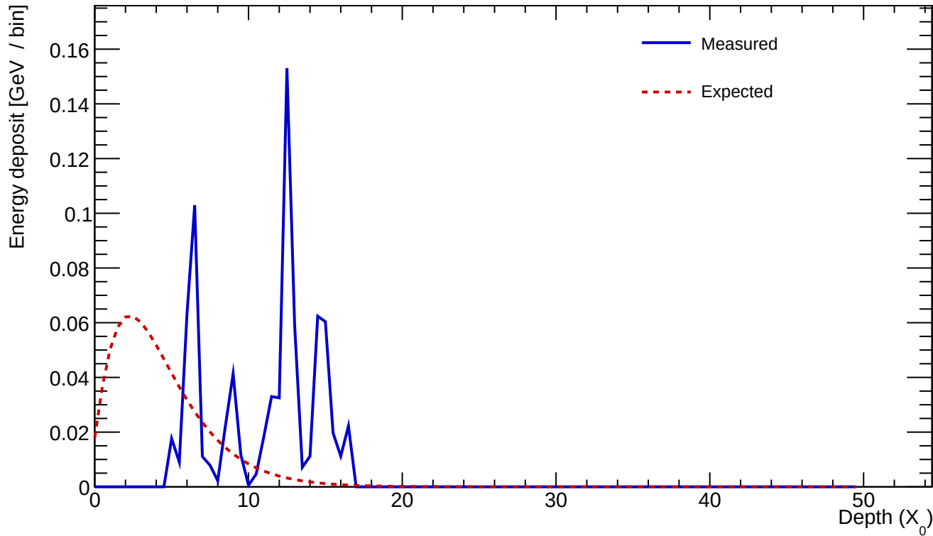
Cluster 151 E=0.785 GeV profileStart=11.00 X_0 \chi=0.7517
