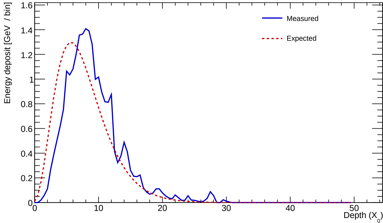
Cluster 188 E=23.496 GeV profileStart=1.50 X_0 \chi=0.1365
