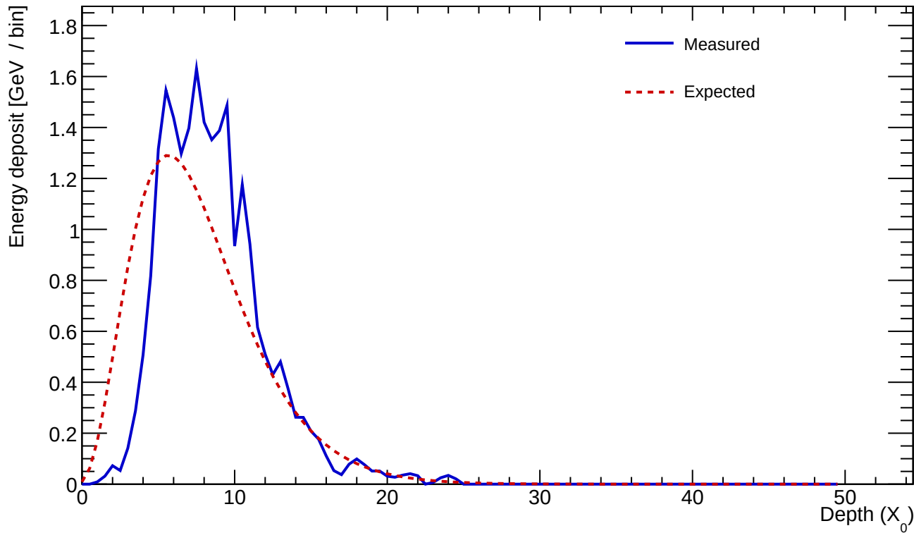
Cluster 239 E=23.379 GeV profileStart=1.50 X_0 \chi=0.2364
