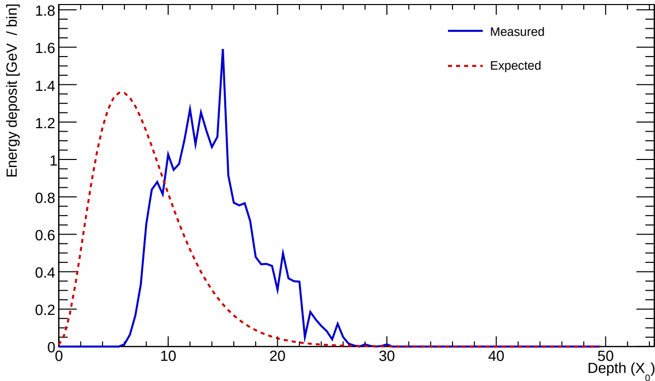
Cluster 660 E=24.713 GeV profileStart=6.00 X_0 \chi=0.1775
