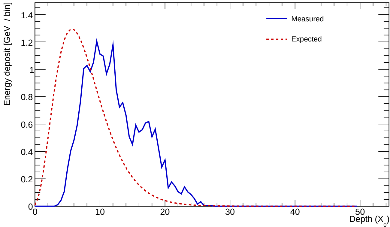
Cluster 336 E=23.433 GeV profileStart=4.00 X_0 \chi=0.2154
