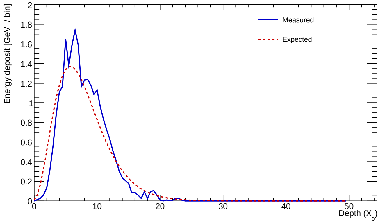
Cluster 47 E=24.954 GeV profileStart=0.50 X_0 \chi=0.1693
