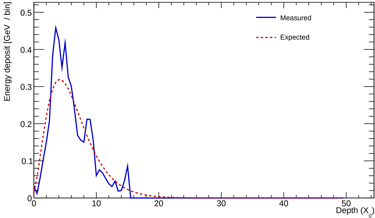
Cluster 596 E=5.055 GeV profileStart=0.50 X_0 \chi=0.2509
