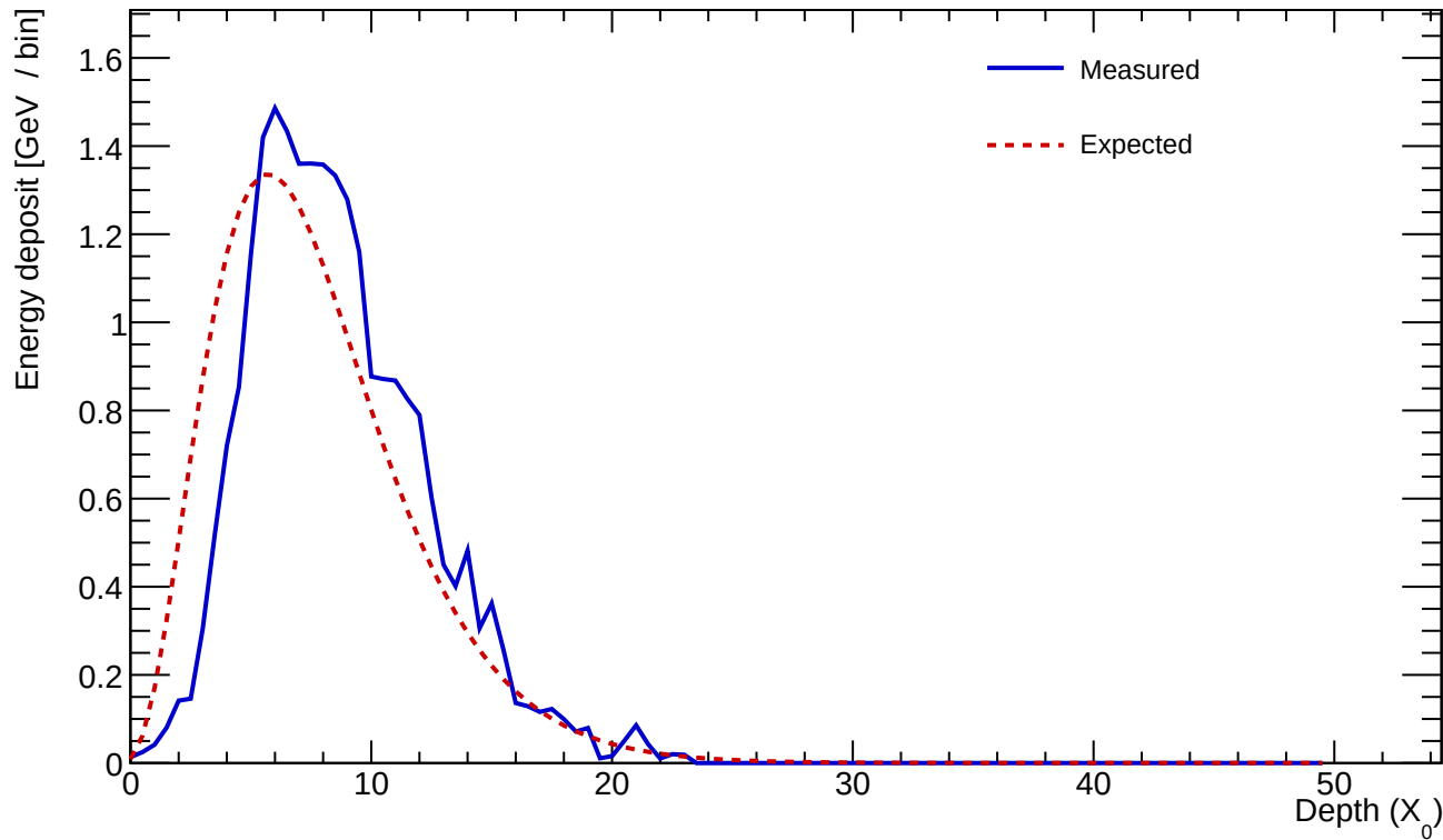
Cluster 268 E=24.289 GeV profileStart=1.50 X_0 \chi=0.1171
