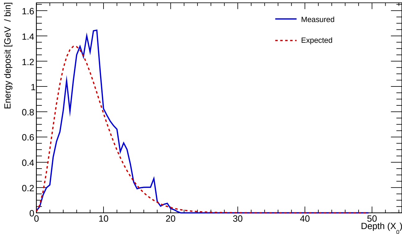
Cluster 645 E=23.926 GeV profileStart=1.00 X_0 \chi=0.1378
