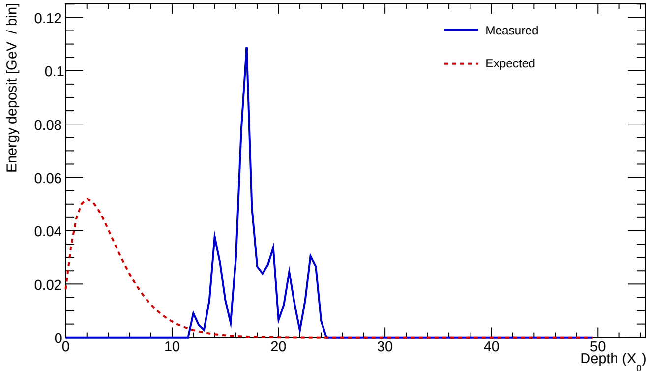
Cluster 758 E=0.628 GeV profileStart=13.50 X_0 \chi=0.5725
