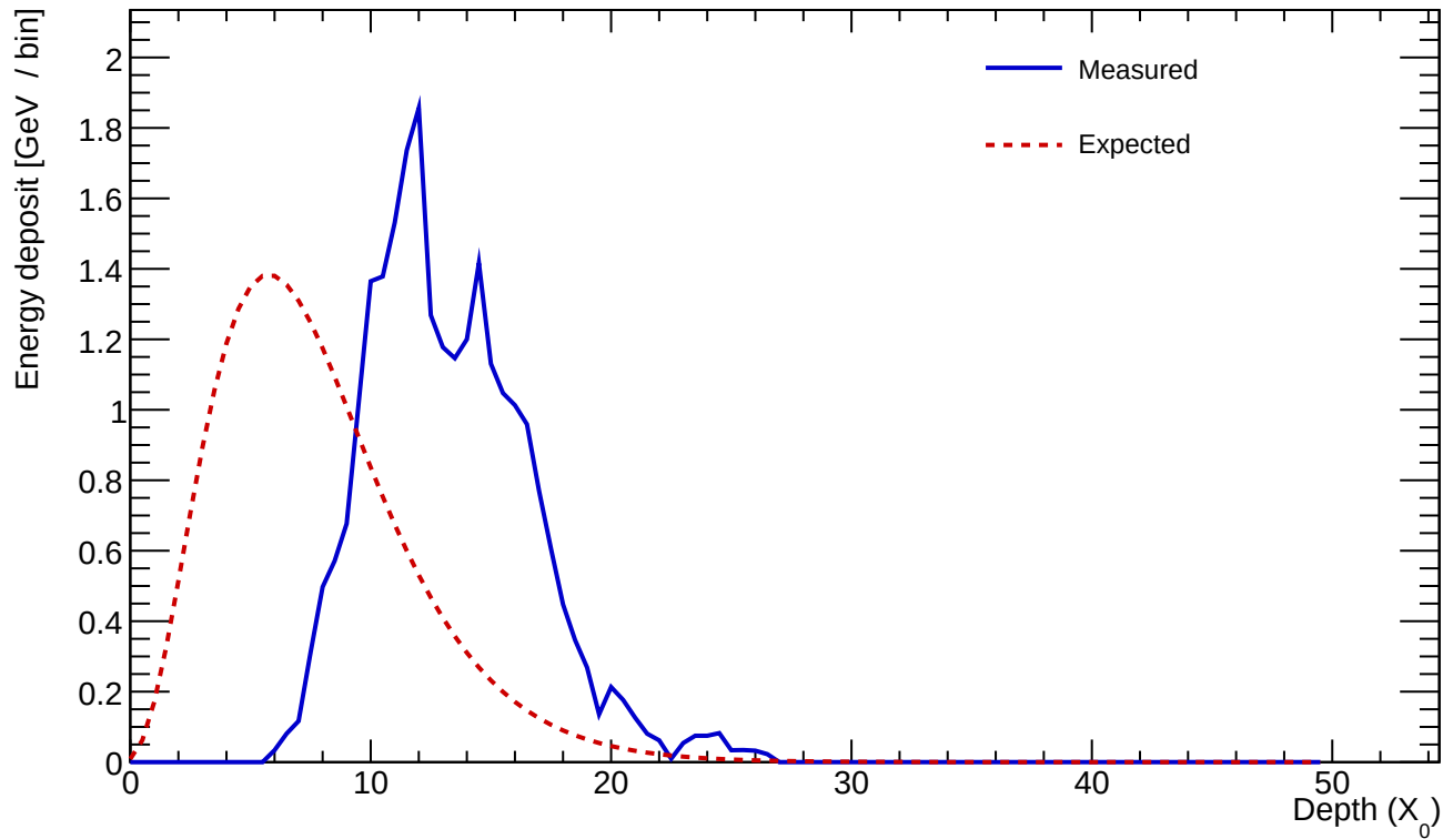
Cluster 373 E=25.187 GeV profileStart=6.00 X_0 \chi=0.1833
