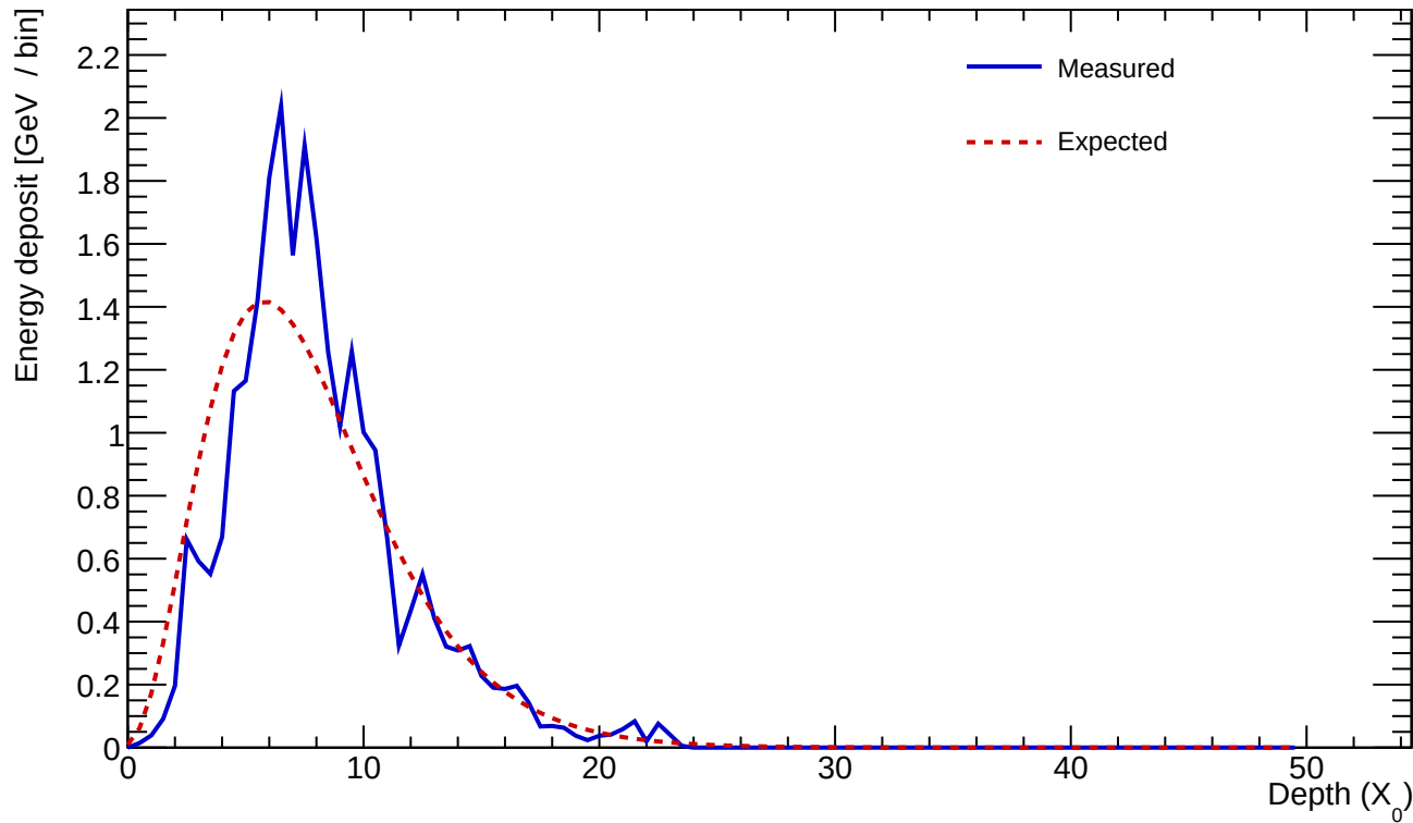
Cluster 519 E=25.859 GeV profileStart=0.50 X_0 \chi=0.2166
