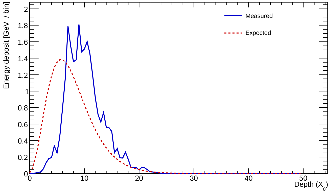
Cluster 79 E=25.199 GeV profileStart=3.00 X_0 \chi=0.2156
