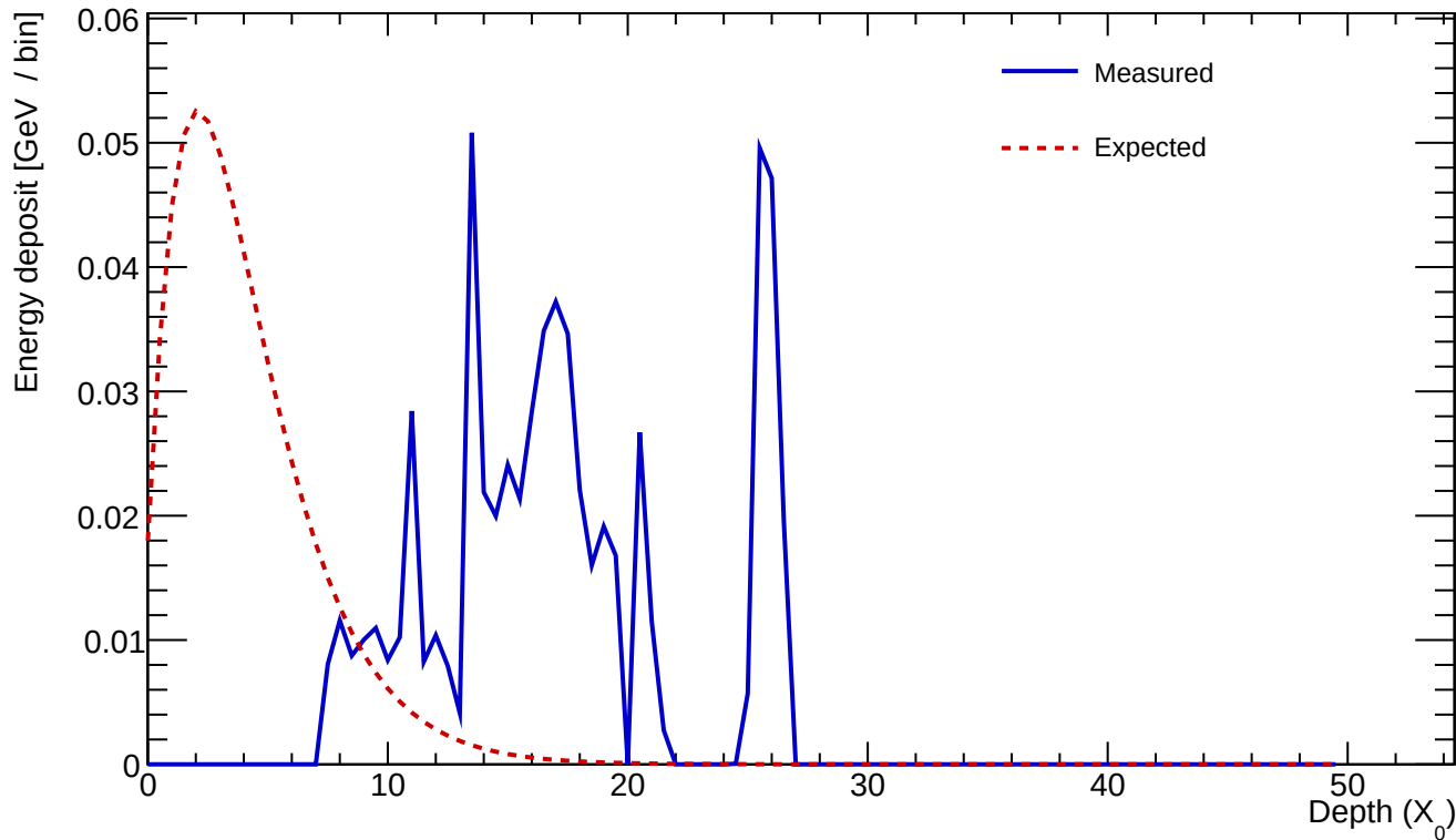
Cluster 340 E=0.637 GeV profileStart=12.50 X_0 \chi=0.7573
