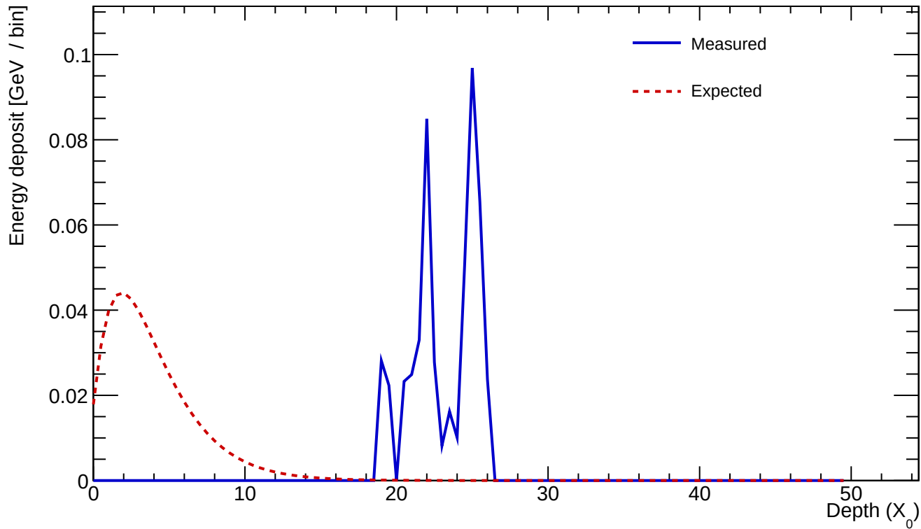
Cluster 664 E=0.516 GeV profileStart=20.50 X_0 \chi=0.6561
