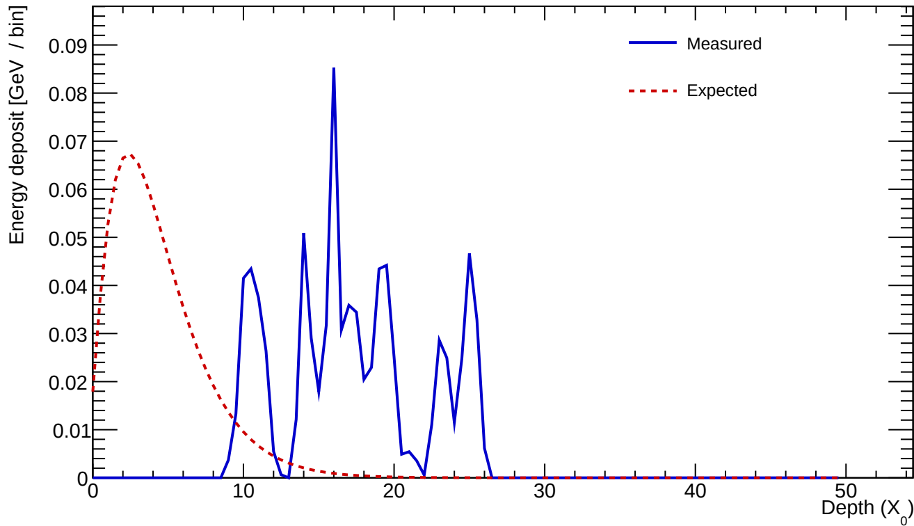
Cluster 554 E=0.857 GeV profileStart=13.50 X_0 \chi=0.7721
