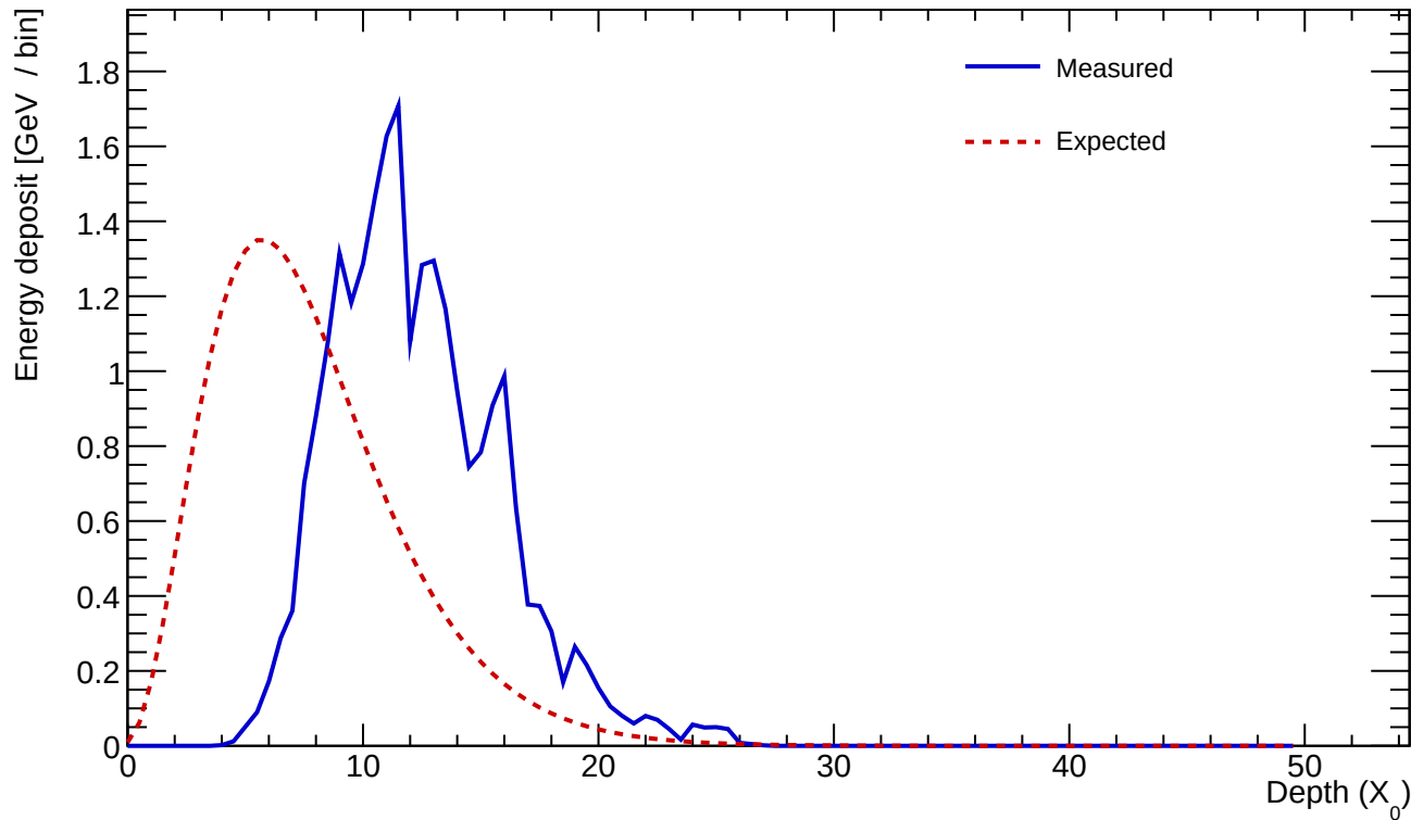
Cluster 161 E=24.575 GeV profileStart=5.00 X_0 \chi=0.1534
