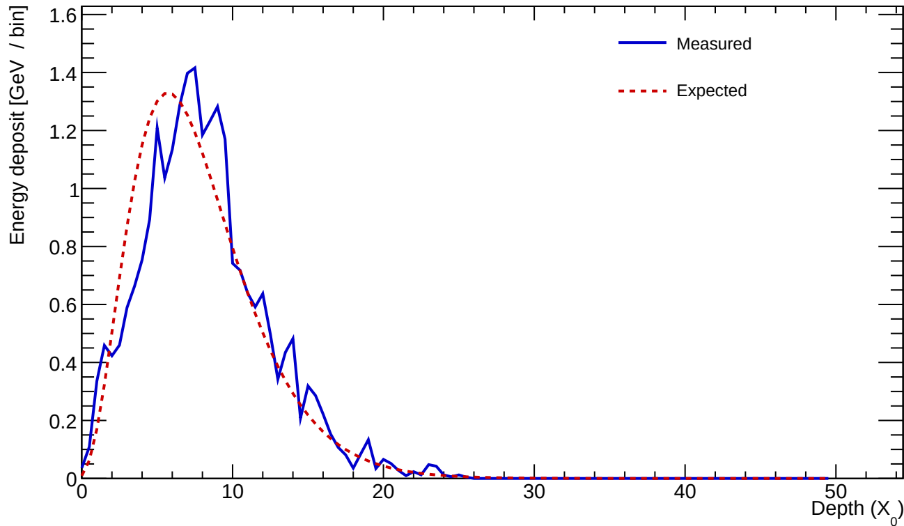
Cluster 573 E=24.134 GeV profileStart=1.00 X_0 \chi=0.1789
