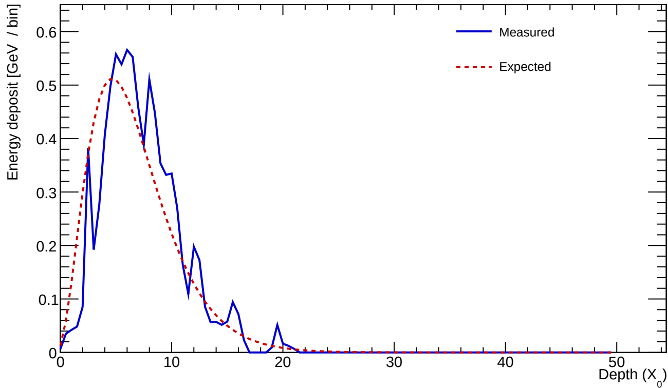
Cluster 441 E=8.522 GeV profileStart=1.00 X_0 \chi=0.1963
