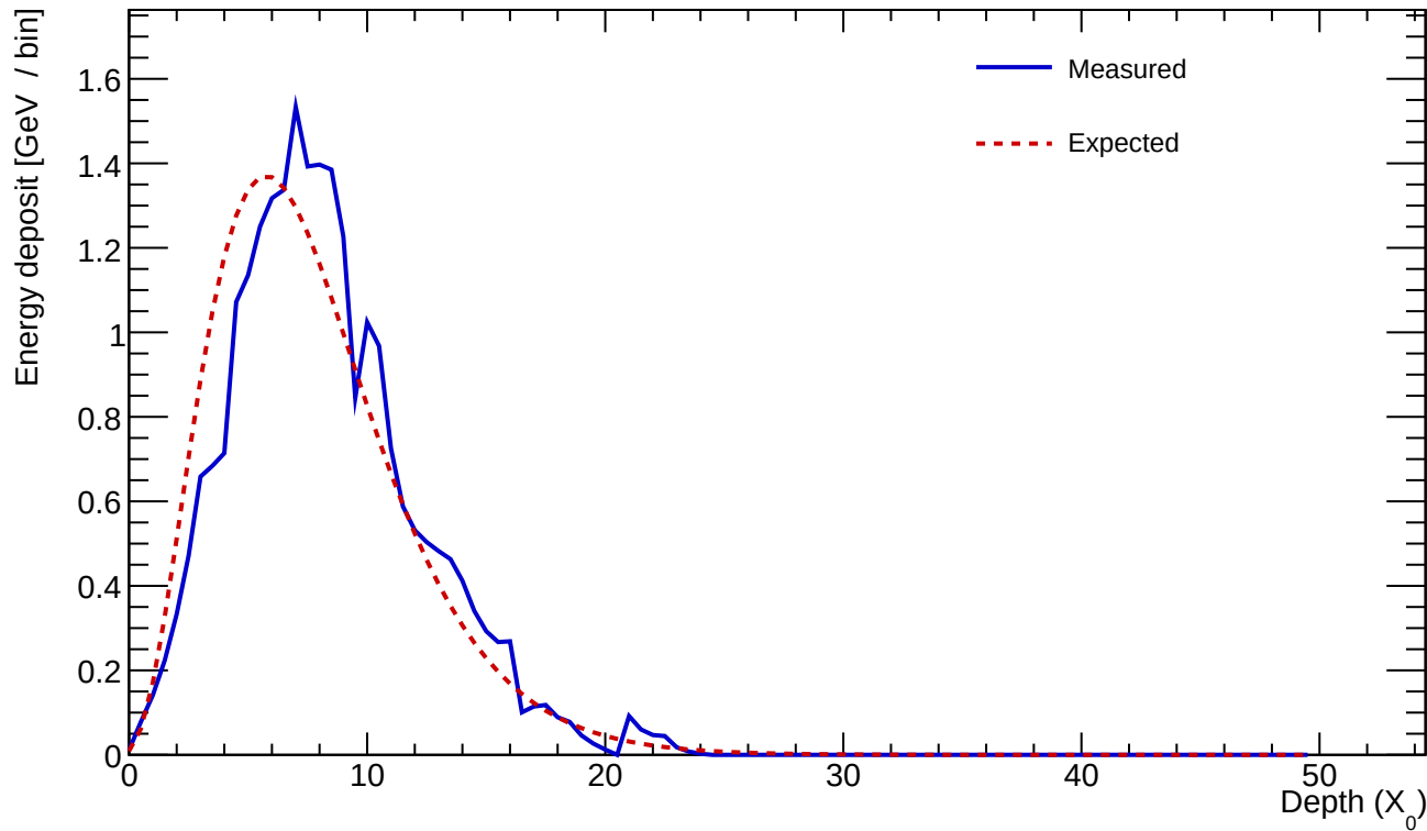
Cluster 315 E=24.935 GeV profileStart=1.00 X_0 \chi=0.1274
