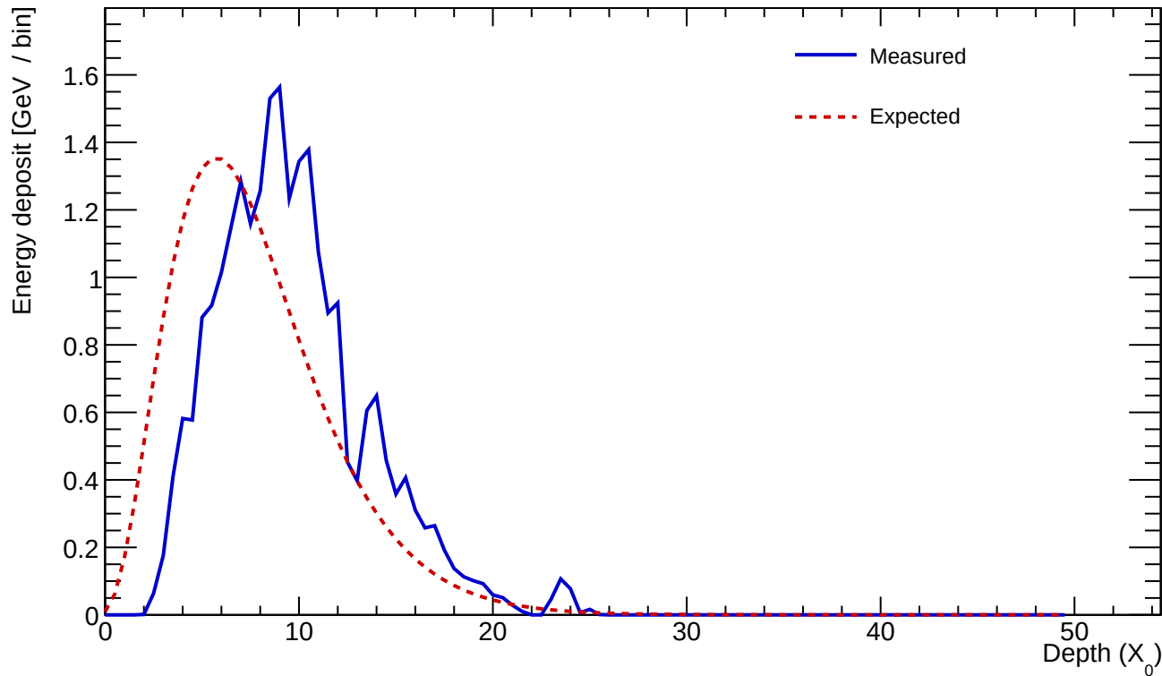
Cluster 211 E=24.615 GeV profileStart=2.00 X_0 \chi=0.1437
