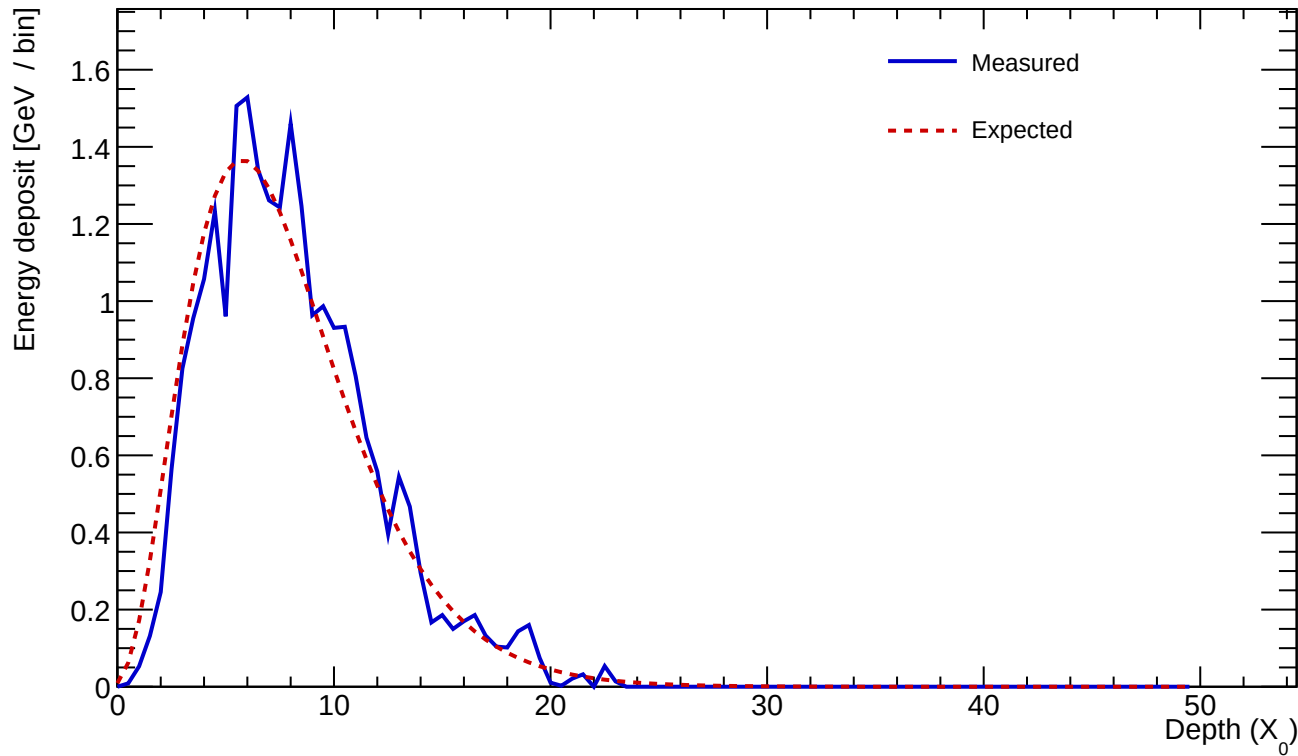
Cluster 133 E=24.854 GeV profileStart=0.50 X_0 \chi=0.1183
