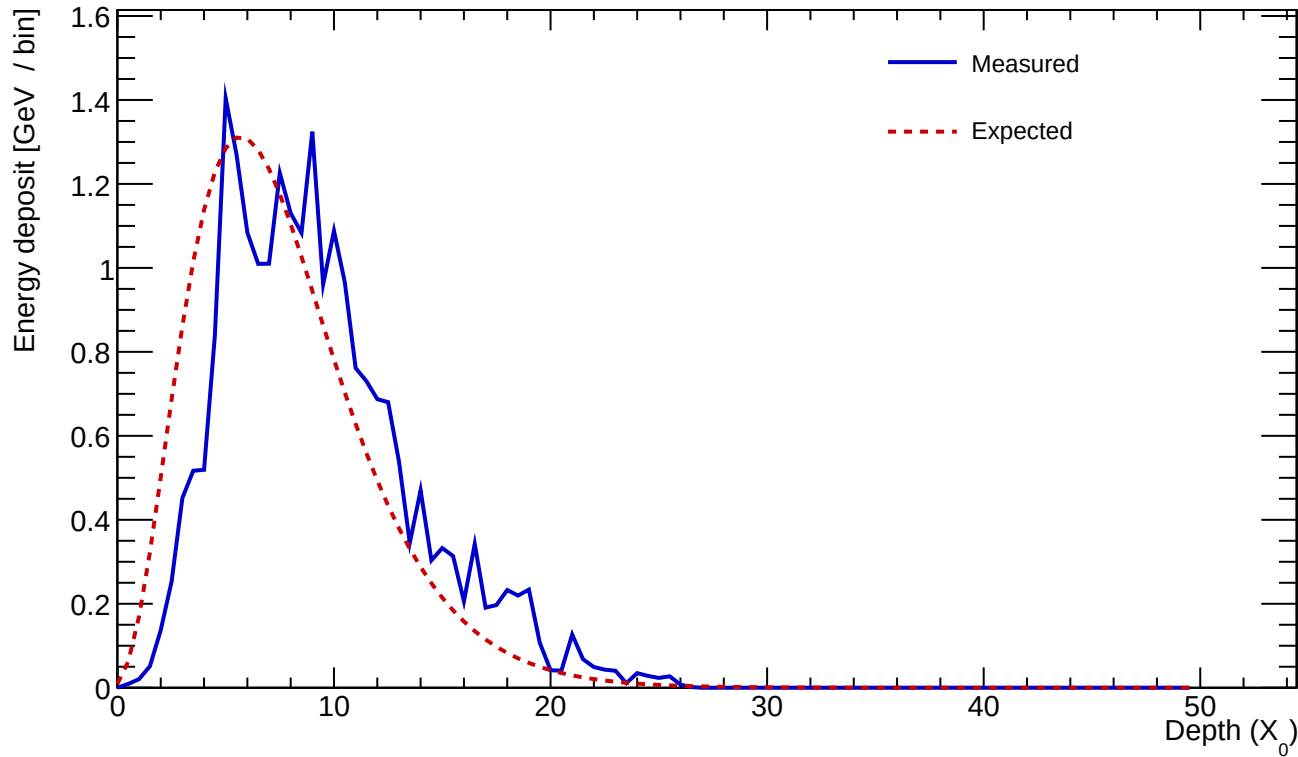
Cluster 665 E=23.789 GeV profileStart=1.50 X_0 \chi=0.1655
