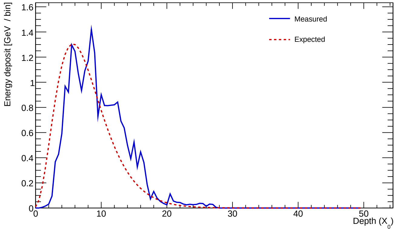
Cluster 788 E=23.640 GeV profileStart=1.50 X_0 \chi=0.1831
