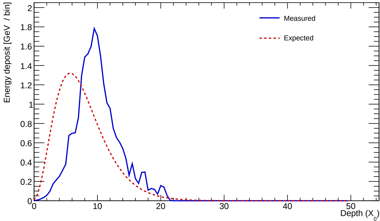
Cluster 70 E=23.963 GeV profileStart=3.00 X_0 \chi=0.2196
