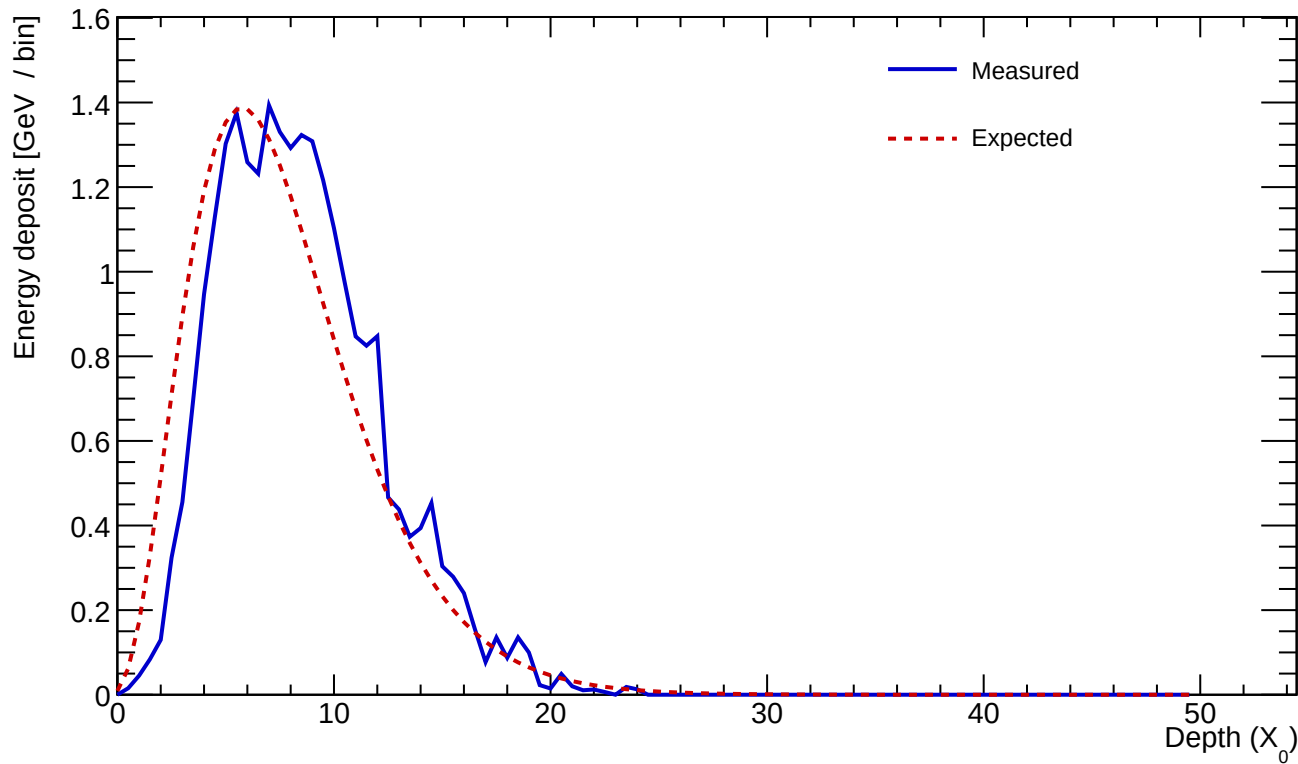
Cluster 85 E=25.262 GeV profileStart=1.00 X_0 \chi=0.0965
