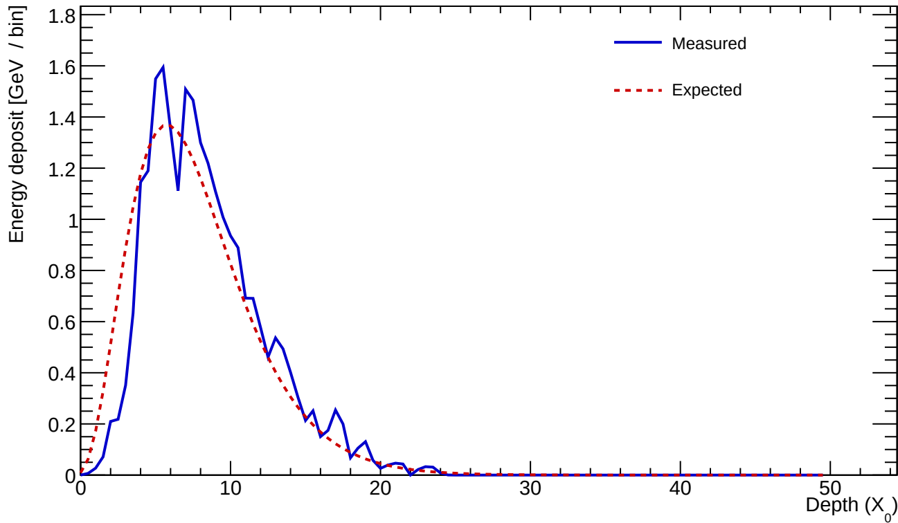
Cluster 416 E=24.902 GeV profileStart=1.00 X_0 \chi=0.1346
