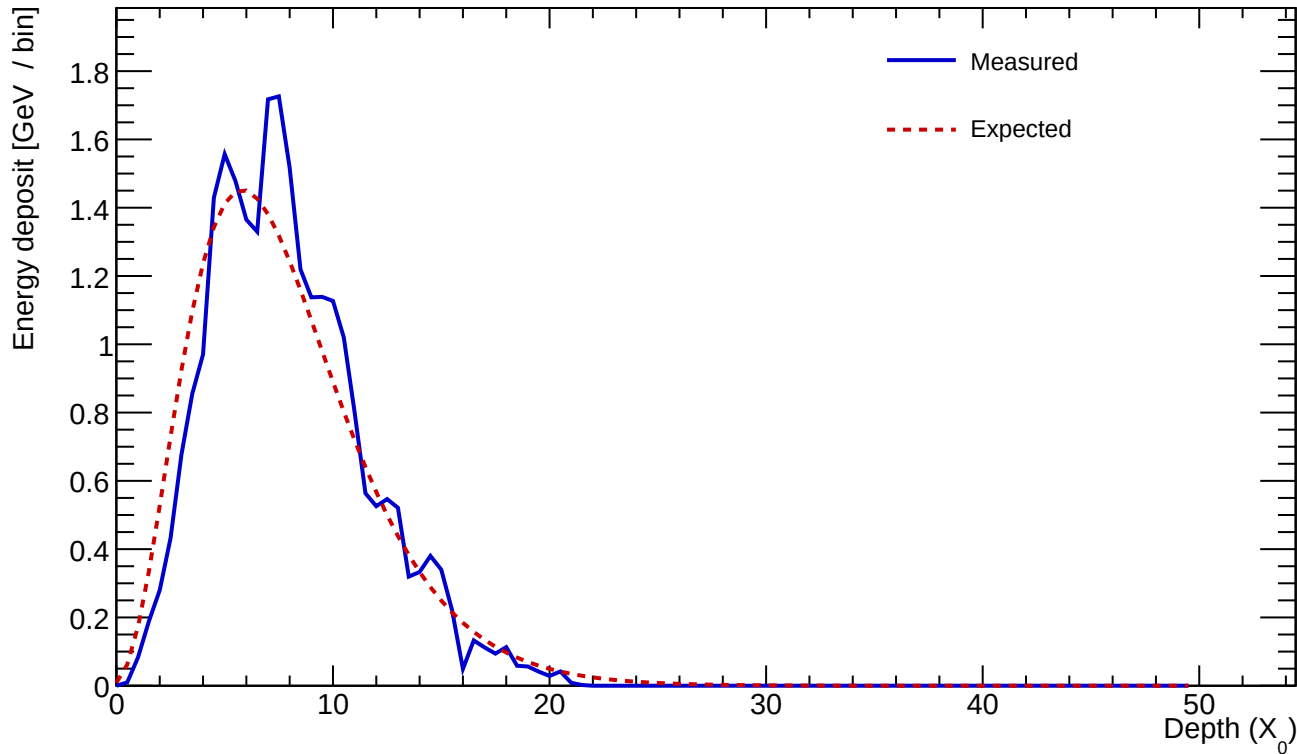
Cluster 357 E=26.545 GeV profileStart=0.50 X_0 \chi=0.1285
