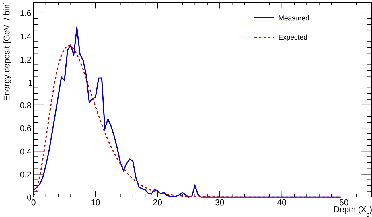
Cluster 145 E=23.892 GeV profileStart=1.00 X_0 \chi=0.1445
