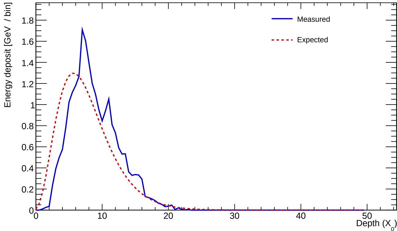
Cluster 657 E=23.510 GeV profileStart=1.50 X_0 \chi=0.1199
