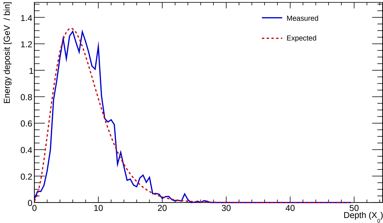
Cluster 812 E=23.900 GeV profileStart=0.50 X_0 \chi=0.1189
