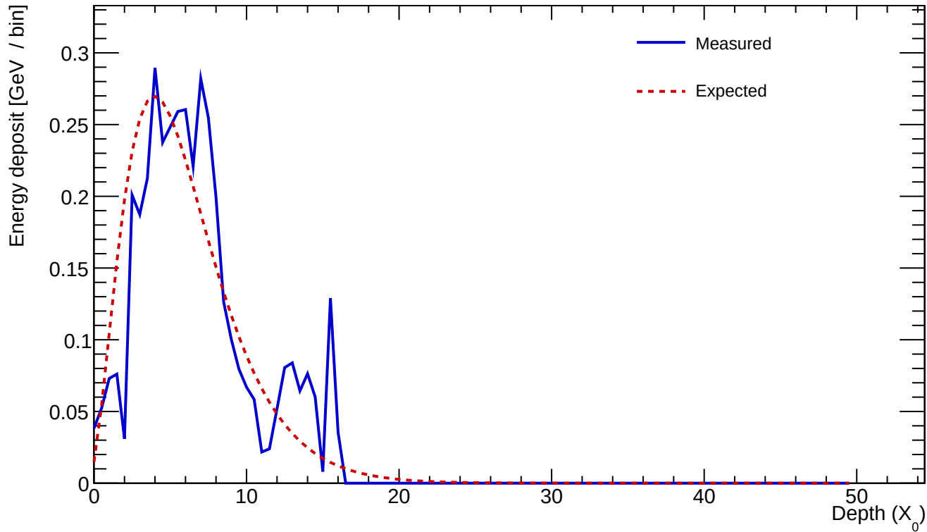
Cluster 822 E=4.190 GeV profileStart=0.50 X_0 \chi=0.2814
