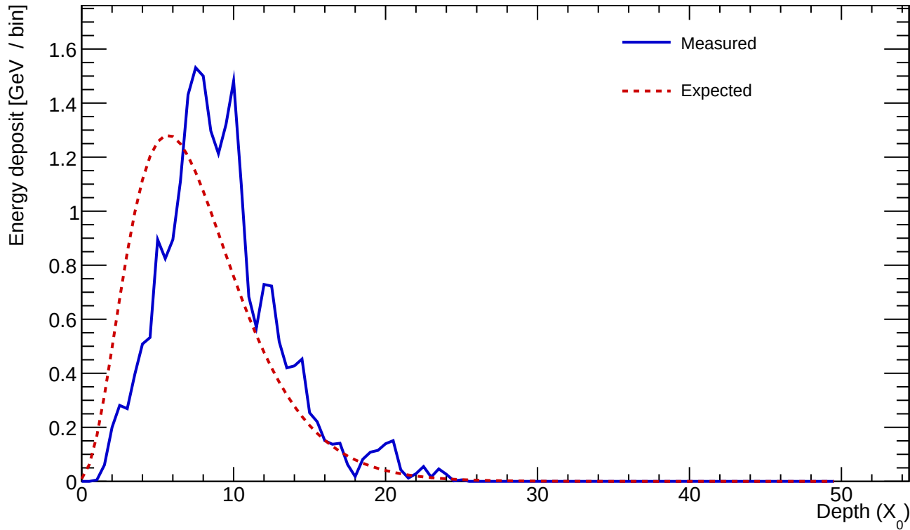
Cluster 165 E=23.188 GeV profileStart=2.00 X_0 \chi=0.2035
