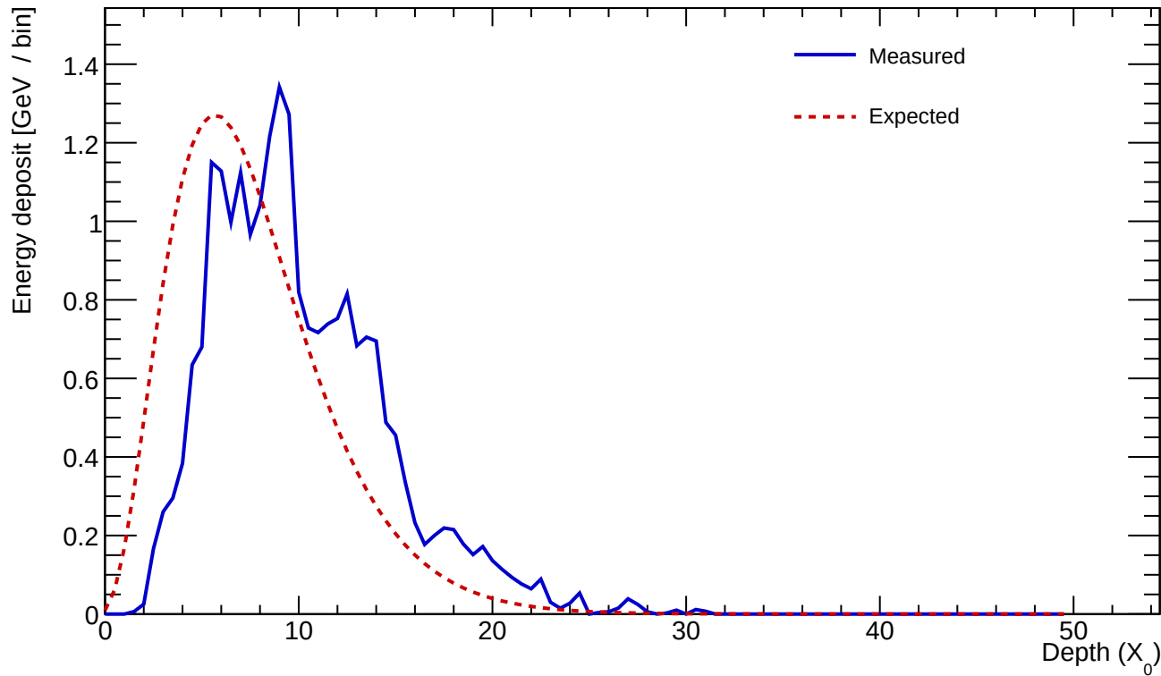
Cluster 293 E=22.991 GeV profileStart=2.00 X_0 \chi=0.1862
