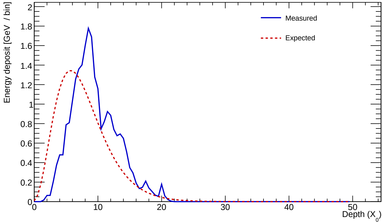
Cluster 407 E=24.435 GeV profileStart=2.00 X_0 \chi=0.1572
