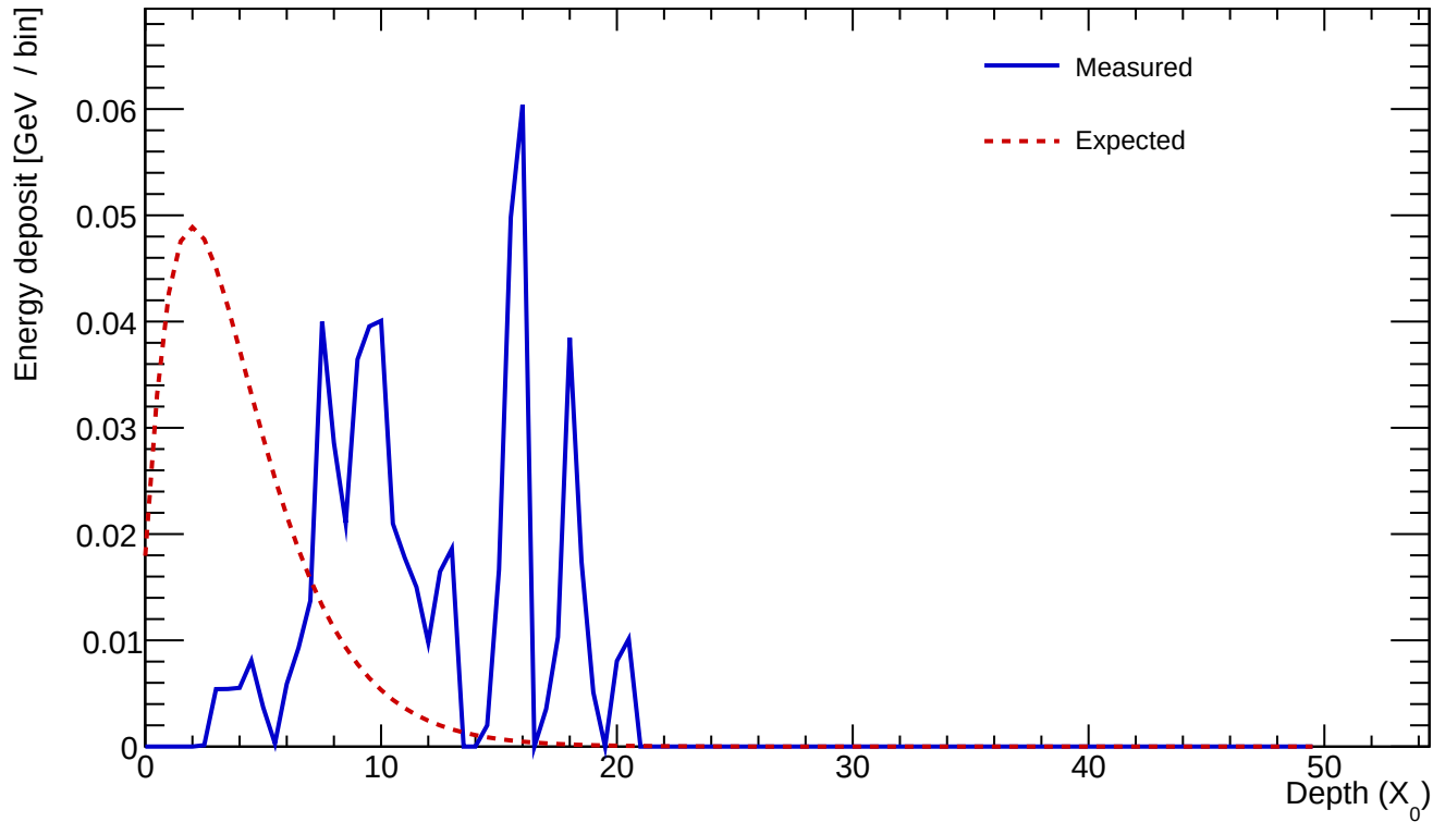
Cluster 631 E=0.584 GeV profileStart=6.50 X_0 \chi=0.7075
