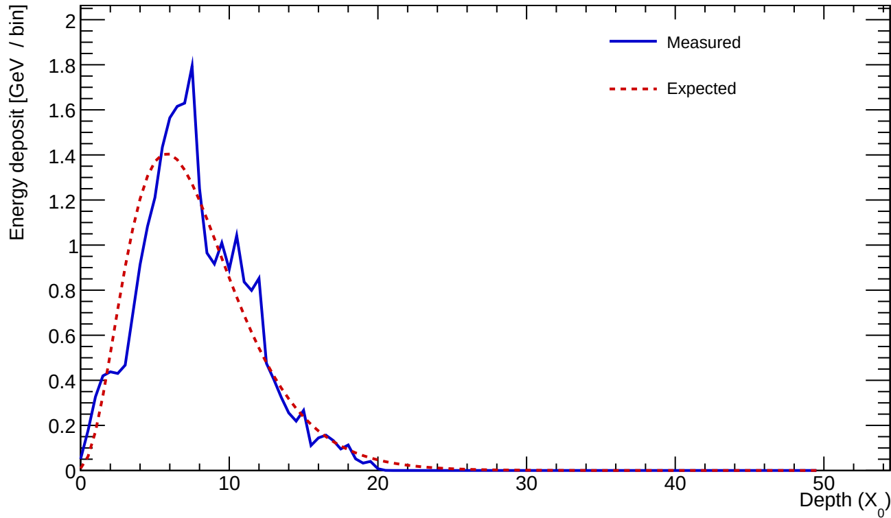
Cluster 180 E=25.640 GeV profileStart=0.50 X_0 \chi=0.1914
