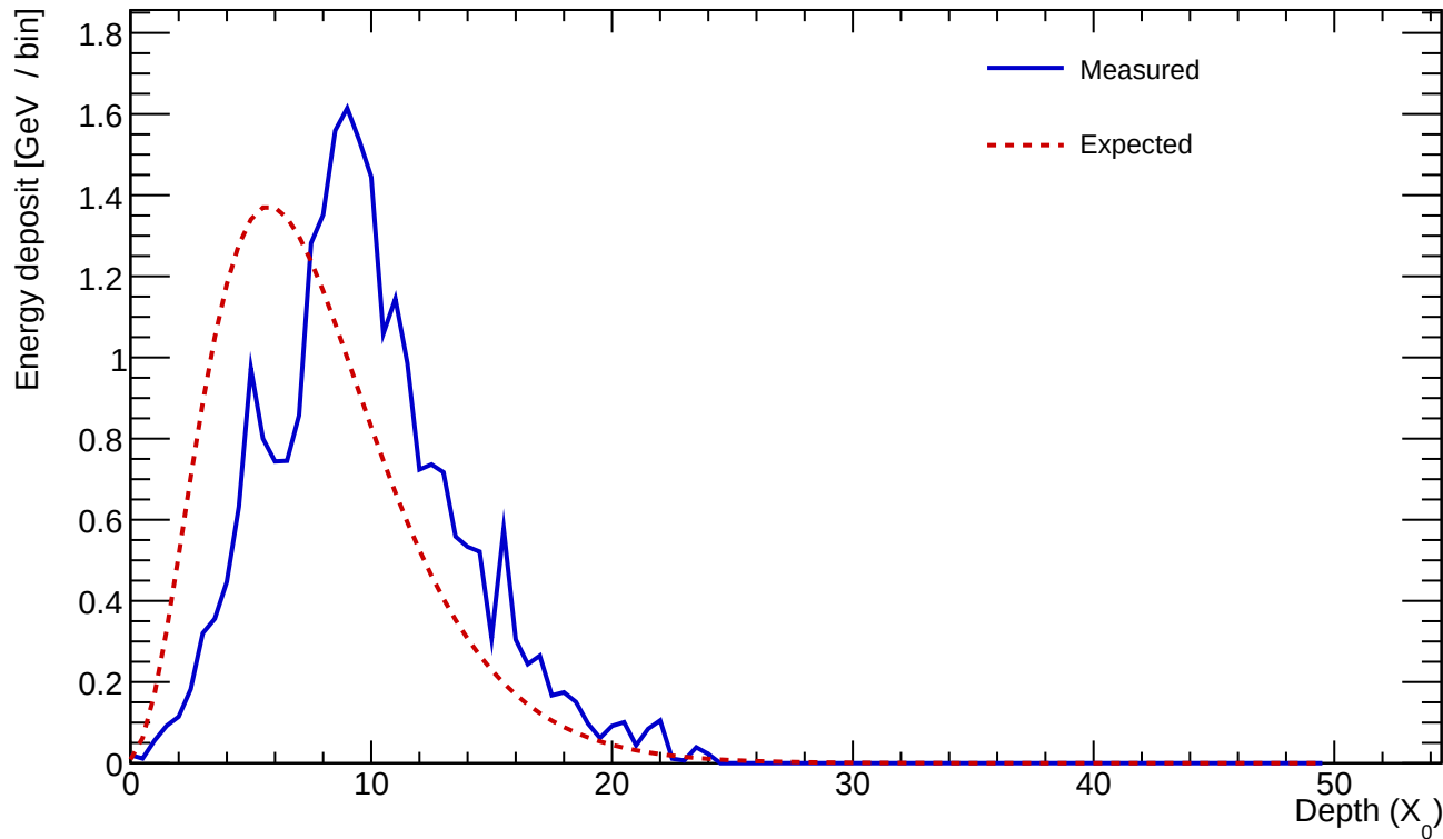
Cluster 851 E=24.977 GeV profileStart=2.00 X_0 \chi=0.1973
