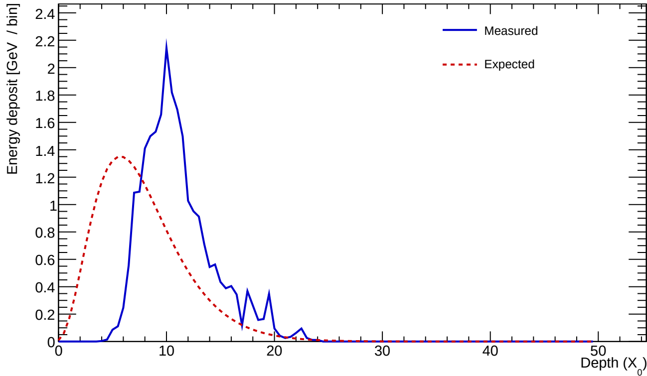
Cluster 606 E=24.551 GeV profileStart=3.50 X_0 \chi=0.2664
