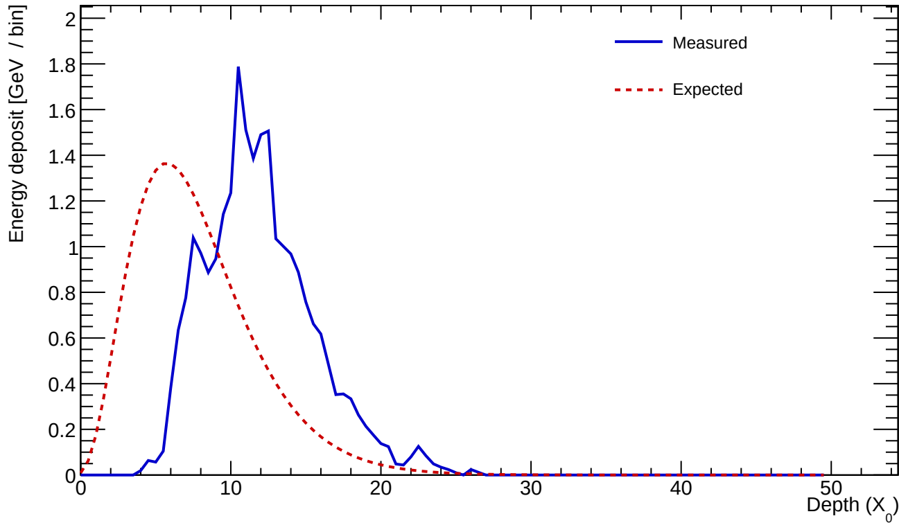
Cluster 761 E=24.841 GeV profileStart=4.50 X_0 \chi=0.1569
