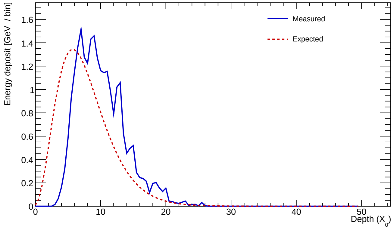
Cluster 131 E=24.401 GeV profileStart=2.50 X_0 \chi=0.1419
