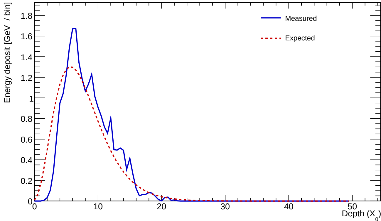
Cluster 783 E=23.587 GeV profileStart=1.00 X_0 \chi=0.1607
