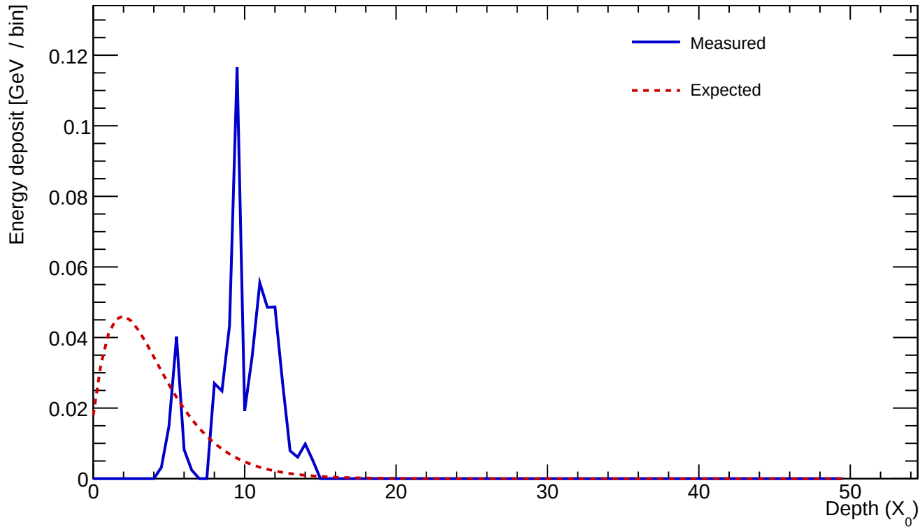
Cluster 709 E=0.544 GeV profileStart=8.00 X_0 \chi=0.5199
