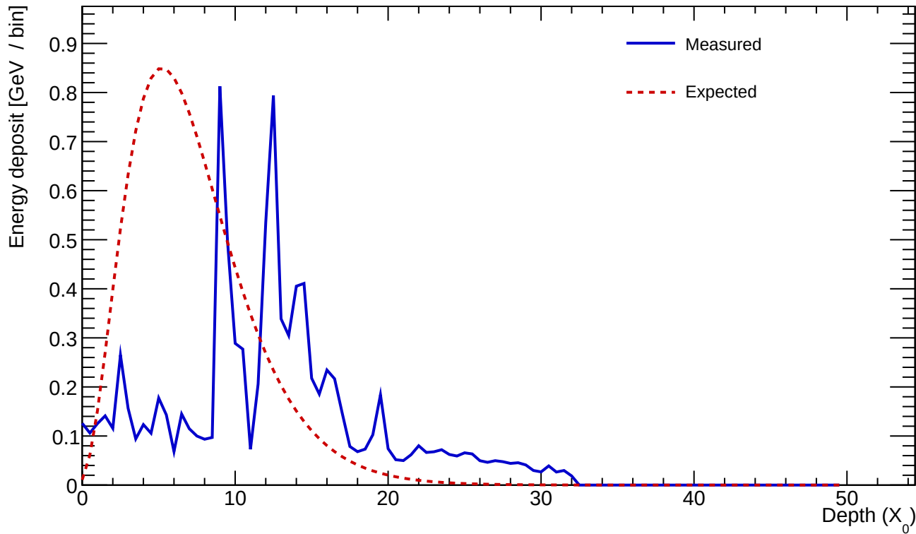
Cluster 227 E=14.846 GeV profileStart=4.00 X_0 \chi=0.9609
