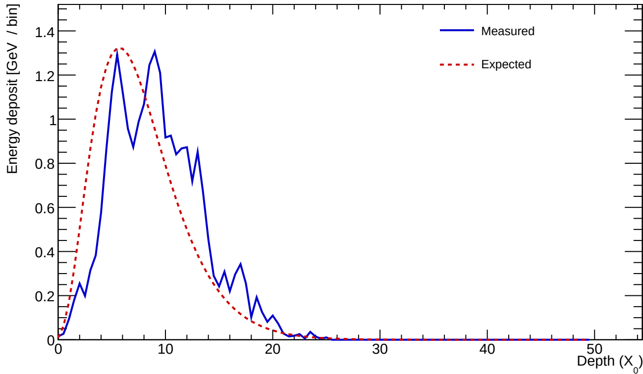
Cluster 626 E=24.016 GeV profileStart=1.50 X_0 \chi=0.1892
