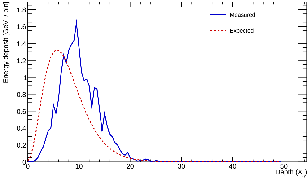
Cluster 536 E=24.002 GeV profileStart=2.50 X_0 \chi=0.1574
