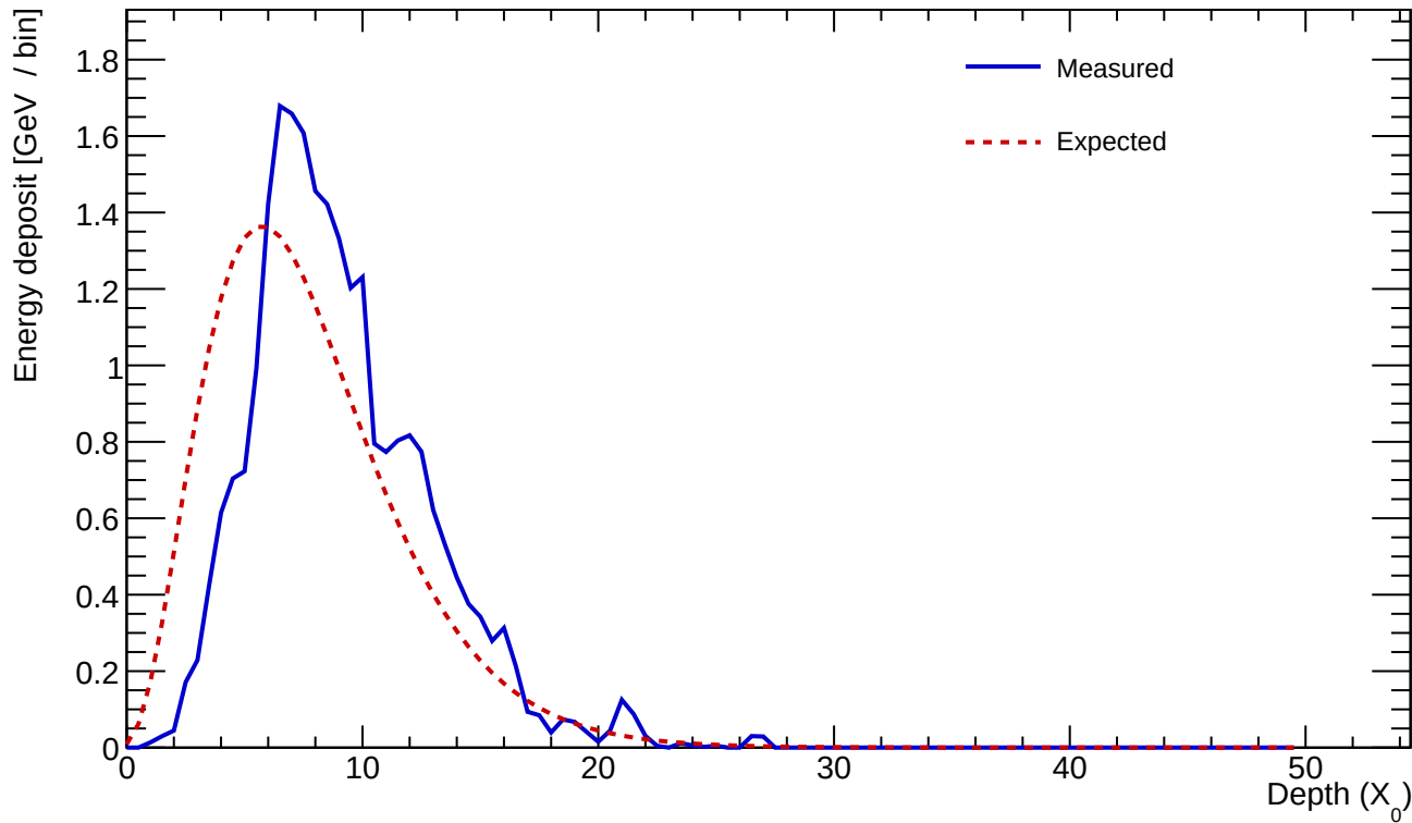
Cluster 540 E=24.836 GeV profileStart=1.50 X_0 \chi=0.1643
