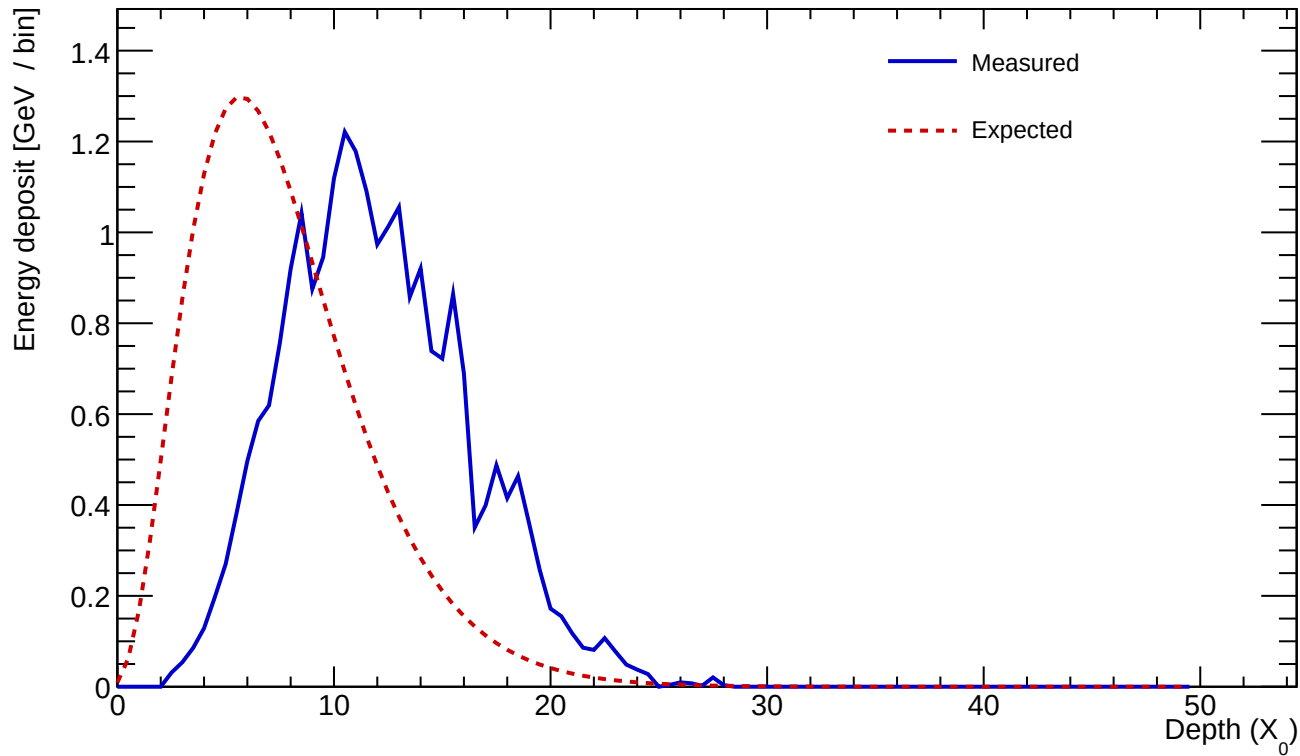
Cluster 559 E=23.524 GeV profileStart=4.50 X_0 \chi=0.1909
