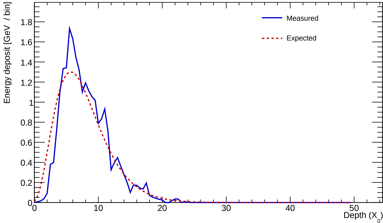
Cluster 535 E=23.583 GeV profileStart=0.50 X_0 \chi=0.1745
