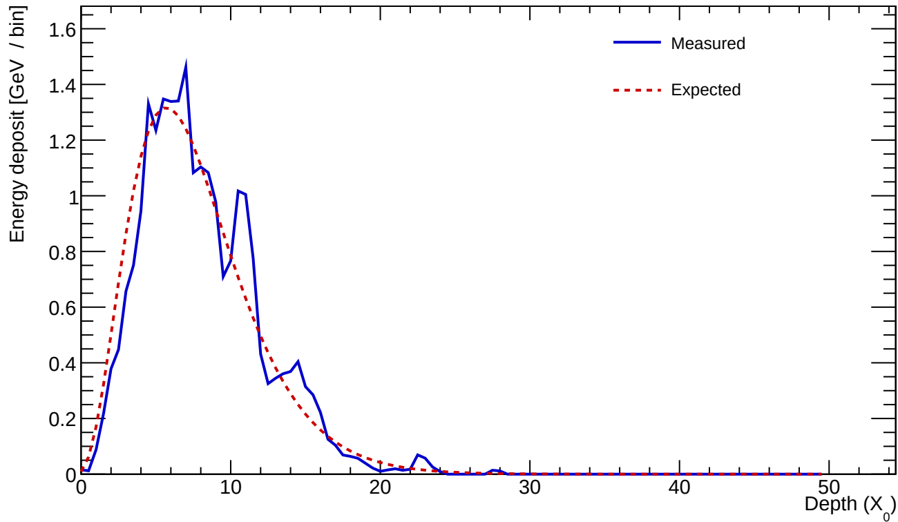
Cluster 35 E=23.891 GeV profileStart=0.50 X_0 \chi=0.1446
