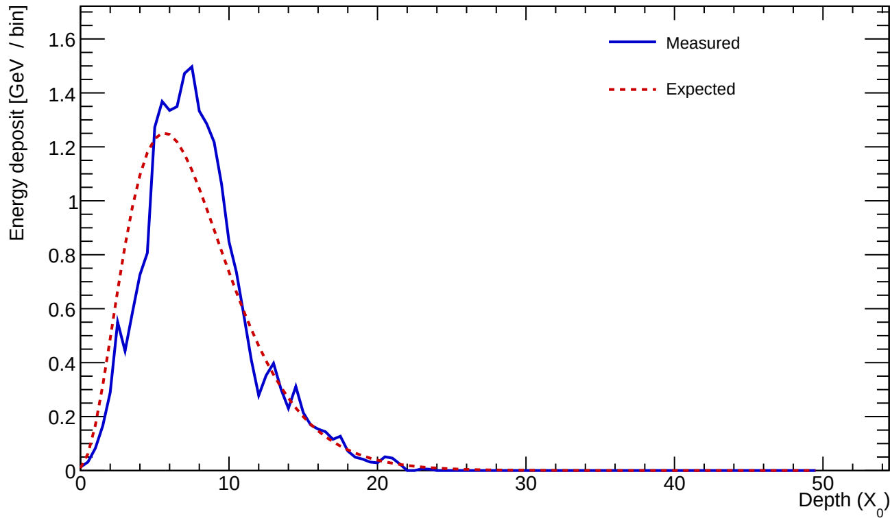
Cluster 563 E=22.610 GeV profileStart=0.50 X_0 \chi=0.1839
