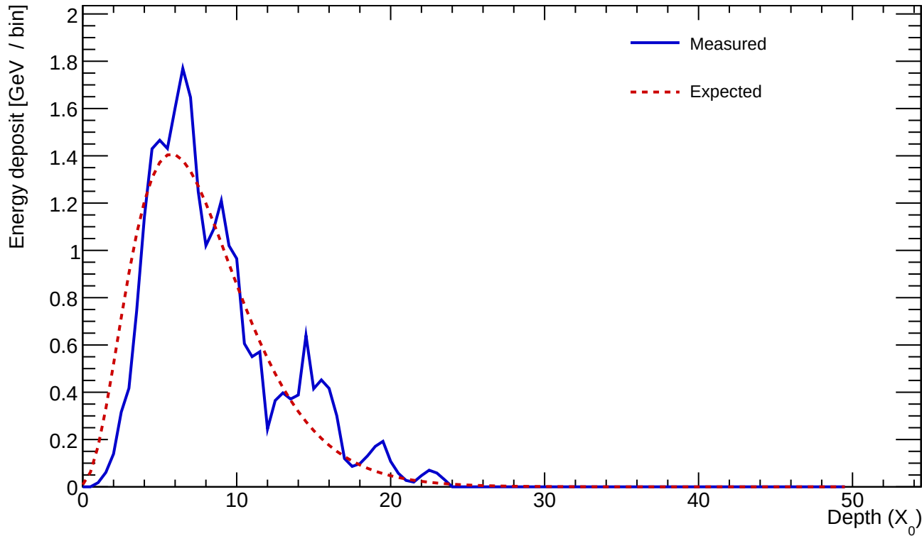
Cluster 110 E=25.668 GeV profileStart=0.50 X_0 \chi=0.2248
