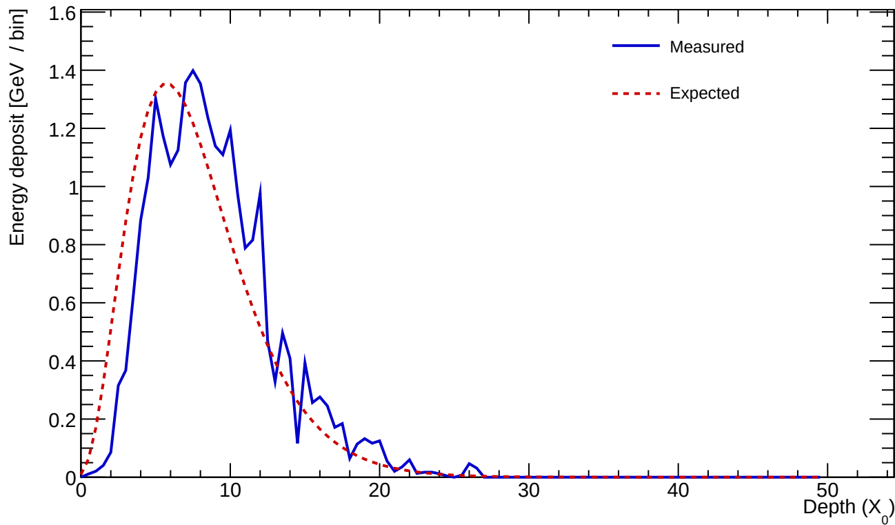
Cluster 615 E=24.612 GeV profileStart=1.00 X_0 \chi=0.1299
