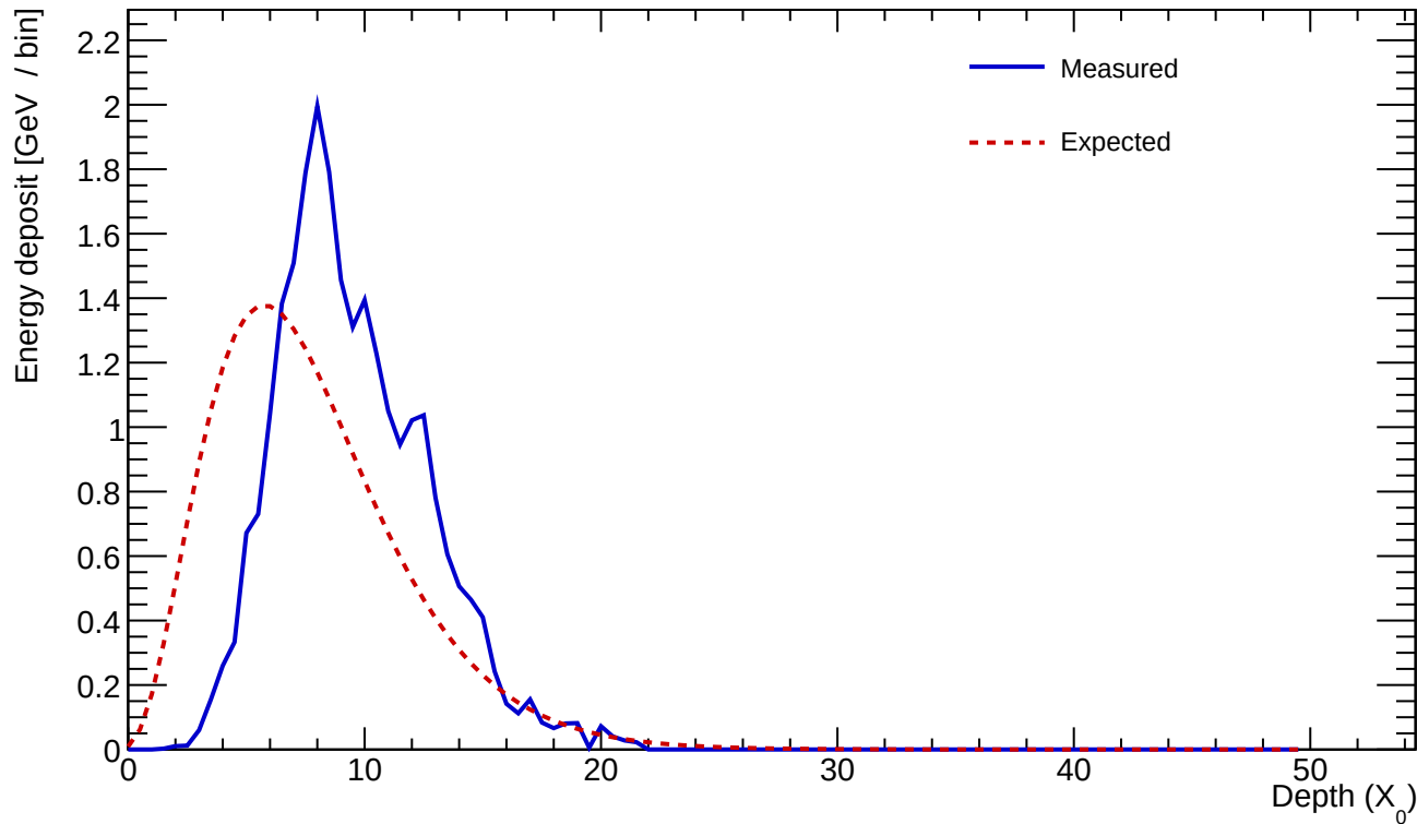
Cluster 279 E=25.089 GeV profileStart=2.50 X_0 \chi=0.1912
