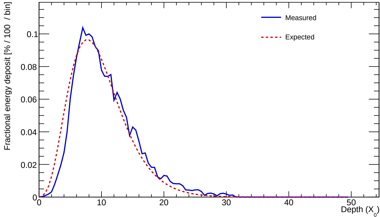
Cluster 3 E=181.271 GeV profileStart=0.50 X_0 \chi=0.1034
