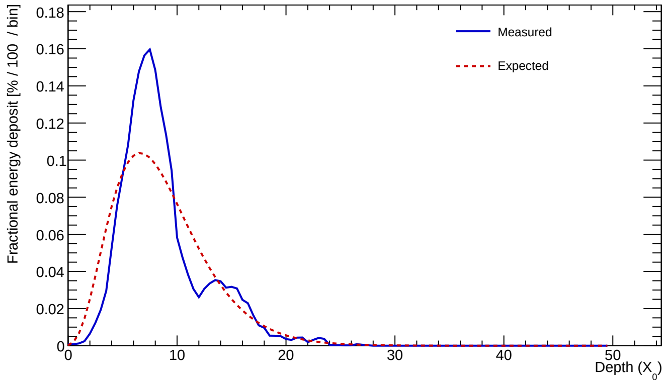
Cluster 4 E=60.106 GeV profileStart=0.50 X_0 \chi=0.3096
