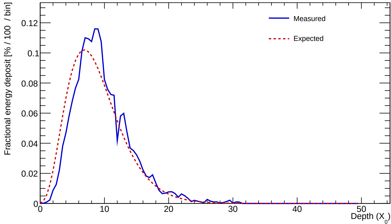
Cluster 7 E=76.019 GeV profileStart=1.00 X_0 \chi=0.1088
