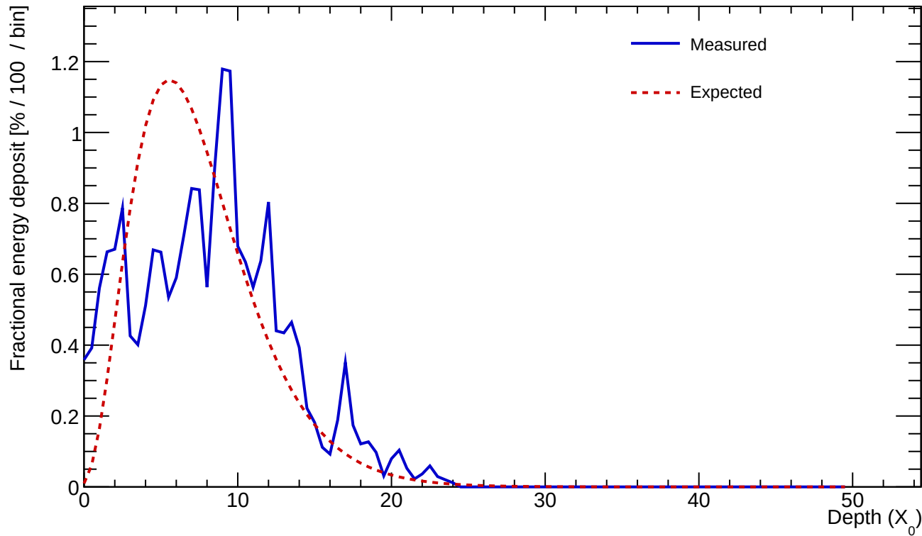
Cluster 27 E=20.599 GeV profileStart=1.50 X_0 \chi=0.4324
