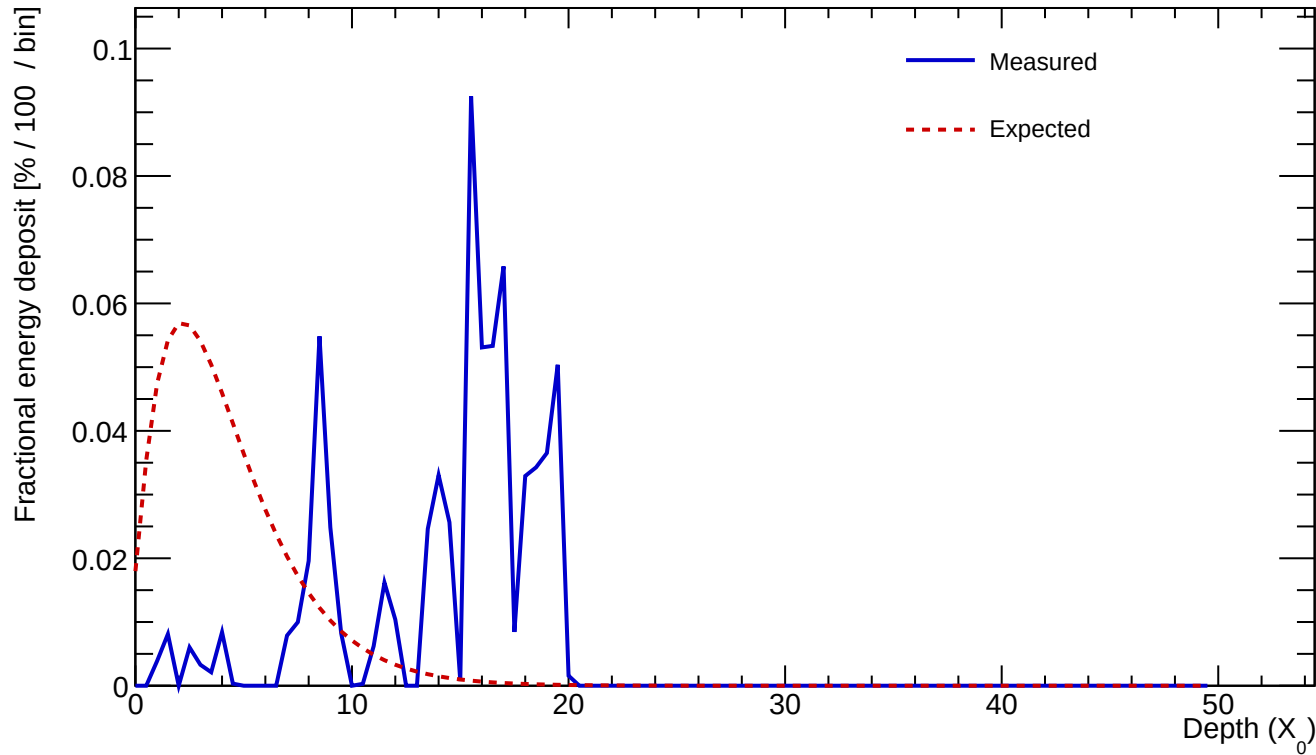
Cluster 31 E=0.704 GeV profileStart=13.50 X_0 \chi=0.5762
