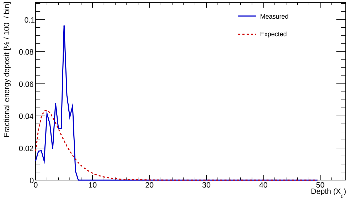
Cluster 22 E=0.508 GeV profileStart=1.50 X_0 \chi=0.4480
