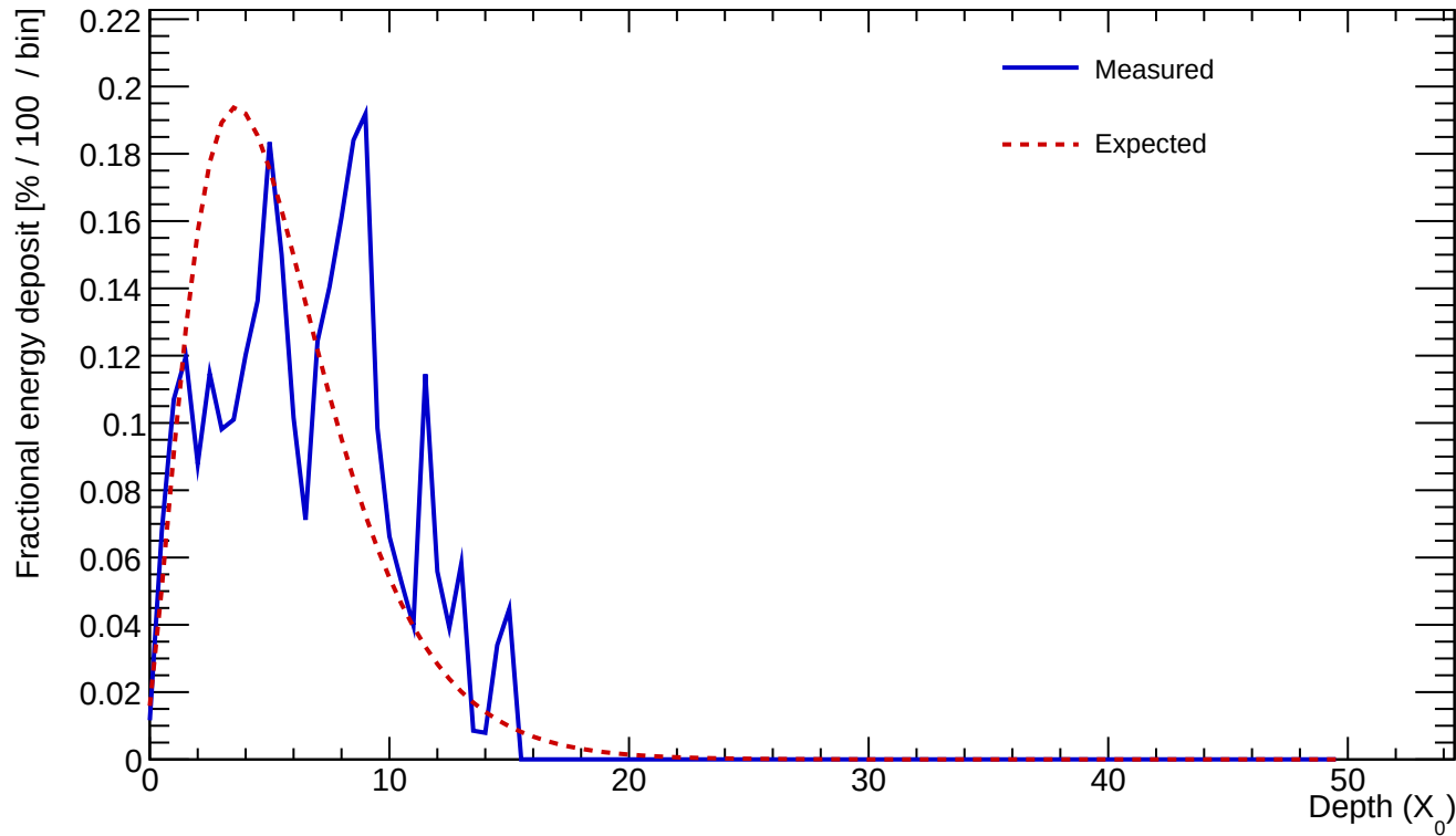
Cluster 7 E=2.893 GeV profileStart=1.00 X_0 \chi=0.4076
