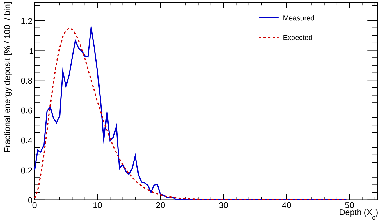
Cluster 82 E=20.589 GeV profileStart=0.50 X_0 \chi=0.2498
