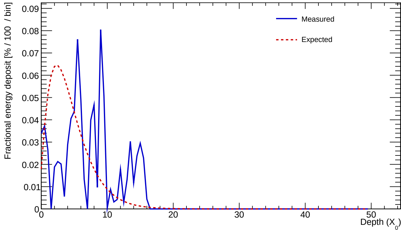
Cluster 79 E=0.815 GeV profileStart=3.50 X_0 \chi=0.7696
