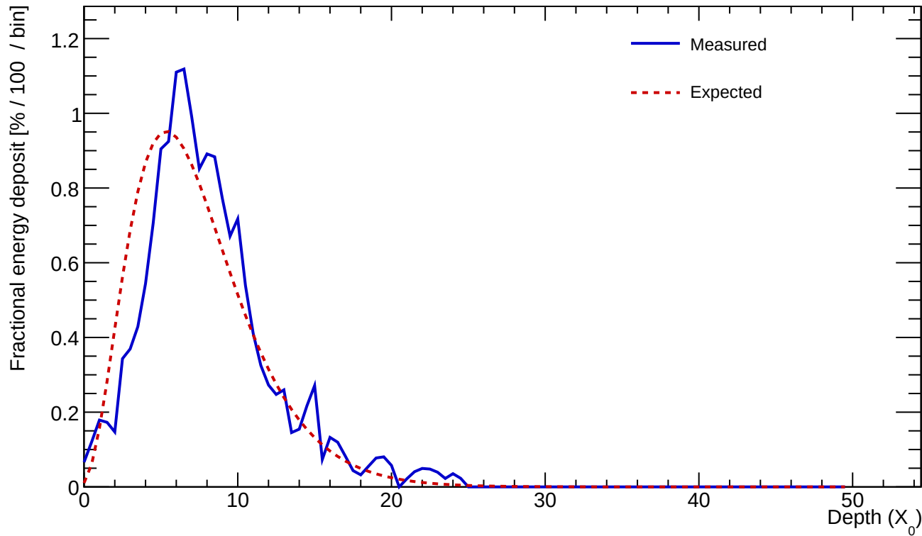
Cluster 11 E=16.792 GeV profileStart=1.00 X_0 \chi=0.1787
