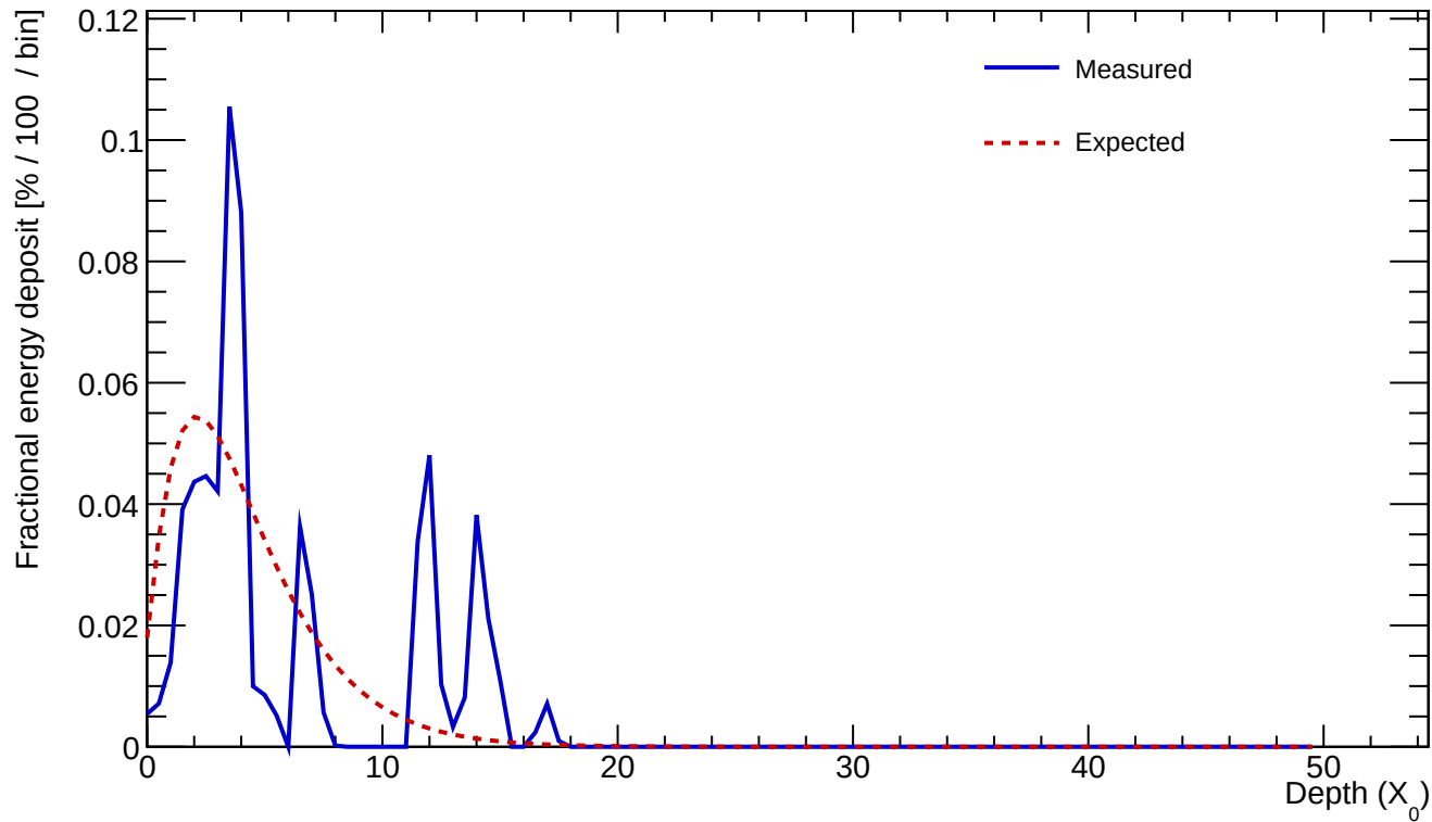
Cluster 90 E=0.665 GeV profileStart=1.00 X_0 \chi=0.8092
