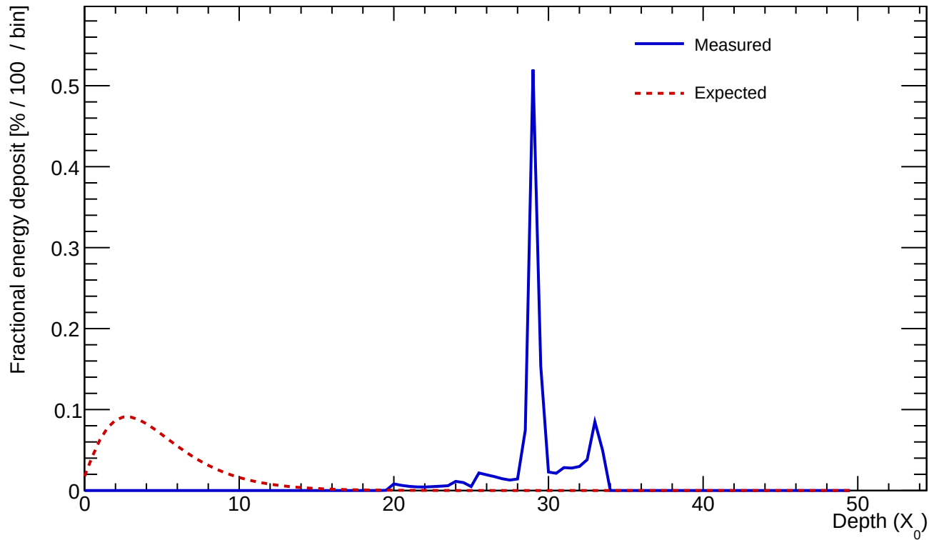
Cluster 67 E=1.221 GeV profileStart=27.00 X_0 \chi=0.8506
