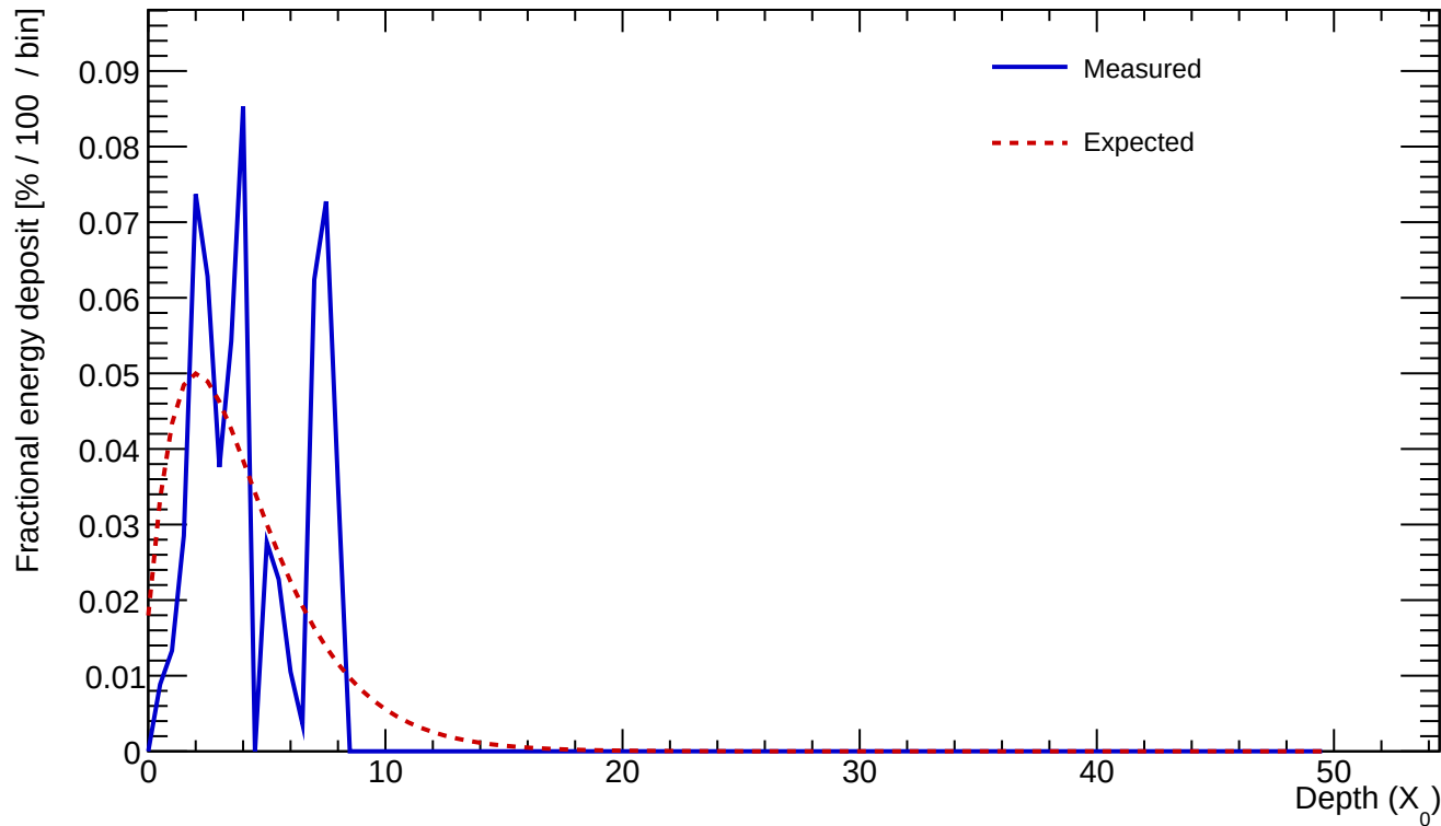
Cluster 41 E=0.599 GeV profileStart=1.00 X_0 \chi=0.5342
