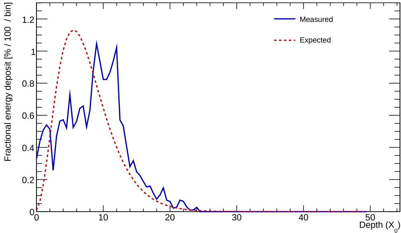
Cluster 59 E=20.248 GeV profileStart=1.50 X_0 \chi=0.3875
