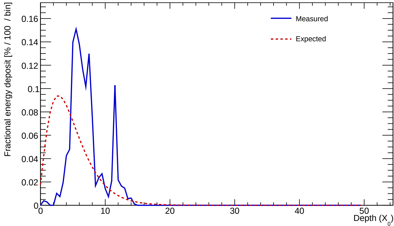
Cluster 18 E=1.267 GeV profileStart=3.50 X_0 \chi=0.4860
