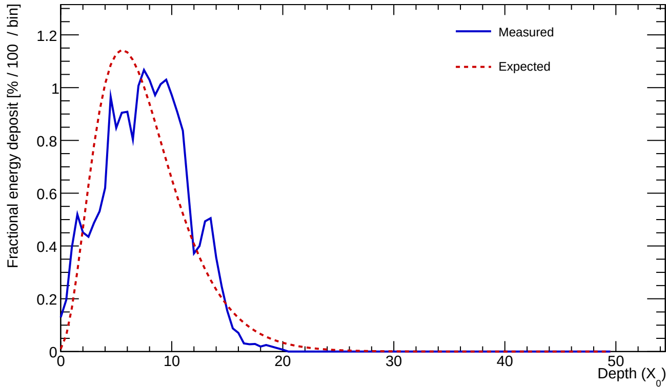
Cluster 66 E=20.485 GeV profileStart=1.00 X_0 \chi=0.2528
