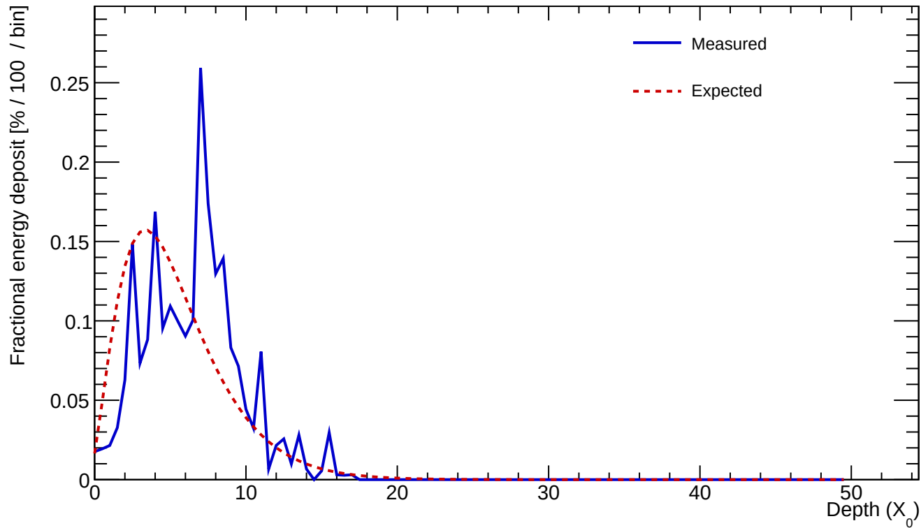
Cluster 45 E=2.285 GeV profileStart=1.00 X_0 \chi=0.4290
