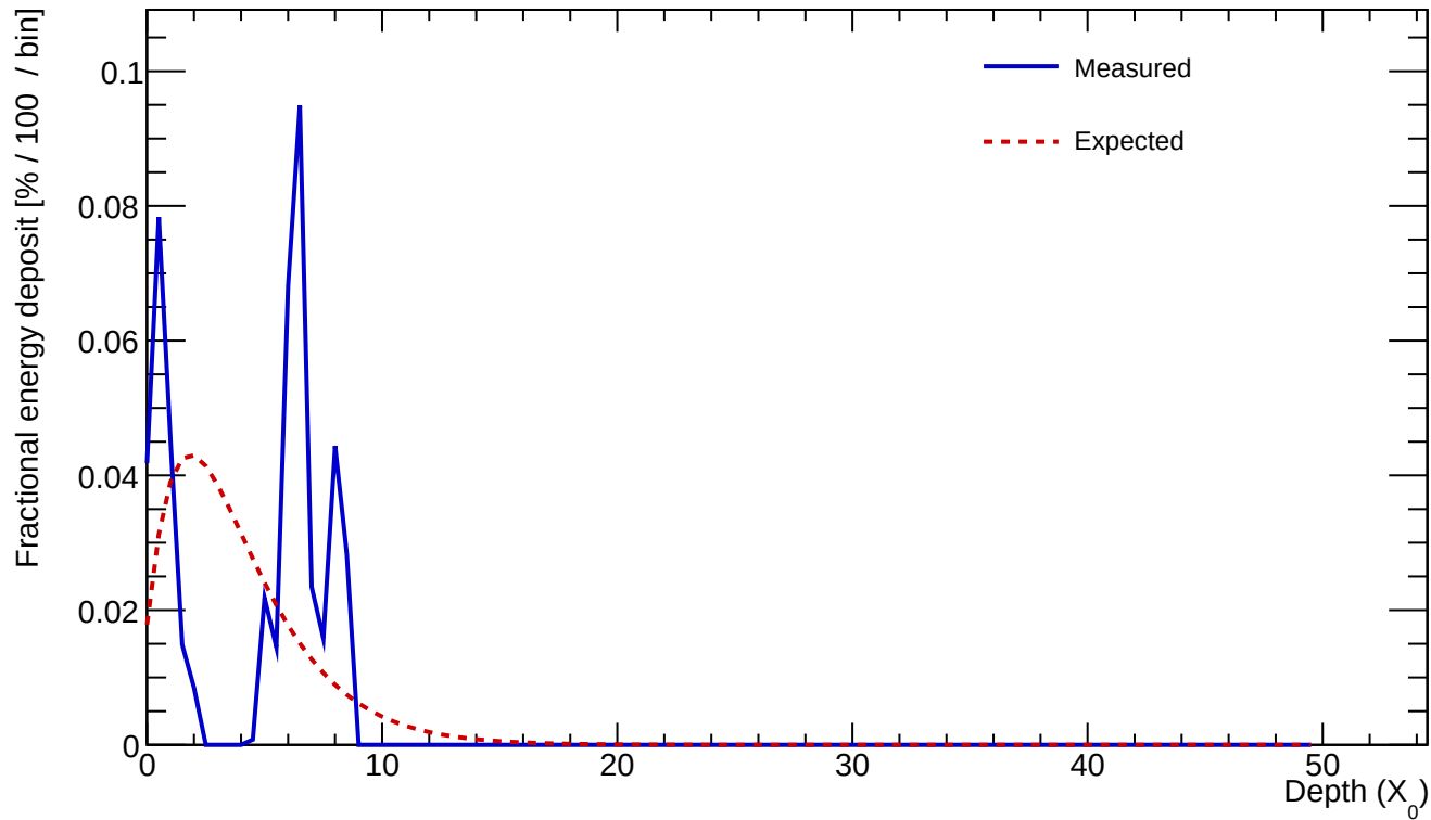
Cluster 37 E=0.501 GeV profileStart=5.00 X_0 \chi=0.6840
