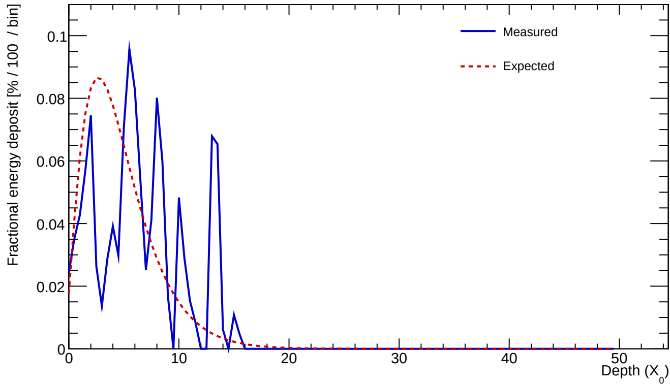
Cluster 52 E=1.153 GeV profileStart=0.50 X_0 \chi=0.6199
