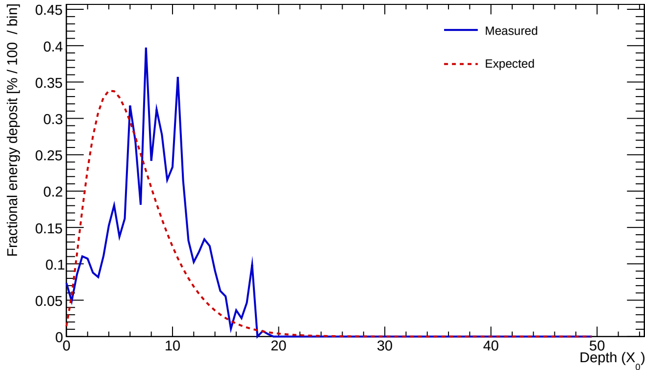
Cluster 12 E=5.401 GeV profileStart=2.50 X_0 \chi=0.3401
