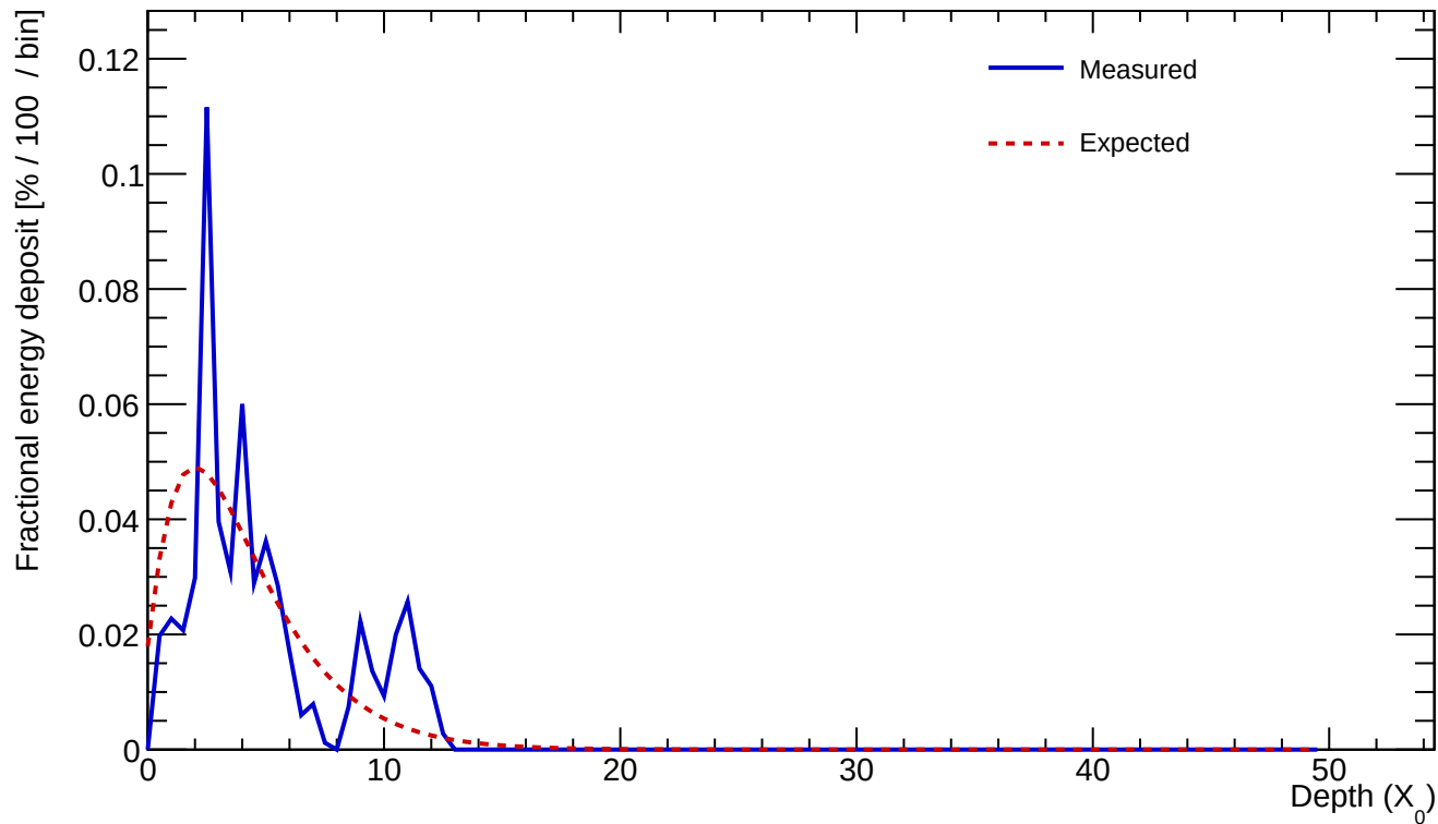
Cluster 17 E=0.587 GeV profileStart=0.50 X_0 \chi=0.5293
