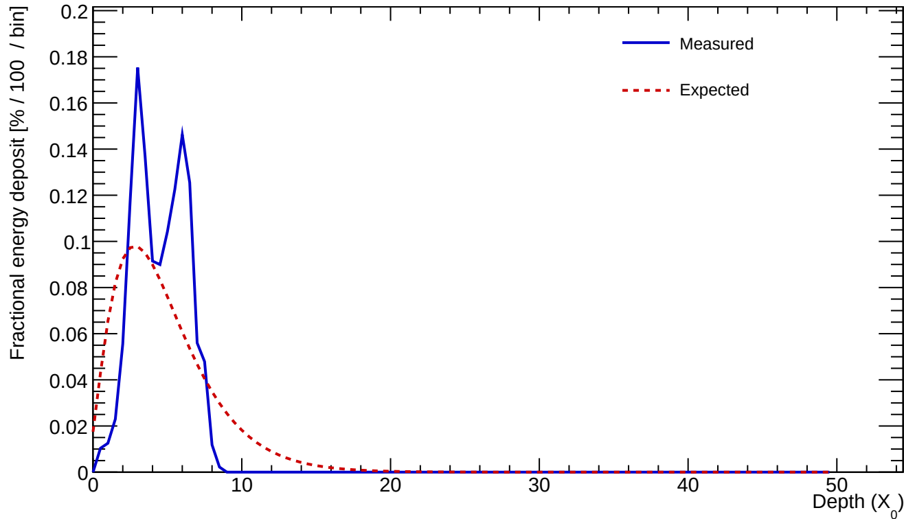
Cluster 3 E=1.329 GeV profileStart=1.00 X_0 \chi=0.3318
