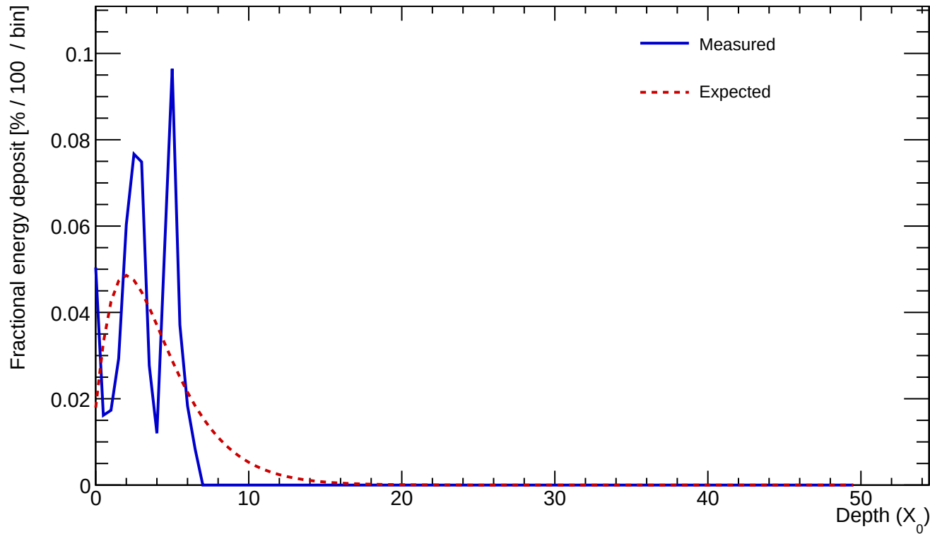
Cluster 34 E=0.579 GeV profileStart=1.00 X_0 \chi=0.4907
