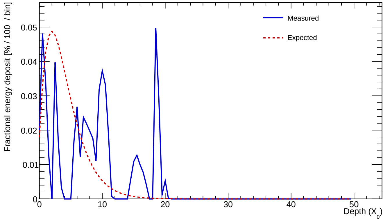
Cluster 58 E=0.582 GeV profileStart=5.50 X_0 \chi=0.9744
