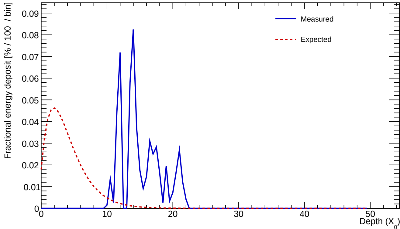
Cluster 57 E=0.546 GeV profileStart=11.00 X_0 \chi=0.6631
