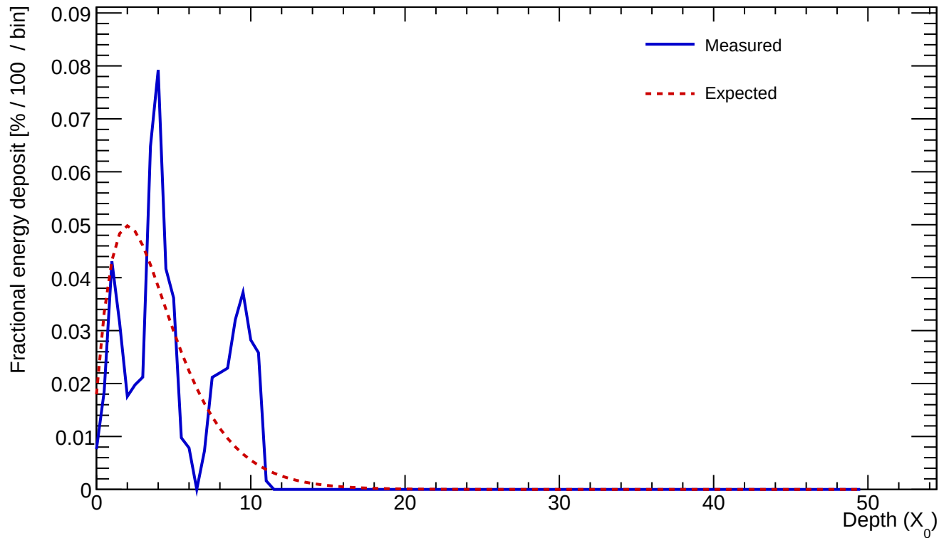
Cluster 49 E=0.597 GeV profileStart=0.50 X_0 \chi=0.6191
