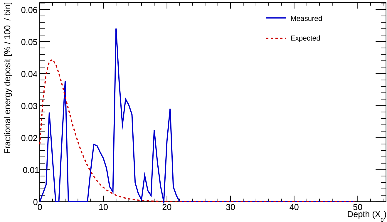
Cluster 21 E=0.520 GeV profileStart=9.50 X_0 \chi=0.8652
