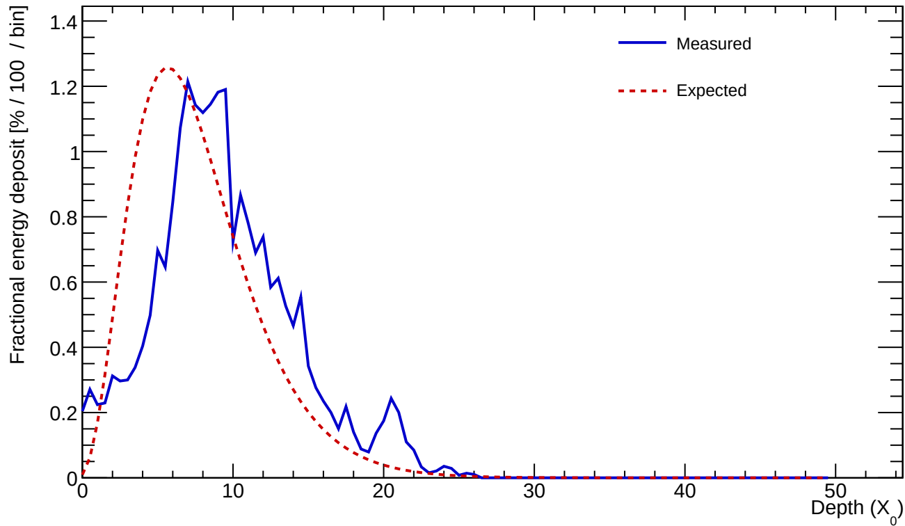
Cluster 36 E=22.720 GeV profileStart=2.00 X_0 \chi=0.2192
