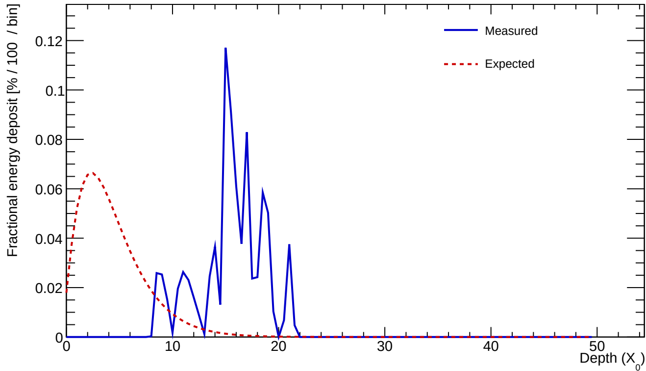
Cluster 53 E=0.844 GeV profileStart=13.50 X_0 \chi=0.6131
