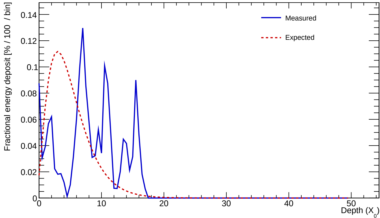
Cluster 26 E=1.546 GeV profileStart=5.00 X_0 \chi=0.6786
