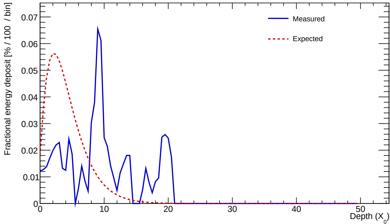
Cluster 25 E=0.695 GeV profileStart=6.50 X_0 \chi=0.8784
