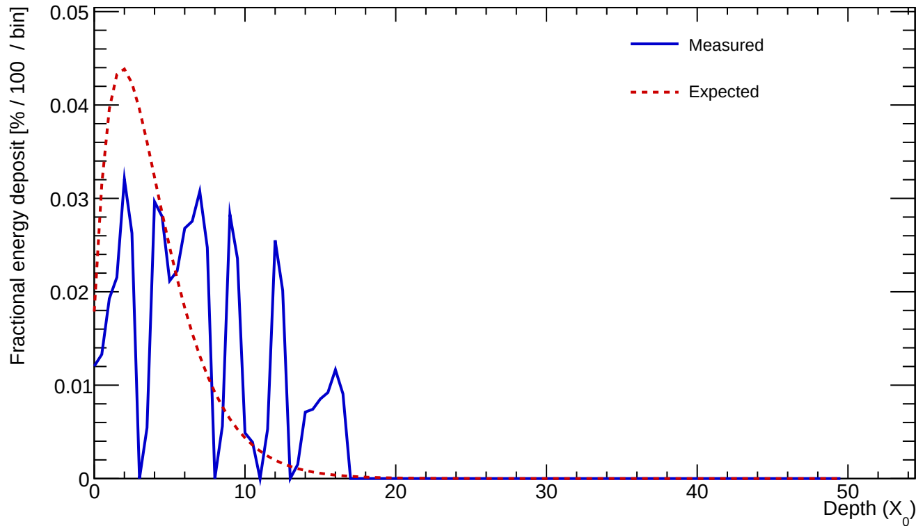
Cluster 42 E=0.513 GeV profileStart=1.00 X_0 \chi=0.6851
