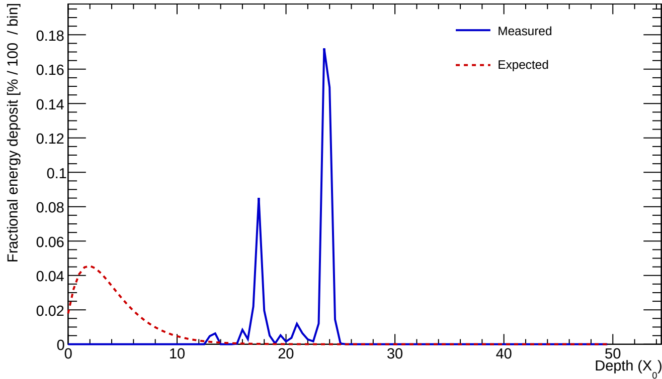
Cluster 91 E=0.536 GeV profileStart=23.00 X_0 \chi=0.8817
