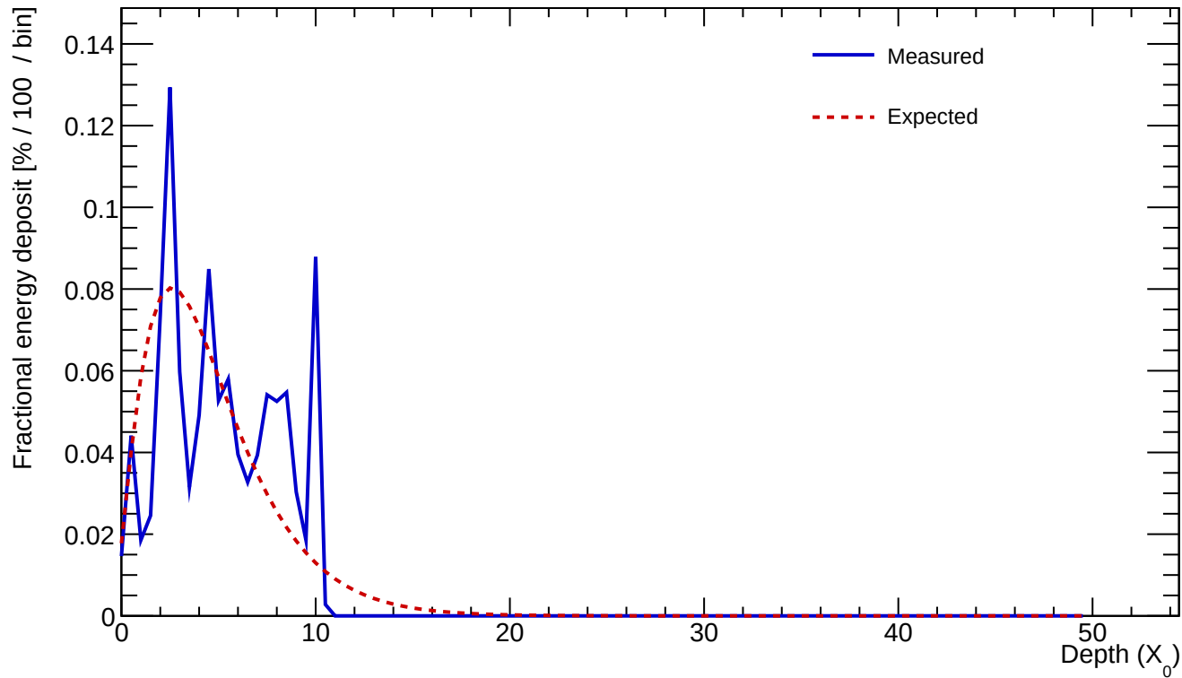
Cluster 14 E=1.053 GeV profileStart=0.50 X_0 \chi=0.4286
