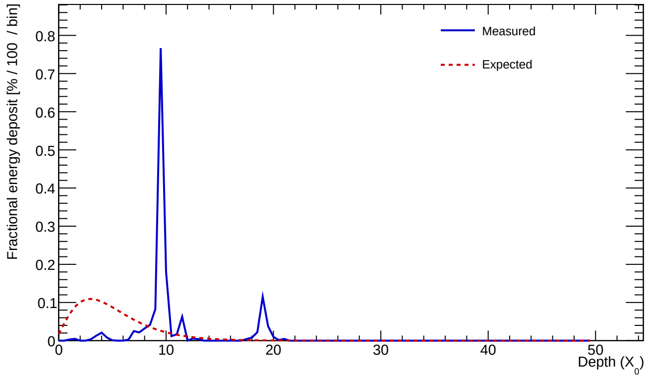
Cluster 85 E=1.509 GeV profileStart=6.50 X_0 \chi=1.2264
