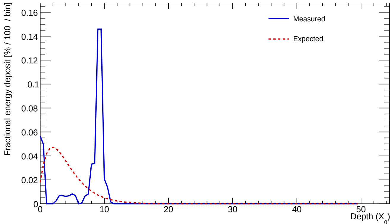
Cluster 55 E=0.561 GeV profileStart=7.50 X_0 \chi=0.7653
