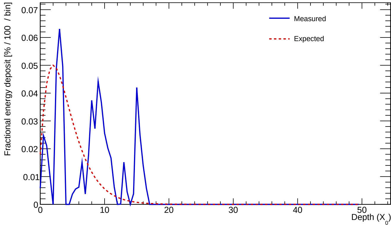
Cluster 8 E=0.600 GeV profileStart=0.50 X_0 \chi=0.9329
