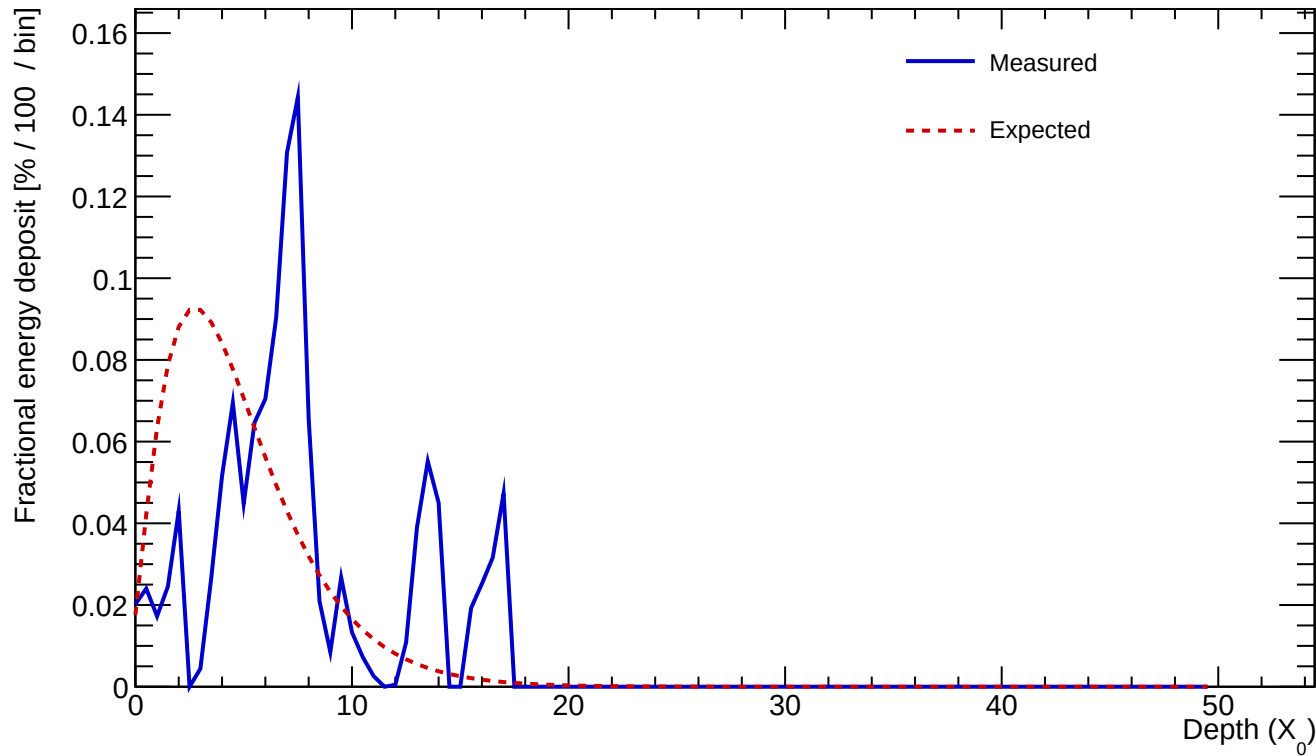
Cluster 23 E=1.245 GeV profileStart=3.00 X_0 \chi=0.6629
