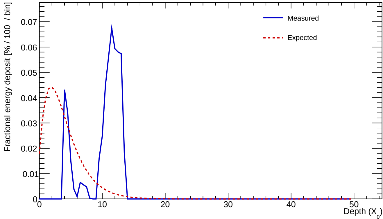
Cluster 69 E=0.517 GeV profileStart=9.50 X_0 \chi=0.4253
