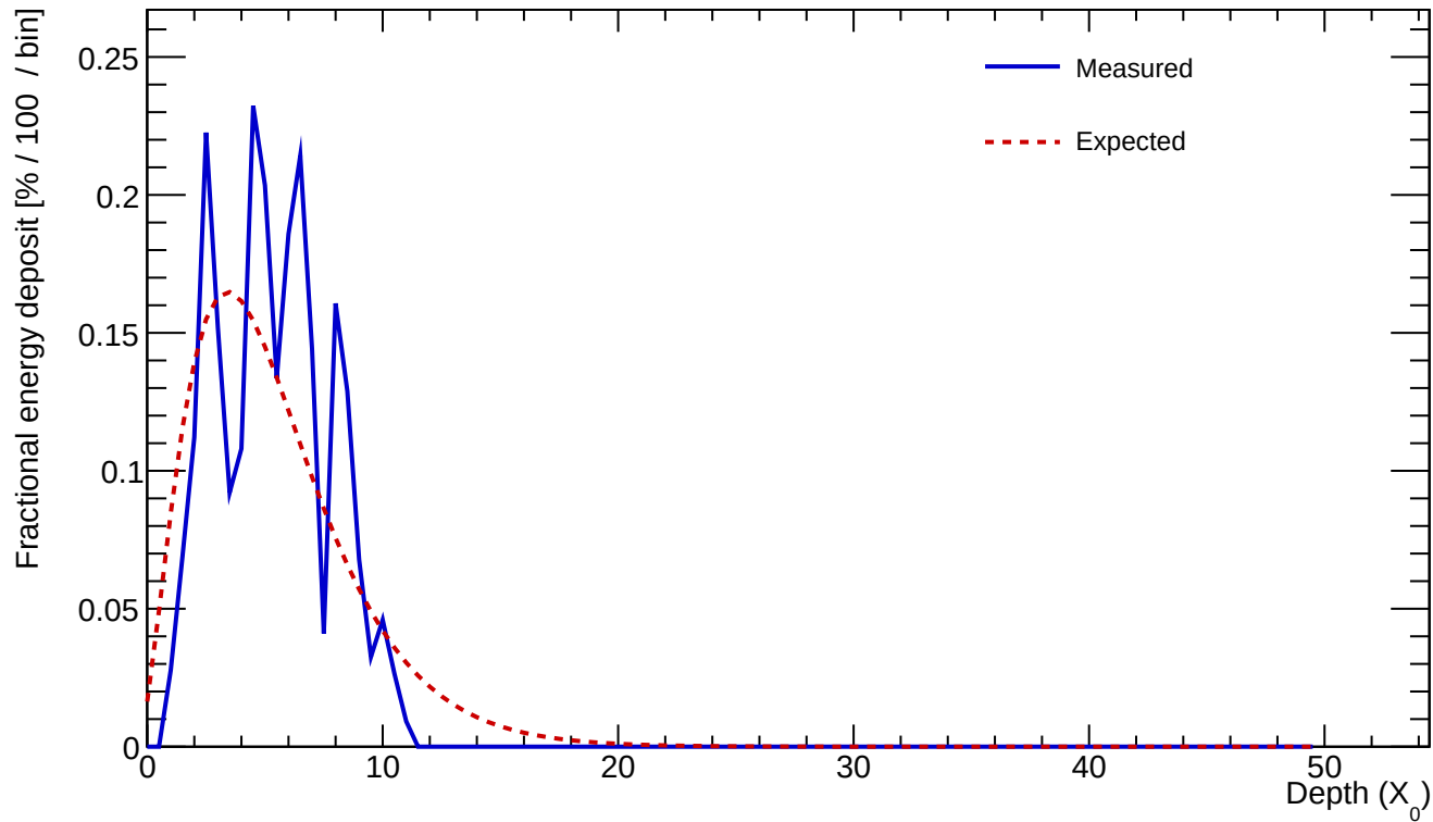
Cluster 44 E=2.410 GeV profileStart=0.50 X_0 \chi=0.3362
