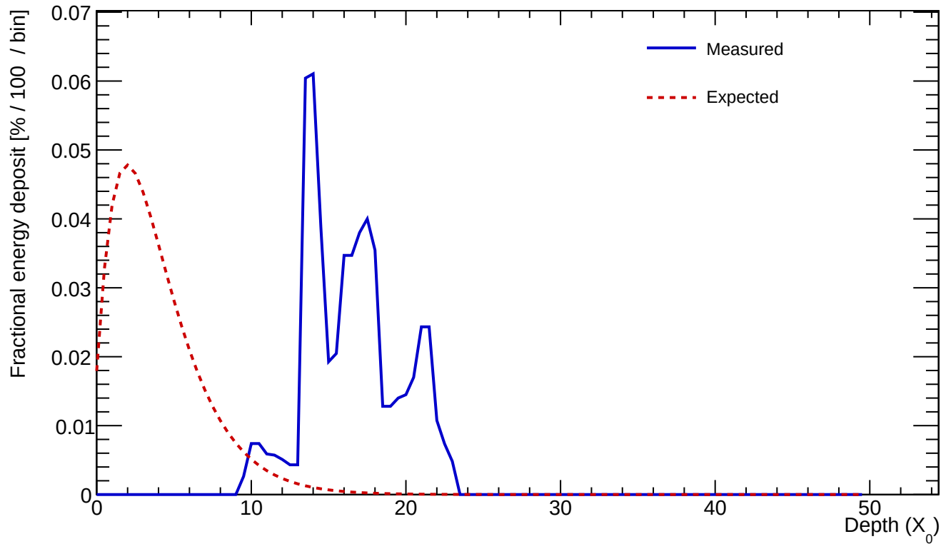
Cluster 68 E=0.568 GeV profileStart=13.00 X_0 \chi=0.4485
