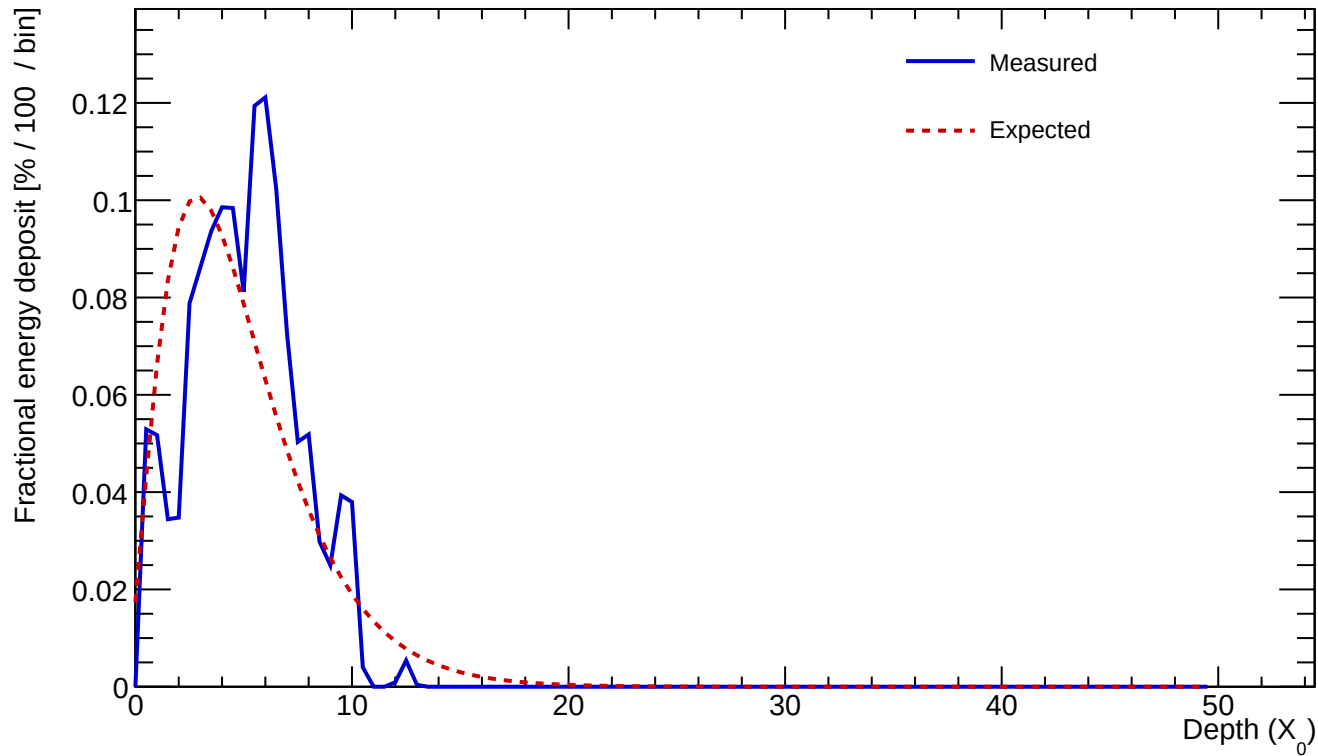
Cluster 43 E=1.371 GeV profileStart=1.00 X_0 \chi=0.2927
