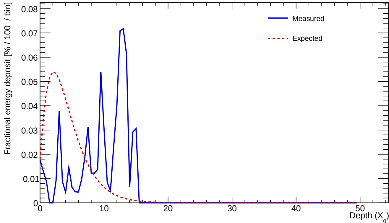
Cluster 84 E=0.659 GeV profileStart=11.50 X_0 \chi=0.6931
