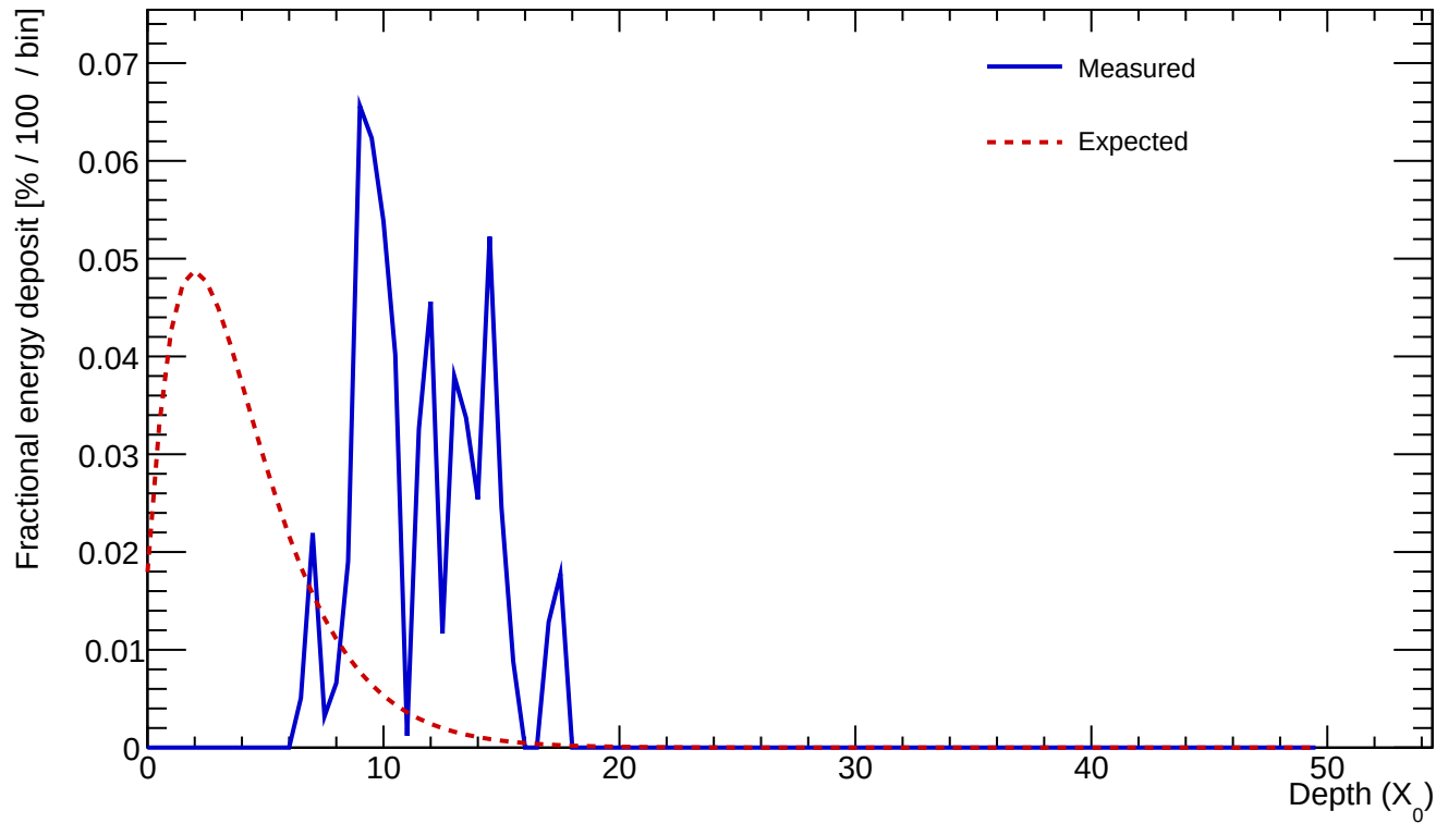
Cluster 63 E=0.582 GeV profileStart=8.50 X_0 \chi=0.4725
