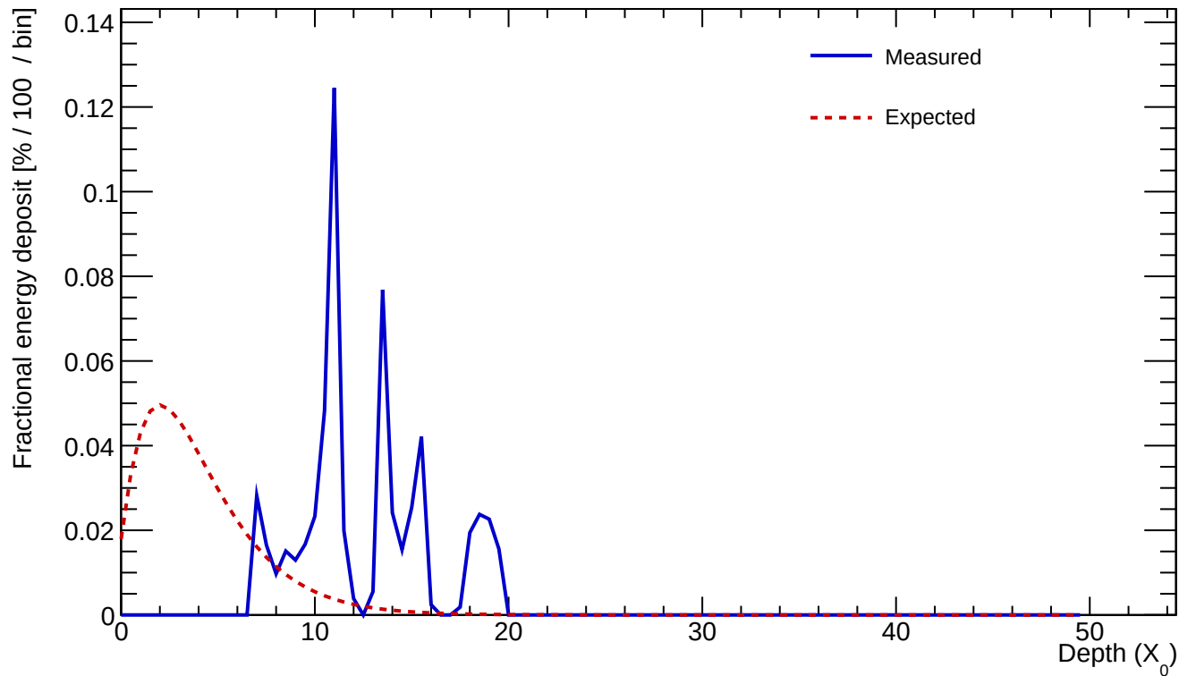
Cluster 50 E=0.594 GeV profileStart=9.00 X_0 \chi=0.8564
