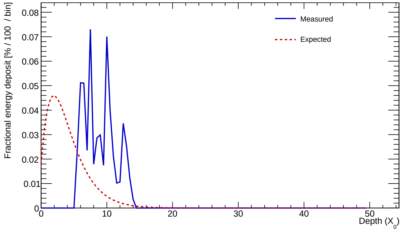
Cluster 73 E=0.543 GeV profileStart=5.50 X_0 \chi=0.4686
