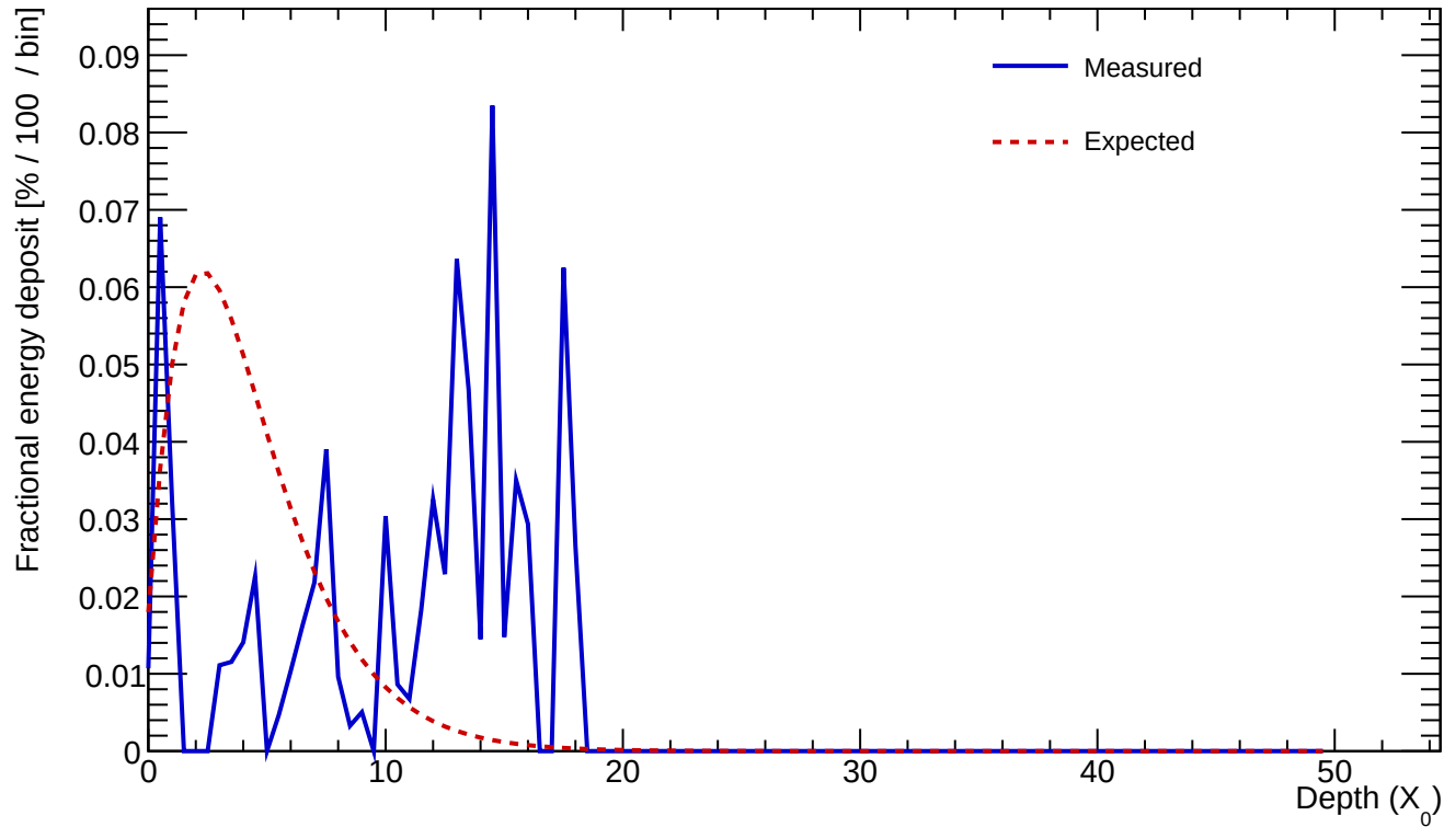
Cluster 24 E=0.777 GeV profileStart=11.50 X_0 \chi=0.8138
