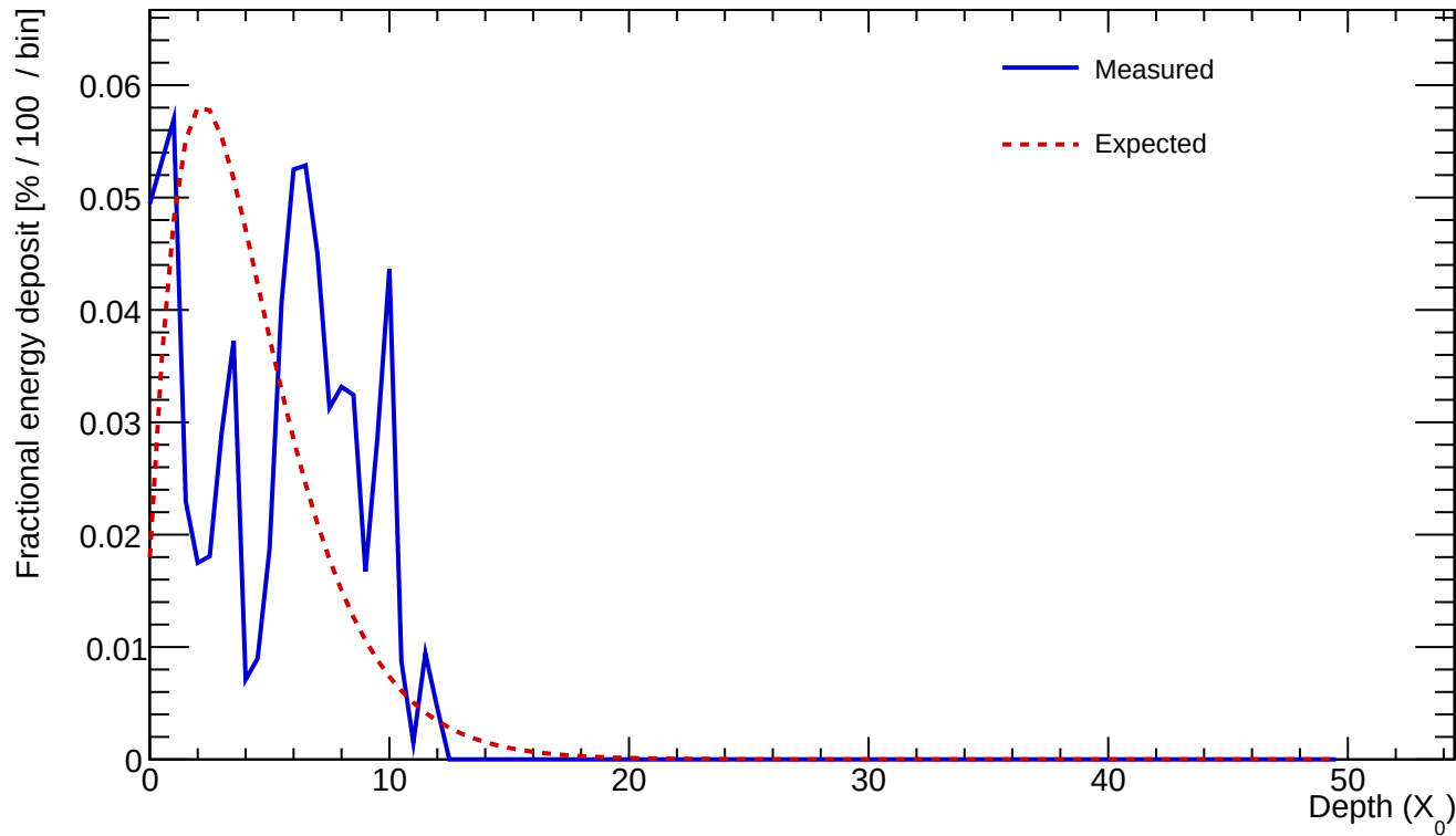
Cluster 89 E=0.720 GeV profileStart=2.50 X_0 \chi =0.6216
