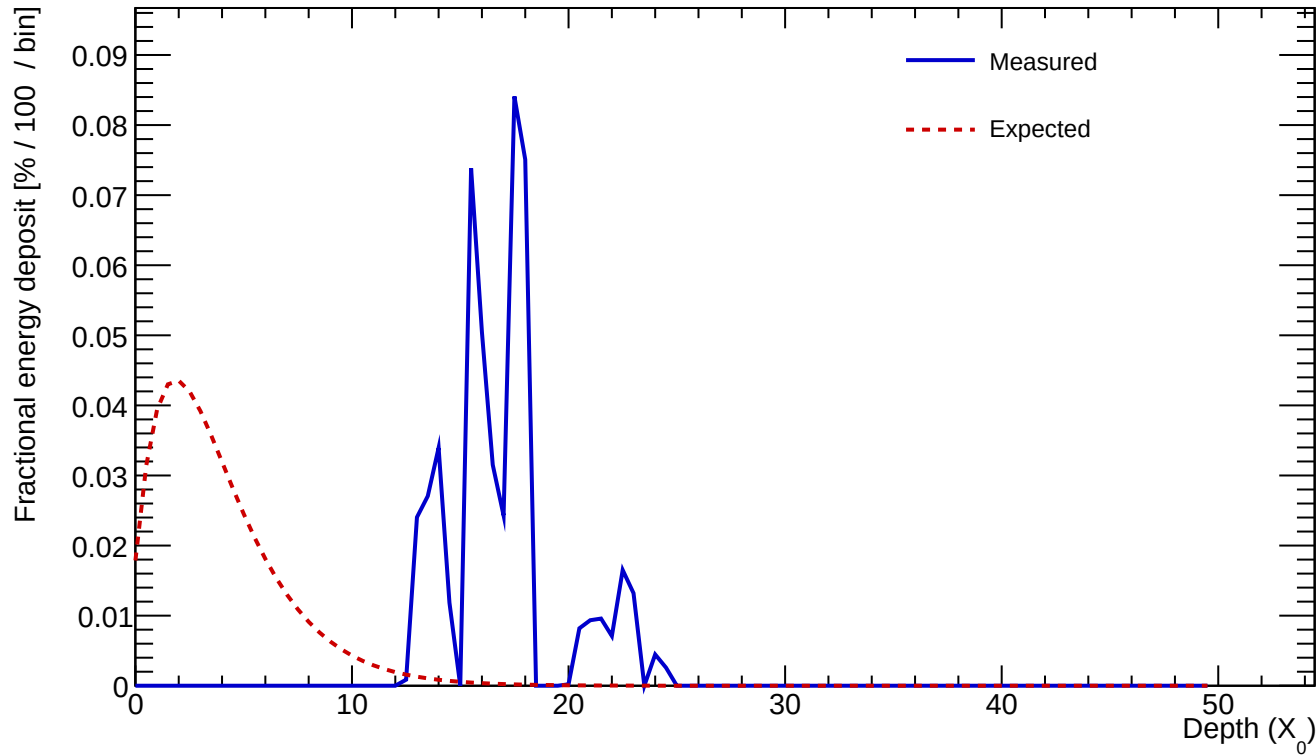
Cluster 48 E=0.508 GeV profileStart=13.00 X_0 \chi=0.6913
