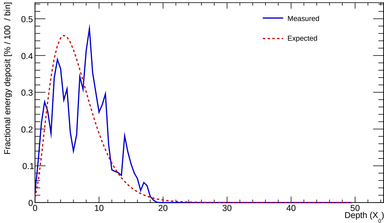
Cluster 10 E=7.477 GeV profileStart=0.50 X_0 \chi=0.3944
