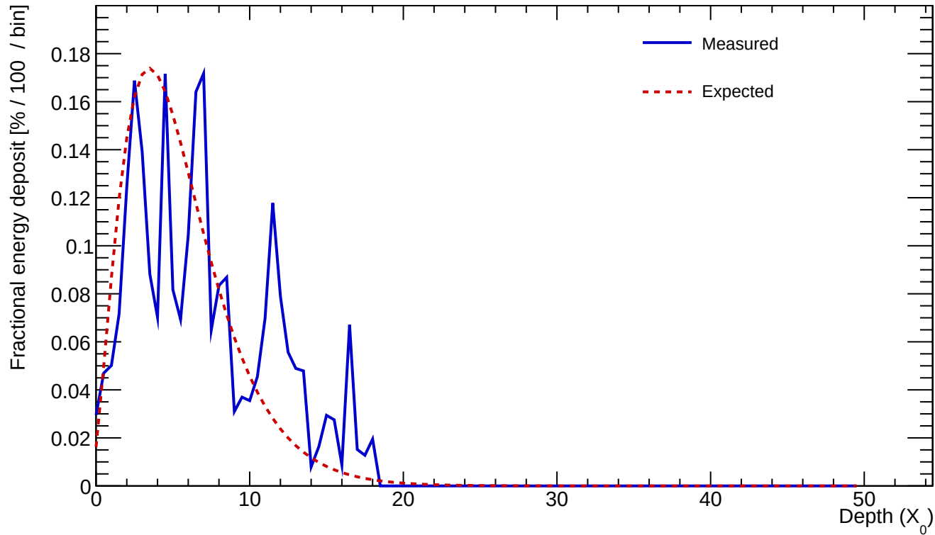
Cluster 20 E=2.560 GeV profileStart=0.50 X_0 \chi=0.4444
