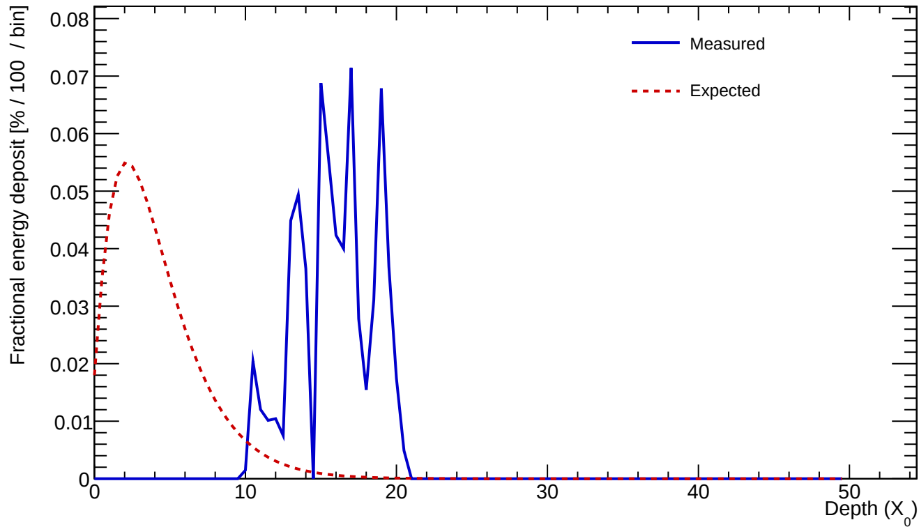
Cluster 9 E=0.672 GeV profileStart=12.50 X_0 \chi=0.4464
