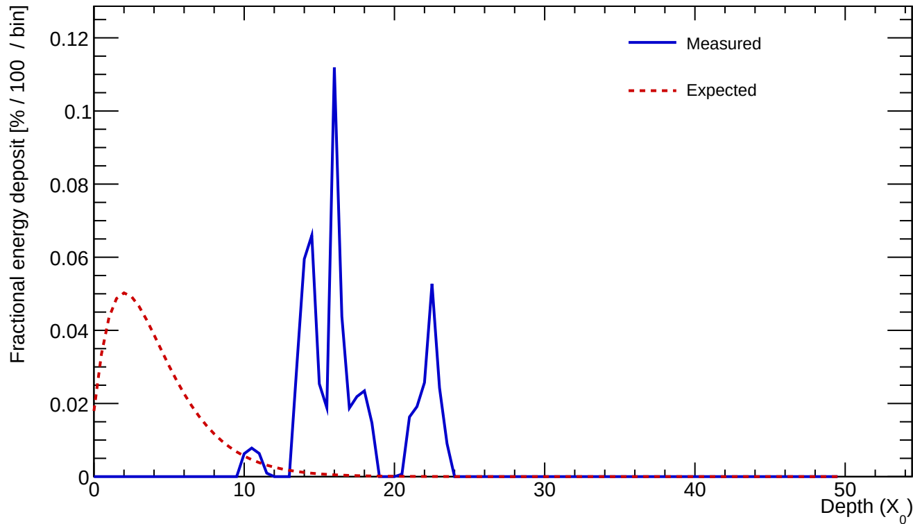
Cluster 60 E=0.604 GeV profileStart=13.00 X_0 \chi=0.6901
