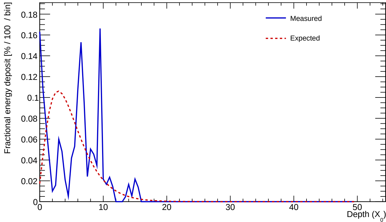
Cluster 74 E=1.457 GeV profileStart=2.50 X_0 \chi=0.8129
