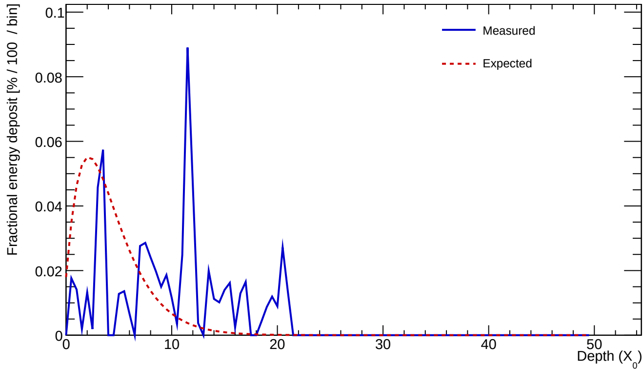
Cluster 56 E=0.675 GeV profileStart=2.00 X_0 \chi=0.9727
