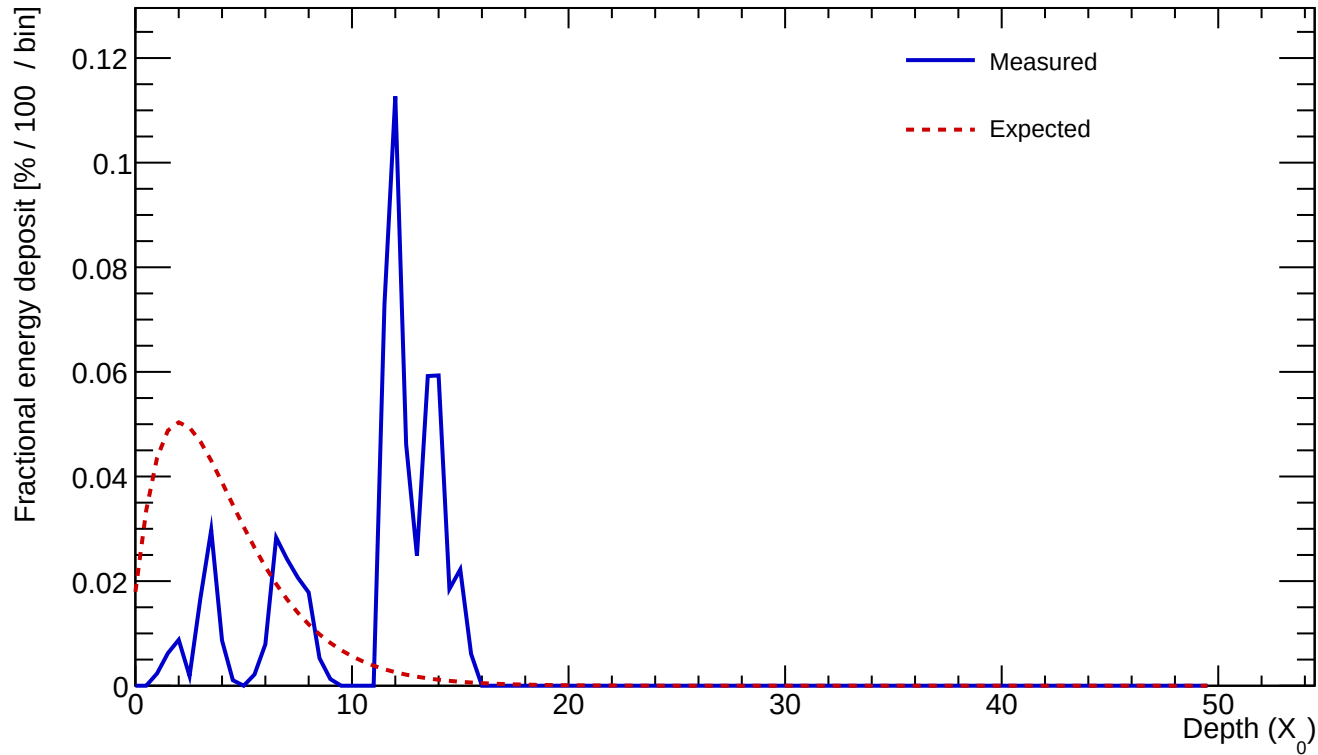
Cluster 16 E=0.605 GeV profileStart=11.00 X_0 \chi=0.6632
