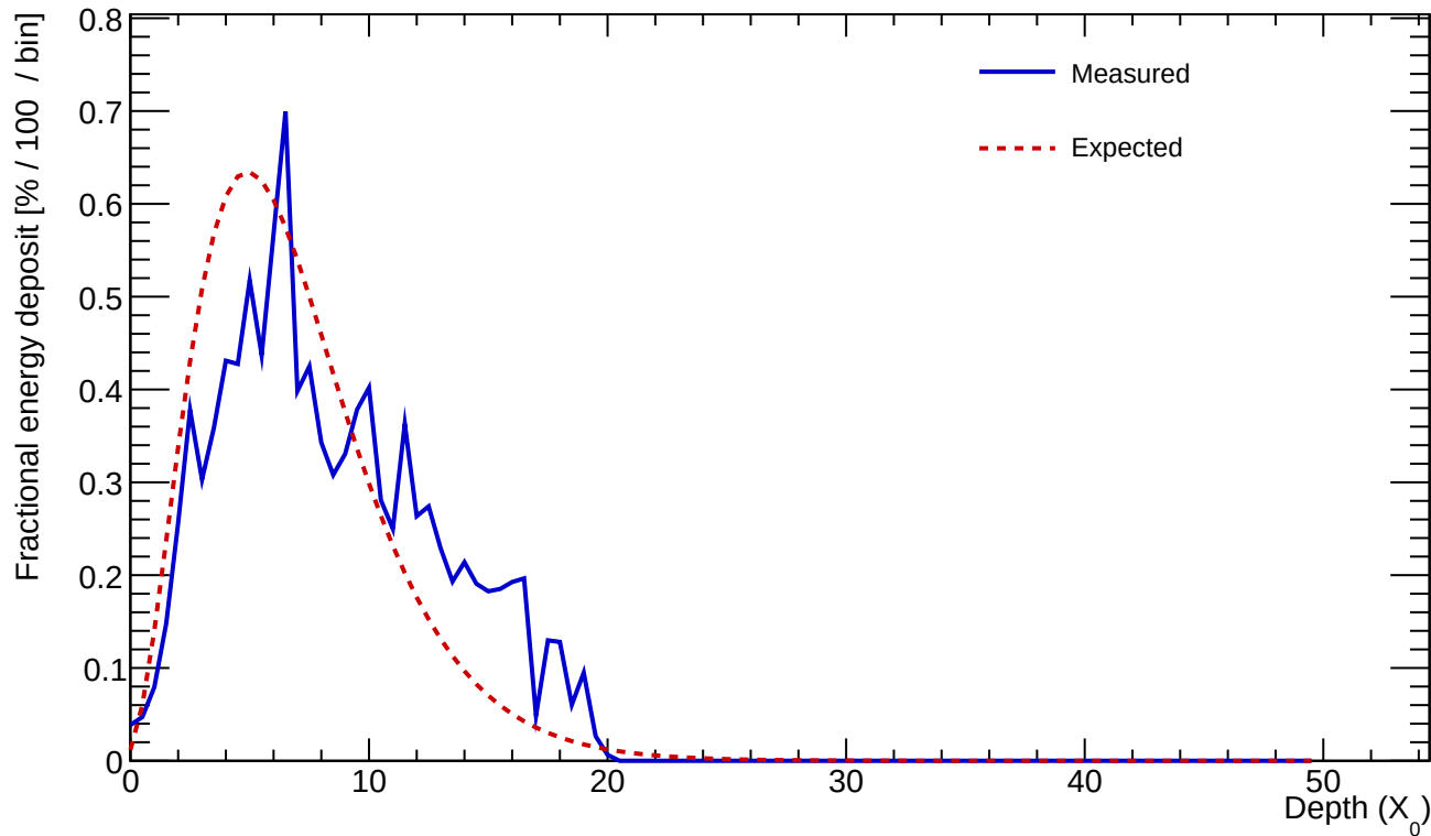
Cluster 13 E=10.784 GeV profileStart=0.50 X_0 \chi=0.3186
