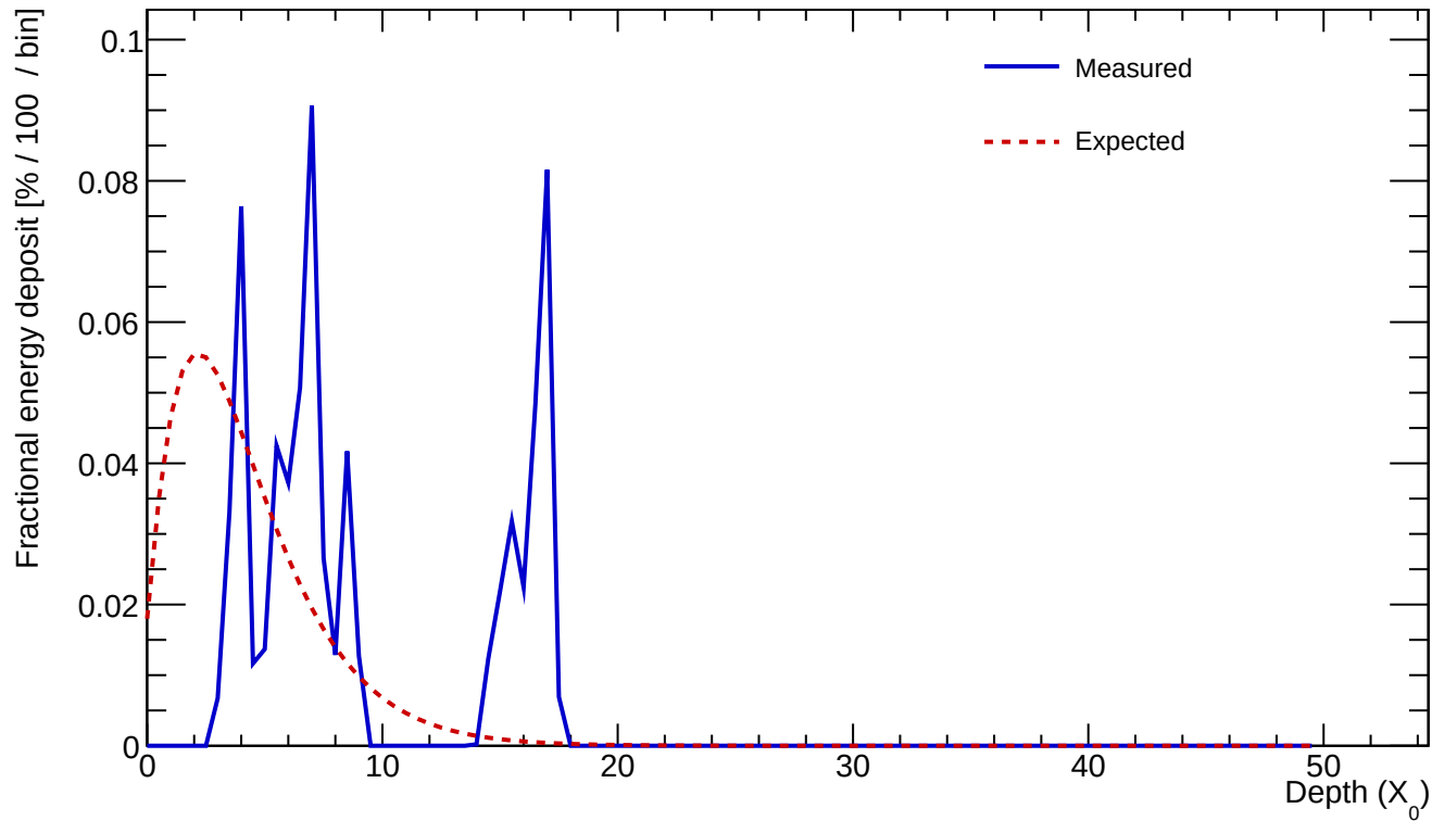
Cluster 38 E=0.682 GeV profileStart=3.00 X_0 \chi=0.8579
