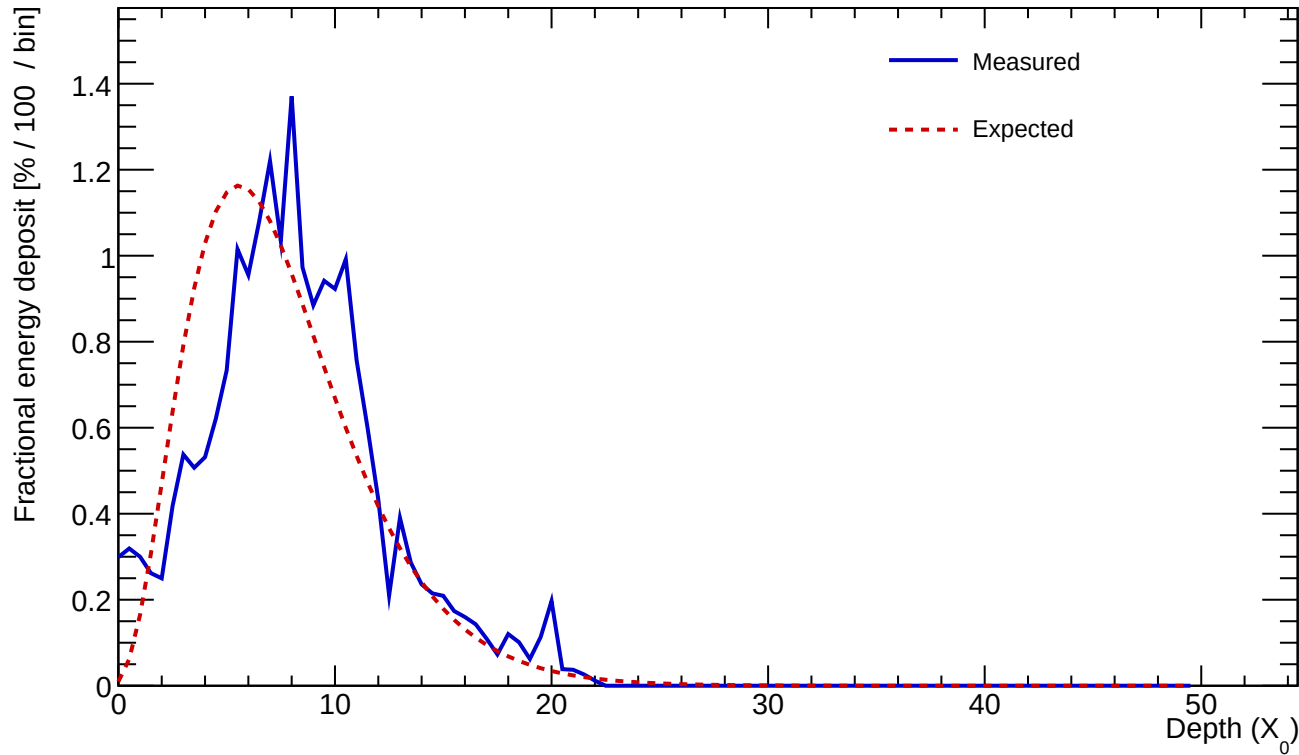
Cluster 15 E=20.871 GeV profileStart=1.00 X_0 \chi=0.2317
