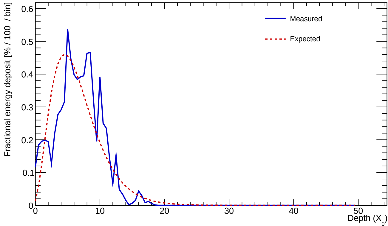
Cluster 28 E=7.577 GeV profileStart=1.50 X_0 \chi=0.3141
