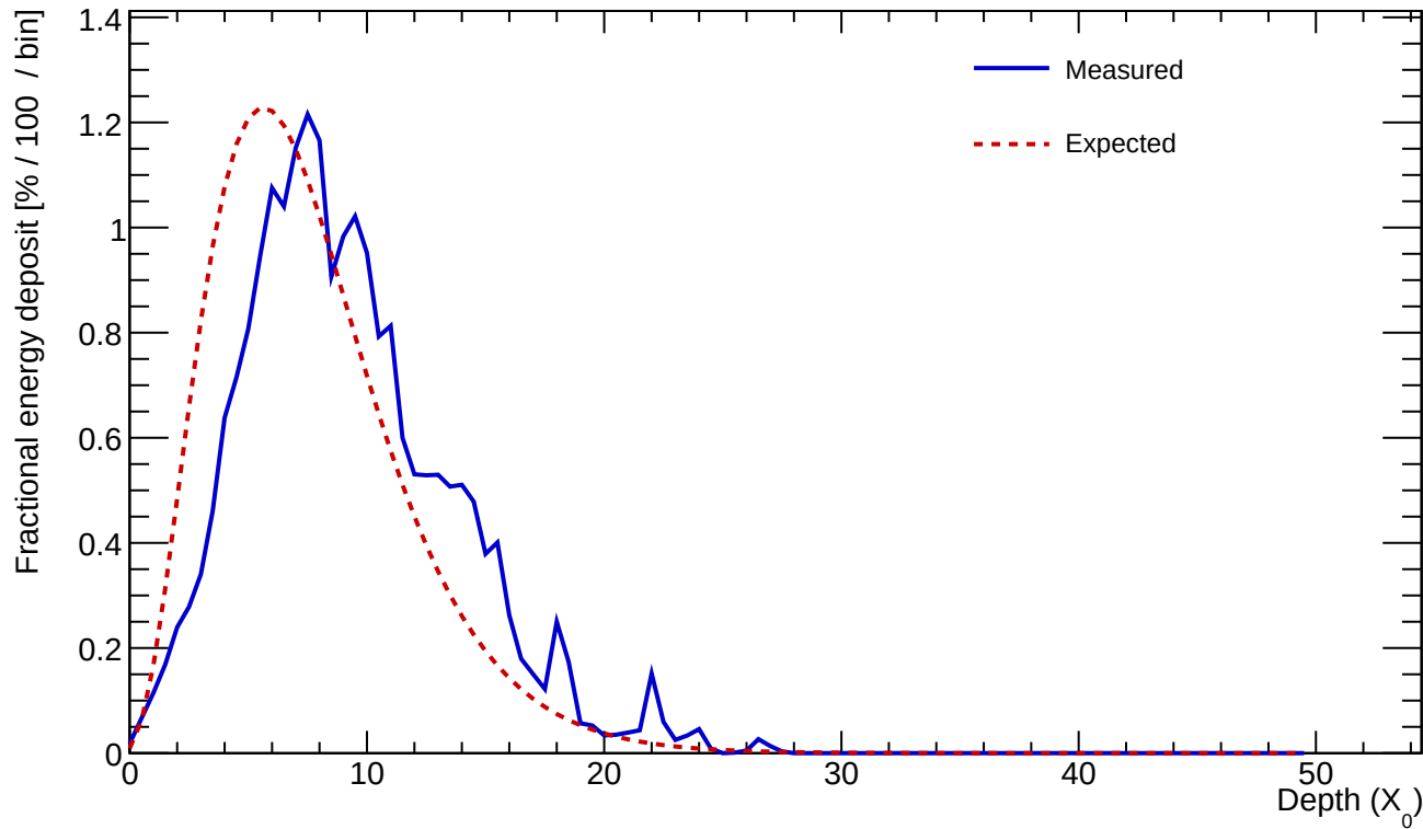
Cluster 88 E=22.150 GeV profileStart=1.50 X_0 \chi=0.1536
