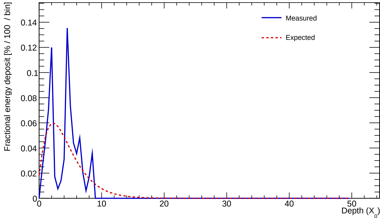
Cluster 54 E=0.744 GeV profileStart=0.50 X_0 \chi =0.5691
