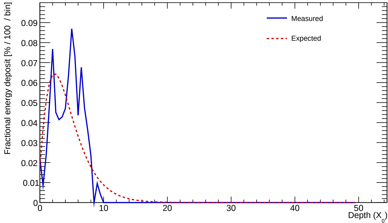
Cluster 40 E=0.813 GeV profileStart=1.00 X_0 \chi=0.3604
