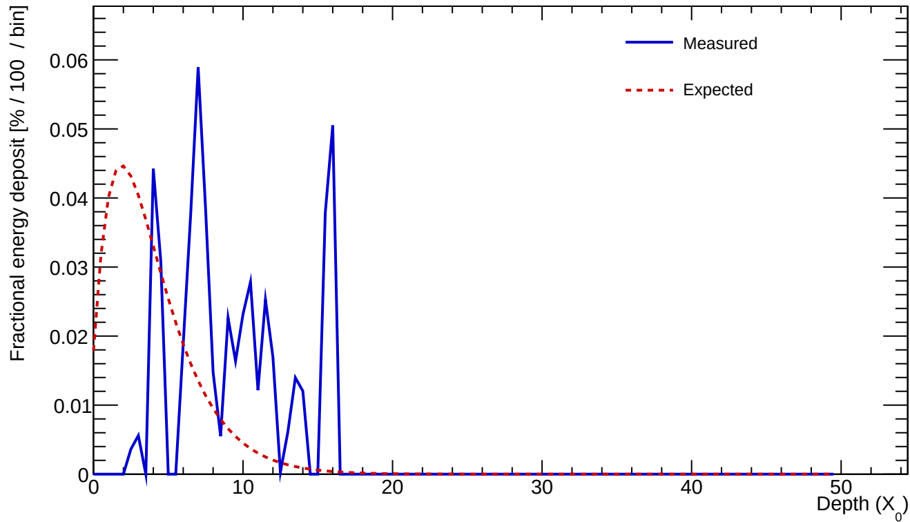
Cluster 83 E=0.523 GeV profileStart=6.00 X_0 \chi=0.6231
