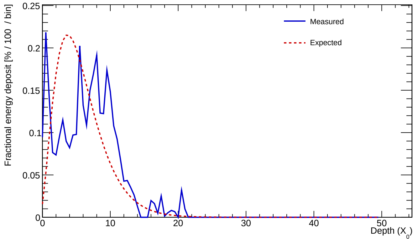
Cluster 19 E=3.260 GeV profileStart=1.50 X_0 \chi=0.4876
