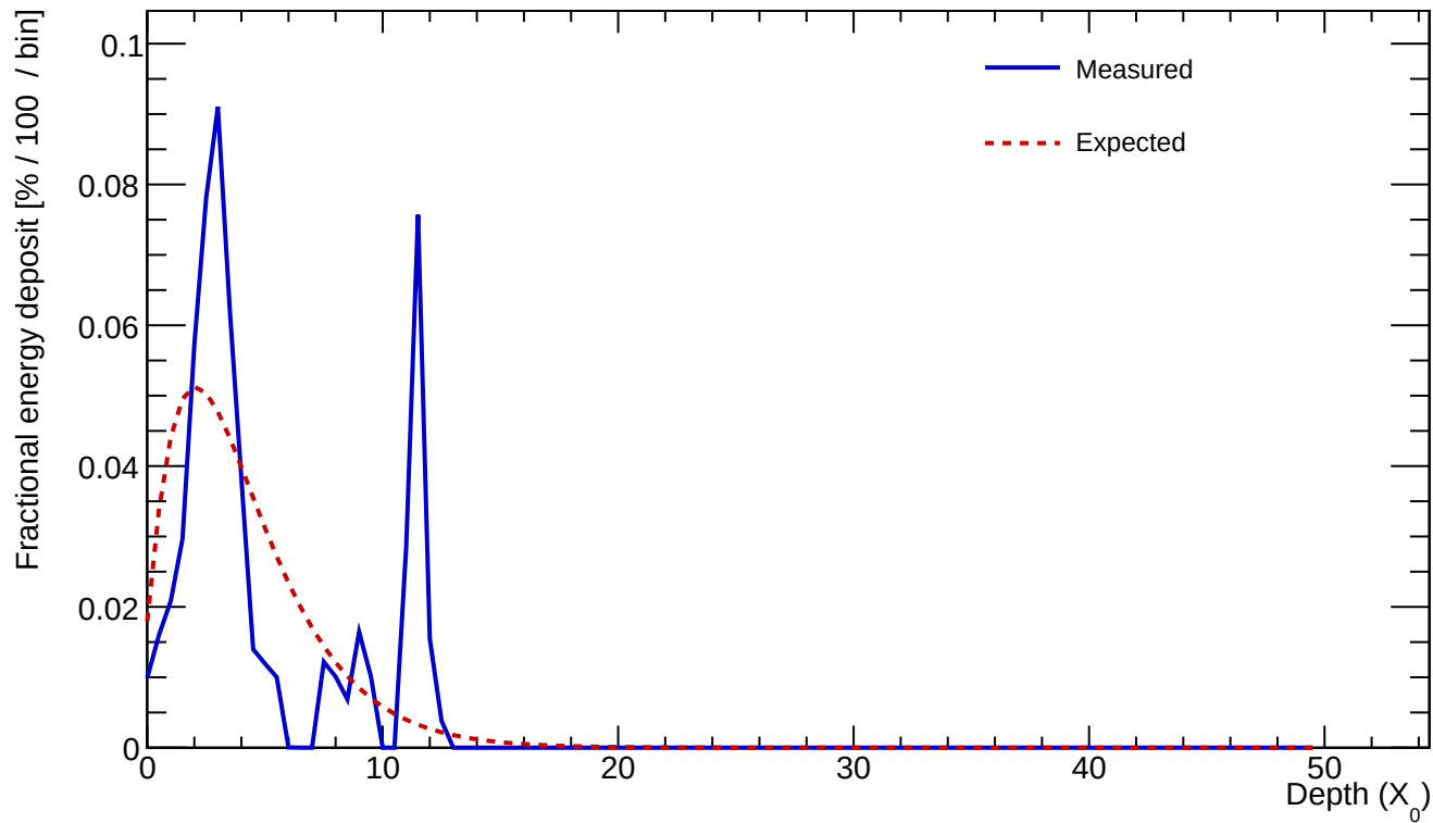
Cluster 62 E=0.619 GeV profileStart=0.50 X_0 \chi=0.6773
