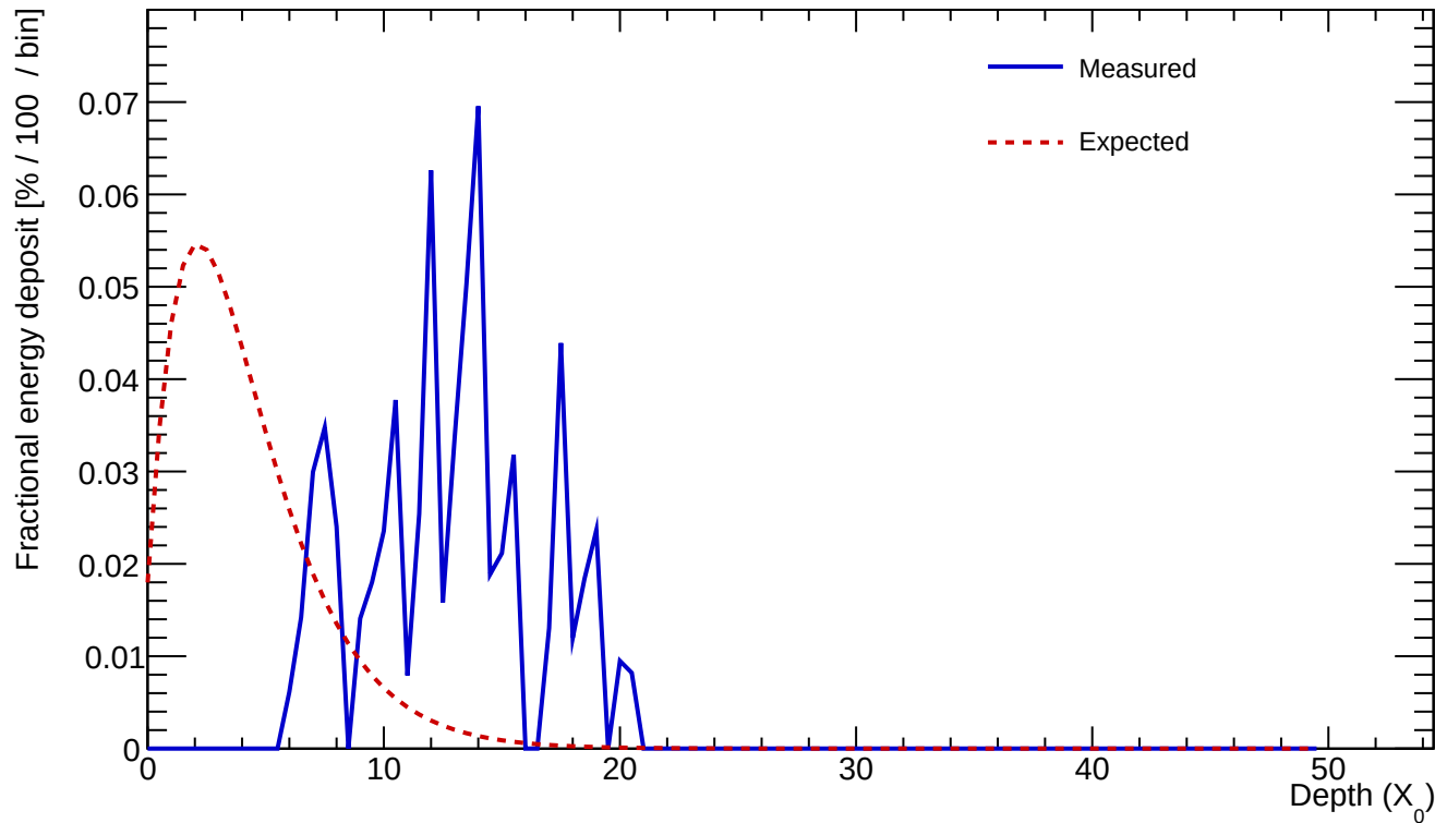
Cluster 51 E=0.668 GeV profileStart=9.50 X_0 \chi=0.6776
