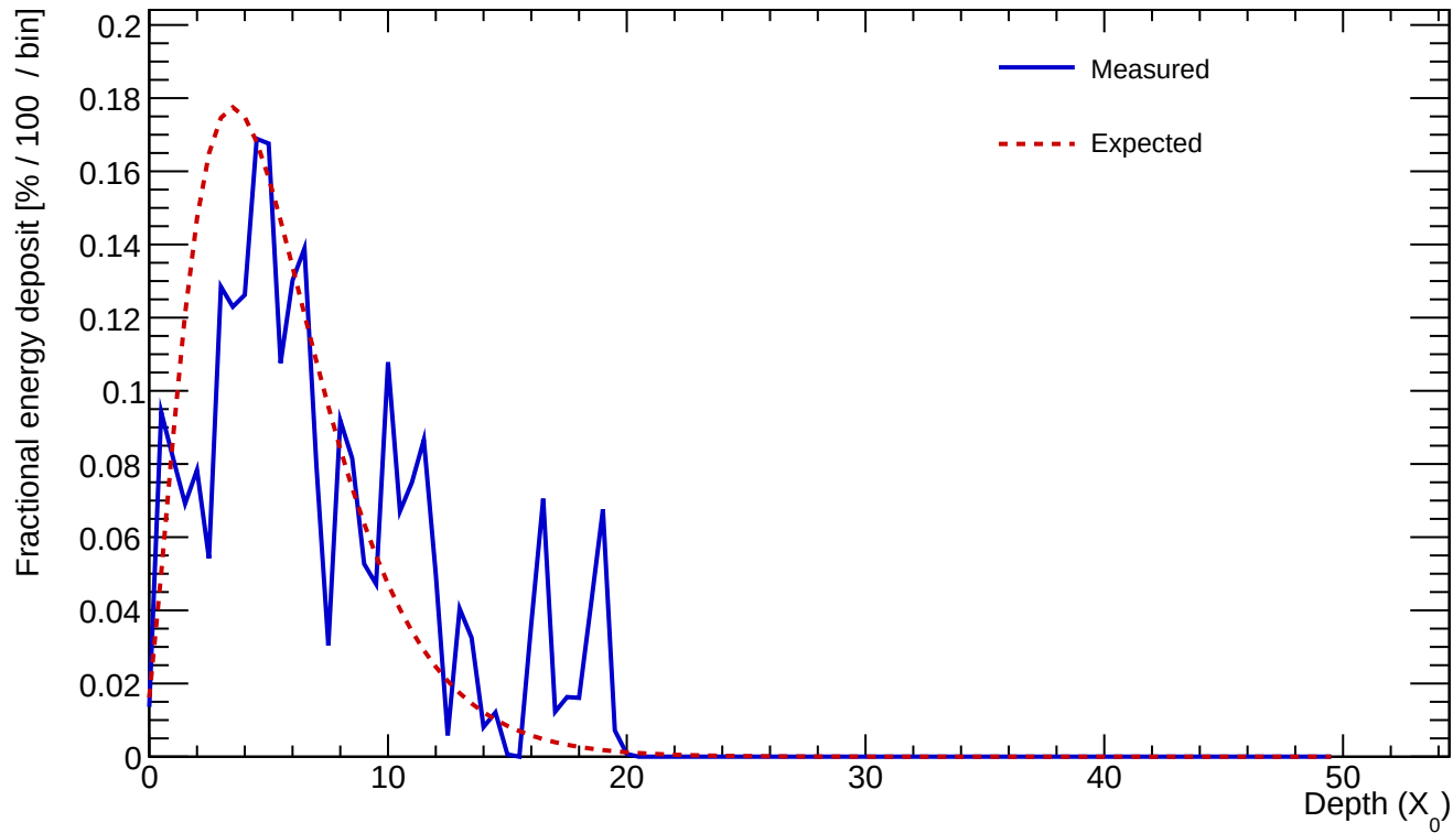
Cluster 35 E=2.620 GeV profileStart=0.50 X_0 \chi=0.4400
