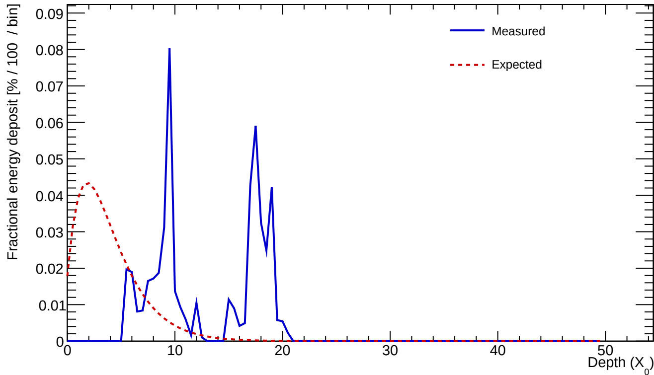
Cluster 5 E=0.505 GeV profileStart=5.50 X_0 \chi=1.0522
