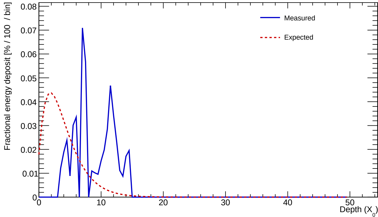
Cluster 76 E=0.510 GeV profileStart=5.00 X_0 \chi=0.7073
