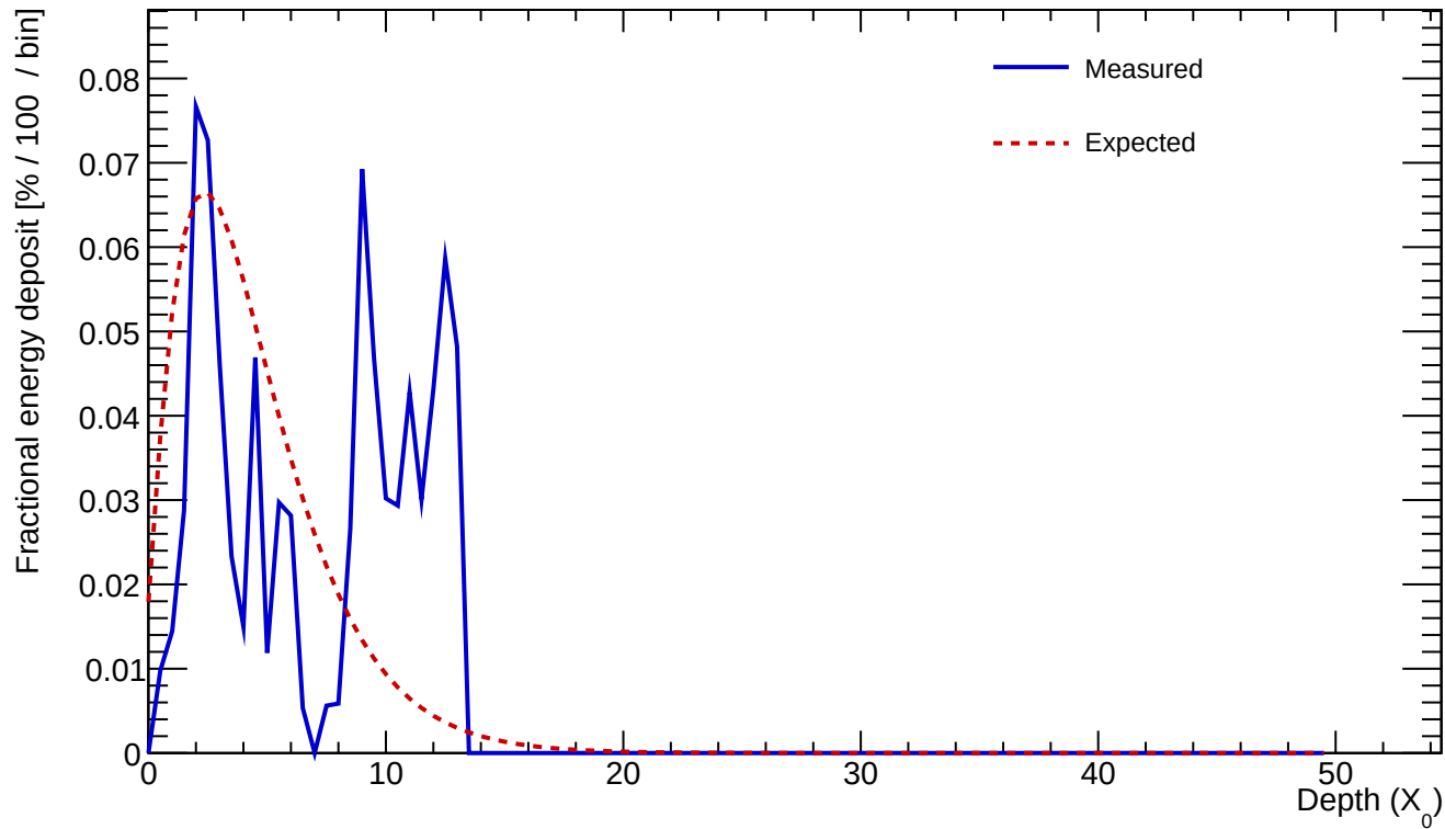
Cluster 86 E=0.845 GeV profileStart=0.50 X_0 \chi=0.7572
