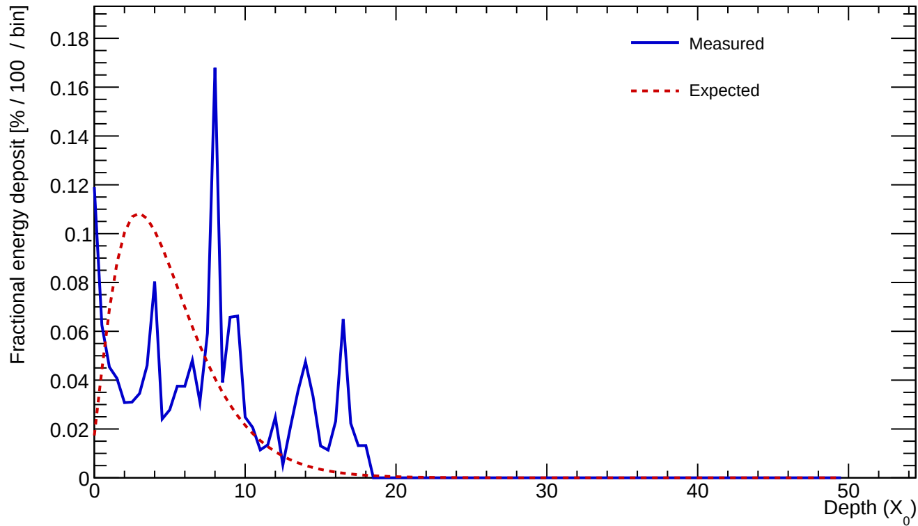
Cluster 33 E=1.494 GeV profileStart=2.50 X_0 \chi=0.8167
