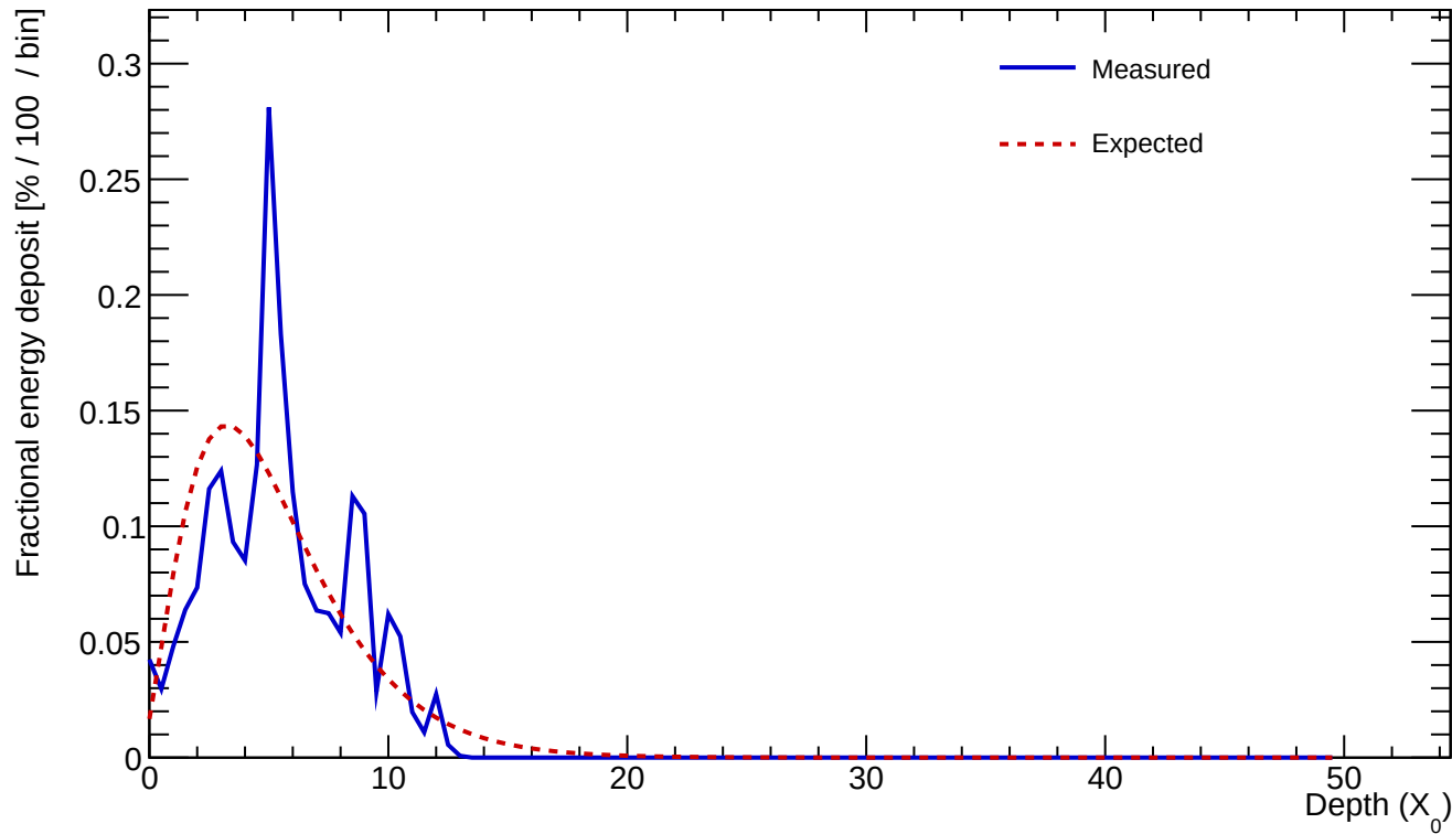
Cluster 71 E=2.063 GeV profileStart=0.50 X_0 \chi=0.3642
