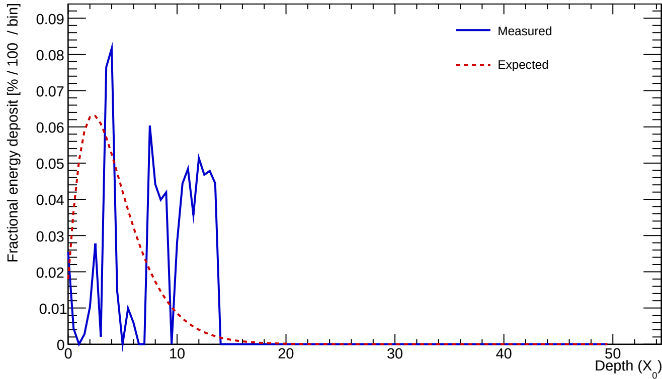
Cluster 4 E=0.795 GeV profileStart=7.50 X_0 \chi=0.6265
