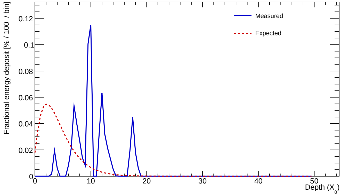
Cluster 75 E=0.671 GeV profileStart=6.50 X_0 \chi=0.8198
