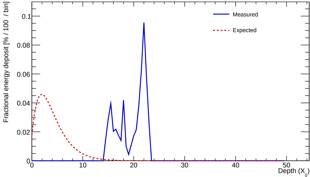
Cluster 61 E=0.544 GeV profileStart=20.00 X_0 \chi=0.5856
