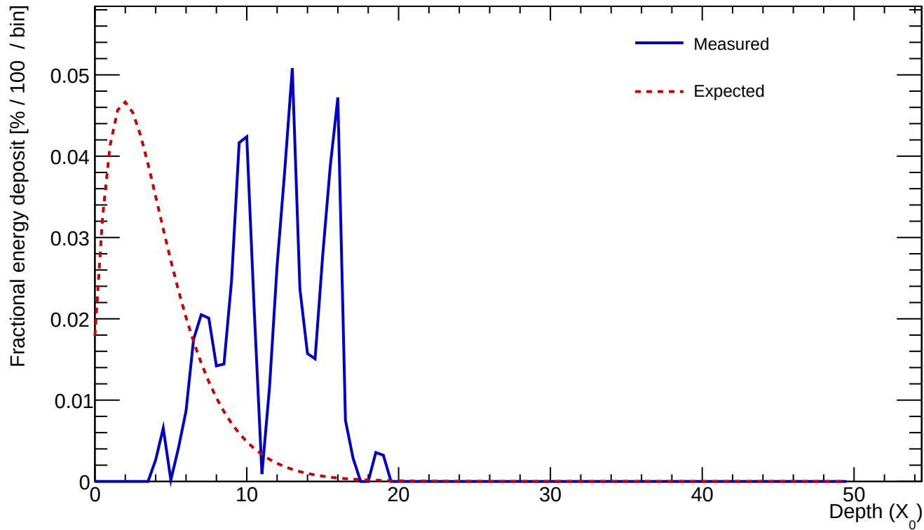
Cluster 46 E=0.552 GeV profileStart=8.50 X_0 \chi=0.6430
