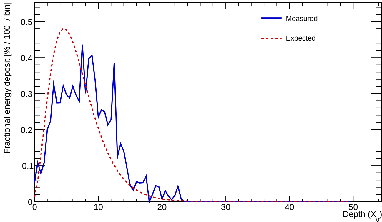
Cluster 29 E=7.952 GeV profileStart=1.50 X_0 \chi =0.3381
