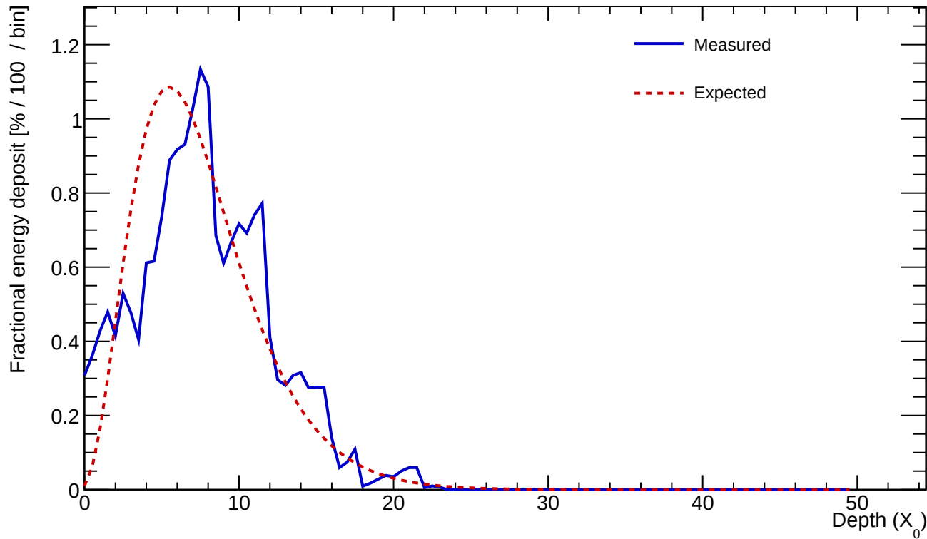
Cluster 47 E=19.376 GeV profileStart=1.00 X_0 \chi=0.2881
