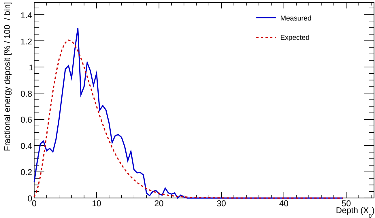
Cluster 2 E=21.689 GeV profileStart=1.50 X_0 \chi=0.2132
