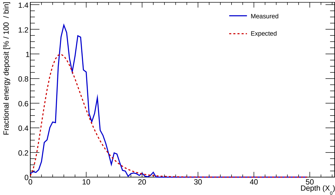
Cluster 80 E=17.658 GeV profileStart=1.00 X_0 \chi=0.2225
