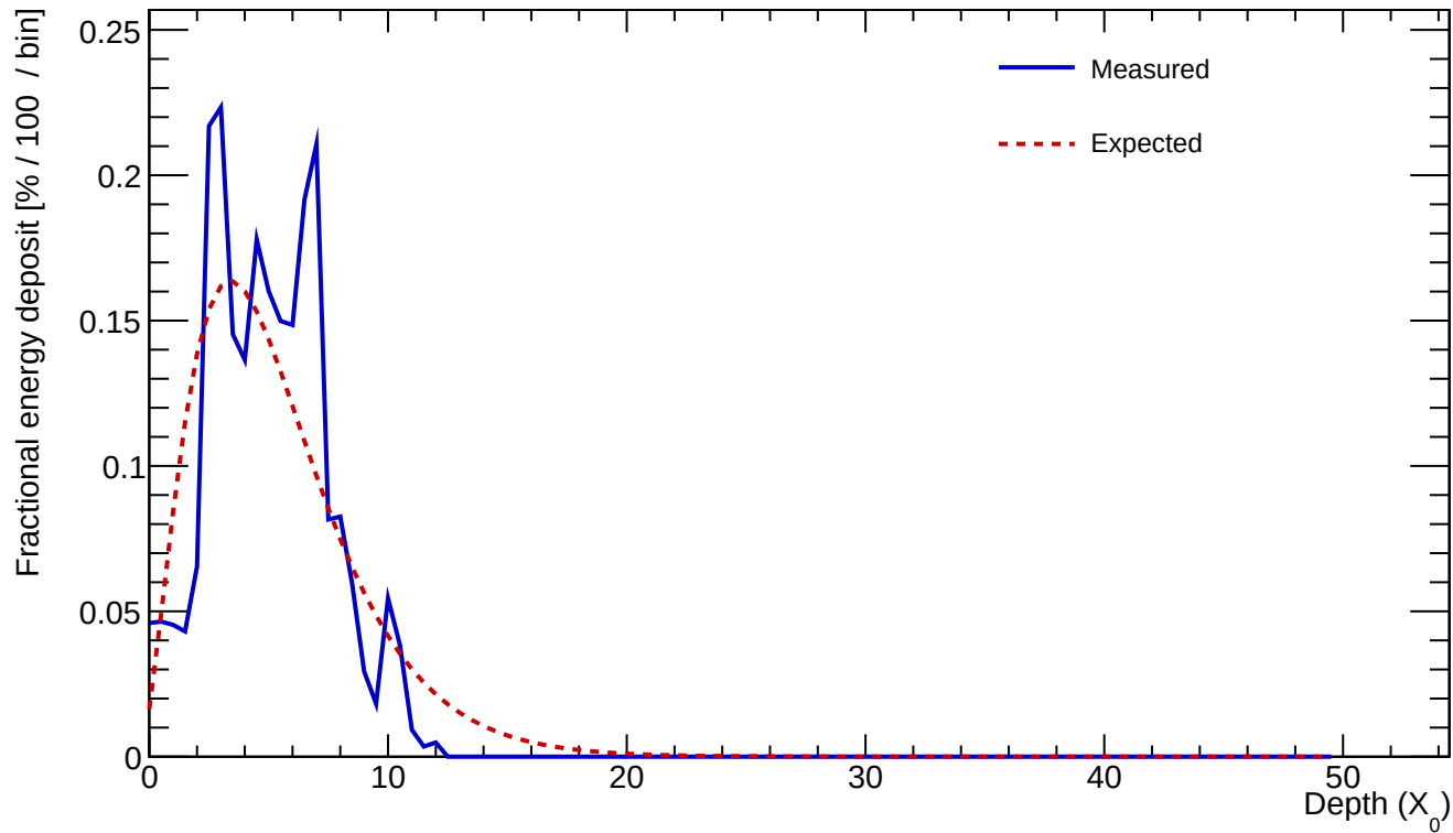
Cluster 65 E=2.389 GeV profileStart=0.50 X_0 \chi=0.3148
