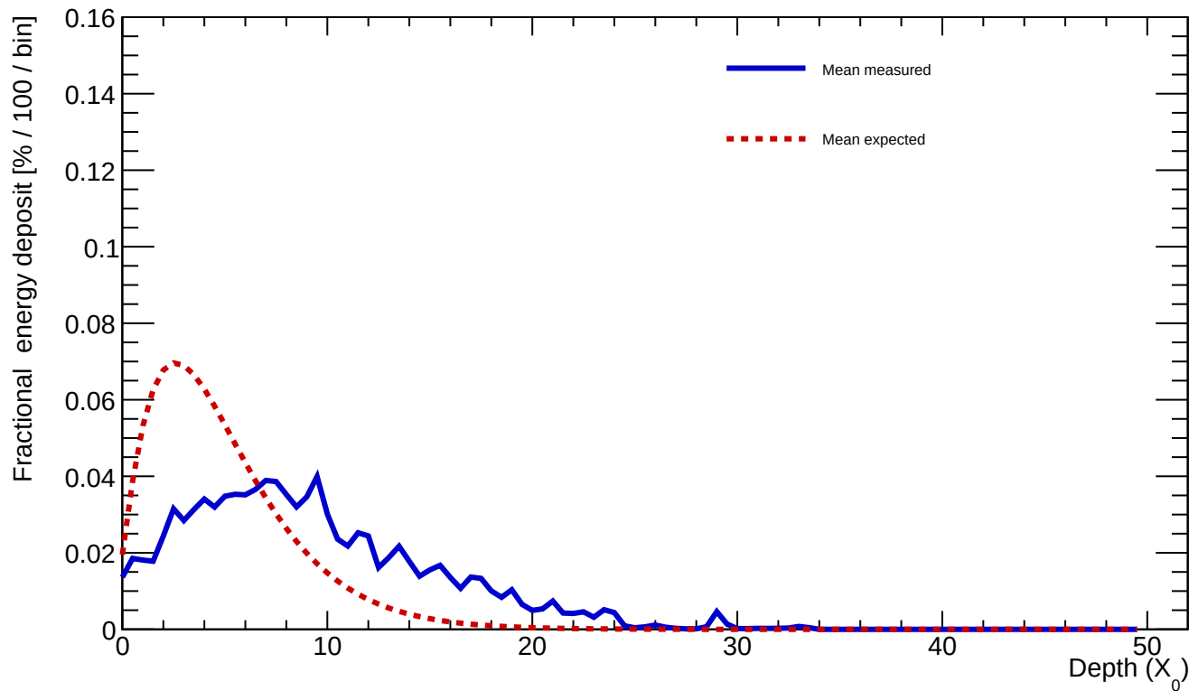
Average longitudinal profile (92 clusters): measured vs expected
