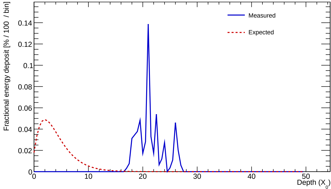
Cluster 78 E=0.584 GeV profileStart=17.50 X_0 \chi=0.5752
