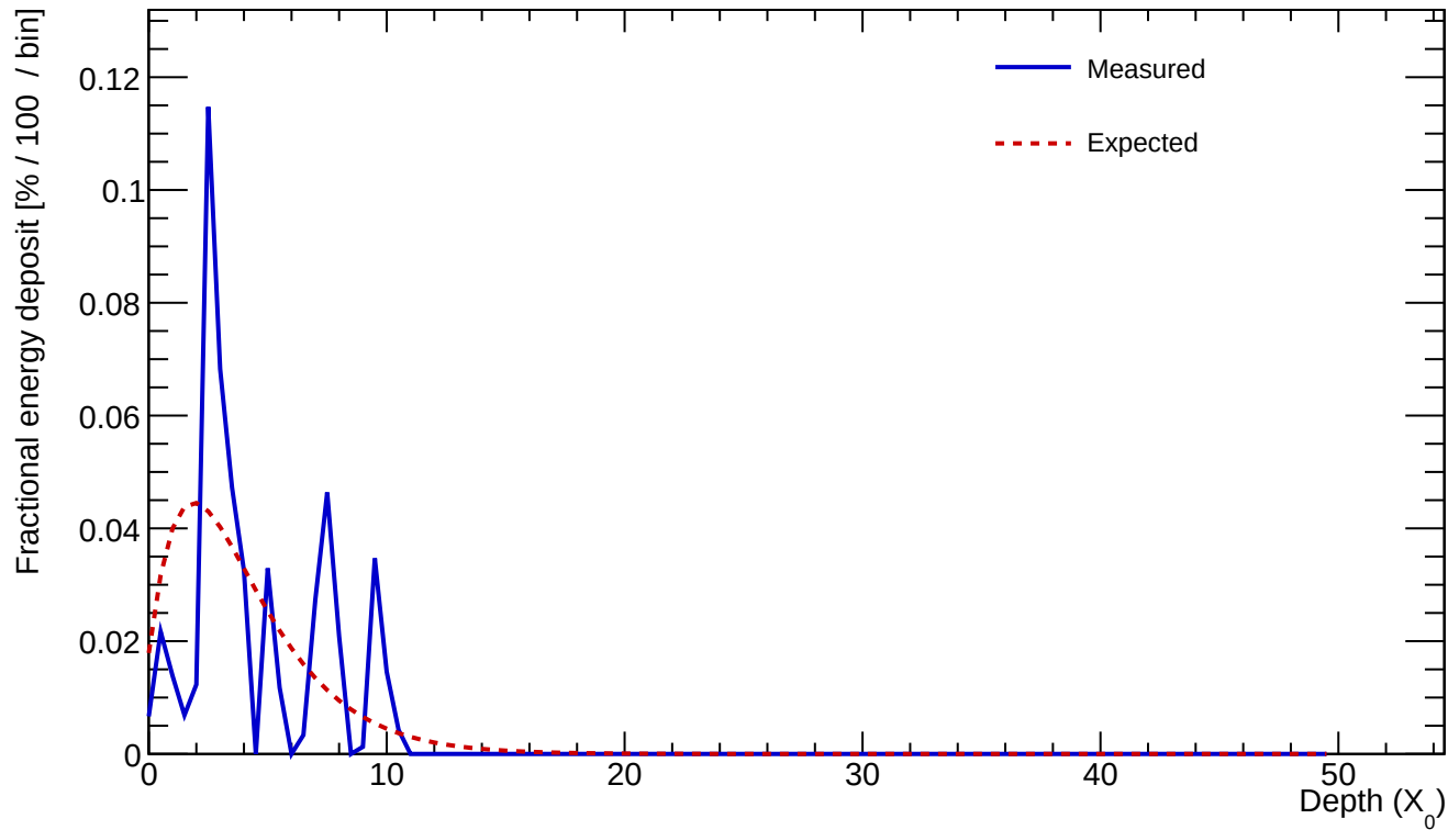
Cluster 72 E=0.522 GeV profileStart=1.00 X_0 \chi=0.7482
