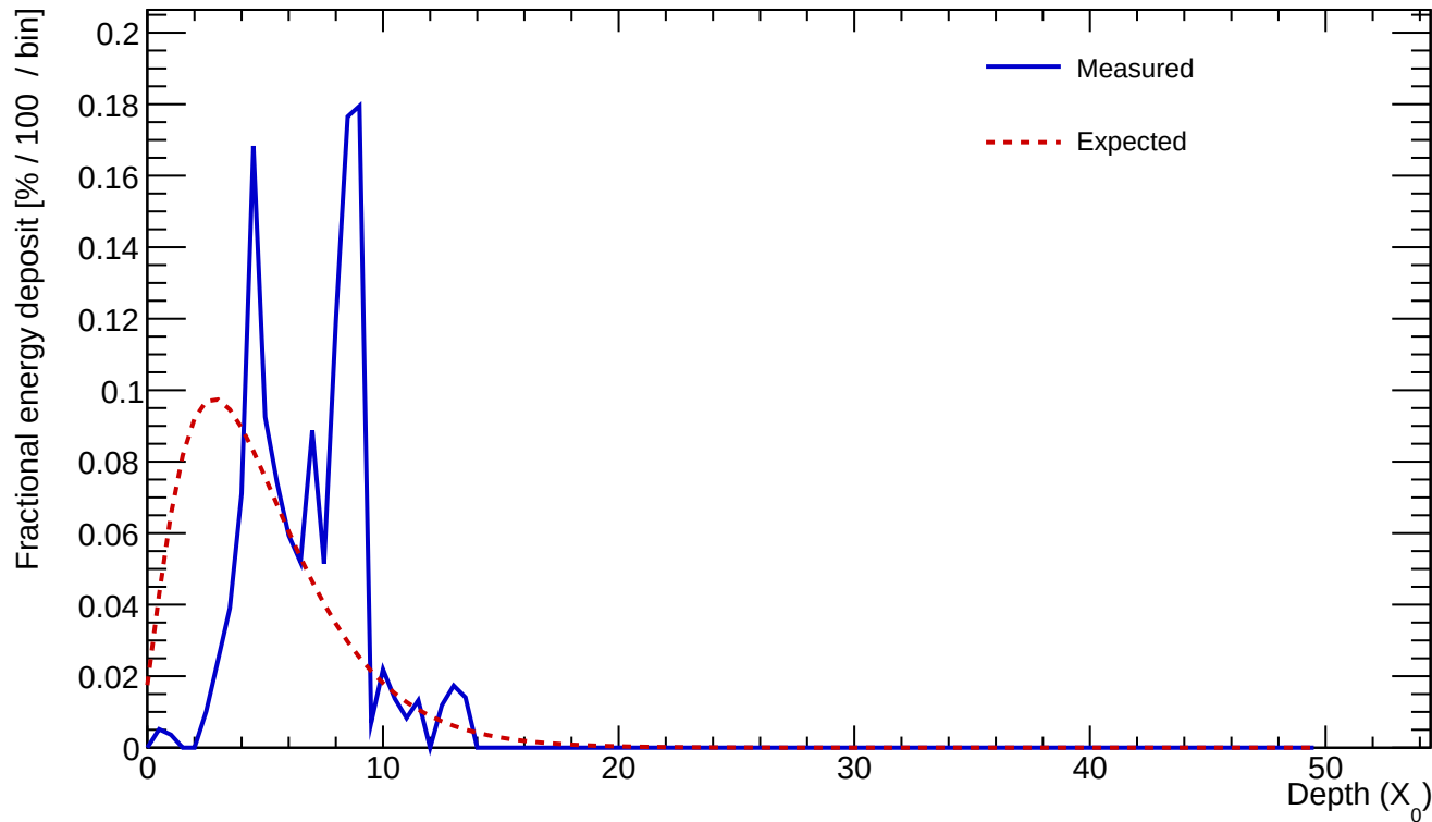
Cluster 77 E=1.323 GeV profileStart=3.00 X_0 \chi=0.5328
