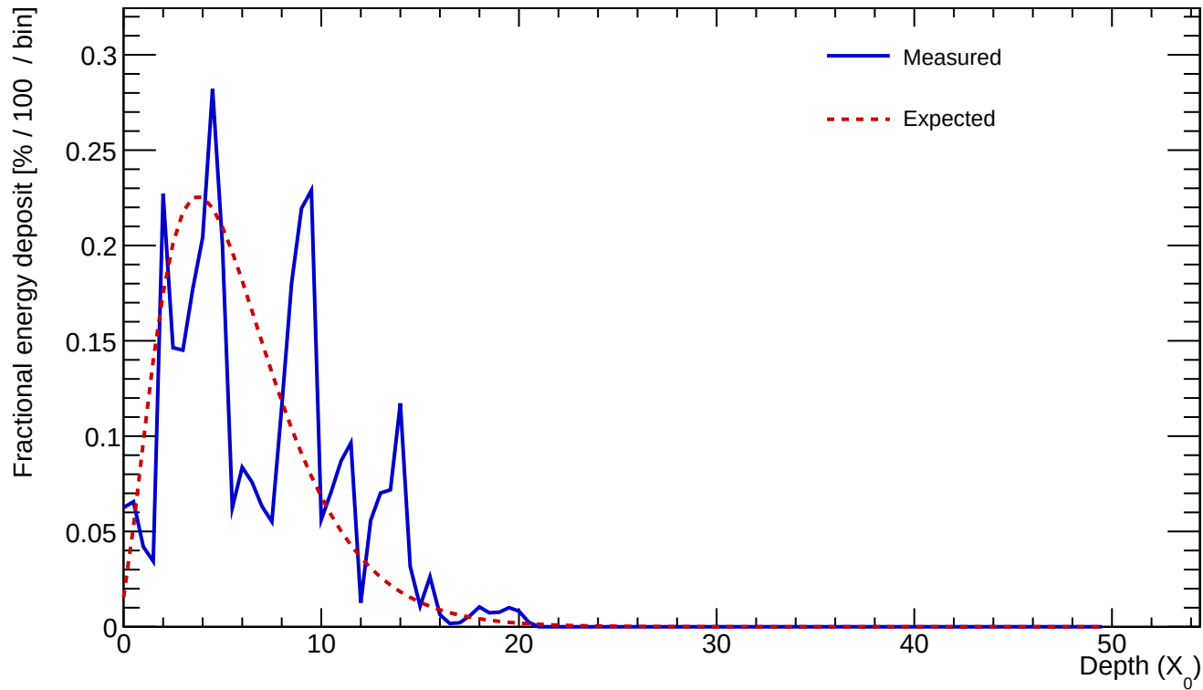
Cluster 39 E=3.440 GeV profileStart=1.00 X_0 \chi=0.5198
