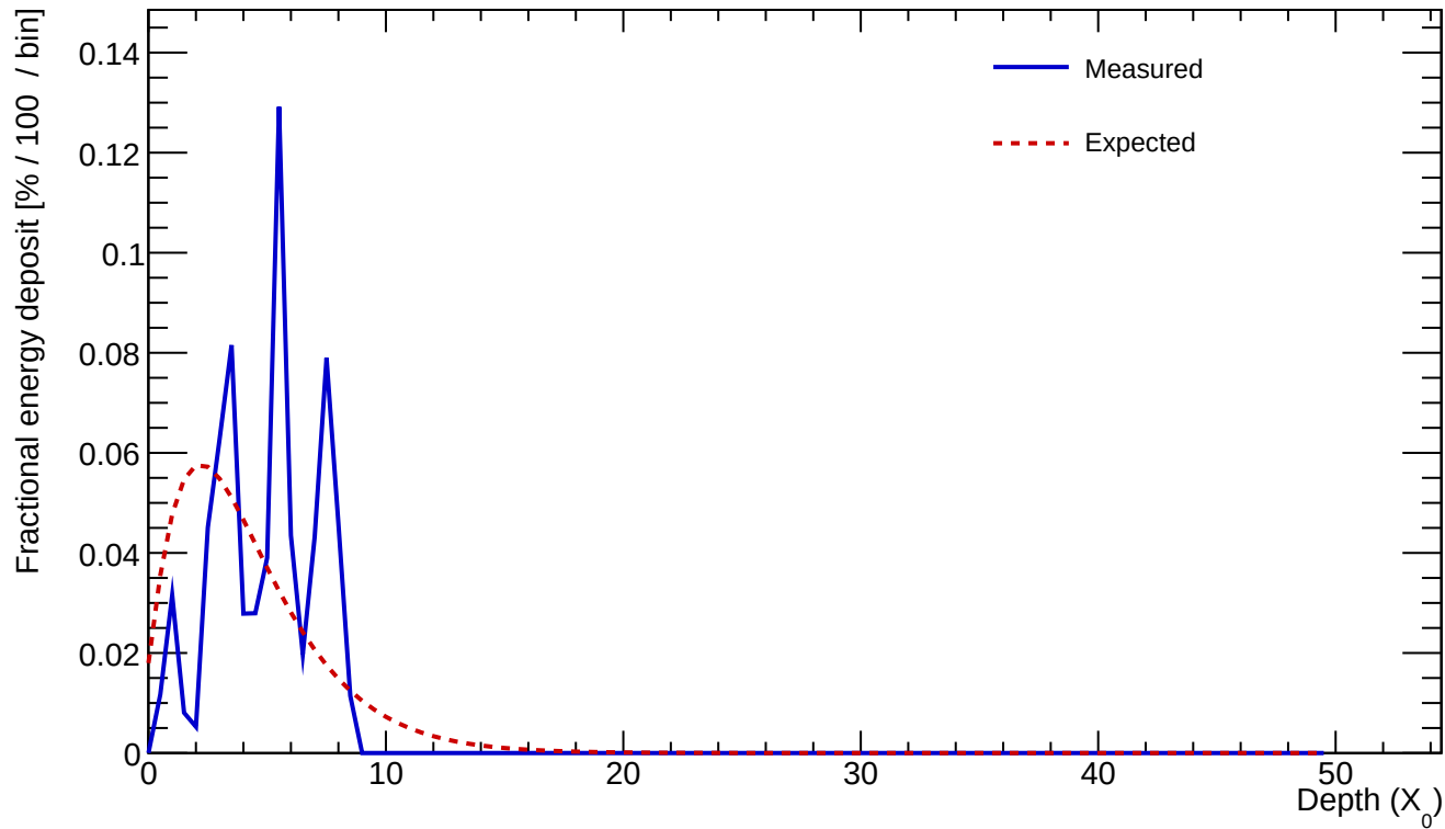
Cluster 30 E=0.713 GeV profileStart=2.00 X_0 \chi=0.5106
