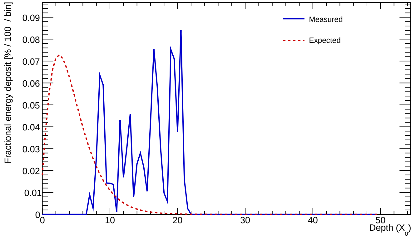
Cluster 953 E=0.939 GeV profileStart=7.50 X_0 \chi=0.8989
