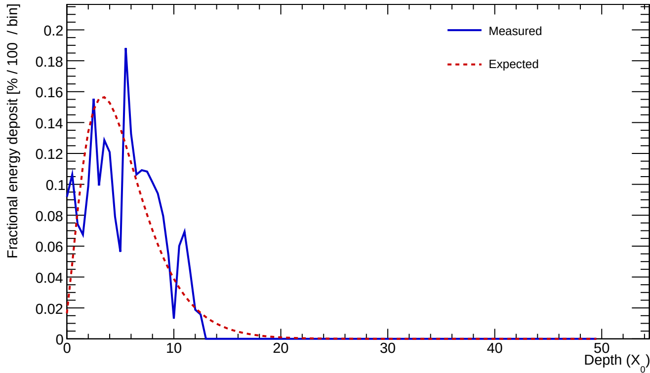
Cluster 761 E=2.274 GeV profileStart=0.50 X_0 \chi=0.3511
