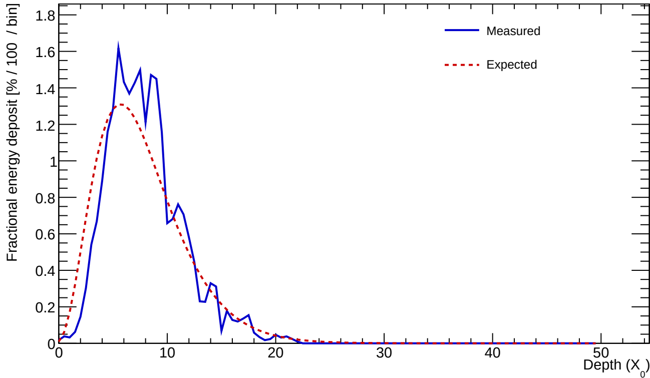
Cluster 1157 E=23.774 GeV profileStart=1.00 X_0 \chi=0.1759
