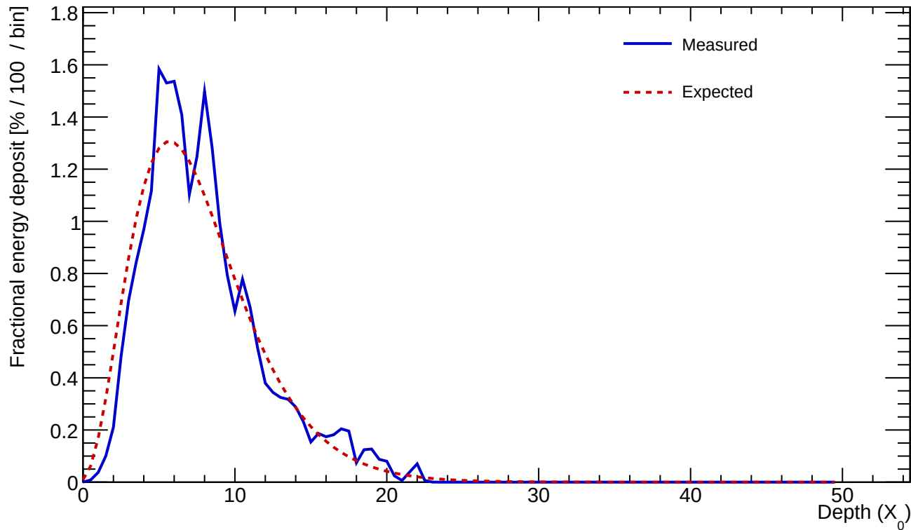
Cluster 778 E=23.679 GeV profileStart=0.50 X_0 \chi=0.1550
