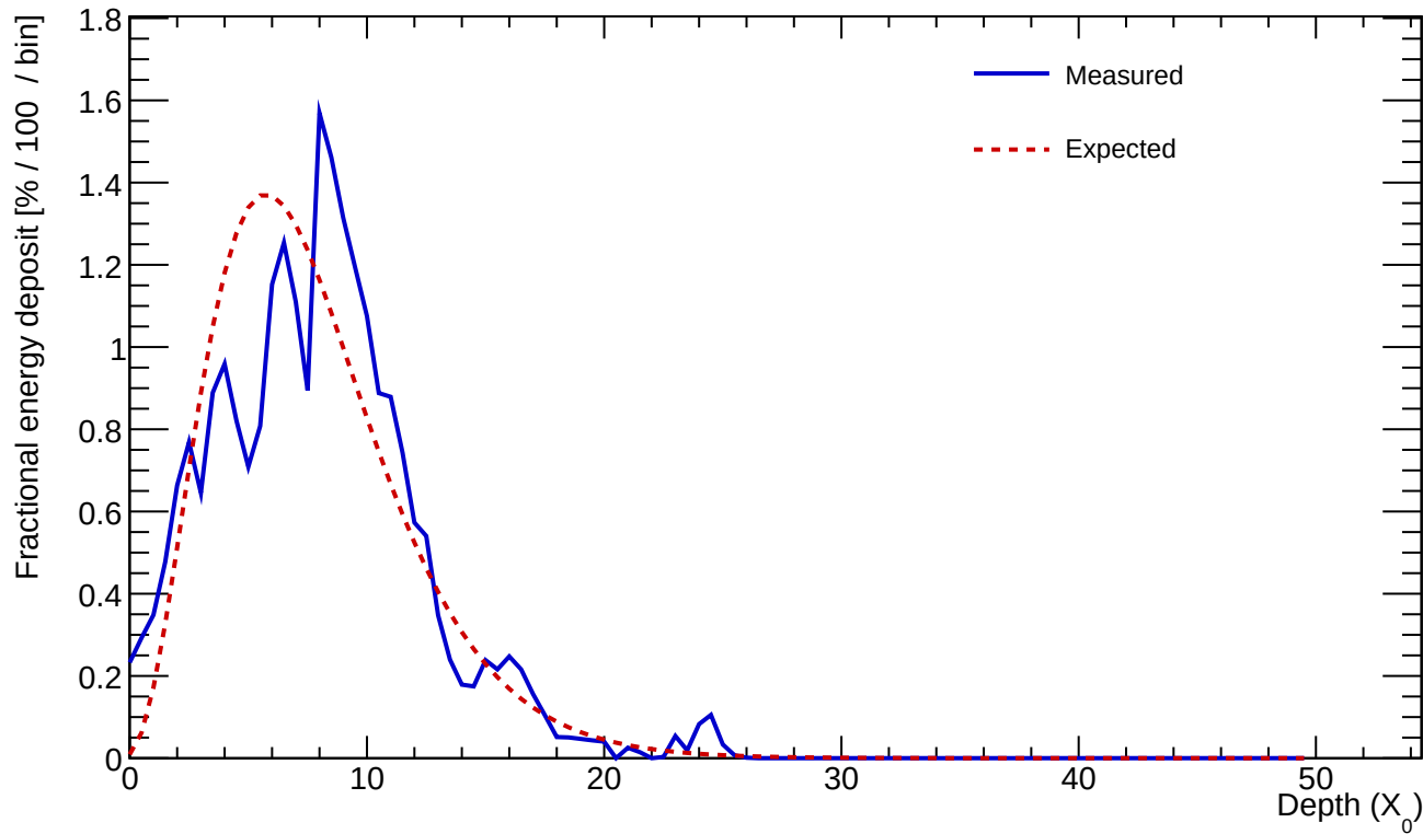
Cluster 100 E=24.960 GeV profileStart=0.50 X_0 \chi=0.2829
