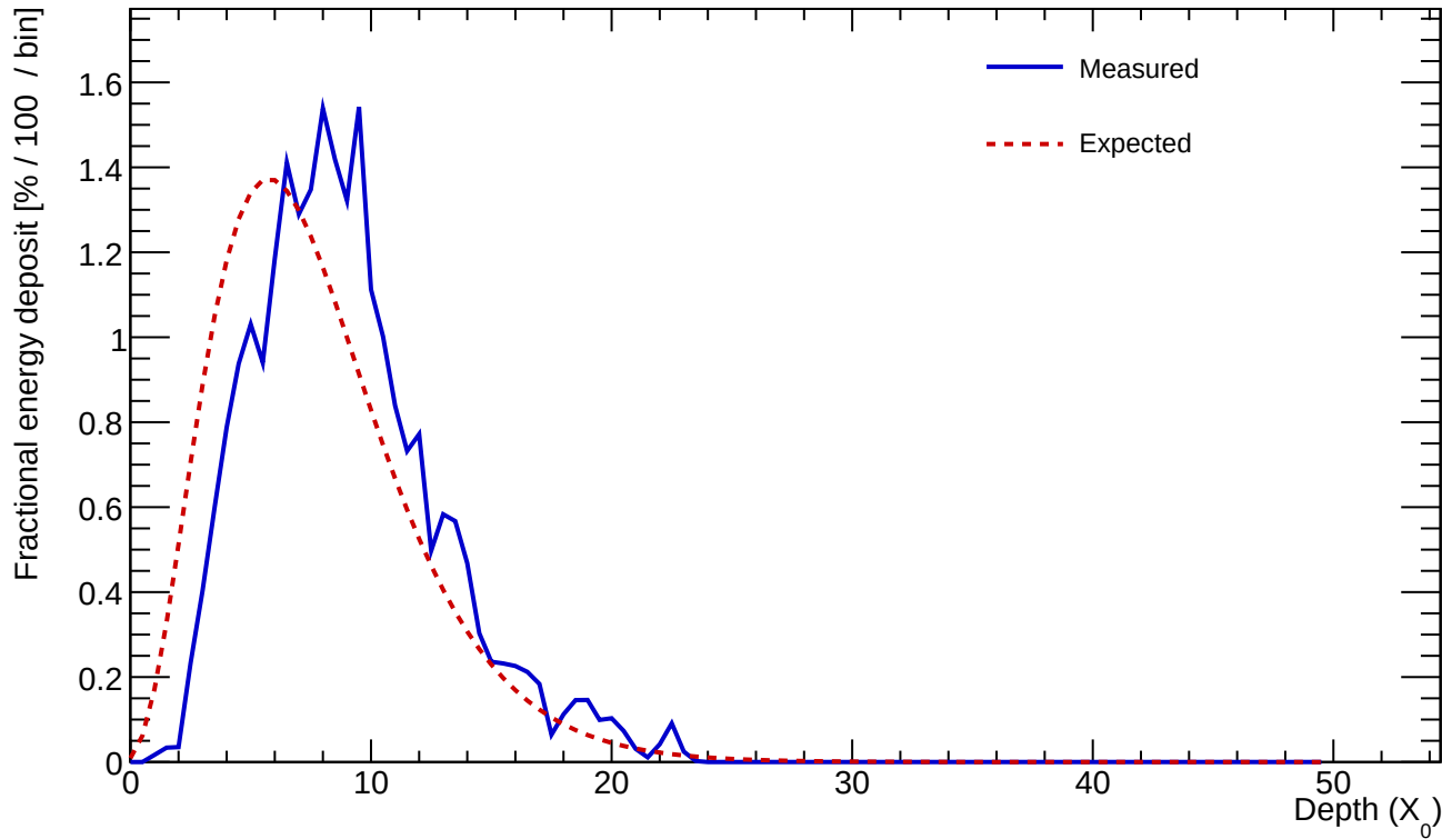
Cluster 832 E=24.986 GeV profileStart=1.50 X_0 \chi=0.1168
