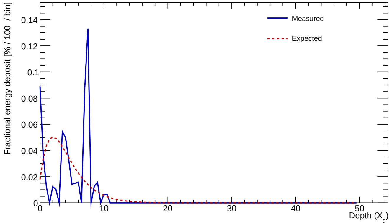
Cluster 1171 E=0.604 GeV profileStart=2.00 X_0 \chi=0.9333
