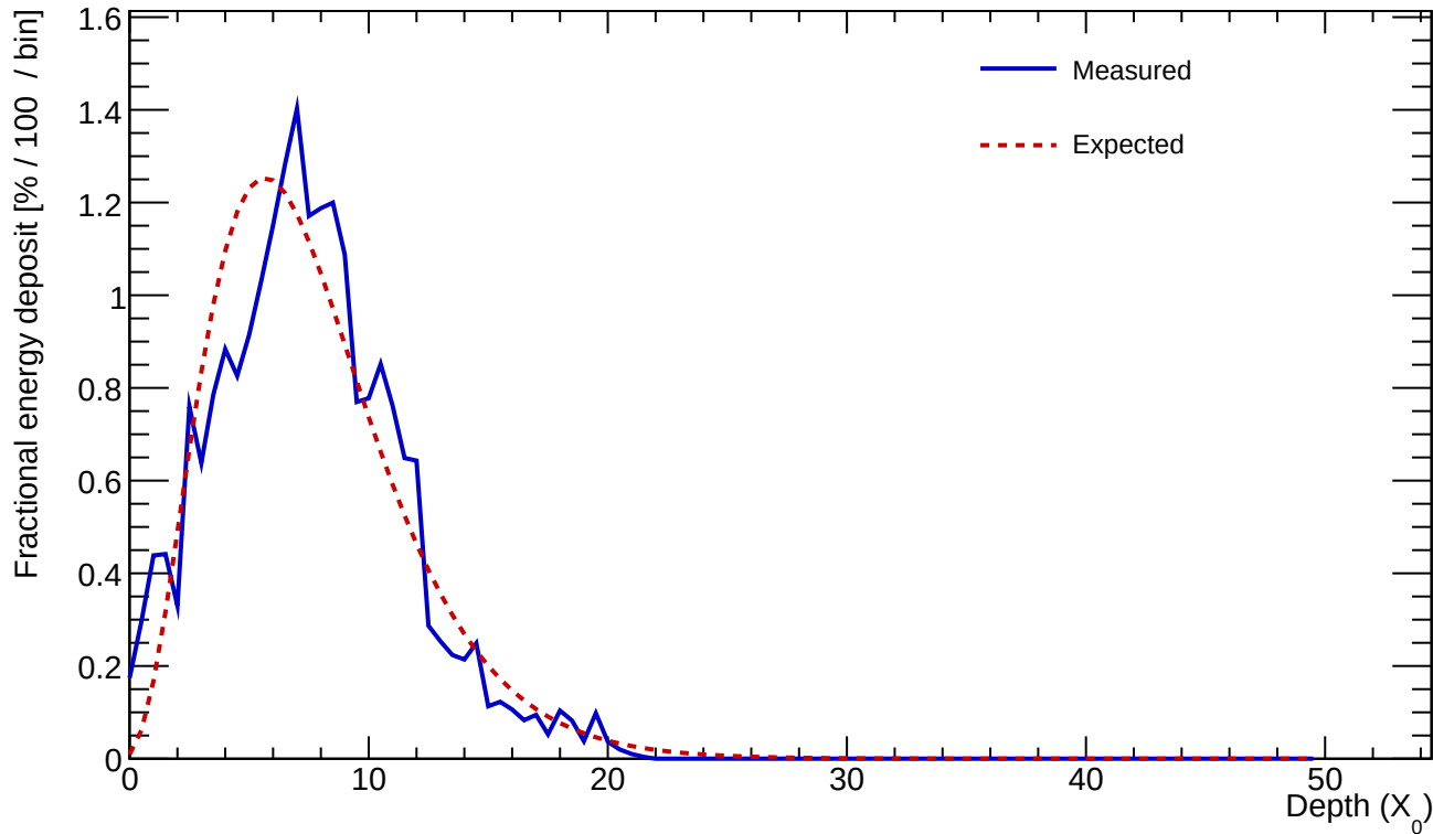
Cluster 456 E=22.646 GeV profileStart=0.50 X_0 \chi=0.2054
