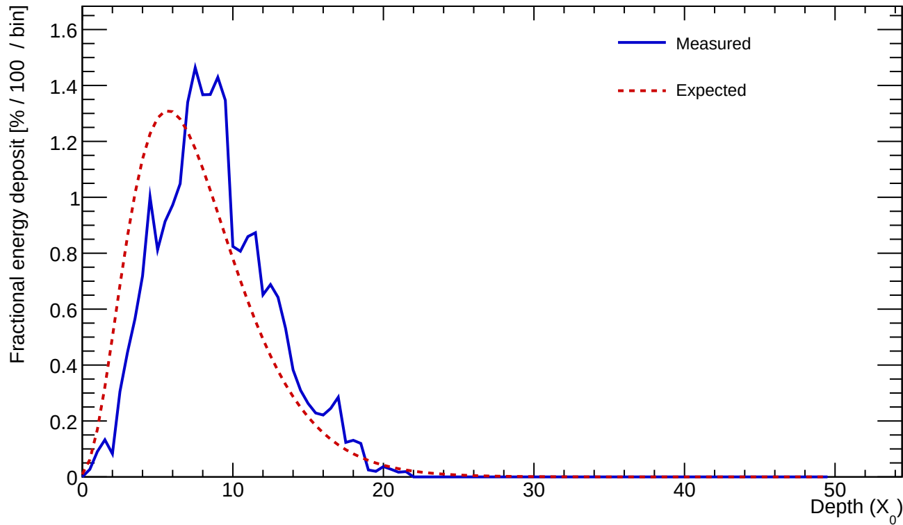
Cluster 725 E=23.760 GeV profileStart=1.50 X_0 \chi=0.1654
