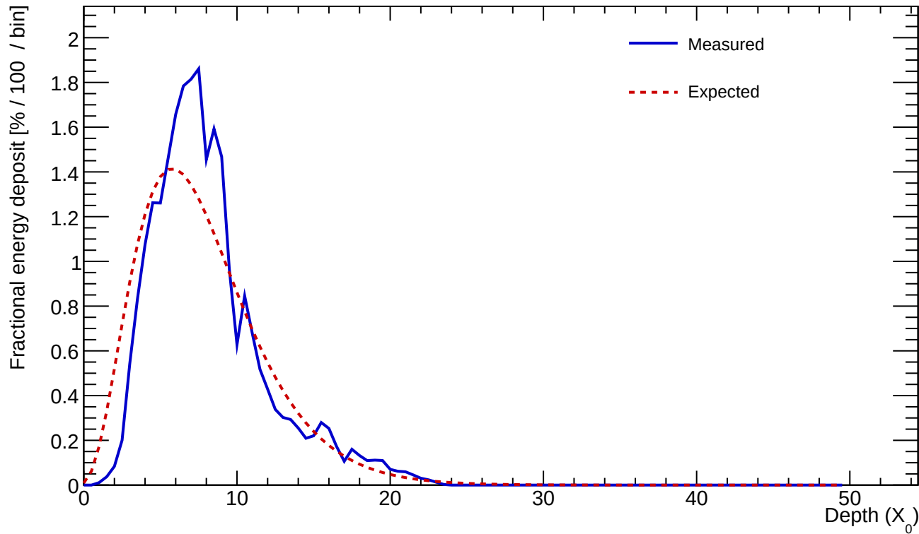
Cluster 934 E=25.816 GeV profileStart=0.50 X_0 \chi=0.2206
