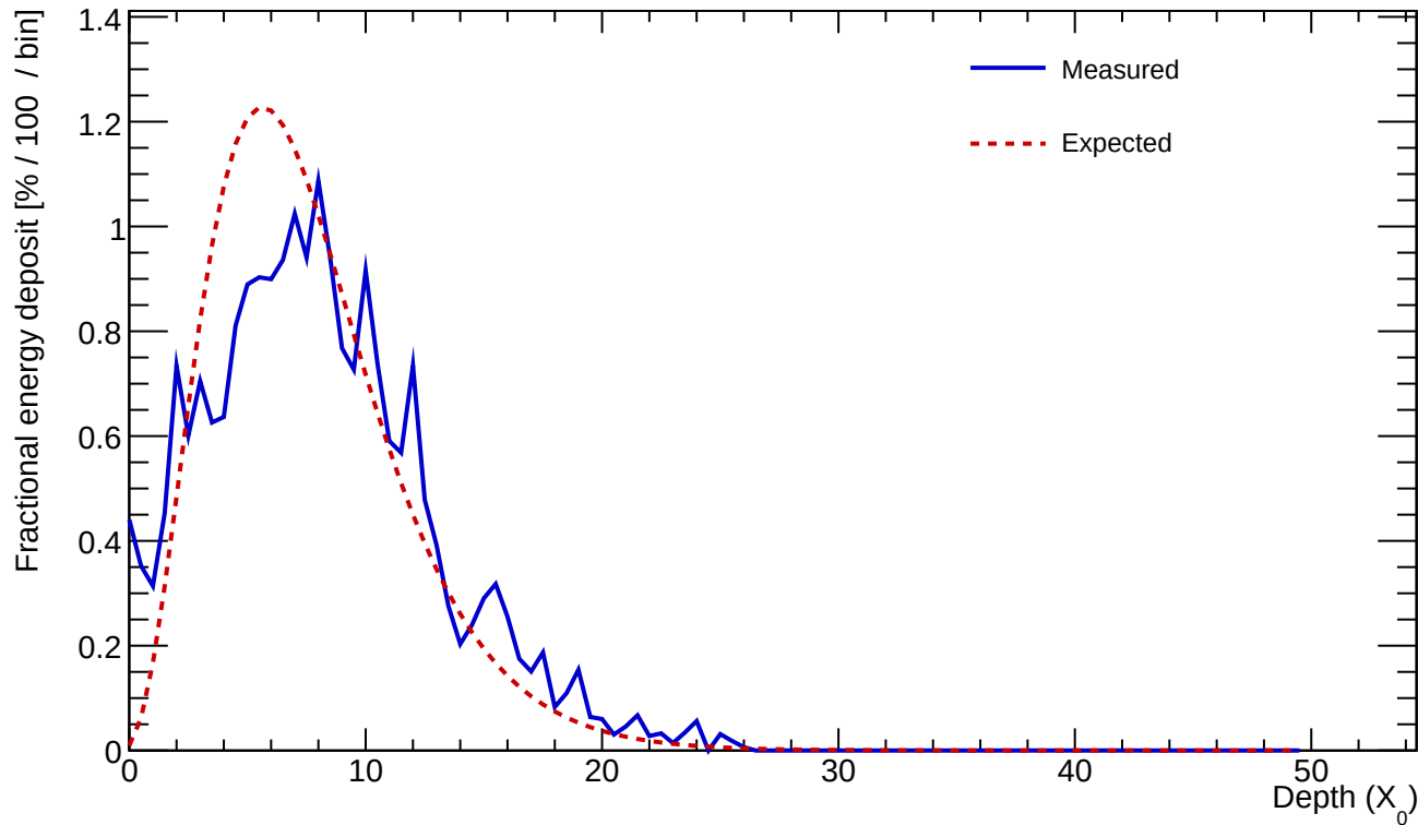
Cluster 120 E=22.137 GeV profileStart=0.50 X_0 \chi=0.2750
