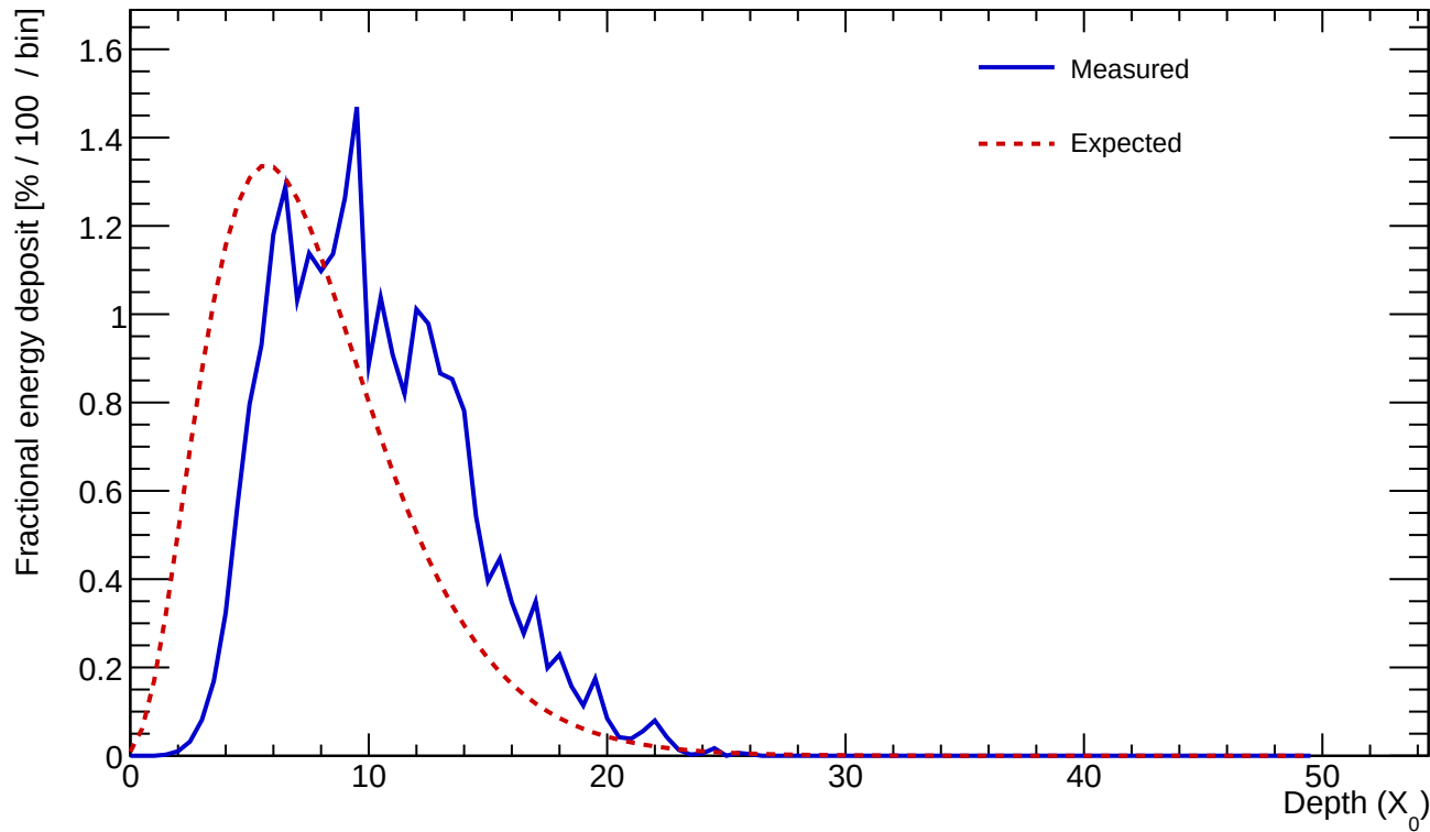
Cluster 385 E=24.286 GeV profileStart=2.50 X_0 \chi=0.1580
