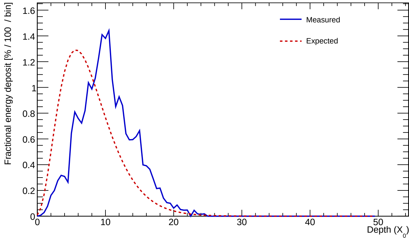
Cluster 414 E=23.379 GeV profileStart=3.00 X_0 \chi=0.1974
