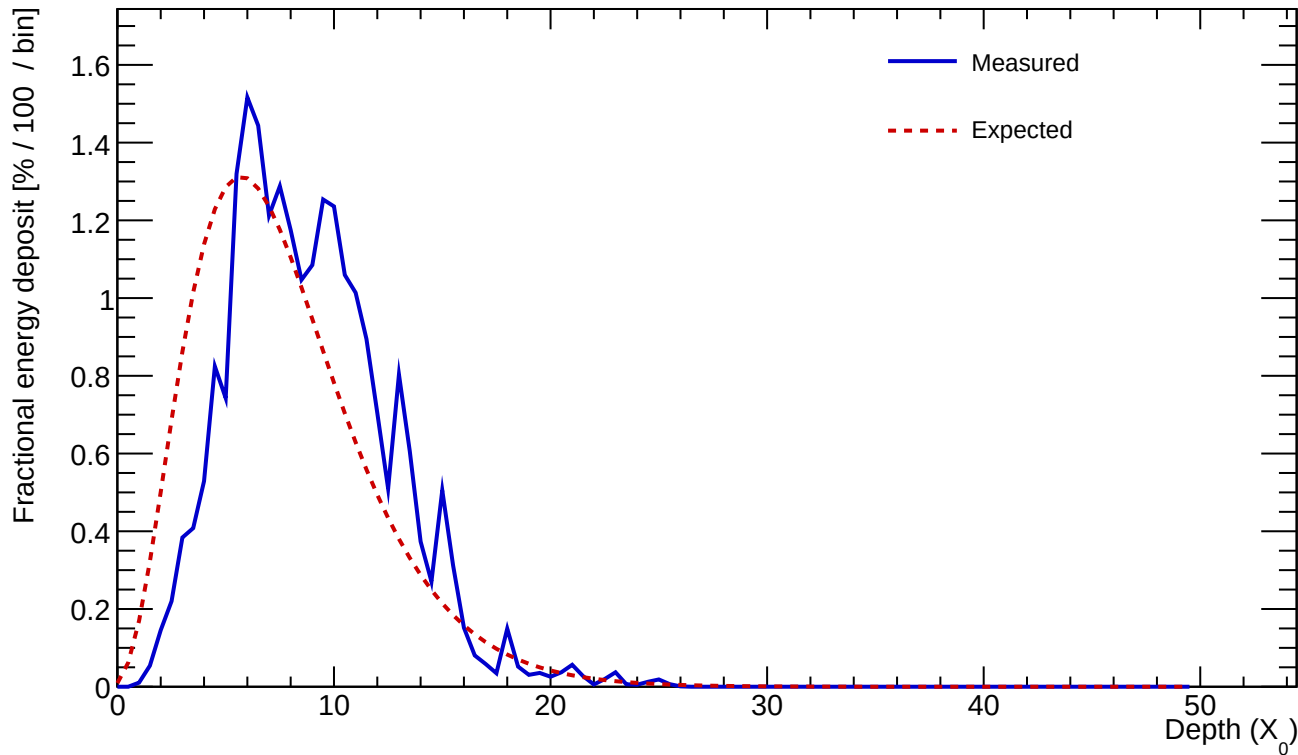
Cluster 353 E=23.802 GeV profileStart=1.50 X_0 \chi=0.1837
