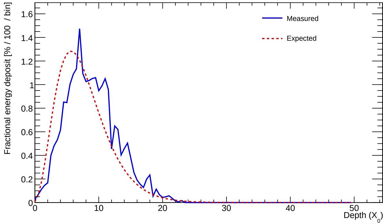
Cluster 889 E=23.241 GeV profileStart=1.50 X_0 \chi=0.1730
