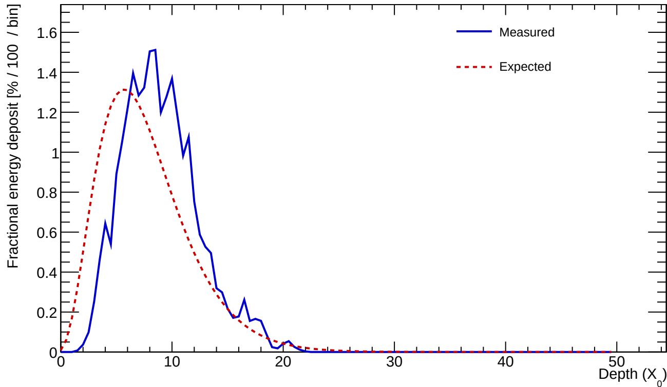
Cluster 837 E=23.847 GeV profileStart=1.50 X_0 \chi=0.1509
