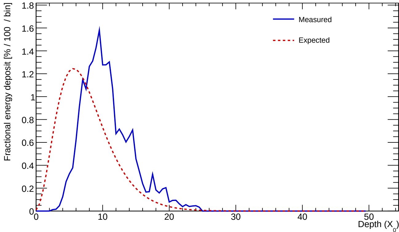
Cluster 514 E=22.469 GeV profileStart=3.50 X_0 \chi=0.1617
