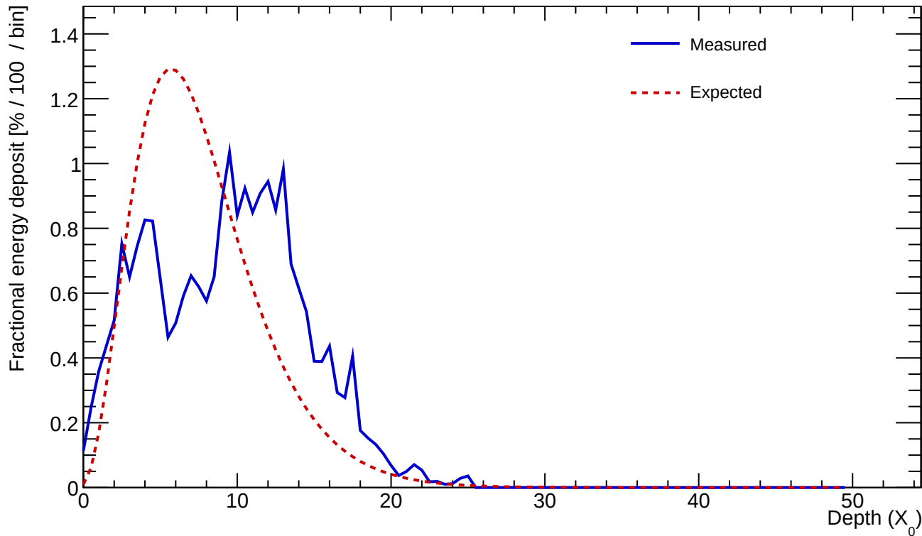
Cluster 403 E=23.407 GeV \text{profileStart}=2.50 X_0 \chi=0.4667
