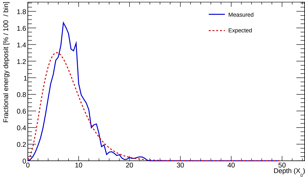
Cluster 348 E=23.636 GeV profileStart=1.00 X_0 \chi=0.1716
