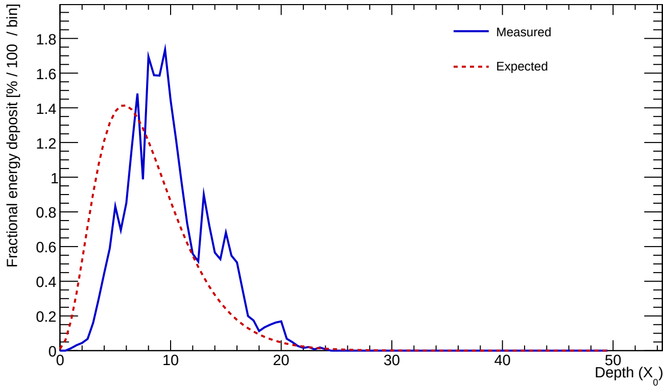
Cluster 787 E=25.830 GeV profileStart=2.50 X_0 \chi=0.2098
