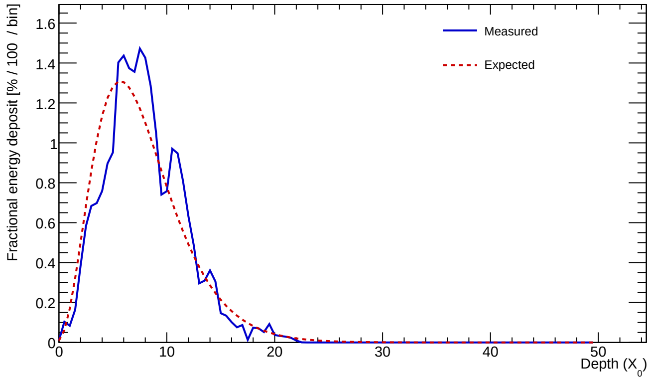
Cluster 117 E=23.720 GeV profileStart=0.50 X_0 \chi=0.1770
