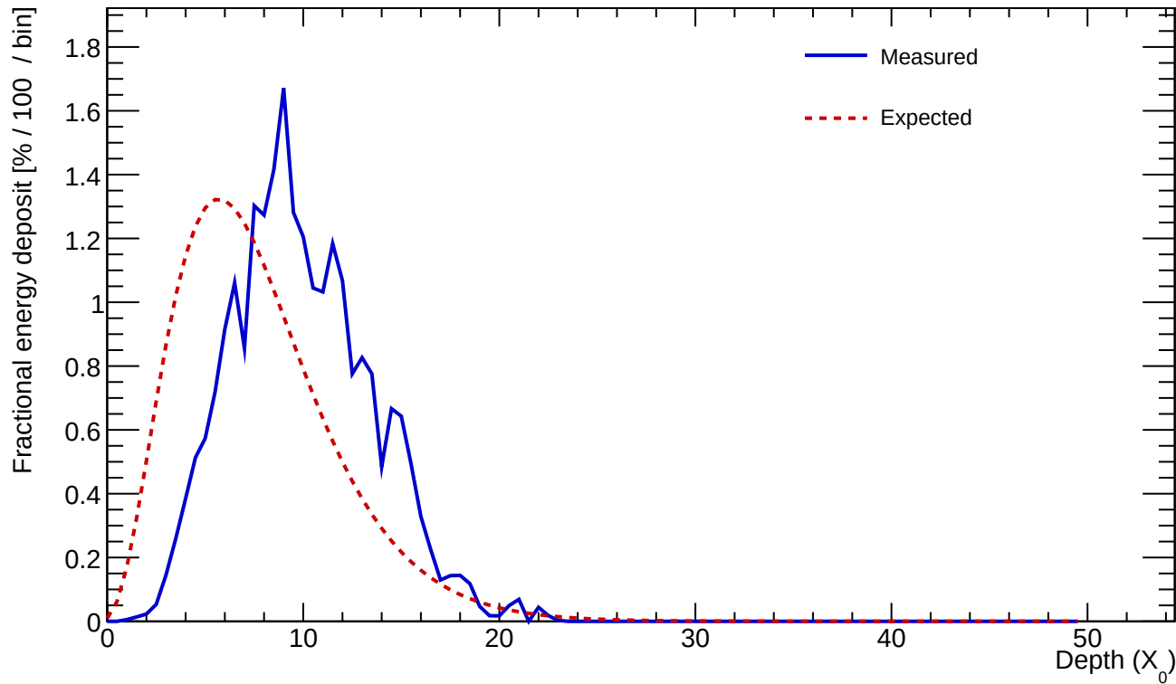
Cluster 822 E=24.016 GeV profileStart=2.50 X_0 \chi=0.1595
