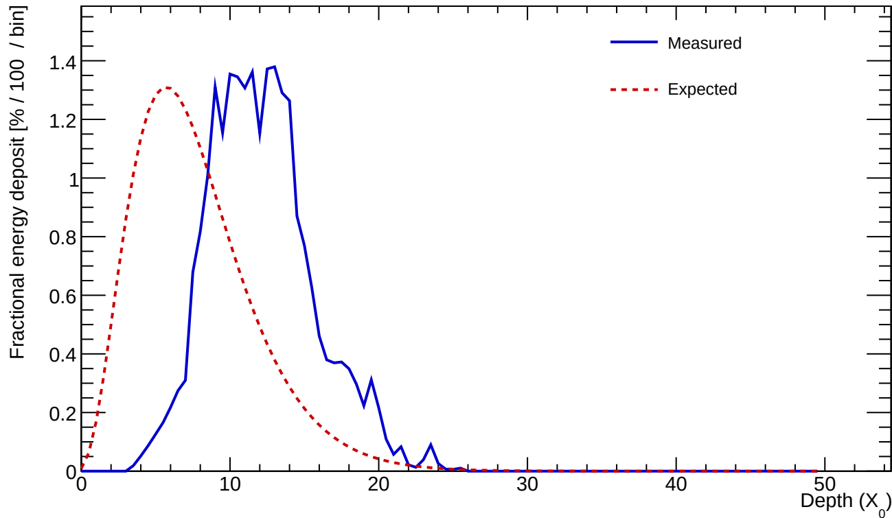
Cluster 174 E=23.759 GeV \text{profileStart}=5.00 X_0 \chi=0.1555
