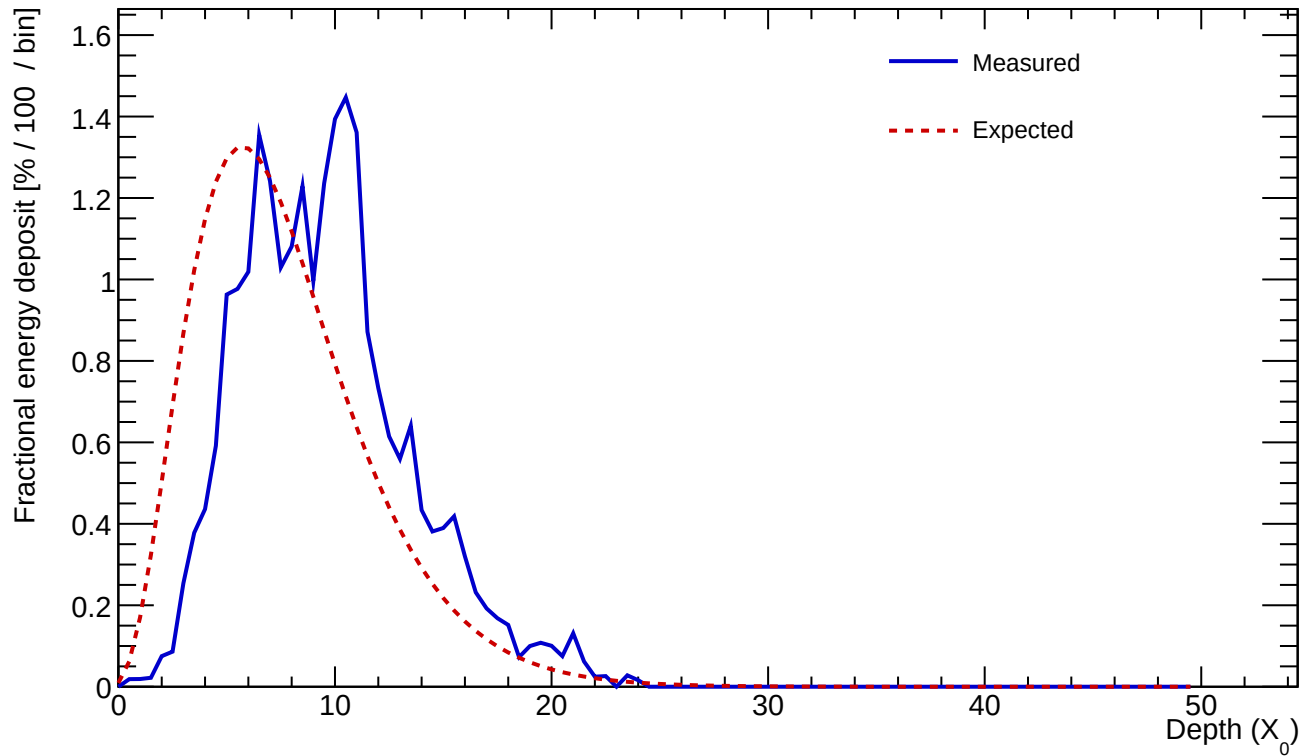
Cluster 760 E=24.060 GeV profileStart=2.00 X_0 \chi=0.1565
