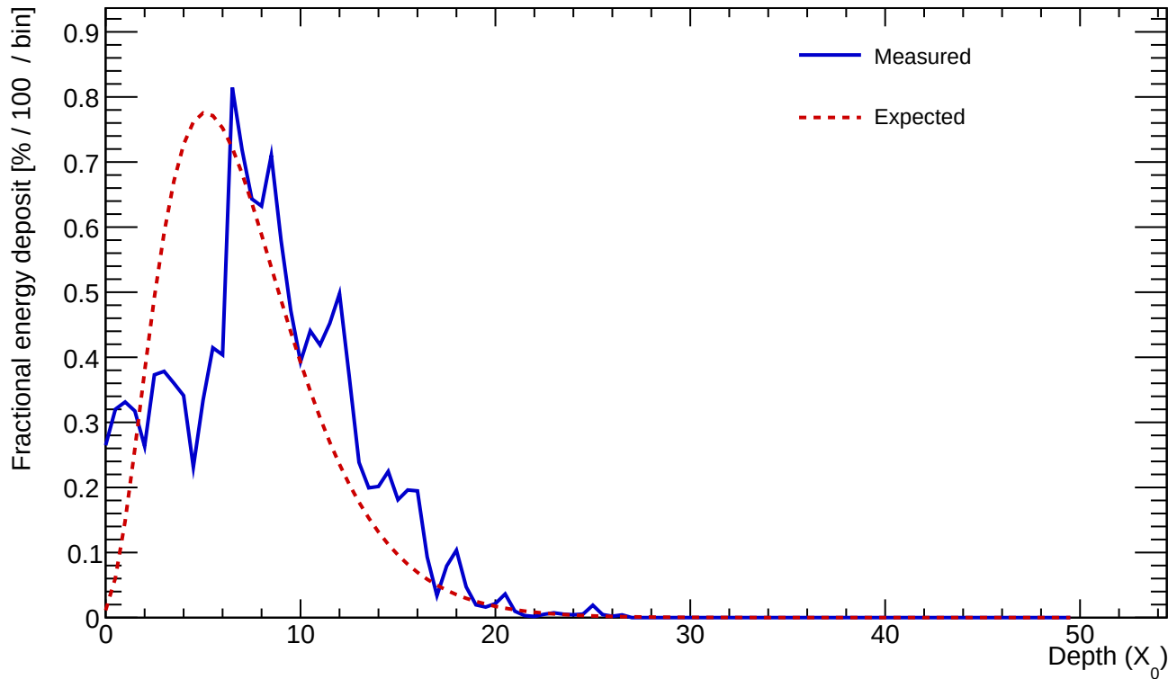
Cluster 314 E=13.436 GeV profileStart=1.00 X_0 \chi=0.3543
