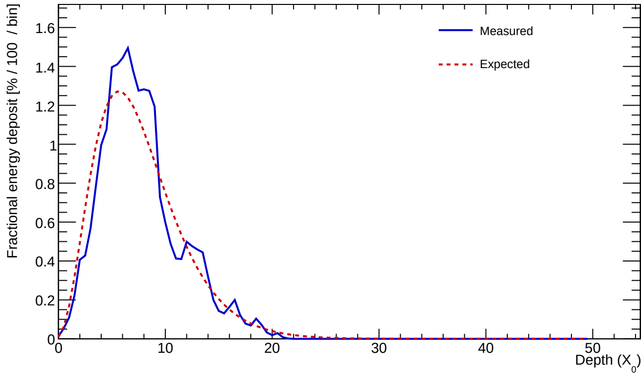
Cluster 443 E=23.008 GeV profileStart=0.50 X_0 \chi=0.1669
