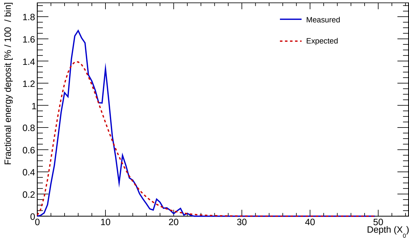
Cluster 688 E=25.411 GeV profileStart=0.50 X_0 \chi=0.1412
