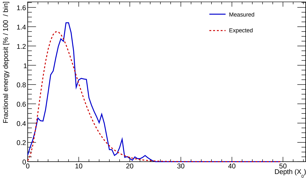
Cluster 582 E=24.528 GeV profileStart=1.00 X_0 \chi=0.1782
