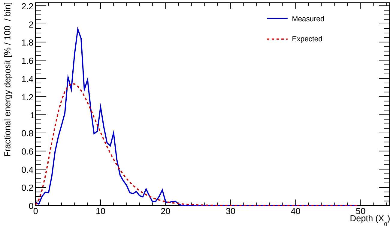
Cluster 922 E=24.385 GeV profileStart=0.50 X_0 \chi=0.2064
