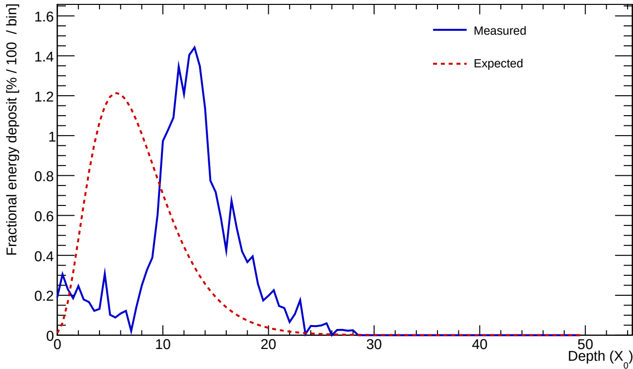
Cluster 1119 E=21.875 GeV profileStart=6.50 X_0 \chi=0.3098
