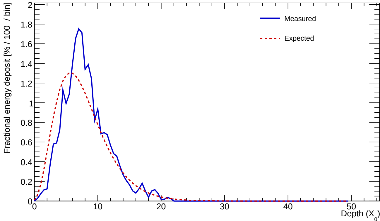
Cluster 850 E=23.630 GeV profileStart=1.00 X_0 \chi=0.1875
