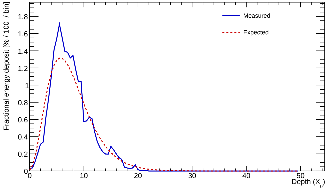
Cluster 944 E=23.855 GeV profileStart=0.50 X_0 \chi=0.1741
