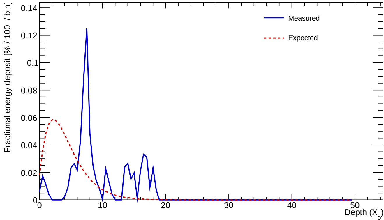
Cluster 1109 E=0.724 GeV profileStart=4.50 X_0 \chi=0.8132
