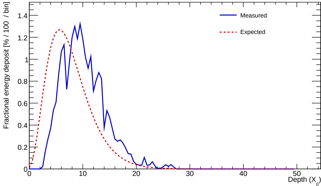
Cluster 446 E=22.940 GeV profileStart=2.50 X_0 \chi=0.1411
