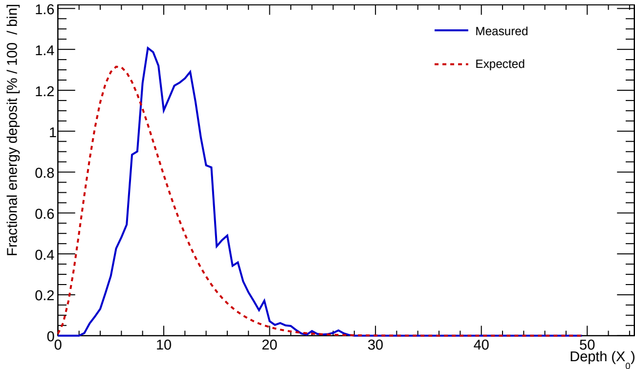
Cluster 124 E=23.887 GeV profileStart=4.00 X_0 \chi=0.1636
