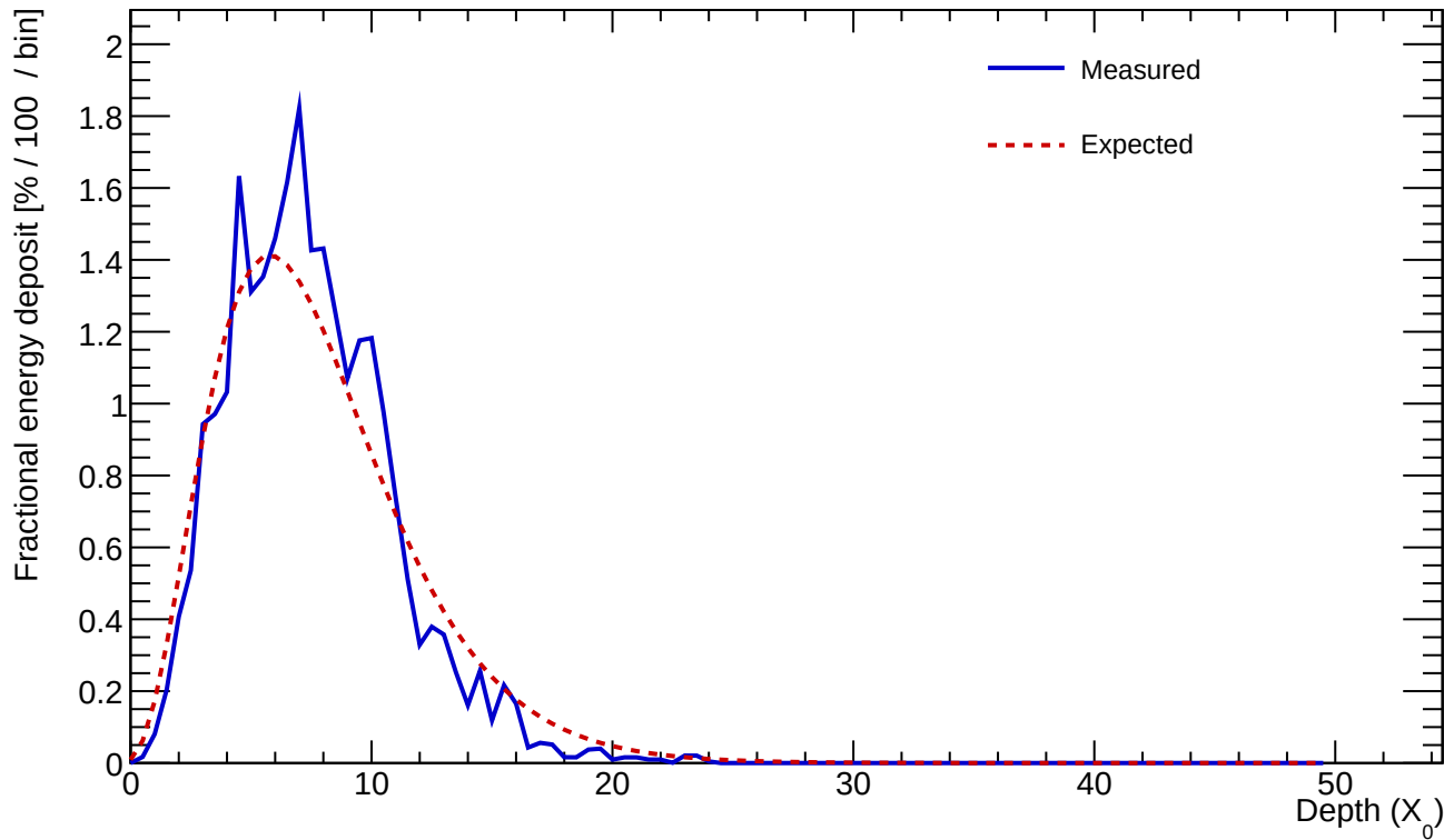
Cluster 428 E=25.758 GeV profileStart=0.50 X_0 \chi=0.1798
