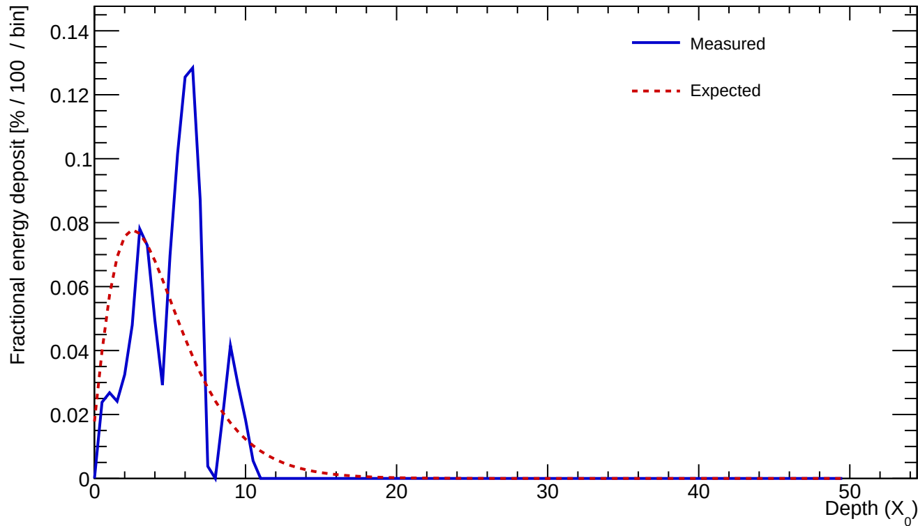
Cluster 1128 E=1.015 GeV profileStart=1.50 X_0 \chi=0.4753
