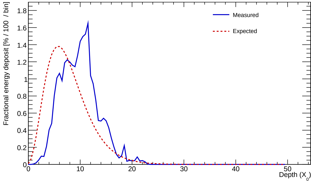
Cluster 804 E=25.151 GeV profileStart=2.50 X_0 \chi=0.1886
