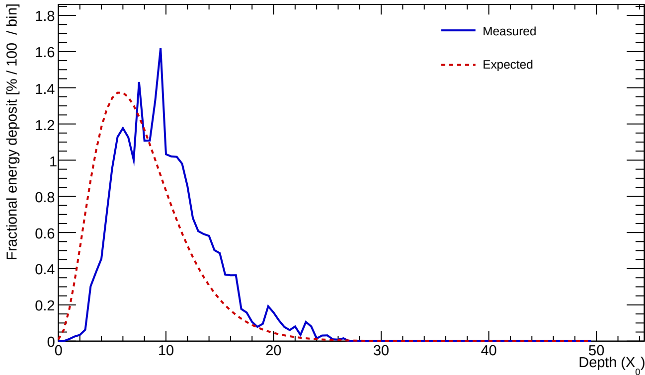
Cluster 967 E=25.043 GeV profileStart=2.00 X_0 \chi=0.1347
