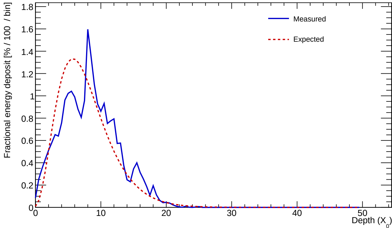
Cluster 215 E=24.184 GeV \text{profileStart}=1.00 X_0 \chi=0.2540
