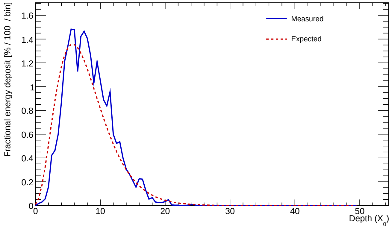
Cluster 602 E=24.669 GeV profileStart=1.00 X_0 \chi=0.1363
