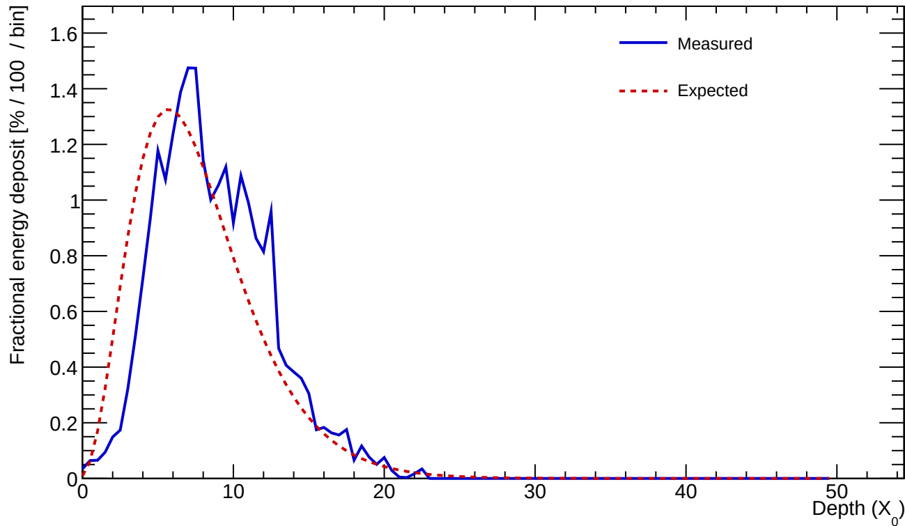
Cluster 329 E=24.087 GeV profileStart=1.50 X_0 \chi=0.1383
