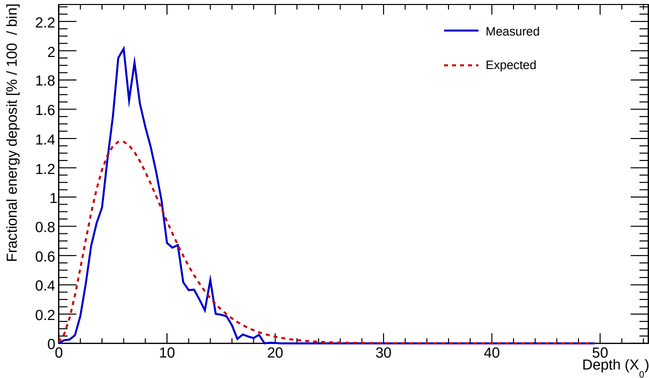
Cluster 142 E=25.136 GeV profileStart=0.50 X_0 \chi=0.2518
