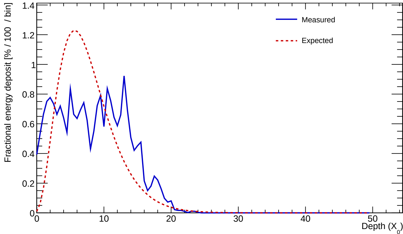
Cluster 148 E=22.162 GeV profileStart=1.00 X_0 \chi=0.5120
