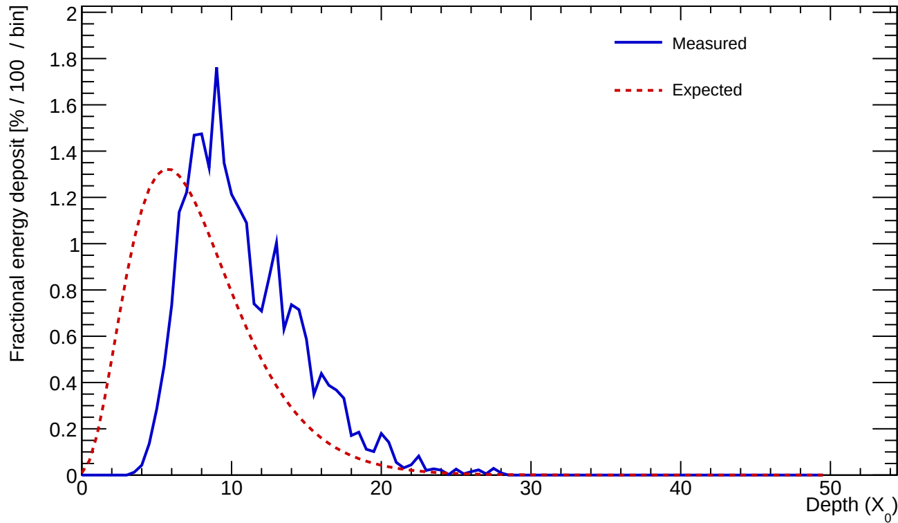
Cluster 335 E=24.015 GeV profileStart=3.50 X_0 \chi=0.1677
