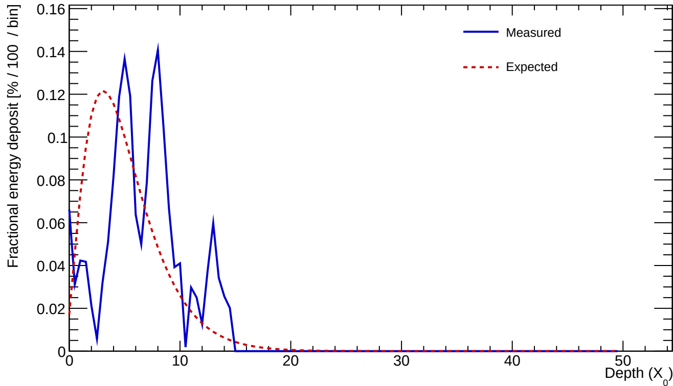
Cluster 1174 E=1.706 GeV profileStart=2.50 X_0 \chi=0.4405
