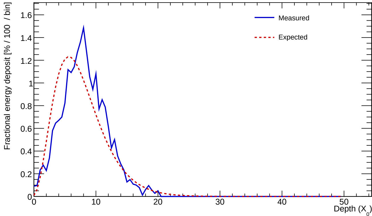
Cluster 598 E=22.195 GeV profileStart=1.00 X_0 \chi=0.1798
