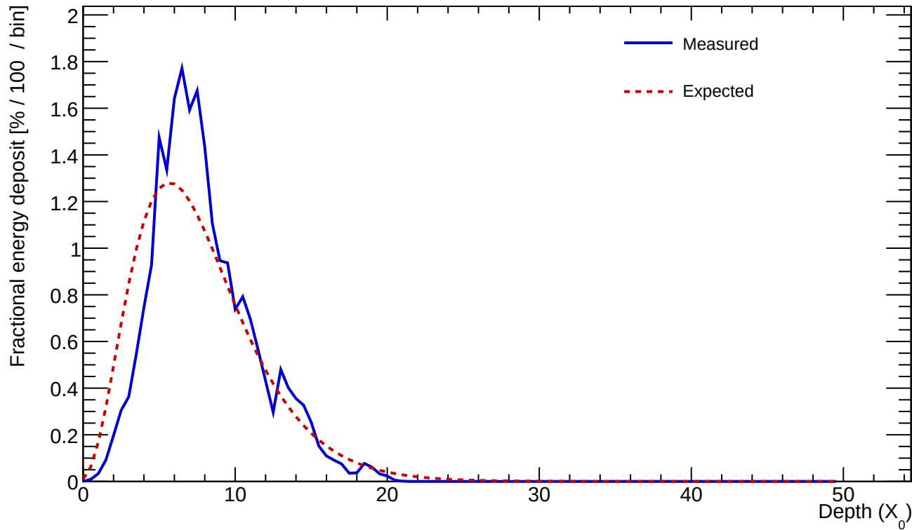
Cluster 20 E=23.171 GeV profileStart=1.00 X_0 \chi=0.2008
