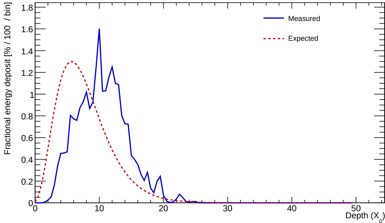
Cluster 820 E=23.576 GeV profileStart=3.00 X_0 \chi=0.2549
