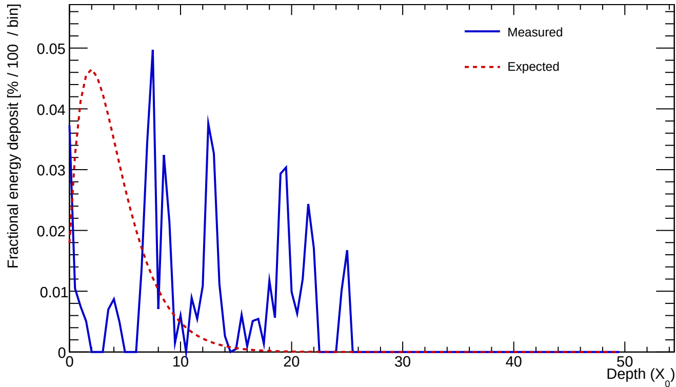
Cluster 1177 E=0.550 GeV \text{profileStart}=6.50 X_0 \chi=1.0117
