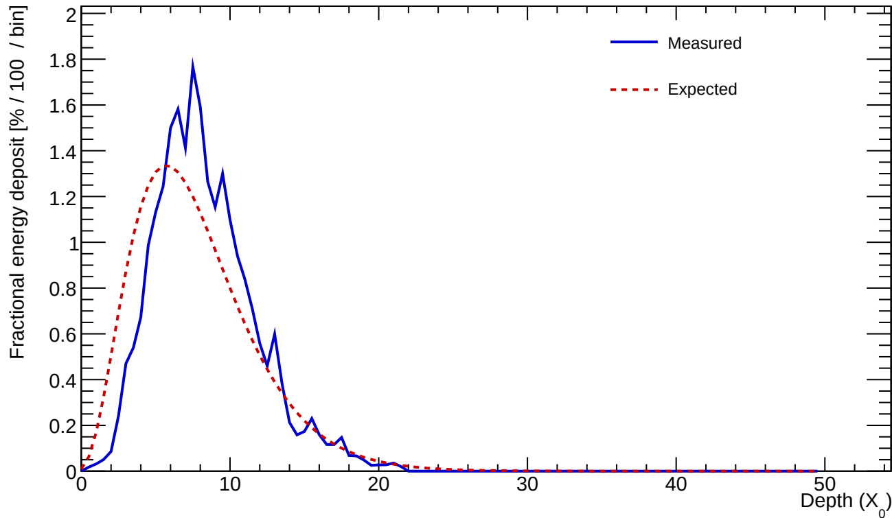
Cluster 662 E=24.260 GeV profileStart=1.00 X_0 \chi=0.1587
