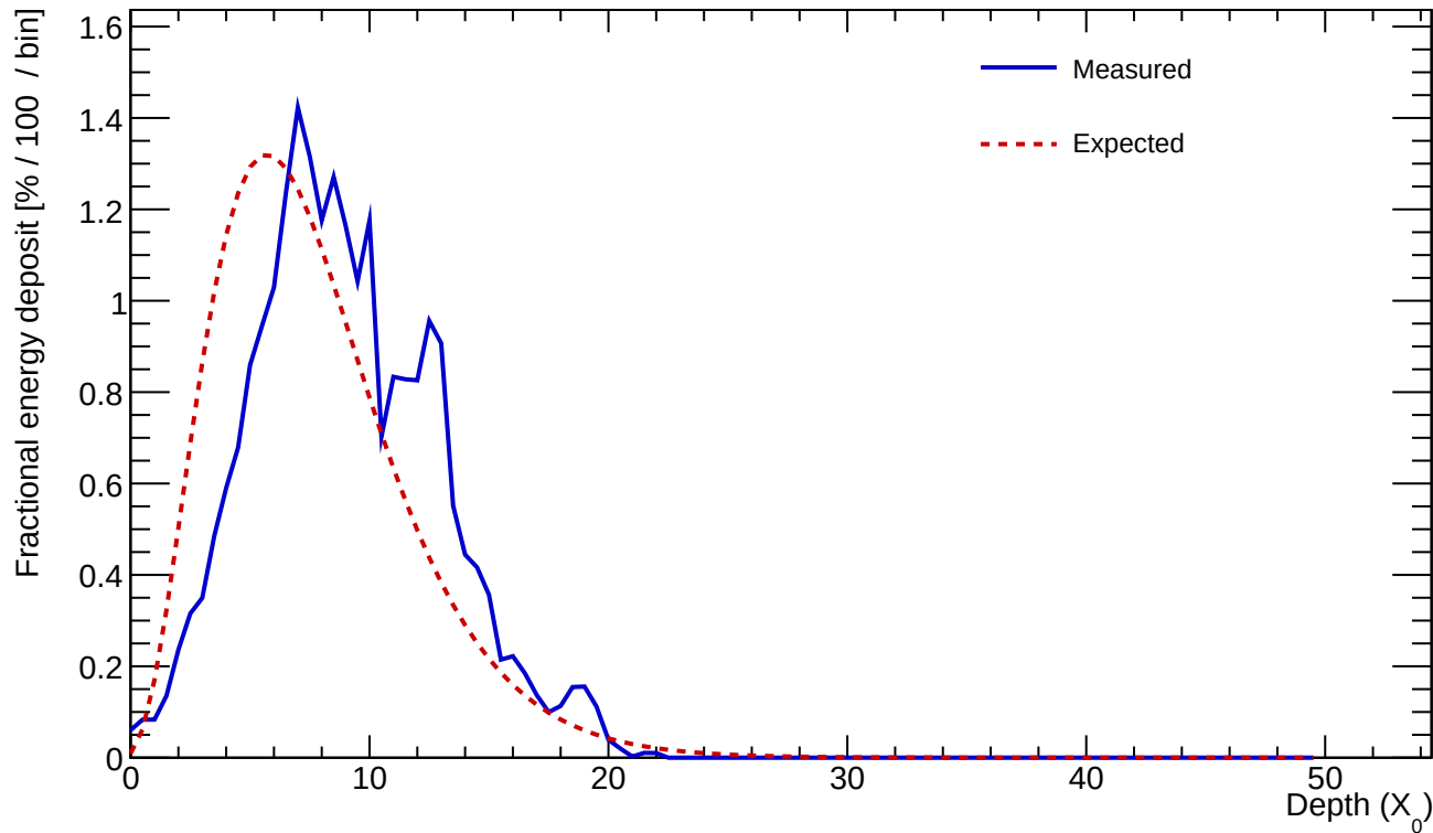
Cluster 221 E=23.953 GeV profileStart=1.50 X_0 \chi=0.1614
