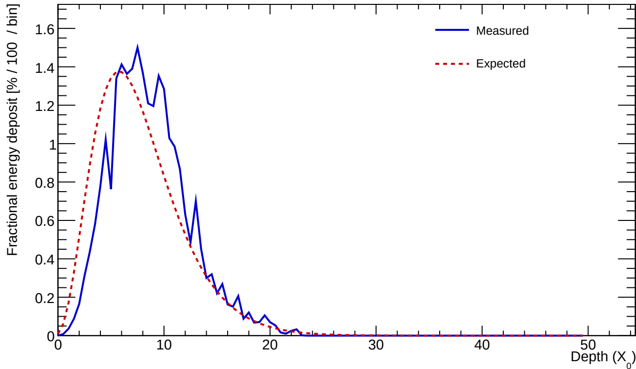
Cluster 273 E=25.045 GeV profileStart=1.00 X_0 \chi=0.1258
