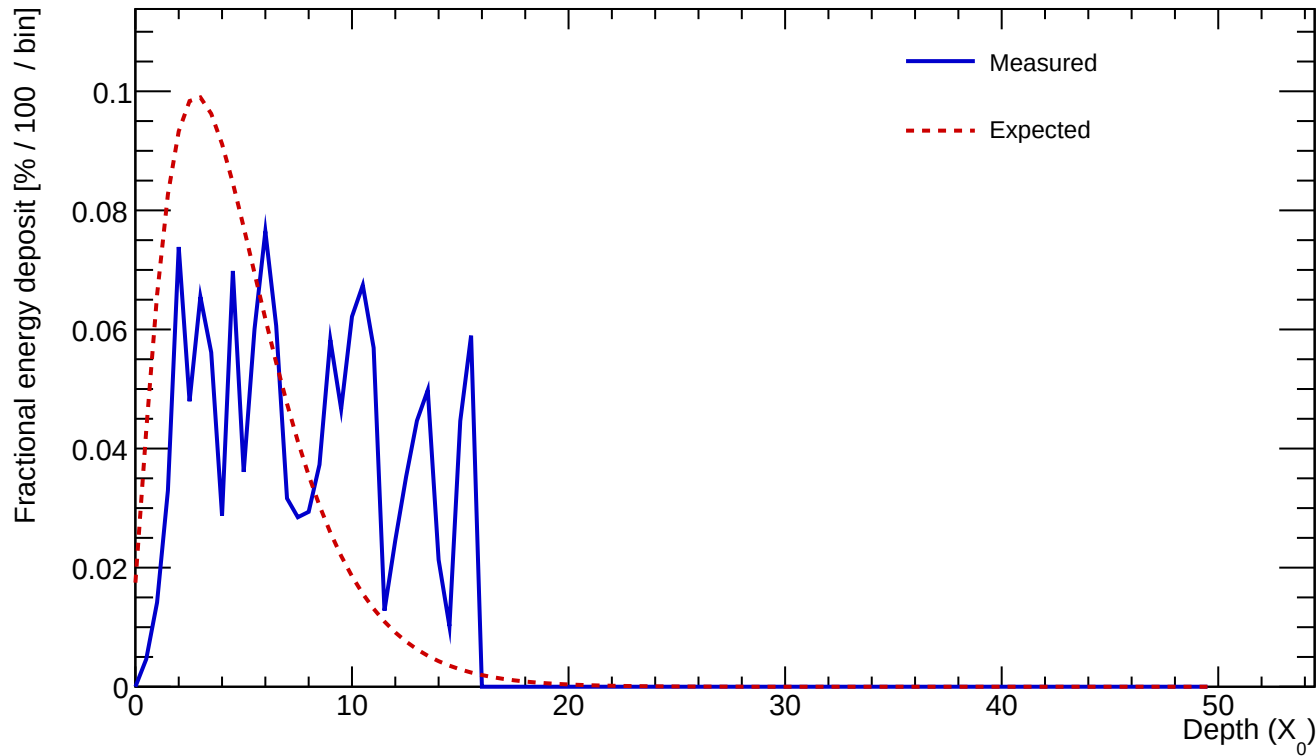
Cluster 1059 E=1.347 GeV profileStart=1.00 X_0 \chi=0.5423
