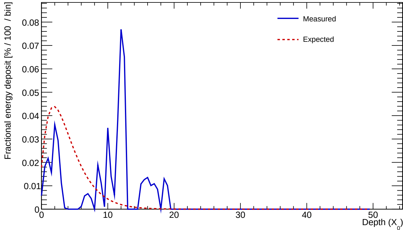
Cluster 253 E=0.512 GeV profileStart=0.50 X_0 \chi=1.2271
