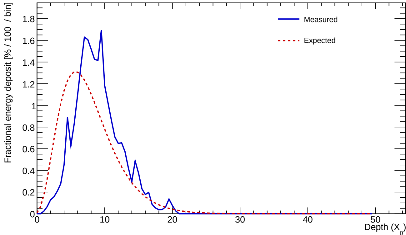
Cluster 643 E=23.763 GeV profileStart=2.00 X_0 \chi=0.1984
