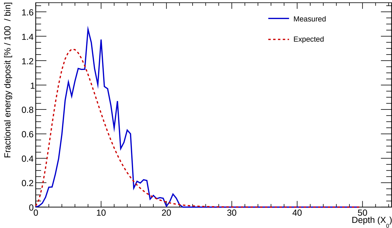
Cluster 755 E=23.452 GeV profileStart=1.50 X_0 \chi=0.1677
