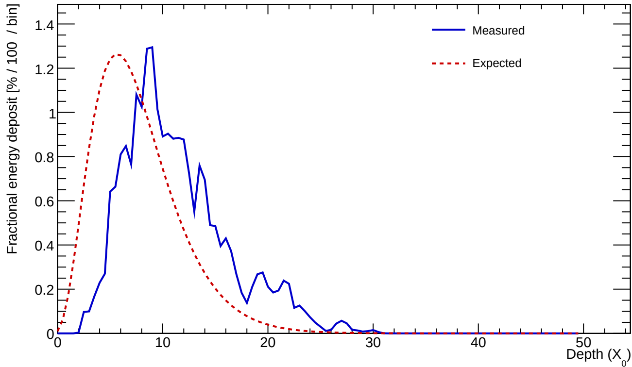
Cluster 681 E=22.847 GeV profileStart=3.00 X_0 \chi=0.2073
