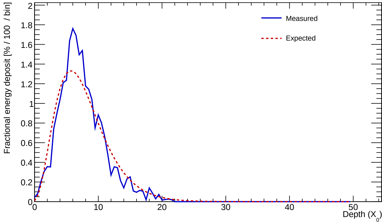
Cluster 573 E=24.193 GeV profileStart=0.50 X_0 \chi=0.1799
