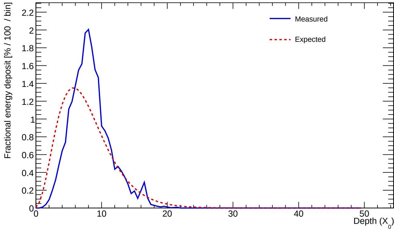
Cluster 989 E=24.545 GeV profileStart=1.50 X_0 \chi=0.2648
