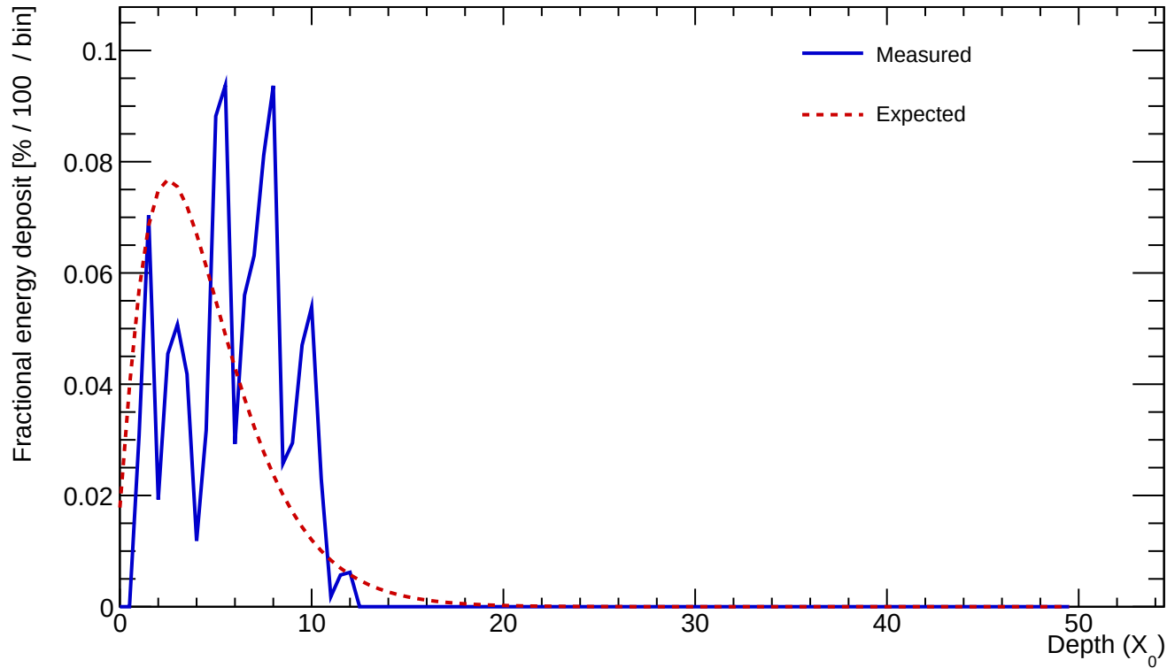
Cluster 213 E=1.000 GeV profileStart=2.00 X_0 \chi=0.5087
