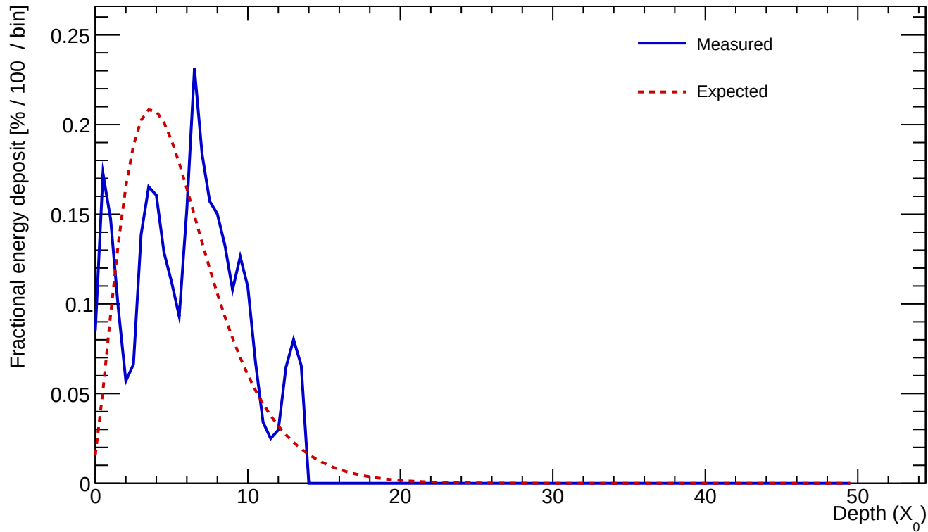
Cluster 729 E=3.143 GeV profileStart=1.50 X_0 \chi=0.3689
