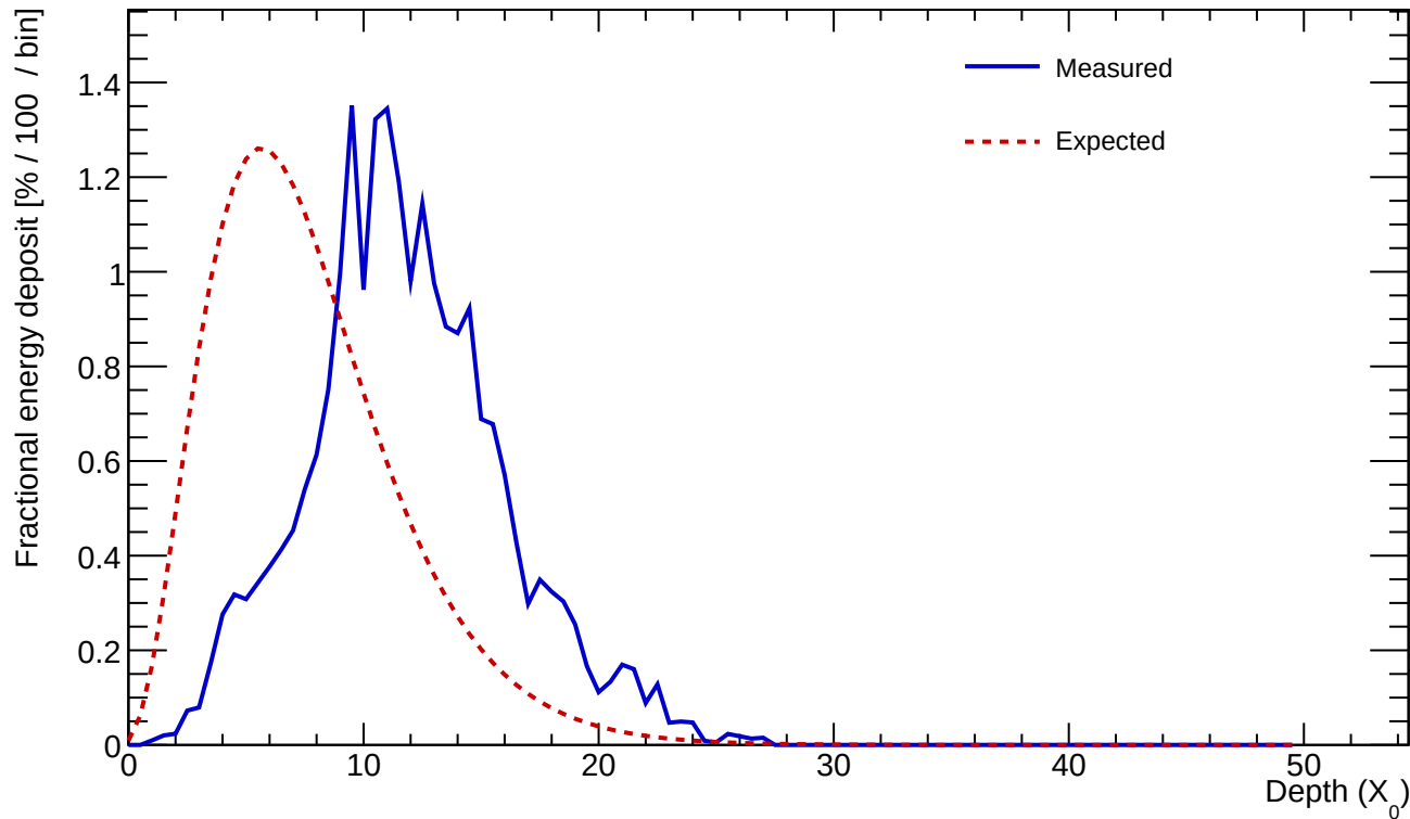
Cluster 159 E=22.795 GeV profileStart=5.00 X_0 \chi=0.2058
