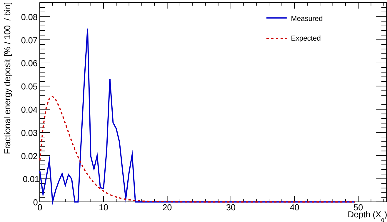
Cluster 1027 E=0.536 GeV profileStart=6.00 X_0 \chi=0.7162
