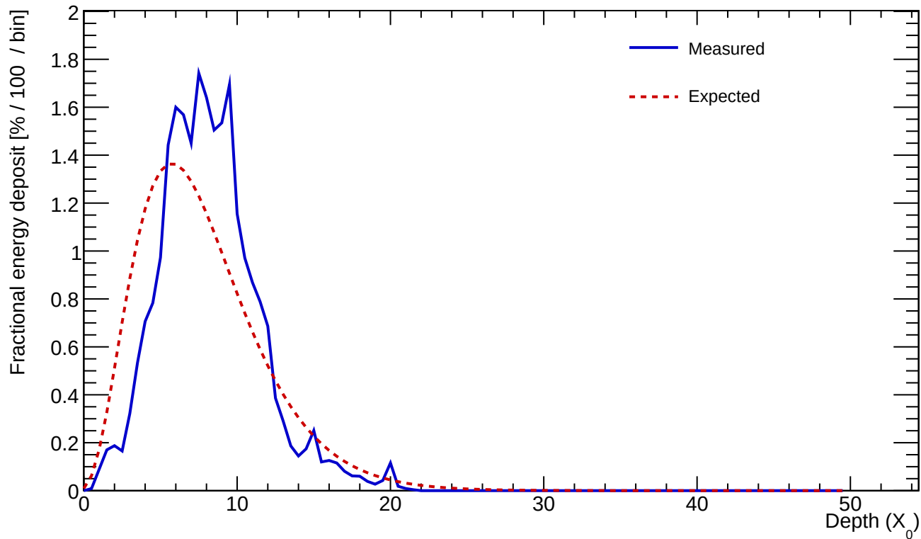
Cluster 224 E=24.839 GeV \text{profileStart}=1.50 X_0 \chi=0.2458
