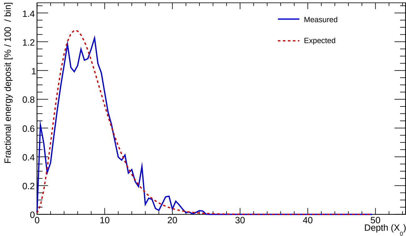
Cluster 470 E=23.156 GeV \text{profileStart}=0.50 X_0 \chi=0.1827
