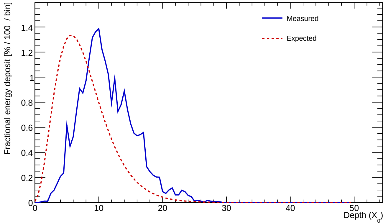
Cluster 720 E=24.230 GeV profileStart=4.00 X_0 \chi=0.1650
