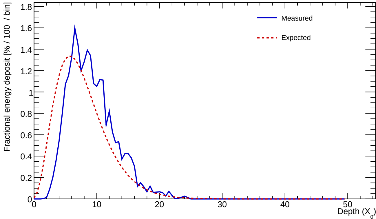
Cluster 798 E=24.293 GeV profileStart=1.50 X_0 \chi=0.1274
