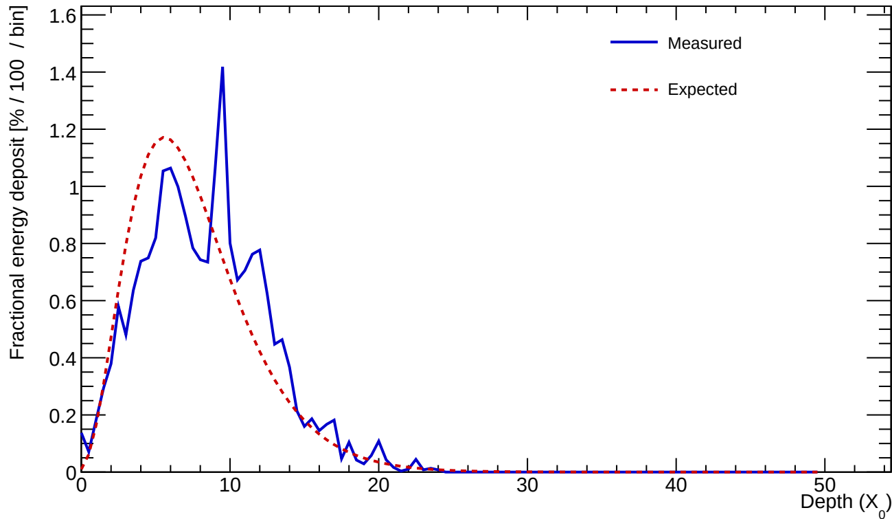
Cluster 438 E=21.033 GeV profileStart=1.00 X_0 \chi=0.2459
