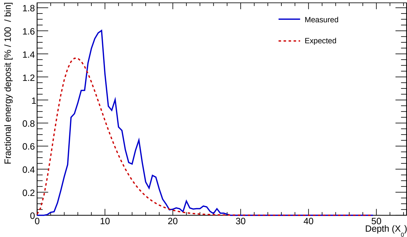
Cluster 51 E=24.823 GeV profileStart=2.50 X_0 \chi=0.1596
