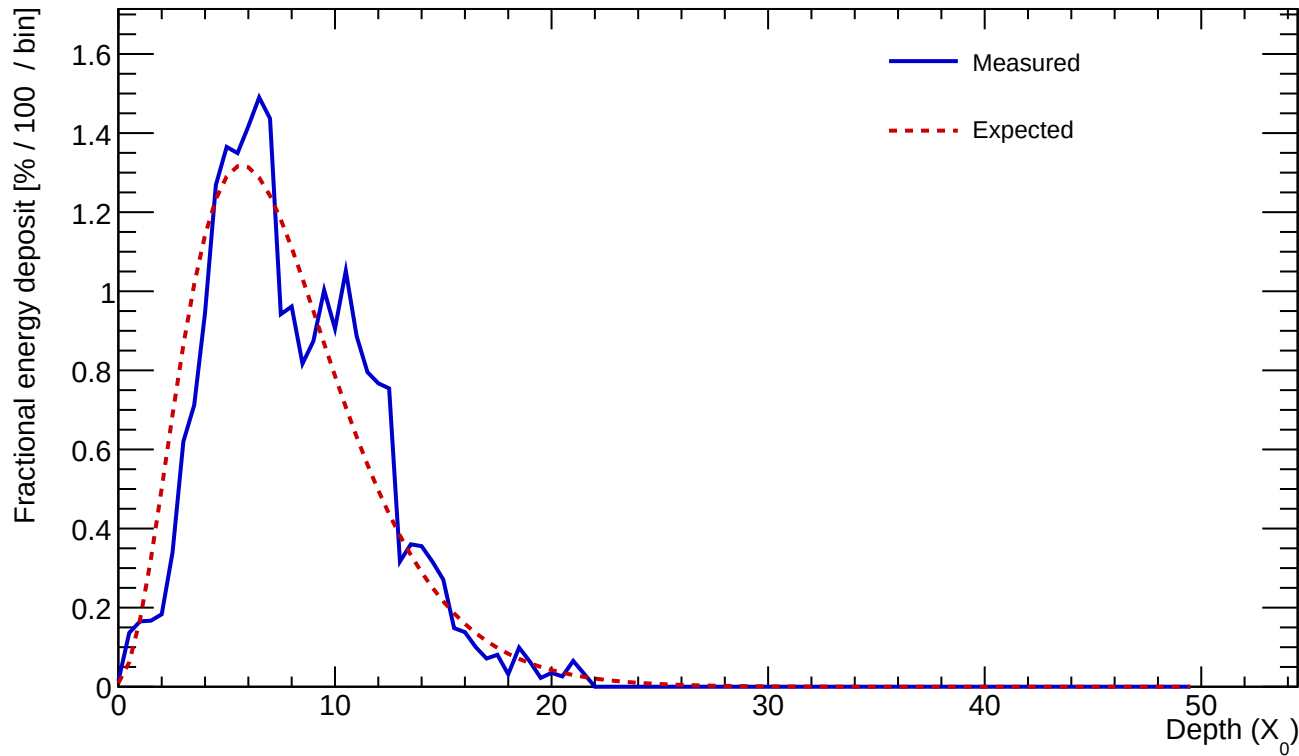
Cluster 417 E=23.903 GeV profileStart=0.50 X_0 \chi=0.1837
