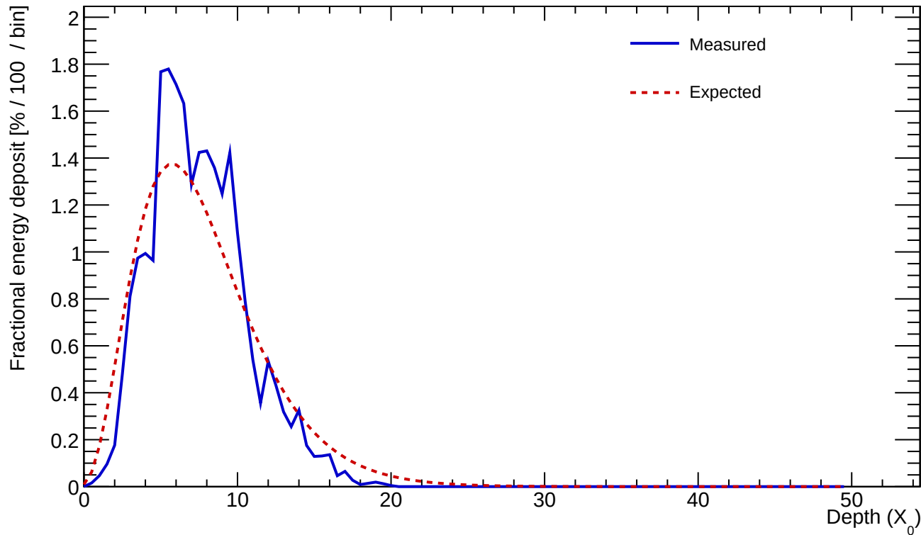
Cluster 899 E=25.019 GeV profileStart=0.50 X_0 \chi=0.2255
