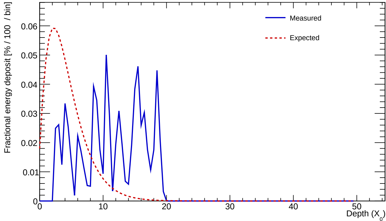
Cluster 1061 E=0.739 GeV profileStart=8.00 X_0 \chi=0.8927
