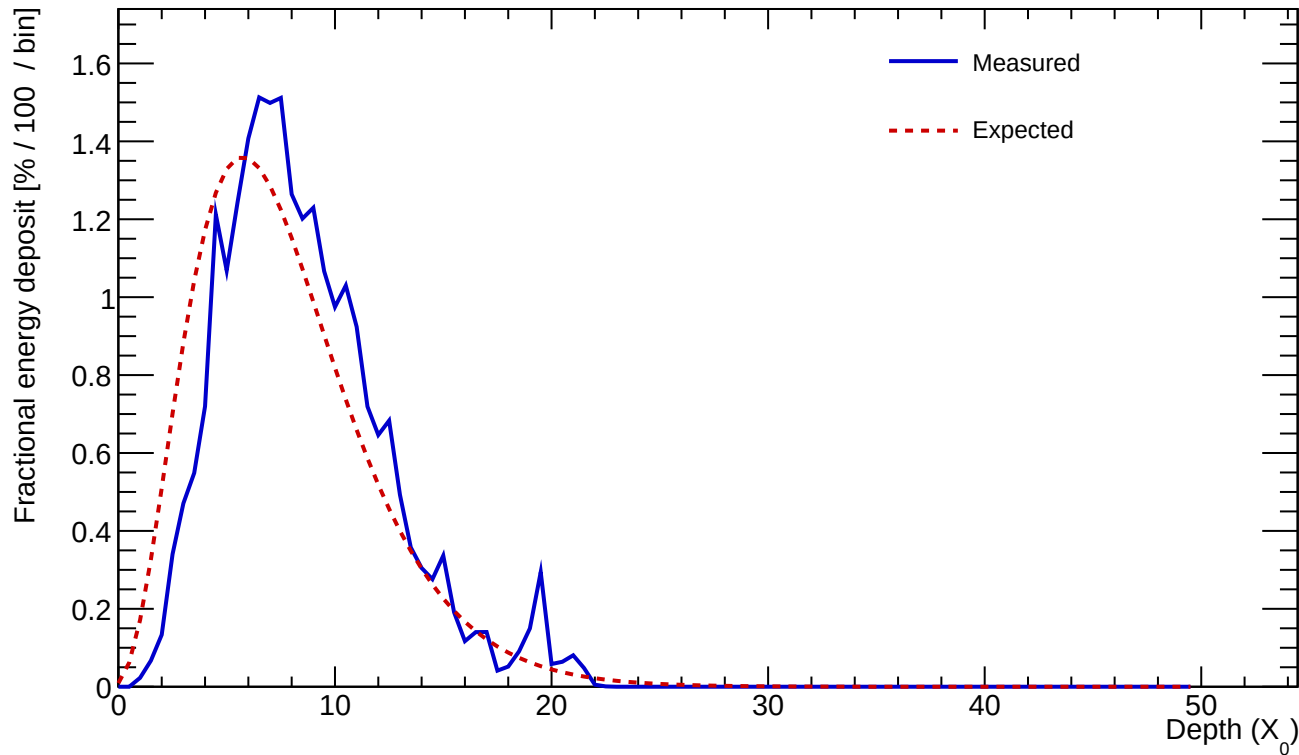
Cluster 639 E=24.738 GeV profileStart=1.00 X_0 \chi=0.1180
