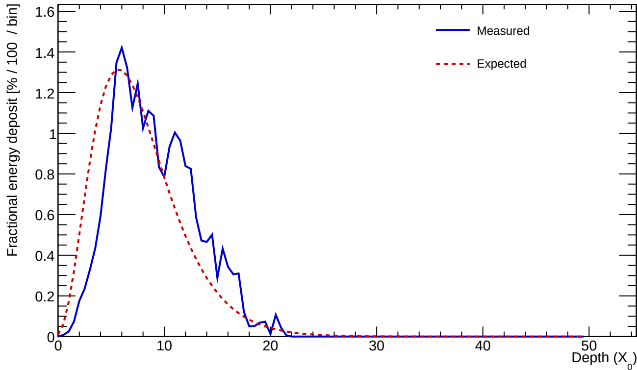
Cluster 102 E=23.833 GeV profileStart=1.50 X_0 \chi=0.1622
