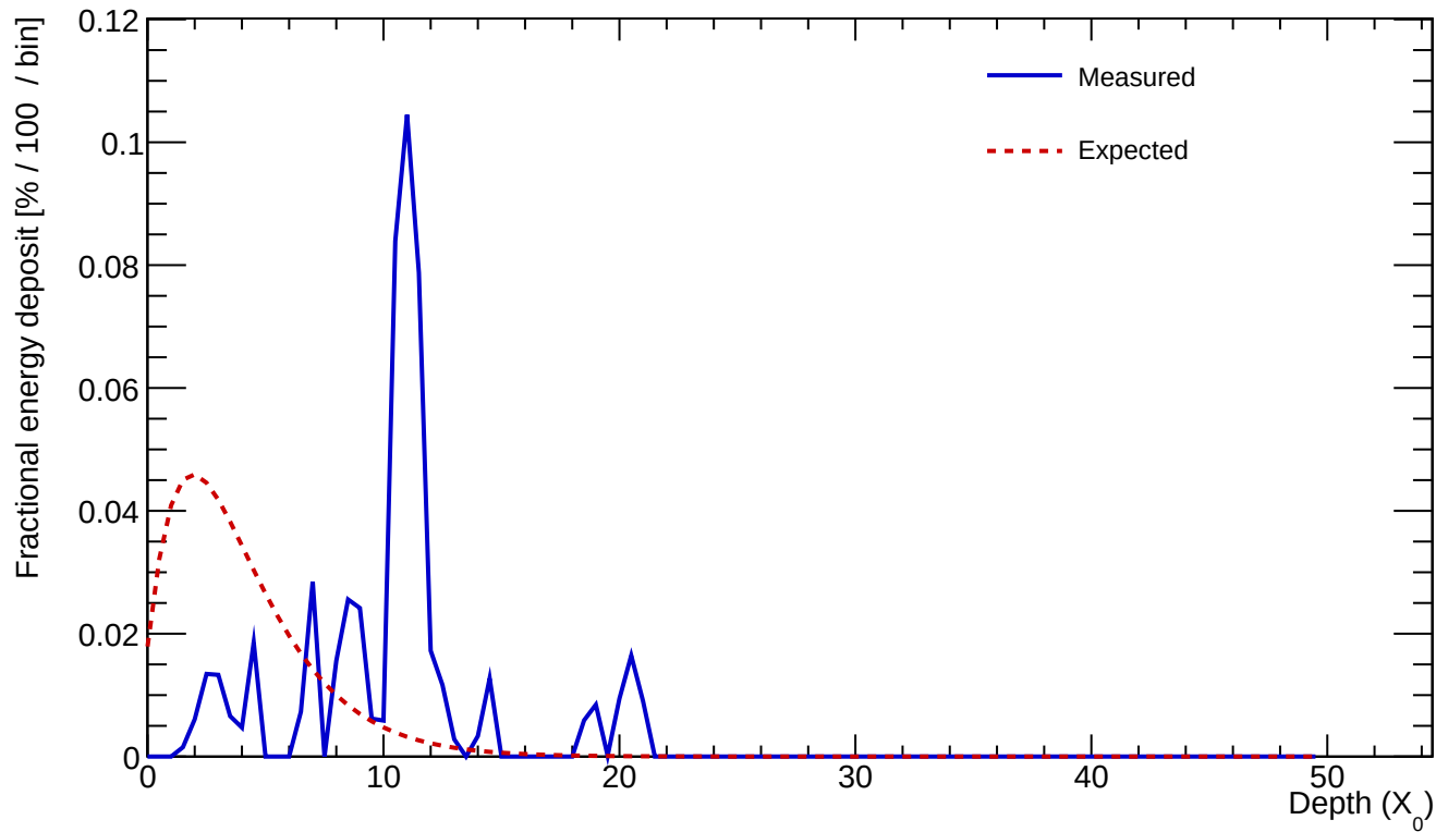
Cluster 1036 E=0.542 GeV \text{profileStart}=8.00 X_0 \chi=1.0037
