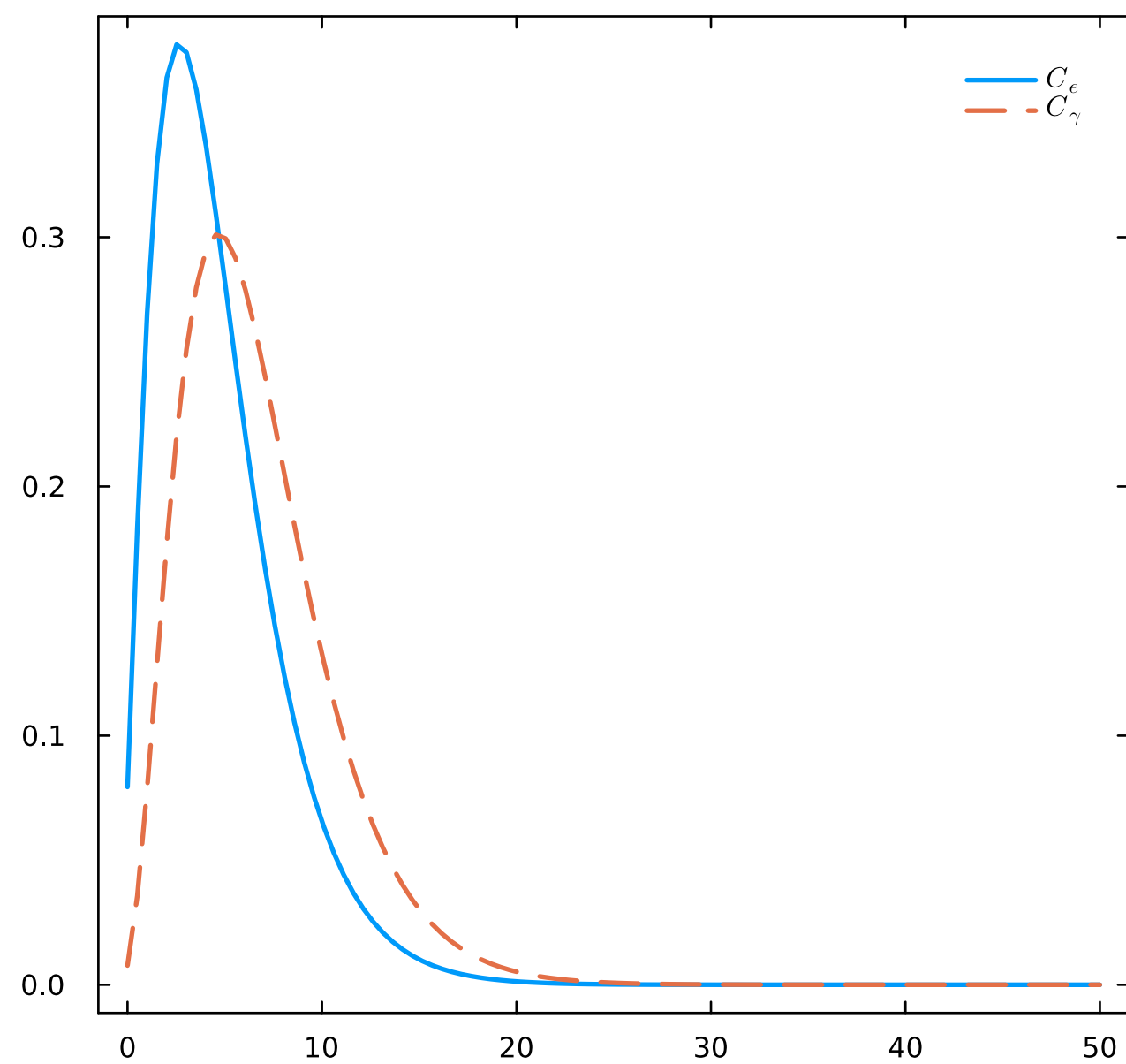
E = 100.0 GeV
