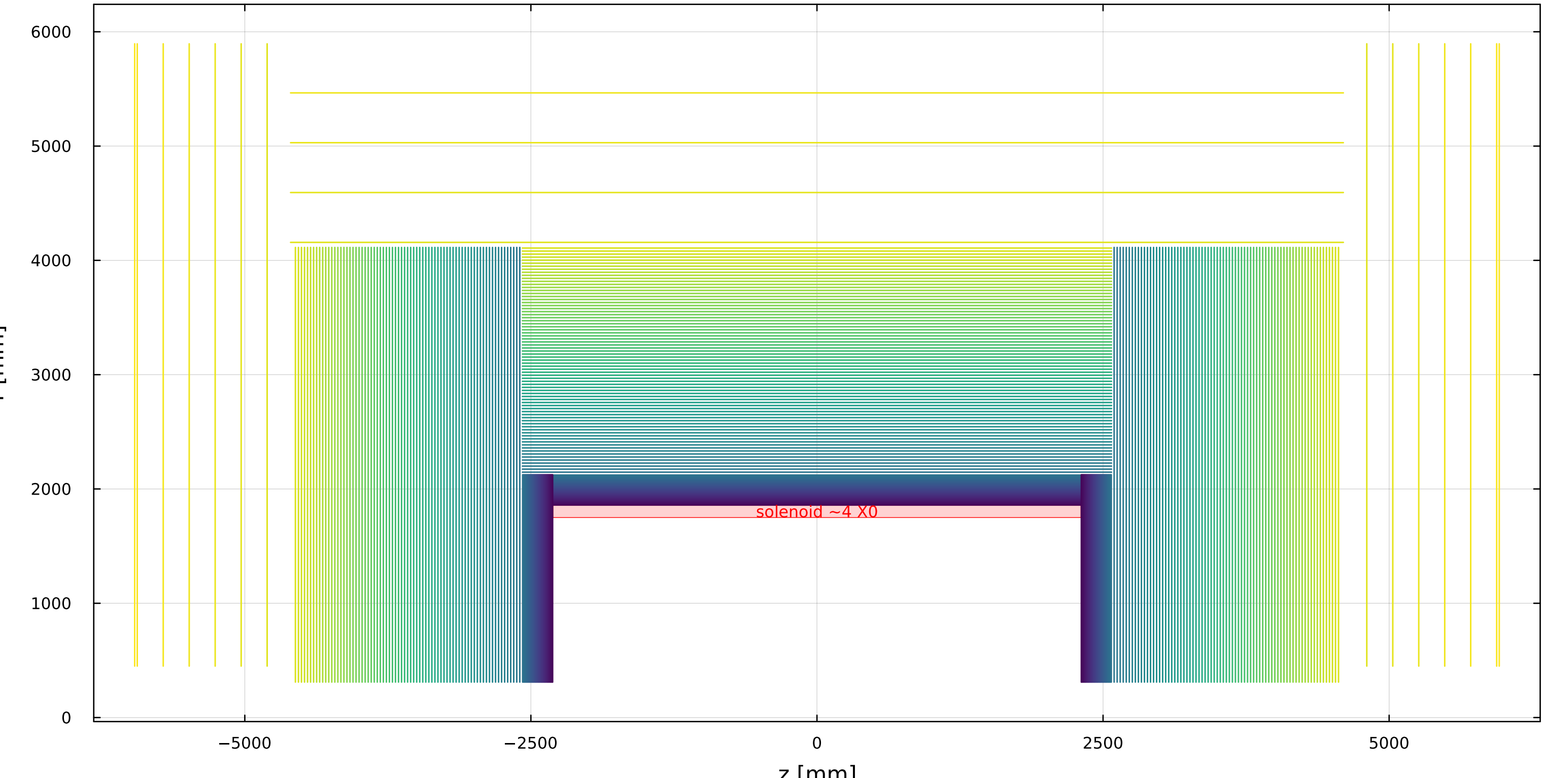
MAIA r-z cross-section - nominal (color = pseudolayer)
