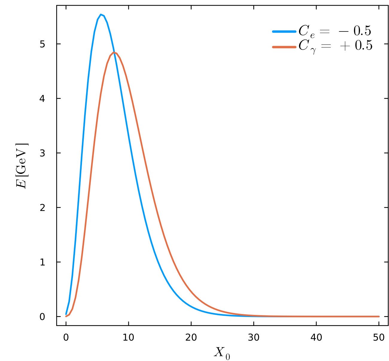
E = 100.0 GeV
