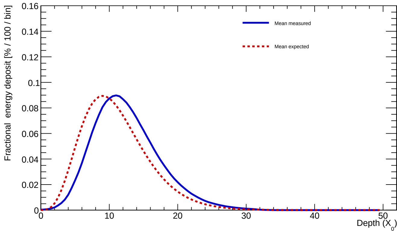
Average longitudinal profile (260 clusters): measured vs expected
