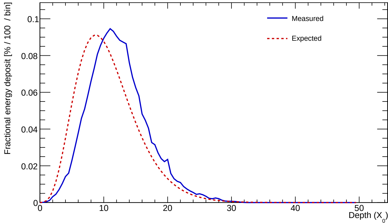
Cluster 89 E=500.593 GeV profileStart=2.00 X_0 \chi=0.0846
