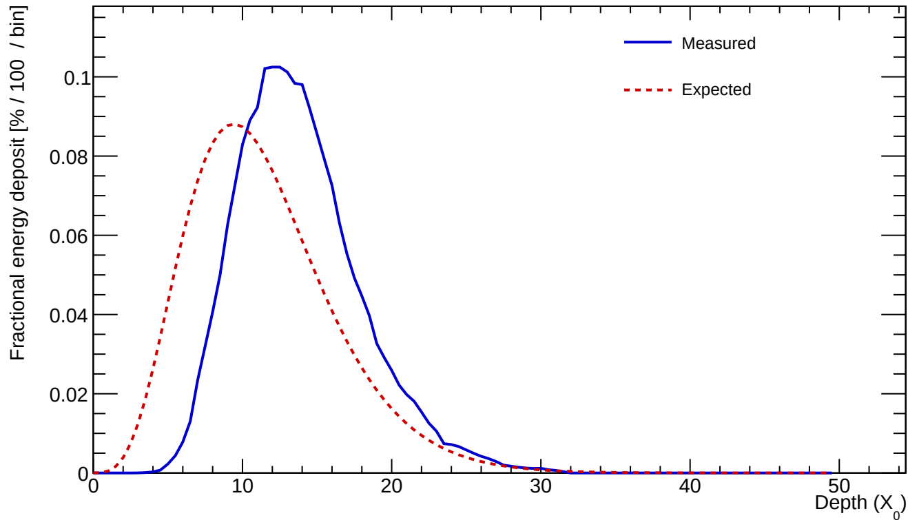
Cluster 85 E=984.017 GeV profileStart=3.00 X_0 \chi=0.1513
