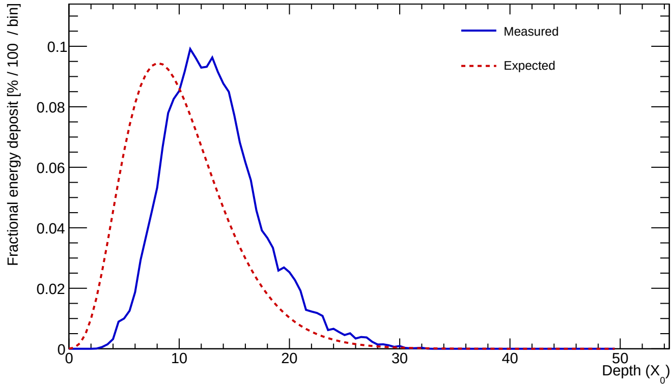
Cluster 153 E=260.661 GeV profileStart=3.50 X_0 \chi=0.0746
