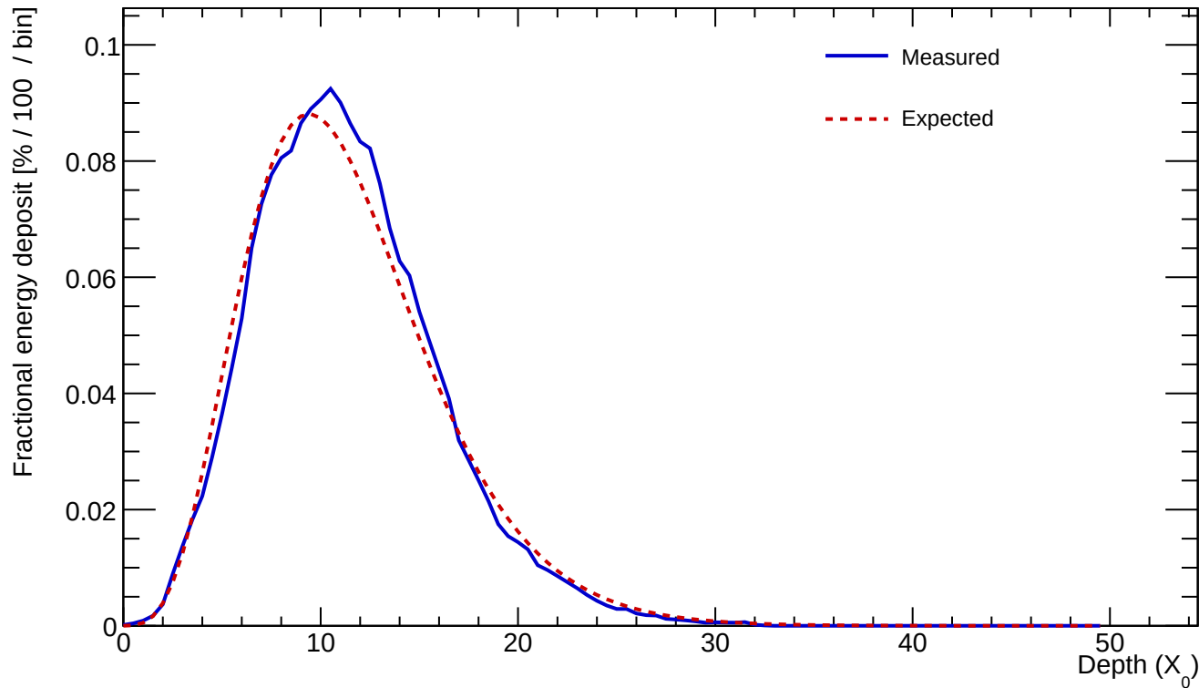
Cluster 185 E=979.540 GeV profileStart=0.50 X_0 \chi=0.0738
