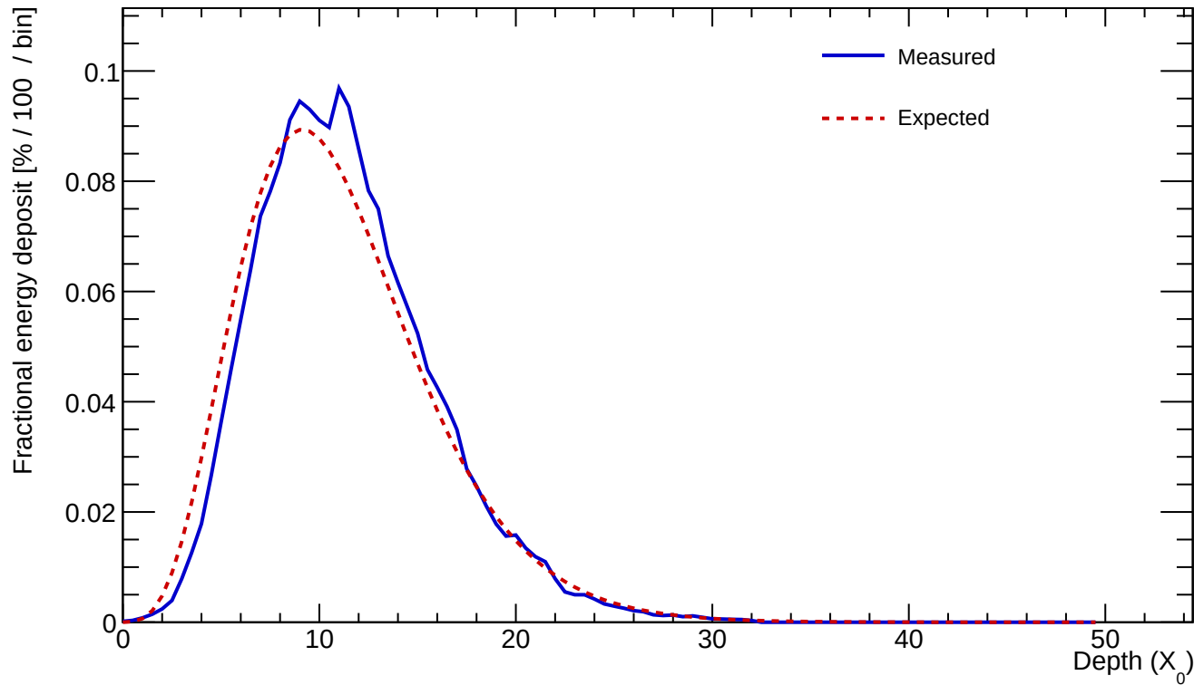
Cluster 6 E=735.772 GeV profileStart=0.50 X_0 \chi=0.0591
