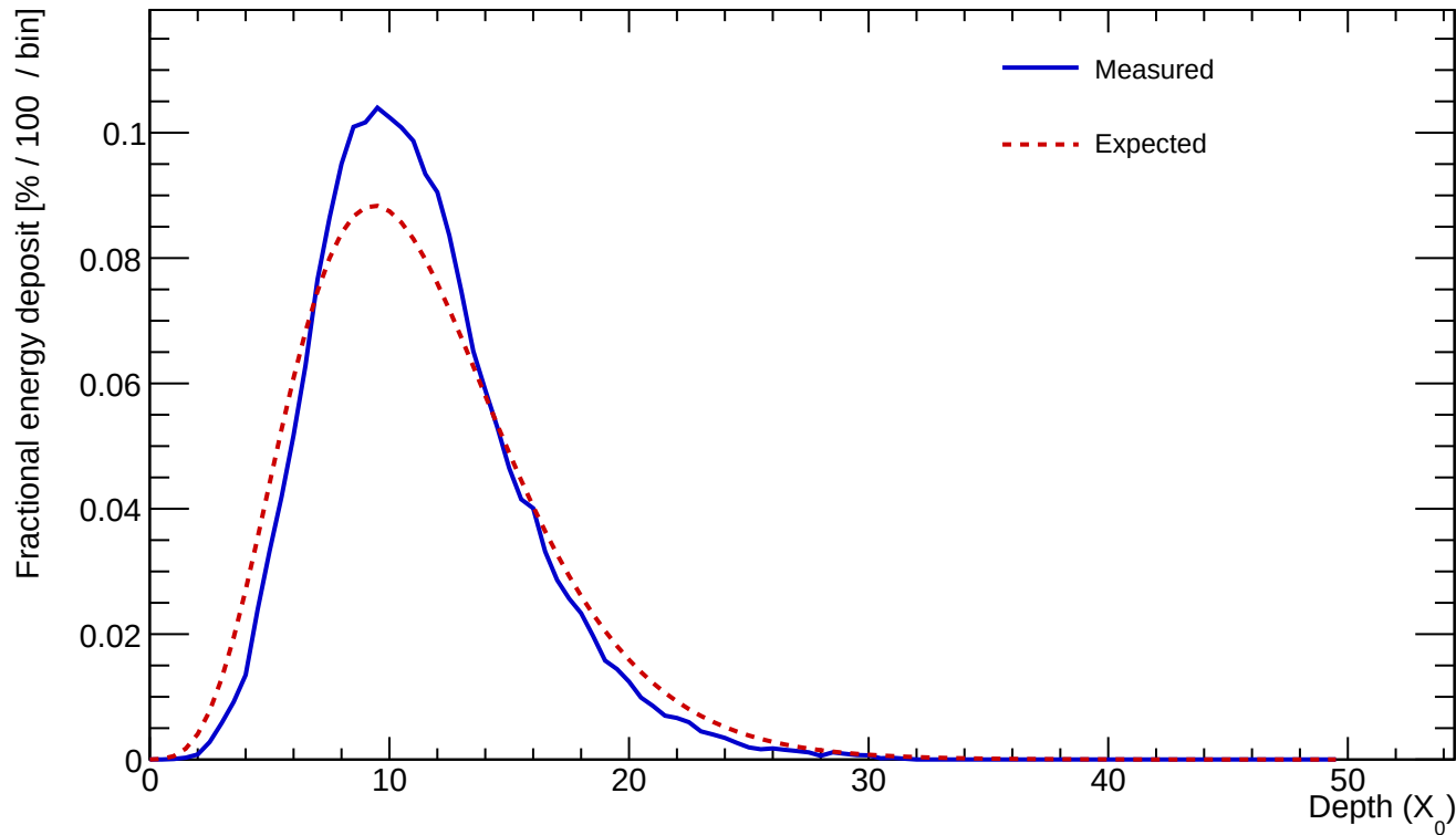
Cluster 138 E=922.184 GeV profileStart=0.50 X_0 \chi=0.1555
