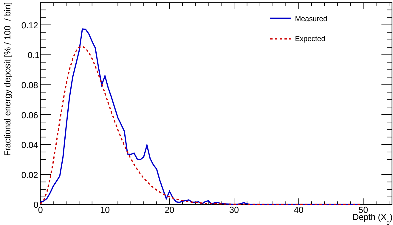
Cluster 78 E=47.977 GeV profileStart=1.00 X_0 \chi=0.1194
