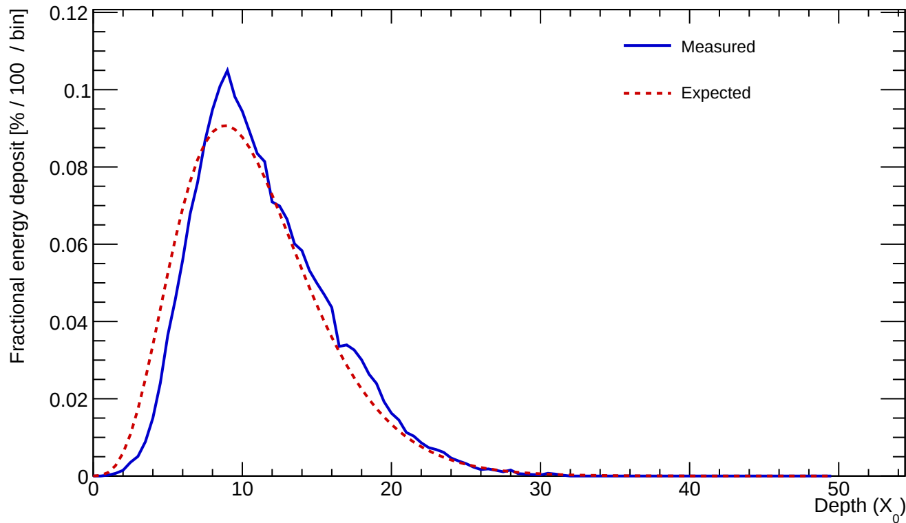
Cluster 126 E=543.545 GeV profileStart=0.50 X_0 \chi=0.0836
