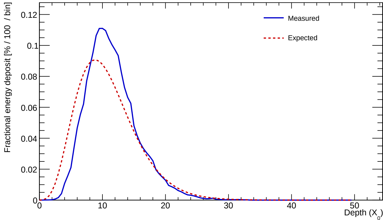
Cluster 44 E=554.164 GeV profileStart=1.00 X_0 \chi=0.1792
