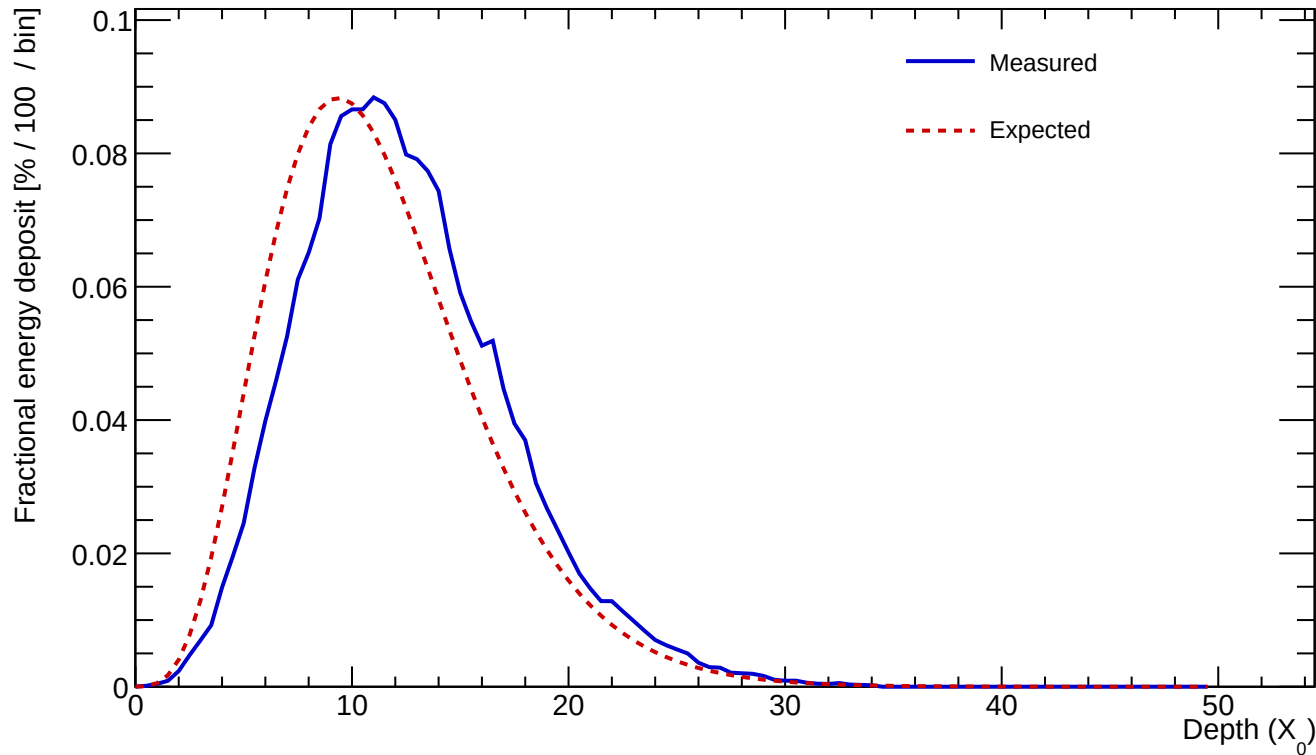
Cluster 221 E=926.275 GeV profileStart=1.50 X_0 \chi=0.0597
