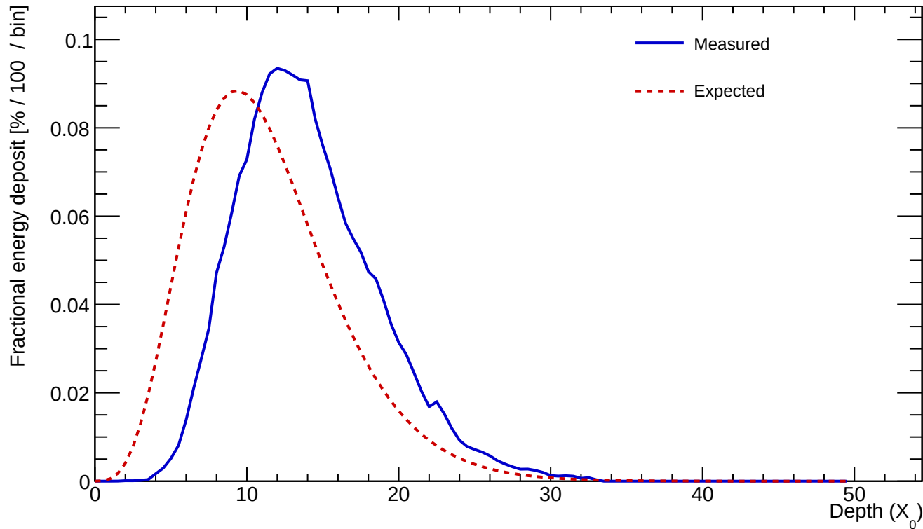
Cluster 84 E=917.657 GeV profileStart=3.00 X_0 \chi=0.0519
