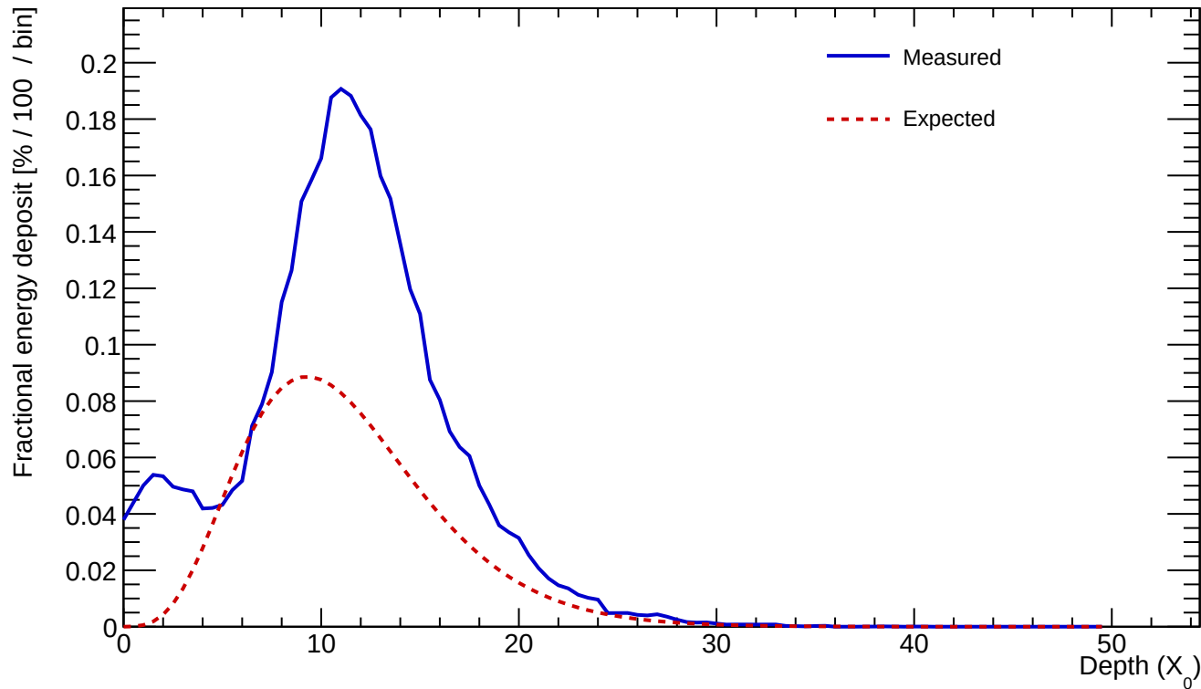
Cluster 3 E=860.846 GeV profileStart=1.00 X_0 \chi=0.2590
