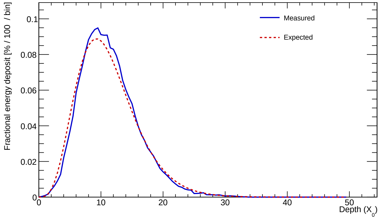
Cluster 11 E=833.134 GeV profileStart=0.50 X_0 \chi=0.0712
