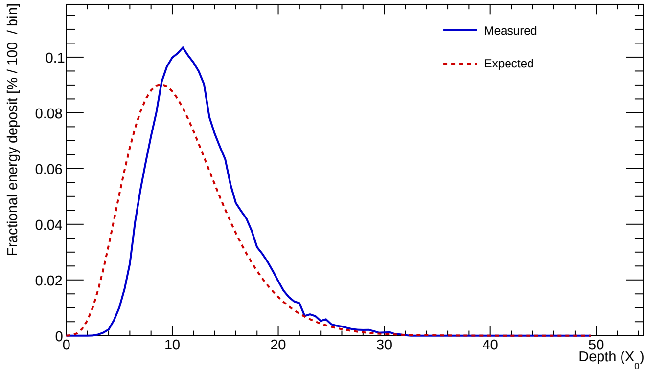
Cluster 9 E=605.459 GeV profileStart=2.00 X_0 \chi=0.1119
