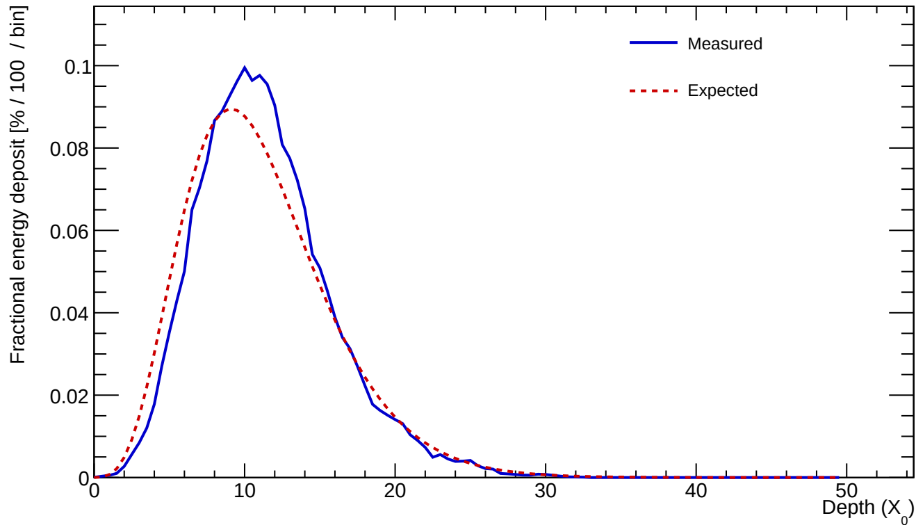
Cluster 224 E=714.284 GeV profileStart=0.50 X_0 \chi=0.0978
