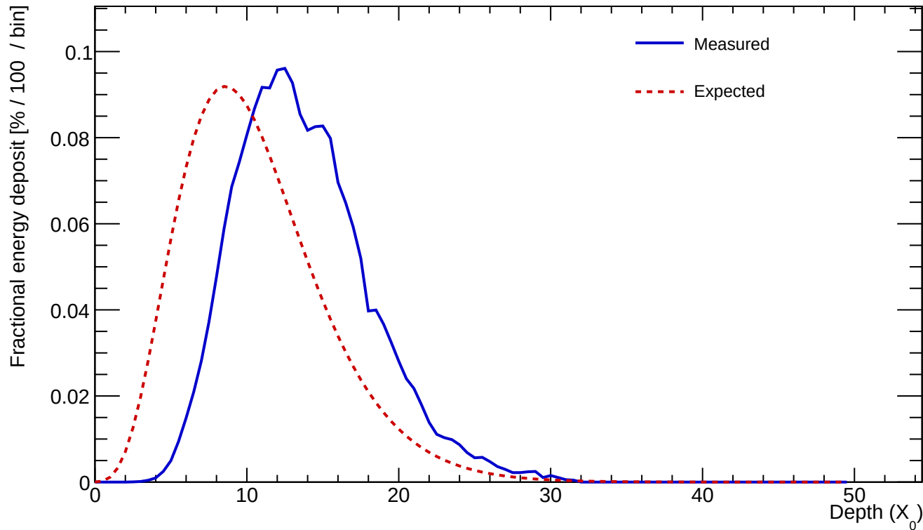
Cluster 15 E=427.585 GeV profileStart=3.50 X_0 \chi=0.0614
