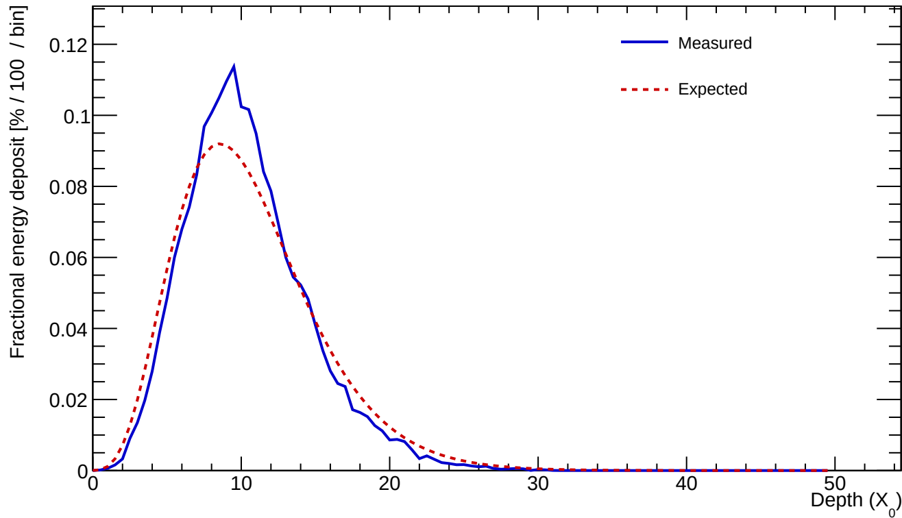
Cluster 34 E=421.725 GeV profileStart=0.50 X_0 \chi=0.1365
