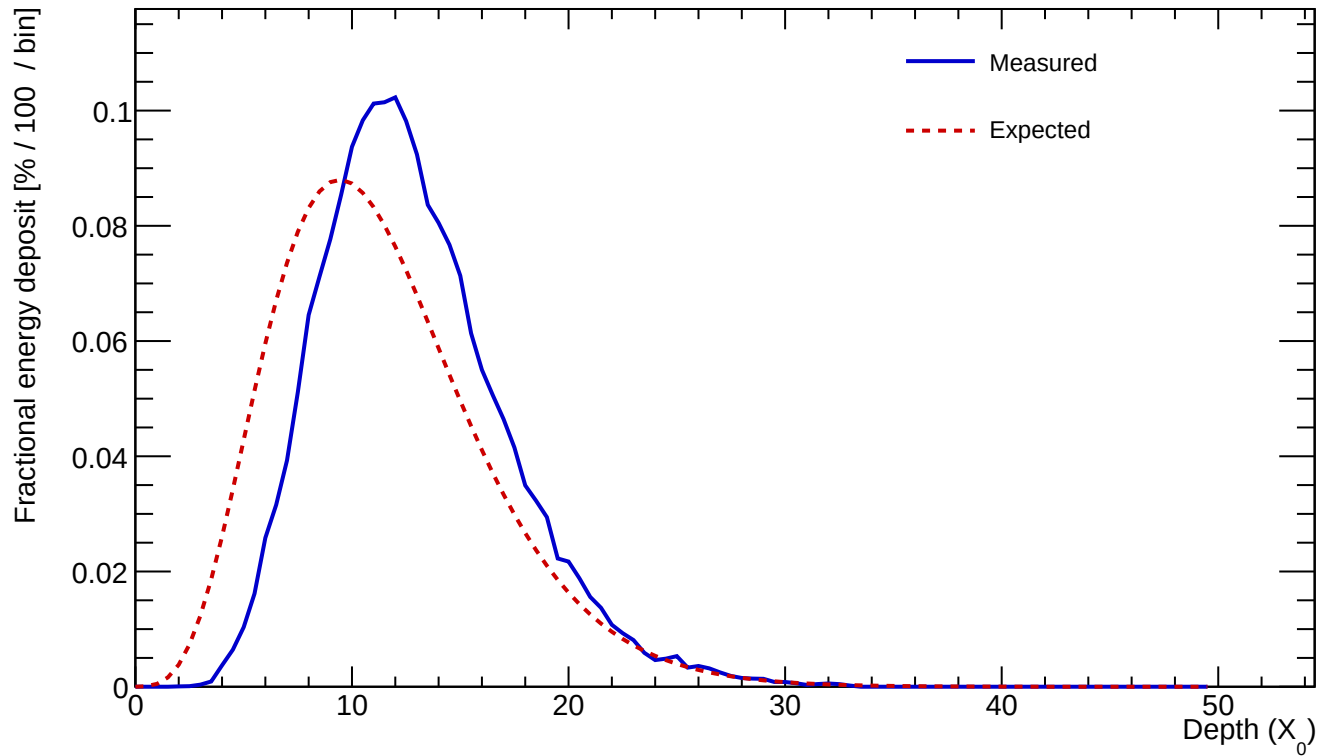
Cluster 5 E=1002.032 GeV profileStart=2.00 X_0 \chi=0.1202
