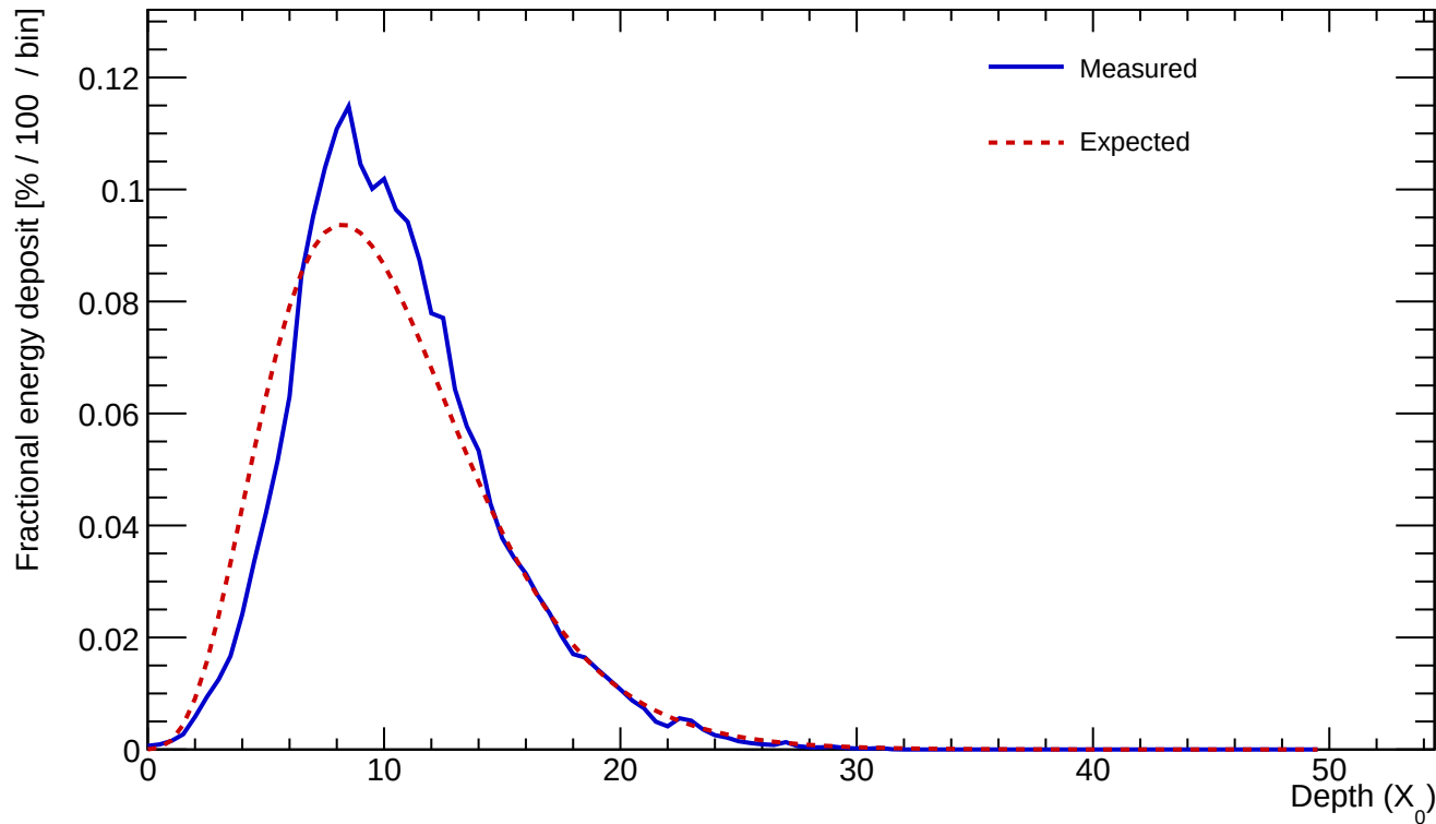
Cluster 97 E=295.807 GeV profileStart=0.50 X_0 \chi=0.1308
