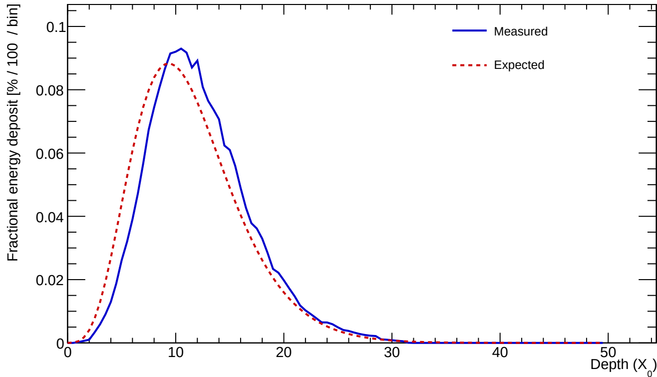
Cluster 33 E=929.979 GeV profileStart=1.00 X_0 \chi=0.0457
