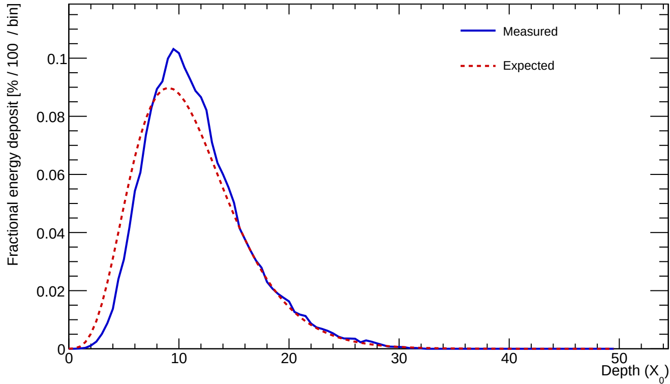
Cluster 194 E=666.243 GeV profileStart=0.50 X_0 \chi=0.0945
