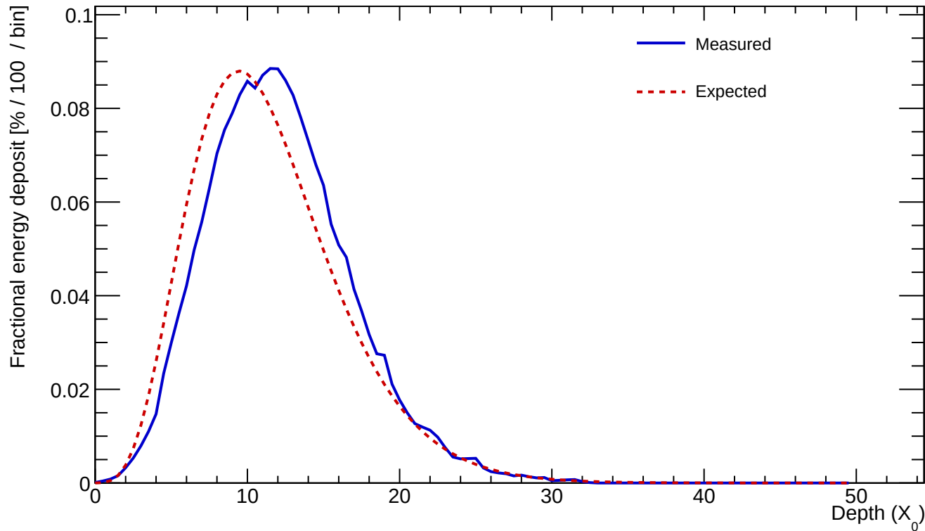
Cluster 203 E=1010.360 GeV profileStart=1.00 X_0 \chi=0.0729
