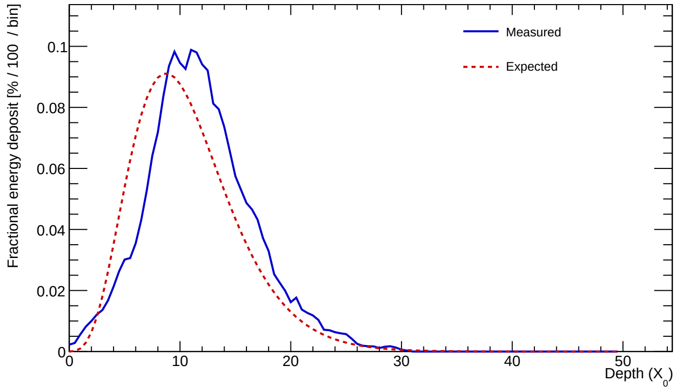
Cluster 143 E=499.187 GeV profileStart=1.50 X_0 \chi=0.1068
