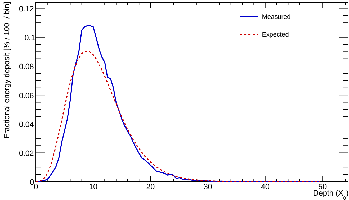
Cluster 13 E=570.082 GeV profileStart=0.50 X_0 \chi=0.1467
