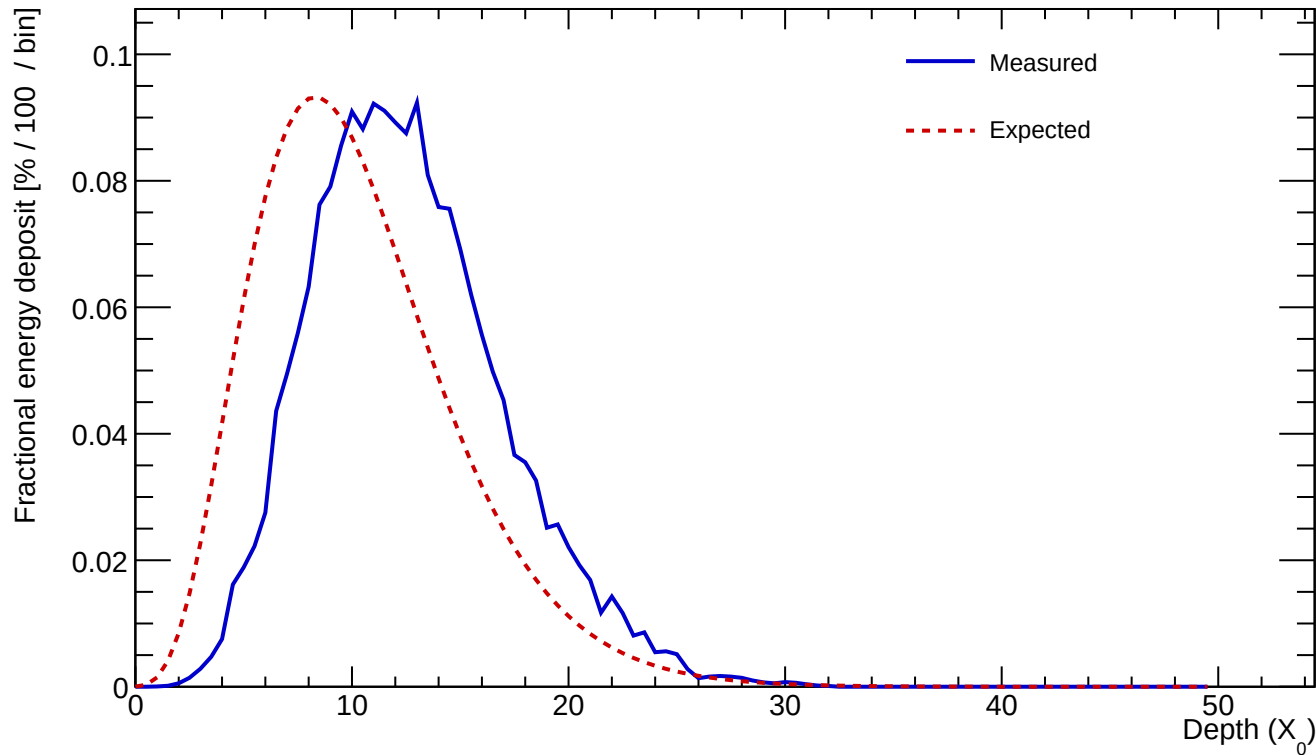
Cluster 98 E=327.017 GeV profileStart=2.50 X_0 \chi=0.0622
