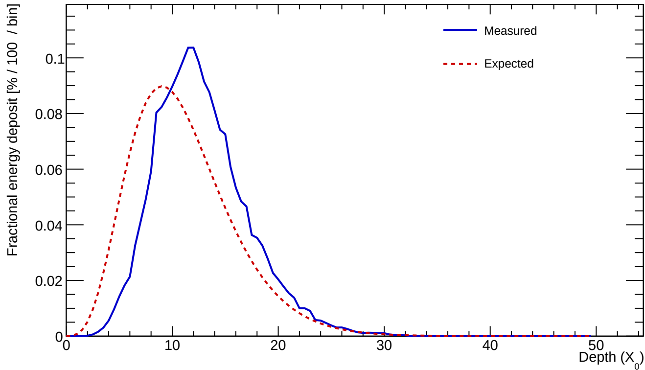
Cluster 57 E=669.163 GeV profileStart=2.00 X_0 \chi=0.1124
