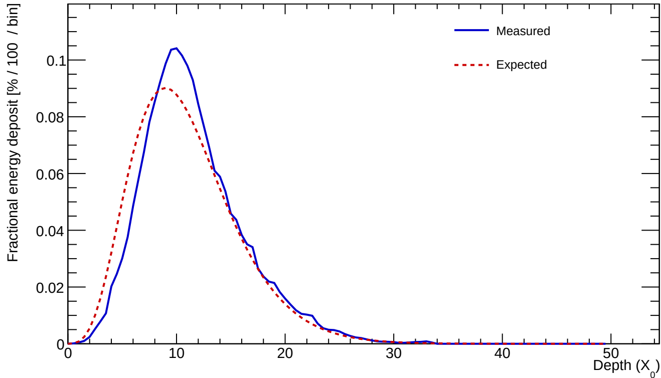
Cluster 238 E=618.905 GeV profileStart=0.50 X_0 \chi=0.0974
