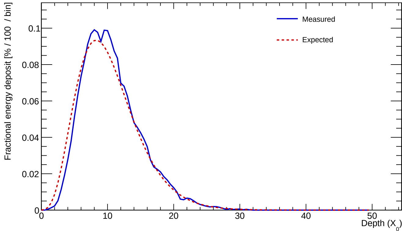
Cluster 61 E=318.743 GeV profileStart=0.50 X_0 \chi=0.0685
