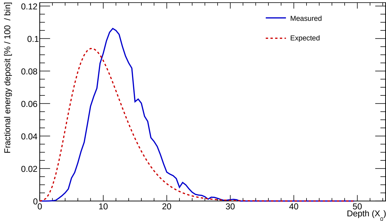
Cluster 52 E=287.505 GeV profileStart=3.00 X_0 \chi=0.1073
