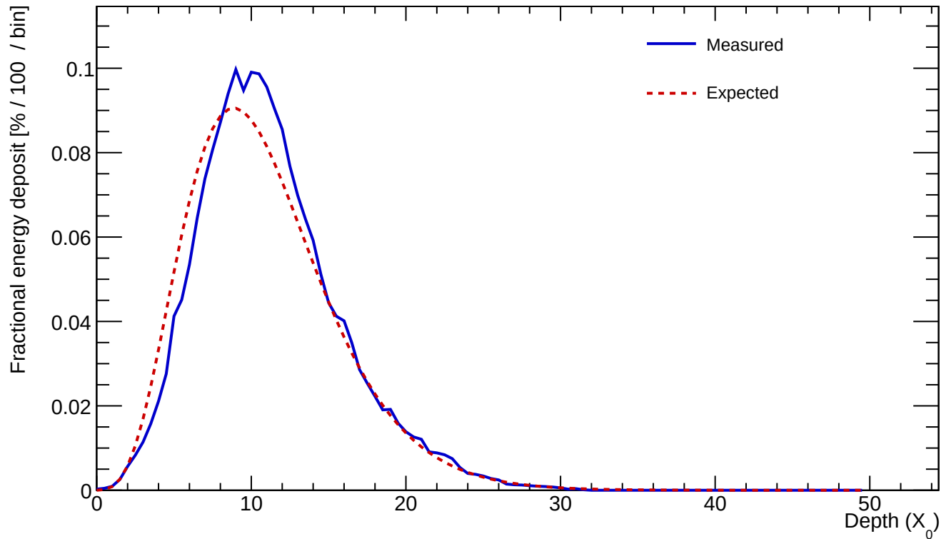
Cluster 132 E=567.957 GeV profileStart=0.50 X_0 \chi=0.0775
