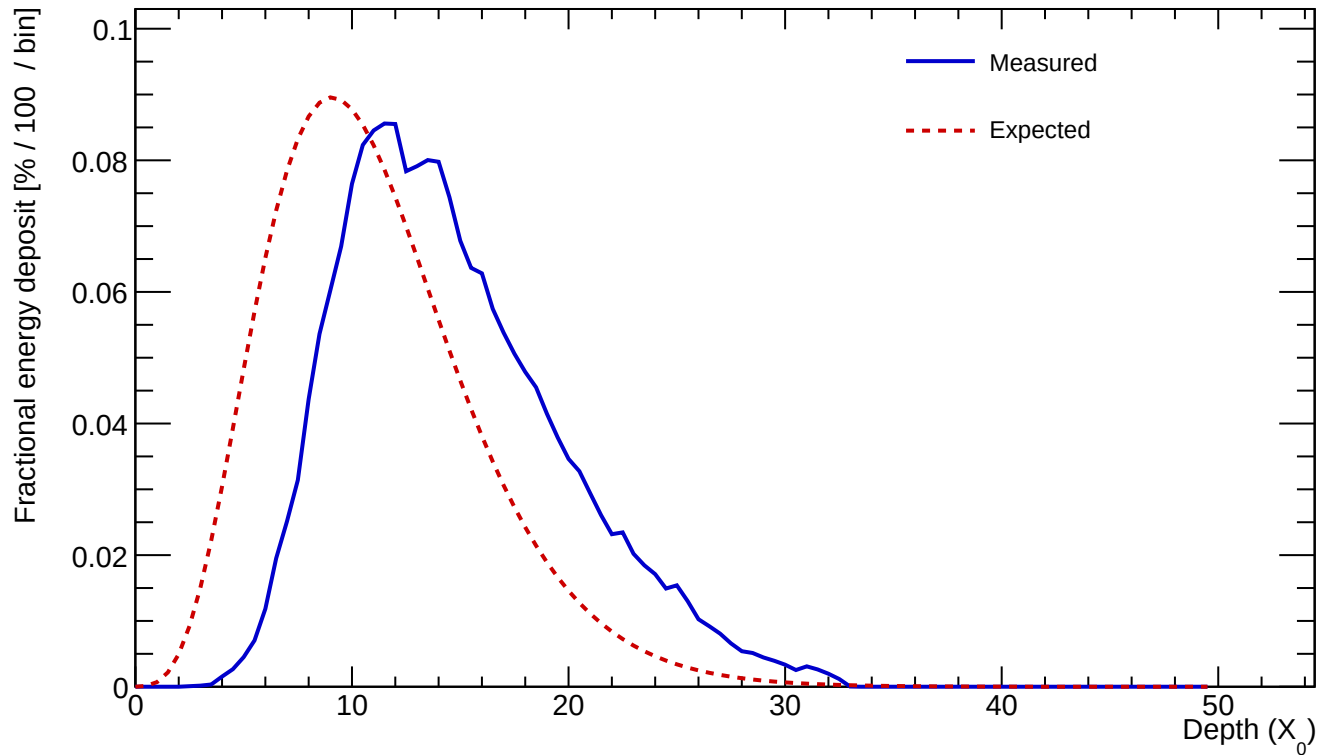
Cluster 41 E=703.234 GeV profileStart=3.50 X_0 \chi=0.1037
