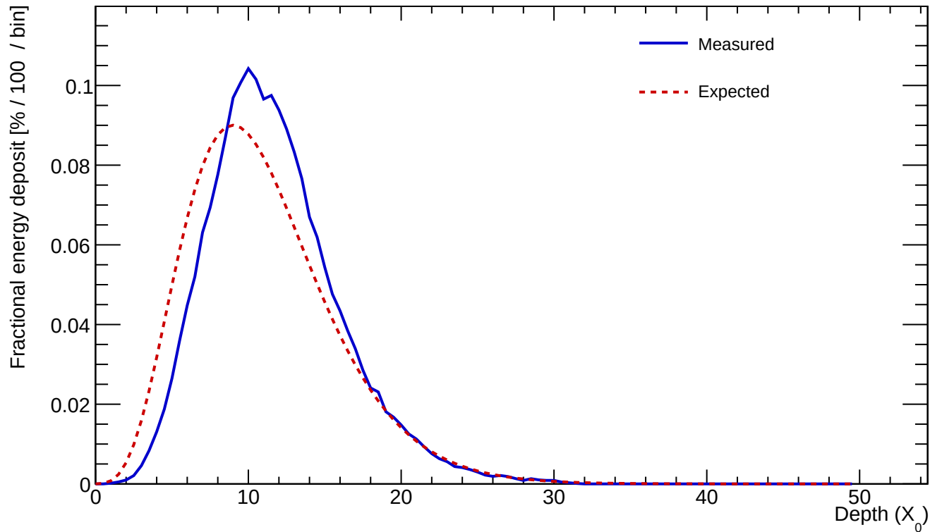
Cluster 23 E=636.145 GeV profileStart=1.00 X_0 \chi=0.1145
