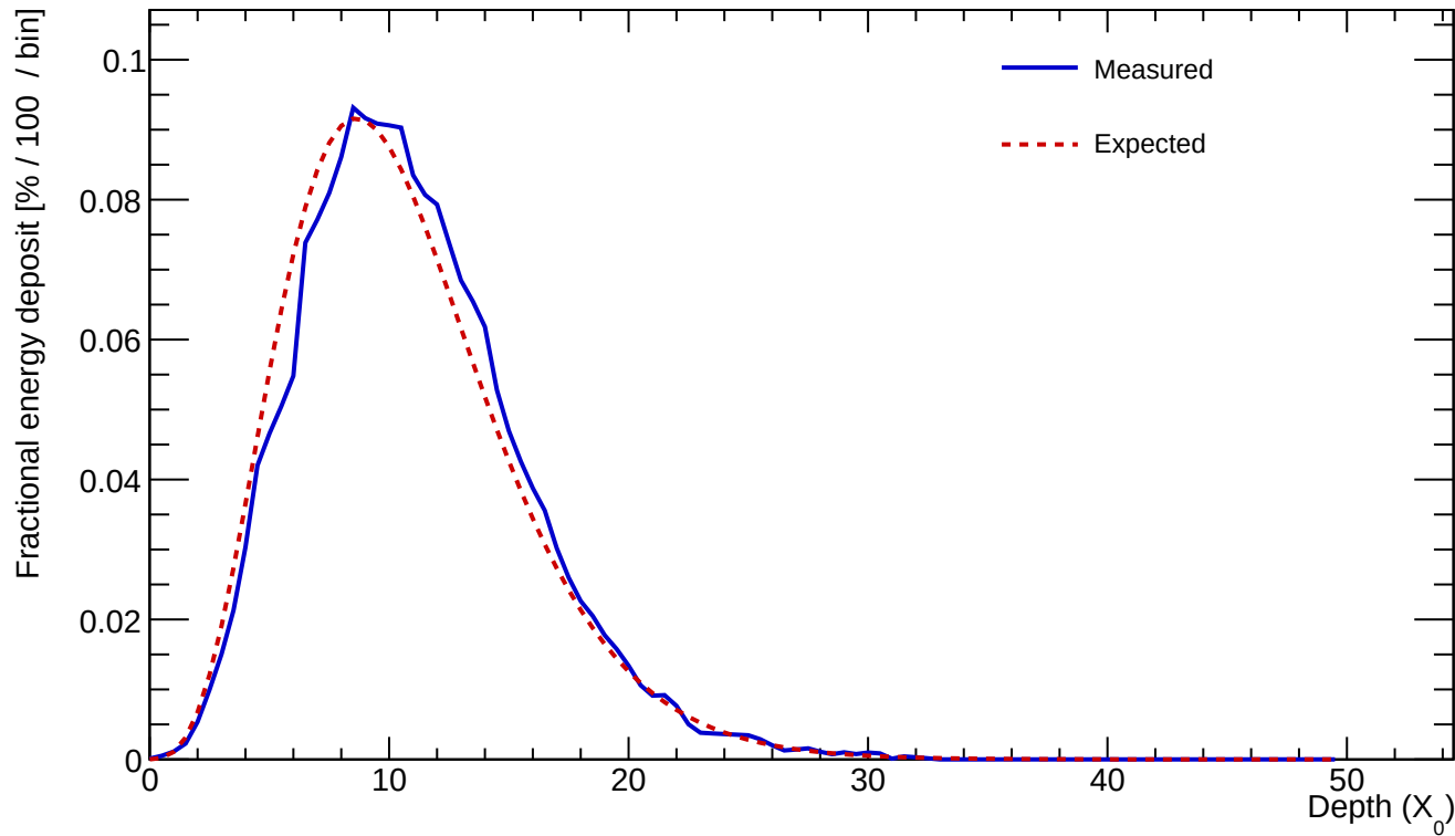
Cluster 39 E=454.072 GeV profileStart=0.50 X_0 \chi=0.0469
