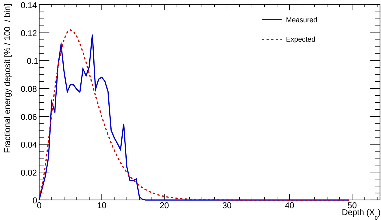
Cluster 17 E=12.246 GeV profileStart=0.50 X_0 \chi=0.2511
