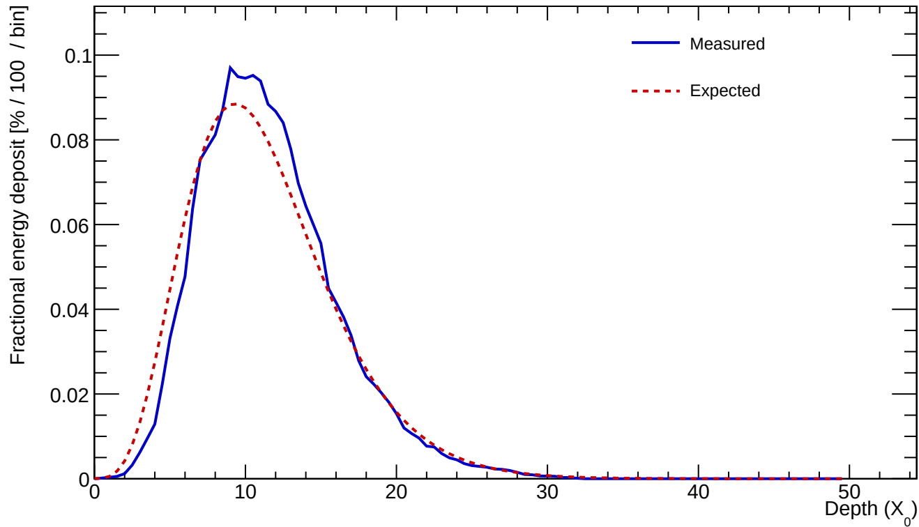
Cluster 30 E=888.224 GeV profileStart=0.50 X_0 \chi=0.0894
