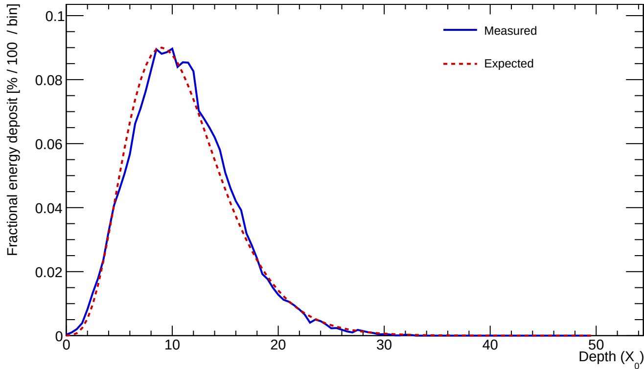
Cluster 62 E=640.344 GeV profileStart=0.50 X_0 \chi=0.0727
