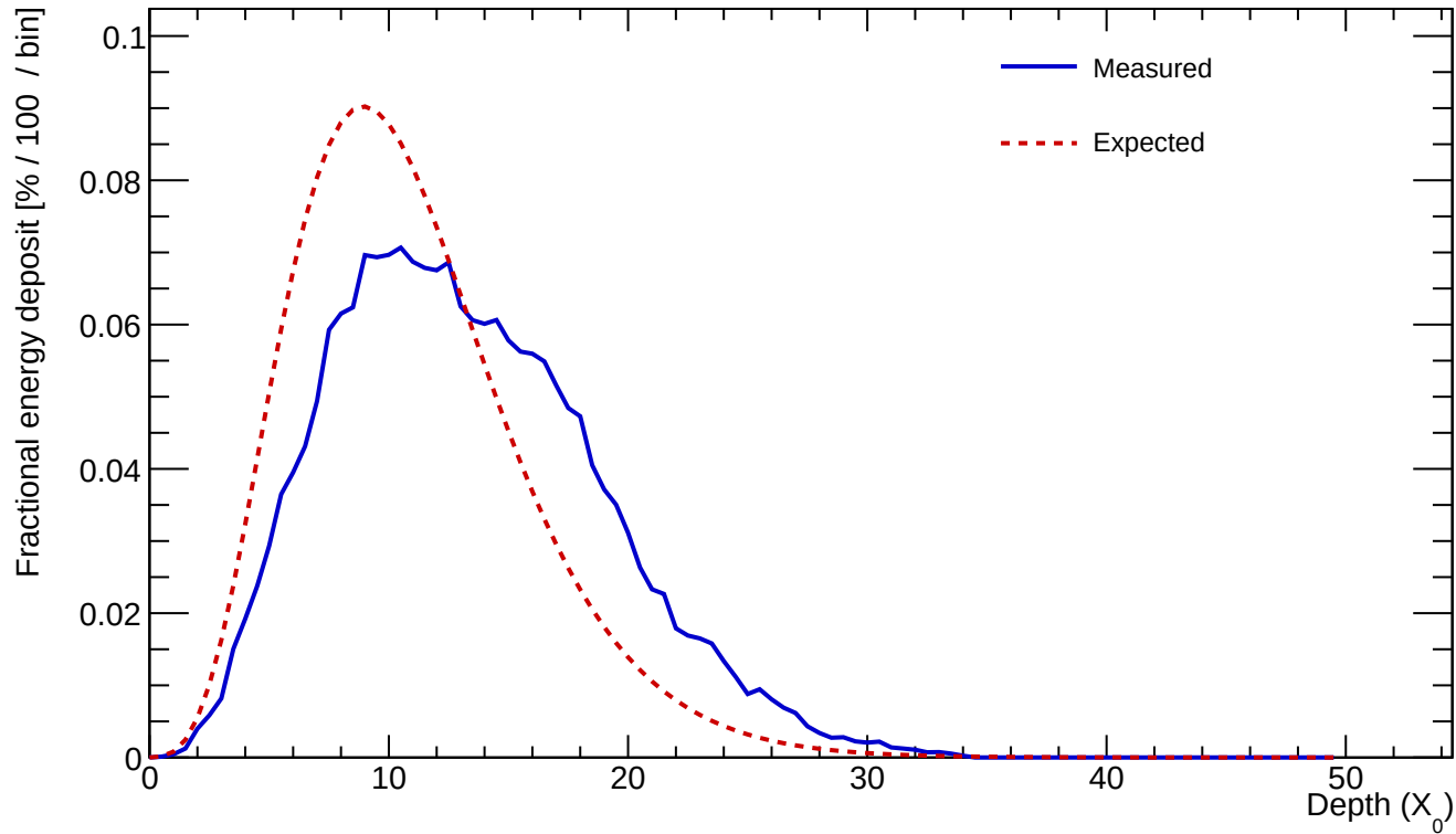
Cluster 4 E=608.651 GeV profileStart=2.00 X_0 \chi=0.2319
