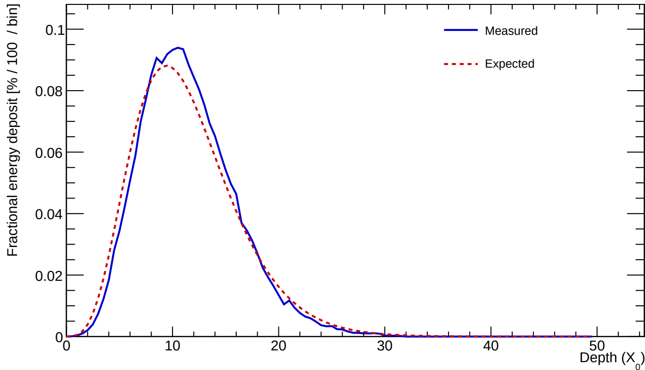
Cluster 43 E=973.936 GeV profileStart=0.50 X_0 \chi=0.0704
