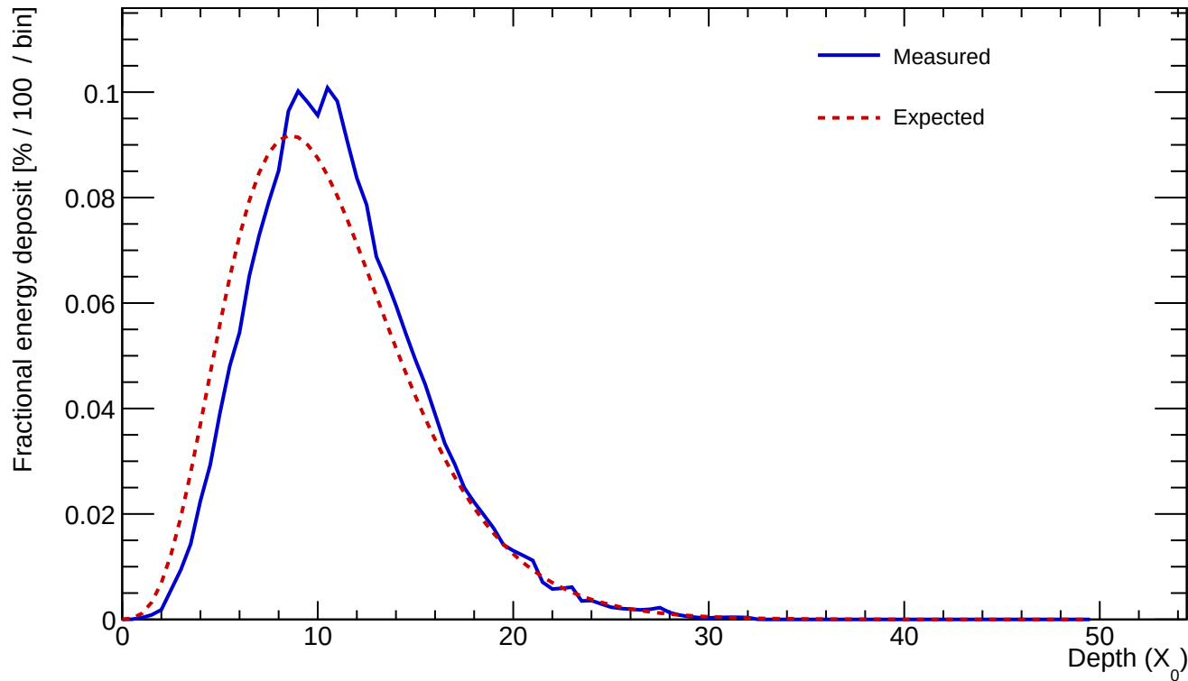
Cluster 55 E=438.574 GeV profileStart=1.00 X_0 \chi=0.0793
