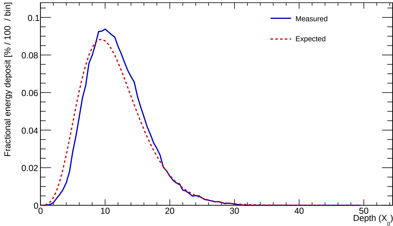
Cluster 96 E=925.144 GeV profileStart=1.00 X_0 \chi=0.0728
