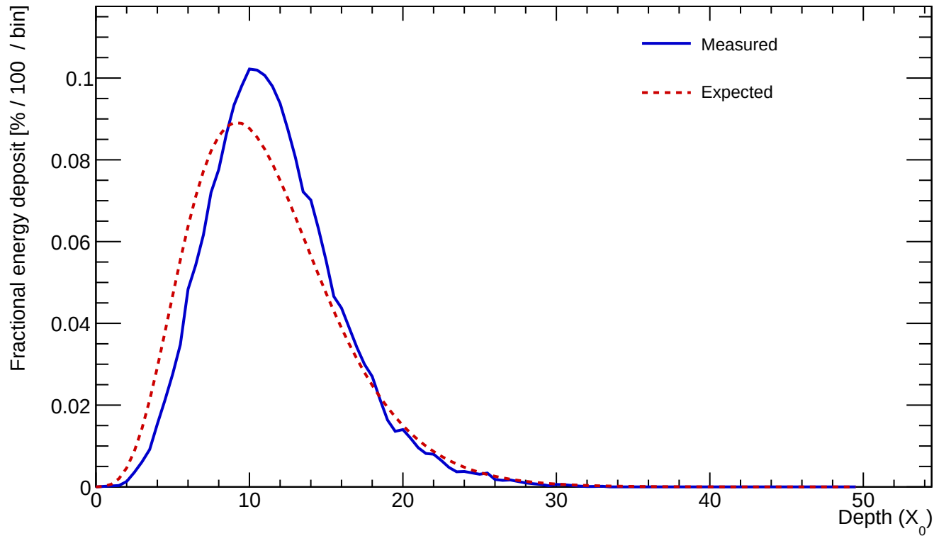
Cluster 40 E=770.350 GeV profileStart=1.00 X_0 \chi=0.1140
