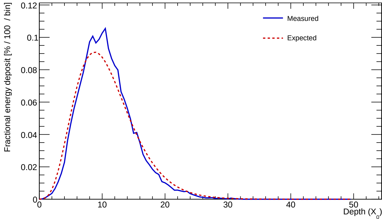
Cluster 18 E=533.003 GeV profileStart=0.50 X_0 \chi=0.1154
