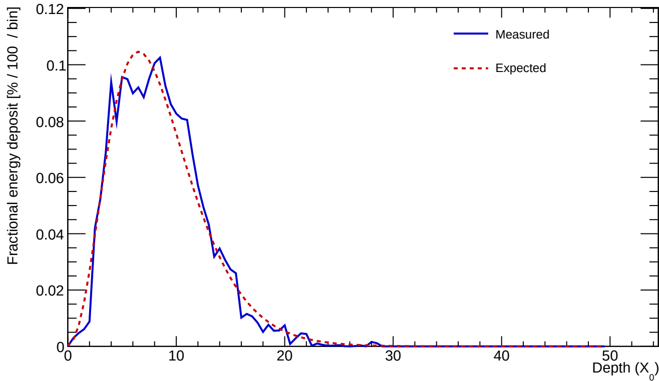
Cluster 106 E=54.391 GeV profileStart=0.50 X_0 \chi=0.1272
