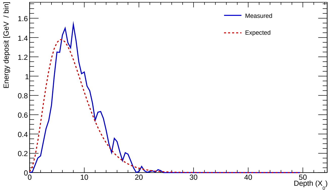
Cluster 68 E=25.142 GeV profileStart=1.00 X_0 \chi=0.1120
