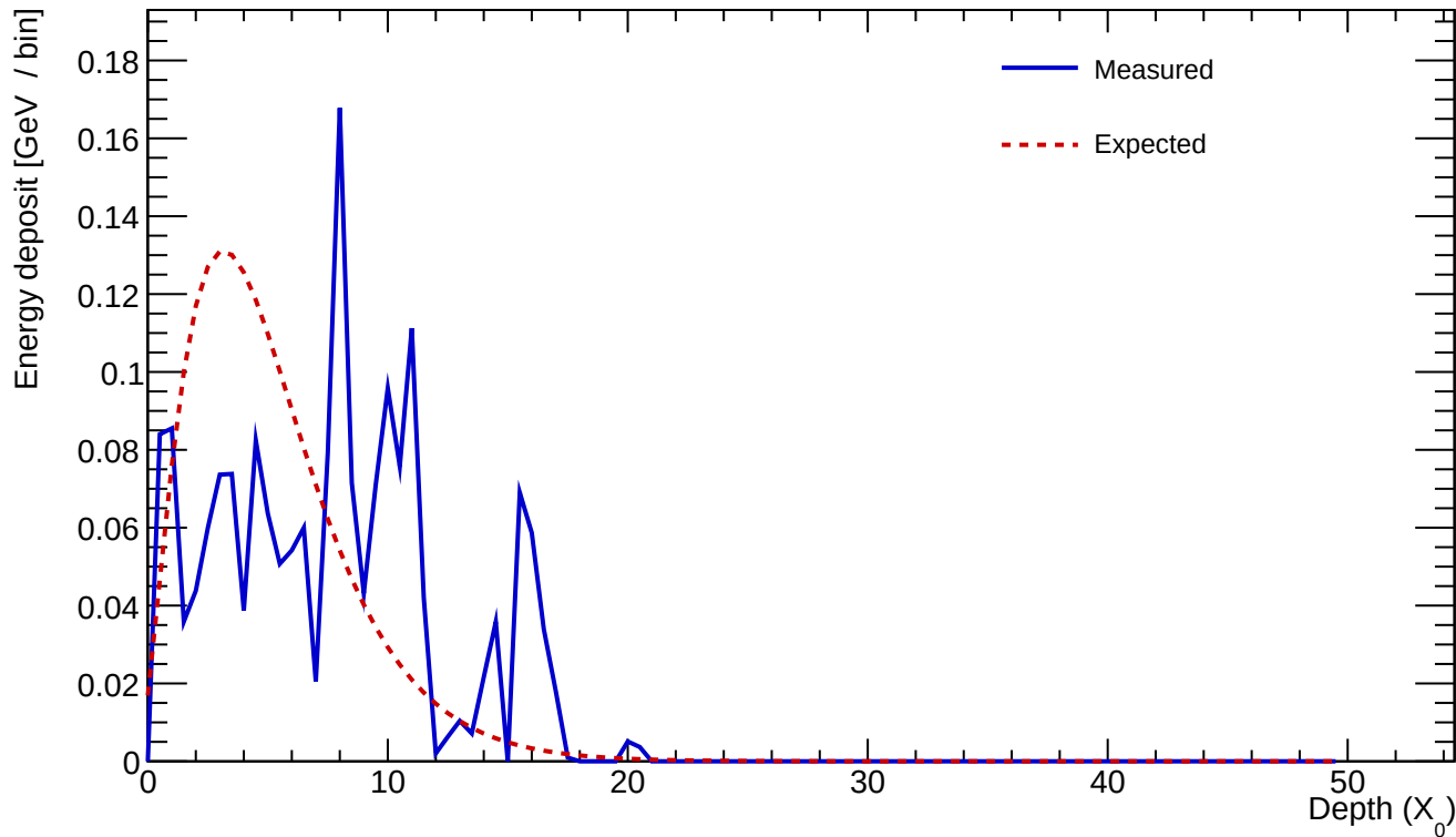
Cluster 565 E=1.857 GeV profileStart=1.50 X_0 \chi=0.7136
