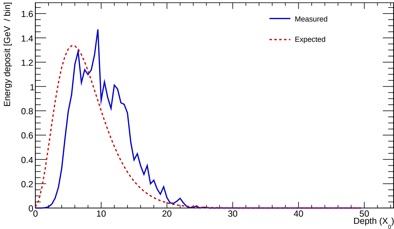
Cluster 385 E=24.286 GeV profileStart=2.50 X_0 \chi=0.1580
