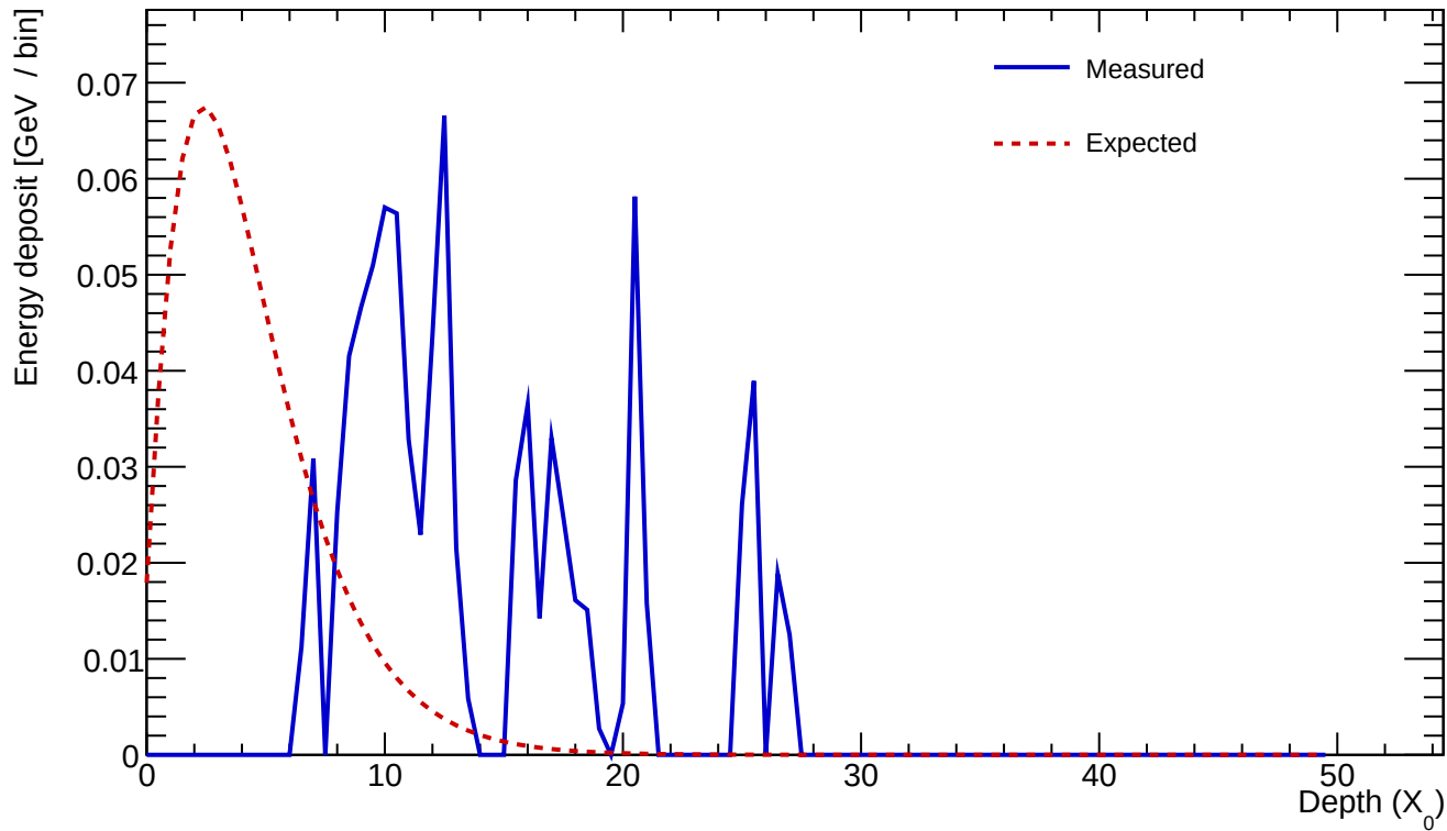
Cluster 530 E=0.860 GeV profileStart=8.00 X_0 \chi=0.6810
