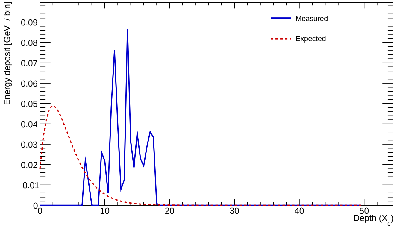
Cluster 234 E=0.586 GeV profileStart=9.50 X_0 \chi=0.5525
