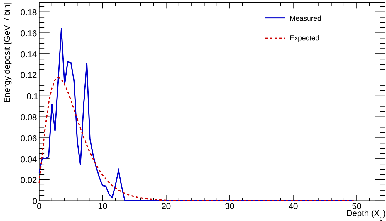
Cluster 1014 E=1.639 GeV profileStart=0.50 X_0 \chi=0.3111
