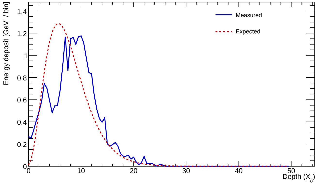
Cluster 450 E=23.314 GeV profileStart=1.50 X_0 \chi=0.3190
