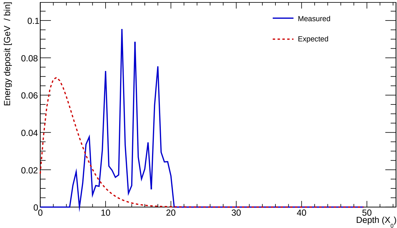
Cluster 206 E=0.889 GeV profileStart=9.00 X_0 \chi=0.8424
