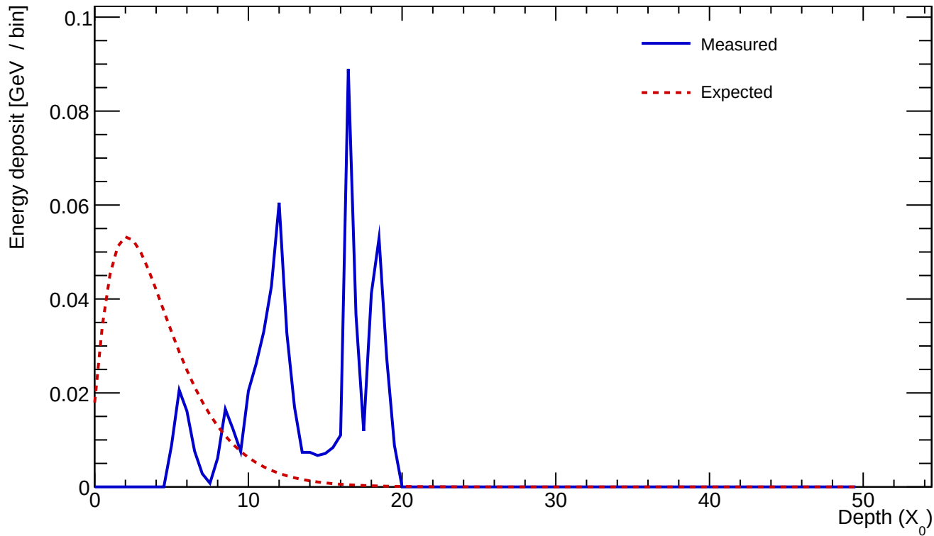
Cluster 231 E=0.648 GeV profileStart=10.00 X_0 \chi=0.8230
