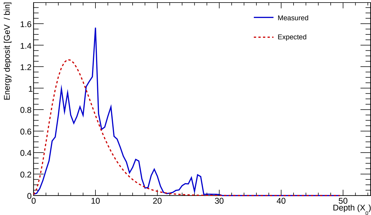
Cluster 646 E=22.881 GeV profileStart=1.00 X_0 \chi=0.3213
