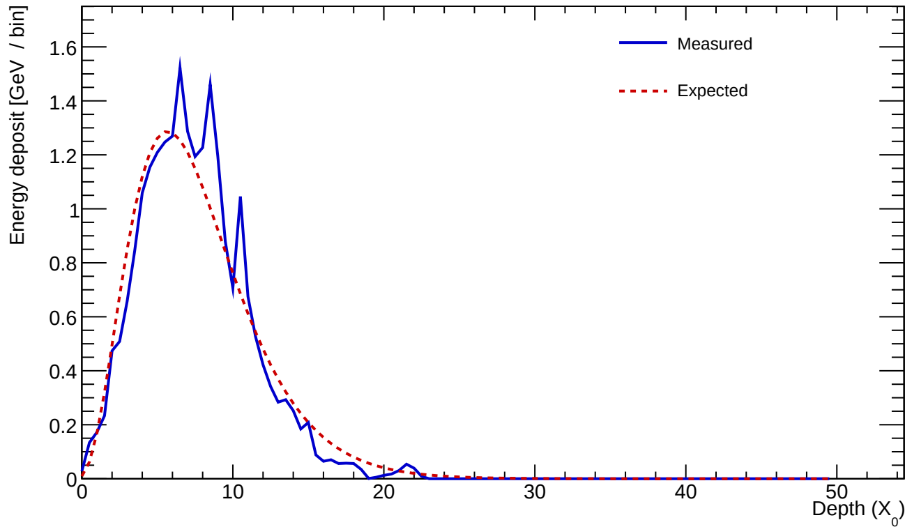
Cluster 888 E=23.291 GeV profileStart=0.50 X_0 \chi=0.1533
