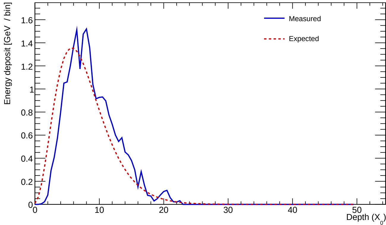
Cluster 436 E=24.652 GeV profileStart=1.00 X_0 \chi=0.1234
