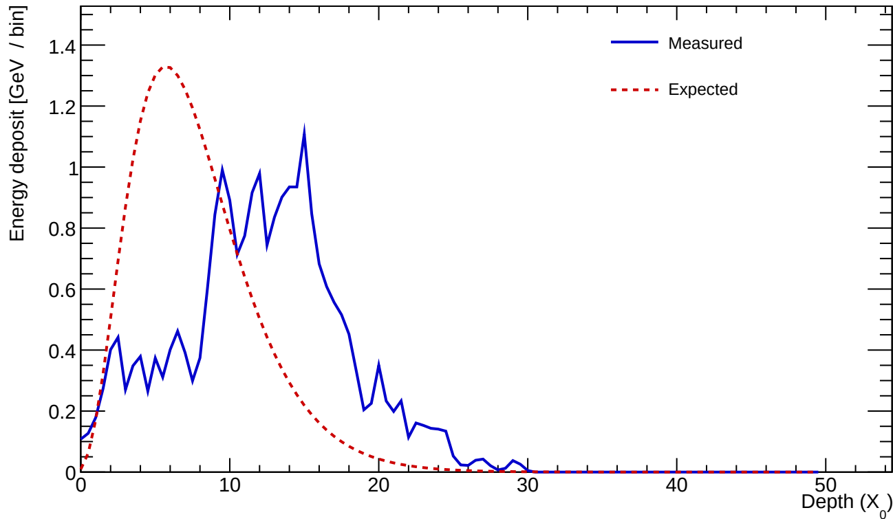
Cluster 293 E=24.145 GeV profileStart=6.00 X_0 \chi=0.4131
