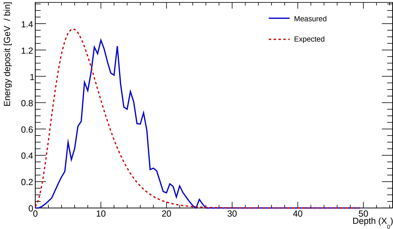
Cluster 686 E=24.735 GeV profileStart=4.00 X_0 \chi=0.2096
