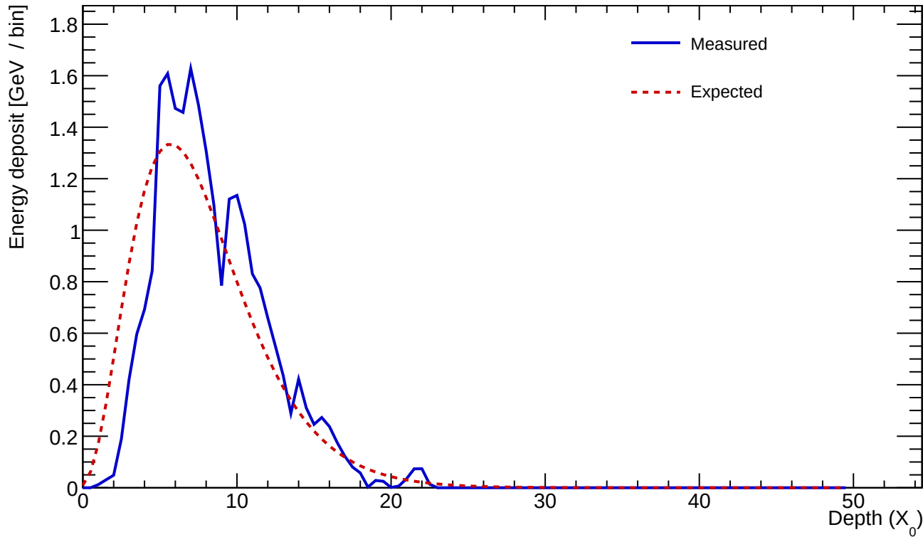
Cluster 402 E=24.241 GeV profileStart=1.00 X_0 \chi=0.1779
