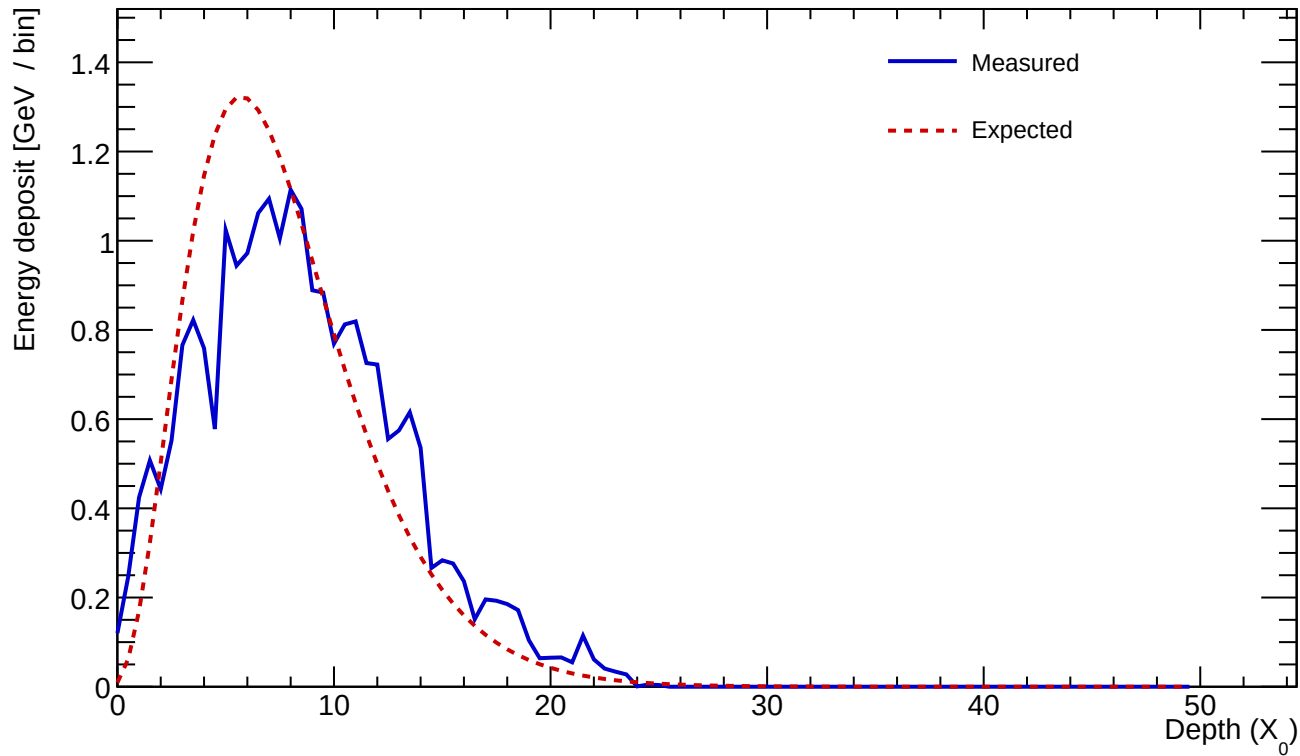
Cluster 921 E=24.009 GeV profileStart=0.50 X_0 \chi=0.2497
