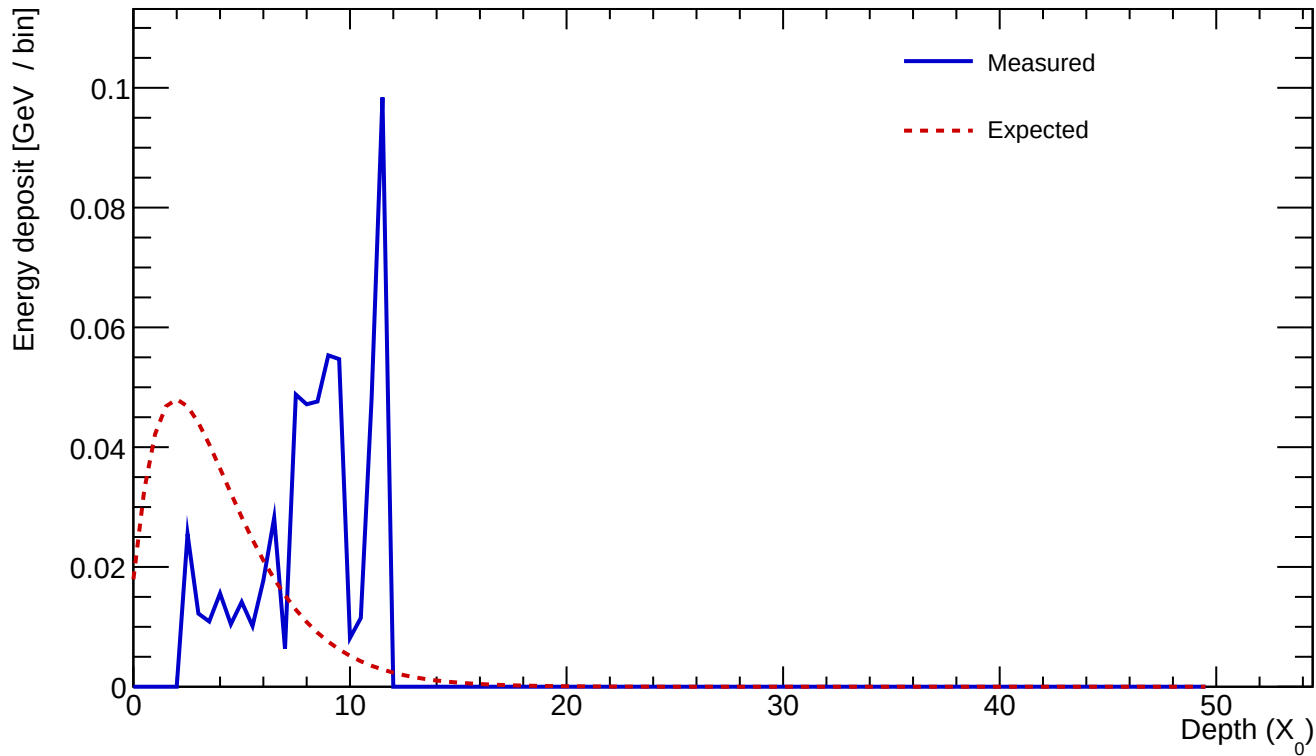
Cluster 149 E=0.571 GeV profileStart=6.00 X_0 \chi=0.4164
