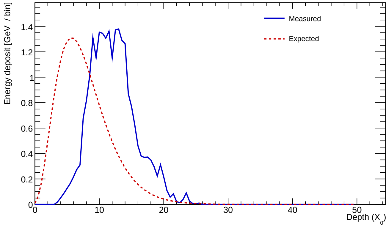
Cluster 174 E=23.759 GeV profileStart=5.00 X_0 \chi=0.1555
