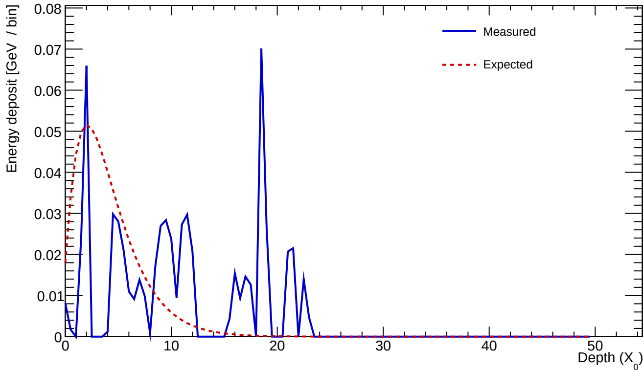
Cluster 396 E=0.622 GeV profileStart=4.00 X_0 \chi=1.0656
