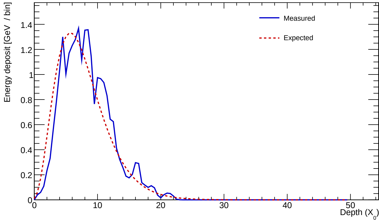
Cluster 339 E=24.160 GeV profileStart=1.00 X_0 \chi=0.1405
