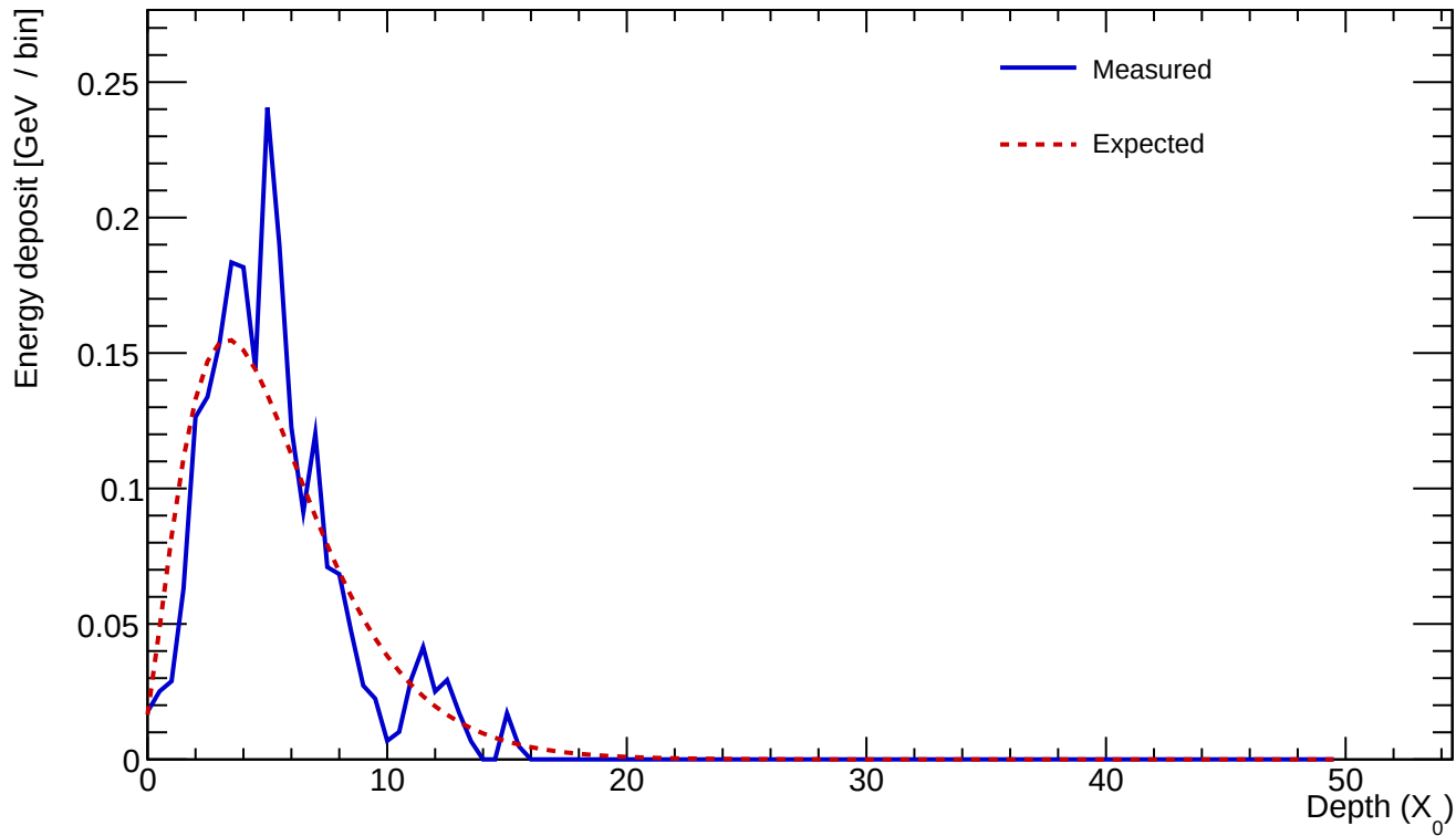
Cluster 38 E=2.247 GeV profileStart=0.50 X_0 \chi=0.2630
