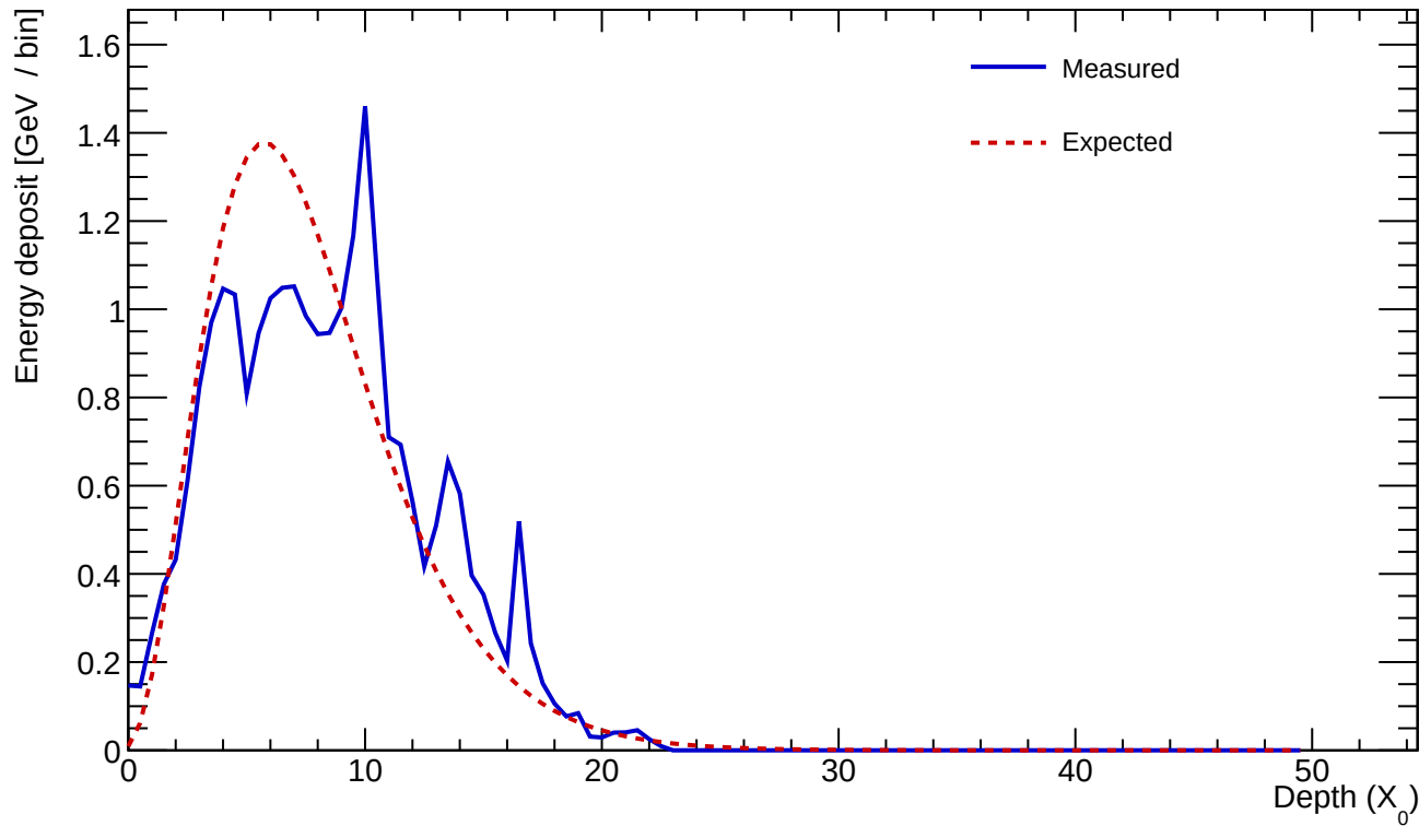
Cluster 40 E=25.068 GeV profileStart=0.50 X_0 \chi=0.2586
