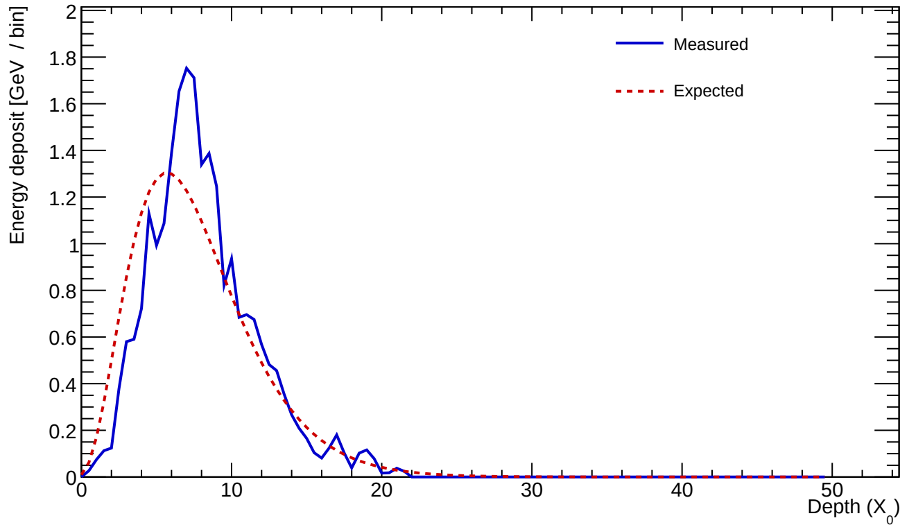
Cluster 850 E=23.630 GeV profileStart=1.00 X_0 \chi=0.1875
