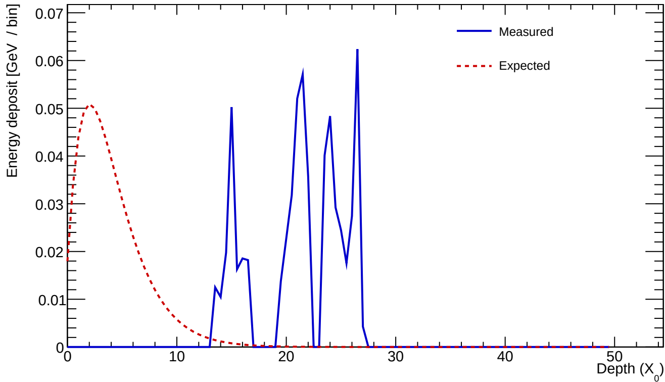
Cluster 216 E=0.613 GeV profileStart=19.50 X_0 \chi=0.5940
