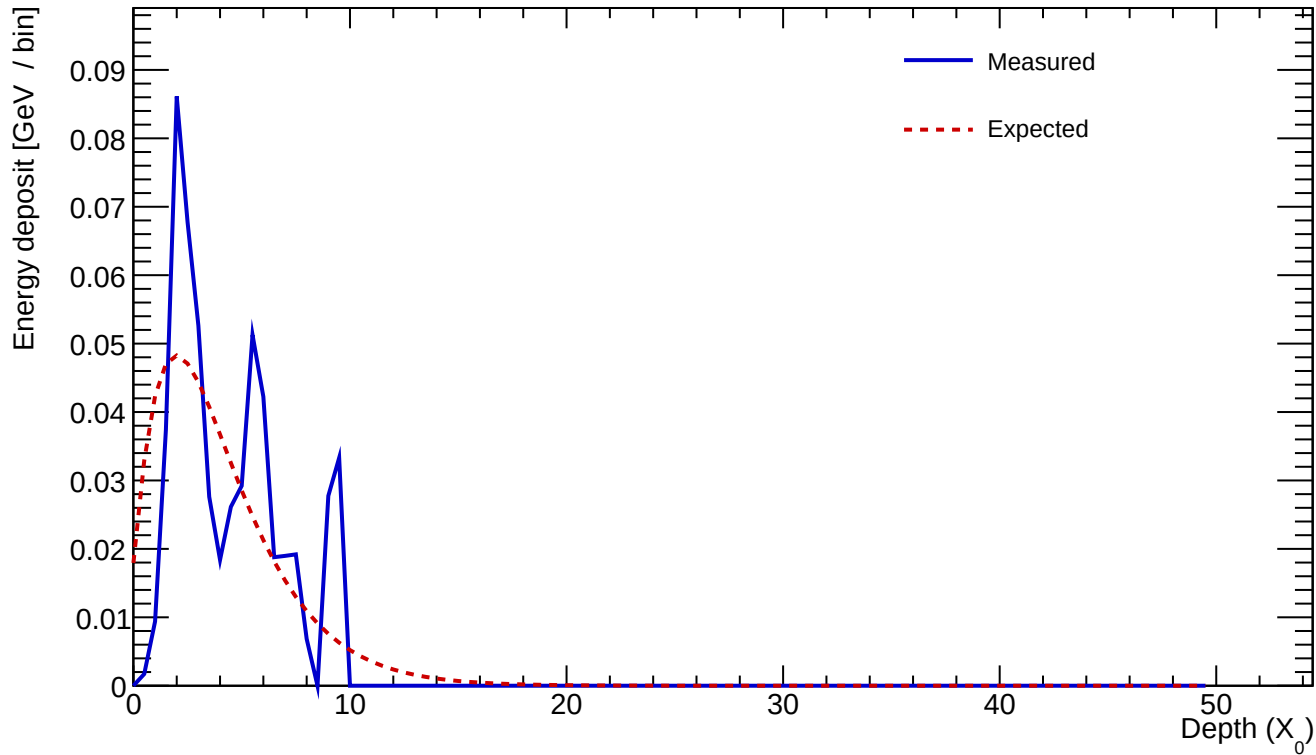
Cluster 972 E=0.575 GeV profileStart=1.00 X_0 \chi=0.4025
