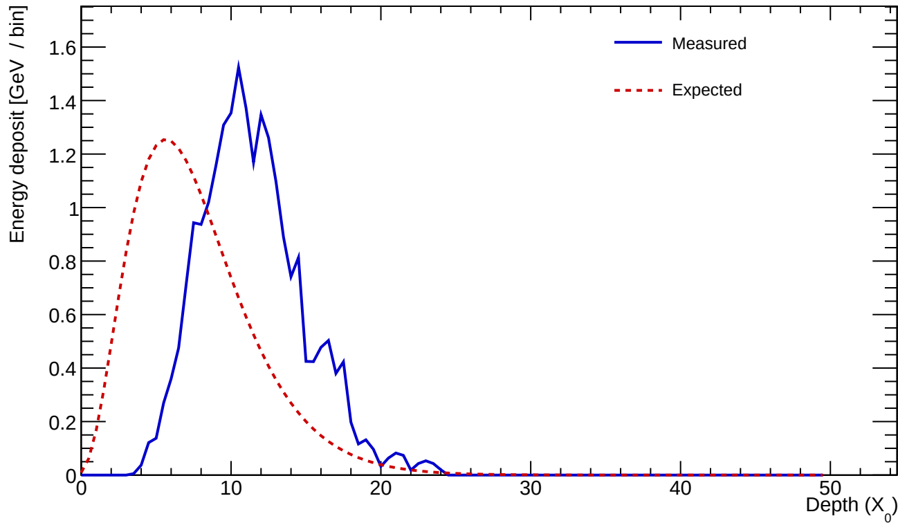
Cluster 45 E=22.659 GeV profileStart=4.50 X_0 \chi=0.1545
