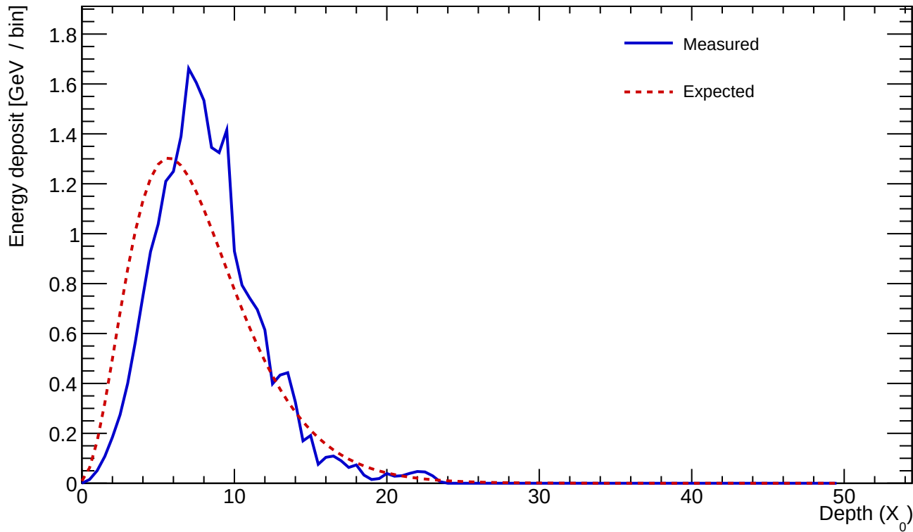
Cluster 348 E=23.636 GeV profileStart=1.00 X_0 \chi=0.1716
