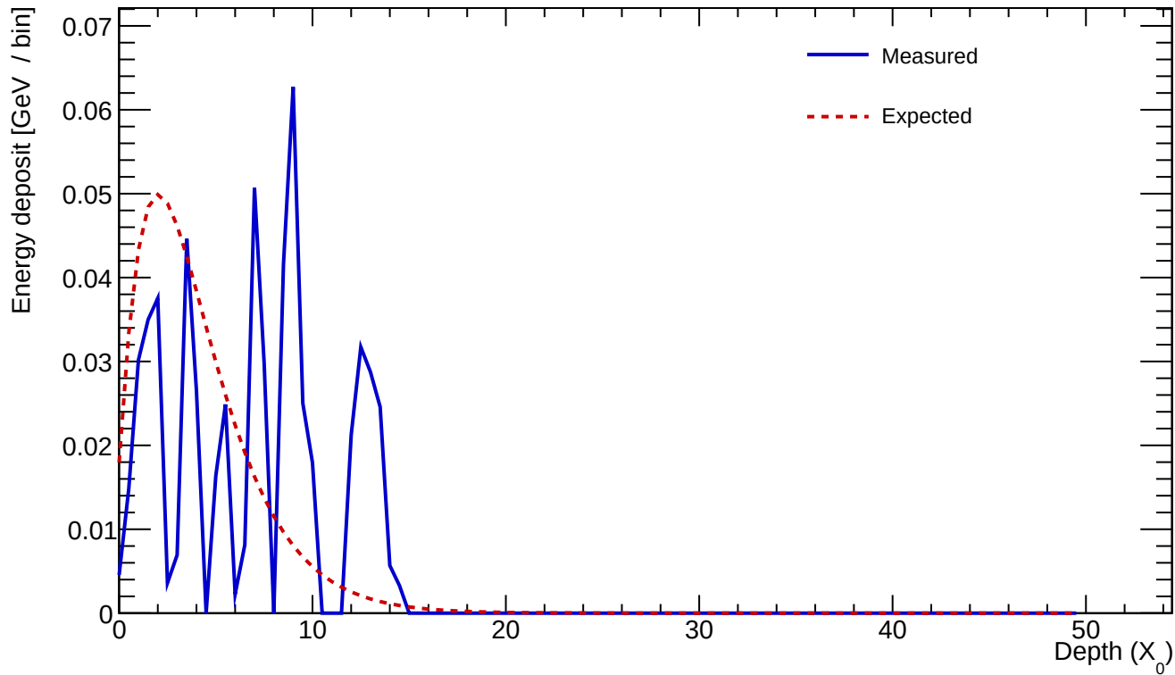
Cluster 194 E=0.598 GeV profileStart=0.50 X_0 \chi=0.8696
