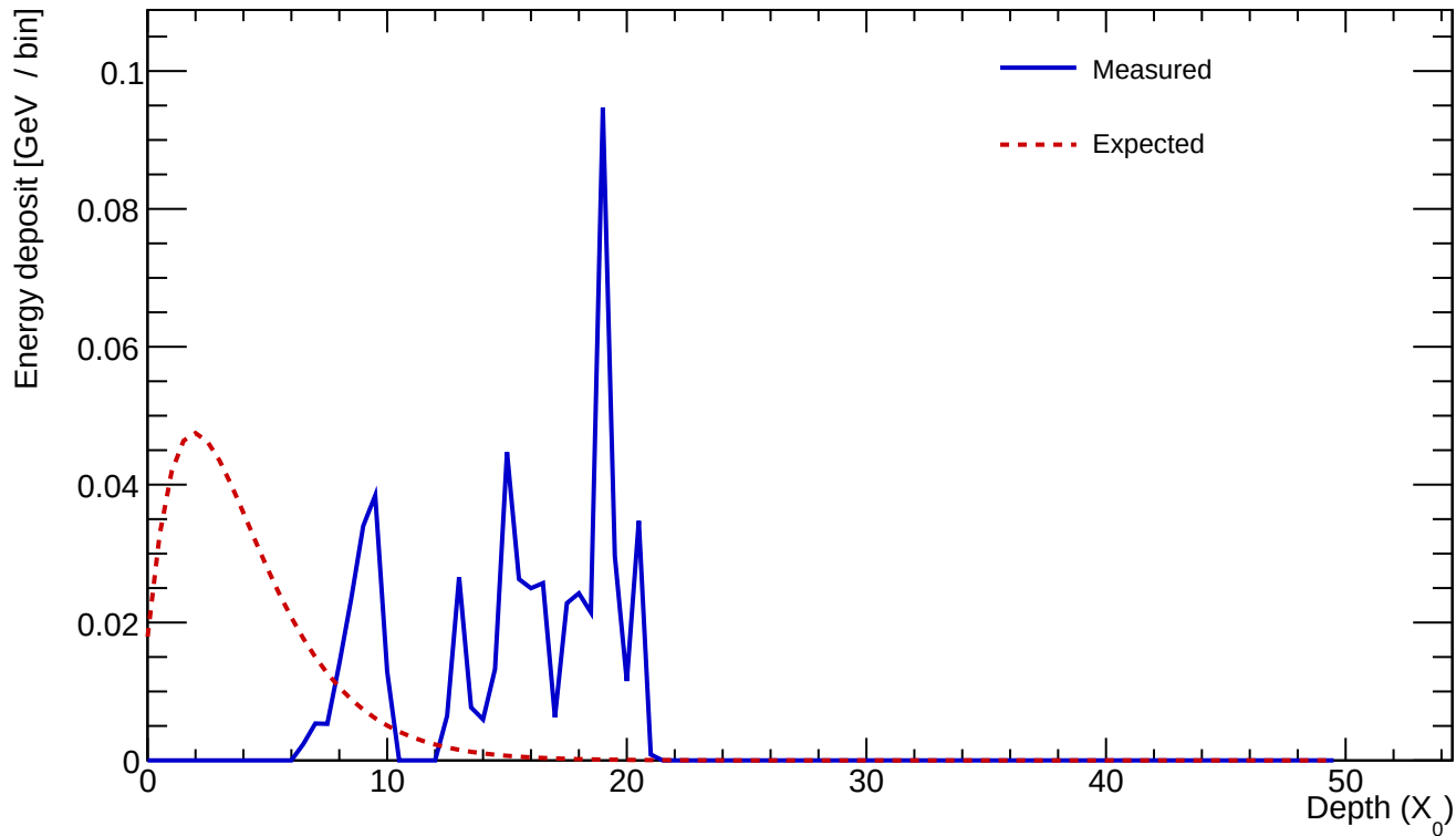
Cluster 383 E=0.564 GeV profileStart=14.50 X_0 \chi=0.7806
