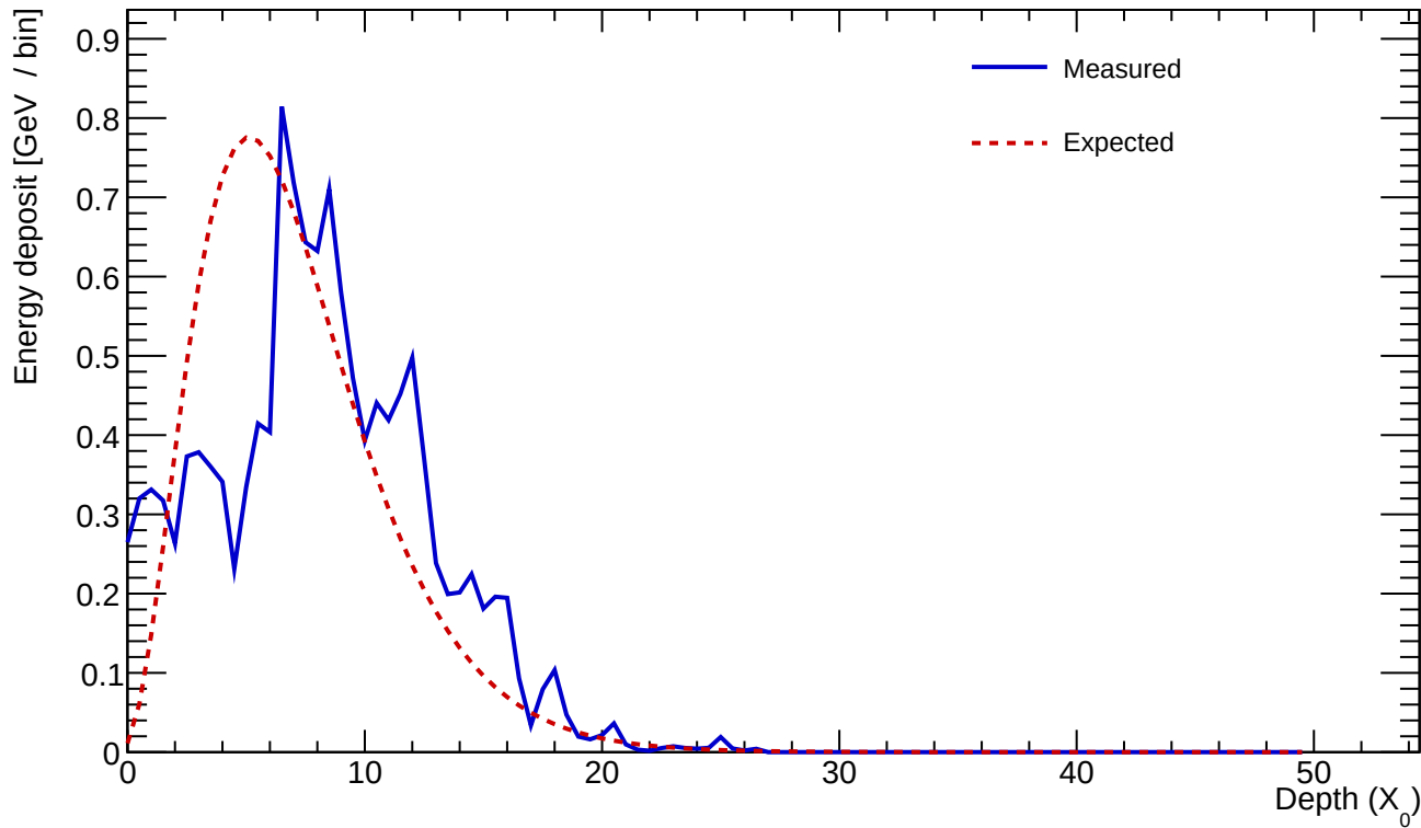
Cluster 314 E=13.436 GeV profileStart=1.00 X_0 \chi=0.3543
