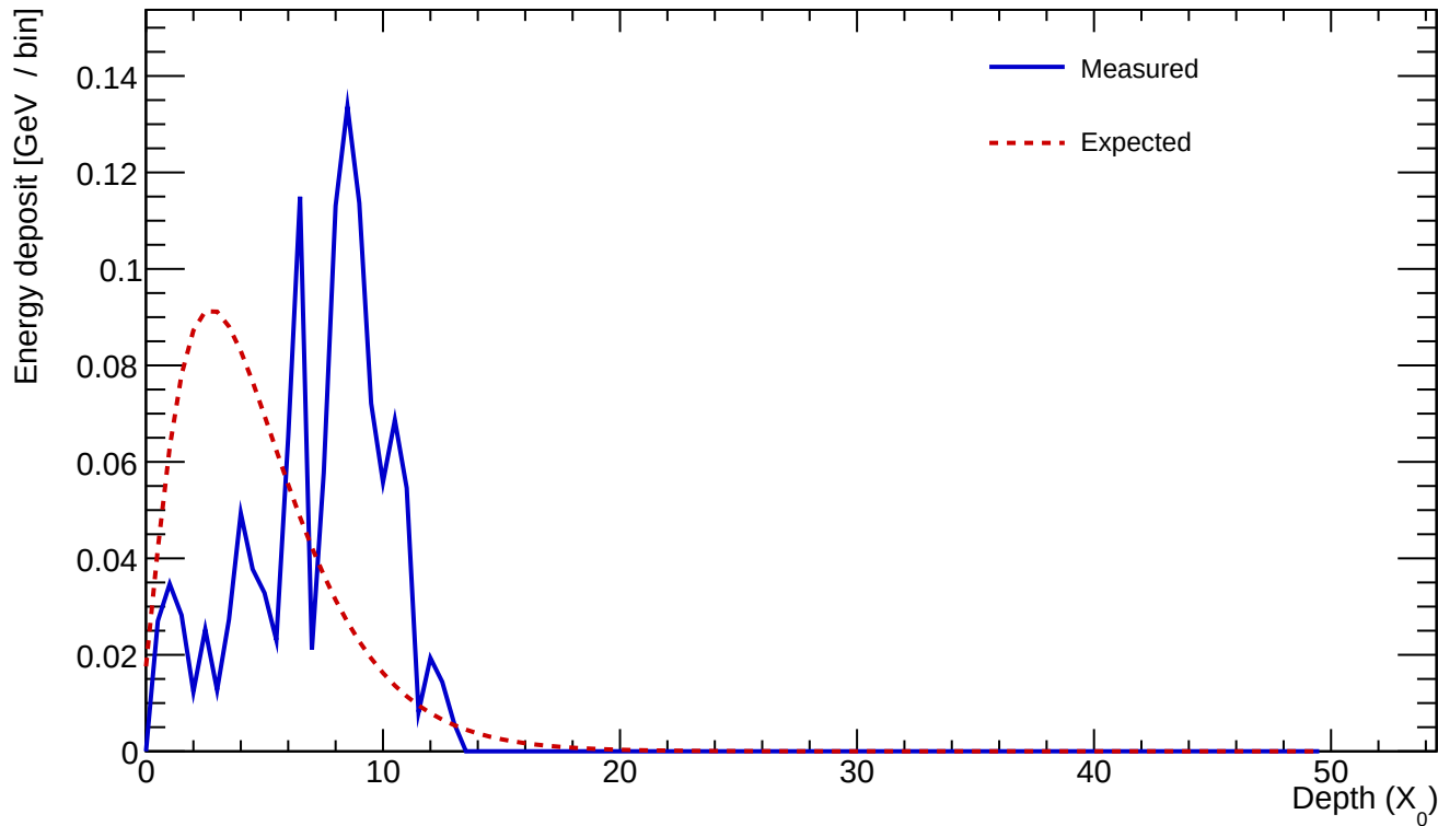
Cluster 1146 E=1.229 GeV profileStart=5.00 X_0 \chi=0.5179
