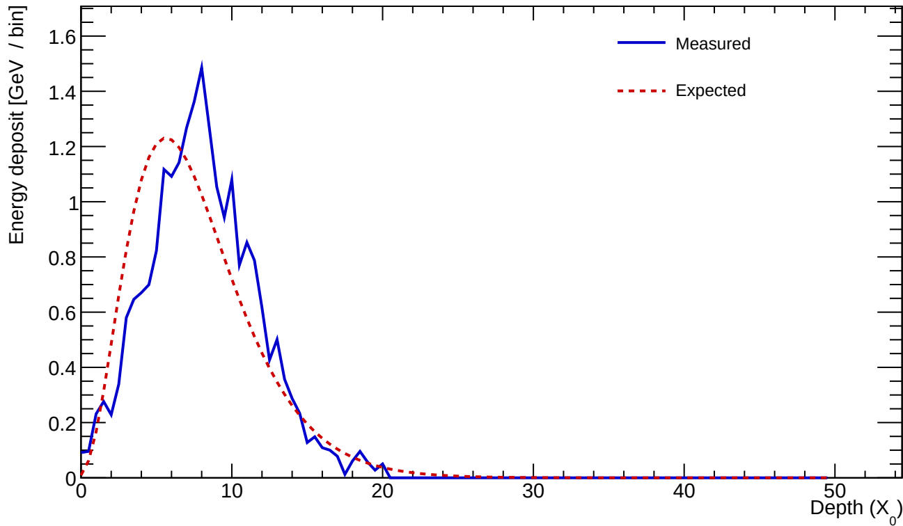
Cluster 598 E=22.195 GeV profileStart=1.00 X_0 \chi=0.1798
