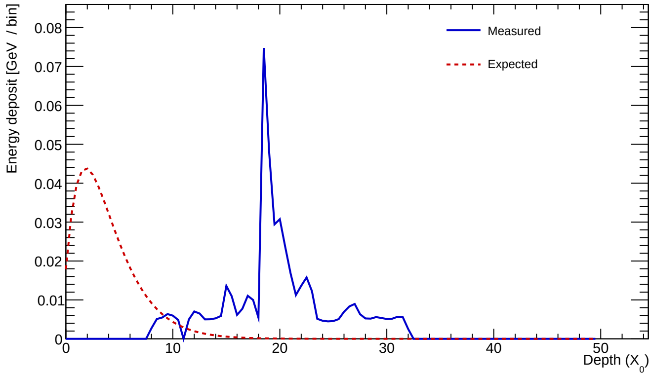
Cluster 262 E=0.511 GeV profileStart=16.50 X_0 \chi=0.7193
