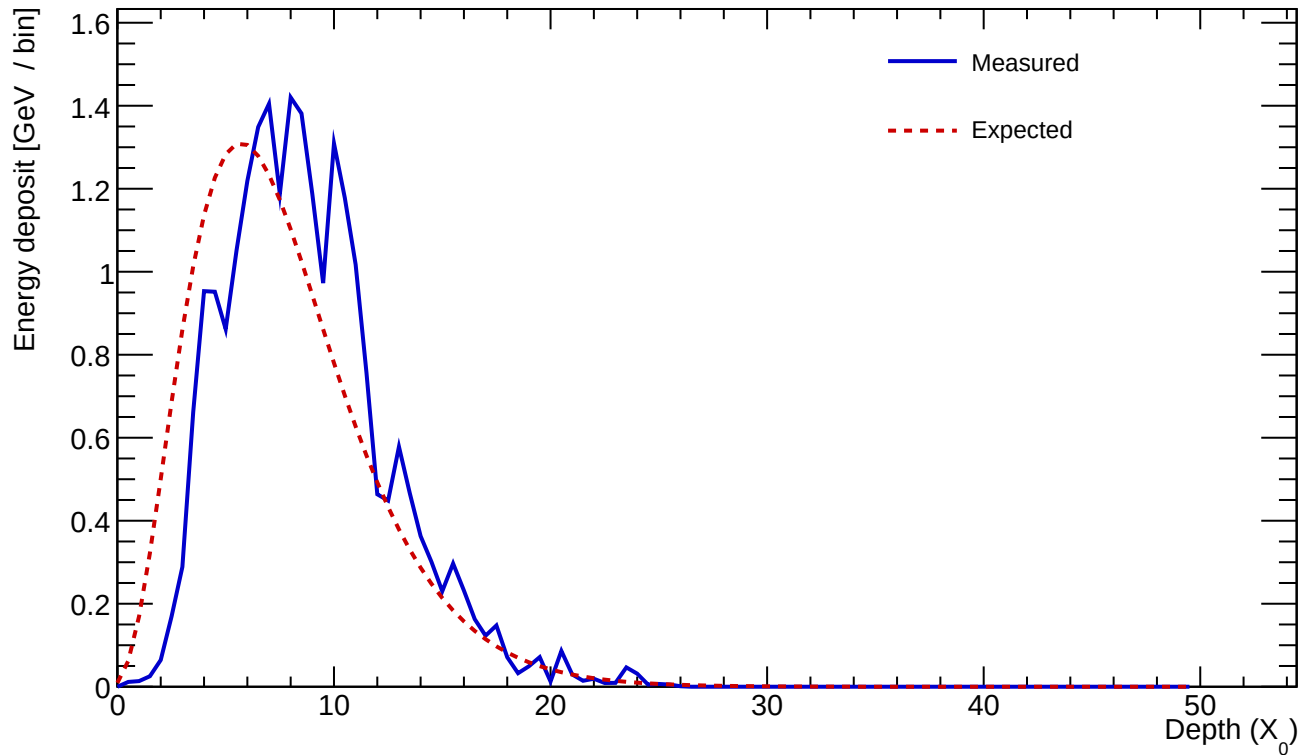
Cluster 367 E=23.748 GeV profileStart=1.50 X_0 \chi=0.1499
