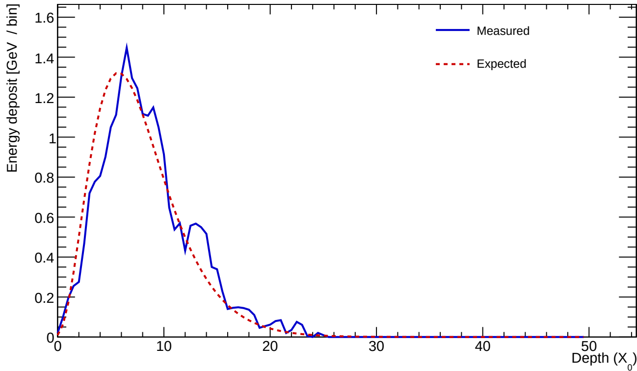
Cluster 303 E=23.973 GeV profileStart=0.50 X_0 \chi=0.1452
