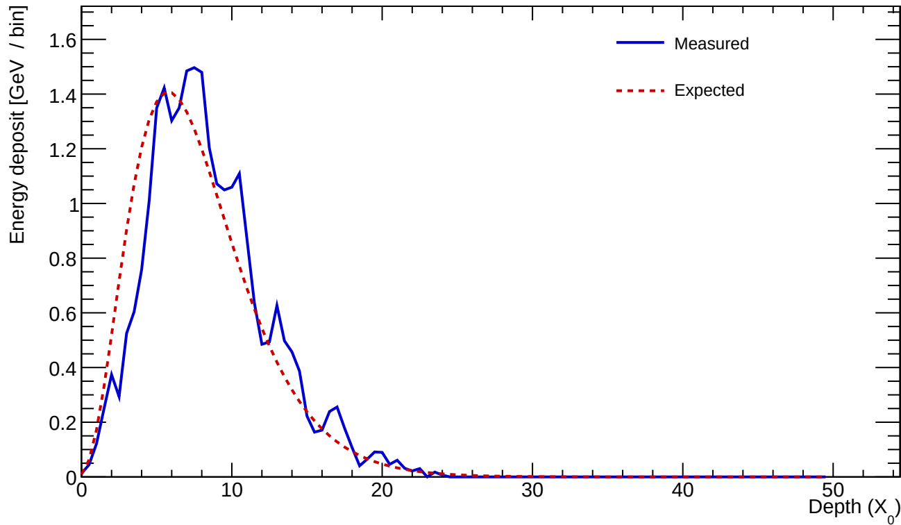
Cluster 728 E=25.666 GeV profileStart=1.00 X_0 \chi=0.1318
