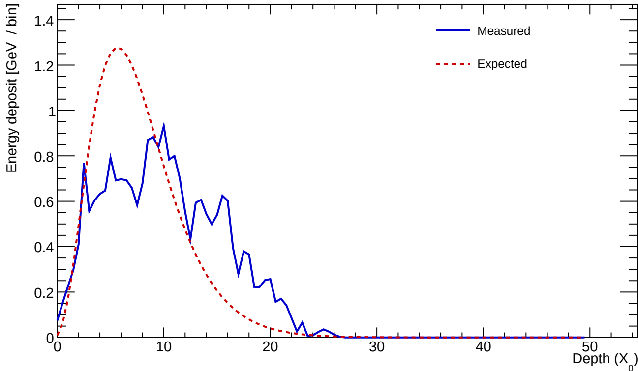
Cluster 531 E=23.103 GeV profileStart=1.50 X_0 \chi=0.4527
