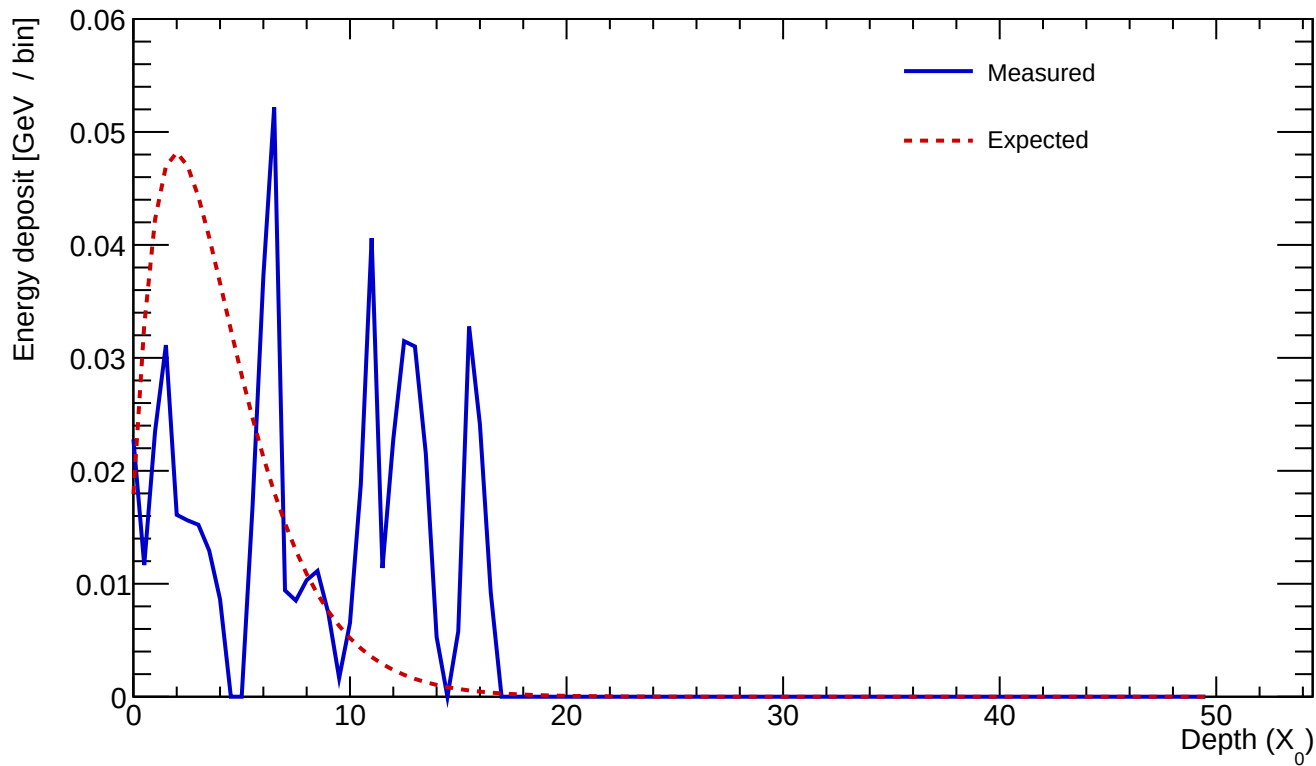
Cluster 674 E=0.574 GeV profileStart=15.50 X_0 \chi=0.9259
