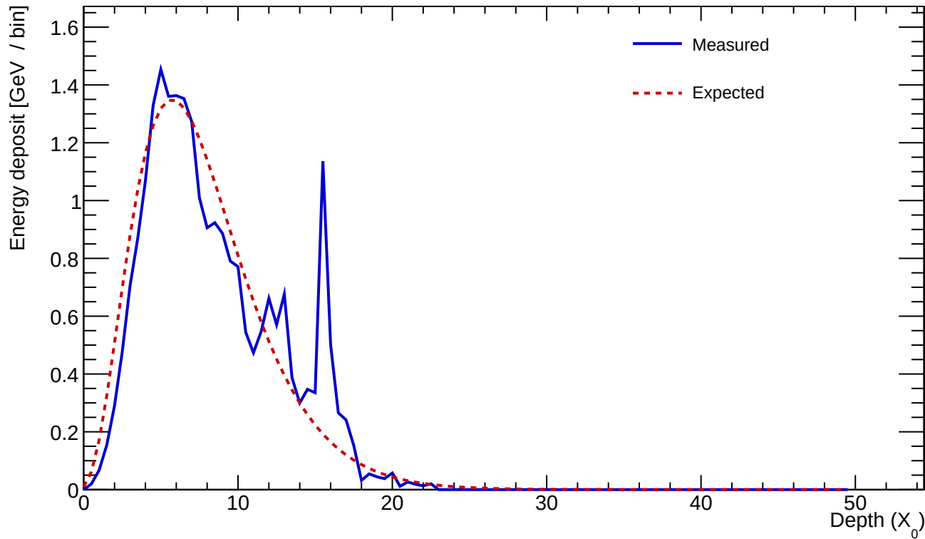
Cluster 53 E=24.523 GeV profileStart=0.50 X_0 \chi=0.1935
