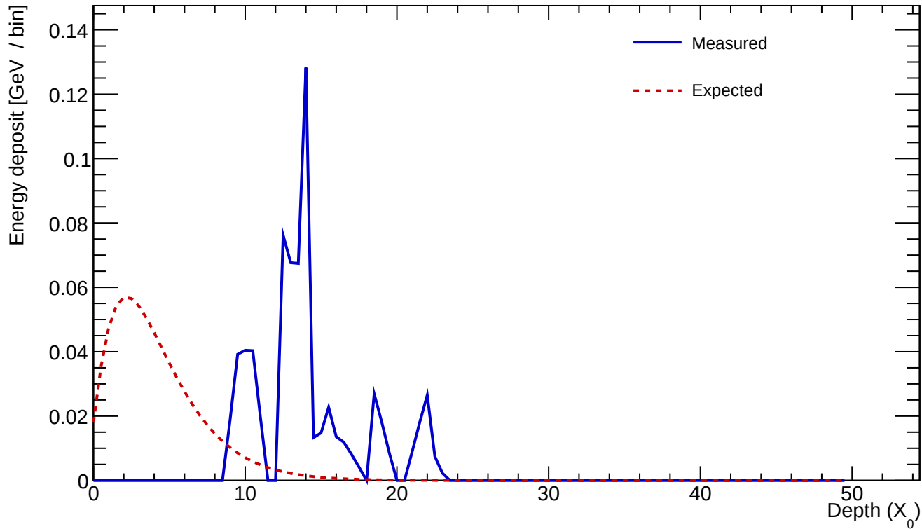
Cluster 356 E=0.703 GeV profileStart=9.00 X_0 \chi=0.7105
