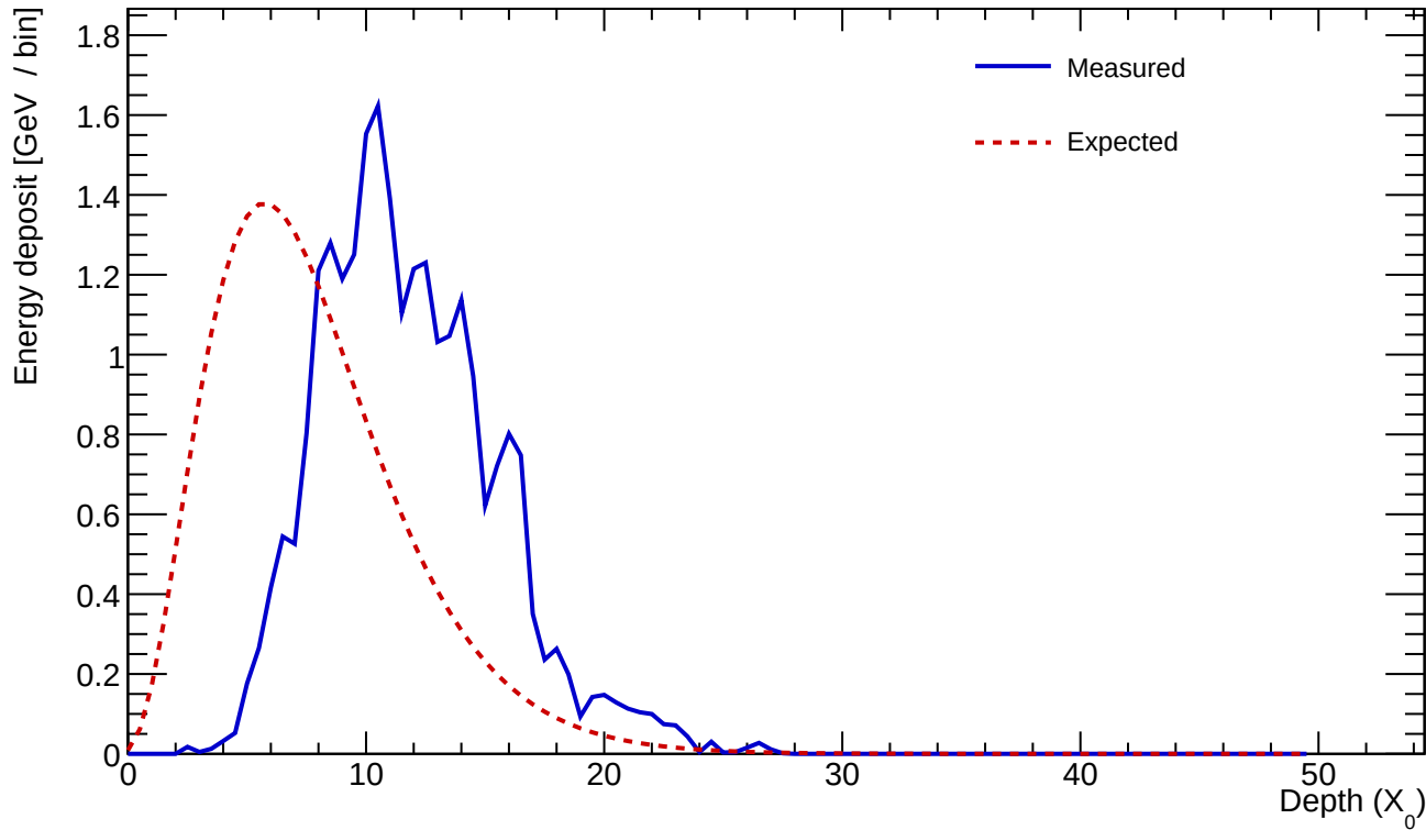
Cluster 212 E=25.118 GeV profileStart=4.50 X_0 \chi=0.1603
