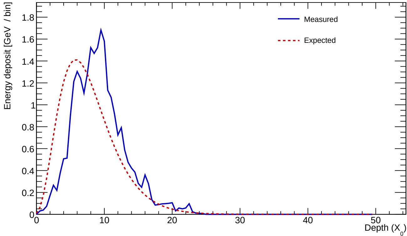
Cluster 405 E=25.754 GeV profileStart=2.00 X_0 \chi=0.1658
