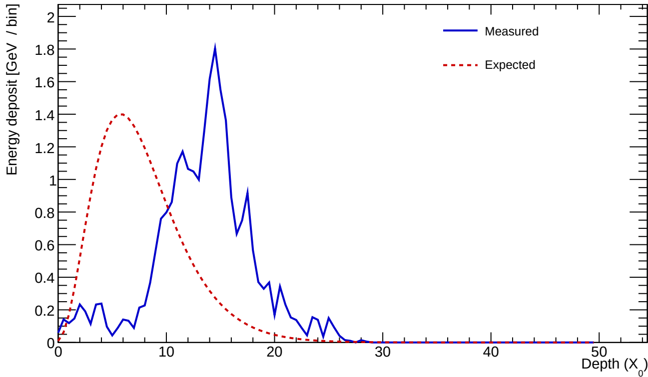
Cluster 870 E=25.545 GeV profileStart=7.00 X_0 \chi=0.3120
