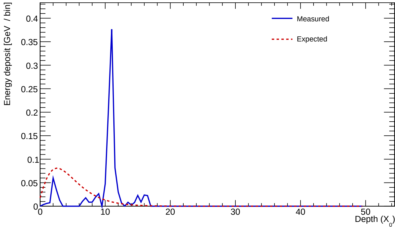
Cluster 1098 E=1.064 GeV profileStart=8.50 X_0 \chi=0.9961
