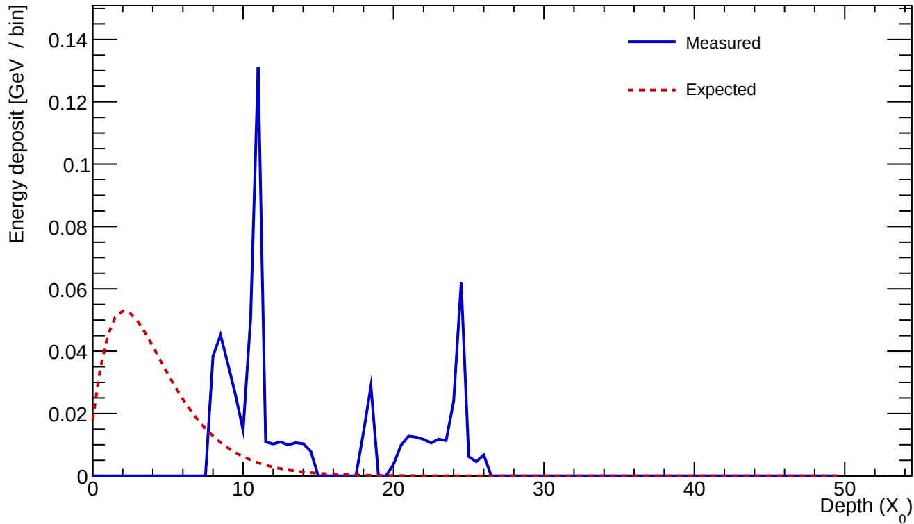
Cluster 452 E=0.643 GeV profileStart=7.50 X_0 \chi=0.9195
