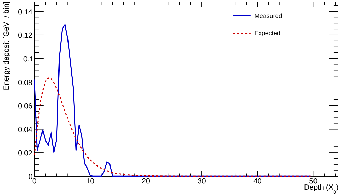
Cluster 800 E=1.104 GeV profileStart=2.00 X_0 \chi=0.6549
