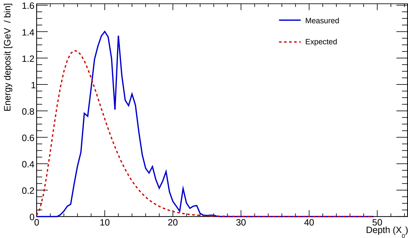
Cluster 330 E=22.714 GeV profileStart=4.50 X_0 \chi=0.1489
