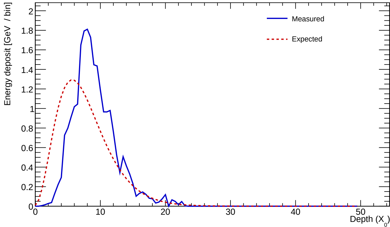
Cluster 372 E=23.417 GeV profileStart=2.00 X_0 \chi=0.2322
