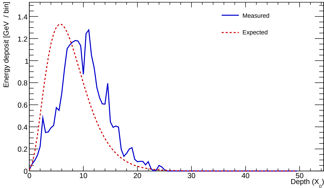
Cluster 735 E=24.171 GeV profileStart=3.00 X_0 \chi=0.2147
