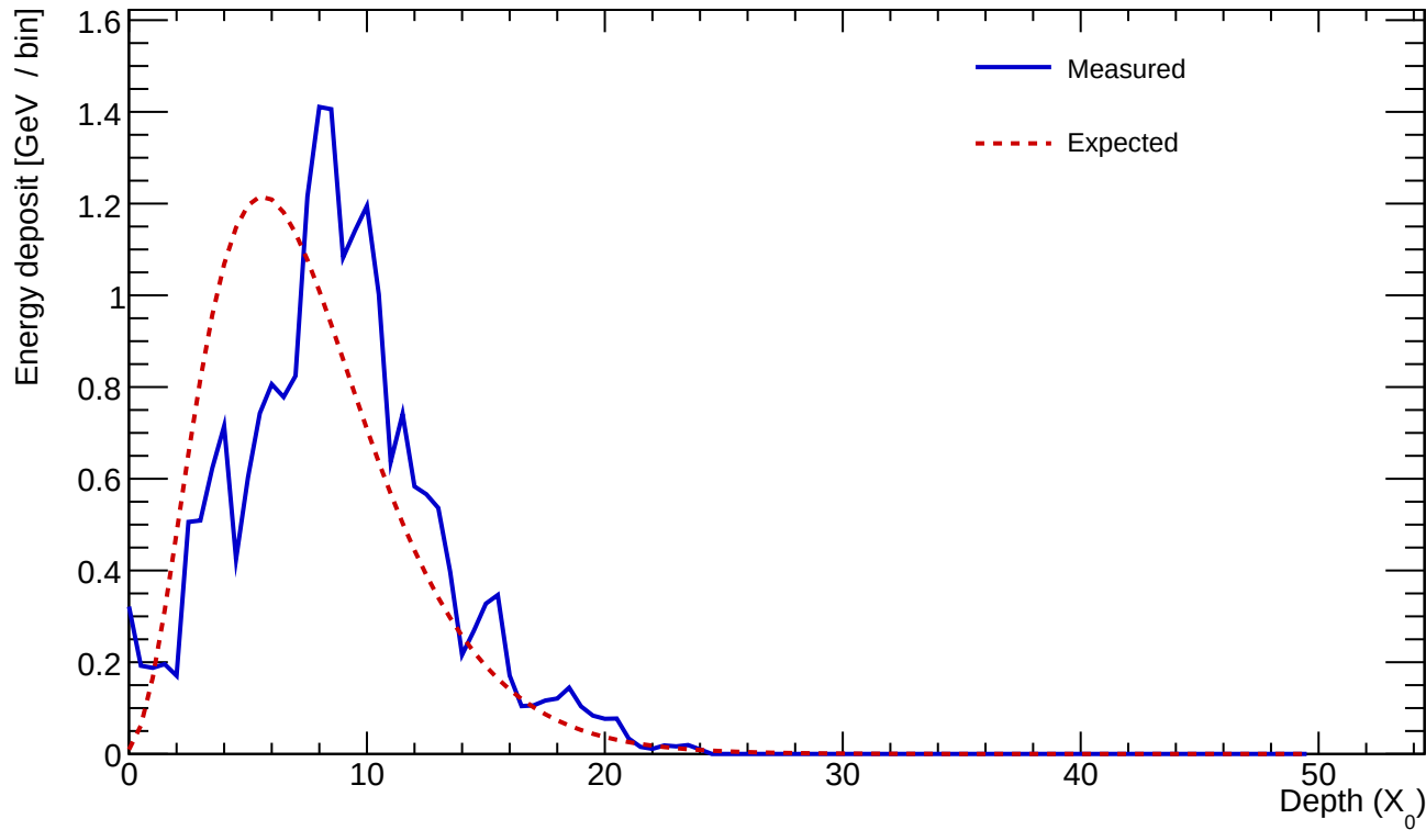
Cluster 947 E=21.902 GeV profileStart=1.50 X_0 \chi=0.2774
