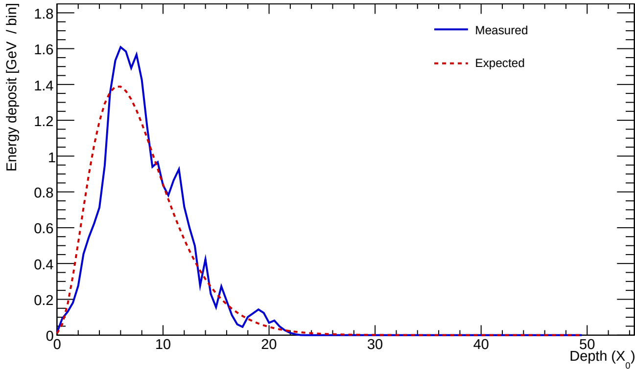
Cluster 346 E=25.337 GeV profileStart=1.00 X_0 \chi=0.1729
