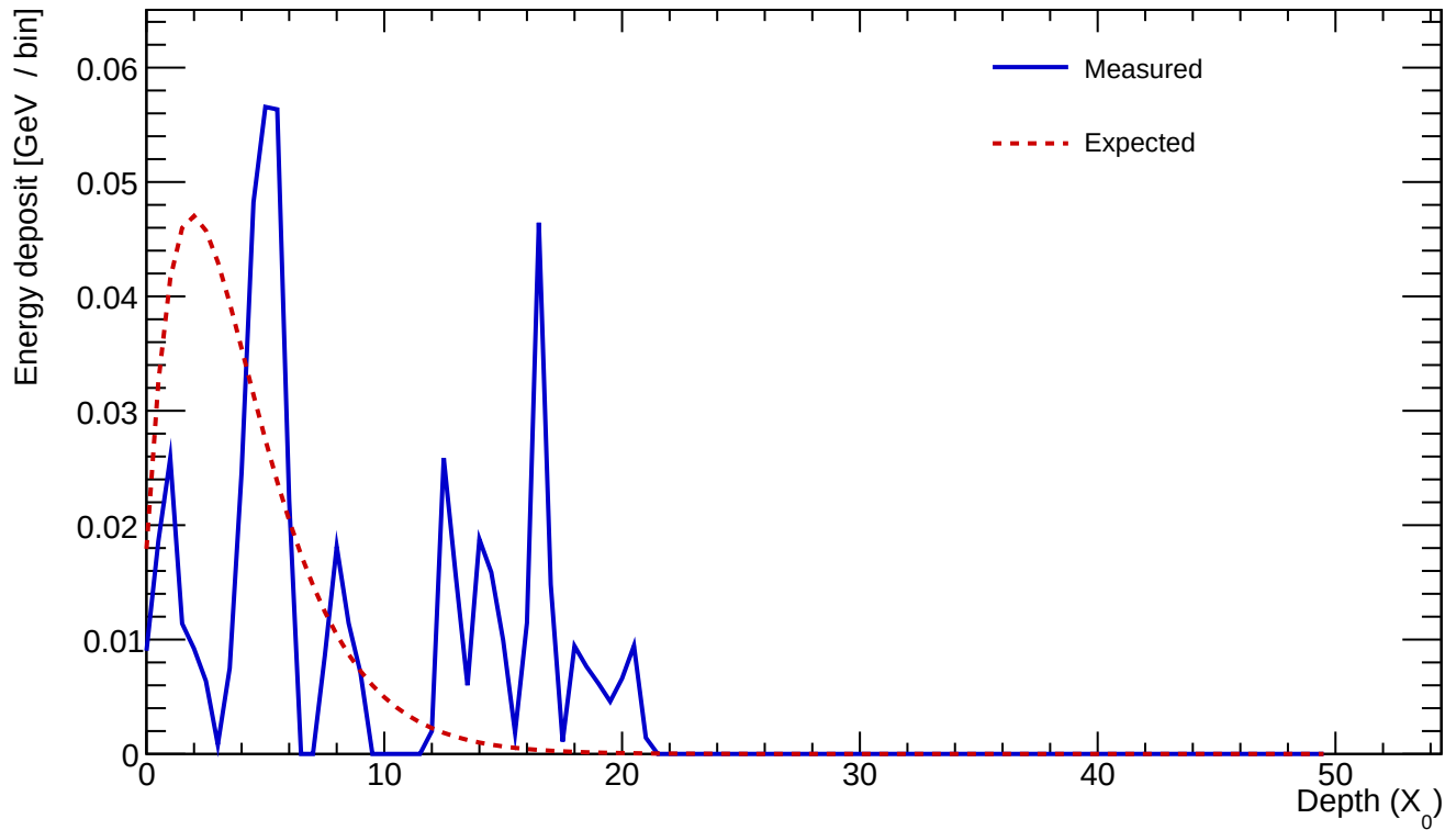
Cluster 175 E=0.557 GeV profileStart=3.50 X_0 \chi=1.0059
