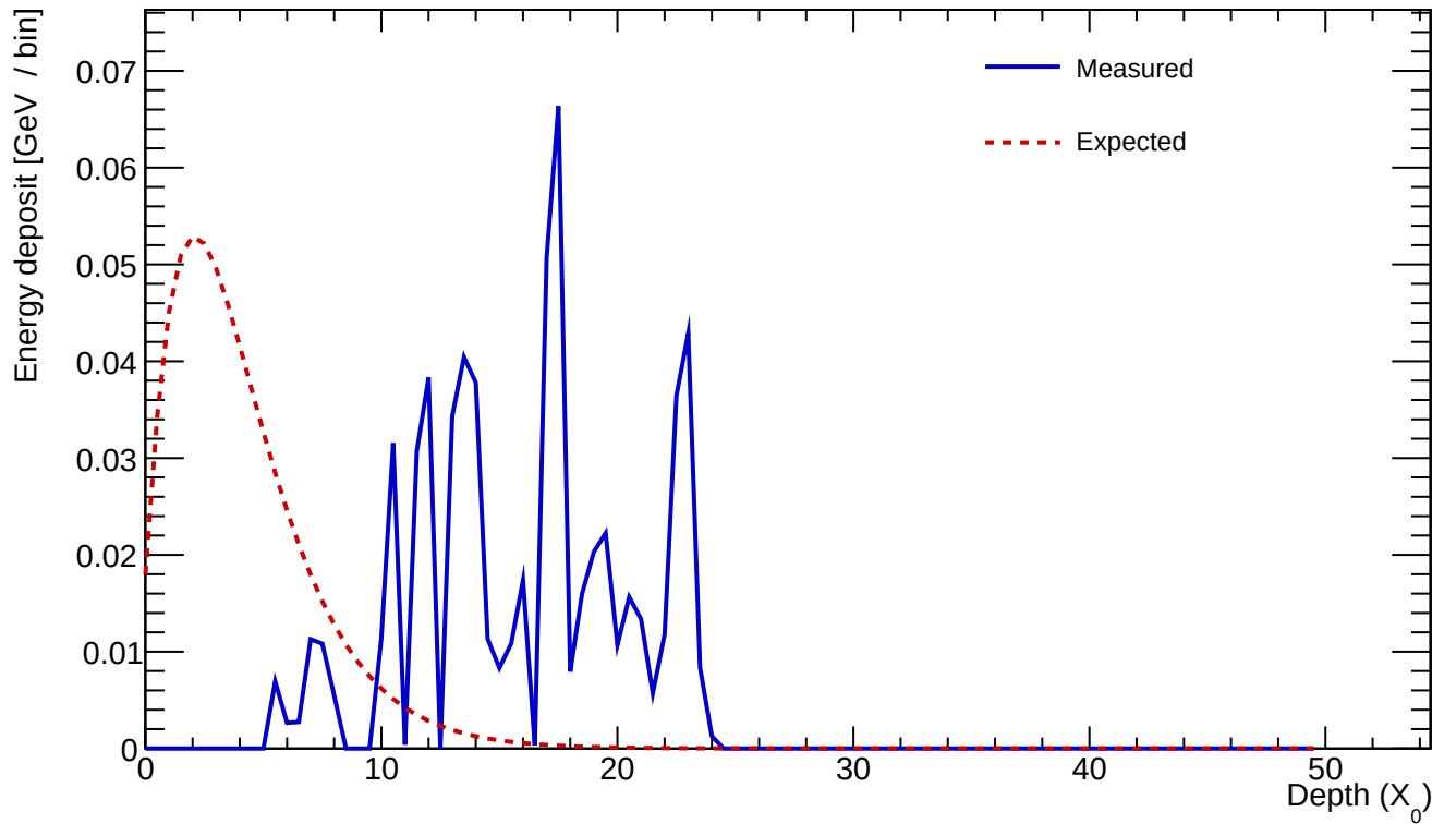
Cluster 118 E=0.643 GeV profileStart=11.50 X_0 \chi=0.8366
