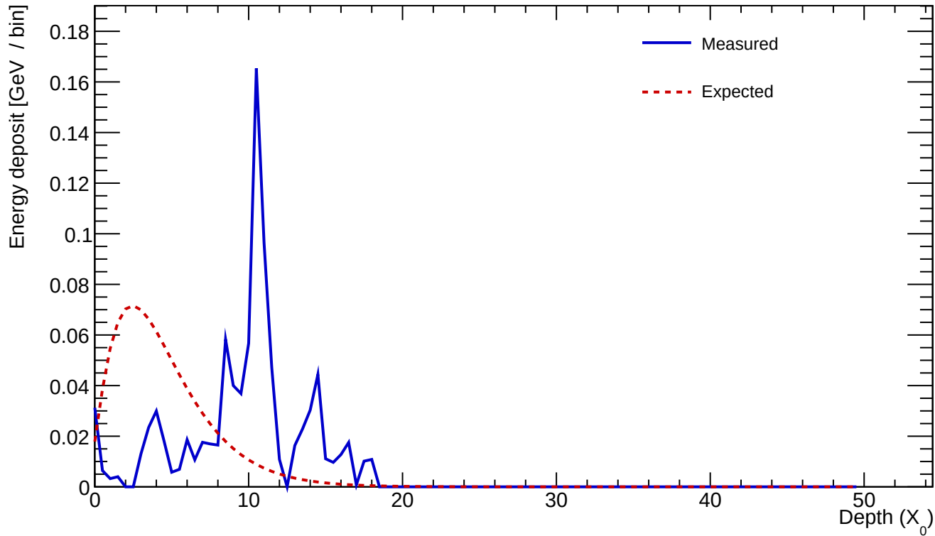
Cluster 119 E=0.921 GeV profileStart=7.50 X_0 \chi=0.6860
