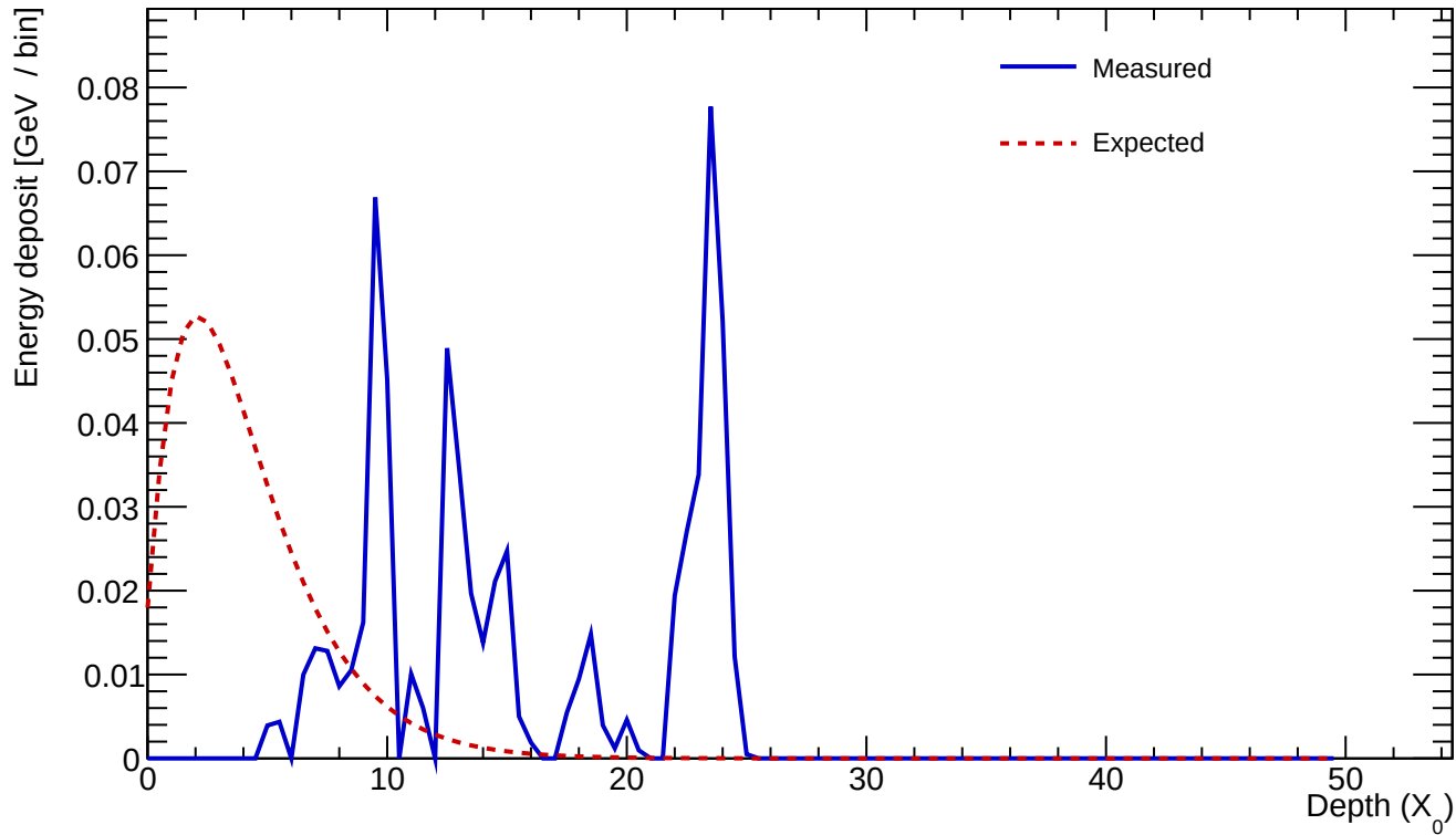
Cluster 645 E=0.641 GeV profileStart=8.00 X_0 \chi=0.9752
