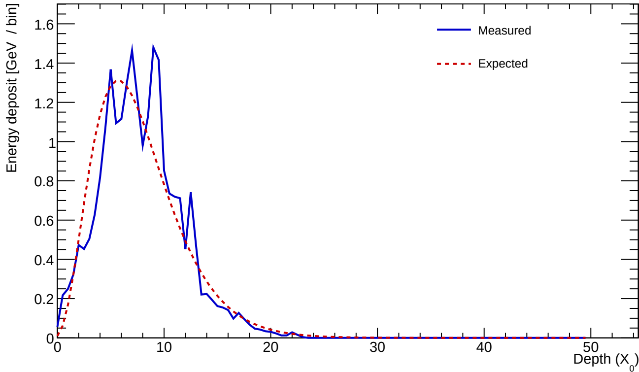
Cluster 370 E=23.773 GeV profileStart=0.50 X_0 \chi=0.1996
