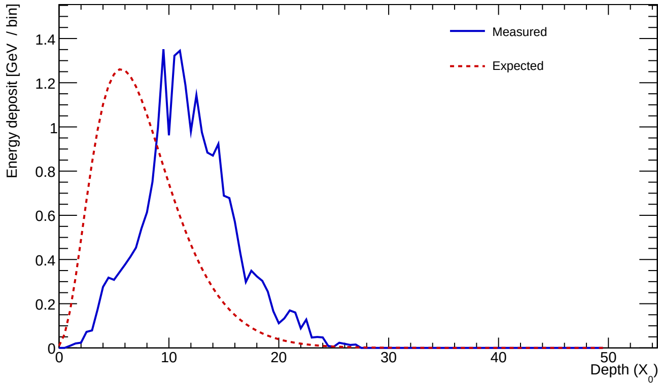
Cluster 159 E=22.795 GeV profileStart=5.00 X_0 \chi=0.2058
