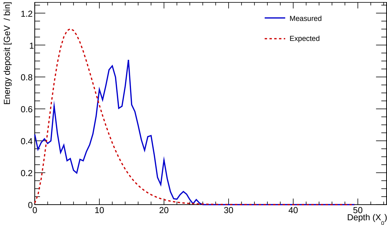
Cluster 219 E=19.683 GeV profileStart=5.50 X_0 \chi=0.5264
