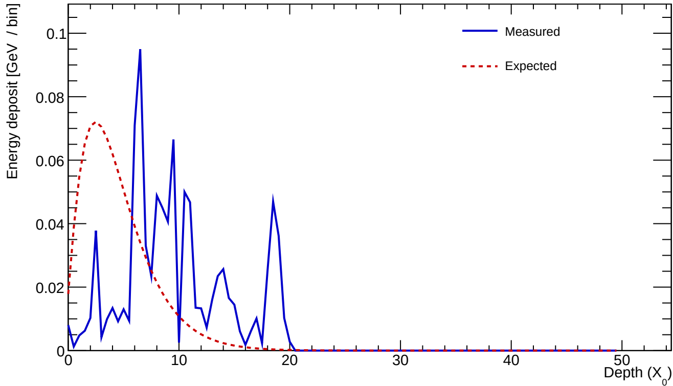
Cluster 923 E=0.929 GeV profileStart=5.00 X_0 \chi=0.6609
