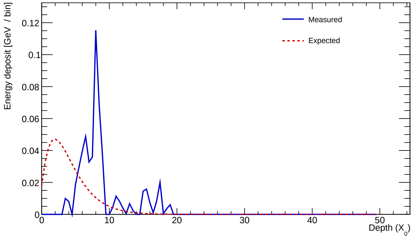
Cluster 508 E=0.558 GeV profileStart=5.00 X_0 \chi=0.6289
