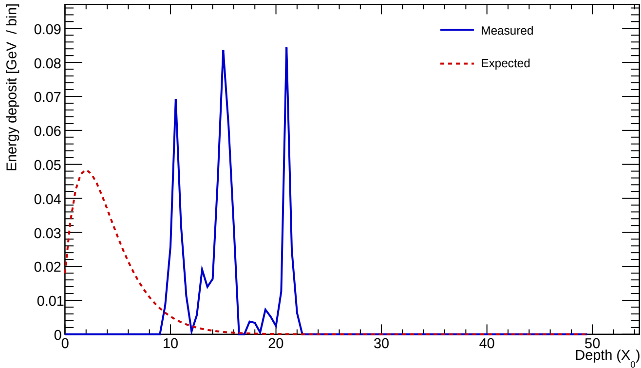
Cluster 341 E=0.577 GeV profileStart=9.50 X_0 \chi=0.9309
