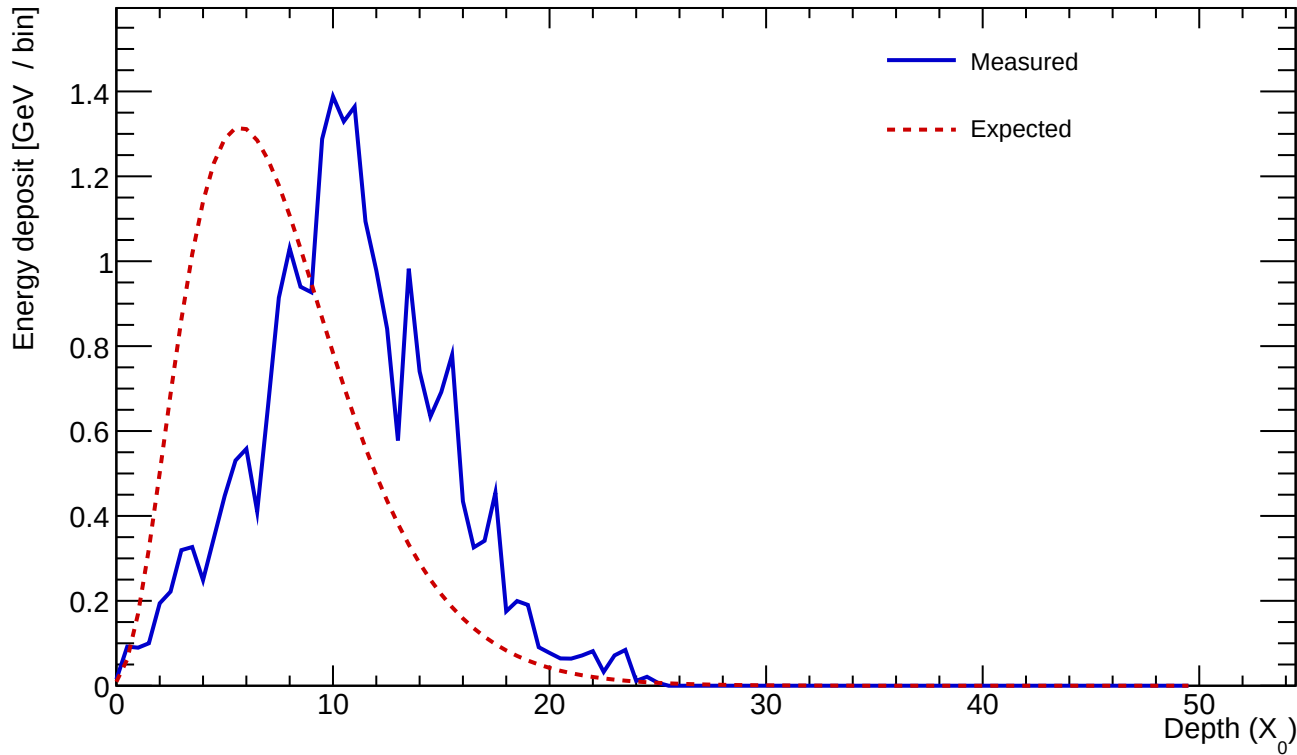
Cluster 924 E=23.858 GeV profileStart=3.50 X_0 \chi=0.2586
