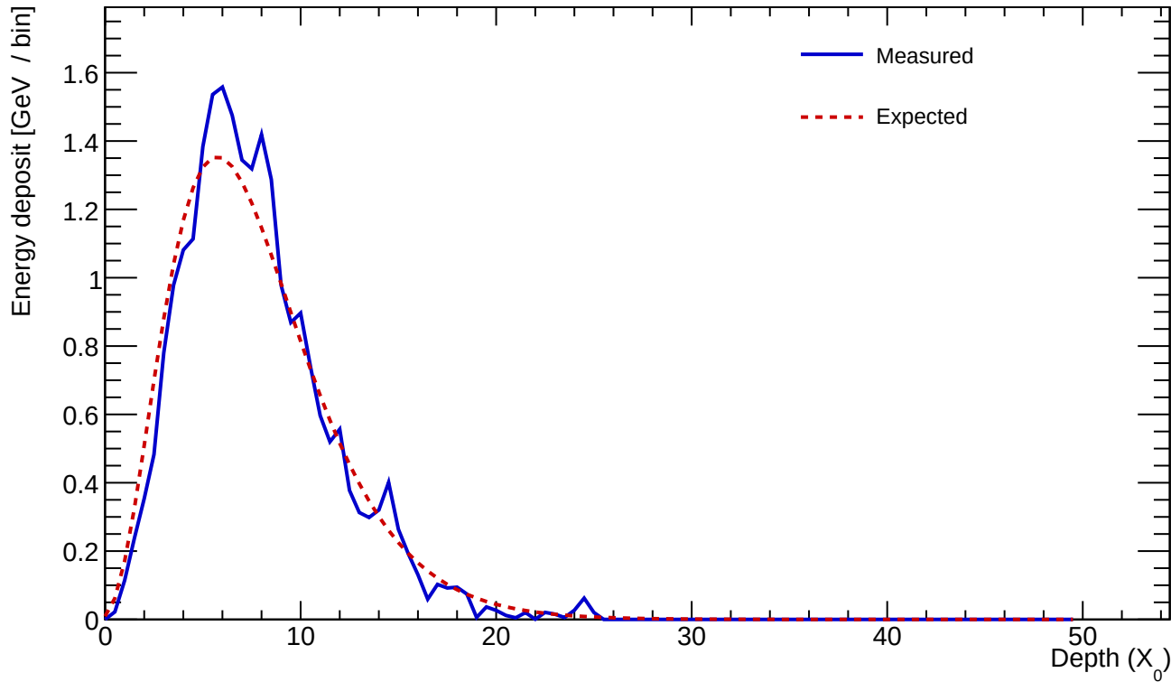
Cluster 494 E=24.622 GeV profileStart=0.50 X_0 \chi=0.1298
