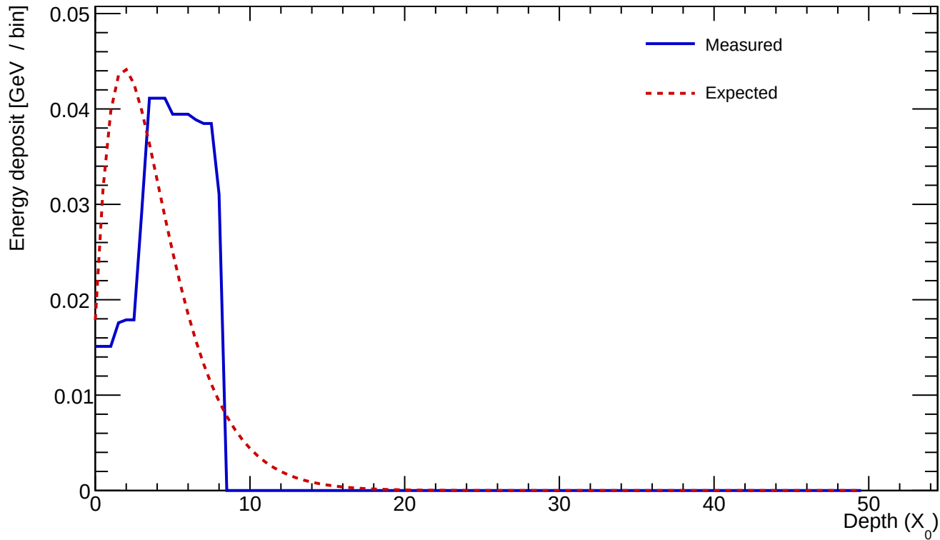
Cluster 655 E=0.516 GeV profileStart=2.50 X_0 \chi=0.2445
