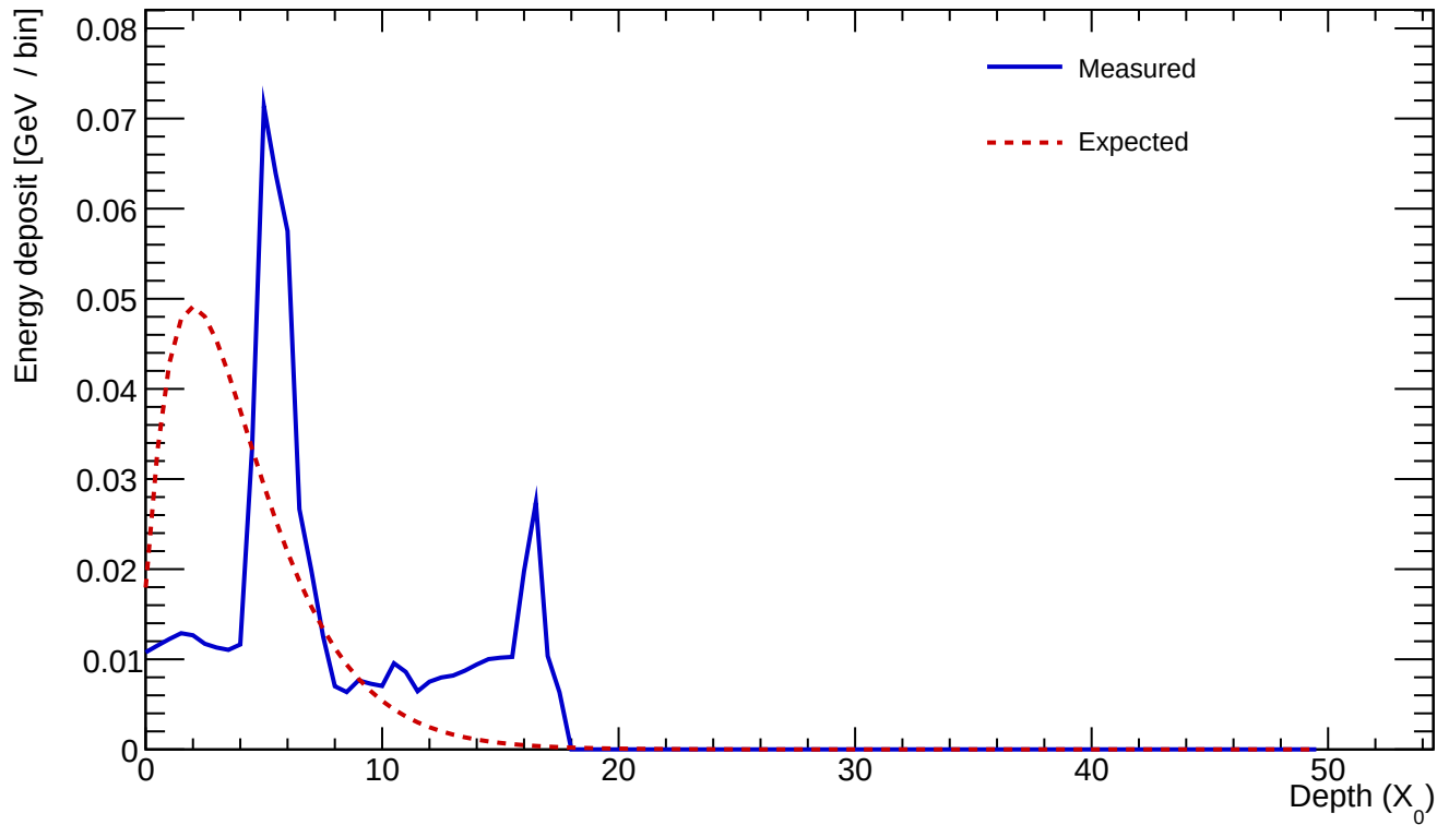
Cluster 162 E=0.587 GeV profileStart=3.00 X_0 \chi=0.7258
