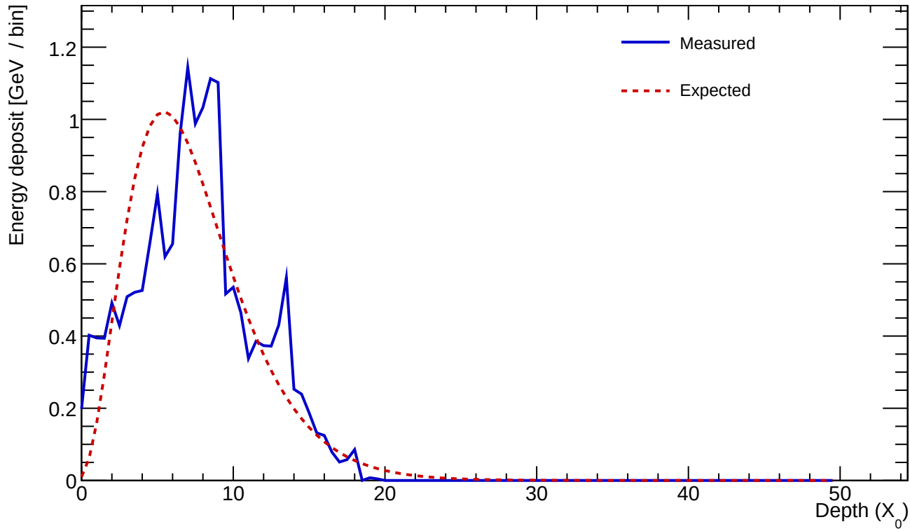
Cluster 298 E=18.130 GeV profileStart=0.50 X_0 \chi=0.3085
