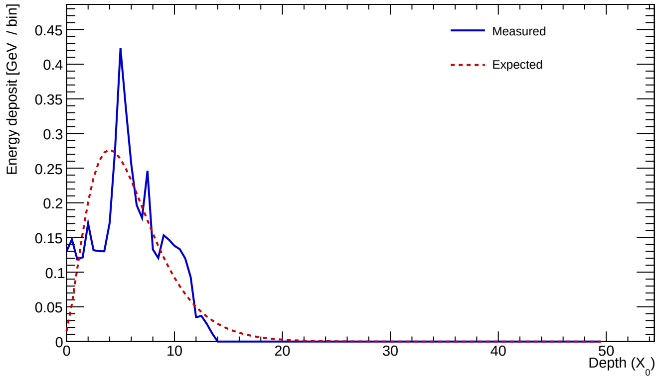
Cluster 810 E=4.310 GeV profileStart=0.50 X_0 \chi=0.3304
