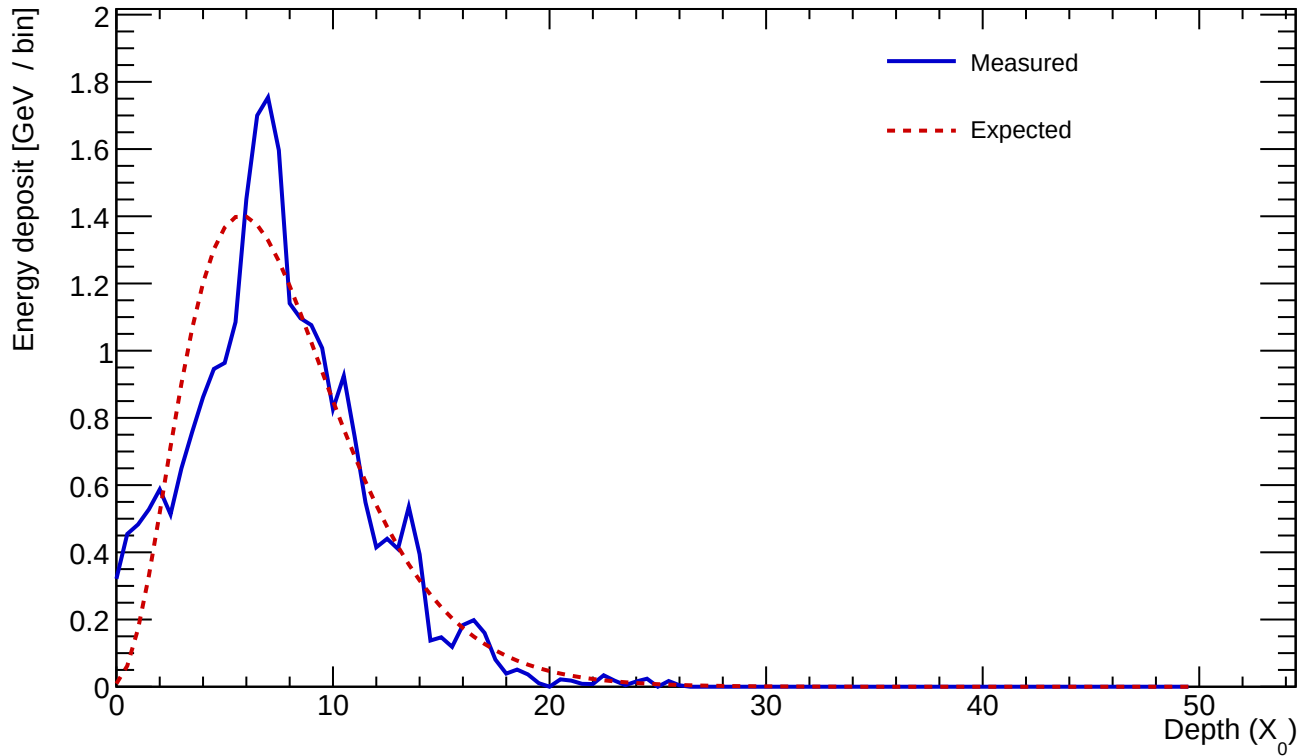
Cluster 769 E=25.550 GeV profileStart=0.50 X_0 \chi=0.2409
