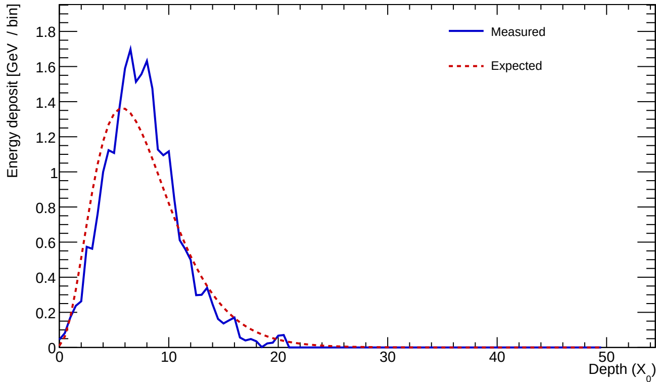
Cluster 593 E=24.786 GeV profileStart=0.50 X_0 \chi=0.1968
