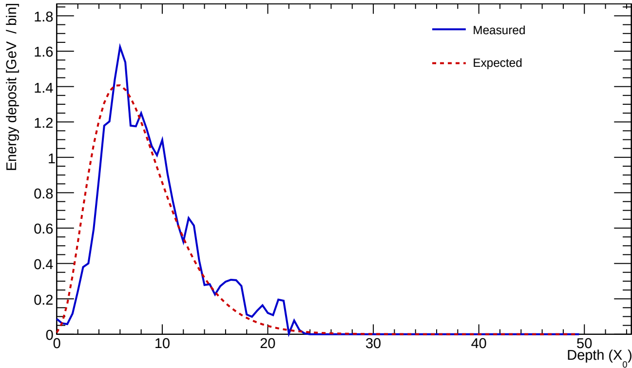
Cluster 983 E=25.704 GeV profileStart=1.00 X_0 \chi=0.1641
