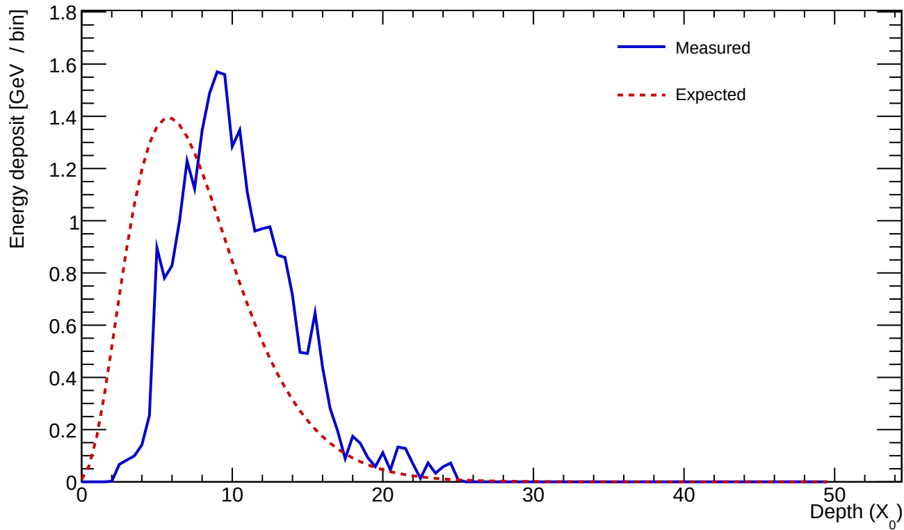
Cluster 249 E=25.411 GeV profileStart=3.00 X_0 \chi=0.1374
