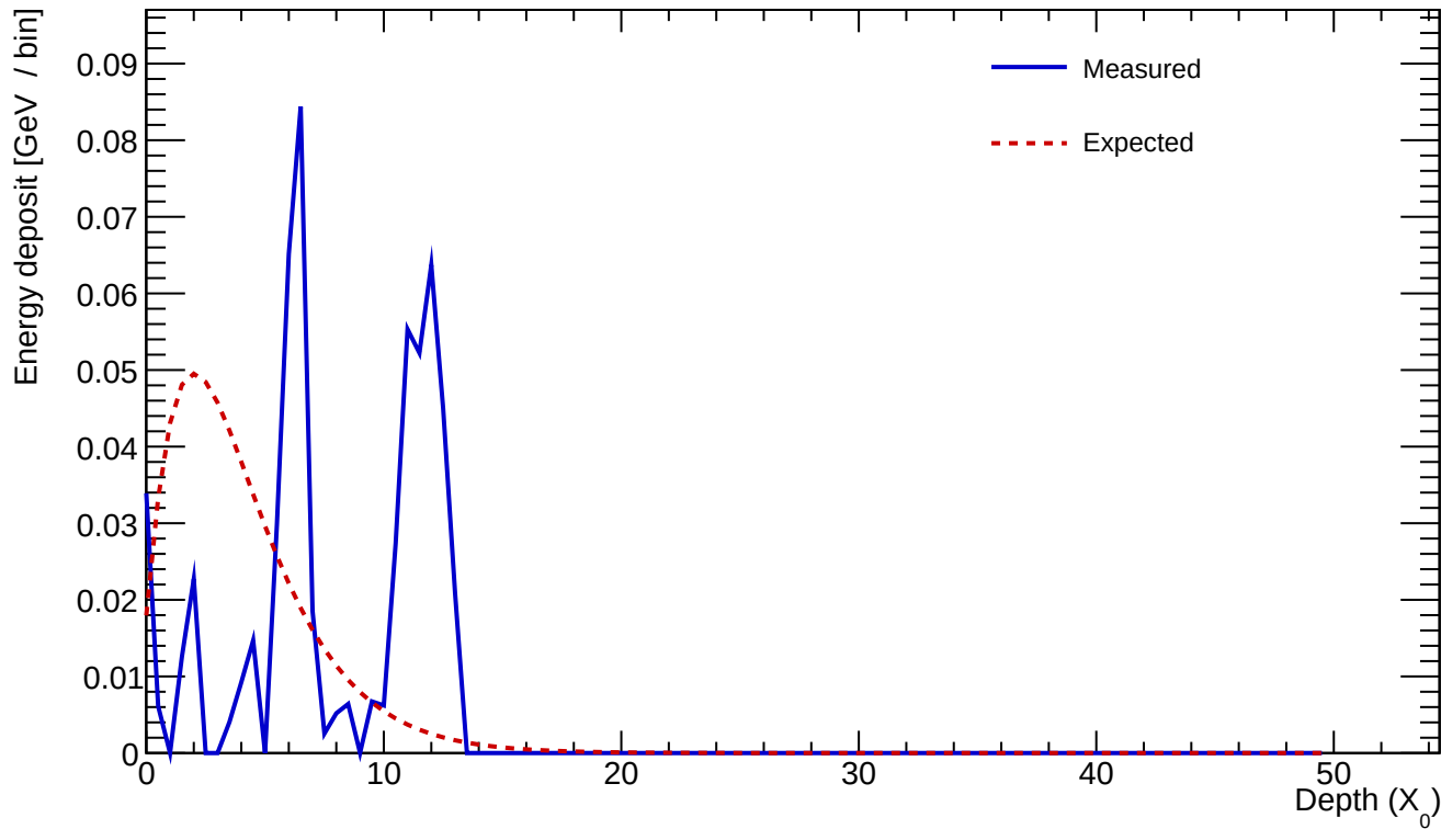
Cluster 865 E=0.593 GeV profileStart=10.00 X_0 \chi=0.6307
