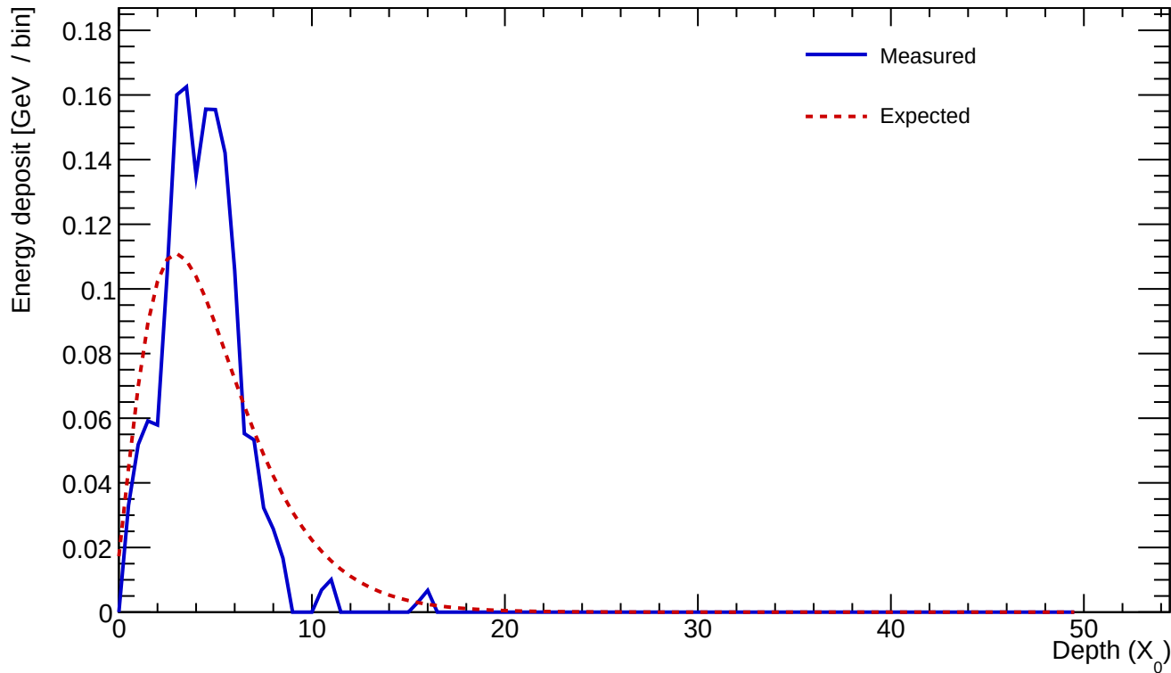
Cluster 969 E=1.533 GeV profileStart=0.50 X_0 \chi=0.4407
