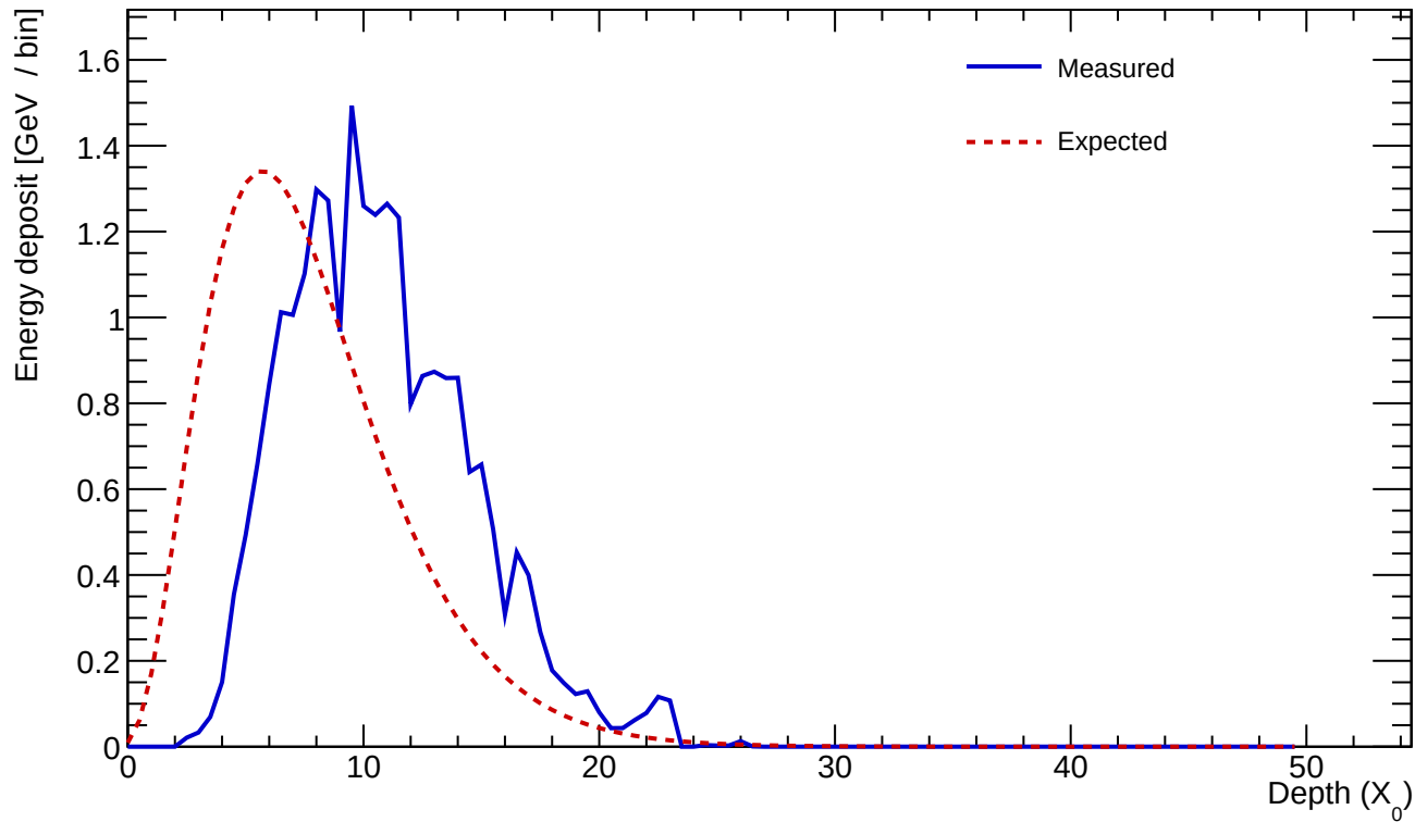
Cluster 29 E=24.385 GeV profileStart=3.00 X_0 \chi=0.1329
