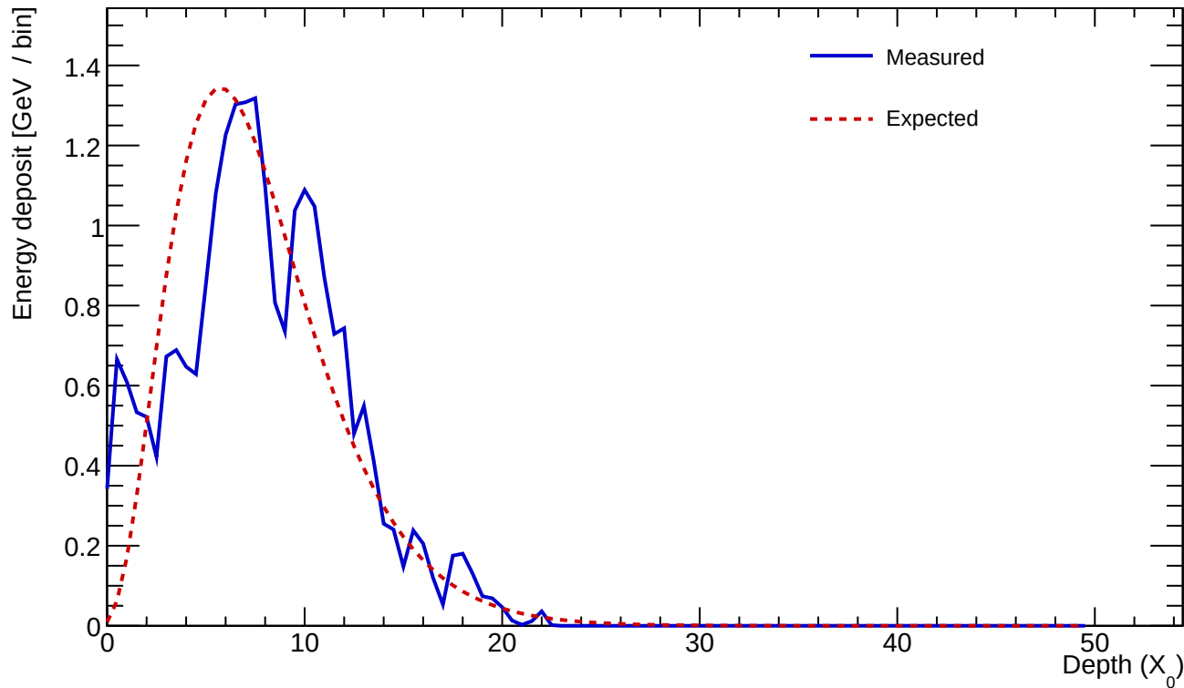
Cluster 591 E=24.417 GeV profileStart=1.00 X_0 \chi=0.2643
