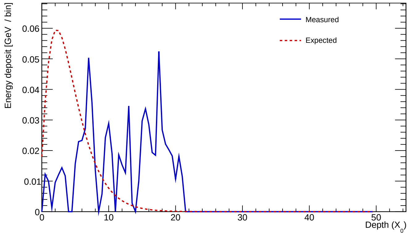
Cluster 81 E=0.741 GeV profileStart=5.00 X_0 \chi=0.9524
