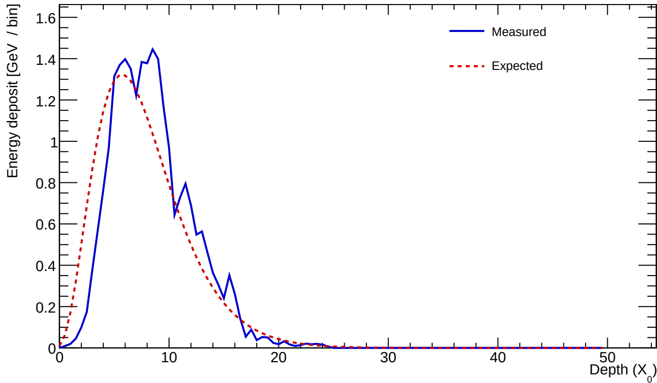
Cluster 631 E=23.998 GeV profileStart=1.00 X_0 \chi=0.1423
