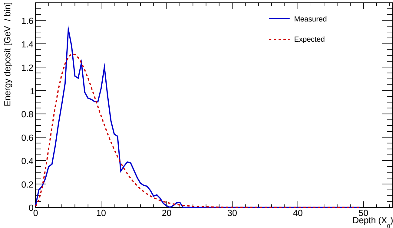
Cluster 246 E=23.807 GeV profileStart=1.00 X_0 \chi=0.1796
