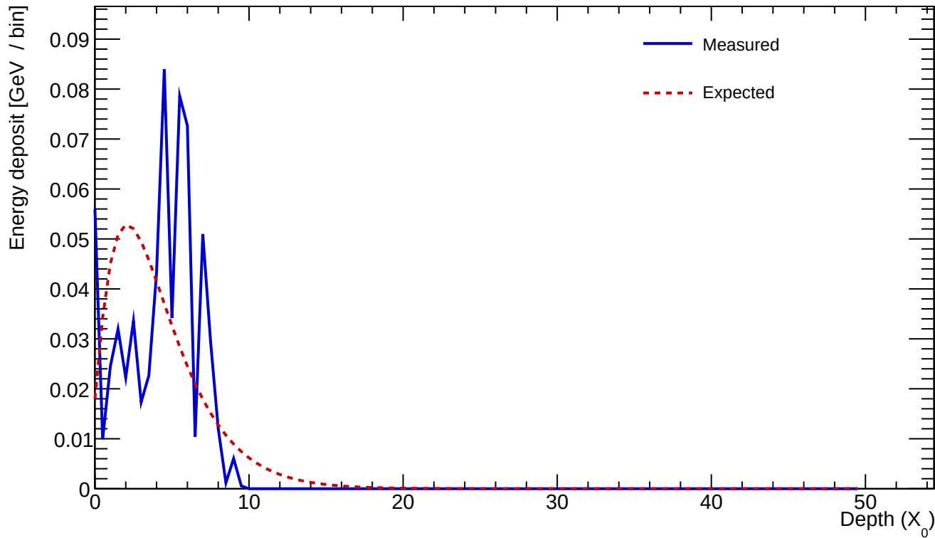
Cluster 805 E=0.642 GeV profileStart=1.00 X_0 \chi=0.6116
