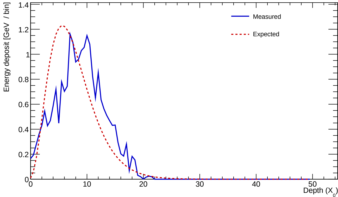
Cluster 554 E=22.169 GeV profileStart=2.00 X_0 \chi=0.2743
