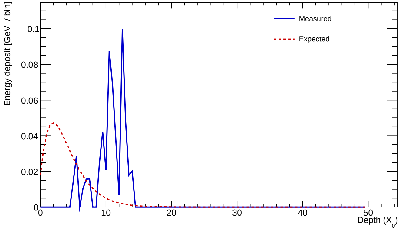
Cluster 384 E=0.559 GeV profileStart=9.00 X_0 \chi=0.5638
