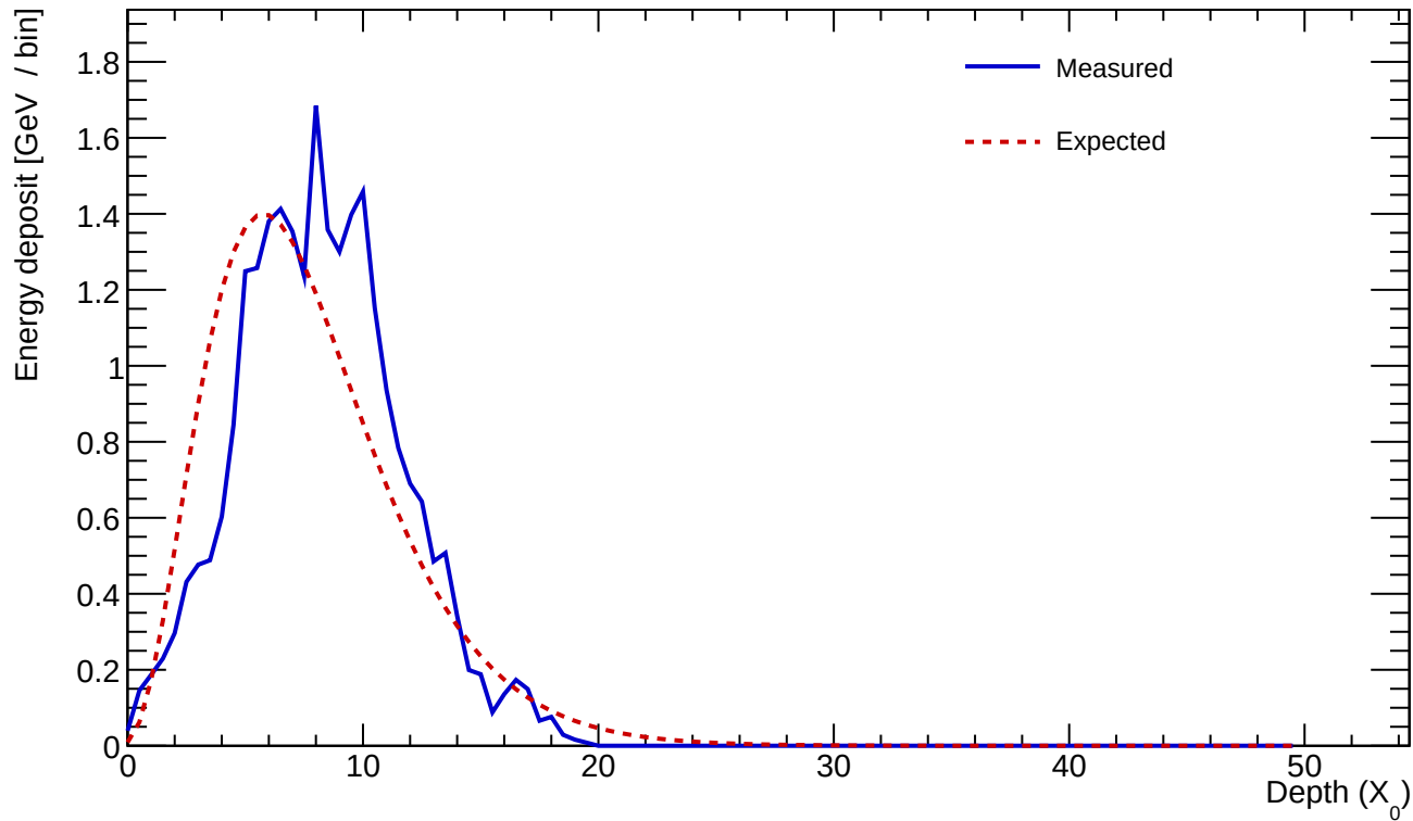
Cluster 5 E=25.499 GeV profileStart=1.00 X_0 \chi=0.1793
