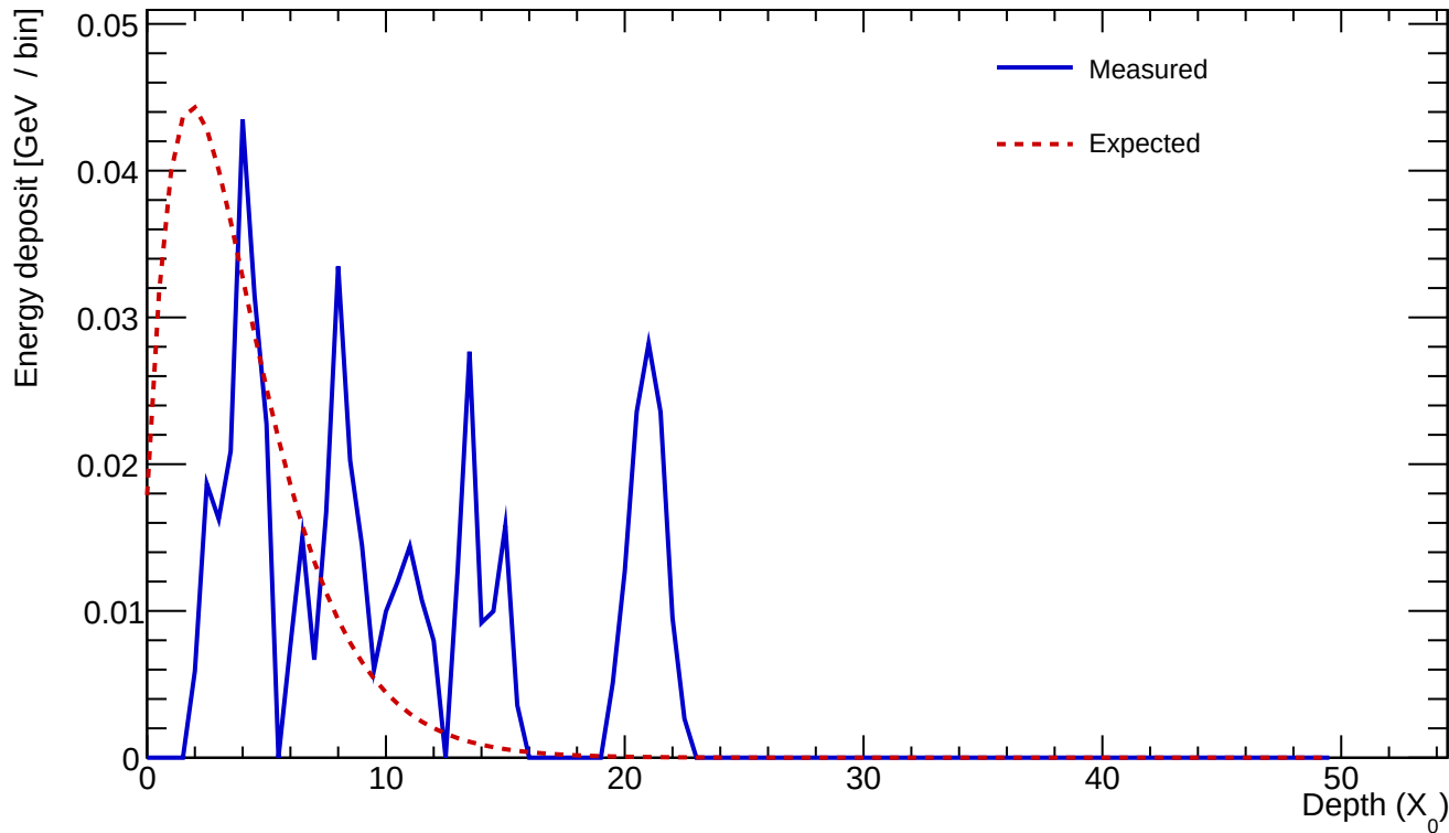
Cluster 1137 E=0.519 GeV profileStart=2.50 X_0 \chi=0.7826
