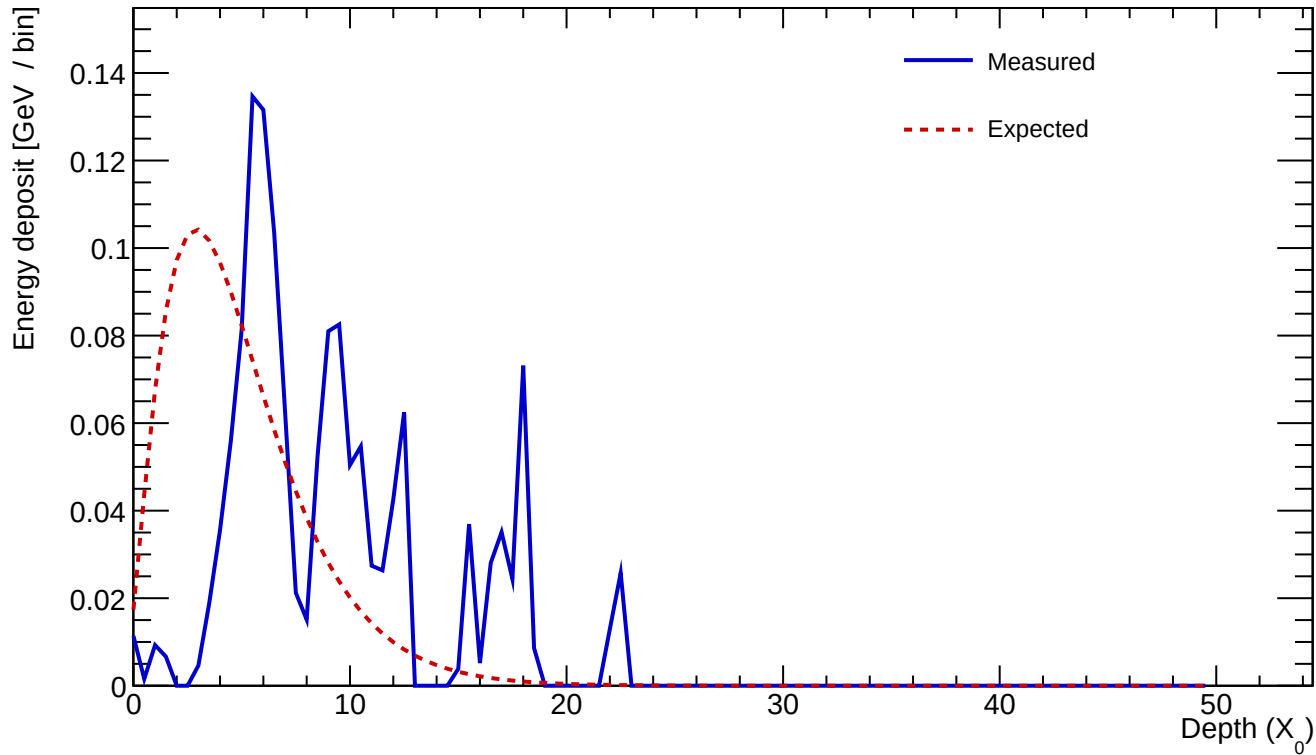
Cluster 731 E=1.428 GeV profileStart=3.50 X_0 \chi=0.5133
