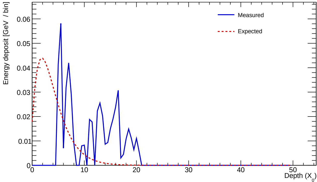
Cluster 238 E=0.513 GeV profileStart=4.50 X_0 \chi=0.8701
