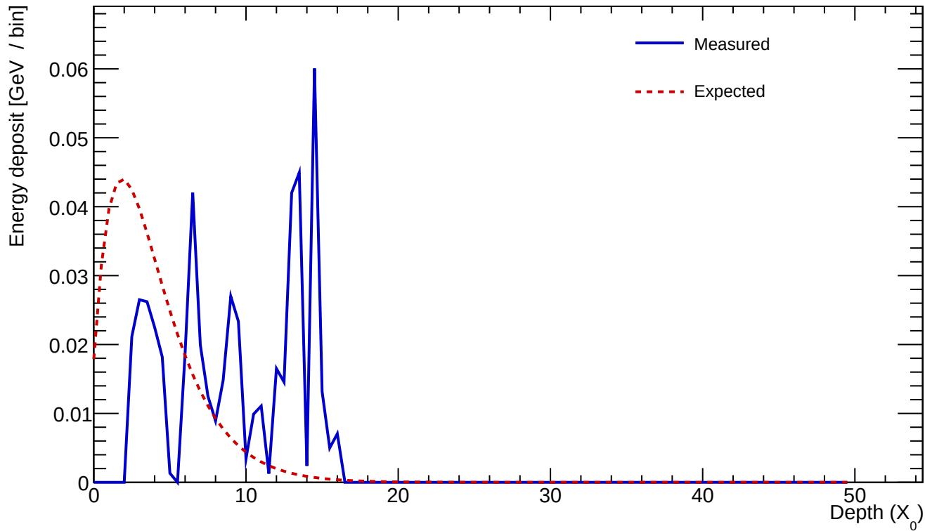
Cluster 567 E=0.515 GeV profileStart=2.50 X_0 \chi=0.8299
