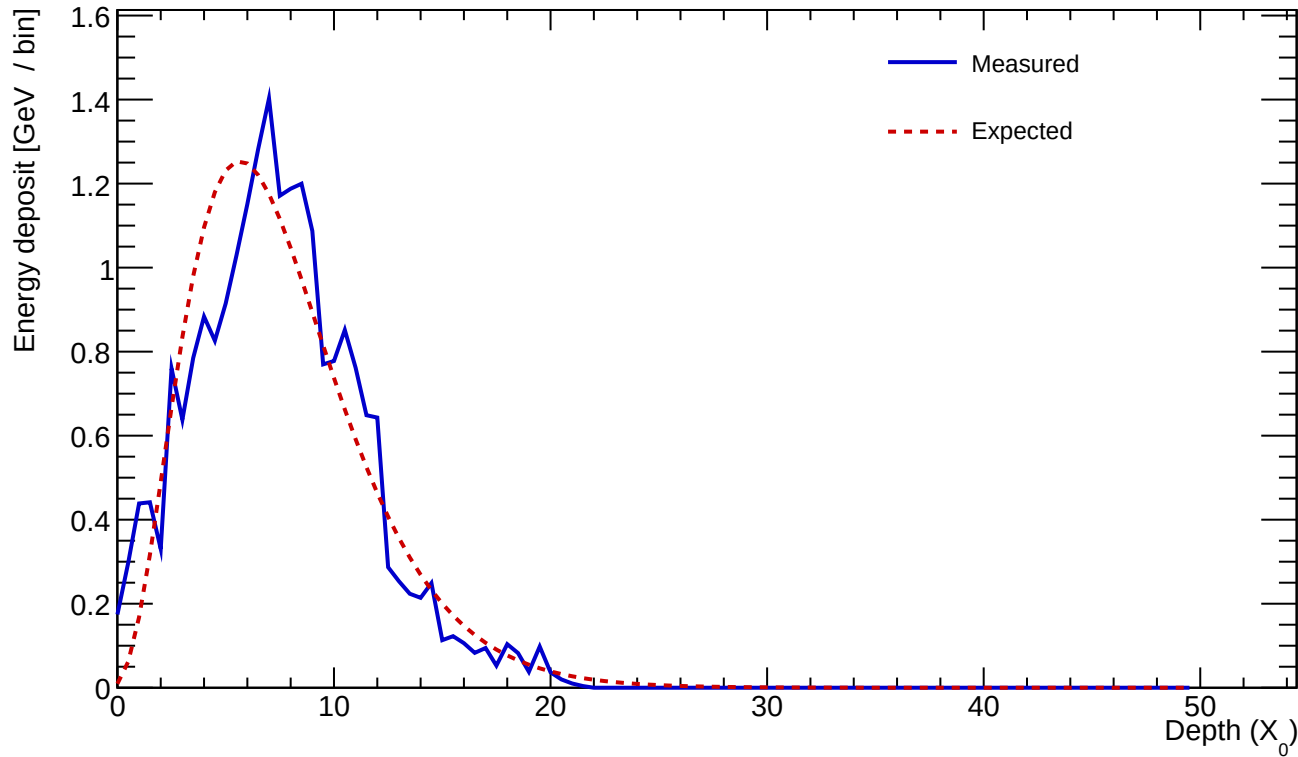
Cluster 456 E=22.646 GeV profileStart=0.50 X_0 \chi=0.2054
