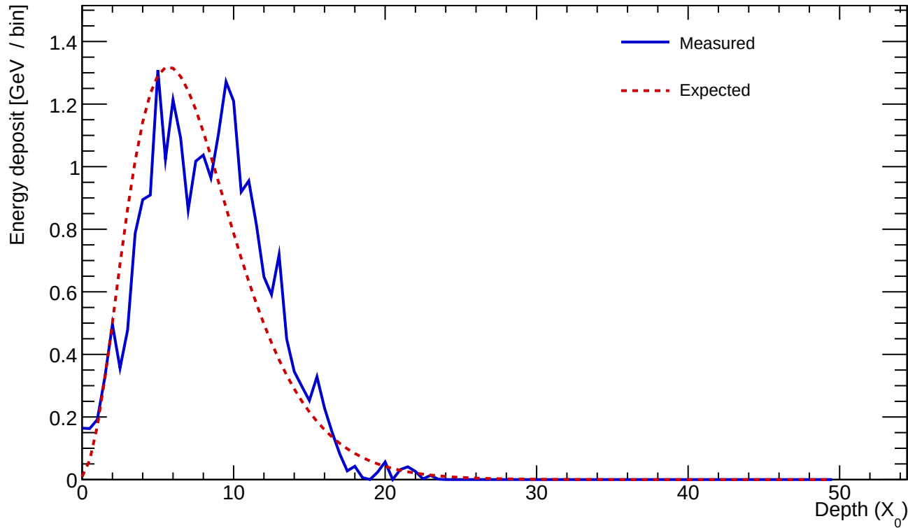
Cluster 17 E=23.925 GeV profileStart=1.00 X_0 \chi=0.2152
