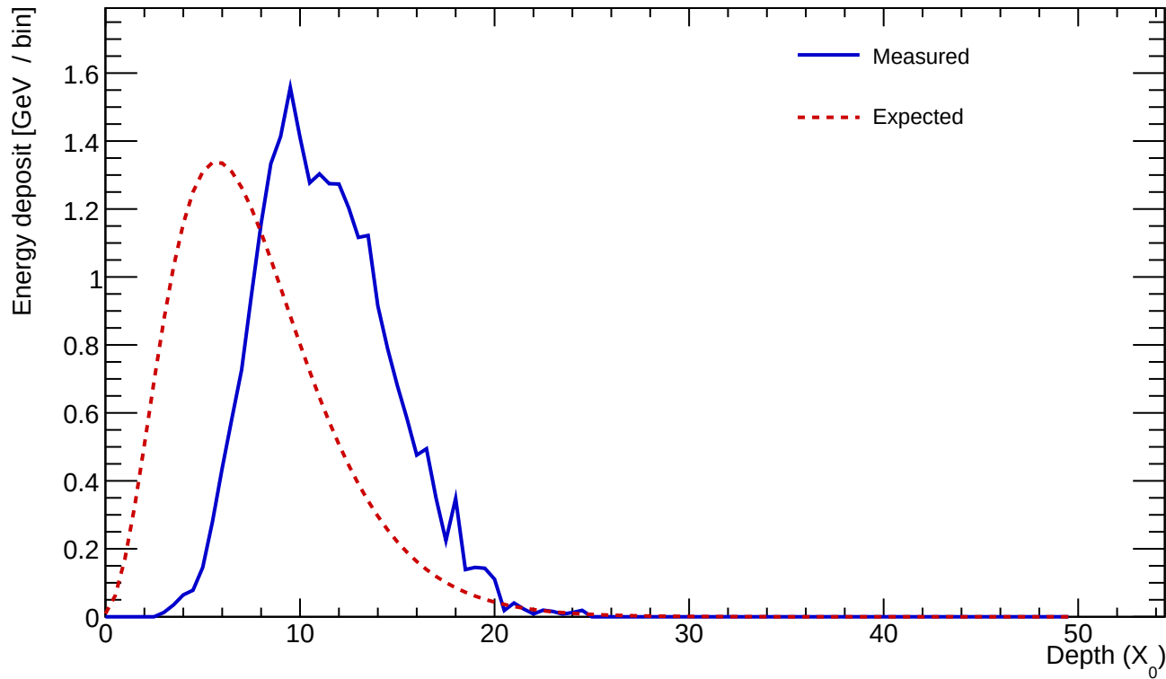
Cluster 13 E=24.314 GeV profileStart=4.00 X_0 \chi=0.1333
