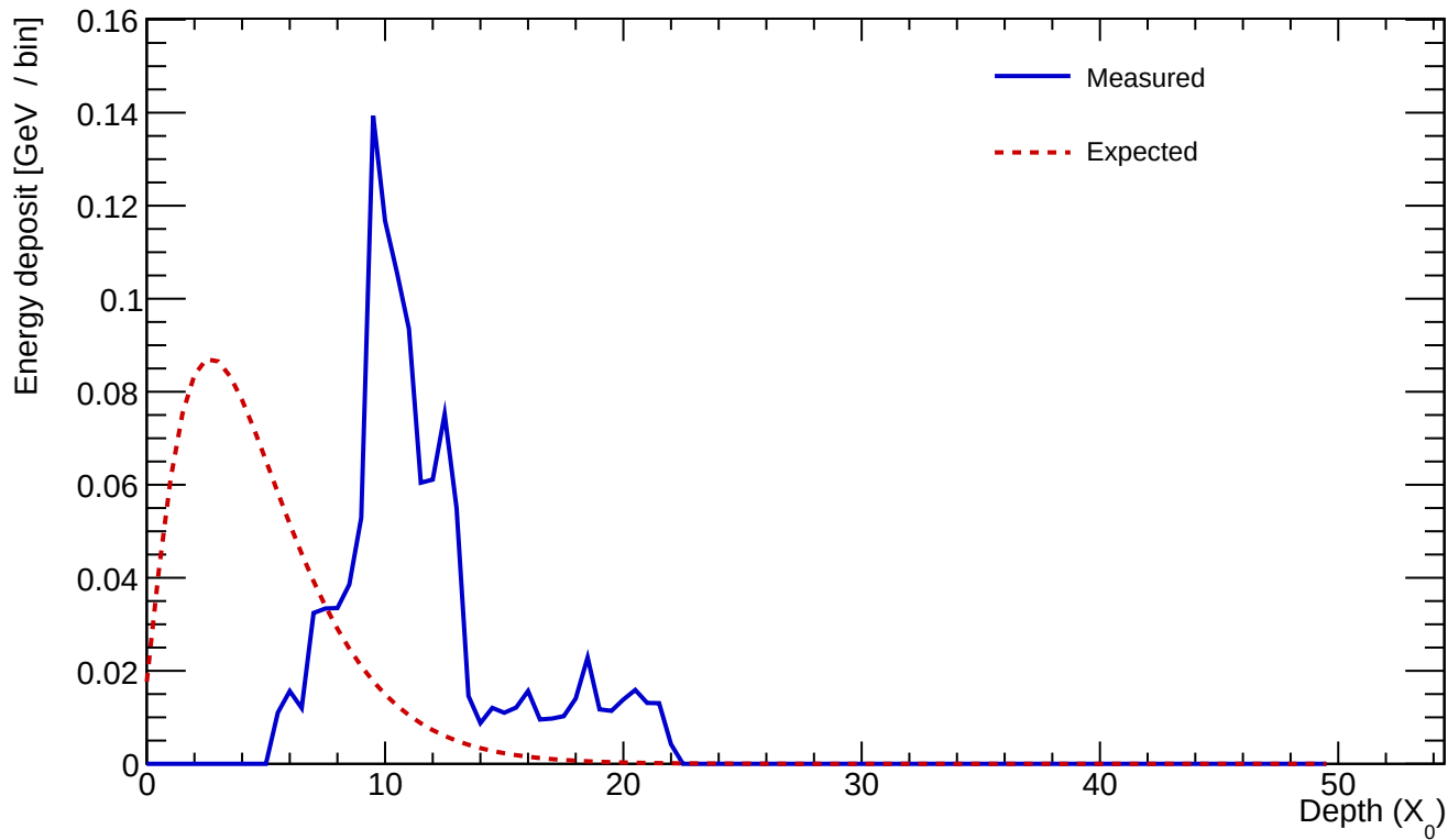
Cluster 115 E=1.160 GeV profileStart=7.00 X_0 \chi=0.4445
