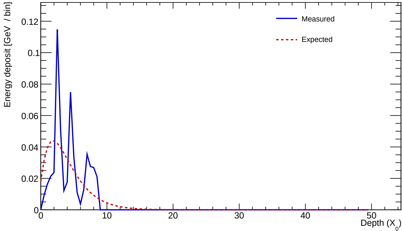
Cluster 611 E=0.513 GeV profileStart=1.00 X_0 \chi=0.5799
