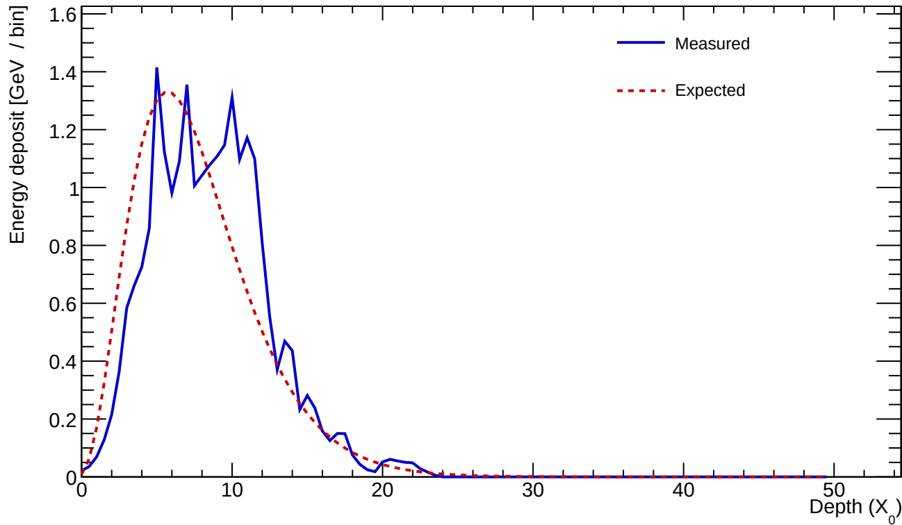
Cluster 344 E=24.143 GeV profileStart=1.00 X_0 \chi=0.1939
