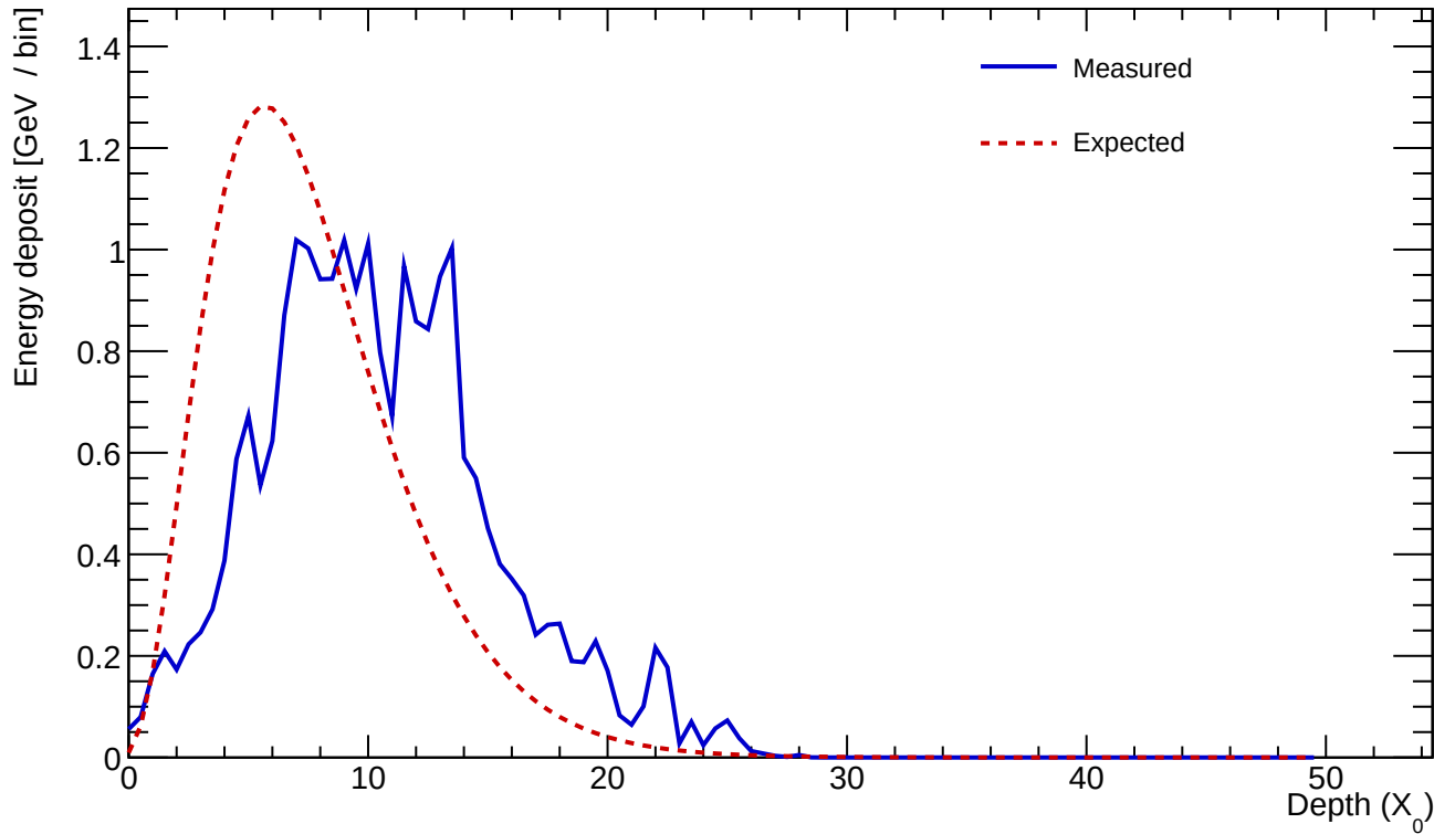
Cluster 472 E=23.218 GeV profileStart=3.00 X_0 \chi=0.2835
