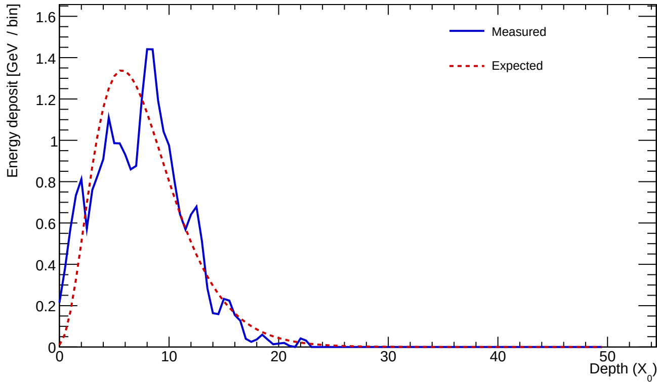
Cluster 256 E=24.325 GeV profileStart=0.50 X_0 \chi=0.2794
