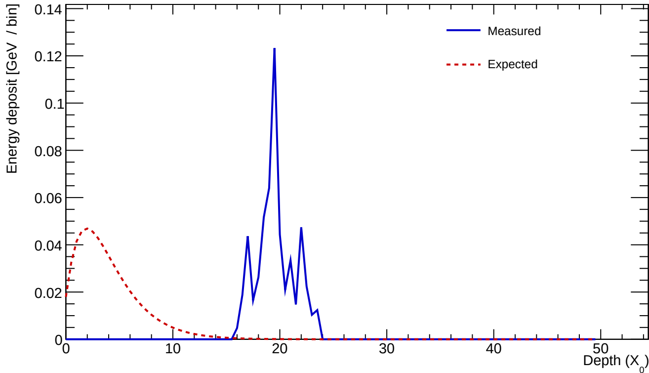
Cluster 971 E=0.555 GeV profileStart=16.50 X_0 \chi=0.4180
