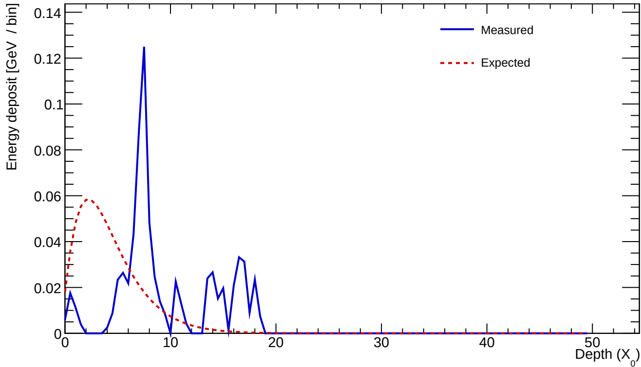
Cluster 1109 E=0.724 GeV \text{profileStart}=4.50 X_0 \chi=0.8132
