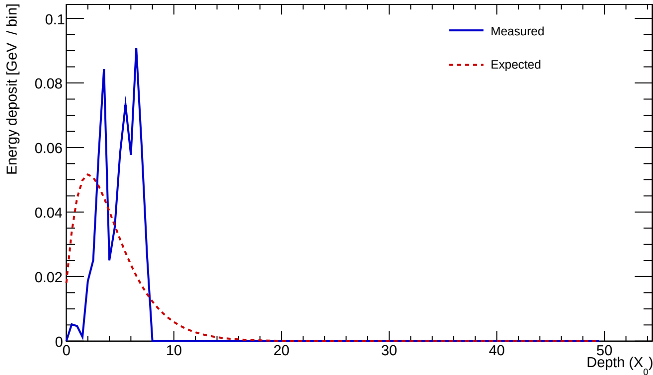
Cluster 1129 E=0.624 GeV profileStart=2.00 X_0 \chi=0.4016
