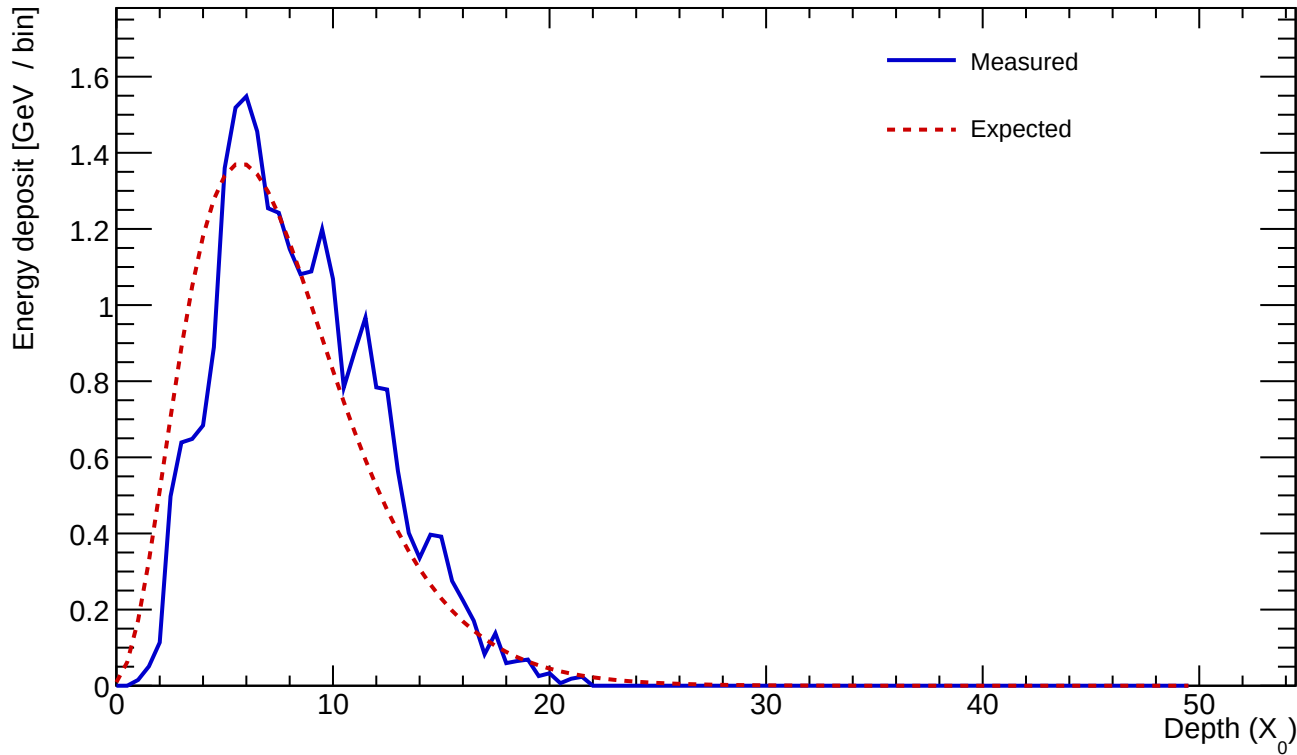
Cluster 721 E=24.971 GeV profileStart=1.00 X_0 \chi=0.1483
