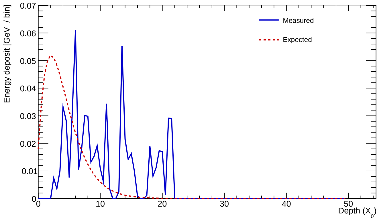
Cluster 1162 E=0.628 GeV profileStart=3.50 X_0 \chi=0.7936
