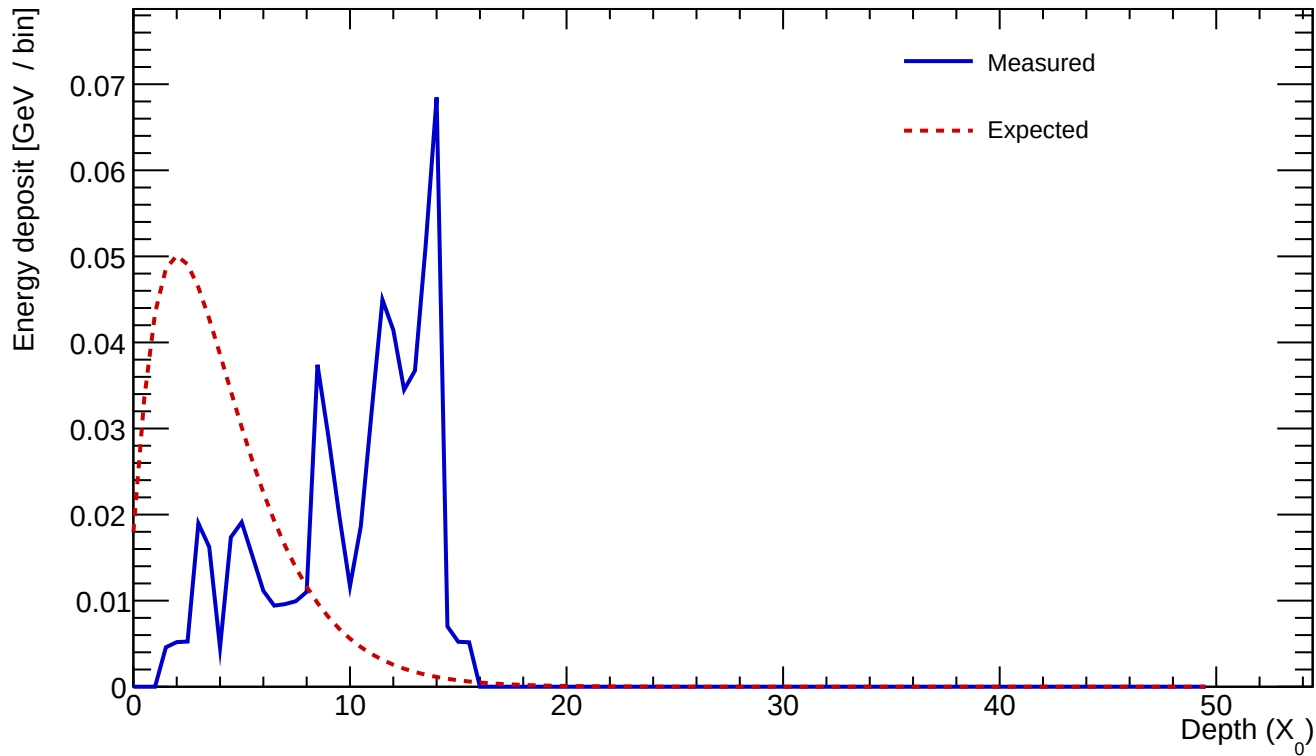
Cluster 296 E=0.601 GeV profileStart=8.00 X_0 \chi=0.6629
