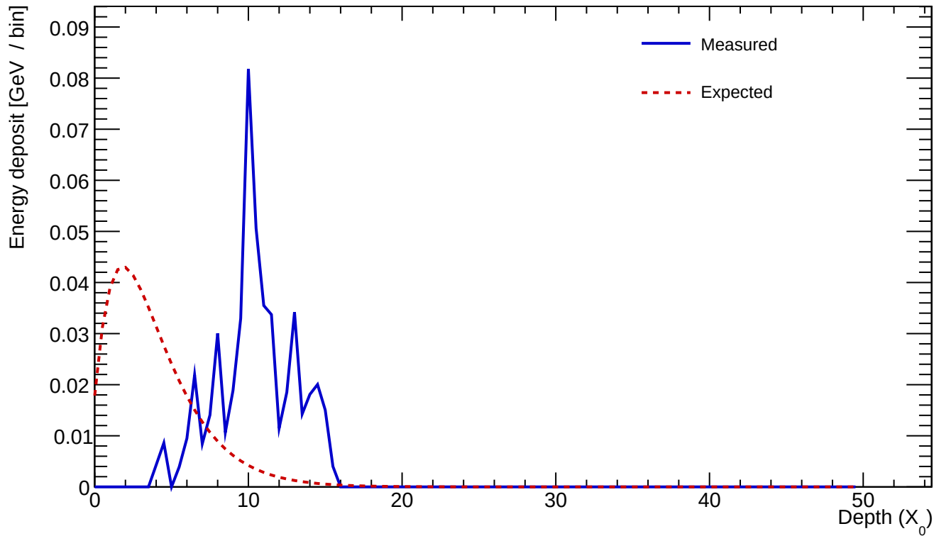
Cluster 128 E=0.501 GeV profileStart=7.50 X_0 \chi=0.4636
