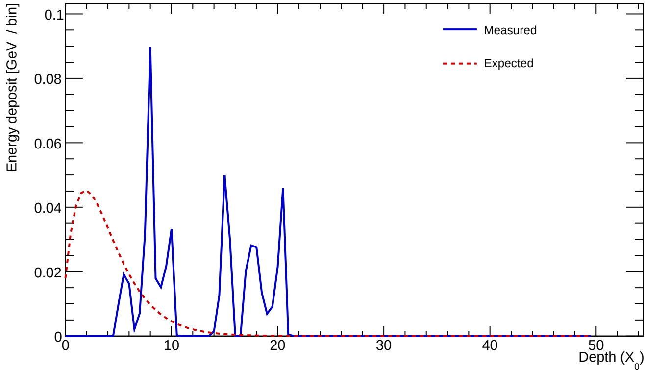
Cluster 251 E=0.531 GeV profileStart=5.50 X_0 \chi=1.1152
