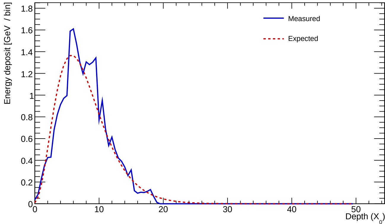
Cluster 126 E=24.872 GeV profileStart=0.50 X_0 \chi=0.1553
