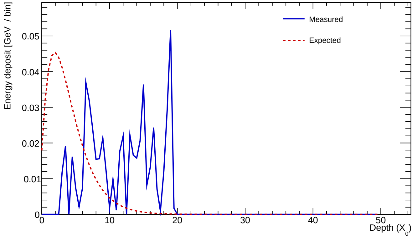
Cluster 93 E=0.533 GeV profileStart=18.00 X_0 \chi=0.8590
