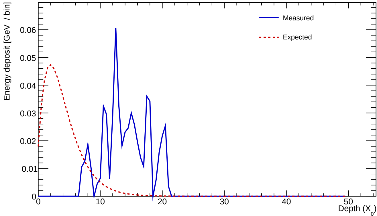
Cluster 698 E=0.562 GeV profileStart=10.00 X_0 \chi=0.5767
