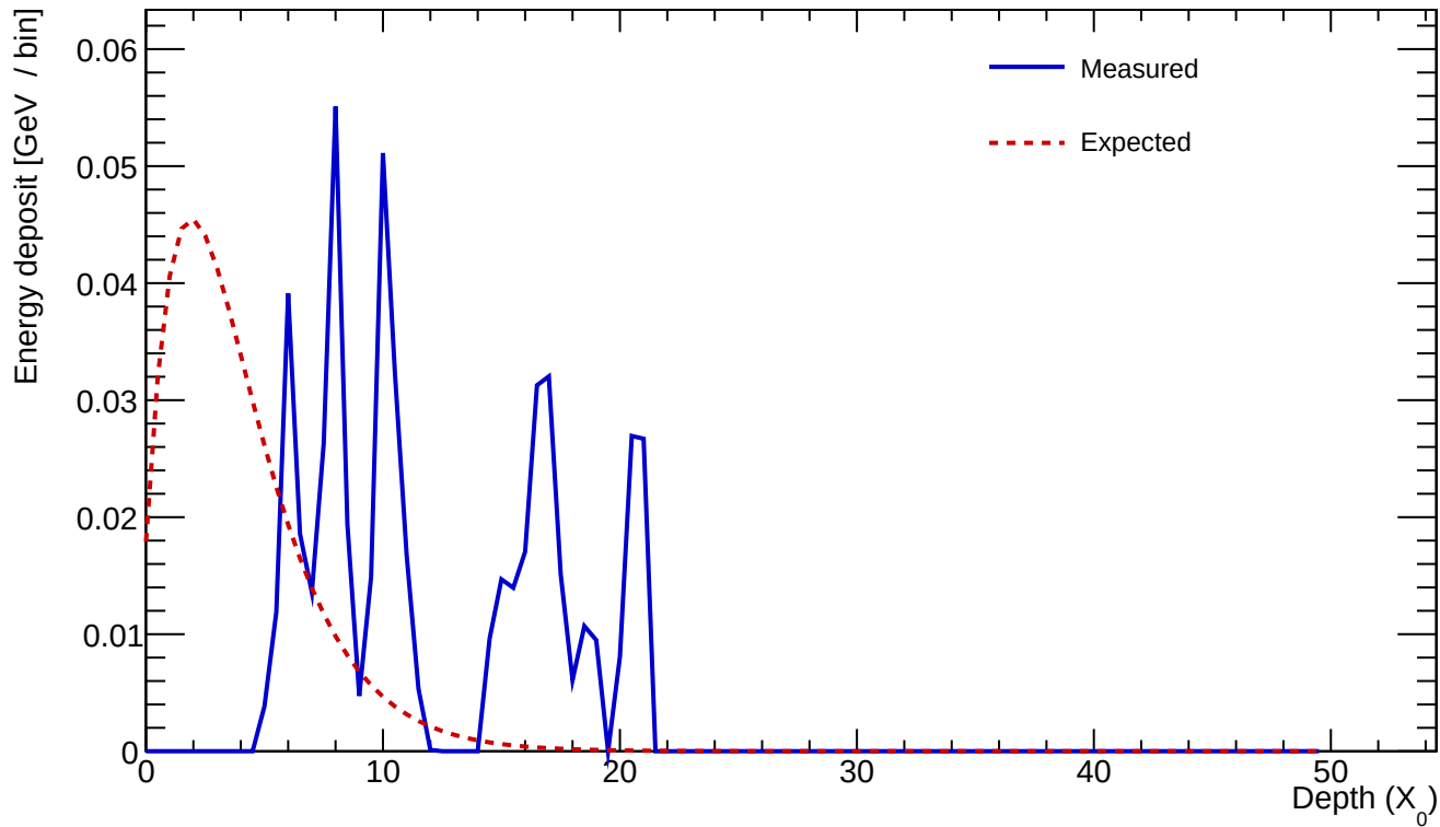
Cluster 409 E=0.535 GeV profileStart=5.50 X_0 \chi=0.8284
