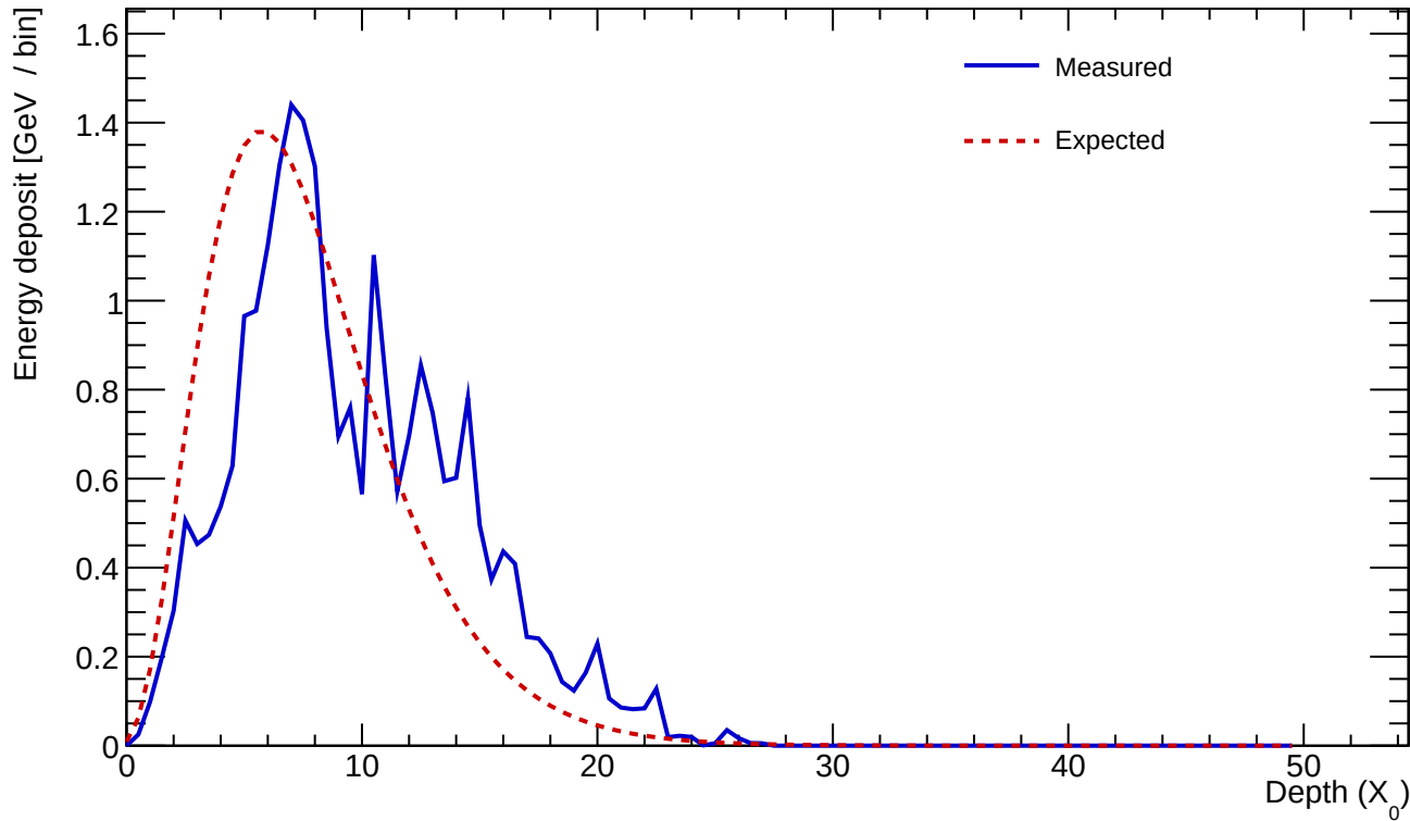
Cluster 104 E=25.162 GeV profileStart=2.00 X_0 \chi=0.2518
