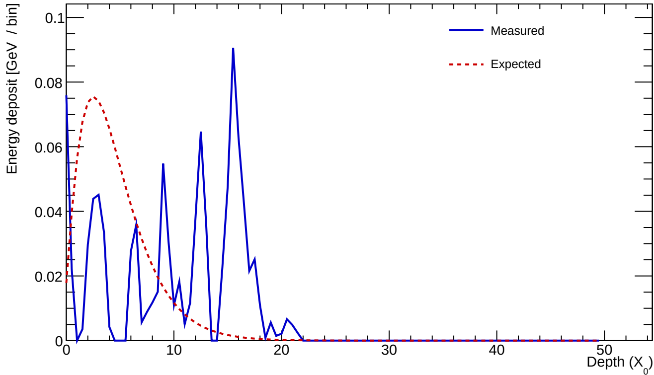
Cluster 991 E=0.980 GeV profileStart=1.50 X_0 \chi=1.1726
