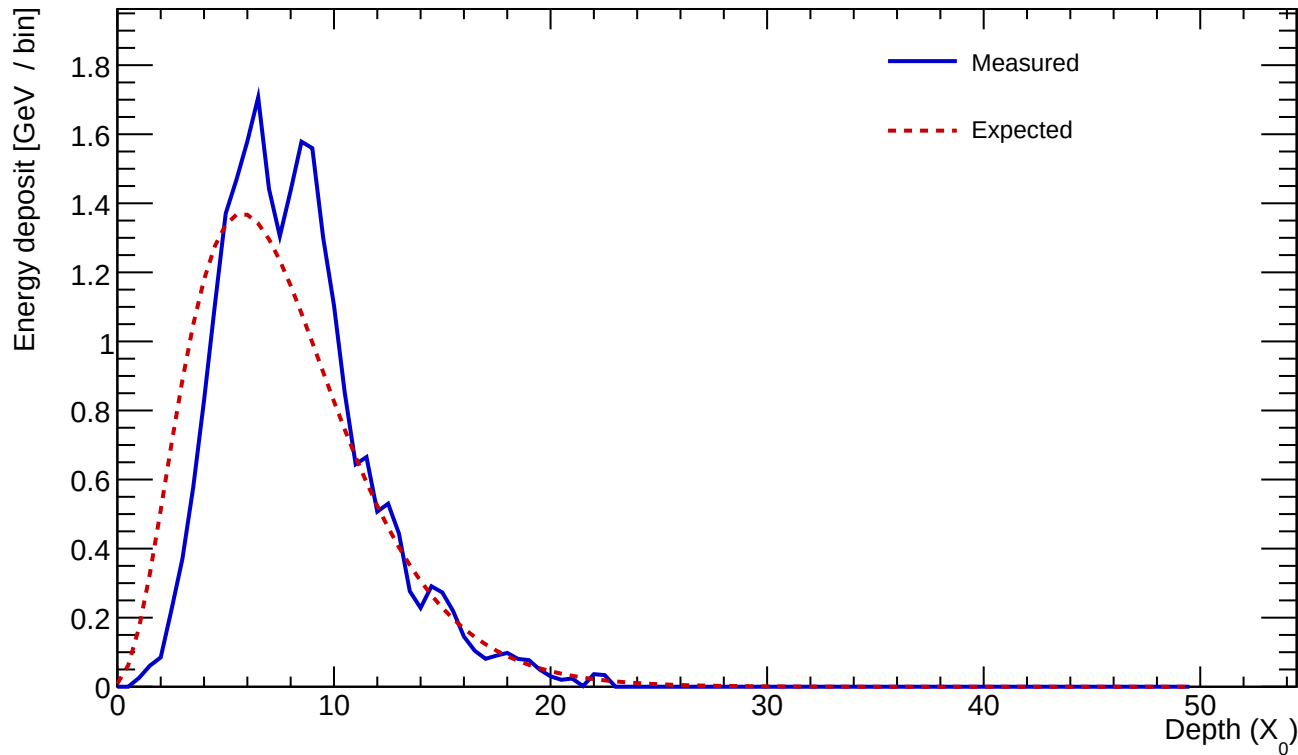
Cluster 207 E=24.929 GeV profileStart=1.00 X_0 \chi=0.1819
