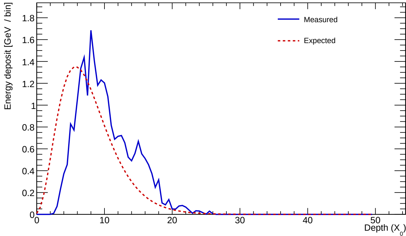
Cluster 481 E=24.555 GeV profileStart=2.50 X_0 \chi=0.1668
