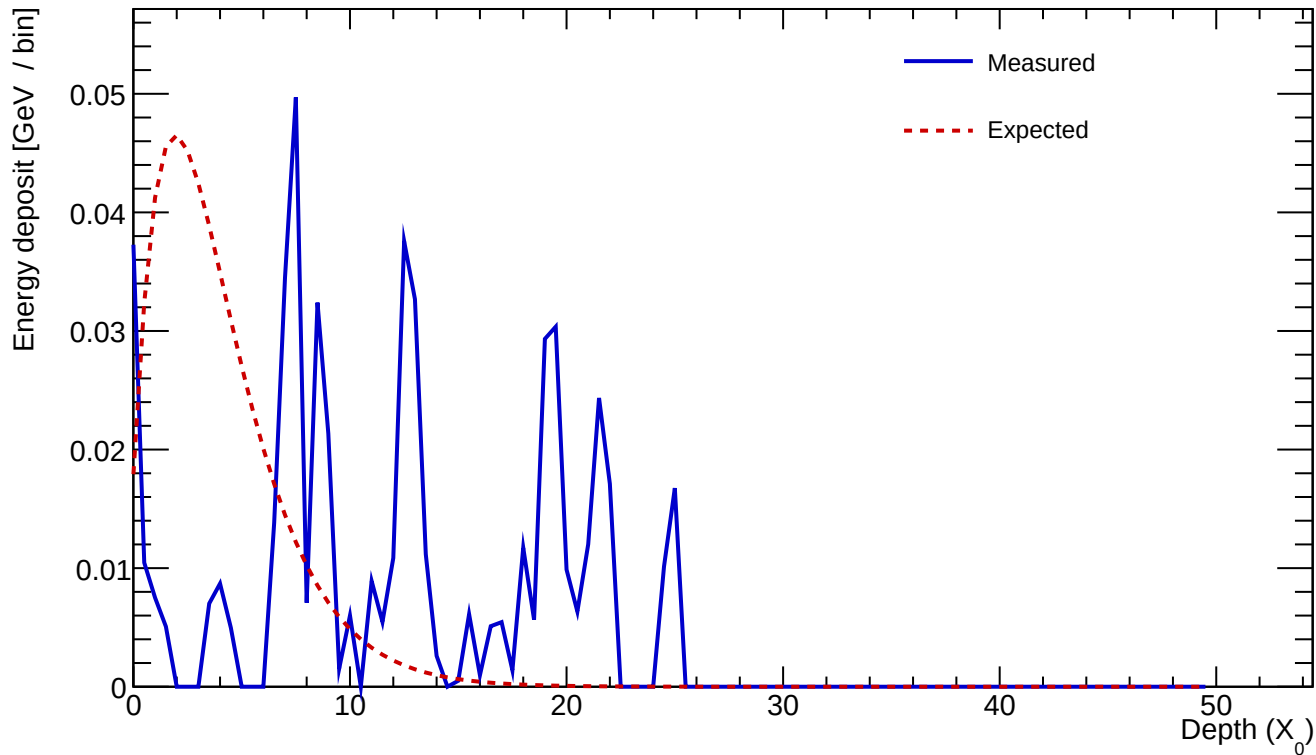
Cluster 1177 E=0.550 GeV profileStart=6.50 X_0 \chi=1.0117
