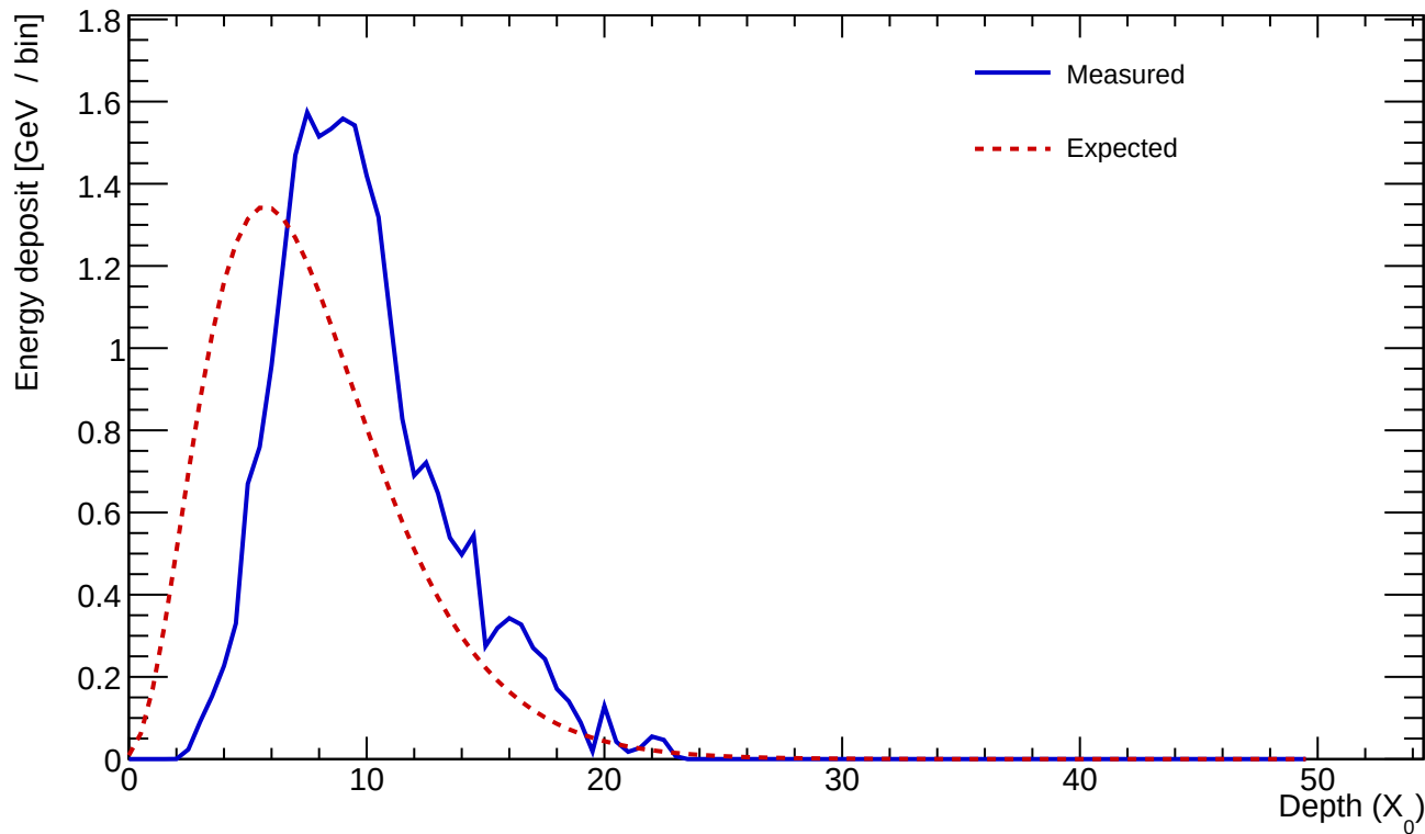
Cluster 852 E=24.413 GeV profileStart=2.50 X_0 \chi=0.1548
