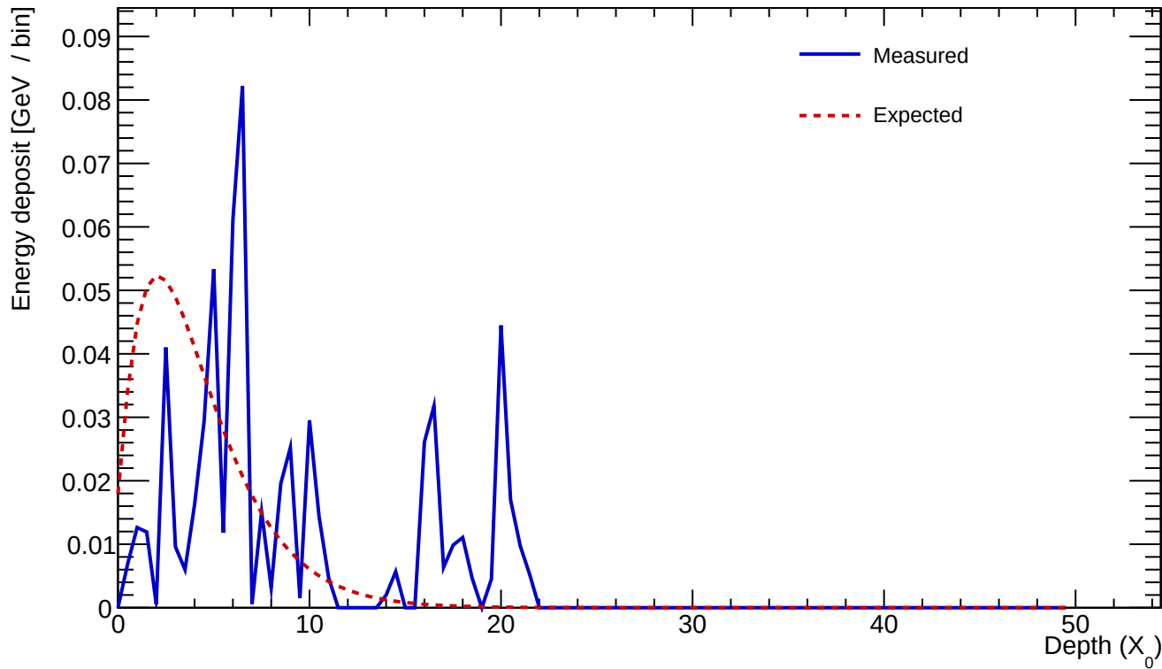
Cluster 881 E=0.635 GeV profileStart=3.50 X_0 \chi=0.9299
