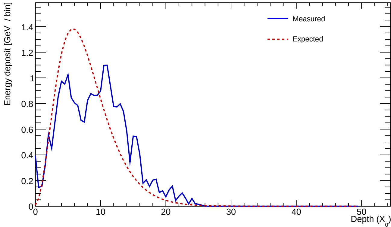
Cluster 394 E=25.162 GeV profileStart=1.00 X_0 \chi=0.3820
