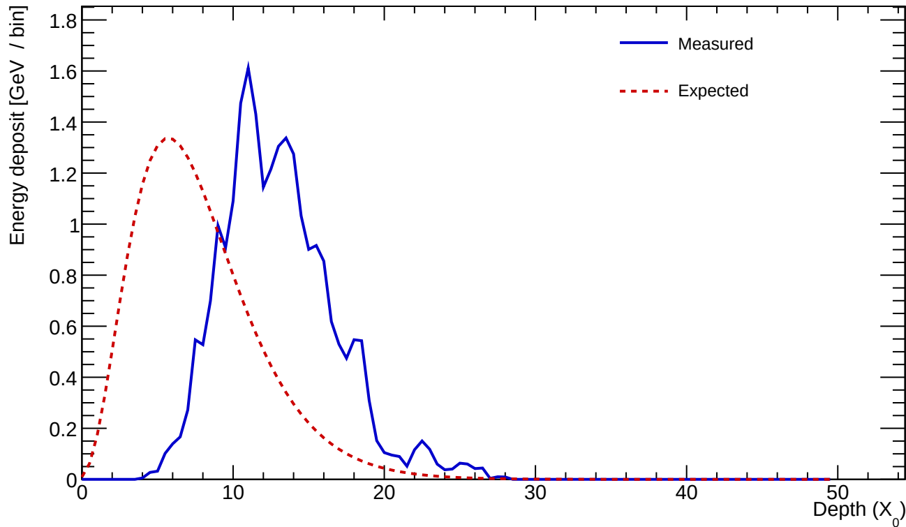
Cluster 943 E=24.278 GeV profileStart=5.50 X_0 \chi=0.1641
