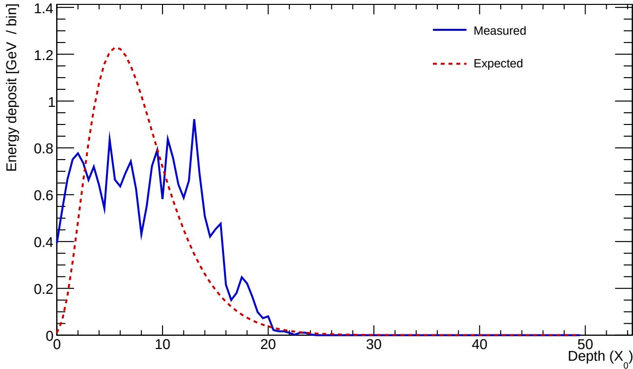
Cluster 148 E=22.162 GeV profileStart=1.00 X_0 \chi=0.5120
