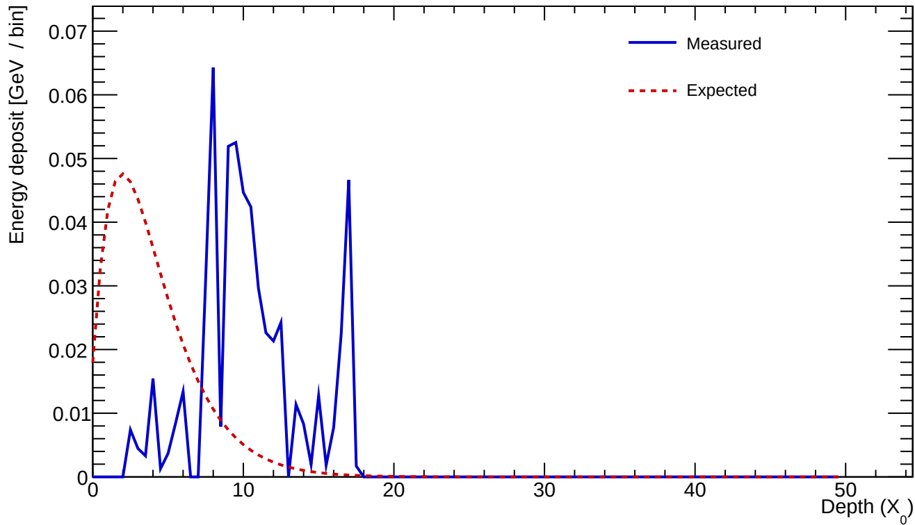
Cluster 233 E=0.565 GeV profileStart=7.00 X_0 \chi=0.5065
