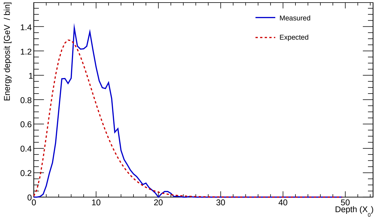
Cluster 9 E=23.359 GeV profileStart=1.50 X_0 \chi=0.1263
