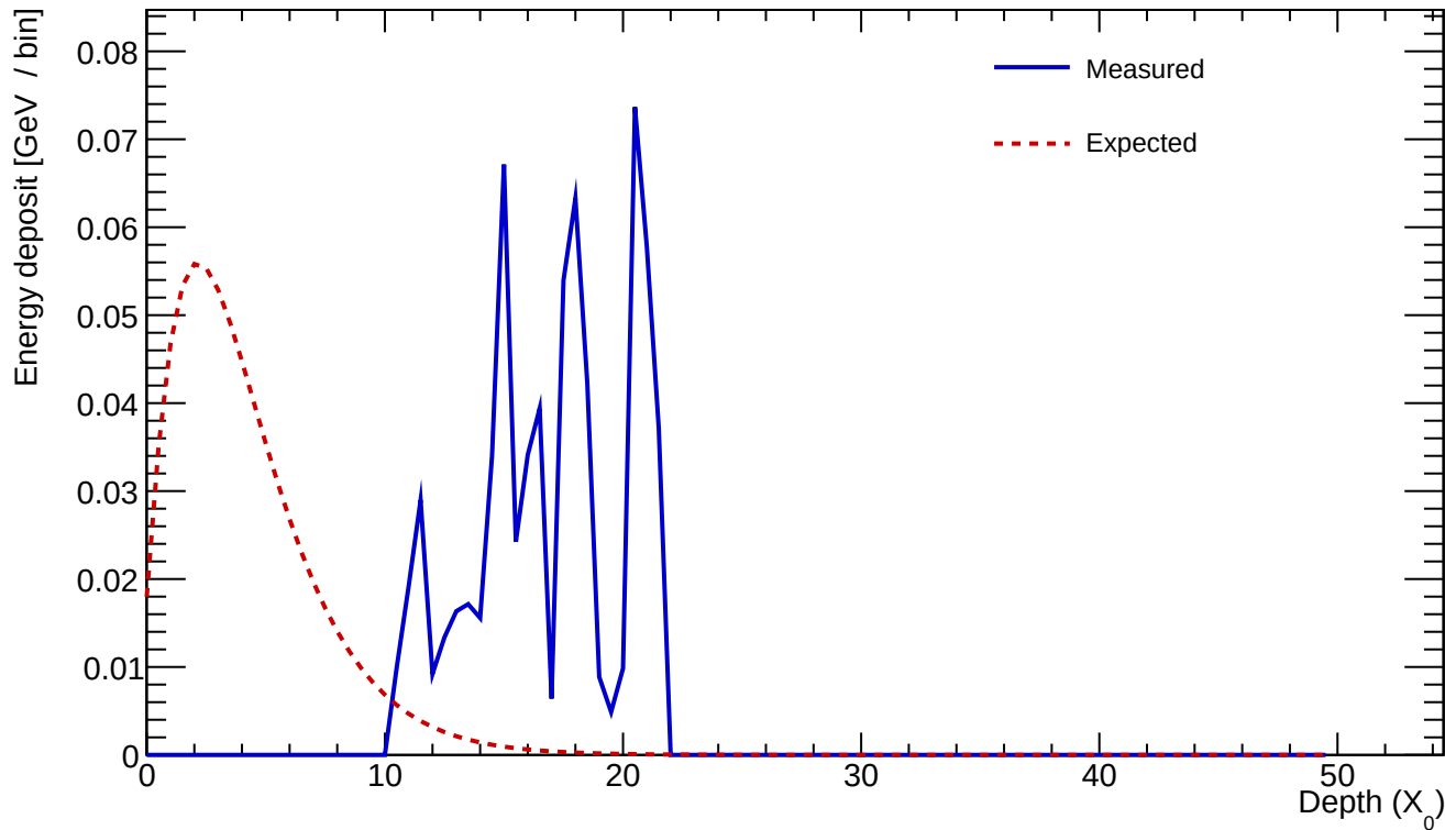
Cluster 319 E=0.687 GeV profileStart=14.00 X_0 \chi=0.6335
