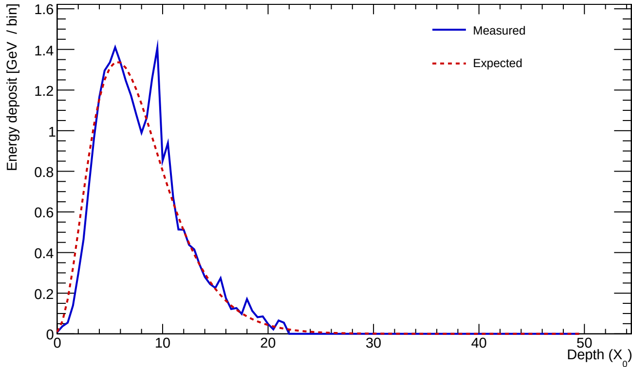
Cluster 634 E=24.324 GeV profileStart=0.50 X_0 \chi=0.1270
