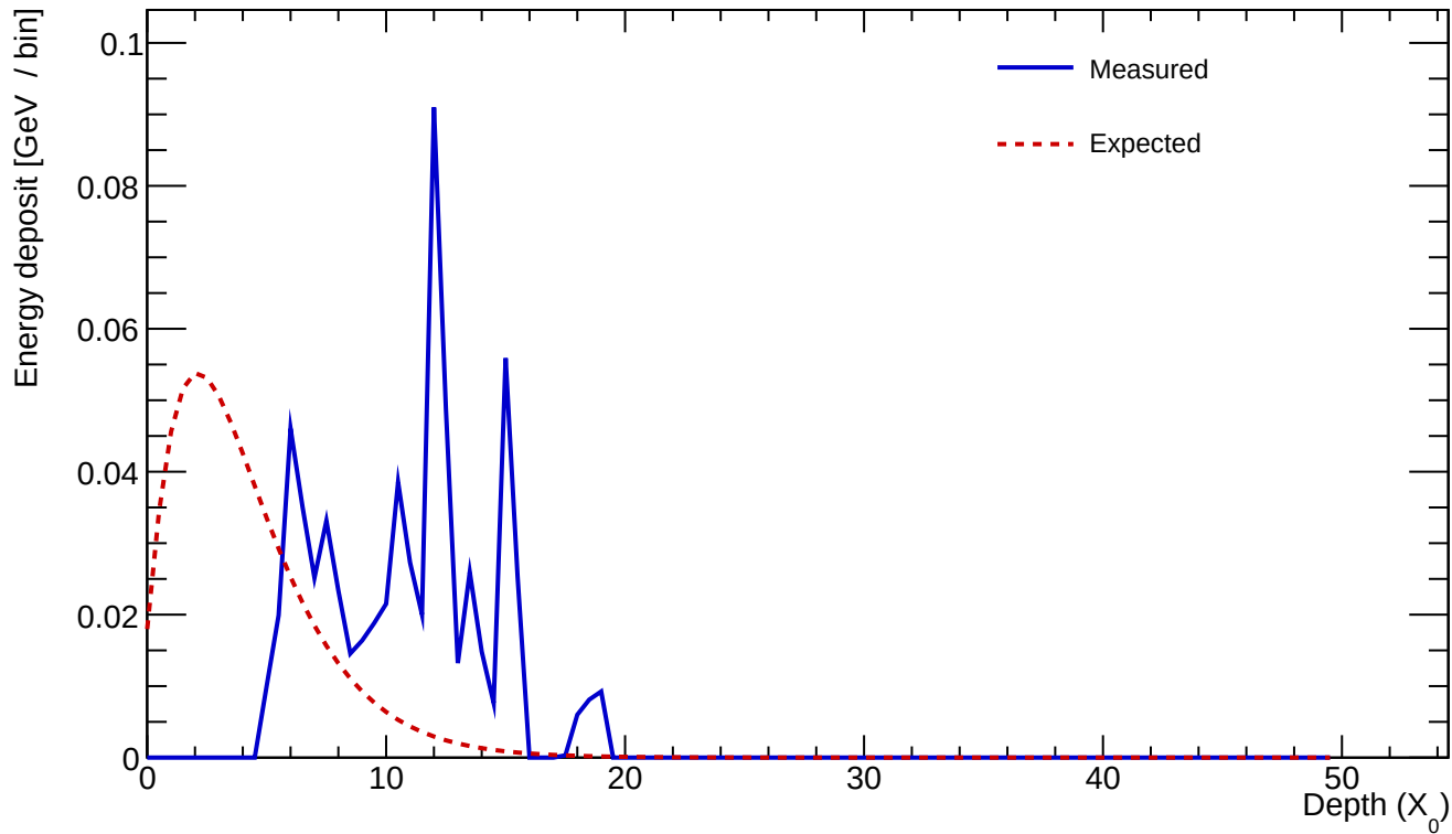
Cluster 1136 E=0.656 GeV profileStart=5.00 X_0 \chi=0.6666
