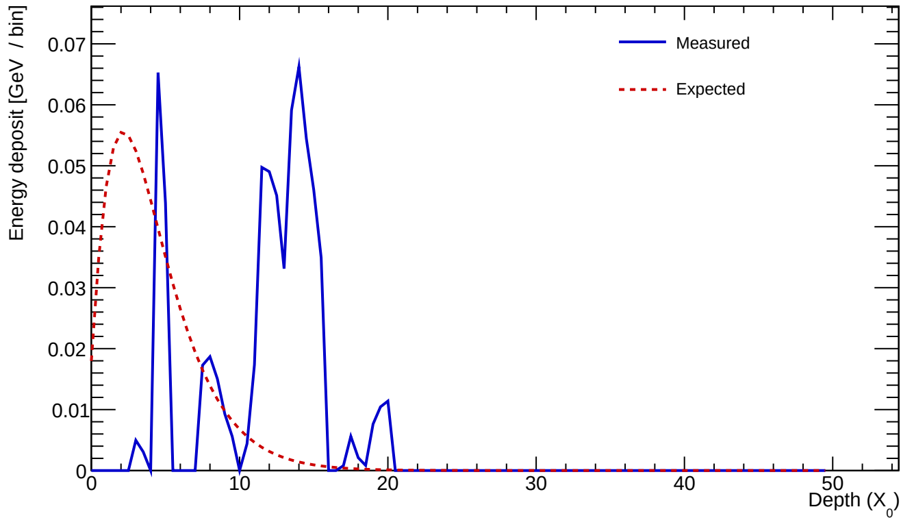
Cluster 412 E=0.681 GeV profileStart=11.00 X_0 \chi=0.6087
