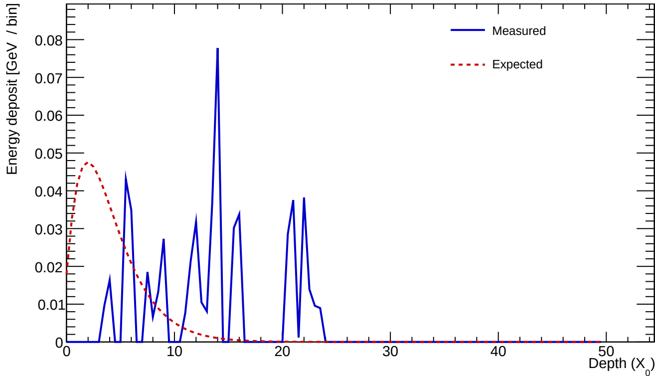
Cluster 263 E=0.565 GeV profileStart=11.50 X_0 \chi=1.1155
