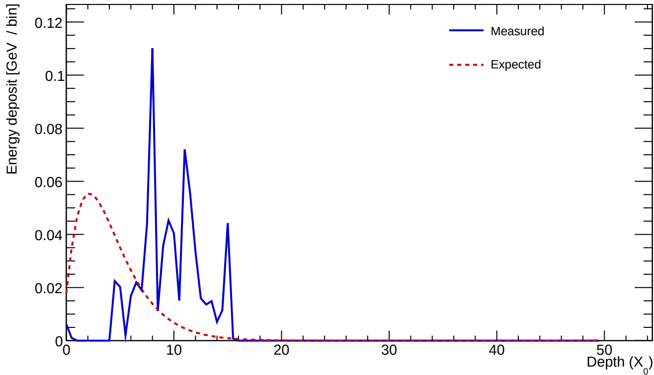
Cluster 454 E=0.681 GeV profileStart=6.00 X_0 \chi=0.5501
