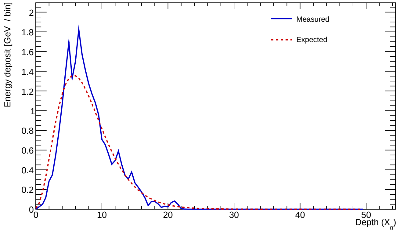
Cluster 520 E=24.682 GeV profileStart=0.50 X_0 \chi=0.1573
