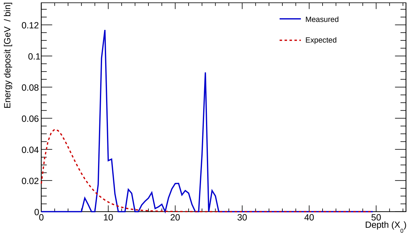
Cluster 83 E=0.642 GeV profileStart=7.00 X_0 \chi=1.1066
