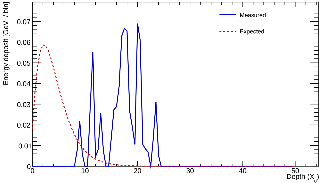
Cluster 703 E=0.730 GeV profileStart=15.00 X_0 \chi=0.6426
