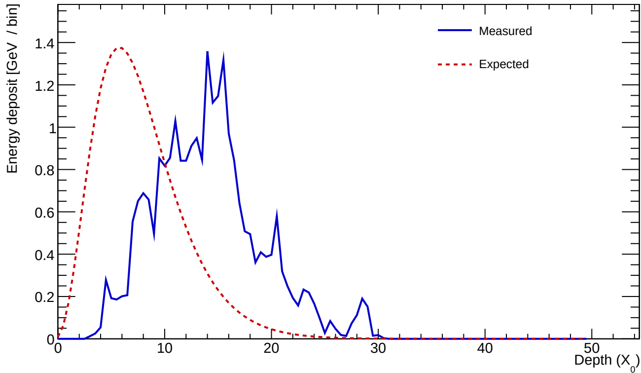
Cluster 360 E=25.065 GeV profileStart=6.50 X_0 \chi=0.3380
