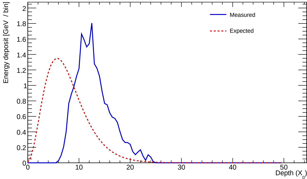
Cluster 561 E=24.526 GeV profileStart=5.50 X_0 \chi=0.1339
