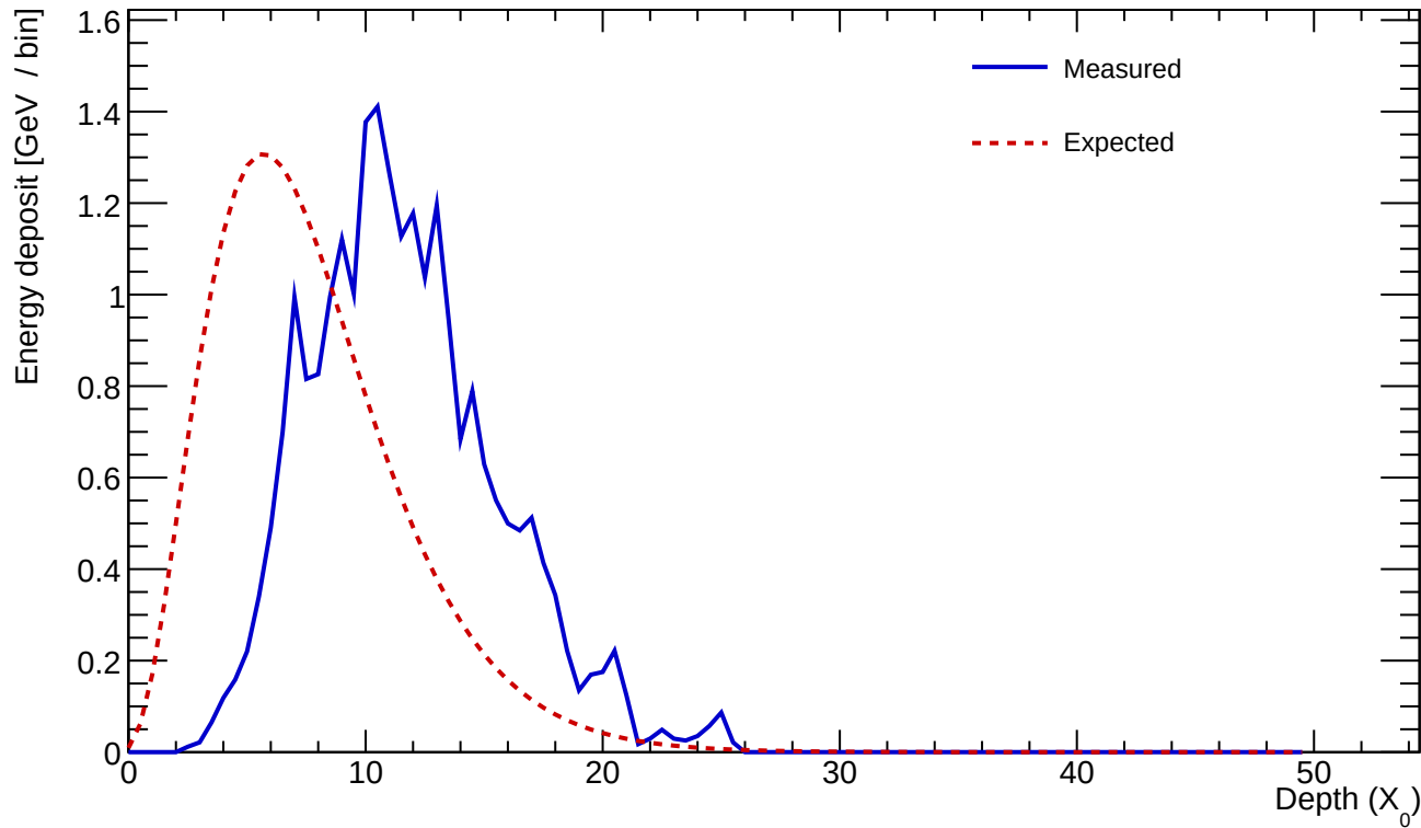
Cluster 467 E=23.720 GeV profileStart=4.00 X_0 \chi=0.1476
