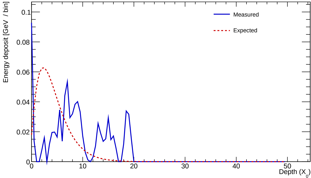
Cluster 840 E=0.791 GeV profileStart=4.00 X_0 \chi=0.7816
