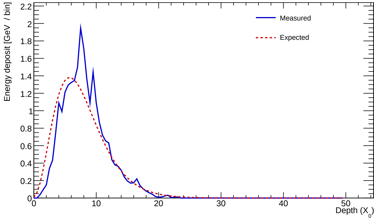
Cluster 189 E=25.136 GeV profileStart=1.00 X_0 \chi=0.1578
