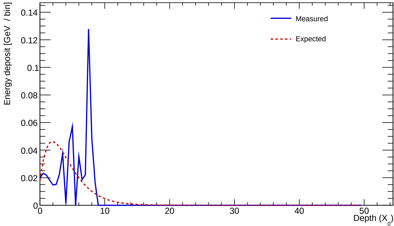
Cluster 638 E=0.547 GeV profileStart=2.50 X_0 \chi=0.6714
