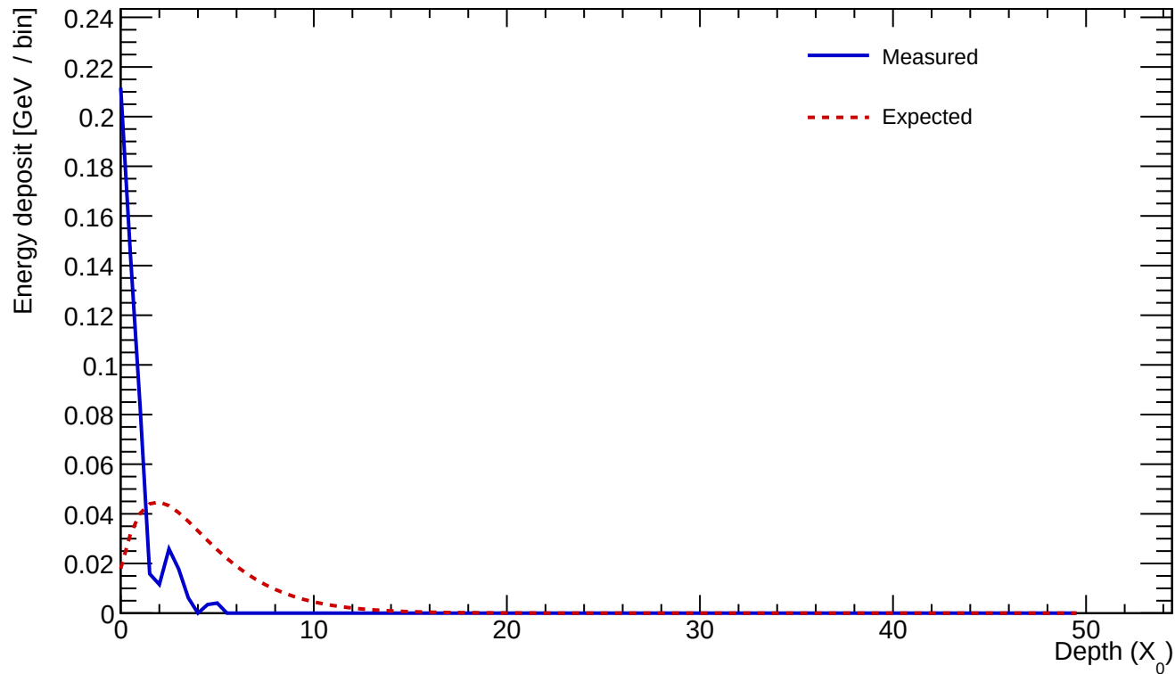
Cluster 56 E=0.525 GeV profileStart=4.50 X_0 \chi=1.0132
