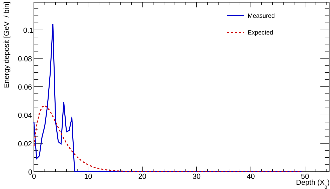
Cluster 22 E=0.552 GeV profileStart=1.00 X_0 \chi=0.3904
