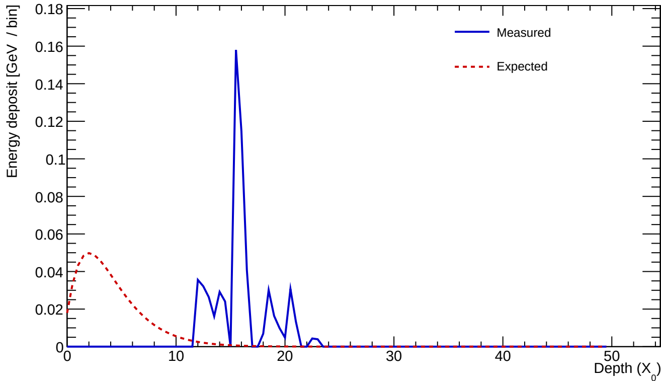
Cluster 448 E=0.597 GeV profileStart=12.00 X_0 \chi=0.8200
