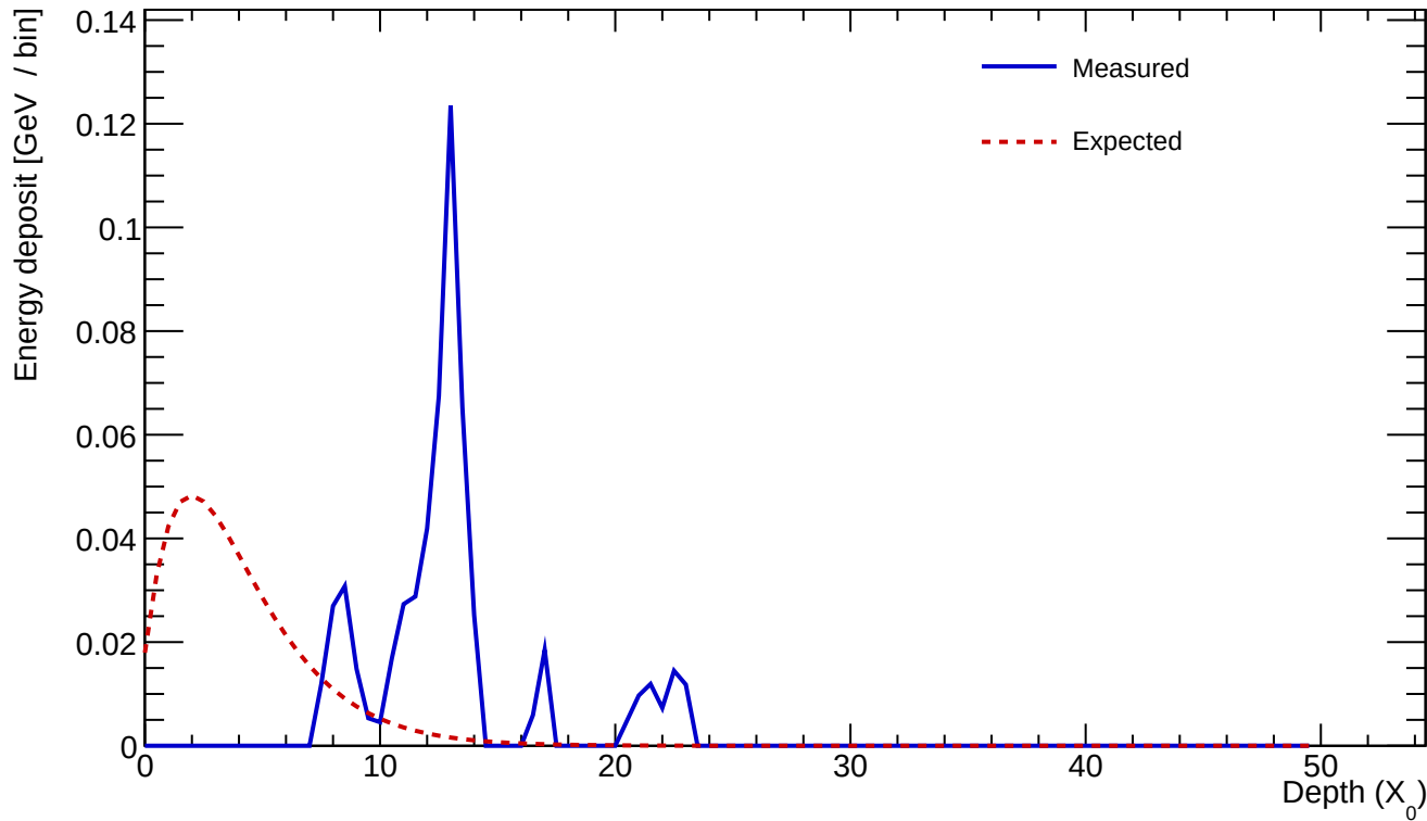
Cluster 459 E=0.575 GeV profileStart=10.50 X_0 \chi=0.8400
