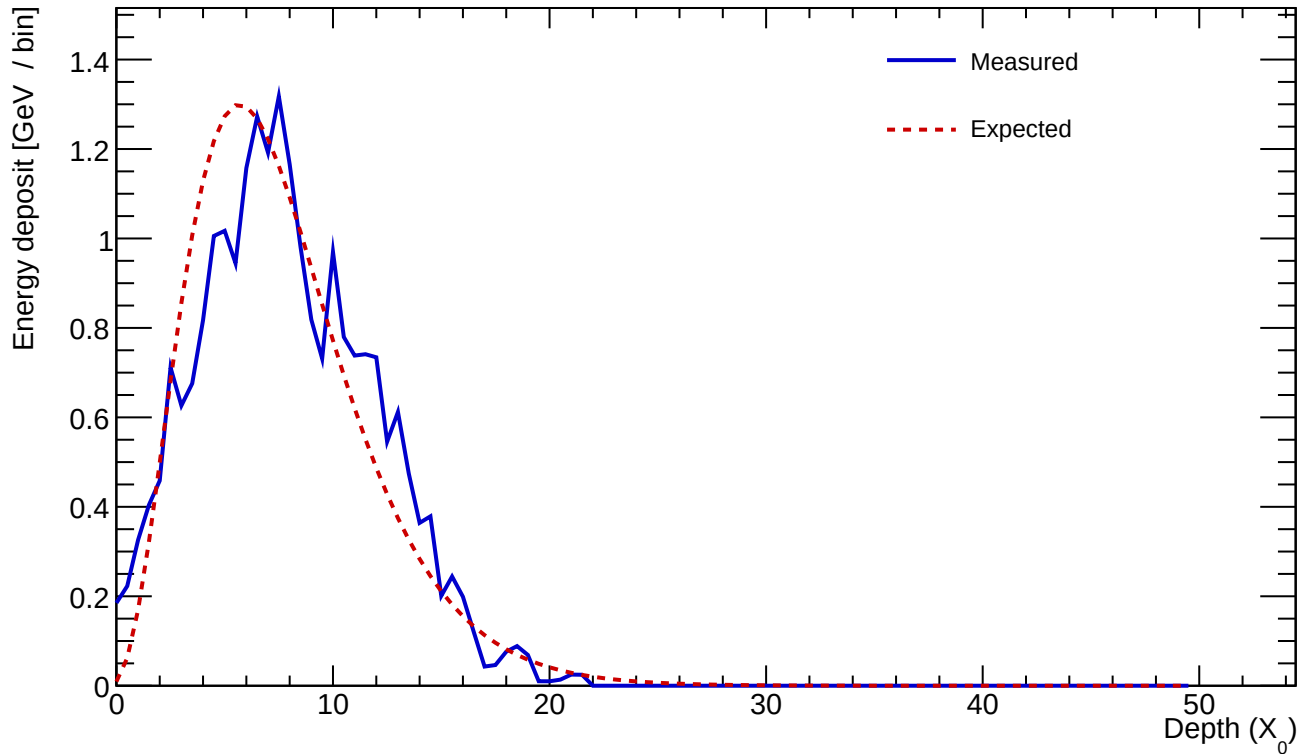
Cluster 227 E=23.540 GeV profileStart=1.00 X_0 \chi=0.1915
