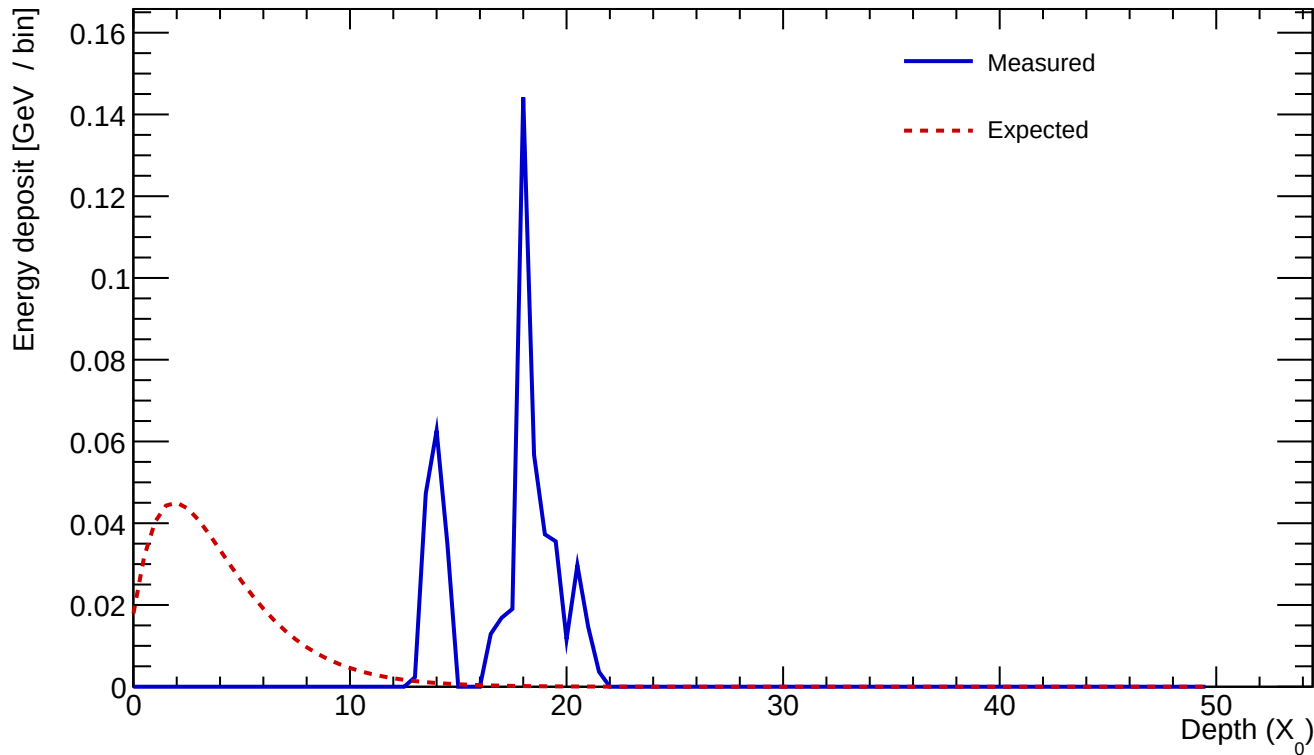
Cluster 281 E=0.529 GeV profileStart=16.50 X_0 \chi=0.6725
