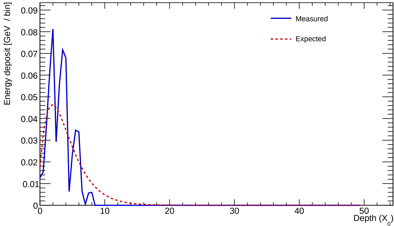
Cluster 44 E=0.548 GeV profileStart=0.50 X_0 \chi=0.4636
