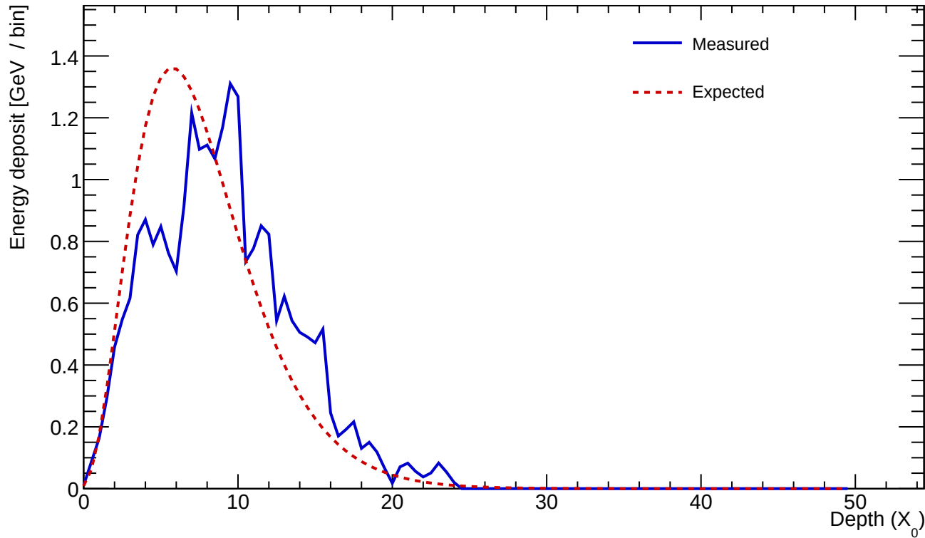
Cluster 163 E=24.761 GeV profileStart=1.00 X_0 \chi=0.2624
