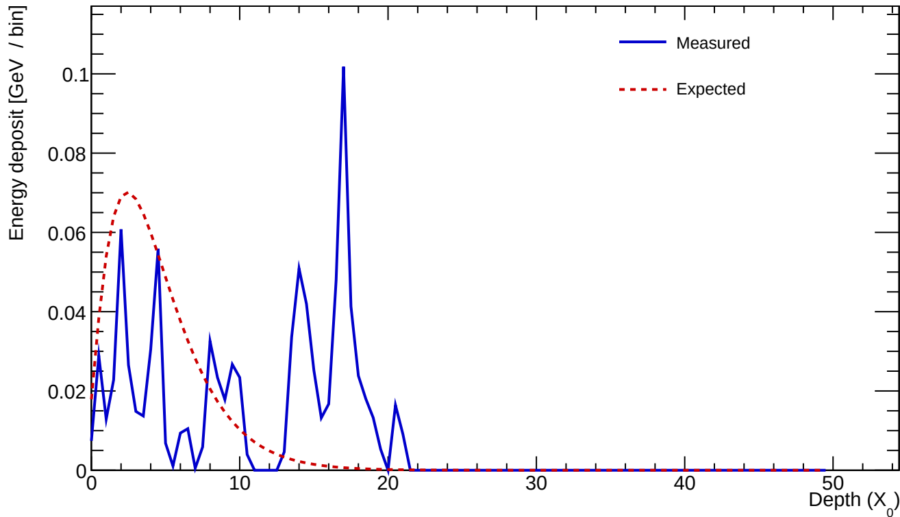
Cluster 1060 E=0.900 GeV profileStart=0.50 X_0 \chi=1.0902
