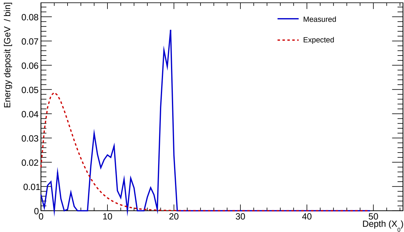
Cluster 824 E=0.582 GeV profileStart=7.50 X_0 \chi=1.0247
