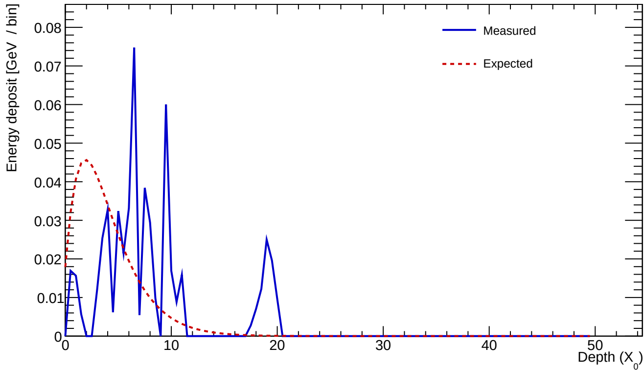
Cluster 697 E=0.537 GeV profileStart=3.00 X_0 \chi=0.7684
