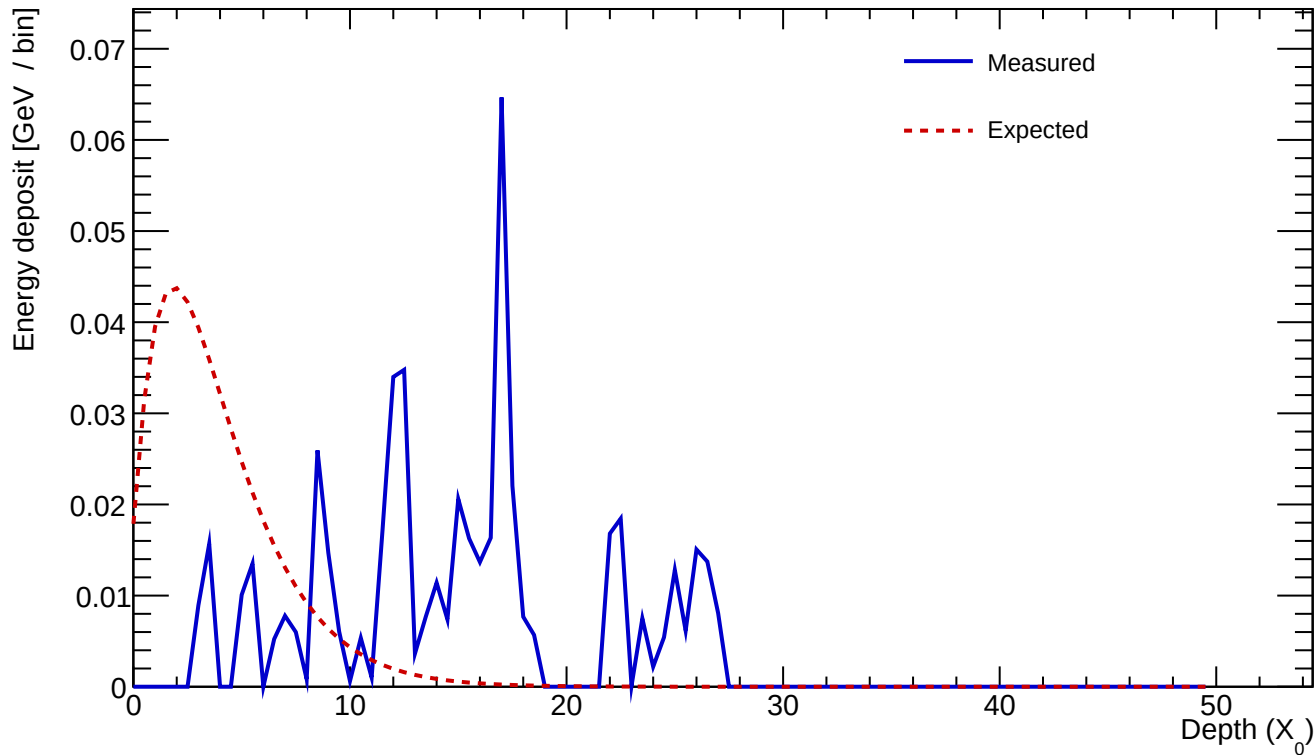
Cluster 524 E=0.511 GeV profileStart=11.50 X_0 \chi=1.0068
