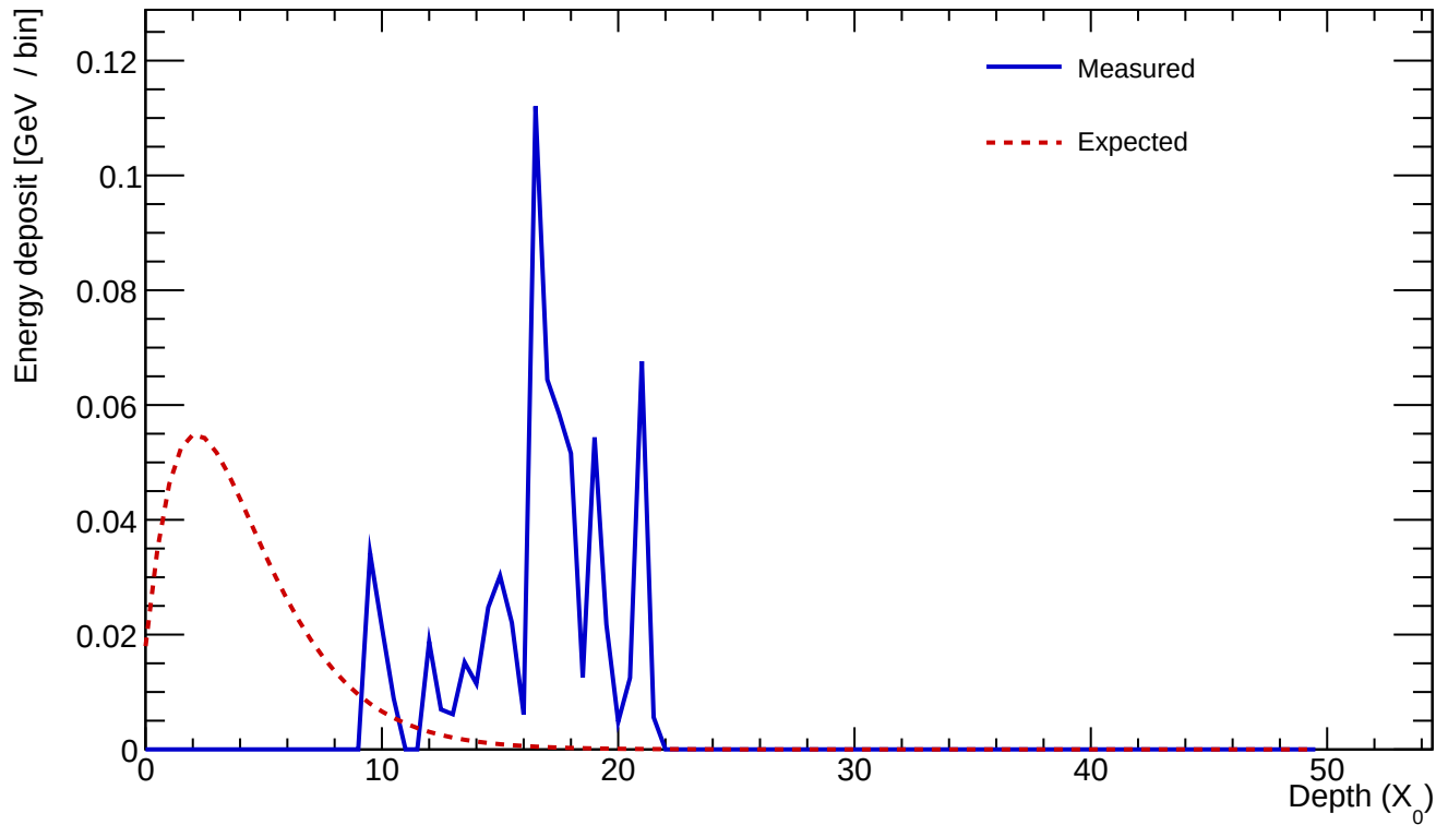
Cluster 564 E=0.672 GeV profileStart=14.50 X_0 \chi=0.6337
