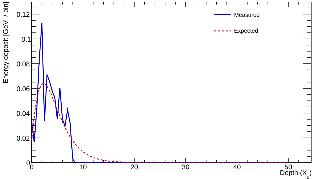
Cluster 1050 E=0.808 GeV profileStart=0.50 X_0 \chi=0.2813
