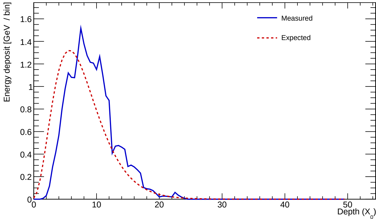
Cluster 594 E=23.945 GeV profileStart=2.00 X_0 \chi=0.1275
