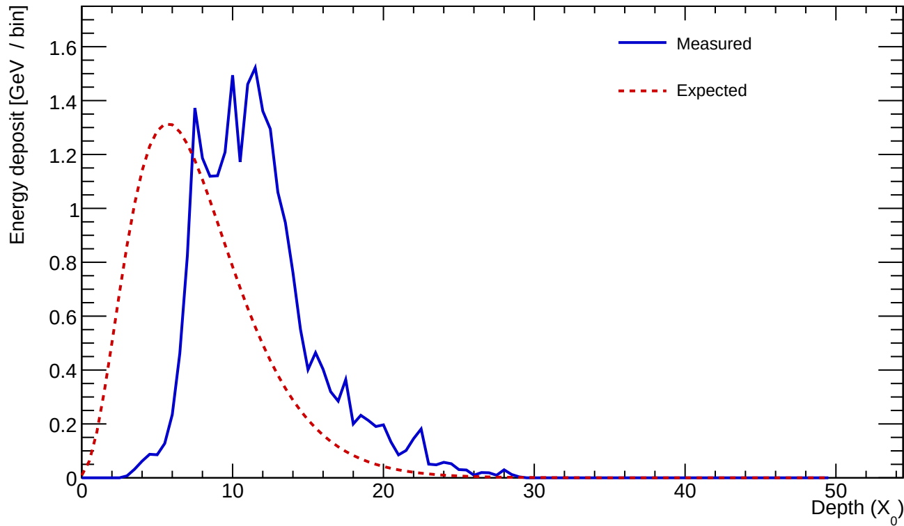
Cluster 636 E=23.841 GeV profileStart=4.50 X_0 \chi=0.1879
