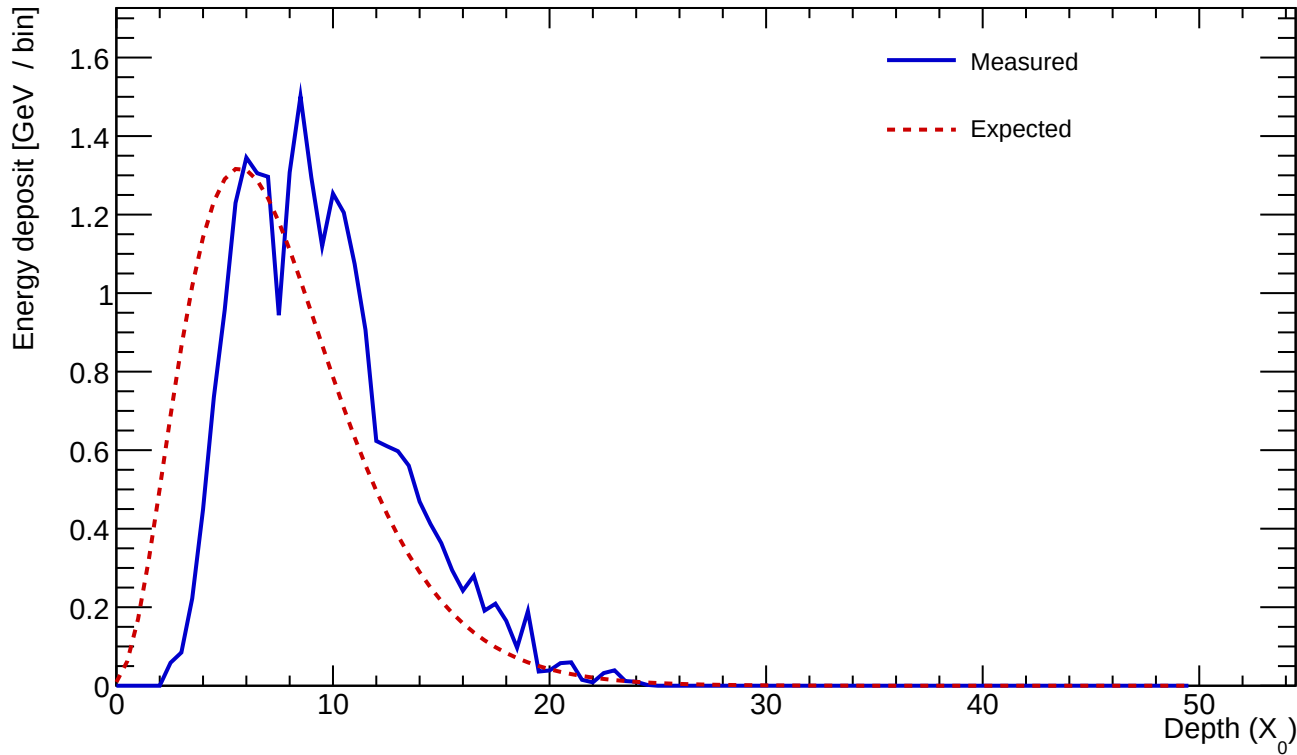
Cluster 342 E=23.905 GeV profileStart=2.00 X_0 \chi=0.1232
