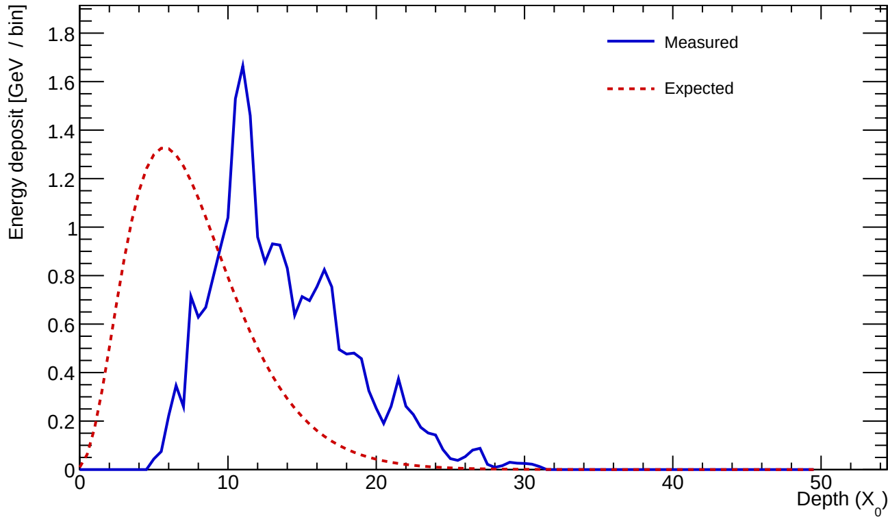
Cluster 816 E=24.089 GeV profileStart=5.50 X_0 \chi=0.2507
