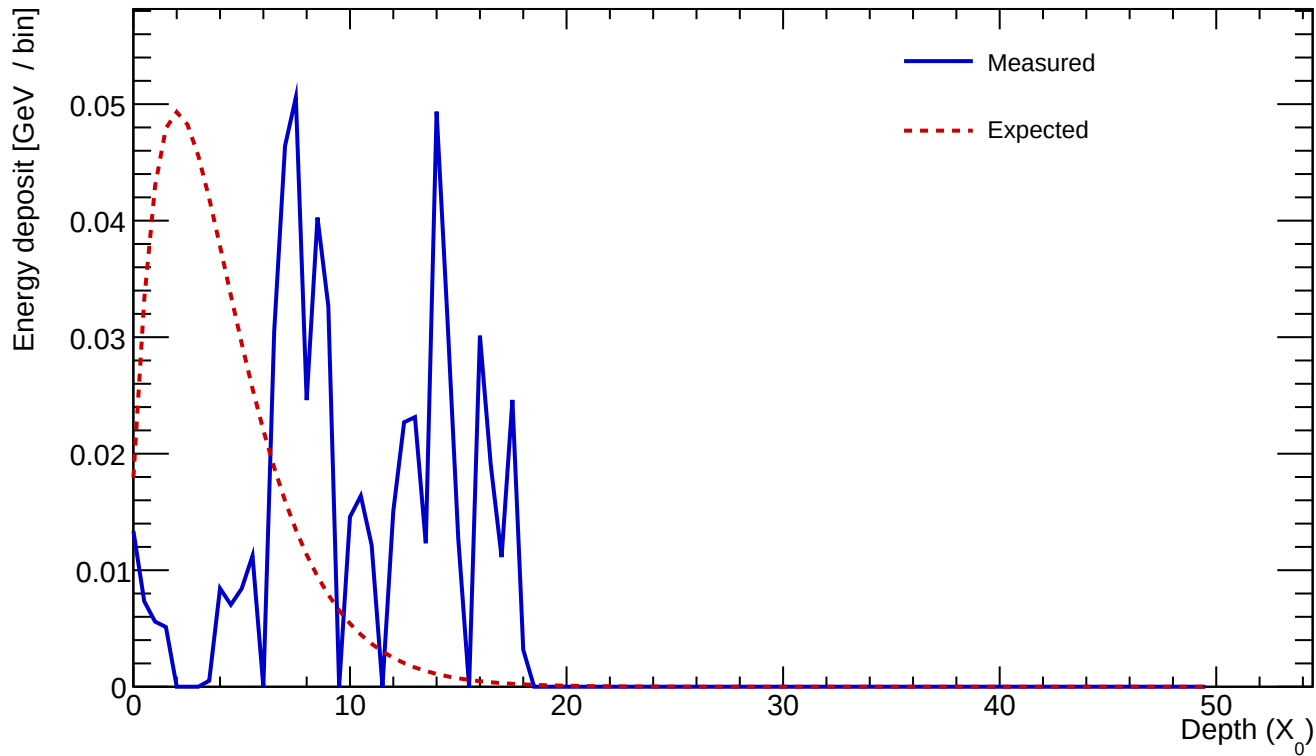
Cluster 261 E=0.590 GeV profileStart=5.50 X_0 \chi=0.7153
