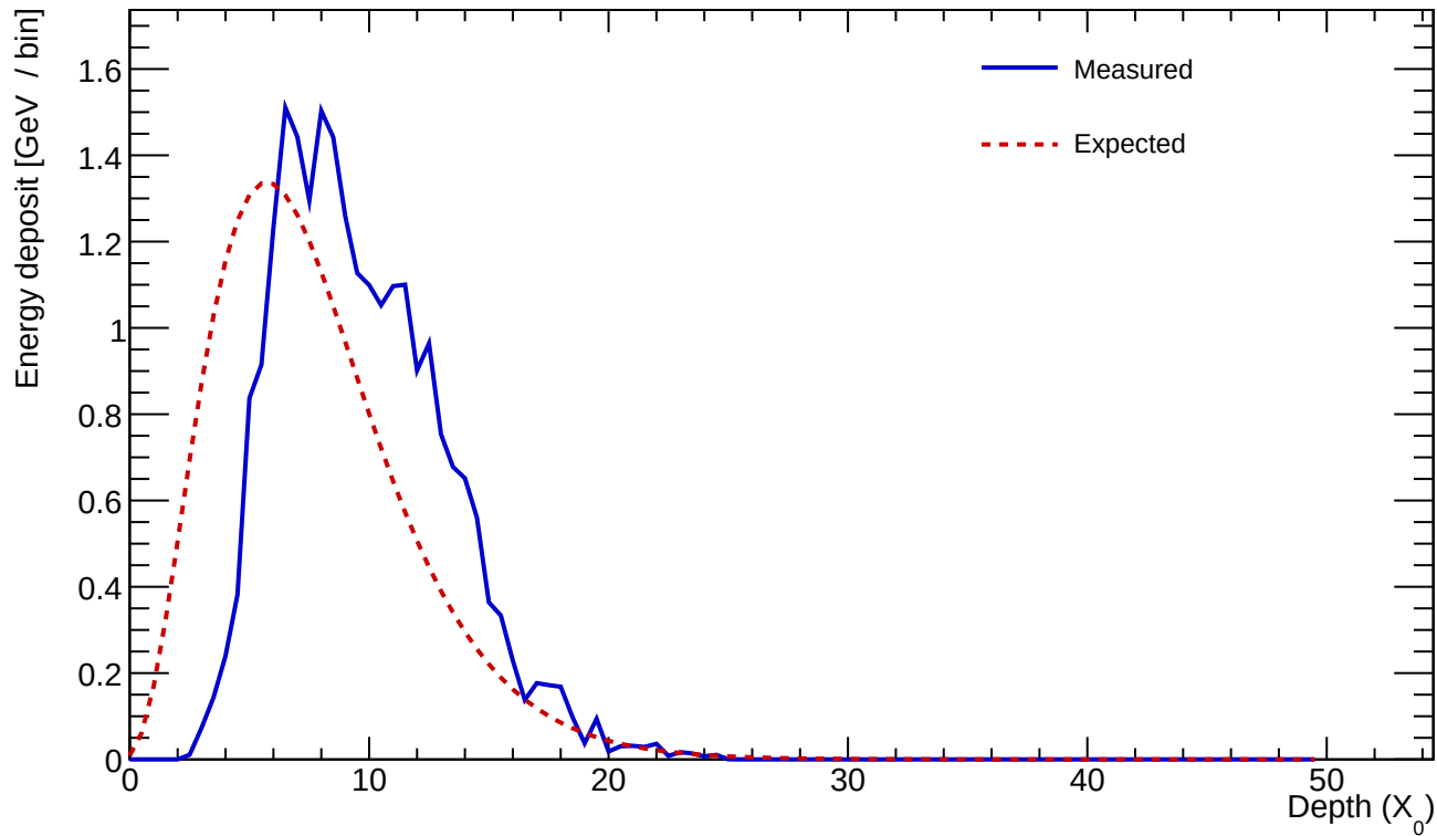
Cluster 722 E=24.285 GeV profileStart=2.50 X_0 \chi=0.1427
