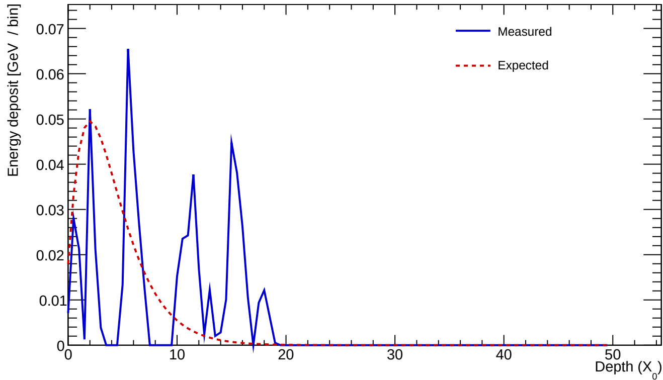
Cluster 15 E=0.592 GeV profileStart=5.00 X_0 \chi=1.0673
