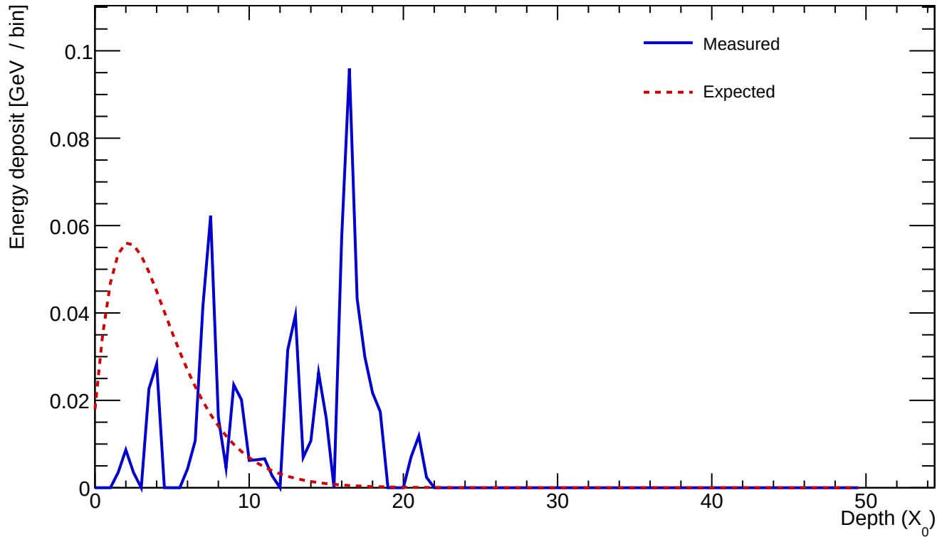
Cluster 765 E=0.690 GeV profileStart=12.50 X_0 \chi=0.9399
