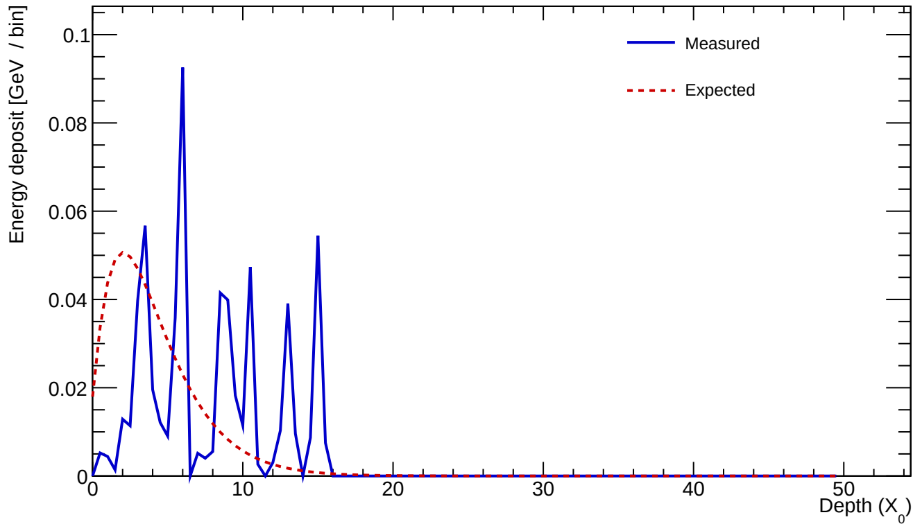
Cluster 67 E=0.609 GeV profileStart=2.00 X_0 \chi=0.8687
