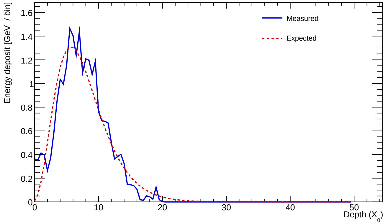
Cluster 828 E=23.685 GeV profileStart=0.50 X_0 \chi=0.1825
