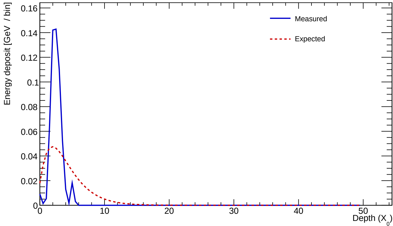
Cluster 461 E=0.564 GeV profileStart=1.00 X_0 \chi=0.7214
