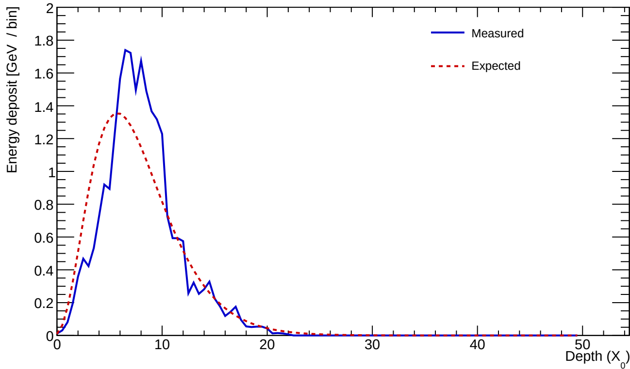
Cluster 566 E=24.641 GeV profileStart=1.00 X_0 \chi=0.2470
