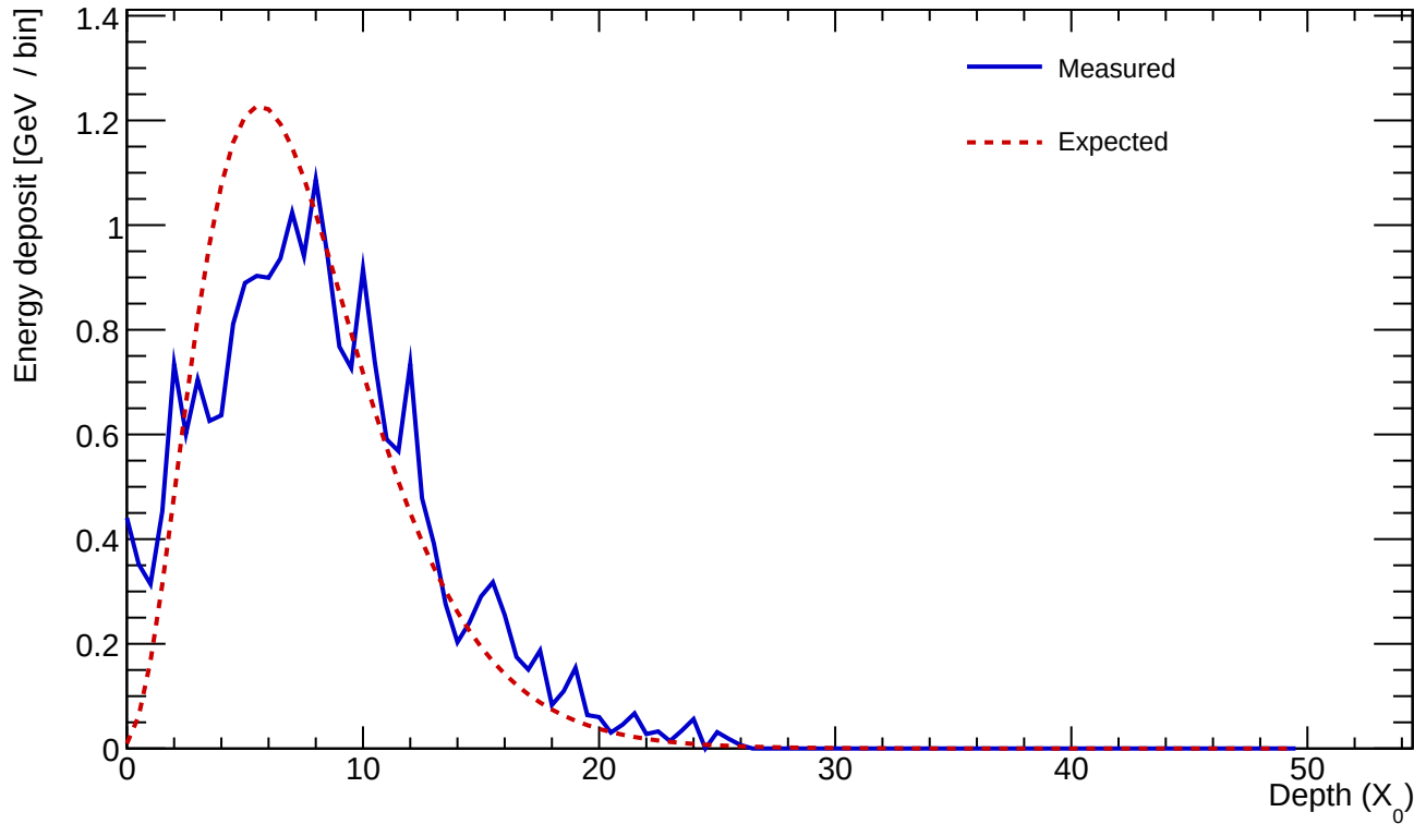
Cluster 120 E=22.137 GeV profileStart=0.50 X_0 \chi=0.2750
