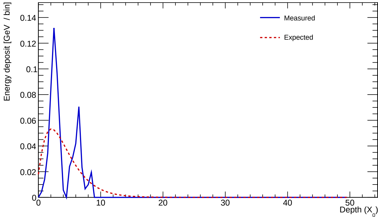
Cluster 1056 E=0.647 GeV profileStart=1.00 X_0 \chi=0.5625
