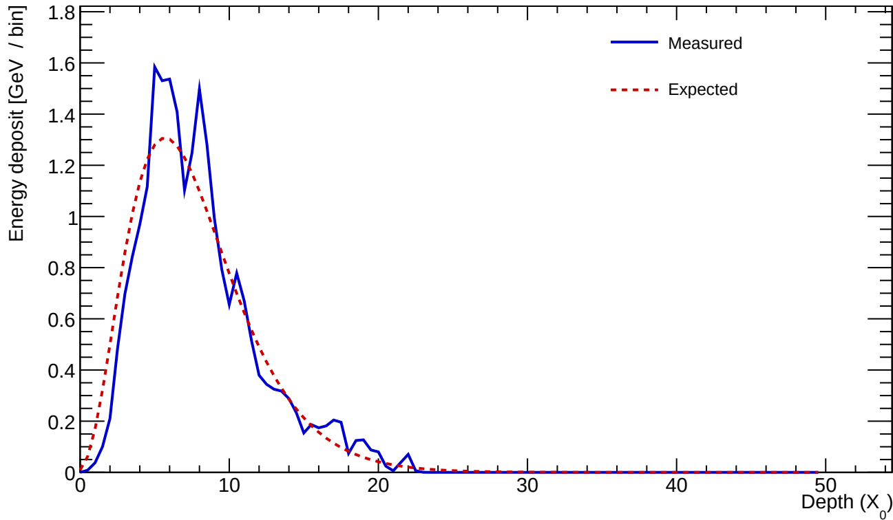
Cluster 778 E=23.679 GeV profileStart=0.50 X_0 \chi=0.1550
