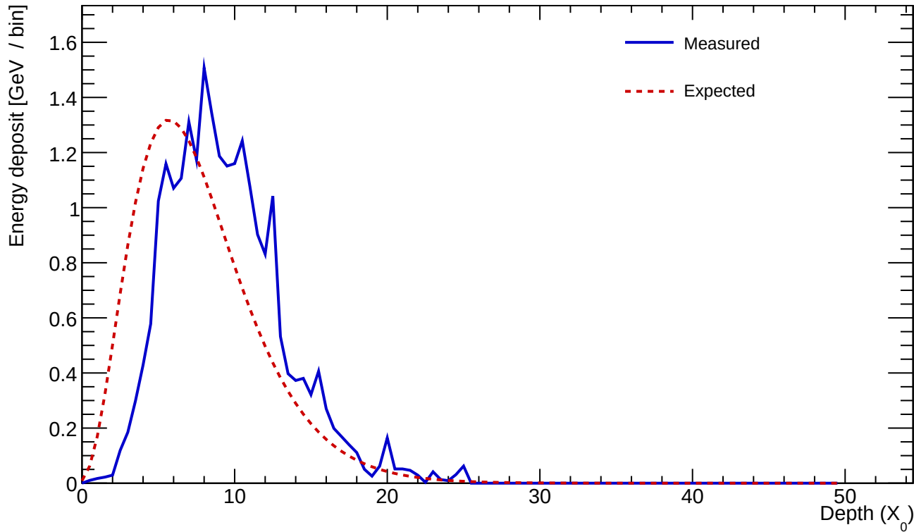
Cluster 245 E=23.917 GeV profileStart=2.00 X_0 \chi=0.1401
