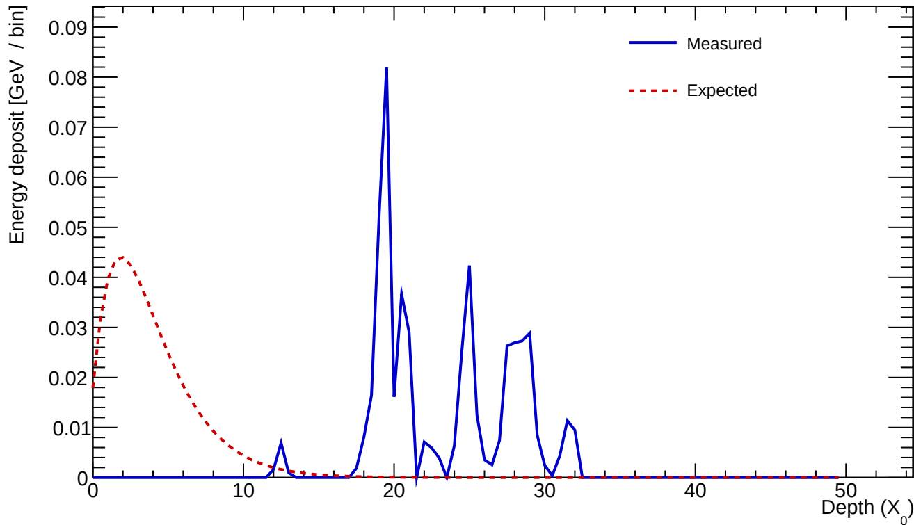
Cluster 788 E=0.514 GeV profileStart=18.00 X_0 \chi=0.8481
