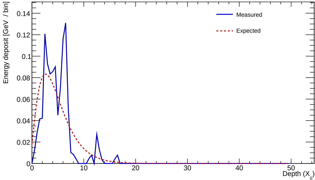
Cluster 512 E=1.104 GeV profileStart=1.00 X_0 \chi=0.4733
