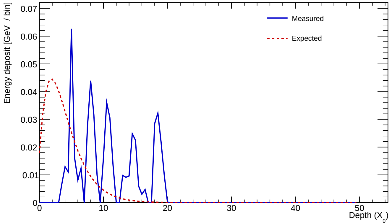
Cluster 442 E=0.521 GeV profileStart=4.00 X_0 \chi=0.8866
