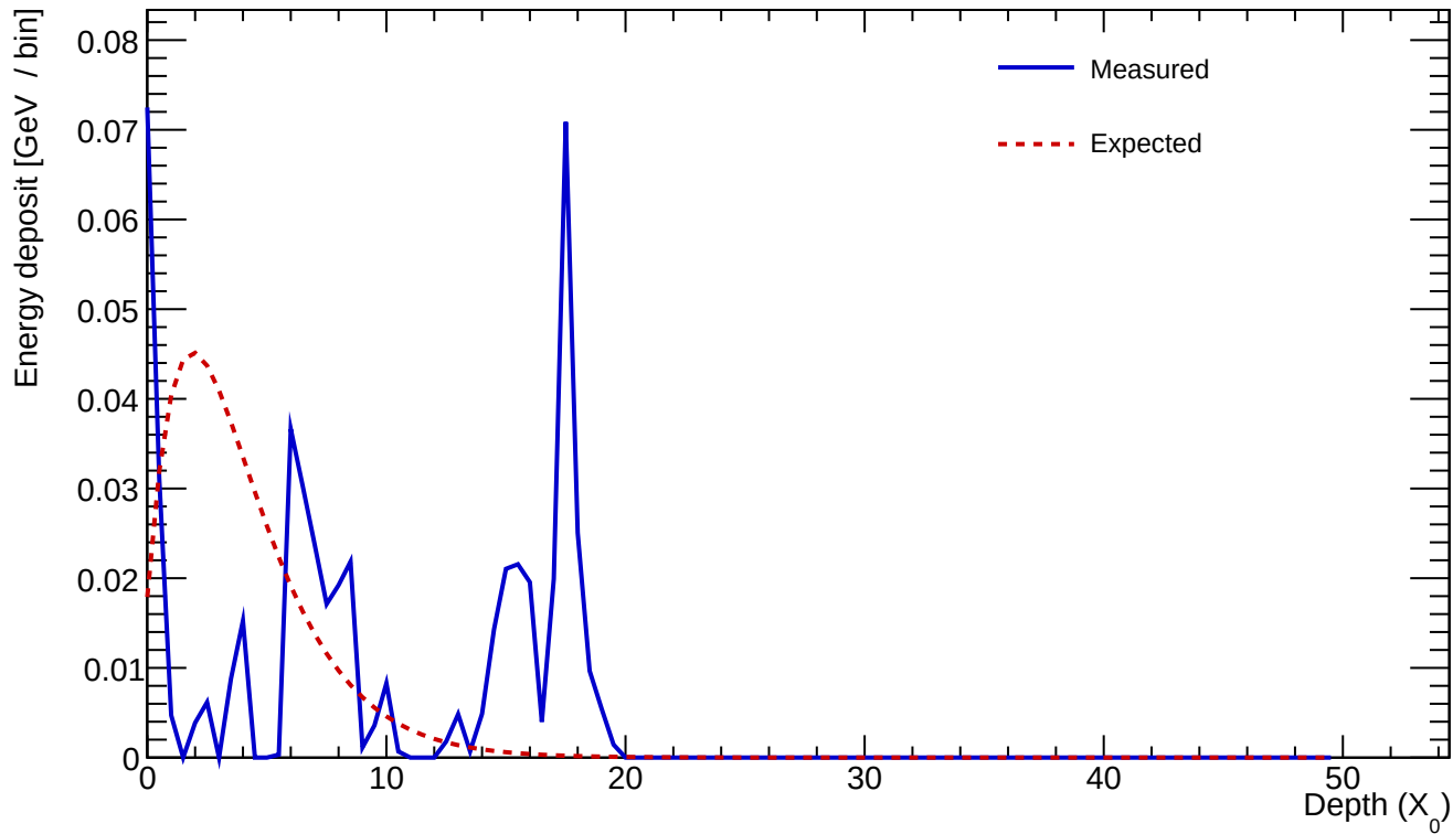
Cluster 815 E=0.530 GeV profileStart=3.50 X_0 \chi =1.1889
