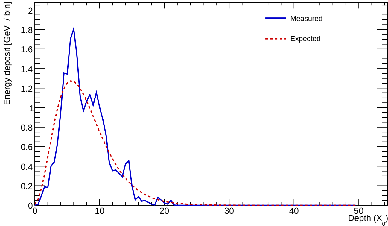
Cluster 529 E=23.055 GeV profileStart=0.50 X_0 \chi=0.2260
