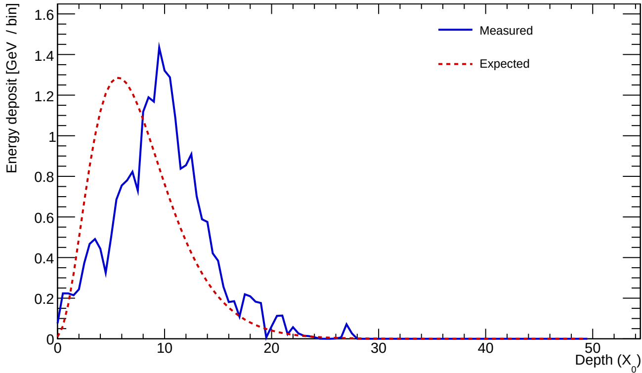
Cluster 113 E=23.295 GeV profileStart=3.00 X_0 \chi=0.2721
