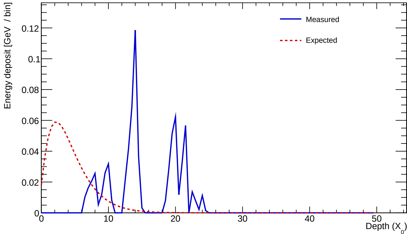
Cluster 555 E=0.733 GeV profileStart=12.00 X_0 \chi=1.0786
