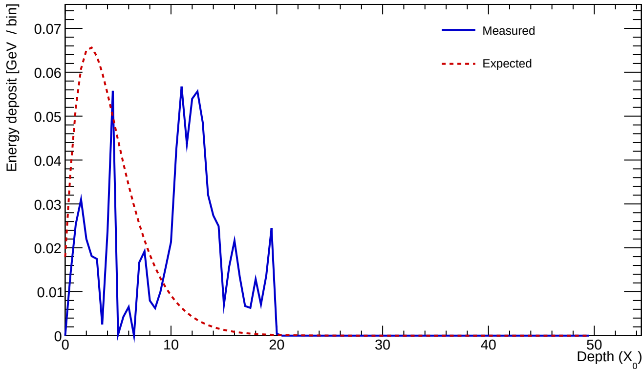
Cluster 1093 E=0.833 GeV profileStart=9.00 X_0 \chi=0.6599
