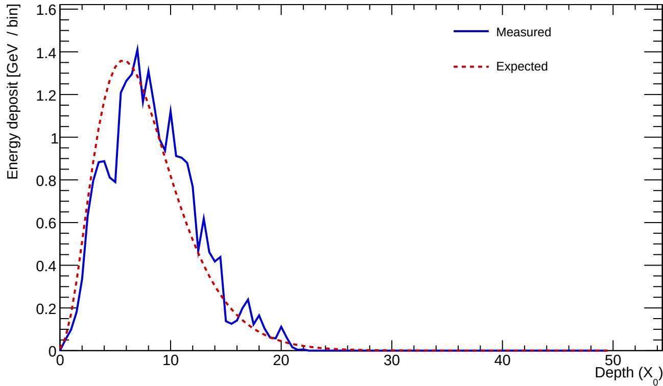
Cluster 557 E=24.737 GeV profileStart=0.50 X_0 \chi=0.1610
