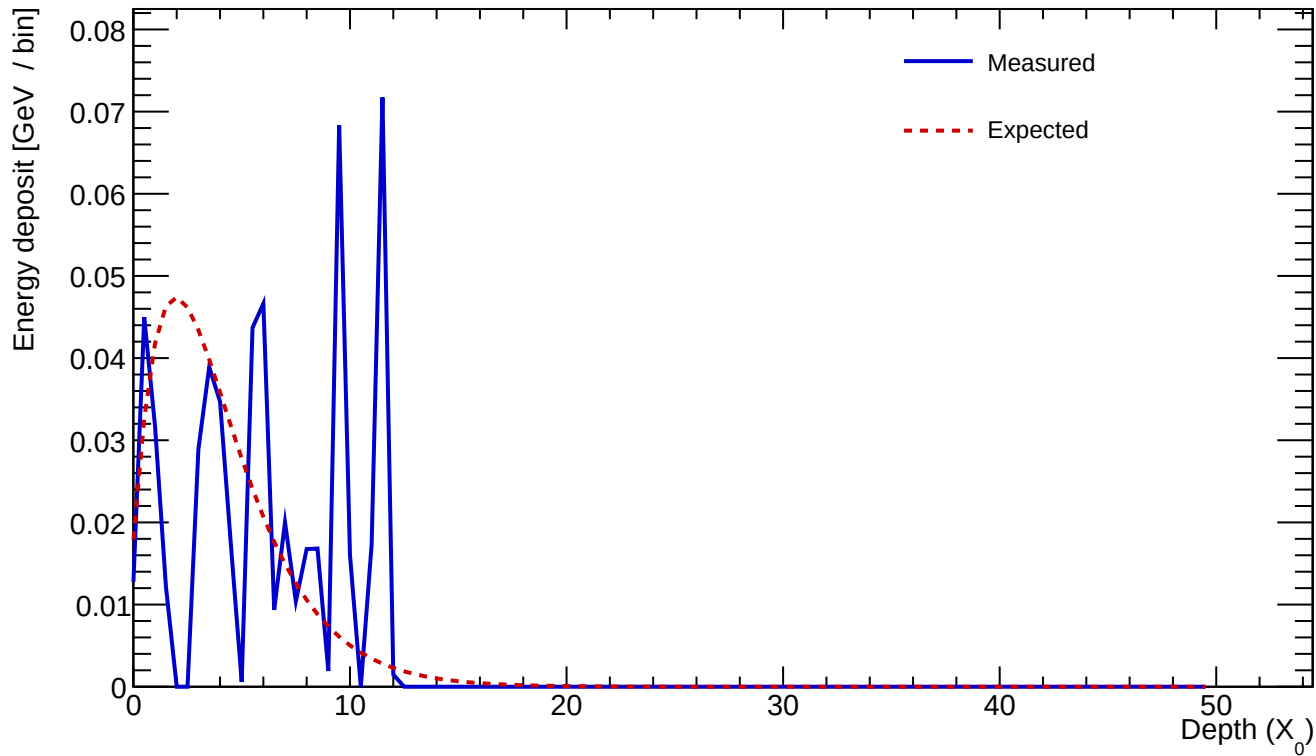
Cluster 218 E=0.563 GeV profileStart=2.50 X_0 \chi=0.7882
