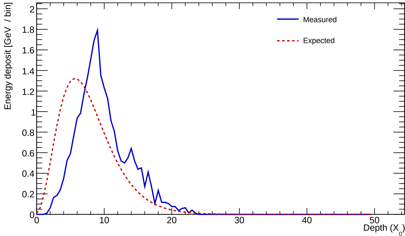
Cluster 937 E=23.972 GeV profileStart=2.50 X_0 \chi=0.1682
