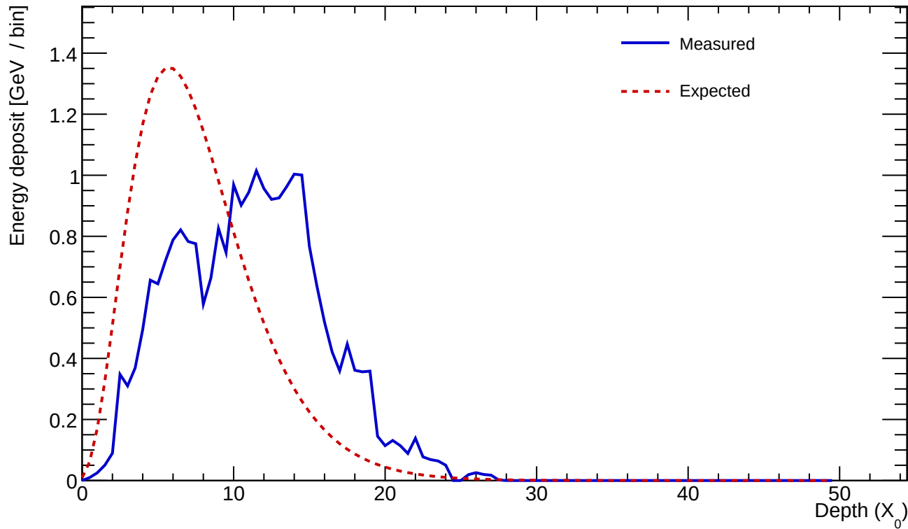
Cluster 364 E=24.601 GeV profileStart=3.50 X_0 \chi=0.3756
