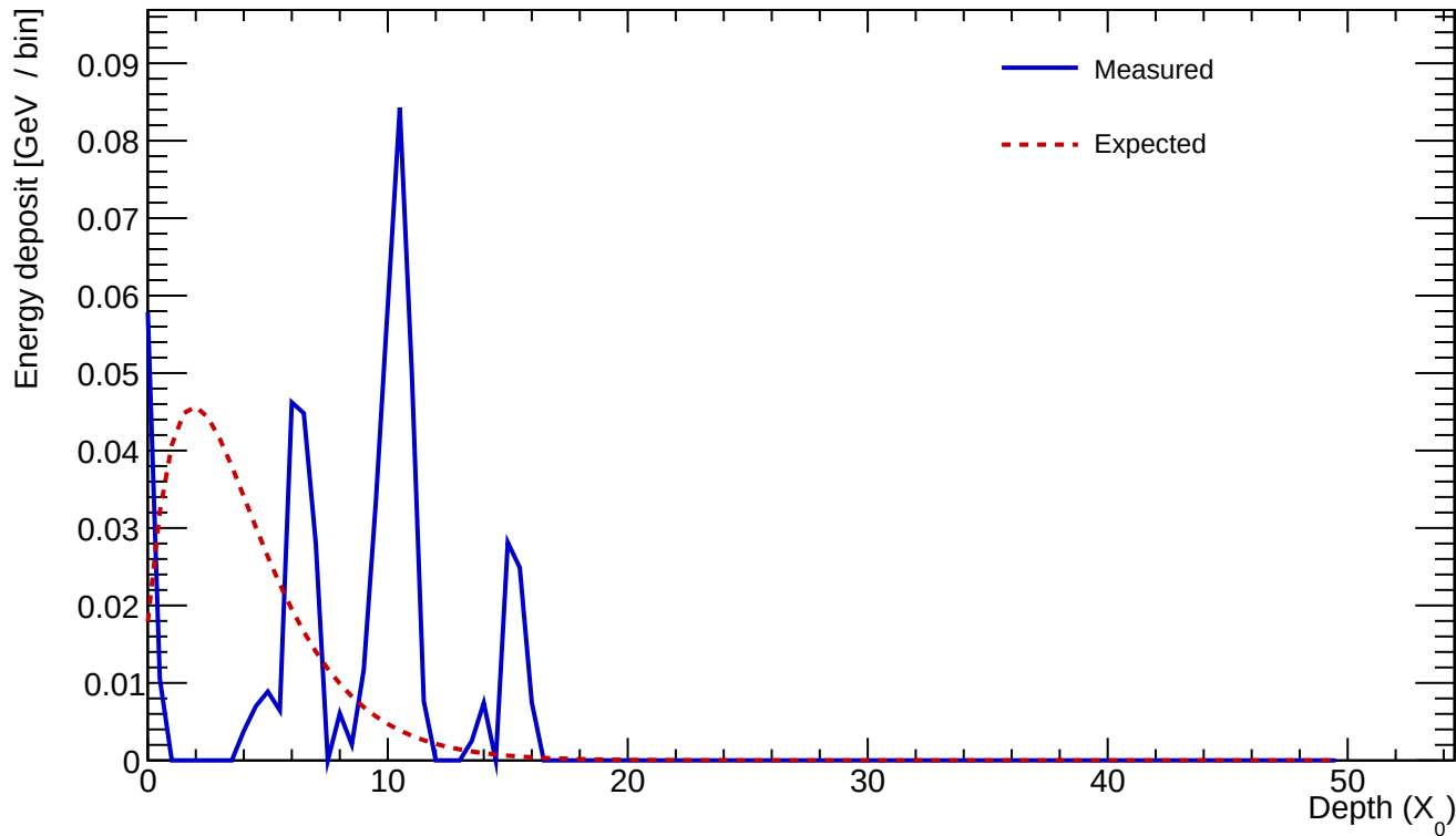
Cluster 497 E=0.538 GeV profileStart=5.00 X_0 \chi=0.9367
