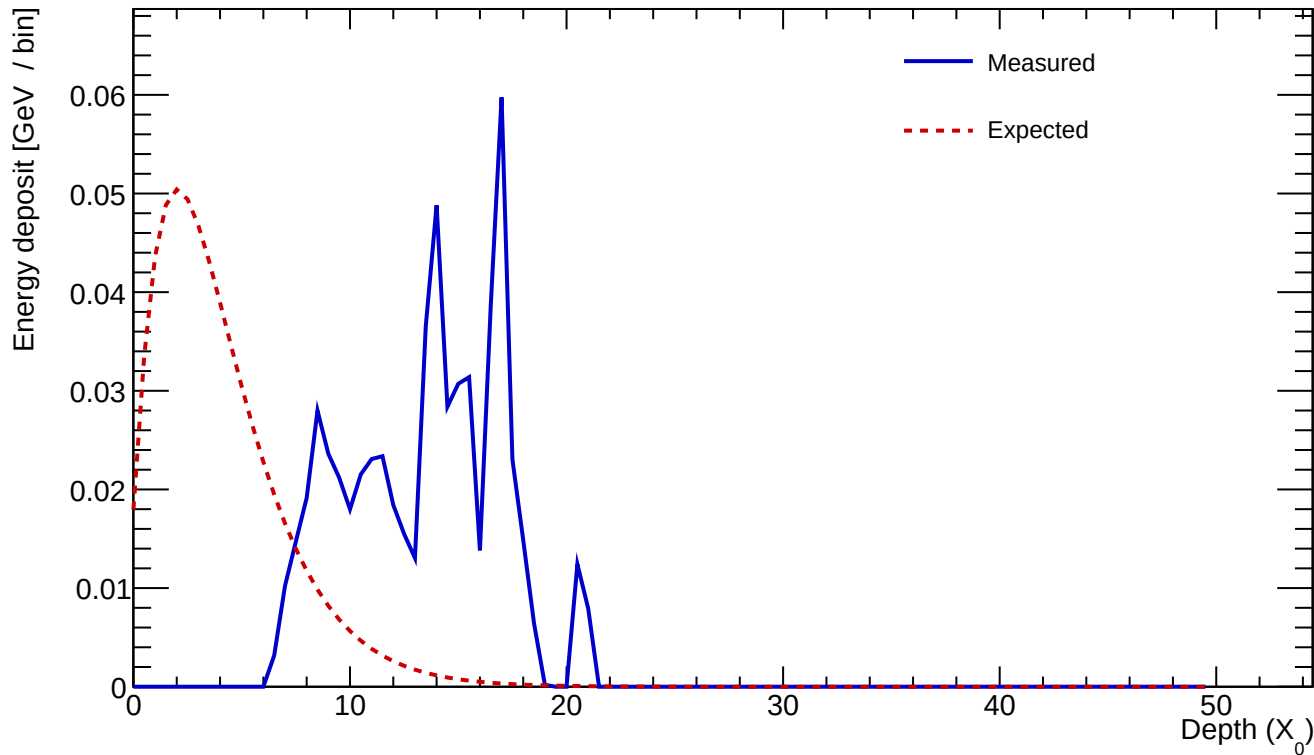
Cluster 464 E=0.606 GeV profileStart=10.50 X_0 \chi=0.6903
