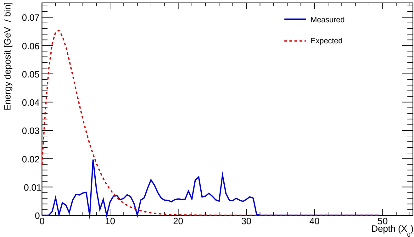
Cluster 858 E=0.828 GeV profileStart=31.00 X_0 \chi=1.0145
