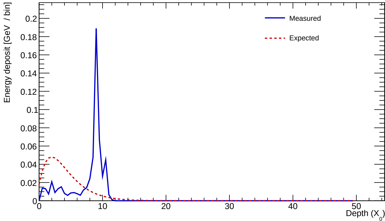
Cluster 241 E=0.571 GeV profileStart=7.50 X_0 \chi=0.6705
