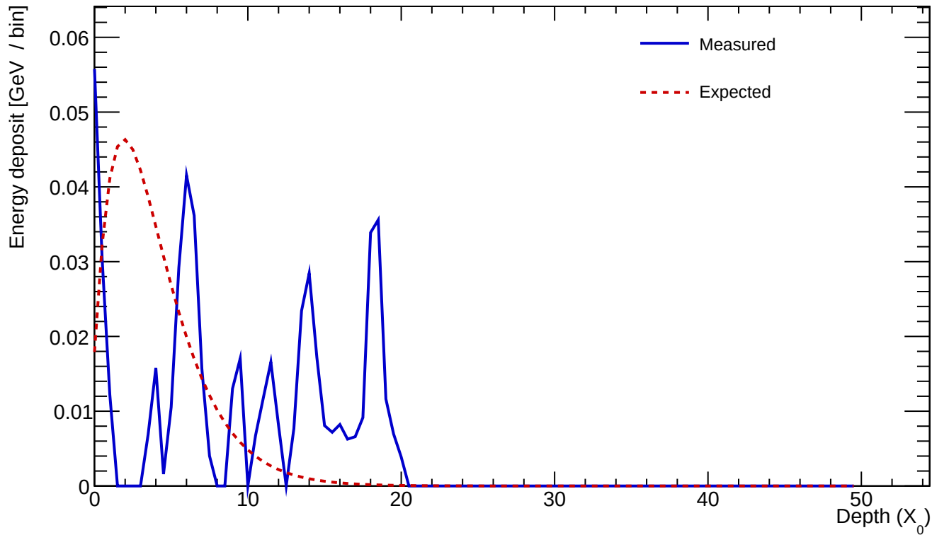
Cluster 950 E=0.547 GeV profileStart=5.00 X_0 \chi=1.0264
