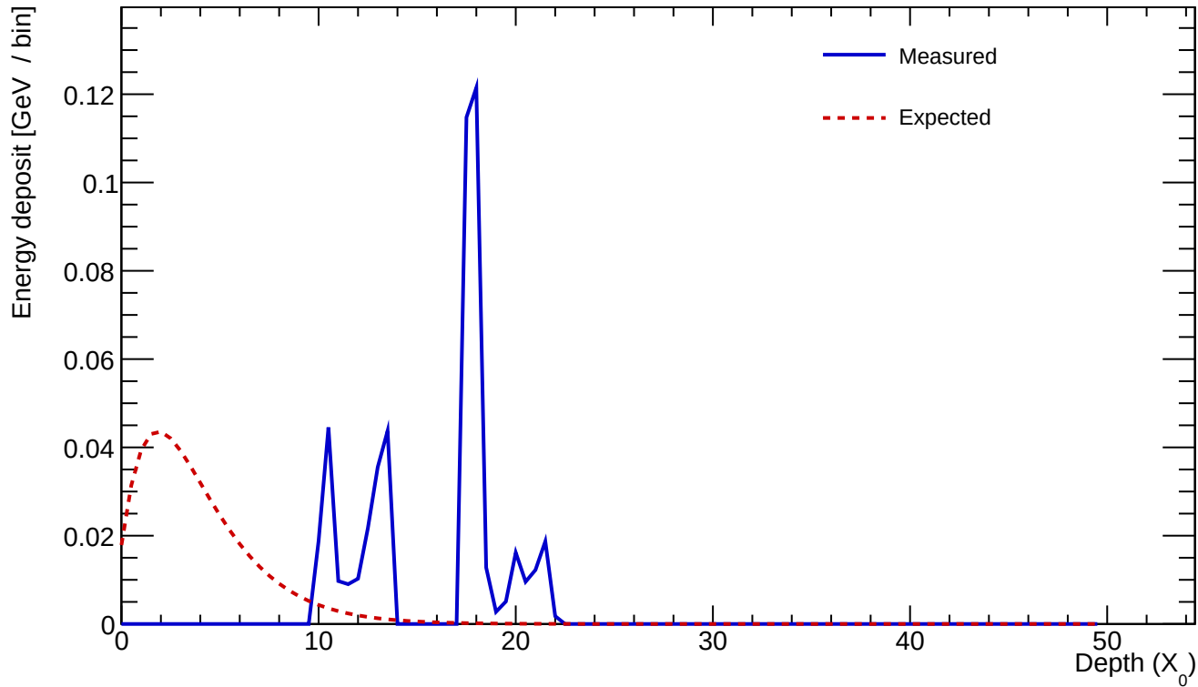
Cluster 98 E=0.509 GeV profileStart=10.00 X_0 \chi=1.1089
