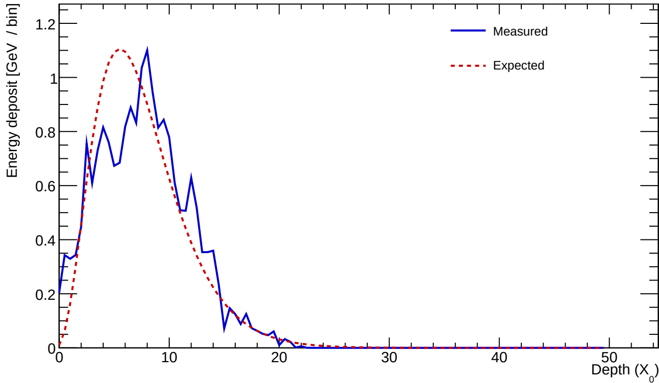
Cluster 841 E=19.751 GeV profileStart=0.50 X_0 \chi=0.2314
