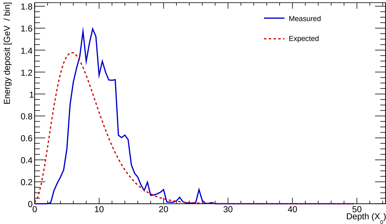
Cluster 368 E=25.100 GeV profileStart=2.50 X_0 \chi=0.1697
