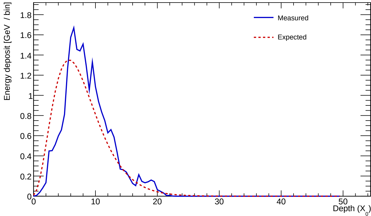
Cluster 672 E=24.547 GeV profileStart=1.50 X_0 \chi=0.1686
