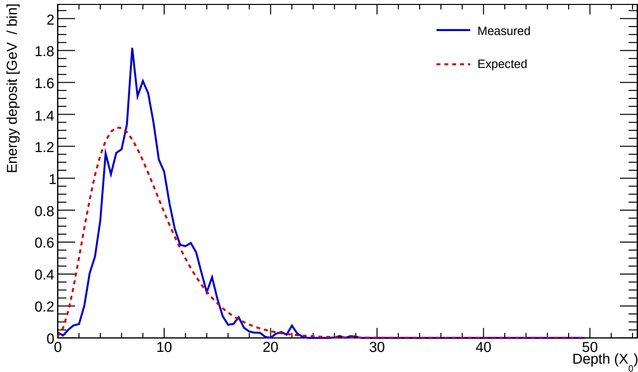
Cluster 834 E=23.927 GeV profileStart=1.50 X_0 \chi=0.1885
