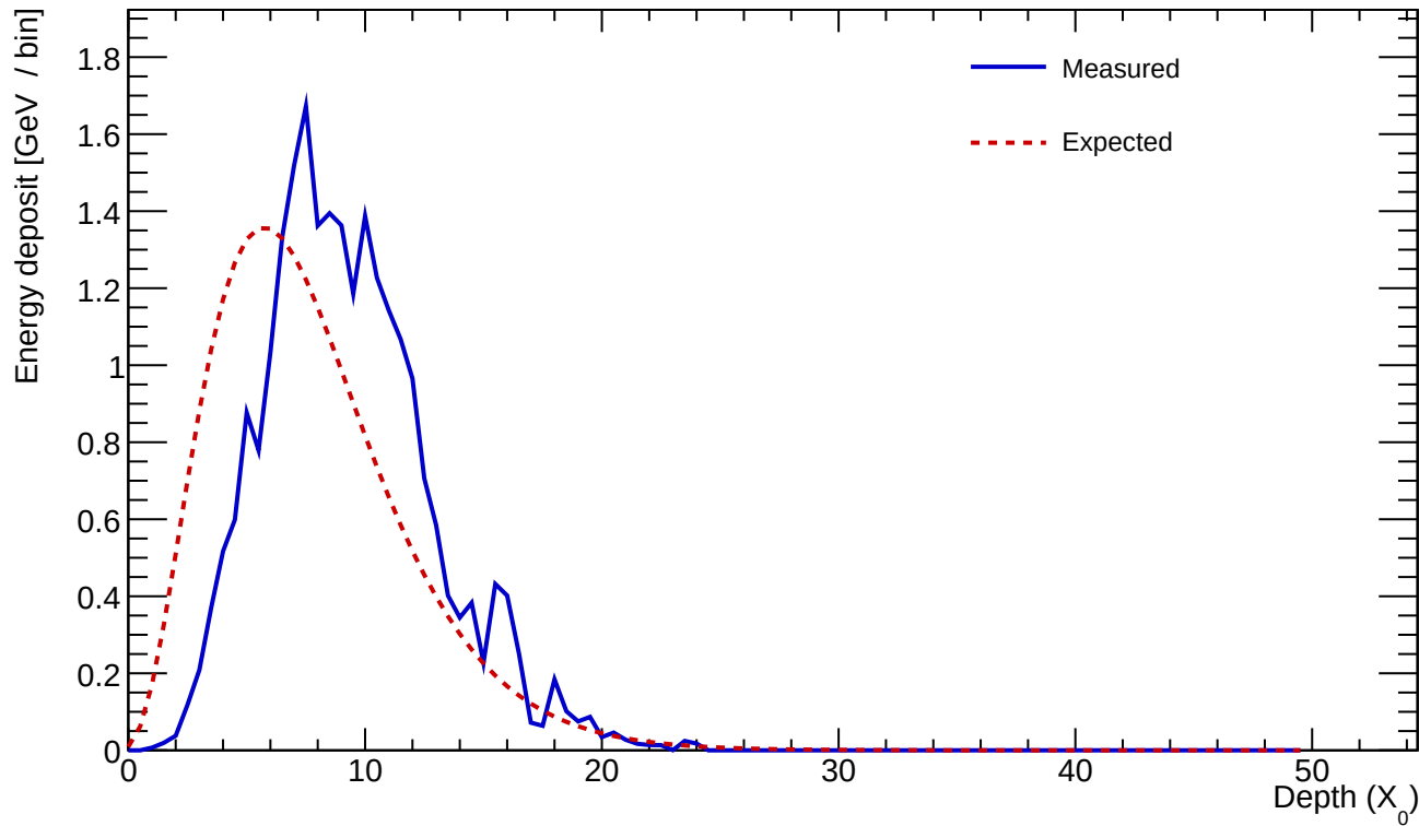
Cluster 425 E=24.695 GeV profileStart=2.00 X_0 \chi=0.1570
