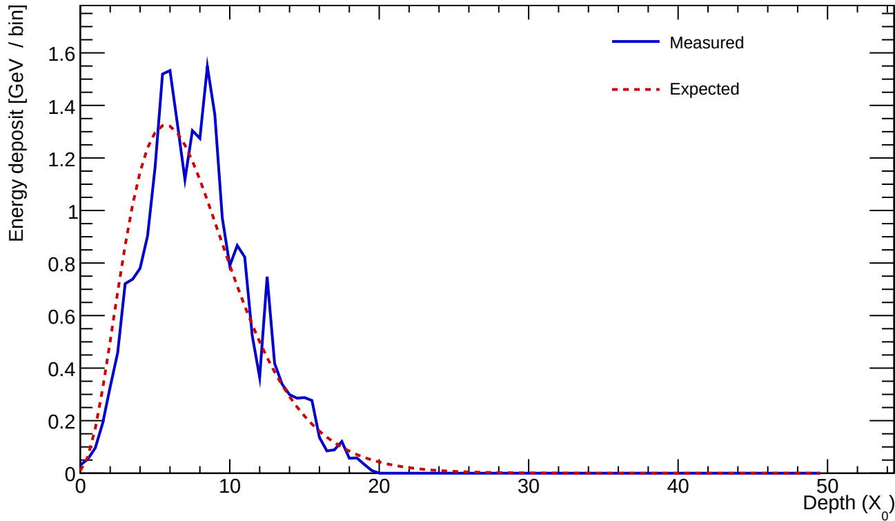
Cluster 605 E=24.040 GeV profileStart=0.50 X_0 \chi=0.1561
