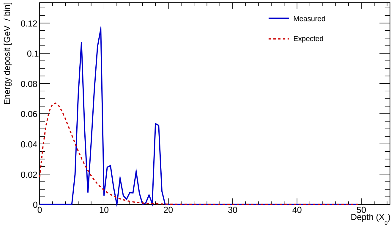
Cluster 558 E=0.853 GeV profileStart=5.00 X_0 \chi=0.7151
