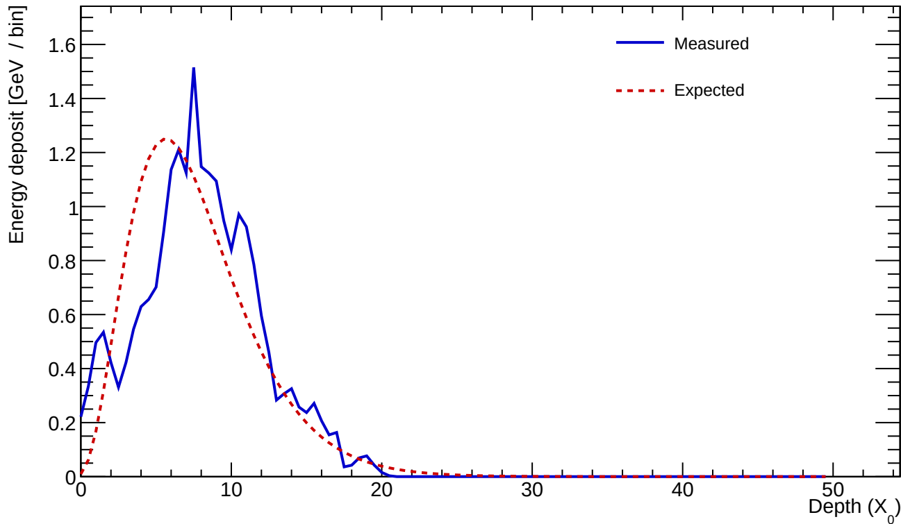
Cluster 701 E=22.569 GeV profileStart=1.00 X_0 \chi=0.2266
