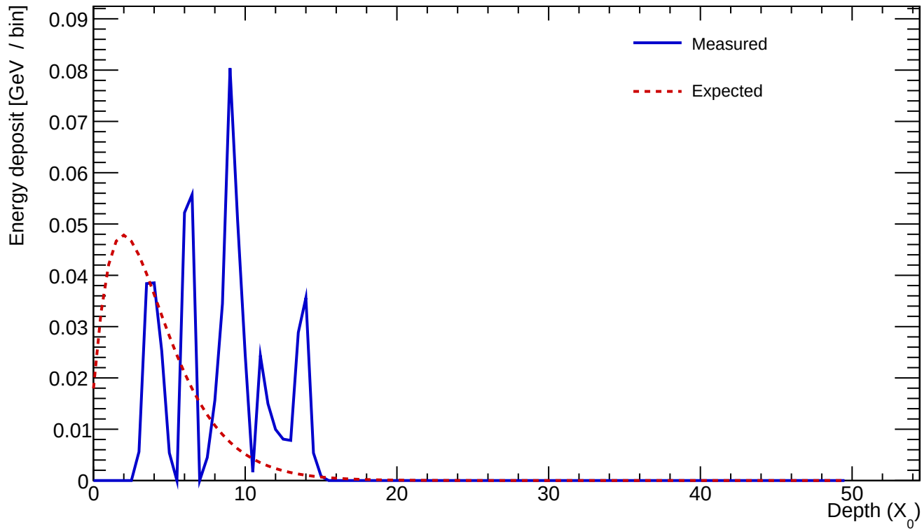
Cluster 465 E=0.569 GeV profileStart=3.50 X_0 \chi=0.7594
