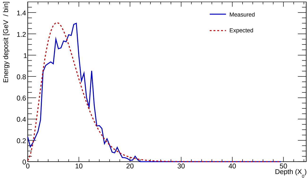
Cluster 812 E=23.669 GeV profileStart=0.50 X_0 \chi=0.1861
