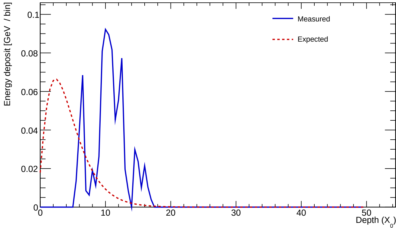
Cluster 272 E=0.843 GeV profileStart=8.00 X_0 \chi=0.5141
