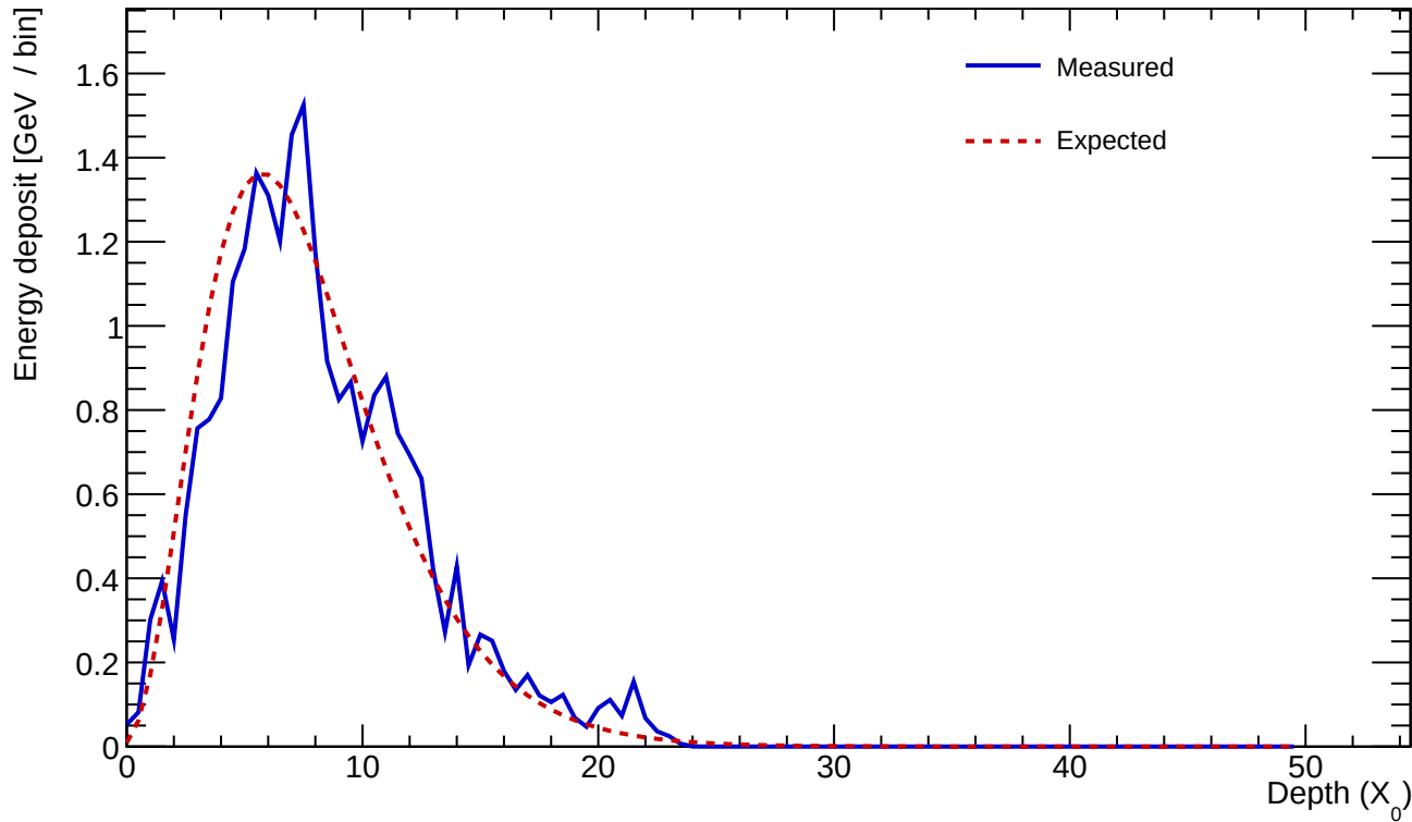
Cluster 225 E=24.787 GeV profileStart=0.50 X_0 \chi=0.1607
