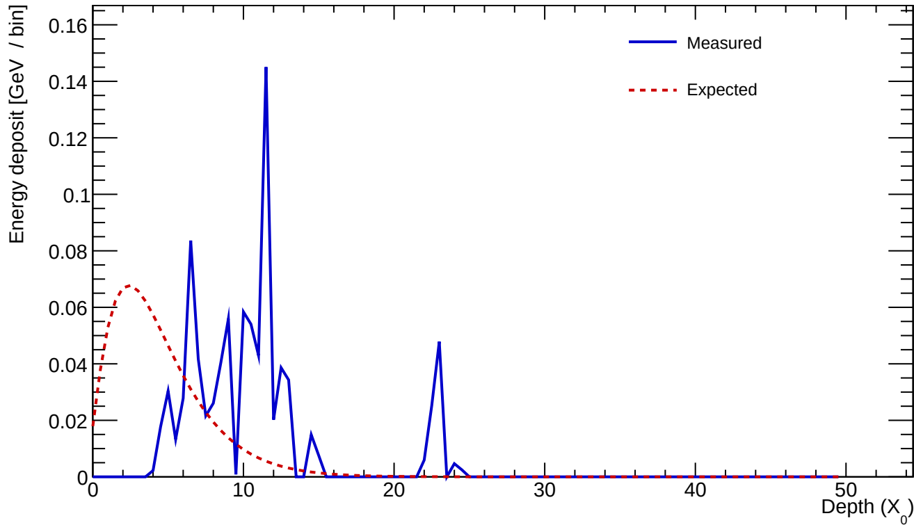
Cluster 702 E=0.864 GeV profileStart=5.50 X_0 \chi=0.7235
