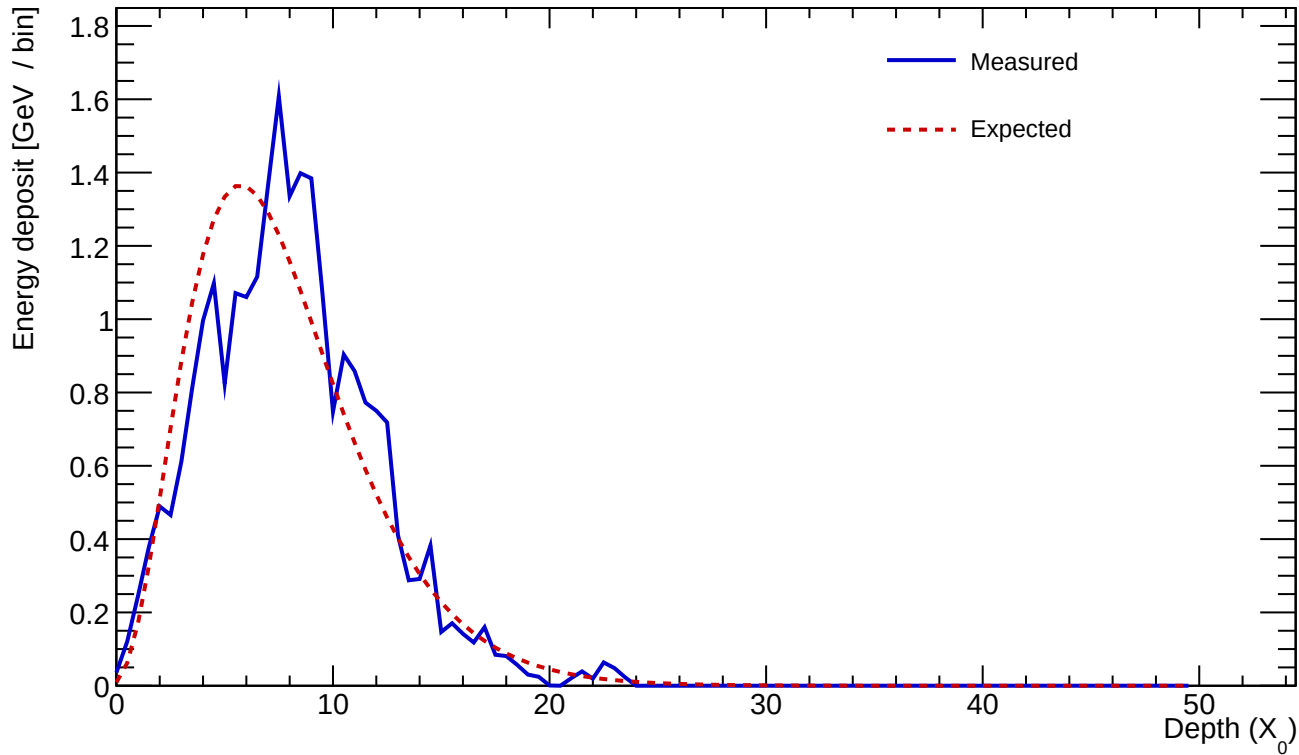
Cluster 63 E=24.846 GeV profileStart=0.50 X_0 \chi=0.2083
