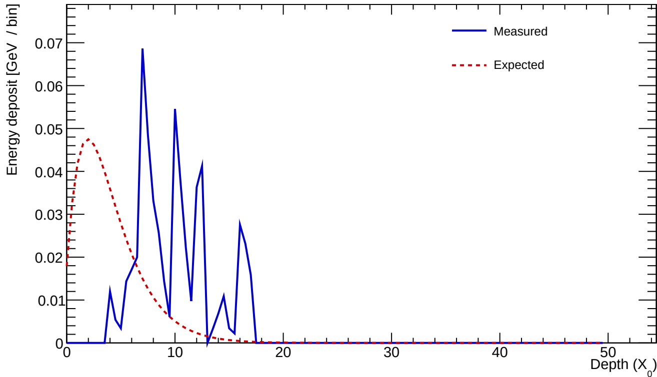
Cluster 1094 E=0.564 GeV profileStart=5.50 X_0 \chi=0.5959
