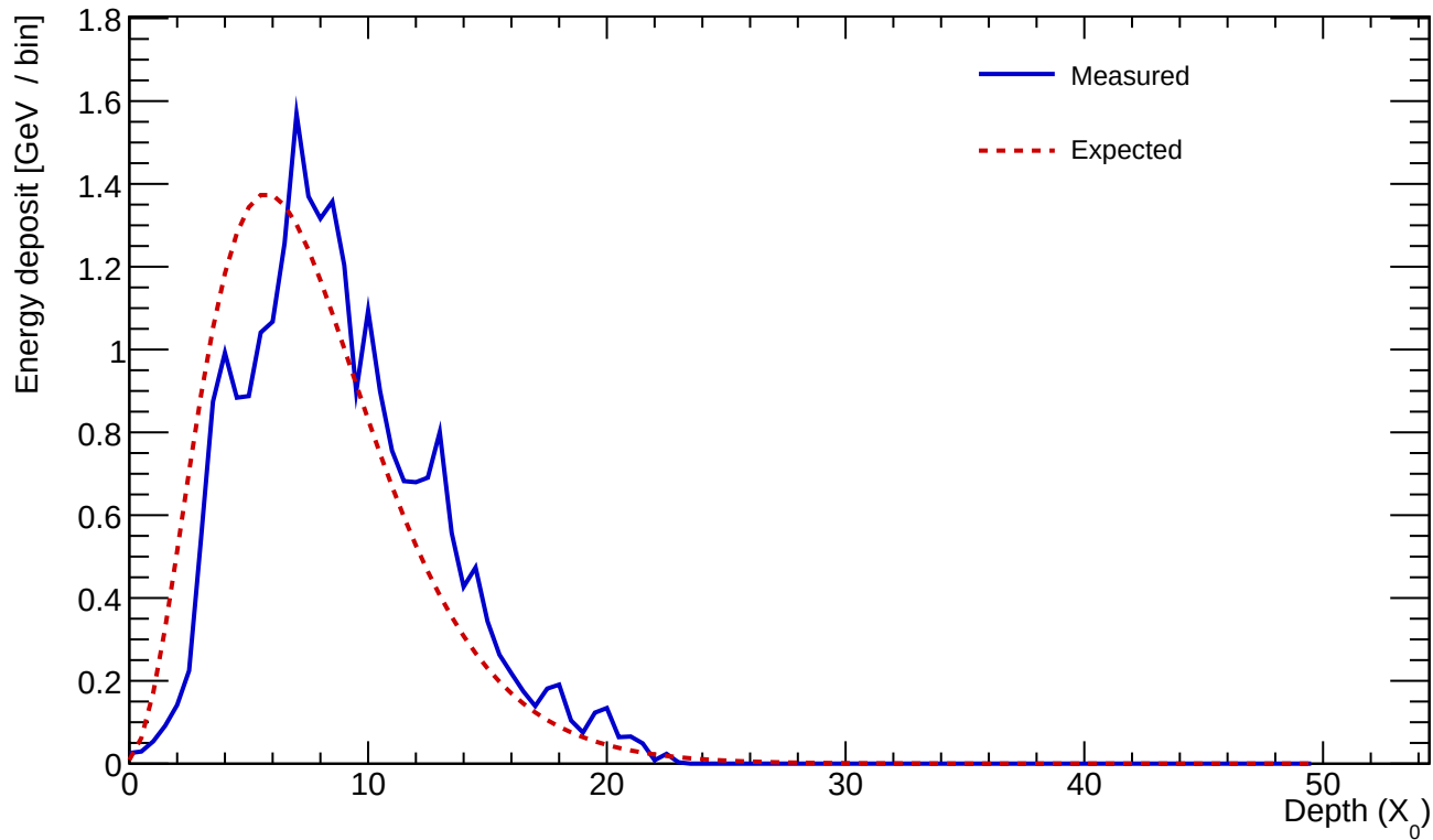
Cluster 395 E=25.049 GeV profileStart=1.00 X_0 \chi=0.1399
