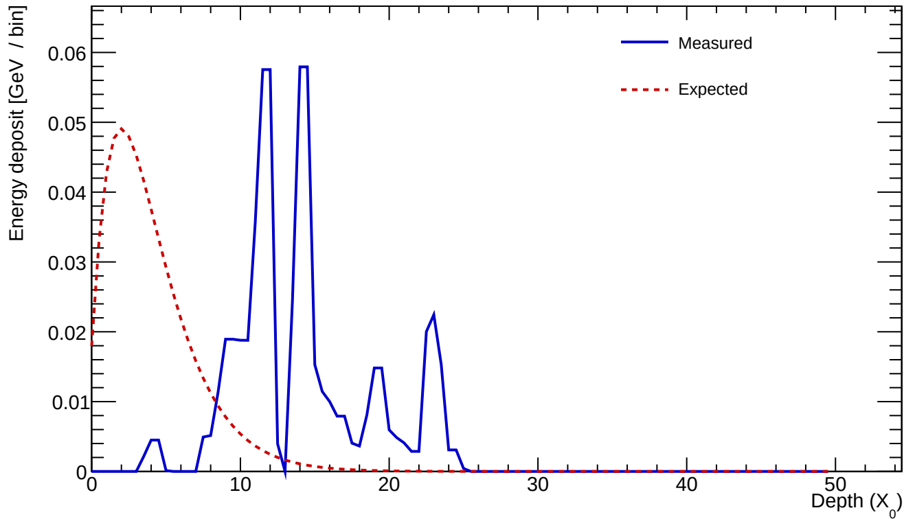
Cluster 1166 E=0.586 GeV profileStart=9.50 X_0 \chi=0.6941
