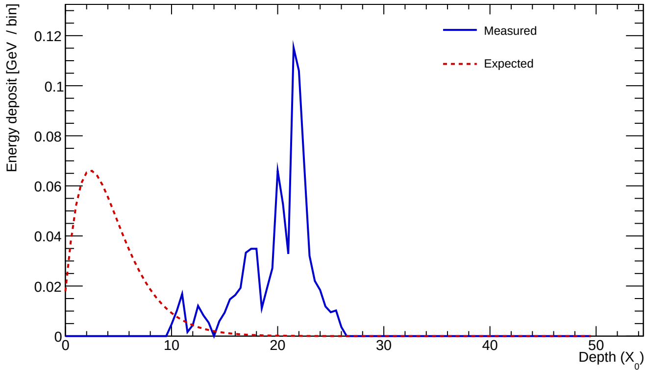
Cluster 1150 E=0.838 GeV profileStart=16.50 X_0 \chi=0.6185
