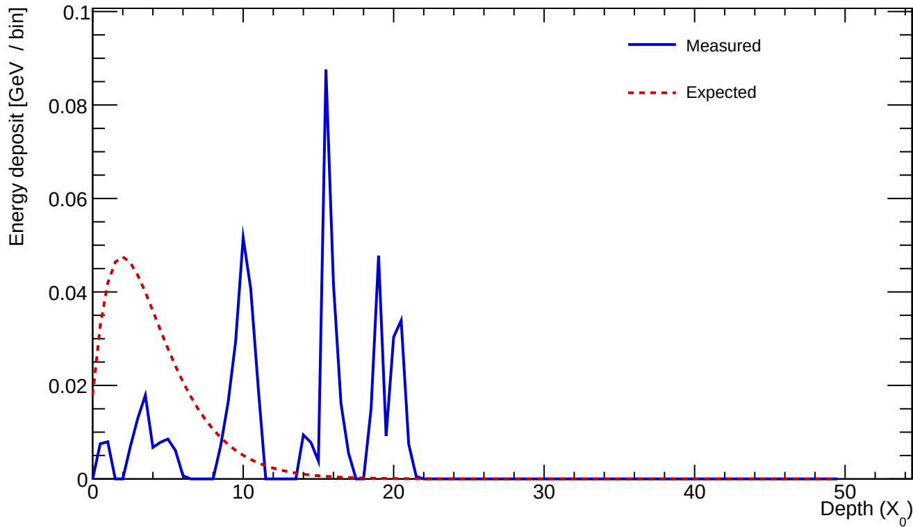
Cluster 683 E=0.564 GeV profileStart=9.00 X_0 \chi=1.1147
