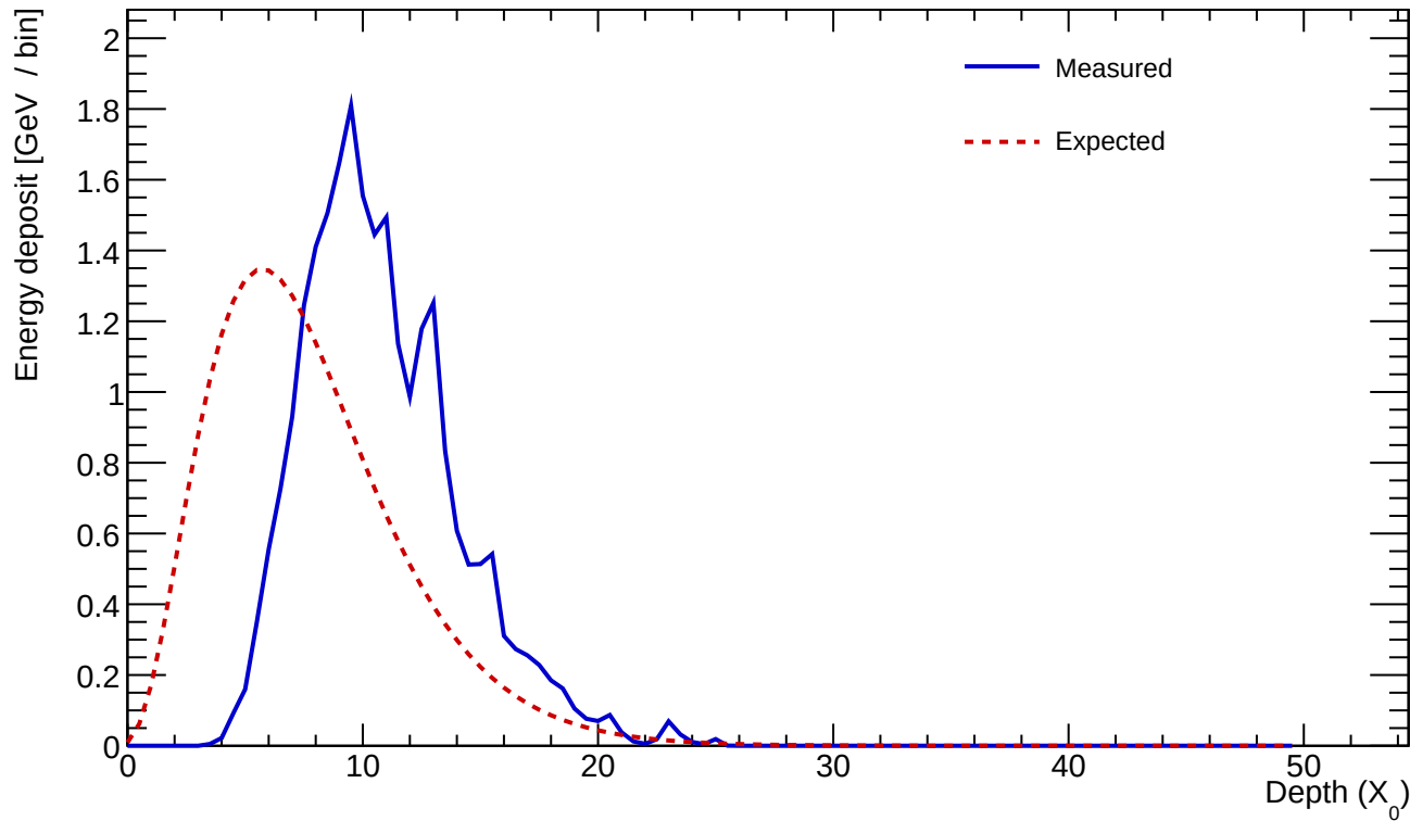
Cluster 410 E=24.480 GeV profileStart=3.50 X_0 \chi=0.2007
