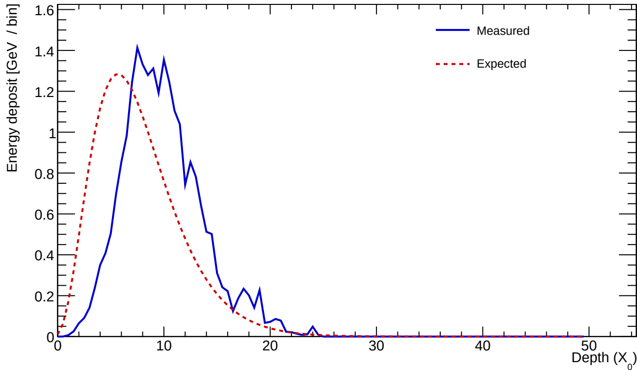
Cluster 995 E=23.243 GeV profileStart=3.00 X_0 \chi=0.1393
