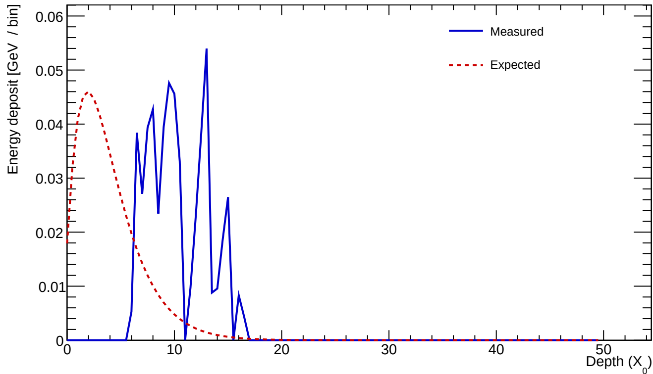
Cluster 52 E=0.543 GeV profileStart=6.50 X_0 \chi=0.4126
