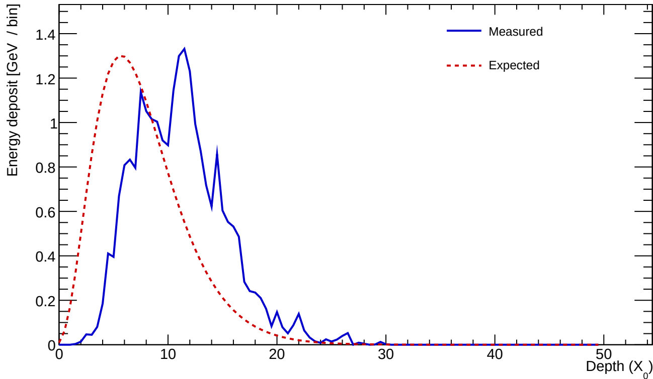
Cluster 613 E=23.576 GeV profileStart=3.50 X_0 \chi=0.1957
