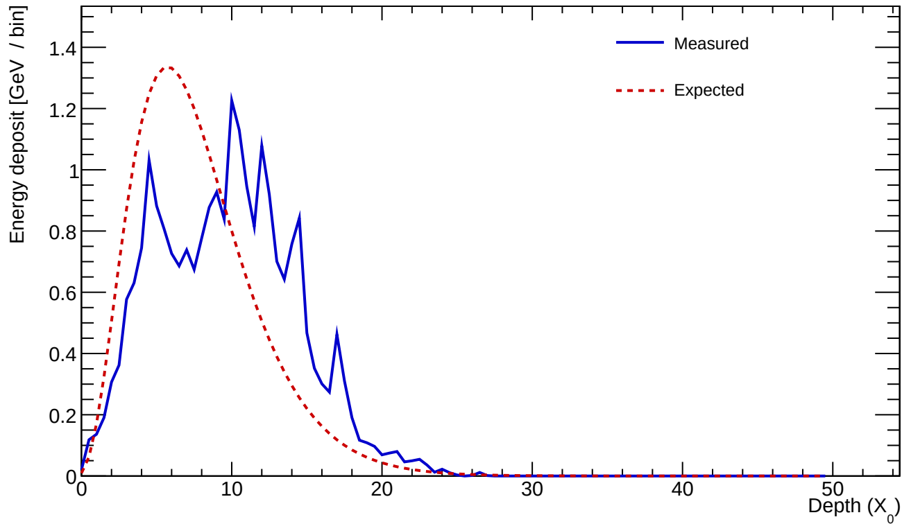
Cluster 18 E=24.263 GeV profileStart=2.00 X_0 \chi=0.3575
