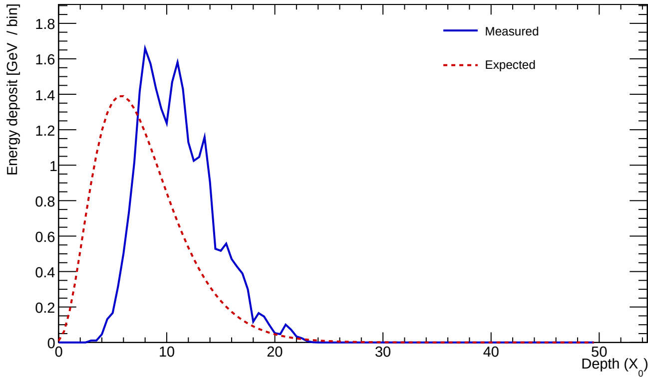
Cluster 205 E=25.365 GeV profileStart=3.50 X_0 \chi=0.1667
