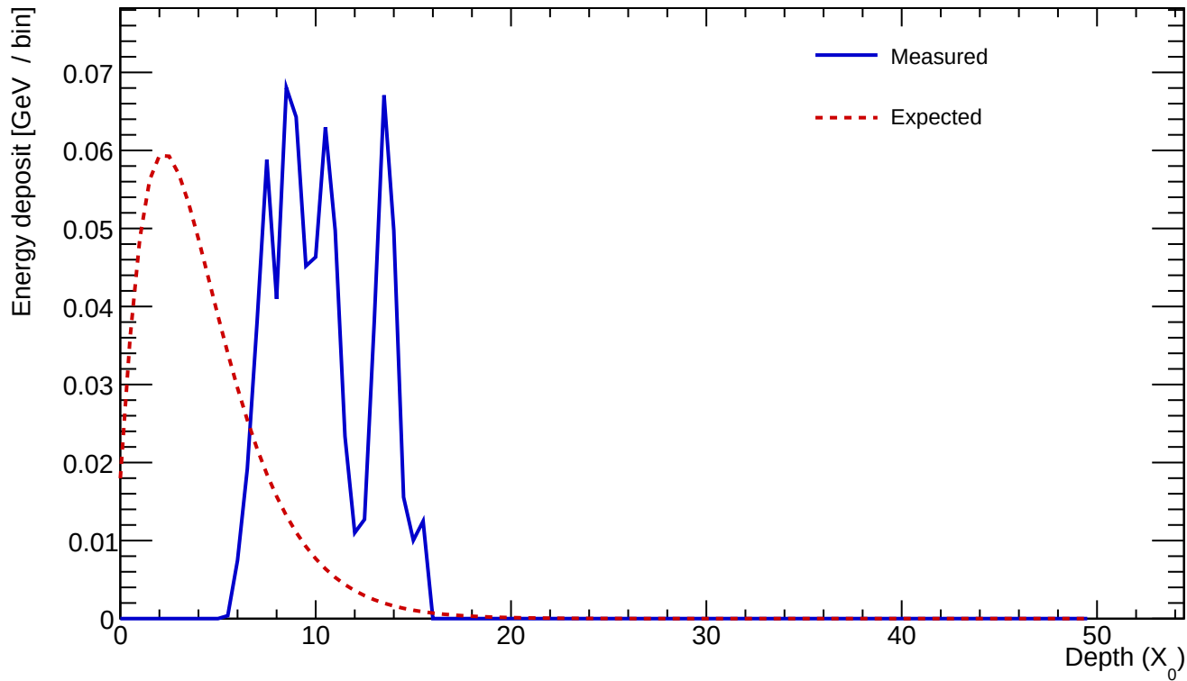
Cluster 331 E=0.741 GeV profileStart=6.50 X_0 \chi=0.3192
