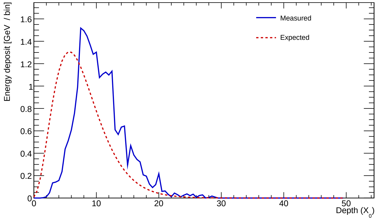
Cluster 794 E=23.671 GeV profileStart=3.00 X_0 \chi=0.1666
