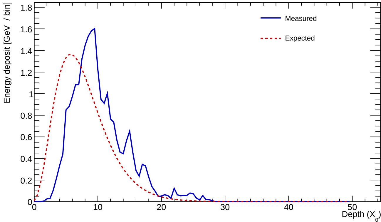
Cluster 51 E=24.823 GeV profileStart=2.50 X_0 \chi=0.1596
