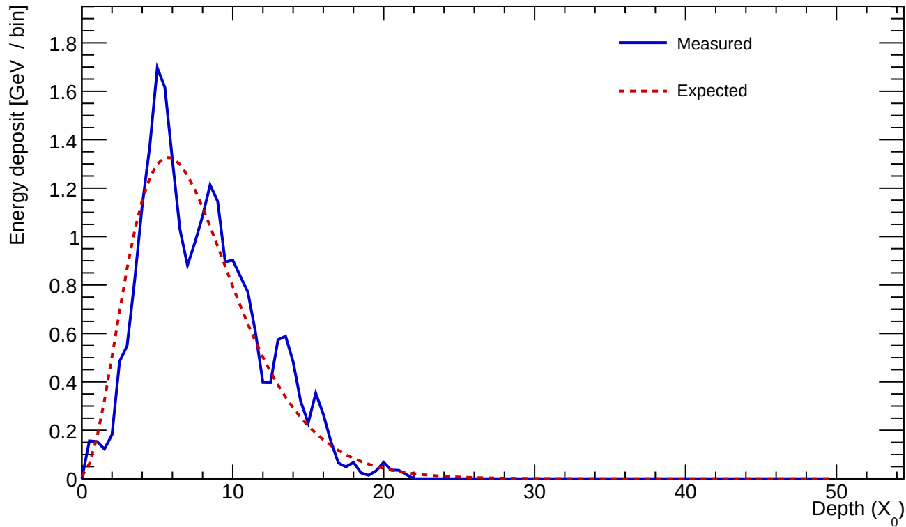
Cluster 664 E=24.109 GeV profileStart=0.50 X_0 \chi=0.1919
