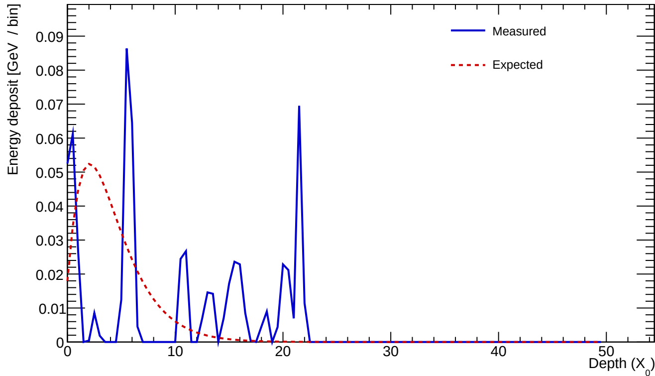
Cluster 4 E=0.635 GeV profileStart=4.50 X_0 \chi=1.3136
