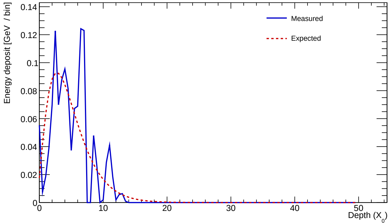
Cluster 501 E=1.247 GeV profileStart=1.00 X_0 \chi=0.4401
