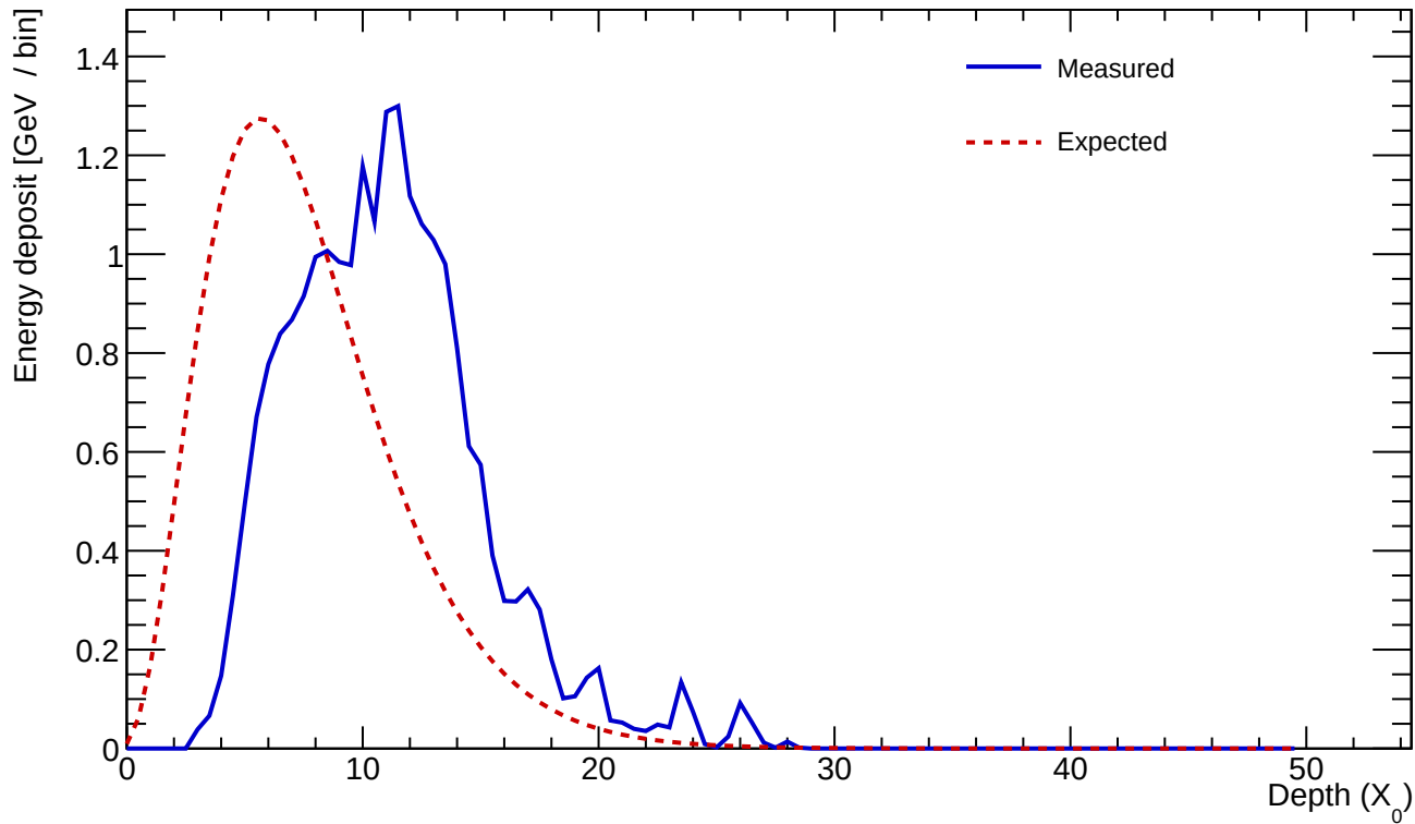
Cluster 883 E=23.079 GeV profileStart=3.50 X_0 \chi=0.2005
