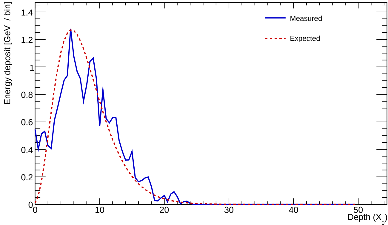
Cluster 548 E=22.944 GeV profileStart=0.50 X_0 \chi=0.2569
