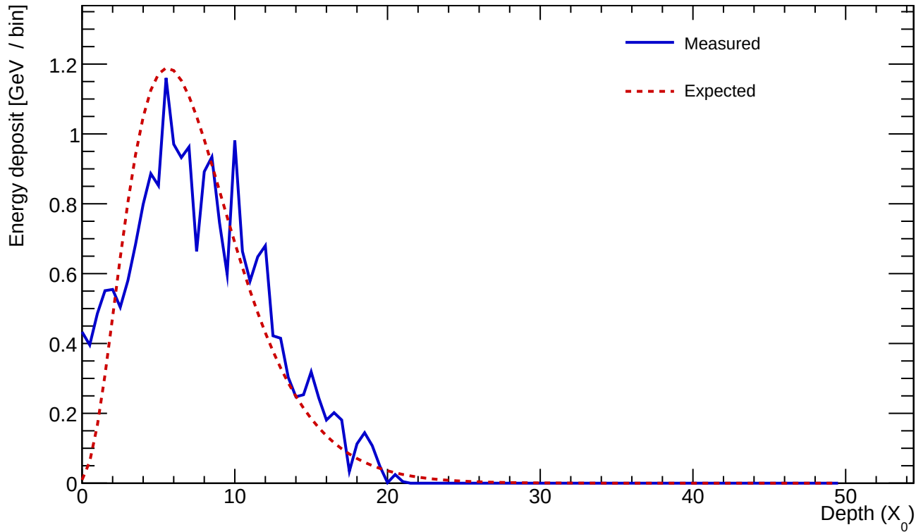
Cluster 203 E=21.382 GeV profileStart=0.50 X_0 \chi=0.2649
