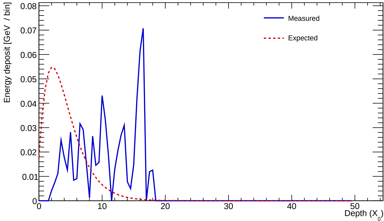
Cluster 633 E=0.670 GeV profileStart=6.00 X_0 \chi=0.9013
