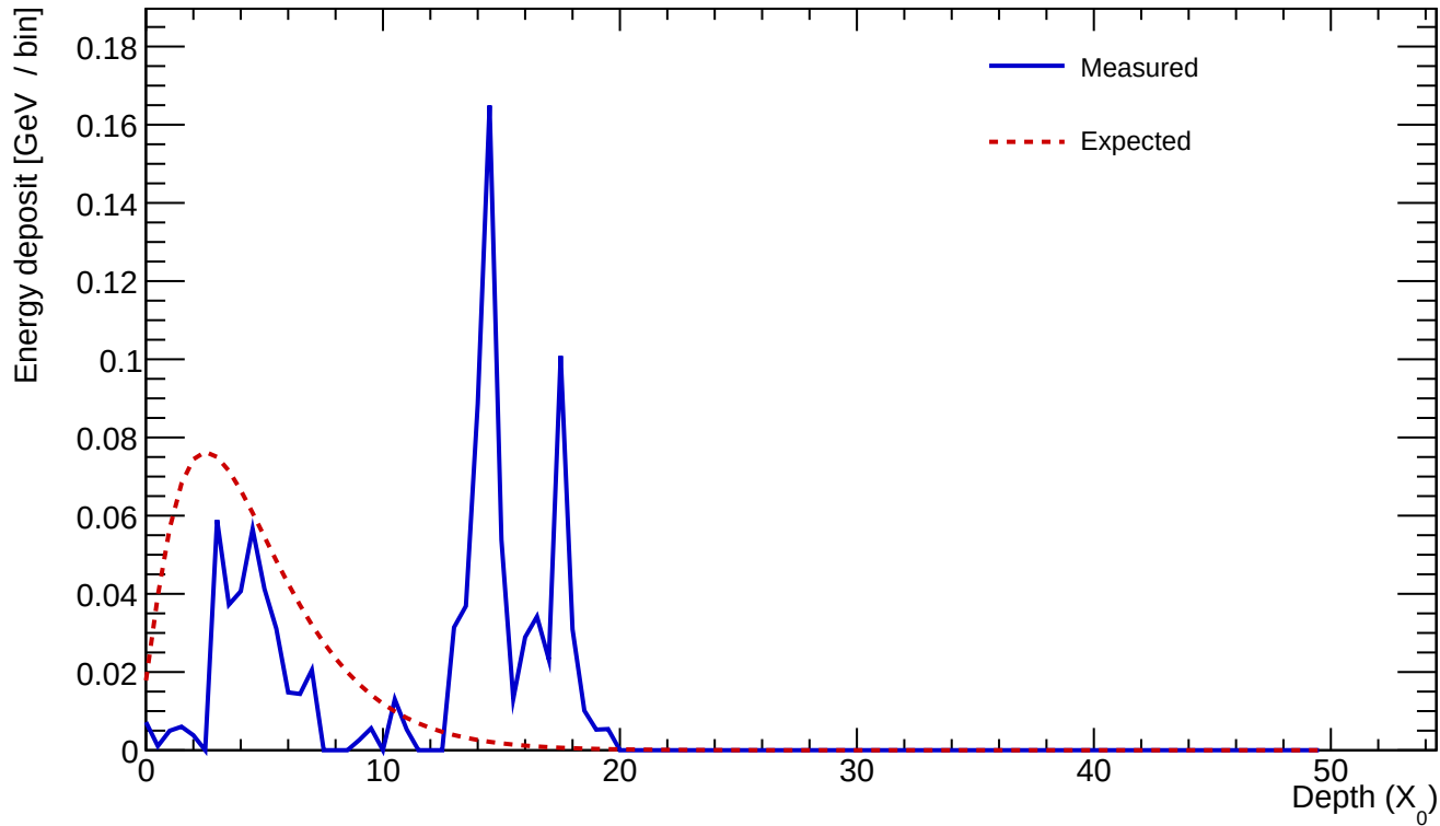
Cluster 513 E=0.993 GeV profileStart=1.50 X_0 \chi=1.2103
