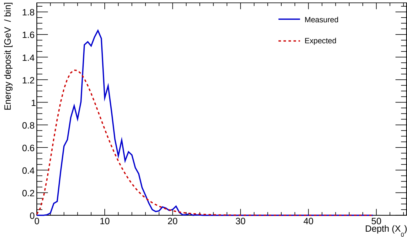
Cluster 819 E=23.279 GeV profileStart=2.00 X_0 \chi=0.1981
