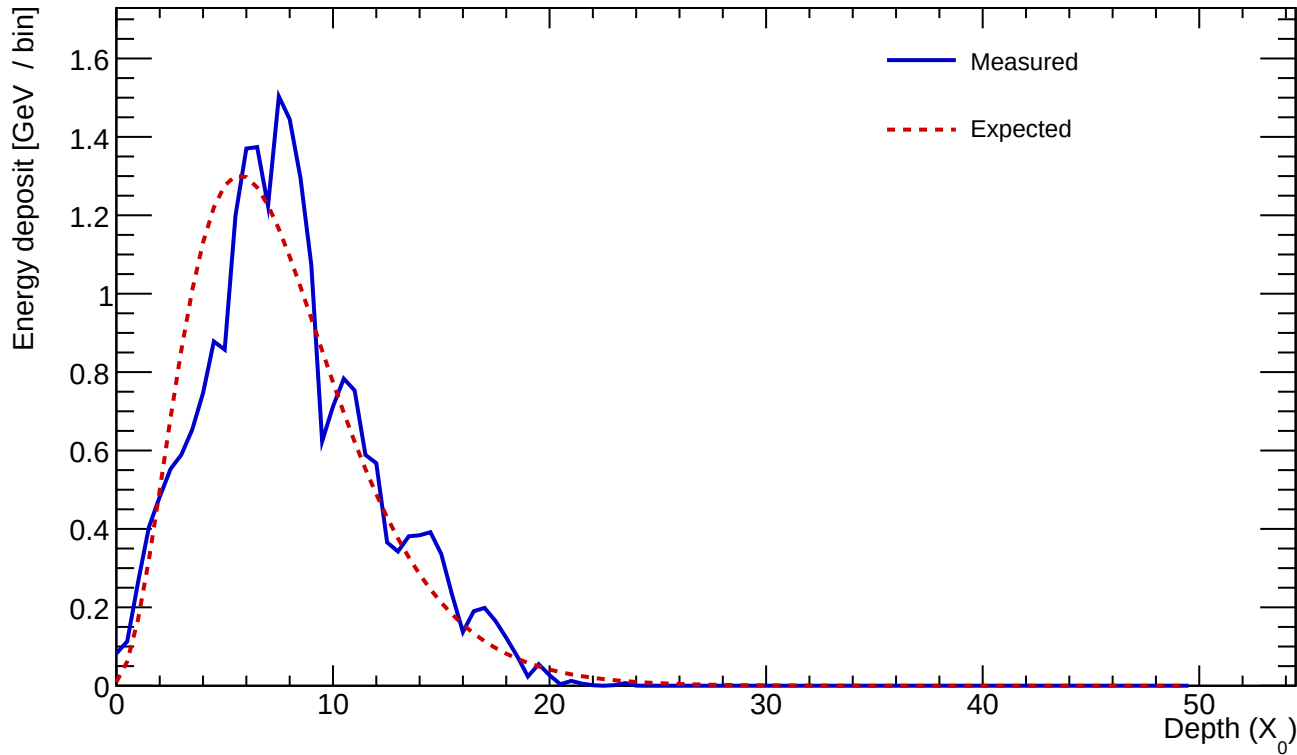
Cluster 191 E=23.595 GeV profileStart=0.50 X_0 \chi=0.1951
