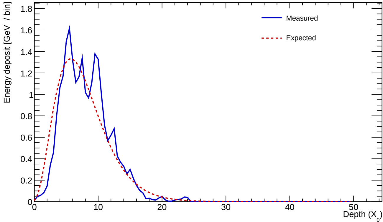
Cluster 84 E=24.182 GeV profileStart=0.50 X_0 \chi=0.1794
