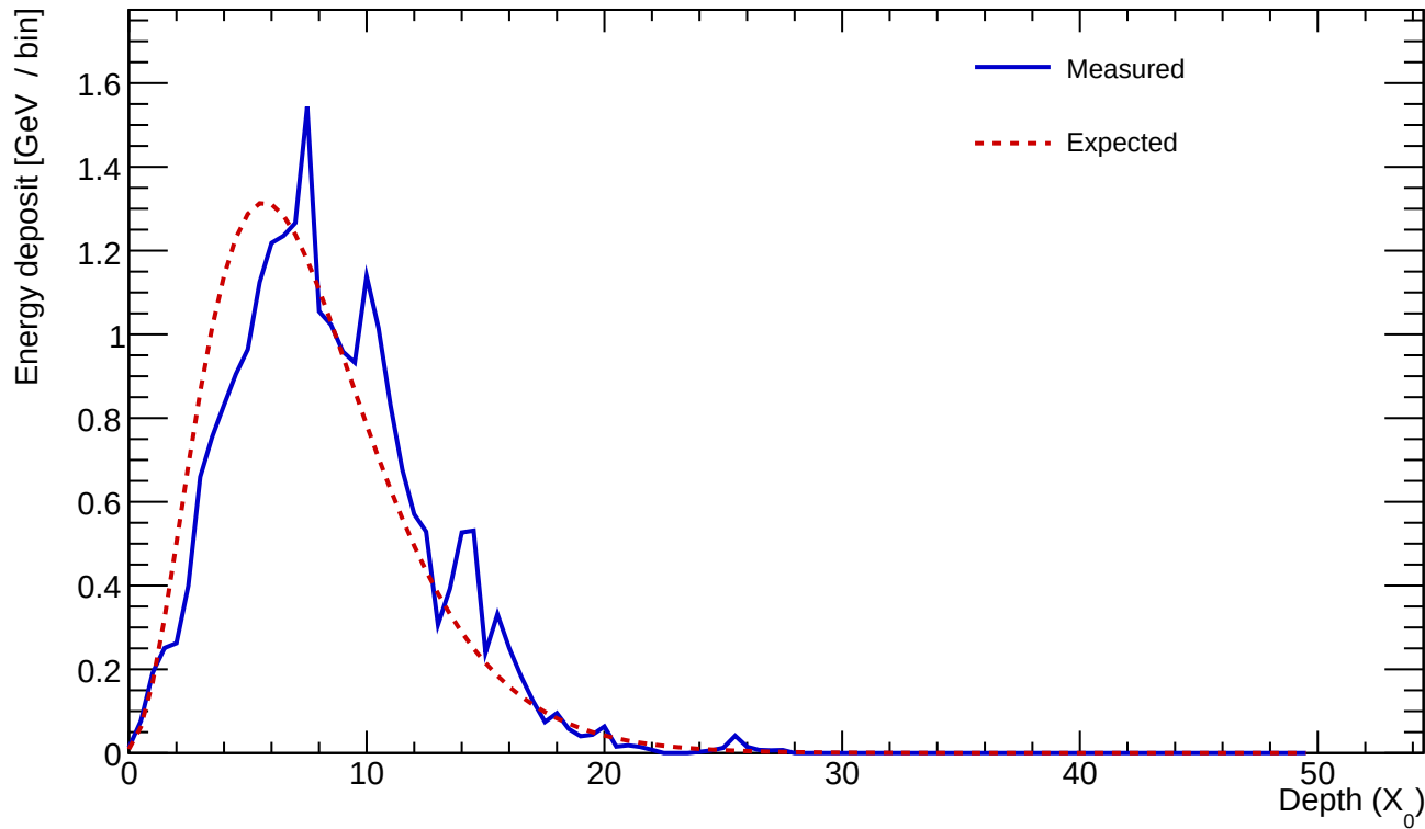
Cluster 54 E=23.842 GeV profileStart=1.00 X_0 \chi=0.1687
