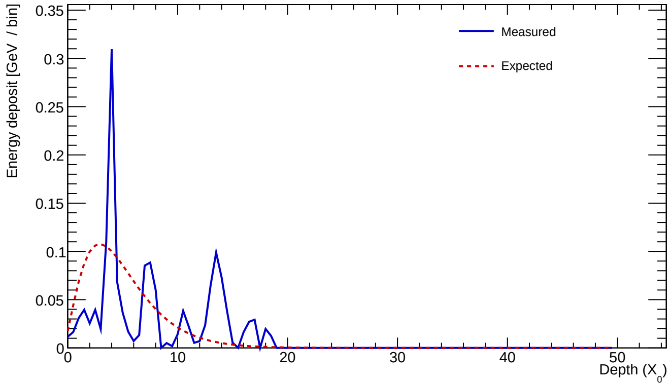
Cluster 775 E=1.480 GeV profileStart=1.00 X_0 \chi=0.8781
