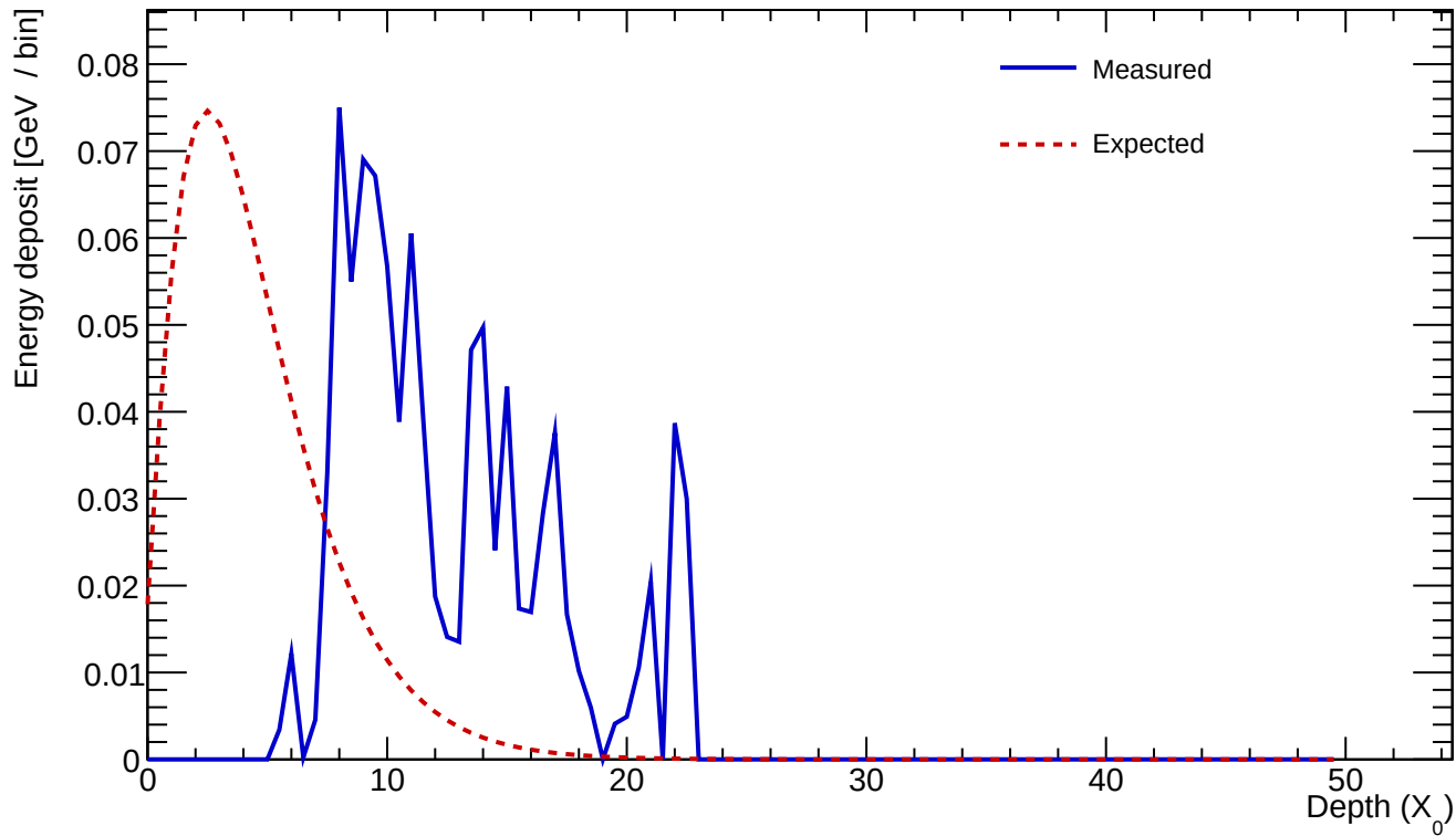
Cluster 337 E=0.967 GeV profileStart=7.00 X_0 \chi=0.4355
