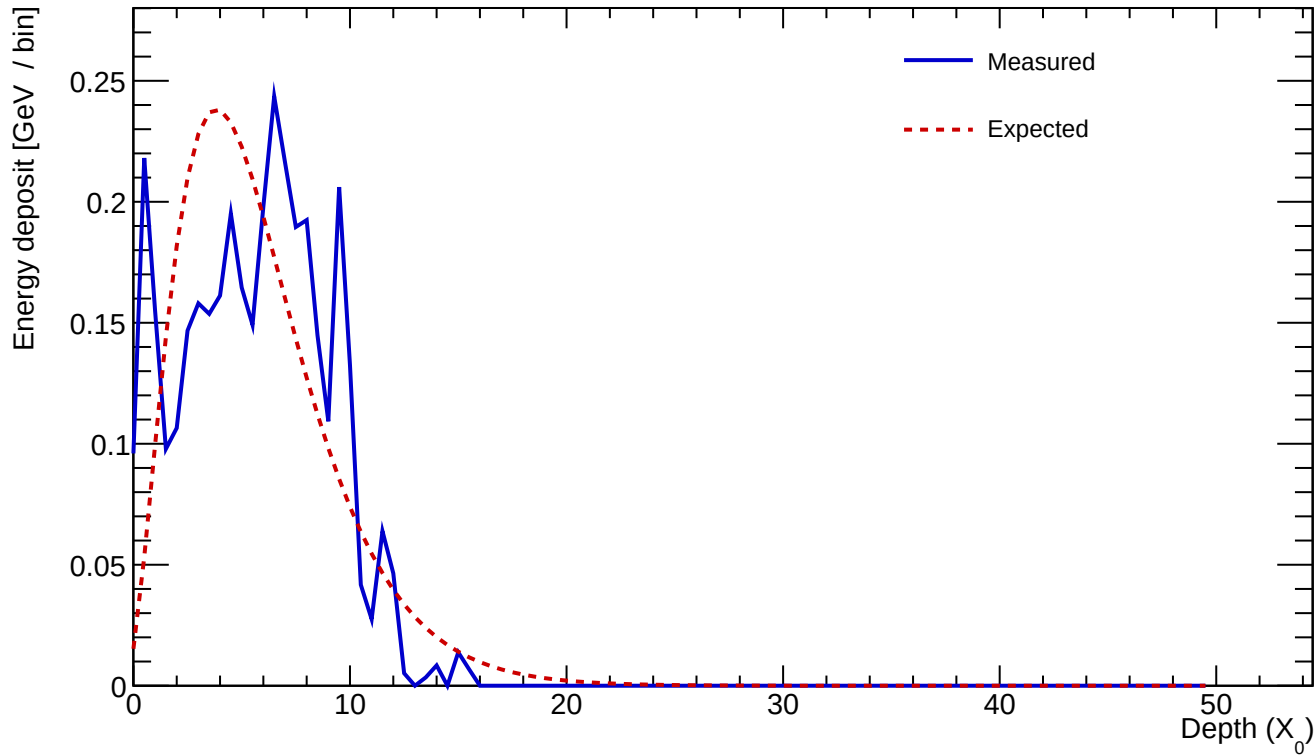
Cluster 946 E=3.652 GeV profileStart=1.00 X_0 \chi=0.3800
