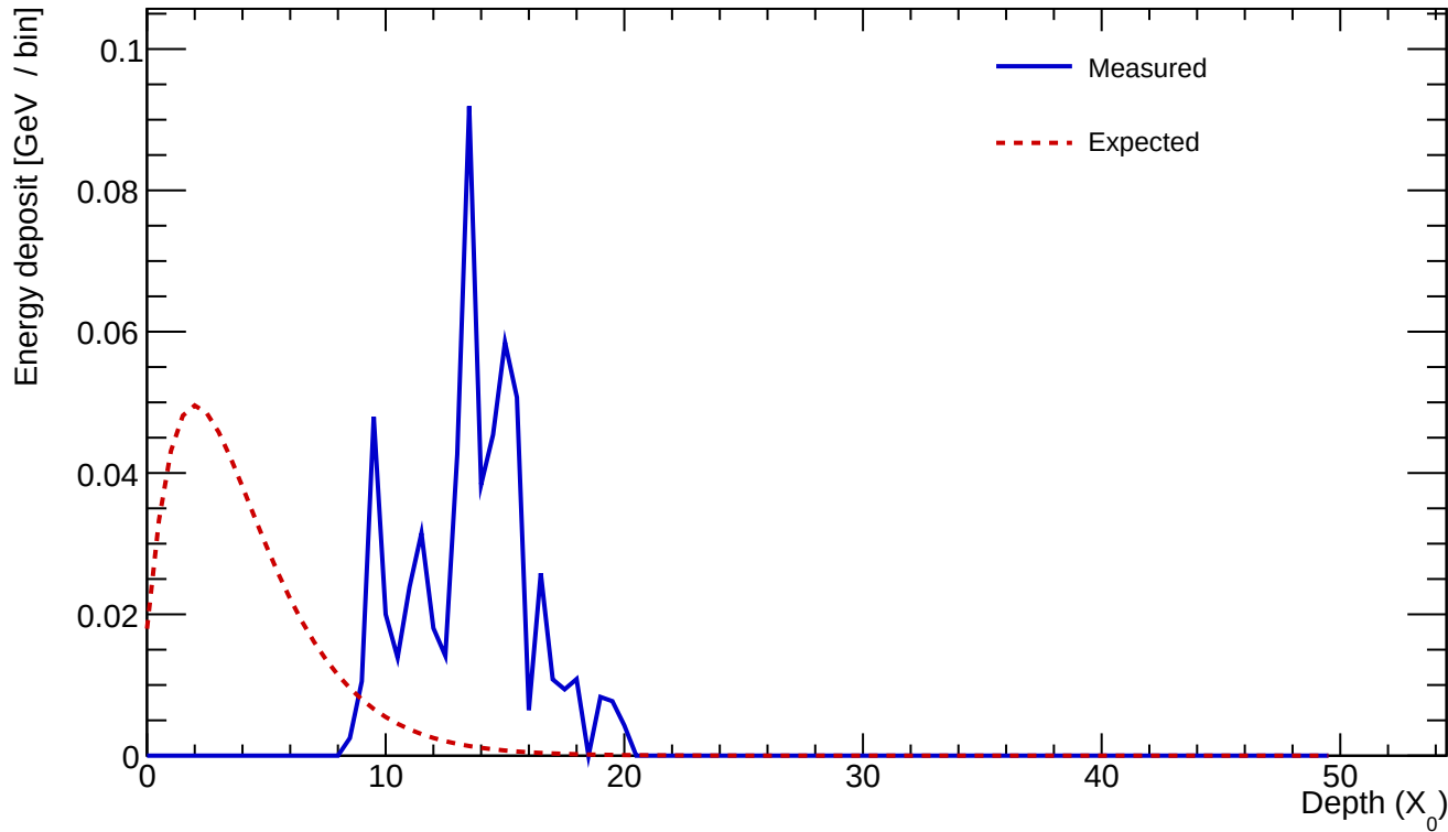
Cluster 484 E=0.594 GeV profileStart=11.00 X_0 \chi=0.5526
