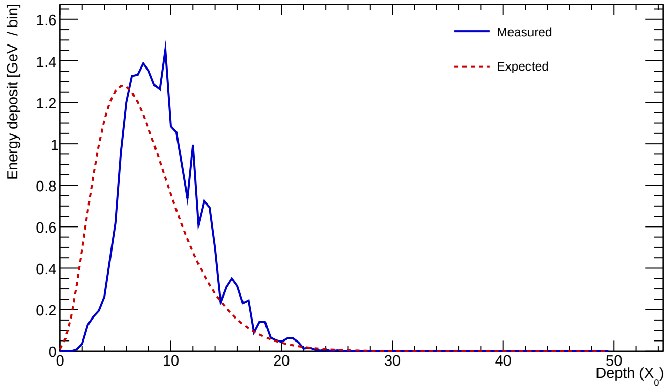
Cluster 46 E=23.139 GeV profileStart=2.00 X_0 \chi=0.1449
