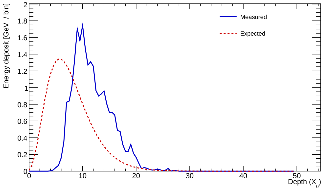
Cluster 285 E=24.390 GeV profileStart=4.50 X_0 \chi=0.1567
