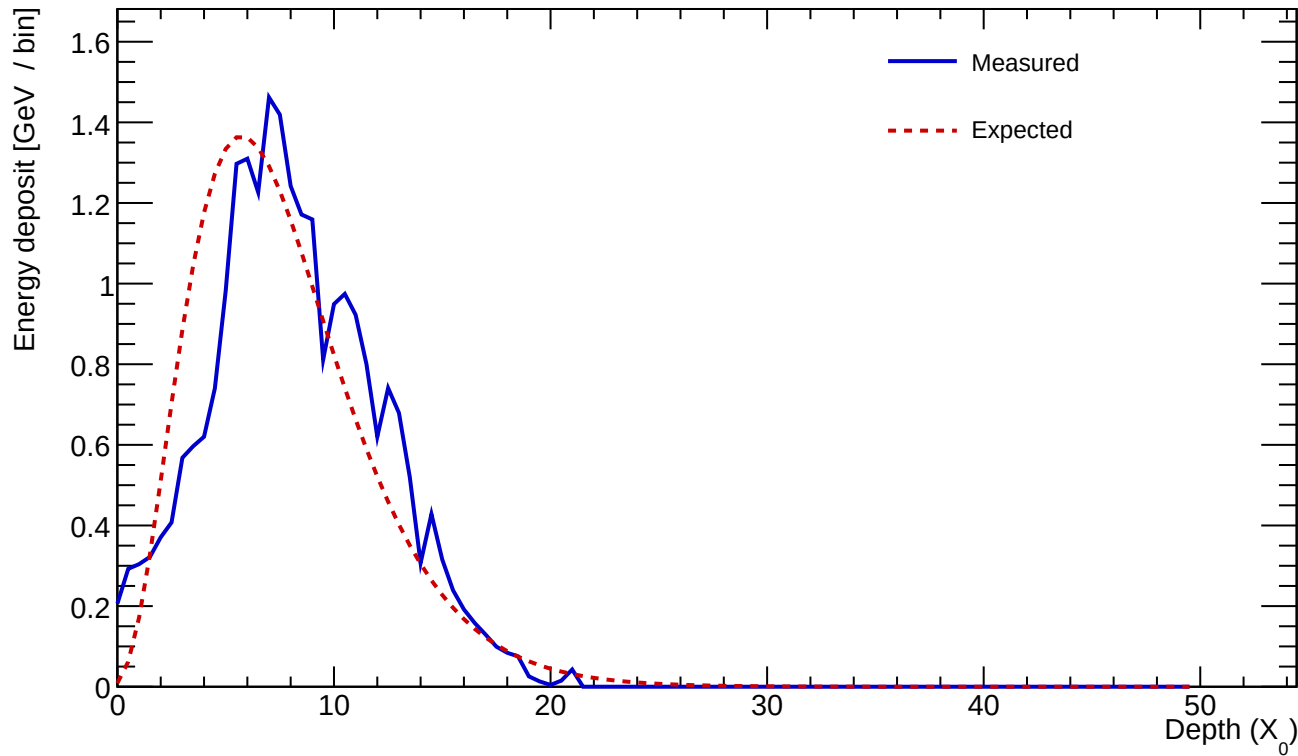
Cluster 406 E=24.844 GeV profileStart=1.00 X_0 \chi=0.1746
