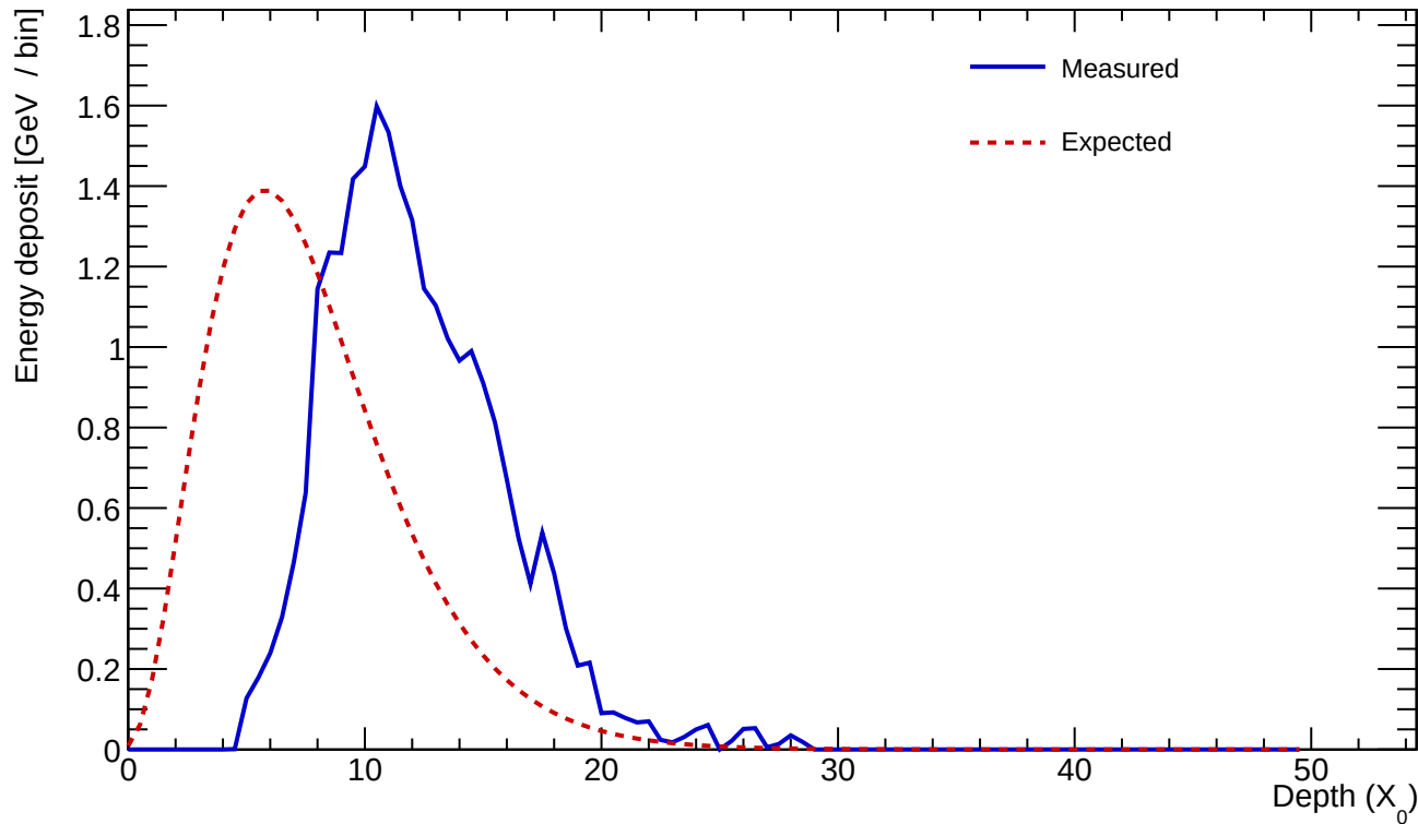
Cluster 157 E=25.344 GeV profileStart=4.50 X_0 \chi=0.1308
