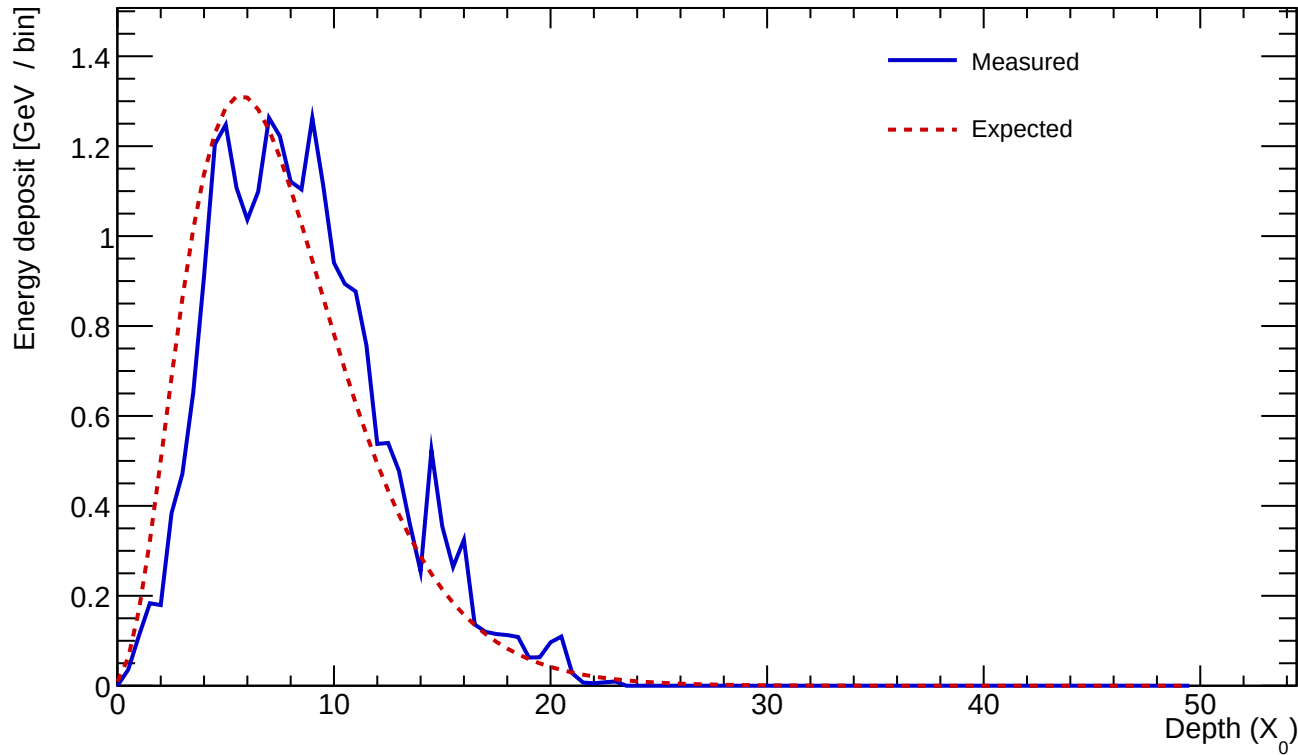
Cluster 439 E=23.796 GeV profileStart=1.00 X_0 \chi=0.1295
