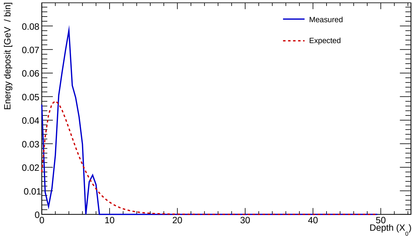
Cluster 563 E=0.573 GeV profileStart=1.50 X_0 \chi=0.3830
