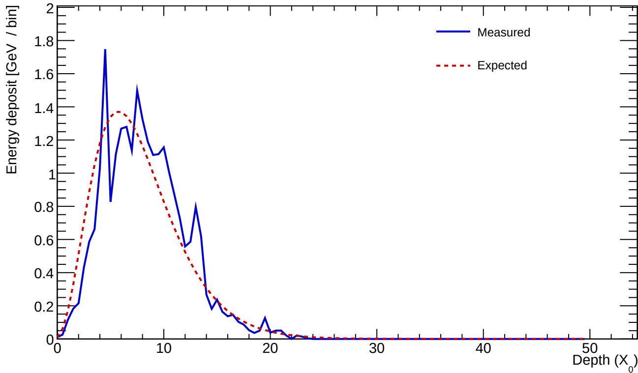
Cluster 49 E=24.977 GeV profileStart=1.00 X_0 \chi=0.1808
