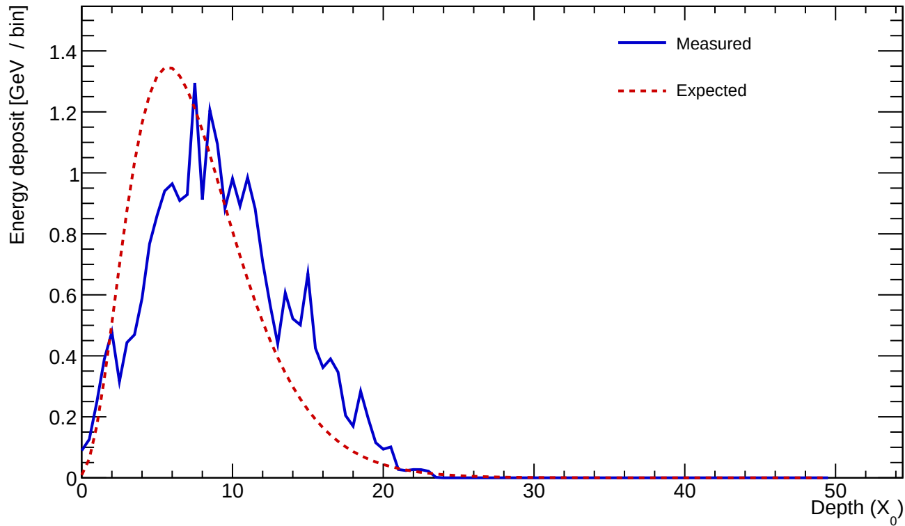
Cluster 95 E=24.478 GeV profileStart=2.00 X_0 \chi=0.2554
