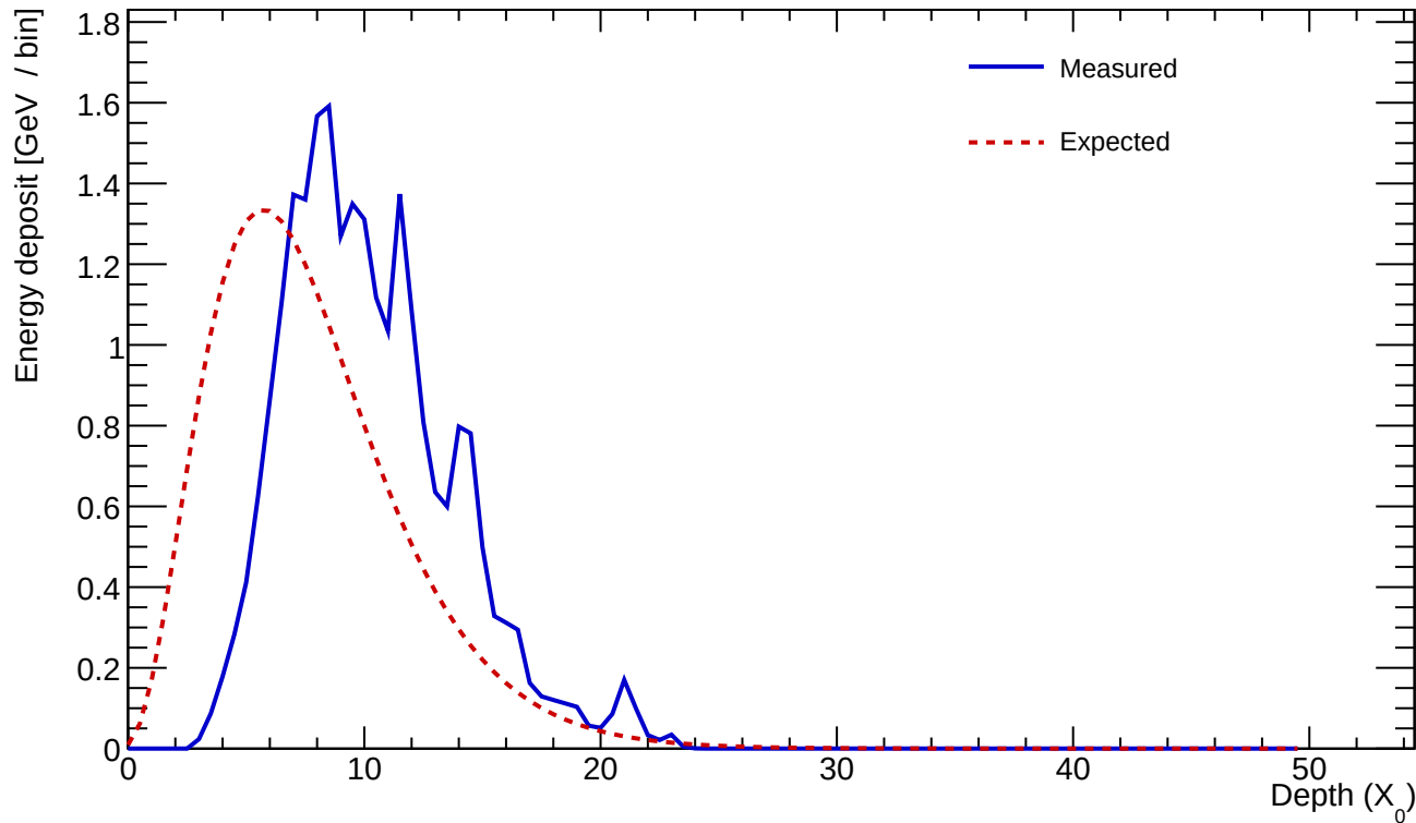
Cluster 949 E=24.254 GeV profileStart=3.00 X_0 \chi=0.1564
