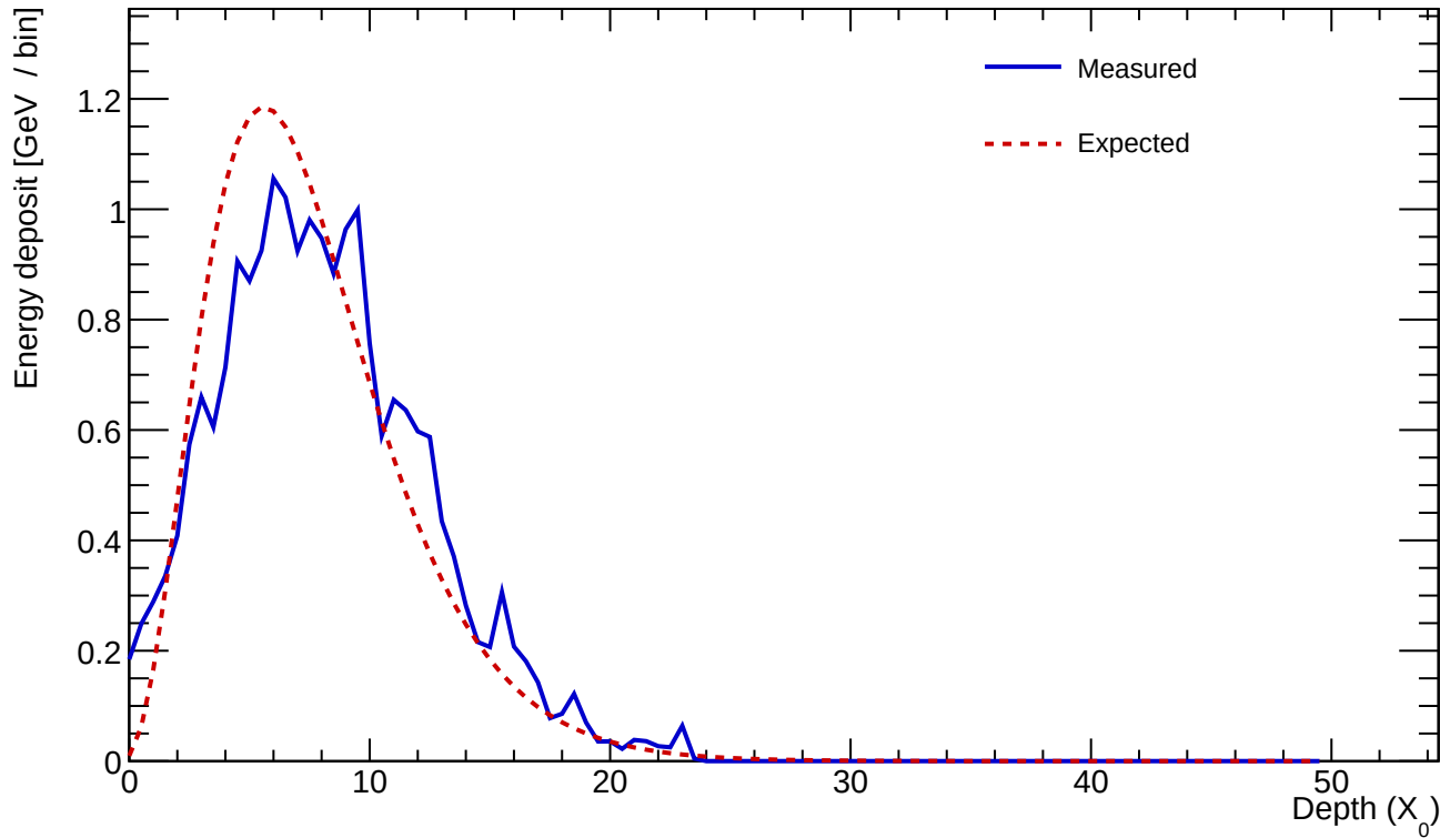
Cluster 867 E=21.310 GeV profileStart=0.50 X_0 \chi=0.1983
