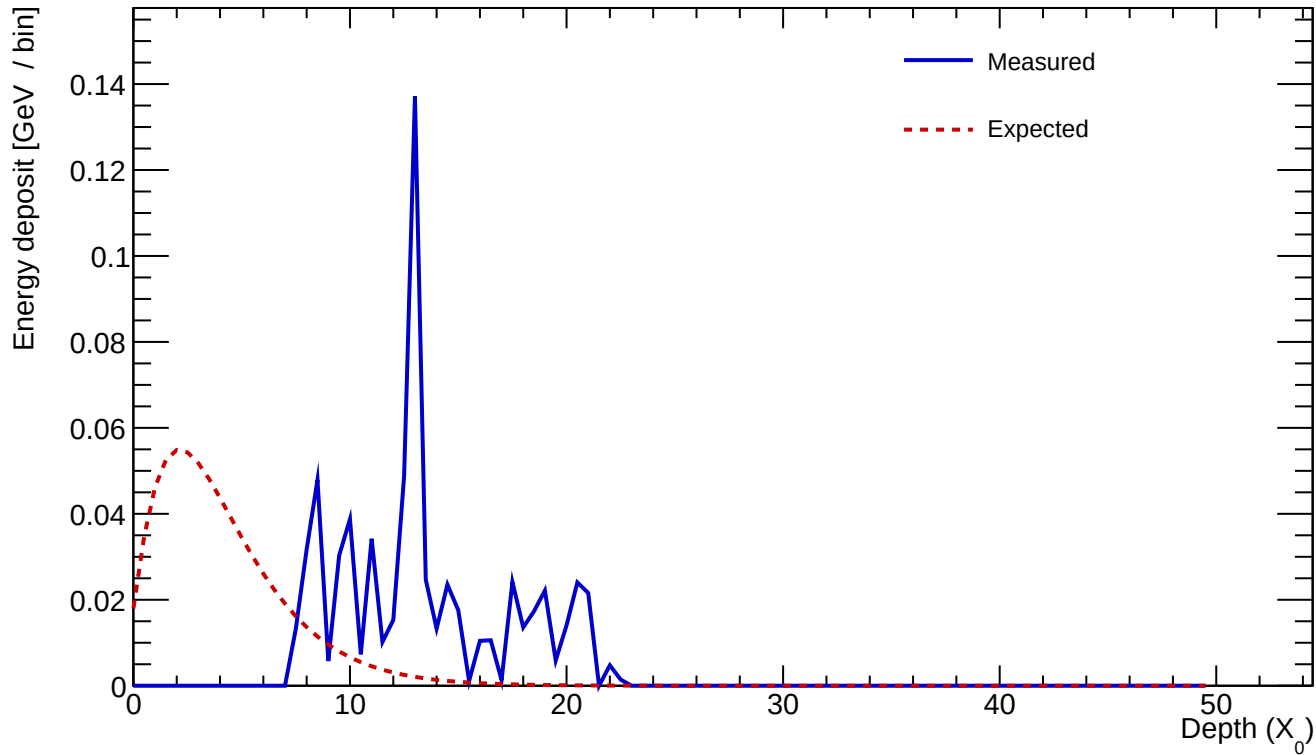
Cluster 964 E=0.672 GeV profileStart=7.50 X_0 \chi=0.7274
