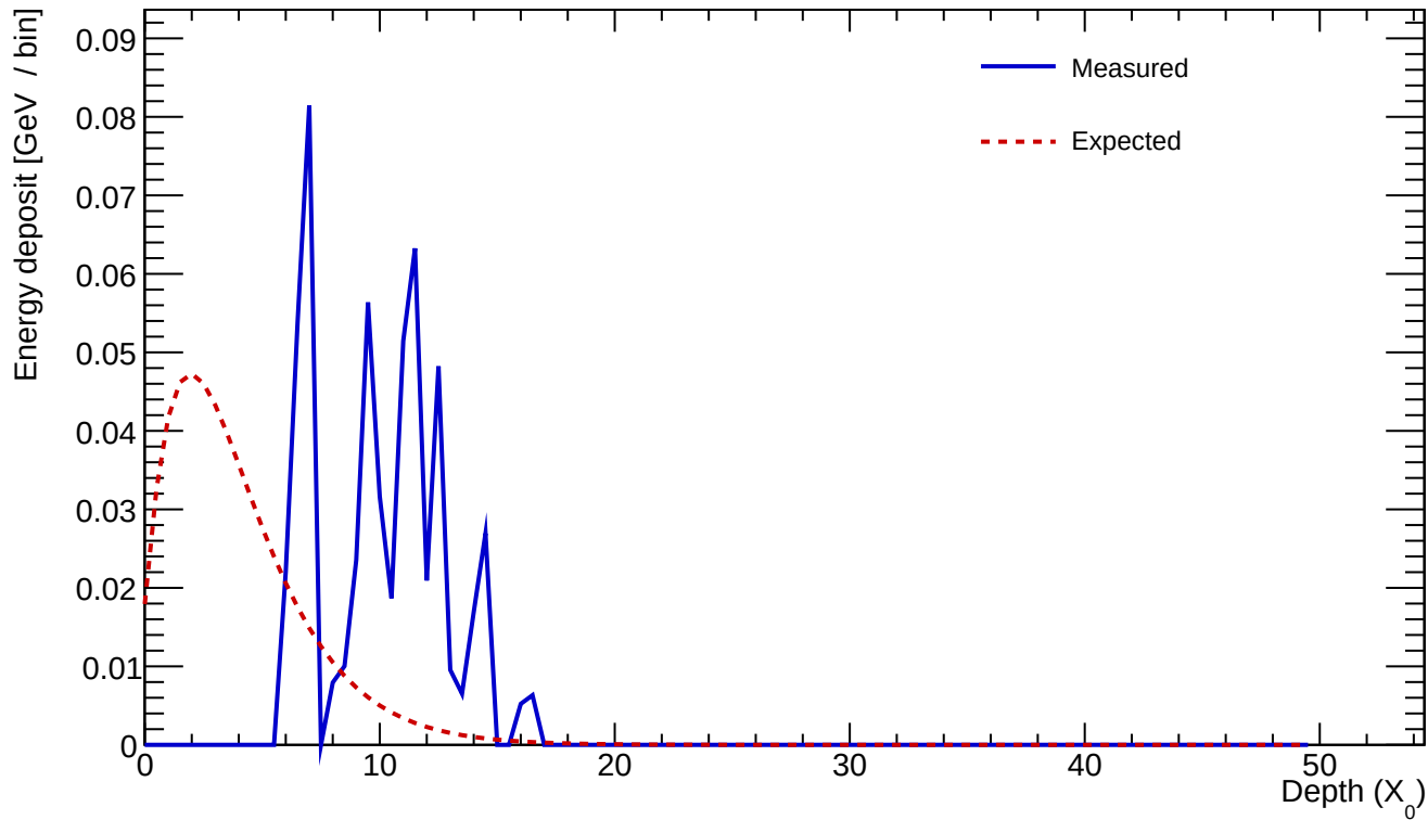
Cluster 258 E=0.561 GeV profileStart=6.00 X_0 \chi=0.6838
