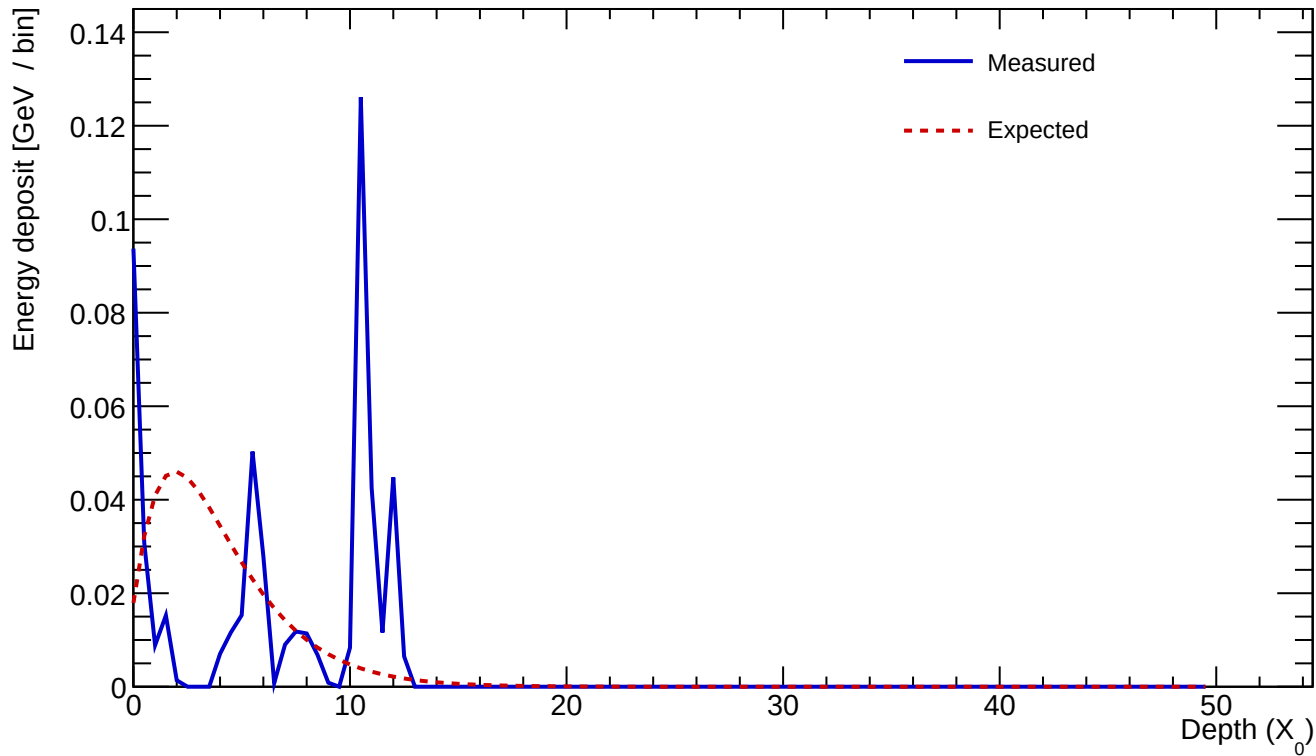
Cluster 665 E=0.543 GeV profileStart=10.00 X_0 \chi=0.8157
