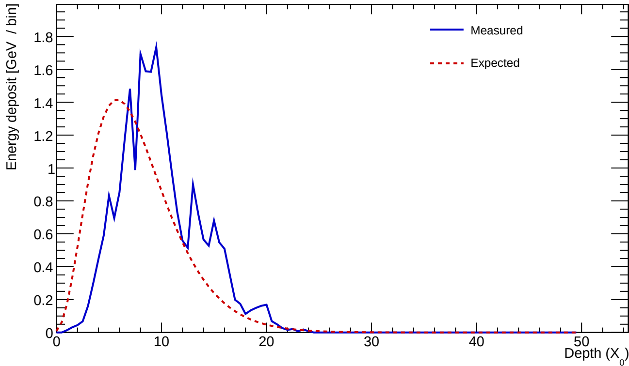
Cluster 787 E=25.830 GeV profileStart=2.50 X_0 \chi=0.2098
