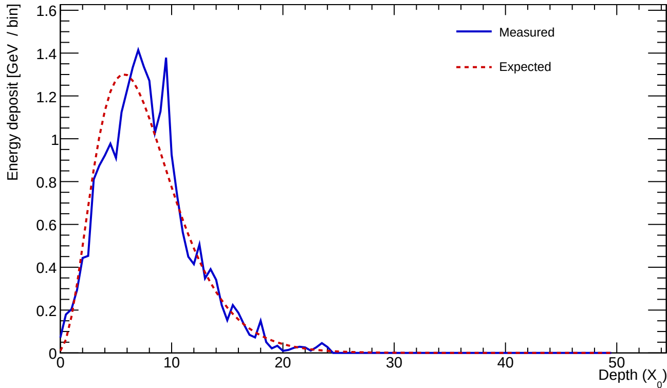
Cluster 679 E=23.597 GeV profileStart=0.50 X_0 \chi=0.1638
