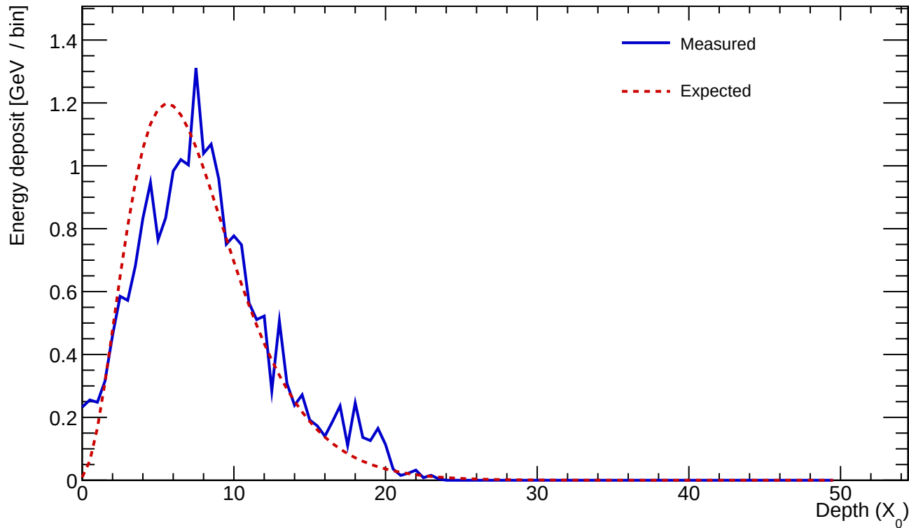
Cluster 229 E=21.553 GeV profileStart=0.50 X_0 \chi=0.2089
