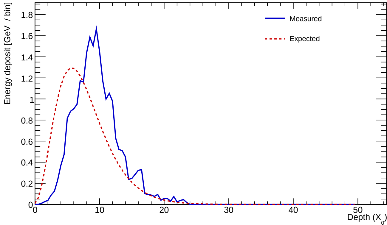
Cluster 986 E=23.451 GeV profileStart=2.50 X_0 \chi=0.1914
