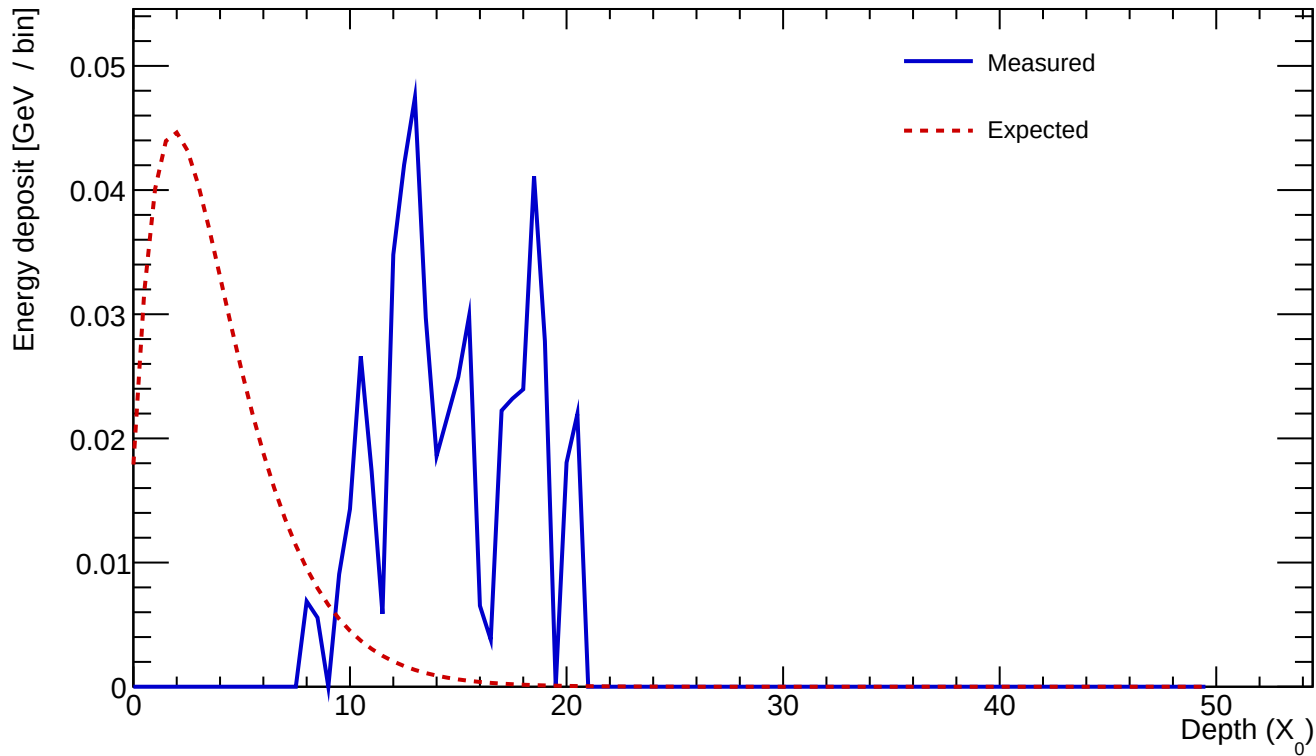
Cluster 325 E=0.523 GeV profileStart=10.00 X_0 \chi=0.5337
