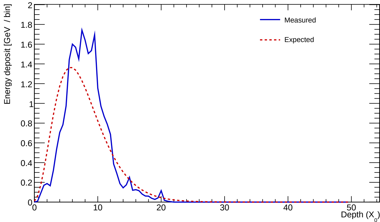
Cluster 224 E=24.839 GeV profileStart=1.50 X_0 \chi=0.2458
