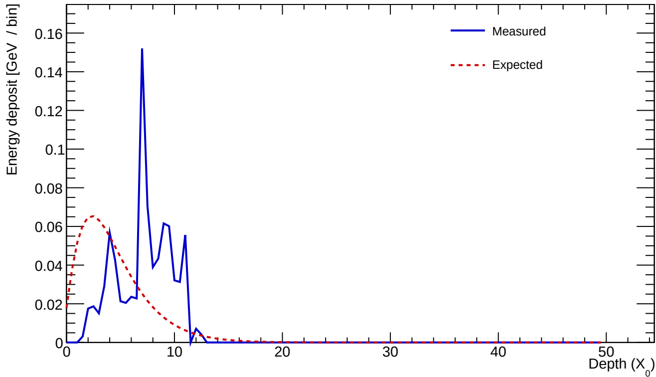
Cluster 422 E=0.828 GeV profileStart=3.50 X_0 \chi=0.6012
