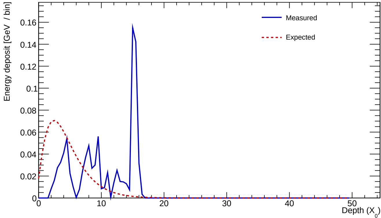
Cluster 434 E=0.906 GeV profileStart=2.50 X_0 \chi=0.8825
