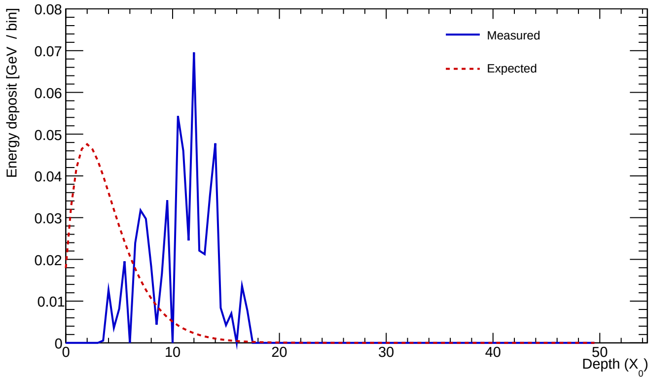
Cluster 316 E=0.565 GeV profileStart=9.00 X_0 \chi=0.6537
