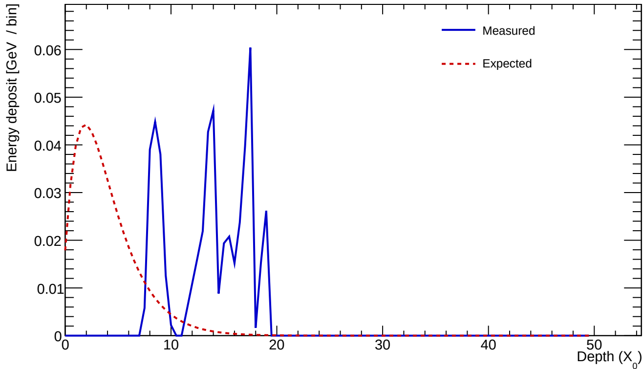
Cluster 712 E=0.518 GeV profileStart=12.50 X_0 \chi=0.6838
