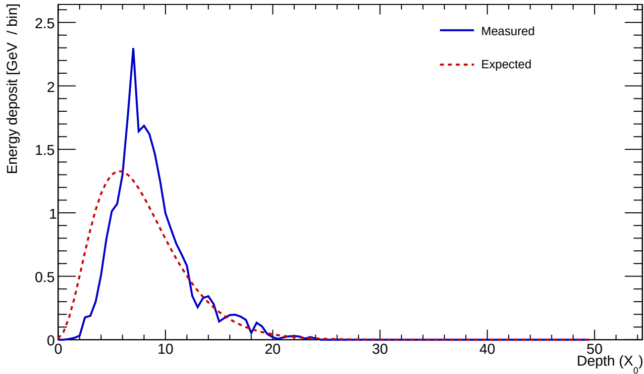
Cluster 36 E=24.136 GeV profileStart=1.50 X_0 \chi=0.2458
