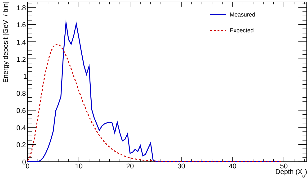
Cluster 451 E=24.980 GeV profileStart=3.00 X_0 \chi=0.2067
