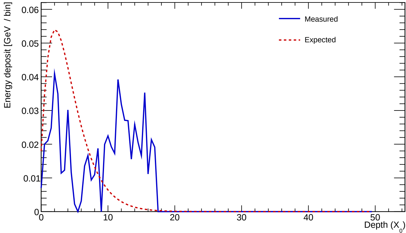
Cluster 808 E=0.659 GeV profileStart=0.50 X_0 \chi=0.9796
