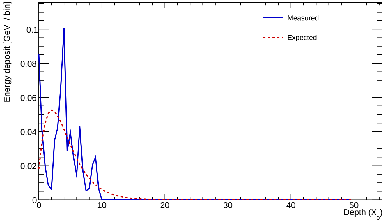
Cluster 1139 E=0.637 GeV profileStart=2.00 X_0 \chi=0.6041
