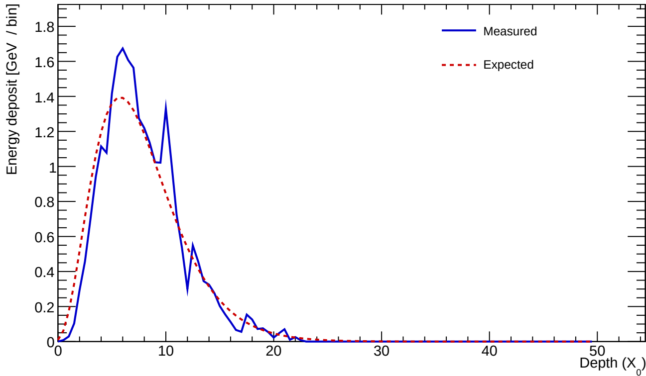
Cluster 688 E=25.411 GeV profileStart=0.50 X_0 \chi=0.1412
