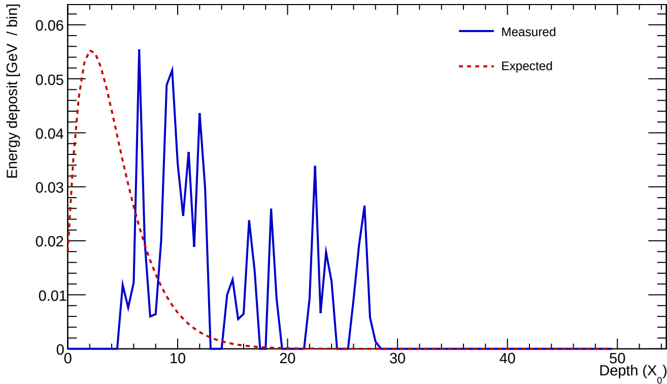
Cluster 1201 E=0.678 GeV profileStart=6.00 X_0 \chi=0.7940
