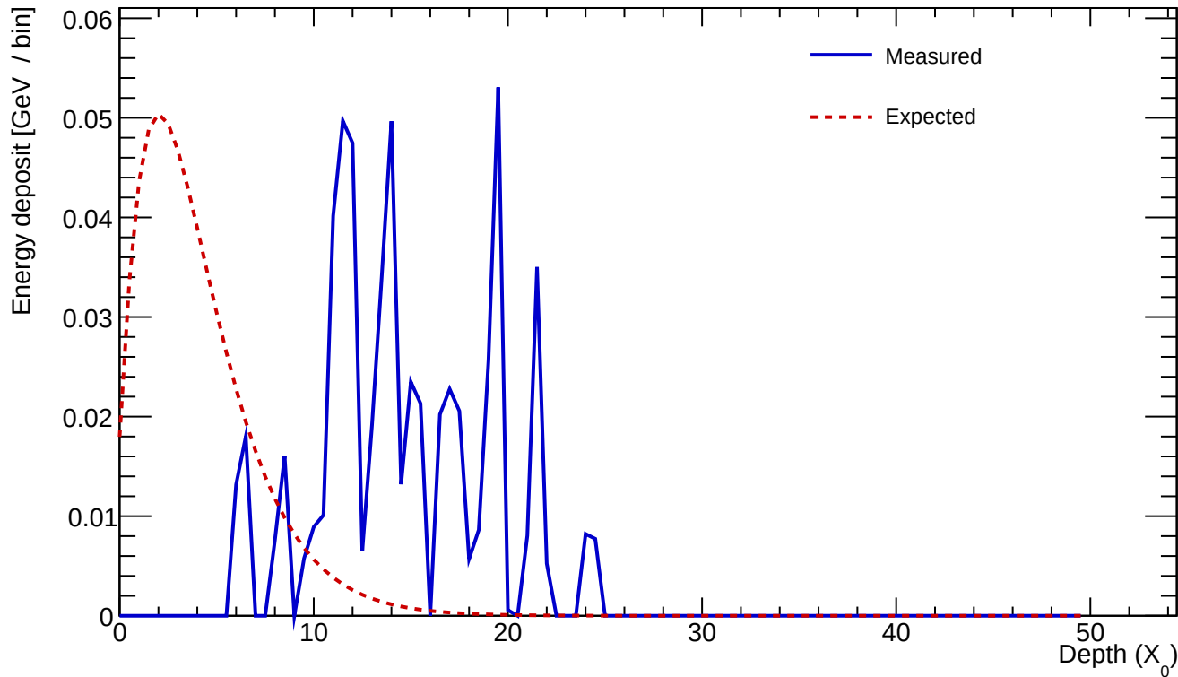
Cluster 518 E=0.606 GeV profileStart=10.00 X_0 \chi=0.6476
