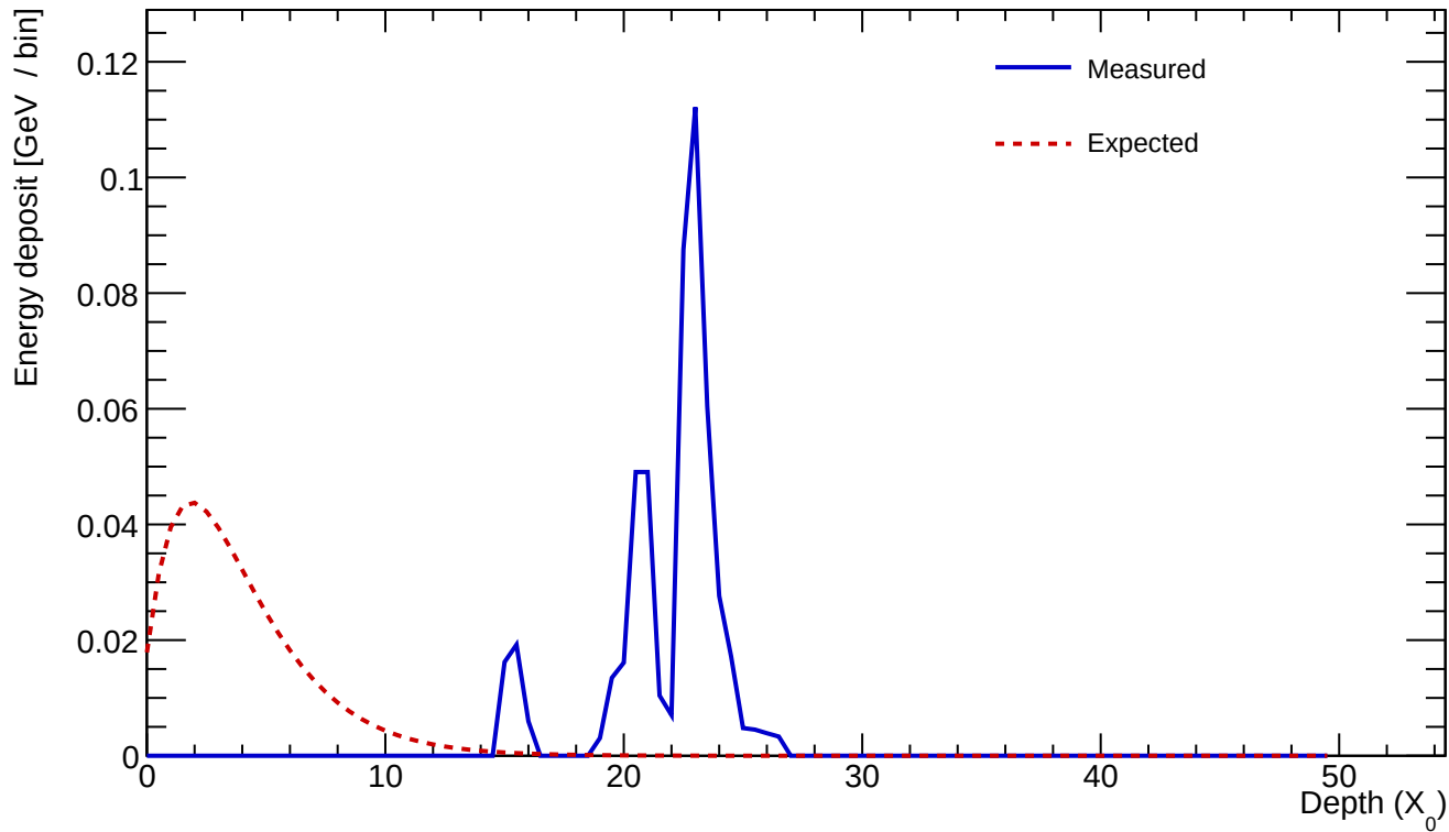
Cluster 445 E=0.511 GeV profileStart=19.50 X_0 \chi=0.6863
