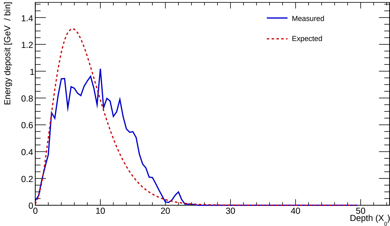
Cluster 121 E=23.896 GeV profileStart=0.50 X_0 \chi=0.3283
