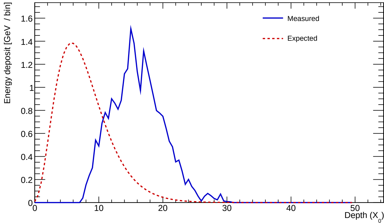
Cluster 651 E=25.221 GeV profileStart=9.00 X_0 \chi=0.2182
