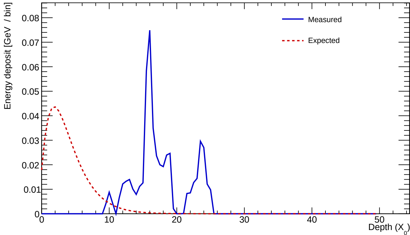
Cluster 960 E=0.509 GeV profileStart=14.00 X_0 \chi=0.7273
