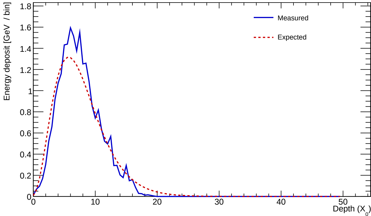
Cluster 282 E=23.865 GeV profileStart=0.50 X_0 \chi=0.1455
