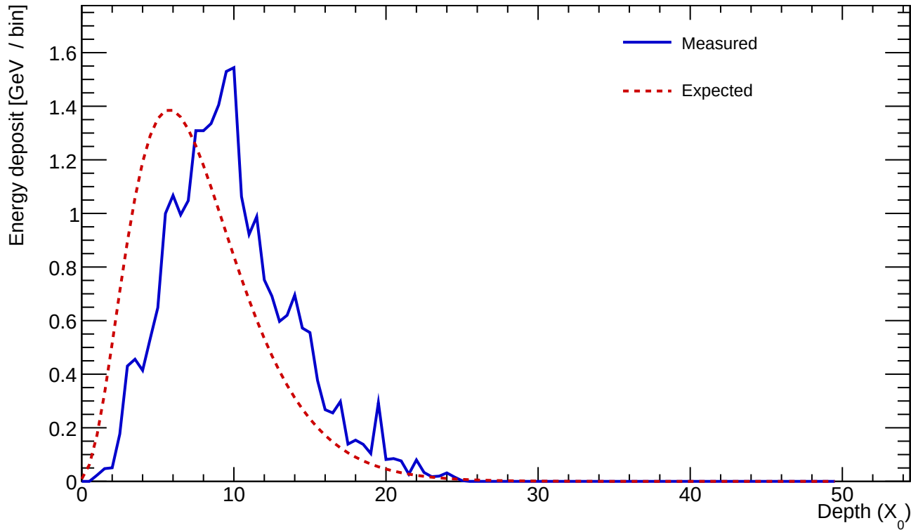
Cluster 332 E=25.273 GeV profileStart=2.50 X_0 \chi=0.1662
