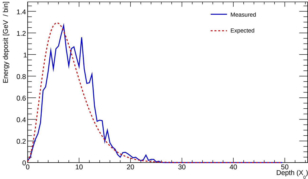
Cluster 614 E=23.445 GeV profileStart=1.00 X_0 \chi=0.1586
