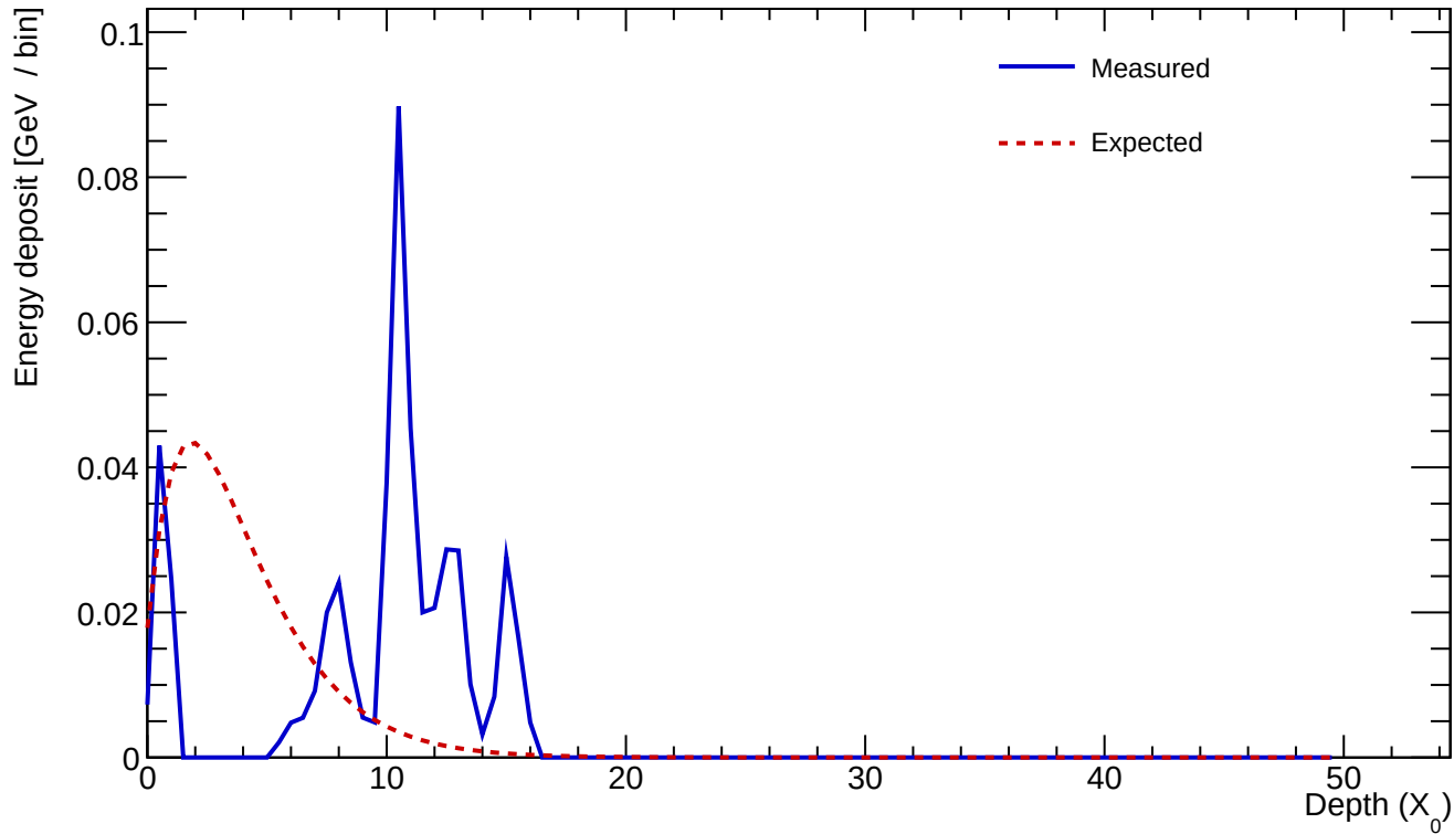
Cluster 243 E=0.506 GeV profileStart=7.50 X_0 \chi=0.6962
