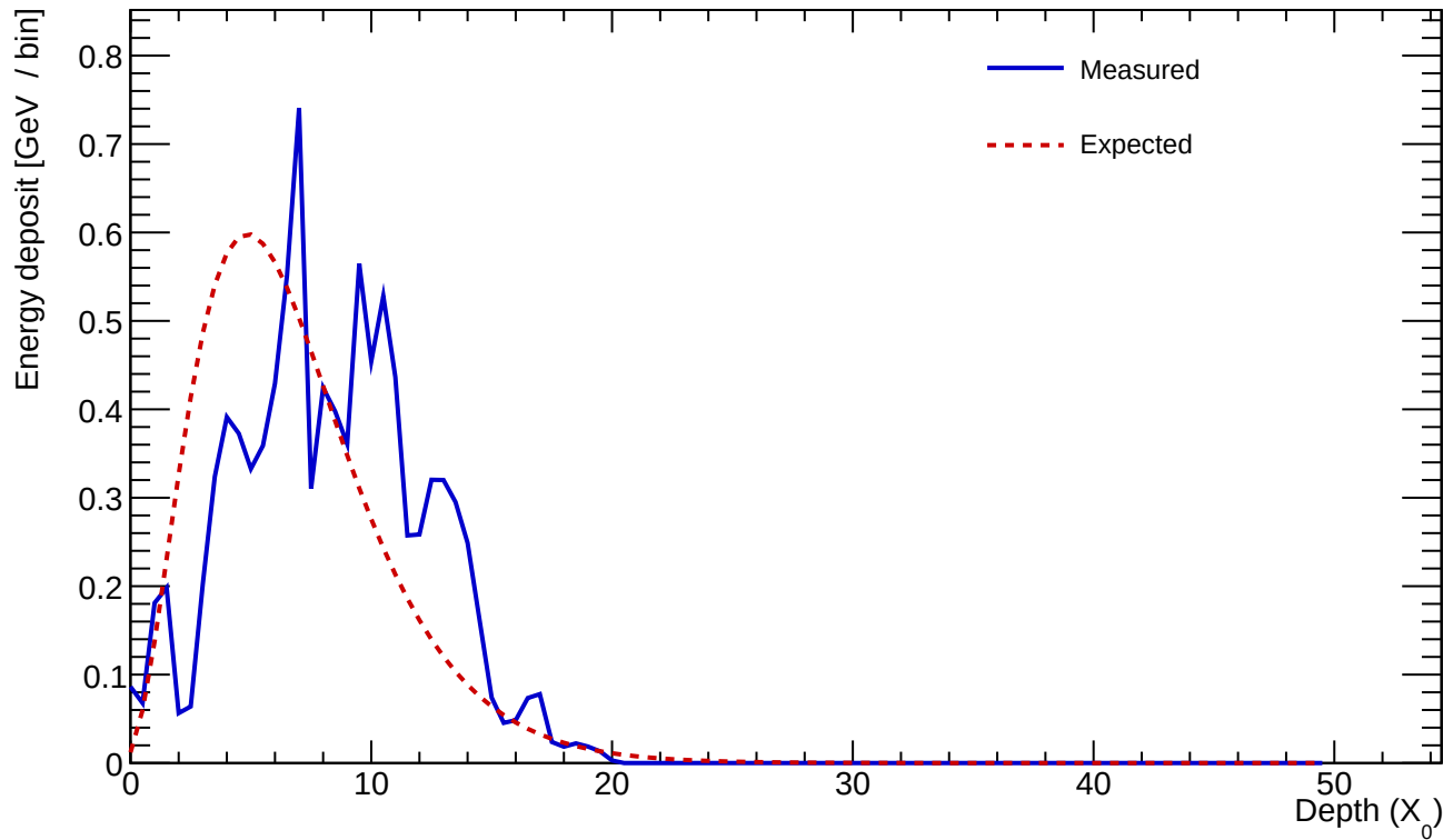
Cluster 727 E=10.113 GeV profileStart=2.00 X_0 \chi=0.3269
