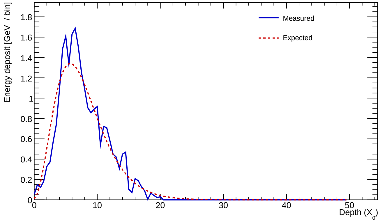
Cluster 129 E=24.359 GeV profileStart=0.50 X_0 \chi=0.1749
