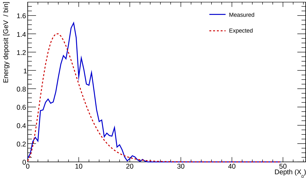
Cluster 132 E=25.572 GeV profileStart=2.00 X_0 \chi=0.2328
