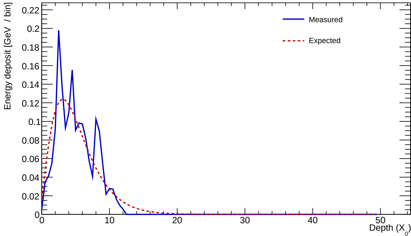
Cluster 1015 E=1.742 GeV profileStart=0.50 X_0 \chi=0.2523
