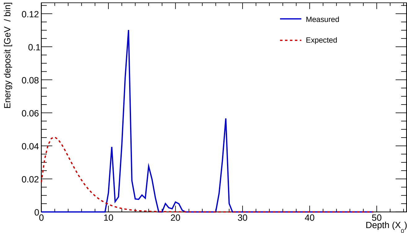
Cluster 226 E=0.533 GeV profileStart=10.00 X_0 \chi=0.8553
