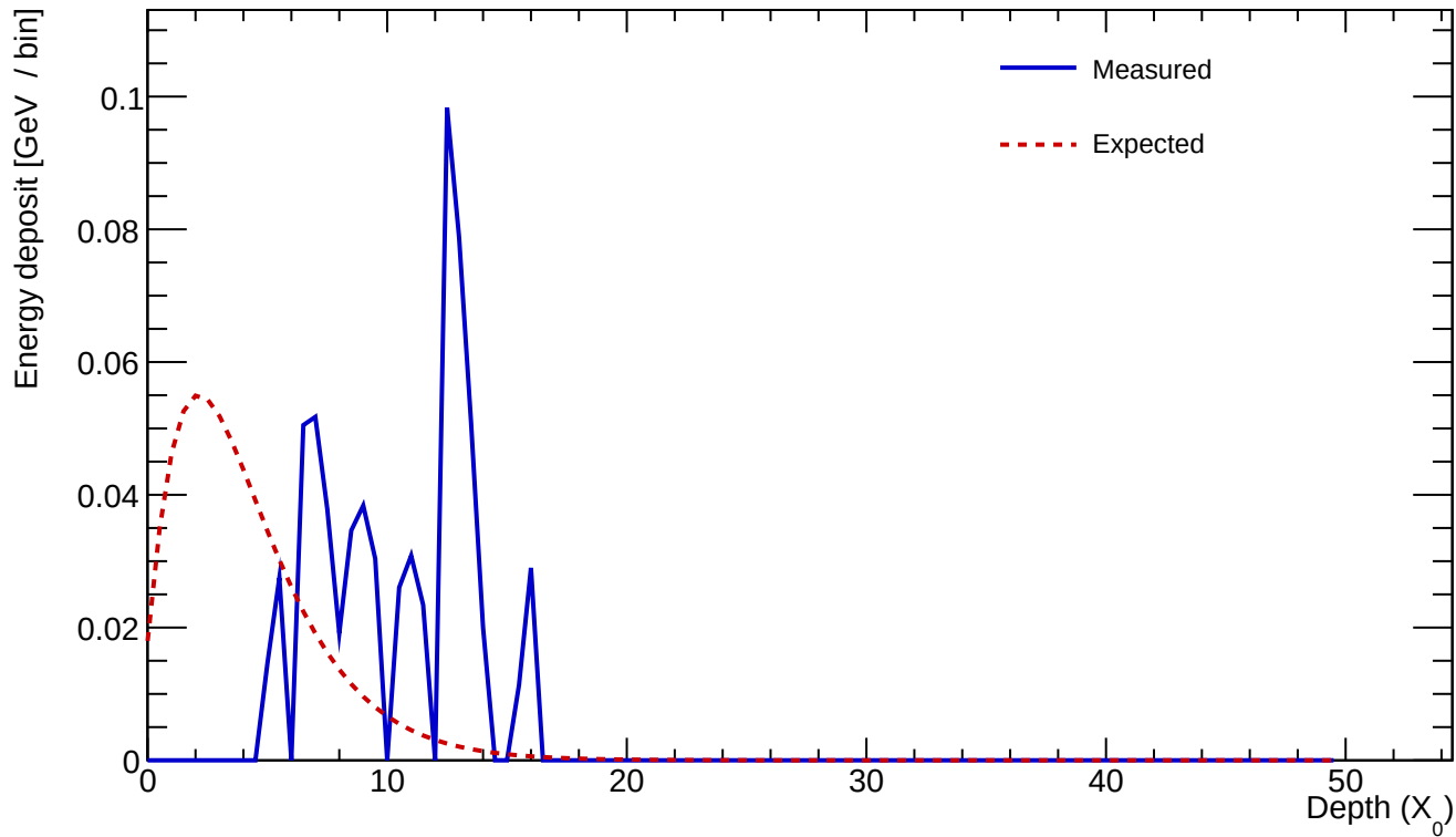
Cluster 818 E=0.673 GeV profileStart=5.00 X_0 \chi=0.6240
