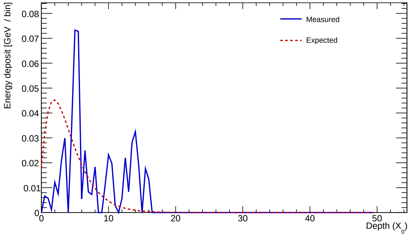
Cluster 911 E=0.531 GeV profileStart=3.00 X_0 \chi=0.8263
