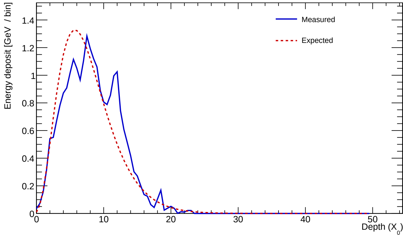
Cluster 228 E=24.090 GeV profileStart=0.50 X_0 \chi=0.1916
