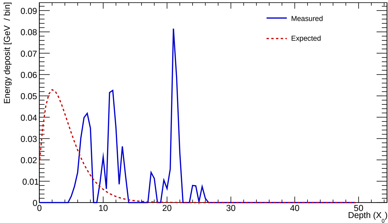
Cluster 294 E=0.643 GeV profileStart=6.00 X_0 \chi=0.9492
