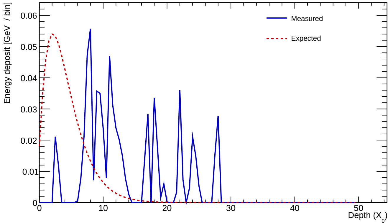
Cluster 658 E=0.659 GeV profileStart=6.50 X_0 \chi=0.7422
