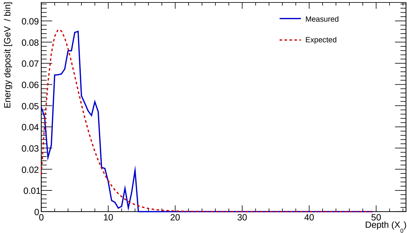
Cluster 404 E=1.142 GeV profileStart=1.00 X_0 \chi=0.2763
