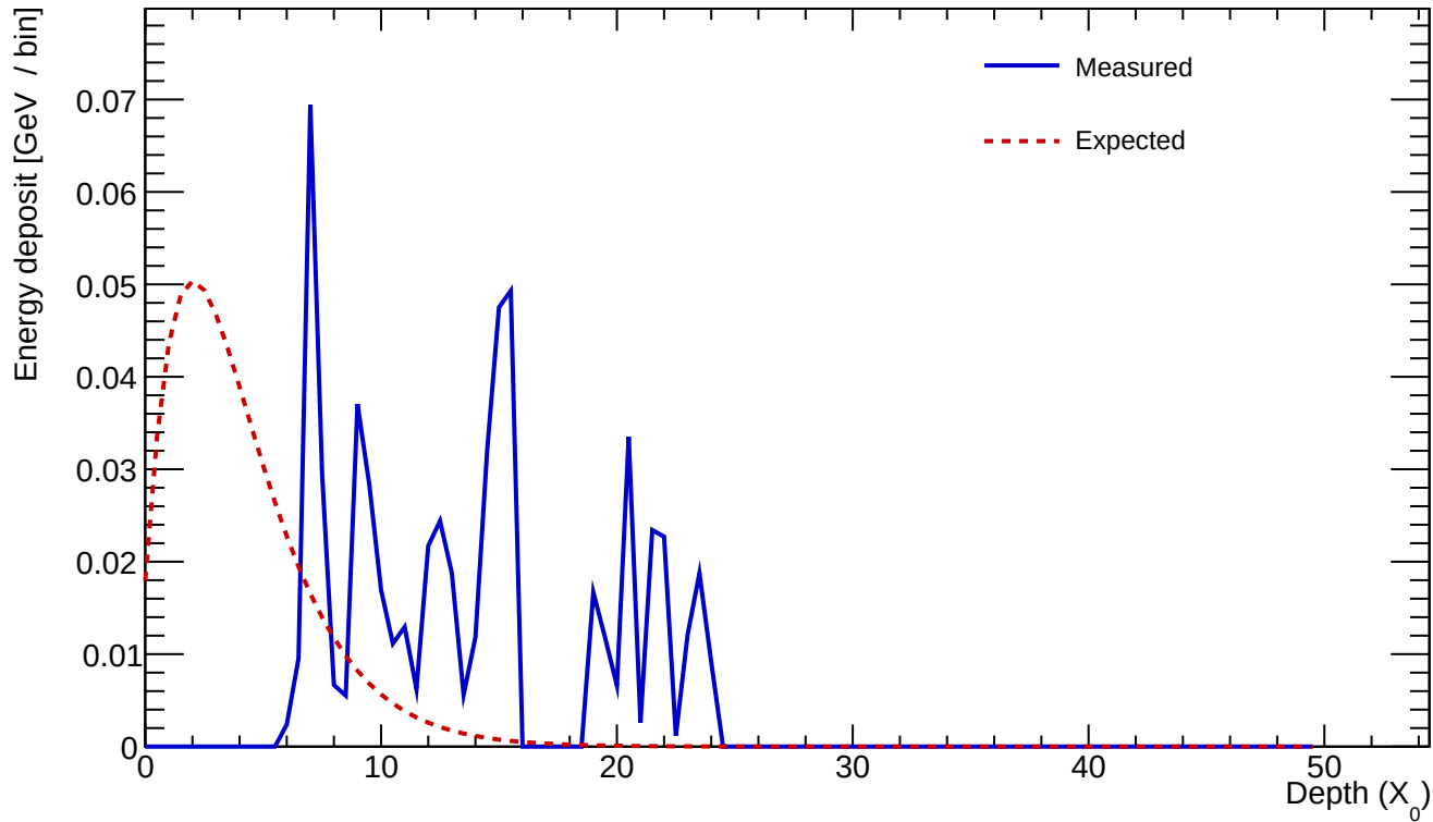
Cluster 628 E=0.605 GeV profileStart=6.50 X_0 \chi=0.9310
