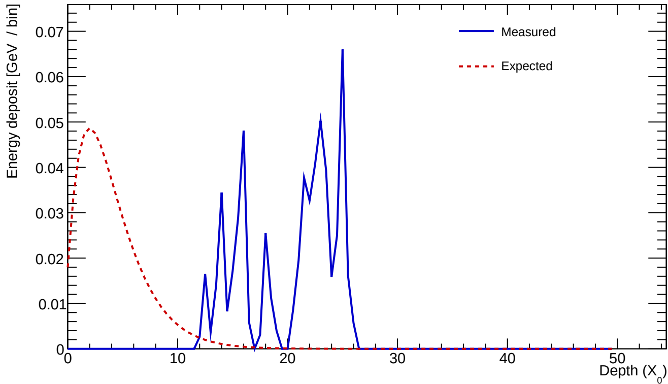
Cluster 365 E=0.580 GeV profileStart=21.00 X_0 \chi=0.6115
