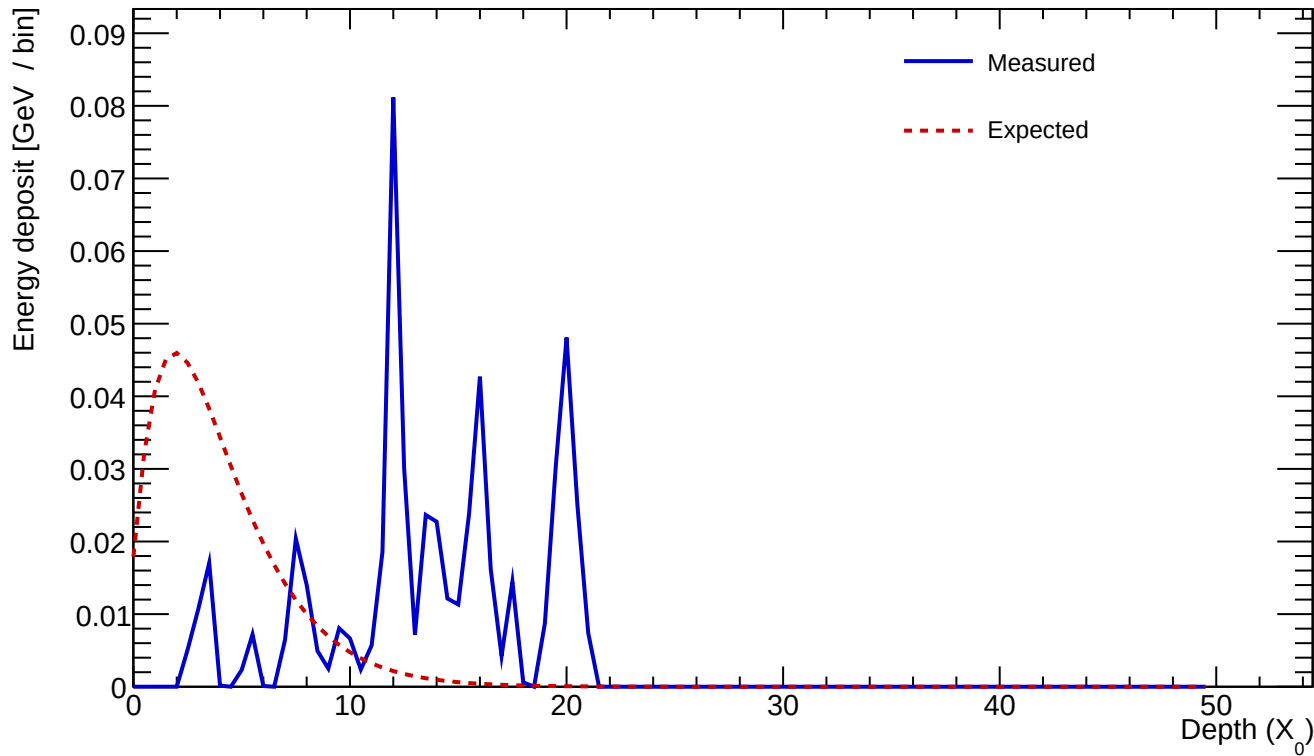
Cluster 696 E=0.542 GeV profileStart=11.00 X_0 \chi=0.8736
