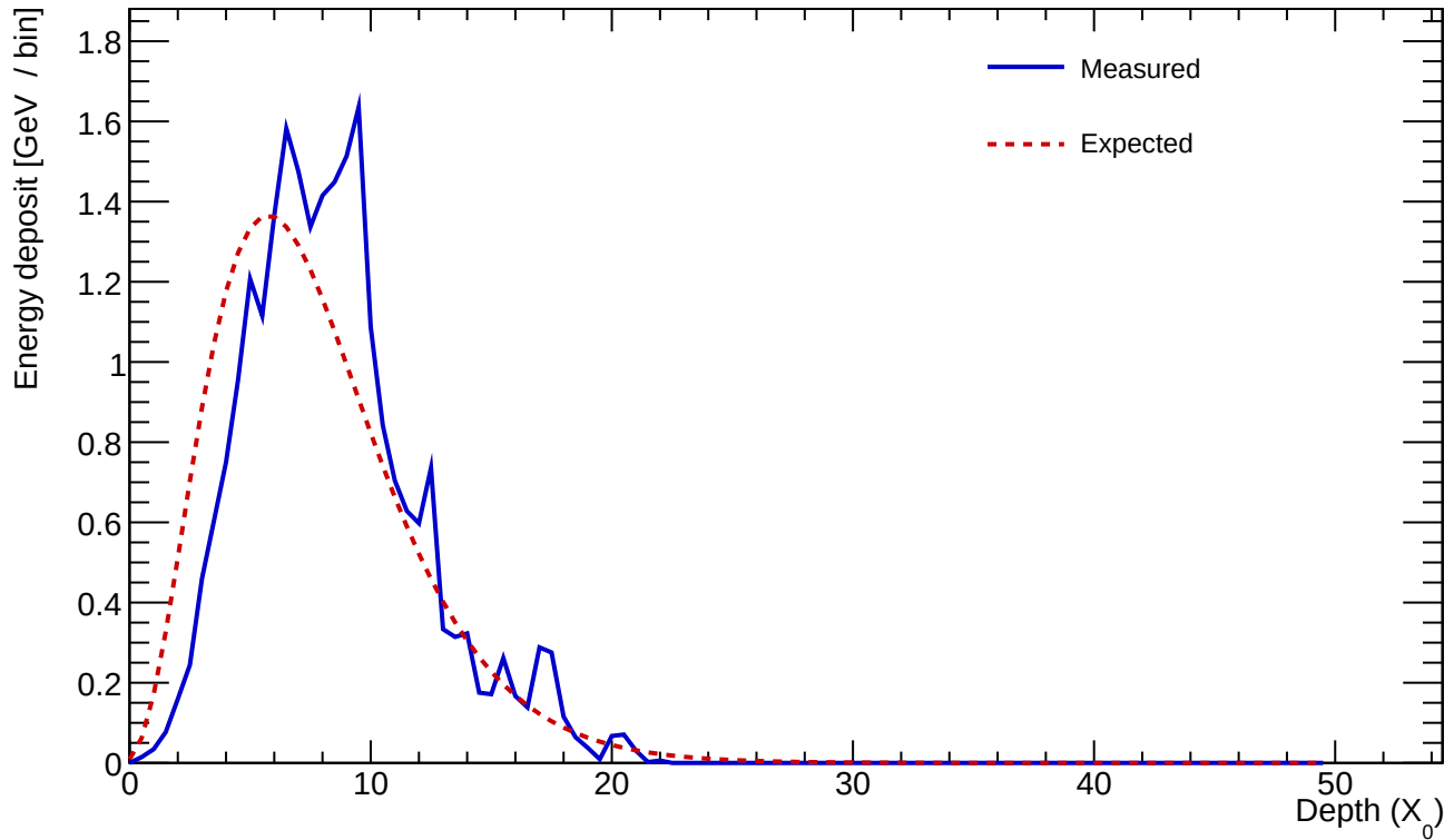
Cluster 894 E=24.842 GeV profileStart=1.00 X_0 \chi=0.1716
