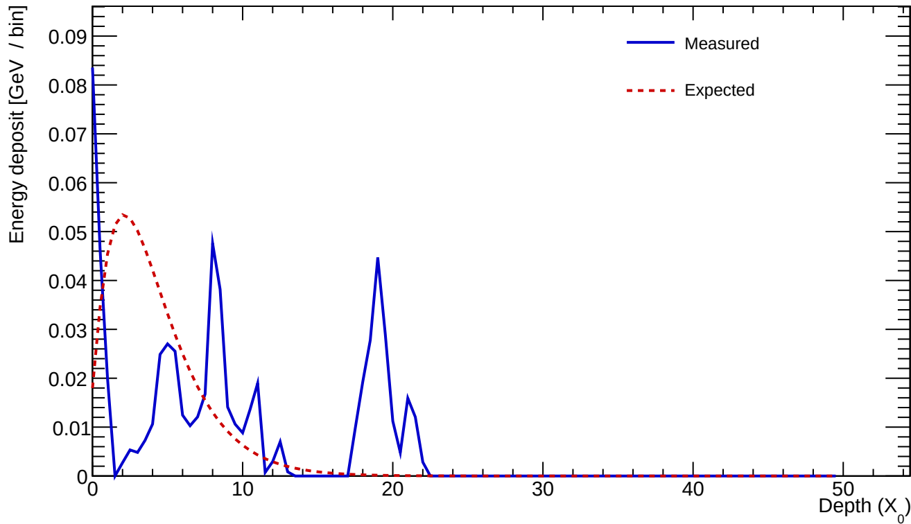
Cluster 57 E=0.651 GeV profileStart=4.00 X_0 \chi=1.0592
