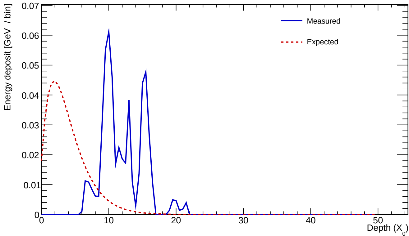
Cluster 186 E=0.524 GeV profileStart=8.50 X_0 \chi=0.6138
