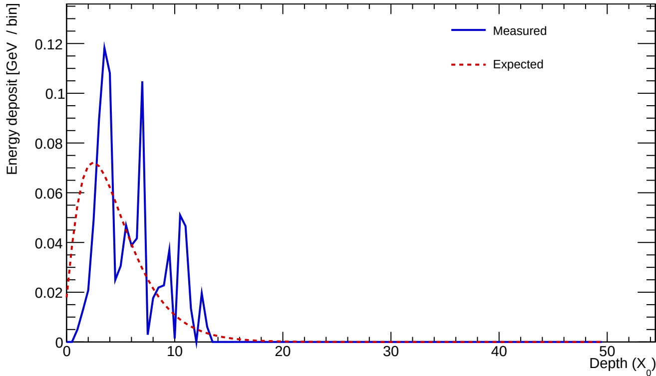
Cluster 1054 E=0.931 GeV profileStart=1.50 X_0 \chi=0.5515
