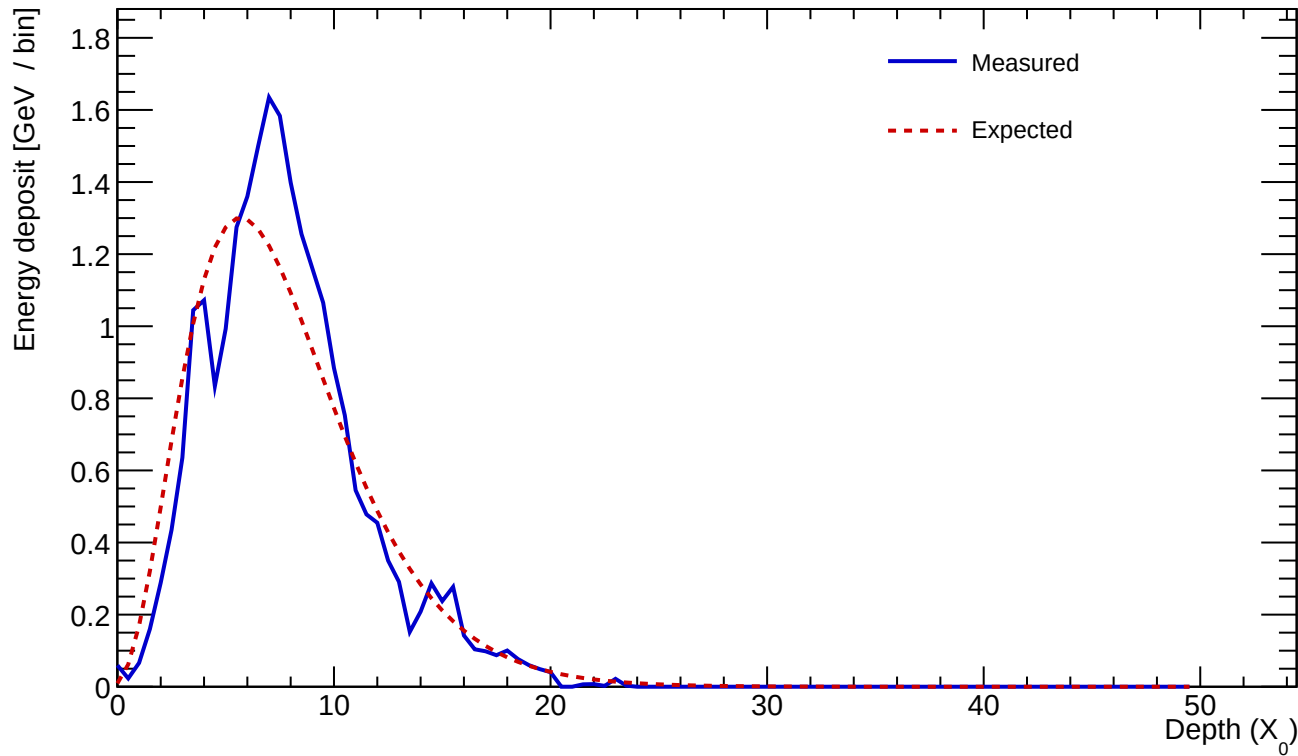
Cluster 248 E=23.562 GeV profileStart=0.50 X_0 \chi=0.1752
