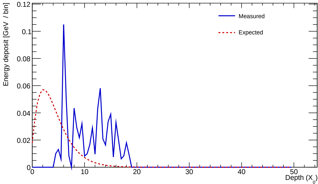
Cluster 654 E=0.705 GeV profileStart=5.00 X_0 \chi=0.8020
