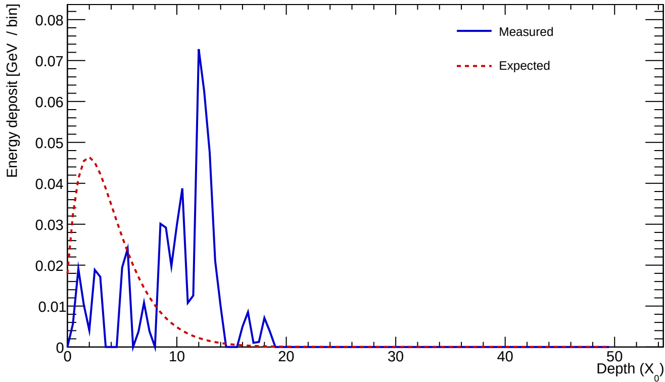
Cluster 791 E=0.548 GeV profileStart=8.50 X_0 \chi=0.7907
