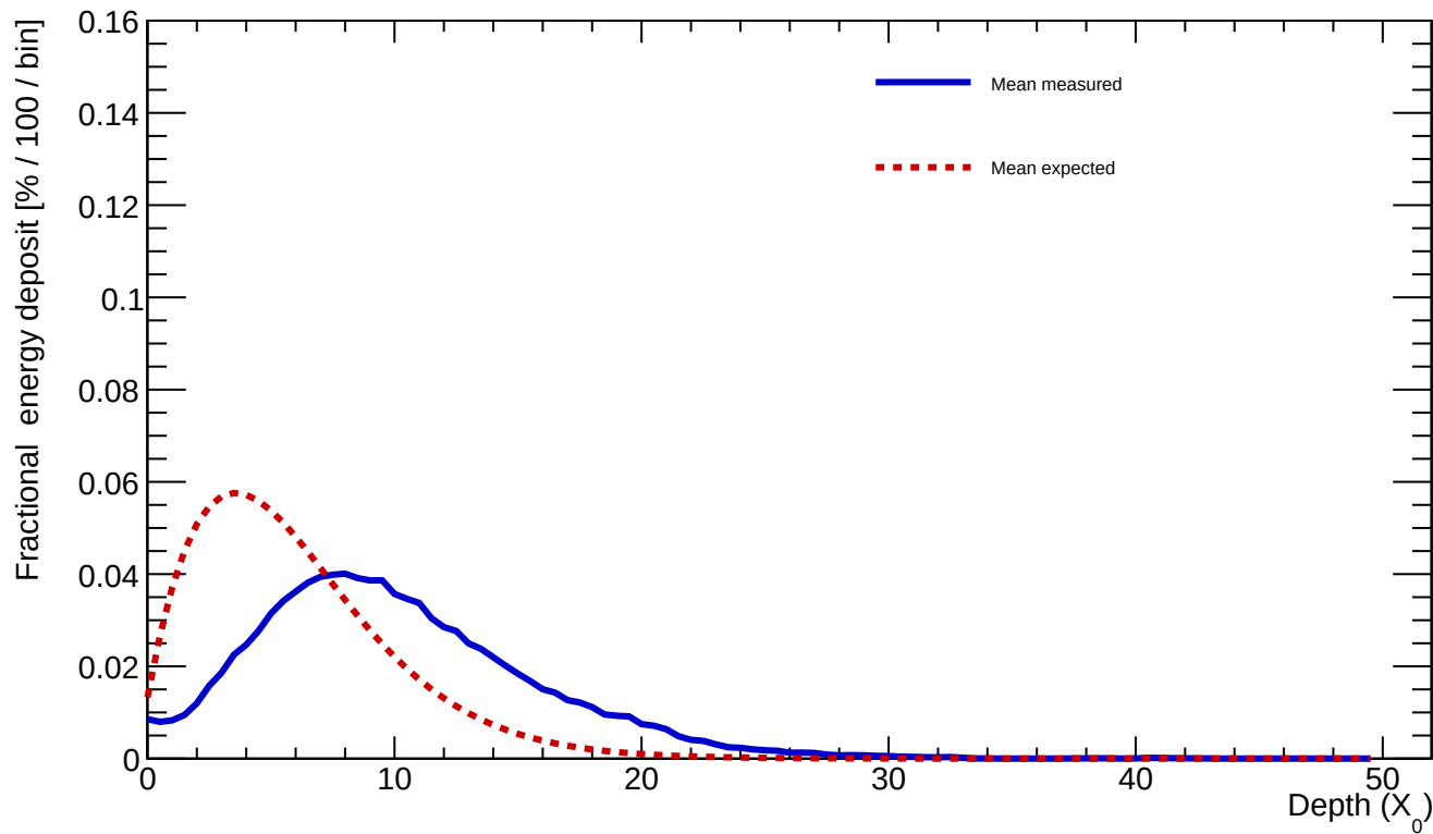
Average longitudinal profile (1209 clusters): measured vs expected
