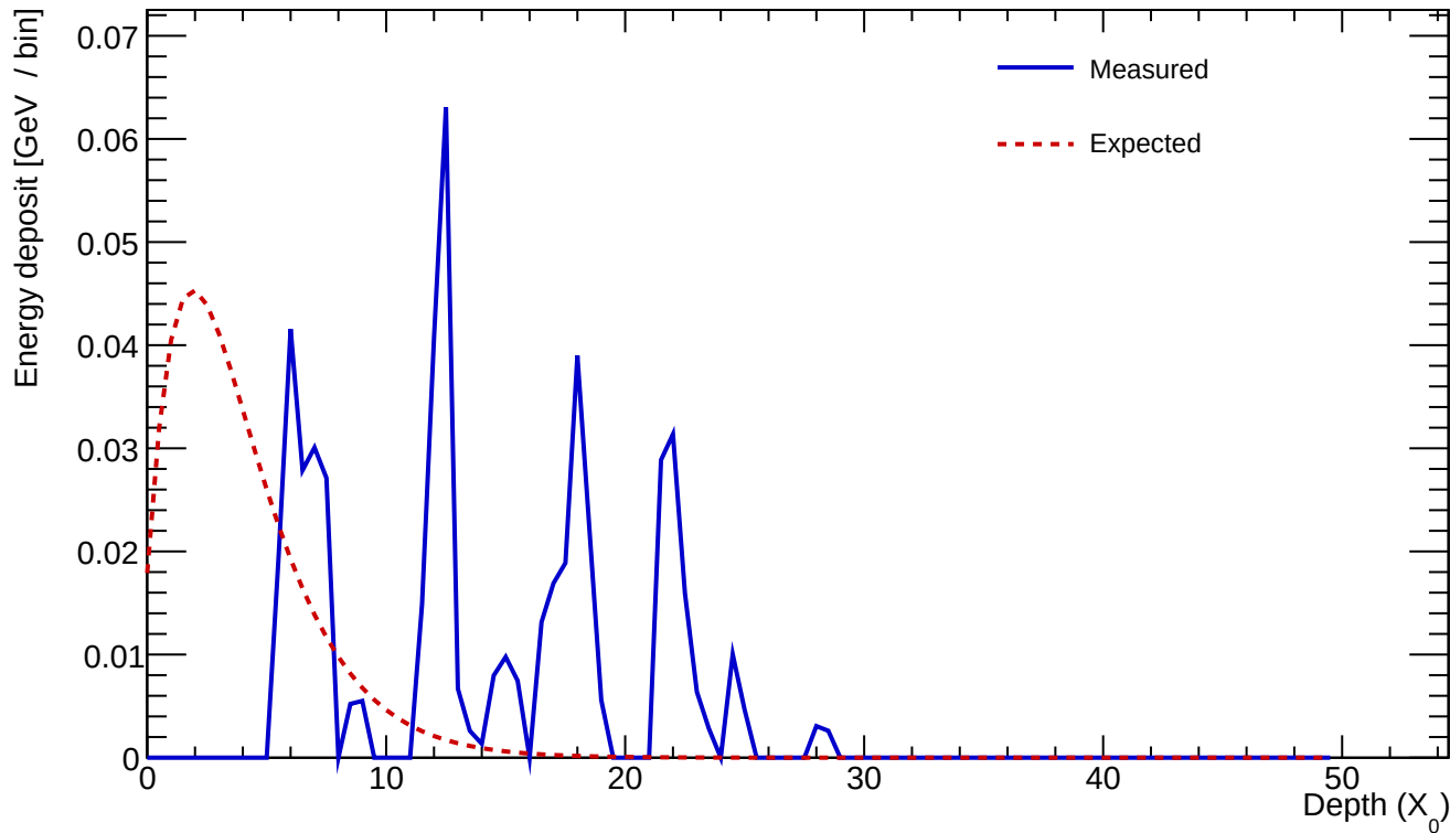
Cluster 1038 E=0.533 GeV profileStart=5.50 X_0 \chi=1.1215
