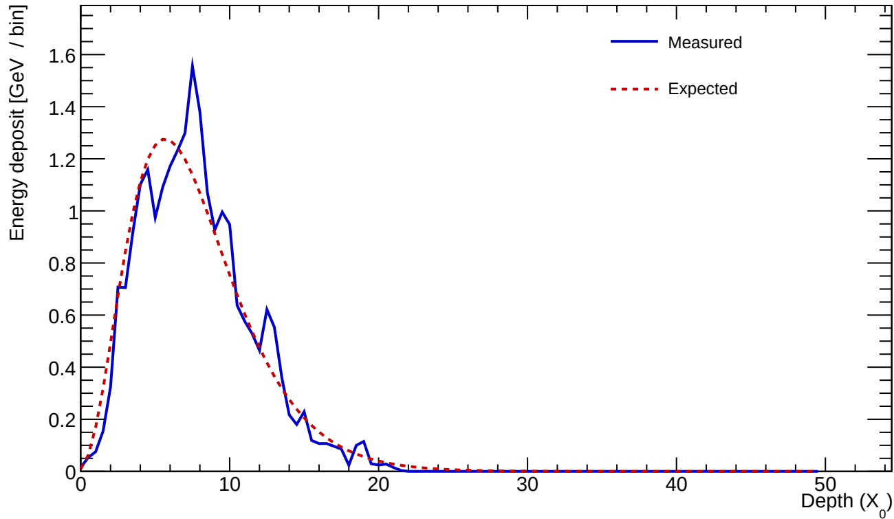
Cluster 187 E=23.082 GeV profileStart=0.50 X_0 \chi=0.1451
