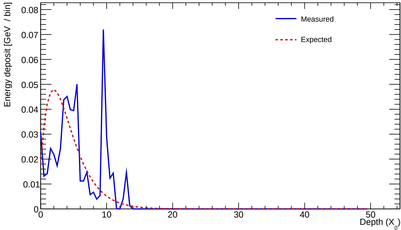
Cluster 247 E=0.570 GeV profileStart=1.00 X_0 \chi=0.6092
