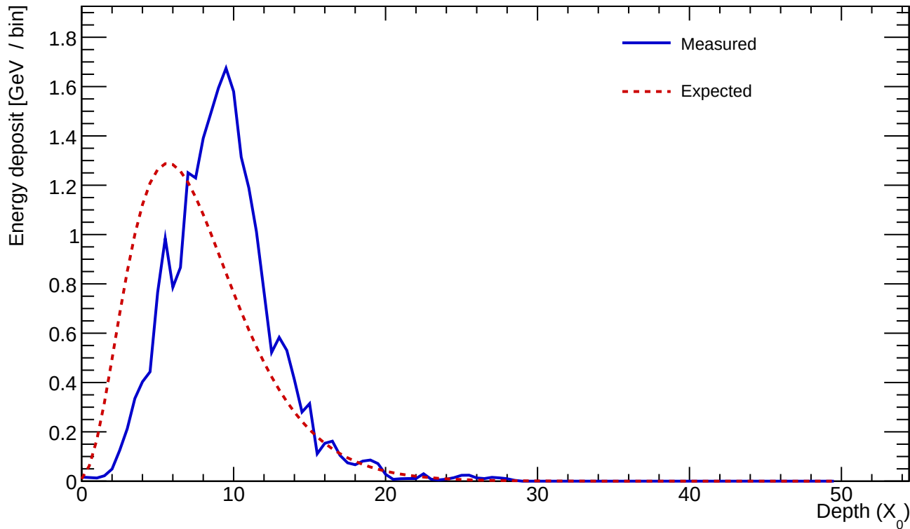
Cluster 707 E=23.330 GeV profileStart=2.00 X_0 \chi=0.2370
