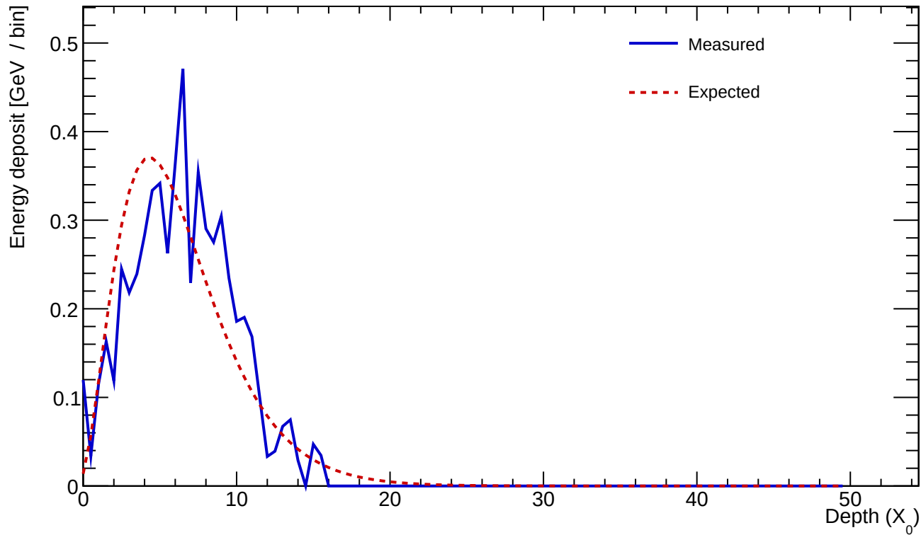
Cluster 854 E=5.968 GeV profileStart=1.00 X_0 \chi=0.2386
