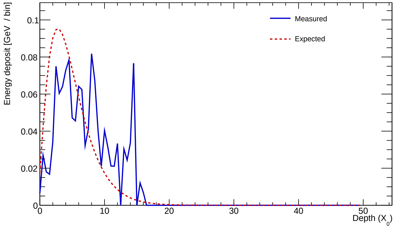
Cluster 375 E=1.287 GeV profileStart=1.50 X_0 \chi=0.4567
