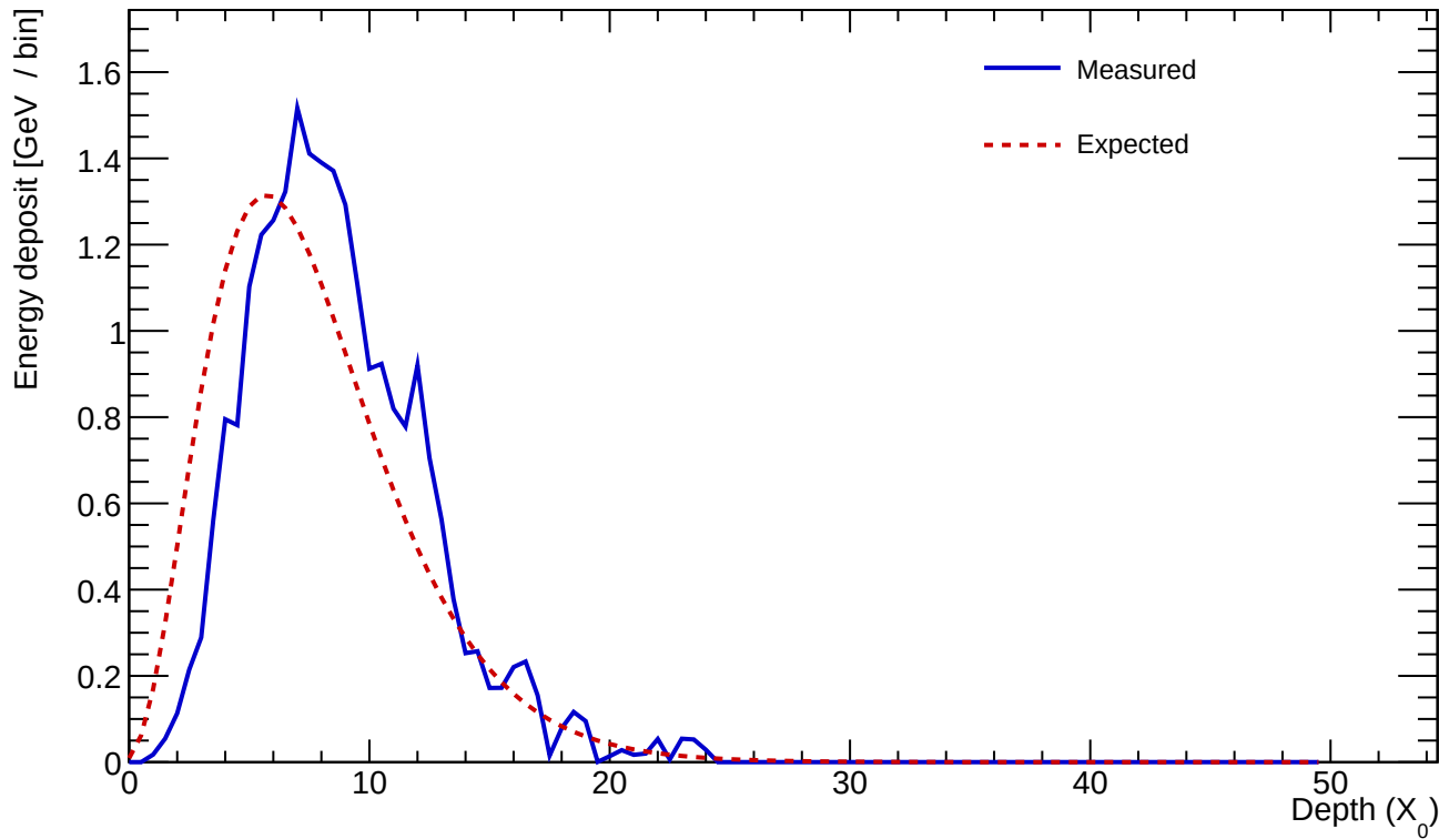
Cluster 862 E=23.863 GeV profileStart=1.50 X_0 \chi=0.1308
