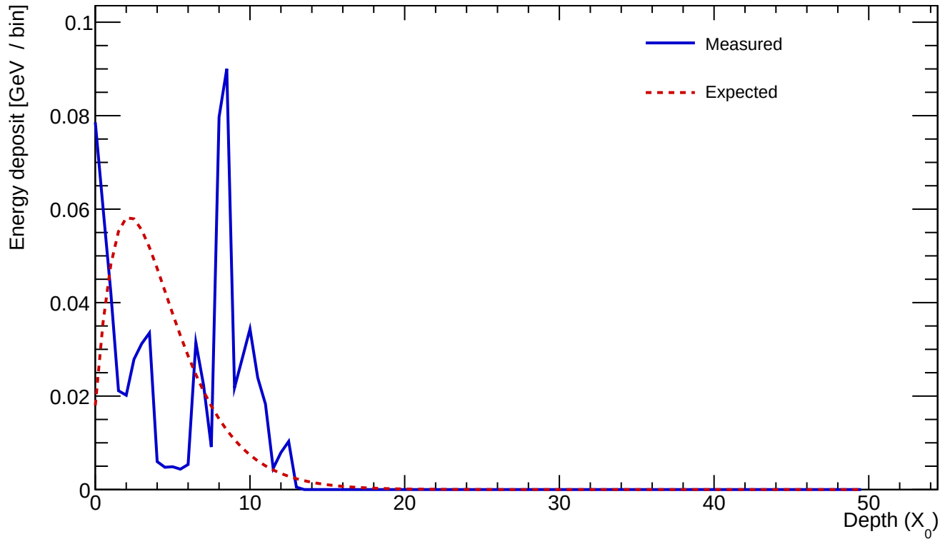
Cluster 1035 E=0.723 GeV profileStart=6.00 X_0 \chi=0.8984
