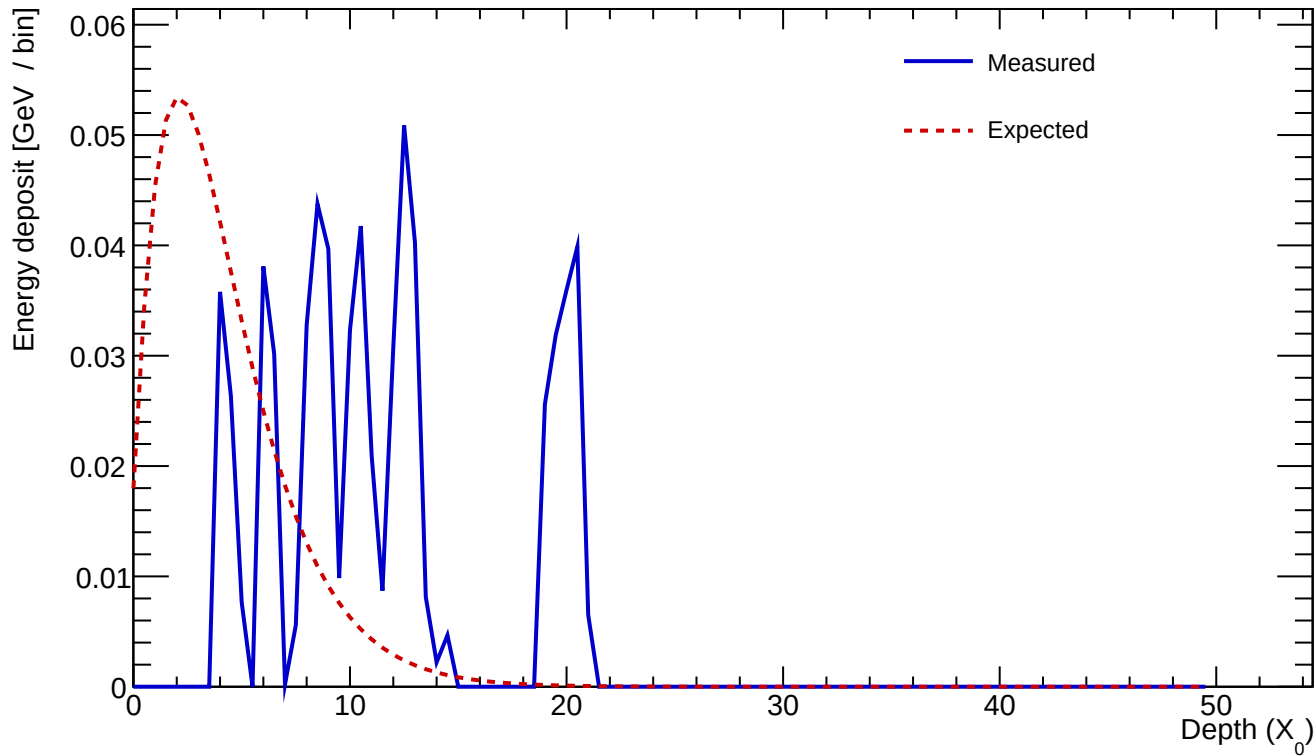
Cluster 421 E=0.650 GeV profileStart=5.50 X_0 \chi=0.8557
