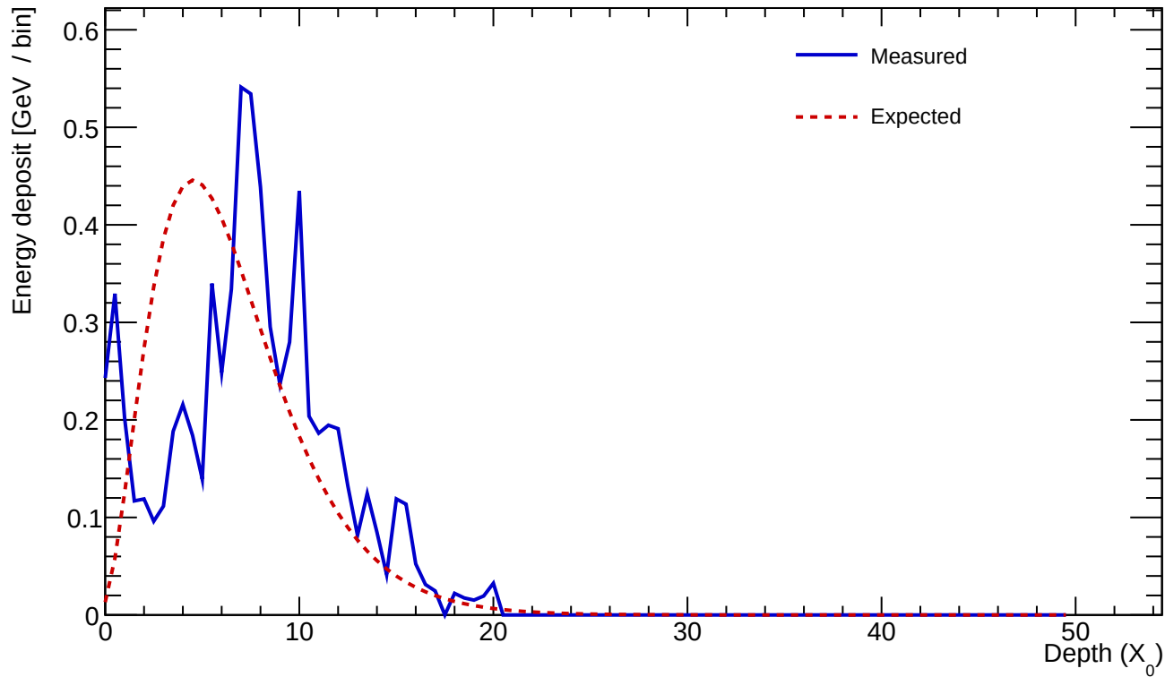
Cluster 670 E=7.316 GeV profileStart=2.00 X_0 \chi=0.4090
