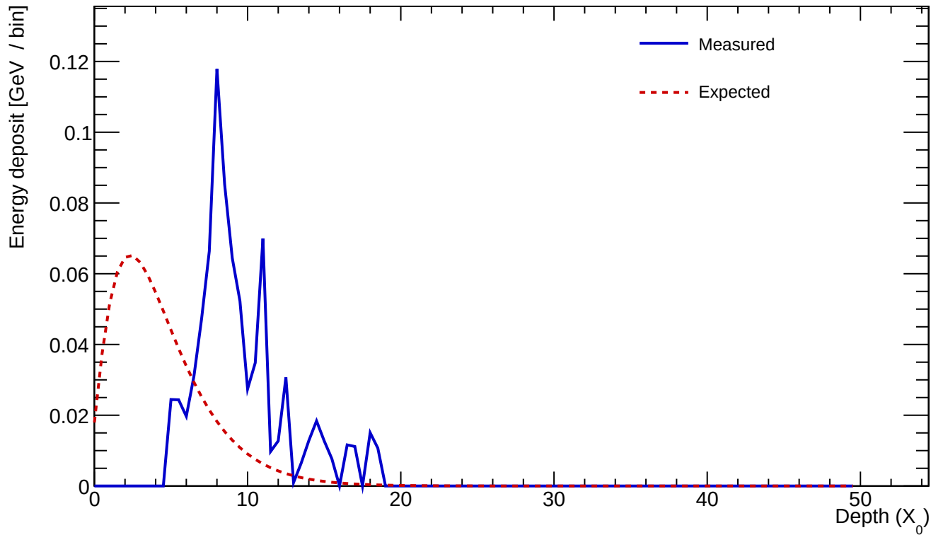
Cluster 279 E=0.826 GeV profileStart=5.50 X_0 \chi=0.4274
