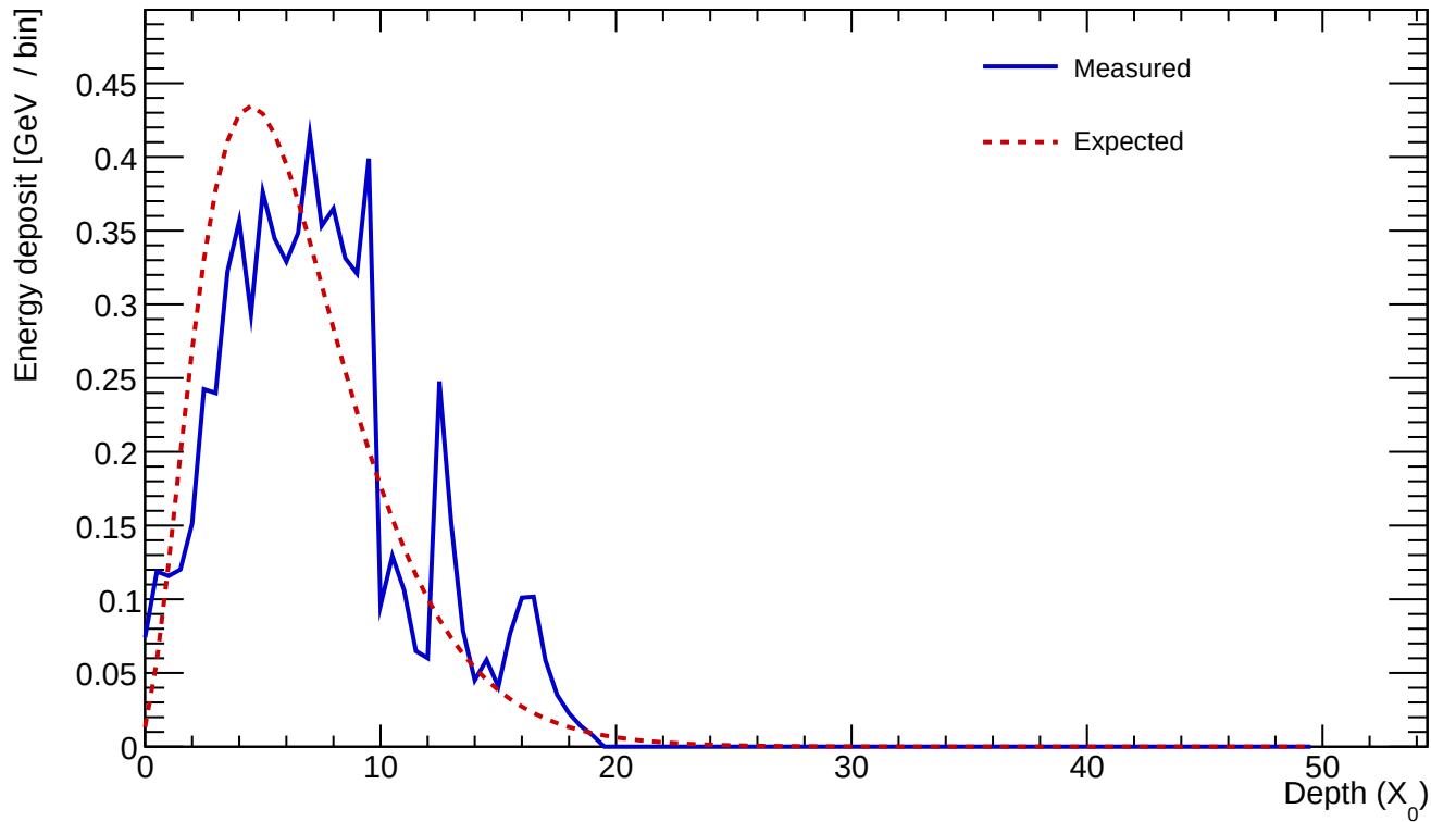
Cluster 637 E=7.114 GeV profileStart=1.00 X_0 \chi=0.2897
