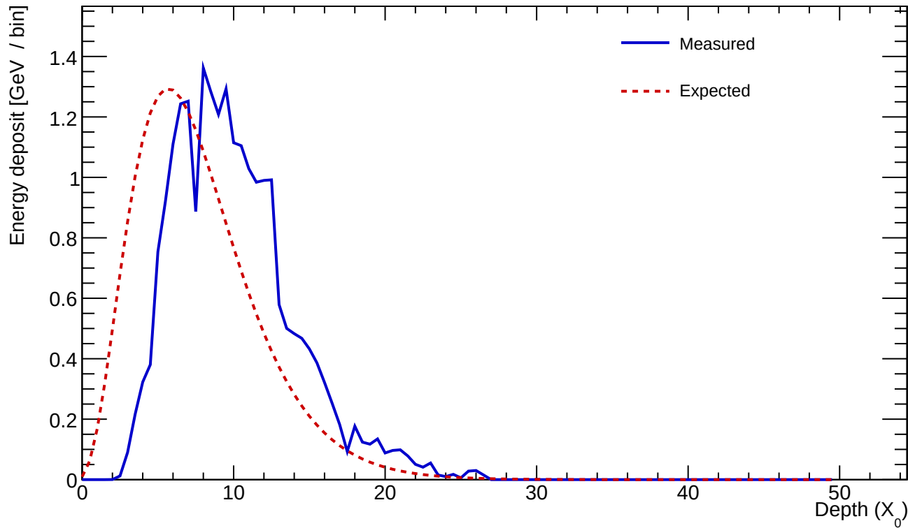
Cluster 718 E=23.431 GeV profileStart=2.50 X_0 \chi=0.1056
