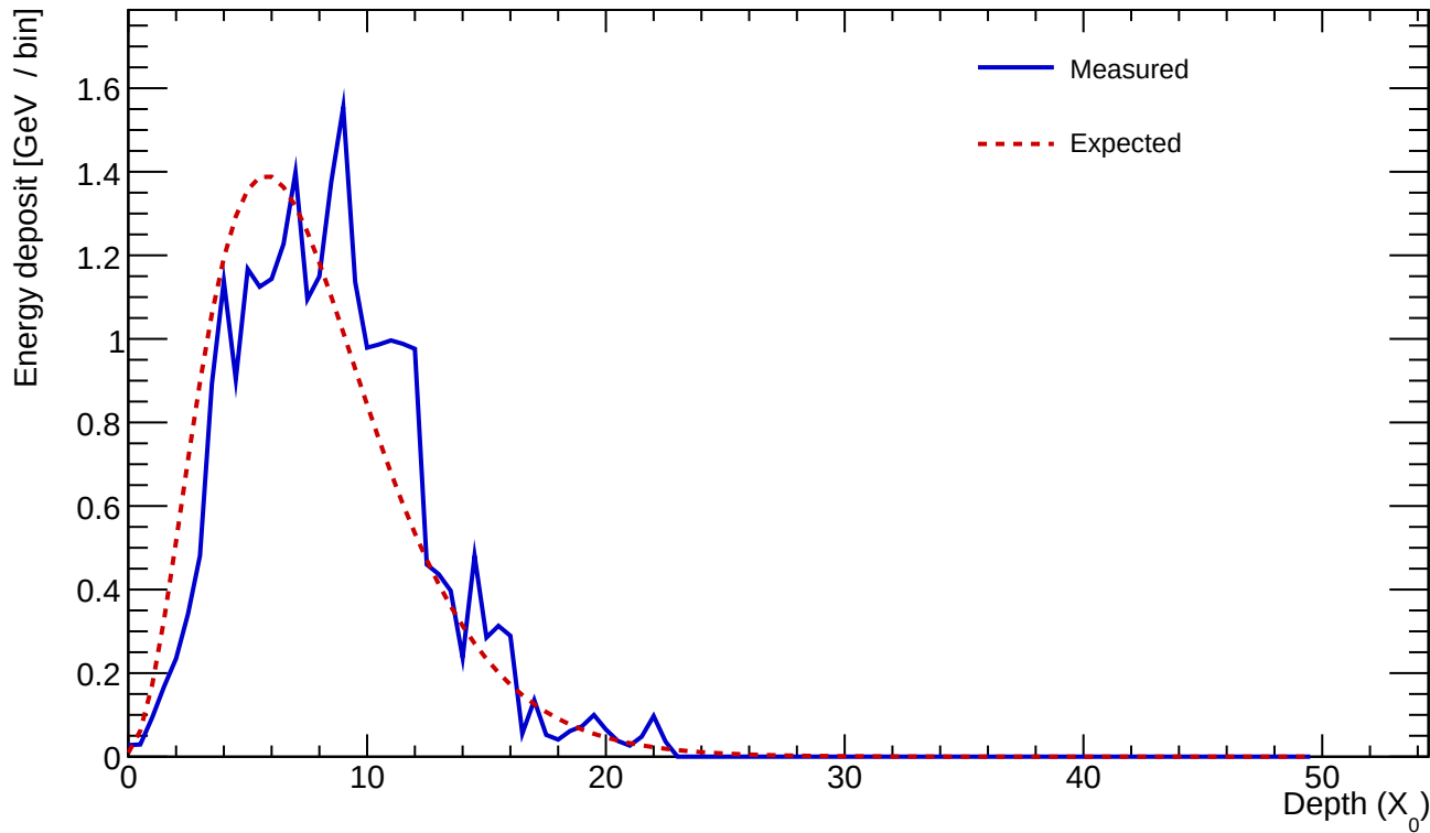
Cluster 895 E=25.339 GeV profileStart=1.00 X_0 \chi=0.1798
