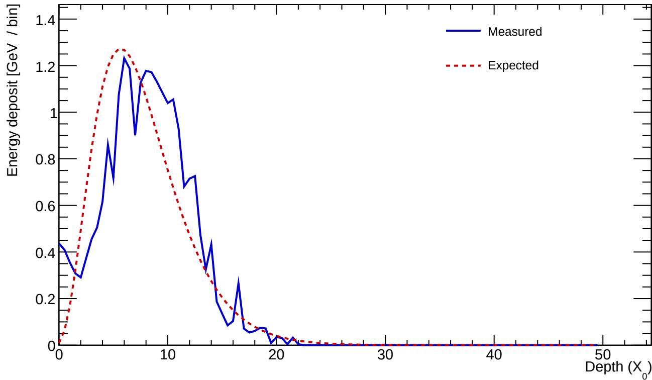
Cluster 59 E=23.017 GeV profileStart=1.50 X_0 \chi=0.2249
