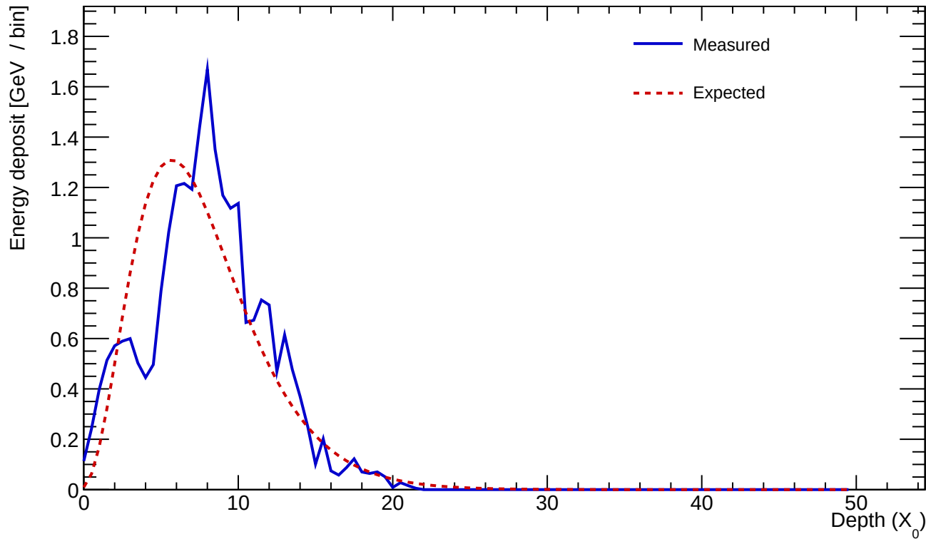
Cluster 77 E=23.742 GeV profileStart=1.50 X_0 \chi=0.2699
