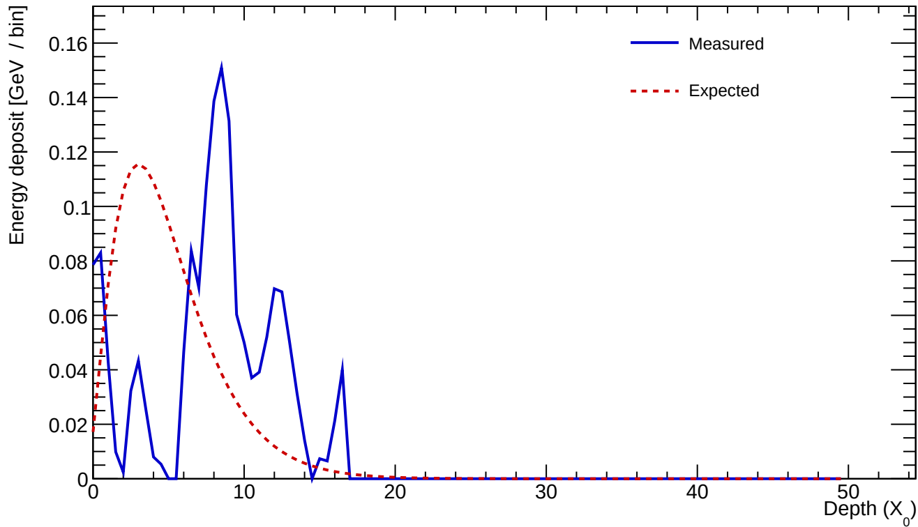
Cluster 823 E=1.608 GeV profileStart=5.50 X_0 \chi=0.5065
