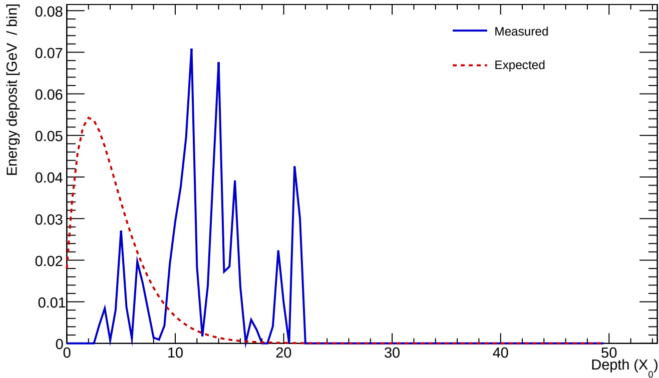
Cluster 982 E=0.663 GeV profileStart=9.50 X_0 \chi=0.7042
