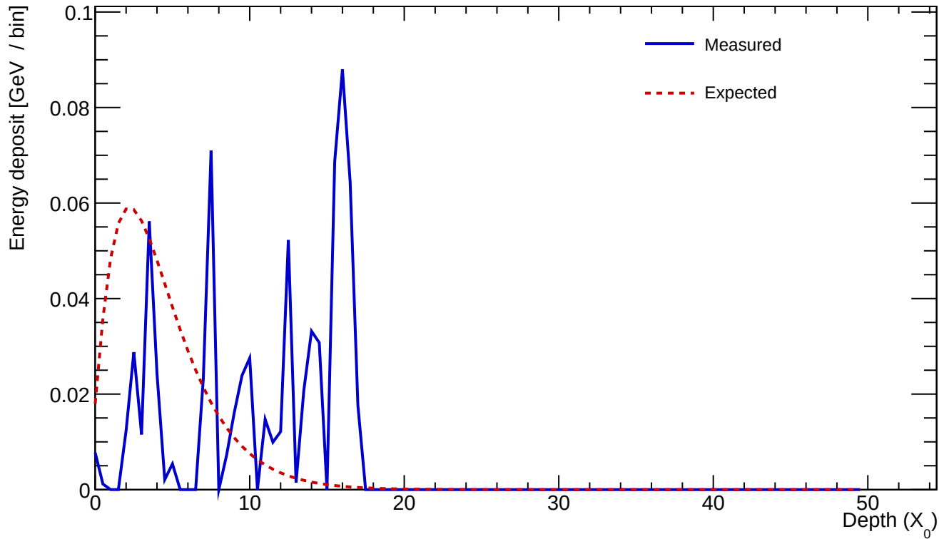
Cluster 184 E=0.732 GeV profileStart=13.50 X_0 \chi=0.7309
