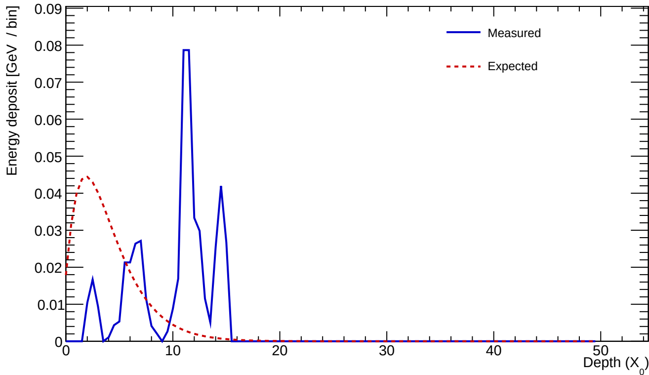
Cluster 297 E=0.521 GeV profileStart=10.00 X_0 \chi=0.7029
