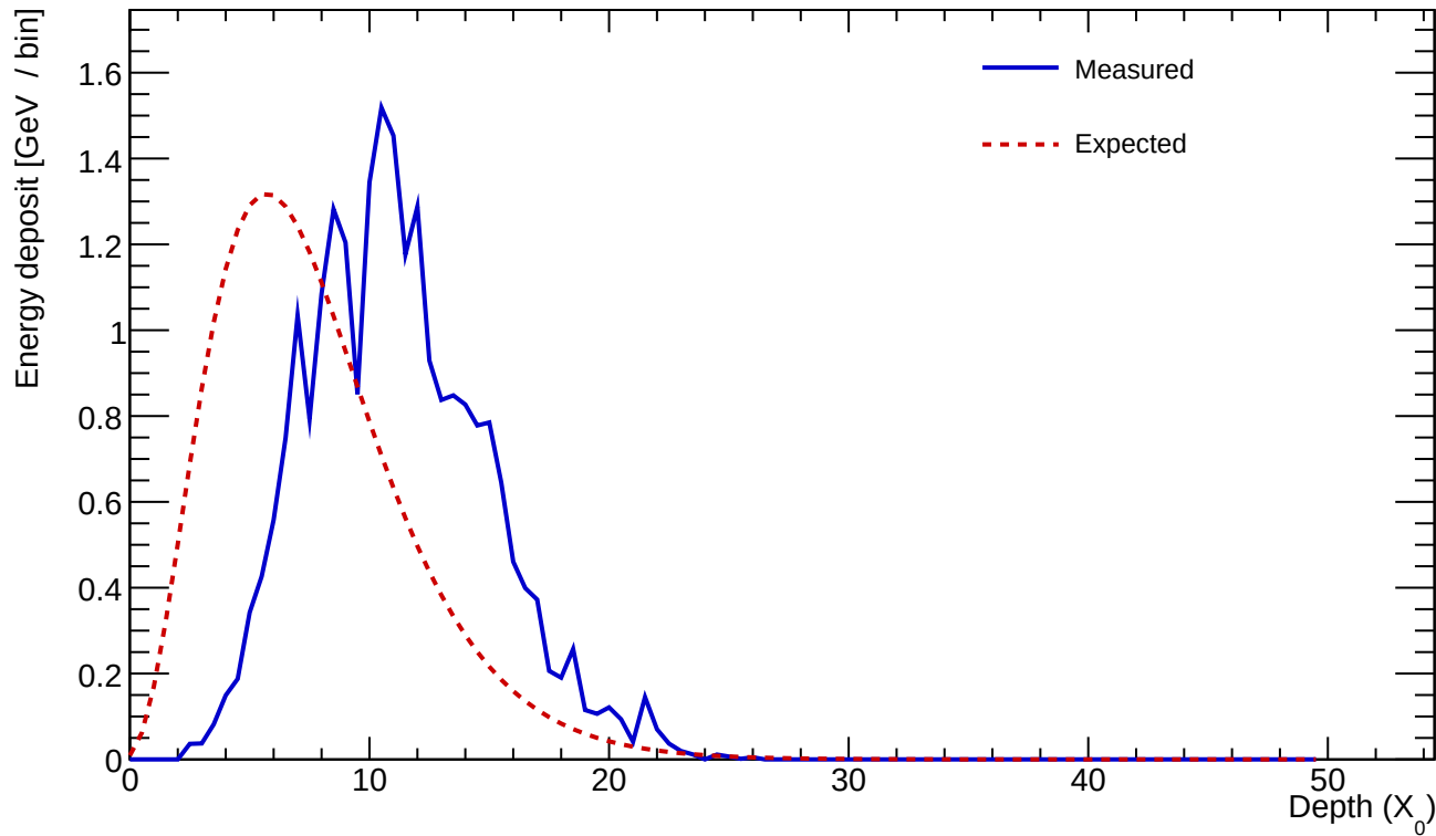
Cluster 678 E=23.920 GeV profileStart=4.00 X_0 \chi=0.1690
