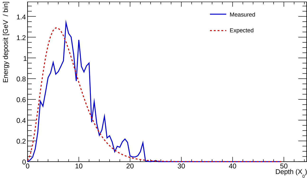
Cluster 138 E=23.377 GeV profileStart=1.00 X_0 \chi=0.2225
