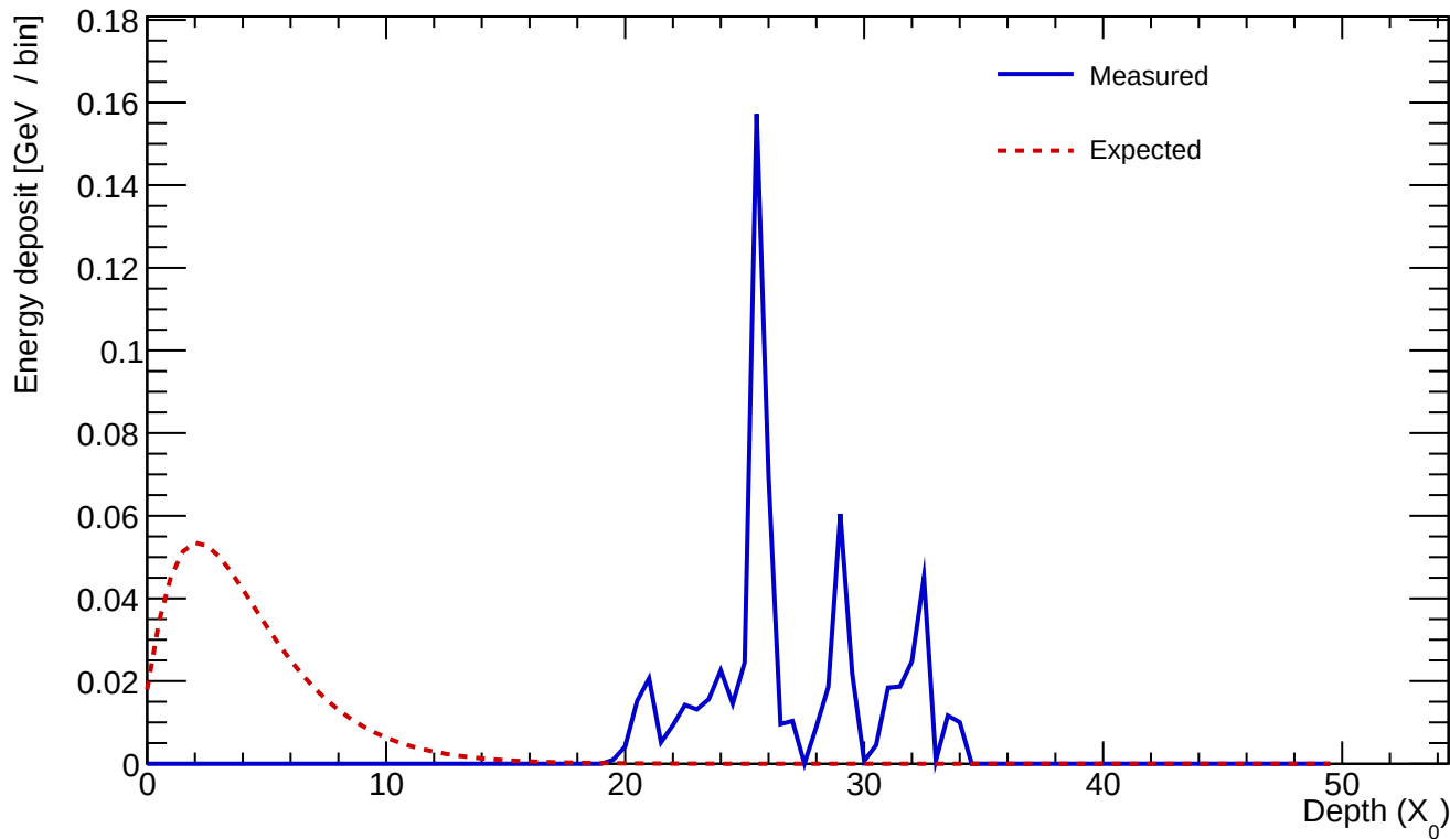
Cluster 624 E=0.651 GeV profileStart=23.50 X_0 \chi=0.8867
