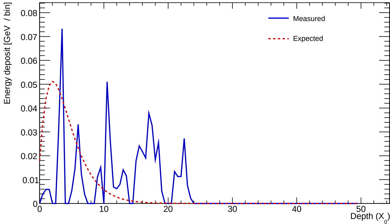
Cluster 387 E=0.617 GeV profileStart=15.00 X_0 \chi=1.0572
