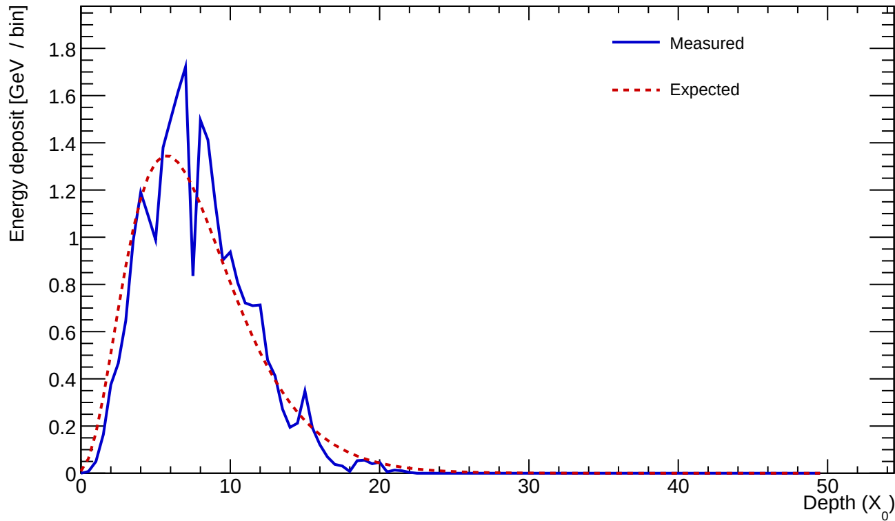
Cluster 745 E=24.465 GeV profileStart=0.50 X_0 \chi=0.1723
