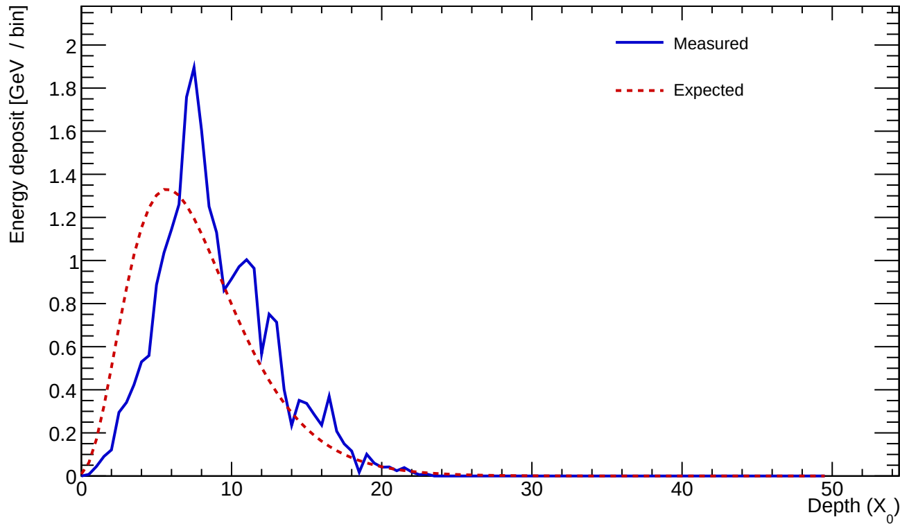
Cluster 496 E=24.171 GeV profileStart=1.50 X_0 \chi=0.1894
