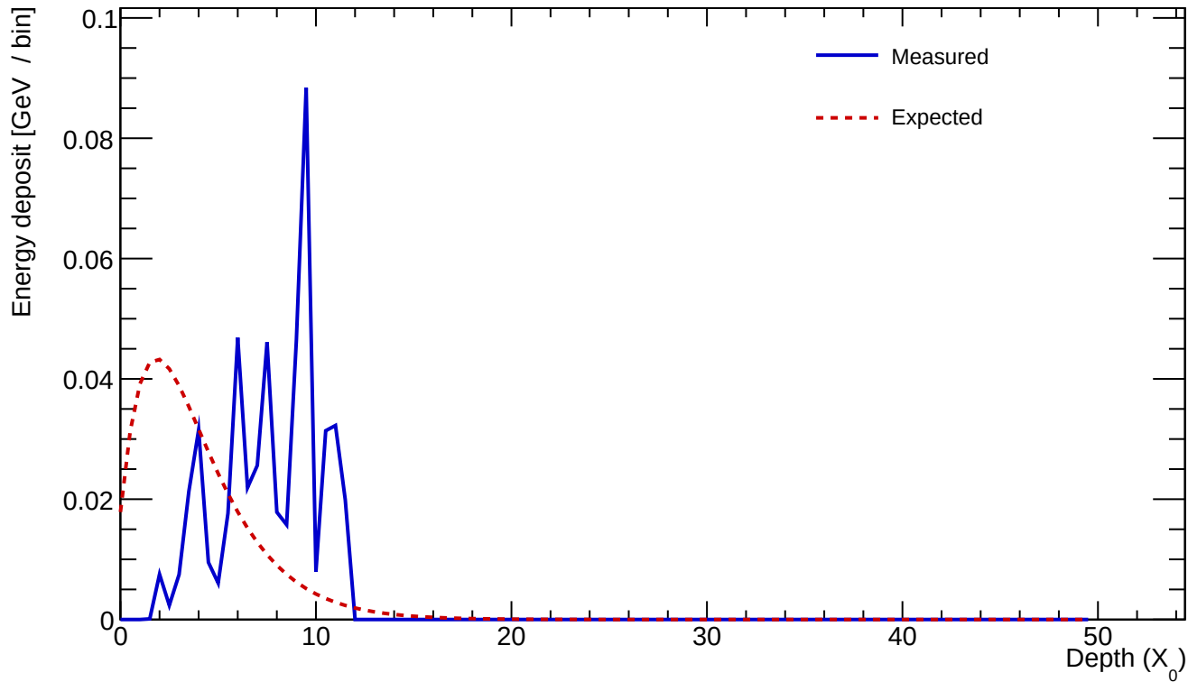
Cluster 503 E=0.504 GeV profileStart=5.50 X_0 \chi=0.5795
