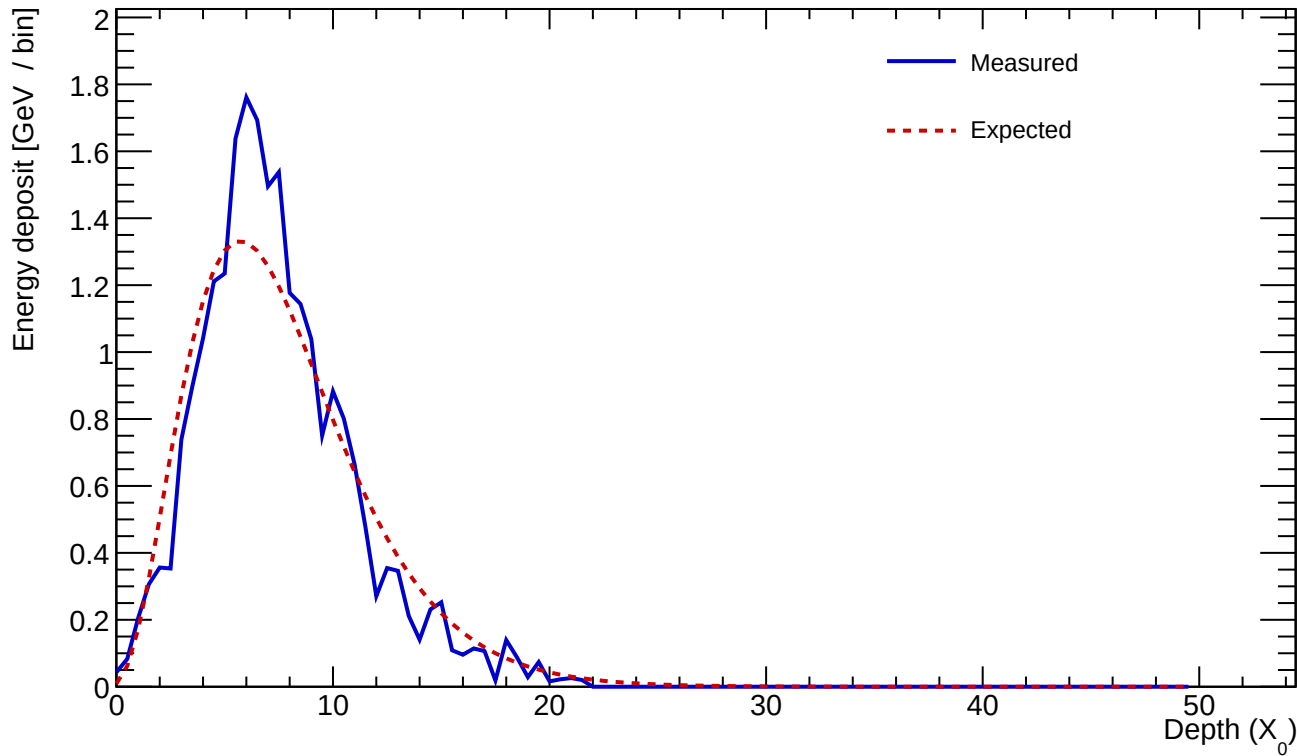
Cluster 573 E=24.193 GeV profileStart=0.50 X_0 \chi=0.1799
