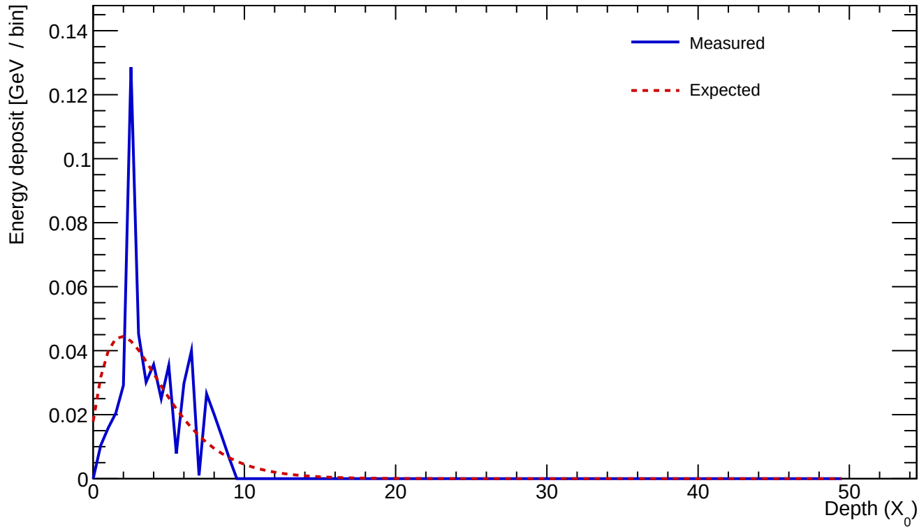
Cluster 716 E=0.521 GeV profileStart=1.00 X_0 \chi=0.4459
