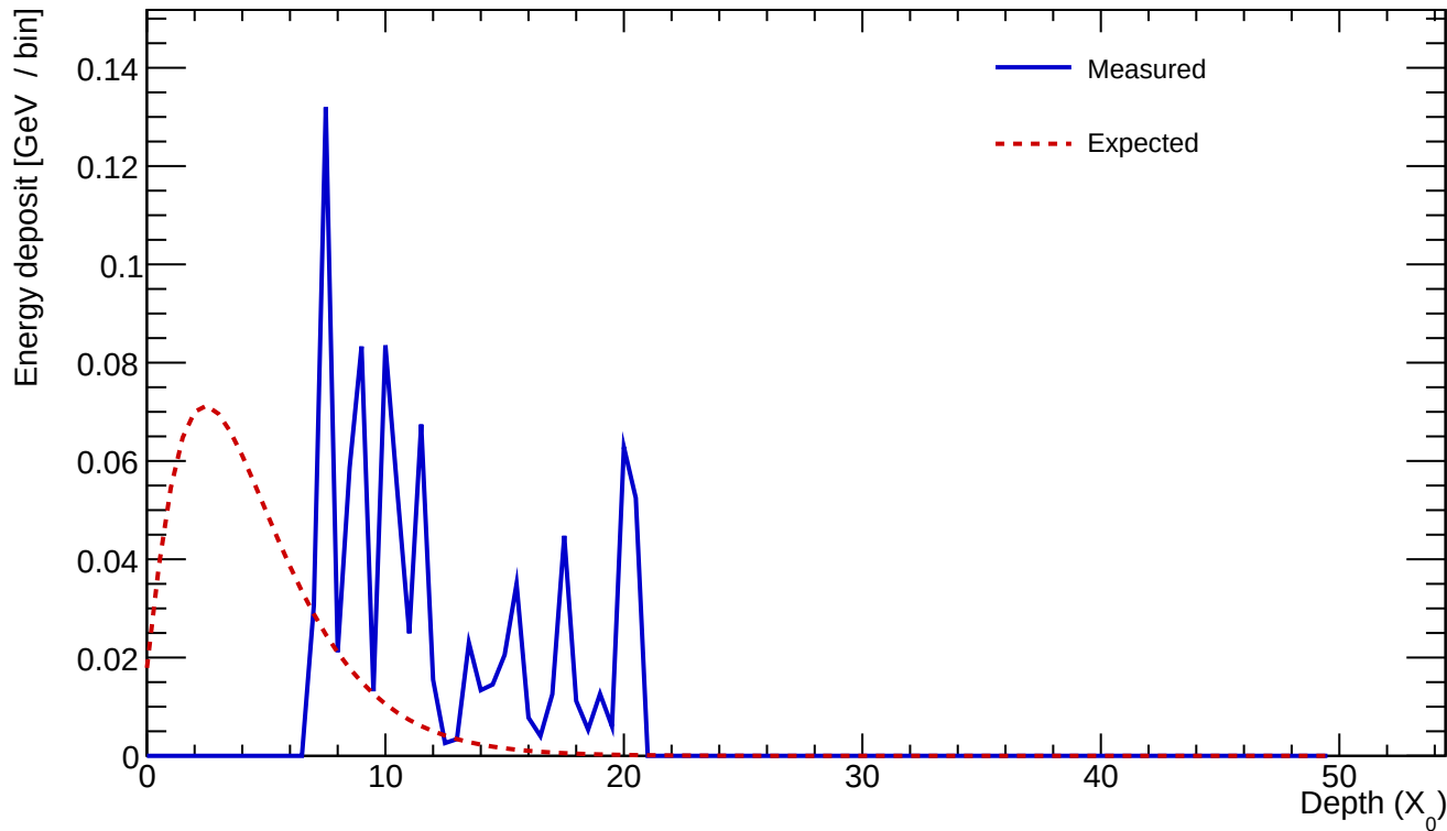
Cluster 1199 E=0.916 GeV profileStart=6.50 X_0 \chi=0.6222
