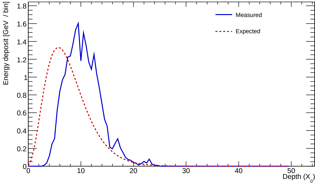
Cluster 106 E=24.189 GeV profileStart=3.50 X_0 \chi=0.1744
