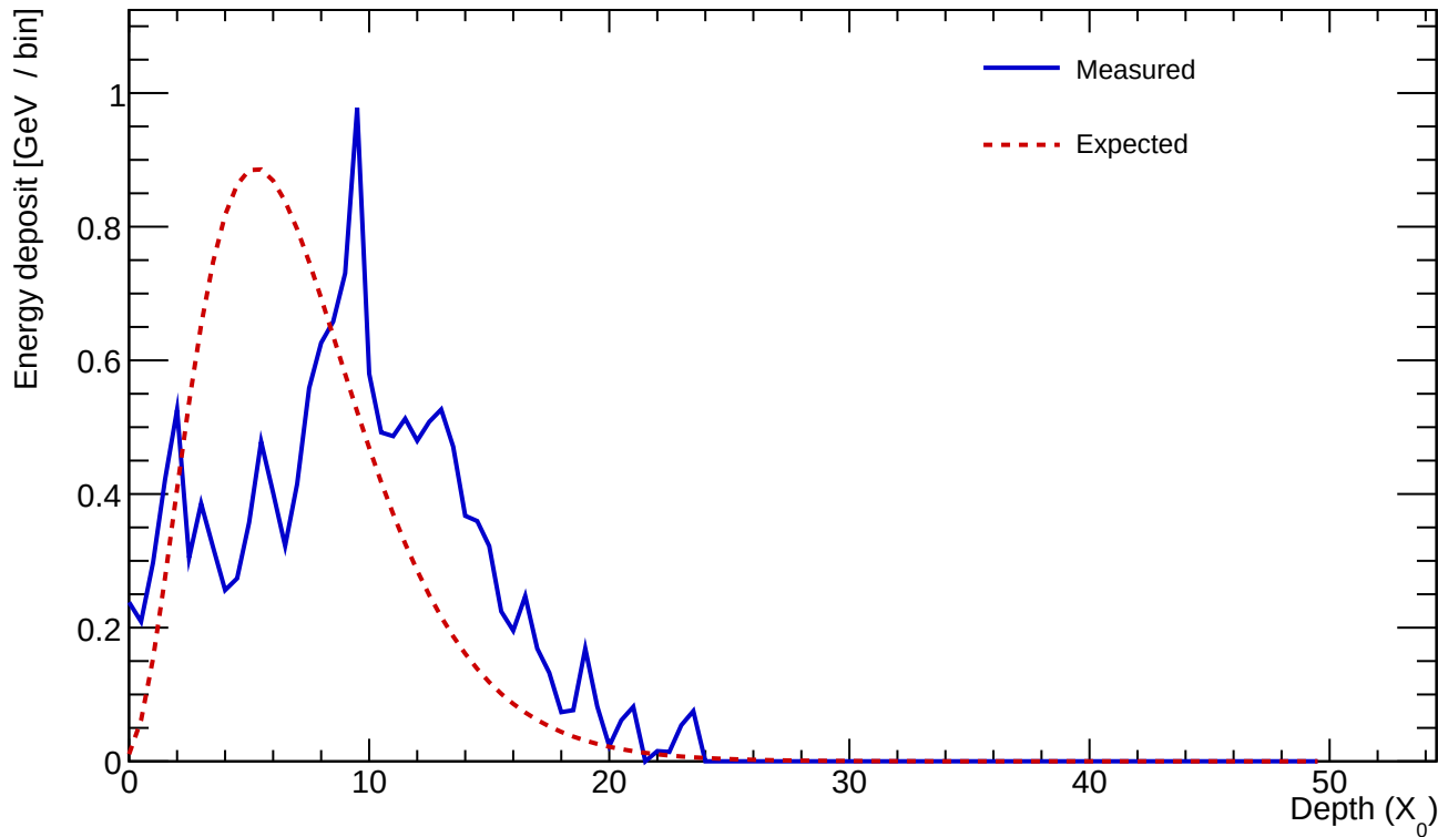
Cluster 165 E=15.558 GeV profileStart=3.00 X_0 \chi=0.4212
