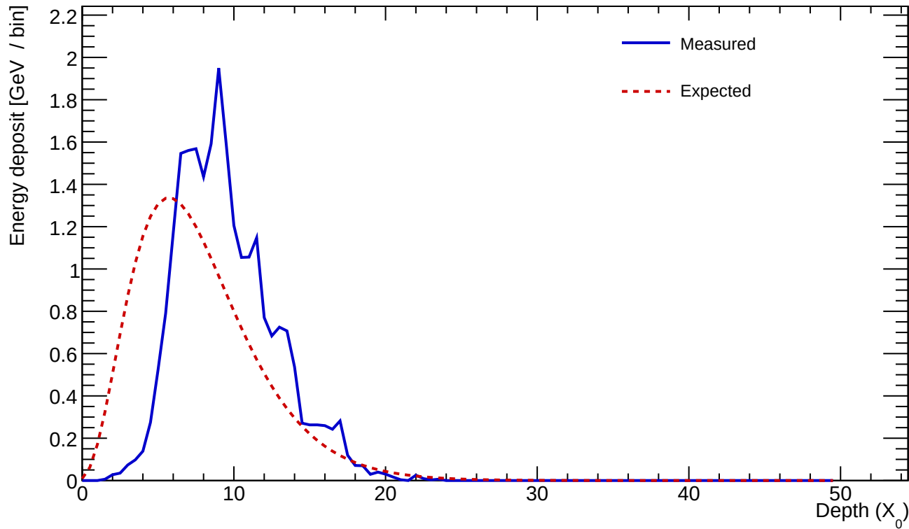
Cluster 146 E=24.265 GeV profileStart=2.50 X_0 \chi=0.2230
