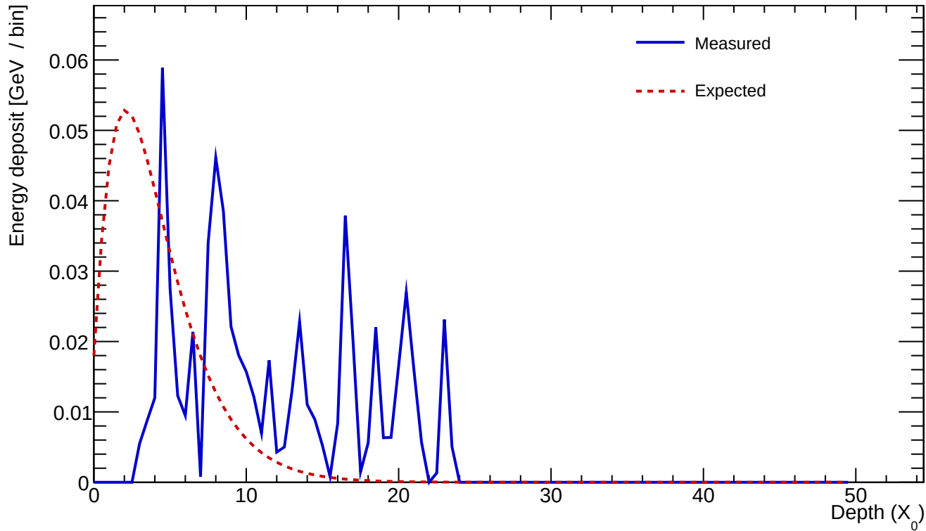
Cluster 914 E=0.642 GeV profileStart=3.50 X_0 \chi=0.8146
