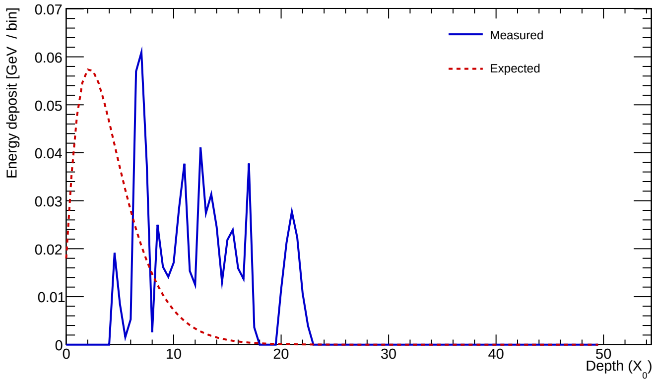
Cluster 1124 E=0.710 GeV profileStart=6.00 X_0 \chi=0.7809
