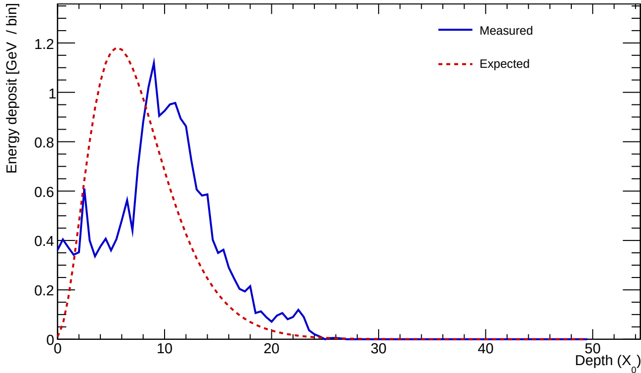
Cluster 193 E=21.223 GeV profileStart=3.00 X_0 \chi=0.3529
