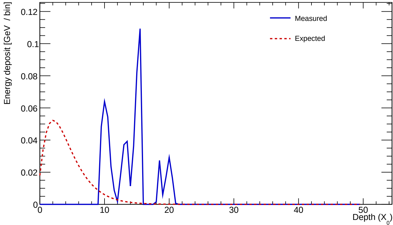
Cluster 507 E=0.633 GeV profileStart=9.00 X_0 \chi=0.8134
