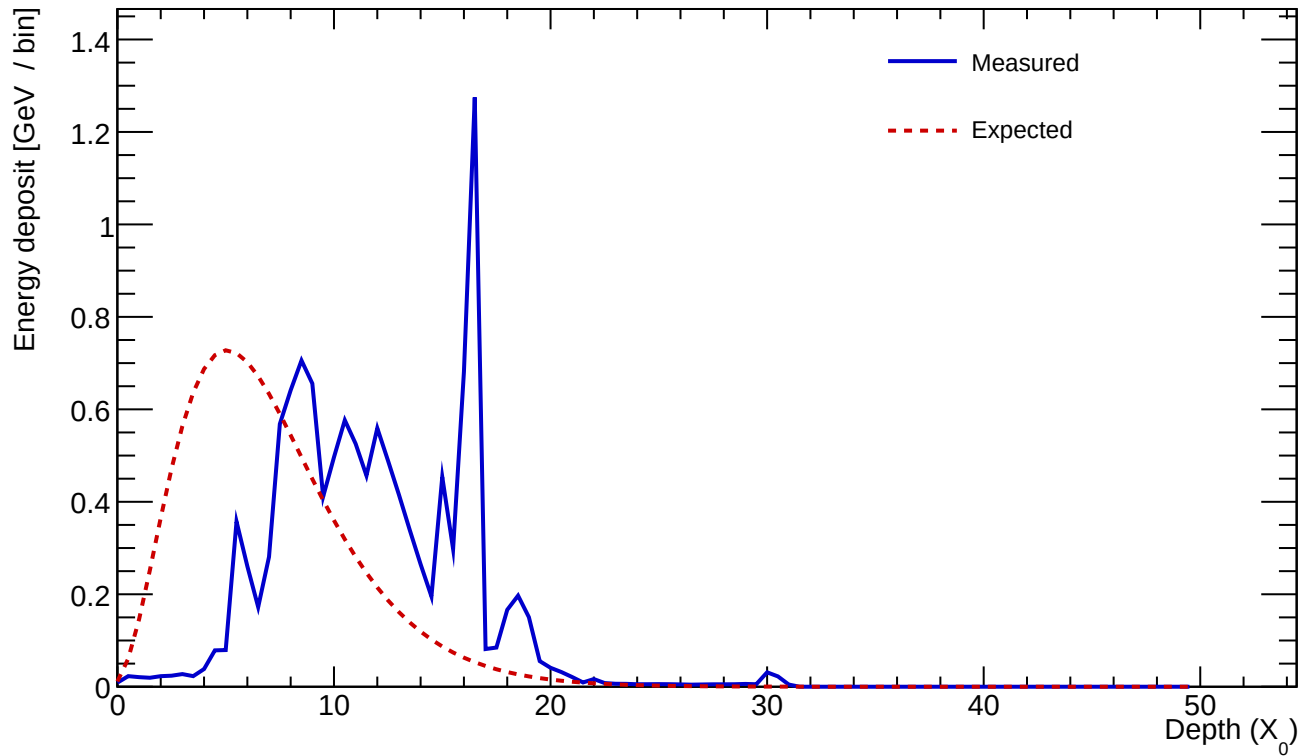
Cluster 240 E=12.530 GeV profileStart=4.00 X_0 \chi=0.3899
