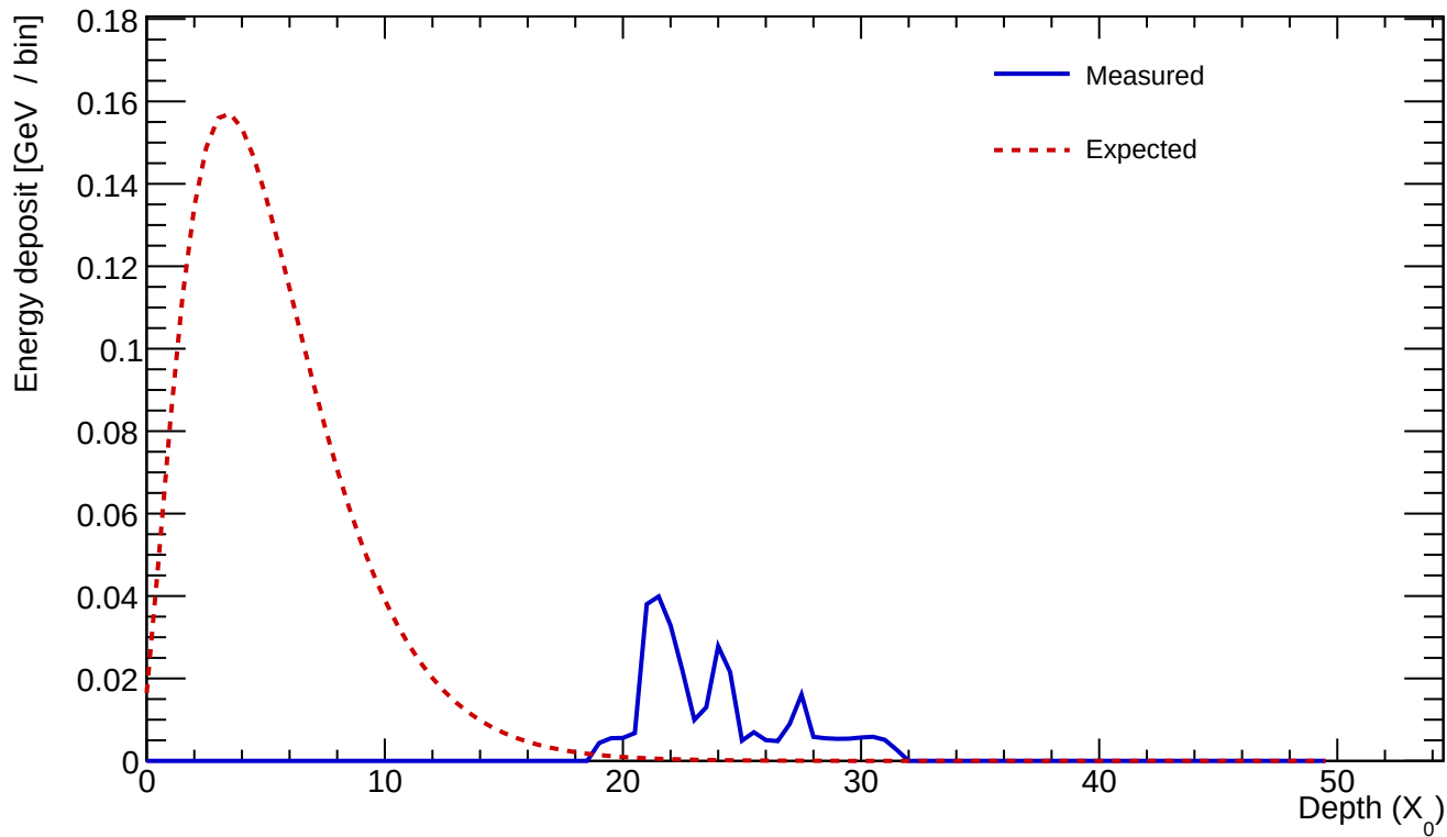
Cluster 302 E=2.284 GeV profileStart=31.00 X_0 \chi=1.0114
