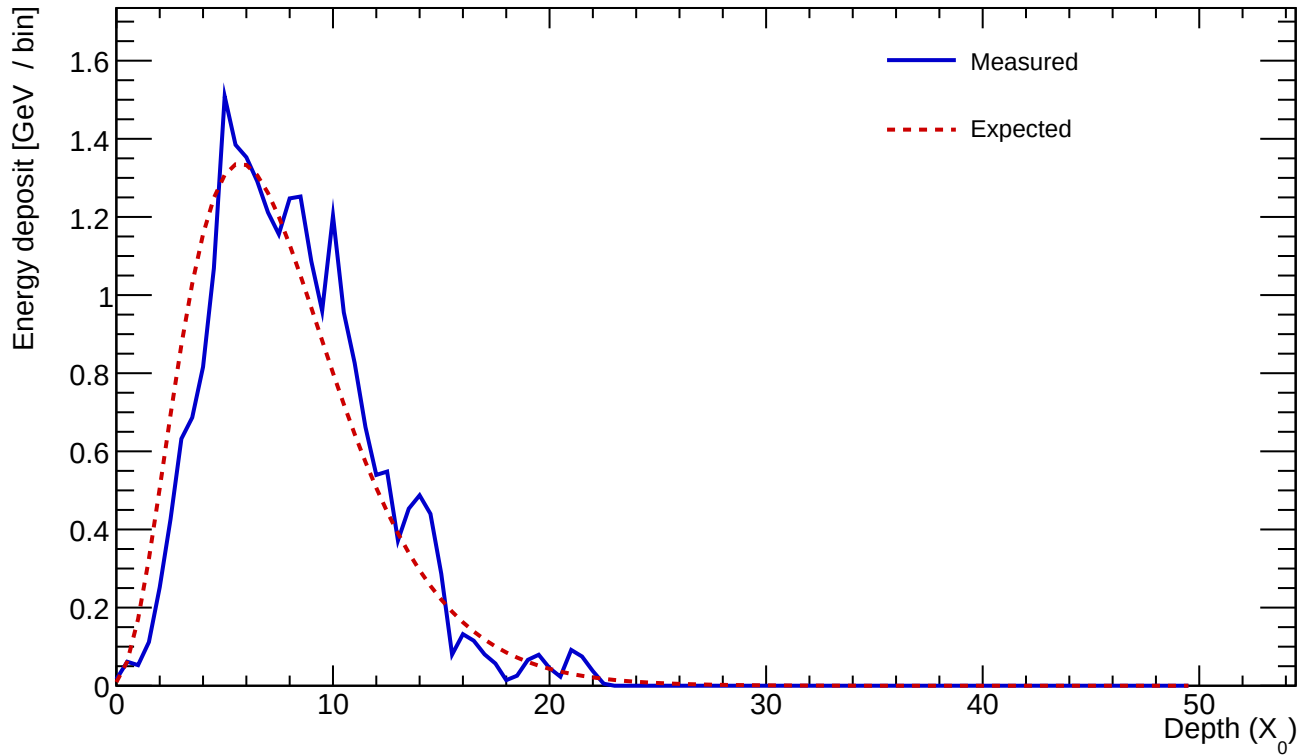
Cluster 432 E=24.276 GeV profileStart=1.00 X_0 \chi=0.1379
