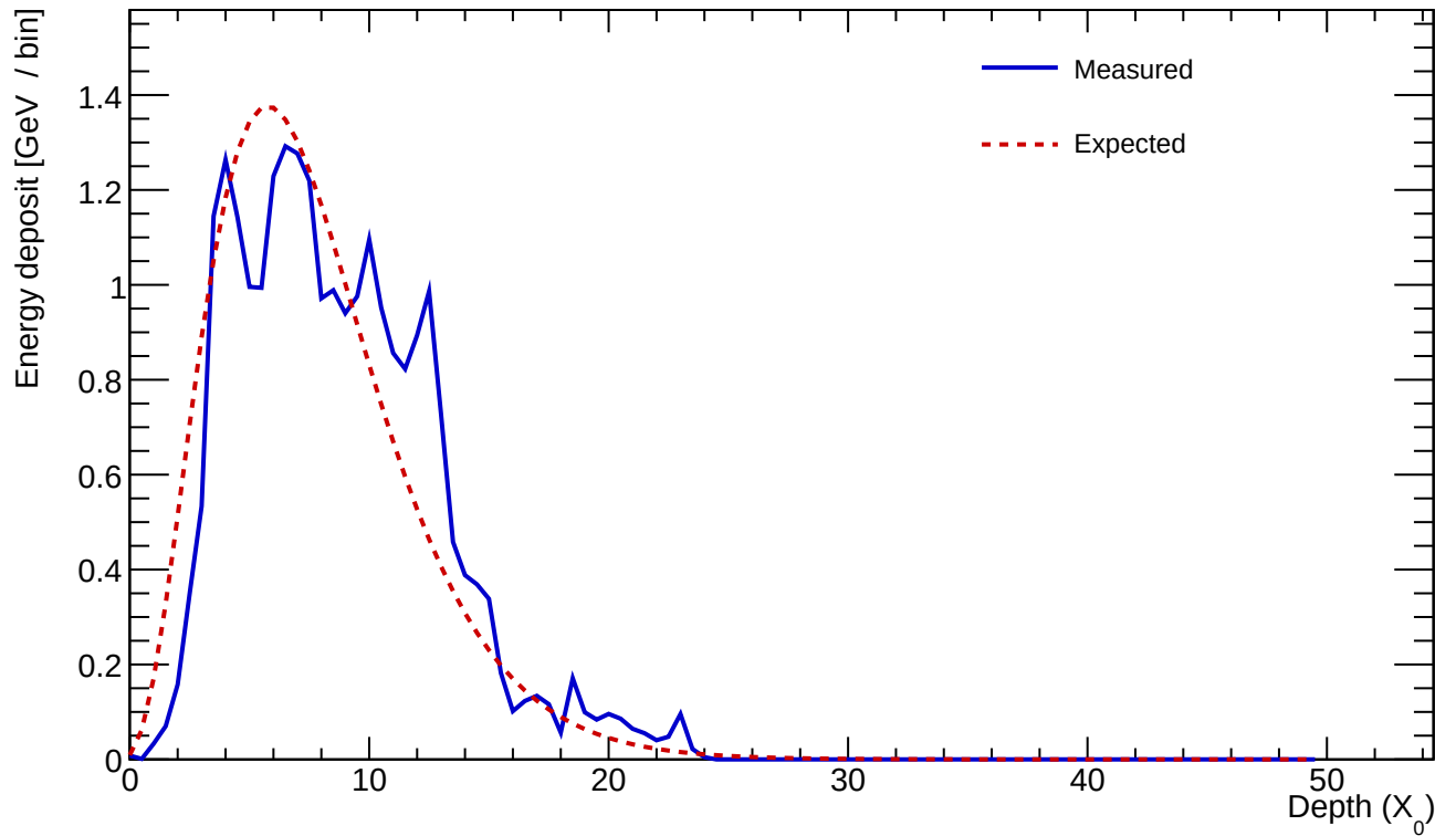
Cluster 689 E=25.053 GeV profileStart=1.00 X_0 \chi=0.1851
