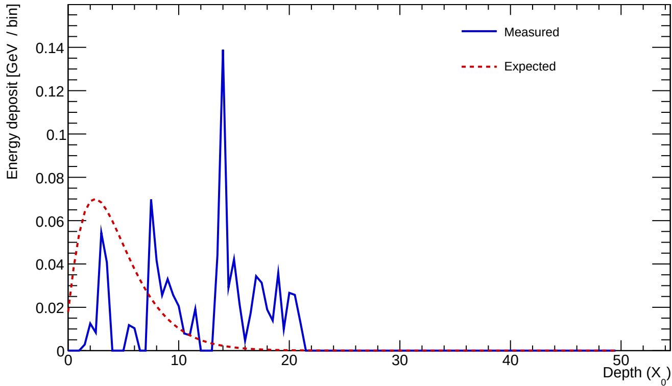
Cluster 630 E=0.899 GeV profileStart=13.00 X_0 \chi=0.9530
