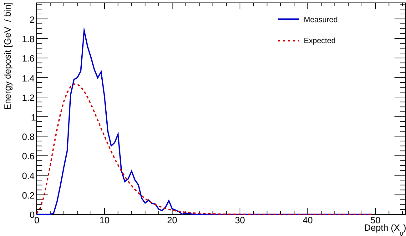
Cluster 535 E=24.242 GeV profileStart=1.50 X_0 \chi=0.2445
