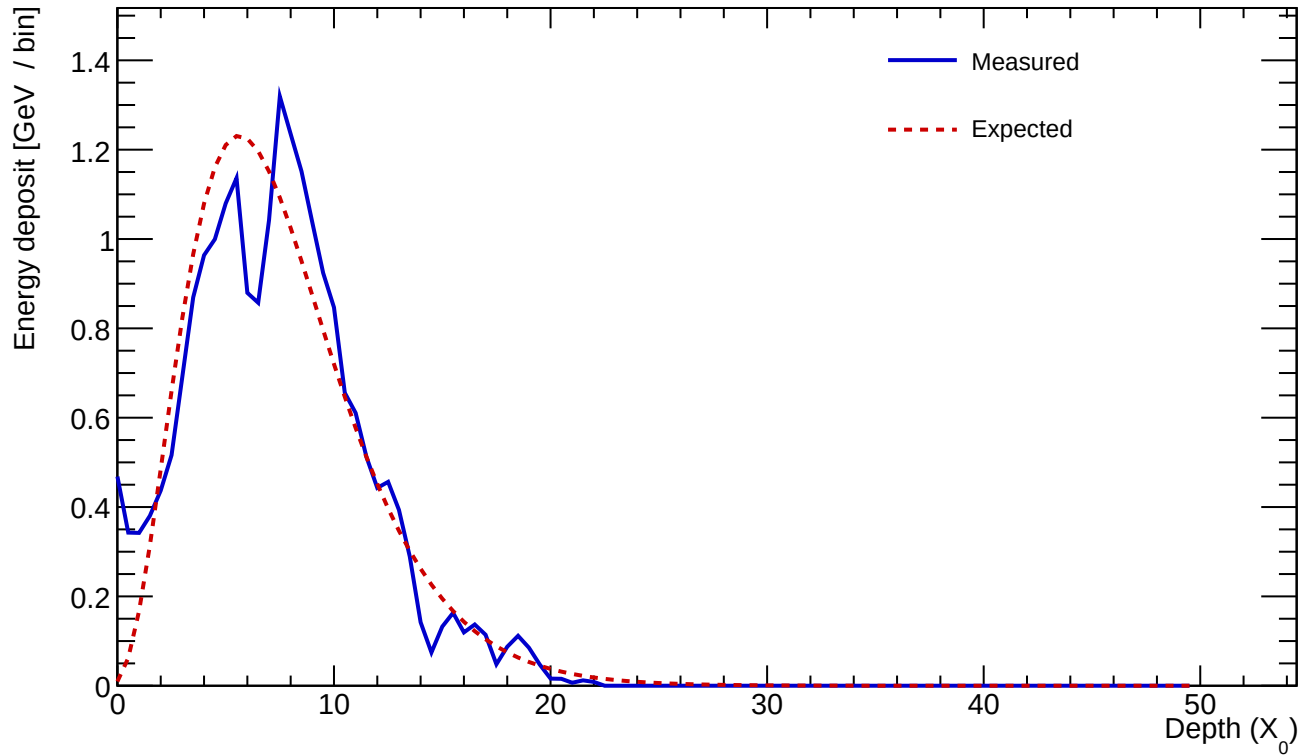
Cluster 519 E=22.202 GeV profileStart=0.50 X_0 \chi=0.1941
