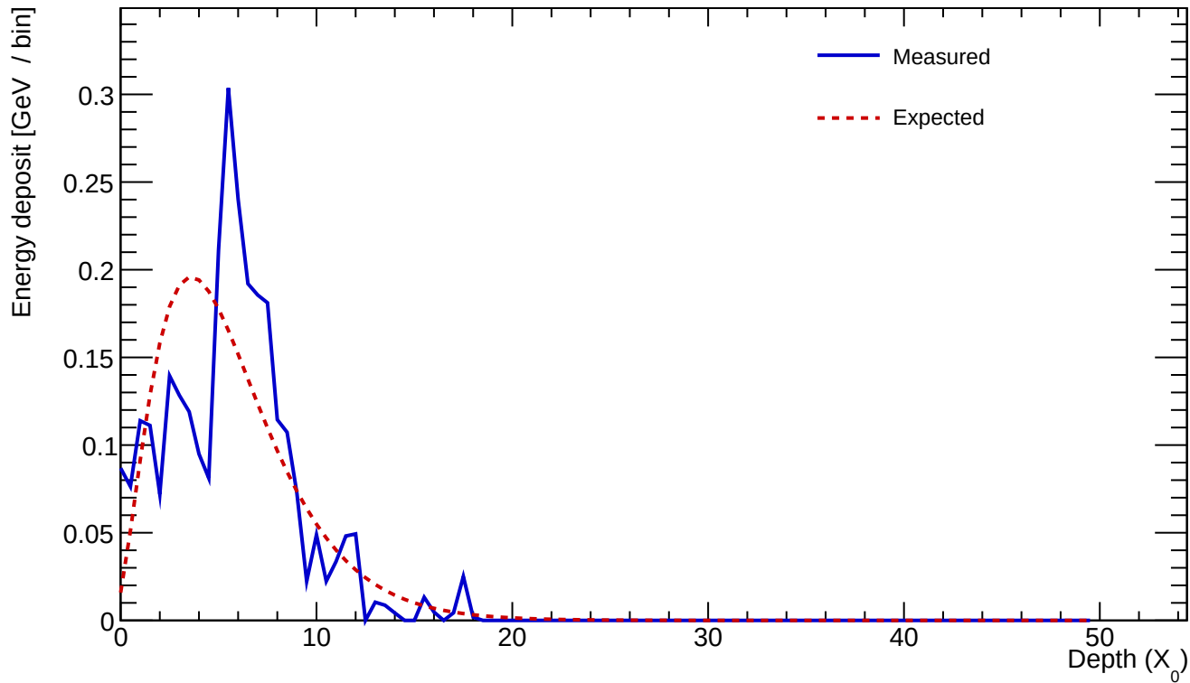
Cluster 825 E=2.929 GeV profileStart=1.00 X_0 \chi=0.4442
