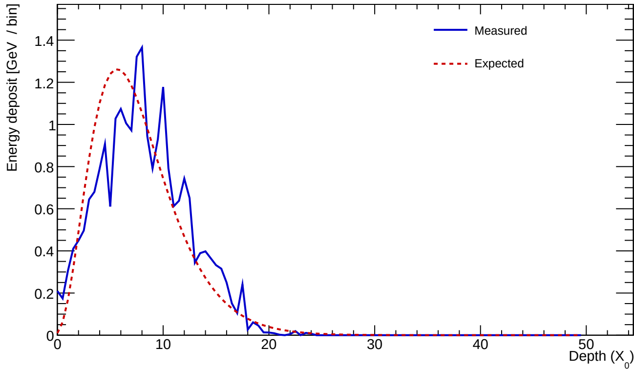
Cluster 802 E=22.828 GeV profileStart=1.00 X_0 \chi=0.2473
