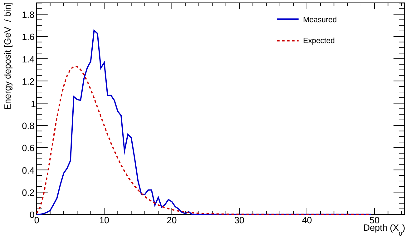
Cluster 887 E=24.195 GeV profileStart=2.50 X_0 \chi=0.1512
