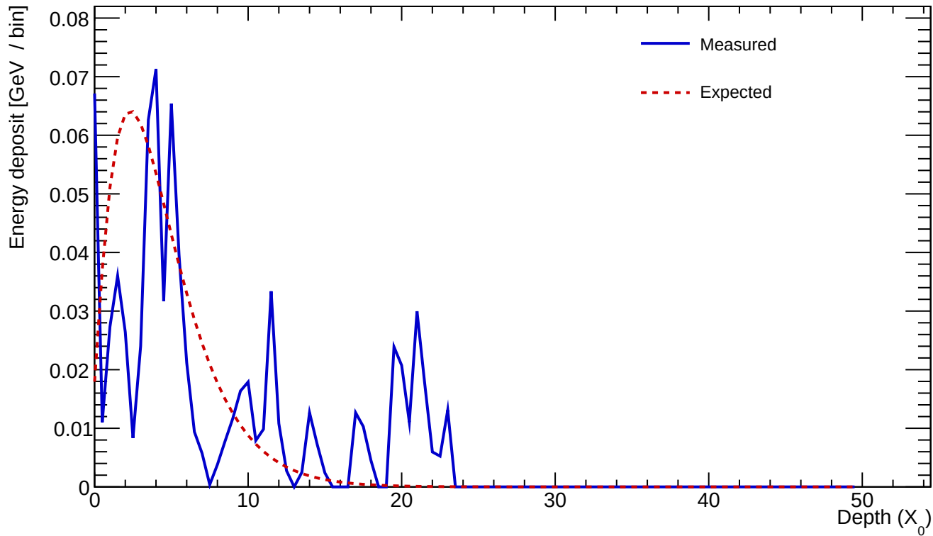
Cluster 295 E=0.810 GeV profileStart=0.50 X_0 \chi=0.7578
