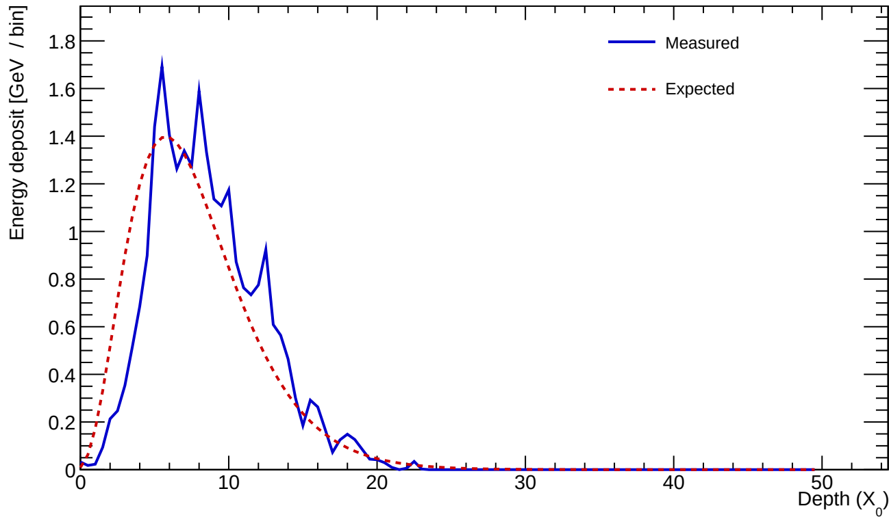
Cluster 480 E=25.475 GeV profileStart=1.50 X_0 \chi=0.1472
