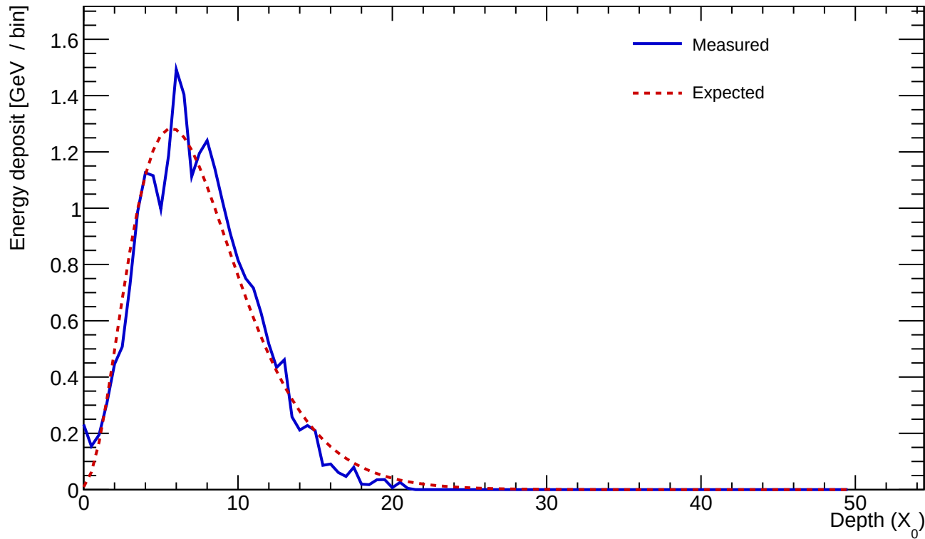
Cluster 37 E=23.236 GeV profileStart=0.50 X_0 \chi=0.1385
