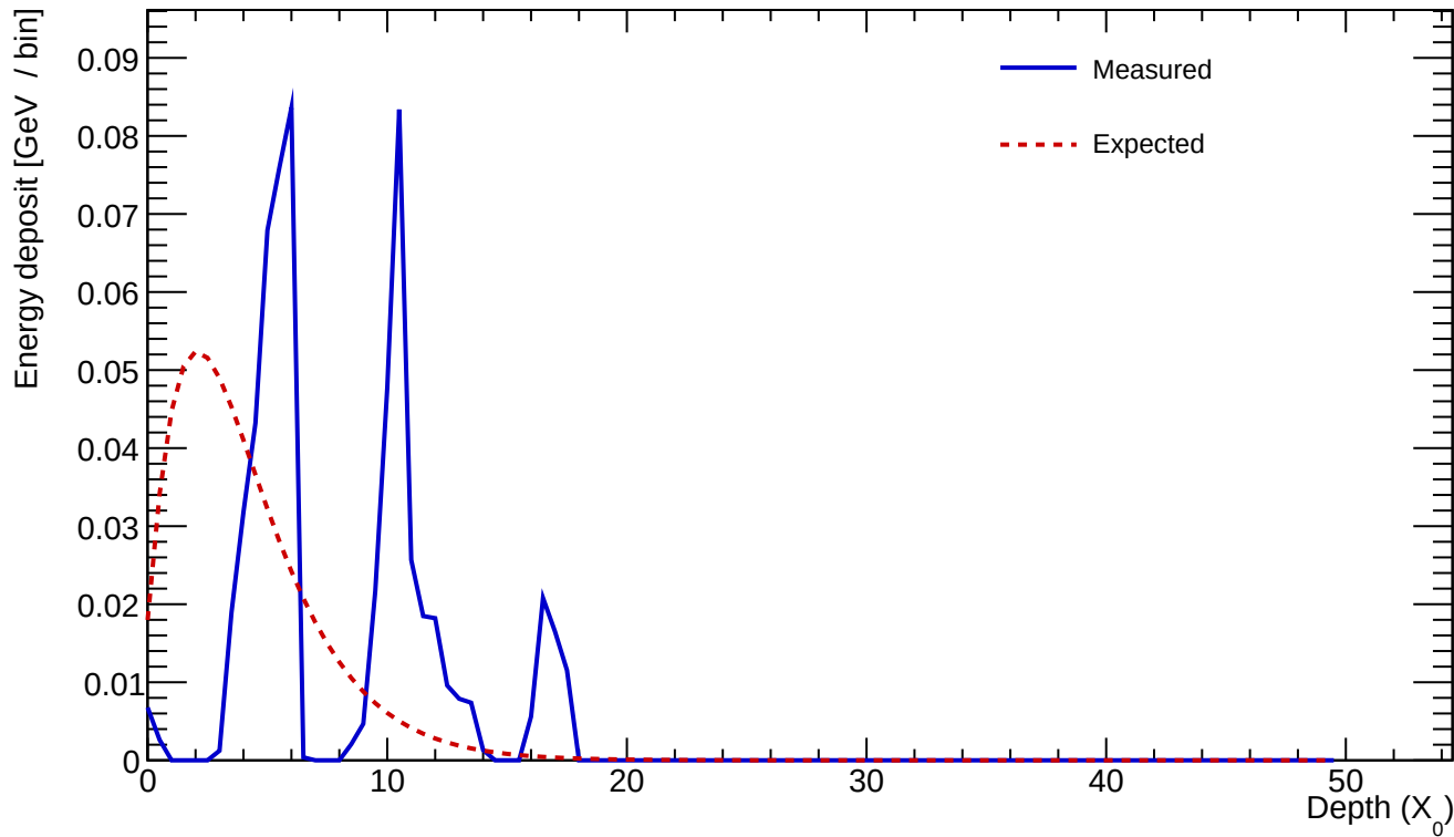
Cluster 127 E=0.635 GeV profileStart=3.50 X_0 \chi=0.7669
