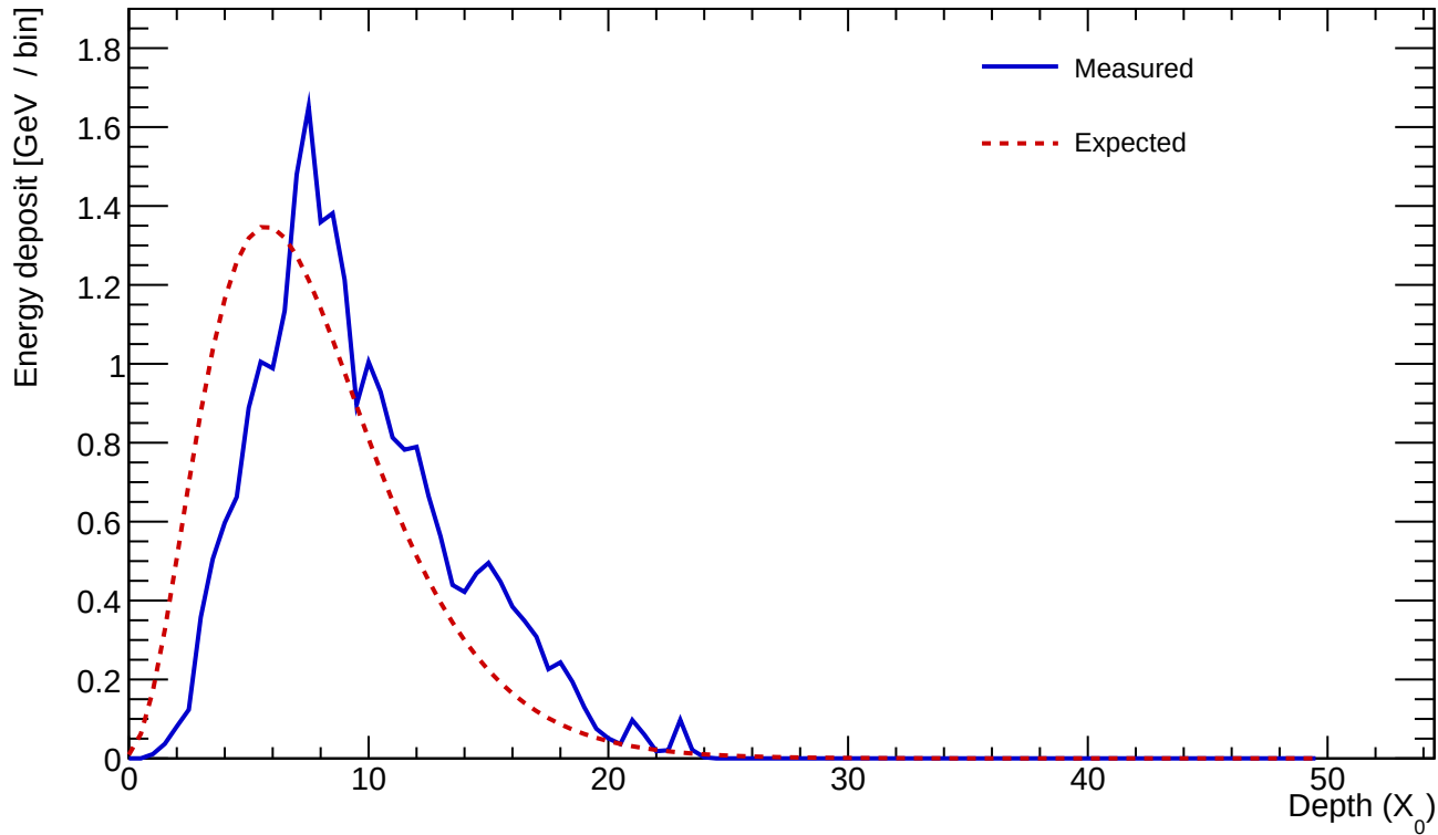
Cluster 64 E=24.508 GeV profileStart=1.50 X_0 \chi=0.1502
