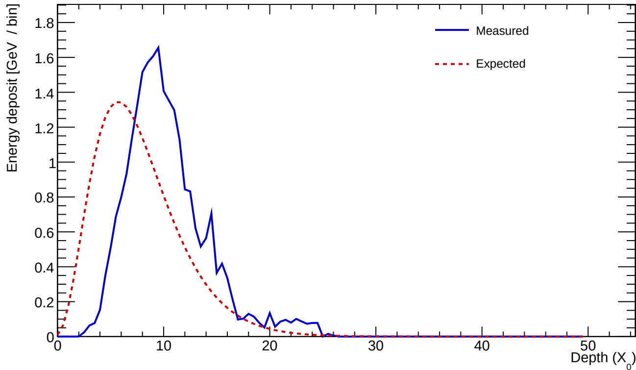
Cluster 581 E=24.458 GeV profileStart=3.00 X_0 \chi=0.1709
