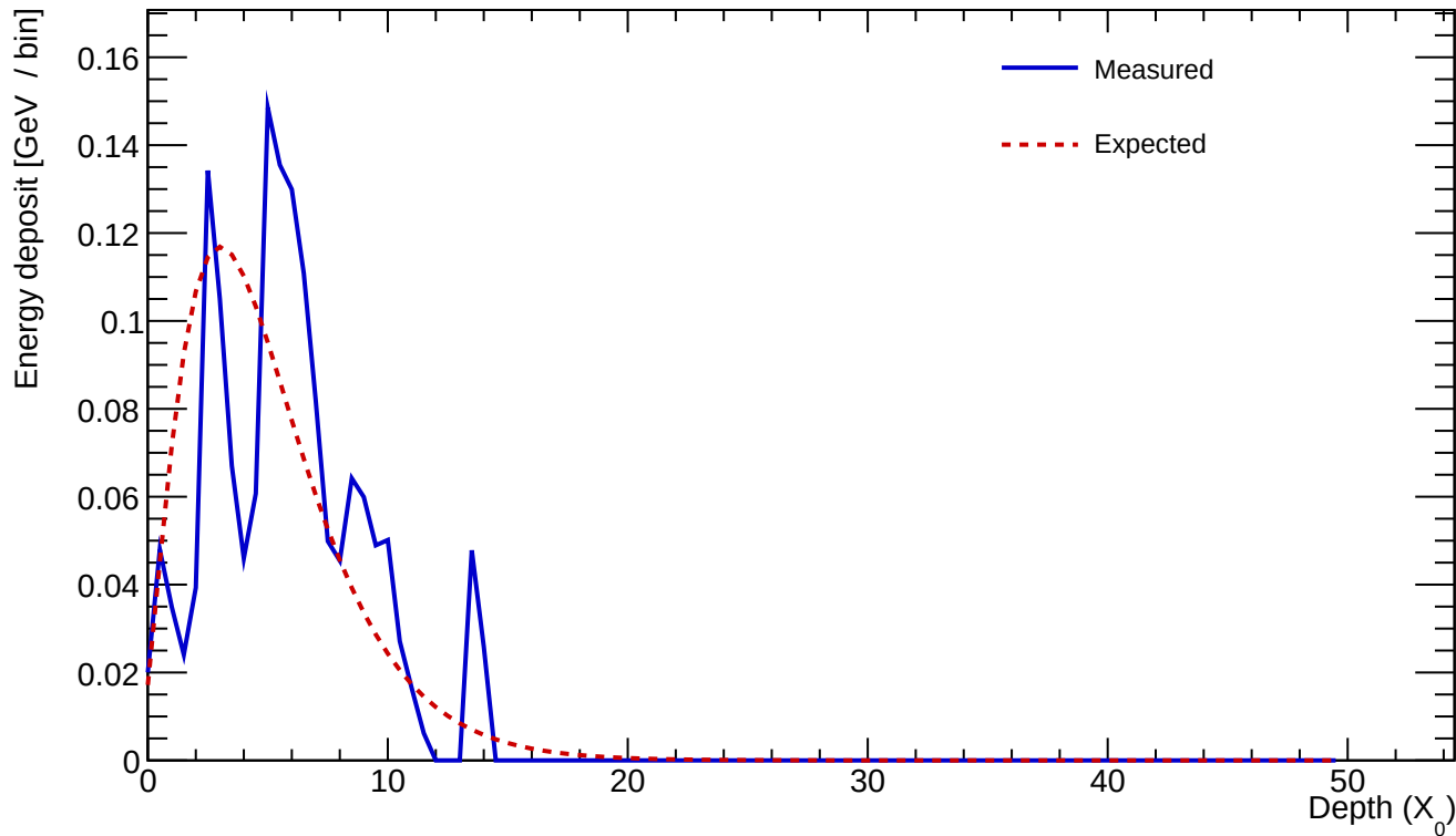
Cluster 985 E=1.628 GeV profileStart=1.50 X_0 \chi=0.4064
