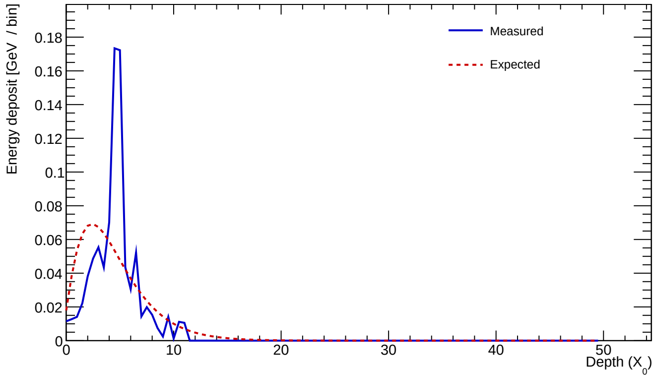
Cluster 660 E=0.885 GeV profileStart=1.50 X_0 \chi=0.5265
