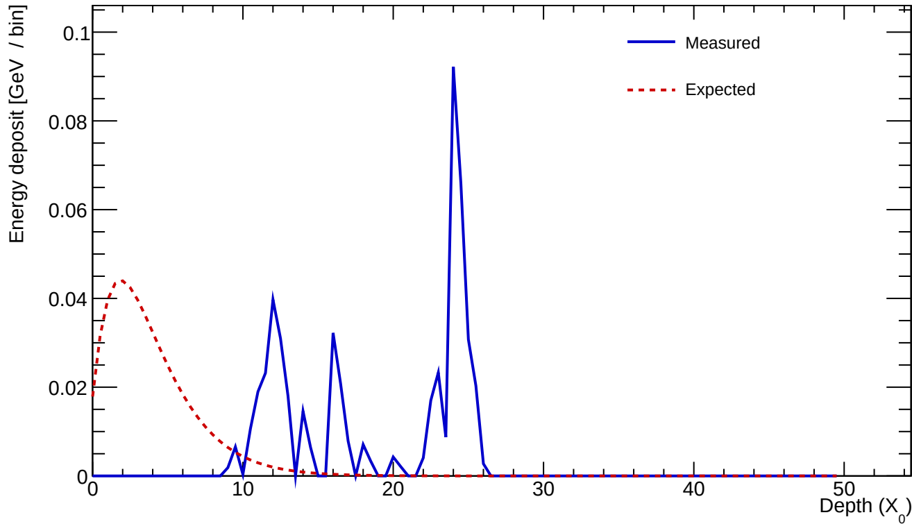
Cluster 11 E=0.514 GeV profileStart=10.50 X_0 \chi=1.0632
