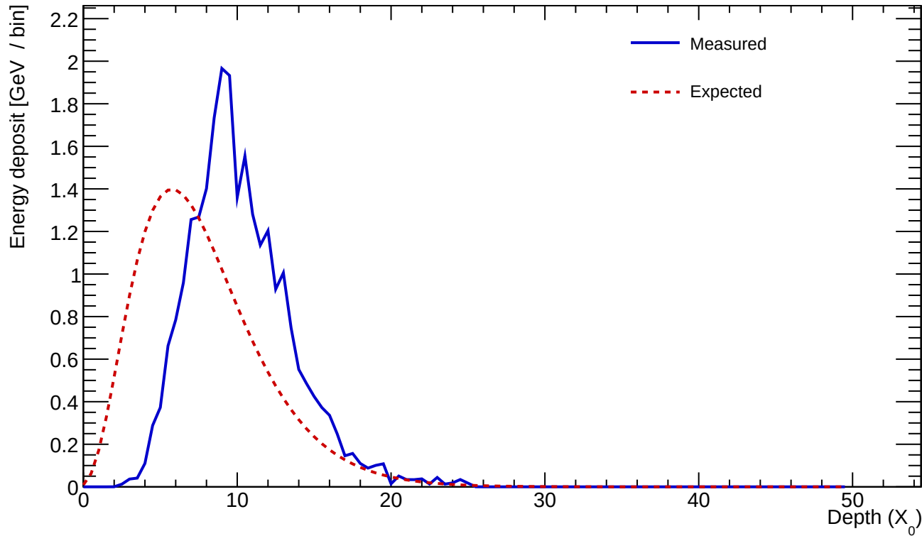
Cluster 168 E=25.481 GeV profileStart=3.00 X_0 \chi=0.1840
