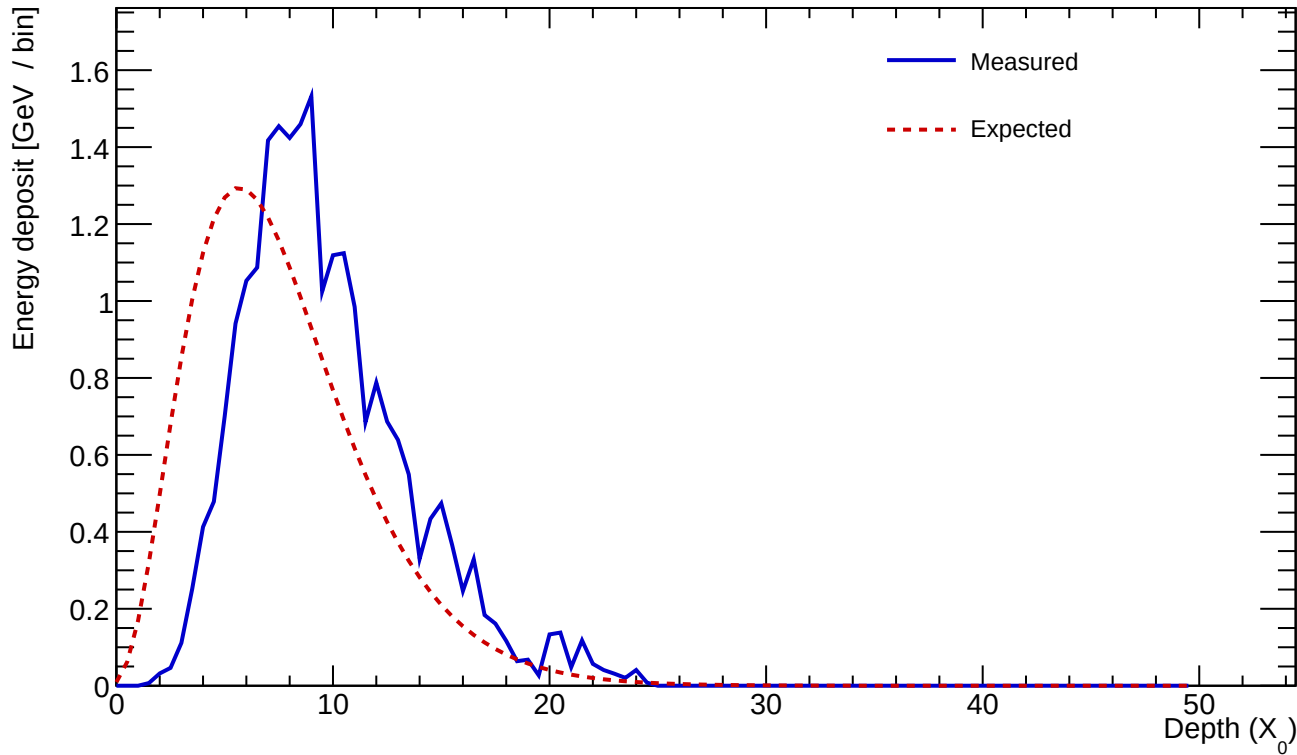
Cluster 455 E=23.444 GeV profileStart=2.00 X_0 \chi=0.1413
