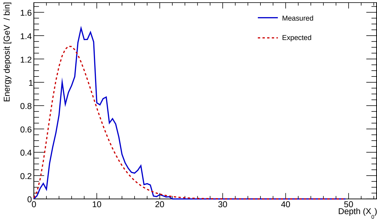
Cluster 725 E=23.760 GeV profileStart=1.50 X_0 \chi=0.1654
