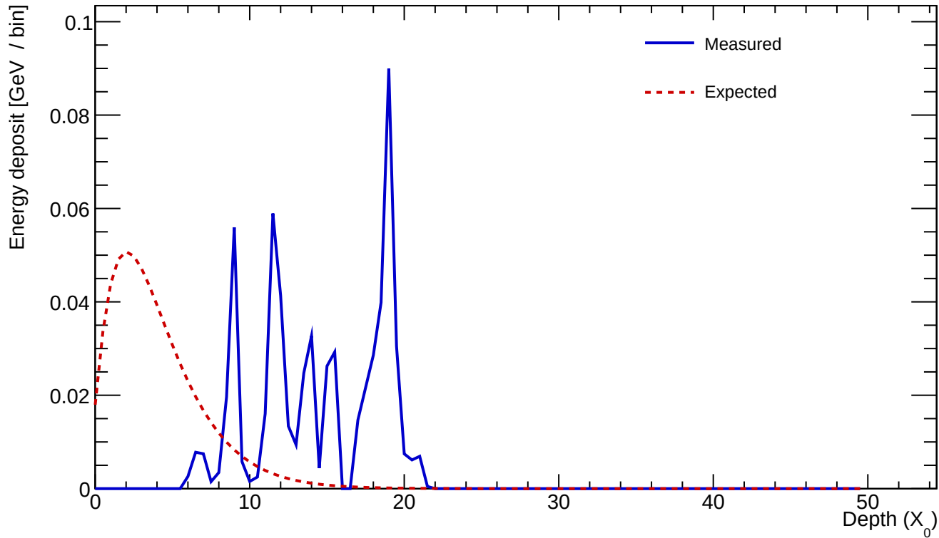
Cluster 361 E=0.611 GeV profileStart=11.00 X_0 \chi=0.8496
