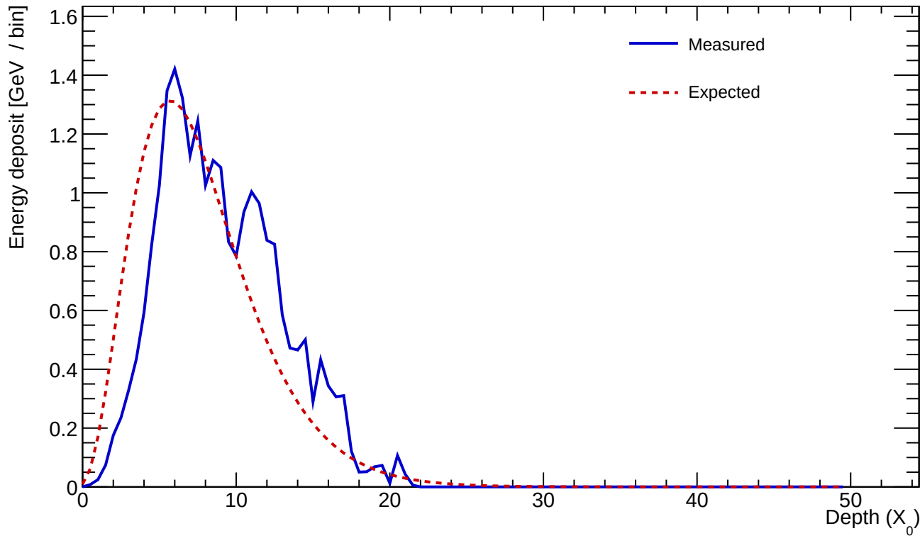
Cluster 102 E=23.833 GeV profileStart=1.50 X_0 \chi=0.1622
