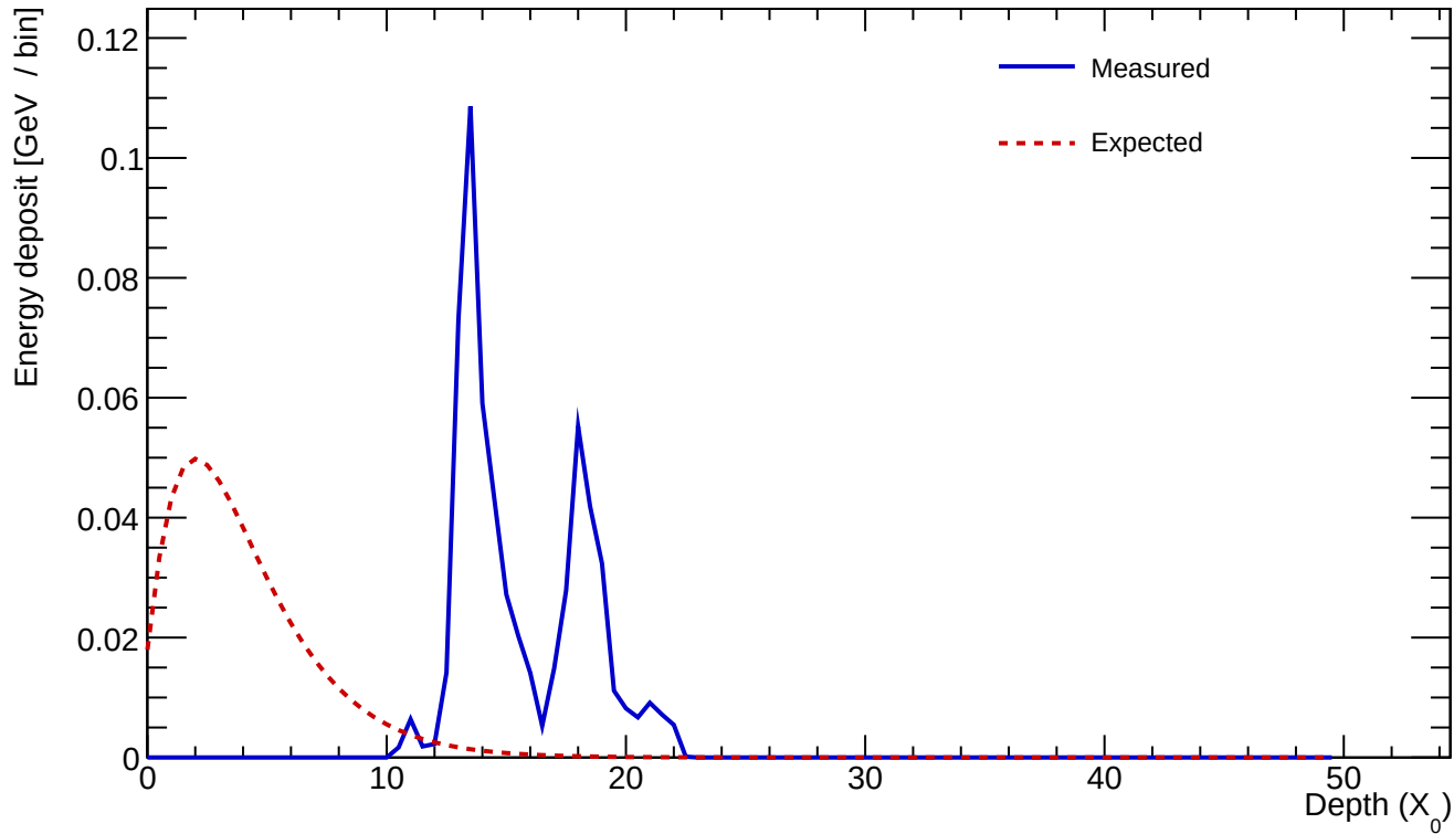
Cluster 777 E=0.597 GeV profileStart=12.00 X_0 \chi=0.5745
