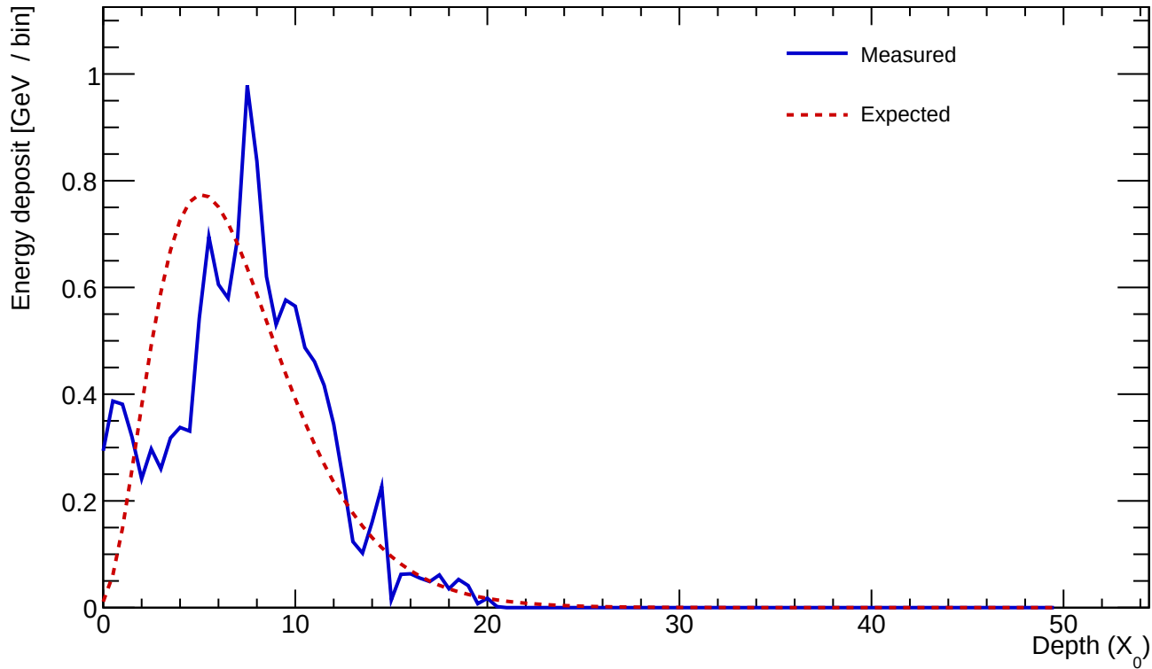
Cluster 399 E=13.411 GeV profileStart=1.50 X_0 \chi=0.3136
