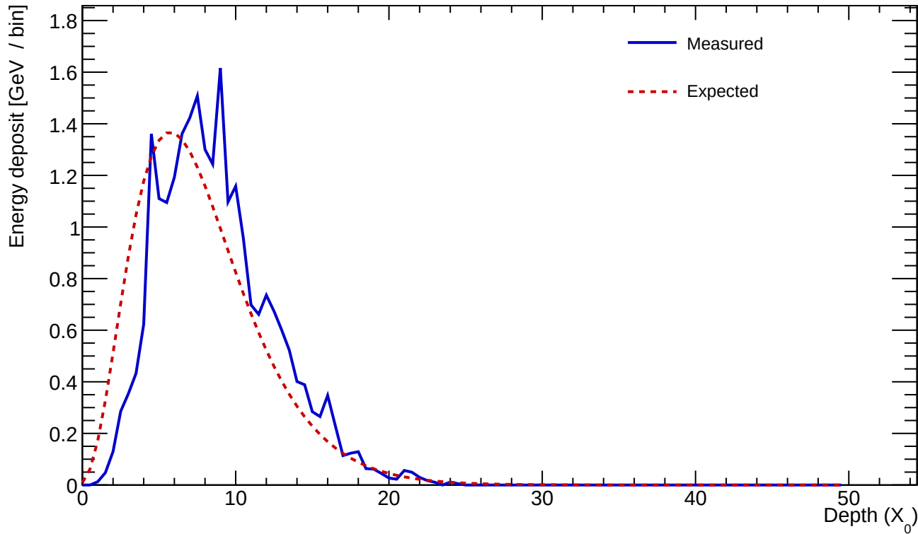
Cluster 849 E=24.879 GeV profileStart=1.50 X_0 \chi=0.1251
