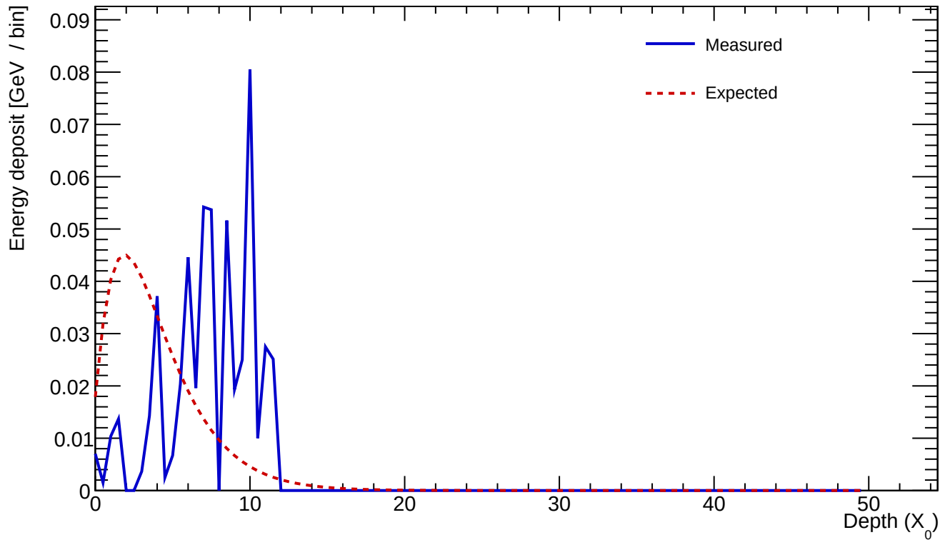
Cluster 589 E=0.528 GeV profileStart=5.50 X_0 \chi=0.5756
