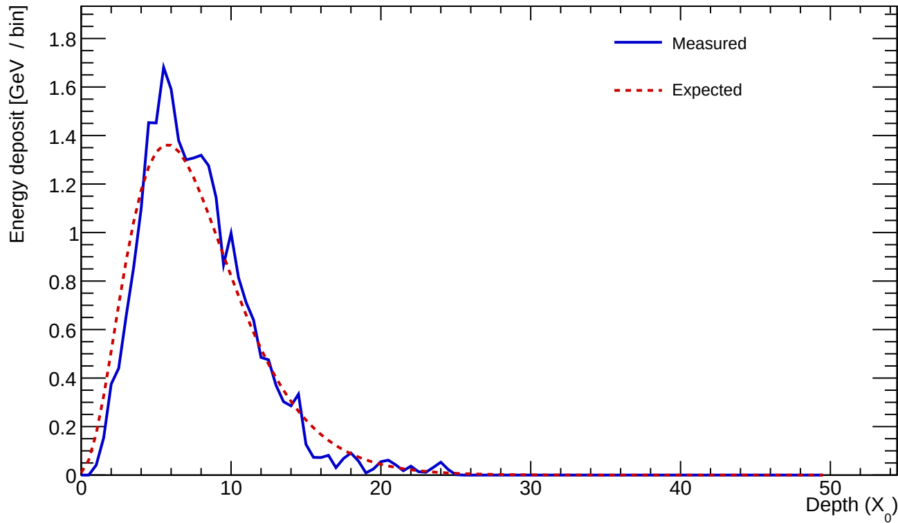
Cluster 35 E=24.792 GeV profileStart=0.50 X_0 \chi=0.1343
