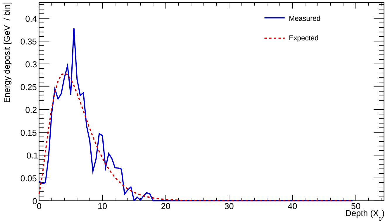
Cluster 204 E=4.366 GeV profileStart=0.50 X_0 \chi=0.2104
