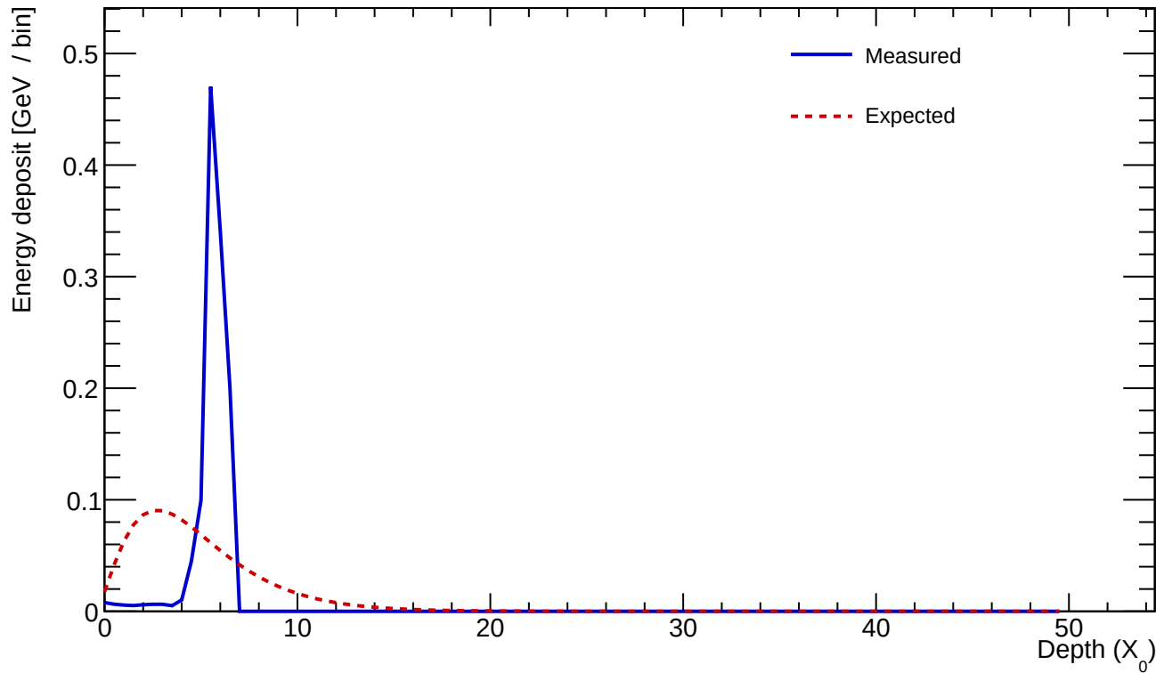
Cluster 1143 E=1.215 GeV profileStart=4.00 X_0 \chi=0.6115
