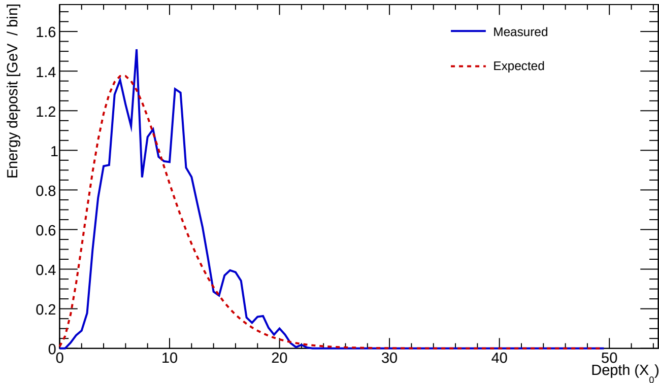
Cluster 789 E=25.086 GeV profileStart=1.00 X_0 \chi=0.1921
