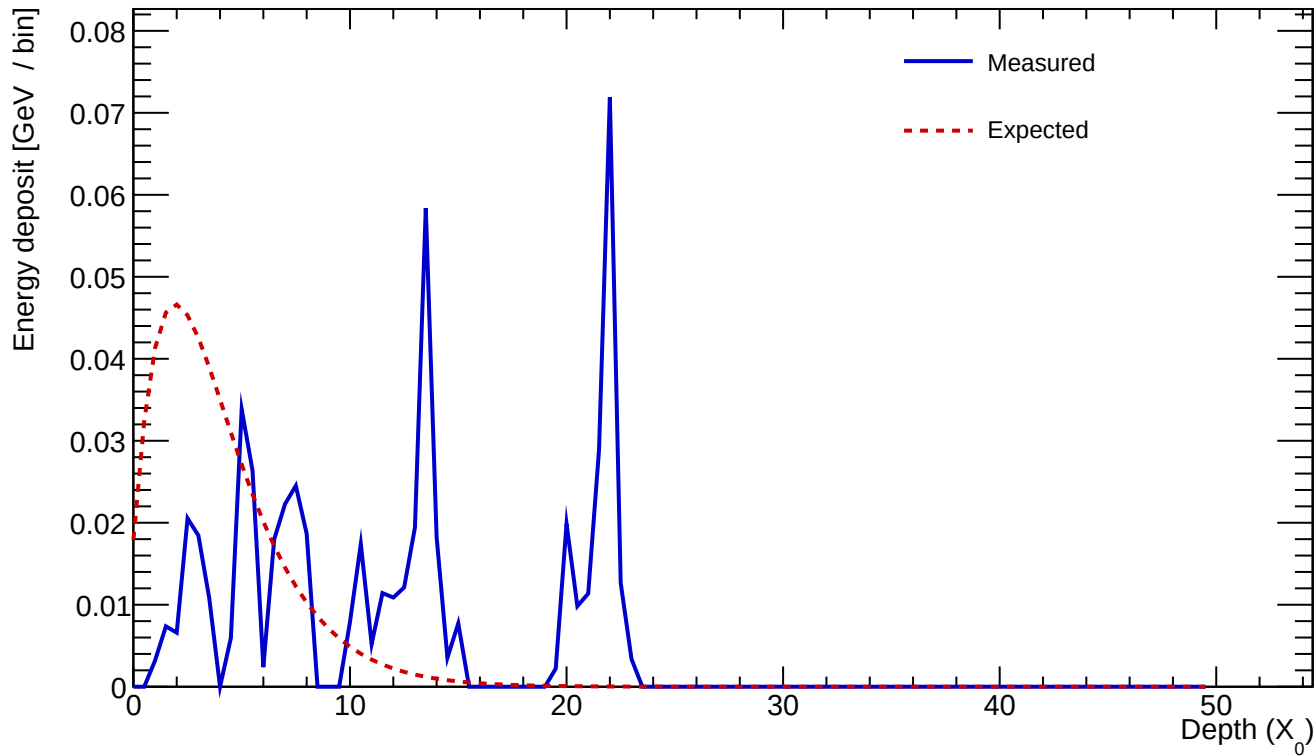
Cluster 232 E=0.551 GeV profileStart=2.00 X_0 \chi=1.0617
