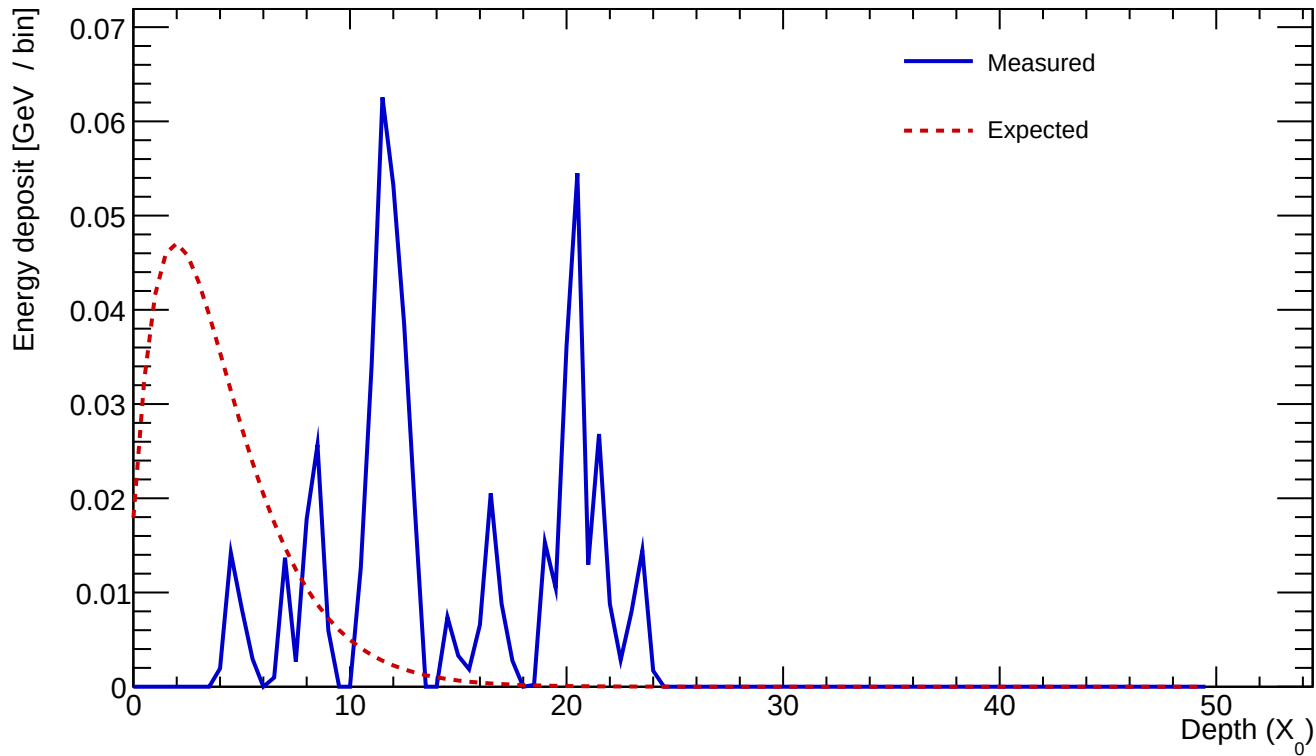
Cluster 323 E=0.557 GeV profileStart=10.50 X_0 \chi=0.9638
