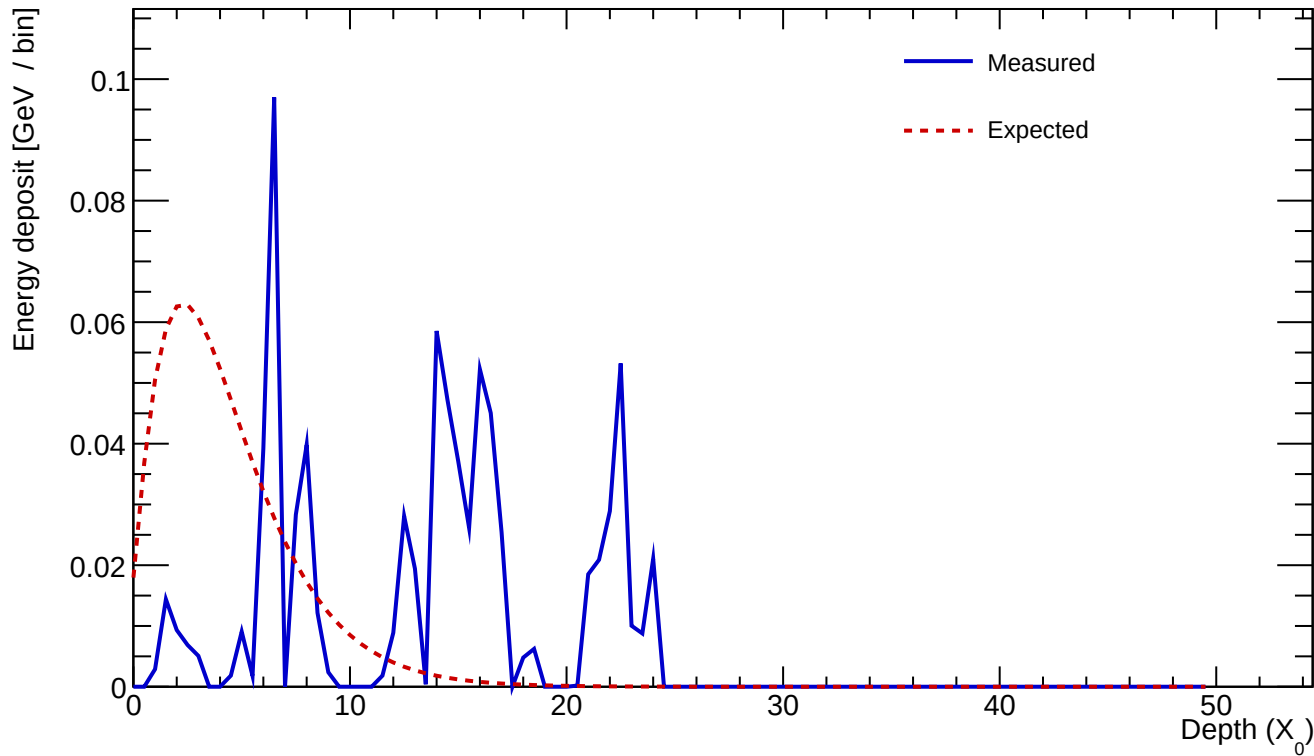
Cluster 741 E=0.793 GeV profileStart=12.00 X_0 \chi=0.9150
