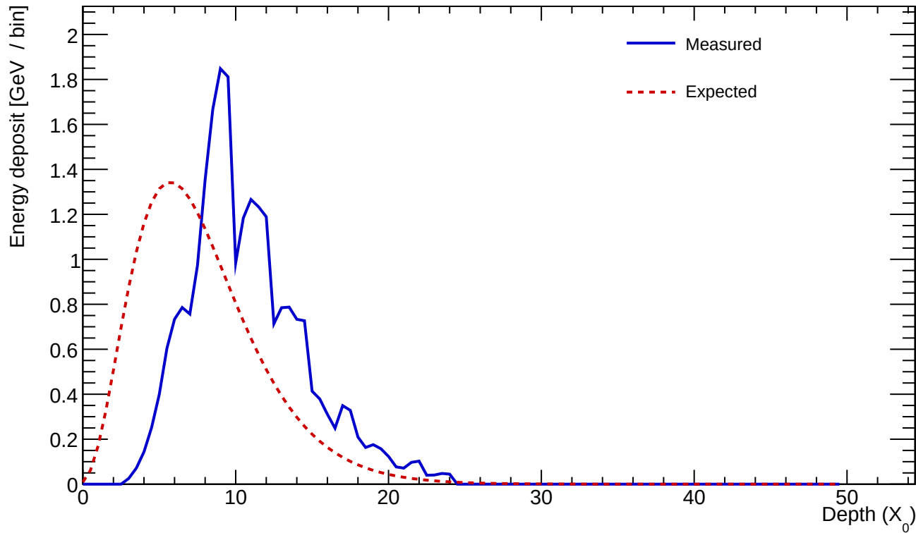
Cluster 704 E=24.405 GeV profileStart=3.50 X_0 \chi=0.1854
