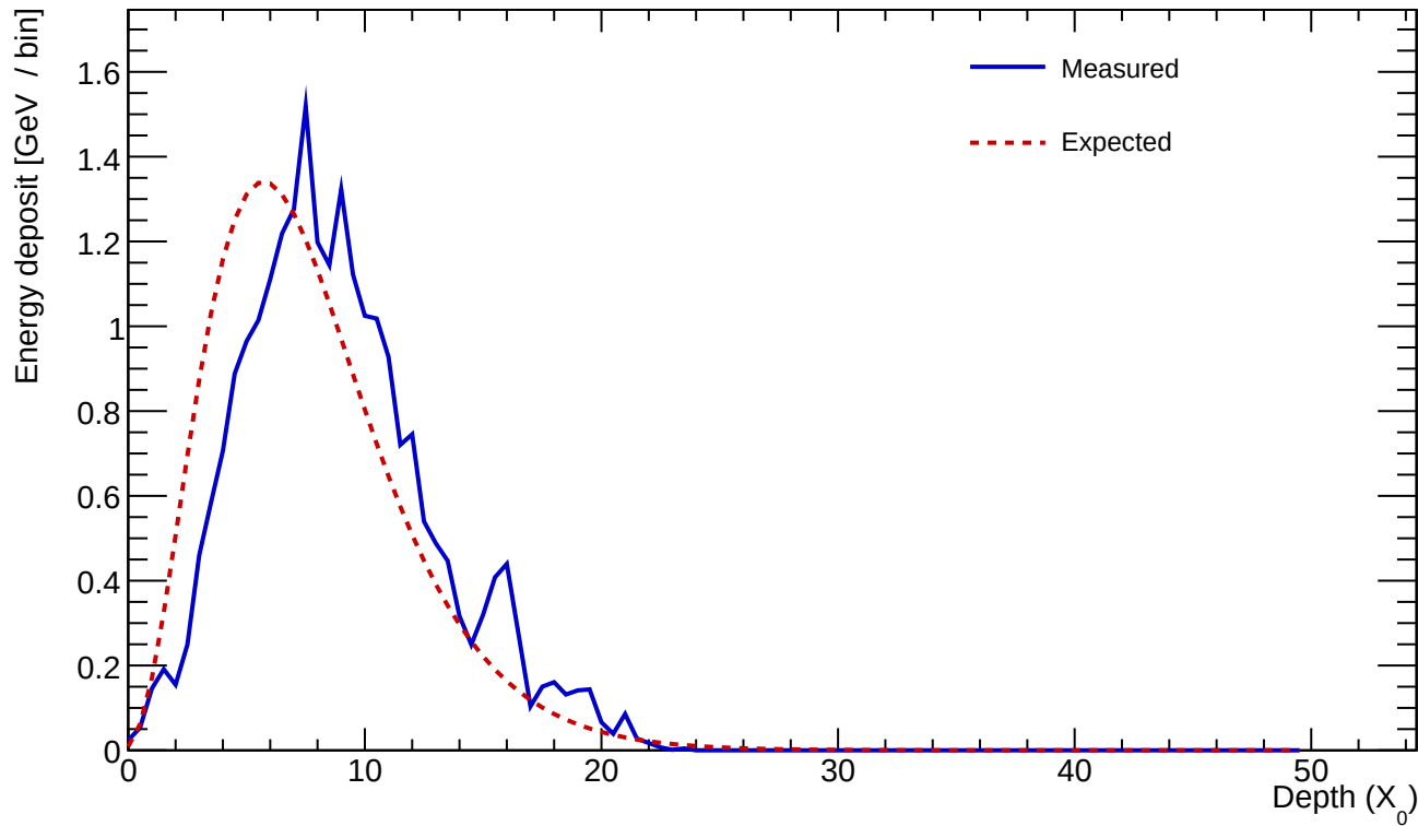
Cluster 917 E=24.345 GeV profileStart=1.50 X_0 \chi=0.1380
