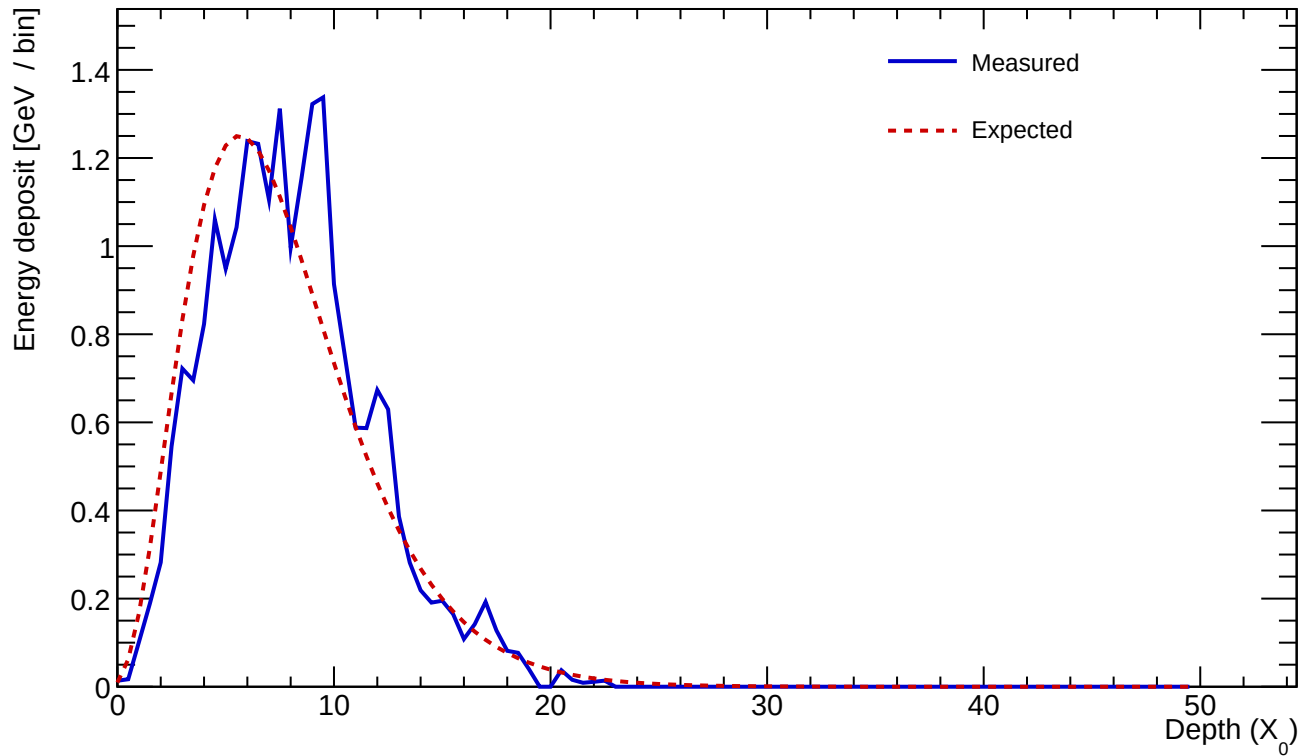
Cluster 510 E=22.578 GeV profileStart=0.50 X_0 \chi=0.1531
