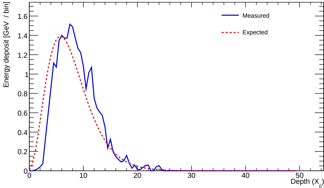
Cluster 739 E=25.339 GeV profileStart=1.50 X_0 \chi=0.1203
