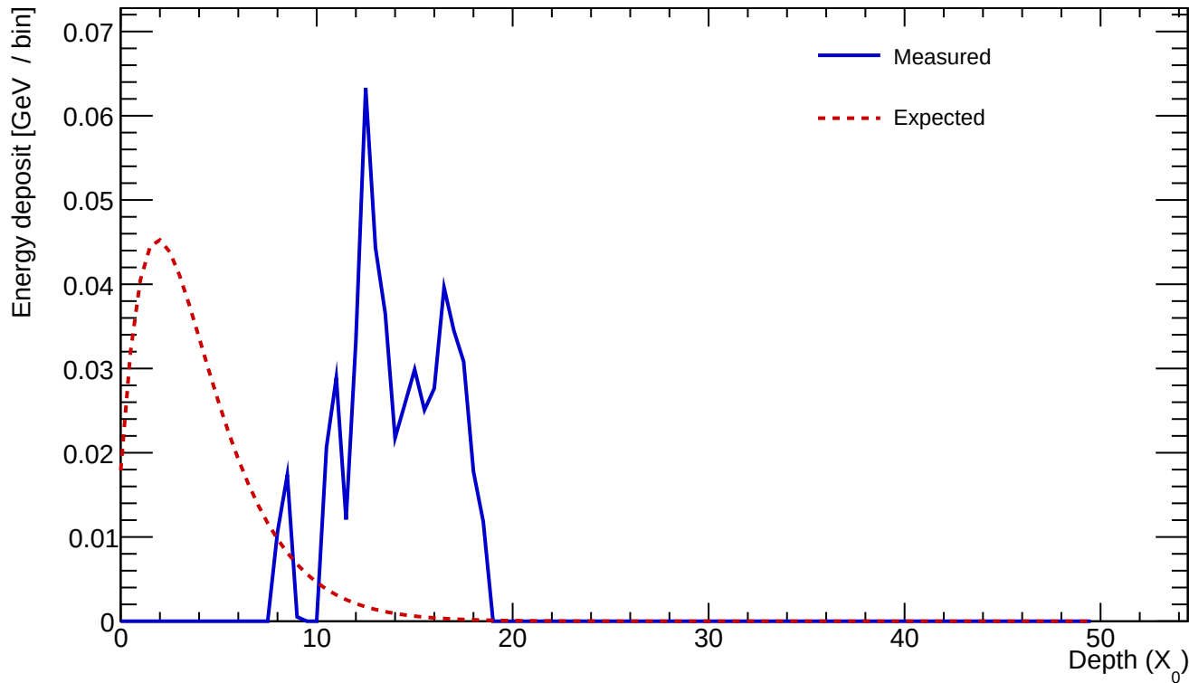
Cluster 963 E=0.532 GeV profileStart=10.50 X_0 \chi=0.3541
