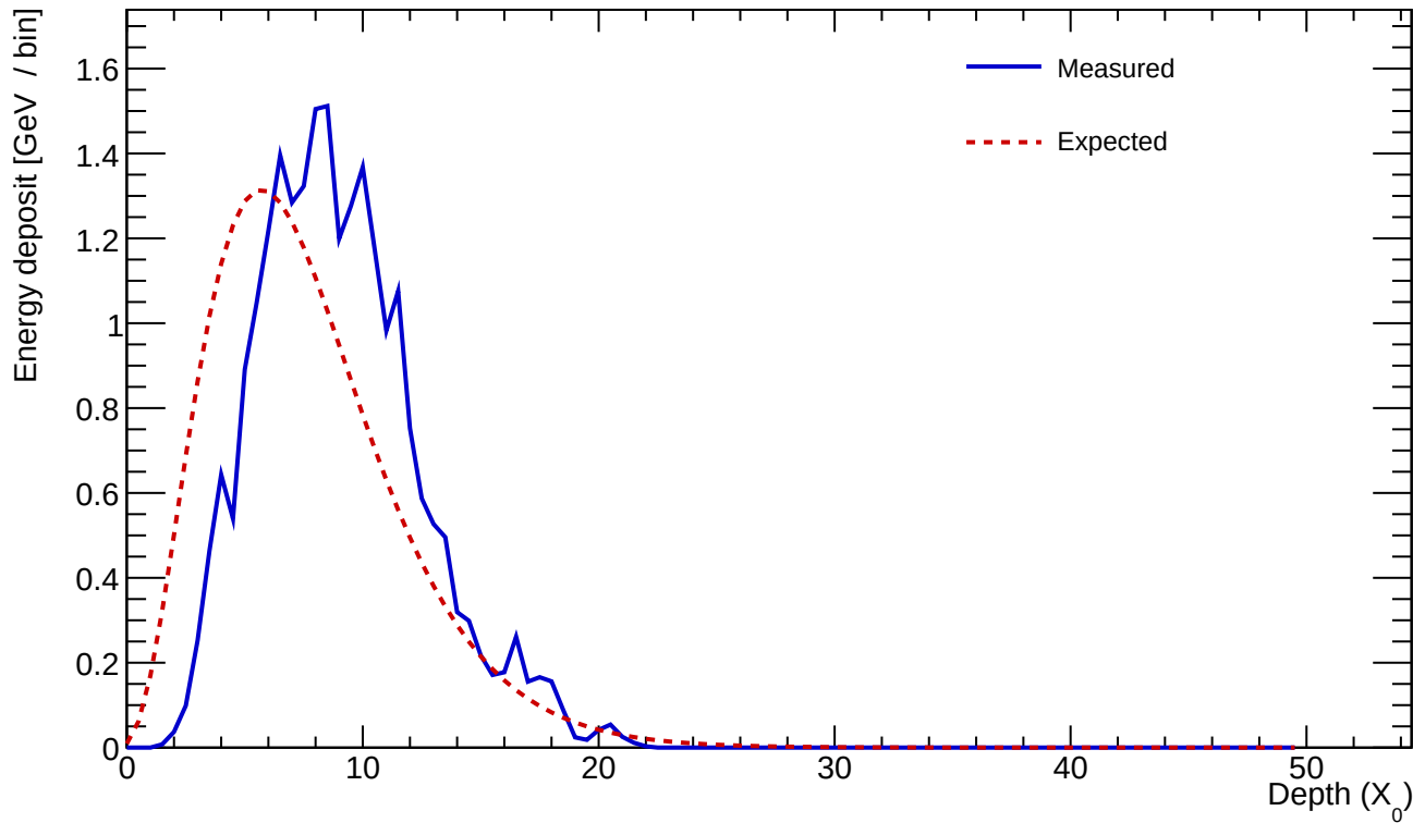
Cluster 837 E=23.847 GeV profileStart=1.50 X_0 \chi=0.1509
