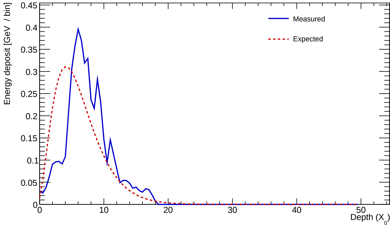
Cluster 1131 E=4.906 GeV profileStart=2.00 X_0 \chi=0.2551
