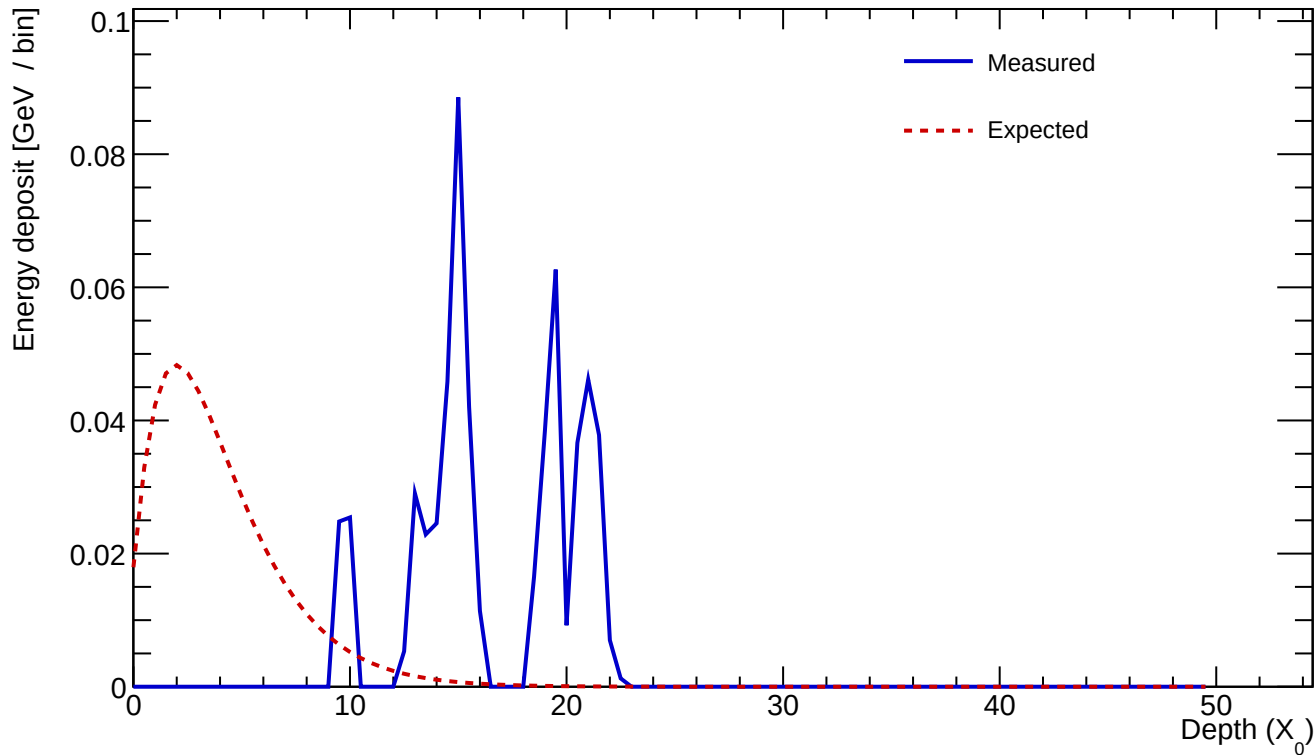
Cluster 546 E=0.576 GeV profileStart=12.50 X_0 \chi=0.8285
