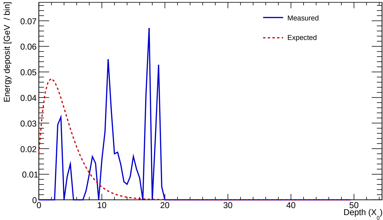
Cluster 408 E=0.563 GeV profileStart=8.50 X_0 \chi=0.9246
