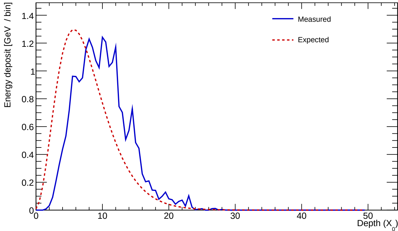
Cluster 158 E=23.489 GeV profileStart=2.50 X_0 \chi=0.1615
