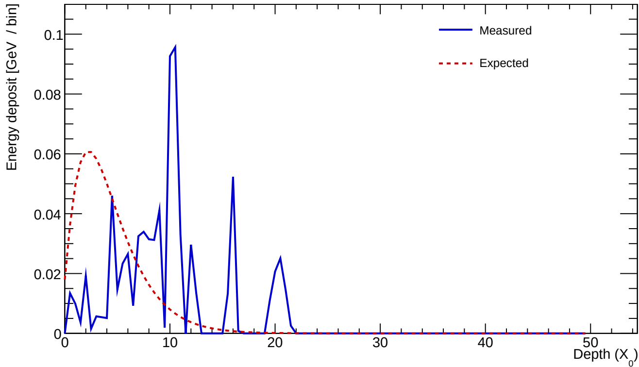
Cluster 267 E=0.761 GeV profileStart=4.00 X_0 \chi=0.9222
