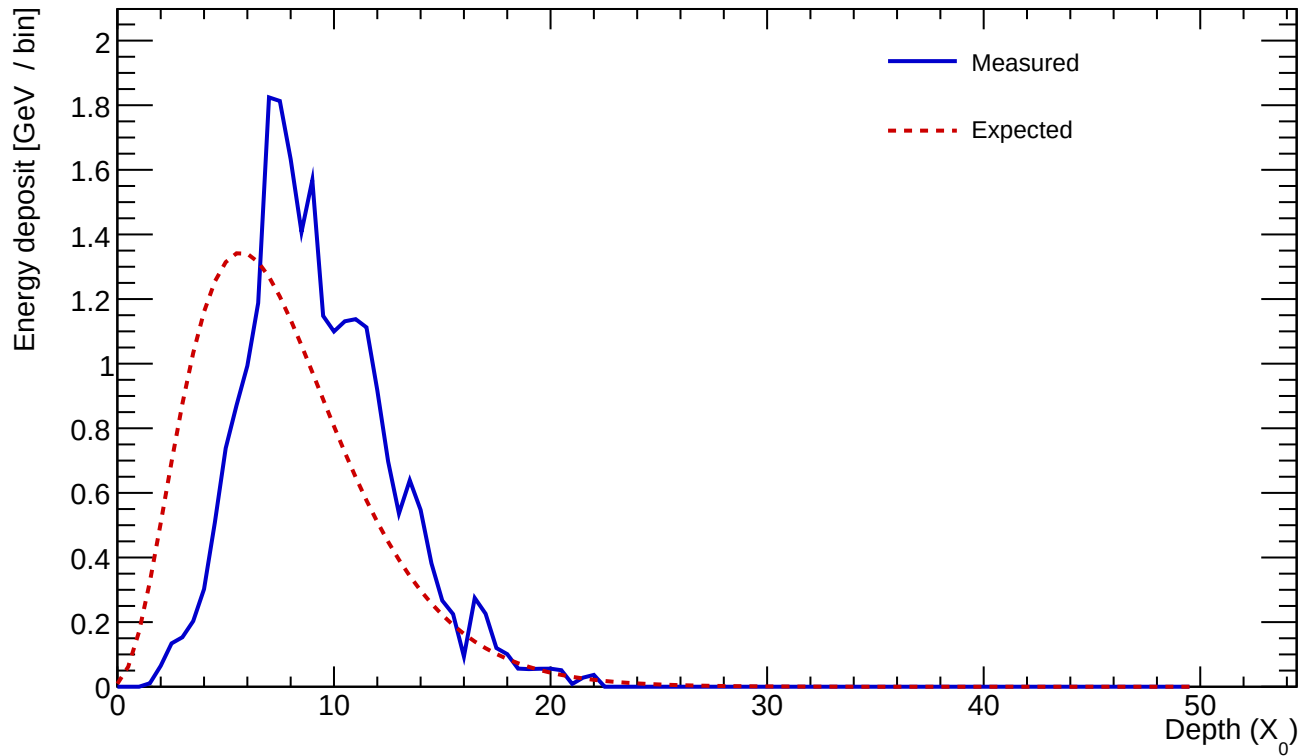
Cluster 210 E=24.414 GeV profileStart=2.50 X_0 \chi=0.1791
