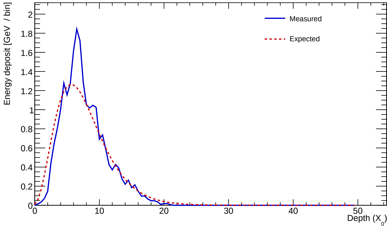
Cluster 882 E=22.848 GeV profileStart=0.50 X_0 \chi=0.1632
