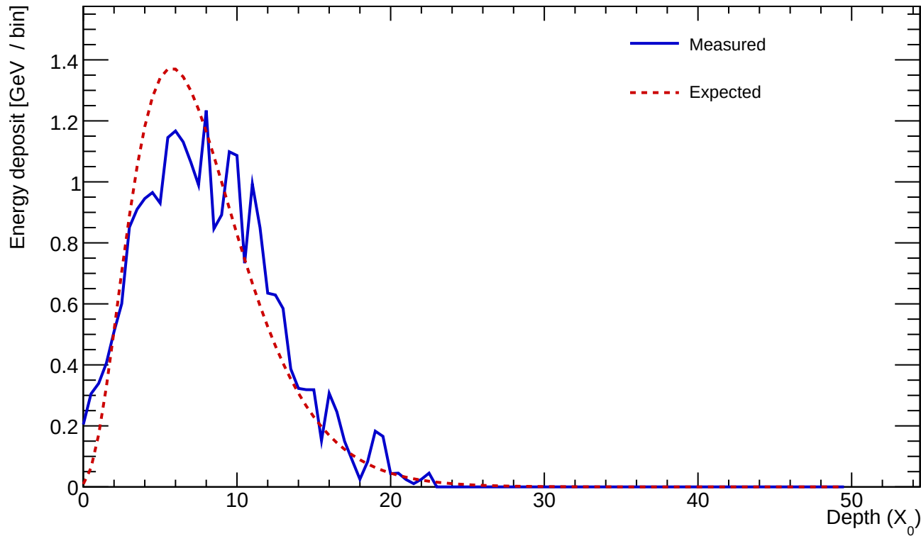
Cluster 486 E=24.984 GeV profileStart=0.50 X_0 \chi=0.2275
