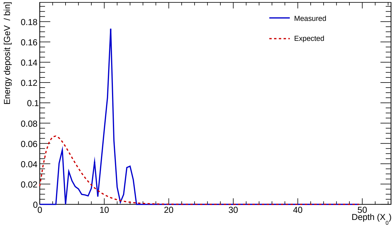
Cluster 140 E=0.857 GeV profileStart=8.00 X_0 \chi=0.6629
