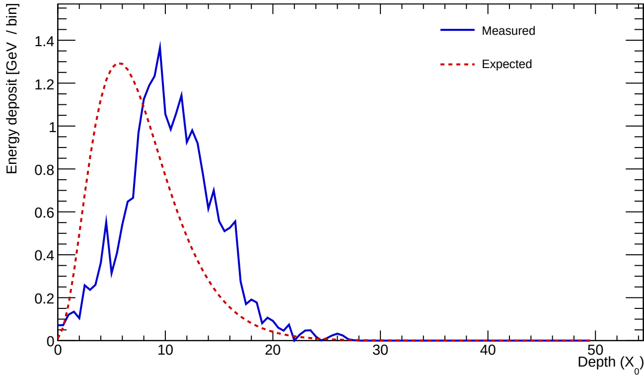
Cluster 378 E=23.445 GeV profileStart=3.50 X_0 \chi=0.2216
