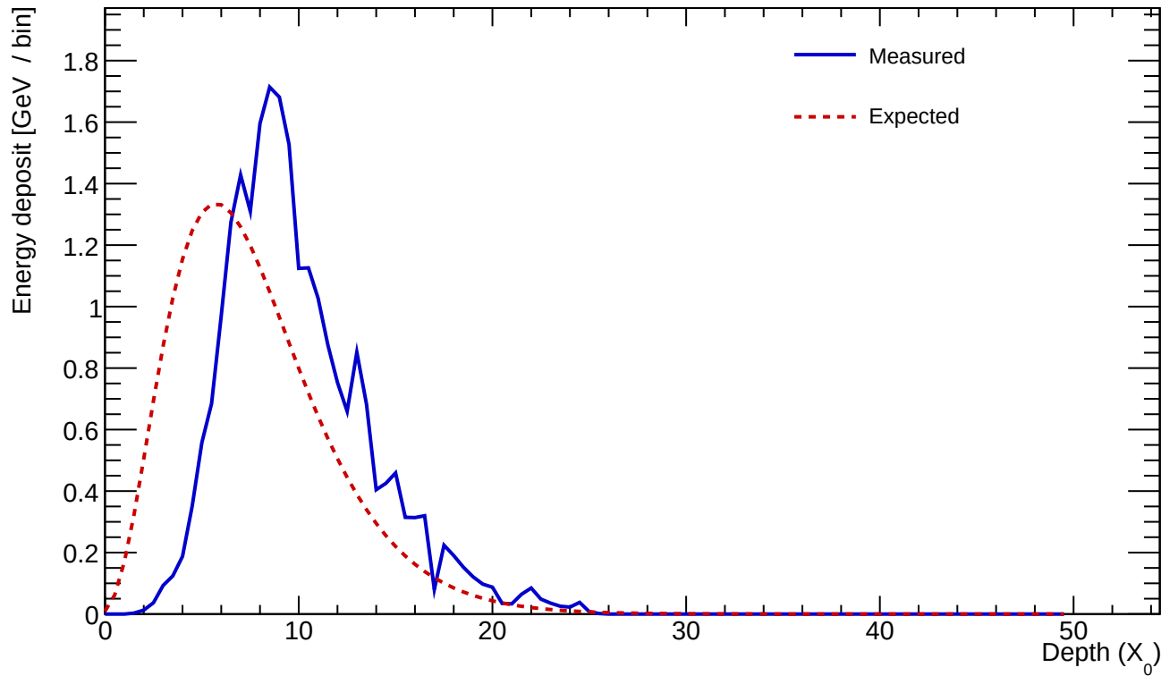
Cluster 786 E=24.238 GeV profileStart=2.50 X_0 \chi=0.1570
