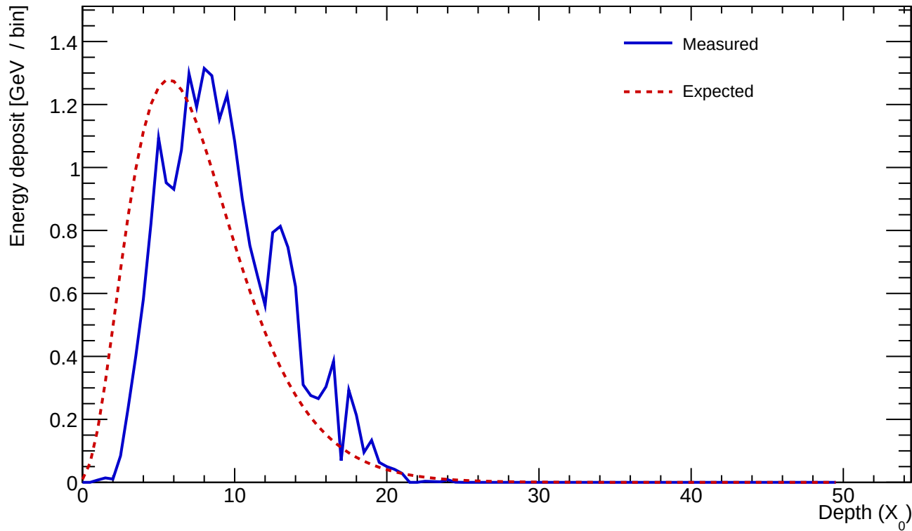
Cluster 714 E=23.140 GeV profileStart=2.00 X_0 \chi=0.1643
