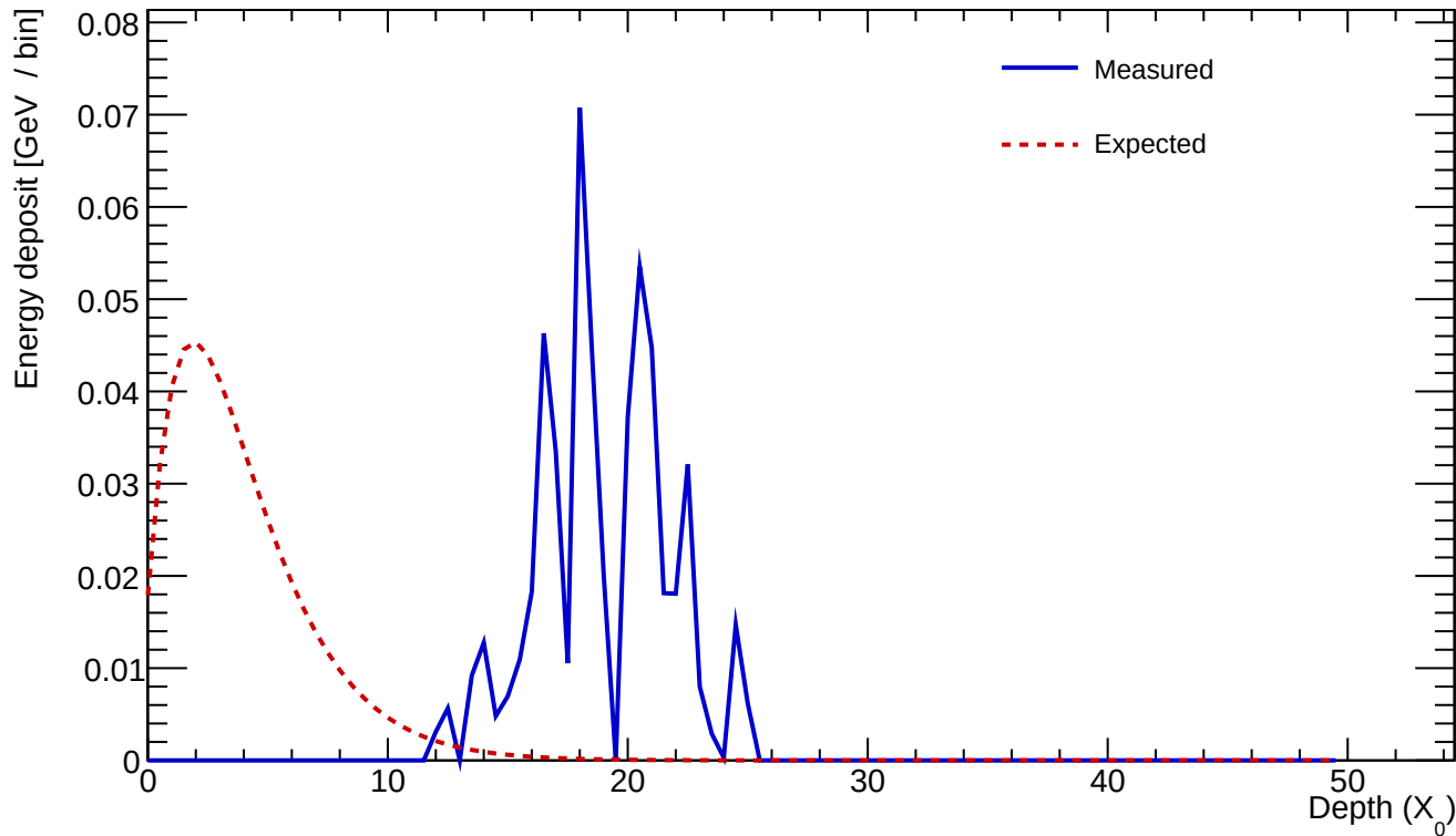
Cluster 992 E=0.533 GeV profileStart=16.00 X_0 \chi=0.5474
