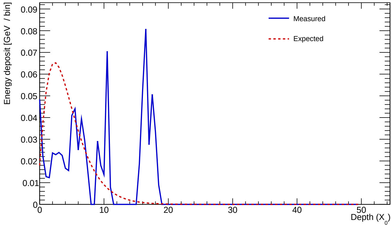
Cluster 685 E=0.826 GeV profileStart=0.50 X_0 \chi=0.9764
