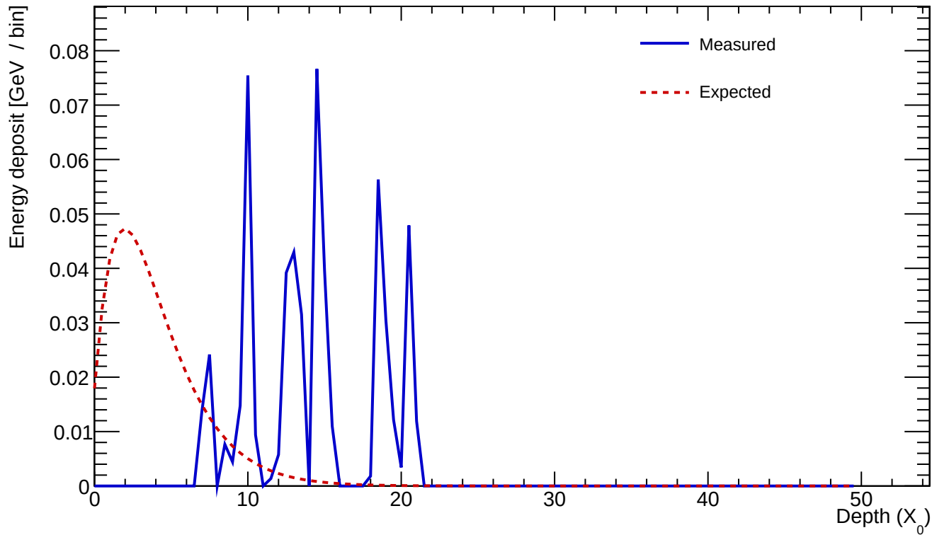
Cluster 424 E=0.562 GeV profileStart=12.00 X_0 \chi=0.9525
