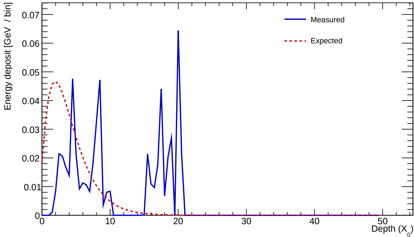
Cluster 139 E=0.552 GeV profileStart=2.00 X_0 \chi=0.9854
