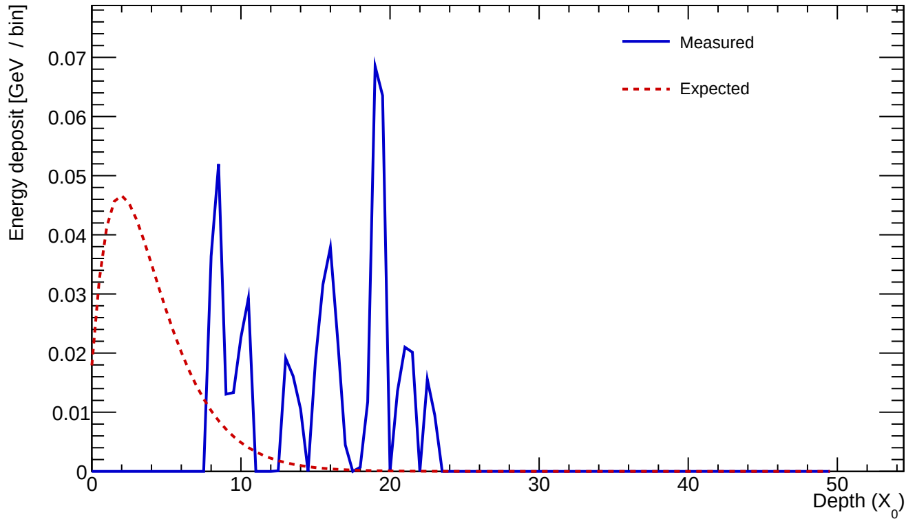
Cluster 495 E=0.551 GeV profileStart=7.50 X_0 \chi=1.0550
