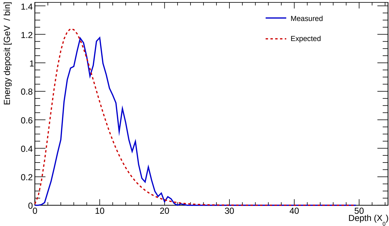
Cluster 650 E=22.358 GeV profileStart=2.00 X_0 \chi=0.1326
