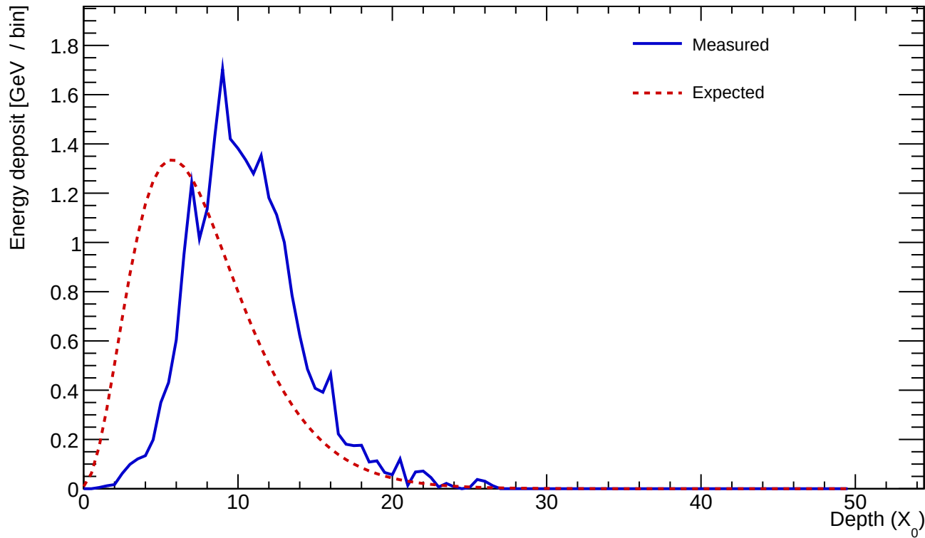
Cluster 312 E=24.271 GeV profileStart=3.50 X_0 \chi=0.1785
