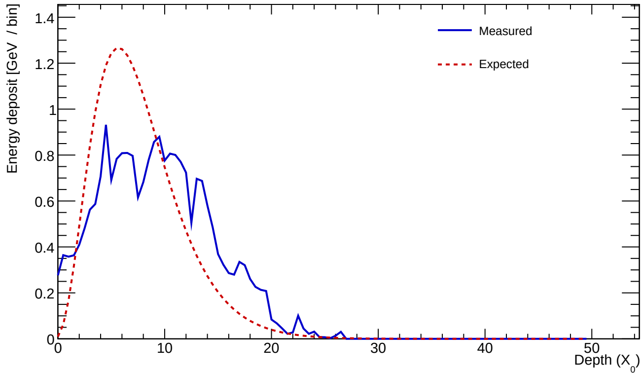
Cluster 588 E=22.901 GeV profileStart=1.00 X_0 \chi=0.3870
