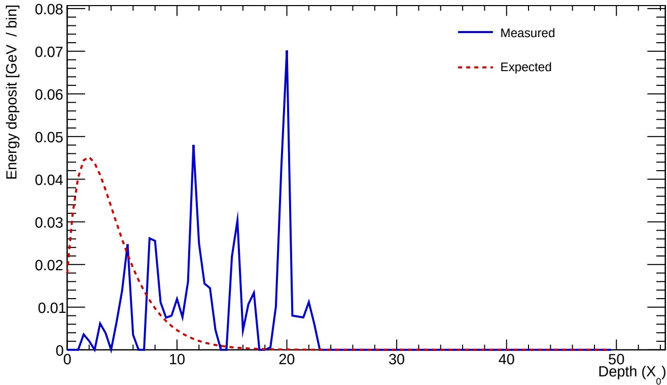
Cluster 166 E=0.531 GeV profileStart=7.50 X_0 \chi=1.0461
