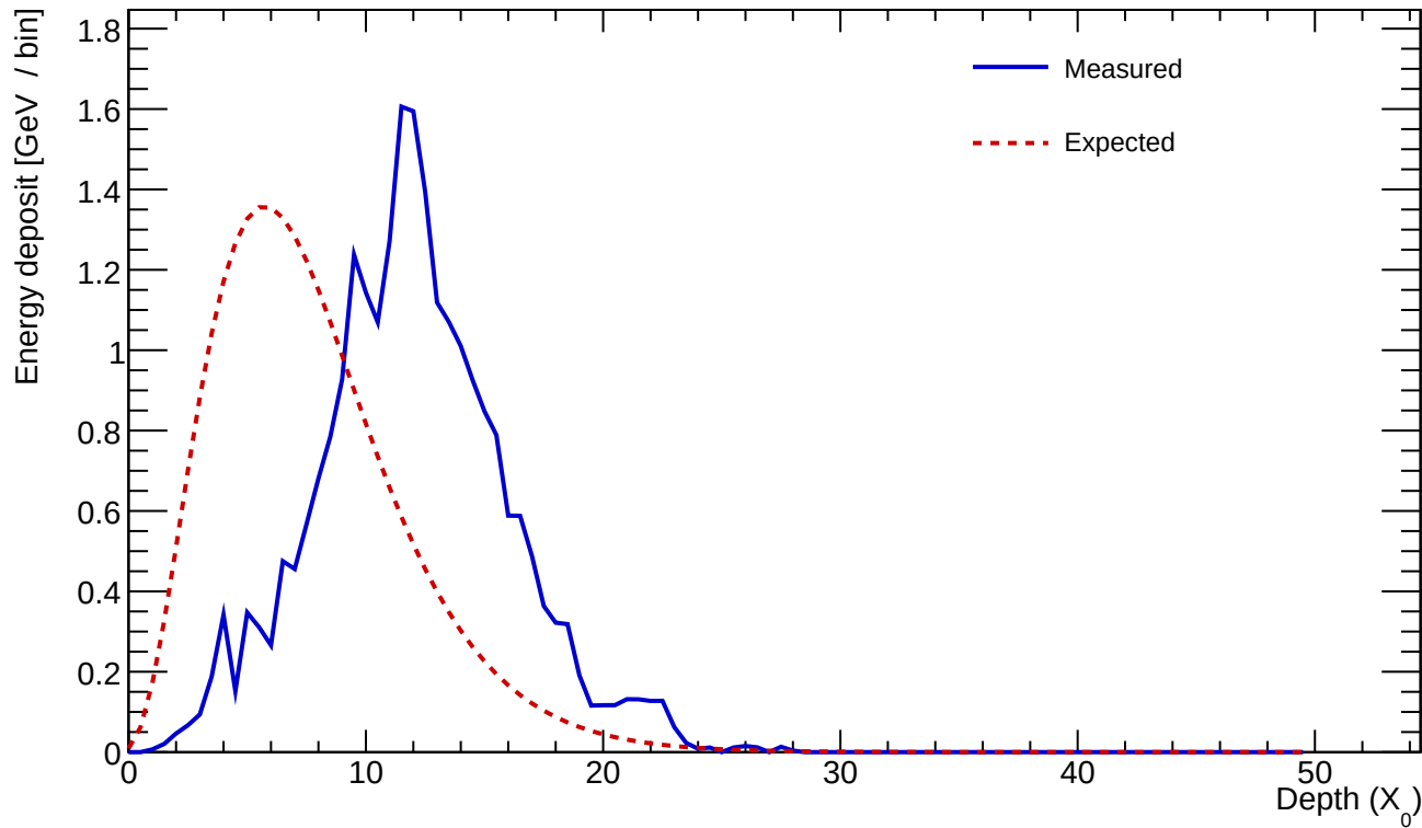
Cluster 61 E=24.696 GeV profileStart=5.00 X_0 \chi=0.2129
