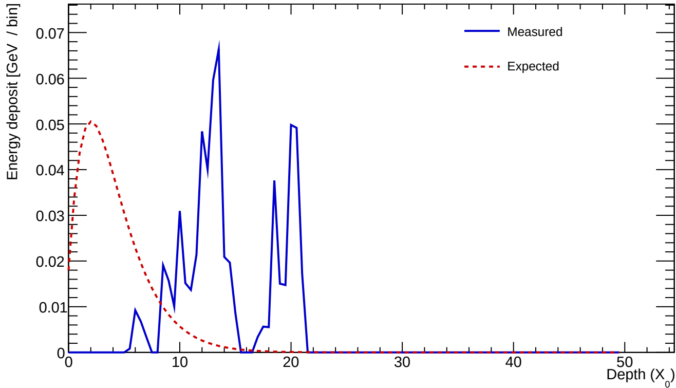
Cluster 482 E=0.608 GeV profileStart=9.50 X_0 \chi=0.7736
