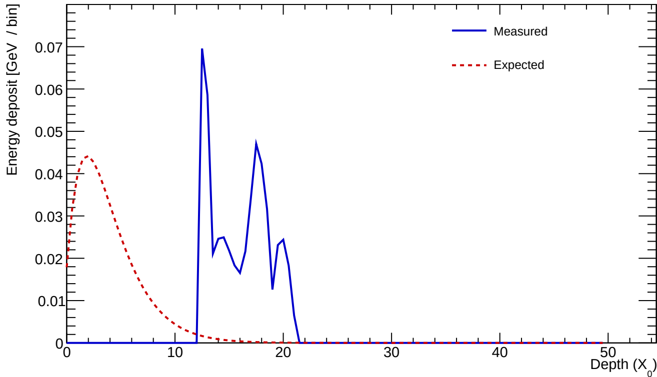
Cluster 270 E=0.517 GeV profileStart=12.50 X_0 \chi=0.5895
