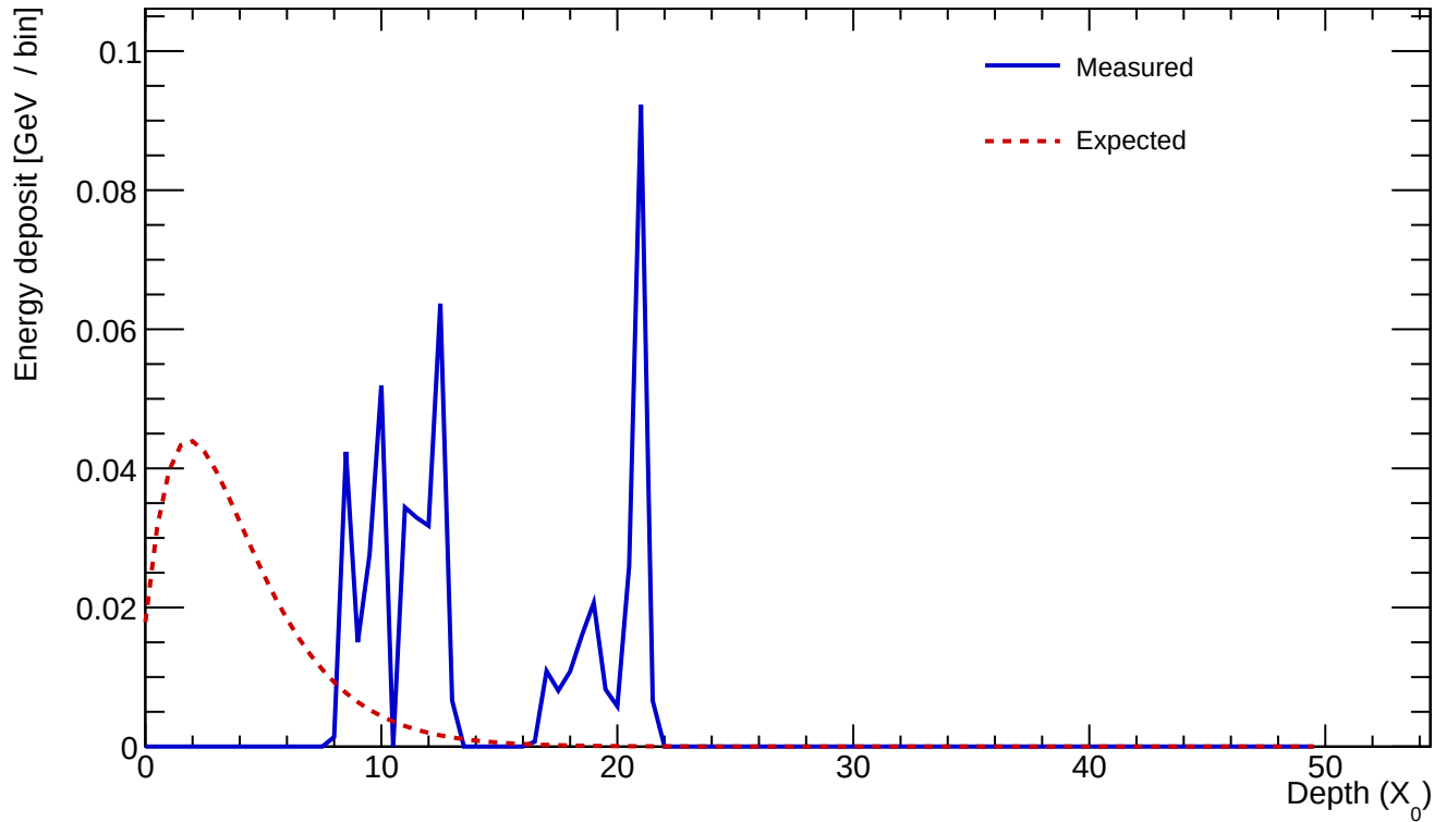
Cluster 877 E=0.514 GeV profileStart=8.00 X_0 \chi=0.8668
