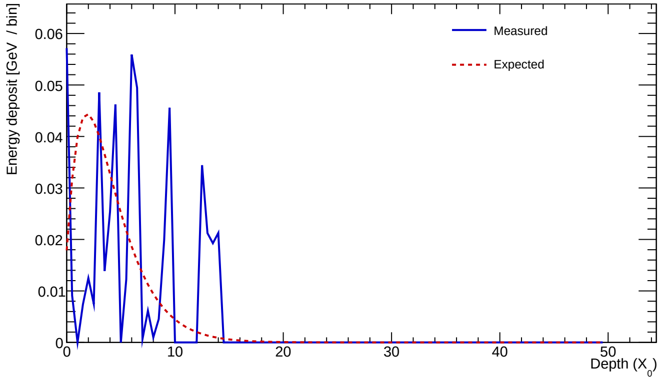
Cluster 304 E=0.519 GeV profileStart=2.00 X_0 \chi=0.9272
