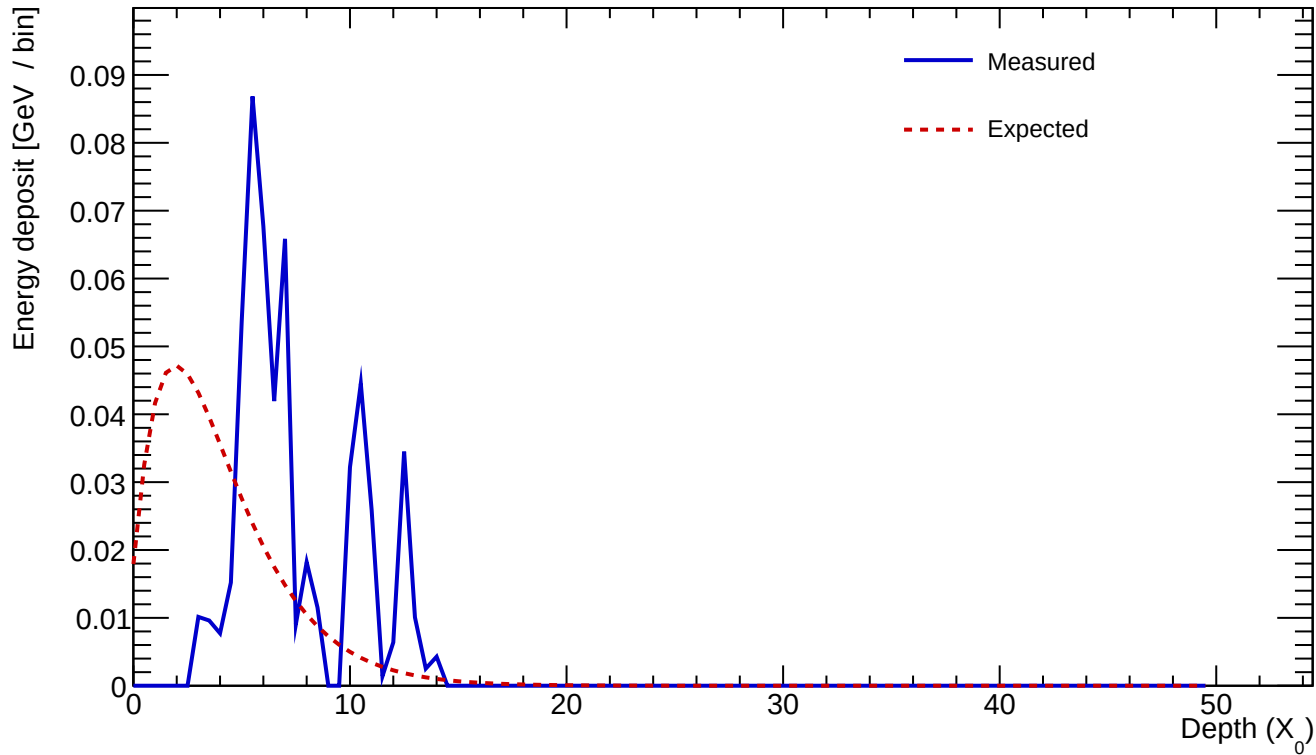
Cluster 717 E=0.559 GeV profileStart=4.00 X_0 \chi=0.6503
