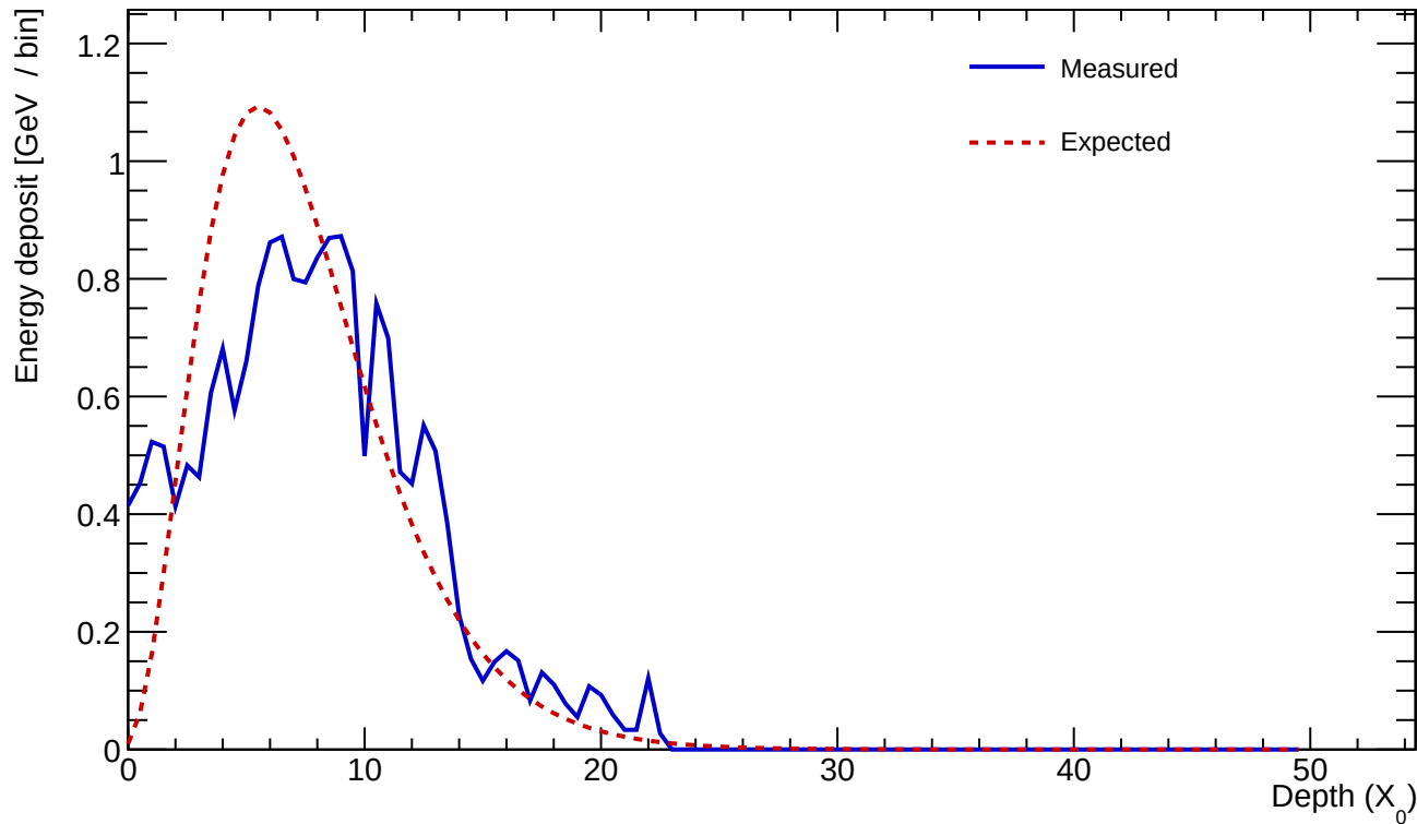
Cluster 244 E=19.514 GeV profileStart=1.00 X_0 \chi=0.3065
