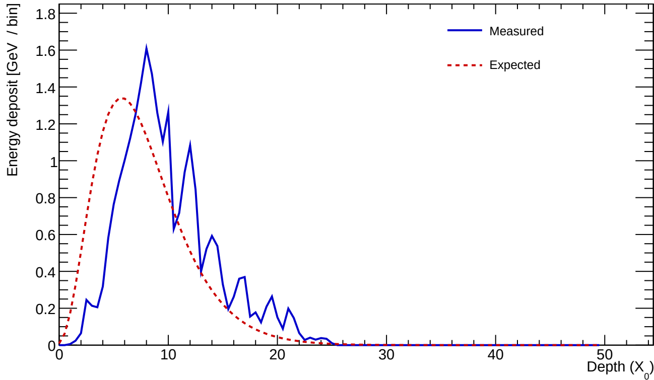
Cluster 76 E=24.352 GeV profileStart=2.50 X_0 \chi=0.1797
