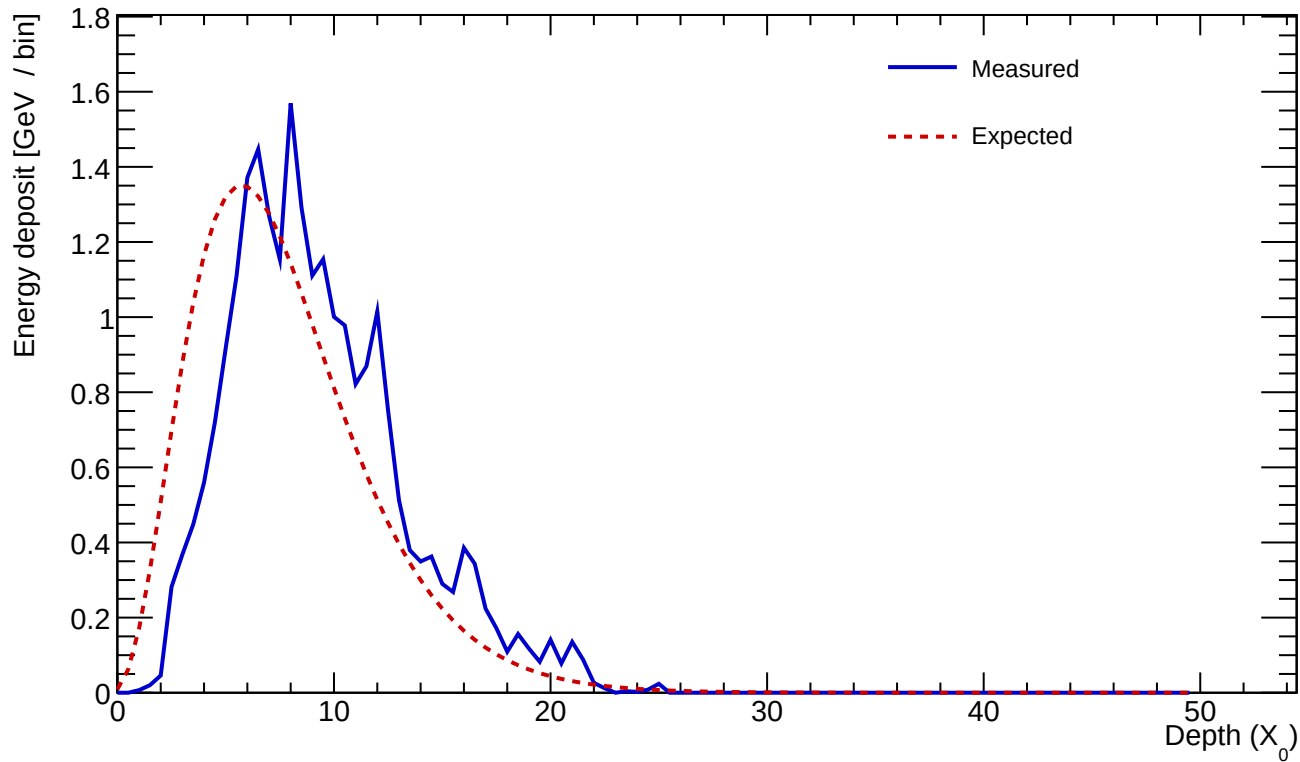
Cluster 99 E=24.551 GeV profileStart=1.50 X_0 \chi=0.1340
