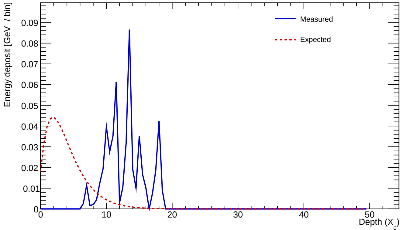
Cluster 265 E=0.518 GeV profileStart=9.00 X_0 \chi=0.5847
