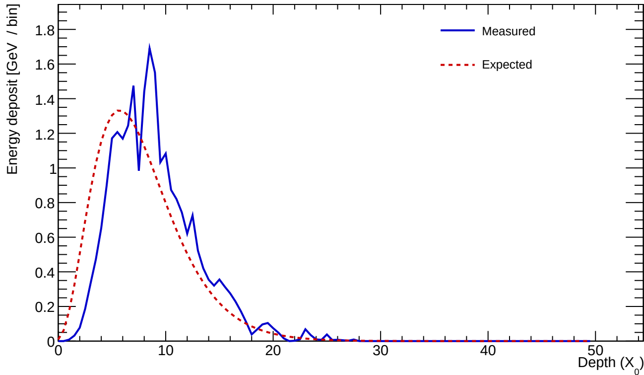
Cluster 369 E=24.203 GeV profileStart=1.50 X_0 \chi=0.1360
