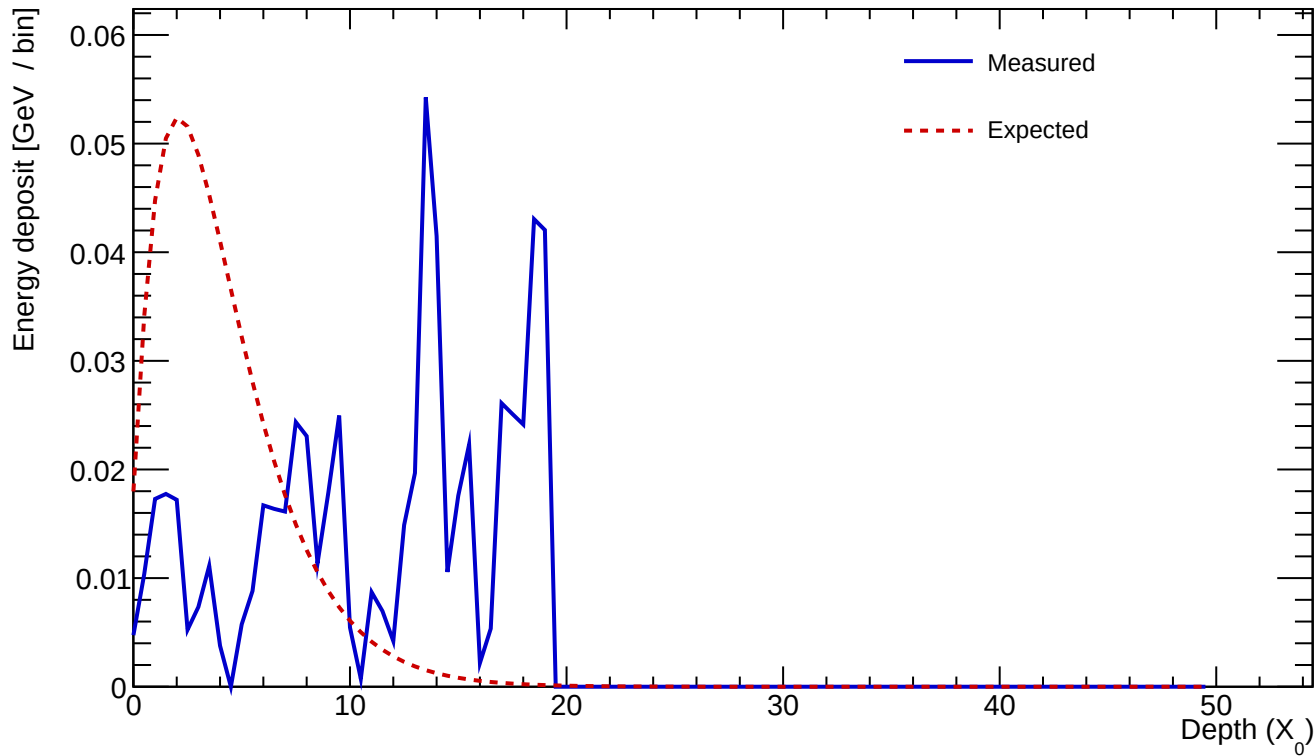
Cluster 366 E=0.635 GeV profileStart=17.50 X_0 \chi=0.8181
