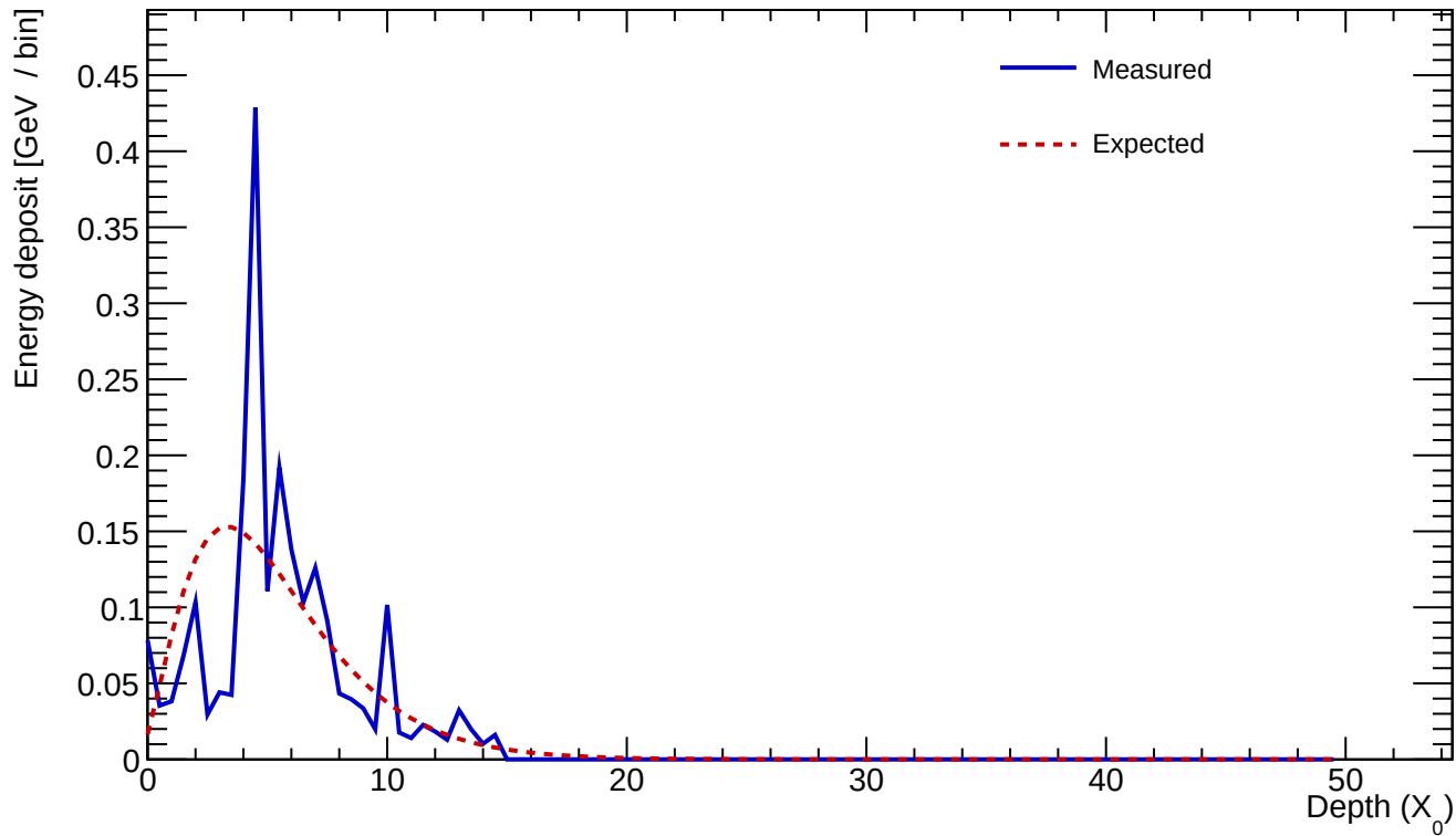
Cluster 307 E=2.216 GeV profileStart=0.50 X_0 \chi=0.5190
