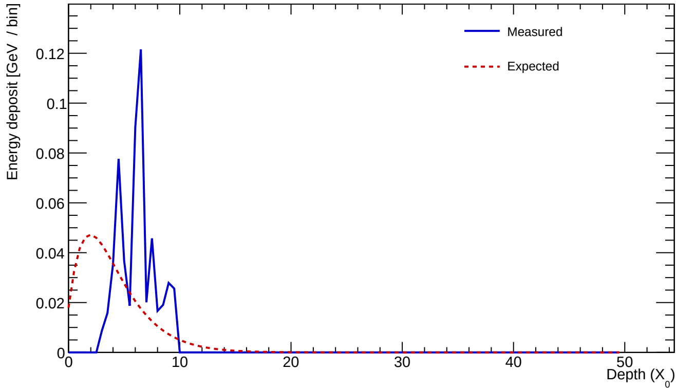
Cluster 388 E=0.560 GeV profileStart=3.50 X_0 \chi=0.4774
