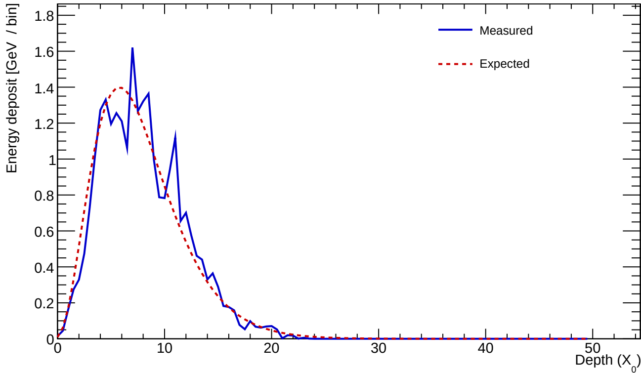
Cluster 811 E=25.500 GeV profileStart=0.50 X_0 \chi=0.1446
