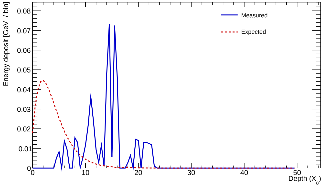
Cluster 666 E=0.523 GeV profileStart=13.00 X_0 \chi=0.9830
