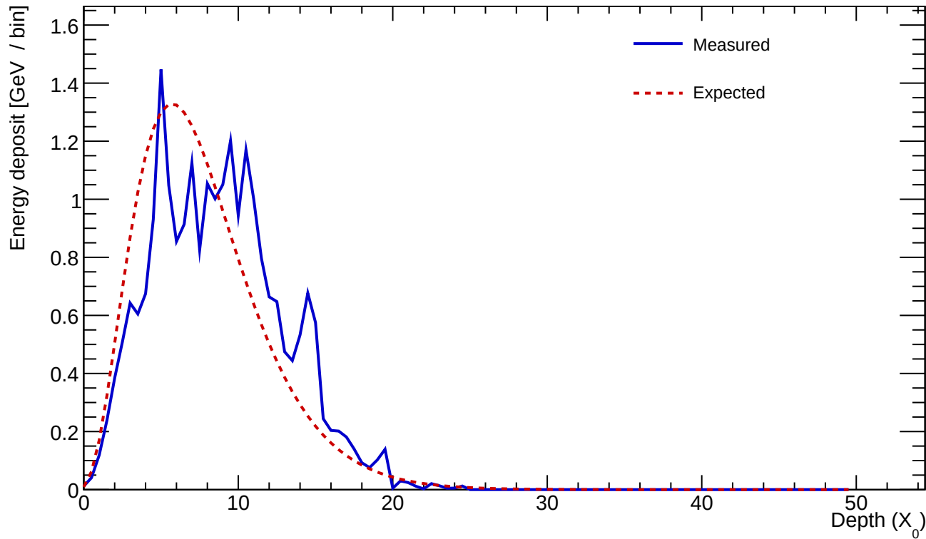
Cluster 466 E=24.115 GeV profileStart=1.00 X_0 \chi=0.2390
