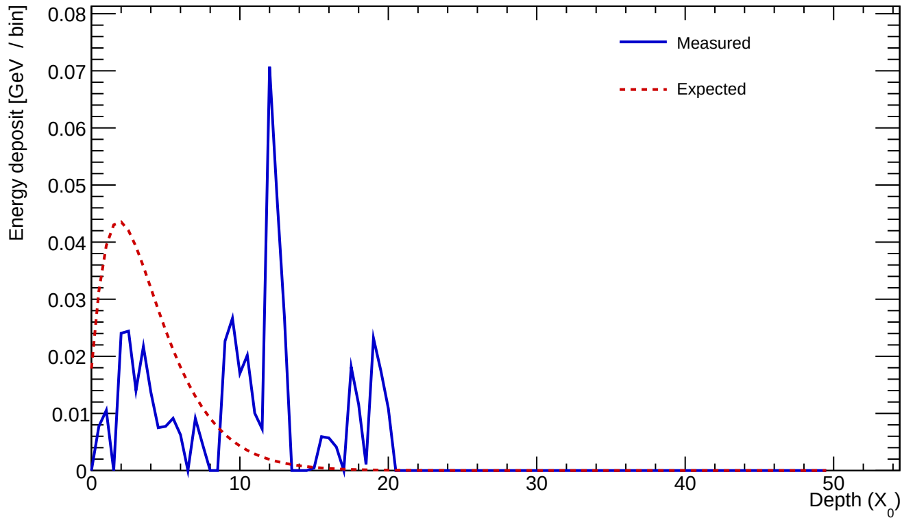
Cluster 28 E=0.508 GeV profileStart=9.00 X_0 \chi=1.0014
