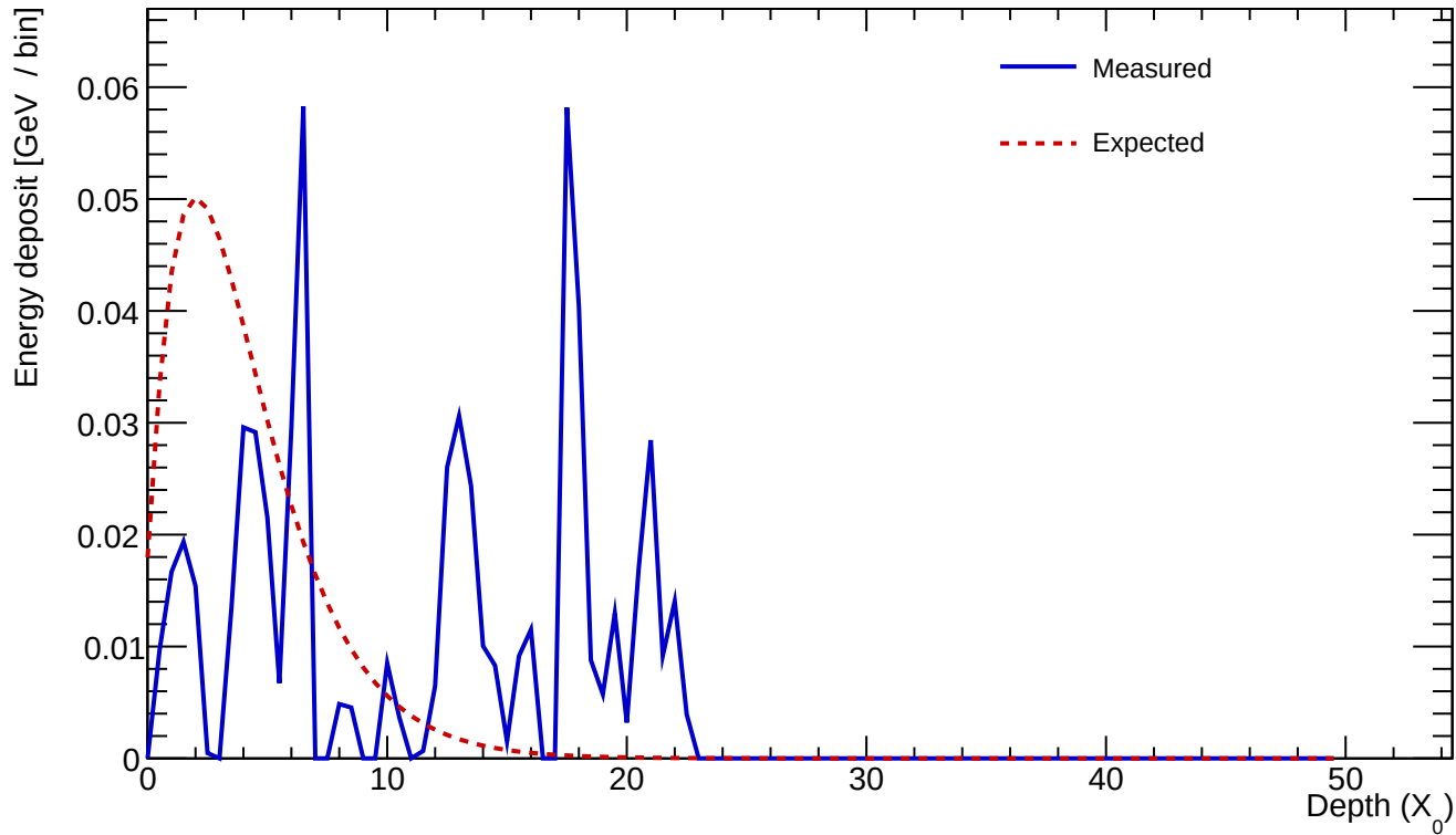
Cluster 259 E=0.602 GeV profileStart=1.00 X_0 \chi=1.1628
