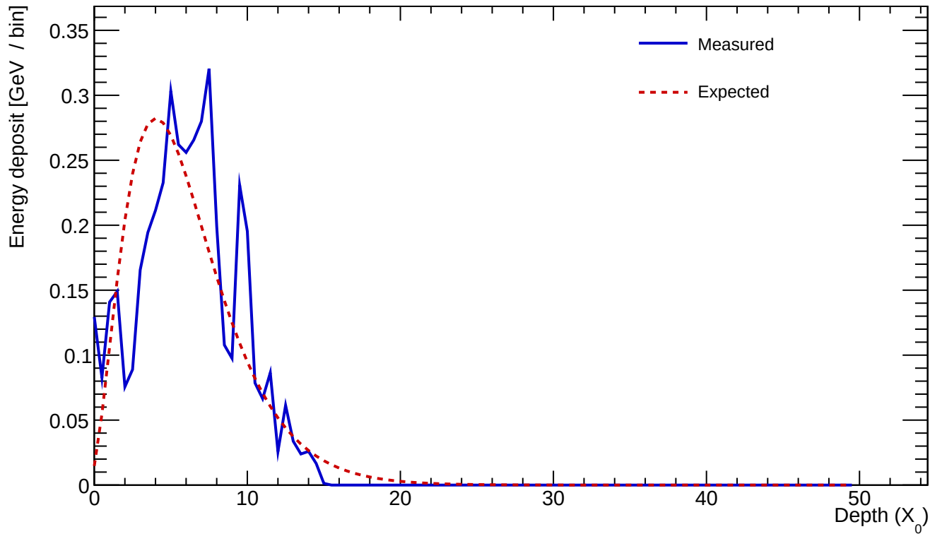
Cluster 269 E=4.409 GeV profileStart=1.50 X_0 \chi=0.3072
