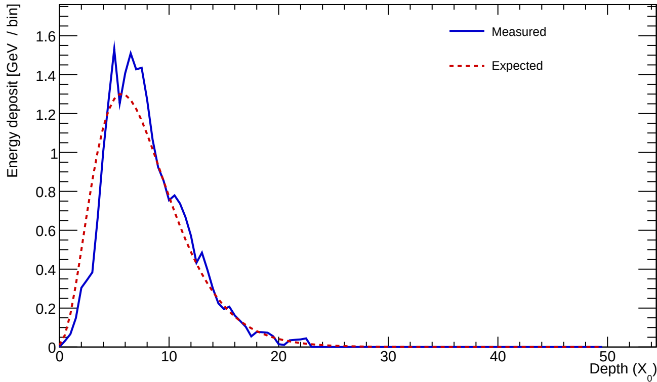
Cluster 511 E=23.574 GeV profileStart=0.50 X_0 \chi=0.1238
