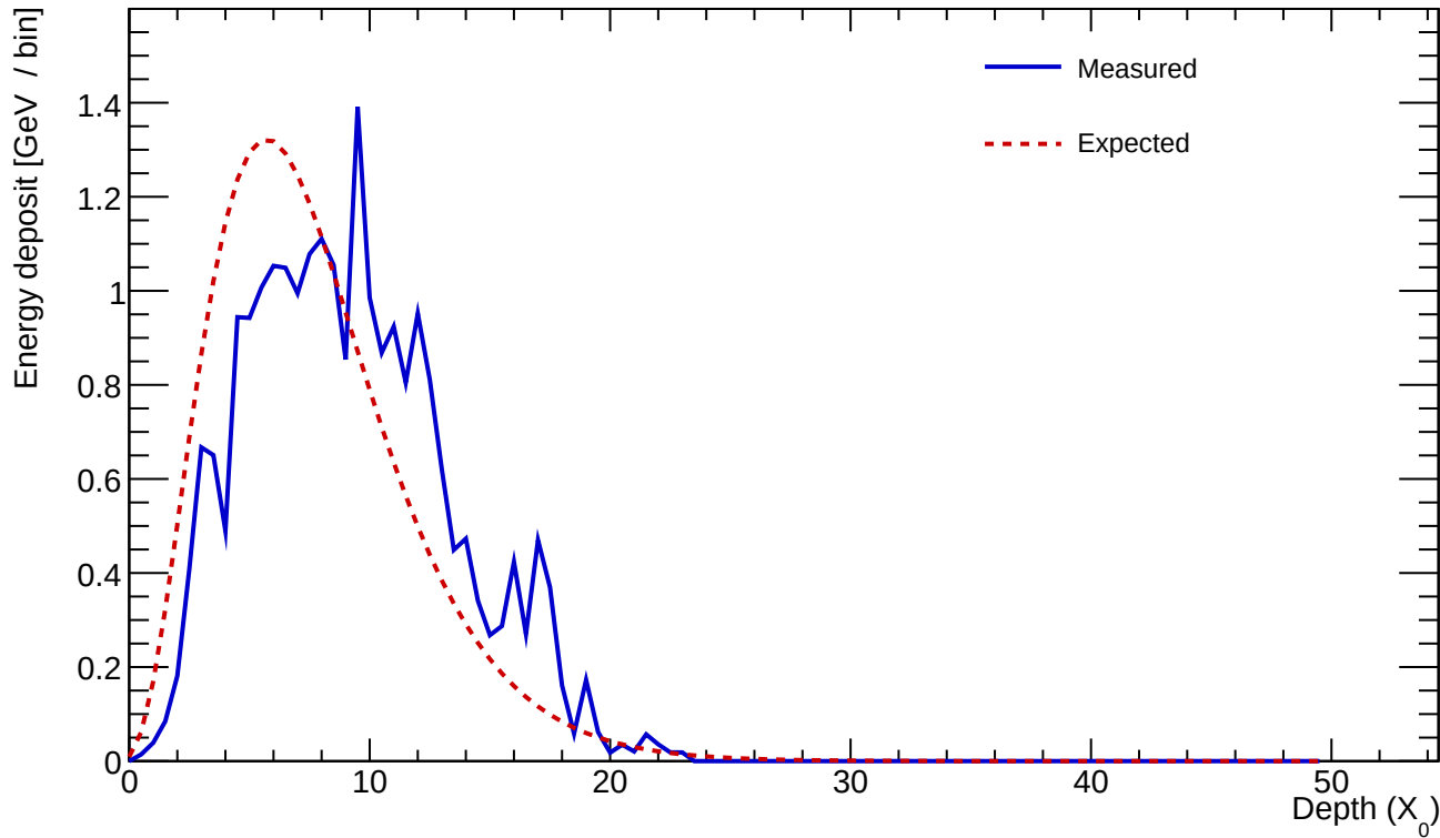
Cluster 30 E=23.990 GeV profileStart=1.50 X_0 \chi=0.2232
