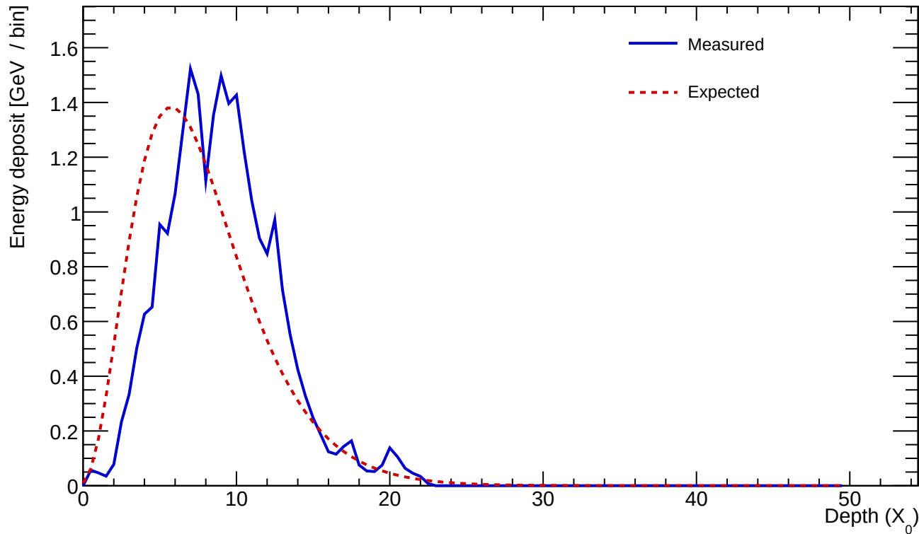
Cluster 188 E=25.183 GeV profileStart=2.00 X_0 \chi=0.1676
