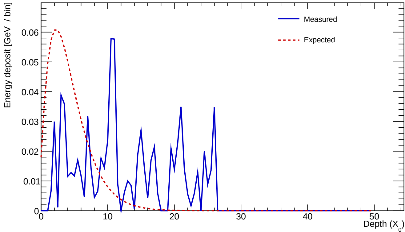
Cluster 133 E=0.763 GeV profileStart=9.00 X_0 \chi=1.0543
