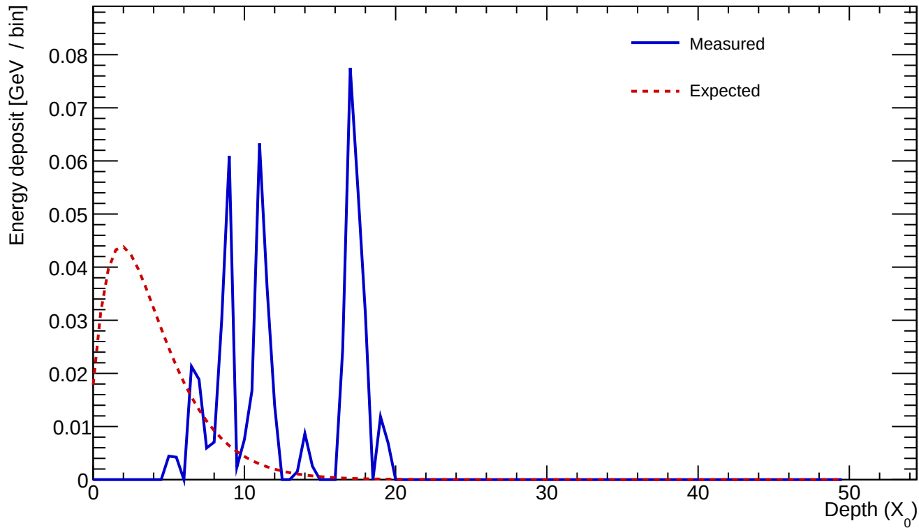
Cluster 209 E=0.513 GeV profileStart=6.50 X_0 \chi=1.0200
