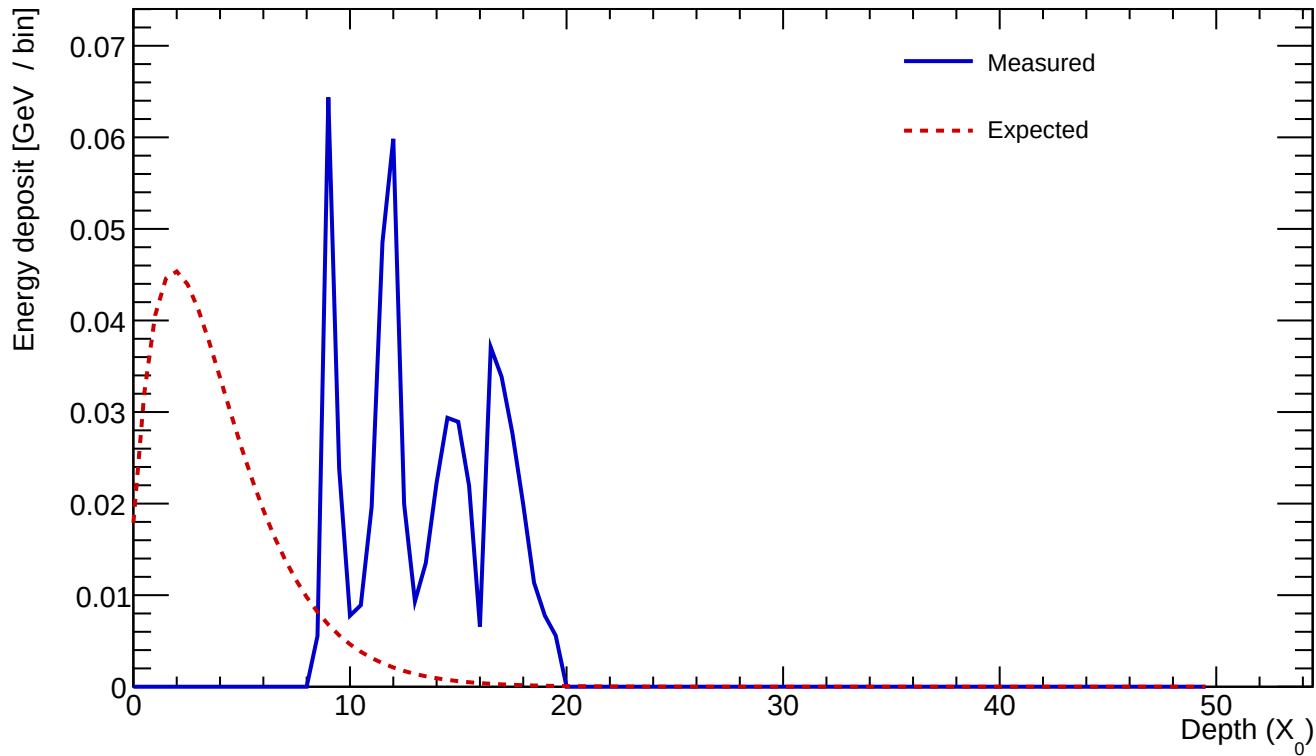
Cluster 230 E=0.534 GeV profileStart=10.50 X_0 \chi=0.6255
