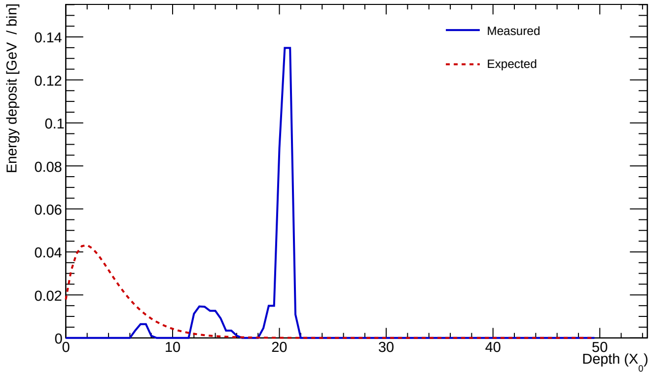
Cluster 474 E=0.503 GeV profileStart=19.00 X_0 \chi=0.7088
