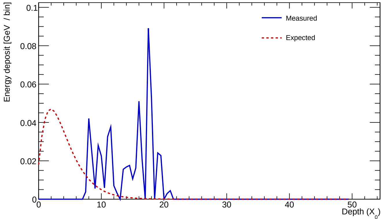
Cluster 1085 E=0.557 GeV profileStart=7.50 X_0 \chi=0.9003
