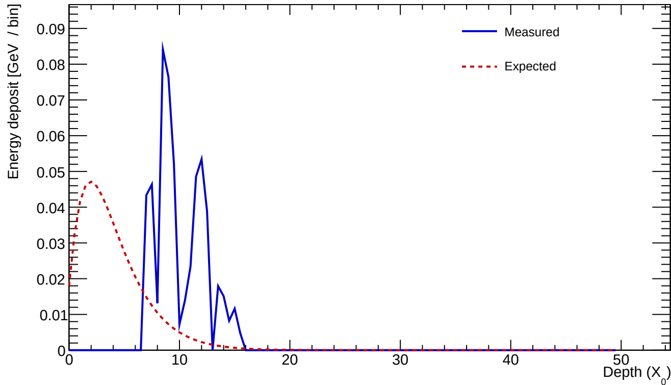
Cluster 8 E=0.559 GeV profileStart=7.00 X_0 \chi=0.5358
