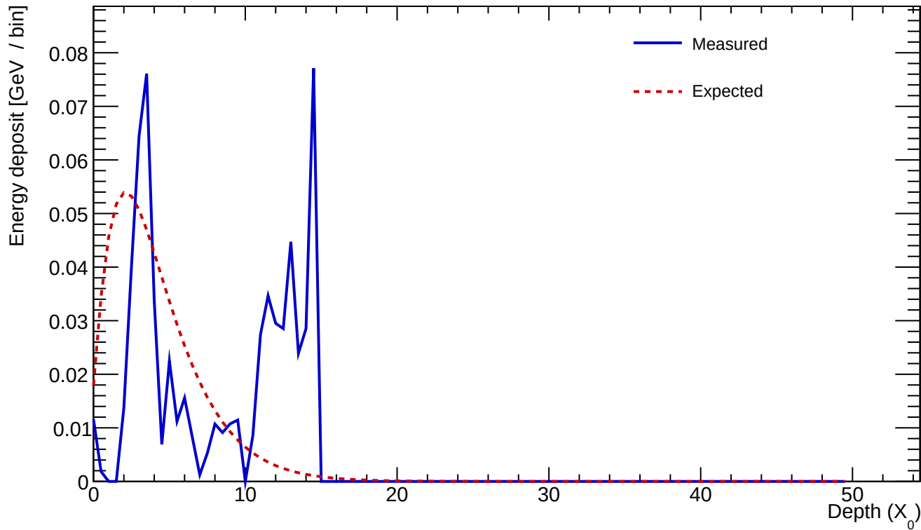
Cluster 1099 E=0.658 GeV profileStart=1.50 X_0 \chi=0.8076
