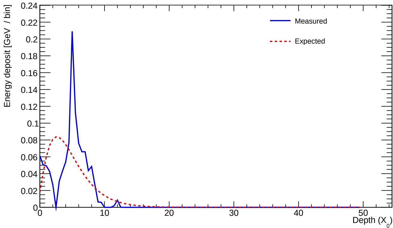
Cluster 734 E=1.108 GeV profileStart=2.00 X_0 \chi=0.6207
