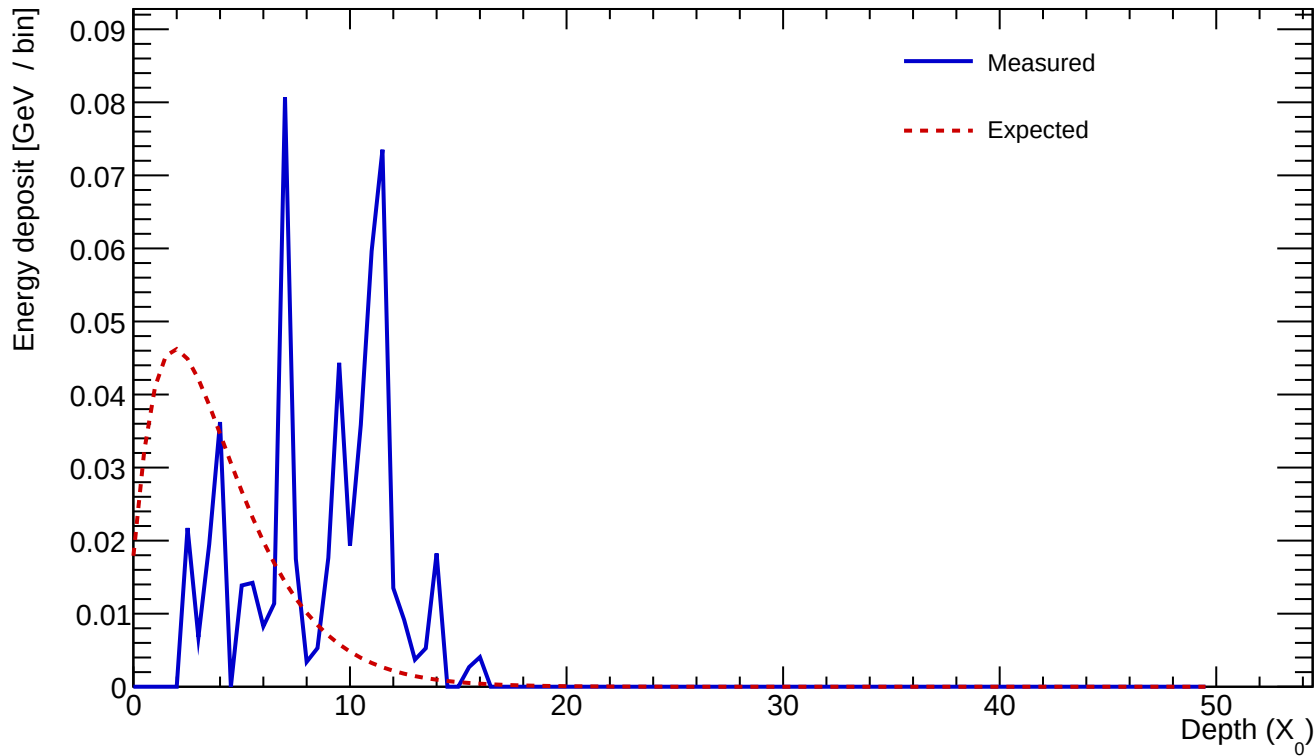
Cluster 109 E=0.546 GeV profileStart=6.50 X_0 \chi=0.8784
