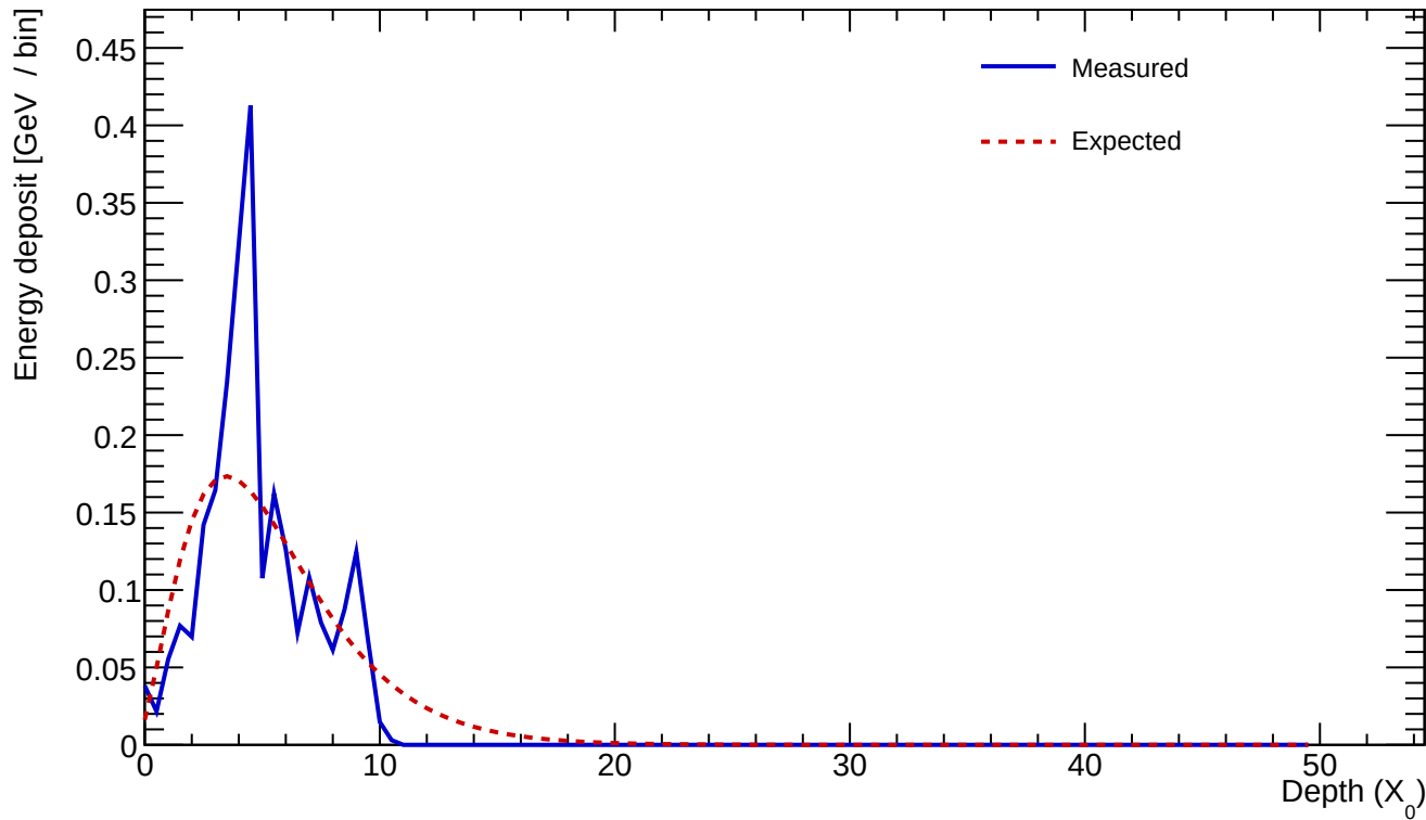
Cluster 916 E=2.553 GeV profileStart=0.50 X_0 \chi=0.3439
