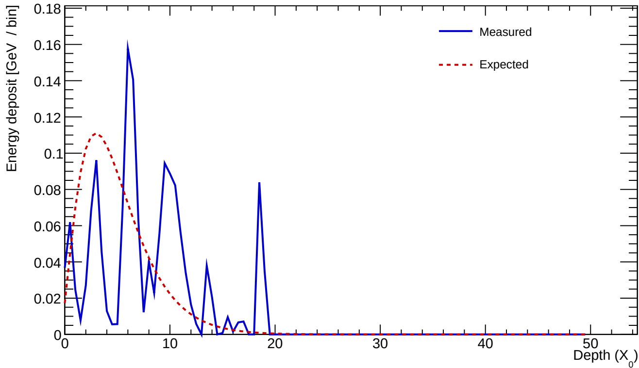
Cluster 418 E=1.535 GeV profileStart=1.50 X_0 \chi=0.7714
