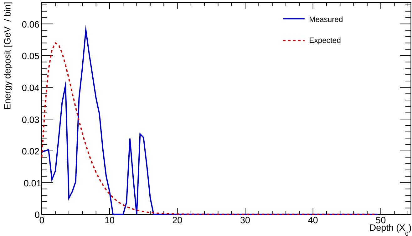
Cluster 147 E=0.659 GeV profileStart=2.50 X_0 \chi=0.6753
