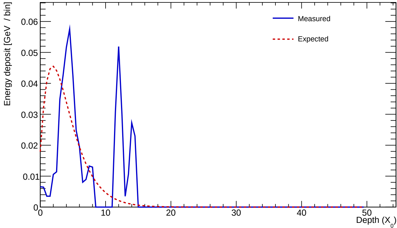
Cluster 235 E=0.536 GeV profileStart=2.00 X_0 \chi=0.6687
