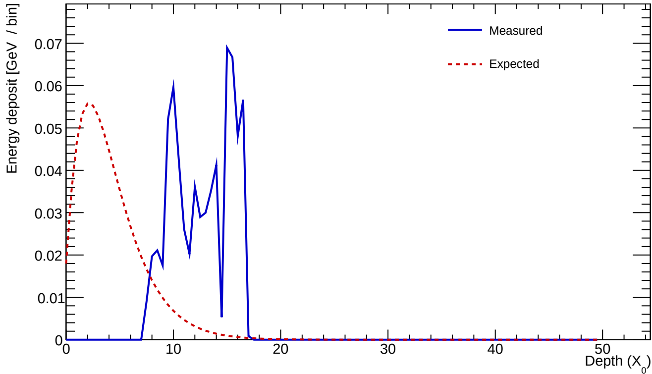
Cluster 743 E=0.686 GeV profileStart=8.00 X_0 \chi=0.5349
