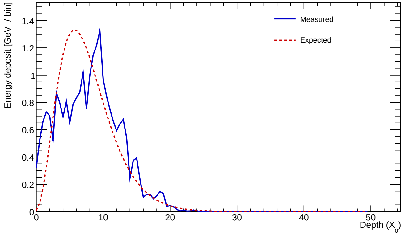
Cluster 783 E=24.188 GeV profileStart=0.50 X_0 \chi=0.3477
