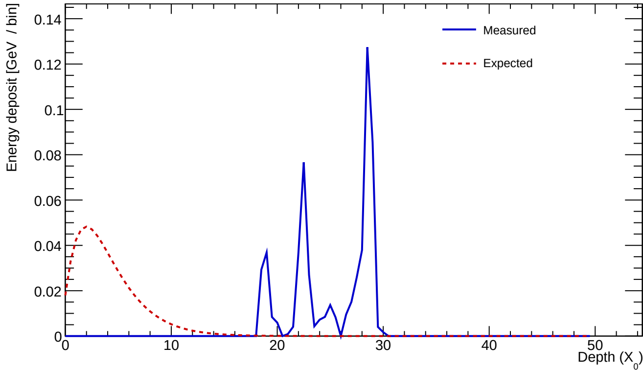
Cluster 12 E=0.575 GeV profileStart=27.00 X_0 \chi=0.7869
