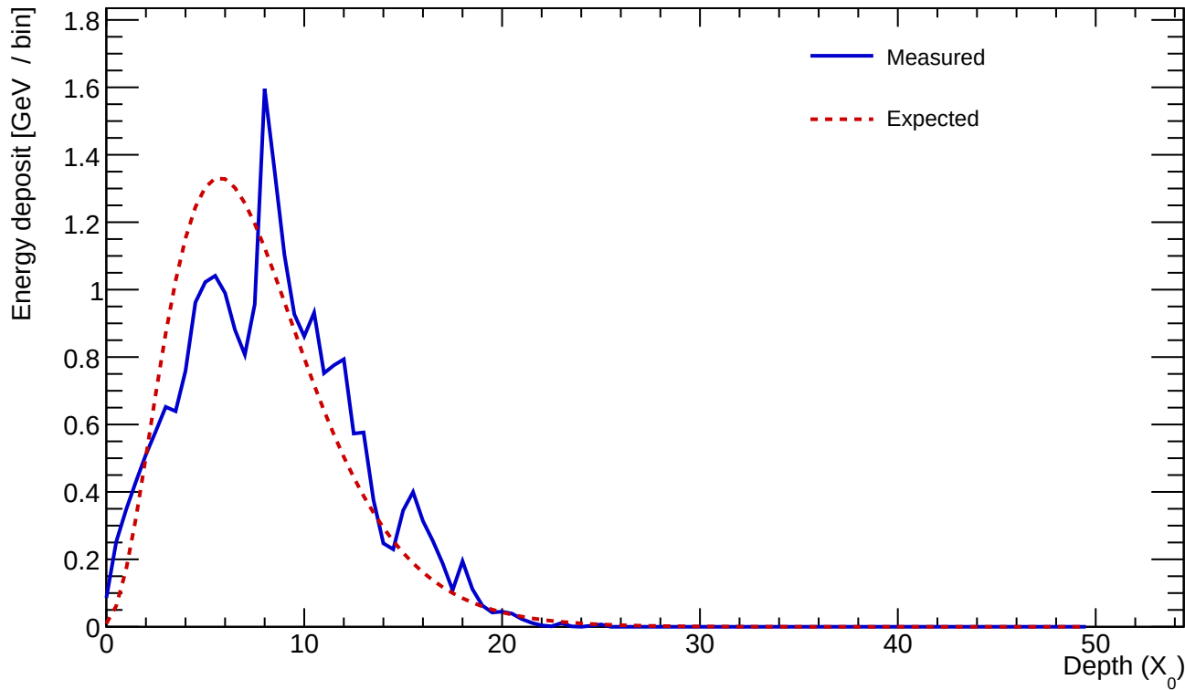
Cluster 215 E=24.184 GeV profileStart=1.00 X_0 \chi=0.2540
