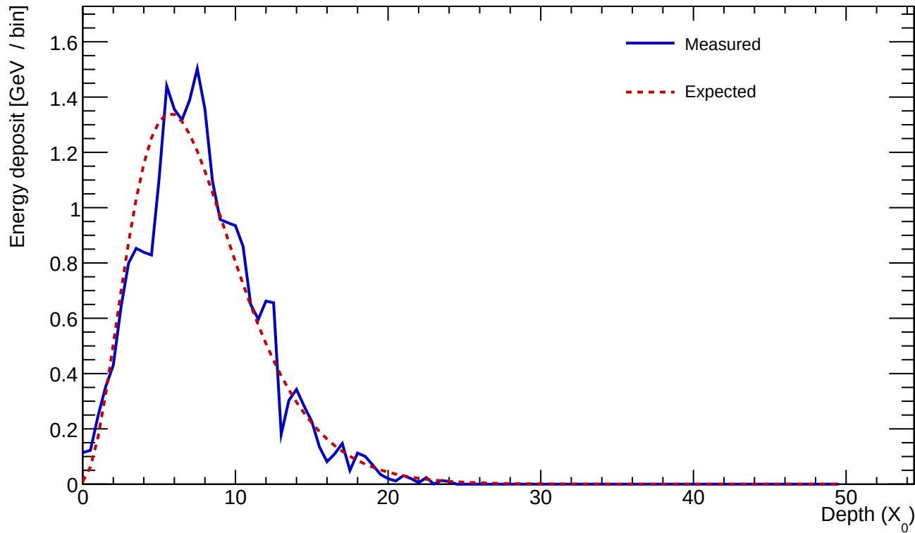
Cluster 929 E=24.356 GeV profileStart=0.50 X_0 \chi=0.1555
