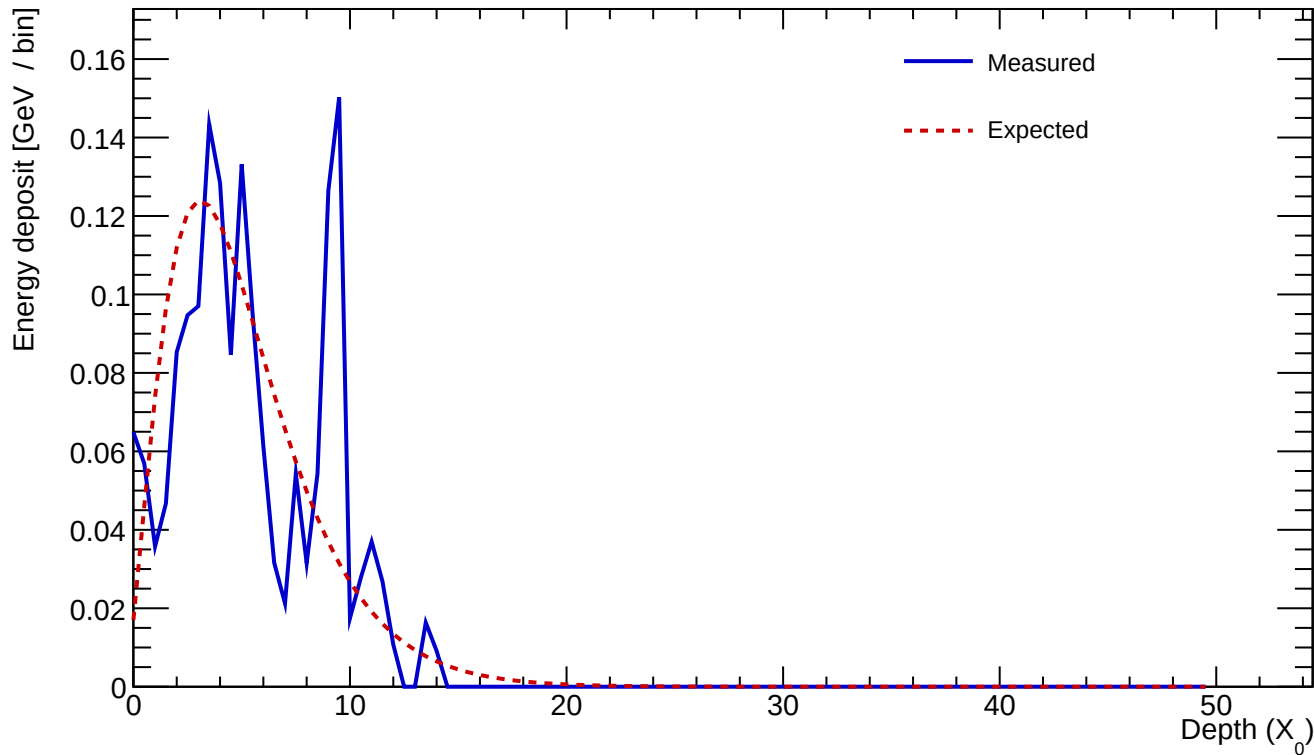
Cluster 1064 E=1.742 GeV profileStart=0.50 X_0 \chi=0.4200
