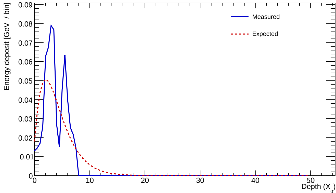
Cluster 75 E=0.609 GeV profileStart=1.00 X_0 \chi=0.3678
