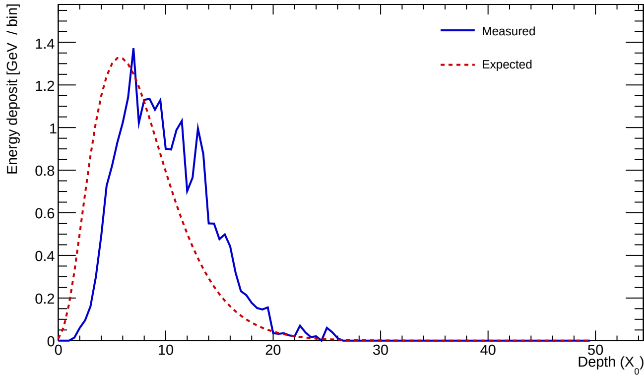
Cluster 733 E=24.107 GeV profileStart=2.00 X_0 \chi=0.1642
