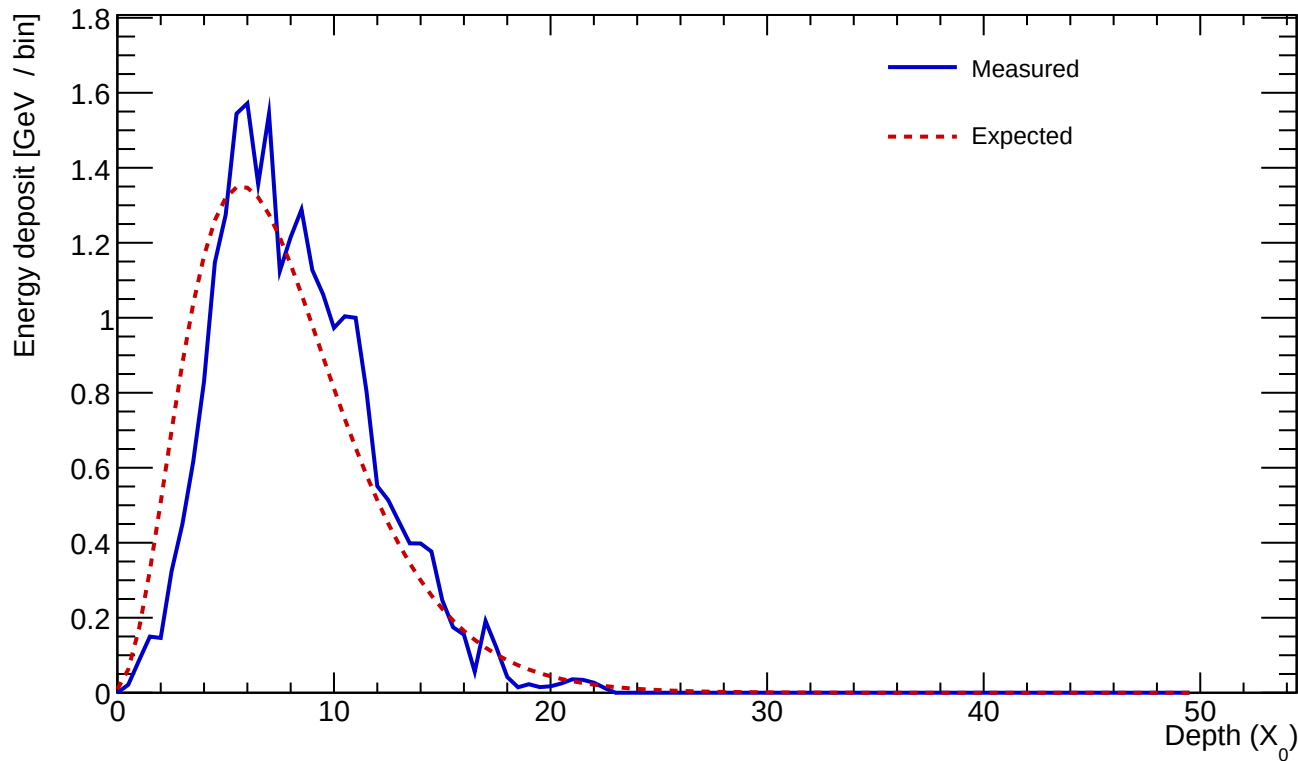
Cluster 873 E=24.544 GeV profileStart=1.00 X_0 \chi=0.1291
