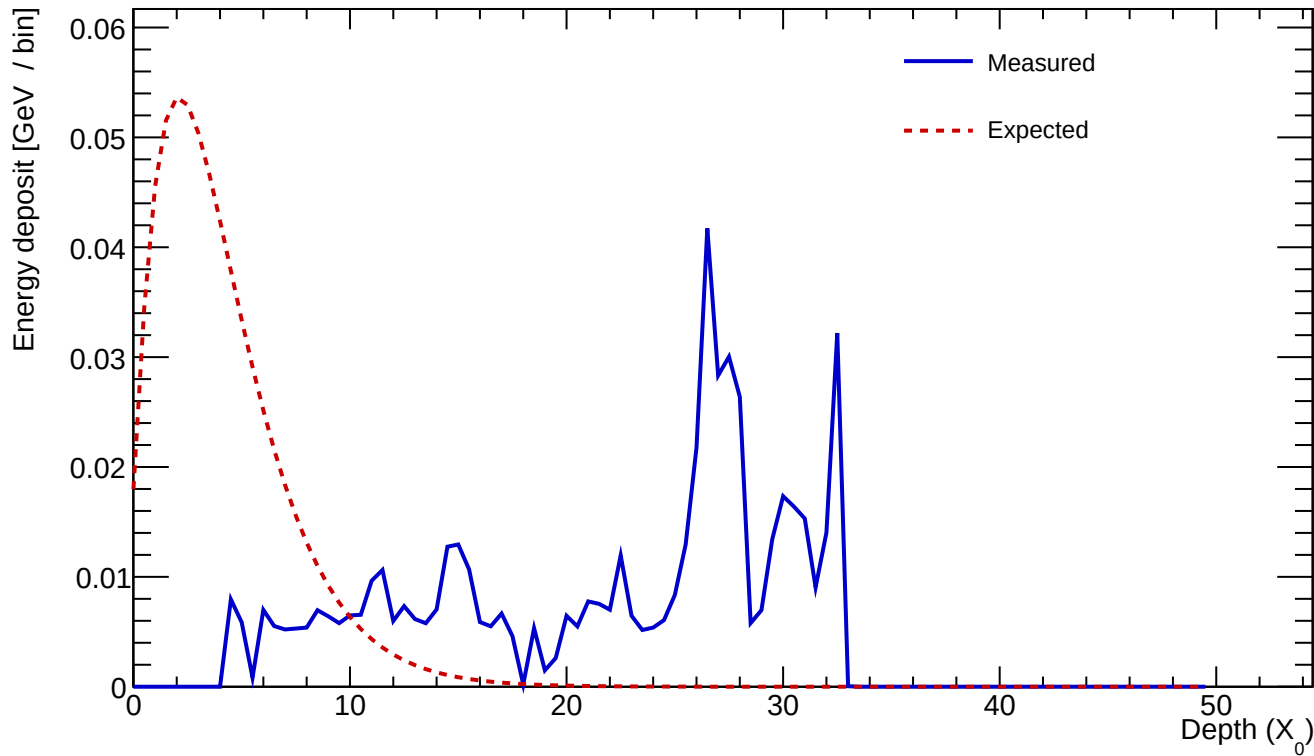
Cluster 172 E=0.654 GeV profileStart=25.50 X_0 \chi=1.0092
