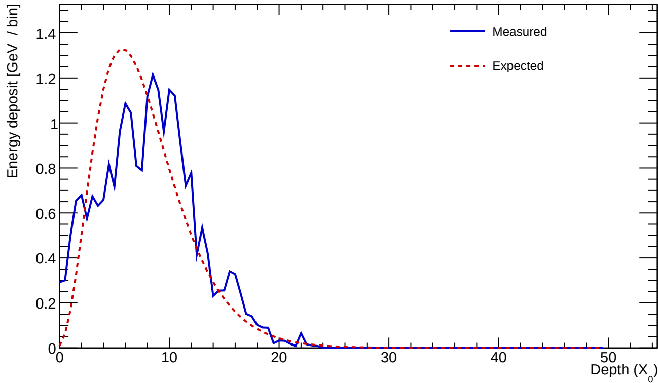
Cluster 462 E=24.124 GeV profileStart=1.00 X_0 \chi=0.3007
