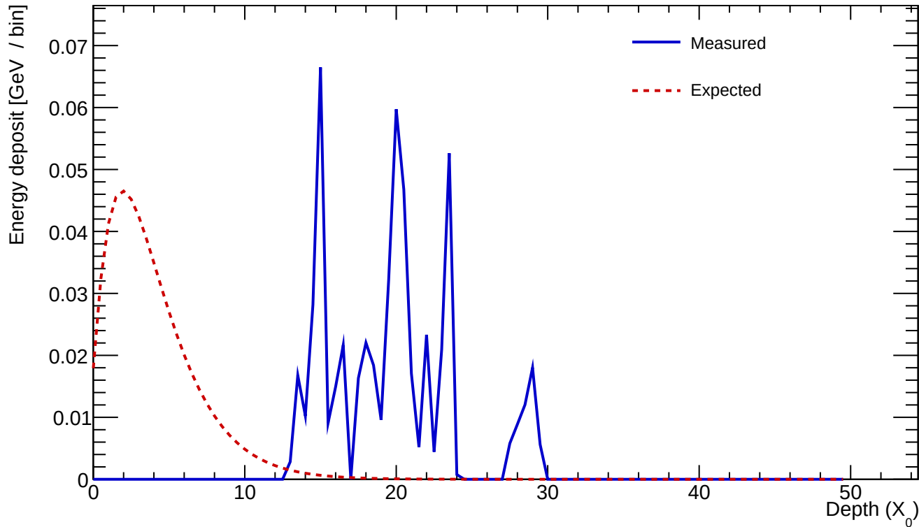
Cluster 125 E=0.550 GeV profileStart=13.50 X_0 \chi=0.8588
