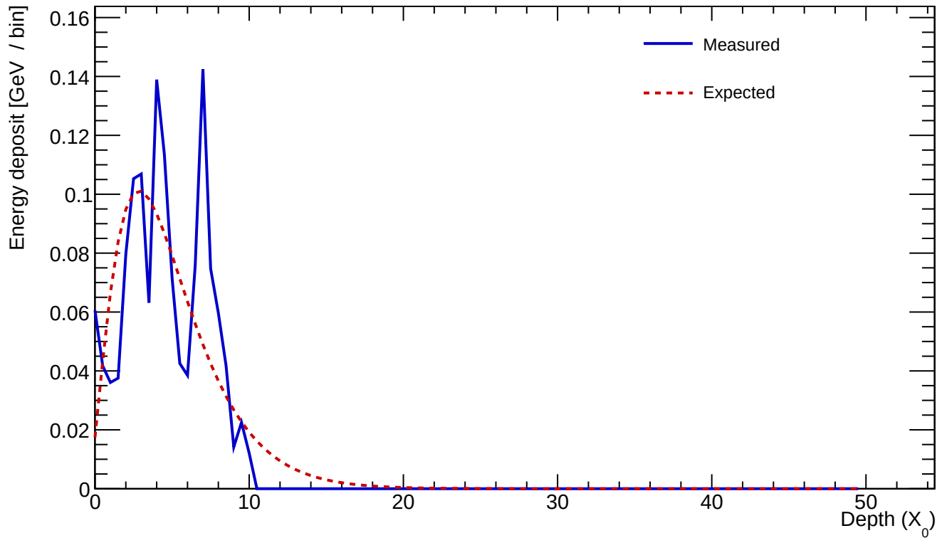
Cluster 420 E=1.379 GeV profileStart=0.50 X_0 \chi=0.3580
