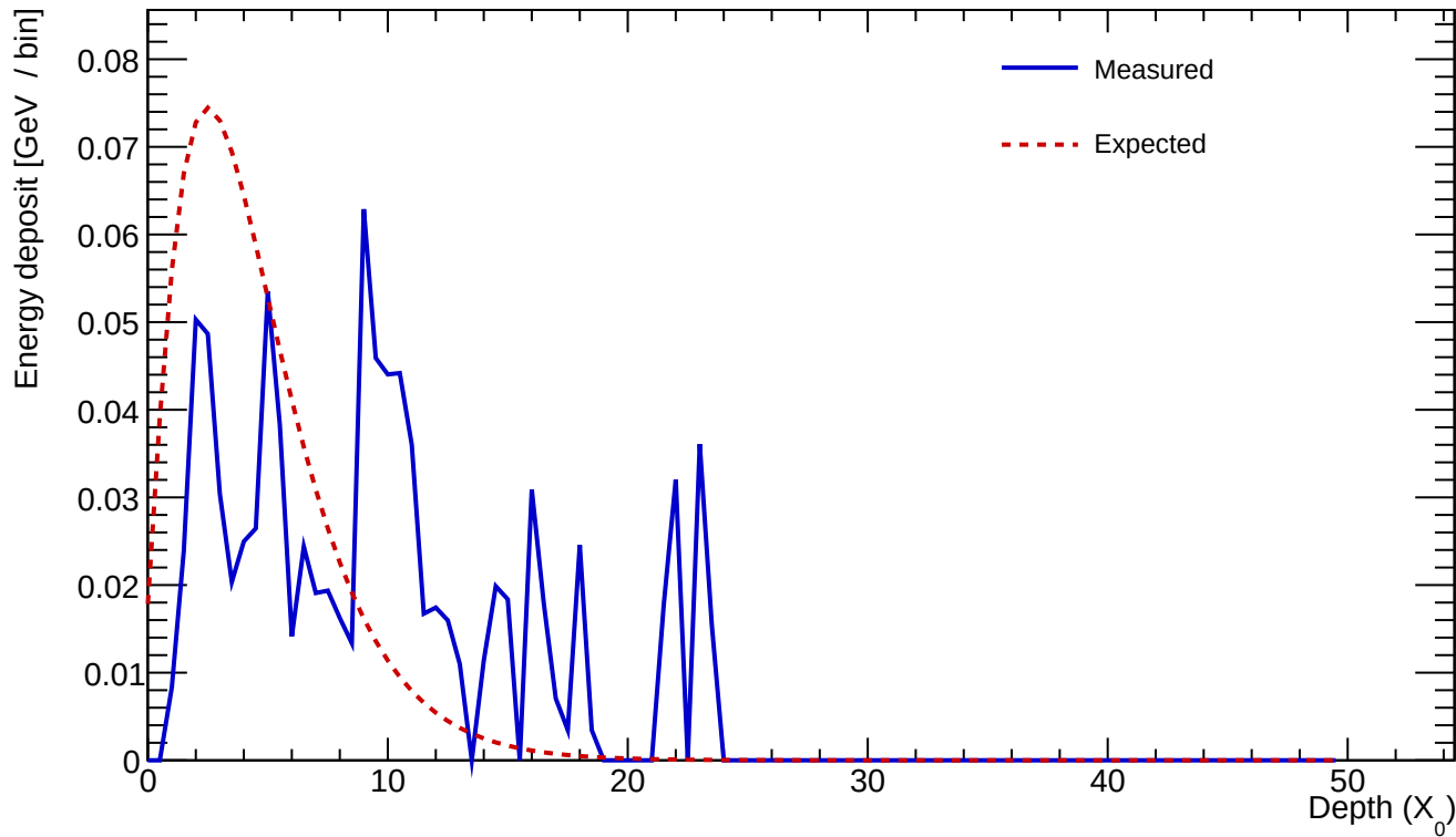
Cluster 545 E=0.964 GeV profileStart=4.00 X_0 \chi=0.8170
