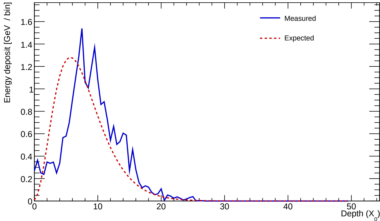
Cluster 318 E=23.171 GeV profileStart=2.00 X_0 \chi=0.2525
