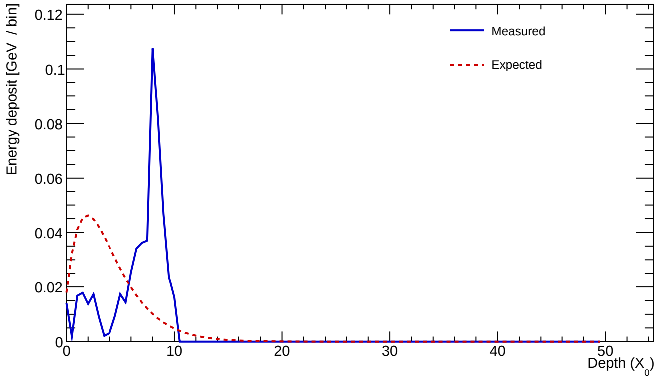
Cluster 483 E=0.545 GeV profileStart=6.00 X_0 \chi=0.5075
