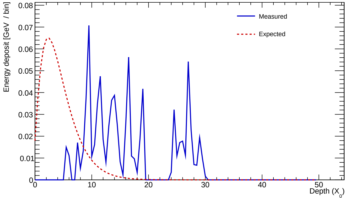
Cluster 942 E=0.822 GeV profileStart=7.50 X_0 \chi=0.8727
