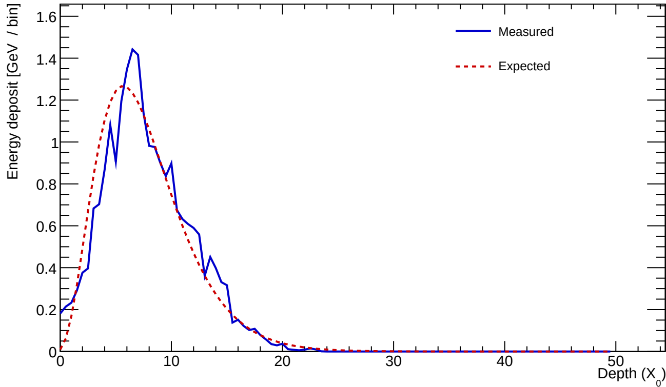
Cluster 10 E=22.907 GeV profileStart=0.50 X_0 \chi=0.1476
