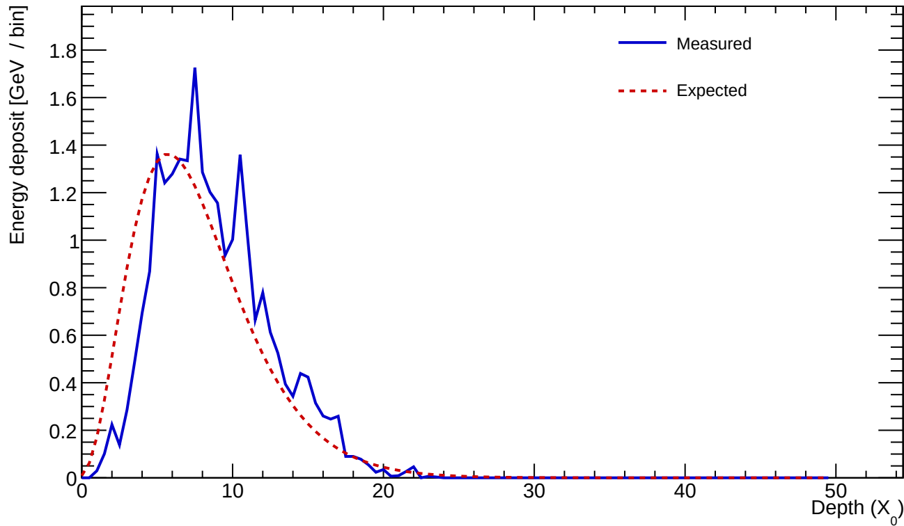
Cluster 290 E=24.792 GeV profileStart=1.50 X_0 \chi=0.1385
