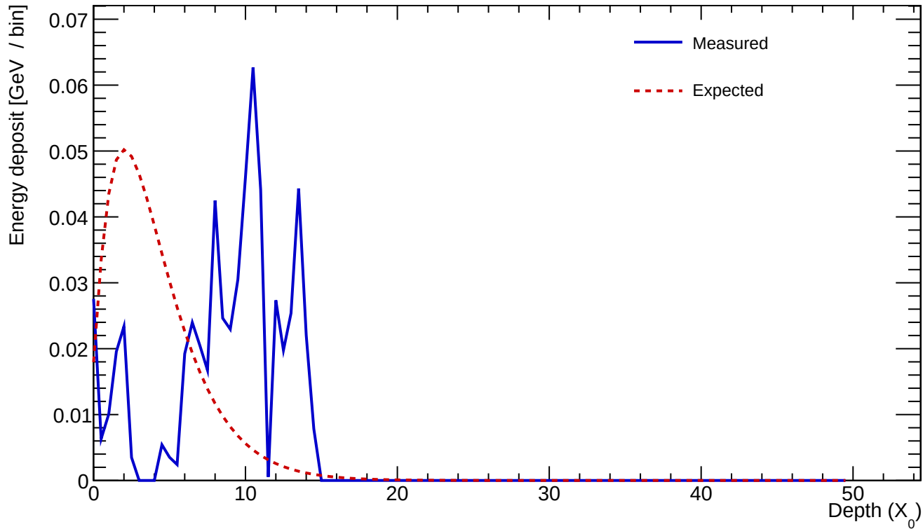
Cluster 933 E=0.603 GeV profileStart=7.00 X_0 \chi=0.5599
