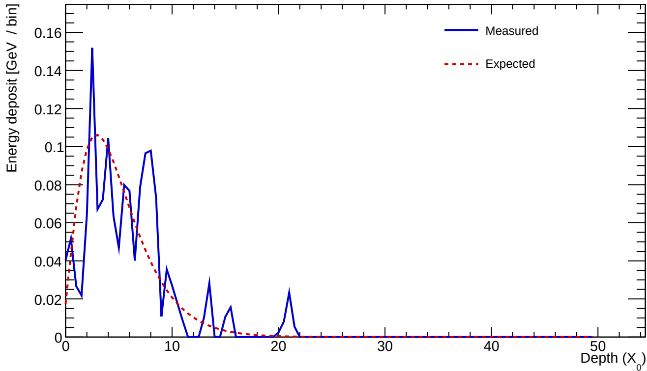
Cluster 313 E=1.458 GeV profileStart=1.00 X_0 \chi=0.4933
