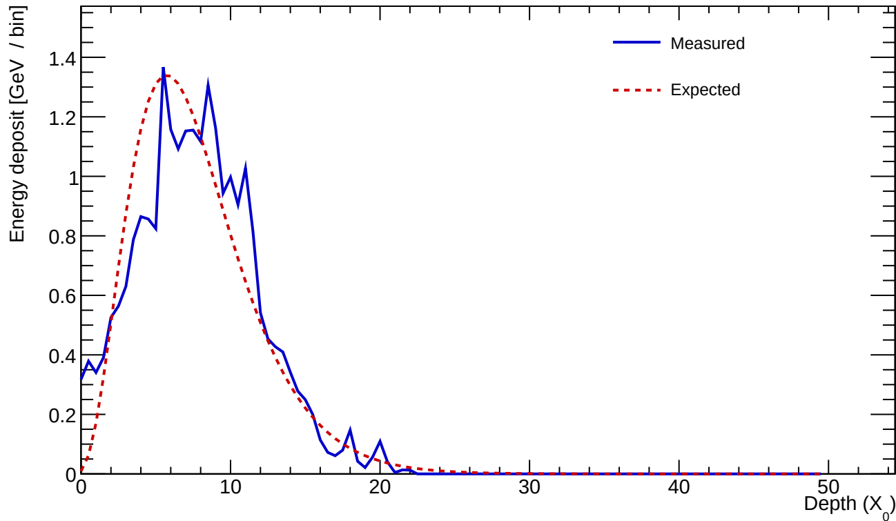
Cluster 799 E=24.352 GeV profileStart=0.50 X_0 \chi=0.2068
