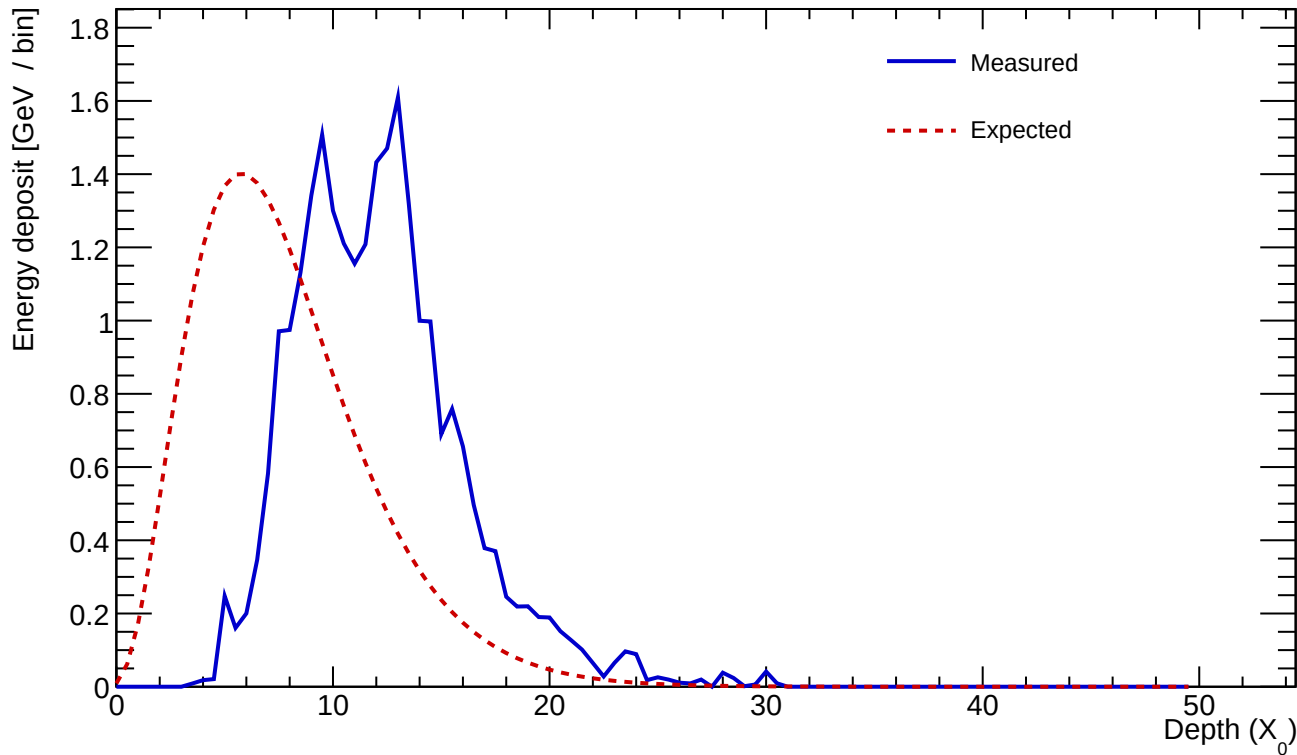
Cluster 151 E=25.577 GeV profileStart=4.50 X_0 \chi=0.1684
