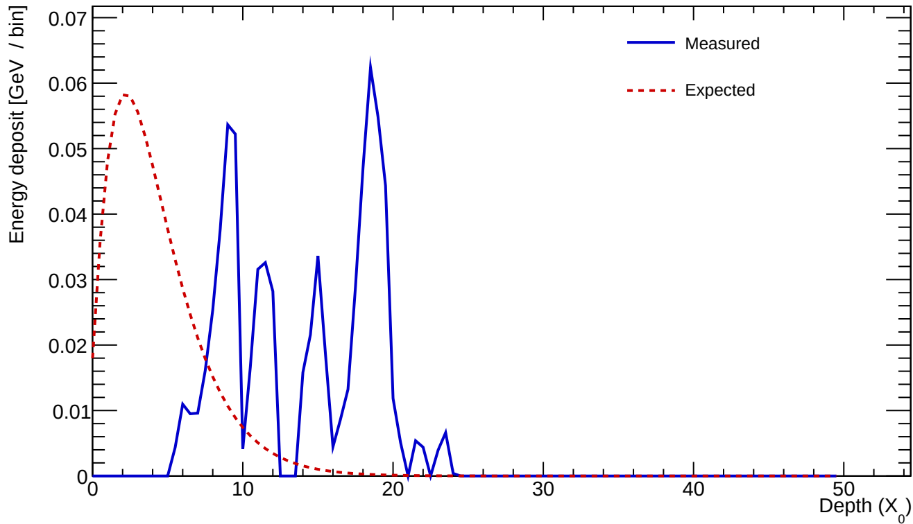
Cluster 796 E=0.724 GeV profileStart=7.50 X_0 \chi=0.8173
