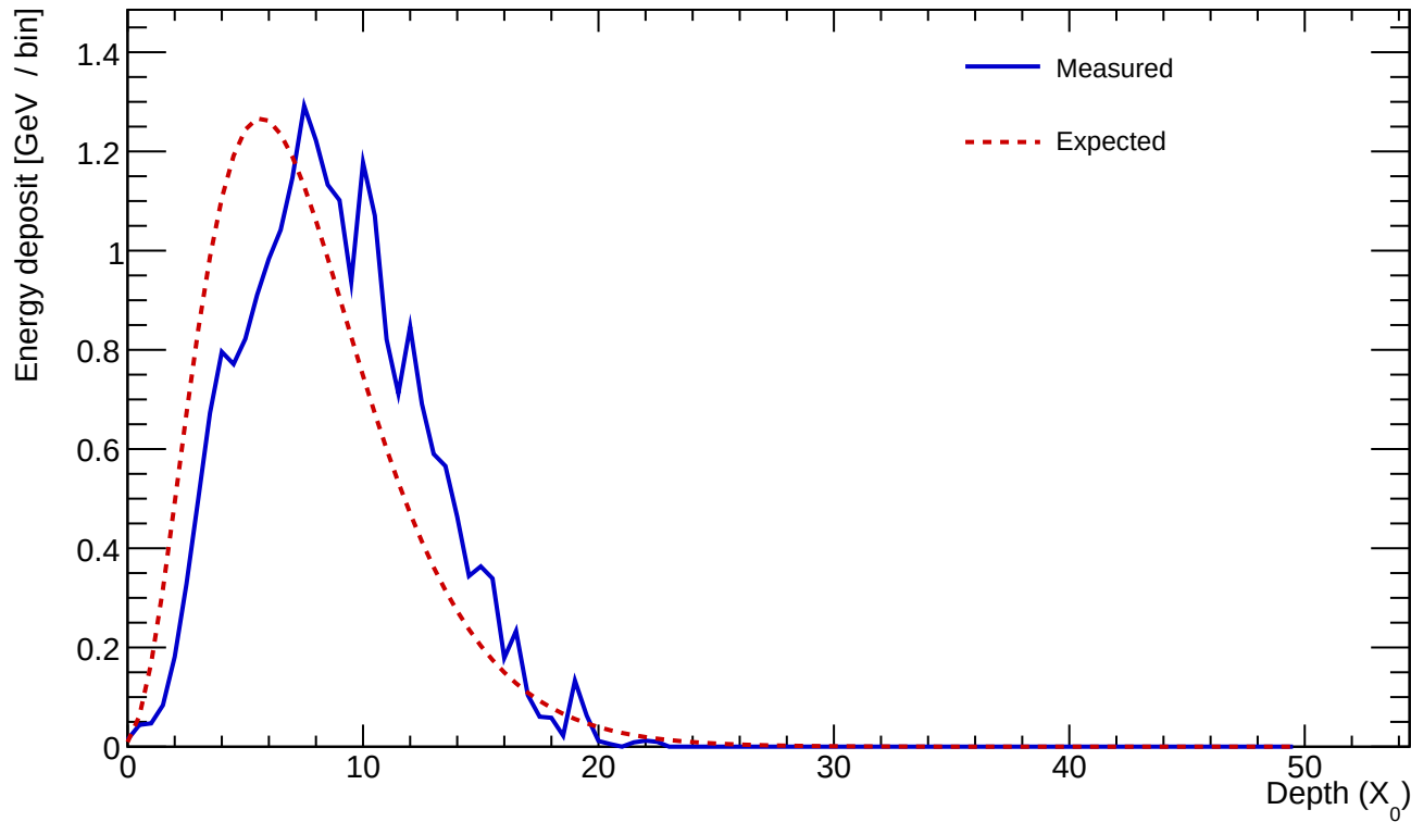
Cluster 907 E=22.913 GeV profileStart=1.50 X_0 \chi=0.1666
