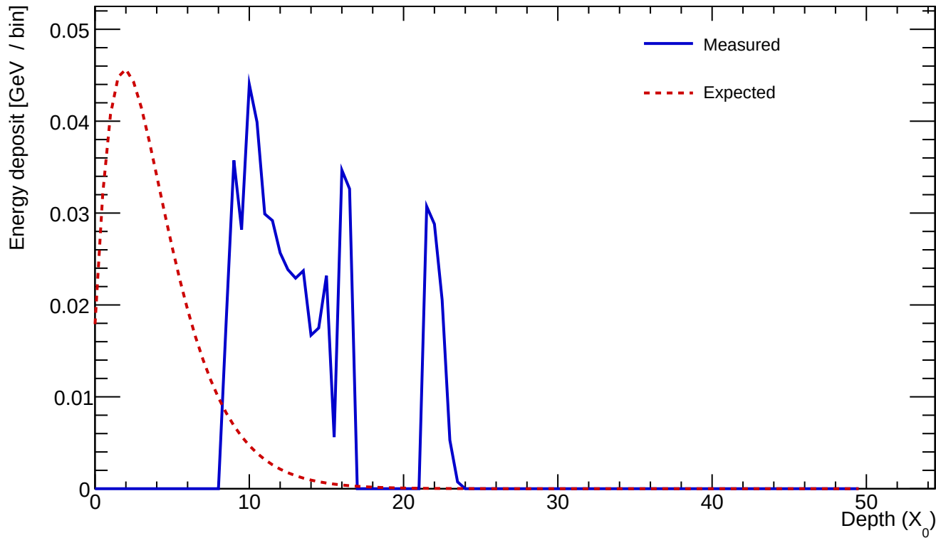
Cluster 108 E=0.538 GeV profileStart=8.50 X_0 \chi=0.5032
