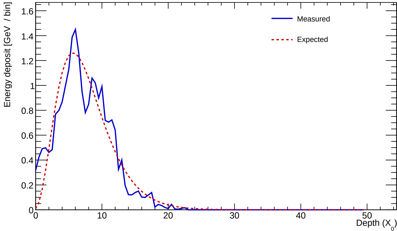
Cluster 349 E=22.796 GeV profileStart=0.50 X_0 \chi=0.2243
