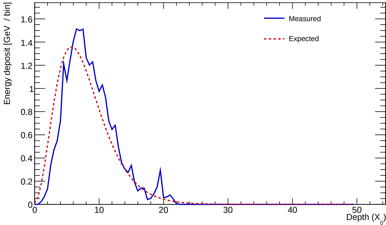
Cluster 639 E=24.738 GeV profileStart=1.00 X_0 \chi=0.1180
