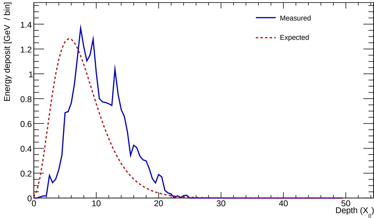
Cluster 941 E=23.220 GeV profileStart=3.00 X_0 \chi=0.1857
