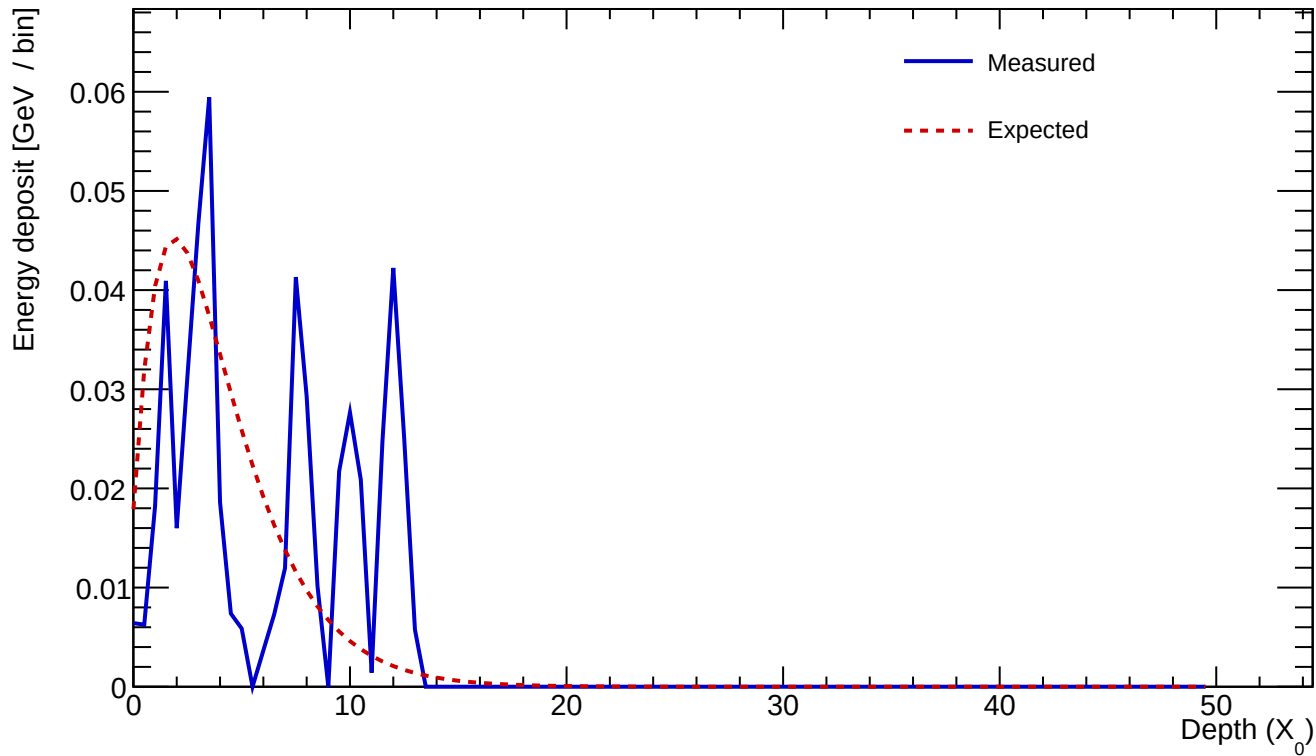
Cluster 533 E=0.531 GeV profileStart=1.00 X_0 \chi=0.7881
