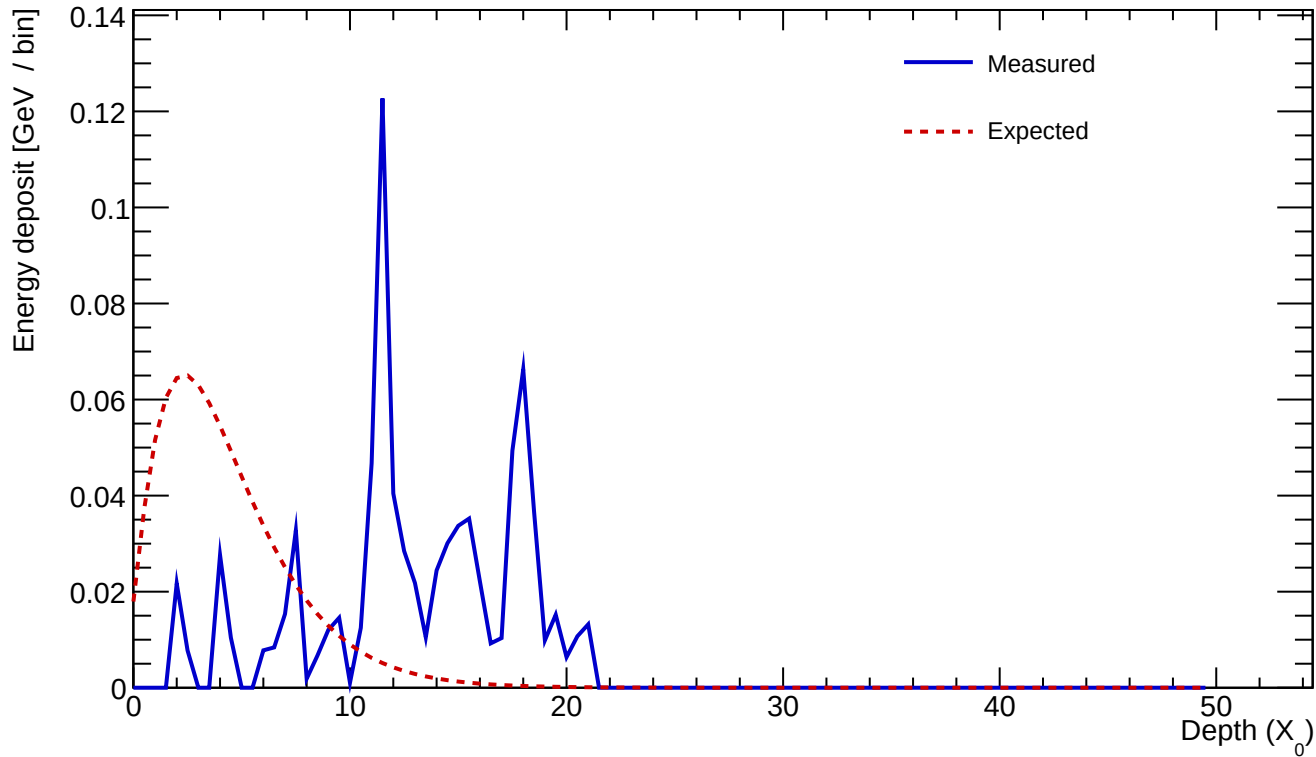
Cluster 283 E=0.824 GeV profileStart=9.50 X_0 \chi=0.7785
