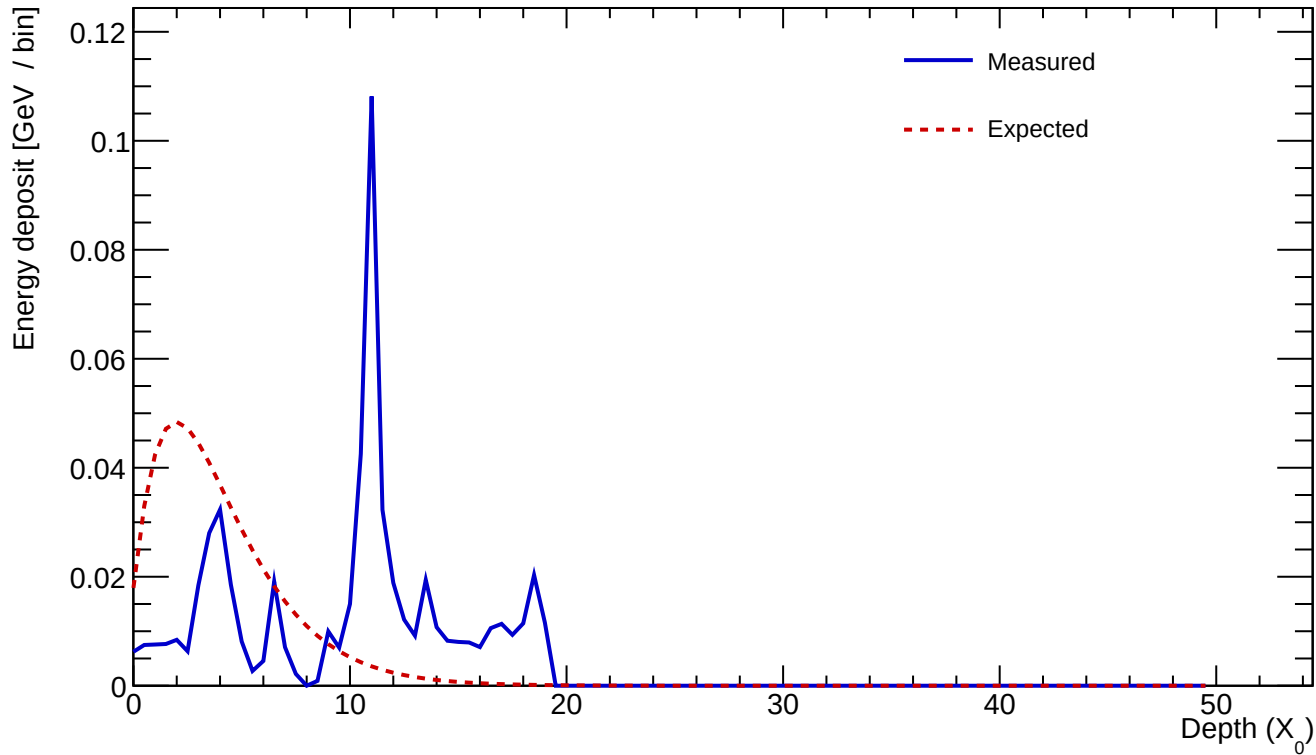
Cluster 740 E=0.577 GeV profileStart=9.00 X_0 \chi=0.8825
