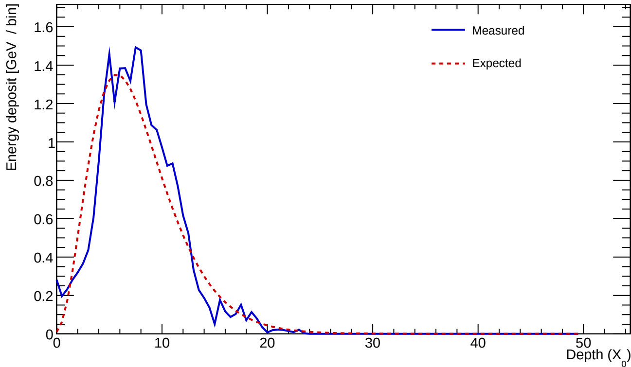
Cluster 930 E=24.552 GeV profileStart=1.00 X_0 \chi=0.1775
