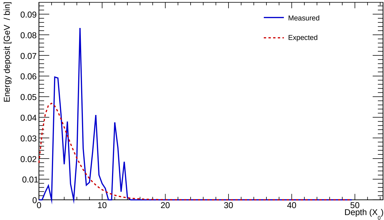
Cluster 291 E=0.554 GeV profileStart=1.50 X_0 \chi=0.7210
