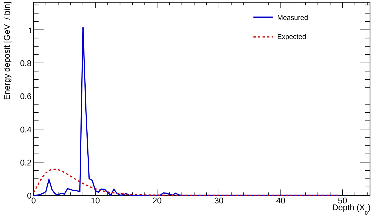
Cluster 1207 E=2.298 GeV profileStart=4.50 X_0 \chi=1.2252
