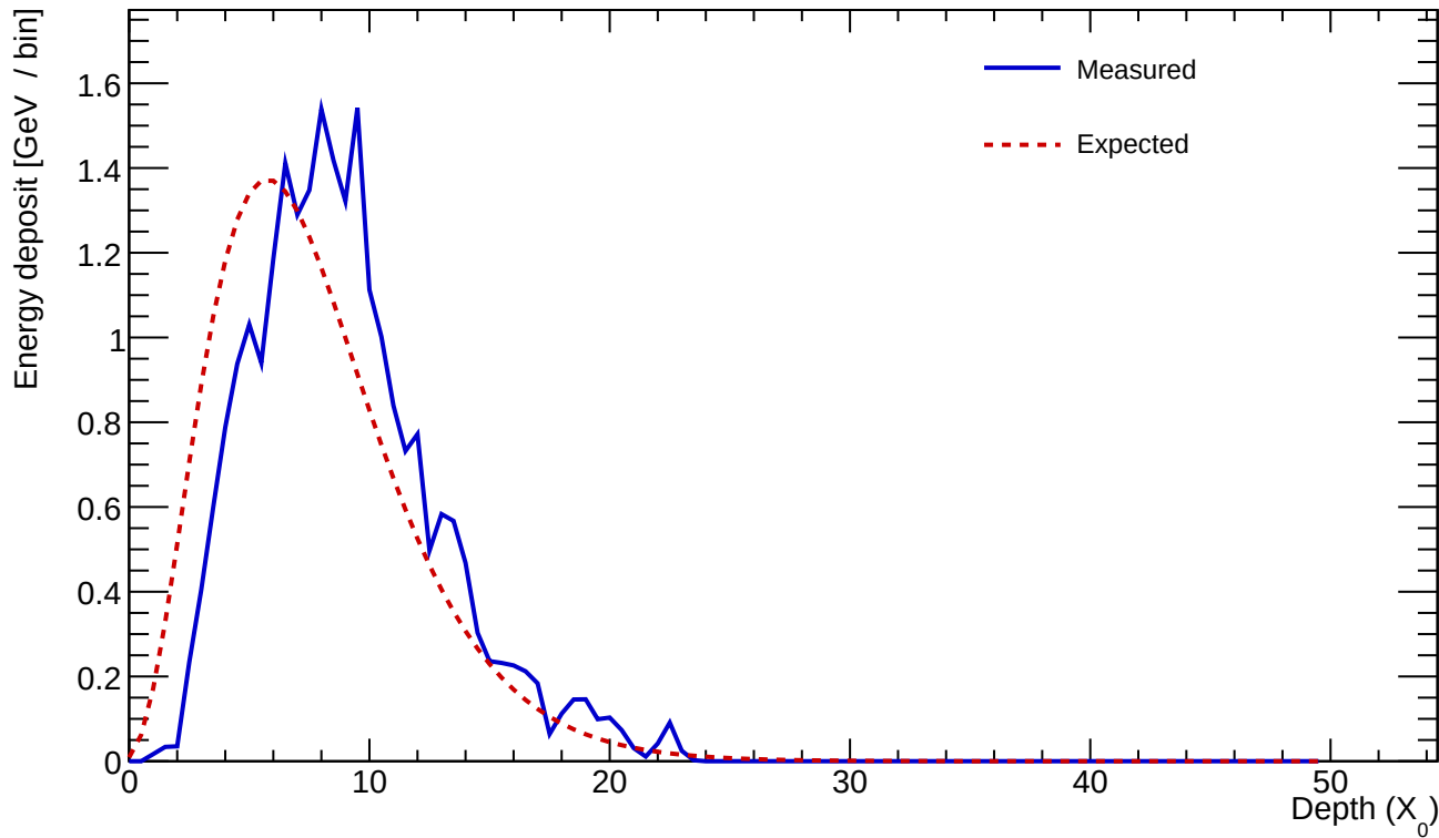
Cluster 832 E=24.986 GeV profileStart=1.50 X_0 \chi=0.1168
