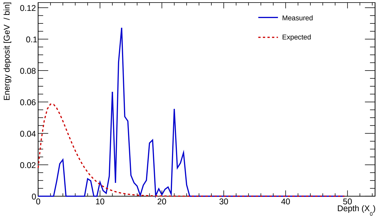
Cluster 521 E=0.730 GeV profileStart=11.00 X_0 \chi=0.8664
