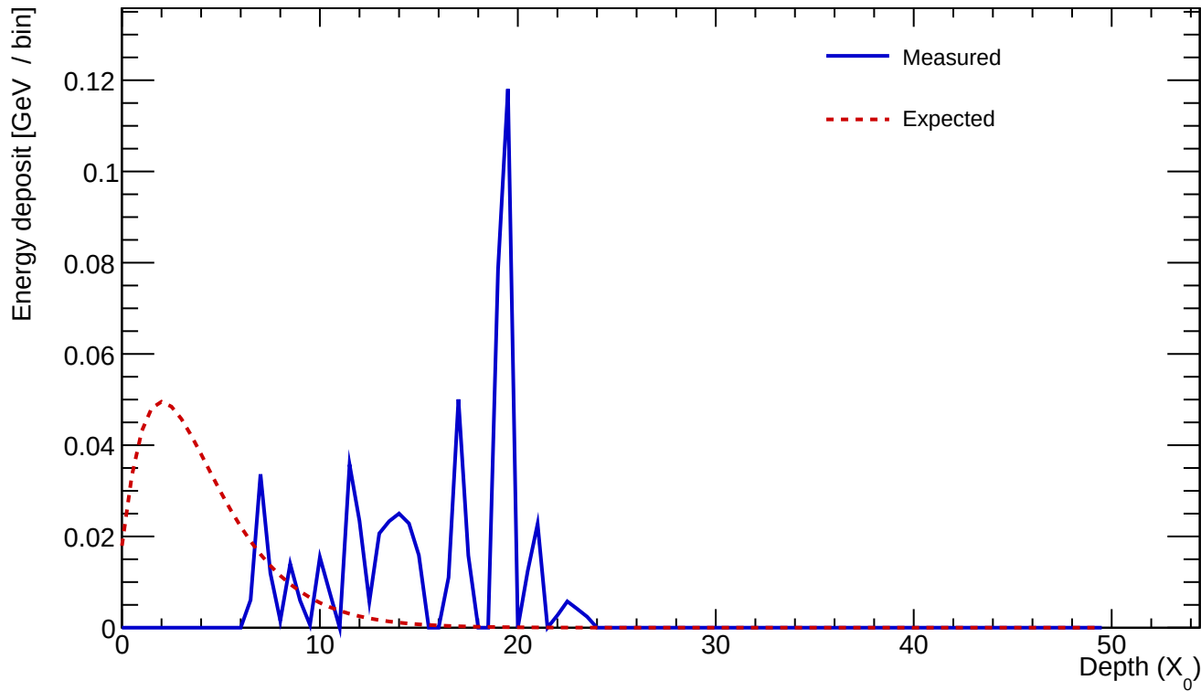
Cluster 939 E=0.593 GeV profileStart=10.00 X_0 \chi=1.0870
