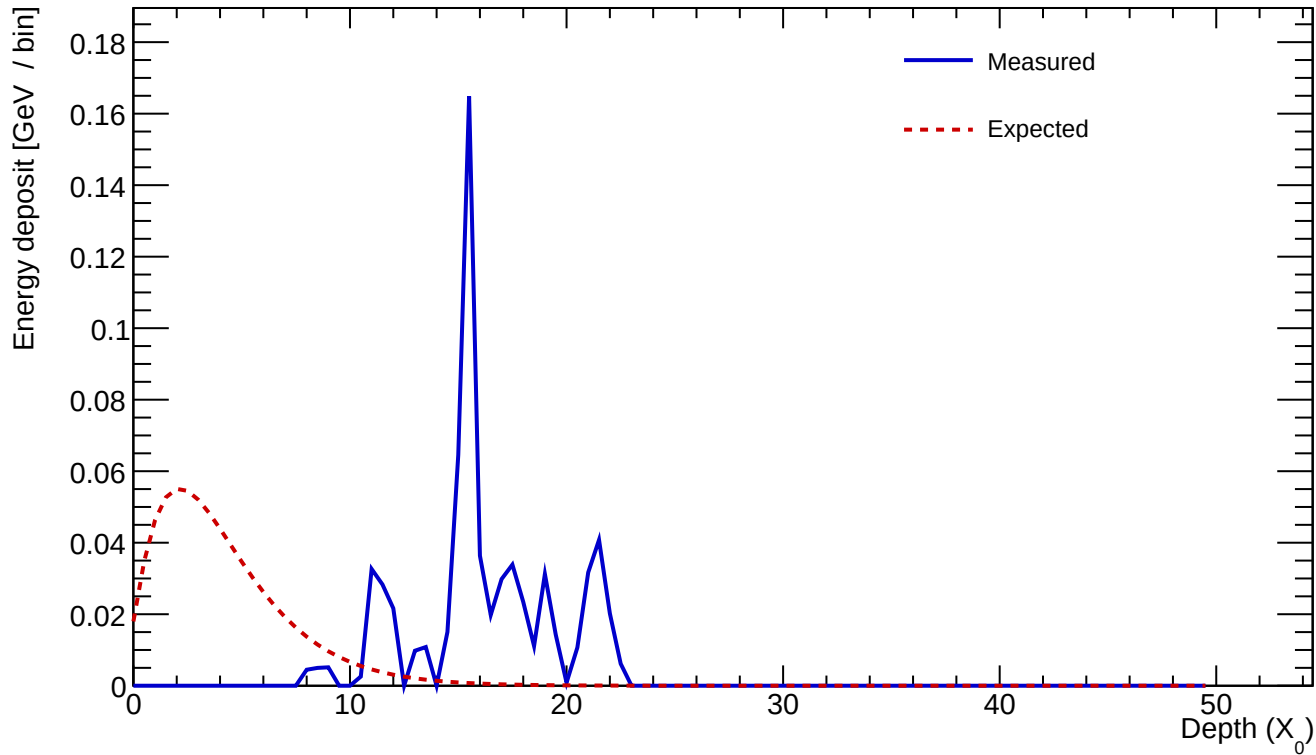
Cluster 16 E=0.675 GeV profileStart=13.50 X_0 \chi=0.7657
