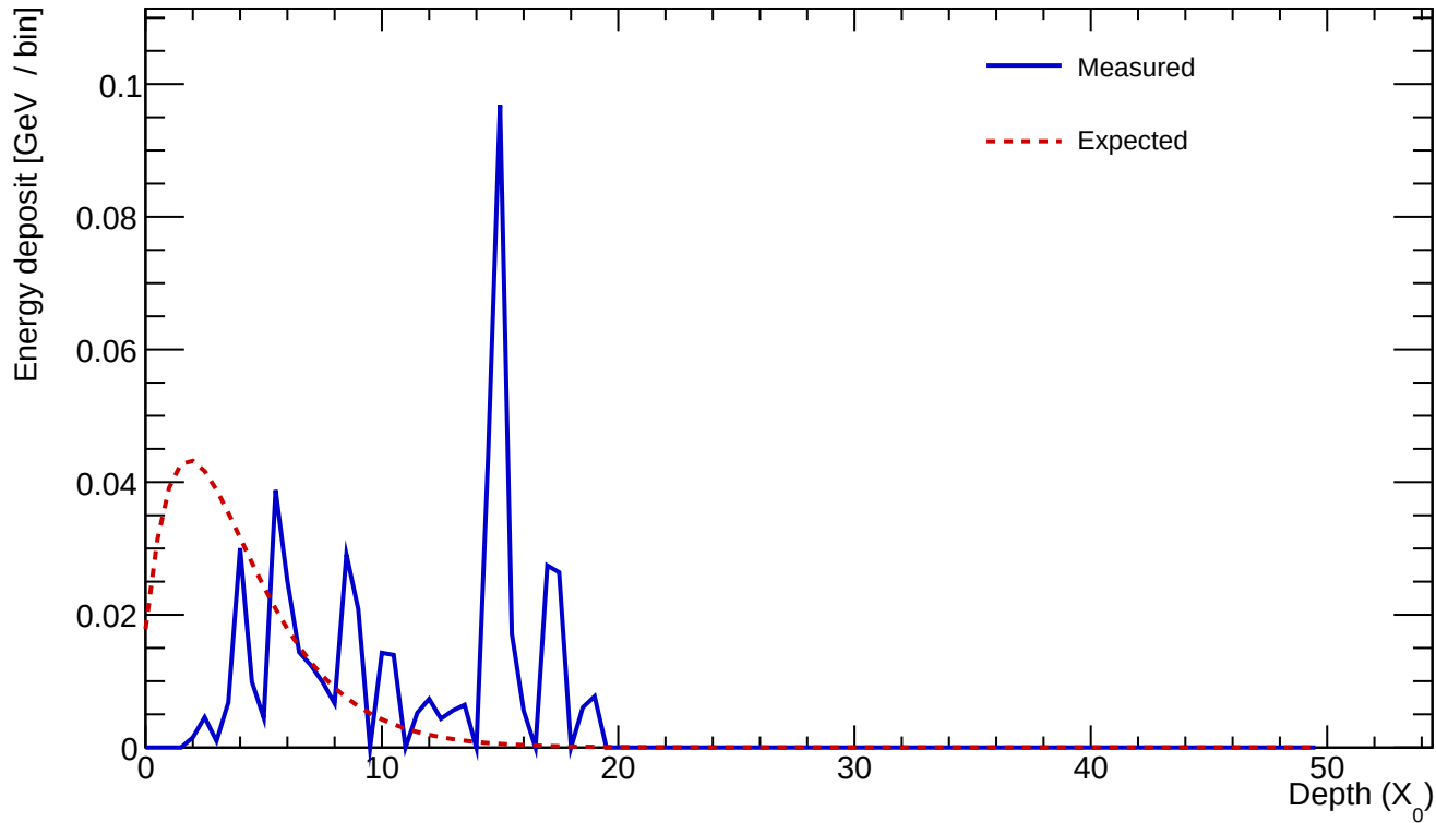
Cluster 449 E=0.504 GeV profileStart=3.50 X_0 \chi=0.9140
