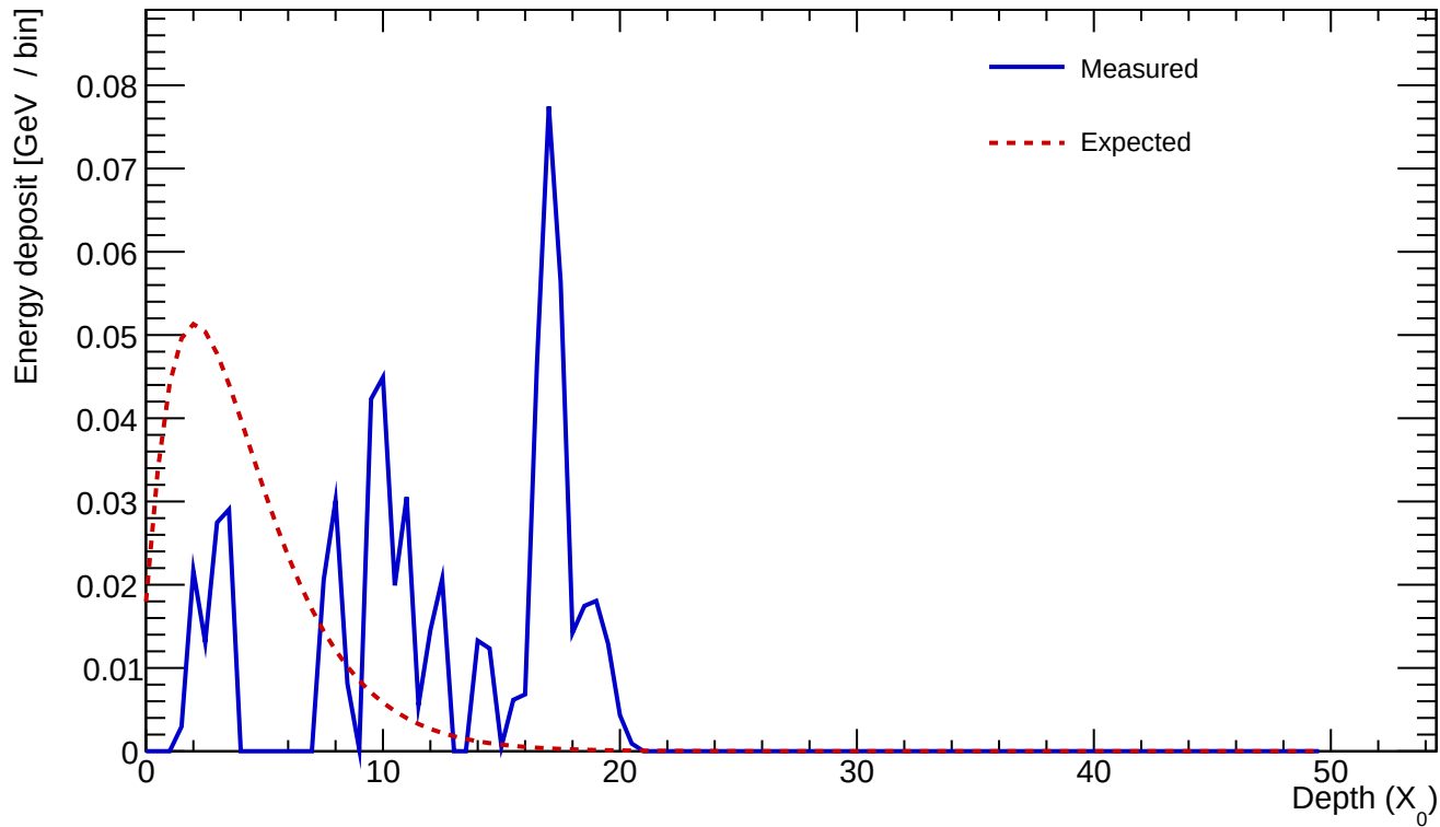
Cluster 87 E=0.619 GeV profileStart=7.50 X_0 \chi=0.9723
