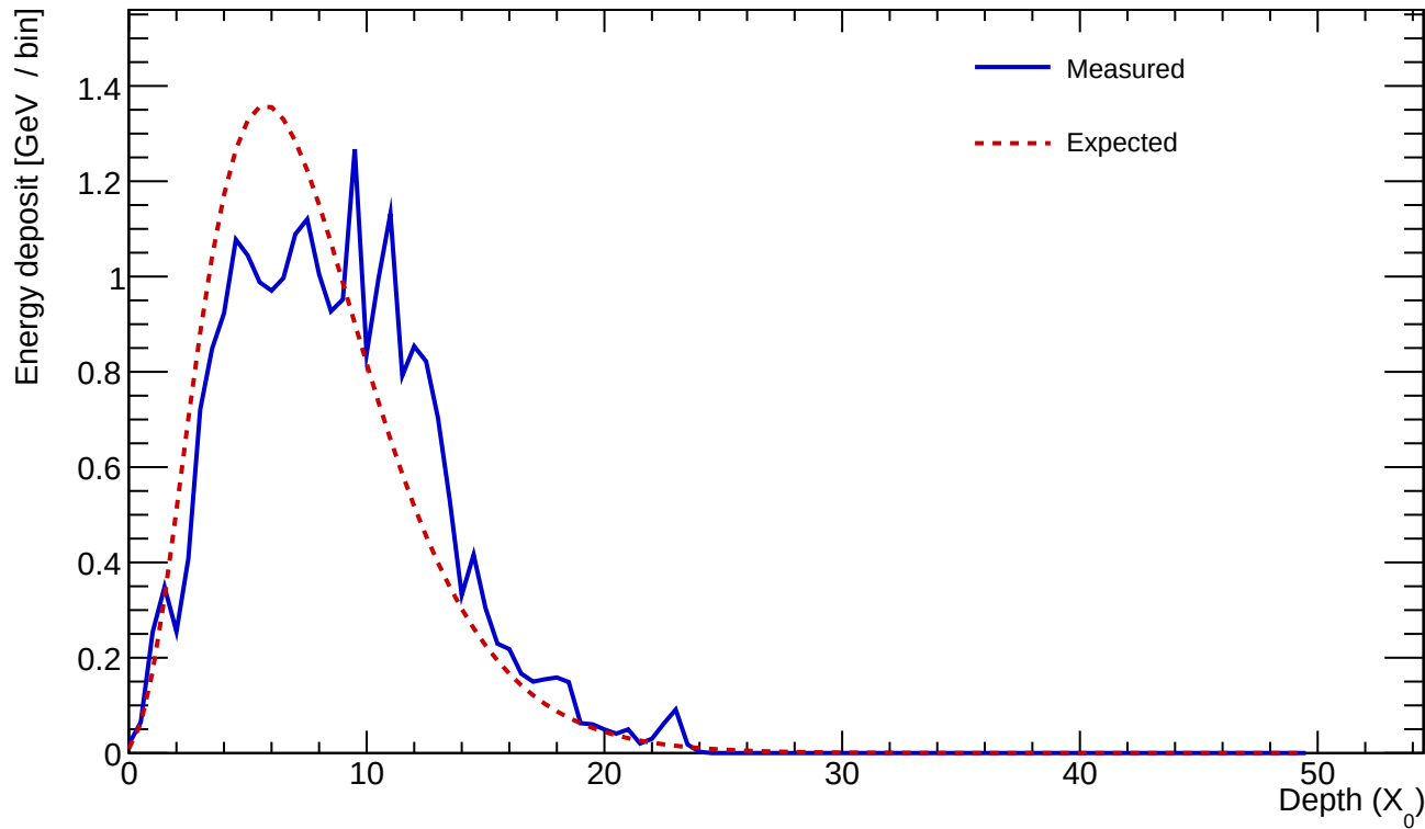
Cluster 386 E=24.710 GeV profileStart=1.00 X_0 \chi=0.2265
