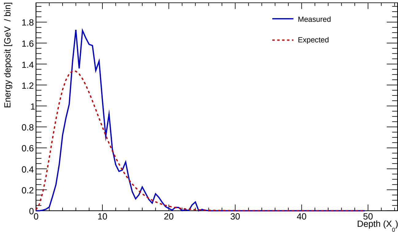
Cluster 719 E=24.241 GeV profileStart=1.50 X_0 \chi=0.2262
