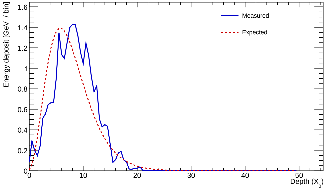
Cluster 80 E=25.350 GeV profileStart=1.50 X_0 \chi=0.2016
