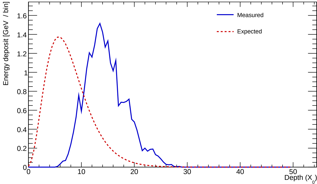
Cluster 975 E=25.008 GeV profileStart=7.00 X_0 \chi=0.1356
