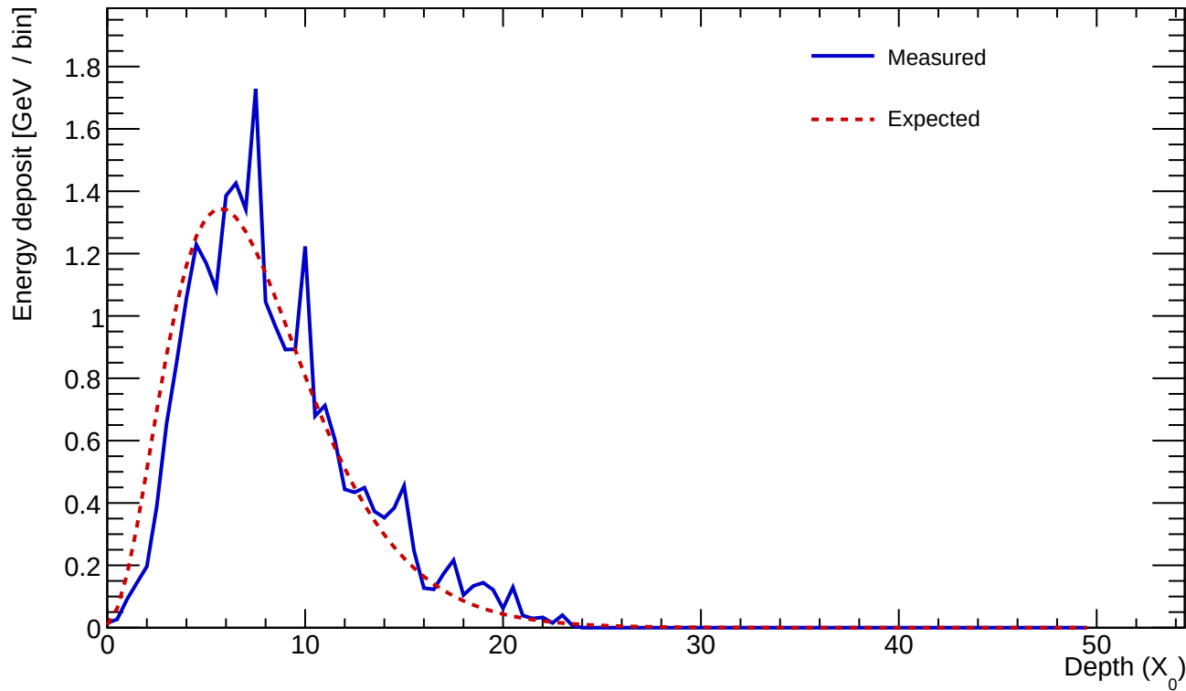
Cluster 431 E=24.443 GeV profileStart=0.50 X_0 \chi=0.1483
