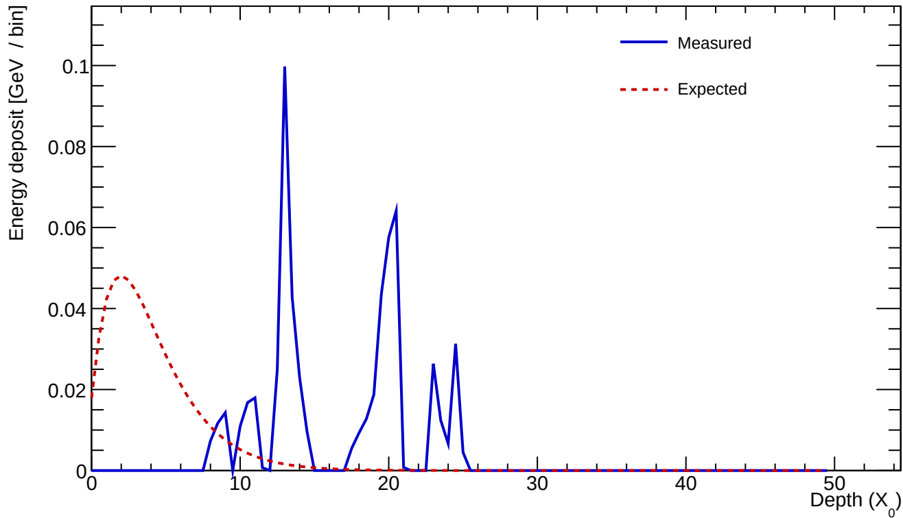
Cluster 615 E=0.573 GeV profileStart=10.50 X_0 \chi=1.1339
