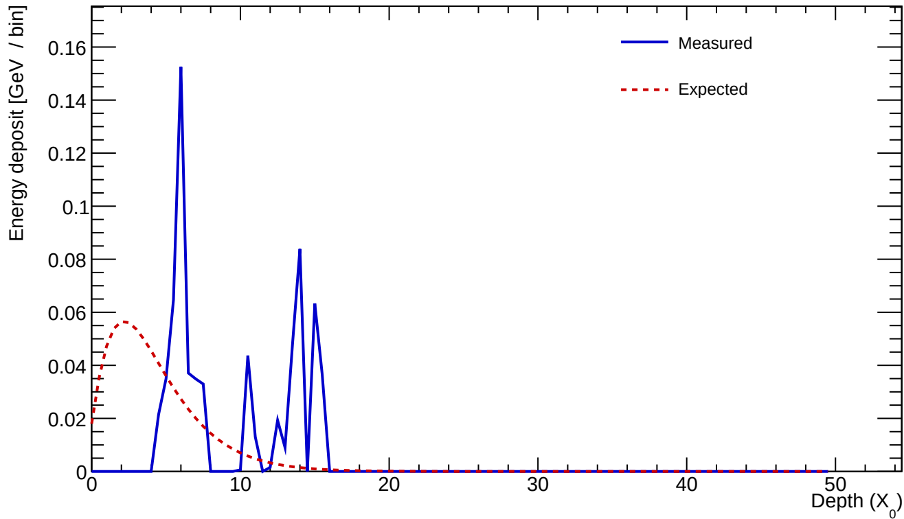
Cluster 715 E=0.697 GeV profileStart=4.00 X_0 \chi=0.9068
