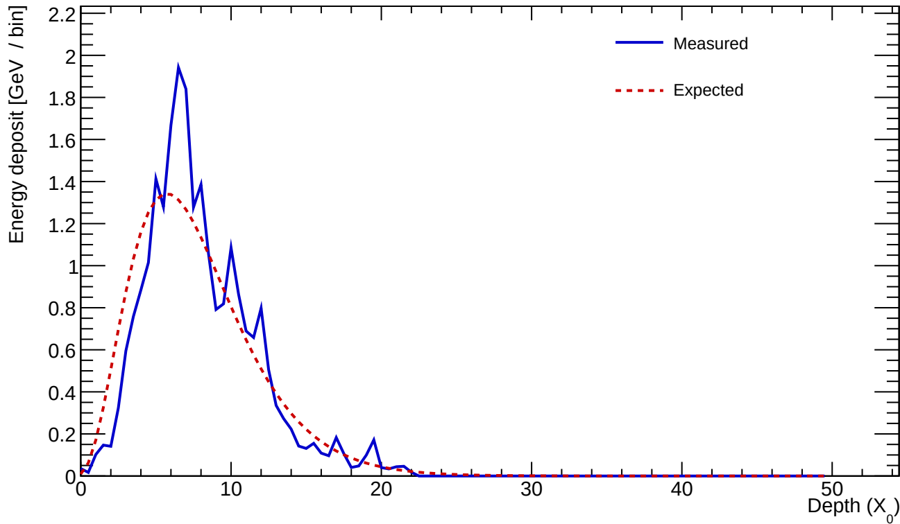
Cluster 922 E=24.385 GeV profileStart=0.50 X_0 \chi=0.2064
