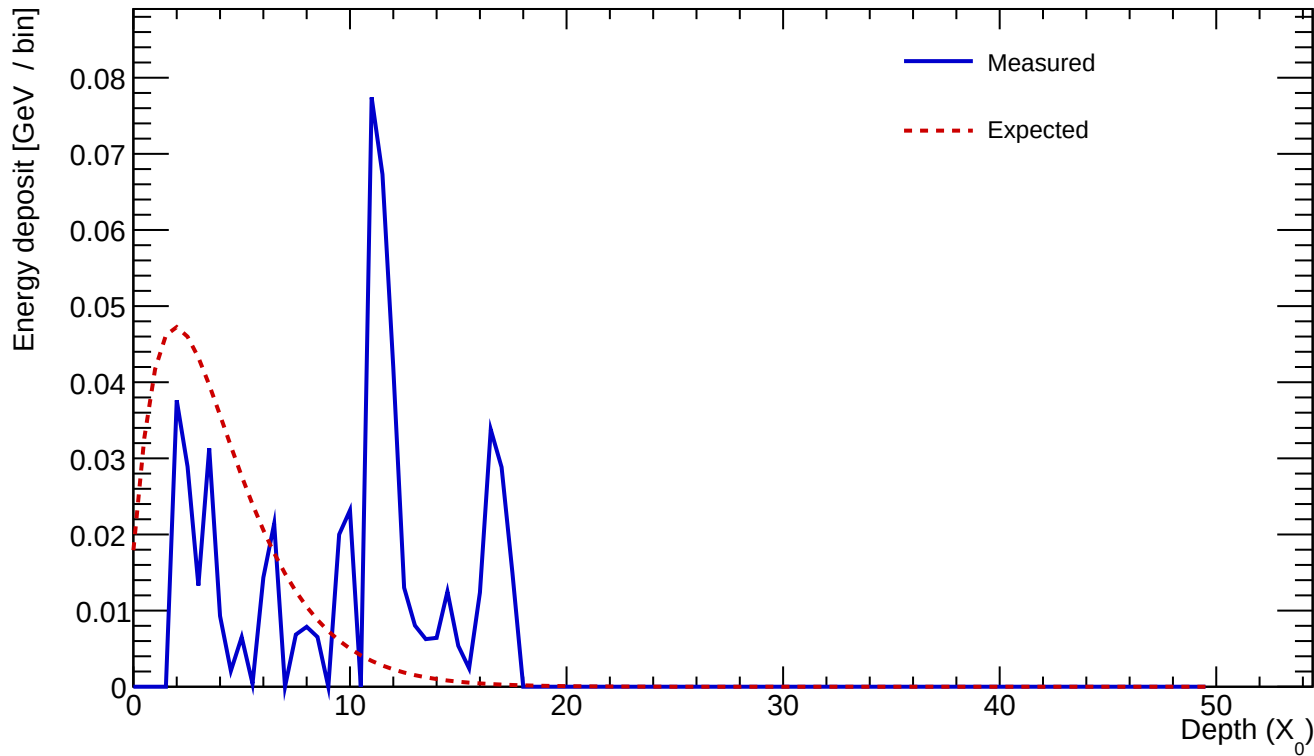
Cluster 1142 E=0.560 GeV profileStart=9.50 X_0 \chi=0.8992
