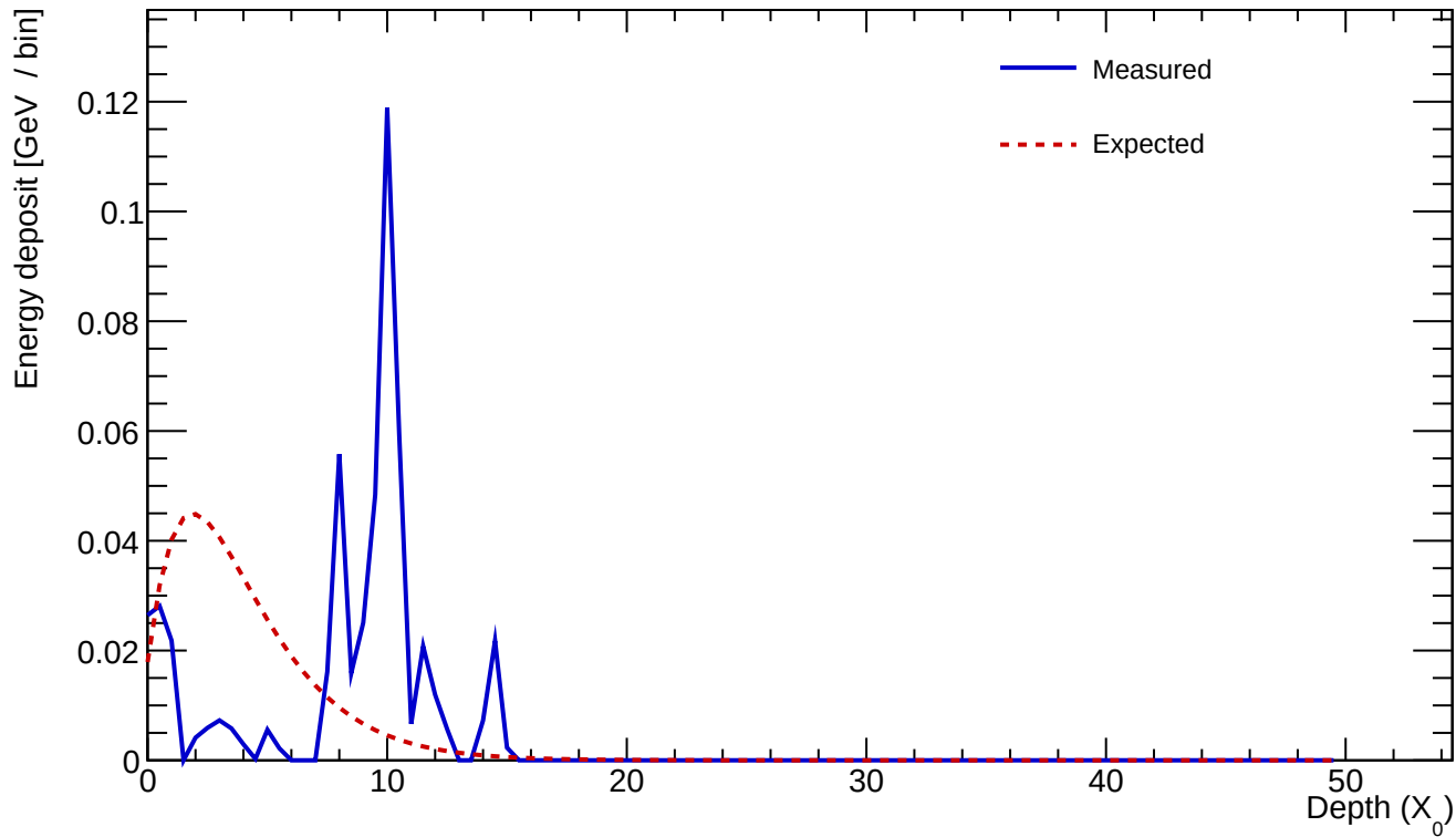
Cluster 78 E=0.527 GeV profileStart=7.50 X_0 \chi=0.7896
