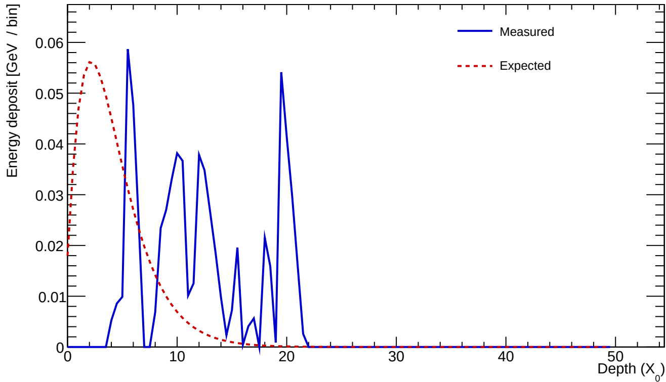
Cluster 609 E=0.691 GeV profileStart=5.00 X_0 \chi=0.8355
