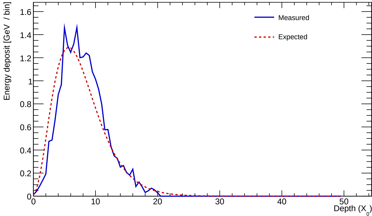
Cluster 292 E=23.340 GeV profileStart=1.00 X_0 \chi=0.1224
