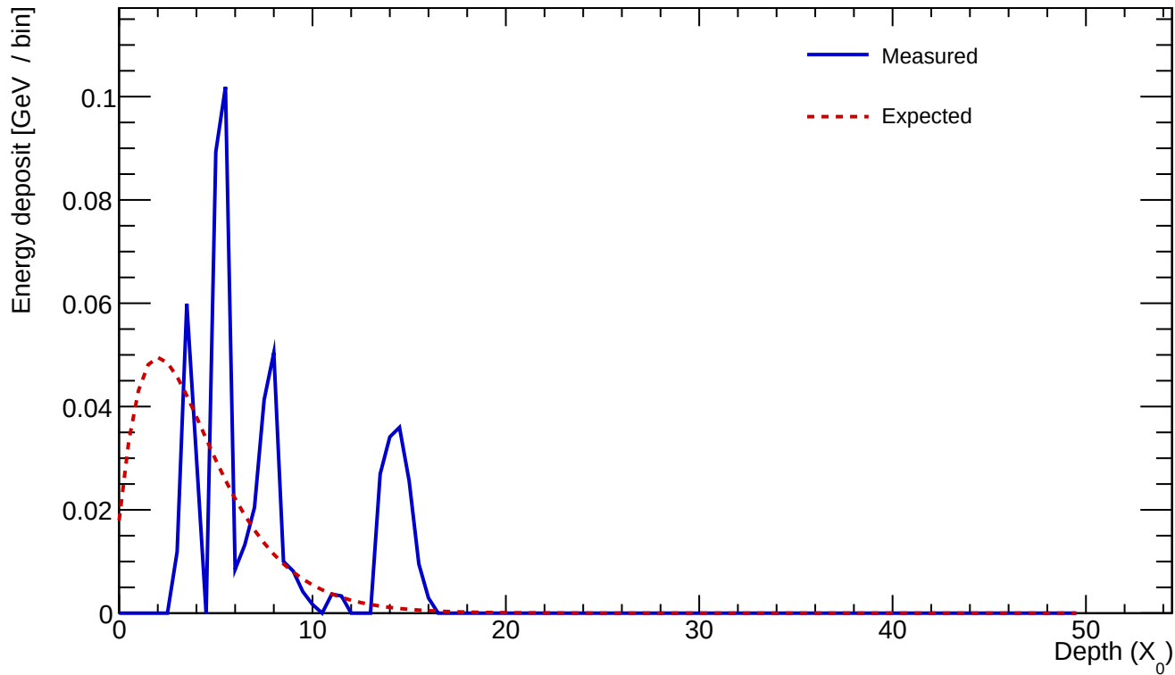
Cluster 892 E=0.593 GeV profileStart=3.00 X_0 \chi=0.8798
