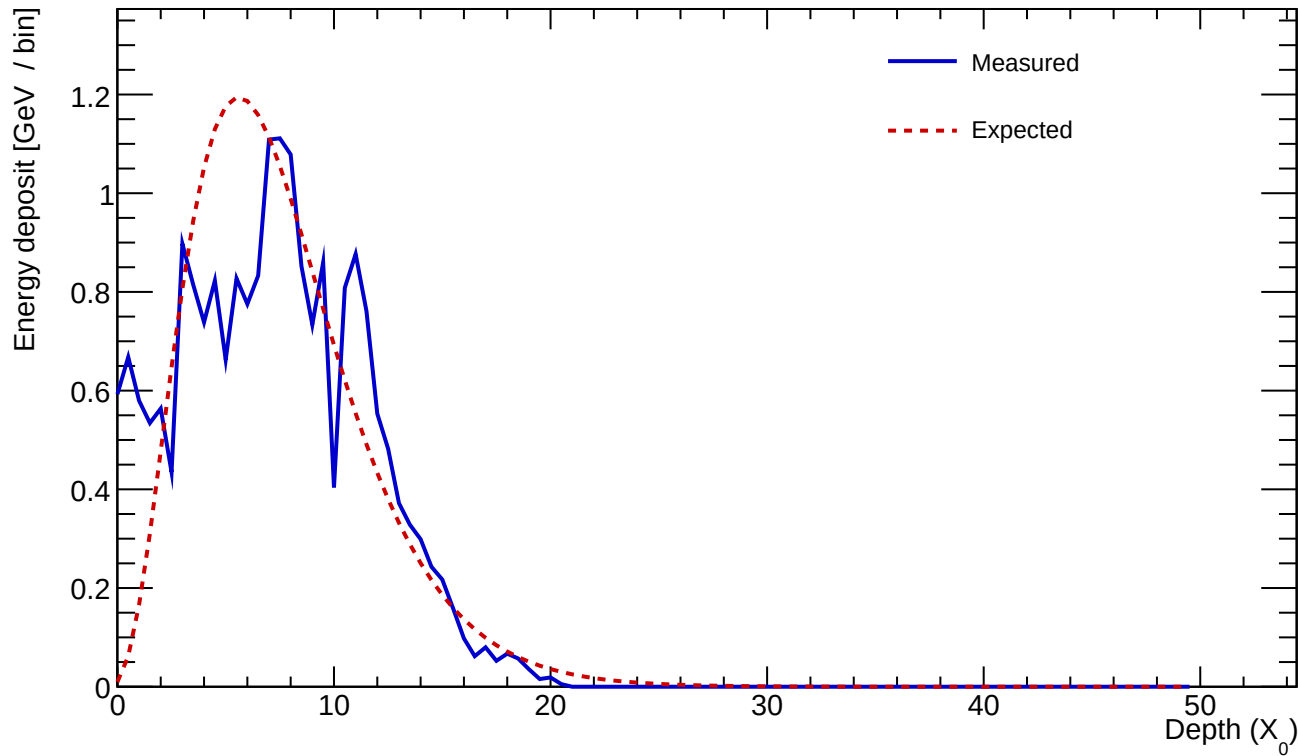
Cluster 864 E=21.484 GeV profileStart=0.50 X_0 \chi=0.3058
