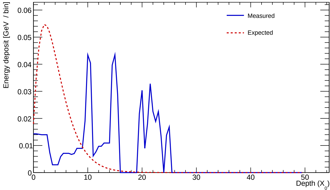
Cluster 60 E=0.669 GeV profileStart=9.00 X_0 \chi=1.1257
