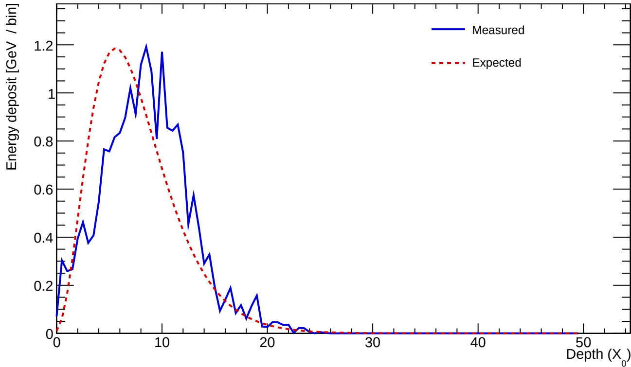
Cluster 1138 E=21.299 GeV profileStart=1.50 X_0 \chi=0.2438
