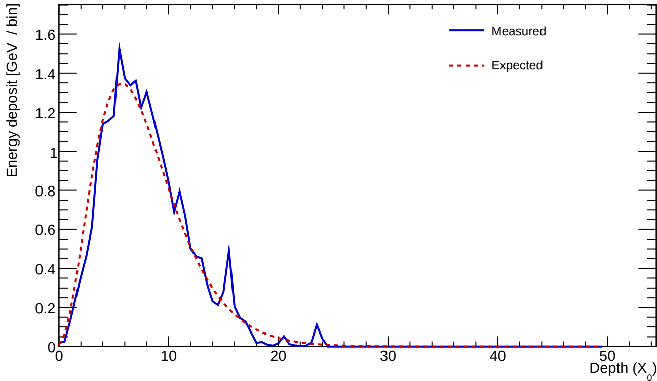
Cluster 612 E=24.468 GeV profileStart=0.50 X_0 \chi=0.1083
