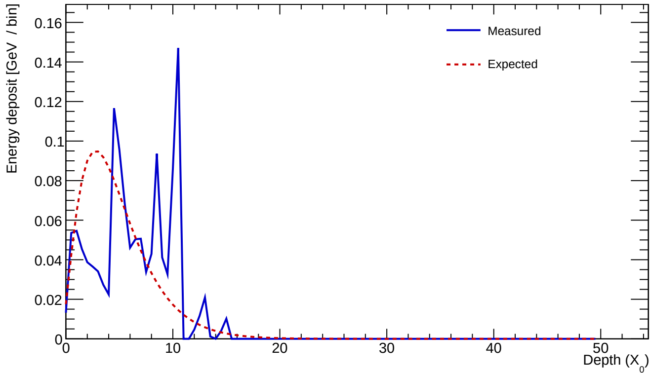
Cluster 527 E=1.283 GeV profileStart=0.50 X_0 \chi=0.6243
