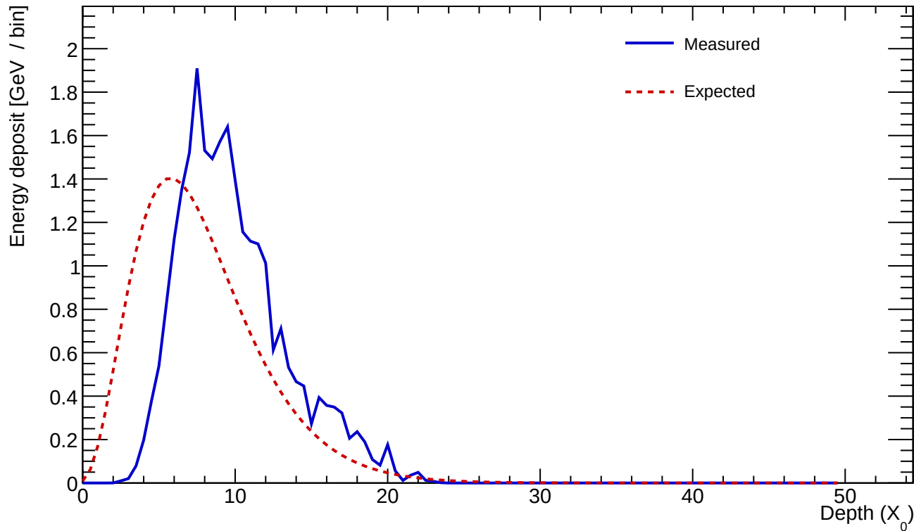
Cluster 300 E=25.603 GeV profileStart=2.50 X_0 \chi=0.1606
