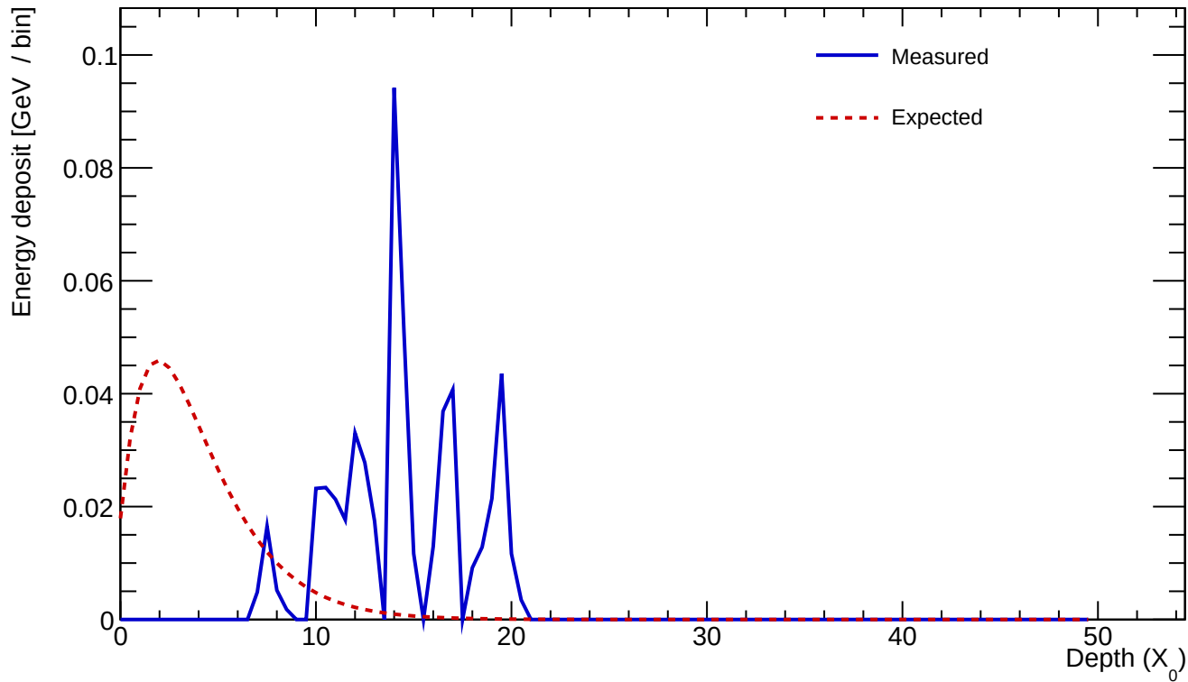
Cluster 363 E=0.542 GeV profileStart=11.50 X_0 \chi=0.7833
