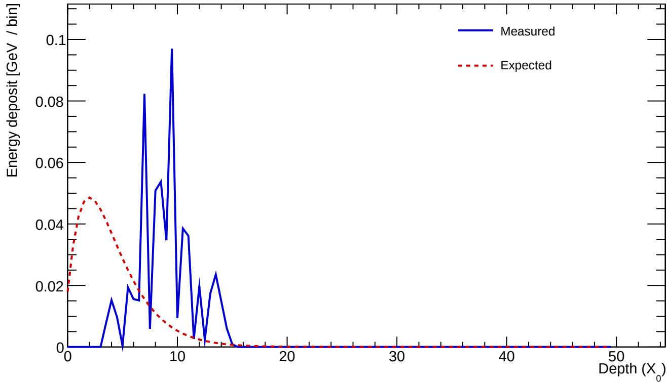
Cluster 878 E=0.579 GeV profileStart=6.00 X_0 \chi=0.5673
