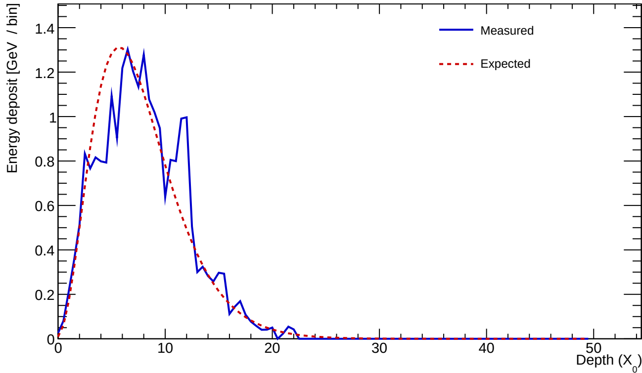
Cluster 803 E=23.785 GeV profileStart=0.50 X_0 \chi=0.1861
