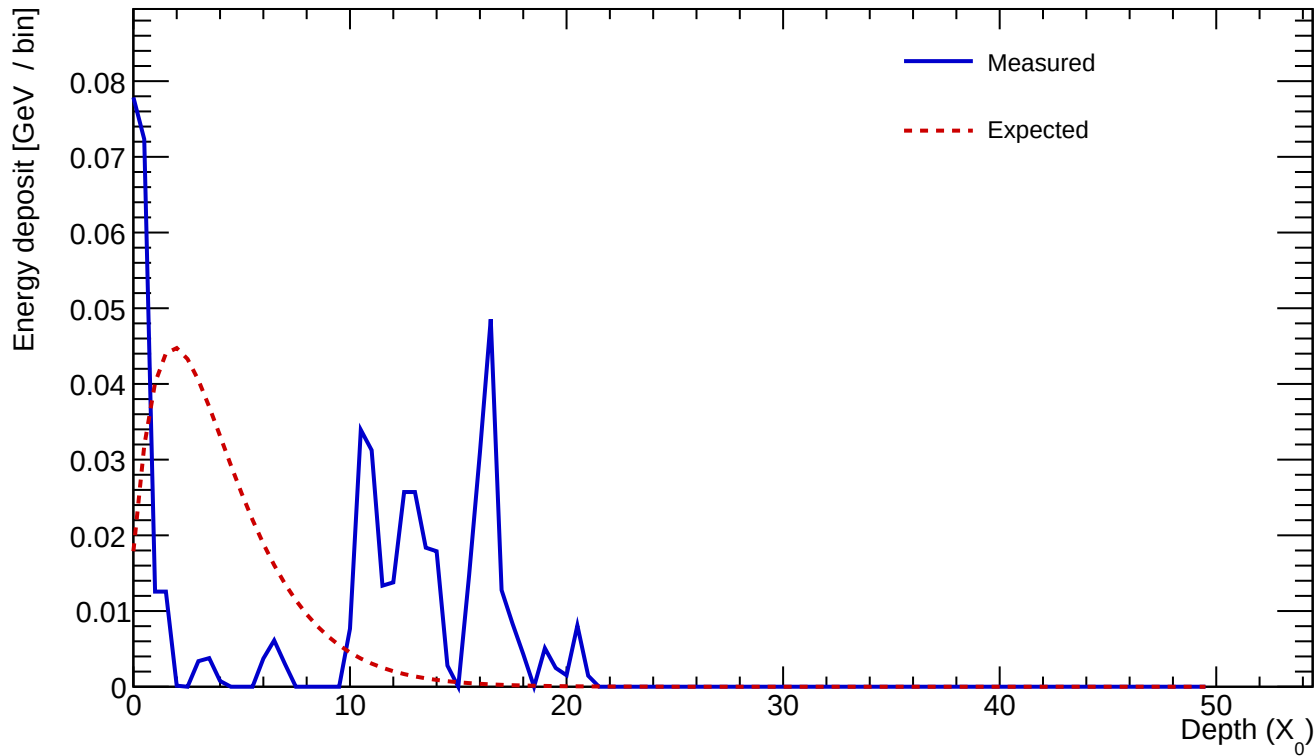
Cluster 587 E=0.525 GeV profileStart=10.00 X_0 \chi=0.9109
