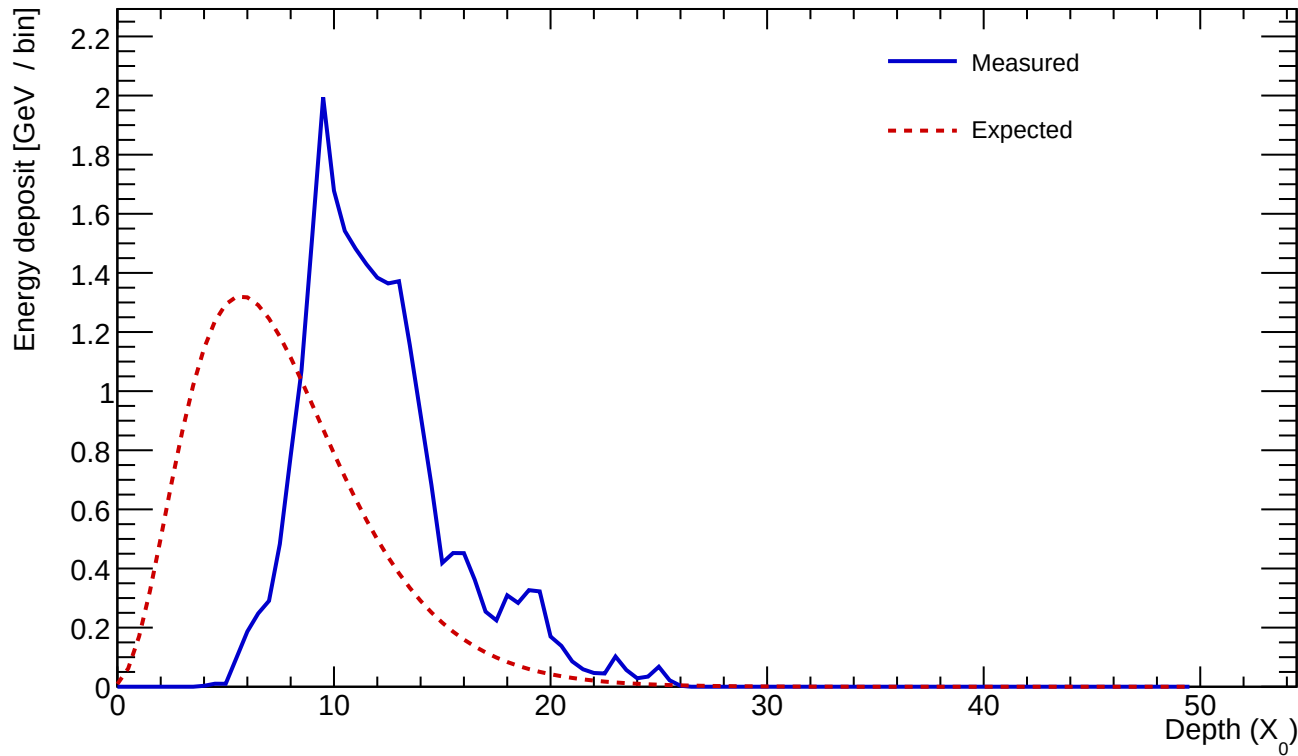
Cluster 653 E=23.975 GeV profileStart=5.00 X_0 \chi=0.2442
