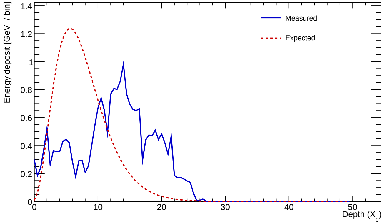
Cluster 754 E=22.342 GeV profileStart=7.00 X_0 \chi=0.5394
