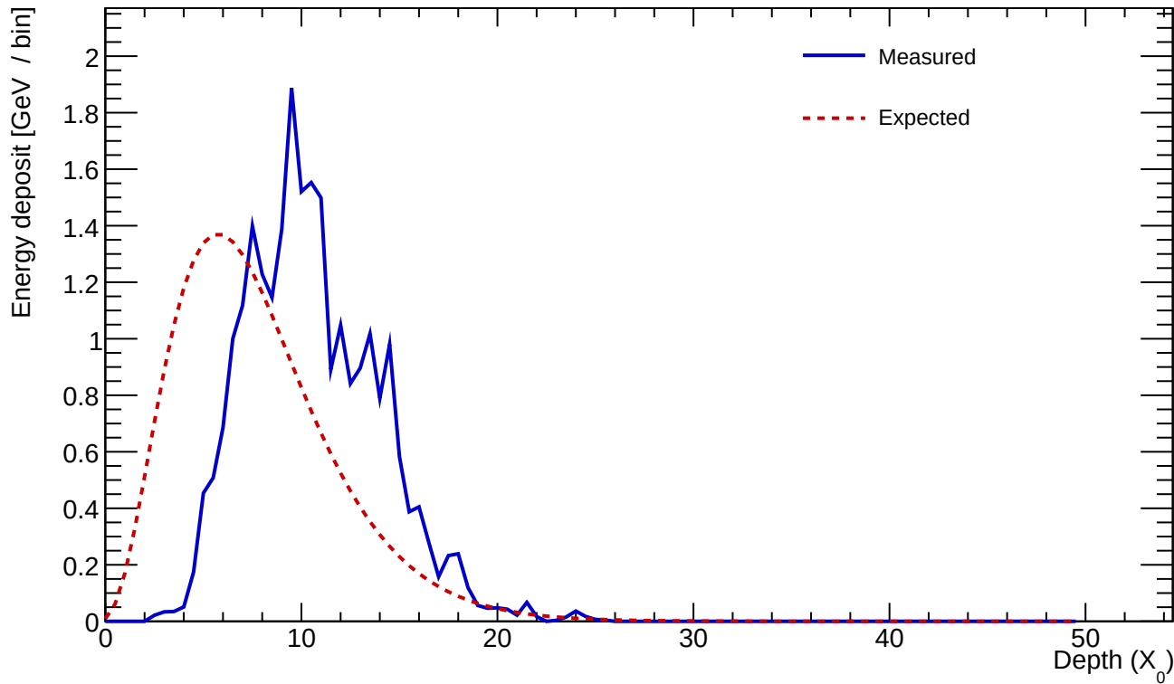
Cluster 623 E=24.951 GeV profileStart=3.50 X_0 \chi=0.1870
