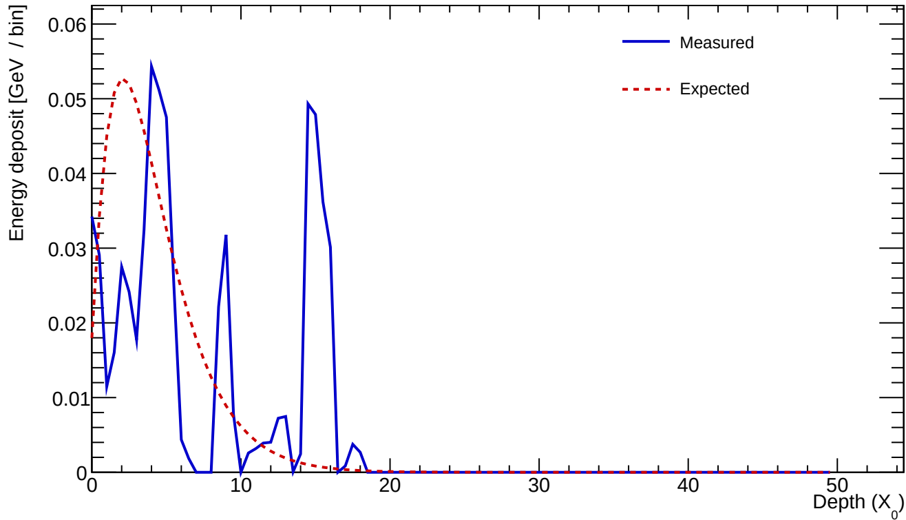
Cluster 962 E=0.640 GeV profileStart=1.50 X_0 \chi=0.8425
