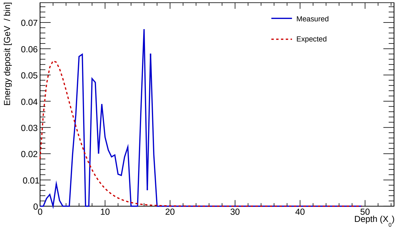
Cluster 694 E=0.680 GeV profileStart=5.00 X_0 \chi=0.5977
