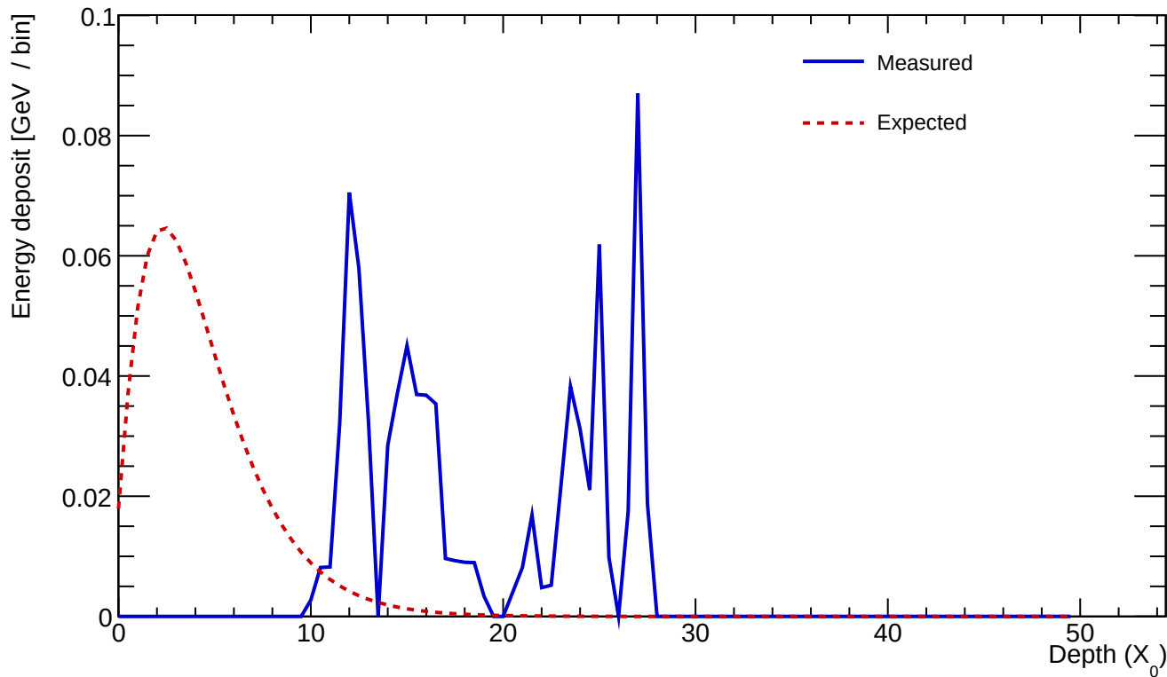
Cluster 154 E=0.818 GeV profileStart=10.50 X_0 \chi=0.7543
