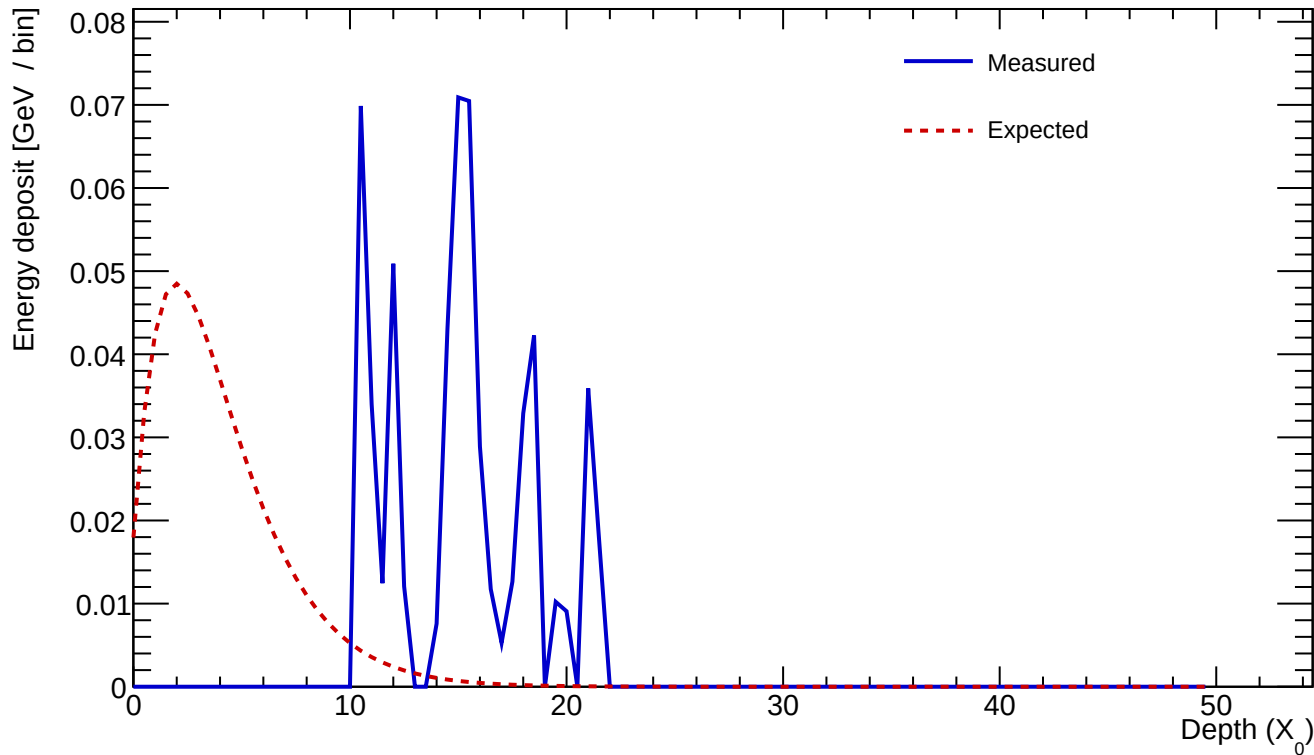
Cluster 195 E=0.578 GeV profileStart=10.50 X_0 \chi=0.8067
