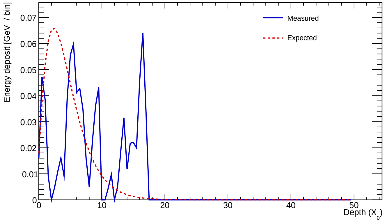
Cluster 692 E=0.836 GeV profileStart=3.50 X_0 \chi=0.7907
