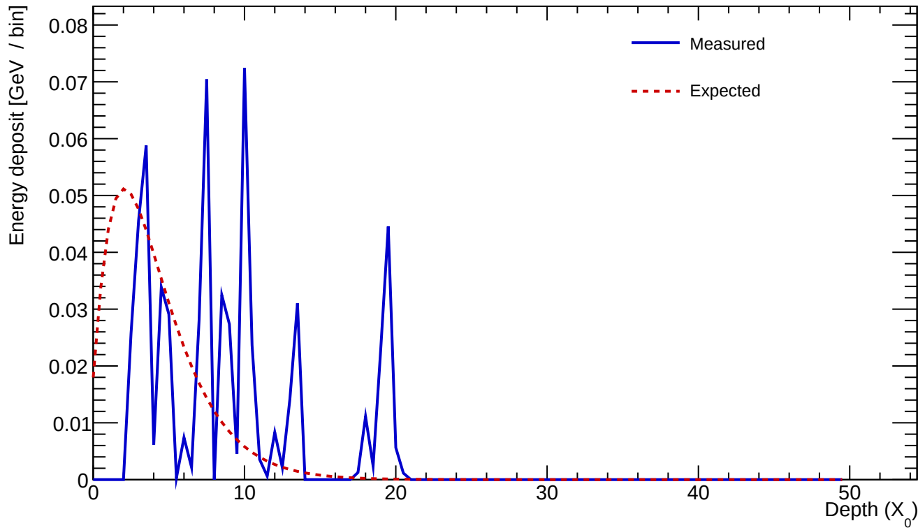
Cluster 358 E=0.617 GeV profileStart=2.00 X_0 \chi=0.8966
