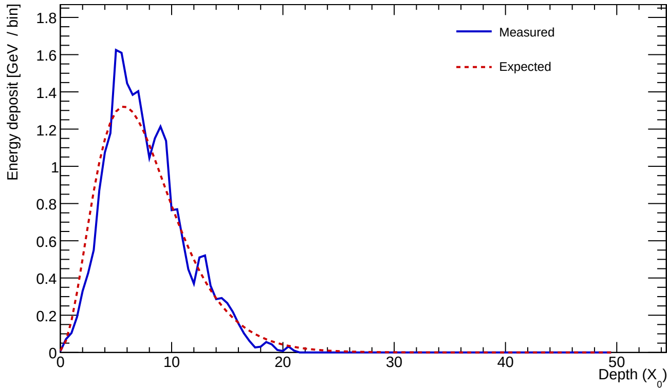
Cluster 90 E=23.987 GeV profileStart=0.50 X_0 \chi=0.1370
