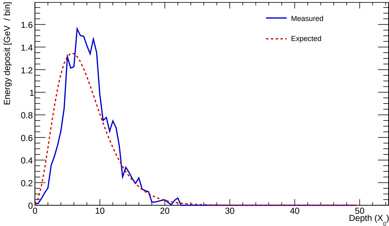
Cluster 738 E=24.446 GeV profileStart=1.00 X_0 \chi=0.1594
