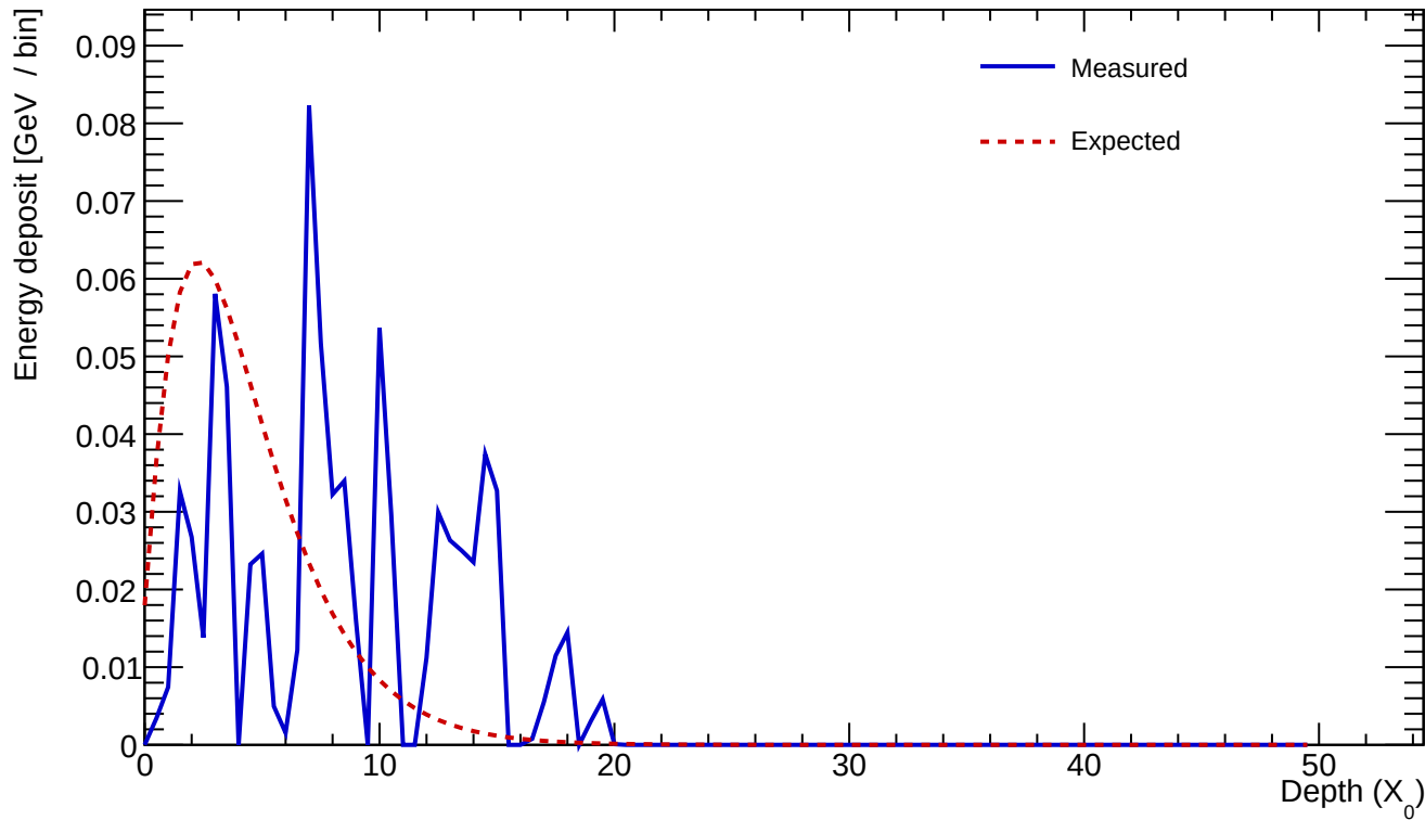
Cluster 616 E=0.782 GeV profileStart=6.50 X_0 \chi=0.8869
