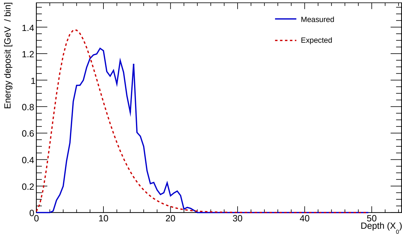
Cluster 199 E=25.130 GeV profileStart=3.00 X_0 \chi=0.1654
