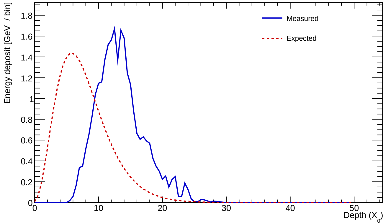
Cluster 433 E=26.218 GeV profileStart=6.00 X_0 \chi=0.1499
