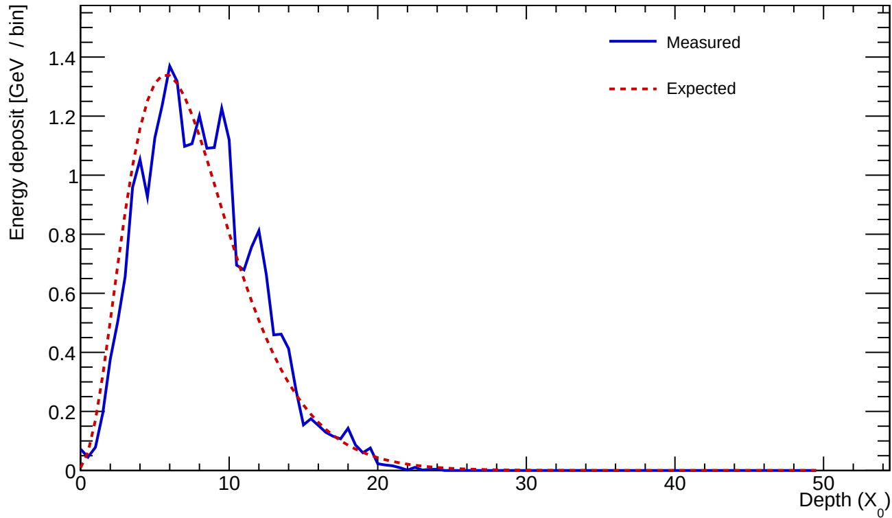
Cluster 66 E=24.350 GeV profileStart=0.50 X_0 \chi=0.1268
