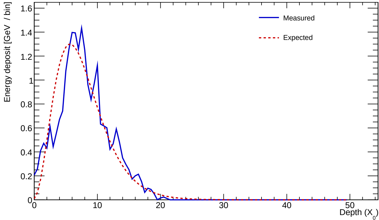
Cluster 79 E=23.550 GeV profileStart=0.50 X_0 \chi=0.2076
