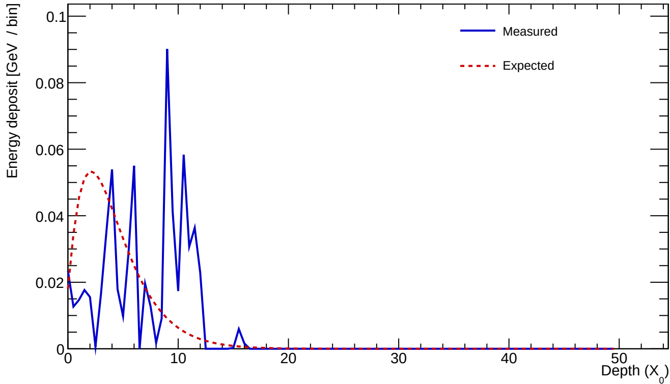
Cluster 1108 E=0.650 GeV profileStart=3.00 X_0 \chi=0.8690
