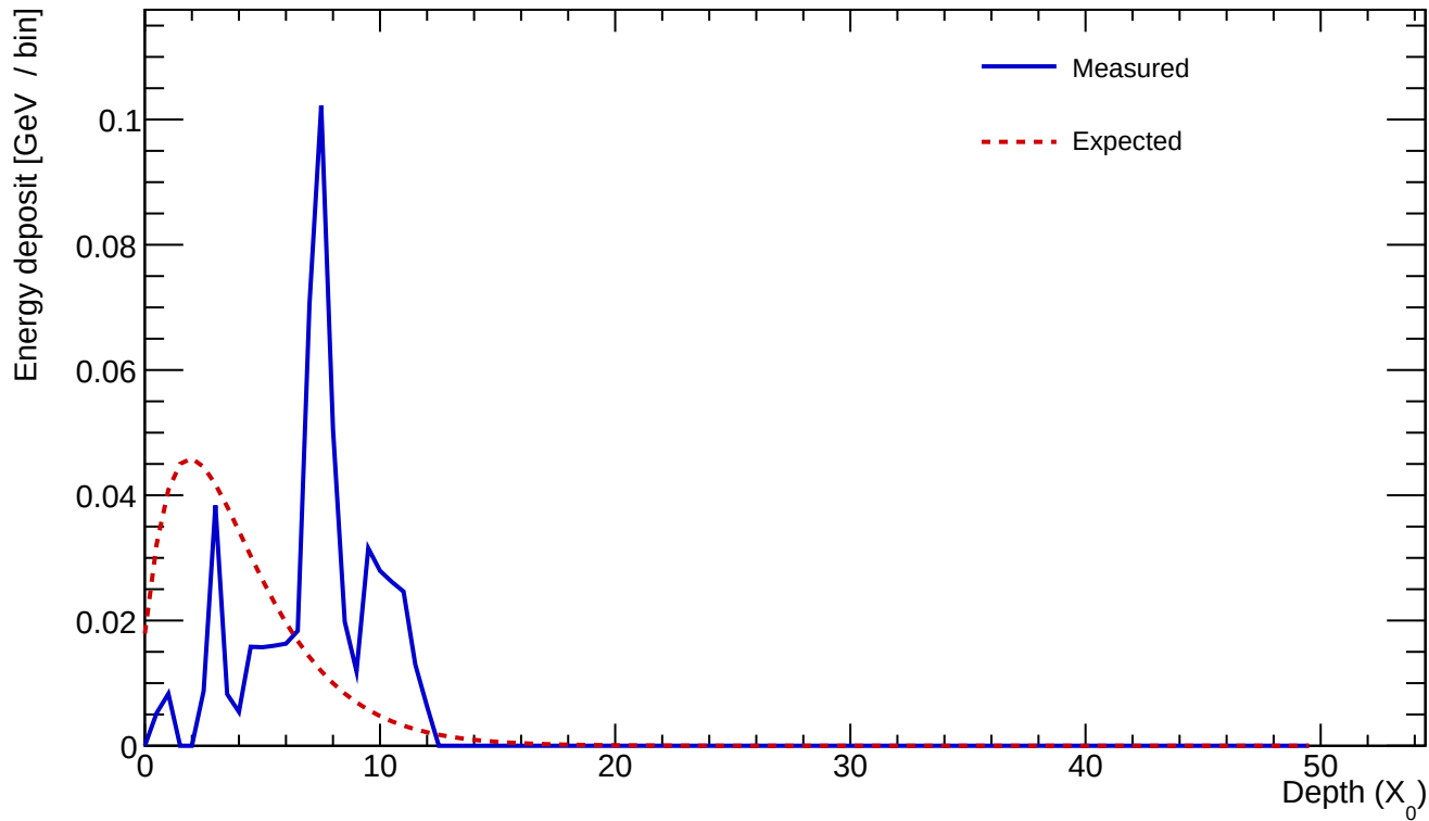
Cluster 190 E=0.541 GeV profileStart=5.50 X_0 \chi=0.5474
