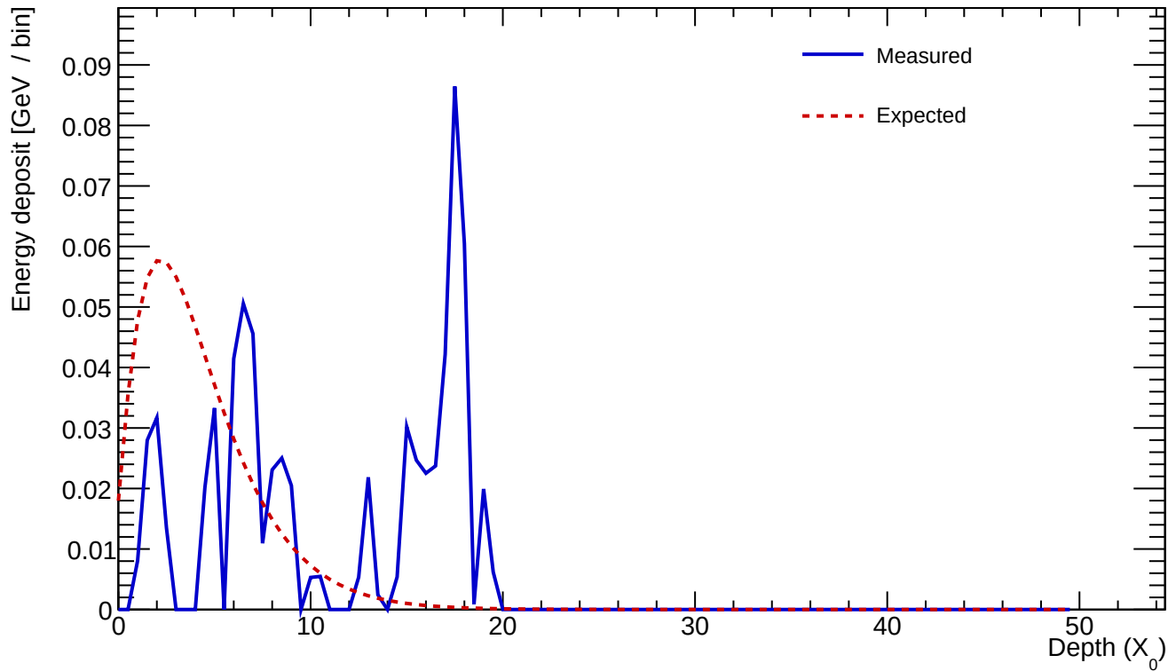
Cluster 621 E=0.715 GeV profileStart=4.50 X_0 \chi=1.0526
