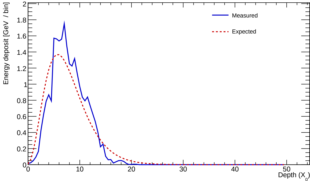
Cluster 748 E=24.908 GeV profileStart=1.00 X_0 \chi=0.1838
