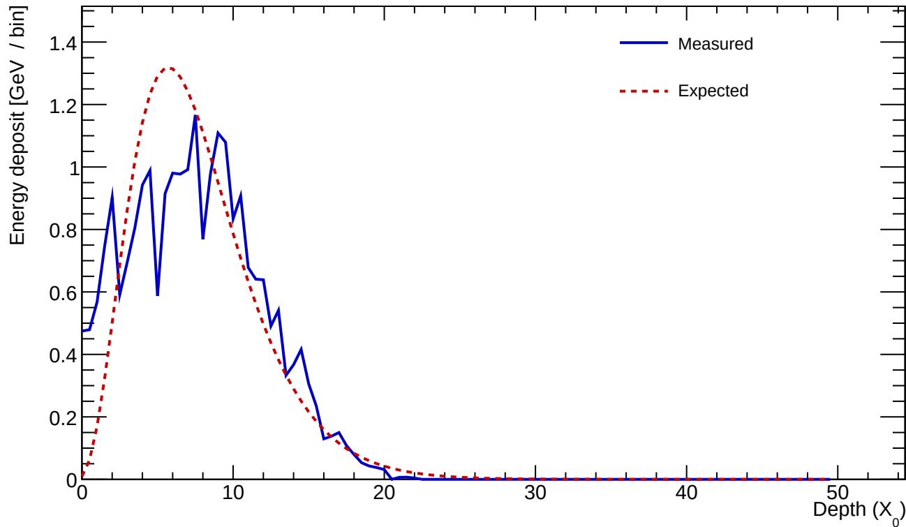
Cluster 773 E=23.921 GeV profileStart=0.50 X_0 \chi=0.2836
