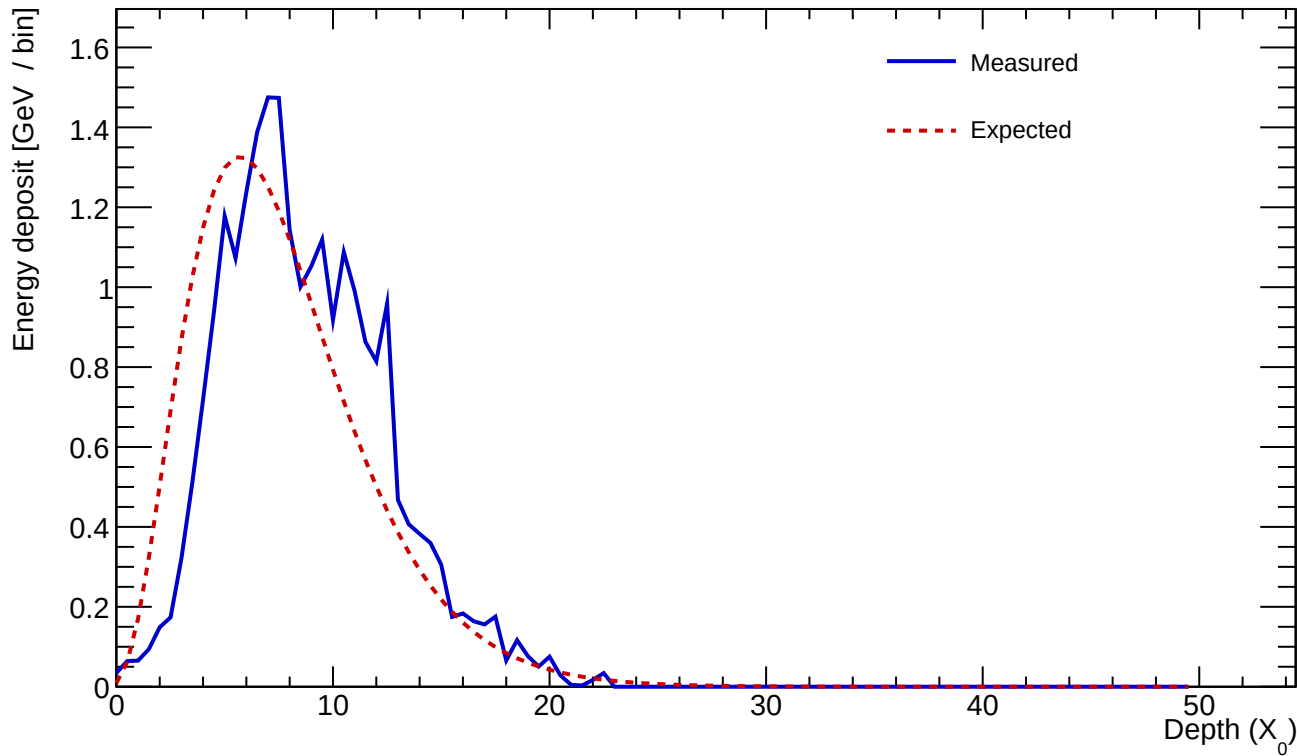
Cluster 329 E=24.087 GeV profileStart=1.50 X_0 \chi=0.1383
