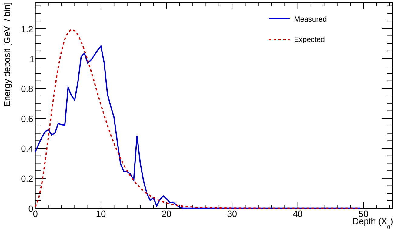
Cluster 771 E=21.455 GeV profileStart=1.50 X_0 \chi=0.3223
