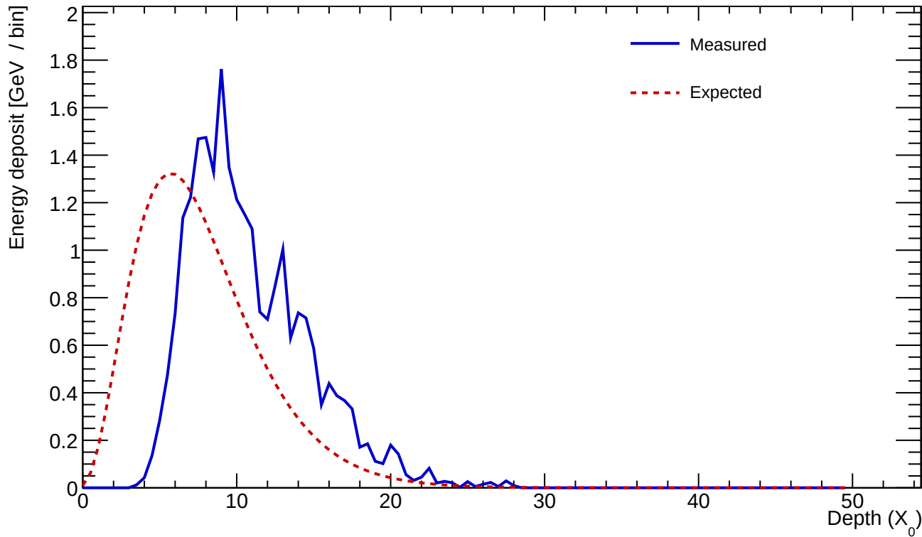
Cluster 335 E=24.015 GeV profileStart=3.50 X_0 \chi=0.1677
