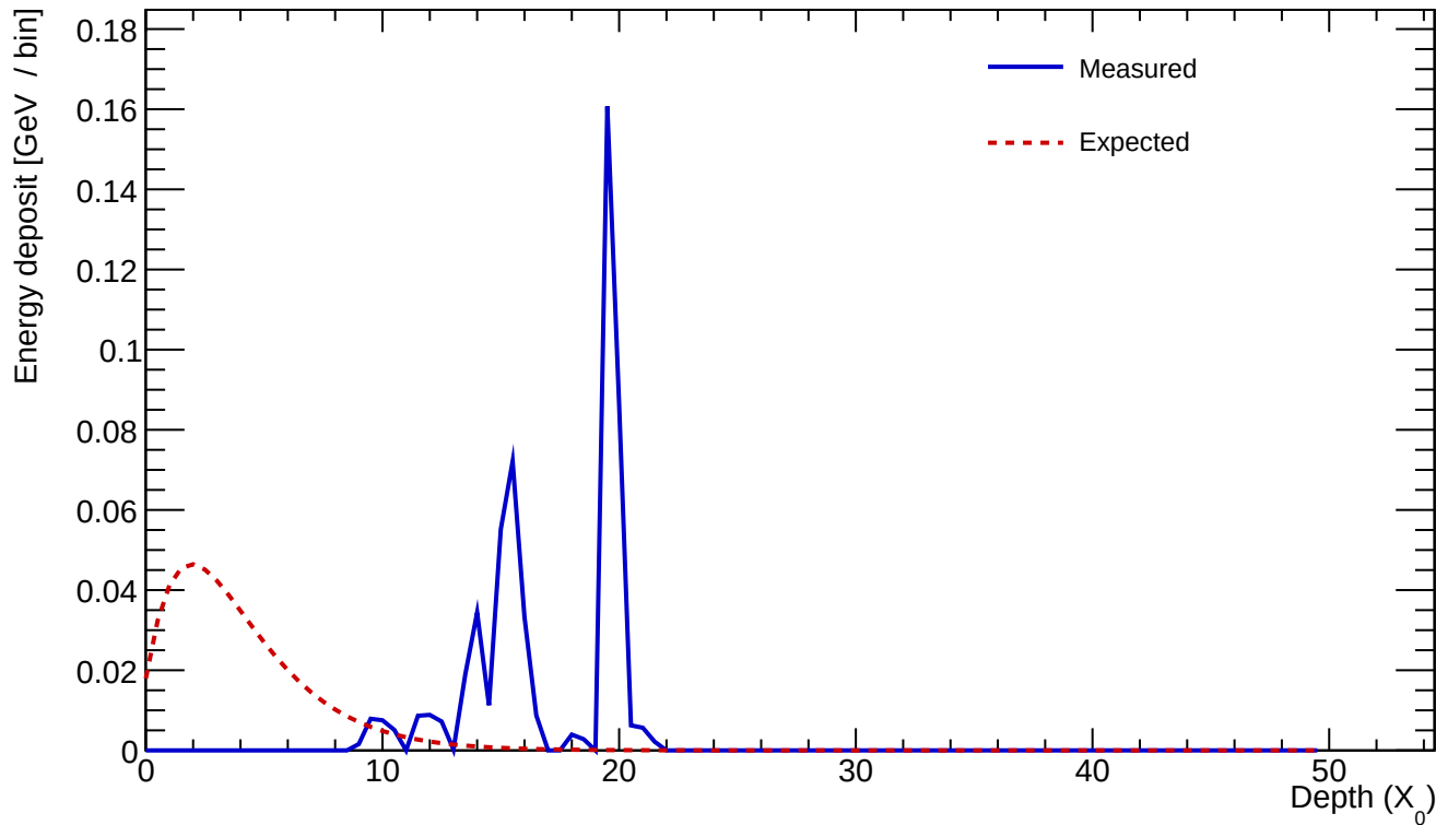
Cluster 552 E=0.549 GeV profileStart=13.50 X_0 \chi=0.9722
