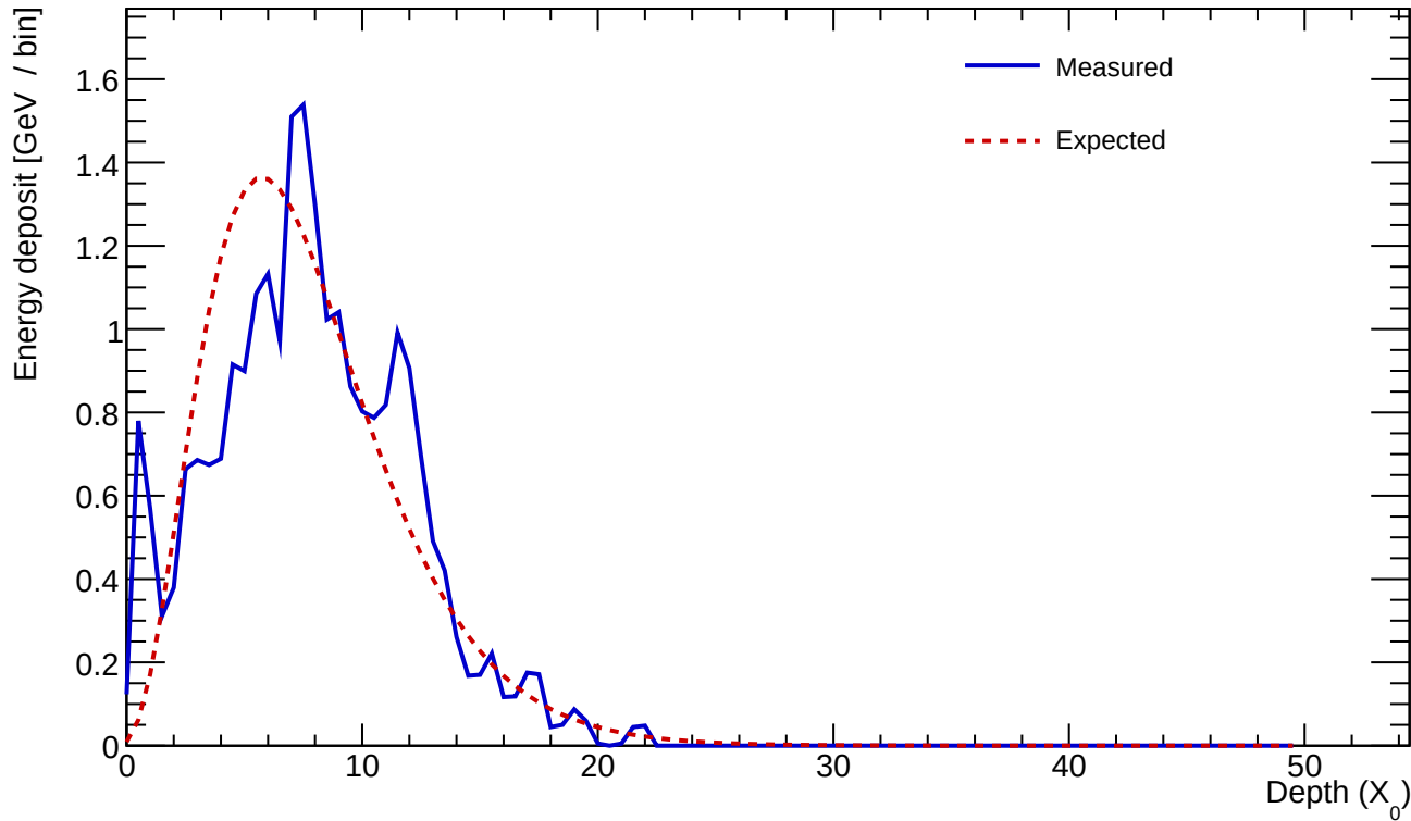
Cluster 569 E=24.807 GeV profileStart=0.50 X_0 \chi=0.2615
