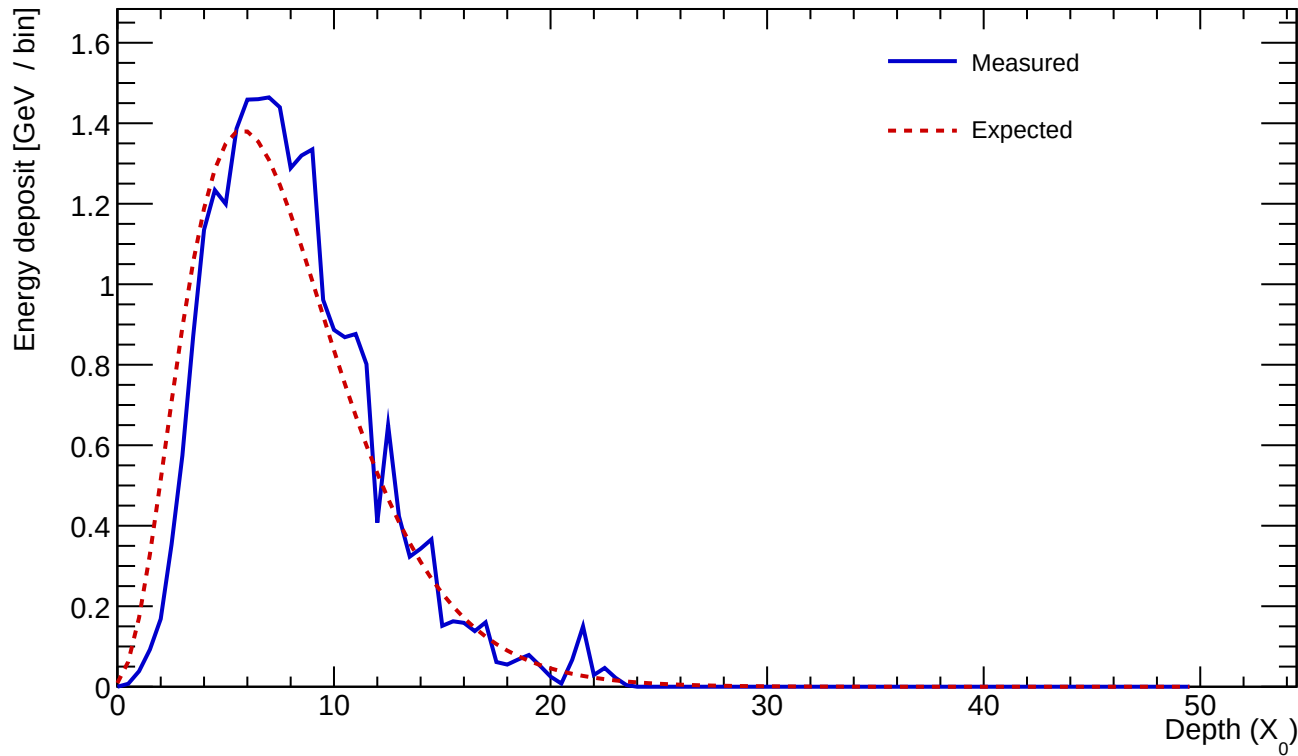
Cluster 311 E=25.173 GeV profileStart=0.50 X_0 \chi=0.1273
