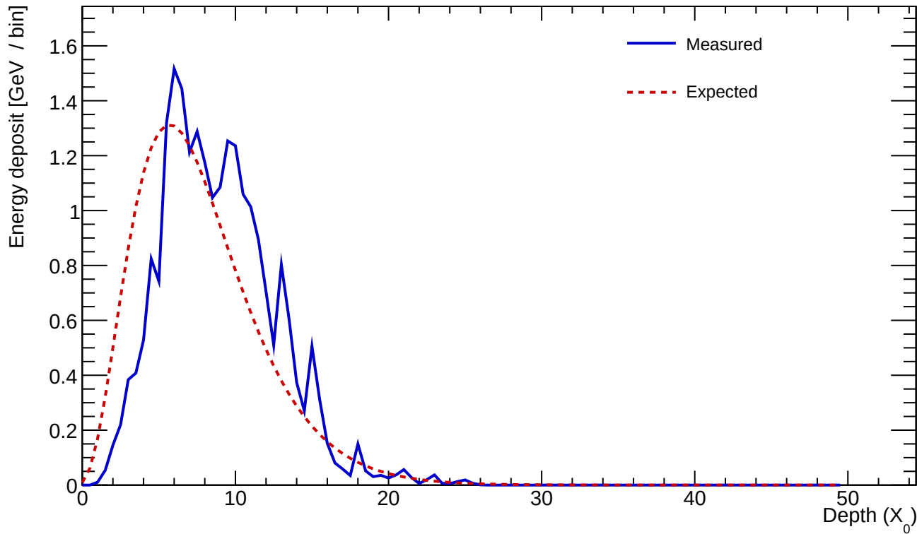
Cluster 353 E=23.802 GeV profileStart=1.50 X_0 \chi=0.1837
