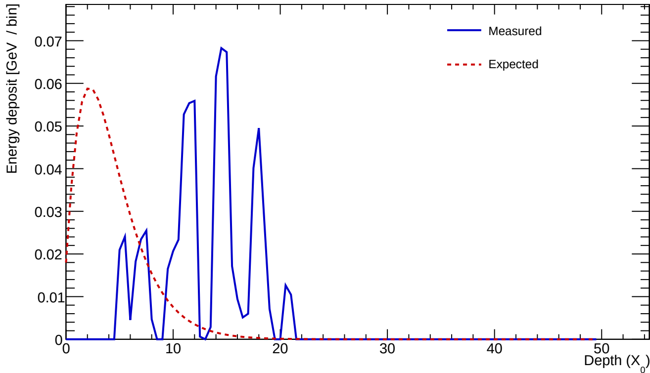
Cluster 536 E=0.732 GeV profileStart=10.00 X_0 \chi=0.7672
