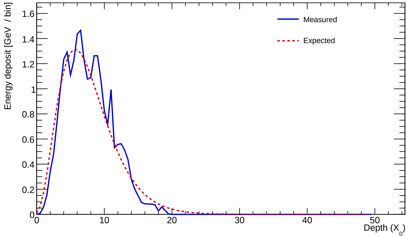
Cluster 504 E=23.825 GeV profileStart=0.50 X_0 \chi=0.1406
