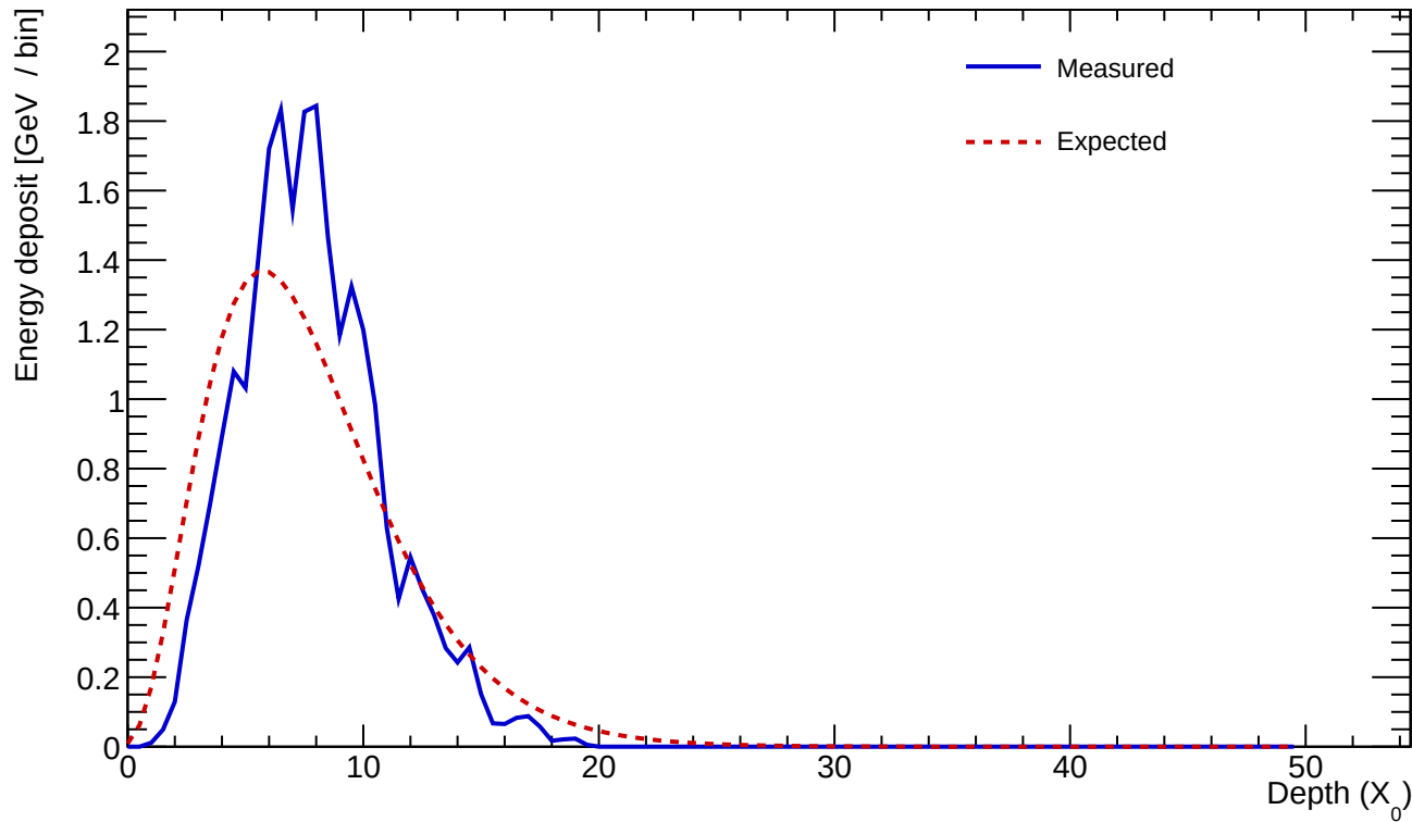
Cluster 21 E=24.902 GeV profileStart=1.00 X_0 \chi=0.2251
