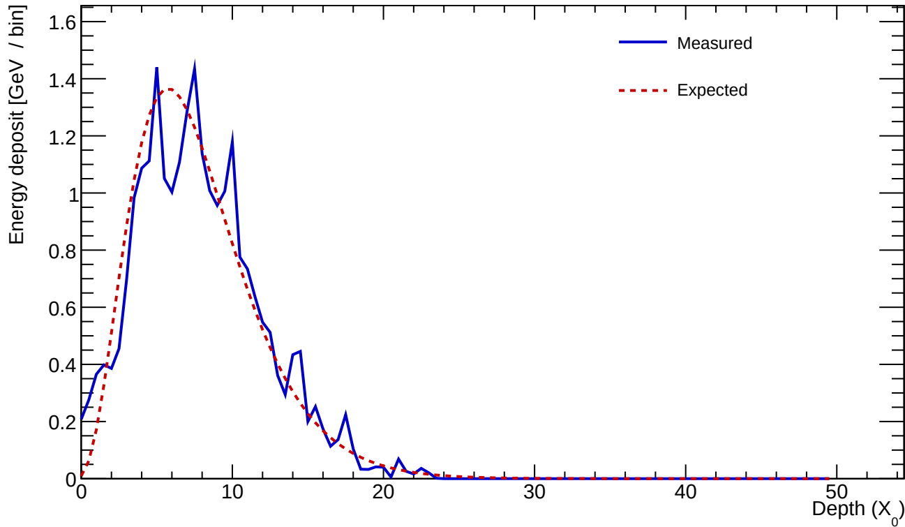
Cluster 601 E=24.843 GeV profileStart=0.50 X_0 \chi=0.1732
