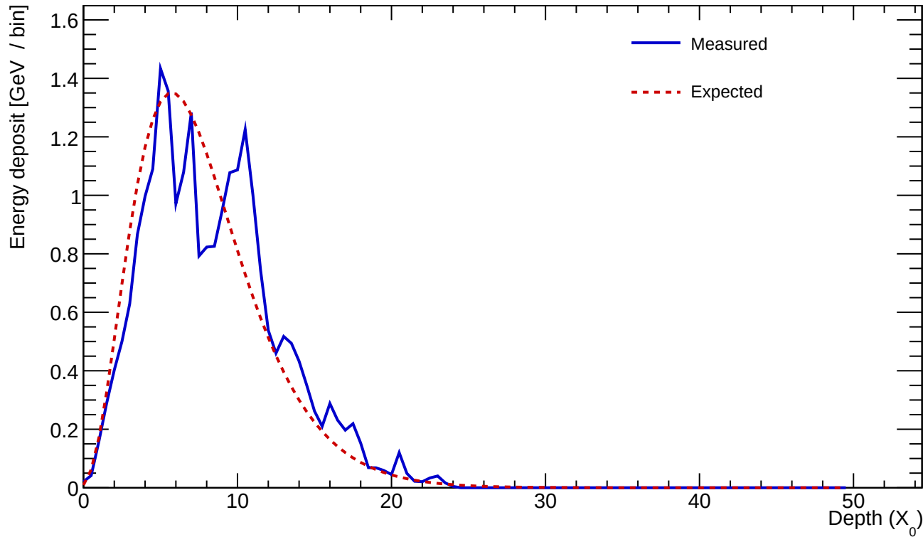
Cluster 893 E=24.541 GeV profileStart=0.50 X_0 \chi=0.1942
