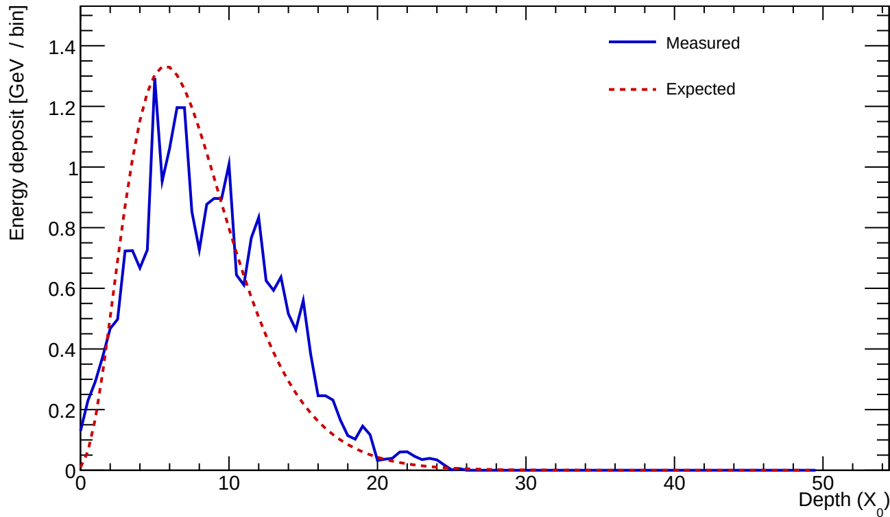
Cluster 134 E=24.200 GeV profileStart=0.50 X_0 \chi=0.2852
