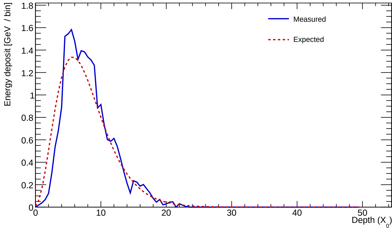
Cluster 284 E=24.299 GeV profileStart=1.00 X_0 \chi=0.1565
