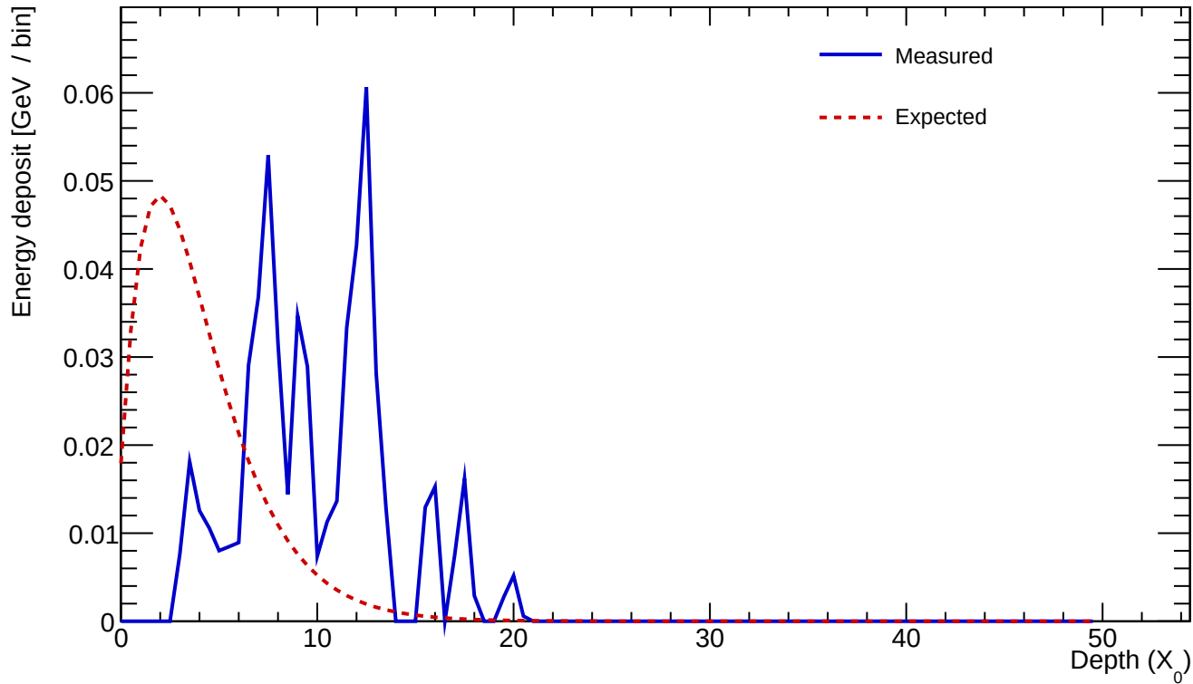
Cluster 350 E=0.576 GeV profileStart=6.00 X_0 \chi=0.6724
