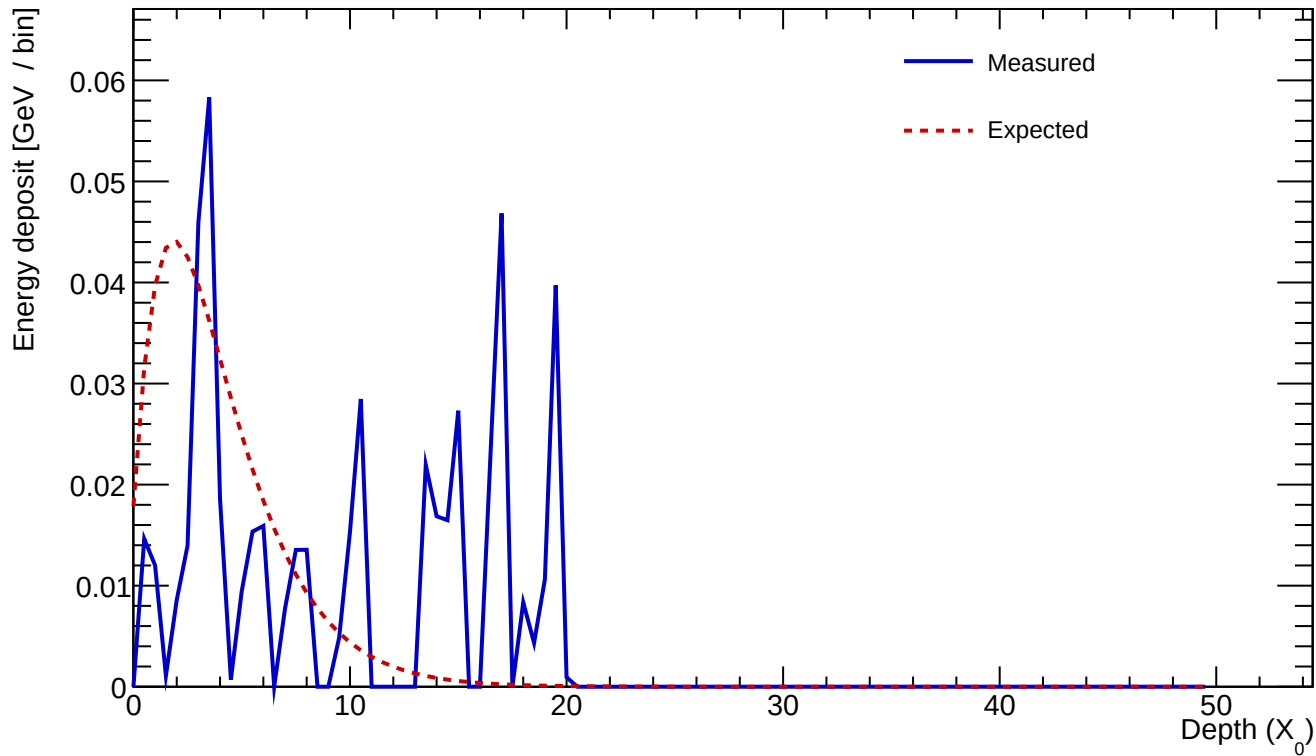
Cluster 1030 E=0.515 GeV profileStart=0.50 X_0 \chi=1.0459
