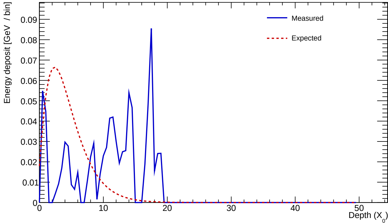
Cluster 976 E=0.846 GeV profileStart=10.00 X_0 \chi=0.8676
