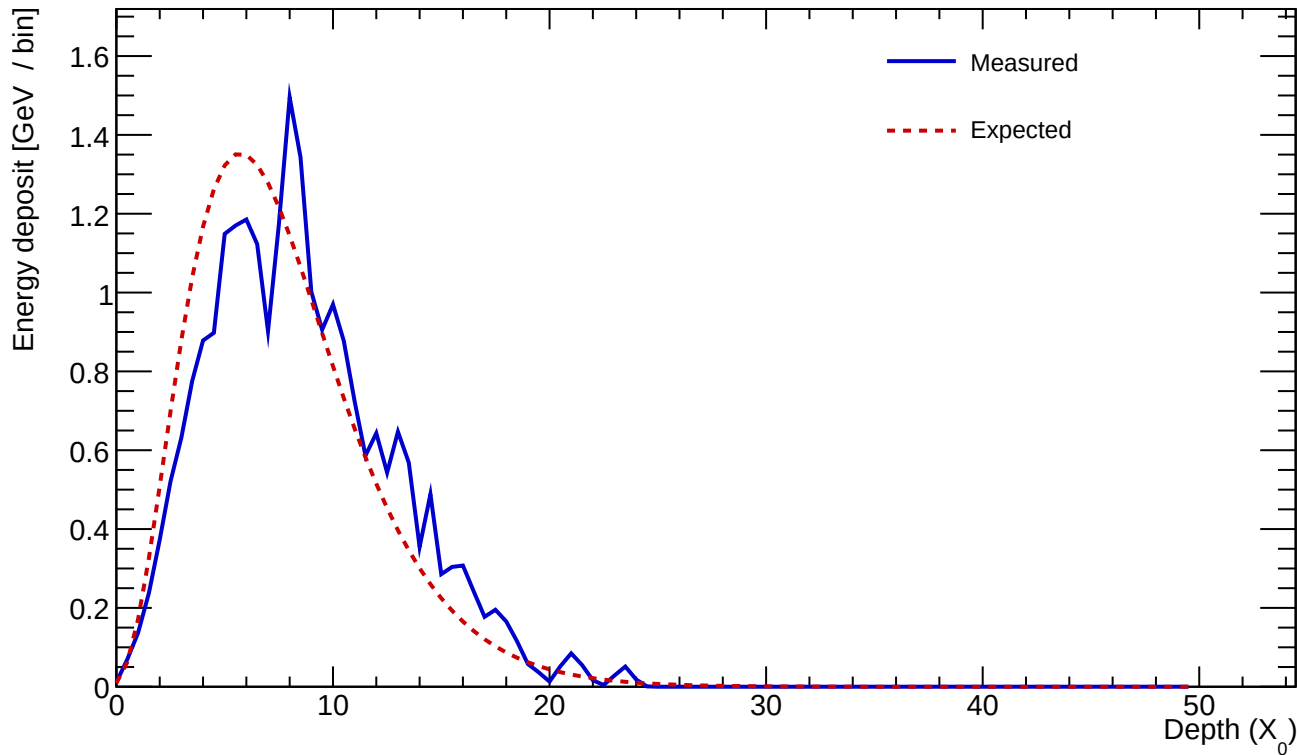
Cluster 458 E=24.593 GeV profileStart=1.00 X_0 \chi=0.1692
