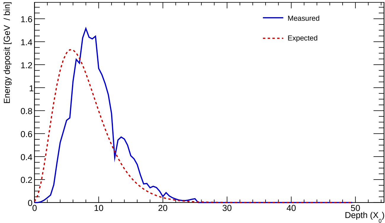
Cluster 208 E=24.183 GeV profileStart=2.00 X_0 \chi=0.1168
