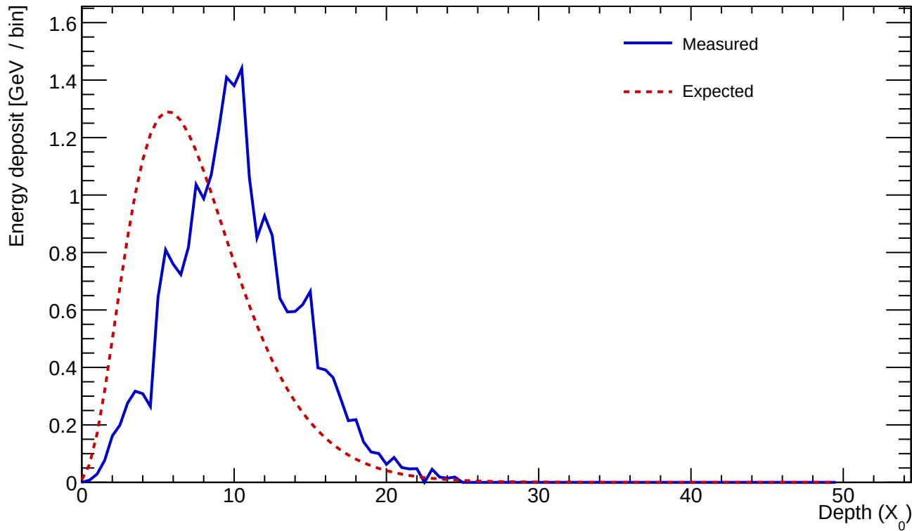
Cluster 414 E=23.379 GeV profileStart=3.00 X_0 \chi=0.1974
