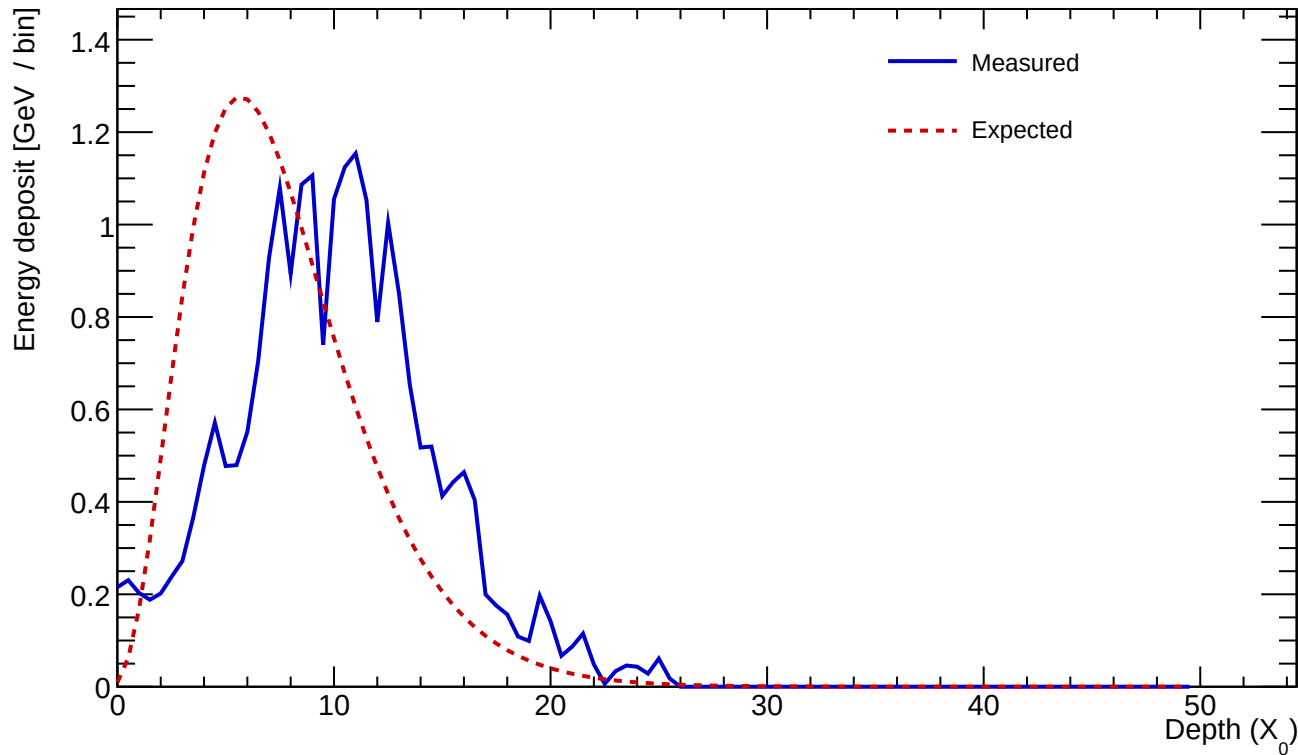
Cluster 936 E=23.087 GeV profileStart=3.50 X_0 \chi=0.2765
