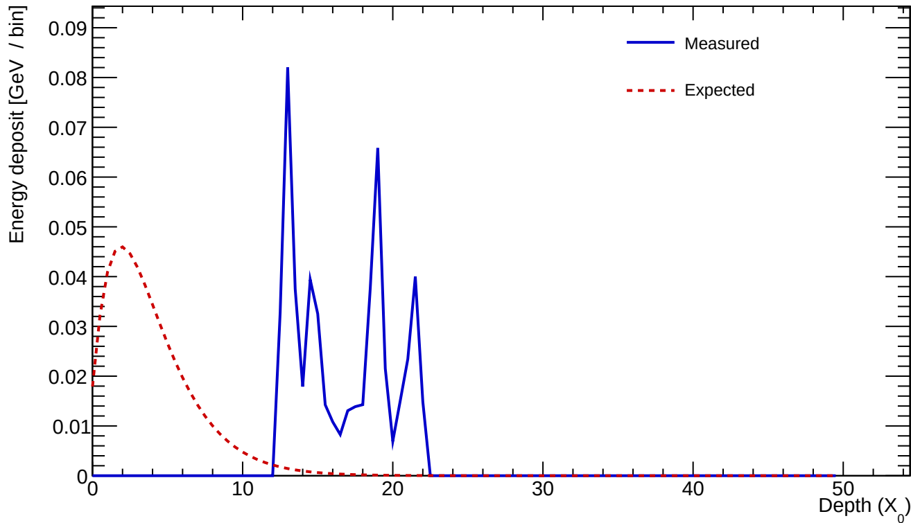
Cluster 276 E=0.542 GeV profileStart=12.00 X_0 \chi=0.6460
