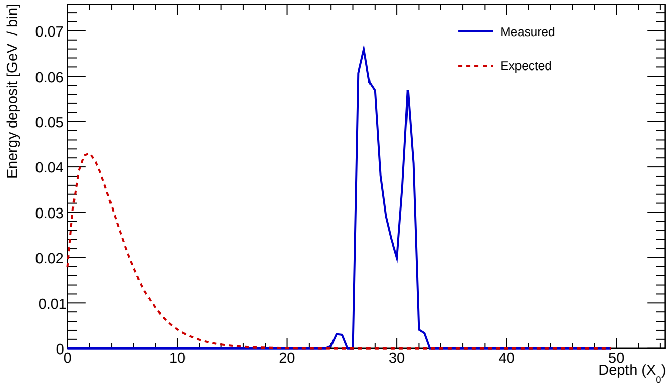
Cluster 502 E=0.501 GeV profileStart=26.00 X_0 \chi=0.4407
