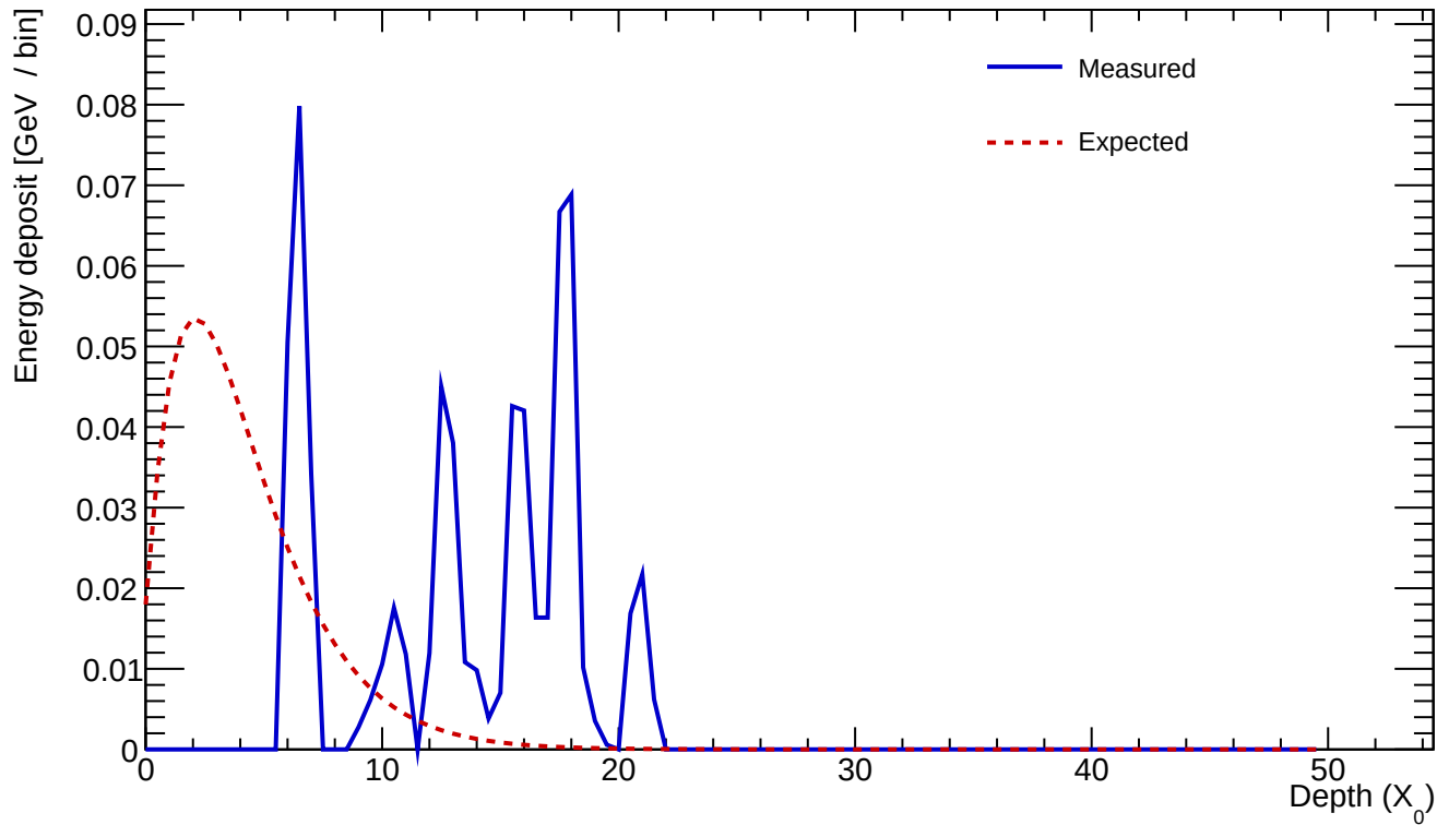
Cluster 397 E=0.652 GeV profileStart=5.00 X_0 \chi=1.1396
