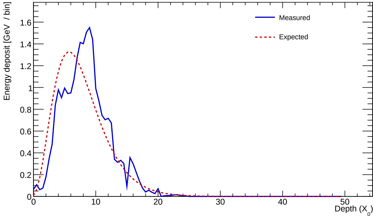
Cluster 523 E=24.078 GeV profileStart=1.00 X_0 \chi=0.1960
