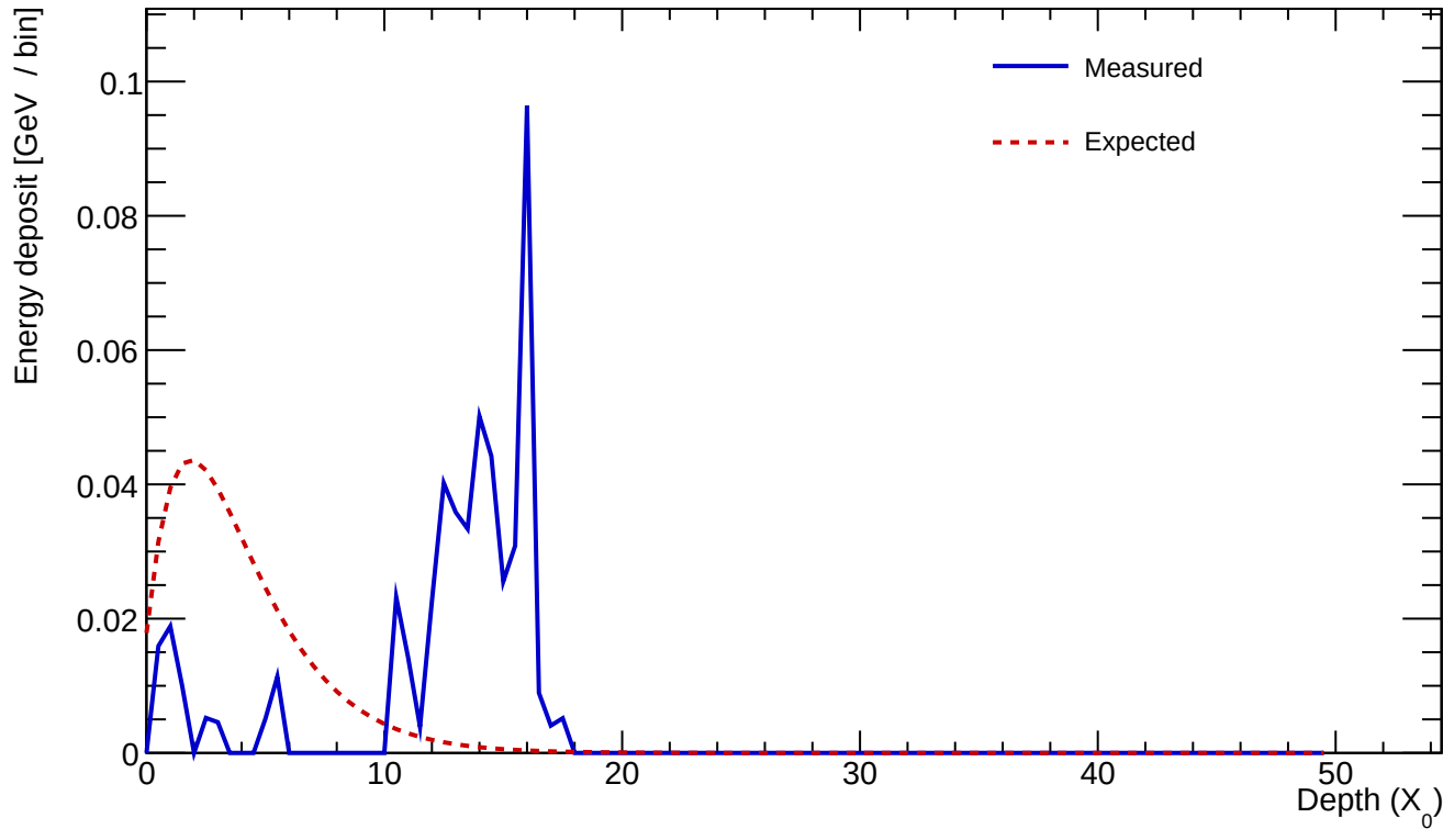
Cluster 998 E=0.510 GeV profileStart=12.00 X_0 \chi=0.5310
