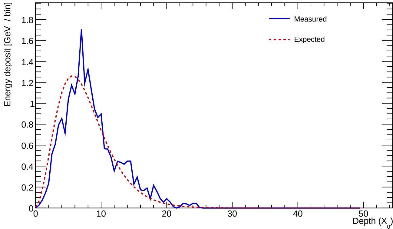
Cluster 913 E=22.780 GeV profileStart=0.50 X_0 \chi=0.1644
