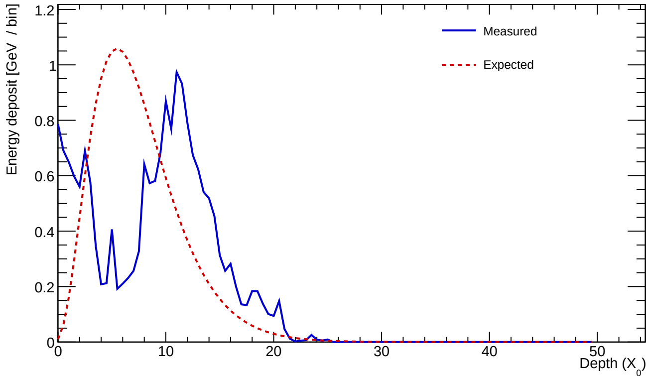
Cluster 772 E=18.852 GeV profileStart=3.50 X_0 \chi=0.5709
