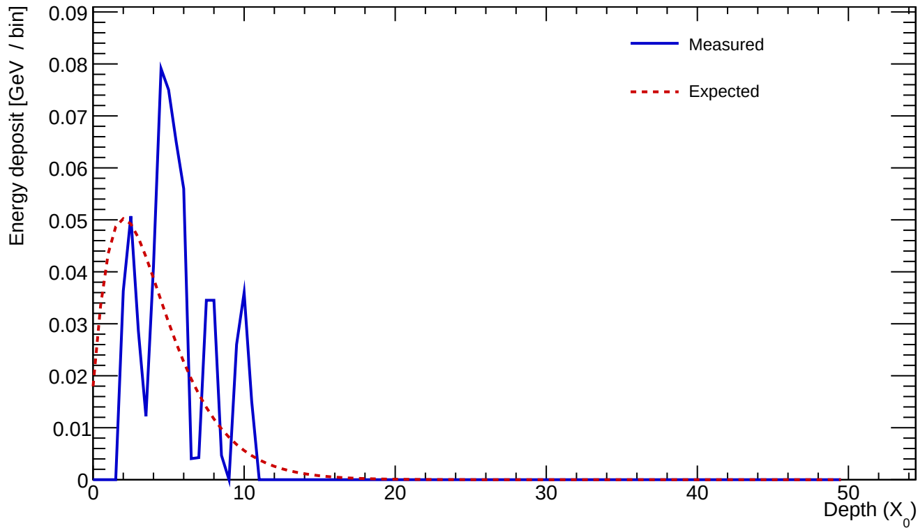
Cluster 957 E=0.603 GeV profileStart=2.00 X_0 \chi=0.5602
