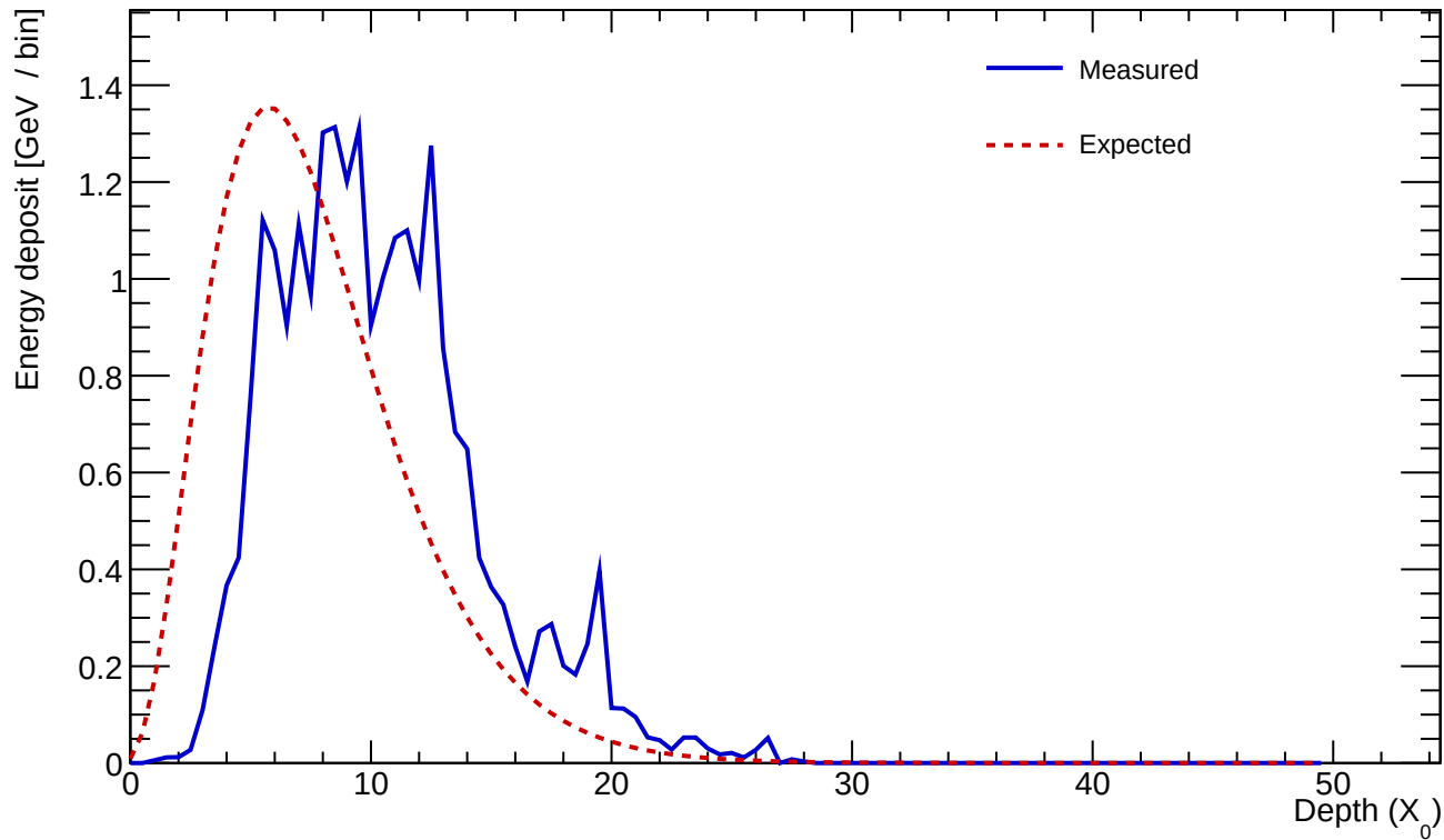
Cluster 152 E=24.633 GeV profileStart=2.50 X_0 \chi=0.1693
