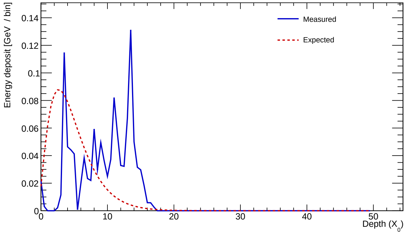
Cluster 268 E=1.172 GeV profileStart=7.00 X_0 \chi=0.7174
