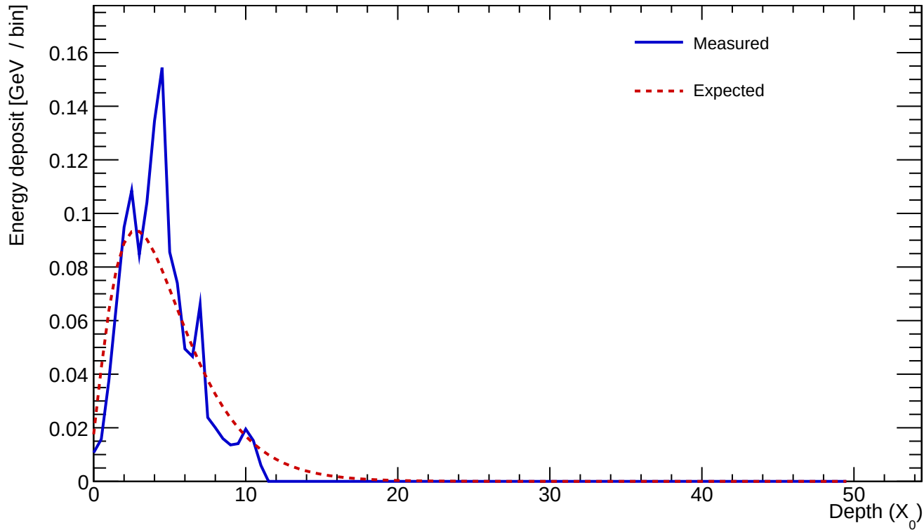
Cluster 684 E=1.261 GeV profileStart=0.50 X_0 \chi=0.2519
