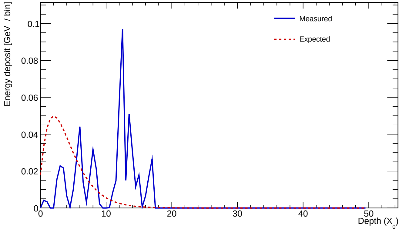
Cluster 71 E=0.598 GeV profileStart=11.00 X_0 \chi=0.8430
