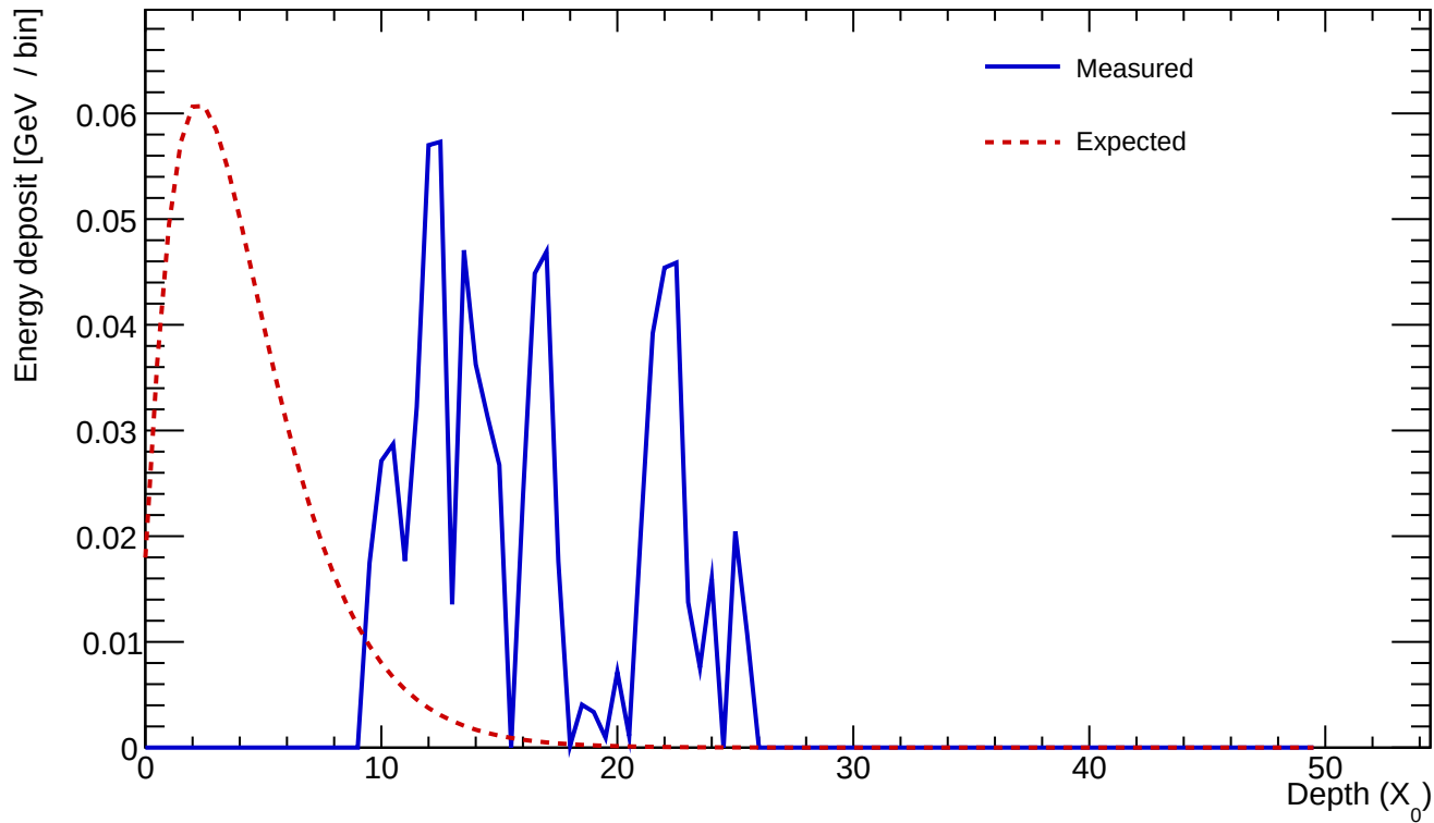
Cluster 682 E=0.762 GeV profileStart=9.50 X_0 \chi=0.6396
