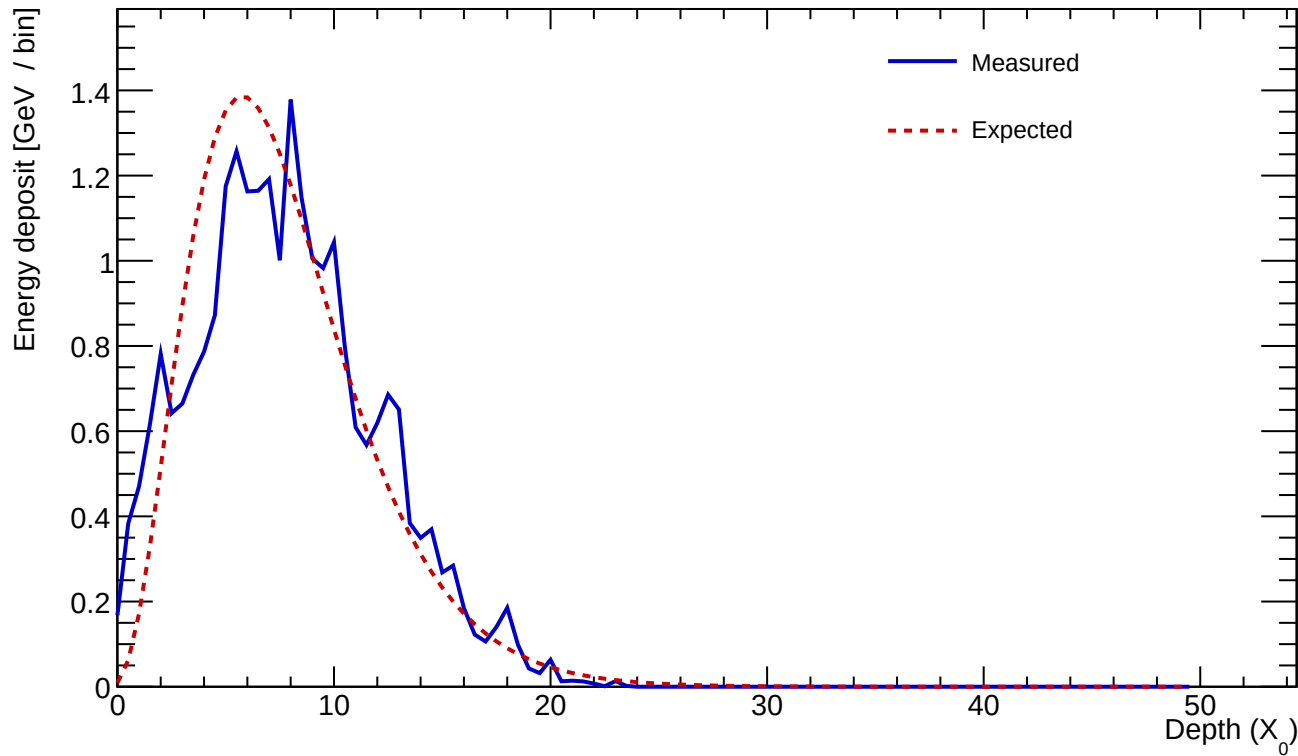
Cluster 321 E=25.252 GeV profileStart=0.50 X_0 \chi=0.2176
