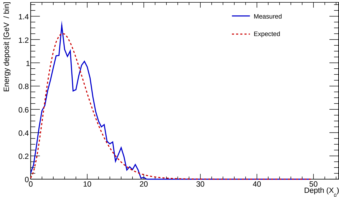
Cluster 732 E=22.626 GeV profileStart=0.50 X_0 \chi=0.1723
