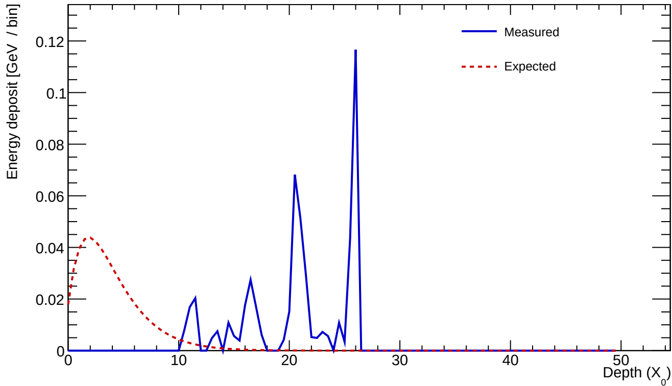
Cluster 185 E=0.512 GeV profileStart=19.50 X_0 \chi=0.8587
