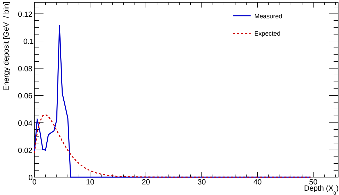
Cluster 135 E=0.542 GeV profileStart=2.00 X_0 \chi=0.4454
