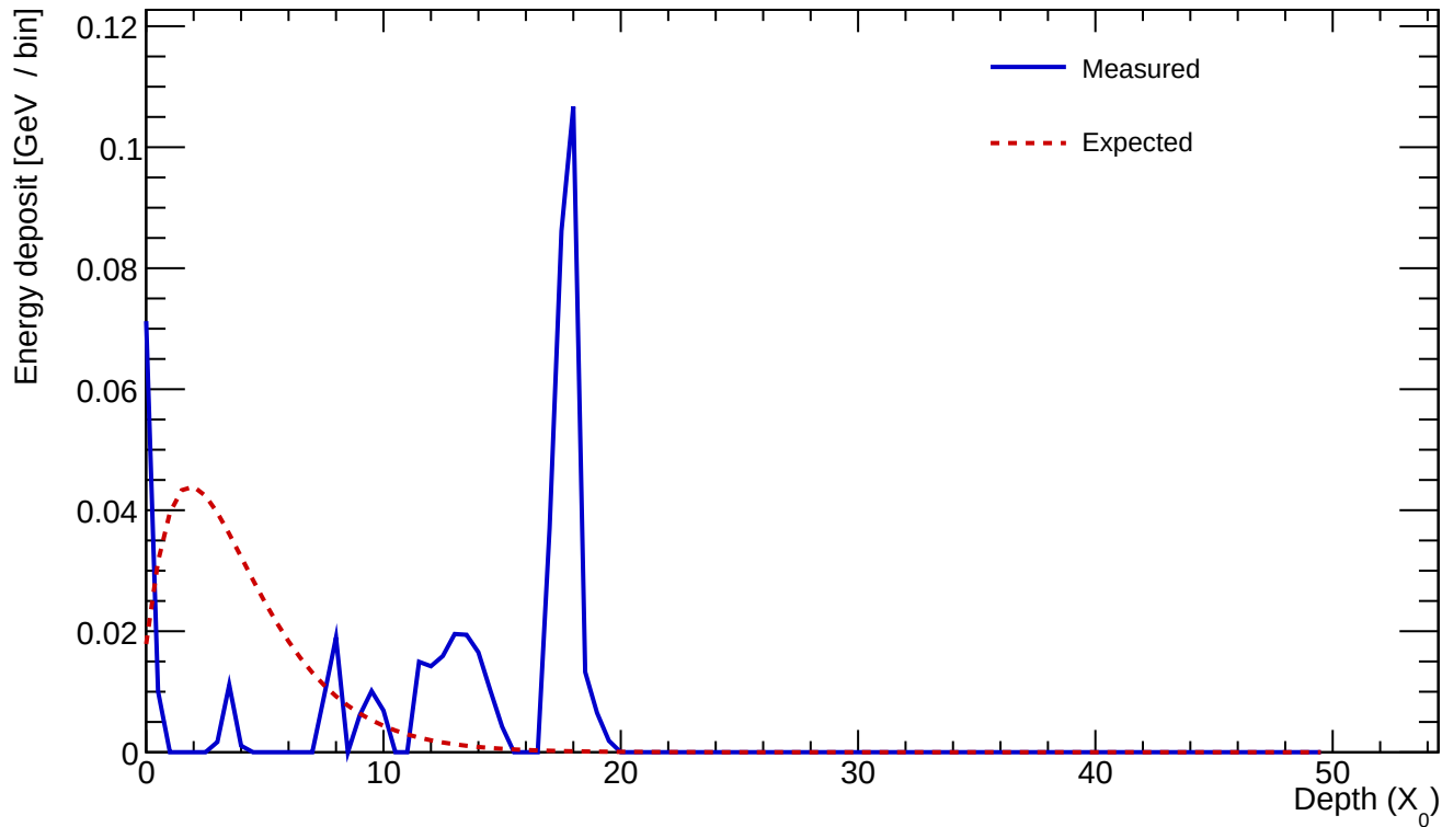
Cluster 334 E=0.513 GeV profileStart=16.50 X_0 \chi=0.8992
