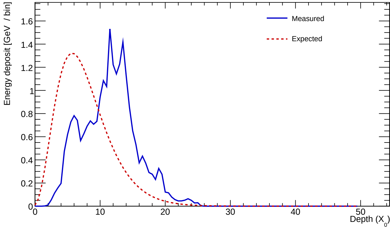
Cluster 663 E=23.976 GeV profileStart=4.00 X_0 \chi=0.3467
