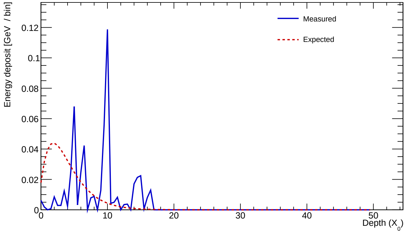
Cluster 908 E=0.513 GeV profileStart=3.50 X_0 \chi=0.9823
