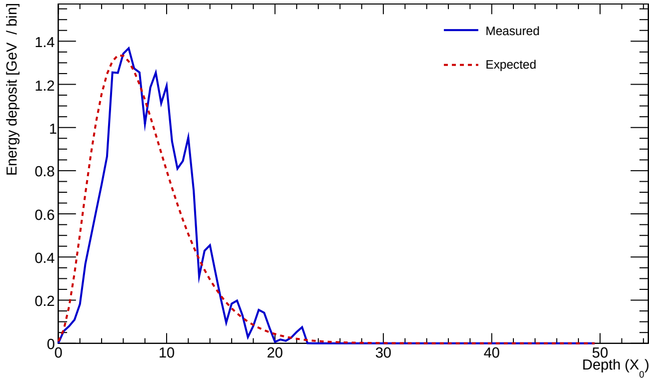
Cluster 912 E=24.266 GeV profileStart=1.00 X_0 \chi=0.1353
