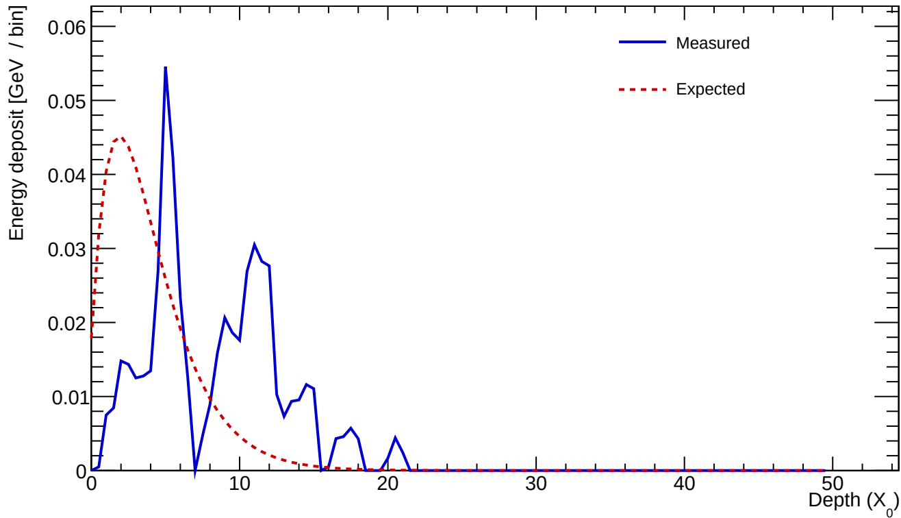
Cluster 111 E=0.531 GeV profileStart=3.50 X_0 \chi=0.7260
