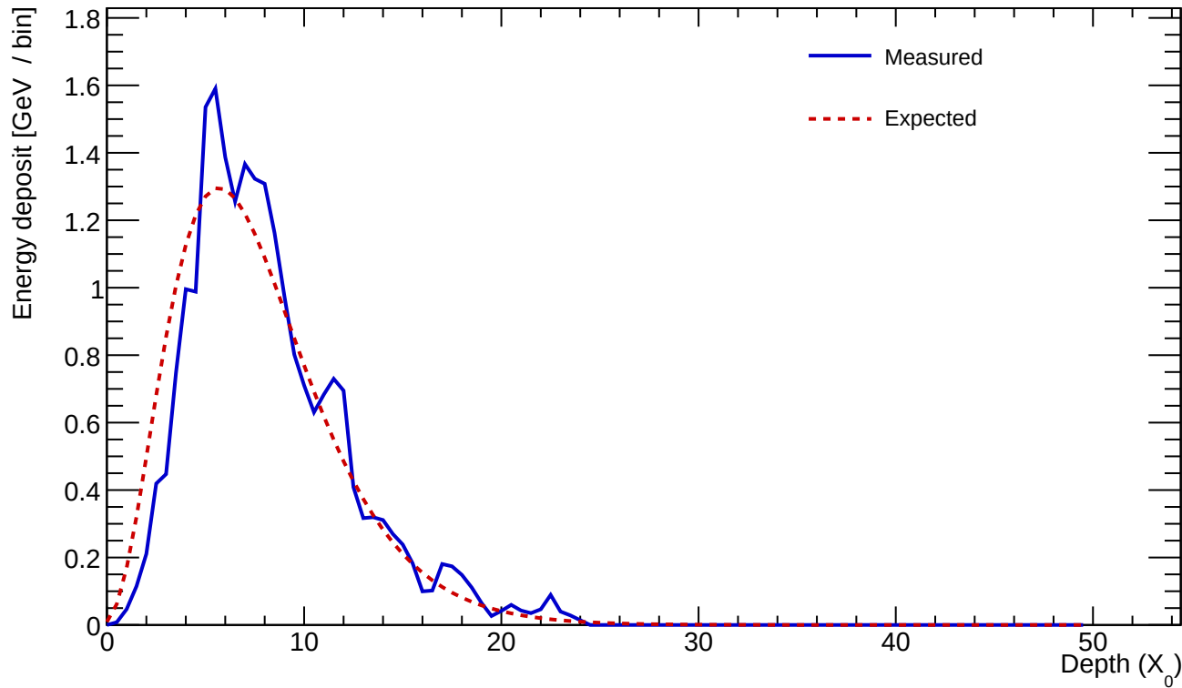
Cluster 774 E=23.484 GeV profileStart=0.50 X_0 \chi=0.1485
