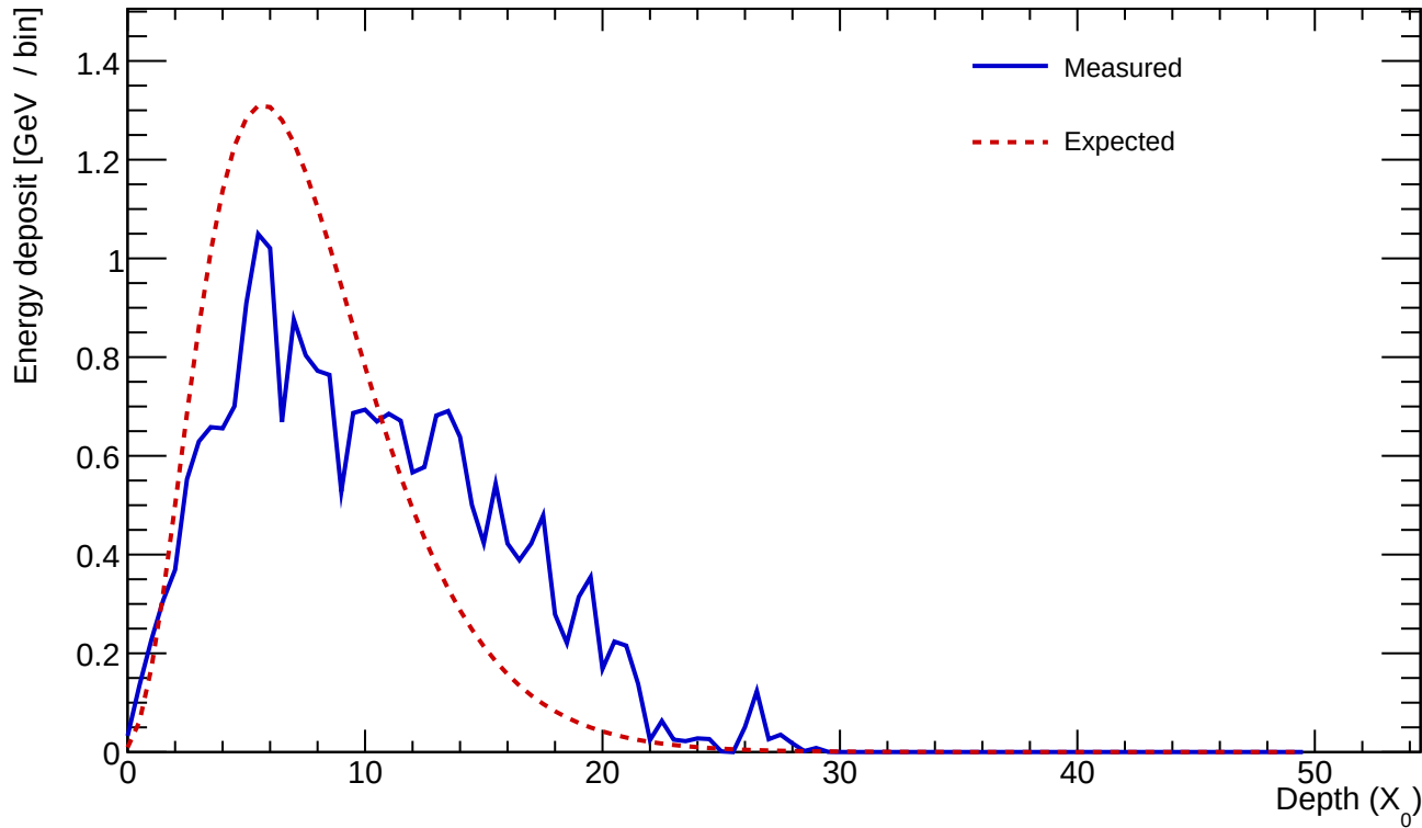
Cluster 586 E=23.768 GeV profileStart=0.50 X_0 \chi=0.4358
