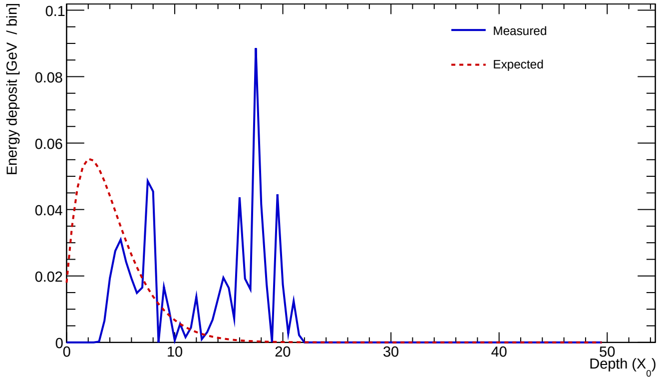
Cluster 415 E=0.678 GeV profileStart=4.00 X_0 \chi=0.9853
