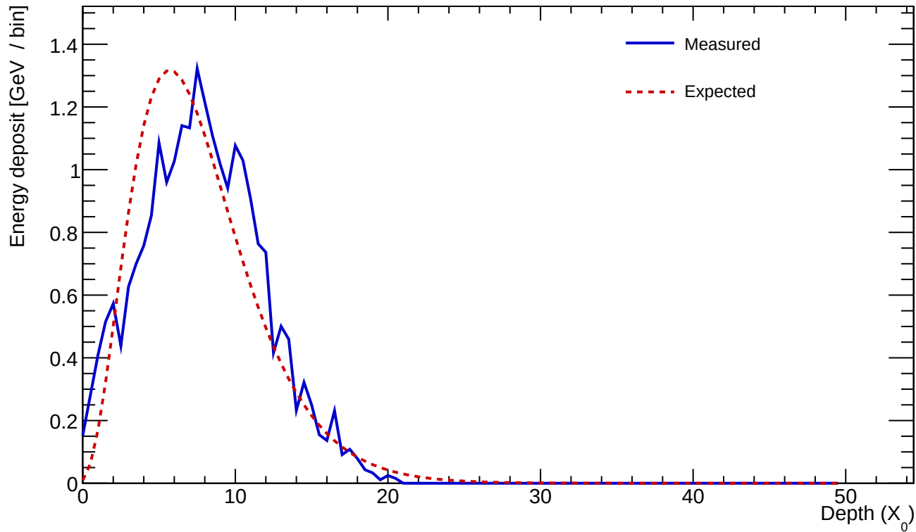
Cluster 709 E=23.881 GeV profileStart=1.00 X_0 \chi=0.2079
