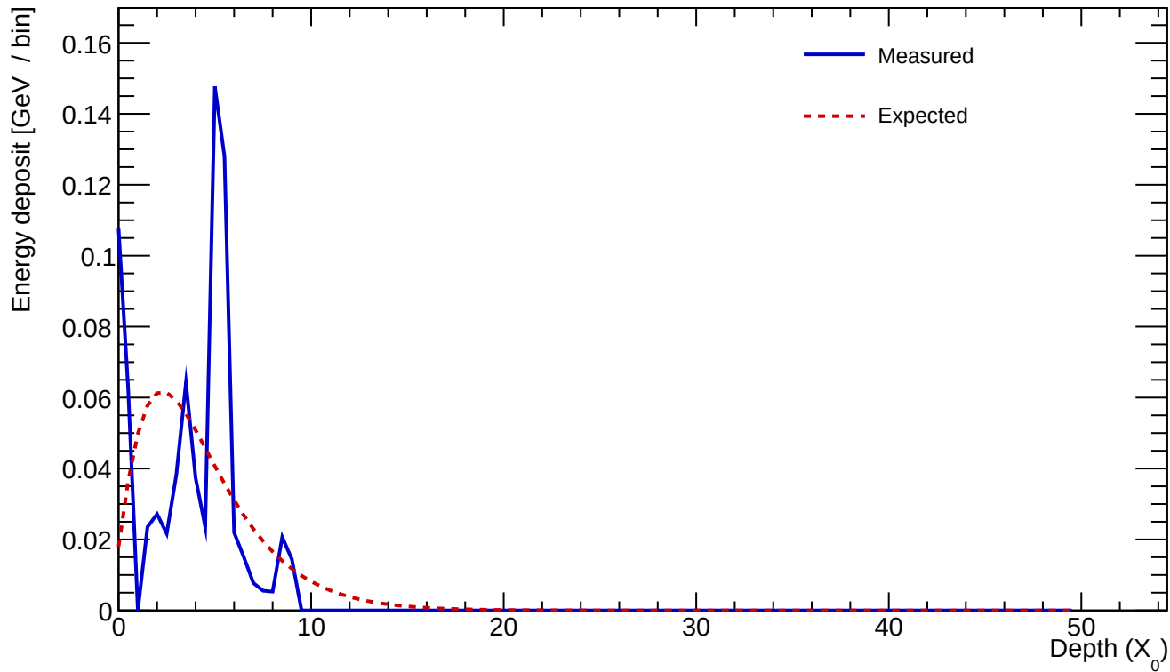
Cluster 116 E=0.772 GeV profileStart=1.50 X_0 \chi=0.7661
