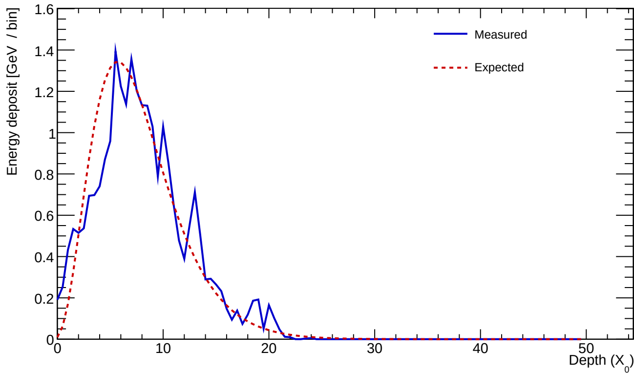
Cluster 652 E=24.410 GeV profileStart=0.50 X_0 \chi=0.2062
