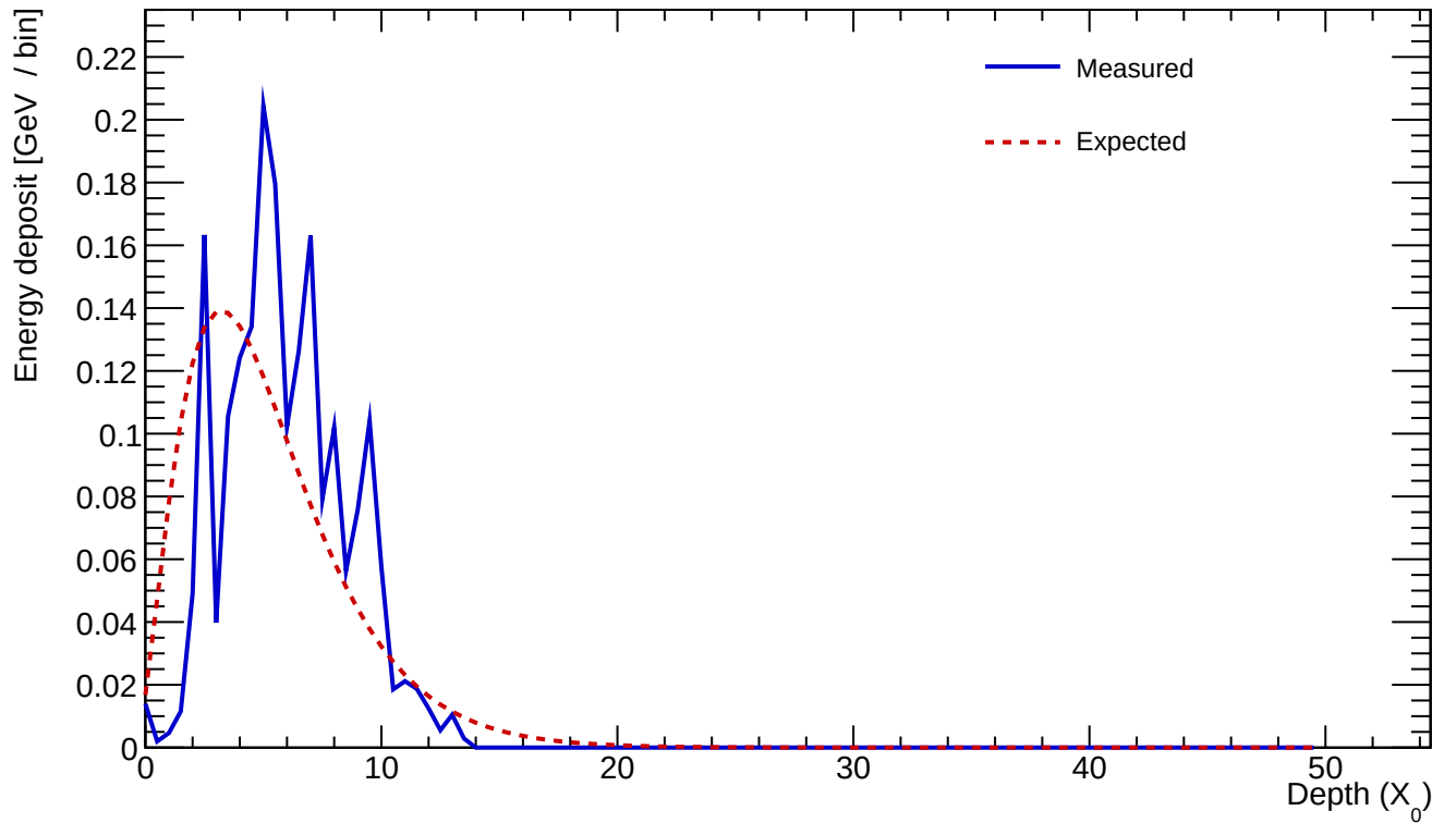
Cluster 562 E=1.988 GeV profileStart=1.50 X_0 \chi=0.3106
