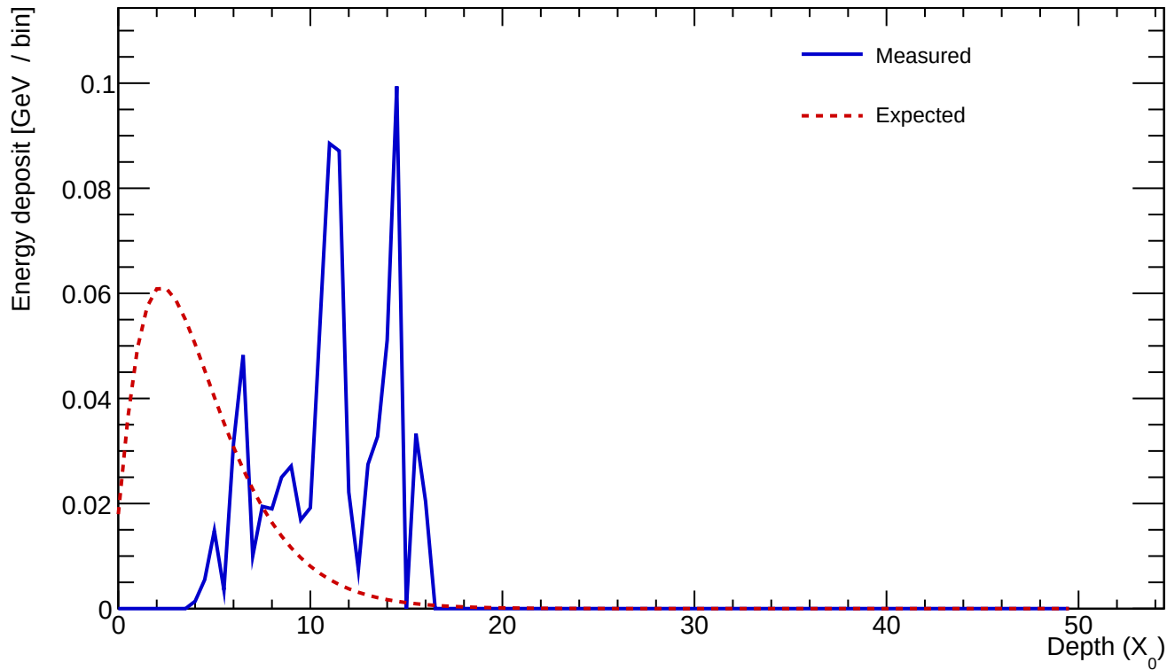
Cluster 705 E=0.765 GeV profileStart=9.50 X_0 \chi=0.6841
