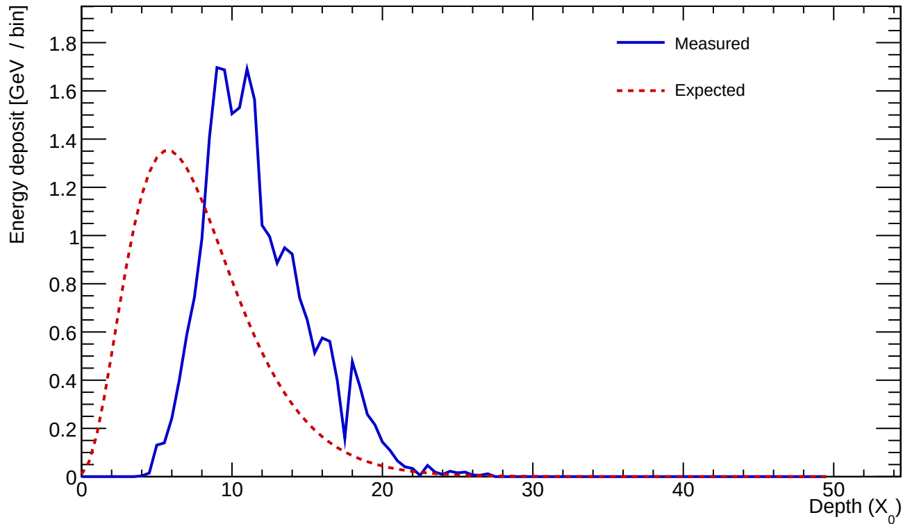
Cluster 906 E=24.602 GeV profileStart=4.50 X_0 \chi=0.1893
