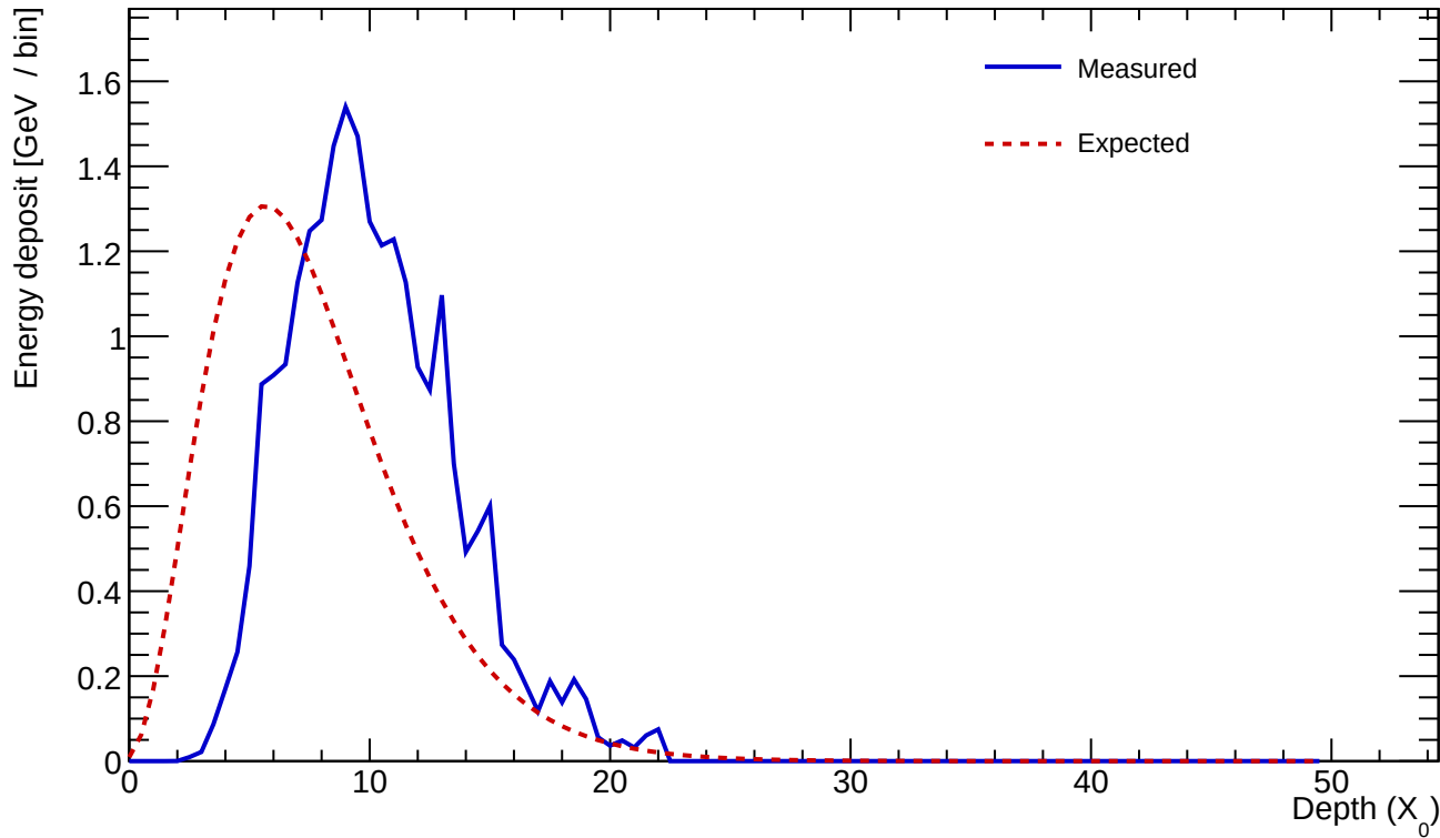
Cluster 309 E=23.693 GeV profileStart=3.00 X_0 \chi=0.1287
