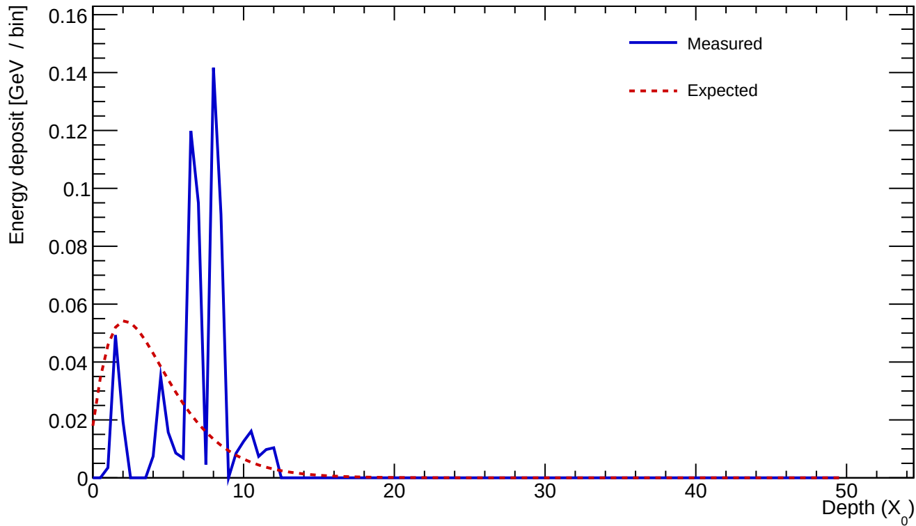
Cluster 767 E=0.662 GeV profileStart=4.00 X_0 \chi=0.9050
