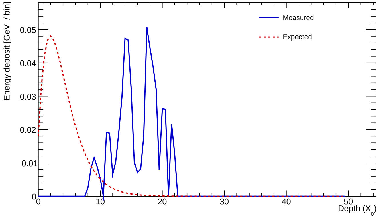
Cluster 347 E=0.571 GeV profileStart=13.00 X_0 \chi=0.6288
