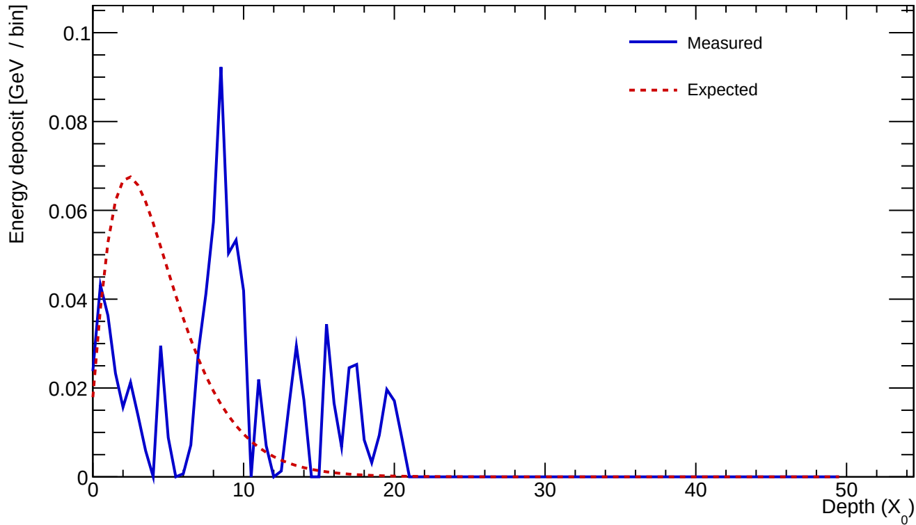
Cluster 764 E=0.861 GeV profileStart=6.50 X_0 \chi=0.8125
