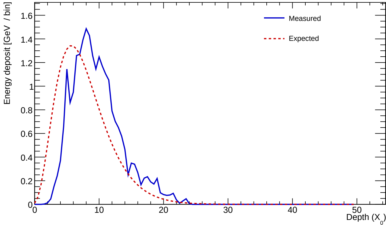
Cluster 379 E=24.408 GeV profileStart=2.00 X_0 \chi=0.1104
