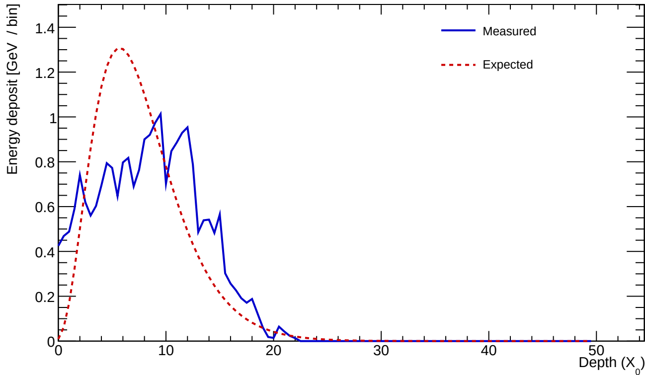
Cluster 278 E=23.698 GeV profileStart=1.50 X_0 \chi=0.3856
