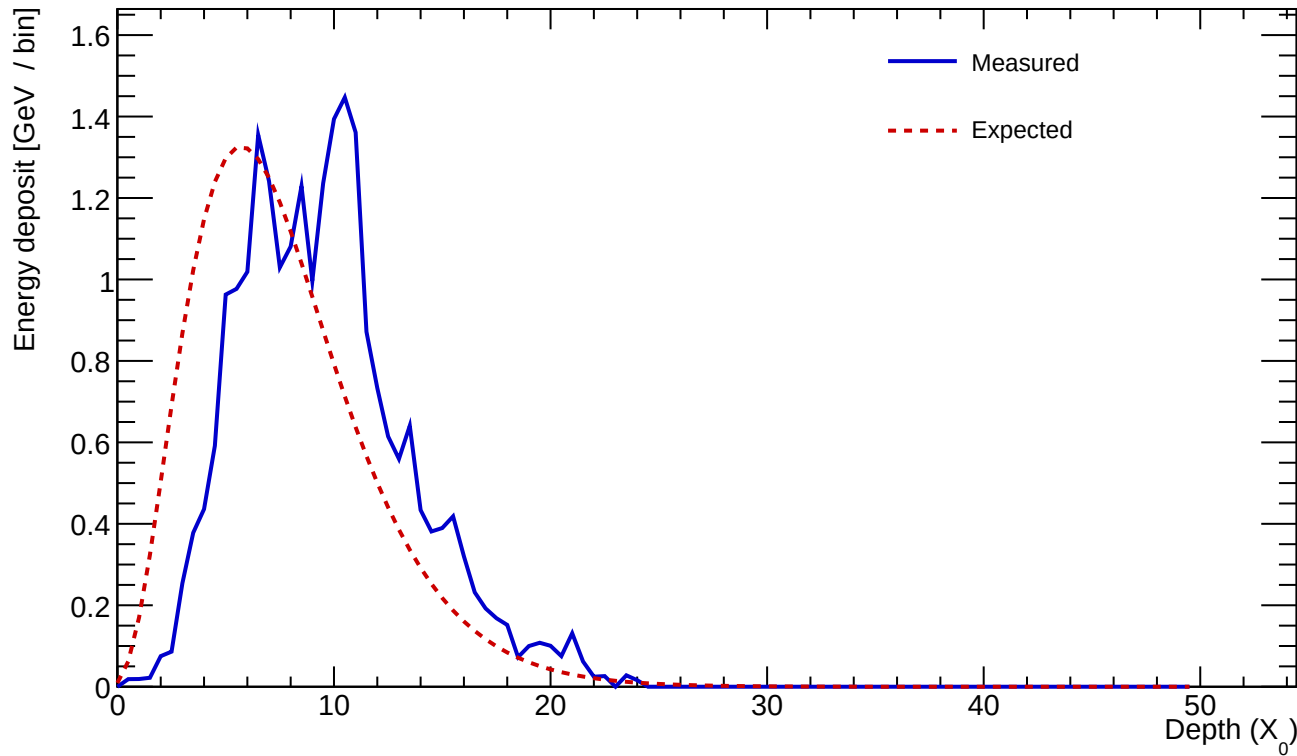
Cluster 760 E=24.060 GeV profileStart=2.00 X_0 \chi=0.1565
