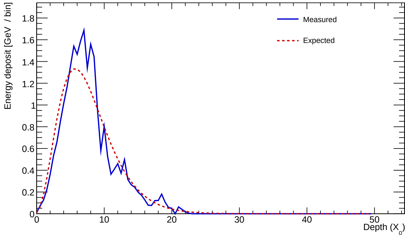
Cluster 237 E=24.199 GeV profileStart=0.50 X_0 \chi=0.1933
