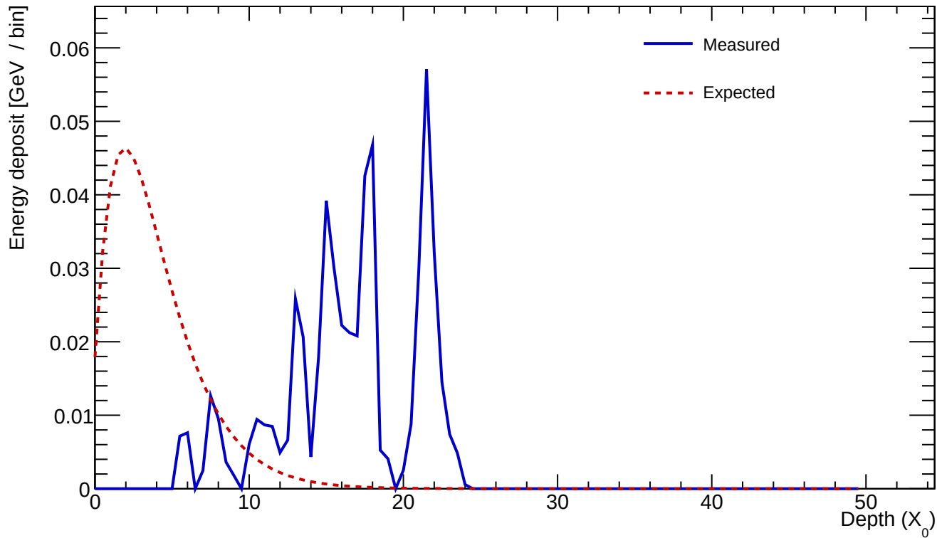
Cluster 473 E=0.548 GeV profileStart=14.50 X_0 \chi=0.7978
