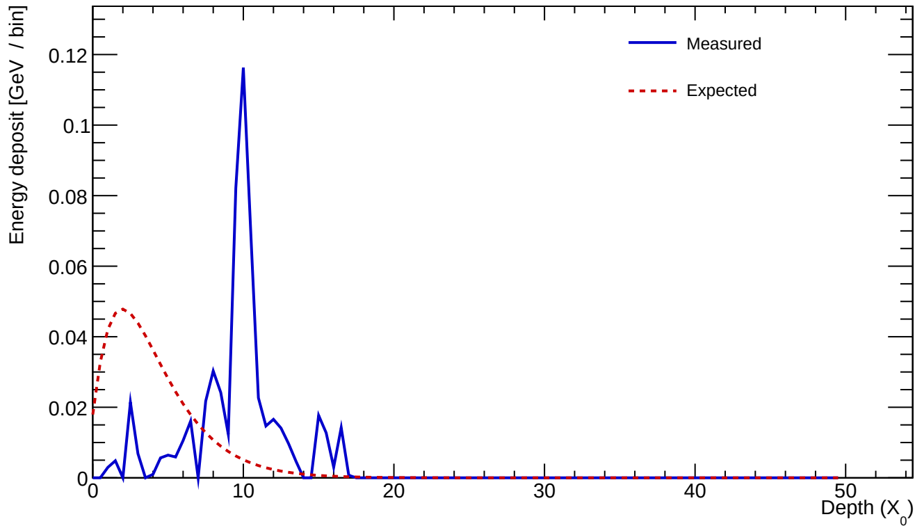
Cluster 599 E=0.568 GeV profileStart=7.50 X_0 \chi=0.7418
