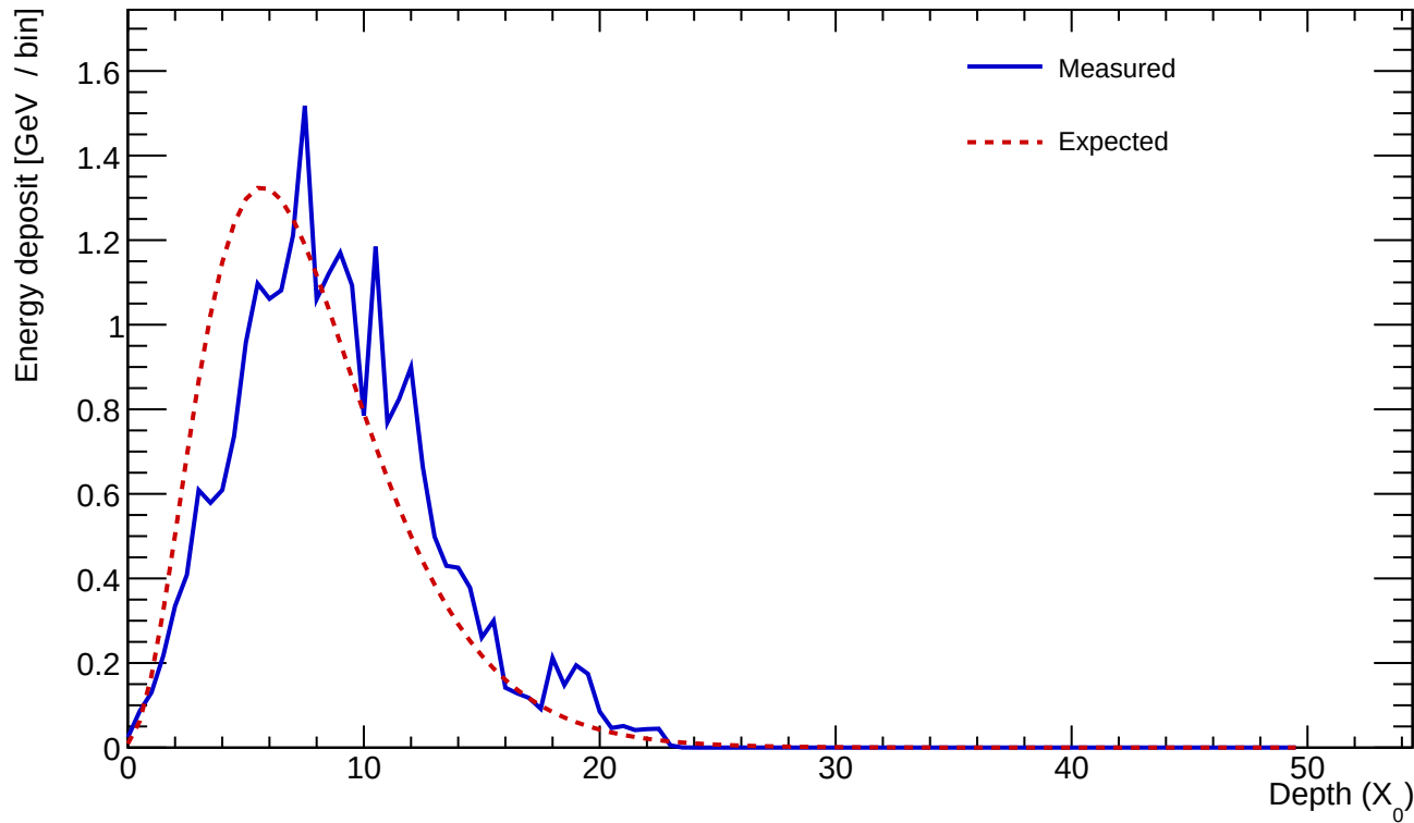
Cluster 155 E=24.048 GeV profileStart=1.50 X_0 \chi=0.1886
