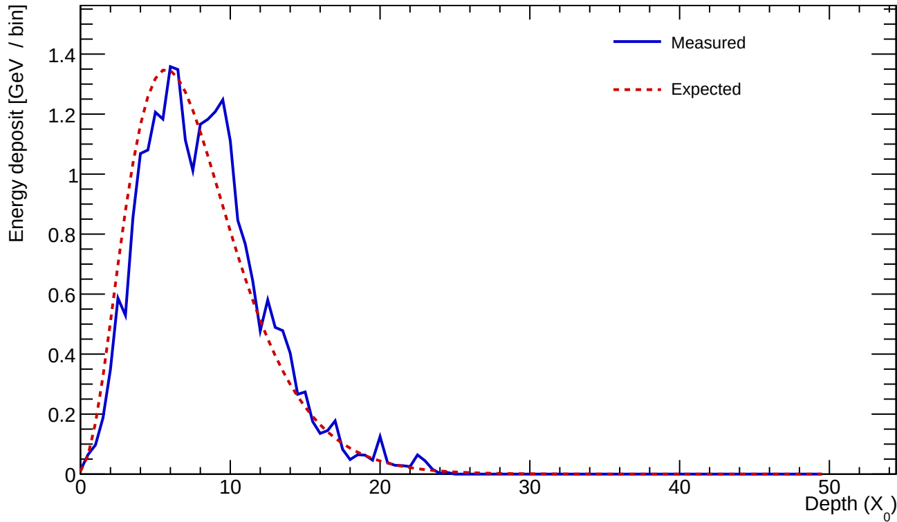
Cluster 493 E=24.511 GeV profileStart=0.50 X_0 \chi=0.1172
