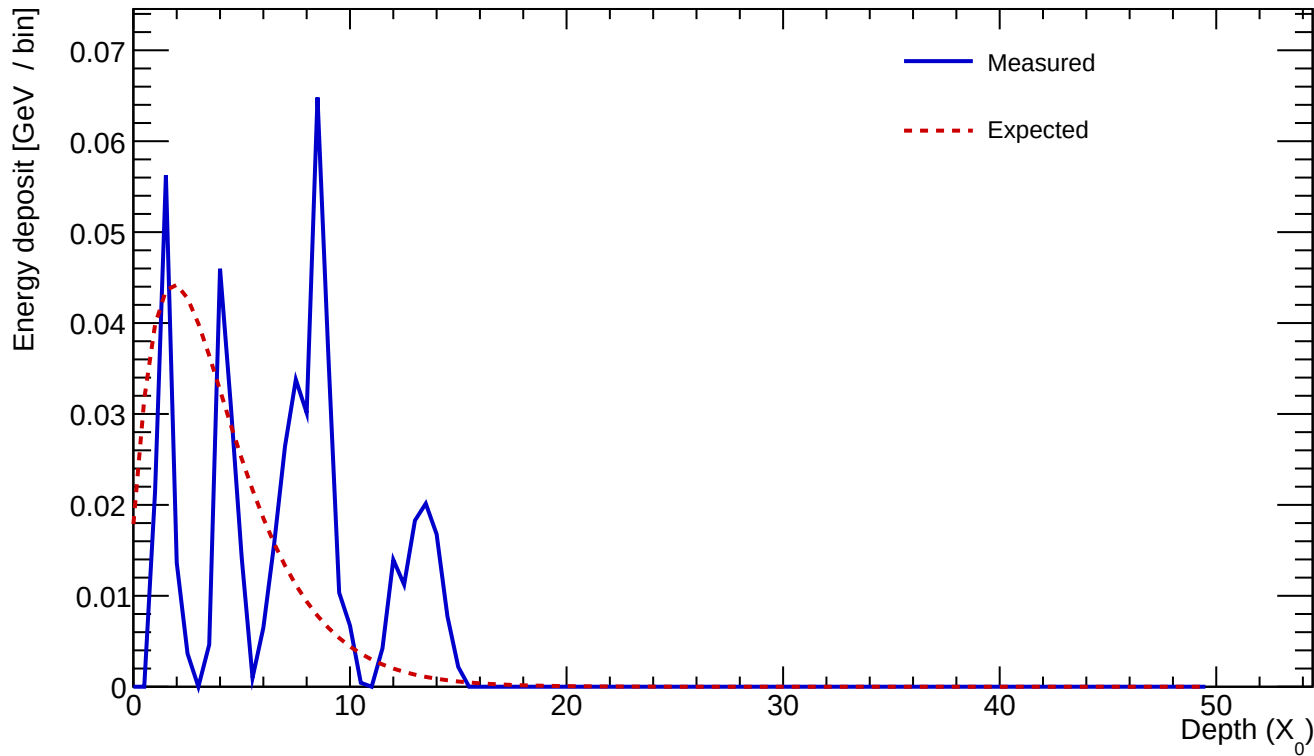
Cluster 876 E=0.518 GeV profileStart=6.50 X_0 \chi=0.8200
