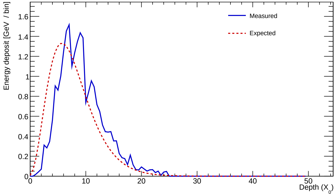
Cluster 73 E=24.158 GeV profileStart=1.50 X_0 \chi=0.1394
