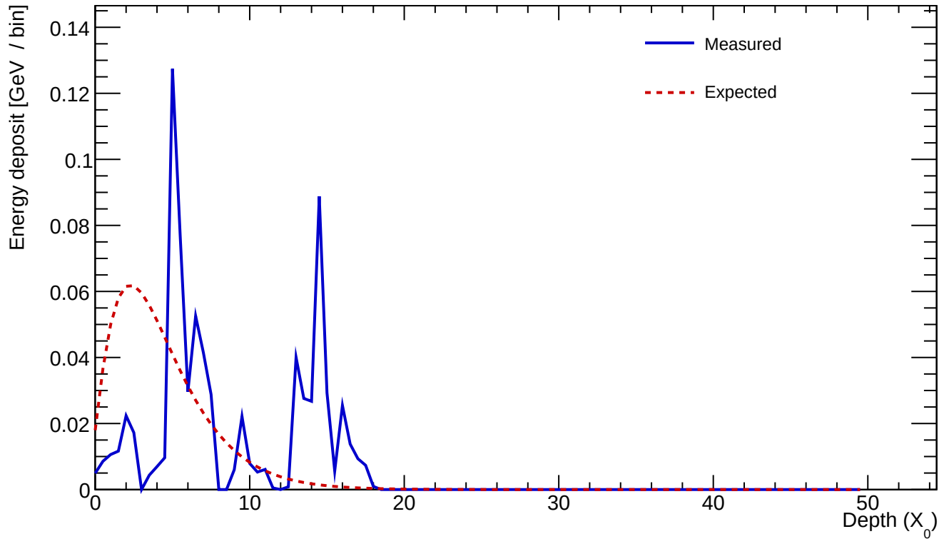
Cluster 137 E=0.777 GeV profileStart=2.50 X_0 \chi=0.9804
