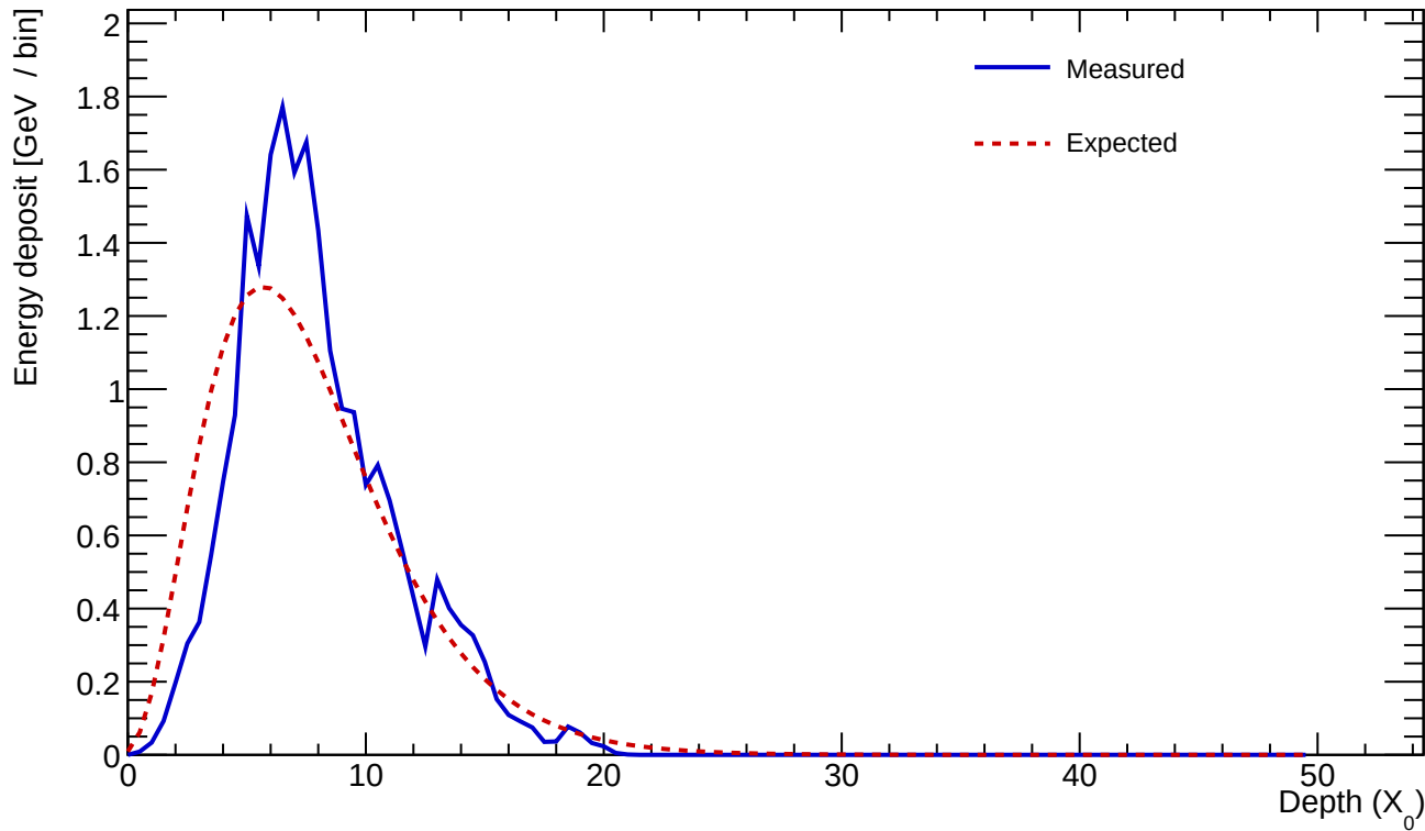
Cluster 20 E=23.171 GeV profileStart=1.00 X_0 \chi=0.2008
