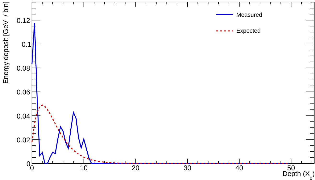
Cluster 539 E=0.584 GeV profileStart=5.00 X_0 \chi=0.7937
