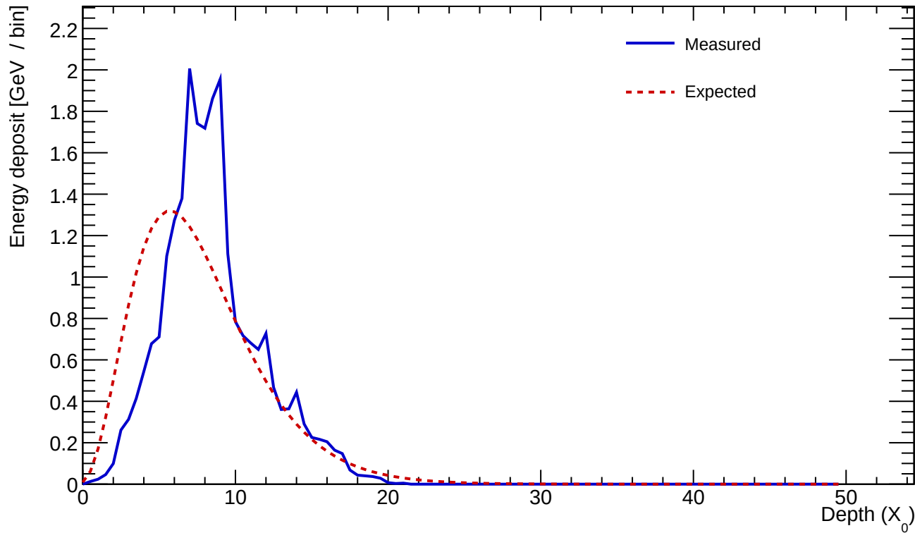
Cluster 82 E=23.928 GeV profileStart=1.50 X_0 \chi=0.2627
