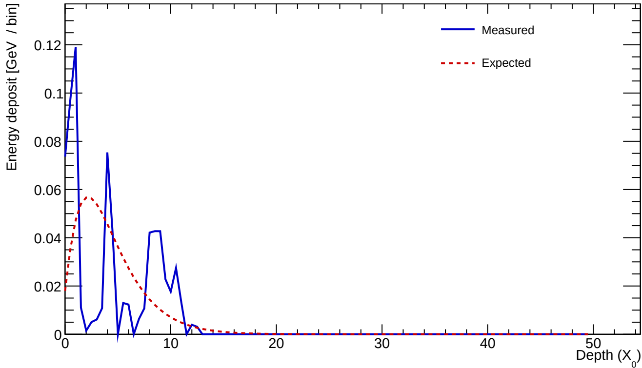
Cluster 792 E=0.700 GeV profileStart=3.50 X_0 \chi=1.0055
