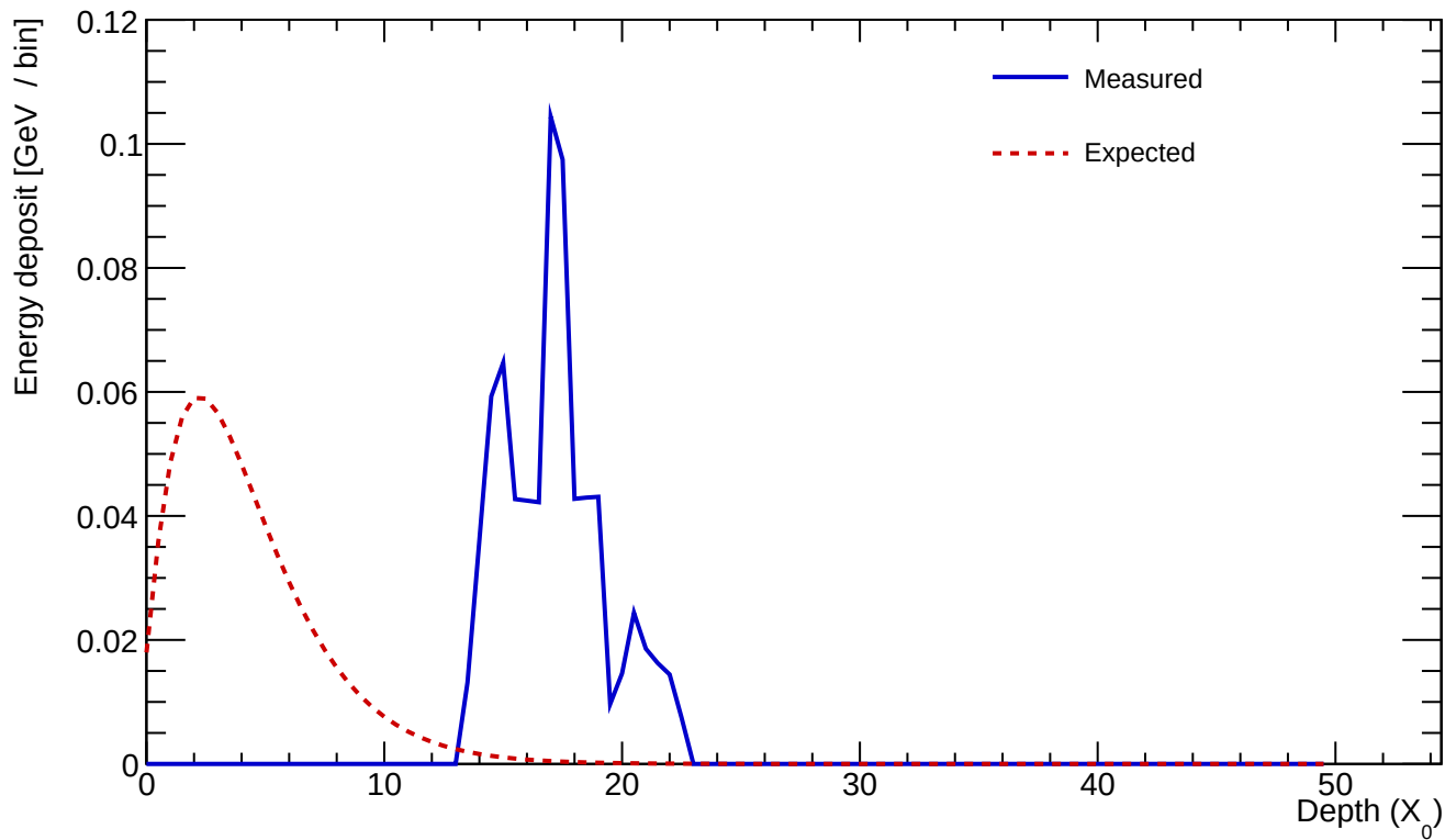
Cluster 965 E=0.737 GeV profileStart=13.50 X_0 \chi=0.3015
