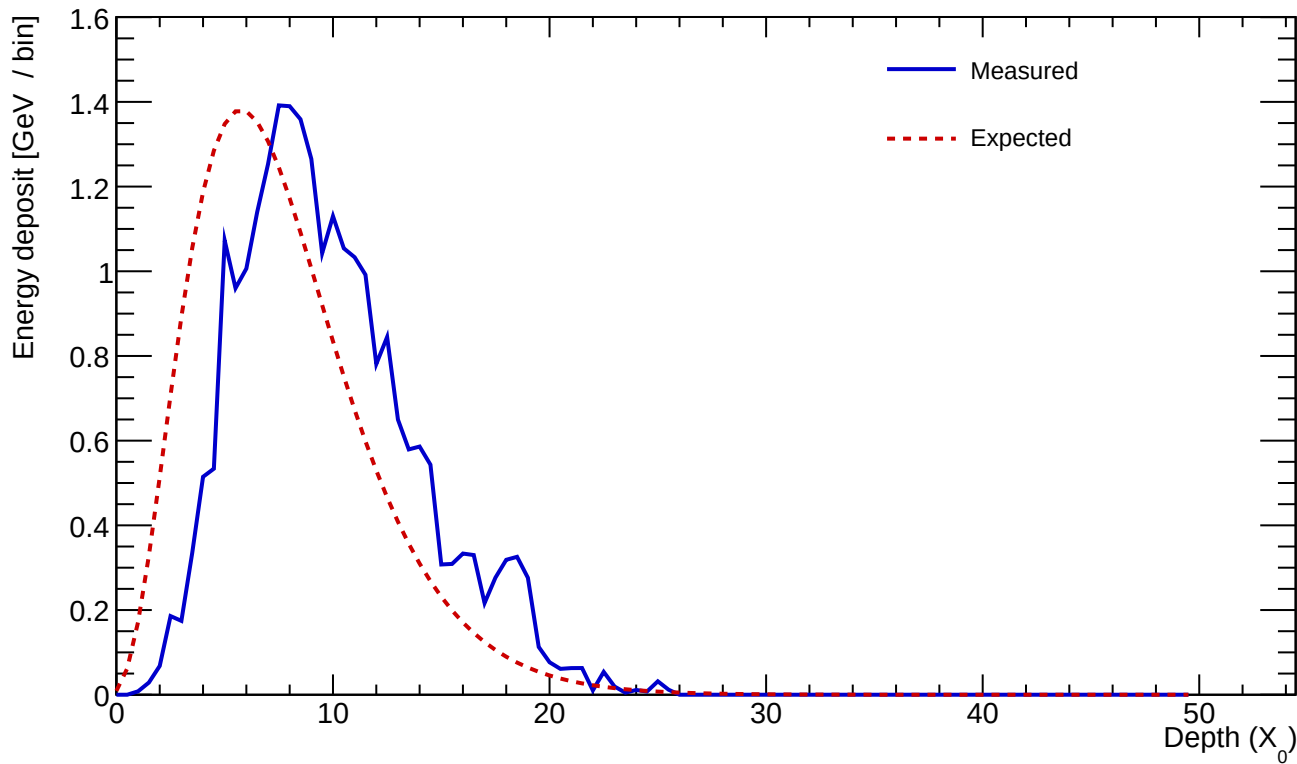
Cluster 909 E=25.142 GeV profileStart=2.00 X_0 \chi=0.1133
