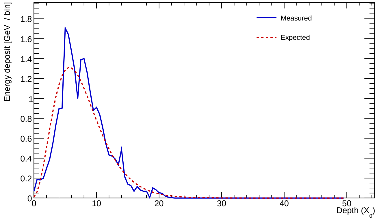
Cluster 91 E=23.758 GeV profileStart=0.50 X_0 \chi=0.1885
