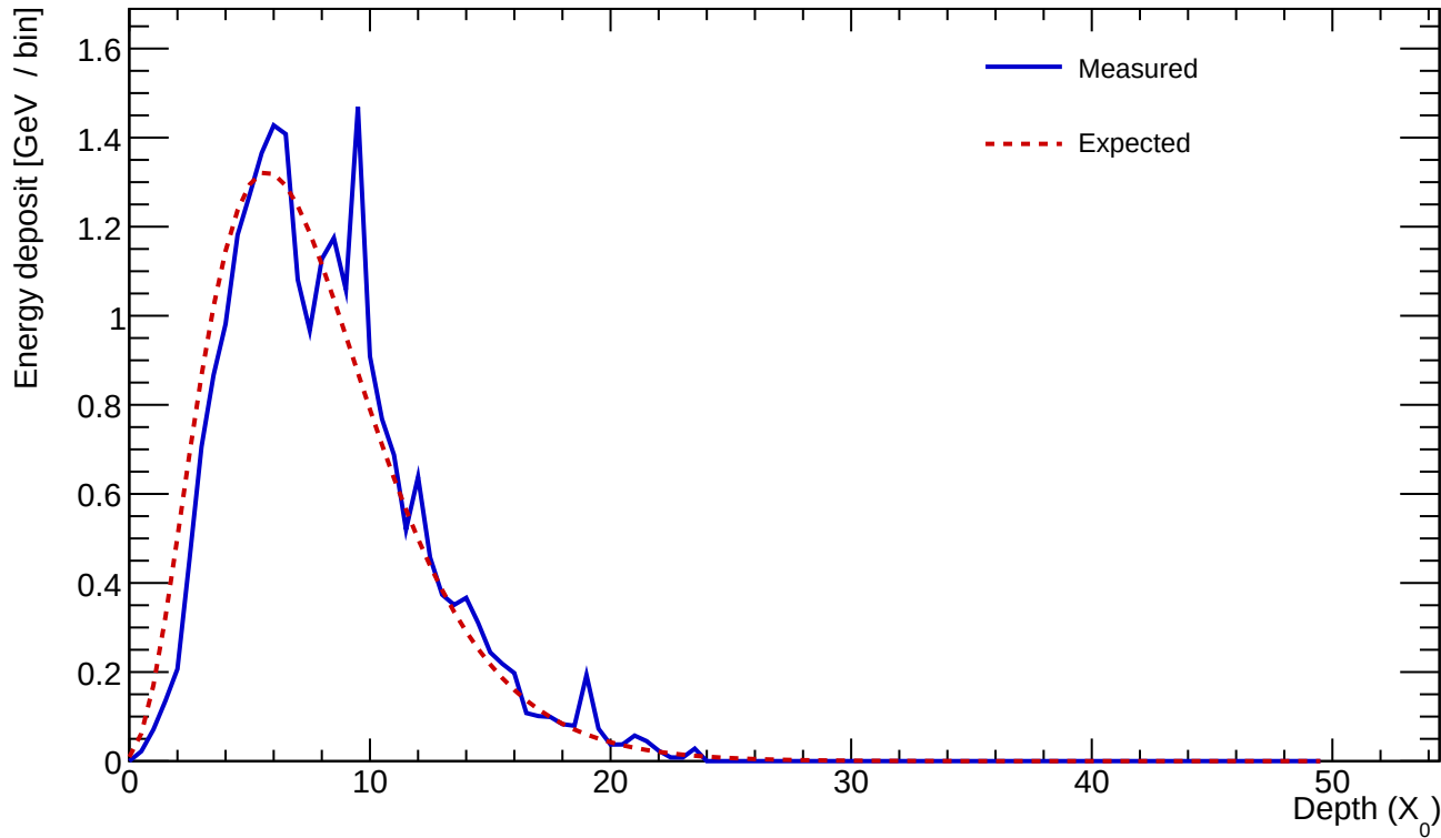
Cluster 516 E=23.998 GeV profileStart=0.50 X_0 \chi=0.1077
