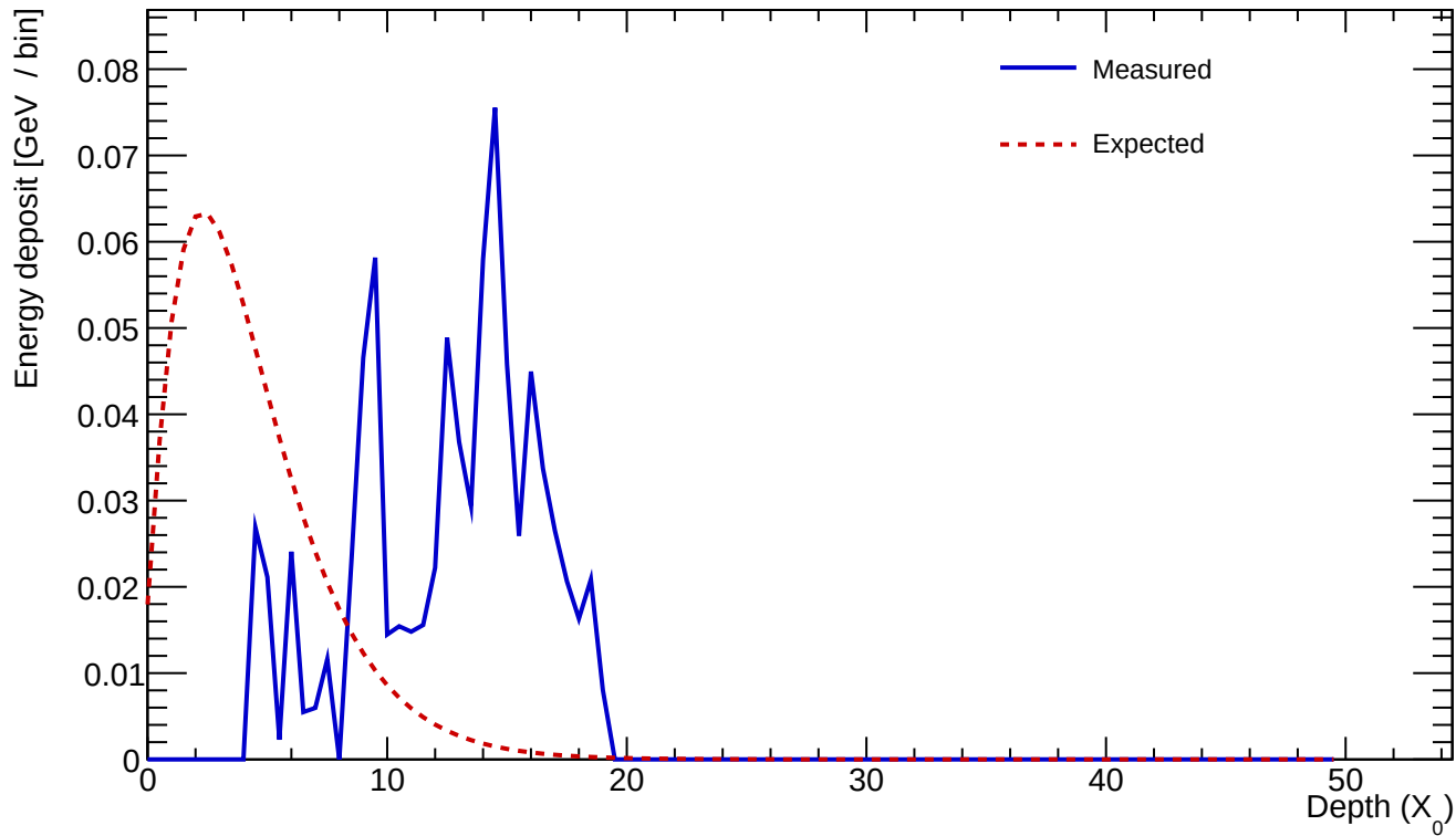
Cluster 70 E=0.799 GeV profileStart=11.50 X_0 \chi=0.5649
