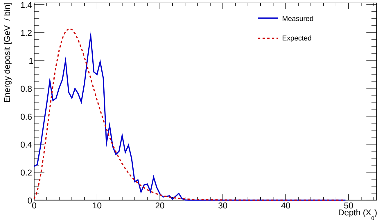
Cluster 861 E=22.110 GeV profileStart=0.50 X_0 \chi=0.3244
