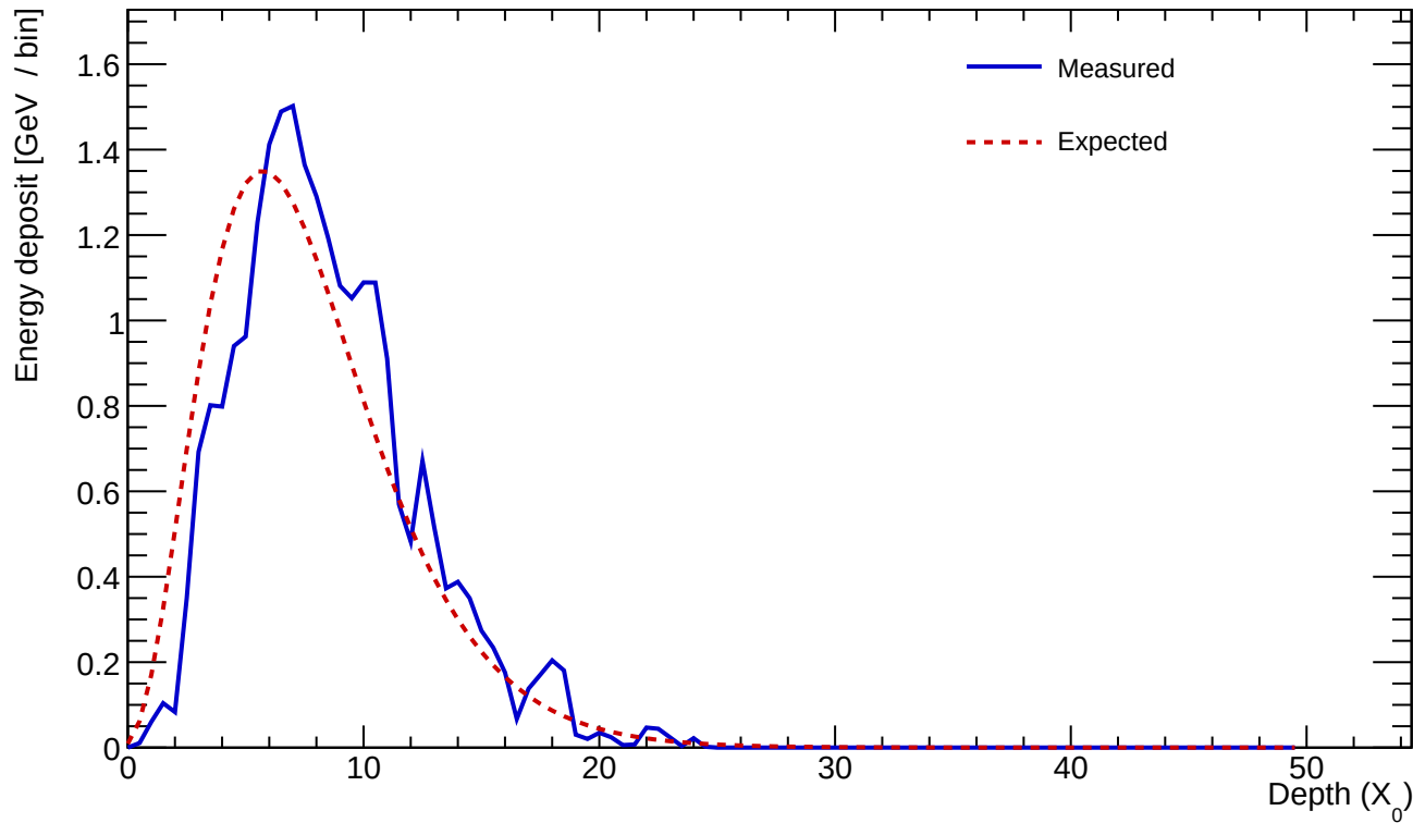
Cluster 167 E=24.565 GeV profileStart=1.00 X_0 \chi=0.1264
