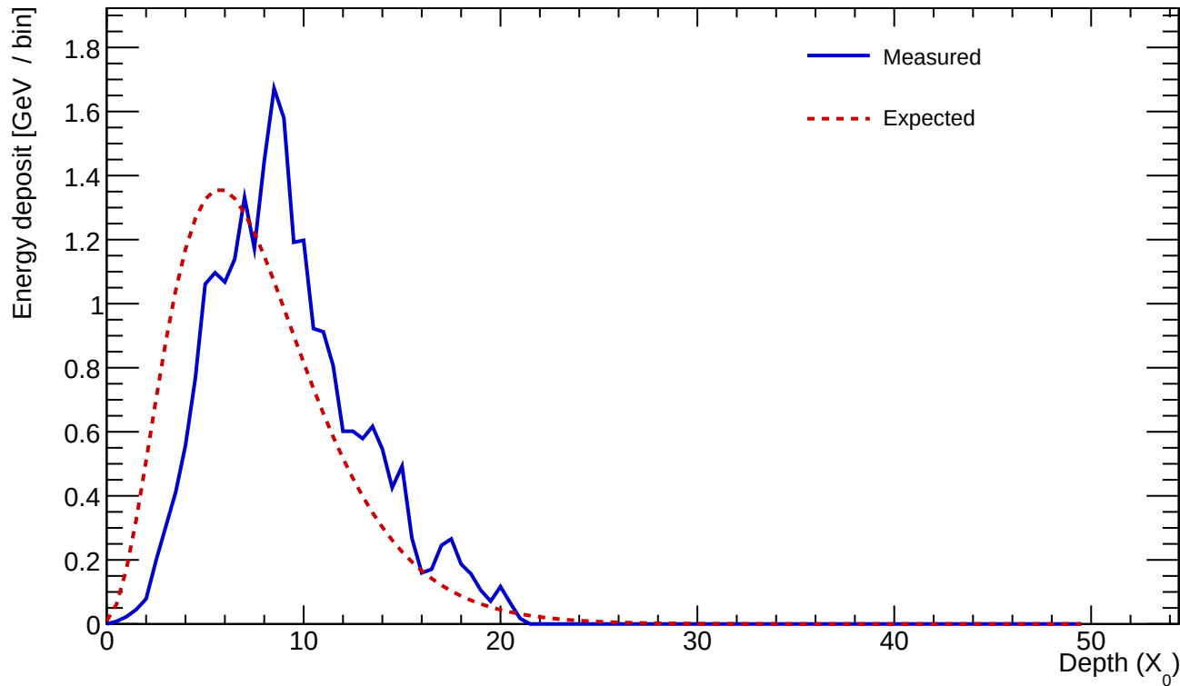
Cluster 257 E=24.678 GeV profileStart=1.50 X_0 \chi=0.1351
