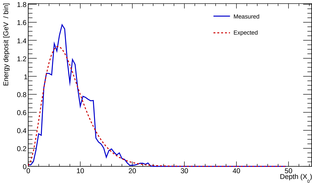
Cluster 299 E=24.185 GeV profileStart=0.50 X_0 \chi=0.1536
