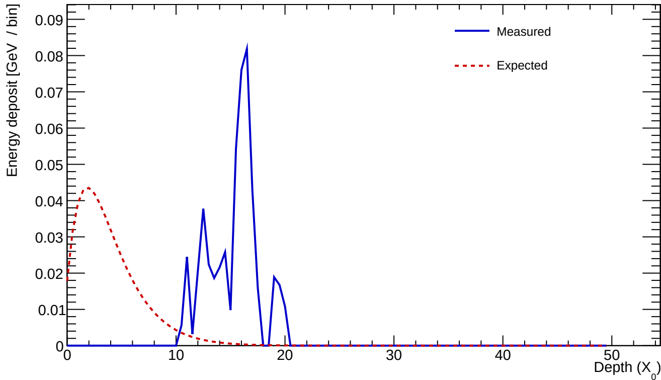
Cluster 785 E=0.508 GeV profileStart=12.00 X_0 \chi=0.6632
