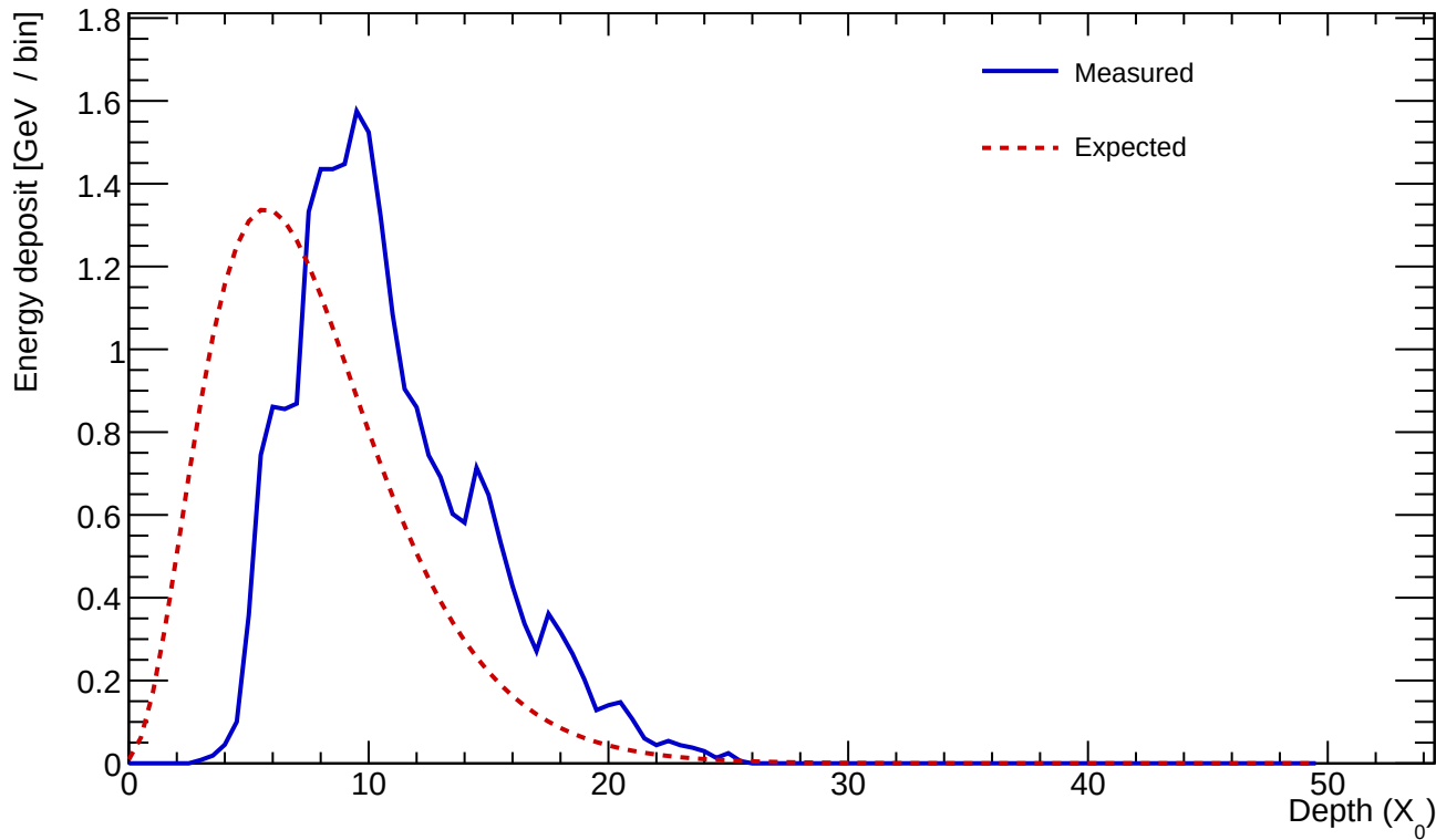
Cluster 220 E=24.313 GeV profileStart=3.00 X_0 \chi=0.1551
