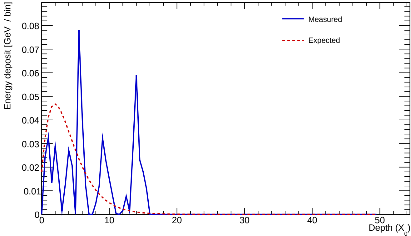
Cluster 928 E=0.553 GeV profileStart=0.50 X_0 \chi=0.9403
