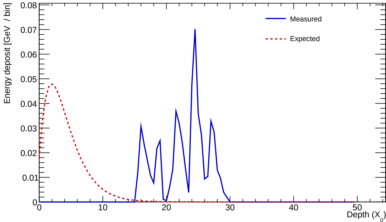
Cluster 635 E=0.569 GeV profileStart=21.00 X_0 \chi=0.6697
