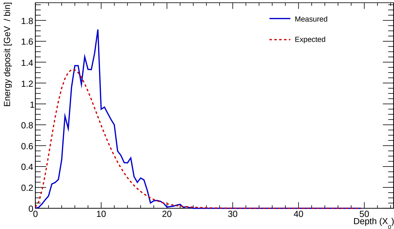
Cluster 143 E=24.138 GeV profileStart=1.50 X_0 \chi=0.1550
