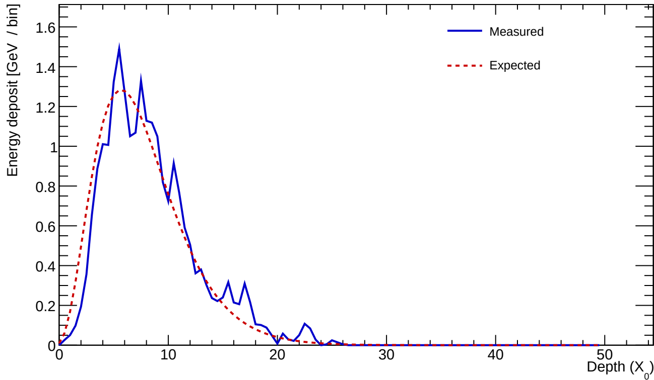
Cluster 413 E=23.217 GeV profileStart=0.50 X_0 \chi=0.1413
