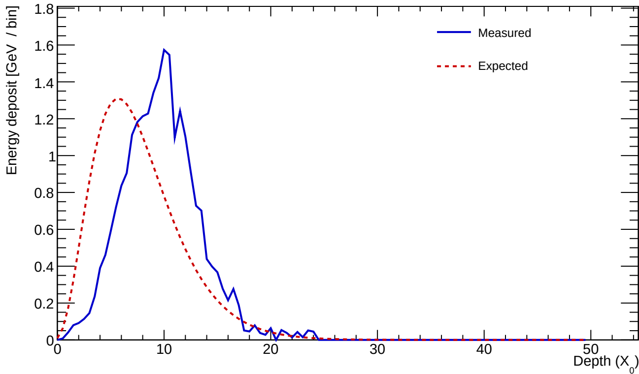
Cluster 910 E=23.743 GeV profileStart=3.00 X_0 \chi=0.2019
