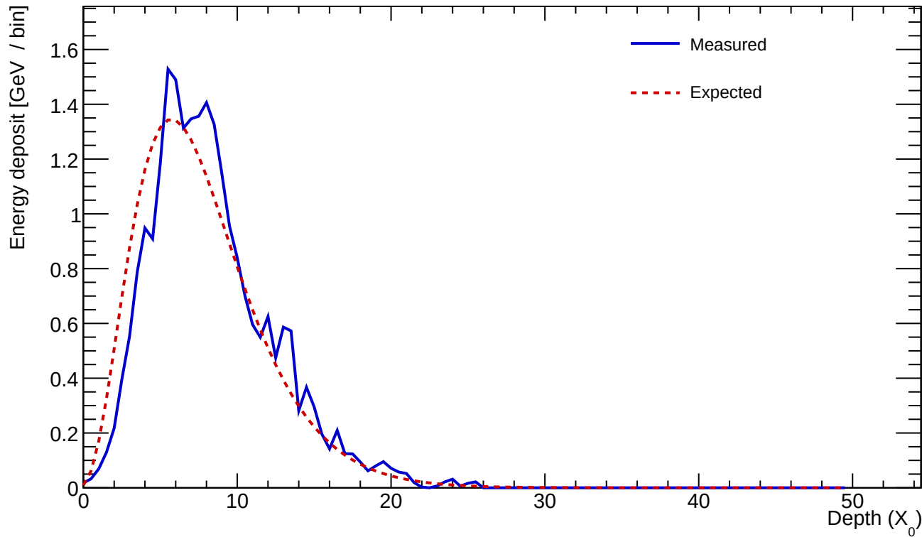
Cluster 1 E=24.439 GeV profileStart=1.00 X_0 \chi=0.1299
