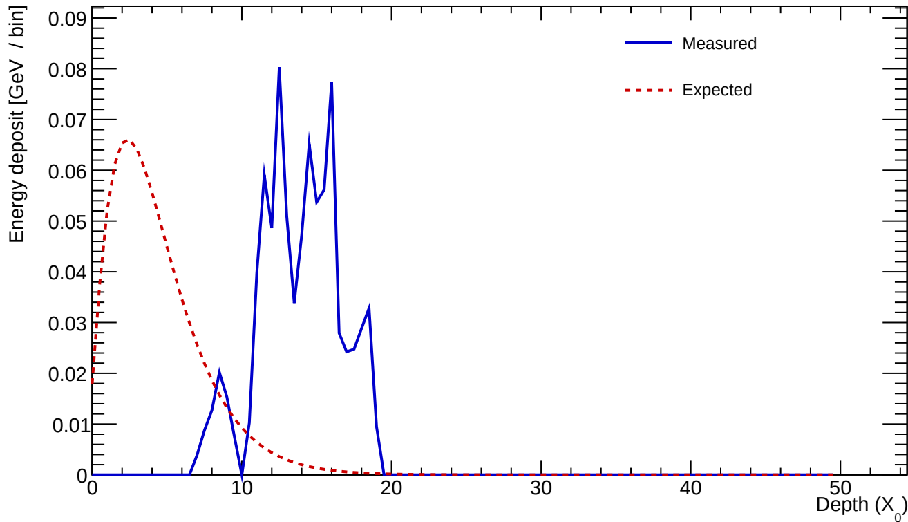
Cluster 107 E=0.839 GeV profileStart=10.50 X_0 \chi=0.3190
