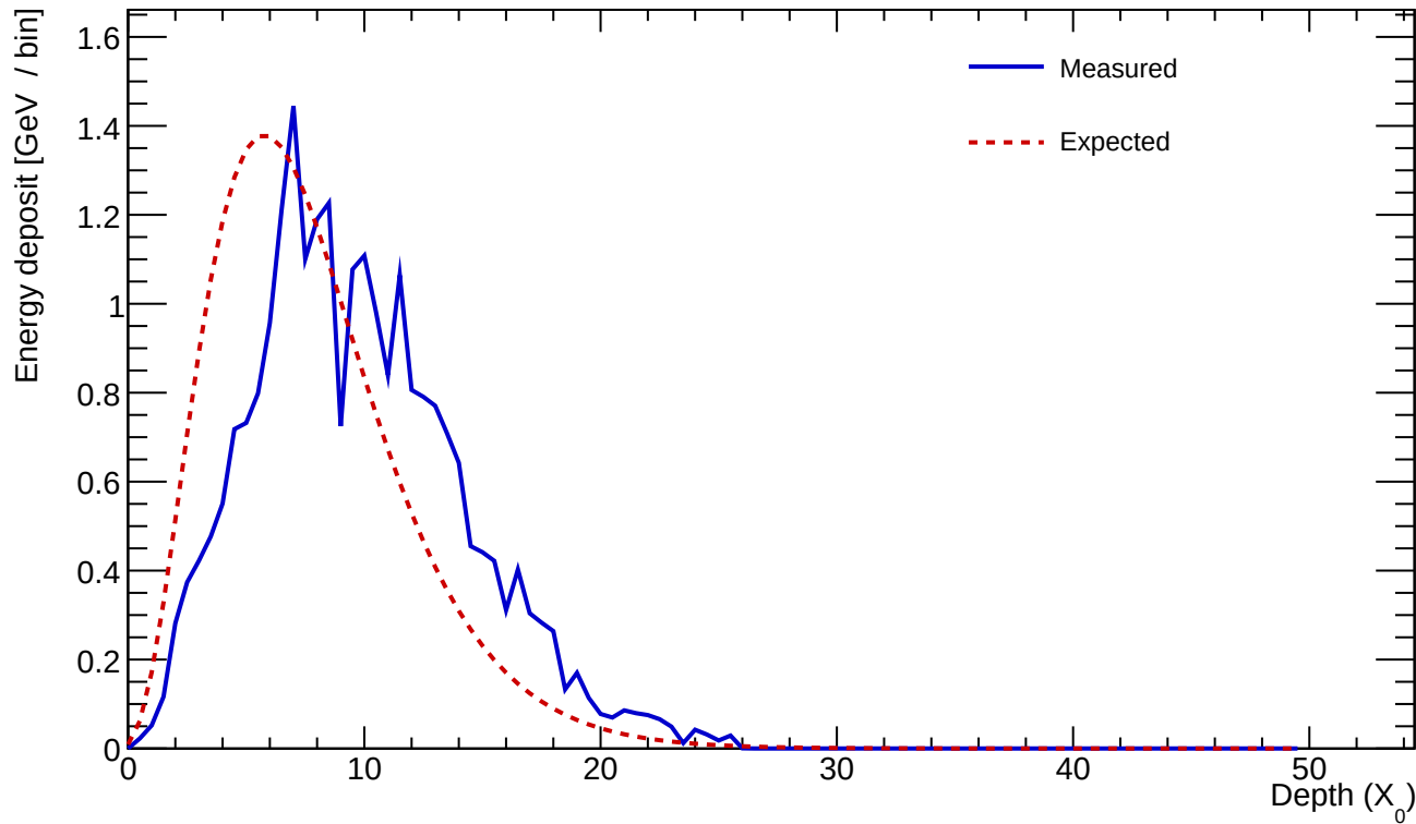
Cluster 744 E=25.125 GeV profileStart=2.00 X_0 \chi=0.1997
