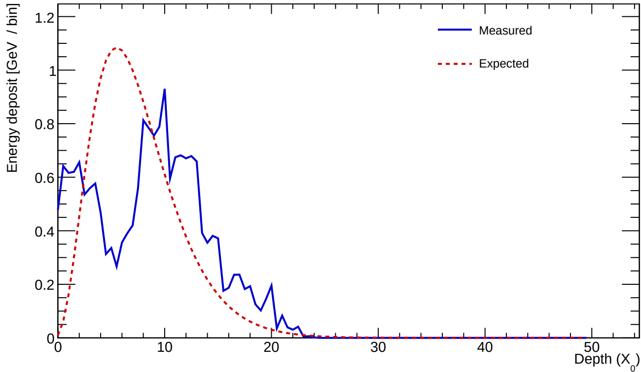
Cluster 793 E=19.344 GeV profileStart=3.00 X_0 \chi=0.5329
