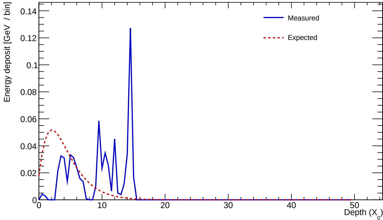
Cluster 932 E=0.626 GeV profileStart=13.50 X_0 \chi=0.8392
