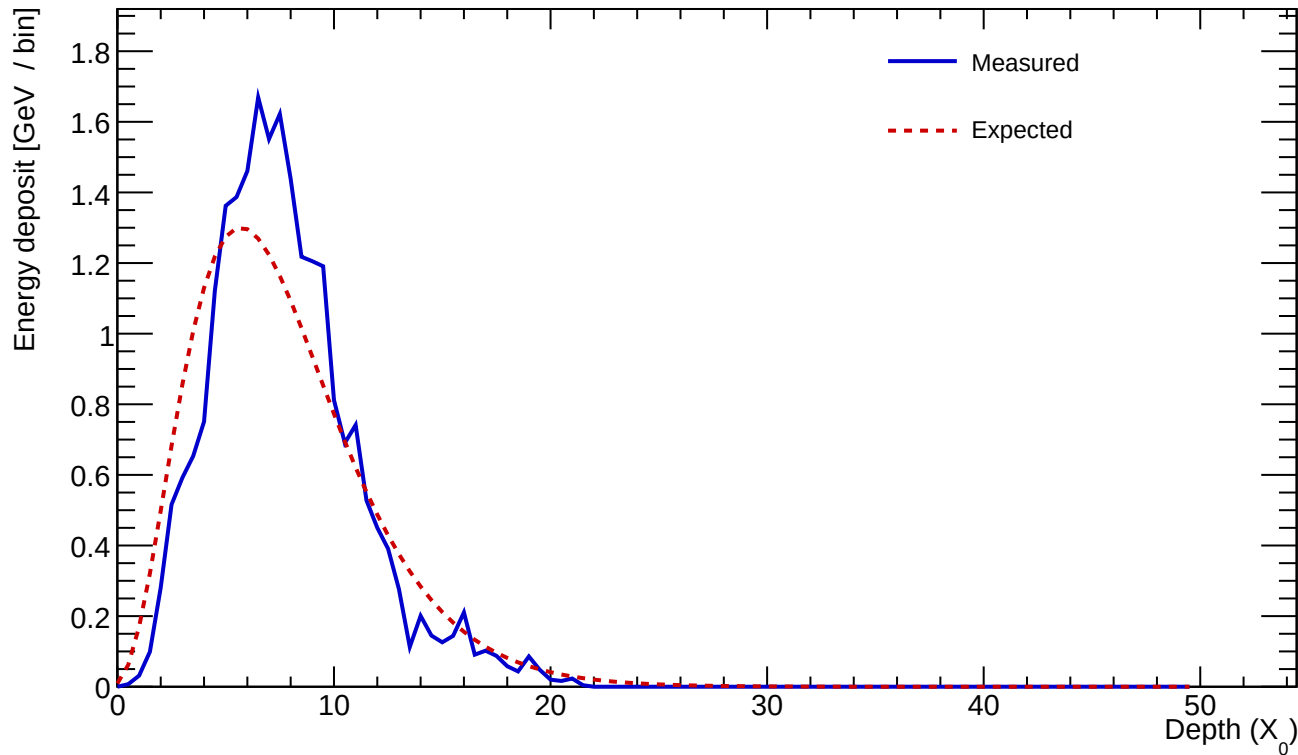
Cluster 556 E=23.563 GeV profileStart=0.50 X_0 \chi=0.1987
