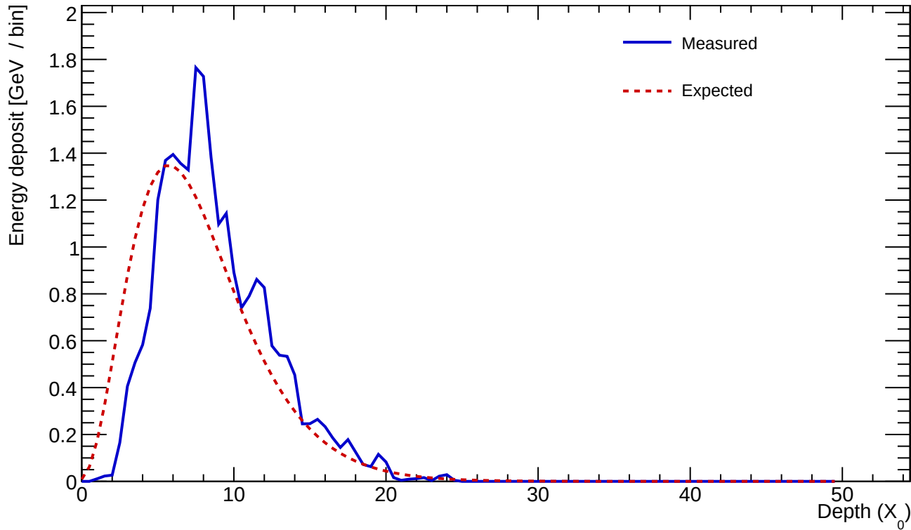
Cluster 677 E=24.510 GeV profileStart=1.50 X_0 \chi=0.1455
