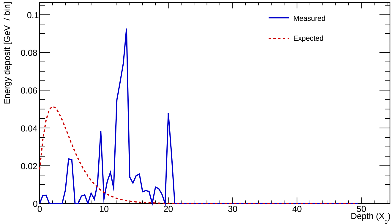
Cluster 618 E=0.621 GeV profileStart=9.00 X_0 \chi=0.8018
