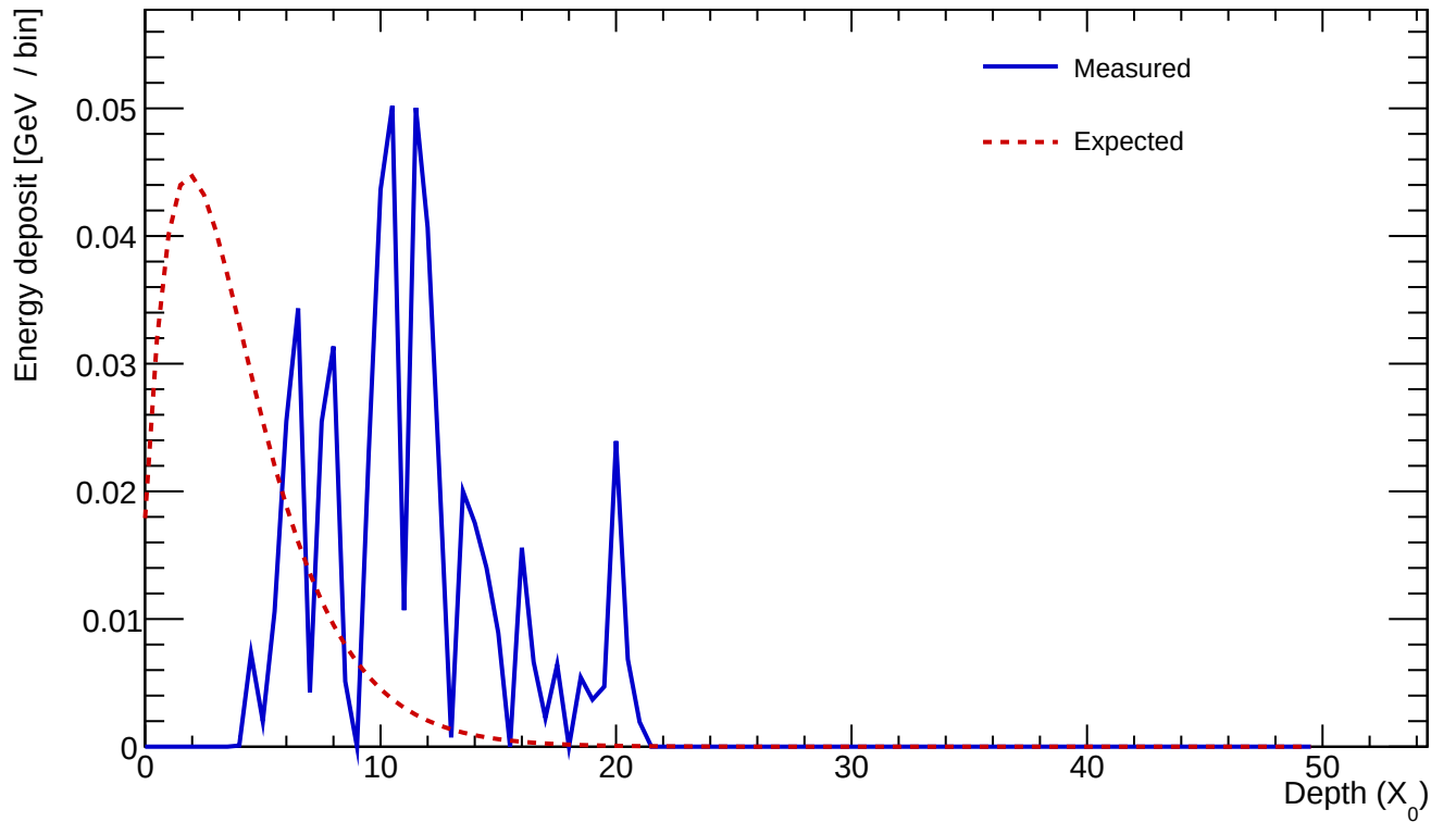
Cluster 153 E=0.524 GeV profileStart=7.50 X_0 \chi=0.6649
