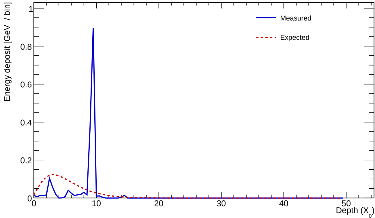
Cluster 1068 E=1.730 GeV profileStart=1.00 X_0 \chi=1.3797
