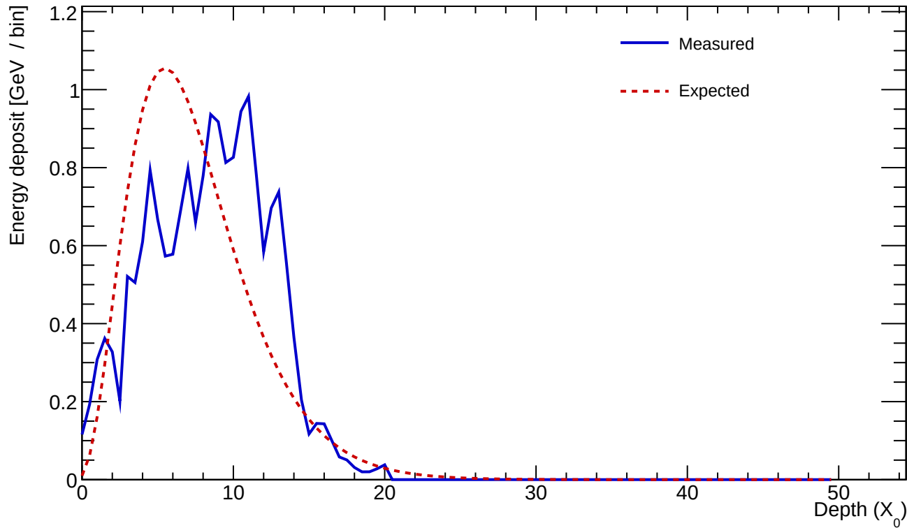
Cluster 377 E=18.783 GeV profileStart=1.50 X_0 \chi=0.3334
