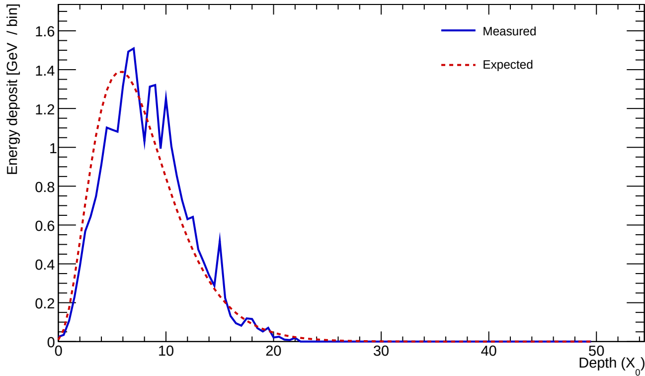
Cluster 860 E=25.345 GeV profileStart=0.50 X_0 \chi=0.1436
