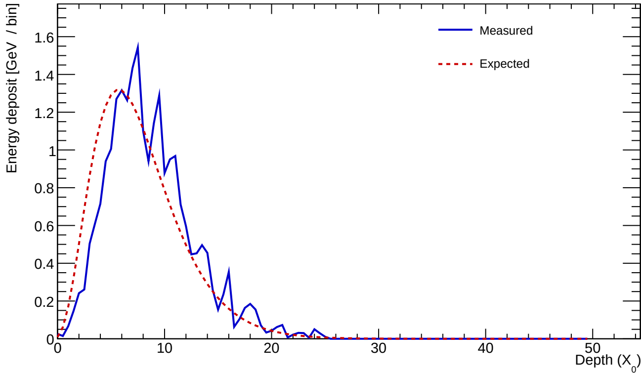
Cluster 668 E=23.923 GeV profileStart=1.00 X_0 \chi=0.1466
