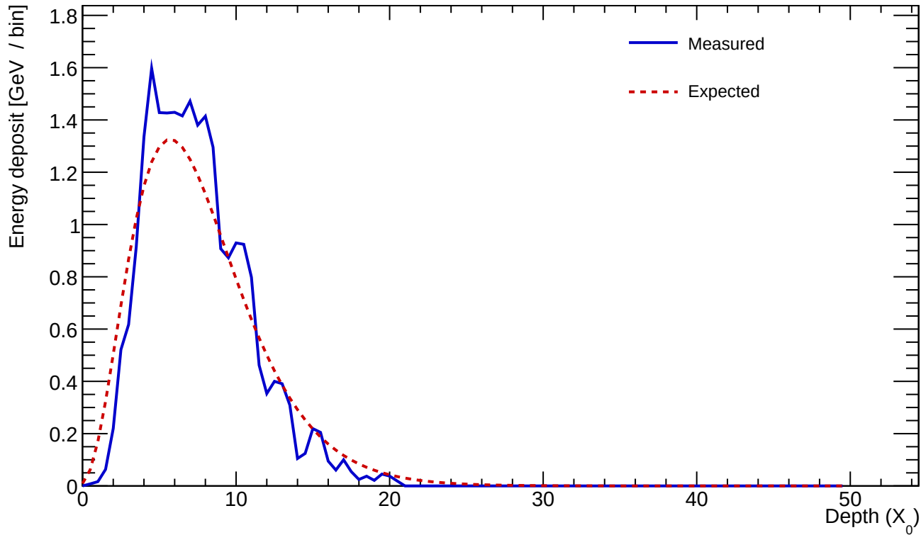
Cluster 196 E=24.050 GeV profileStart=0.50 X_0 \chi=0.1841
