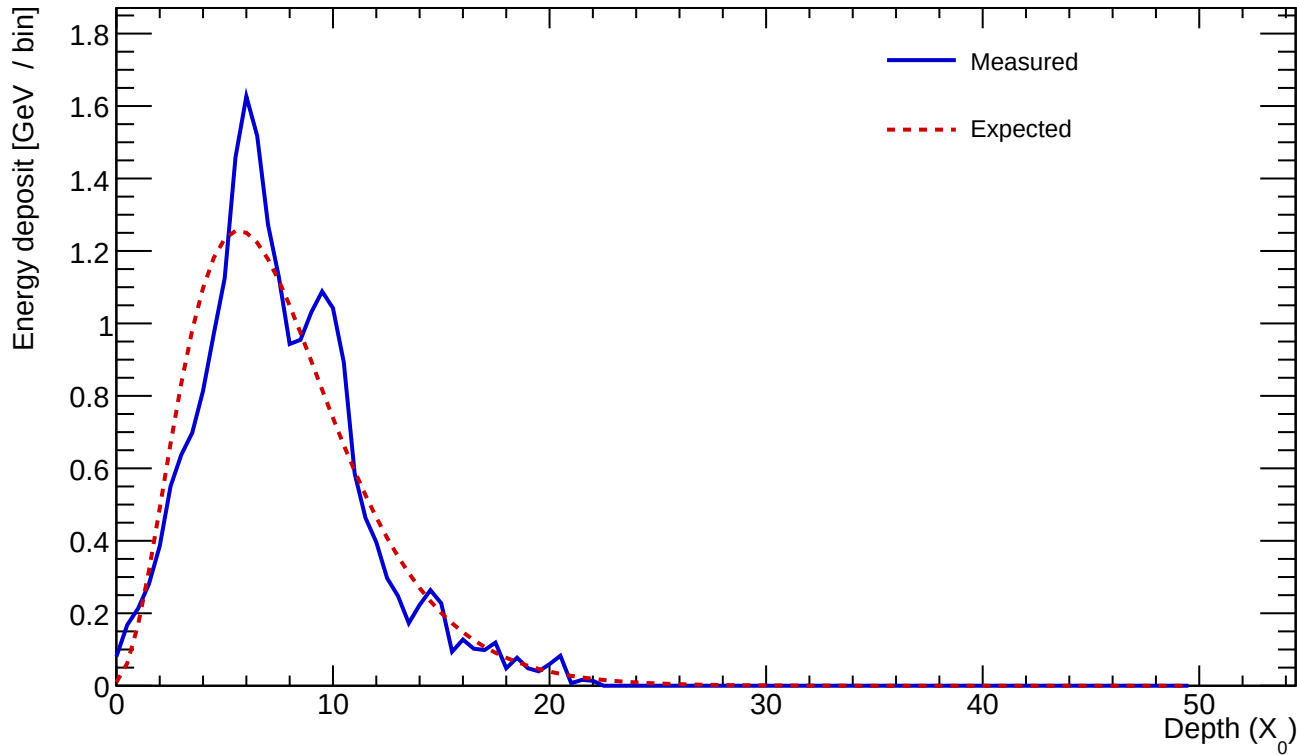
Cluster 580 E=22.692 GeV profileStart=0.50 X_0 \chi=0.1924
