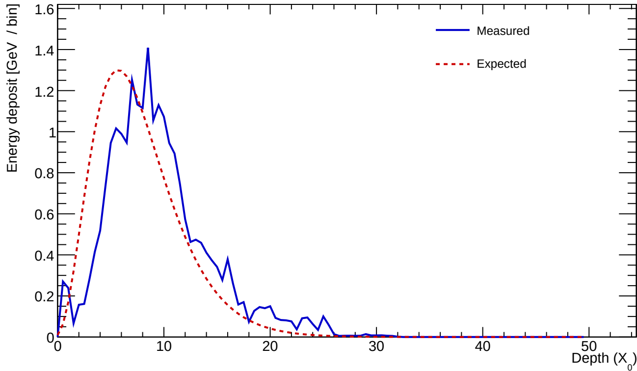
Cluster 859 E=23.566 GeV profileStart=1.50 X_0 \chi=0.1757
