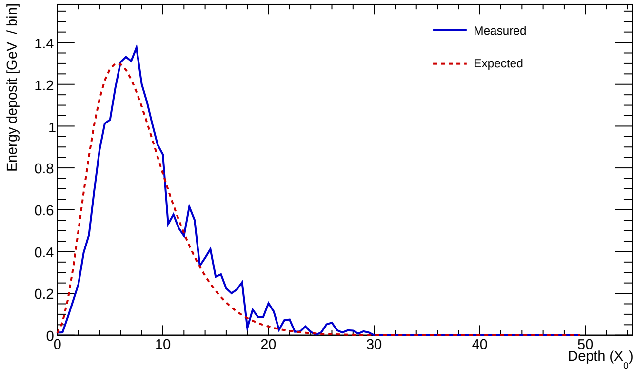
Cluster 661 E=23.574 GeV profileStart=1.00 X_0 \chi=0.1319
