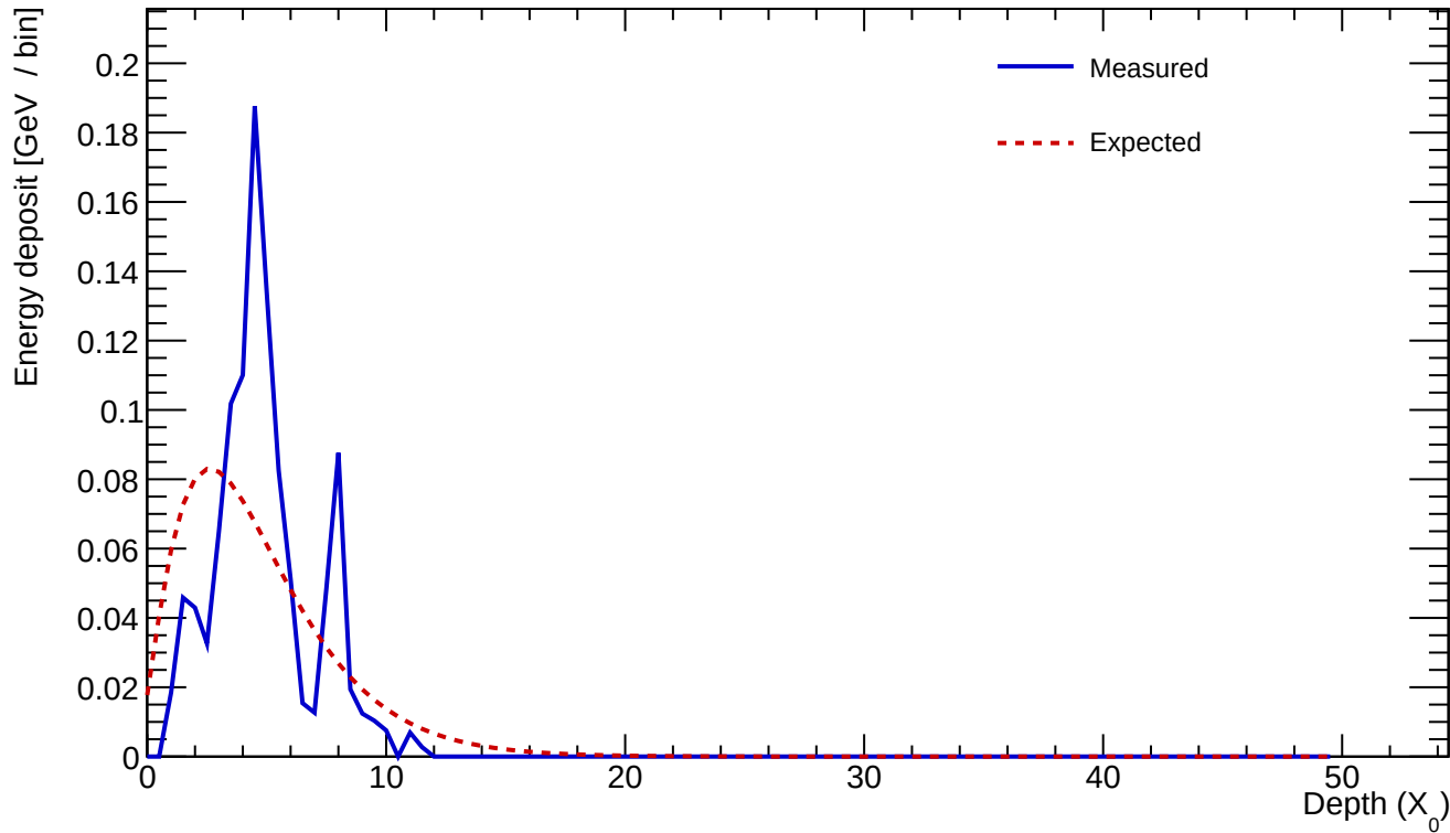
Cluster 324 E=1.096 GeV profileStart=1.00 X_0 \chi=0.4790
