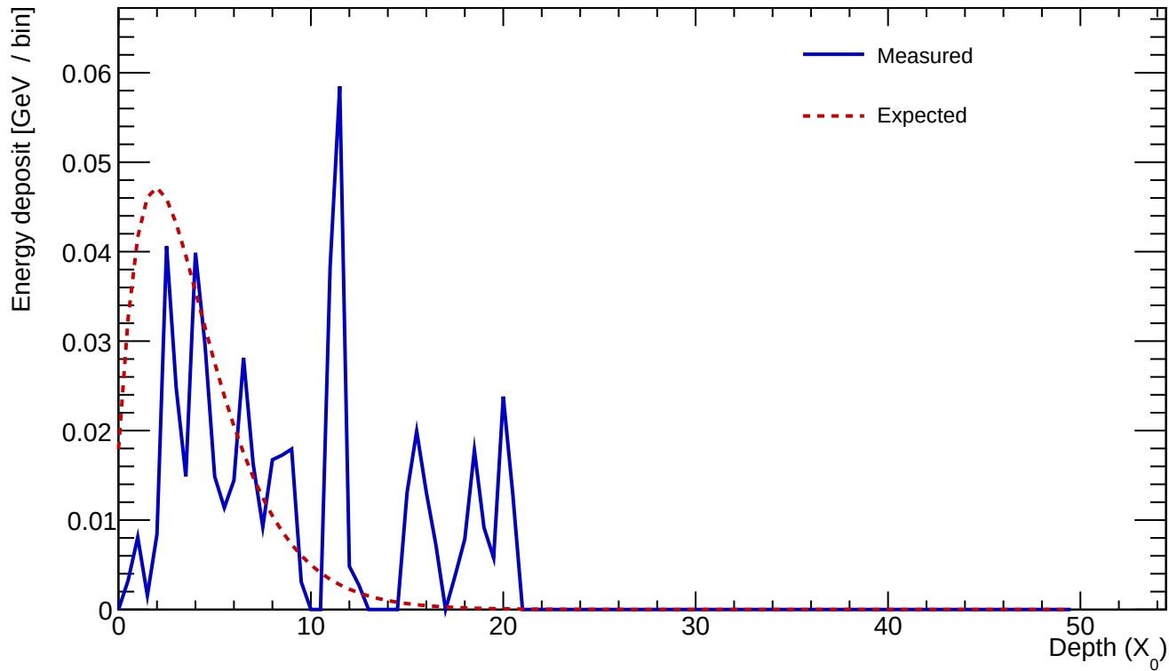
Cluster 89 E=0.559 GeV profileStart=2.00 X_0 \chi=0.8155
