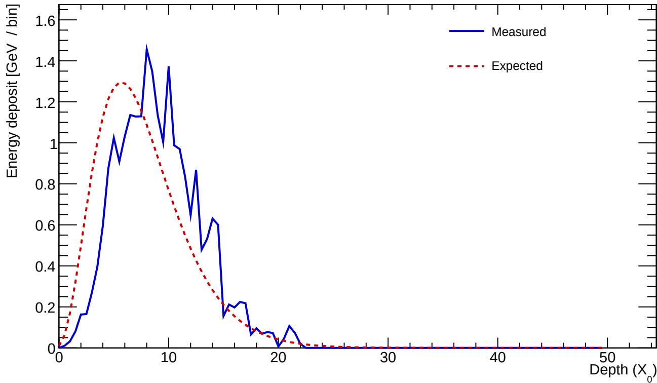
Cluster 755 E=23.452 GeV profileStart=1.50 X_0 \chi=0.1677
