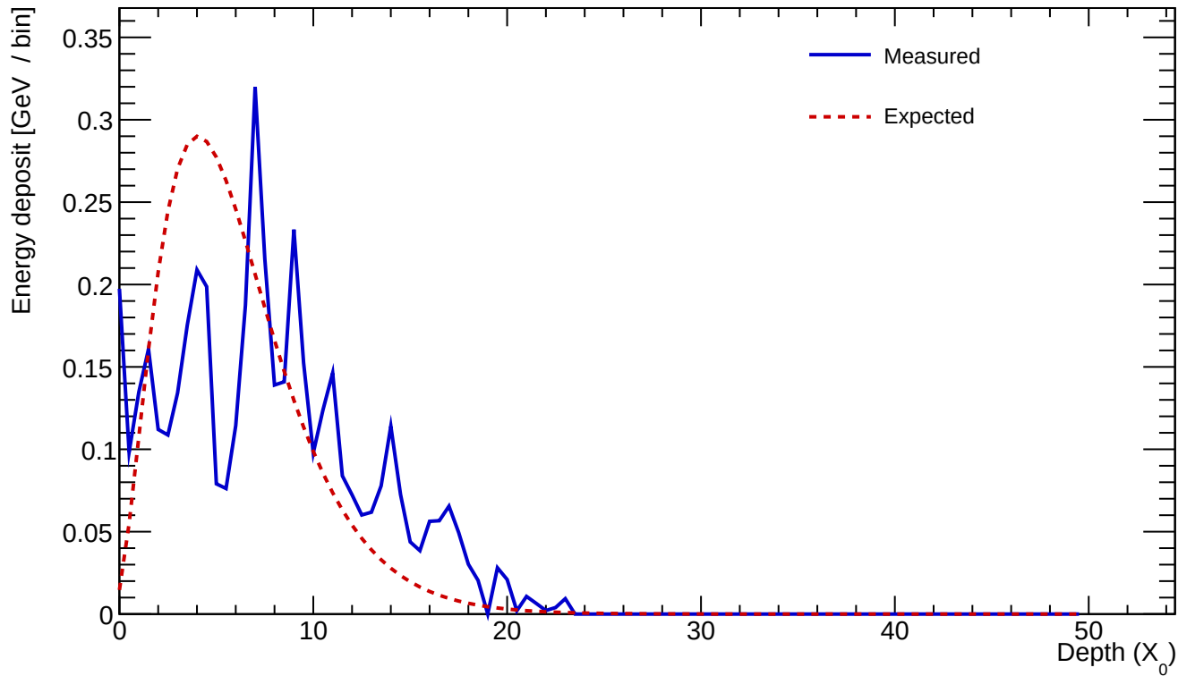
Cluster 169 E=4.543 GeV profileStart=1.50 X_0 \chi=0.5077
