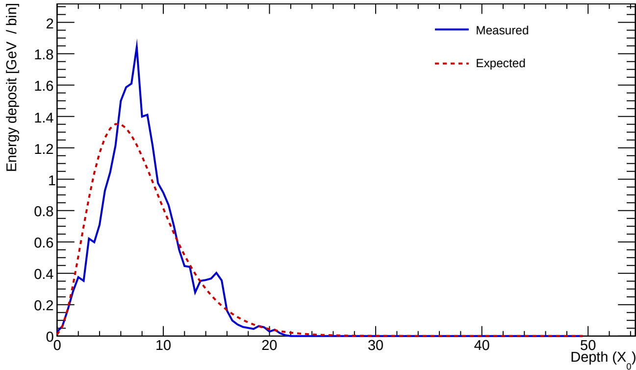
Cluster 617 E=24.615 GeV profileStart=0.50 X_0 \chi=0.2004
