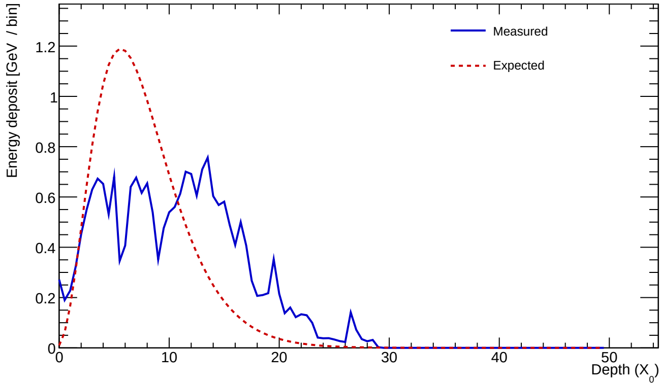
Cluster 880 E=21.378 GeV profileStart=4.00 X_0 \chi=0.5696
