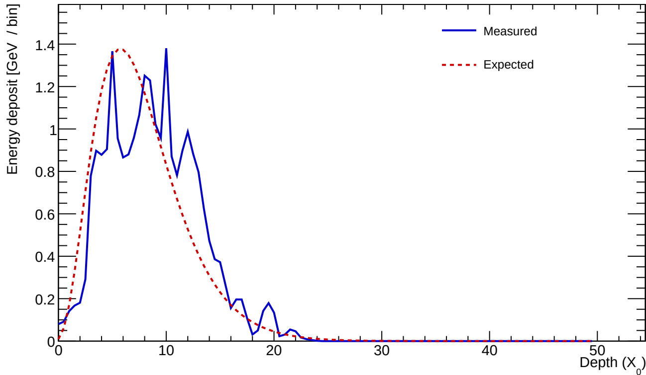
Cluster 517 E=25.057 GeV profileStart=1.00 X_0 \chi=0.2406
