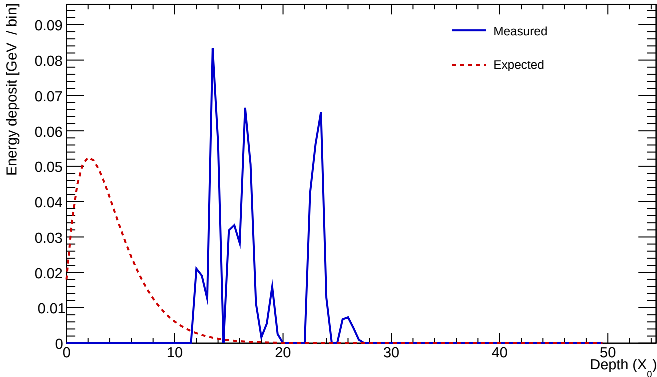
Cluster 260 E=0.636 GeV profileStart=12.00 X_0 \chi=0.8234
