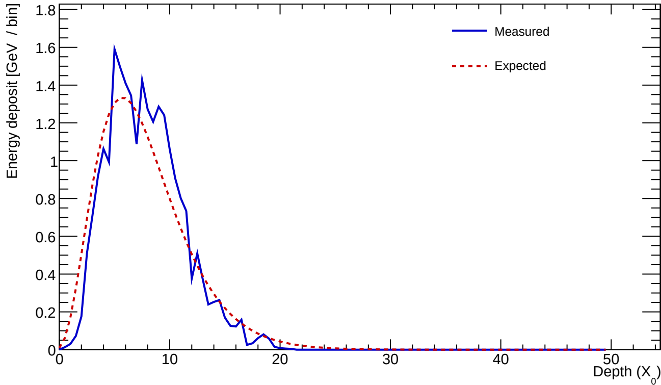
Cluster 897 E=24.228 GeV profileStart=0.50 X_0 \chi=0.1591
