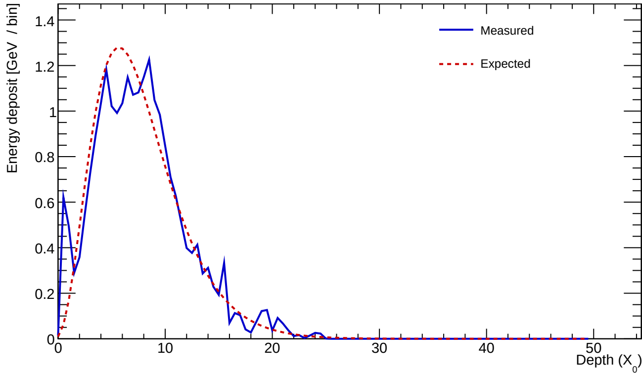
Cluster 470 E=23.156 GeV profileStart=0.50 X_0 \chi=0.1827
