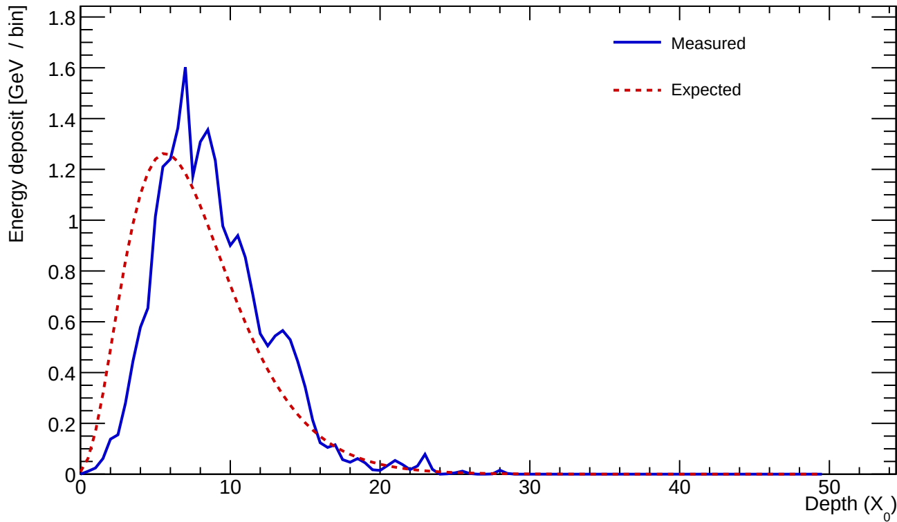
Cluster 807 E=22.828 GeV profileStart=1.50 X_0 \chi=0.1458
