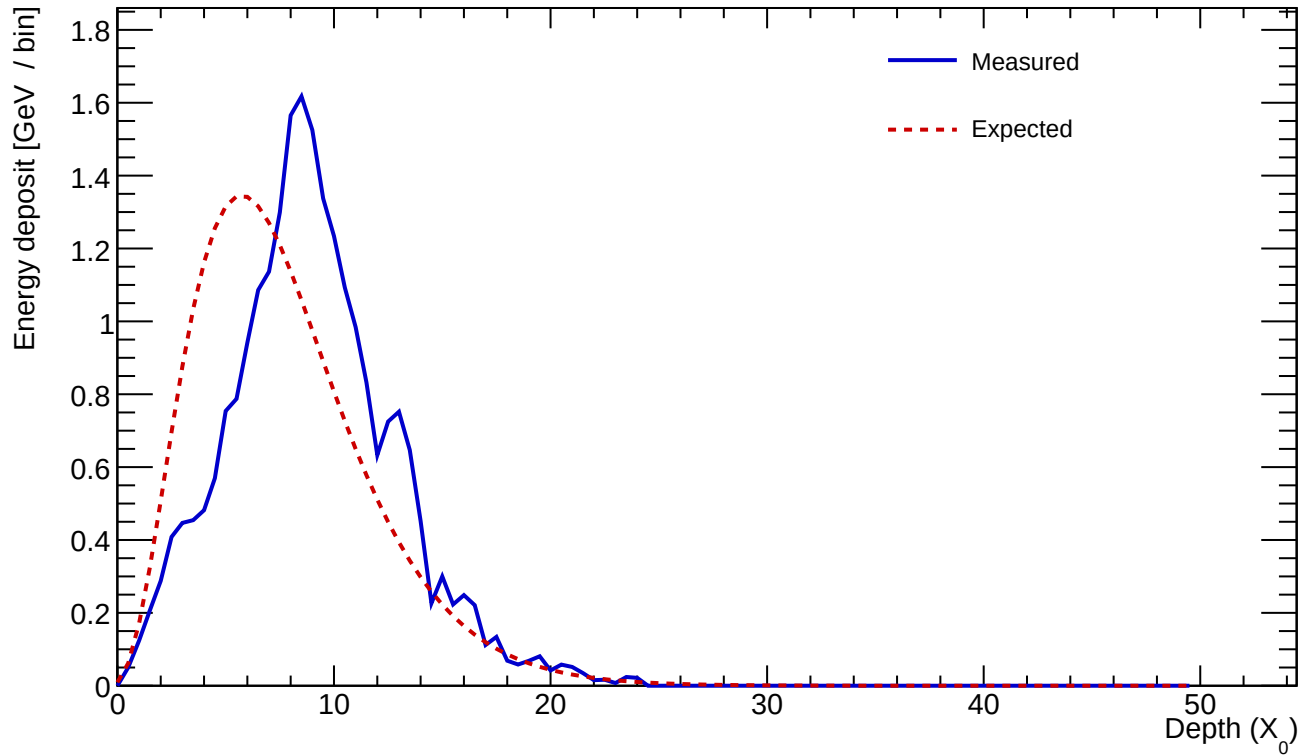
Cluster 528 E=24.444 GeV profileStart=2.00 X_0 \chi=0.2111
