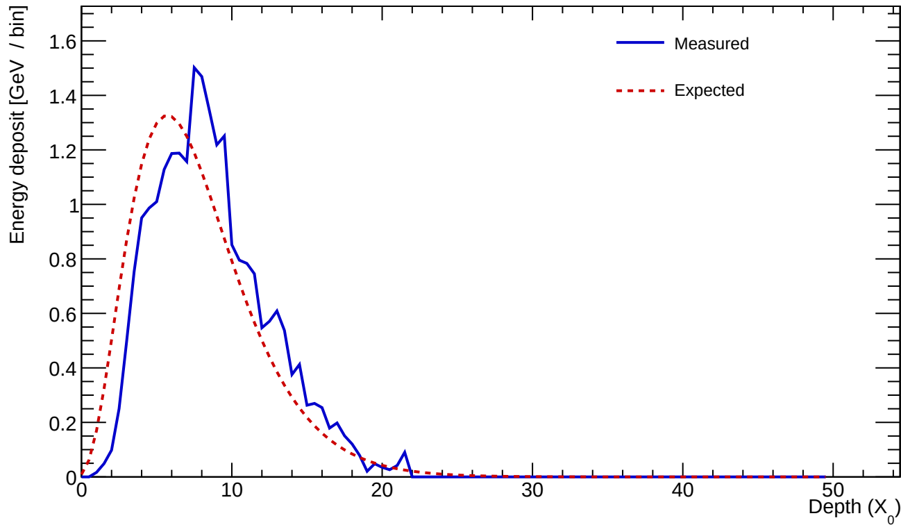
Cluster 758 E=24.062 GeV profileStart=1.00 X_0 \chi=0.1174
