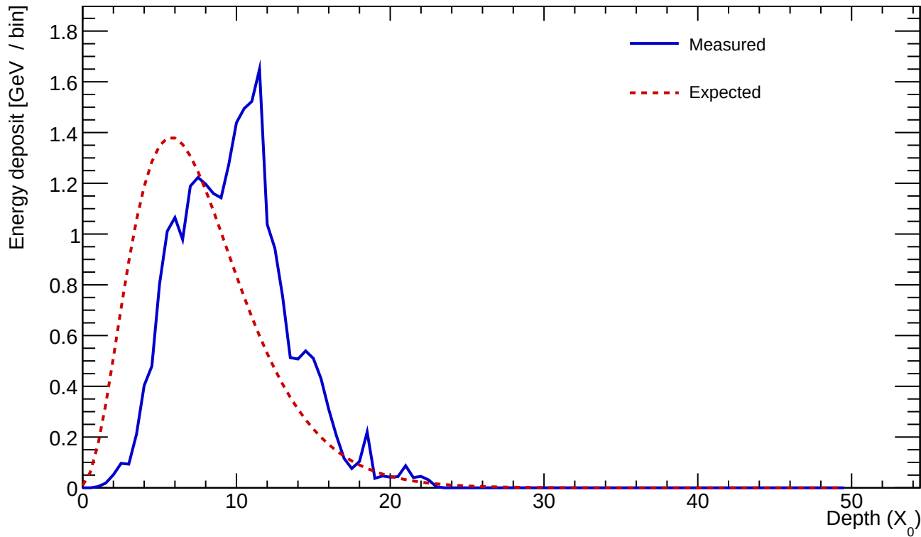
Cluster 804 E=25.151 GeV profileStart=2.50 X_0 \chi=0.1886
