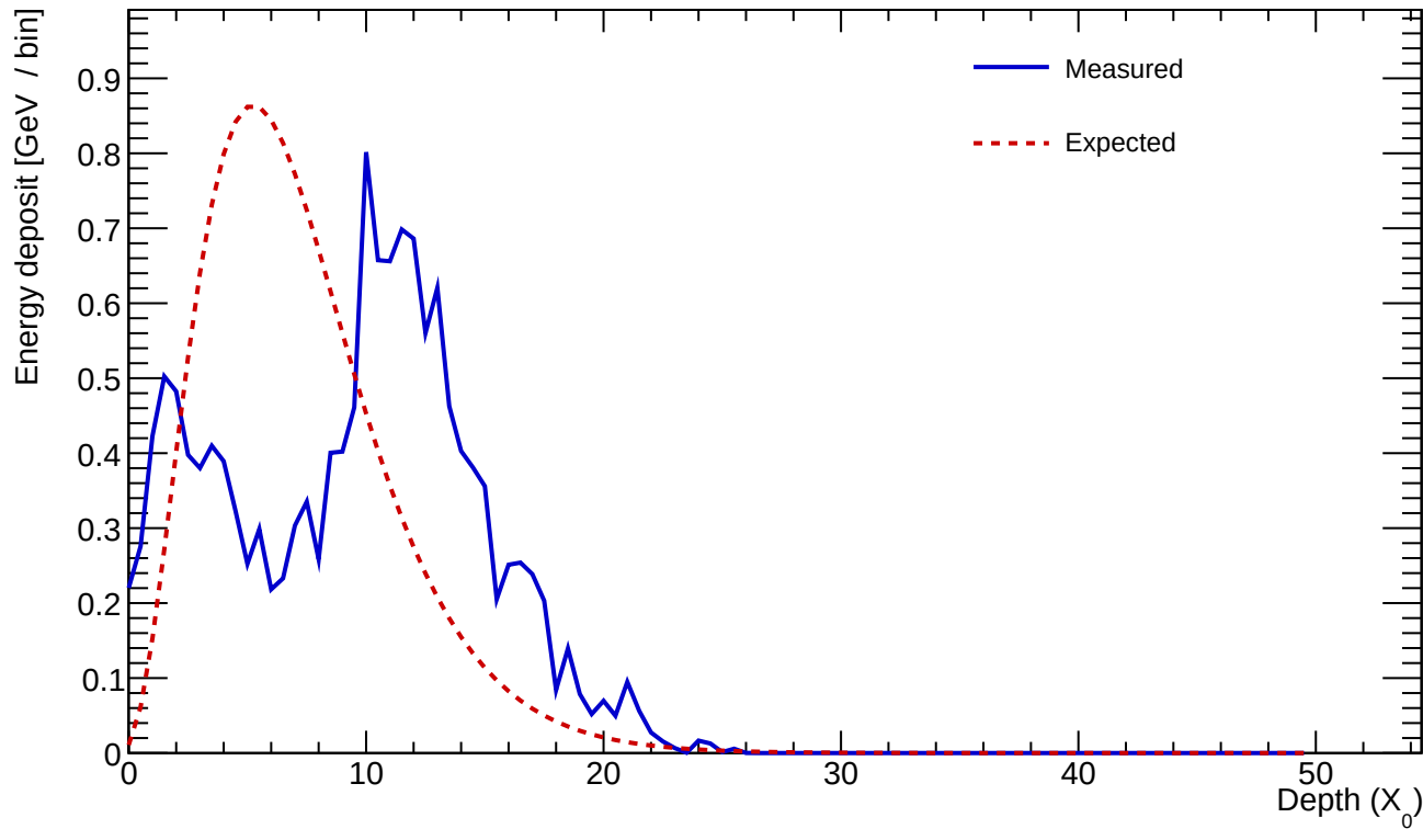
Cluster 136 E=15.113 GeV profileStart=4.00 X_0 \chi=0.5323
