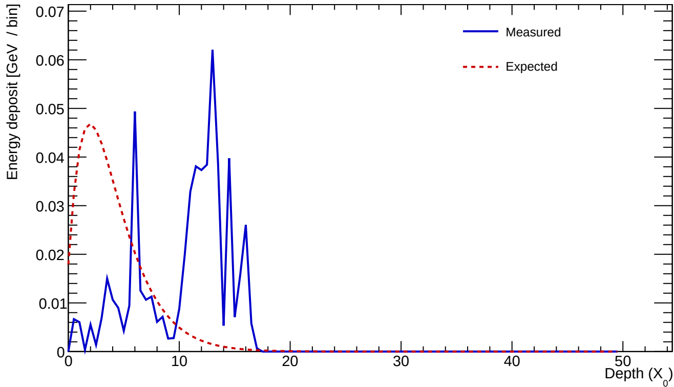
Cluster 956 E=0.554 GeV profileStart=10.50 X_0 \chi=0.5790
