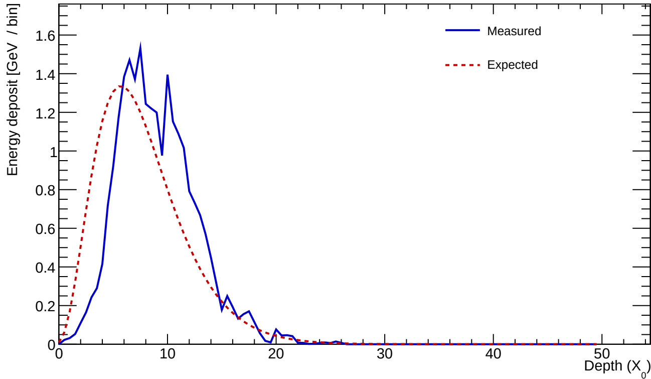
Cluster 266 E=24.265 GeV profileStart=2.00 X_0 \chi=0.1607
