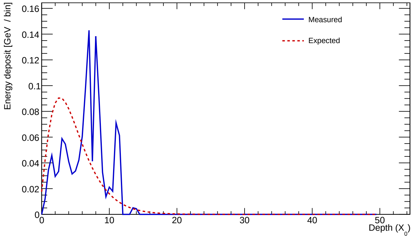
Cluster 50 E=1.215 GeV profileStart=2.00 X_0 \chi=0.6539
