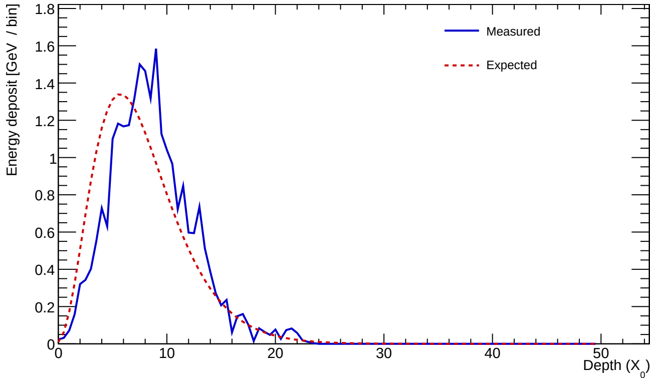
Cluster 640 E=24.347 GeV profileStart=1.50 X_0 \chi=0.1595
