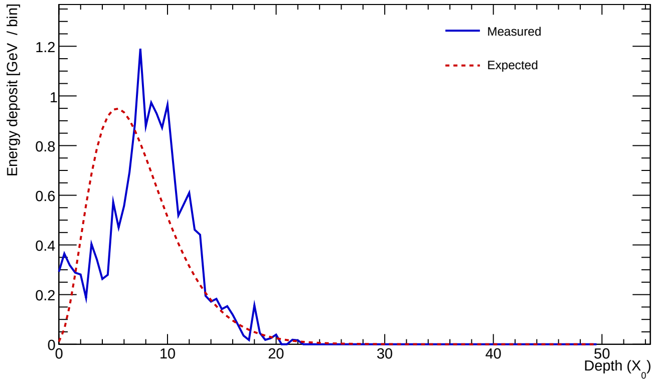
Cluster 33 E=16.750 GeV profileStart=2.50 X_0 \chi=0.3272
