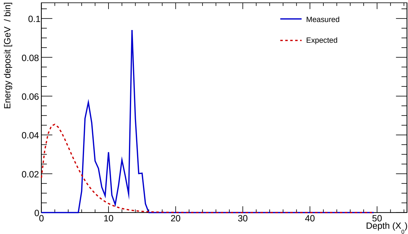
Cluster 197 E=0.535 GeV profileStart=6.00 X_0 \chi=0.6607
