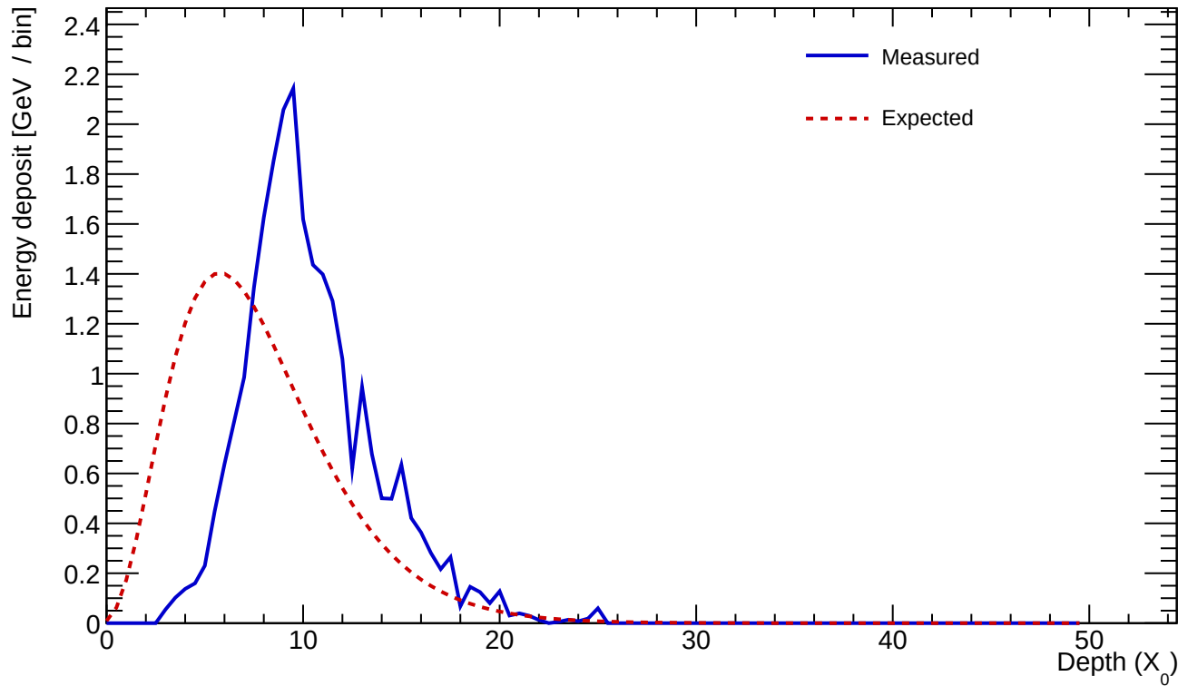
Cluster 886 E=25.584 GeV profileStart=3.50 X_0 \chi=0.2447
