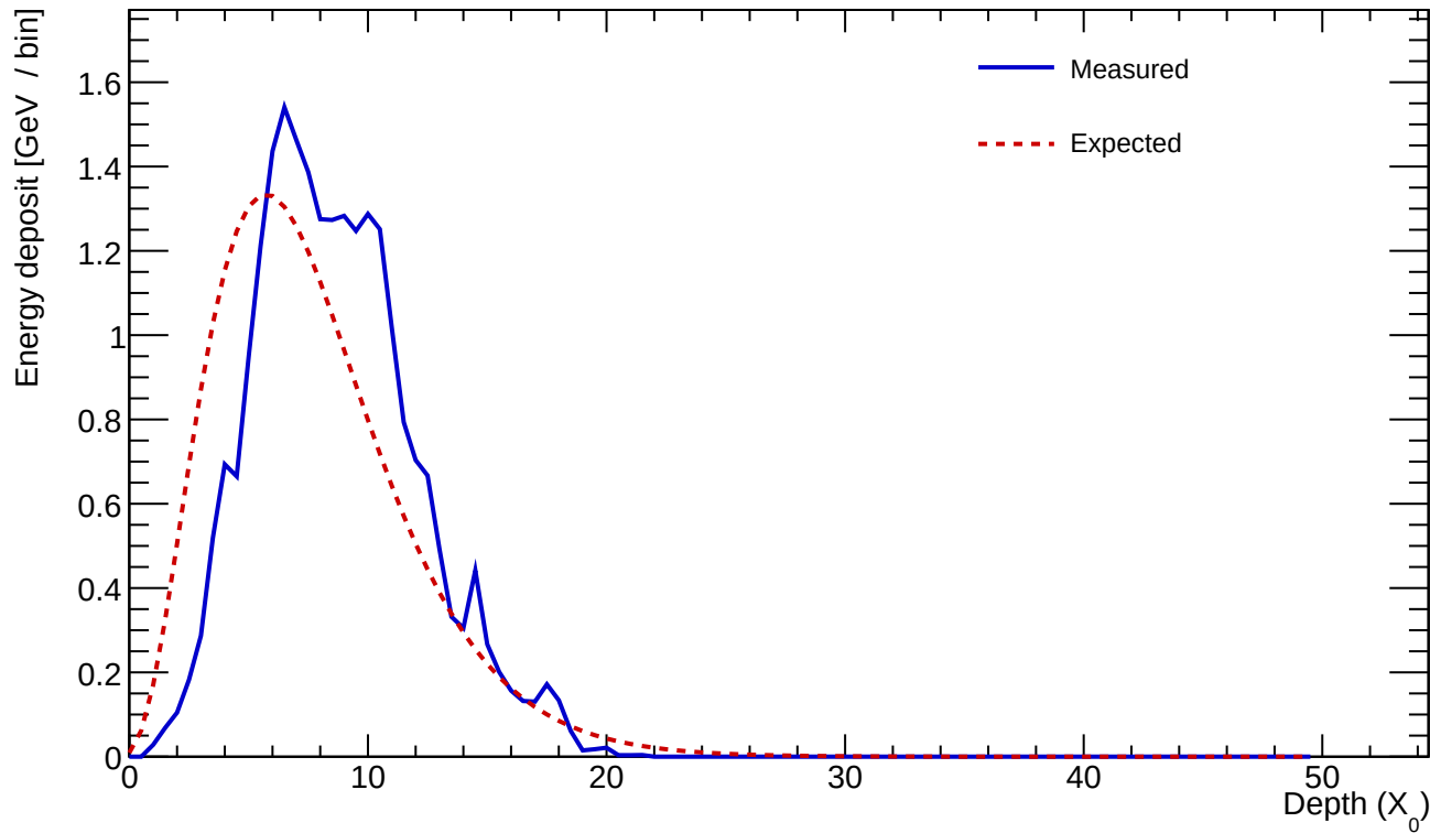
Cluster 122 E=24.222 GeV profileStart=1.50 X_0 \chi=0.1379
