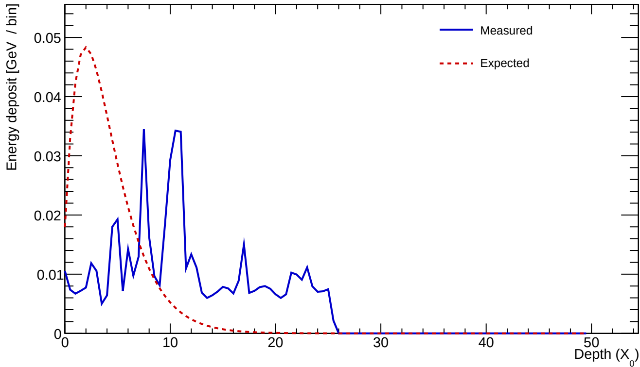
Cluster 547 E=0.576 GeV profileStart=6.00 X_0 \chi=0.8878
