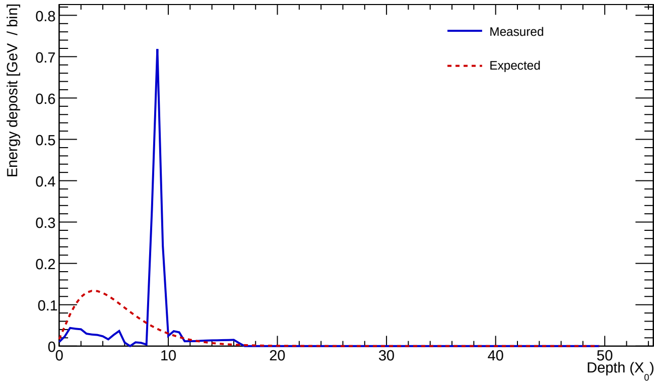
Cluster 958 E=1.903 GeV profileStart=5.00 X_0 \chi=1.2100
