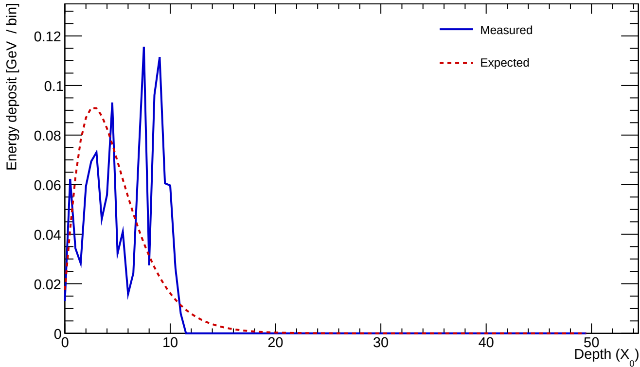
Cluster 198 E=1.224 GeV profileStart=1.00 X_0 \chi=0.5798
