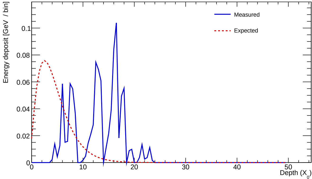
Cluster 476 E=0.984 GeV profileStart=11.00 X_0 \chi=0.8221
