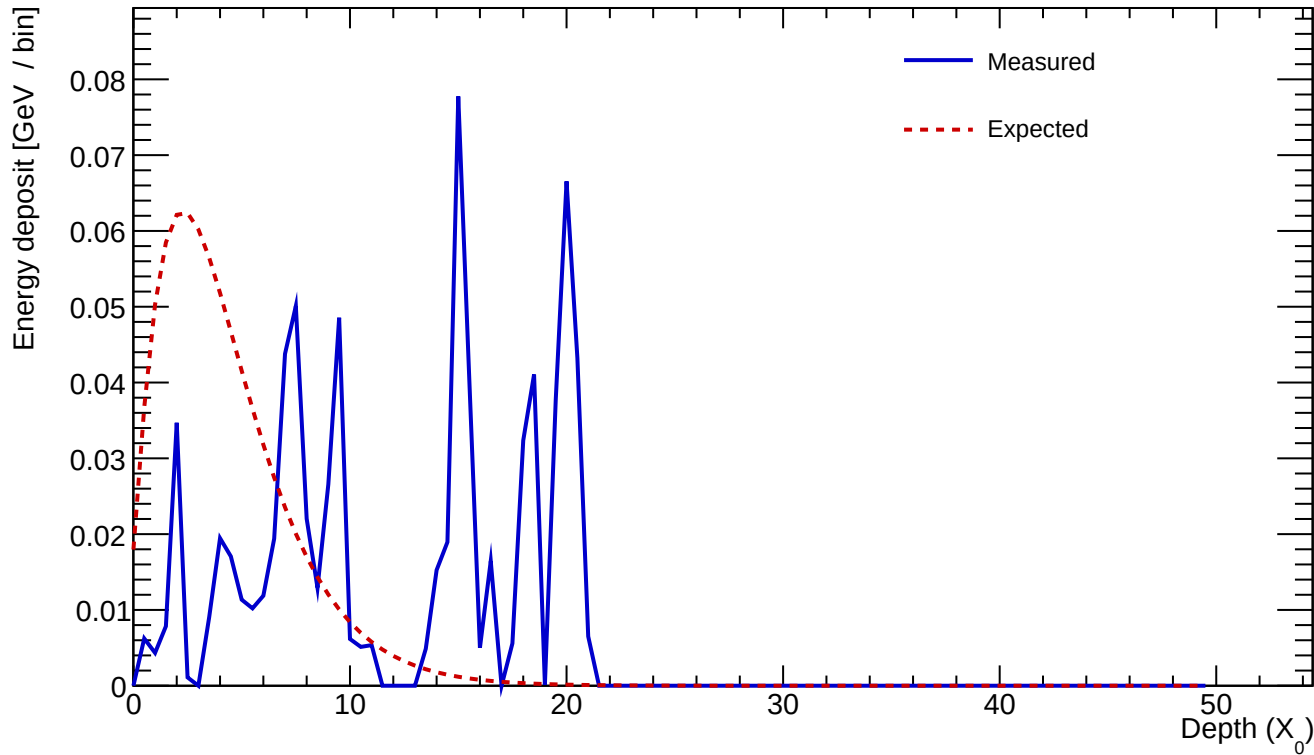
Cluster 607 E=0.786 GeV profileStart=4.00 X_0 \chi=1.1159
