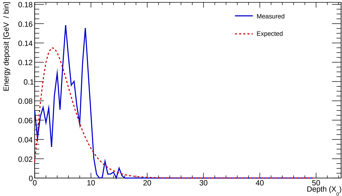
Cluster 759 E=1.924 GeV profileStart=0.50 X_0 \chi=0.4728
