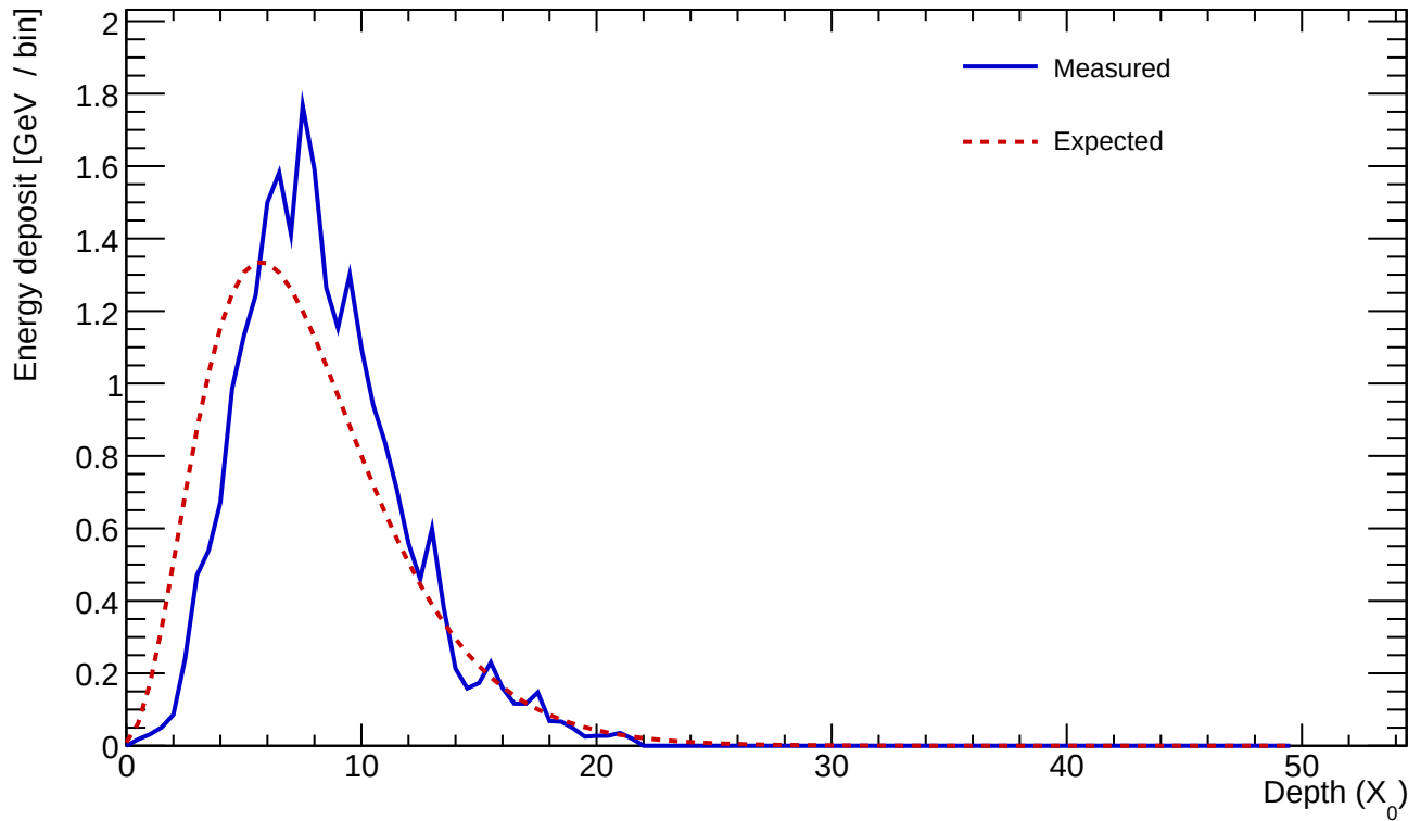
Cluster 662 E=24.260 GeV profileStart=1.00 X_0 \chi=0.1587
