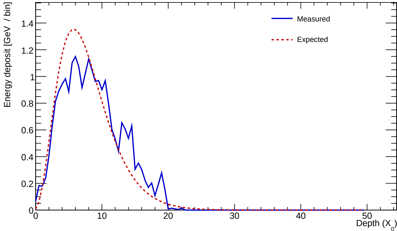
Cluster 879 E=24.610 GeV profileStart=0.50 X_0 \chi=0.2191
