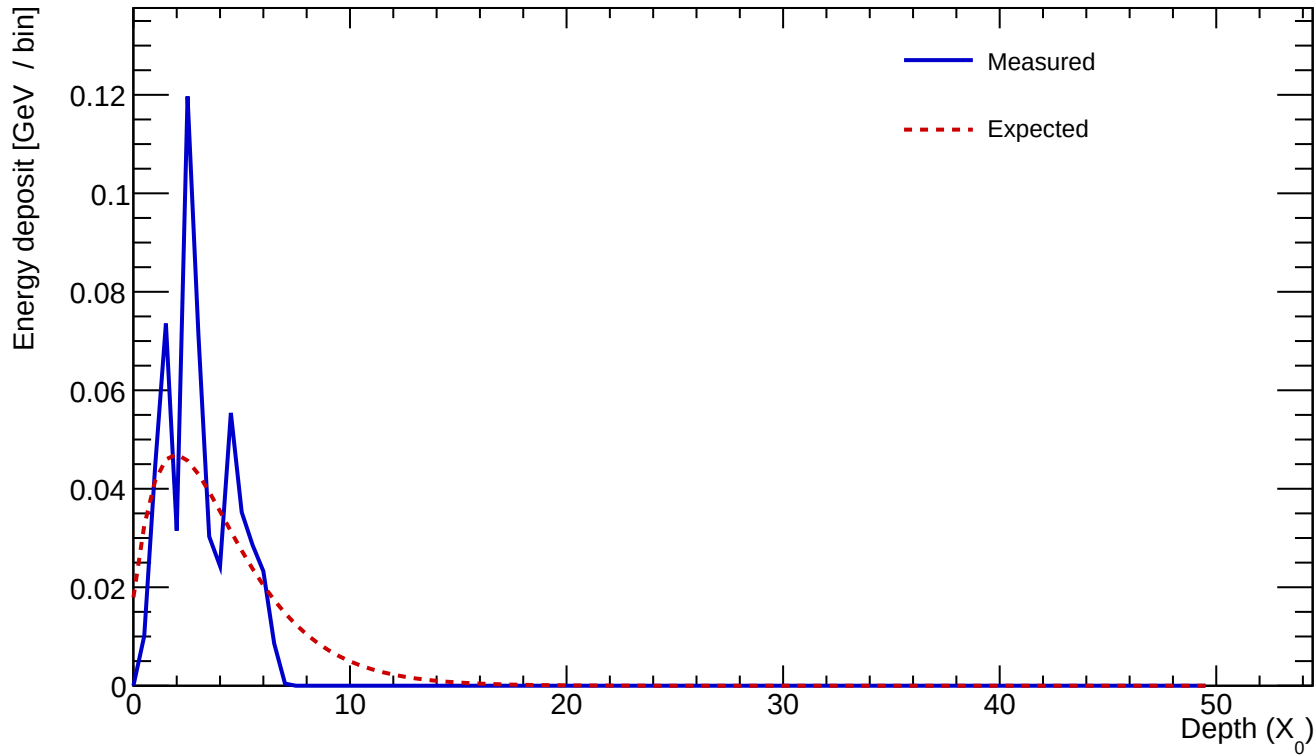
Cluster 961 E=0.557 GeV profileStart=0.50 X_0 \chi=0.4124
