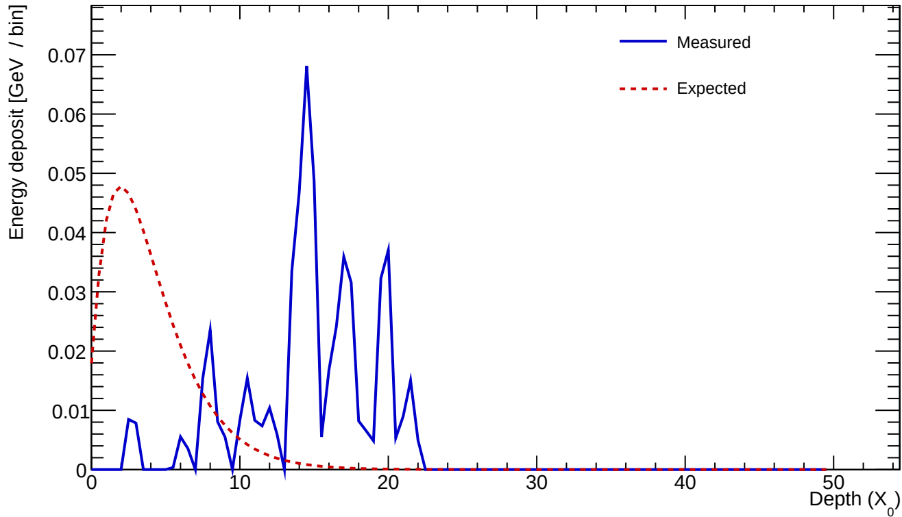
Cluster 708 E=0.568 GeV profileStart=13.00 X_0 \chi=0.6519
