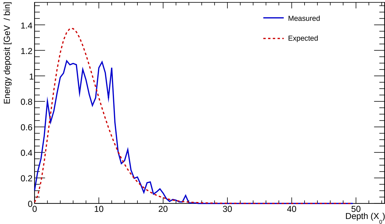
Cluster 41 E=24.998 GeV profileStart=0.50 X_0 \chi=0.2719
