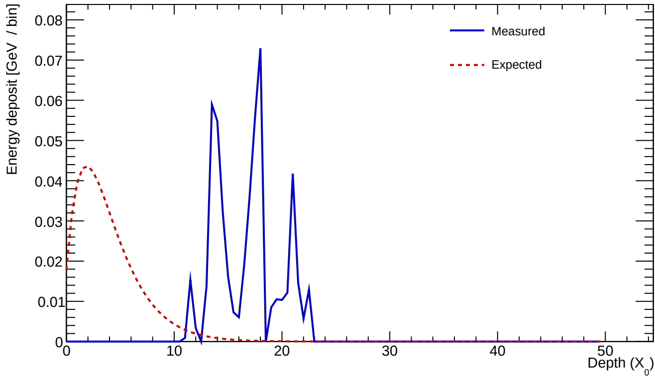
Cluster 673 E=0.509 GeV profileStart=13.00 X_0 \chi=0.6857
