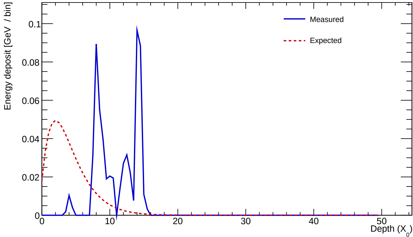
Cluster 620 E=0.592 GeV profileStart=7.00 X_0 \chi=0.6923
