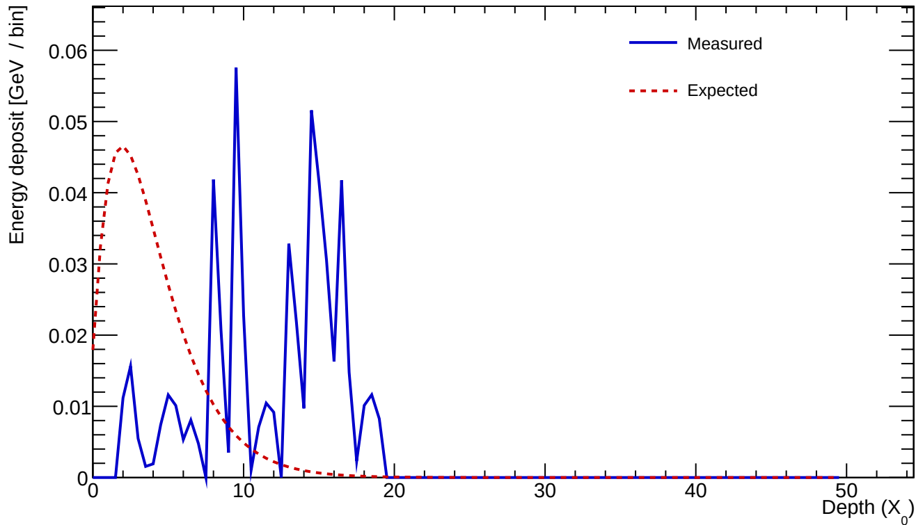
Cluster 817 E=0.551 GeV profileStart=12.50 X_0 \chi=0.8058
