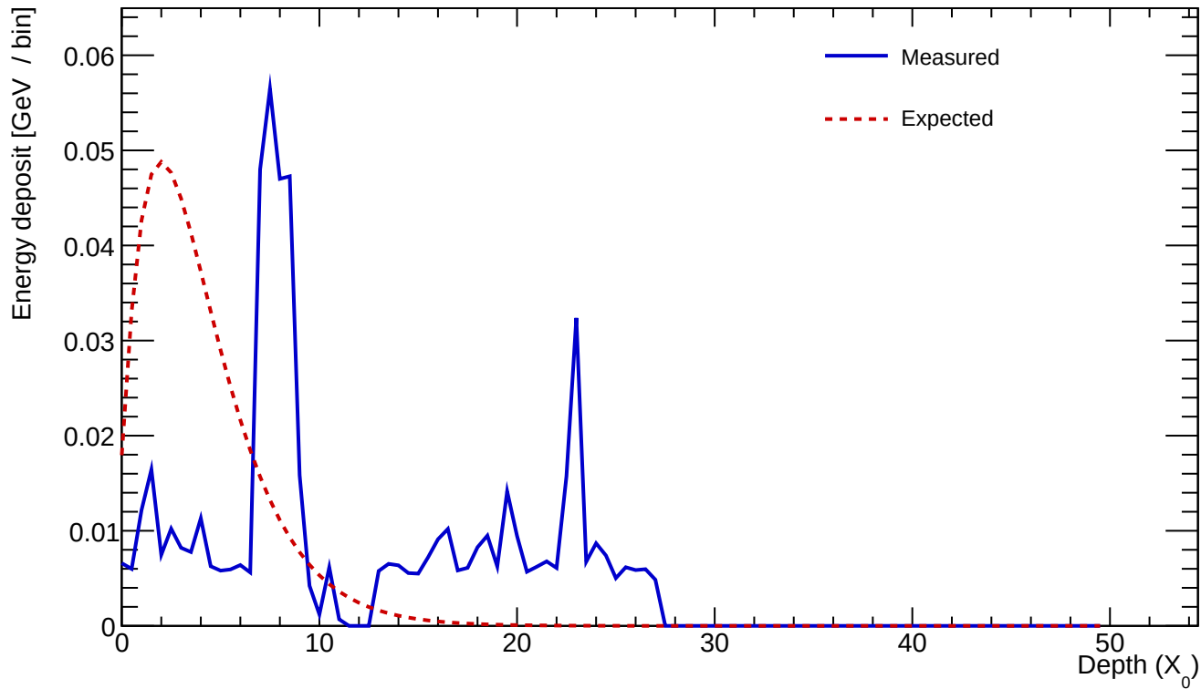
Cluster 544 E=0.582 GeV profileStart=5.50 X_0 \chi=0.9831
