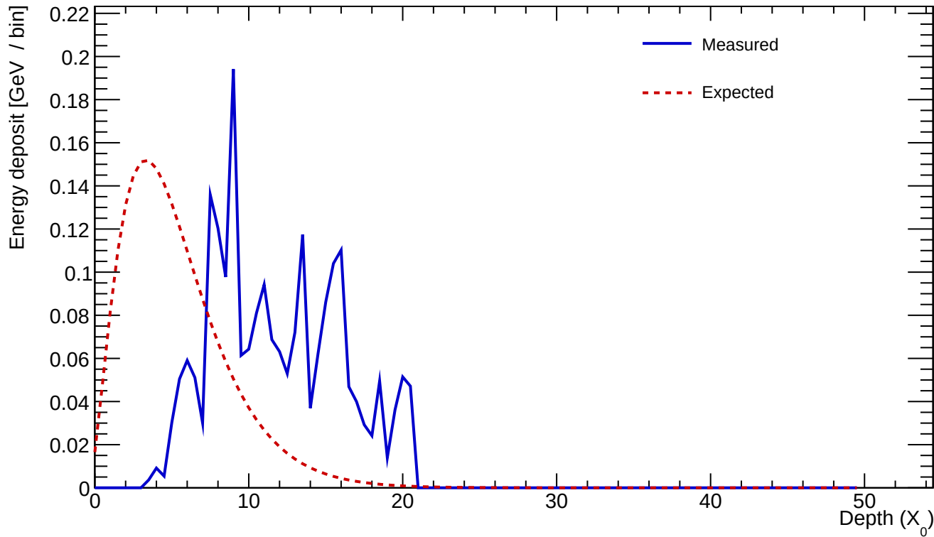
Cluster 1123 E=2.200 GeV profileStart=5.50 X_0 \chi=0.5098
