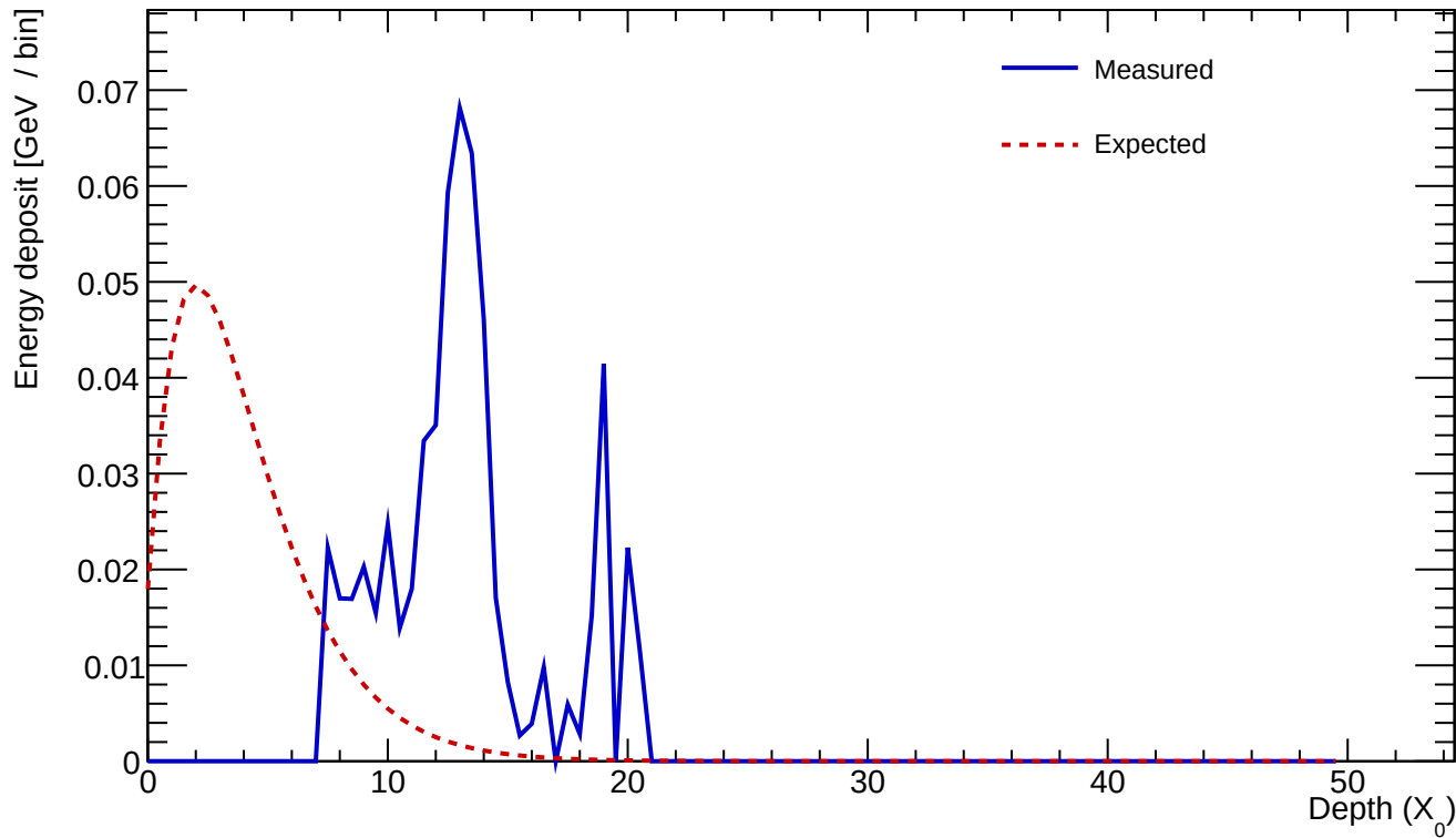
Cluster 160 E=0.595 GeV profileStart=11.00 X_0 \chi=0.6987
