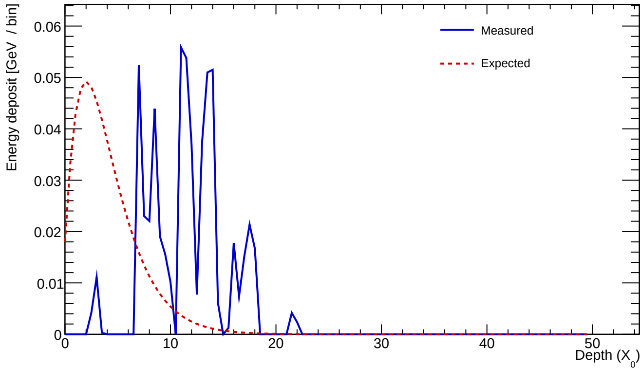
Cluster 333 E=0.588 GeV profileStart=7.50 X_0 \chi=0.7755
