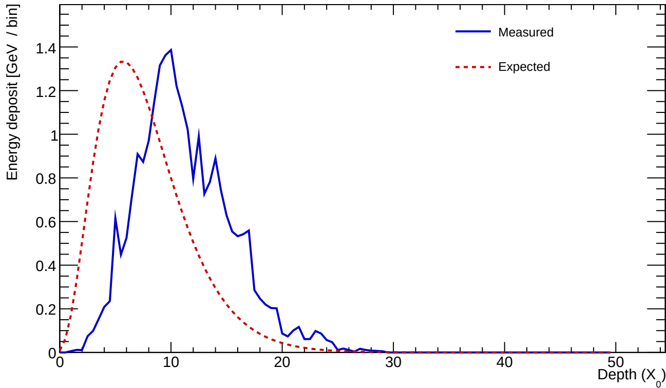
Cluster 720 E=24.230 GeV profileStart=4.00 X_0 \chi=0.1650
