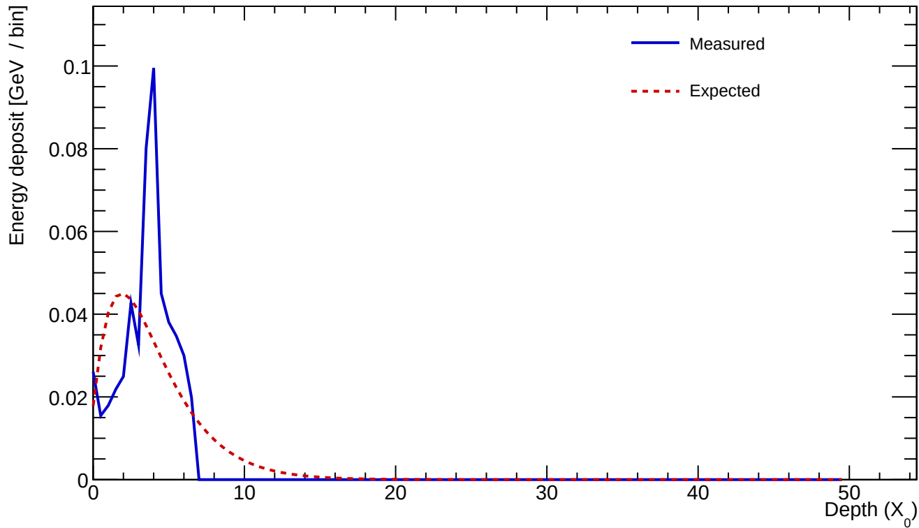
Cluster 866 E=0.529 GeV profileStart=1.50 X_0 \chi=0.3445
