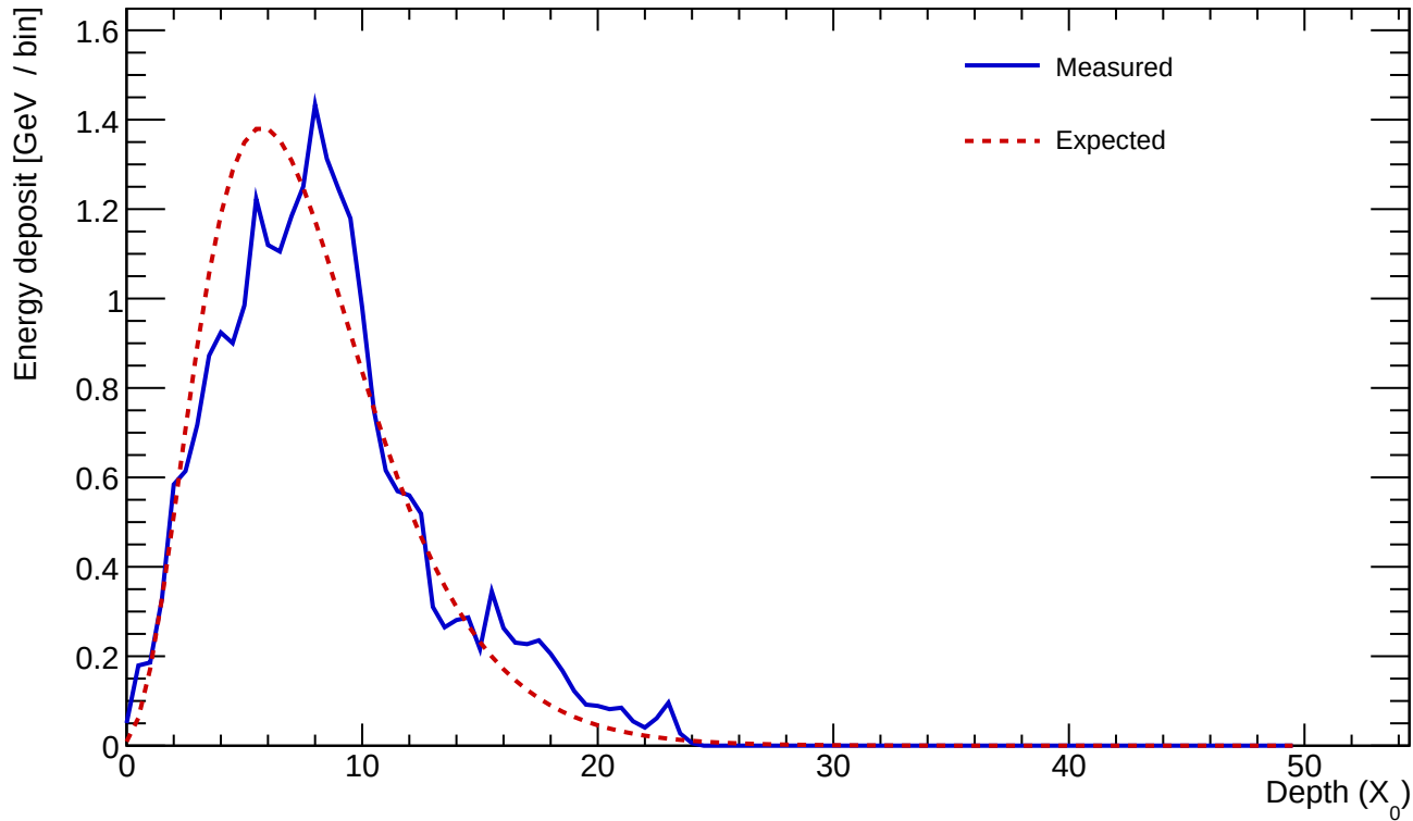
Cluster 255 E=25.175 GeV profileStart=0.50 X_0 \chi=0.1984
