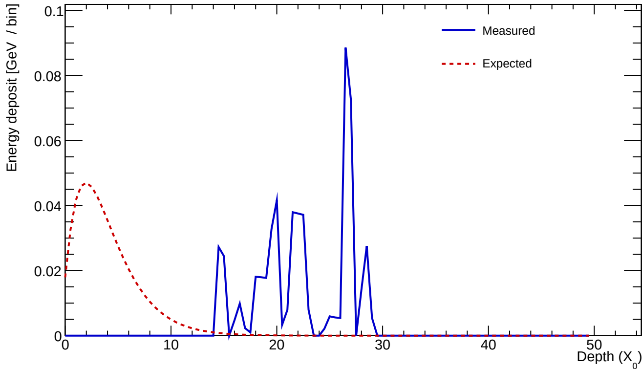
Cluster 549 E=0.557 GeV profileStart=18.00 X_0 \chi=0.8925
