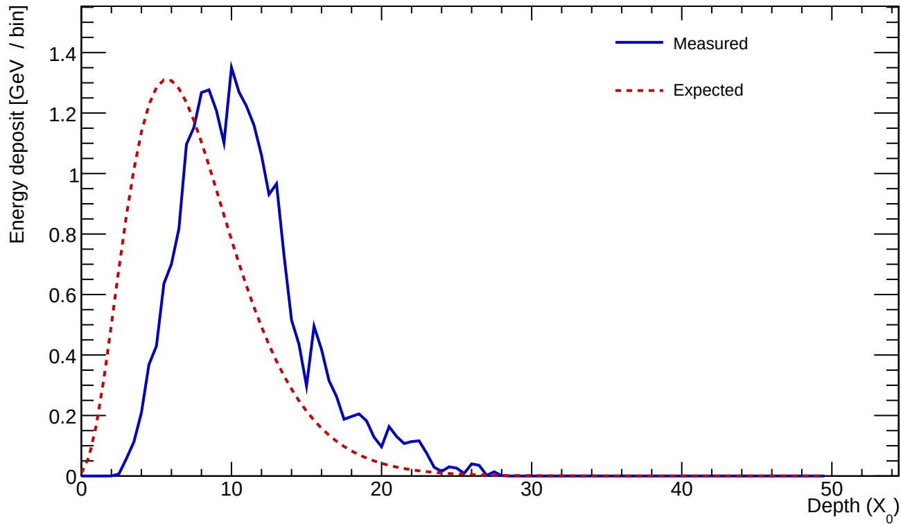
Cluster 559 E=23.777 GeV profileStart=3.50 X_0 \chi=0.1278
