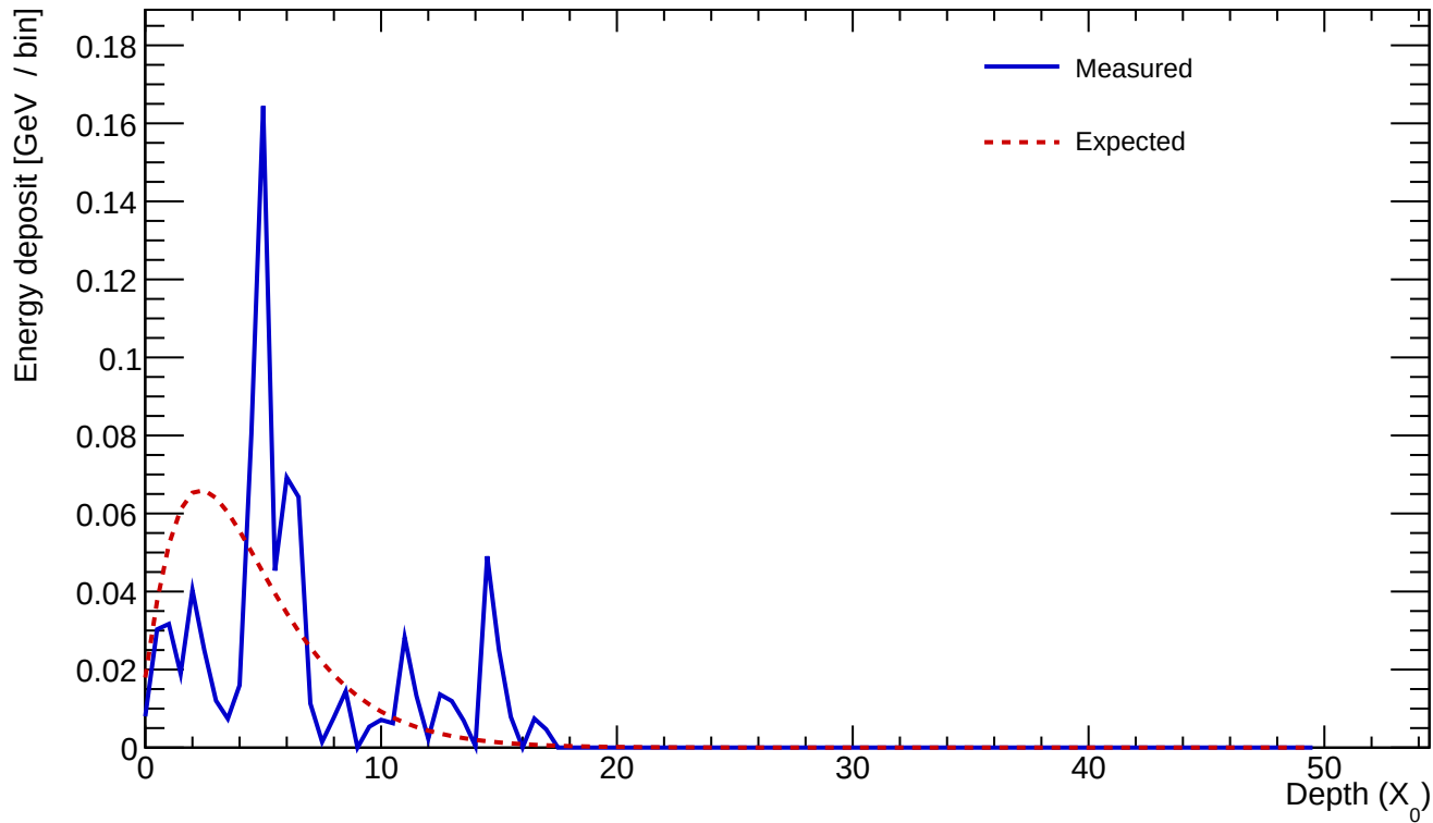
Cluster 757 E=0.838 GeV profileStart=1.50 X_0 \chi=0.8363
