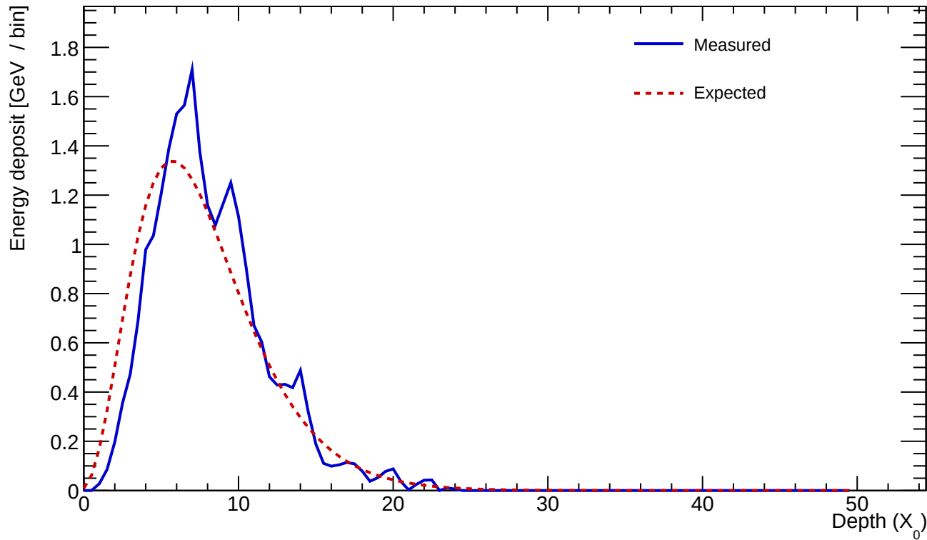
Cluster 730 E=24.331 GeV profileStart=1.00 X_0 \chi=0.1473
