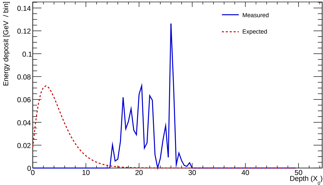
Cluster 14 E=0.926 GeV profileStart=16.50 X_0 \chi=0.6616
