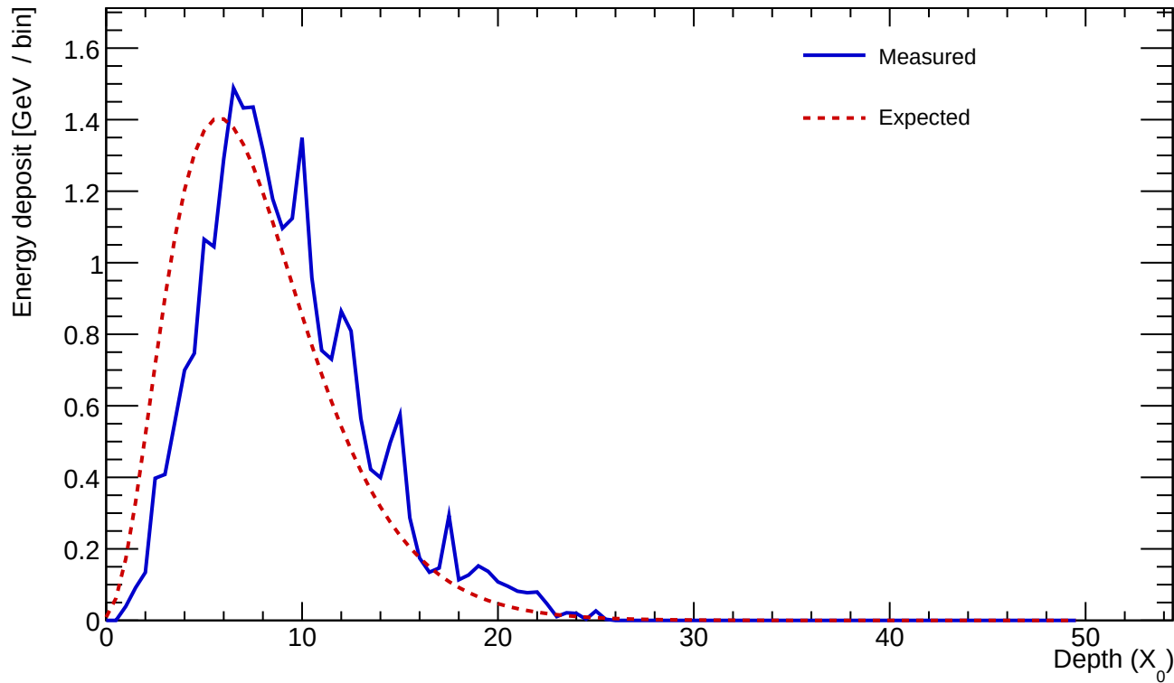
Cluster 277 E=25.604 GeV profileStart=1.50 X_0 \chi=0.1419
