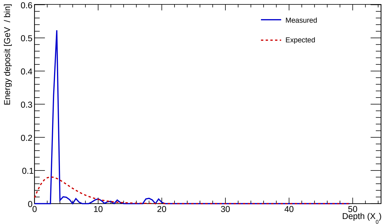
Cluster 746 E=1.057 GeV profileStart=1.00 X_0 \chi=1.4154
