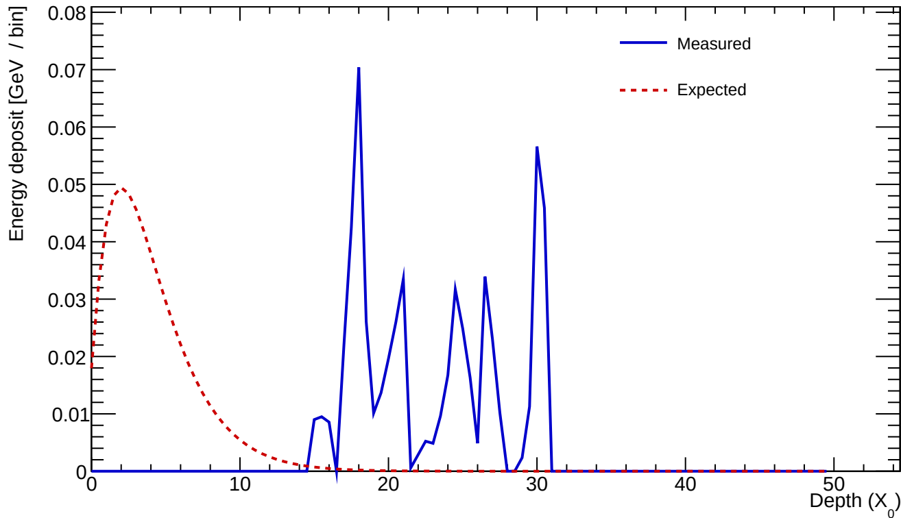
Cluster 604 E=0.592 GeV profileStart=16.50 X_0 \chi=0.7934
