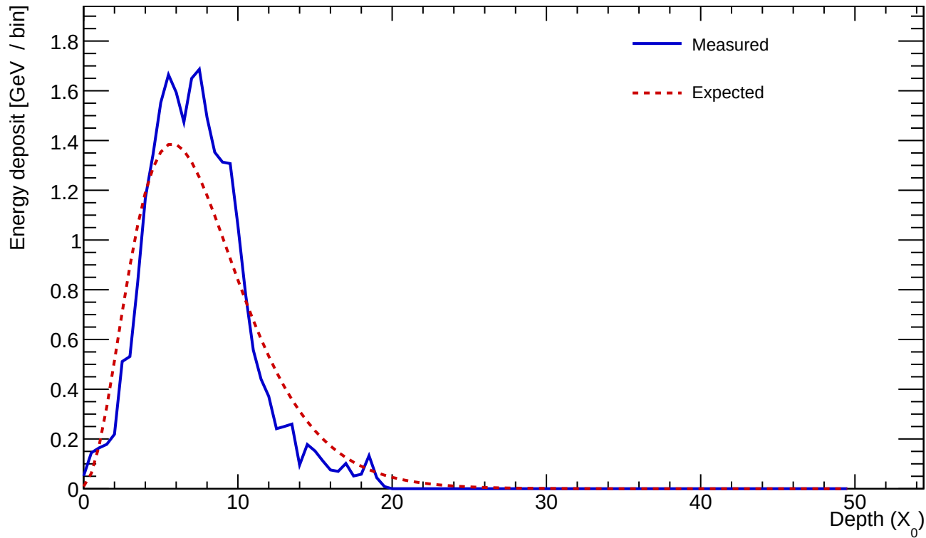
Cluster 948 E=25.267 GeV profileStart=0.50 X_0 \chi=0.2377
