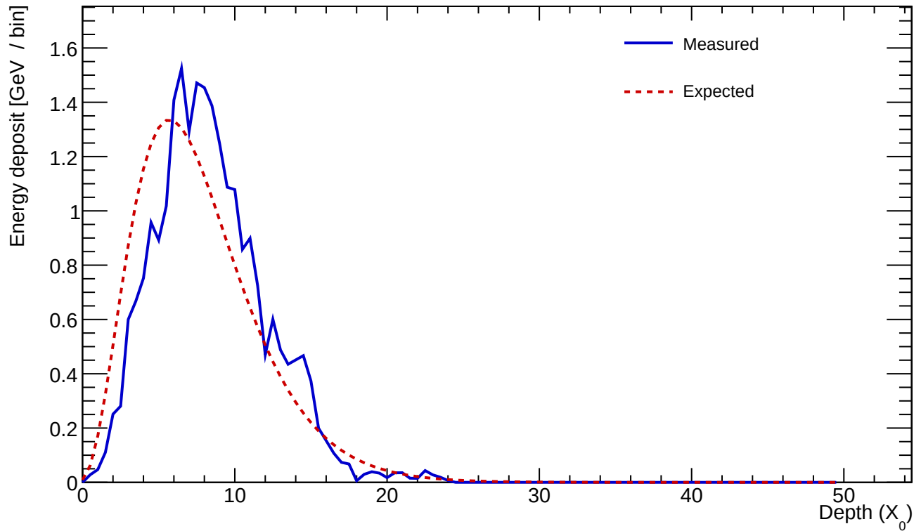
Cluster 92 E=24.248 GeV profileStart=1.00 X_0 \chi=0.1476
