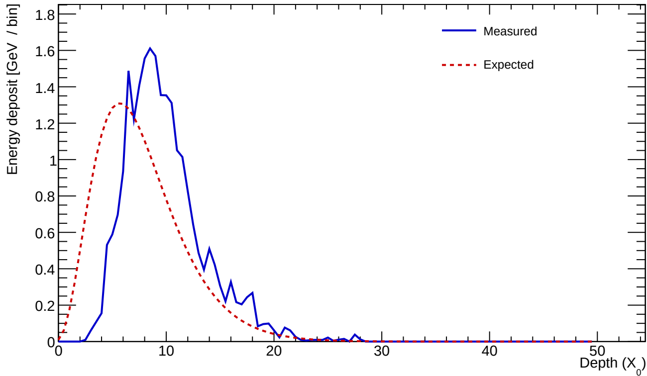
Cluster 85 E=23.759 GeV profileStart=2.50 X_0 \chi=0.1772
