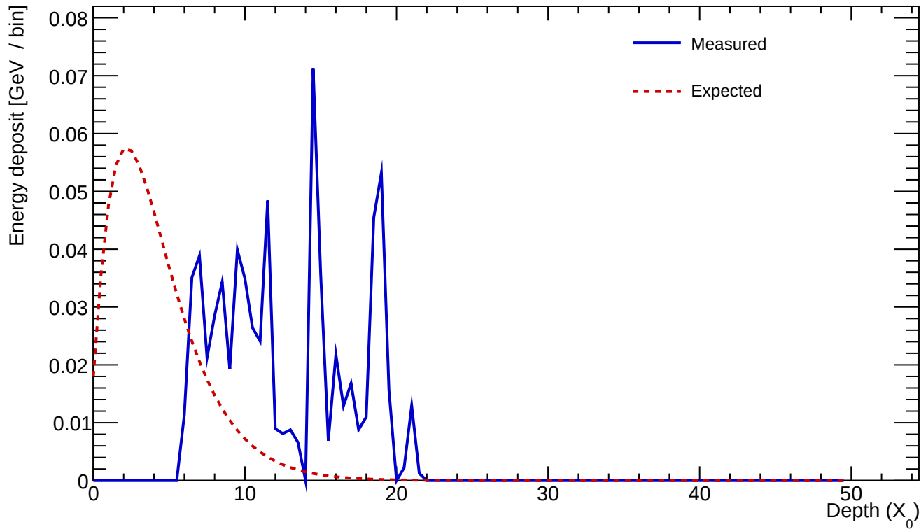
Cluster 182 E=0.710 GeV profileStart=6.00 X_0 \chi=0.7440
