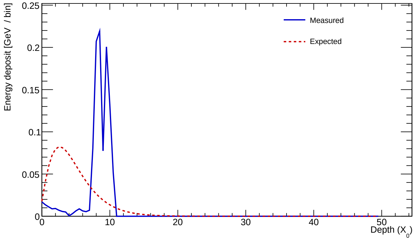
Cluster 626 E=1.083 GeV profileStart=6.50 X_0 \chi=0.5742
