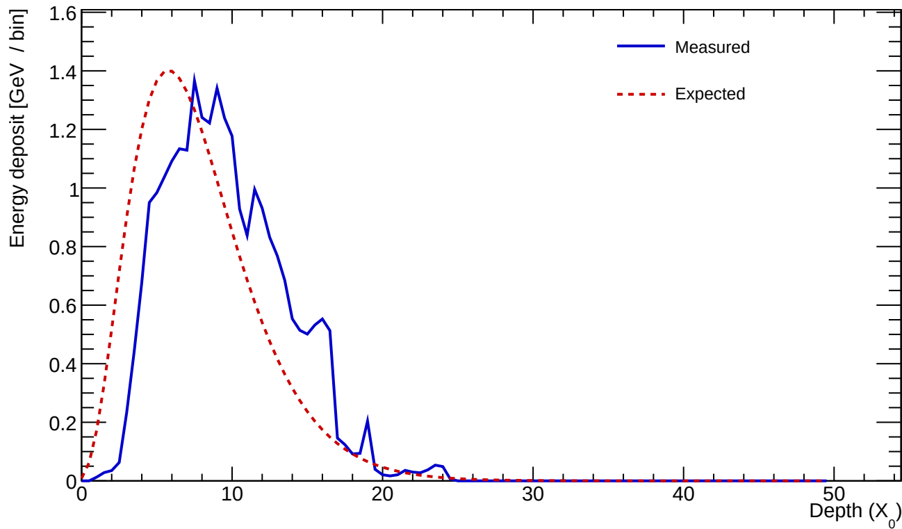
Cluster 984 E=25.547 GeV profileStart=2.00 X_0 \chi=0.1529
