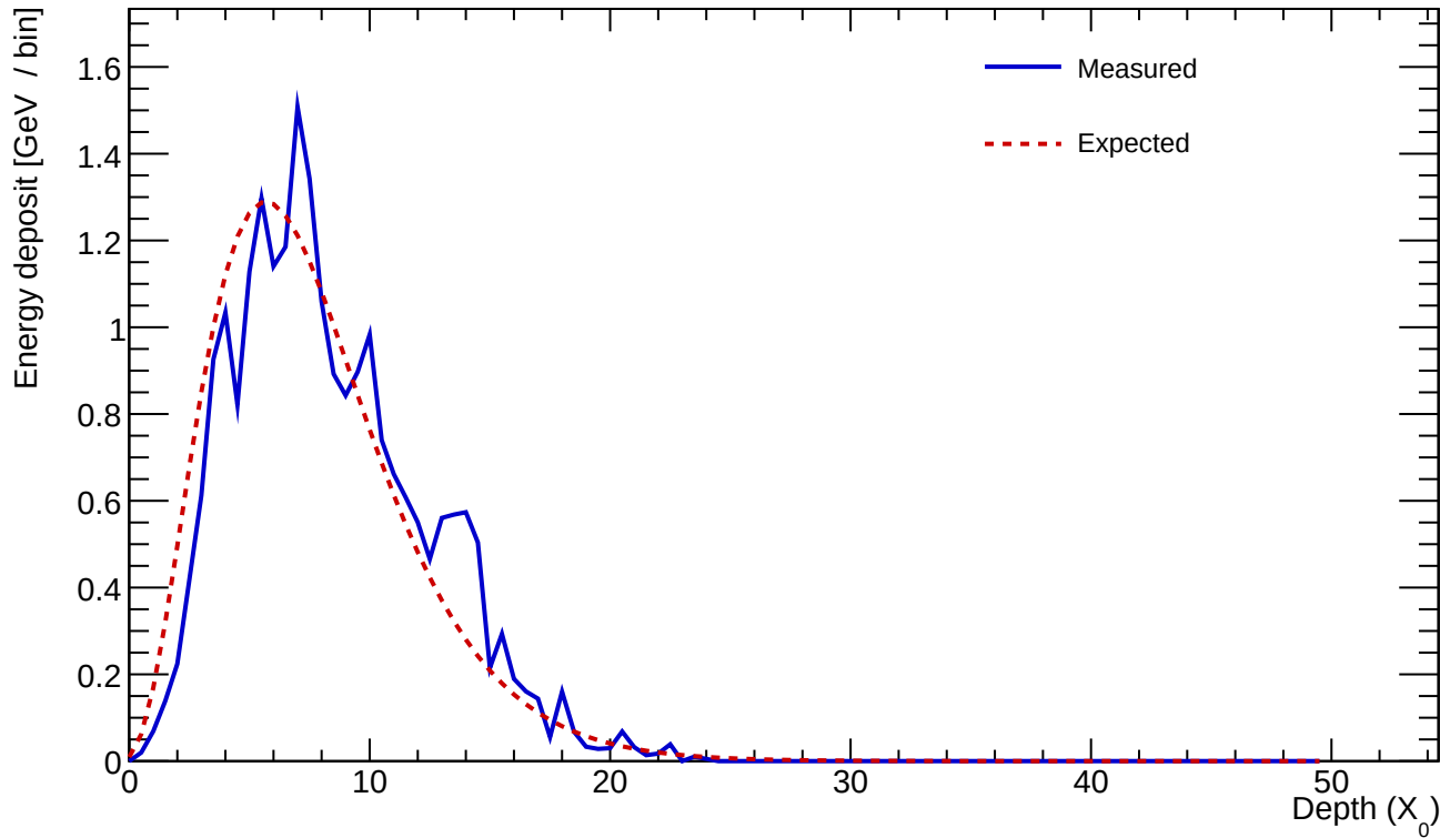
Cluster 336 E=23.334 GeV profileStart=0.50 X_0 \chi=0.1450
