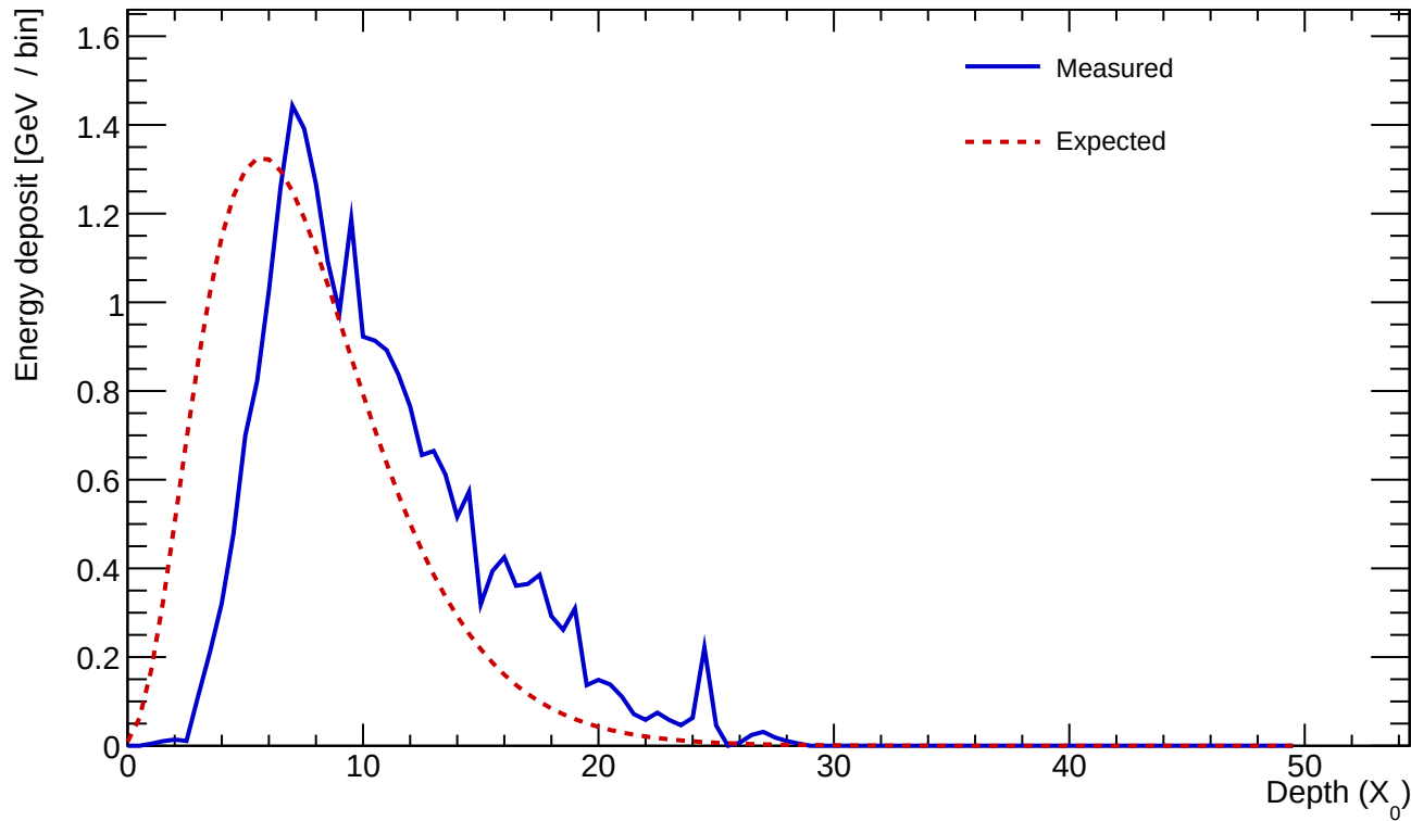
Cluster 543 E=24.068 GeV profileStart=2.50 X_0 \chi=0.1665
