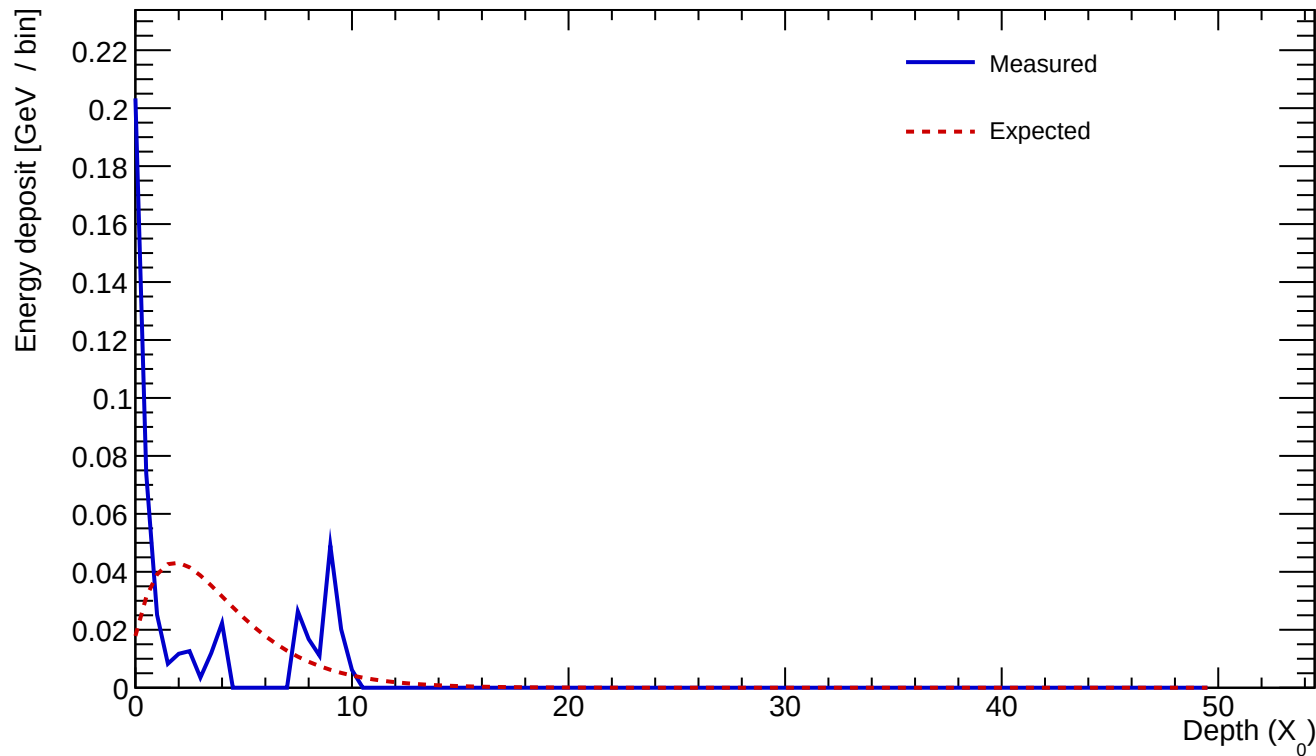
Cluster 48 E=0.502 GeV profileStart=8.00 X_0 \chi=0.9014
