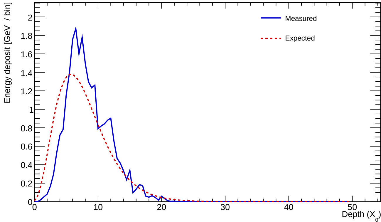
Cluster 114 E=25.119 GeV profileStart=1.50 X_0 \chi=0.1889
