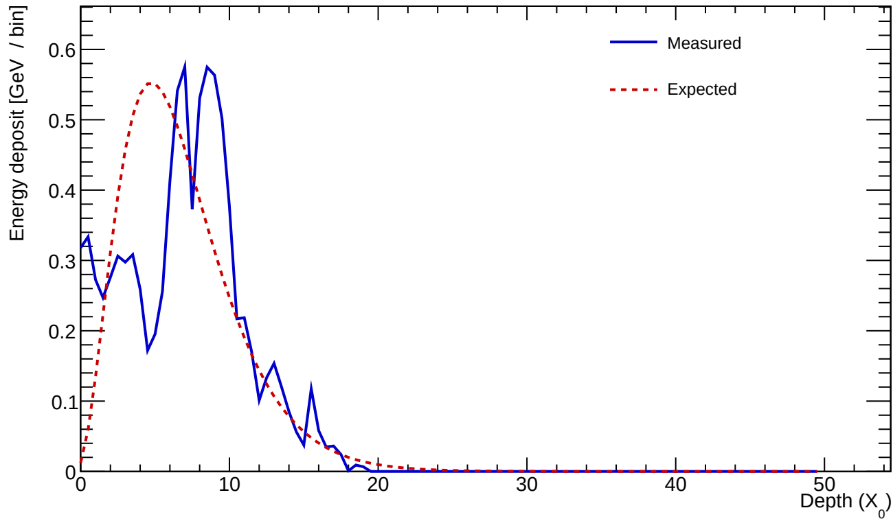
Cluster 306 E=9.272 GeV profileStart=0.50 X_0 \chi=0.4305
