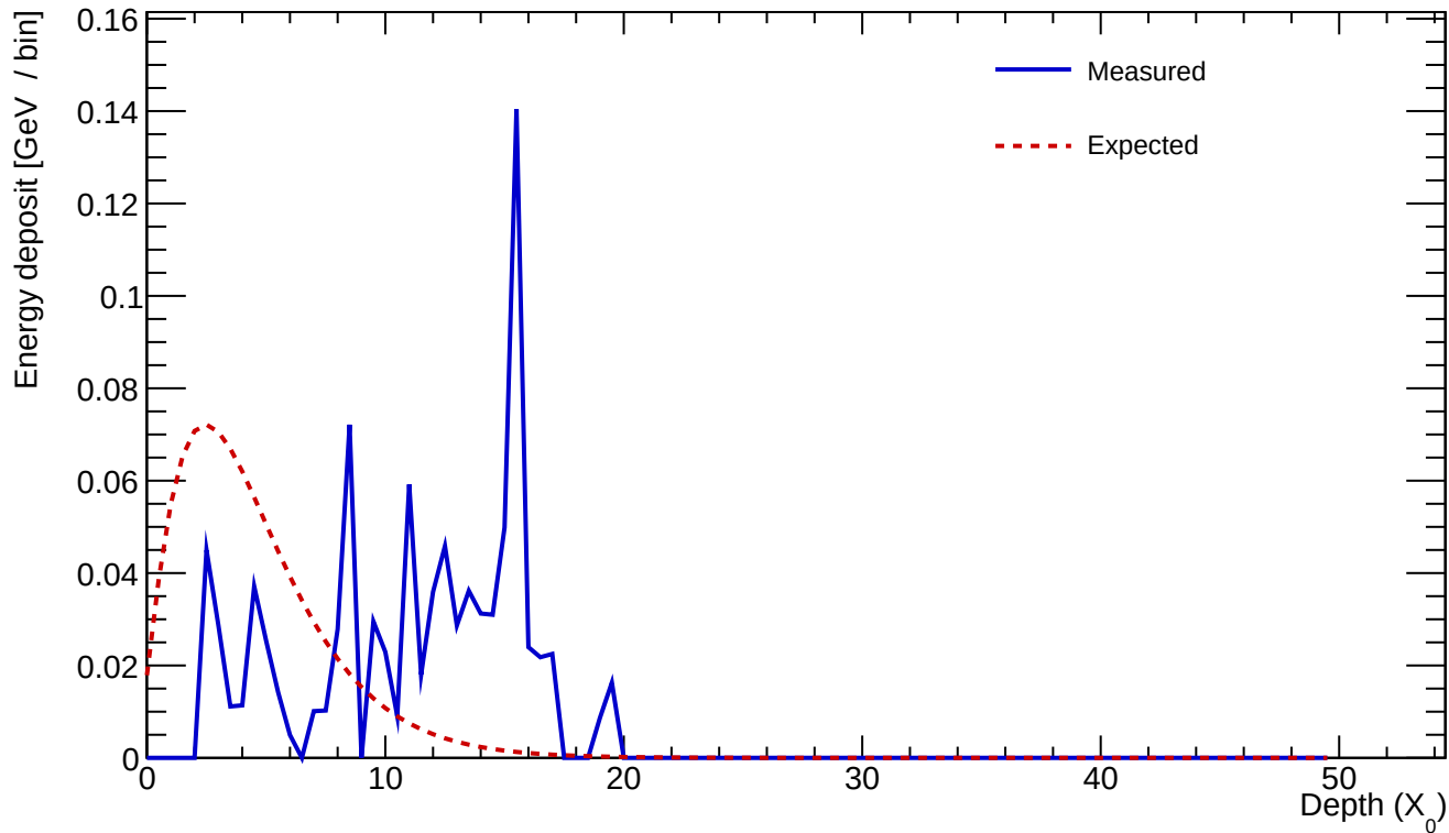
Cluster 550 E=0.929 GeV profileStart=7.50 X_0 \chi=0.7928
