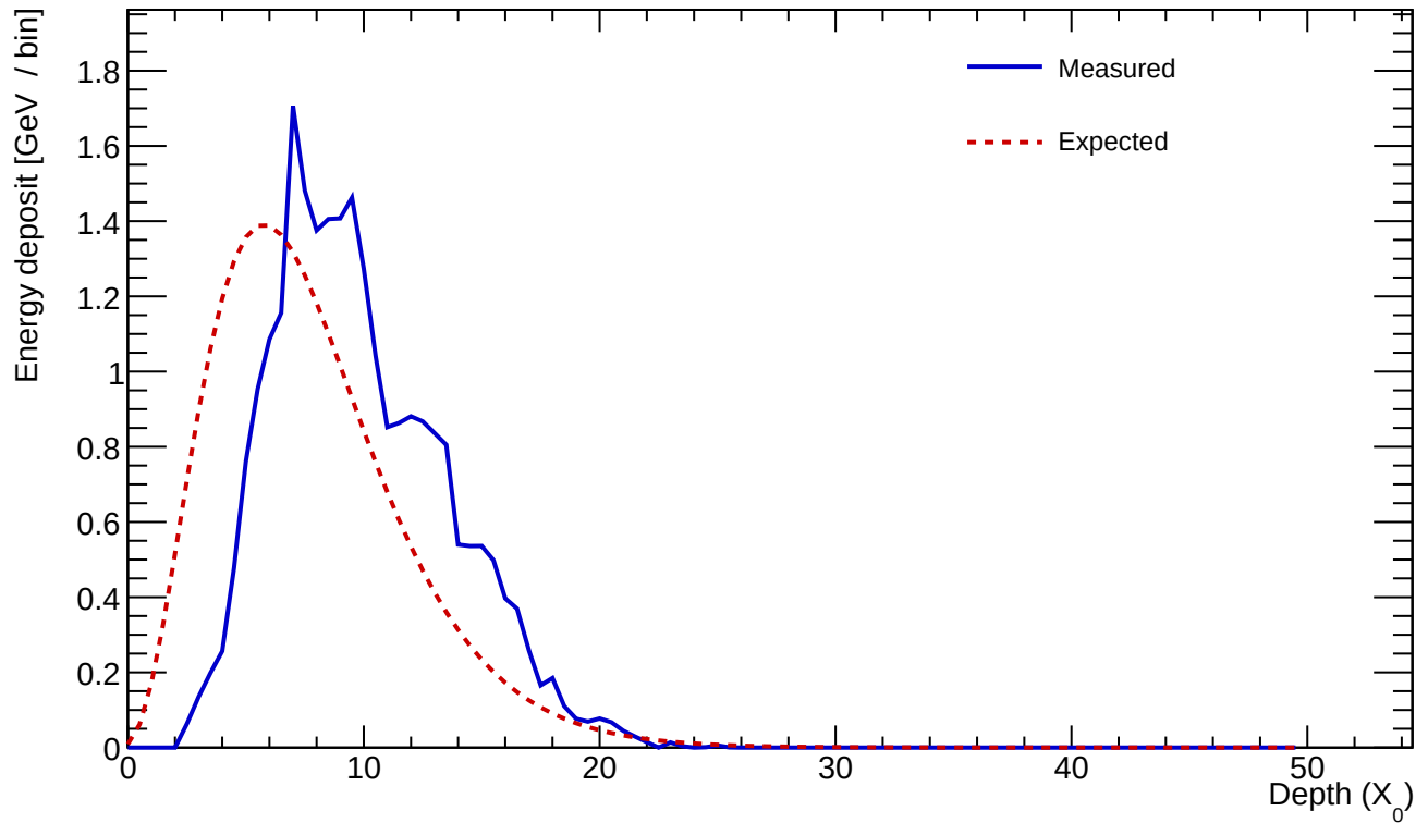
Cluster 391 E=25.346 GeV profileStart=2.50 X_0 \chi=0.1161
