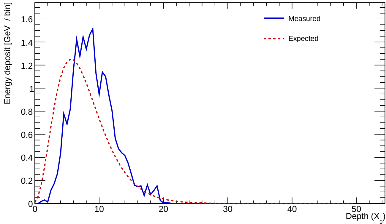
Cluster 42 E=22.573 GeV profileStart=2.00 X_0 \chi=0.1717
