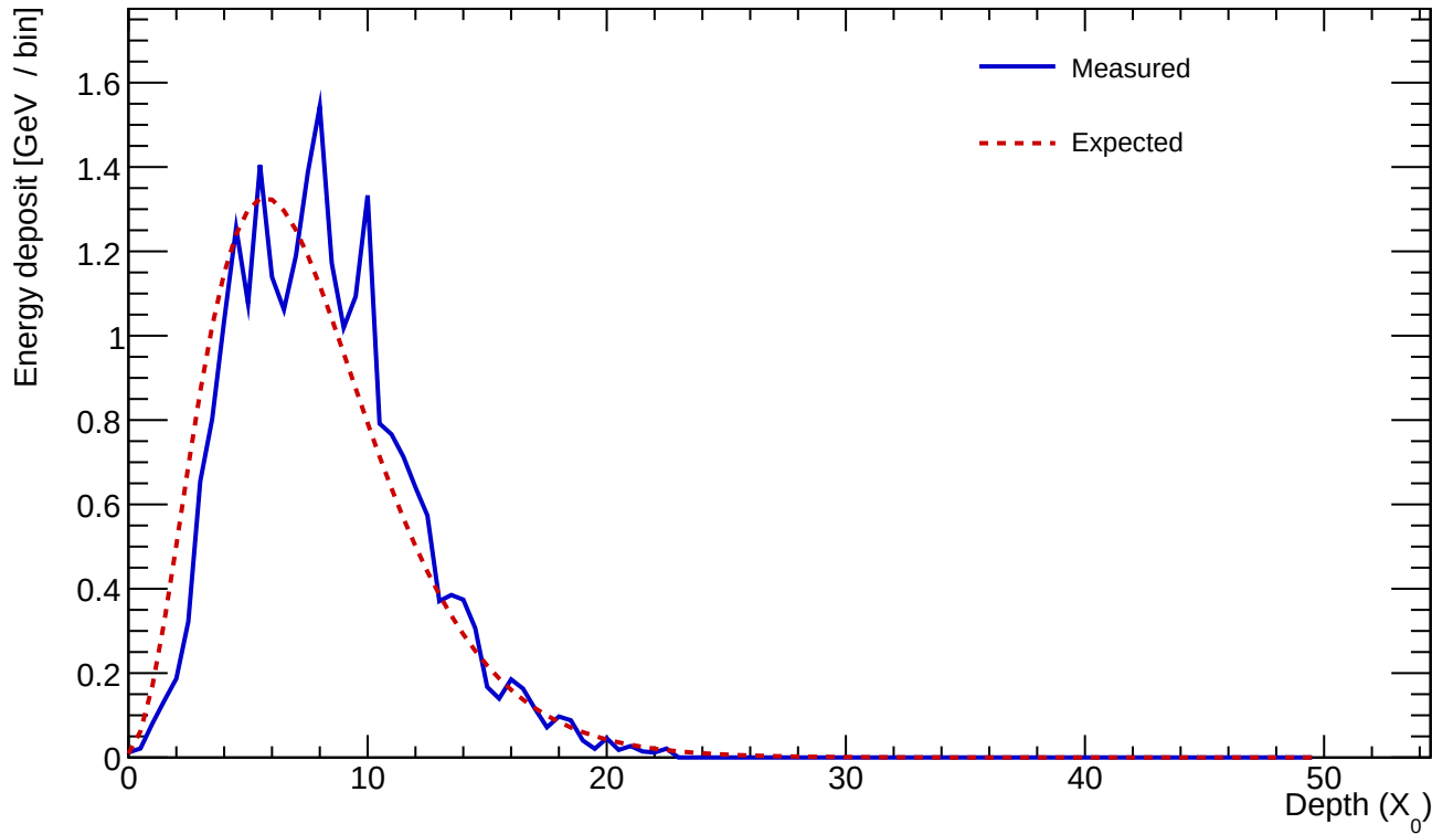
Cluster 669 E=24.075 GeV profileStart=0.50 X_0 \chi=0.1402
