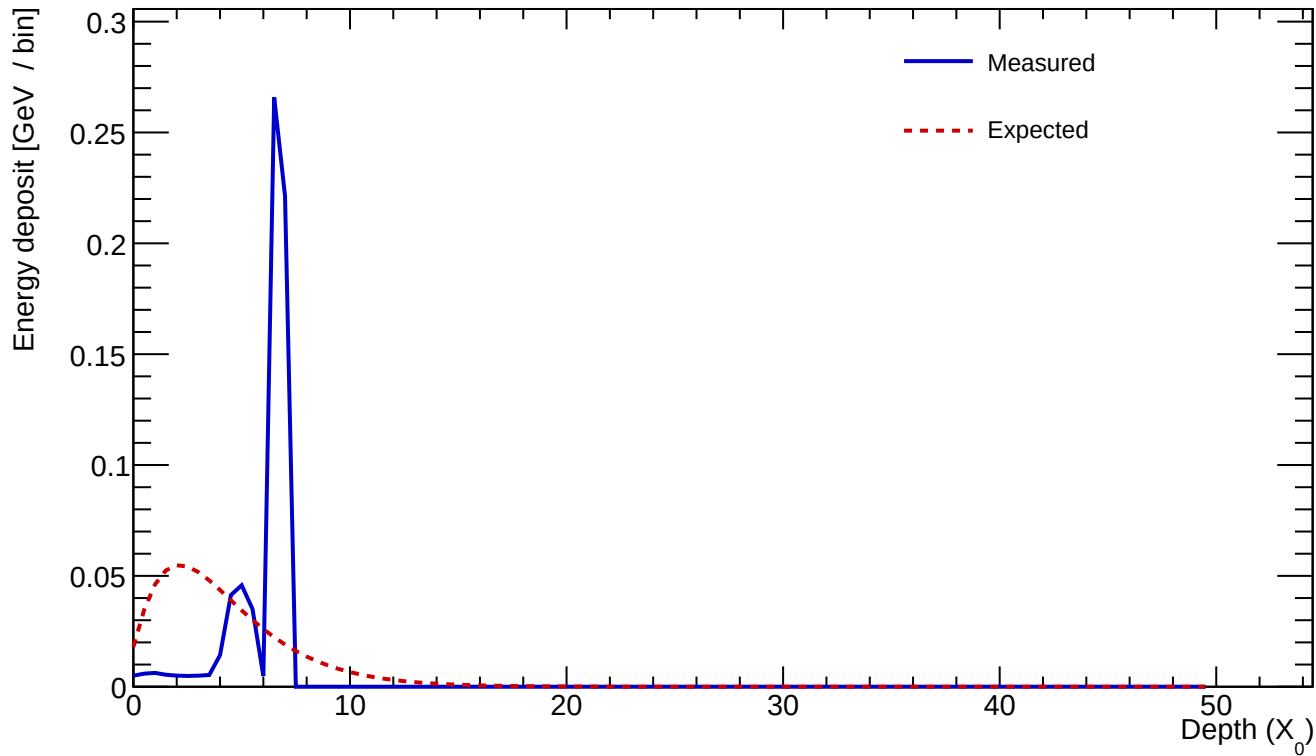
Cluster 766 E=0.671 GeV profileStart=4.00 X_0 \chi=0.4952
