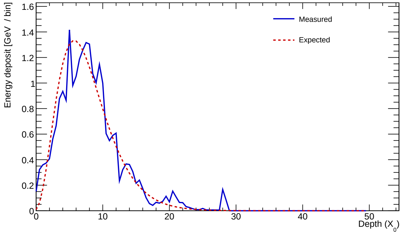
Cluster 192 E=24.185 GeV profileStart=0.50 X_0 \chi=0.1995
