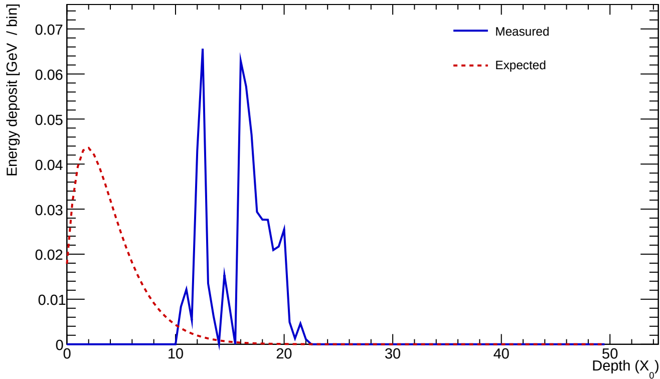
Cluster 595 E=0.509 GeV profileStart=14.50 X_0 \chi=0.6491
