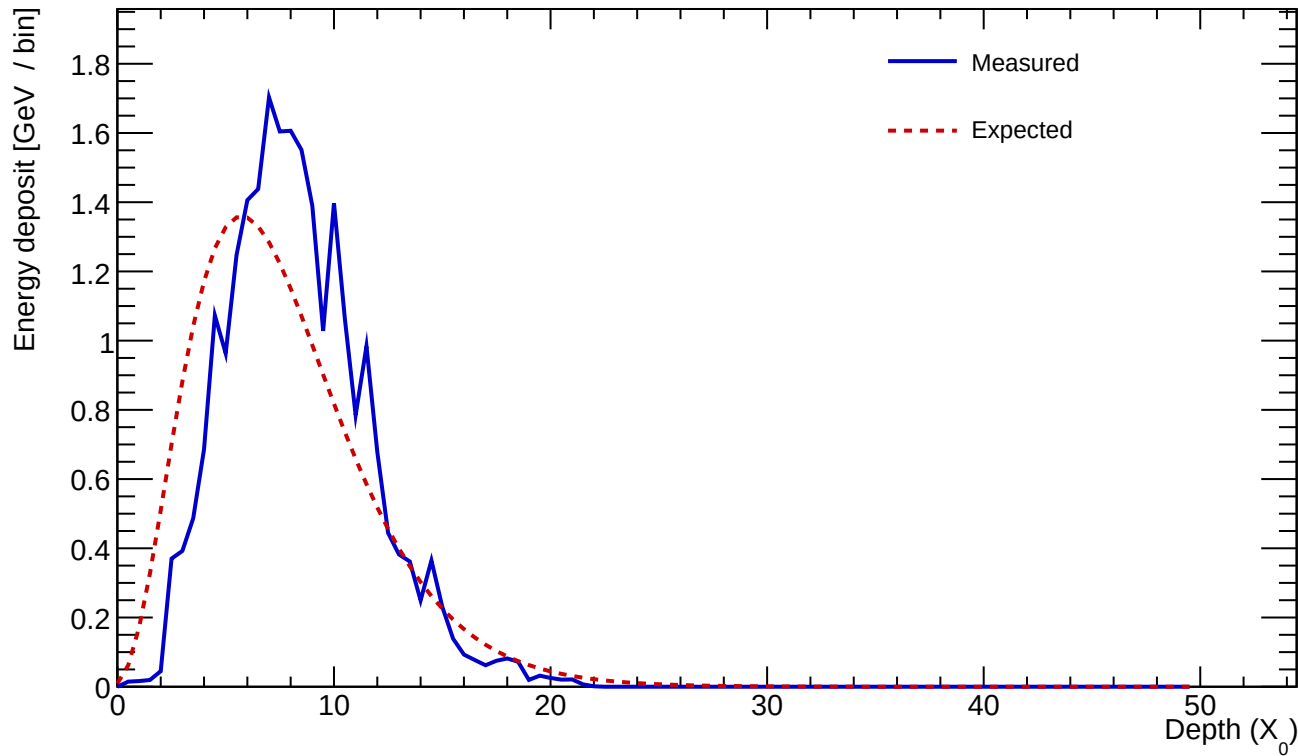
Cluster 352 E=24.710 GeV profileStart=1.00 X_0 \chi=0.2050
