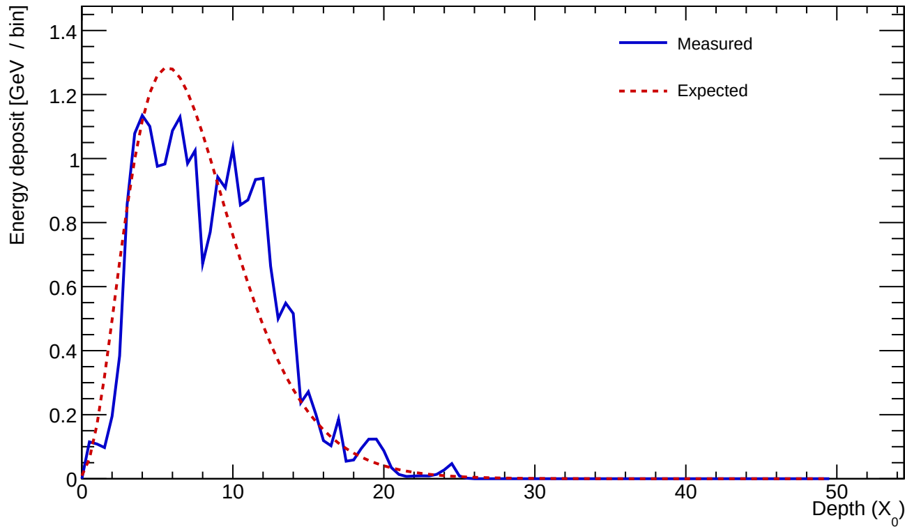
Cluster 345 E=23.247 GeV profileStart=0.50 X_0 \chi=0.2433
