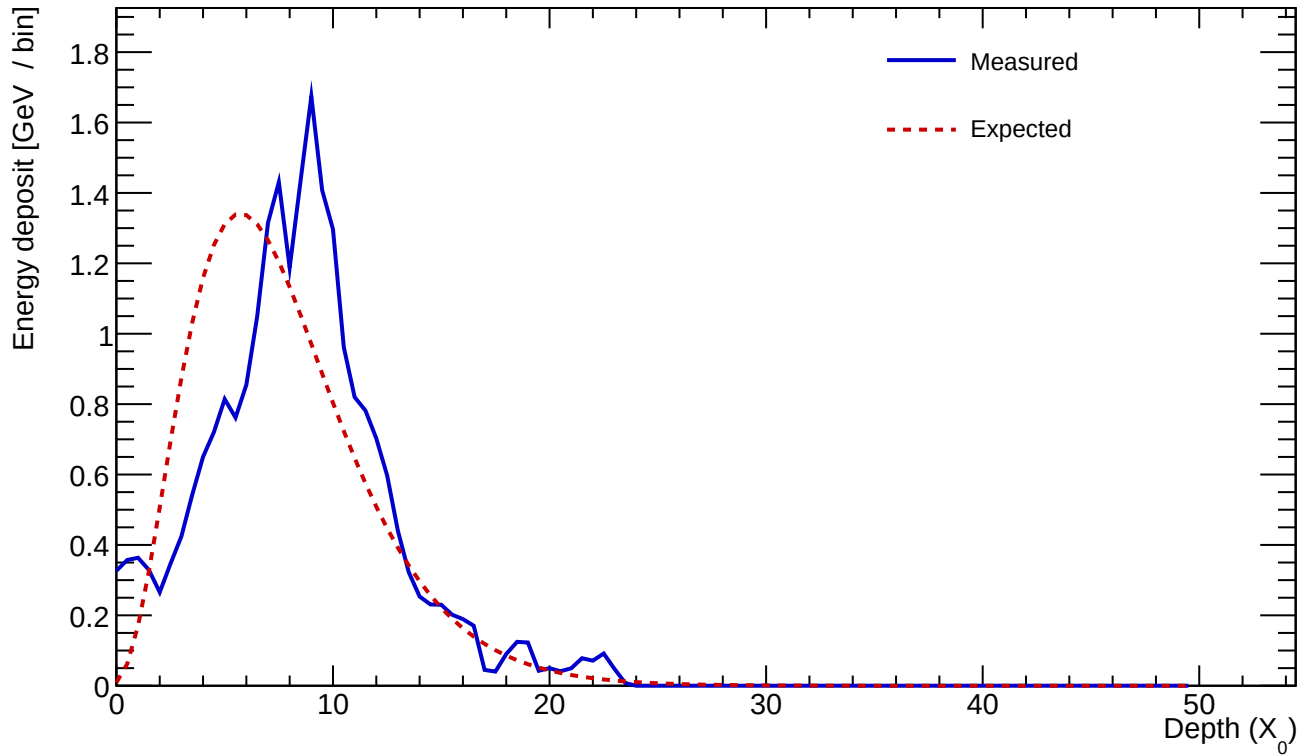
Cluster 320 E=24.354 GeV profileStart=1.50 X_0 \chi=0.2672
