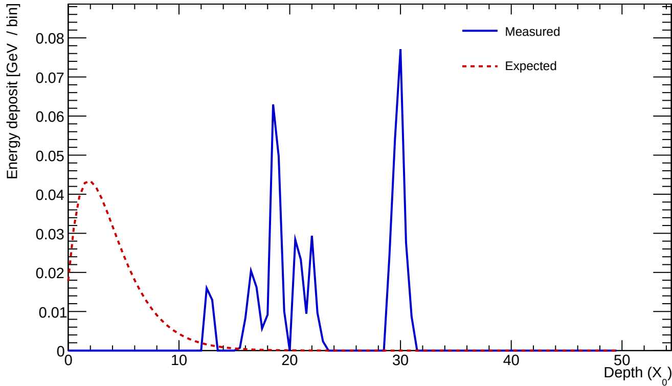
Cluster 1017 E=0.506 GeV profileStart=16.00 X_0 \chi=1.0049
