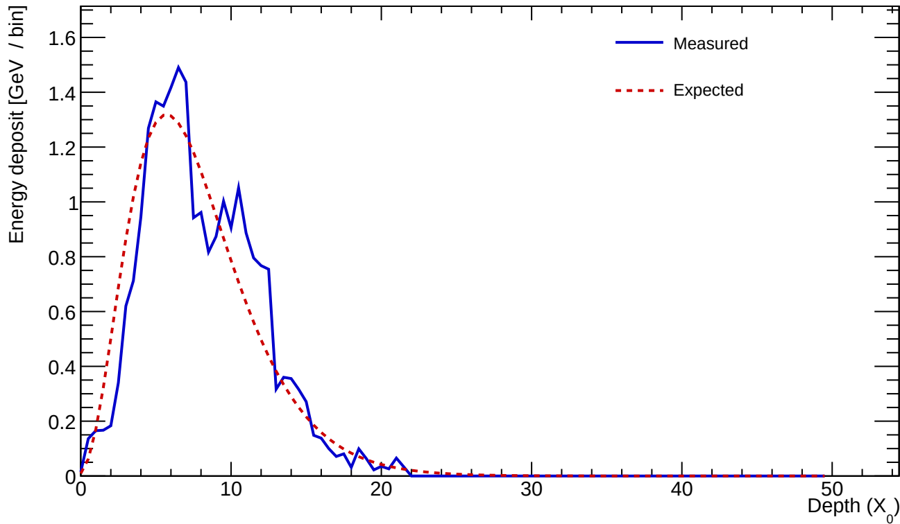
Cluster 417 E=23.903 GeV profileStart=0.50 X_0 \chi=0.1837
