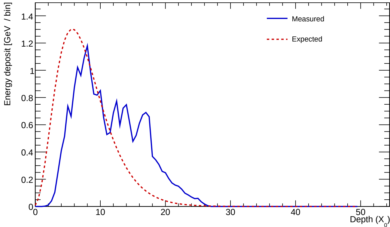
Cluster 274 E=23.600 GeV profileStart=2.50 X_0 \chi=0.3482
