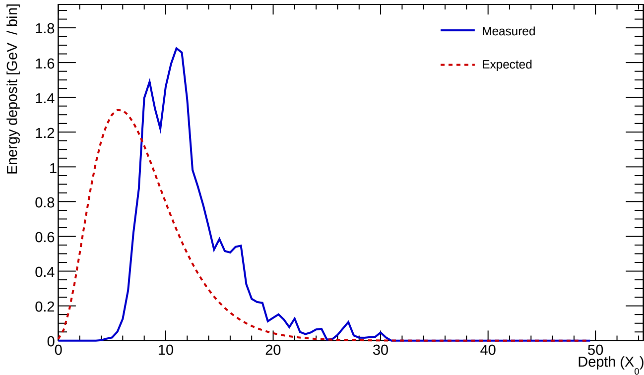
Cluster 973 E=24.119 GeV profileStart=4.50 X_0 \chi=0.2193
