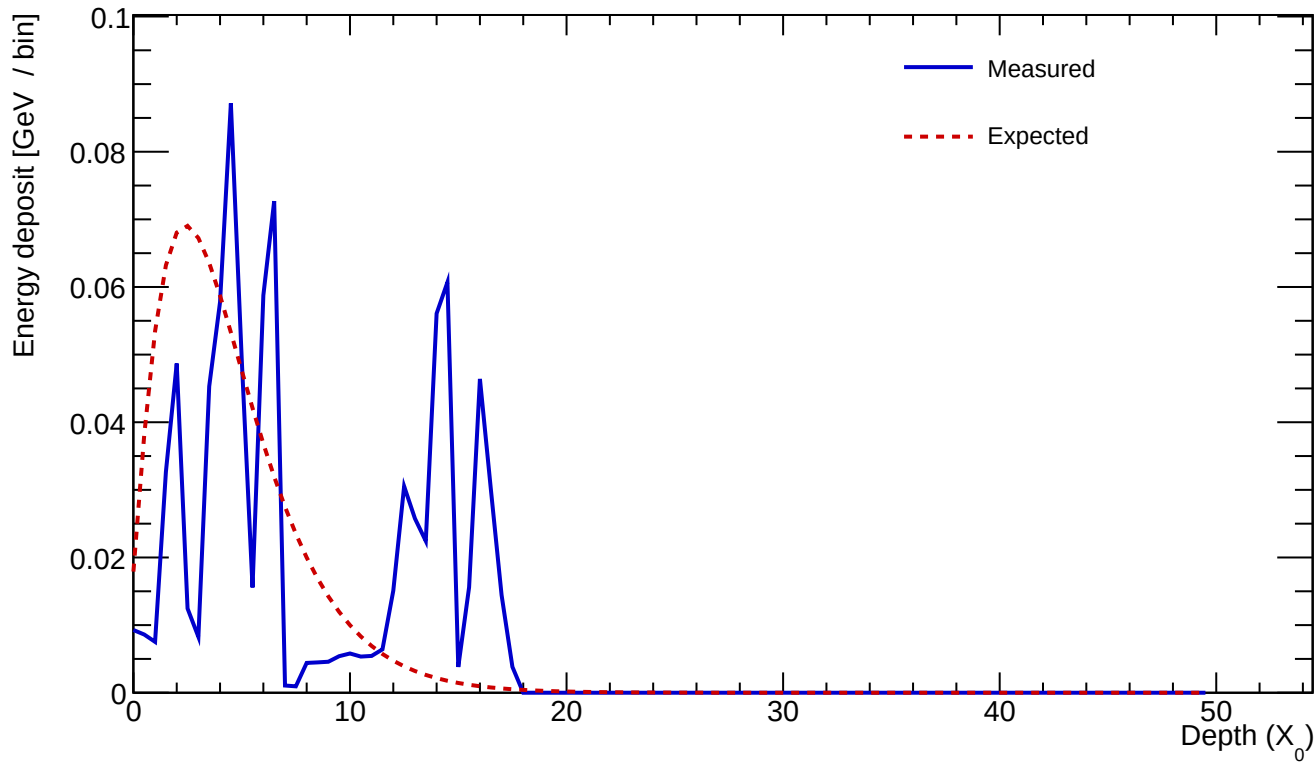
Cluster 578 E=0.883 GeV profileStart=1.00 X_0 \chi=0.8362
