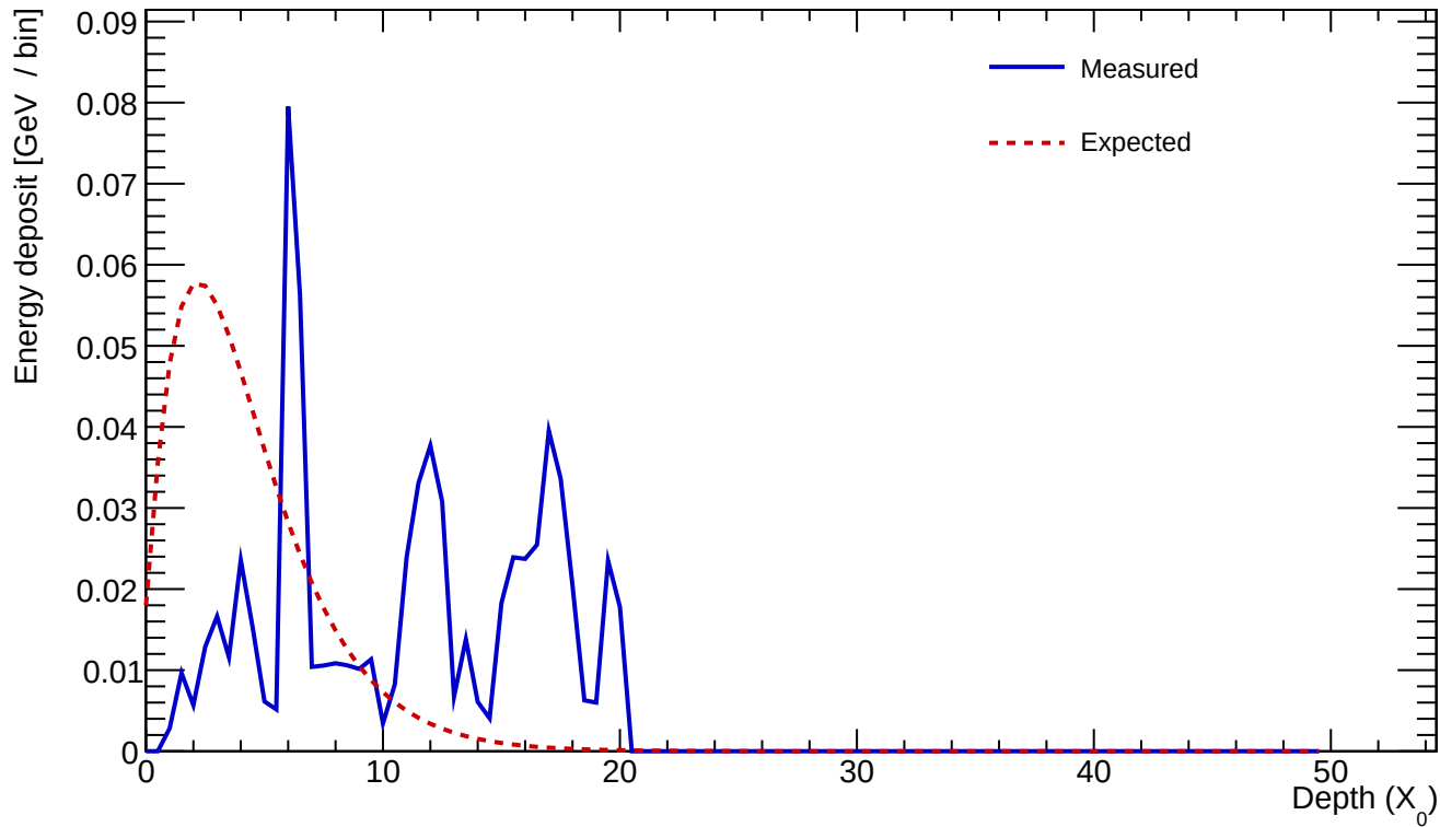
Cluster 173 E=0.715 GeV profileStart=11.00 X_0 \chi=0.9412
