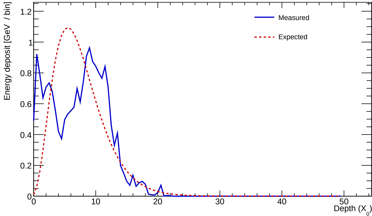
Cluster 797 E=19.530 GeV profileStart=0.50 X_0 \chi=0.5121
