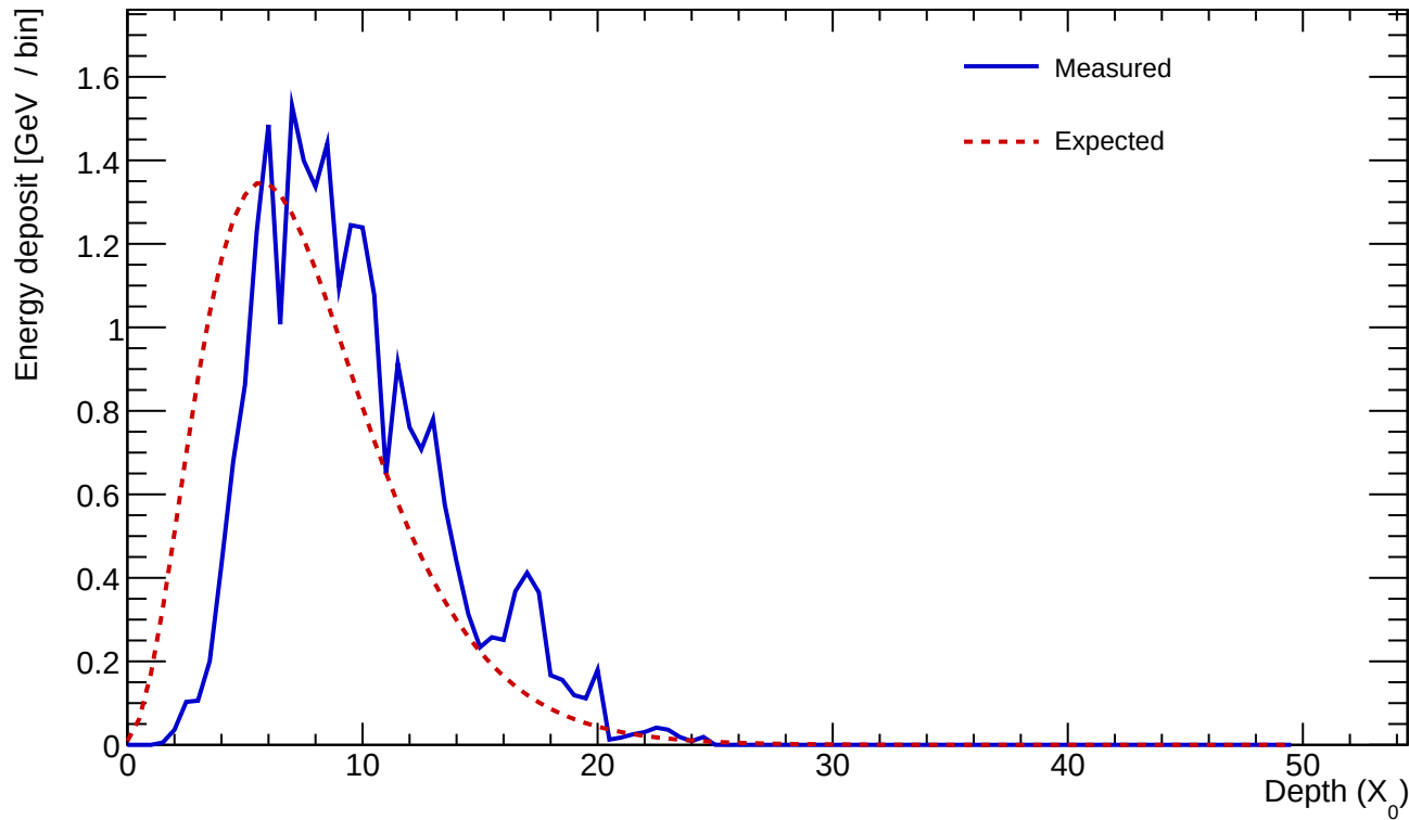
Cluster 940 E=24.478 GeV profileStart=2.00 X_0 \chi=0.1507
