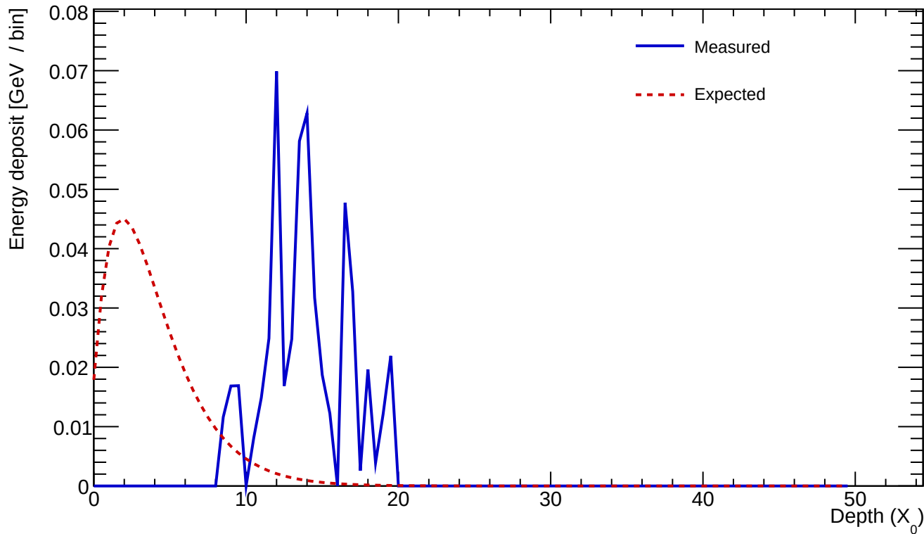
Cluster 706 E=0.529 GeV profileStart=11.00 X_0 \chi=0.5849
