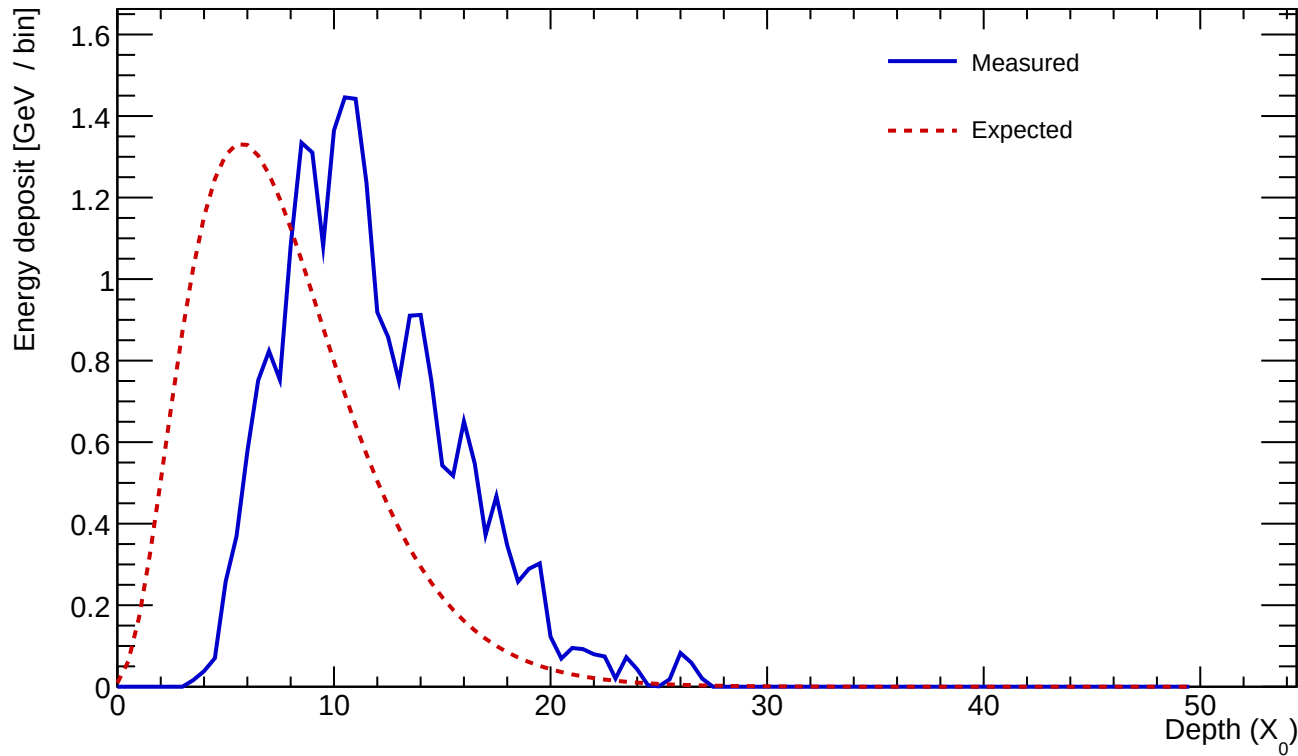
Cluster 925 E=24.201 GeV profileStart=4.00 X_0 \chi=0.1409
