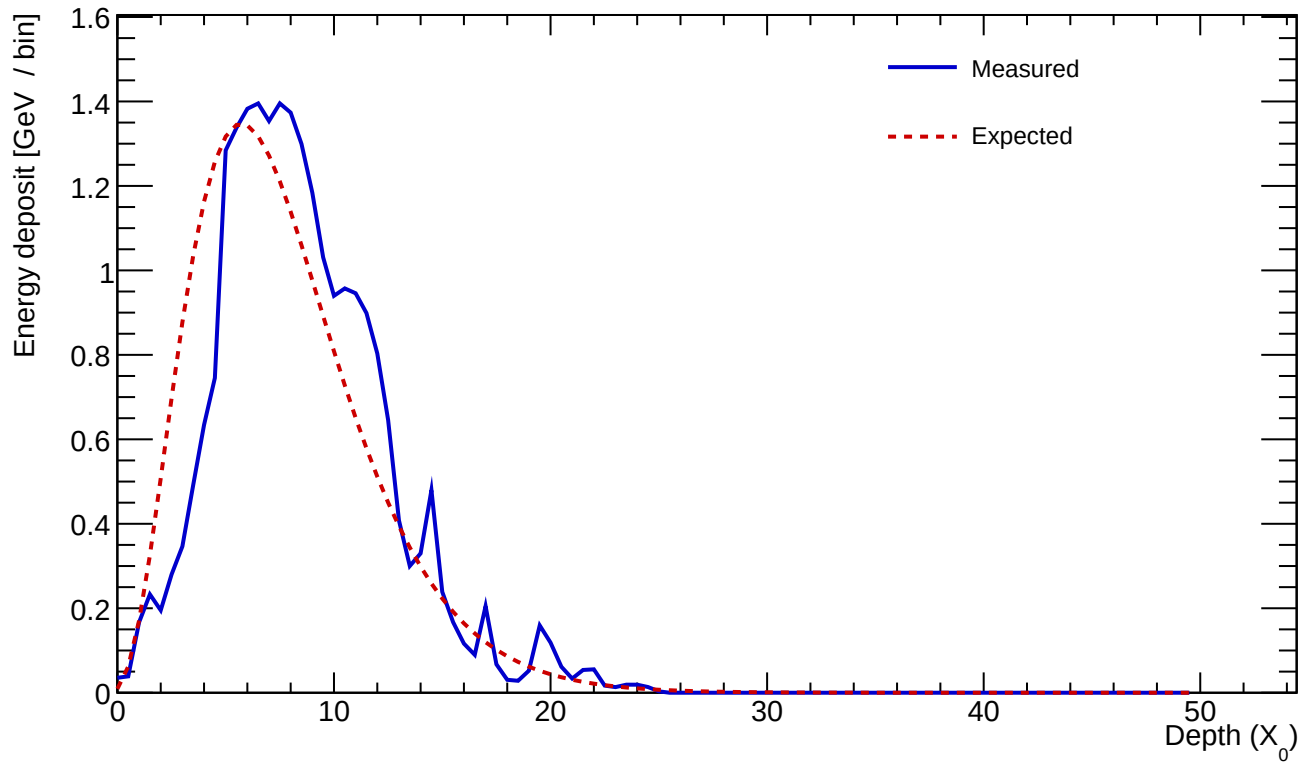
Cluster 144 E=24.475 GeV profileStart=1.50 X_0 \chi=0.1581
