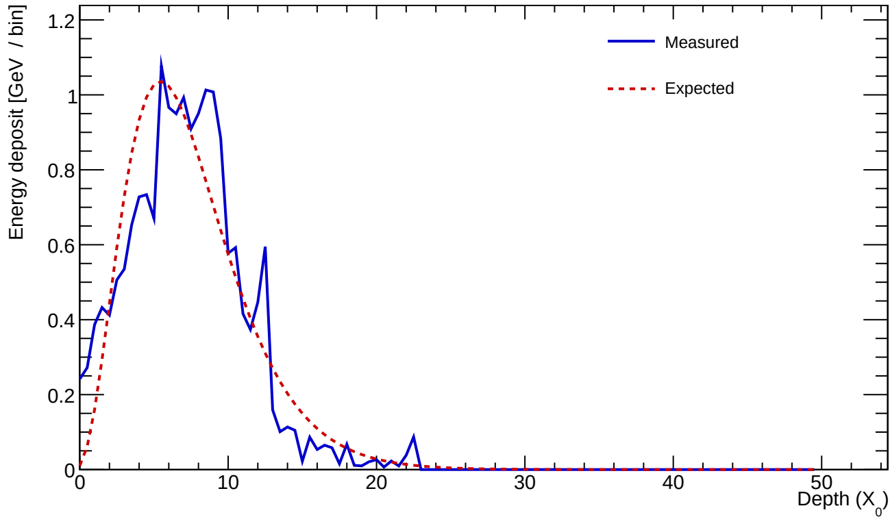
Cluster 690 E=18.402 GeV profileStart=0.50 X_0 \chi=0.2511
