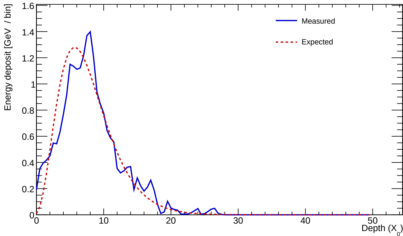
Cluster 381 E=23.146 GeV profileStart=0.50 X_0 \chi=0.2115
