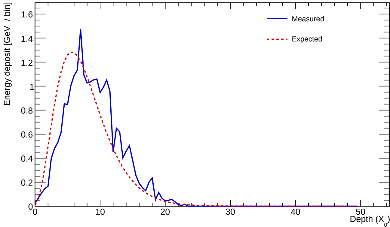
Cluster 889 E=23.241 GeV profileStart=1.50 X_0 \chi=0.1730
