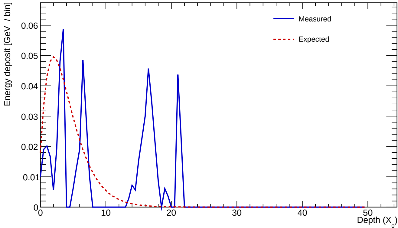
Cluster 842 E=0.593 GeV profileStart=0.50 X_0 \chi=1.0459
