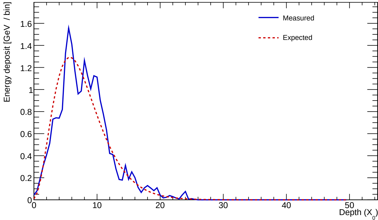
Cluster 776 E=23.401 GeV profileStart=0.50 X_0 \chi=0.1919
