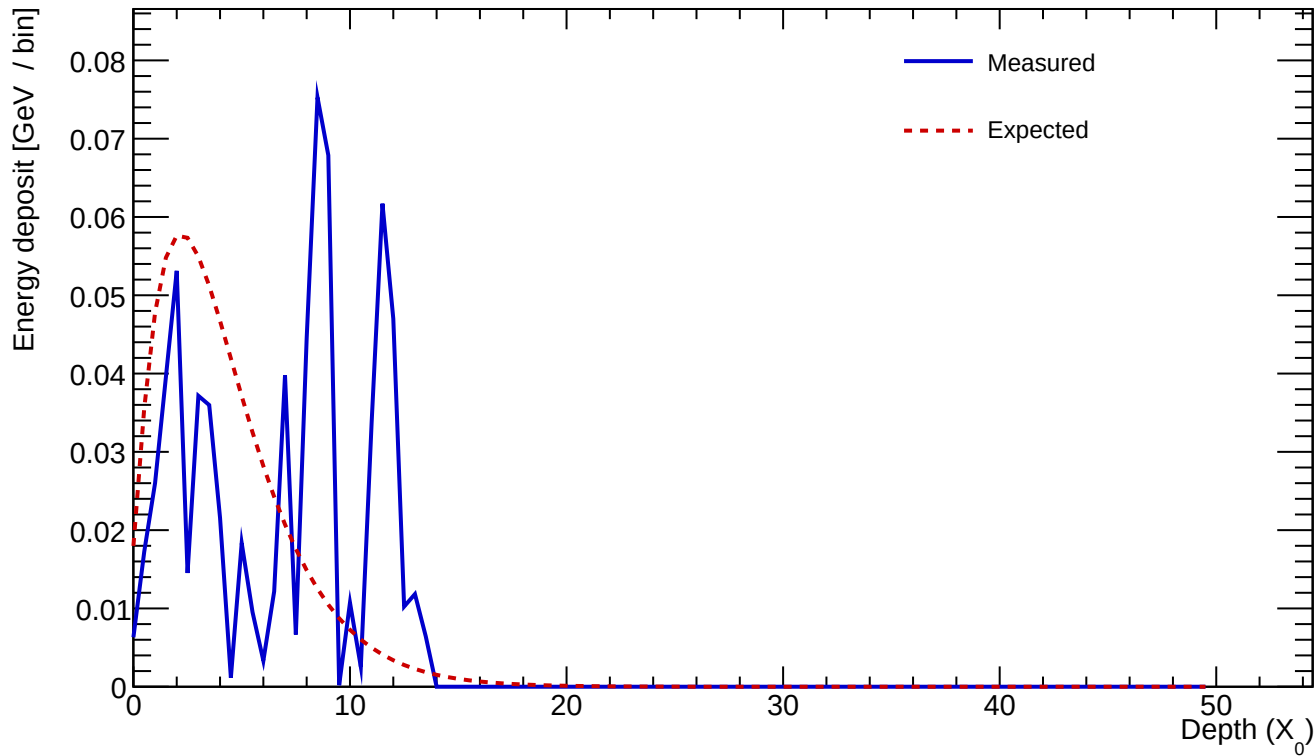
Cluster 460 E=0.715 GeV profileStart=0.50 X_0 \chi=0.8576
