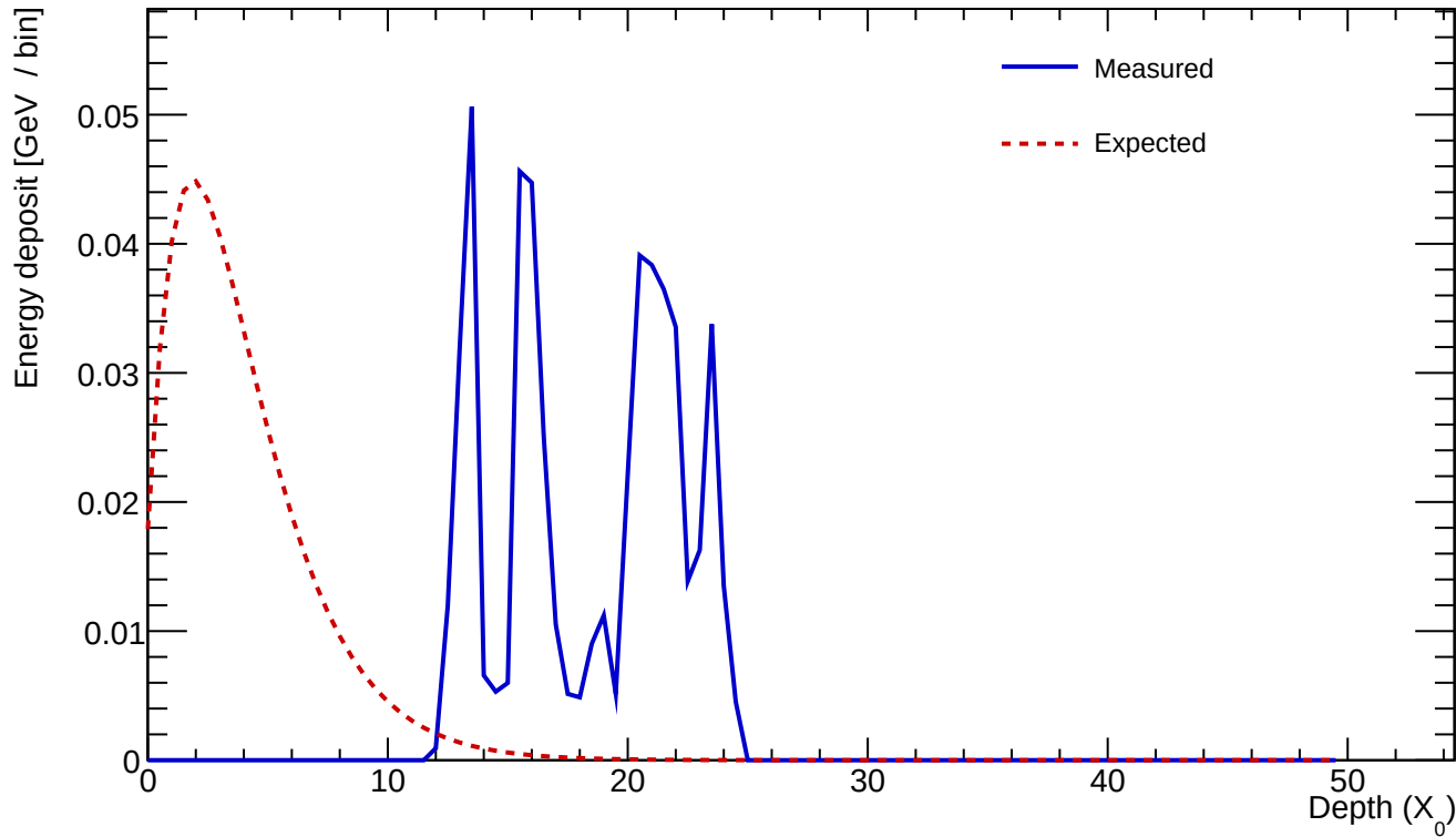
Cluster 918 E=0.526 GeV profileStart=19.50 X_0 \chi=0.7238
