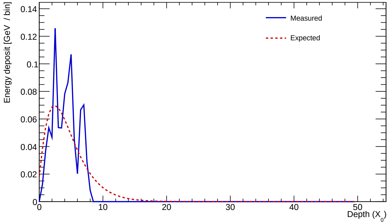
Cluster 131 E=0.893 GeV profileStart=0.50 X_0 \chi=0.3338
