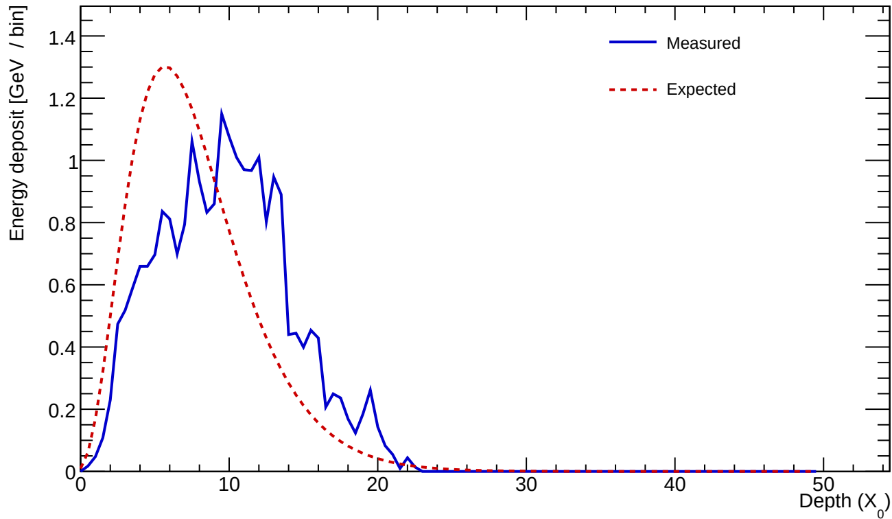
Cluster 176 E=23.594 GeV profileStart=2.50 X_0 \chi=0.2820
