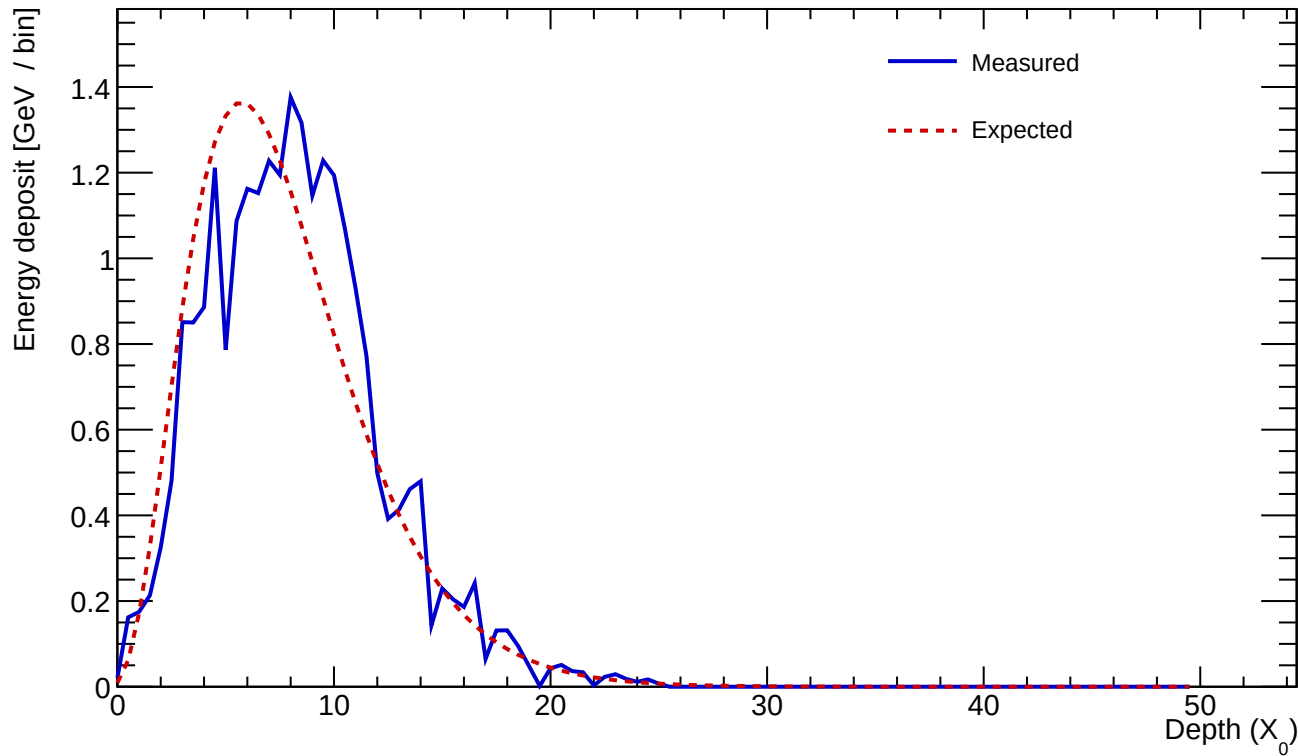
Cluster 3 E=24.815 GeV profileStart=0.50 X_0 \chi=0.1837
