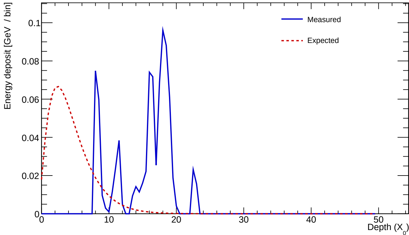
Cluster 649 E=0.847 GeV profileStart=15.00 X_0 \chi=0.7352
