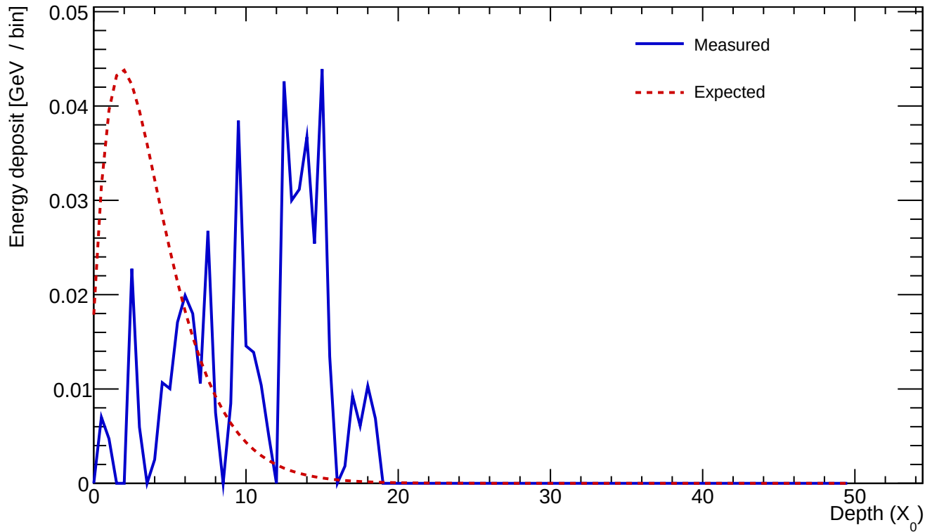
Cluster 978 E=0.512 GeV profileStart=9.00 X_0 \chi=0.8354
