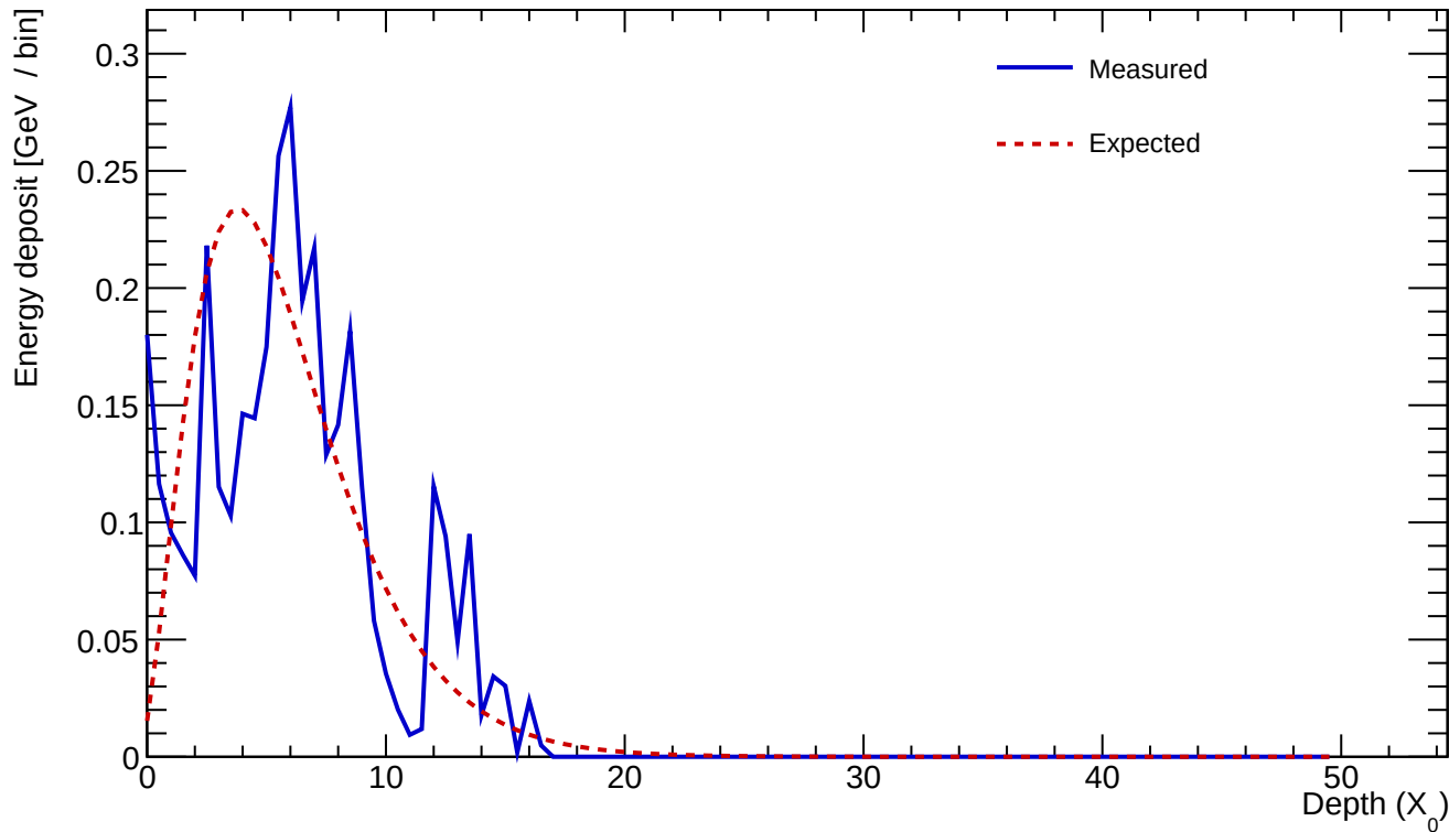
Cluster 1144 E=3.571 GeV profileStart=0.50 X_0 \chi=0.4573
