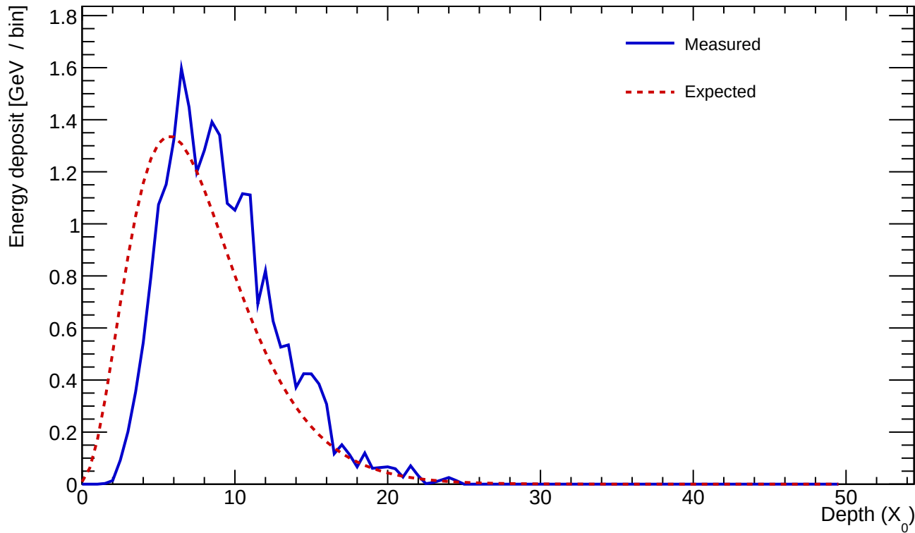
Cluster 798 E=24.293 GeV profileStart=1.50 X_0 \chi=0.1274
