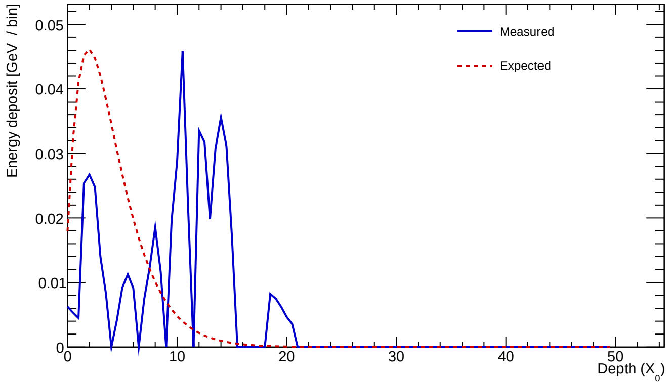
Cluster 286 E=0.545 GeV profileStart=9.50 X_0 \chi=0.7800
