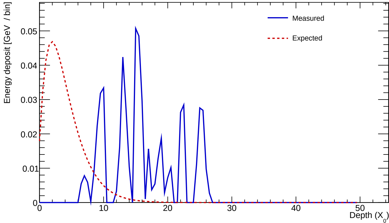
Cluster 844 E=0.555 GeV profileStart=12.50 X_0 \chi=0.9091
