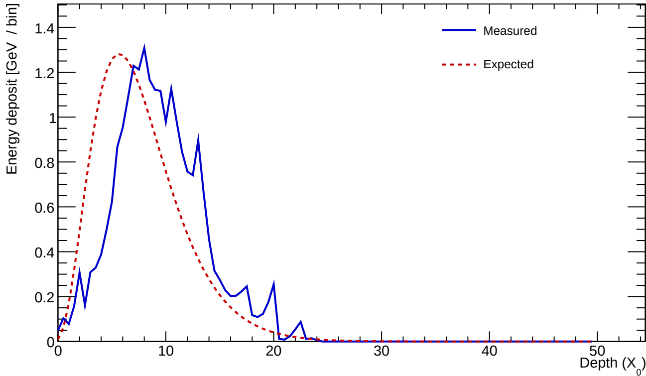
Cluster 357 E=23.202 GeV profileStart=2.50 X_0 \chi=0.1698
