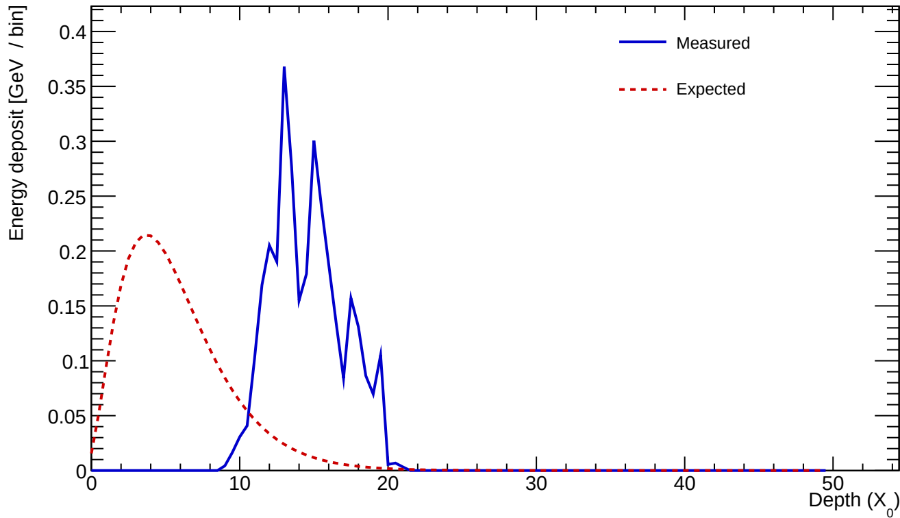
Cluster 419 E=3.250 GeV profileStart=10.00 X_0 \chi=0.2782
