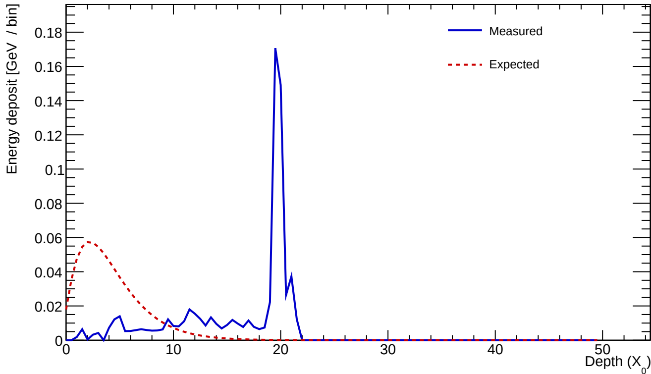
Cluster 988 E=0.709 GeV profileStart=18.50 X_0 \chi=0.8118
