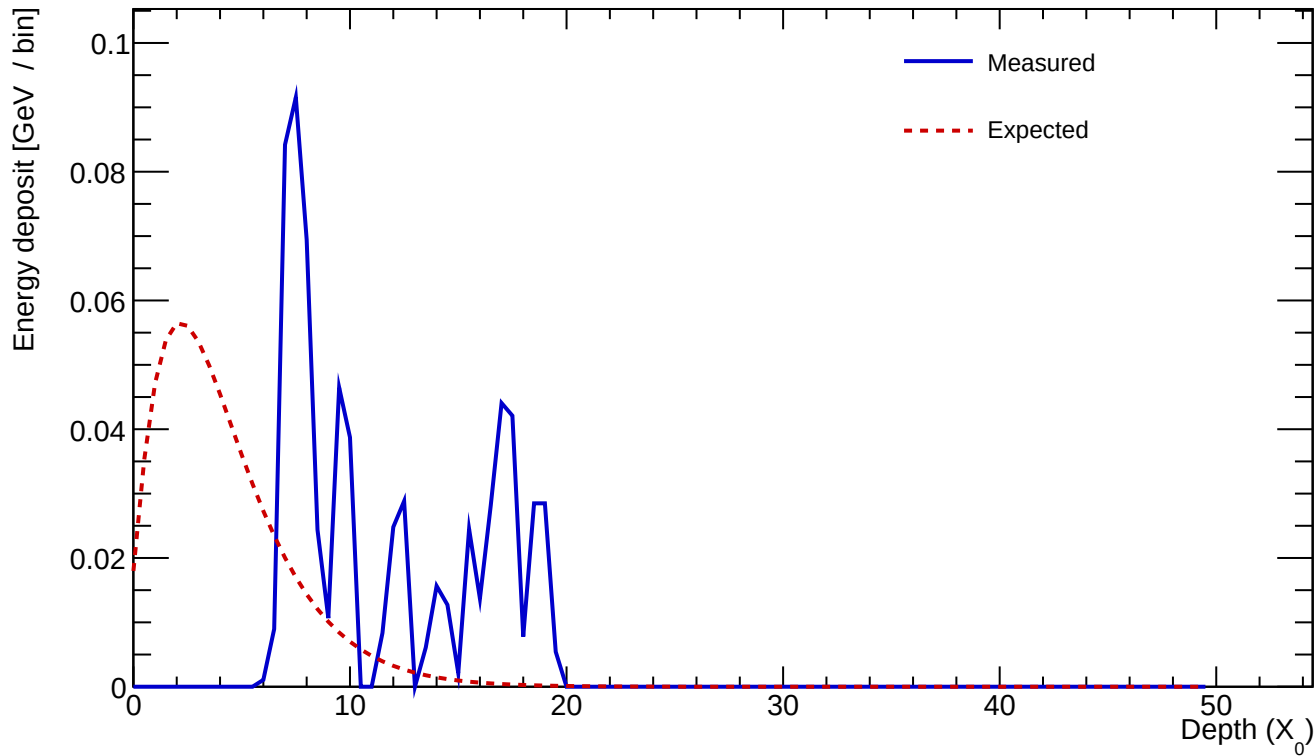
Cluster 1154 E=0.697 GeV profileStart=6.00 X_0 \chi=0.7801
