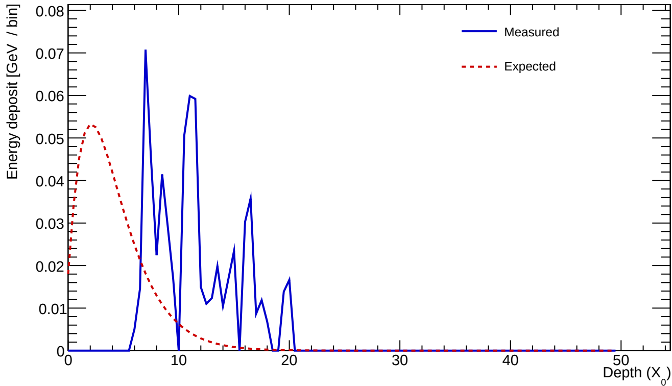
Cluster 857 E=0.648 GeV profileStart=6.50 X_0 \chi=0.6145
