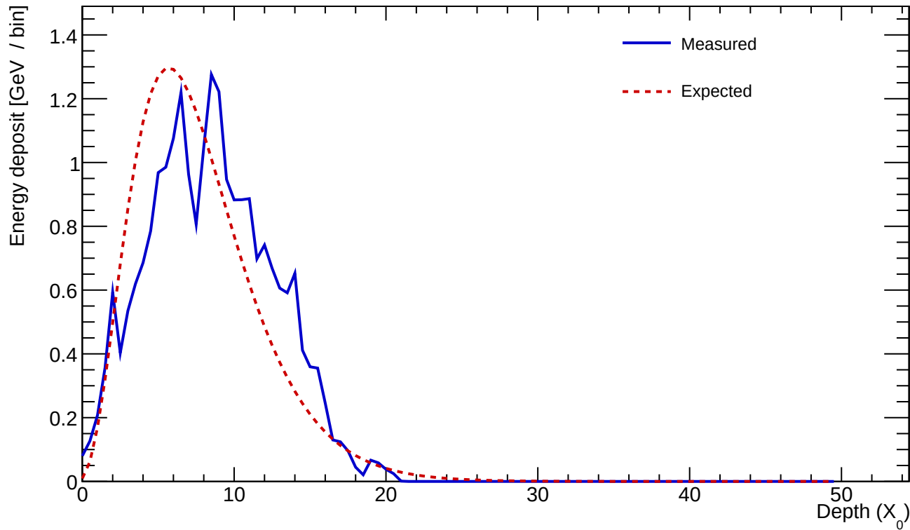
Cluster 222 E=23.490 GeV profileStart=1.50 X_0 \chi=0.2134
