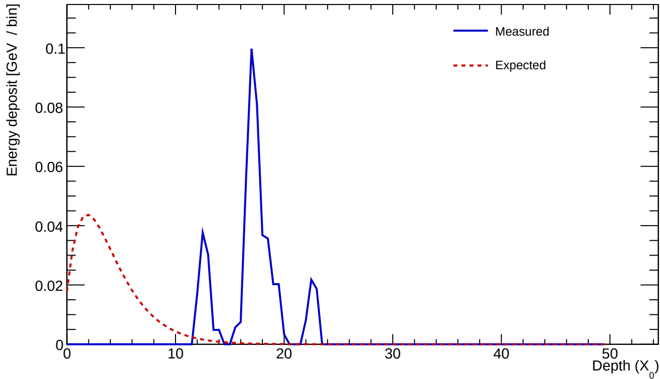
Cluster 830 E=0.510 GeV profileStart=15.50 X_0 \chi=0.7512
