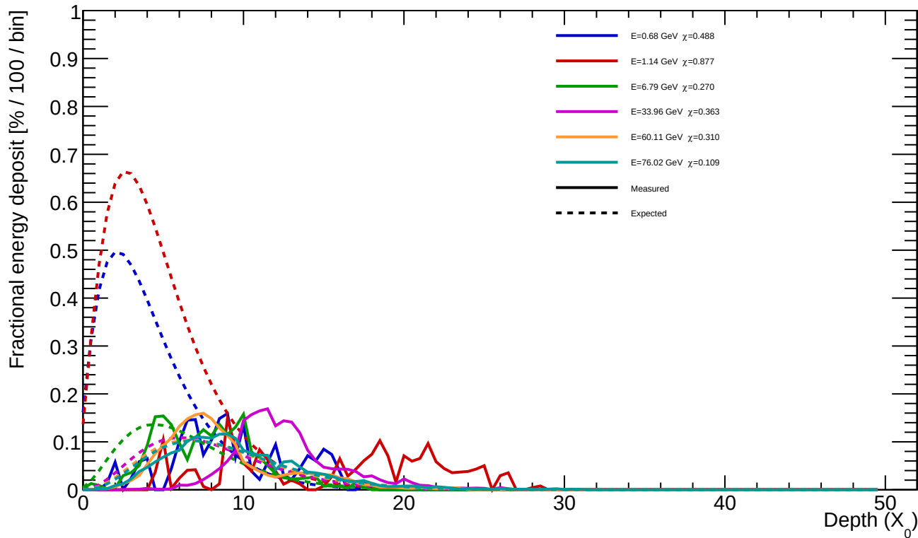
Longitudinal shower profiles: measured (solid) vs expected (dashed)
