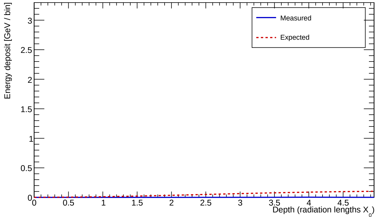
Cluster 5 E=33.961 GeV profileStart=5.50 X_0 \chi=0.3628
