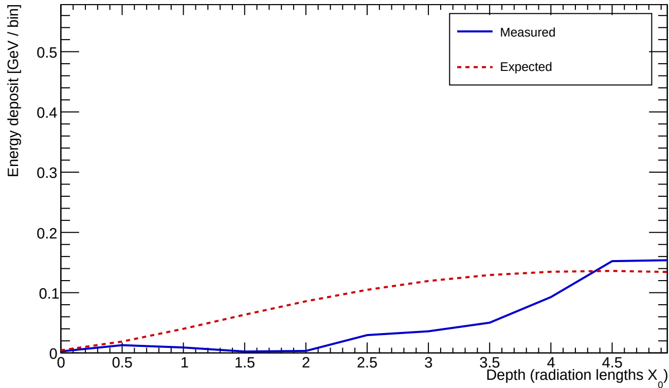
Cluster 8 E=6.788 GeV profileStart=2.00 X_0 \chi=0.2702
