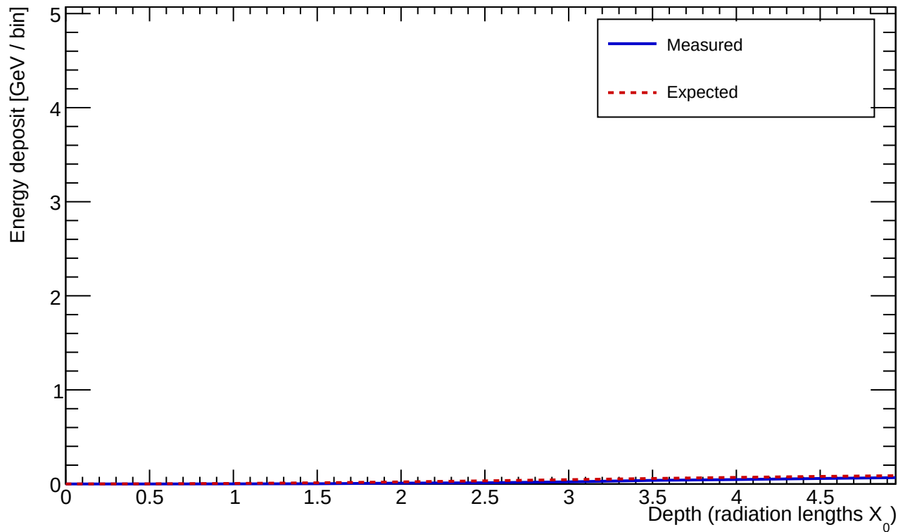
Cluster 7 E=76.019 GeV profileStart=1.00 X_0 \chi=0.1088
