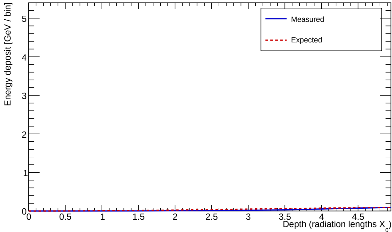
Cluster 4 E=60.106 GeV profileStart=0.50 X_0 \chi=0.3096
