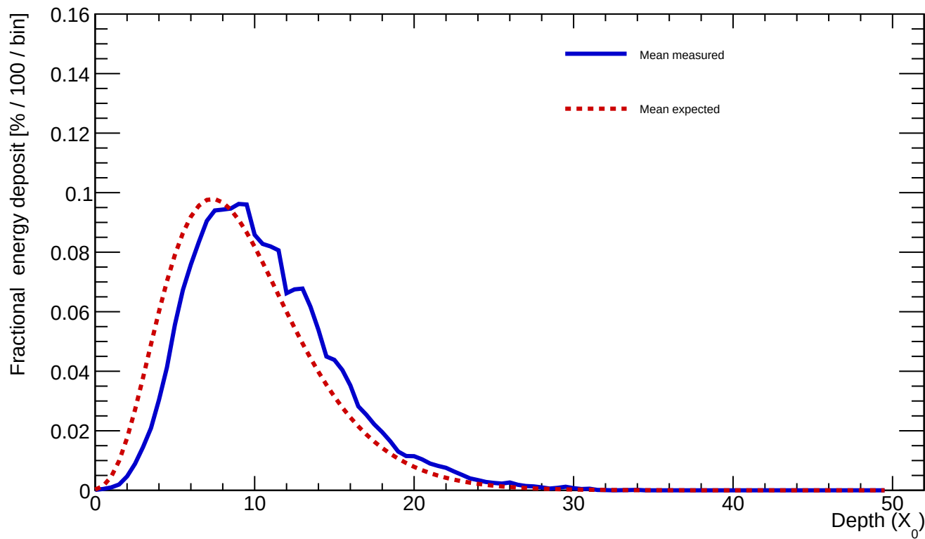
Average longitudinal profile (9 clusters): measured vs expected
