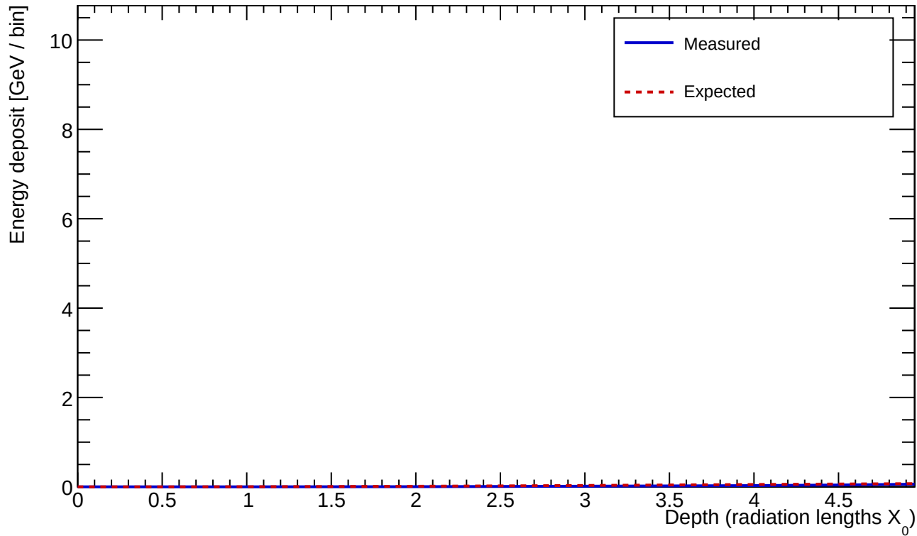
Cluster 3 E=181.271 GeV profileStart=0.50 X_0 \chi=0.1034
