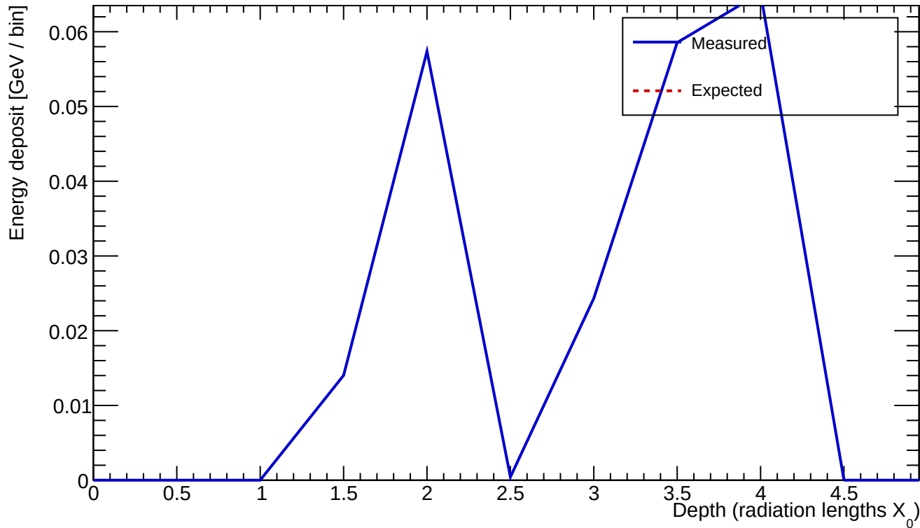
Cluster 6 E=0.678 GeV profileStart=5.50 X_0 \chi=0.4876
