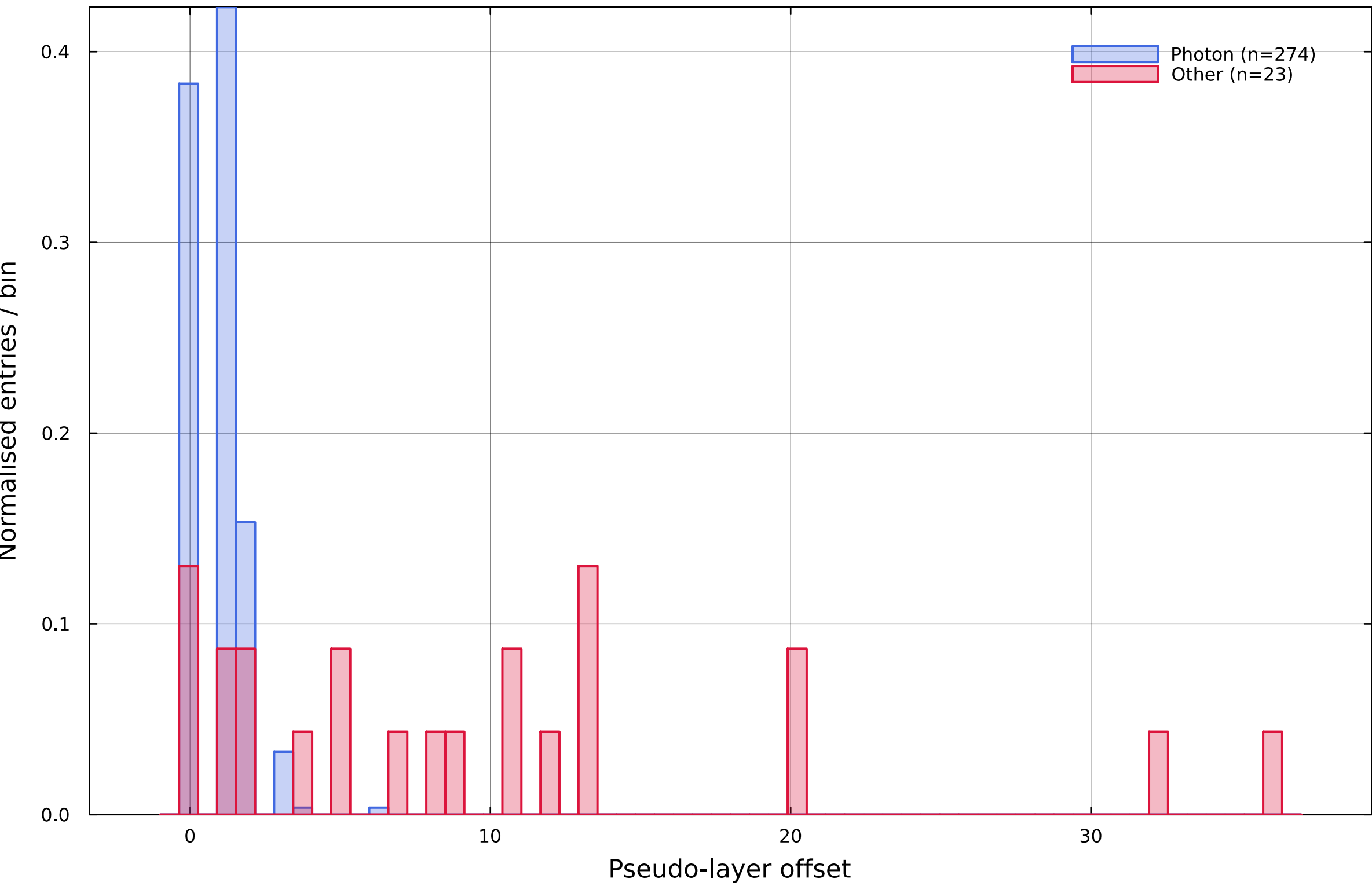
Shower start offset: photon vs other (showerStartLayer – innerLayer)
