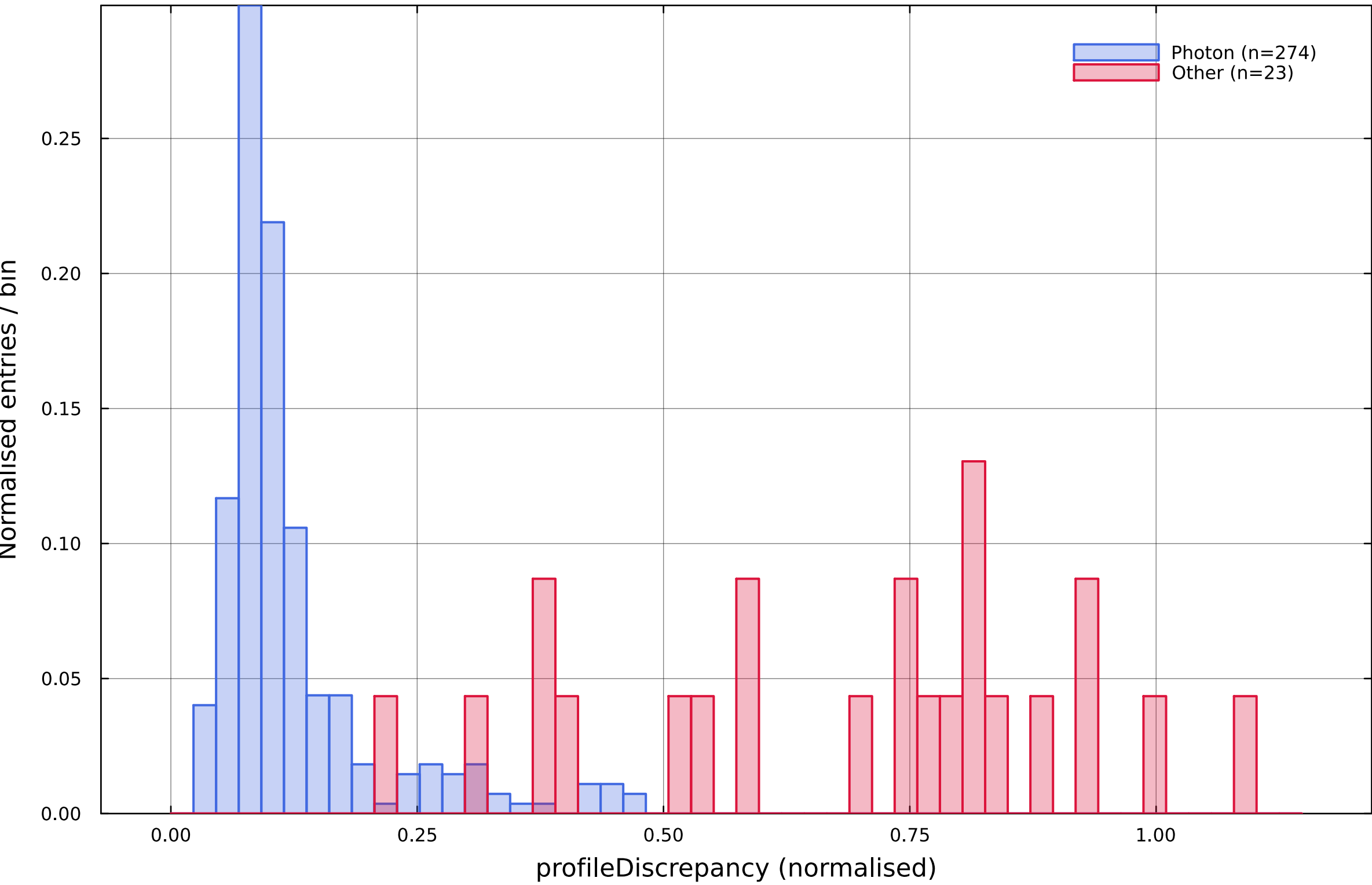
LongProfileDiscrepancy: photon vs other
