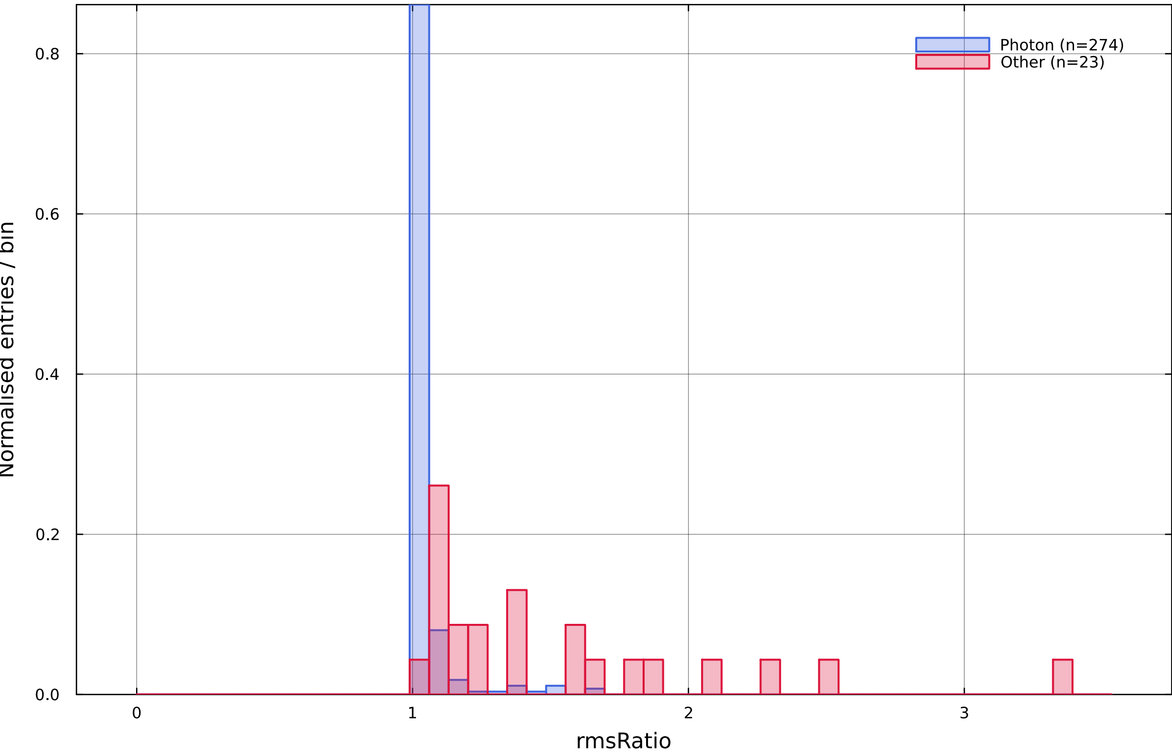
RmsRatio (RmsXYRatio): photon vs other
