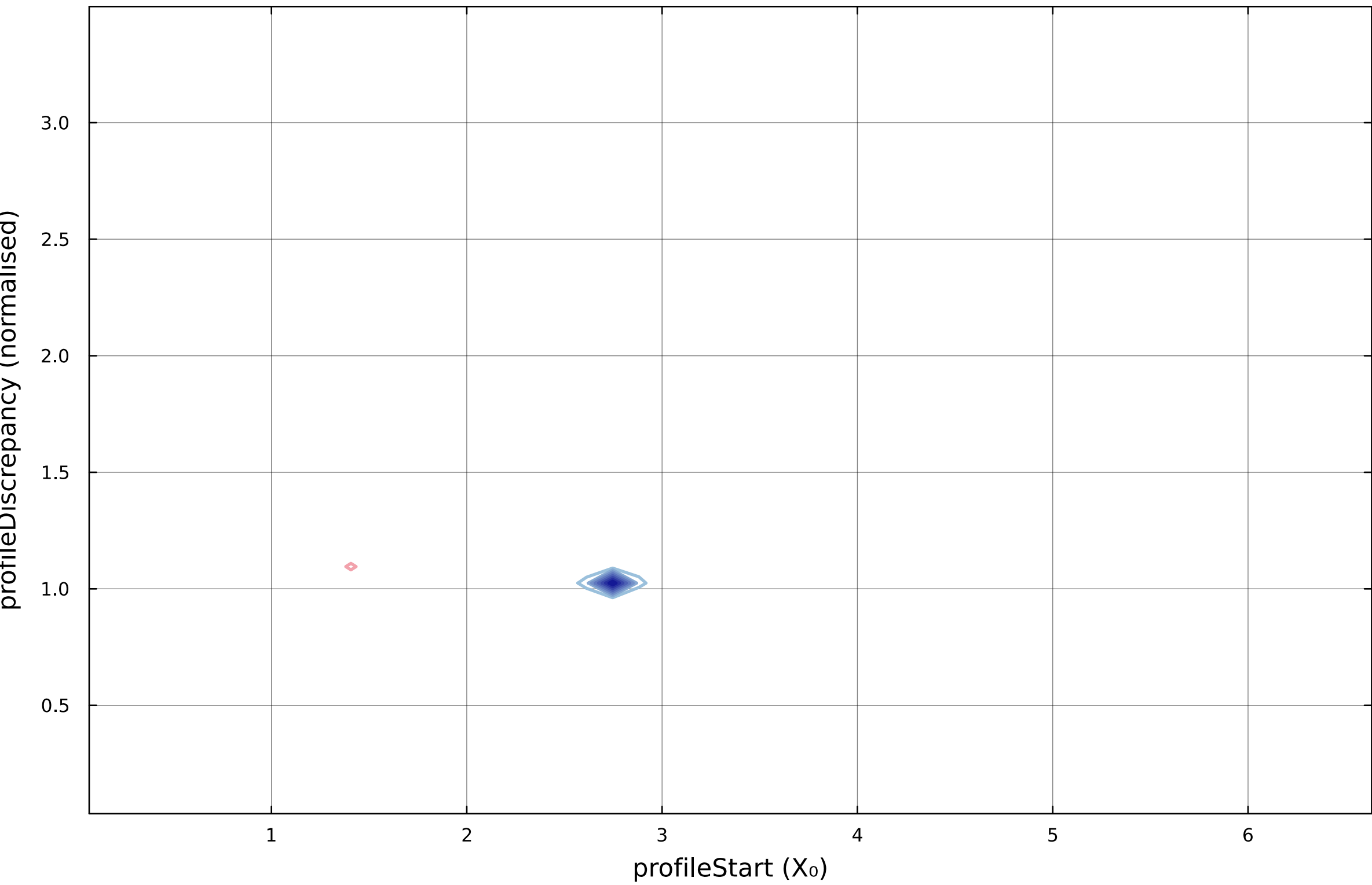
profileStart vs profileDiscrepancy
