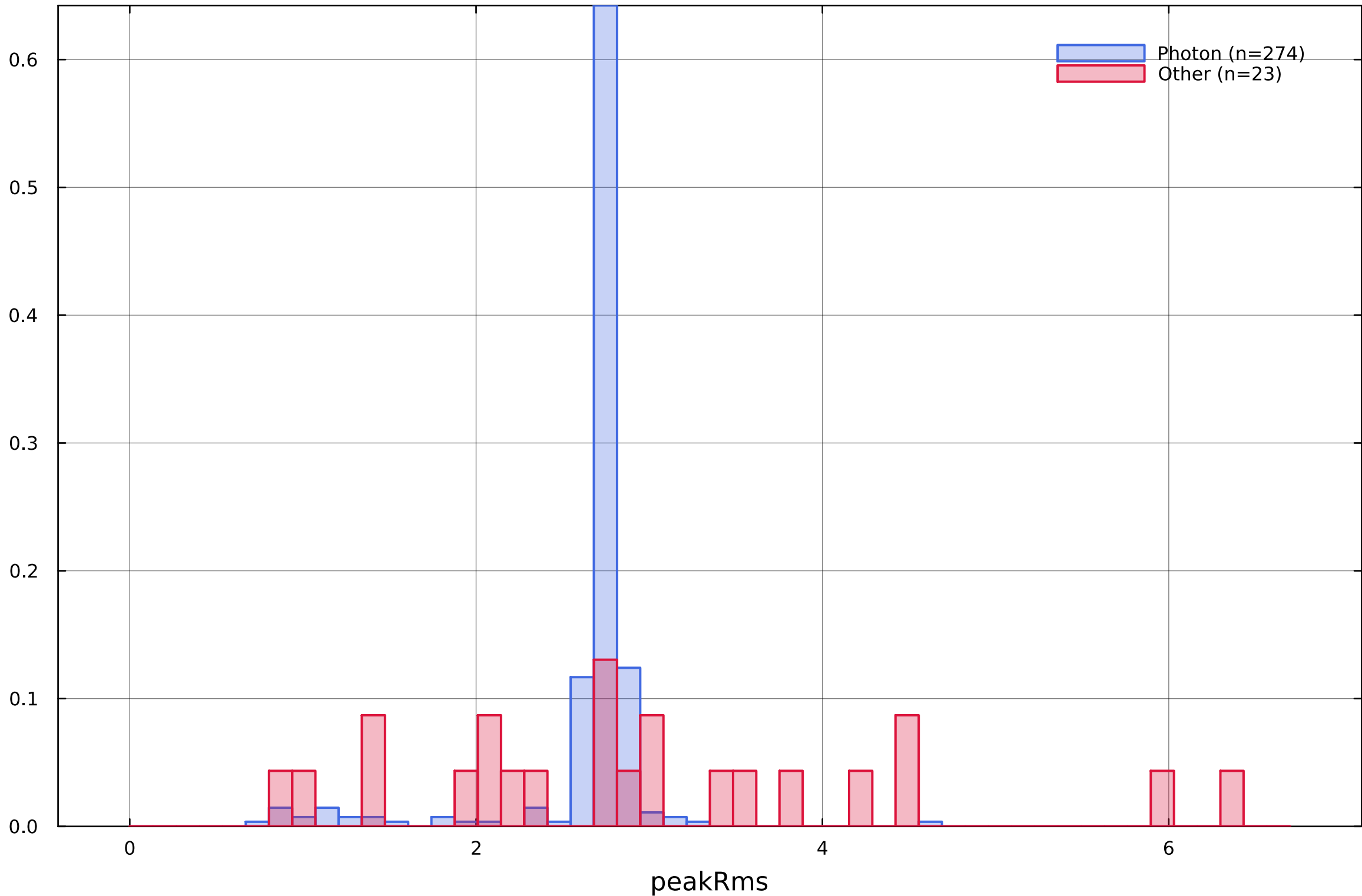
PeakRms: photon vs other
