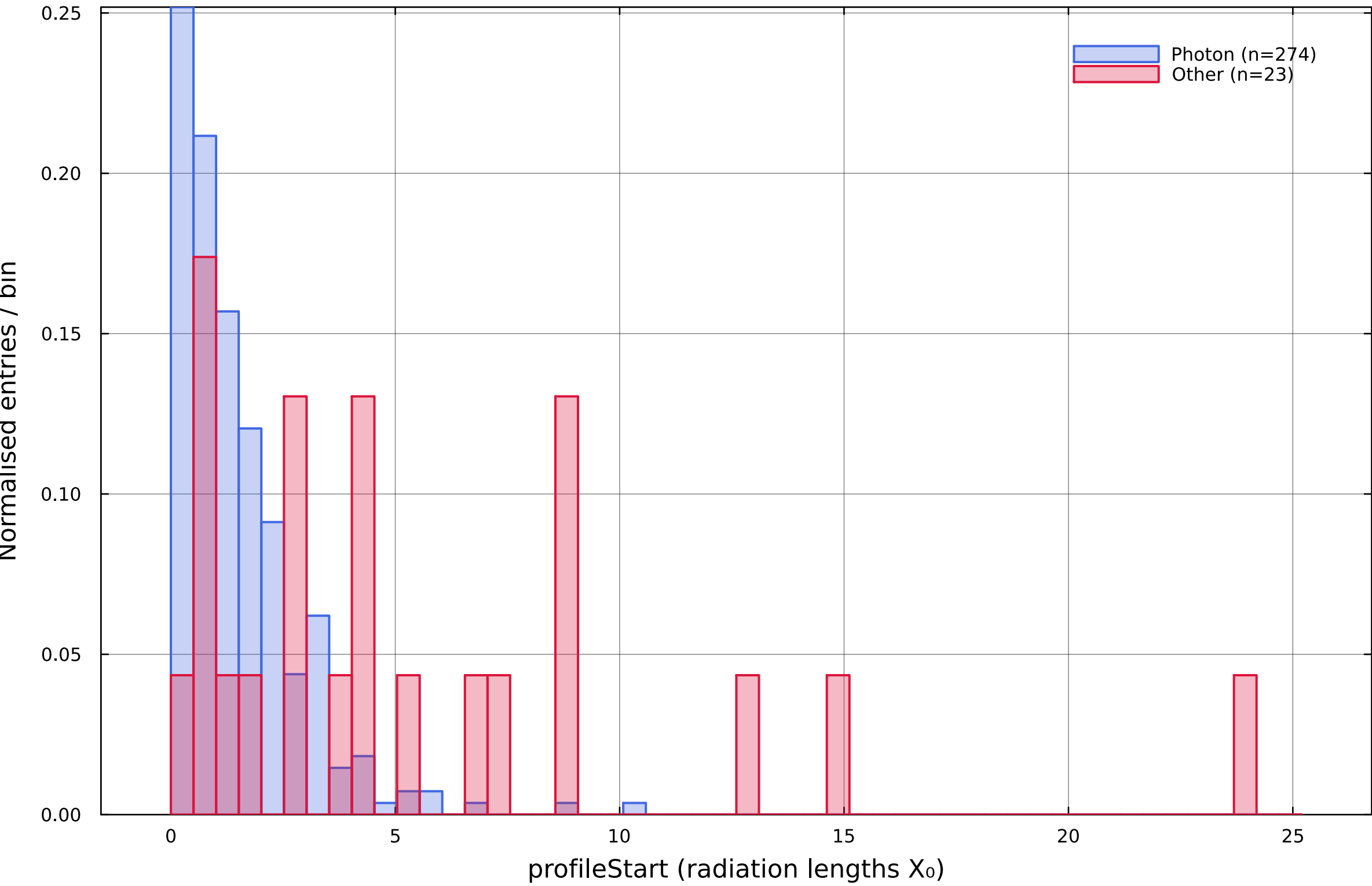
LongProfileStart: photon vs other
