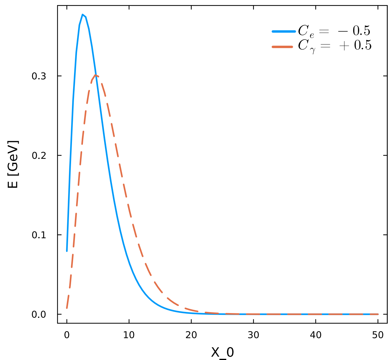
E = 100.0 GeV
