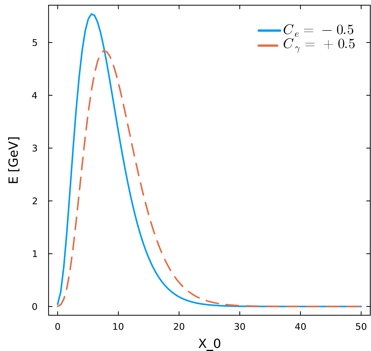
E = 100.0 GeV
