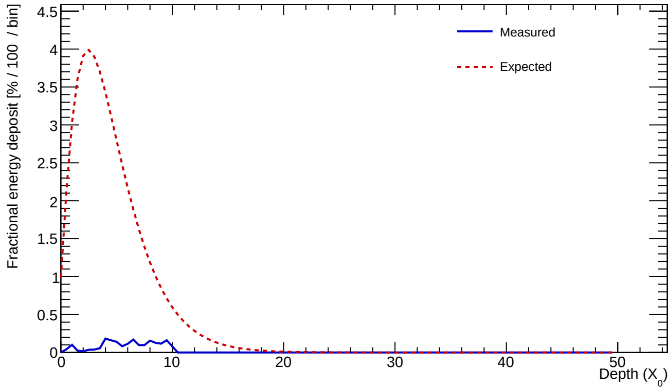
Cluster 2 E=0.931 GeV profileStart=3.00 X_0 \chi=0.3682
