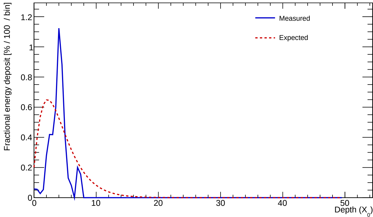
Cluster 1 E=0.721 GeV profileStart=1.50 X_0 \chi=0.5223
