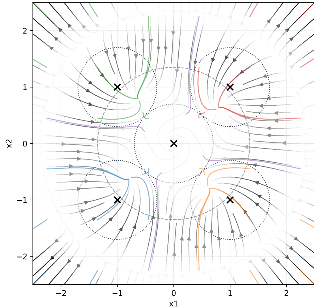
Multiwell Strong Transition: Phase Portrait
