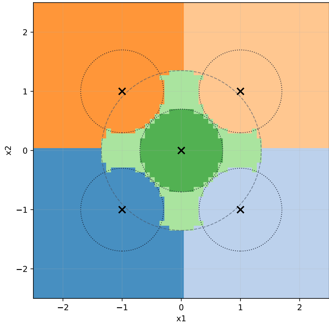
Multiwell Strong Transition: Region Map
