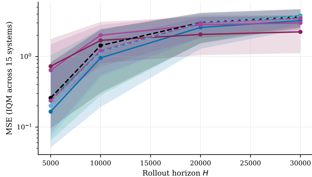
Dysts long-horizon IQM (15 systems, IQR shaded)
