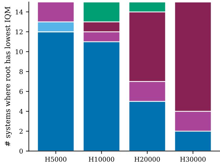
Dysts winner counts per horizon
