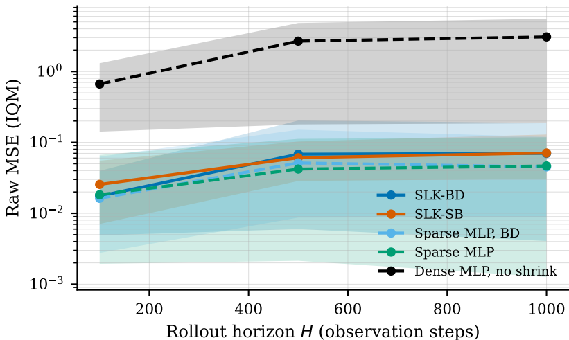
Multibasin forecasting (boundary-emphasized sampling, all rows)
