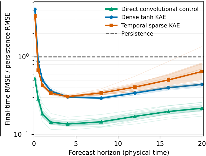
b Representation model: Allen-Cahn ( d_x = 512 )
