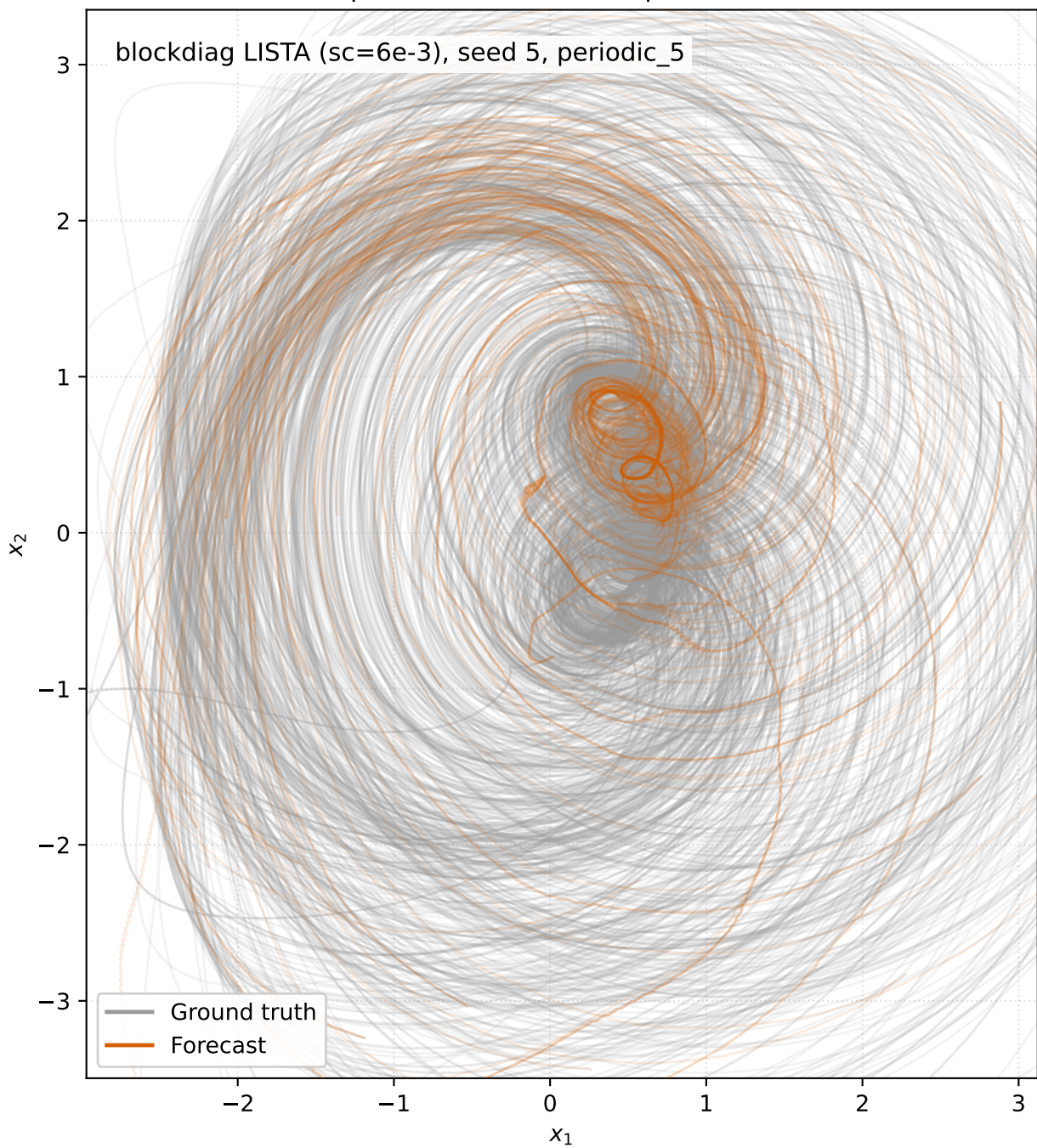
SprottTorus (30000-step forecast)
