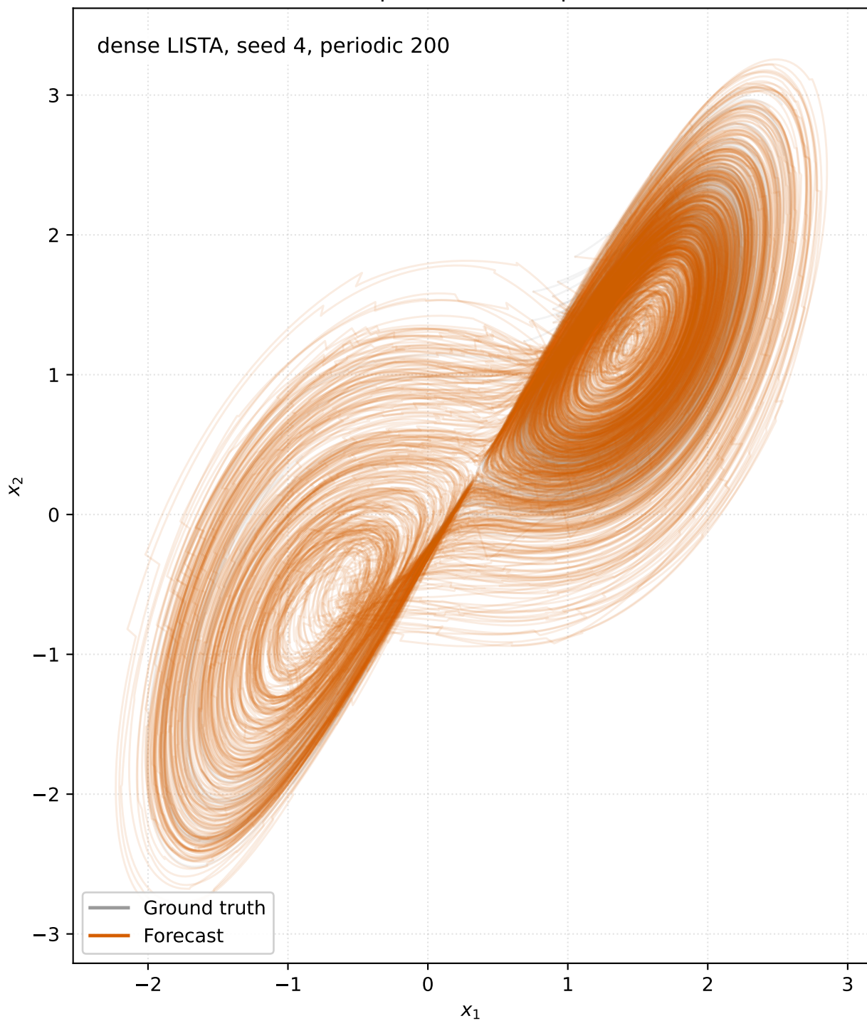
LorenzCoupled (20000-step forecast)
