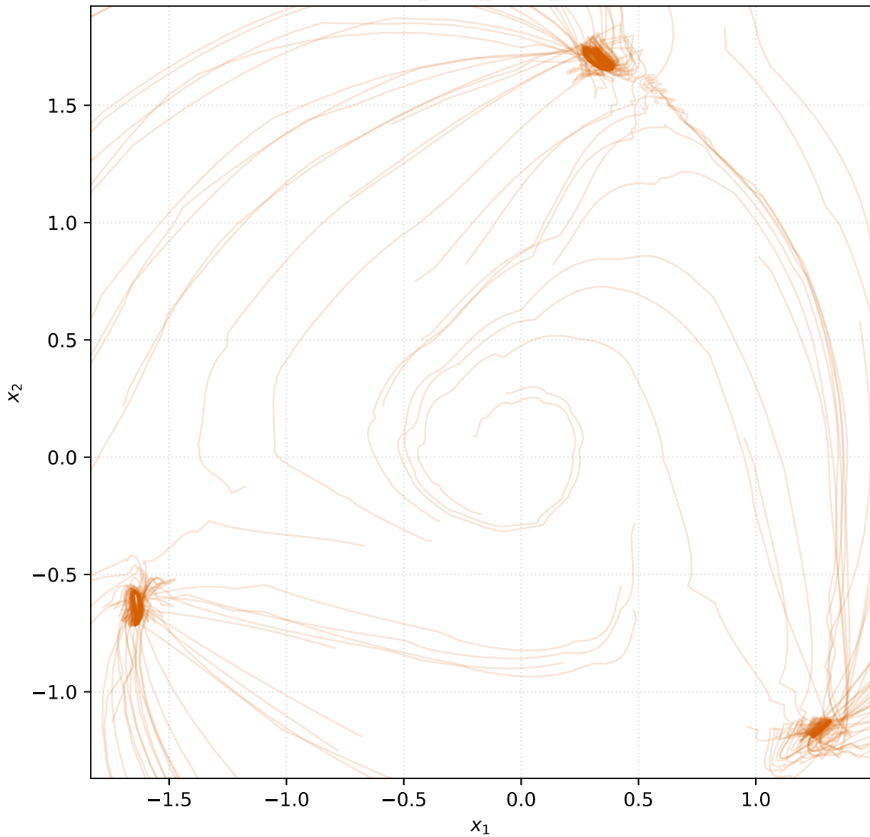
cal_high_cross_3
