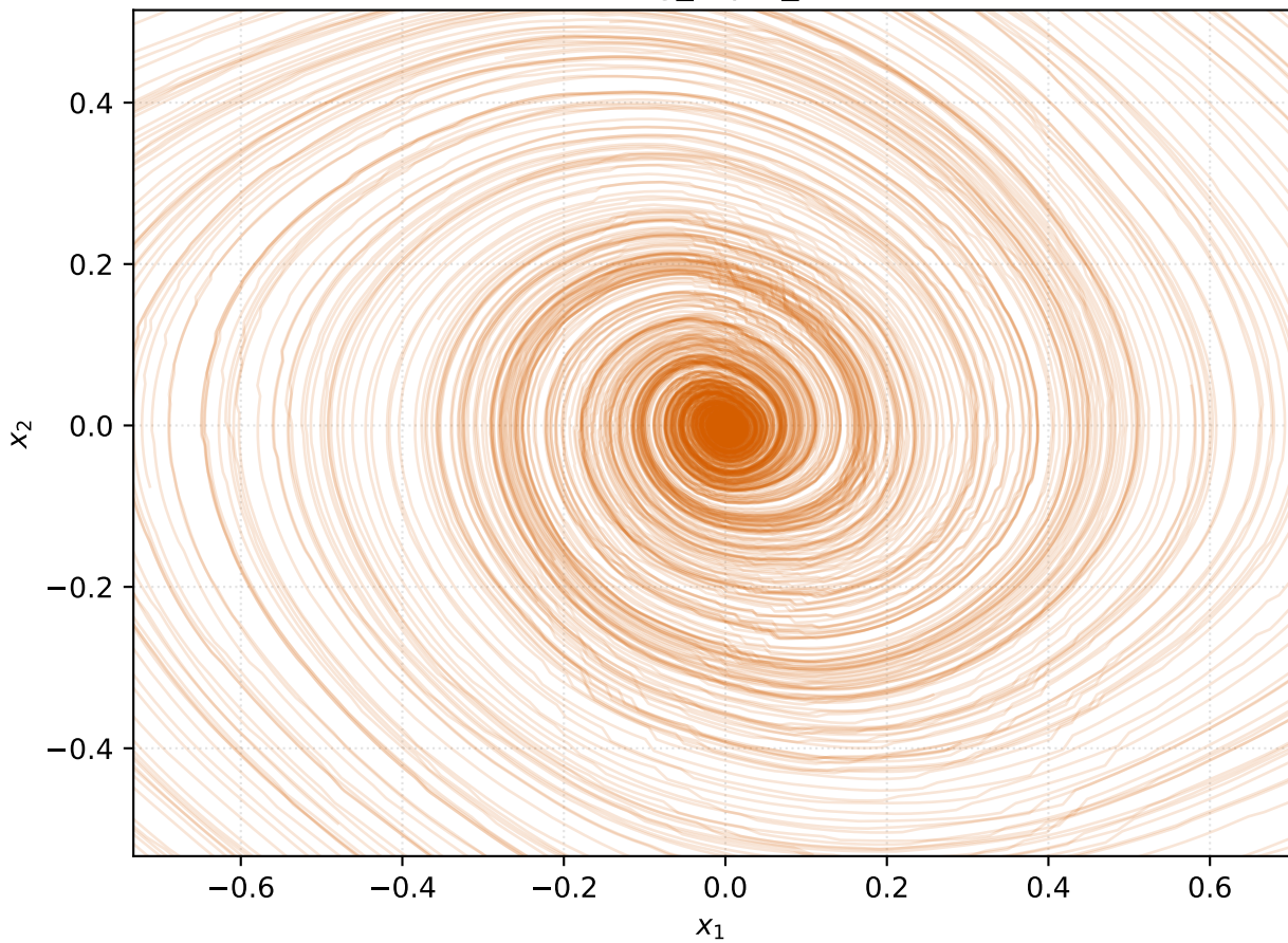
duffing_triple_well
