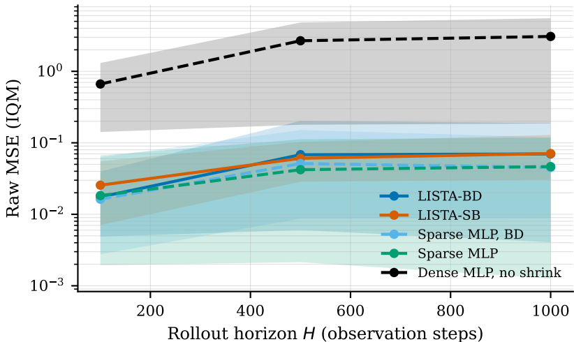
17-system multibasin forecasting performance
