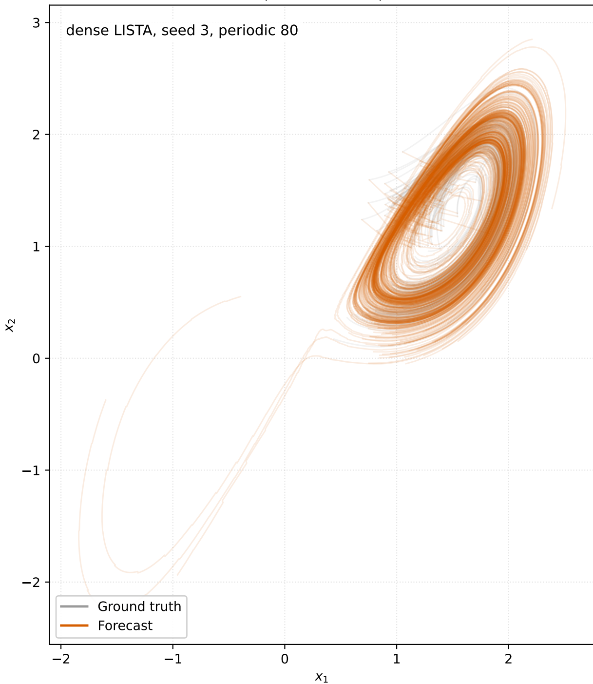
LorenzCoupled (5000-step forecast)
