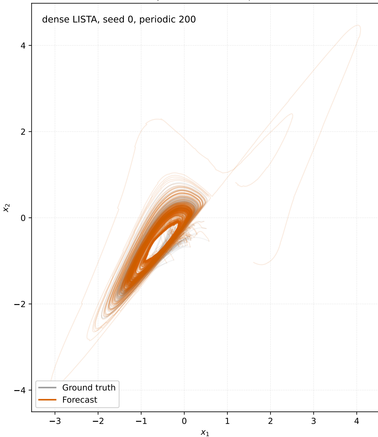
RikitakeDynamo (20000-step forecast)
