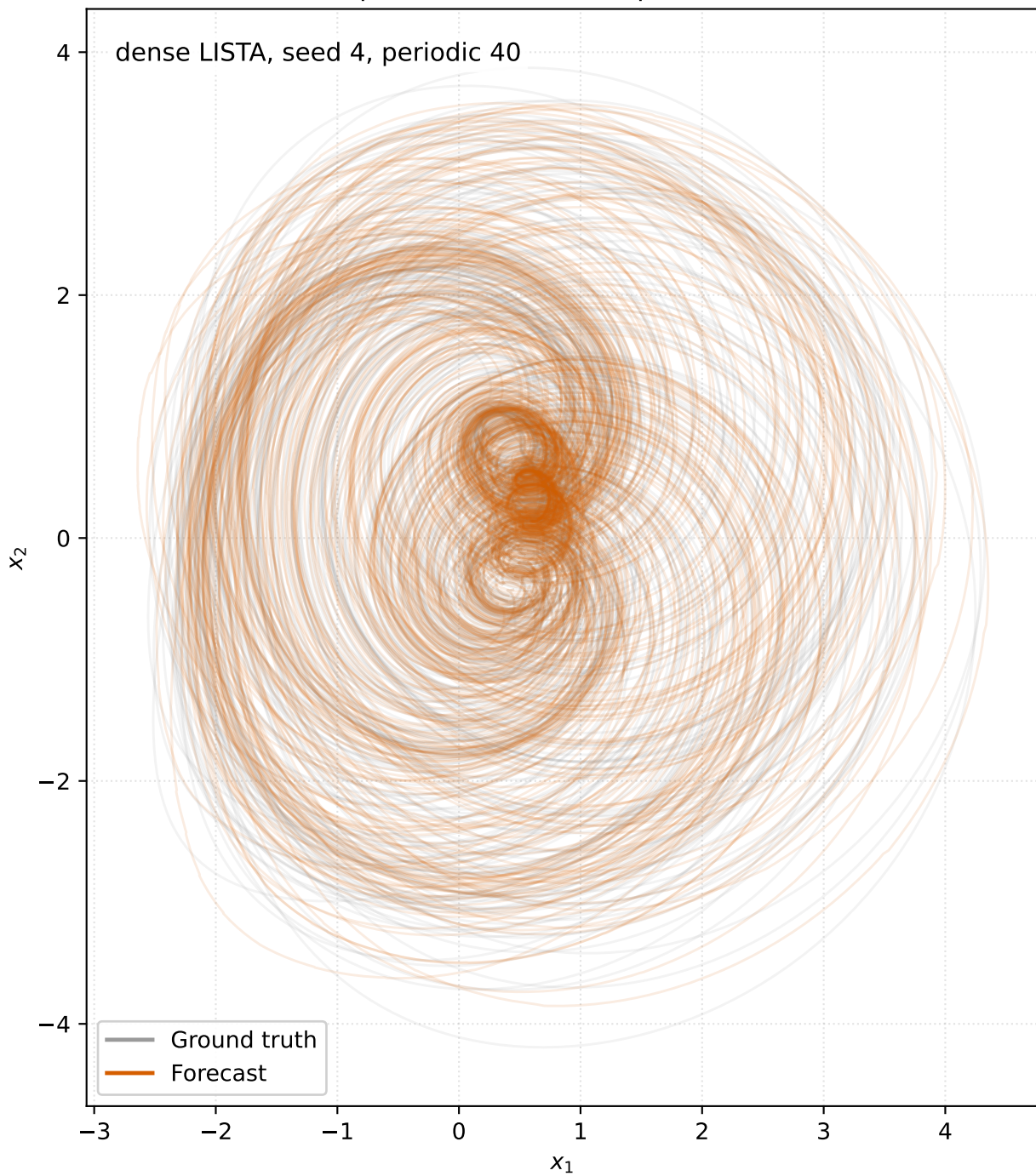
SprottTorus (5000-step forecast)
