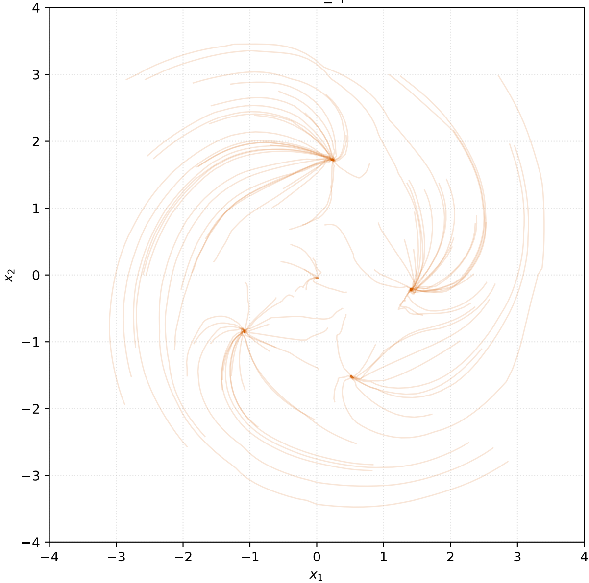
arrested_spiral
