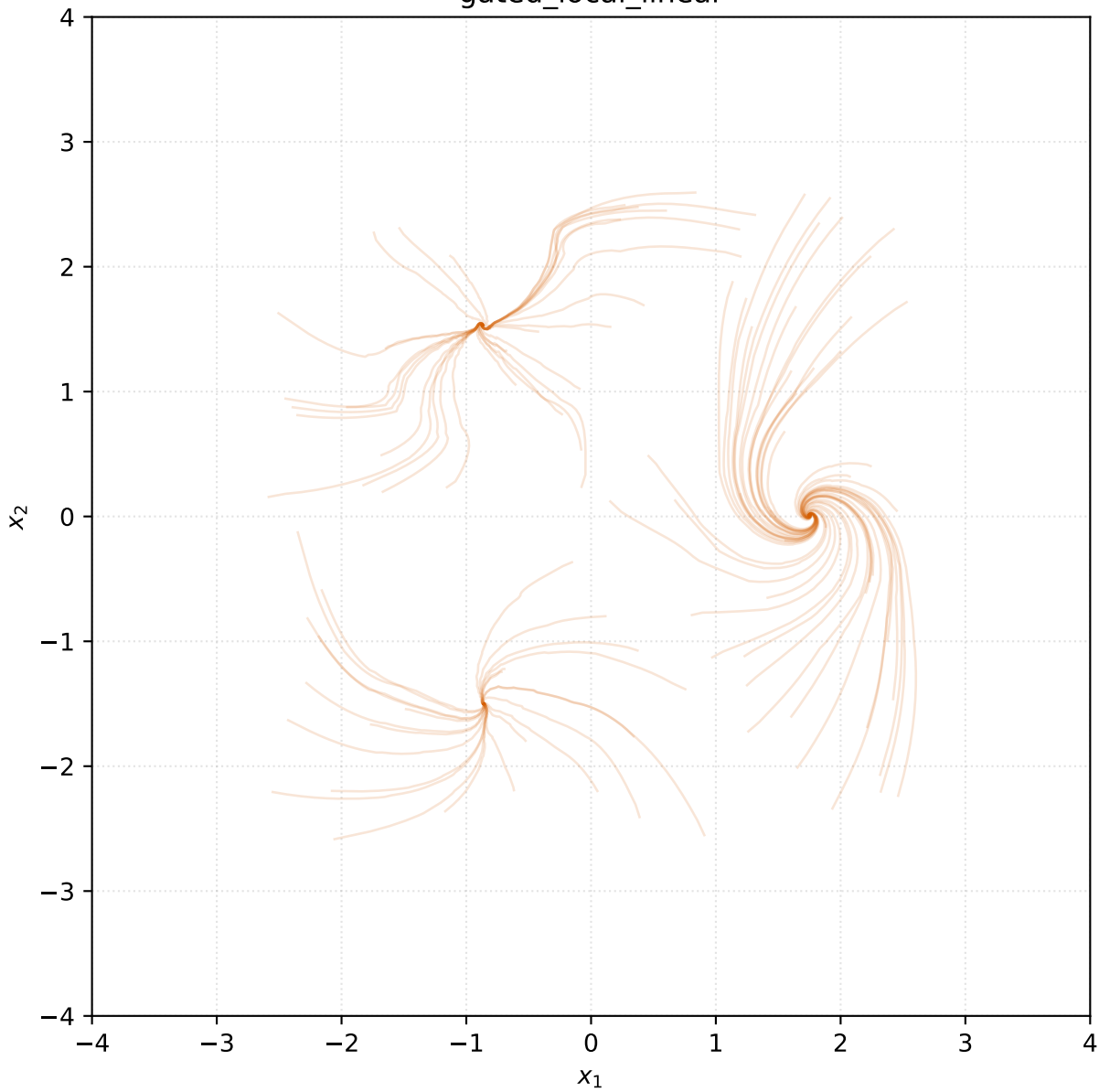
gated_local_linear
