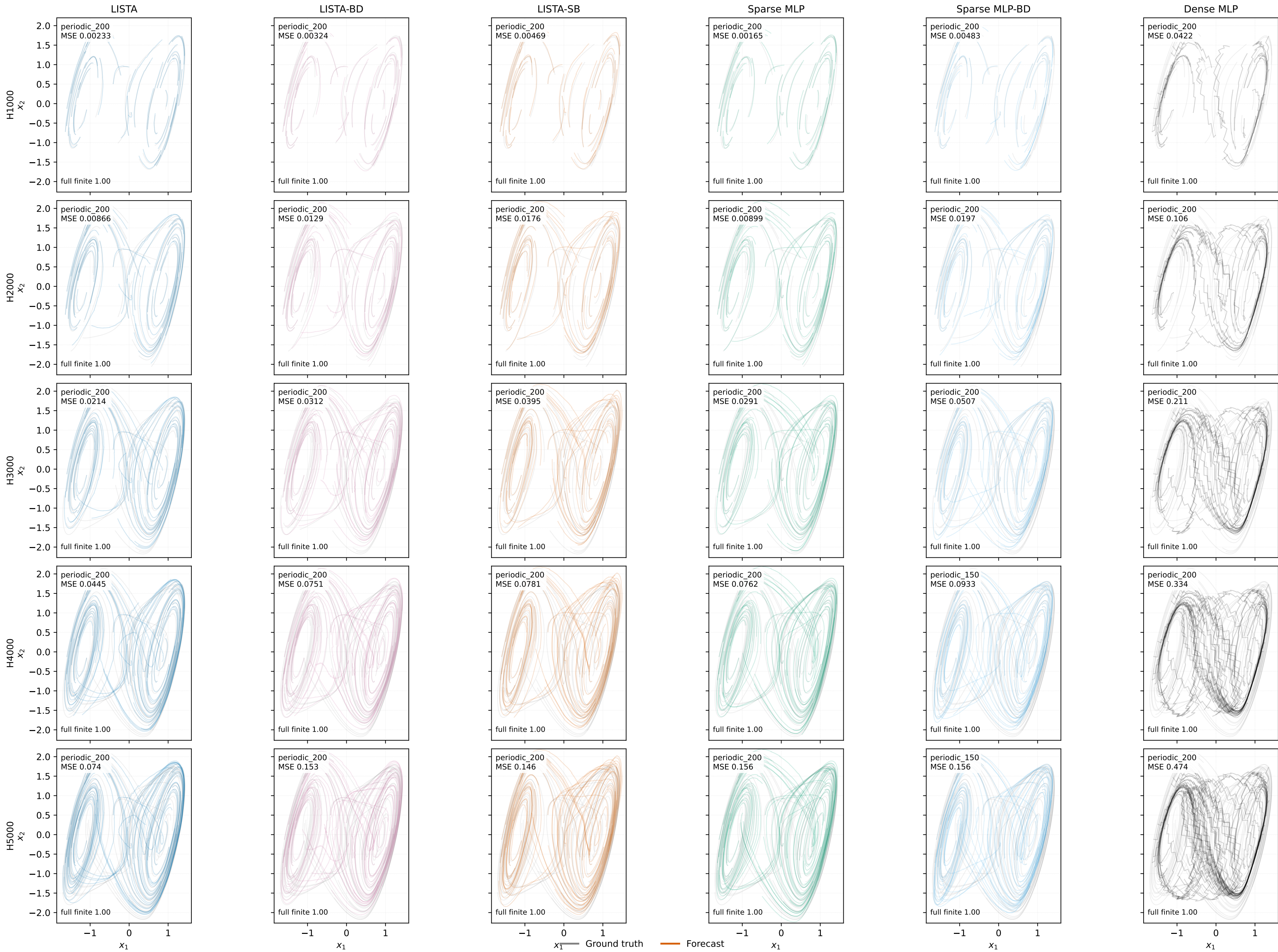
dysts:Chua phase portraits, seed 0
