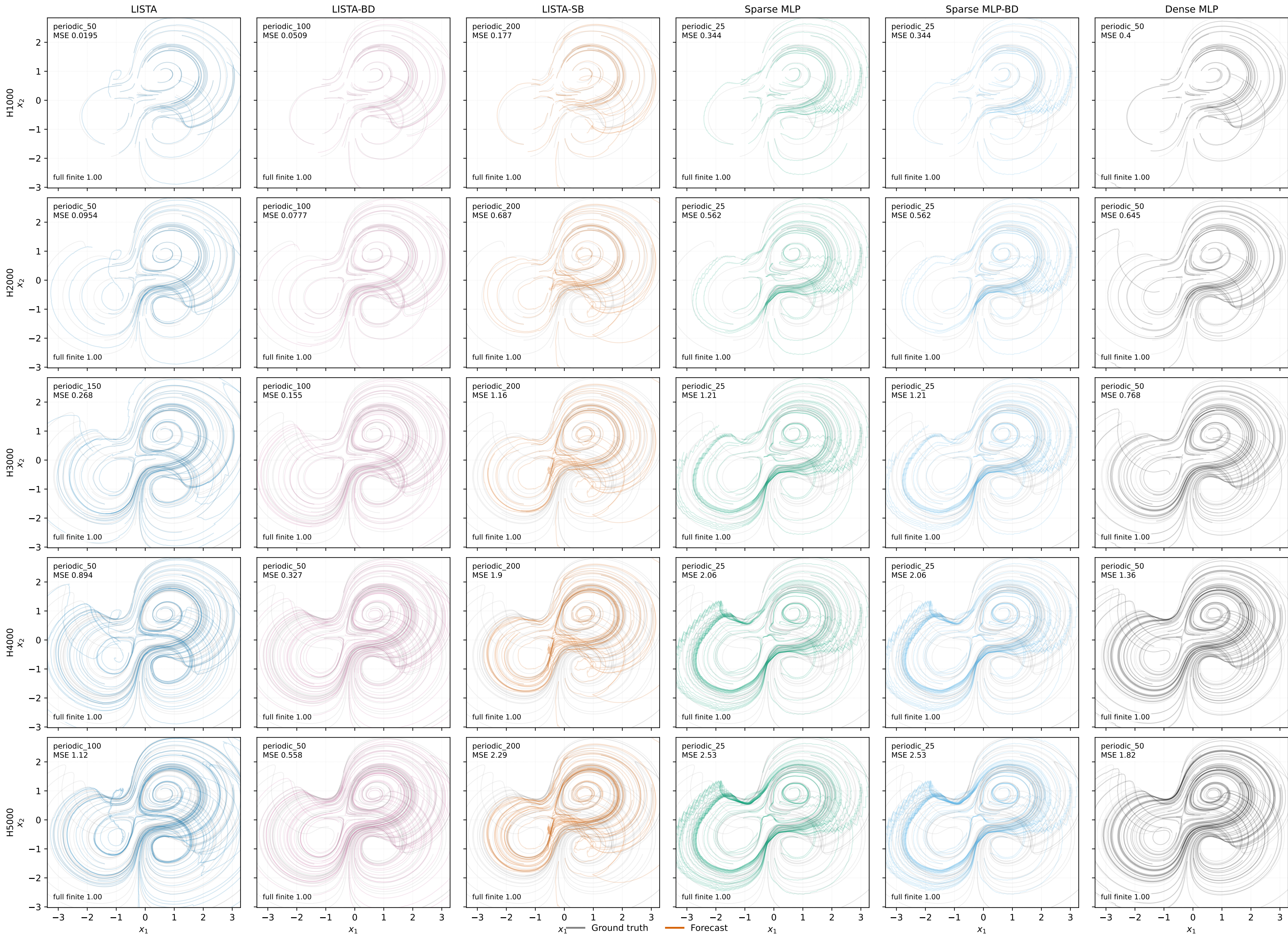
dysts:Dadras phase portraits, seed 0
