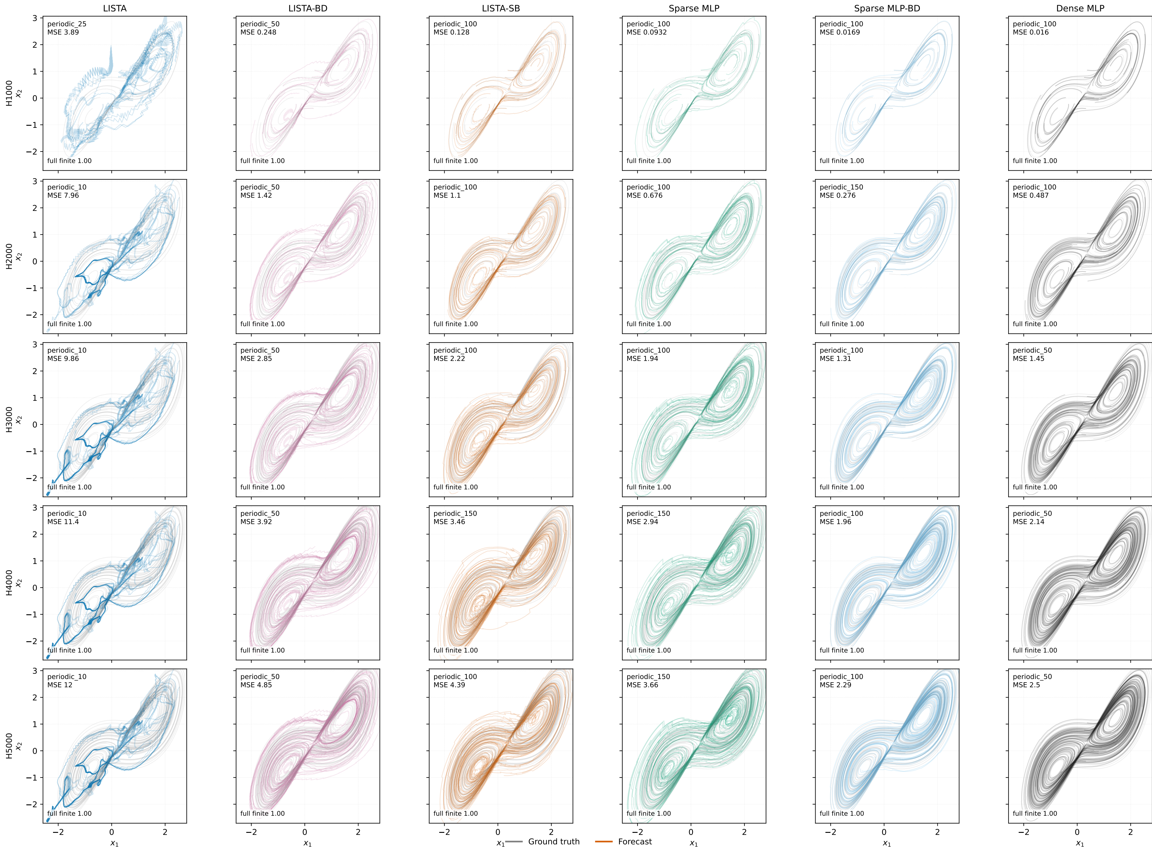
dysts:LorenzCoupled phase portraits, seed 0
