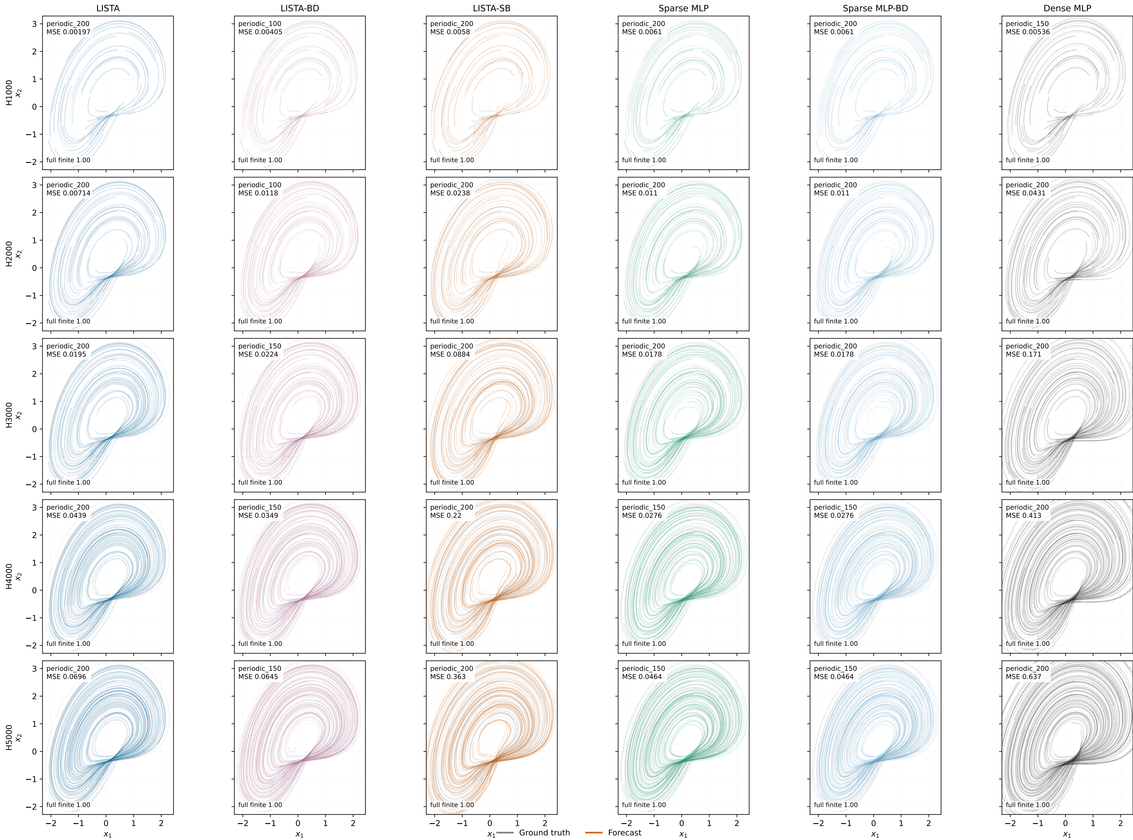
dysts:LuChenCheng phase portraits, seed 0
