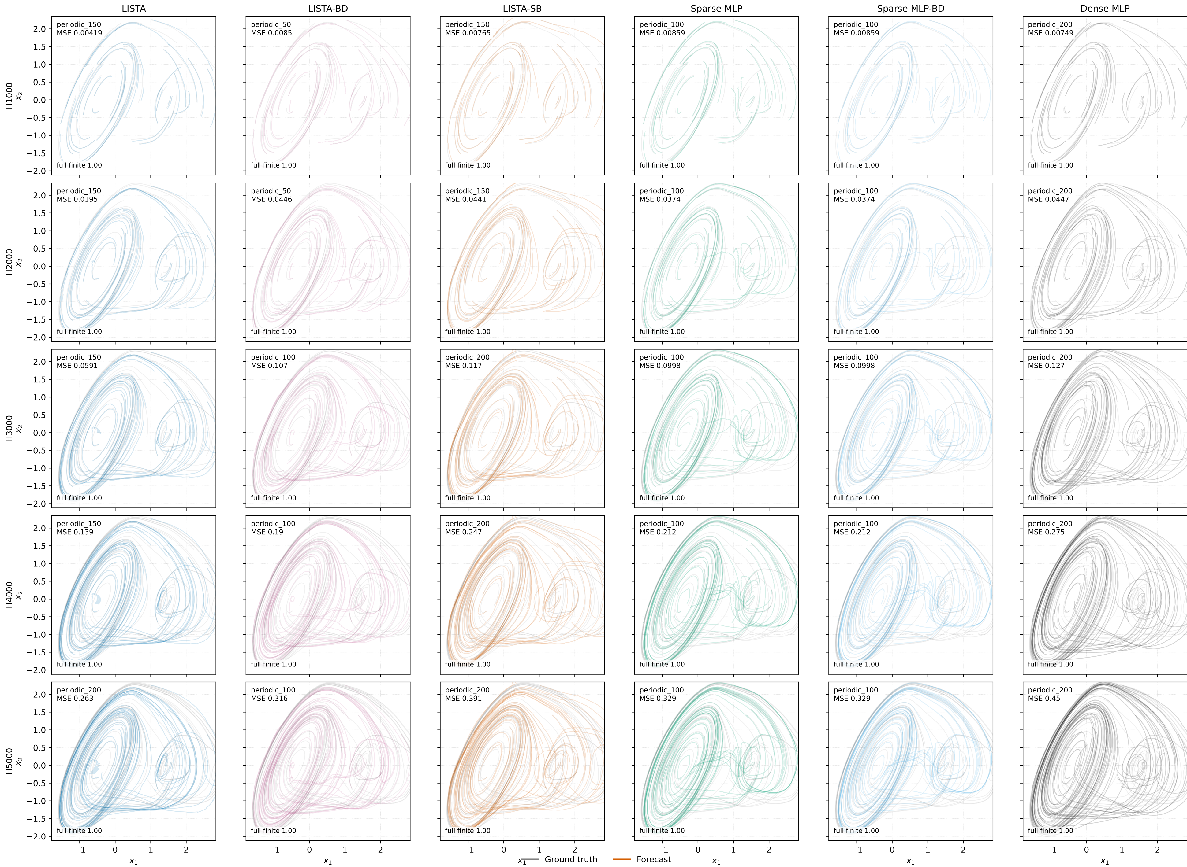
dysts:MultiChua phase portraits, seed 0
