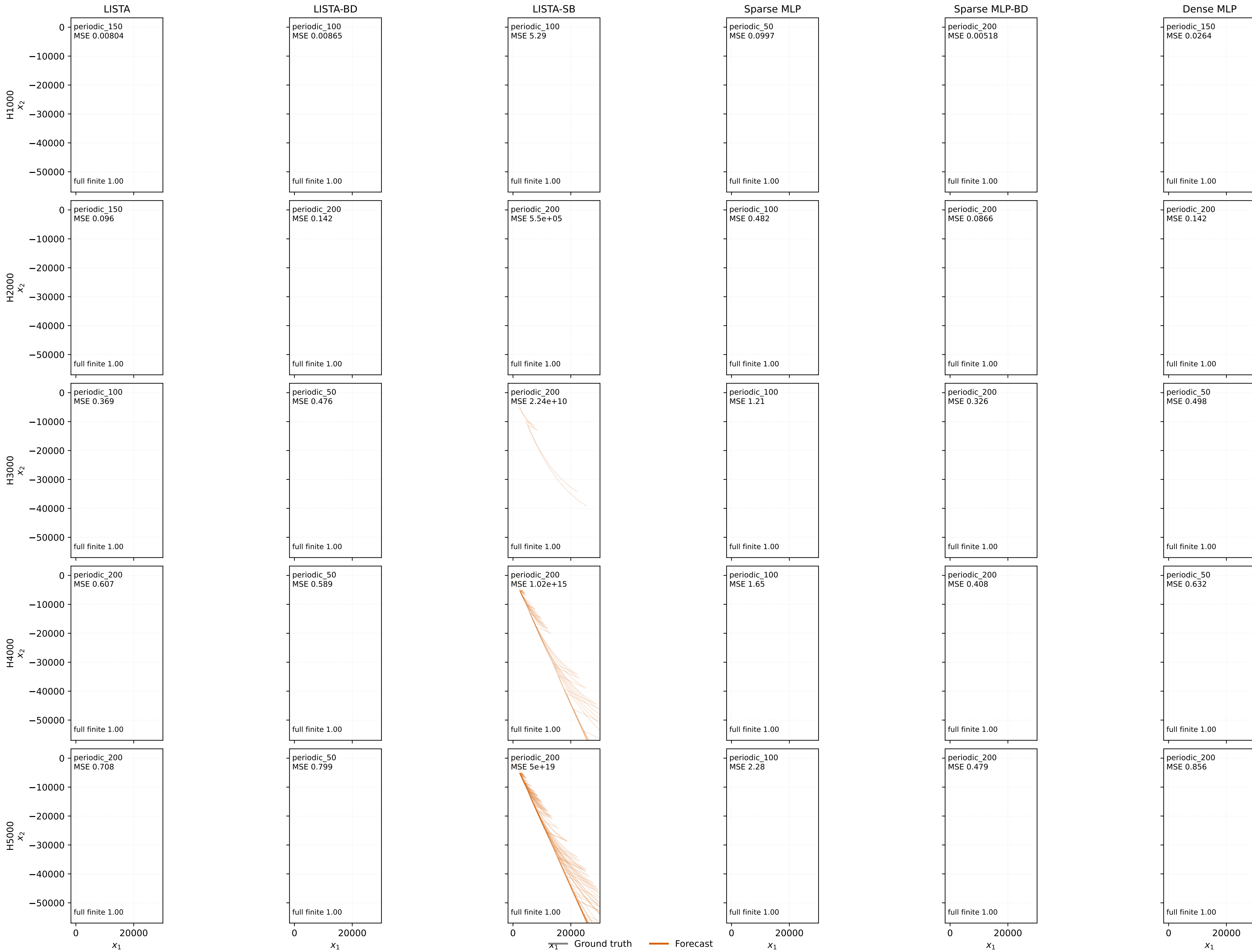
dysts:QiChen phase portraits, seed 0
