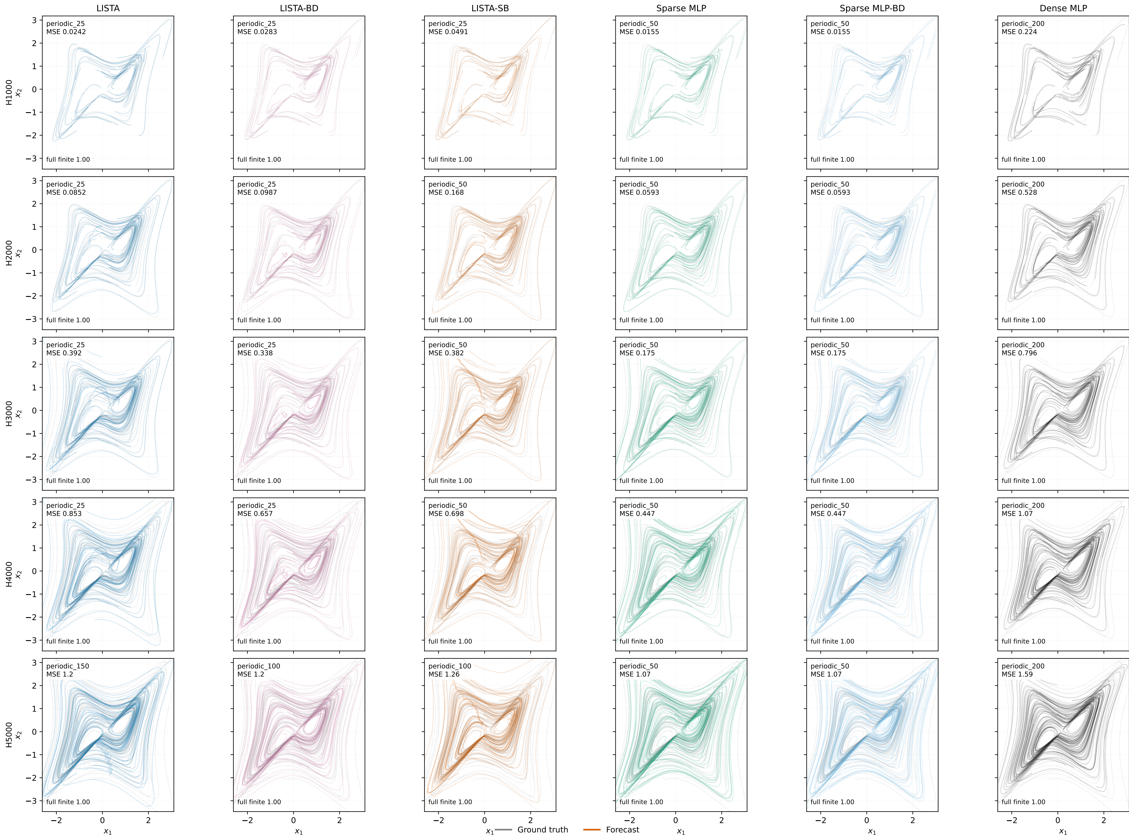
dysts:Sakarya phase portraits, seed 0
