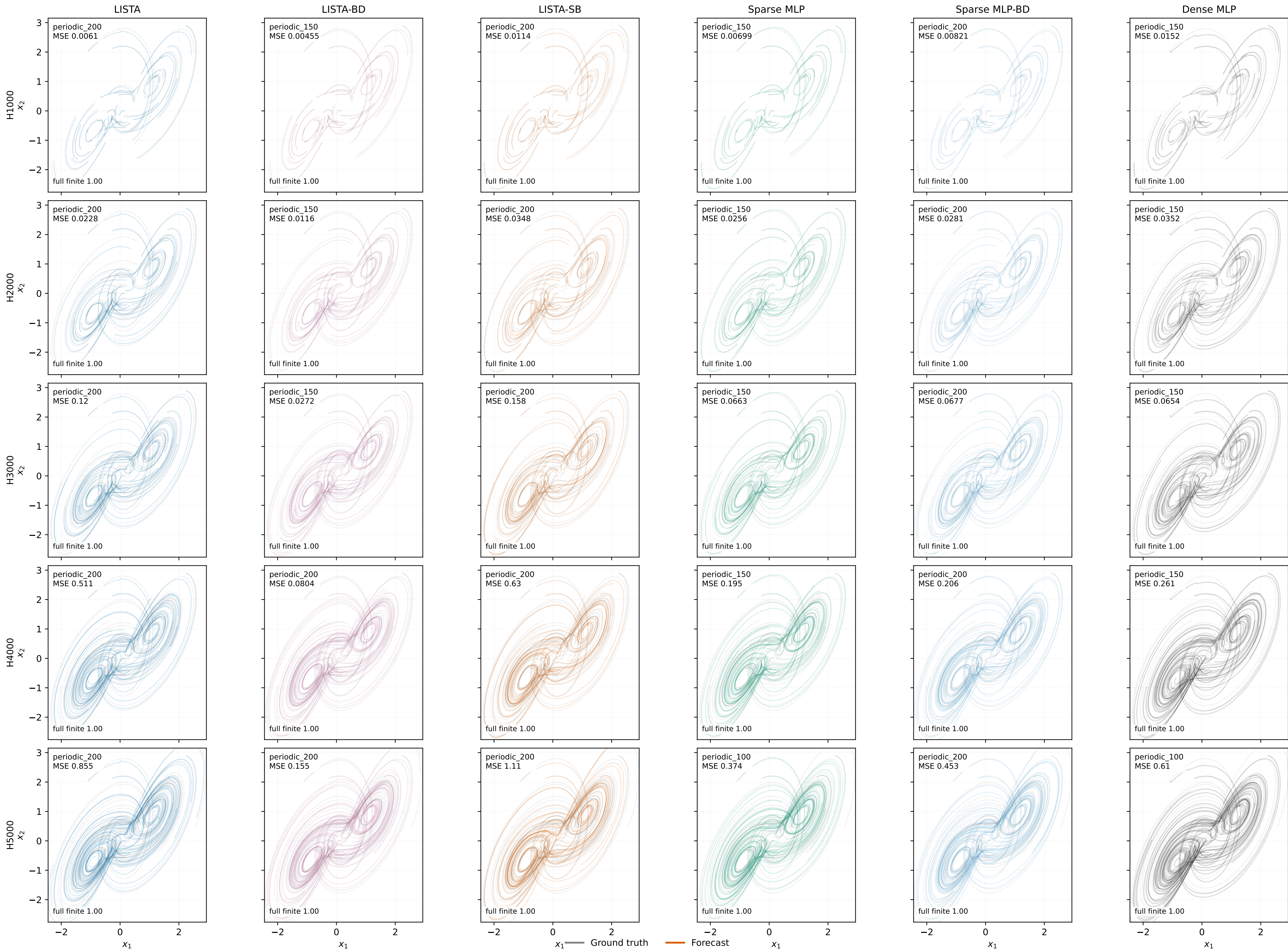
dysts:SanUmSrisuchinwong phase portraits, seed 0
