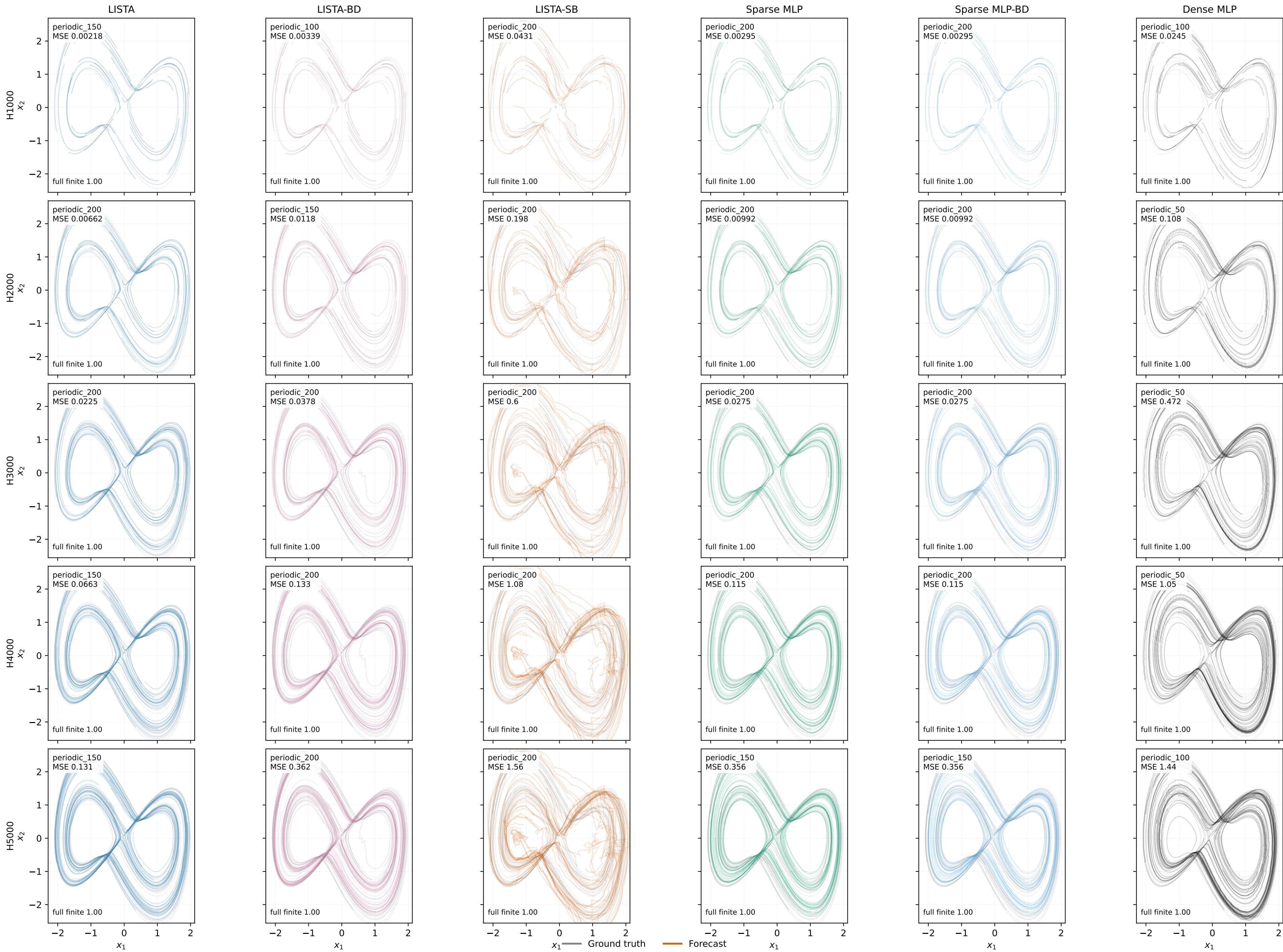
dysts:ShimizuMorioka phase portraits, seed 0
