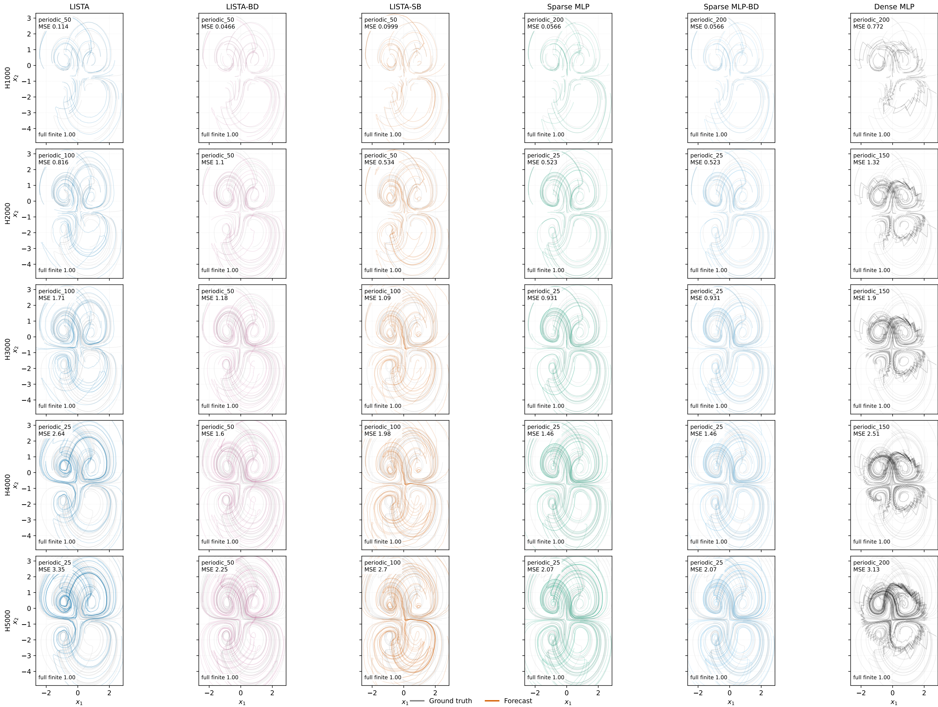
dysts:WangSun phase portraits, seed 0
