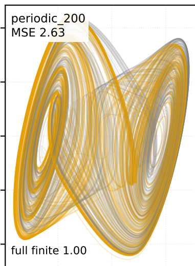
Dense MLP
