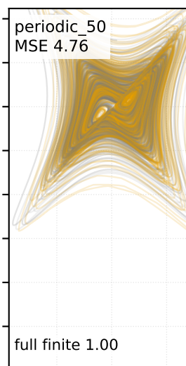
Dense MLP
