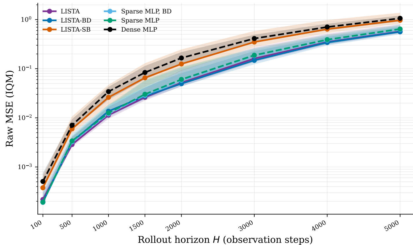
12-system Dysts forecasting performance
