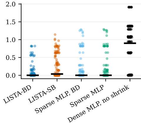
H(B | F_{\text{abs}})
