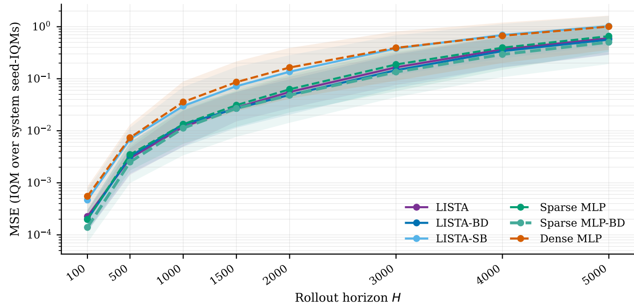
10-system Dysts robust aggregation sensitivity
