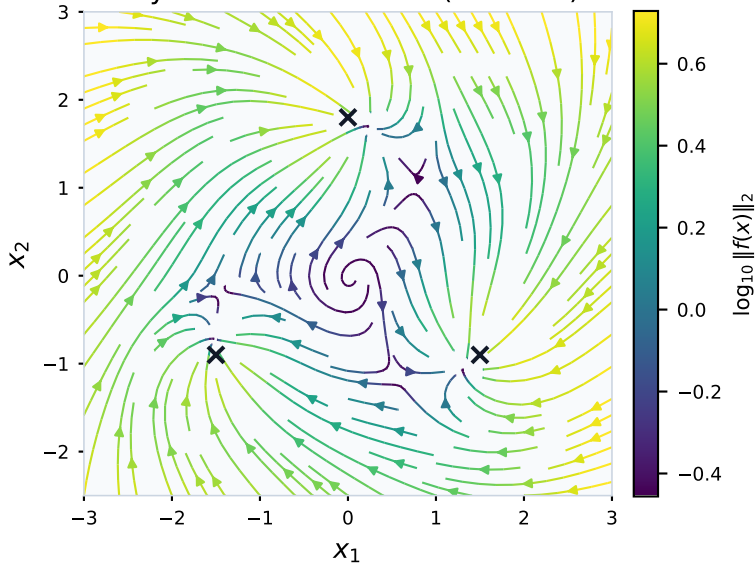
Asymmetric three-well (3 basins)
