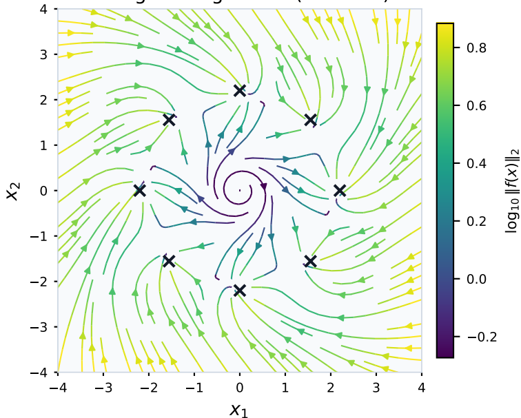
Octagonal eight-well (8 basins)
