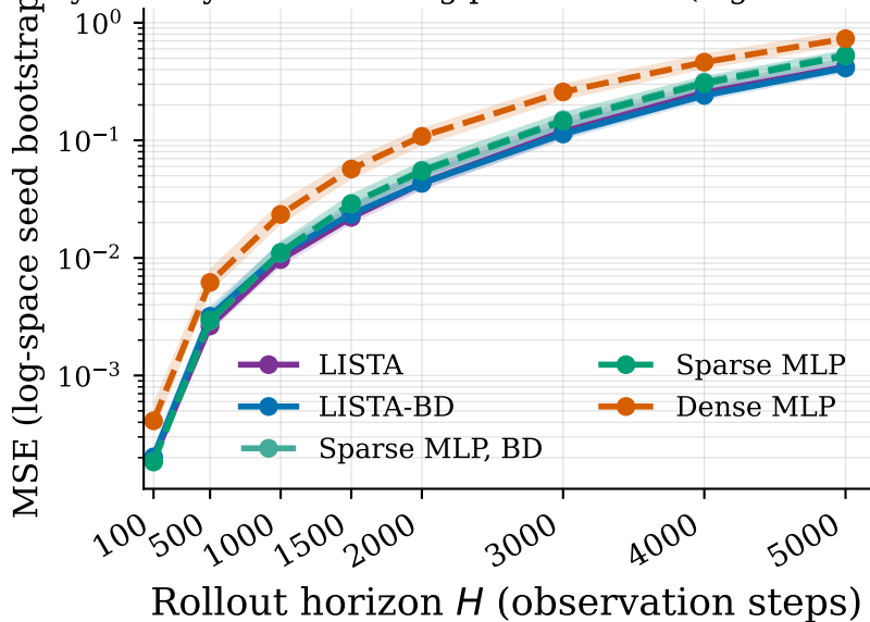
1D-system Dyns forecasting performance (log seed bootstrap)
